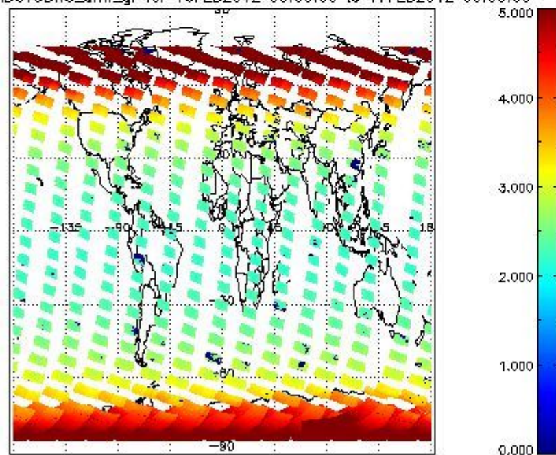
SCIOL2P_NADUV3BRO_amf_gr for 16FEB2012 00:00:00 to 17FEB2012 00:00:00
