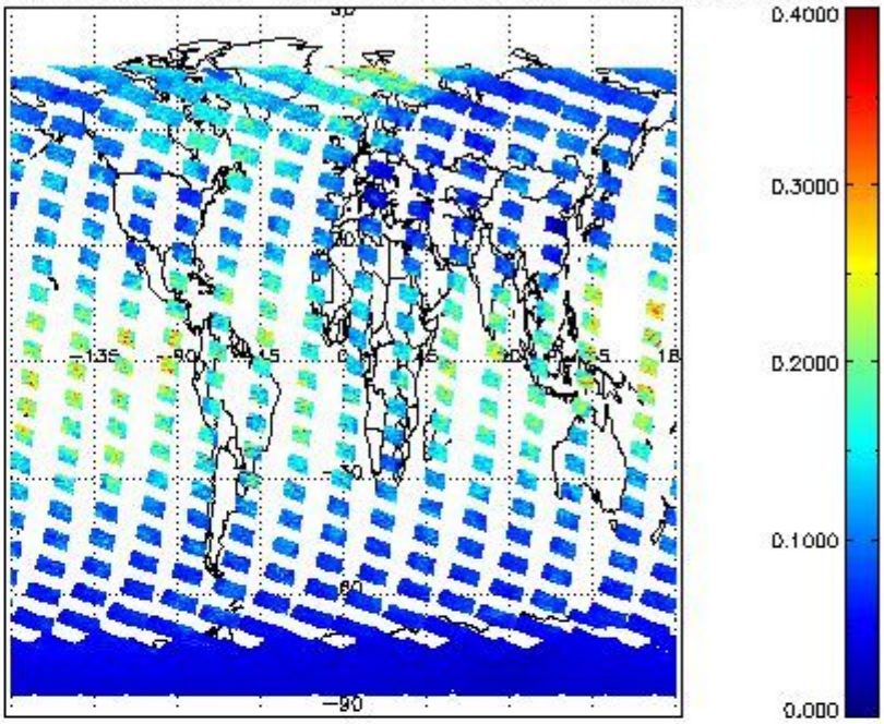
SCIOL2P_NADUV1N02_vcd_err for 16FEB2012 00:00:00 to 17FEB2012 00:00:00
