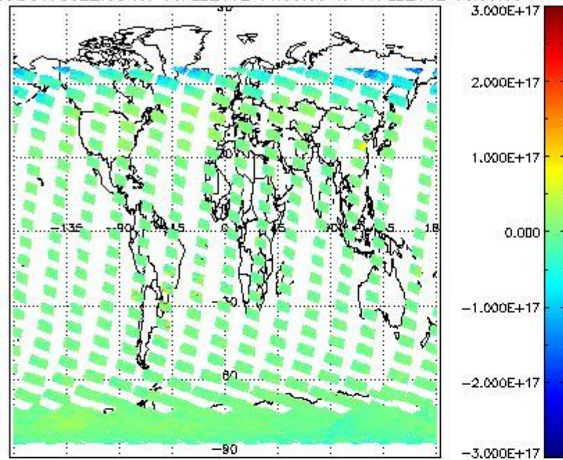
SCIOL2P_NADUV7S02_vcd for 16FEB2012 00:00:00 to 17FEB2012 00:00:00
