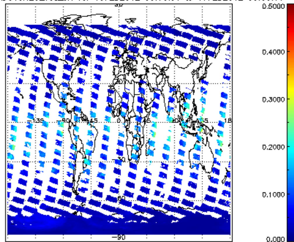
SCIOL2P_NADUV8H2O_vcd_err for 16FEB2012 00:00:00 to 17FEB2012 00:00:00
