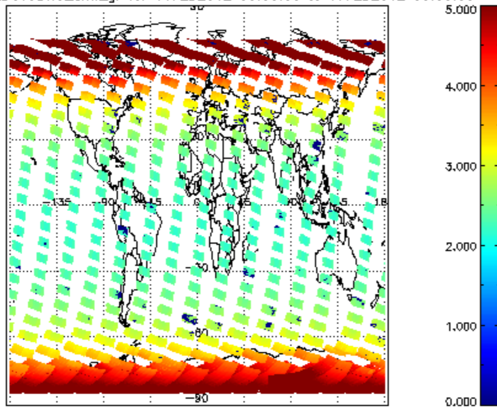
SCIOL2P_NADUV3BRO_amf_gr for 16FEB2012 00:00:00 to 17FEB2012 00:00:00
