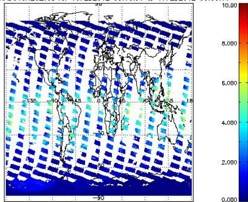
SCIOL2P_NADUV8H2O_vcd for 16FEB2012 00:00:00 to 17FEB2012 00:00:00
