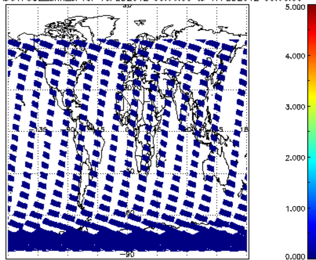
SCIOL2P_NADUV7S02_amf_cl for 16FEB2012 00:00:00 to 17FEB2012 00:00:00
