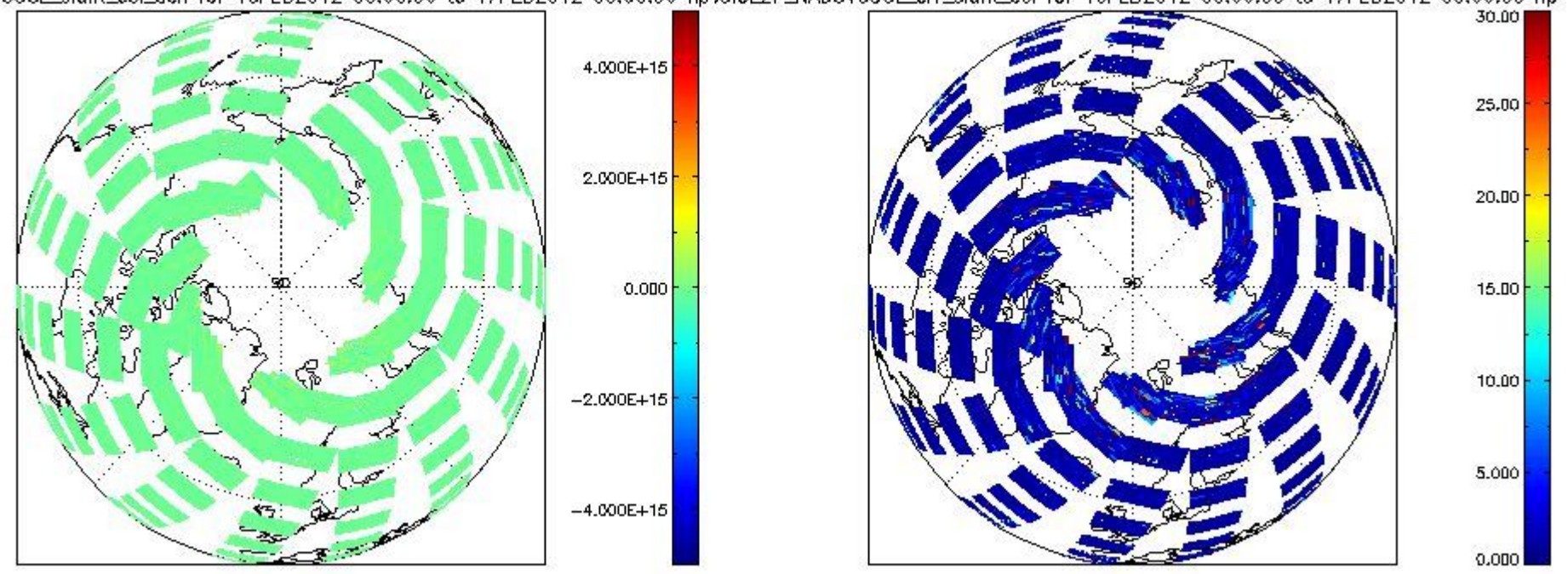
CIOL2P_NADUV6OCL_slant_col_den for 16FEB2012 00:00:00 to 17FEB2012 00:00:00 np; CIOL2P_NADUV6OCL_err_slant_col for 16FEB2012 00:00:00 to 17FEB2012 00:00:00 np
