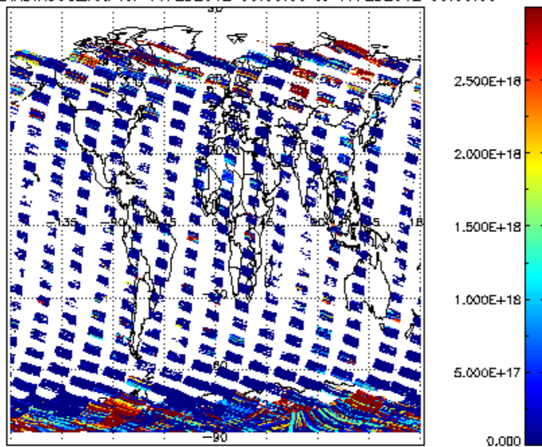
SCIOL2P_NADIR3CO_vcd for 16FEB2012 00:00:00 to 17FEB2012 00:00:00
