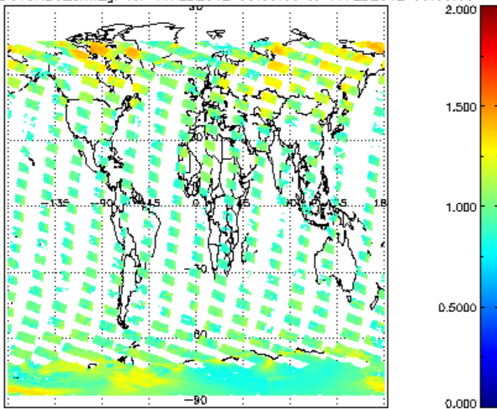
SCIOL2P_NADUV8H2O_amf_gr for 16FEB2012 00:00:00 to 17FEB2012 00:00:00
