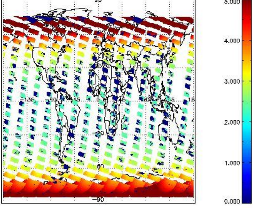
SCIOL2P_NADUV1N02_amf_cl for 16FEB2012 00:00:00 to 17FEB2012 00:00:00
