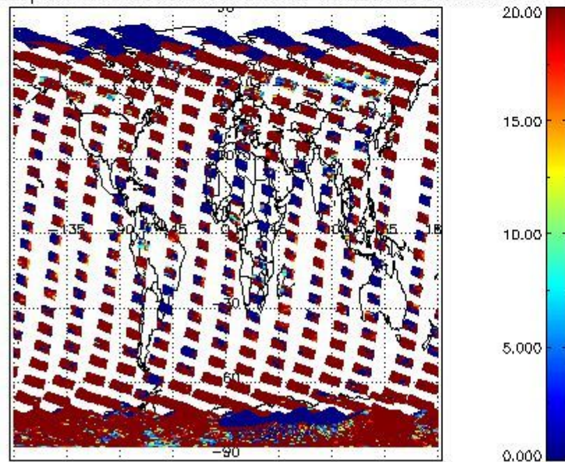
cL_opt_depth for 16FEB2012 00:00:00 to 17FEB2012 00:00:00
