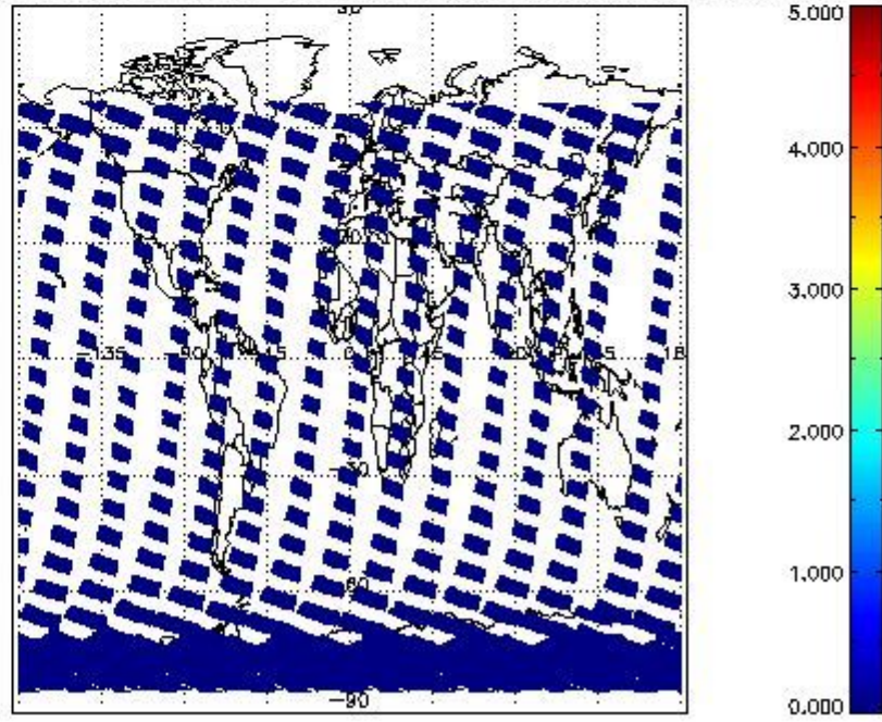
SCIOL2P_NADUV5S02_amf_cl for 16FEB2012 00:00:00 to 17FEB2012 00:00:00
