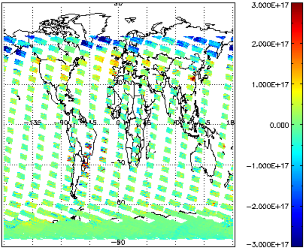
SCIOL2P_NADUV5S02_vcd for 16FEB2012 00:00:00 to 17FEB2012 00:00:00
