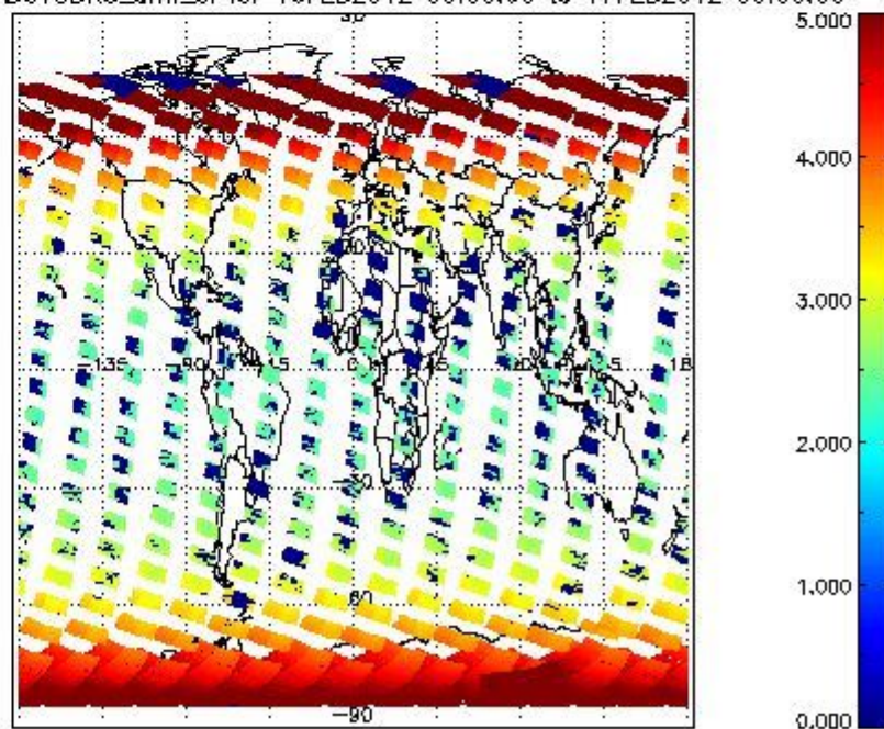
SCIOL2P_NADUV3BRO_amf_cl for 16FEB2012 00:00:00 to 17FEB2012 00:00:00
