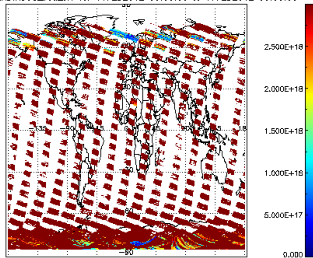
SCIOL2P_NADIR3CO_vcd_err for 16FEB2012 00:00:00 to 17FEB2012 00:00:00
