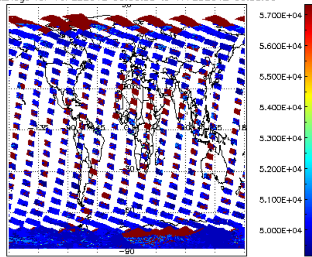
cloud_flags for 16FEB2012 00:00:00 to 17FEB2012 00:00:00
