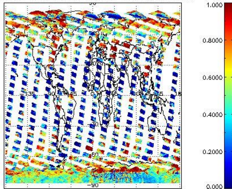
cL_frac for 16FEB2012 00:00:00 to 17FEB2012 00:00:00
