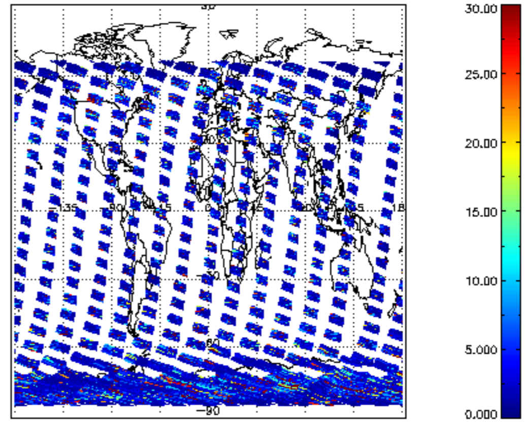
SCIOL2P_NADUV5S02_vcd_err for 16FEB2012 00:00:00 to 17FEB2012 00:00:00
