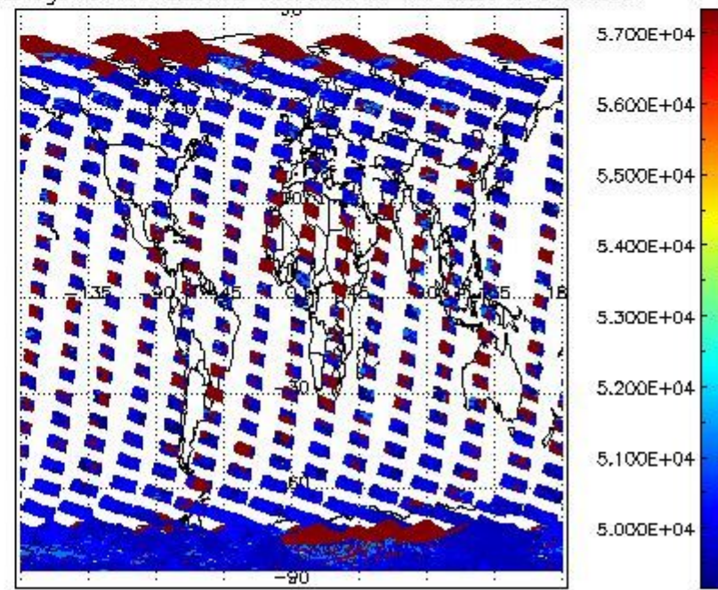
cloud_flags for 16FEB2012 00:00:00 to 17FEB2012 00:00:00
