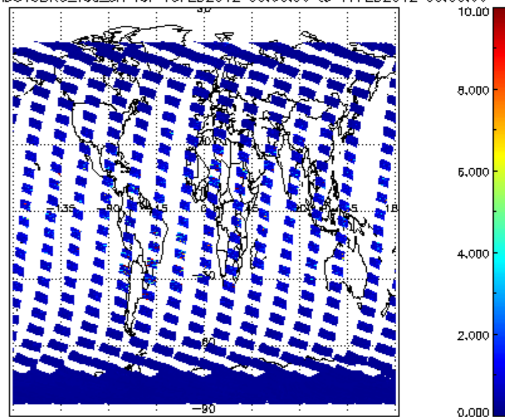
SCIOL2P_NADUV3BRO_vcd_err for 16FEB2012 00:00:00 to 17FEB2012 00:00:00
