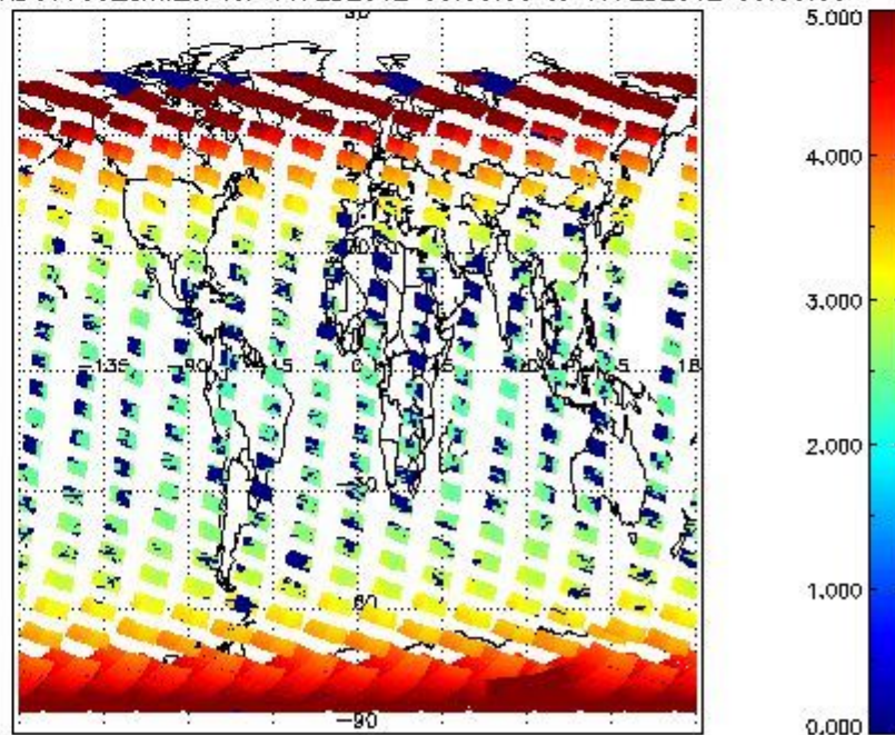
SCIOL2P_NADUV003_amf_cl for 16FEB2012 00:00:00 to 17FEB2012 00:00:00
