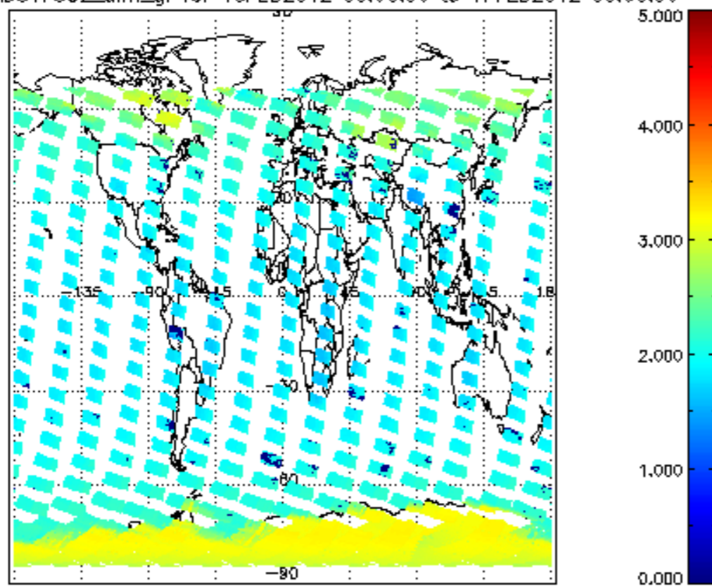
SCIOL2P_NADUV7S02_amf_gr for 16FEB2012 00:00:00 to 17FEB2012 00:00:00
