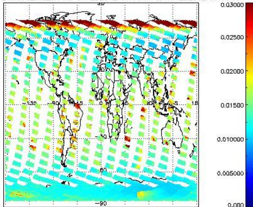
SCIOL2P_NADUV003_vcd_err for 16FEB2012 00:00:00 to 17FEB2012 00:00:00
