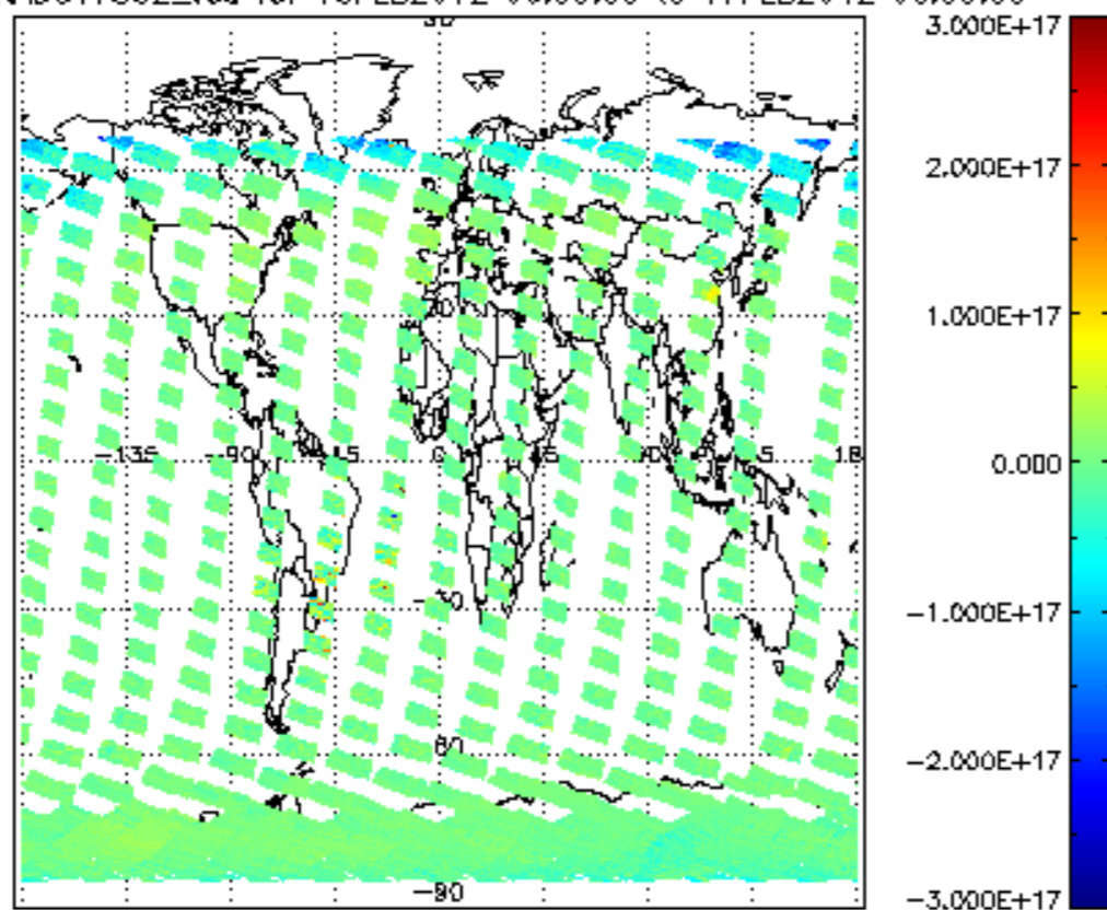
SCIOL2P_NADUV7S02_vcd for 16FEB2012 00:00:00 to 17FEB2012 00:00:00
