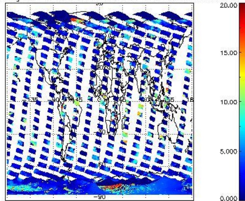
cL_top_height for 16FEB2012 00:00:00 to 17FEB2012 00:00:00
