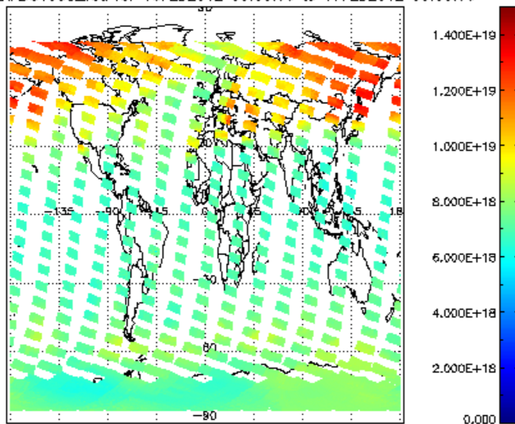
SCIOL2P_NADUV003_vcd for 16FEB2012 00:00:00 to 17FEB2012 00:00:00
