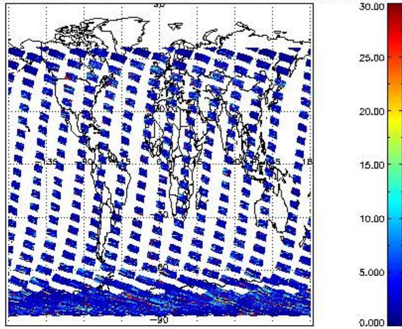
SCIOL2P_NADUV5S02_vcd_err for 16FEB2012 00:00:00 to 17FEB2012 00:00:00
