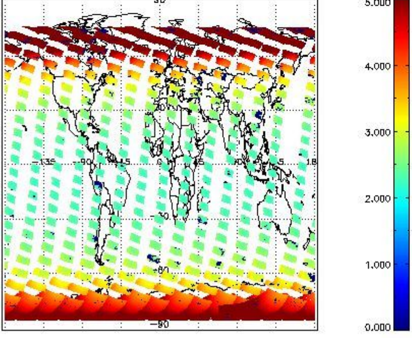
SCIOL2P_NADUV1N02_amf_gr for 16FEB2012 00:00:00 to 17FEB2012 00:00:00
