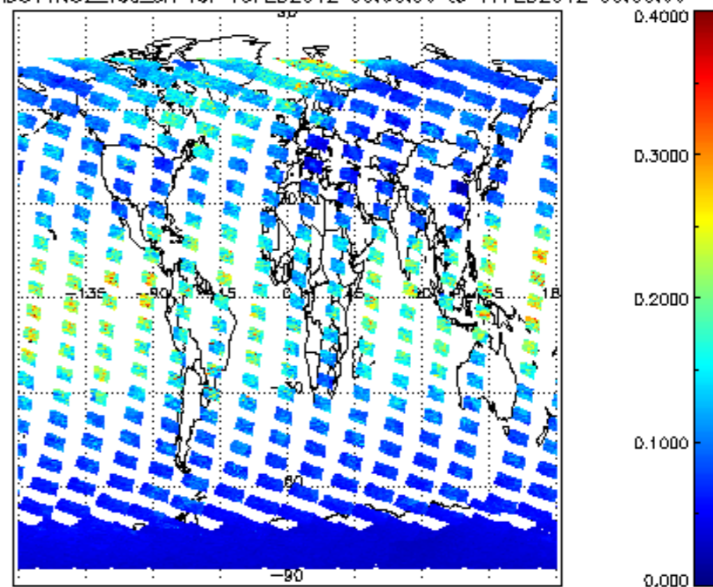
SCIOL2P_NADUV1N02_vcd_err for 16FEB2012 00:00:00 to 17FEB2012 00:00:00
