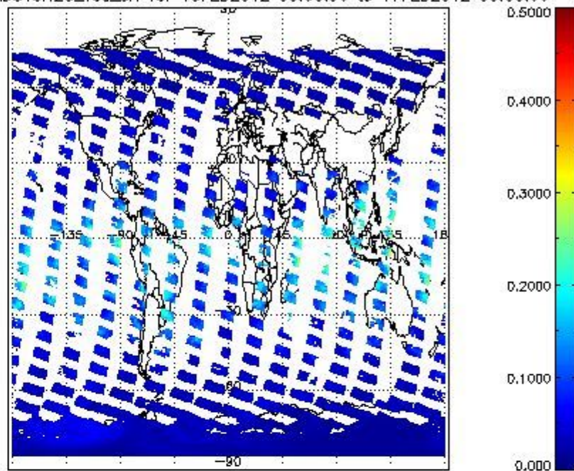
SCIOL2P_NADUV8H2O_vcd_err for 16FEB2012 00:00:00 to 17FEB2012 00:00:00
