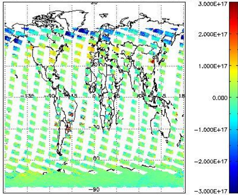
SCIOL2P_NADUV5S02_vcd for 16FEB2012 00:00:00 to 17FEB2012 00:00:00
