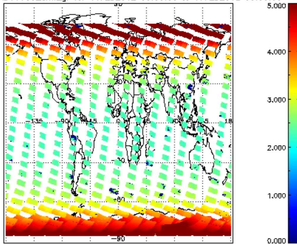
SCIOL2P_NADUV003_amf_gr for 16FEB2012 00:00:00 to 17FEB2012 00:00:00
