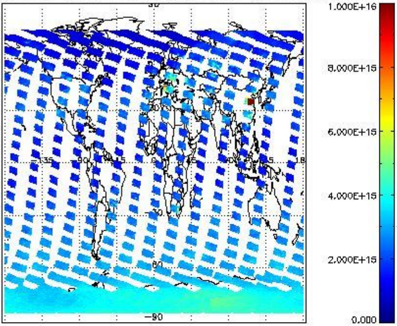
SCIOL2P_NADUV1N02_vcd for 16FEB2012 00:00:00 to 17FEB2012 00:00:00
