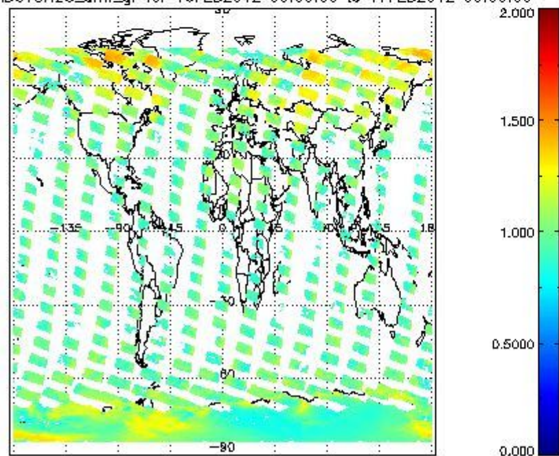
SCIOL2P_NADUV8H2O_amf_gr for 16FEB2012 00:00:00 to 17FEB2012 00:00:00
