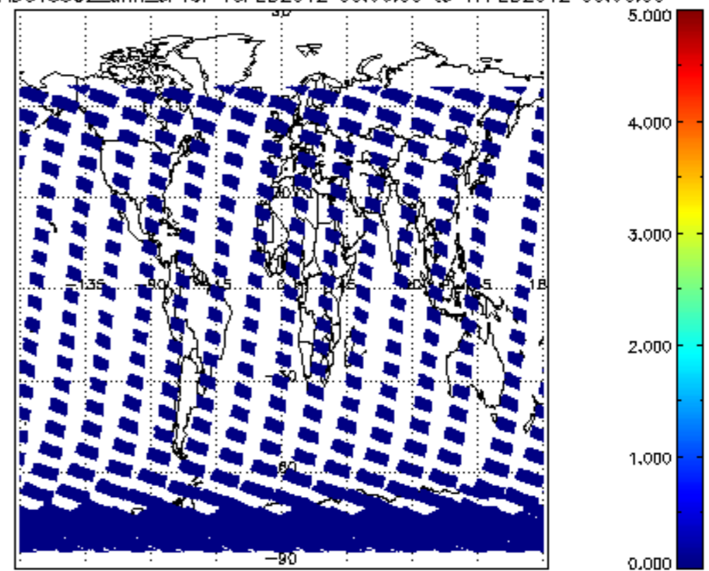
SCIOL2P_NADUV5S02_amf_cl for 16FEB2012 00:00:00 to 17FEB2012 00:00:00
