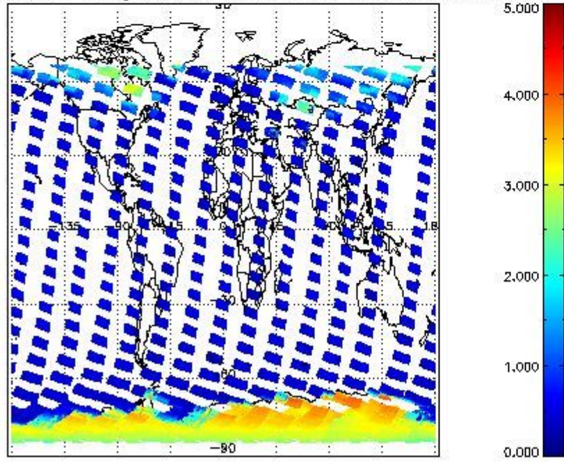
SCIOL2P_NADUV5S02_amf_gr for 16FEB2012 00:00:00 to 17FEB2012 00:00:00
