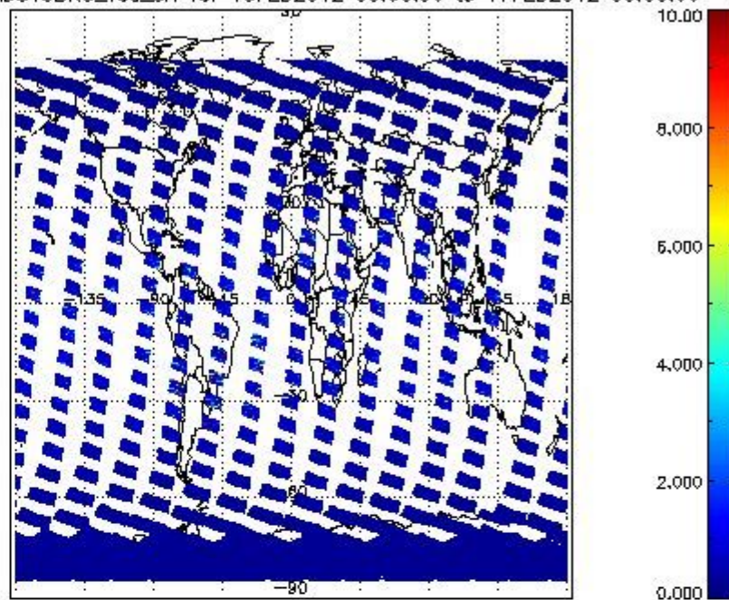
SCIOL2P_NADUV3BRO_vcd_err for 16FEB2012 00:00:00 to 17FEB2012 00:00:00
