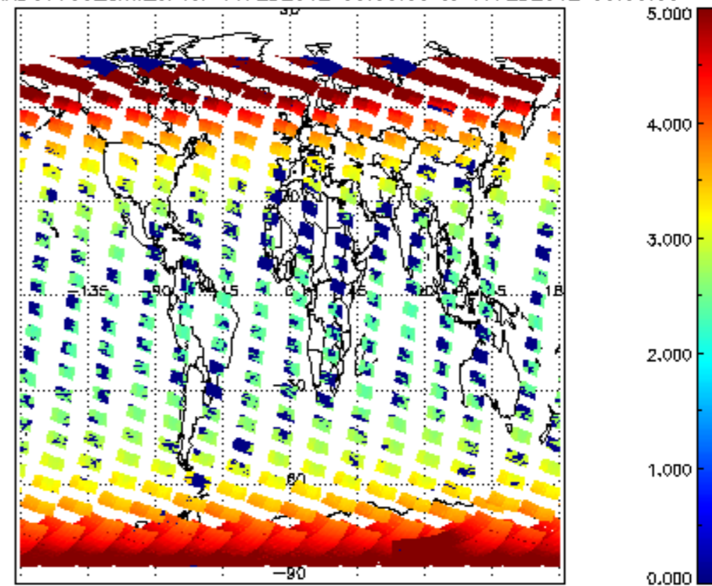
SCIOL2P_NADUV003_amf_cl for 16FEB2012 00:00:00 to 17FEB2012 00:00:00
