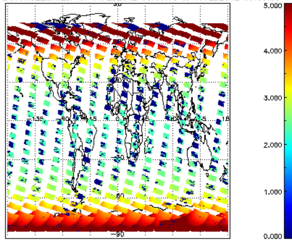
SCIOL2P_NADUV1N02_amf_cl for 16FEB2012 00:00:00 to 17FEB2012 00:00:00
