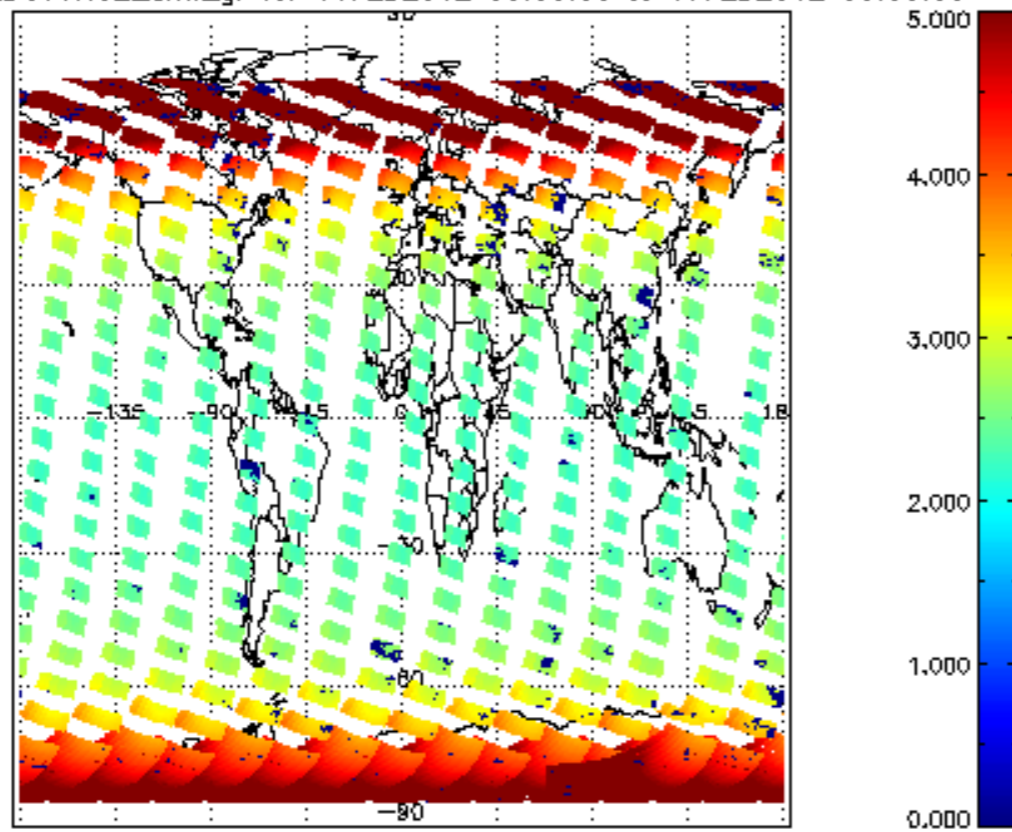
SCIOL2P_NADUV1N02_amf_gr for 16FEB2012 00:00:00 to 17FEB2012 00:00:00
