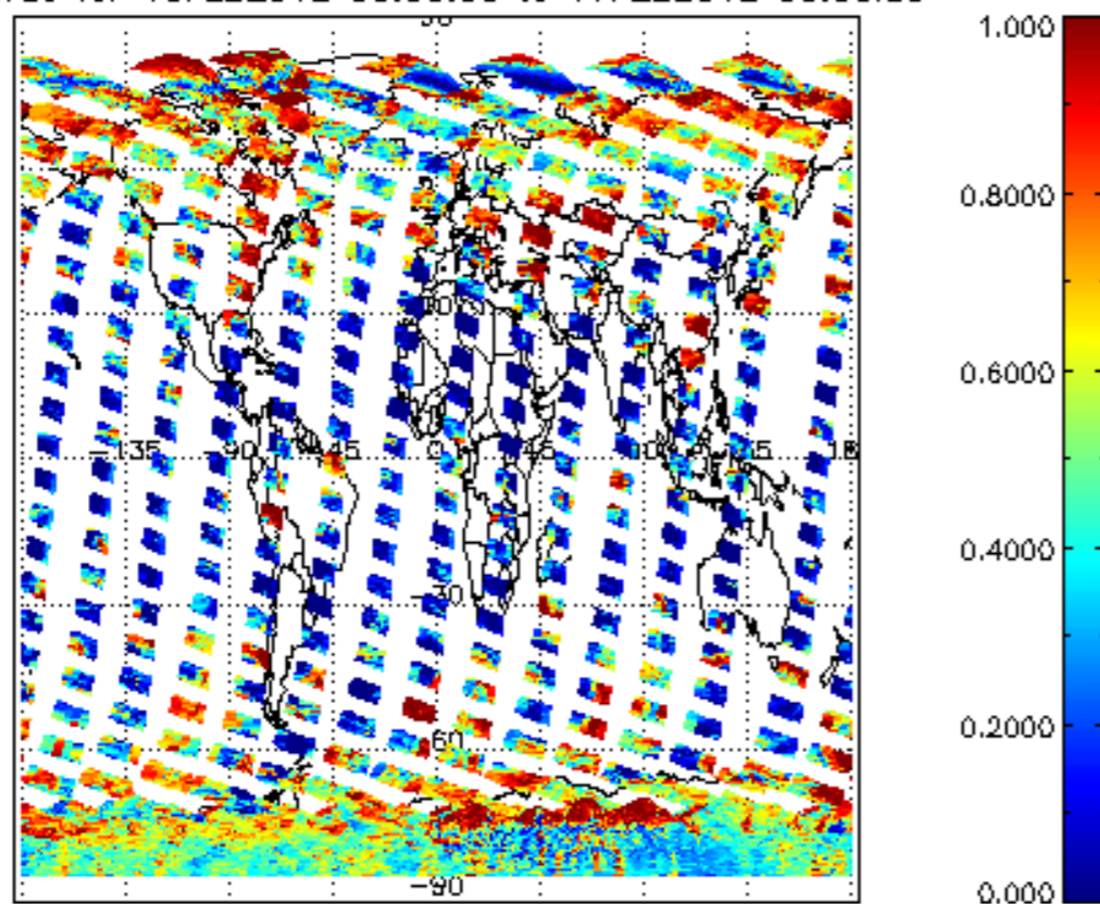
cI_frac for 16FEB2012 00:00:00 to 17FEB2012 00:00:00
