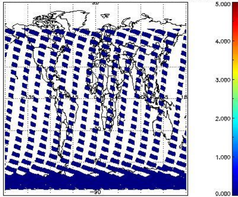
SCIOL2P_NADUV7S02_amf_cl for 16FEB2012 00:00:00 to 17FEB2012 00:00:00
