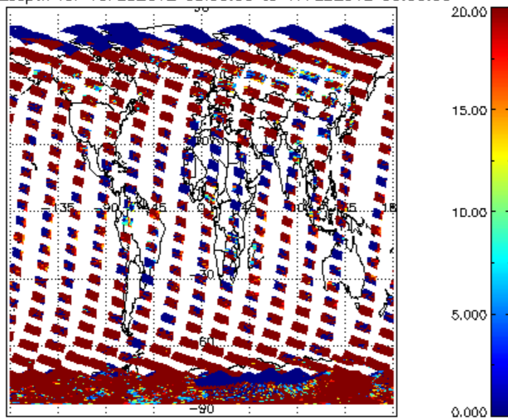
cI_opt_depth for 16FEB2012 00:00:00 to 17FEB2012 00:00:00
