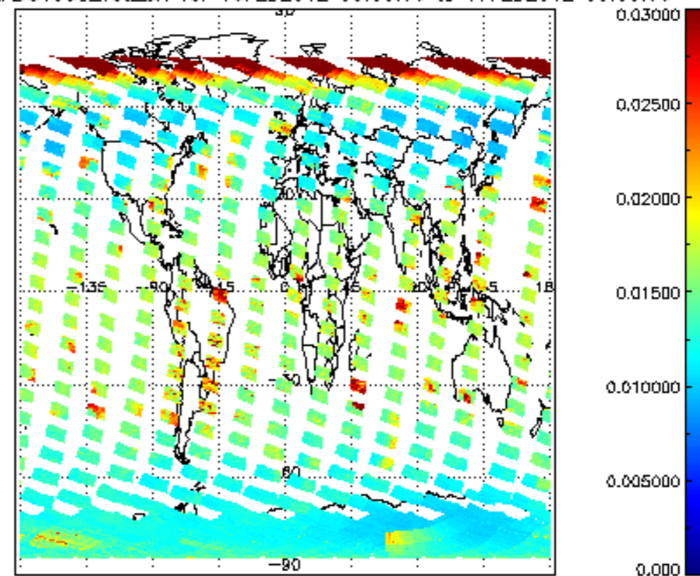
SCIOL2P_NADUV003_vcd_err for 16FEB2012 00:00:00 to 17FEB2012 00:00:00
