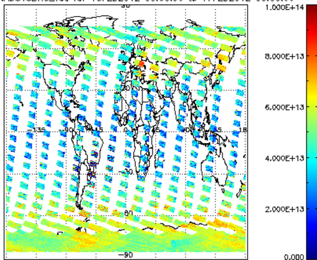
SCIOL2P_NADUV3BRO_vcd for 16FEB2012 00:00:00 to 17FEB2012 00:00:00
