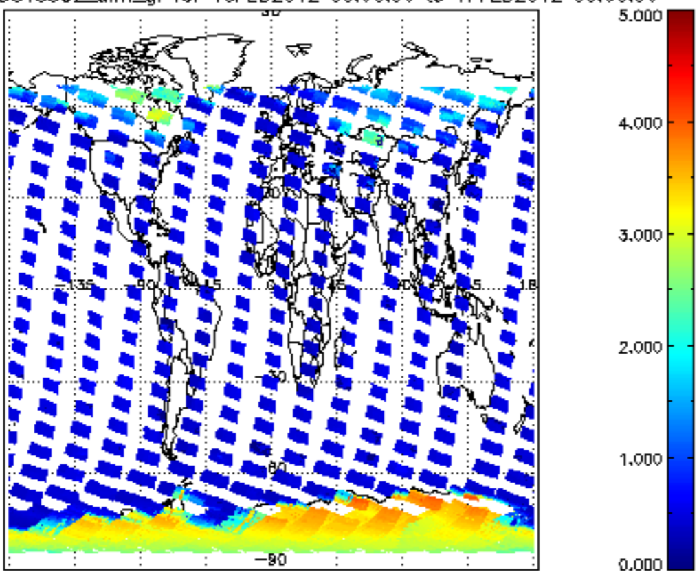
SCIOL2P_NADUV5S02_amf_gr for 16FEB2012 00:00:00 to 17FEB2012 00:00:00
