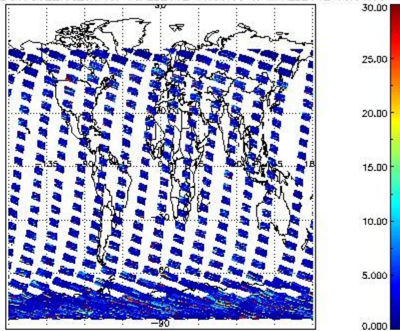
SCIOL2P_NADUV7S02_vcd_err for 16FEB2012 00:00:00 to 17FEB2012 00:00:00
