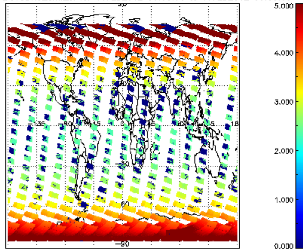
SCIOL2P_NADUV3BRO_amf_cl for 16FEB2012 00:00:00 to 17FEB2012 00:00:00
