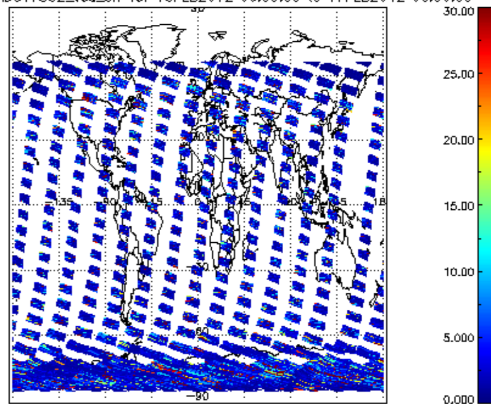
SCIOL2P_NADUV7S02_vcd_err for 16FEB2012 00:00:00 to 17FEB2012 00:00:00
