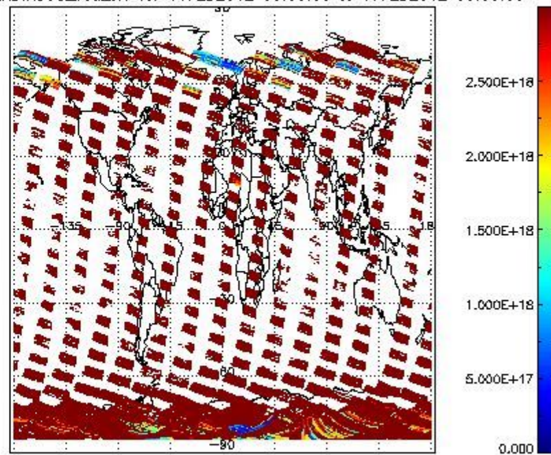
SCIDL2P_NADIR3CO_vcd_err for 16FEB2012 00:00:00 to 17FEB2012 00:00:00
