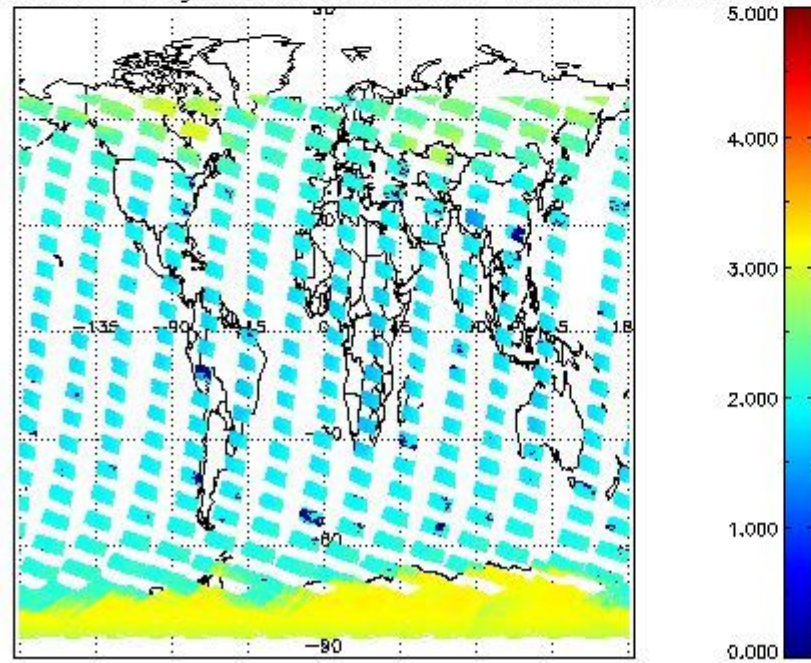
SCIOL2P_NADUV7S02_amf_gr for 16FEB2012 00:00:00 to 17FEB2012 00:00:00
