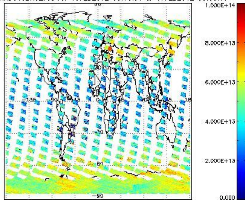
SCIOL2P_NADUV3BRO_vcd for 16FEB2012 00:00:00 to 17FEB2012 00:00:00
