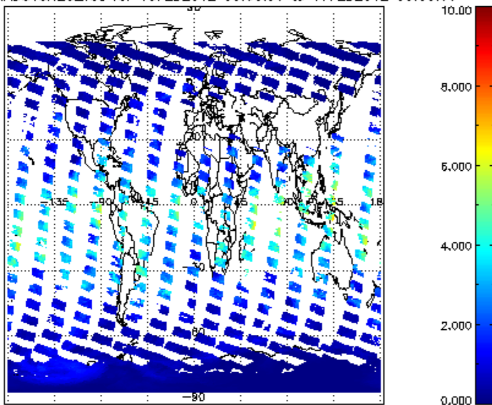
SCIOL2P_NADUV8H2O_vcd for 16FEB2012 00:00:00 to 17FEB2012 00:00:00
