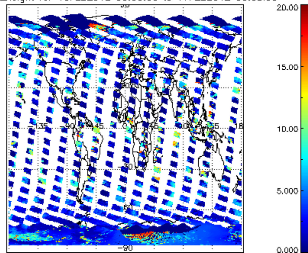
cI_top_height for 16FEB2012 00:00:00 to 17FEB2012 00:00:00
