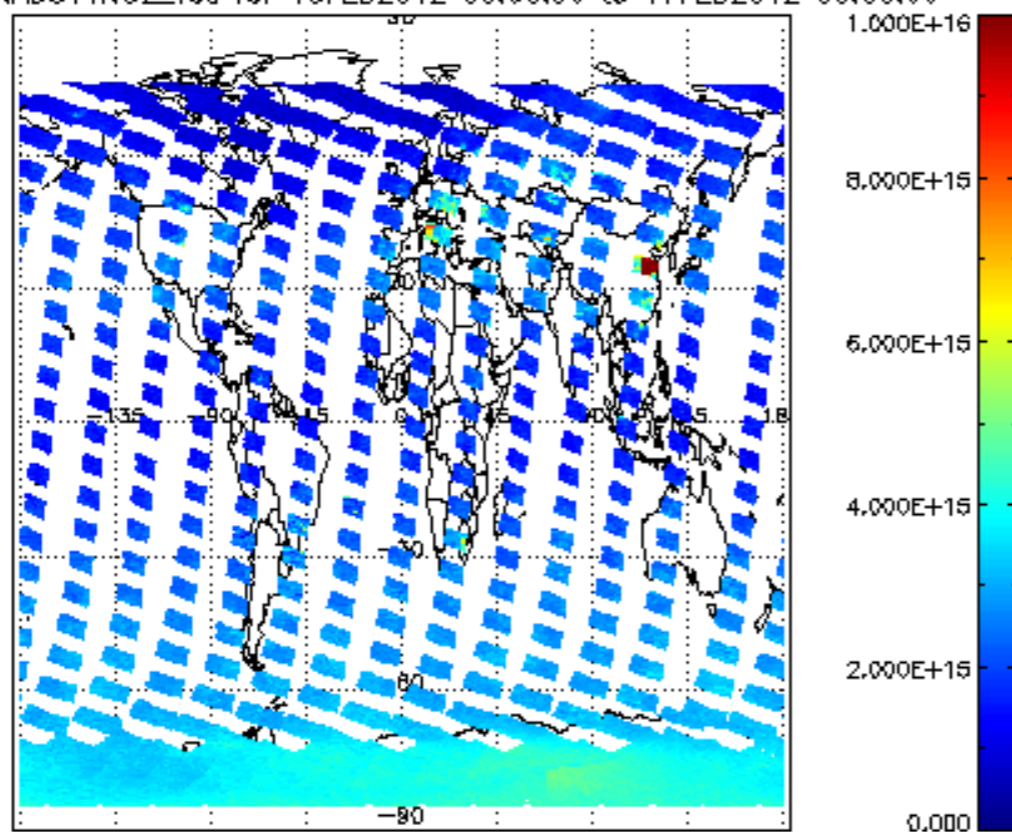
SCIOL2P_NADUV1N02_vcd for 16FEB2012 00:00:00 to 17FEB2012 00:00:00
