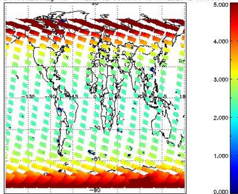
SCIOL2P_NADUV003_amf_gr for 16FEB2012 00:00:00 to 17FEB2012 00:00:00
