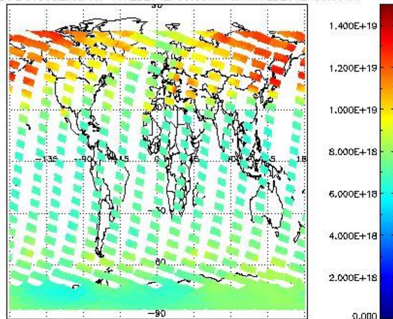
SCIOL2P_NADUV003_vcd for 16FEB2012 00:00:00 to 17FEB2012 00:00:00
