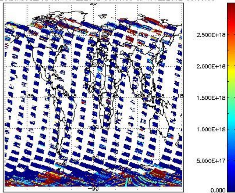
SCIDL2P_NADIR3CO_vcd for 16FEB2012 00:00:00 to 17FEB2012 00:00:00
