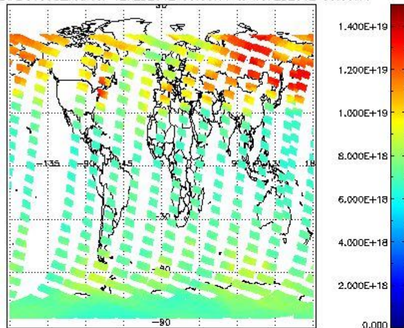
SCIOL2P_NADUV003_vcd for 12FEB2012 00:00:00 to 13FEB2012 00:00:00
