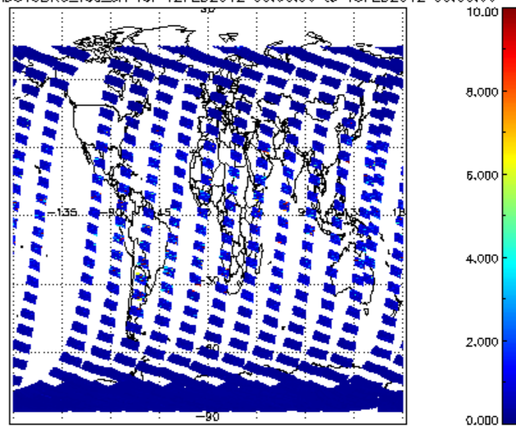
SCIOL2P_NADUV3BRO_vcd_err for 12FEB2012 00:00:00 to 13FEB2012 00:00:00
