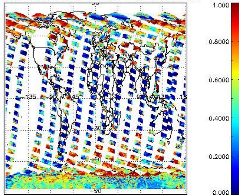
cL_frae for 12FEB2012 00:00:00 to 13FEB2012 00:00:00
