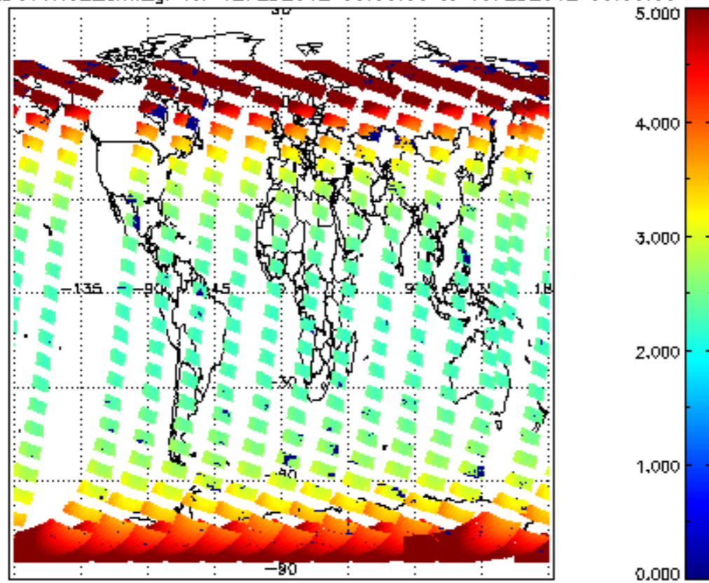
SCIOL2P_NADUV1N02_amf_gr for 12FEB2012 00:00:00 to 13FEB2012 00:00:00
