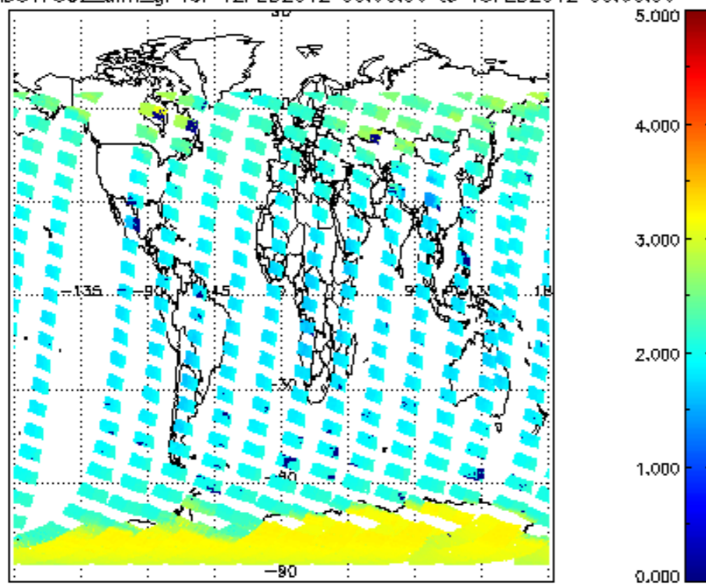
SCIOL2P_NADUV7S02_amf_gr for 12FEB2012 00:00:00 to 13FEB2012 00:00:00
