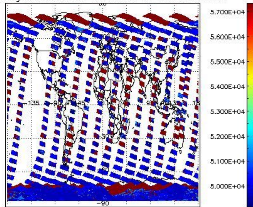
cloud_flags for 12FEB2012 00:00:00 to 13FEB2012 00:00:00
