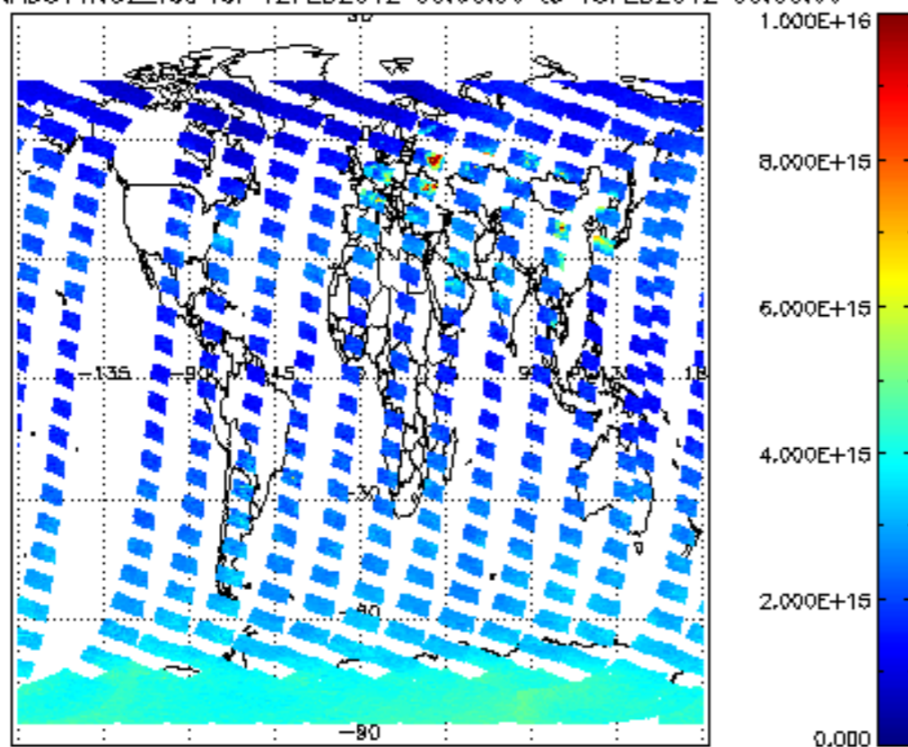
SCIOL2P_NADUV1N02_vcd for 12FEB2012 00:00:00 to 13FEB2012 00:00:00
