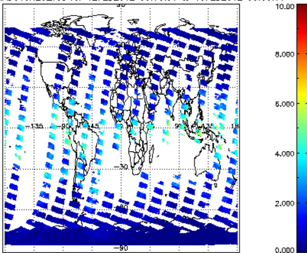
SCIOL2P_NADUV8H2O_vcd for 12FEB2012 00:00:00 to 13FEB2012 00:00:00
