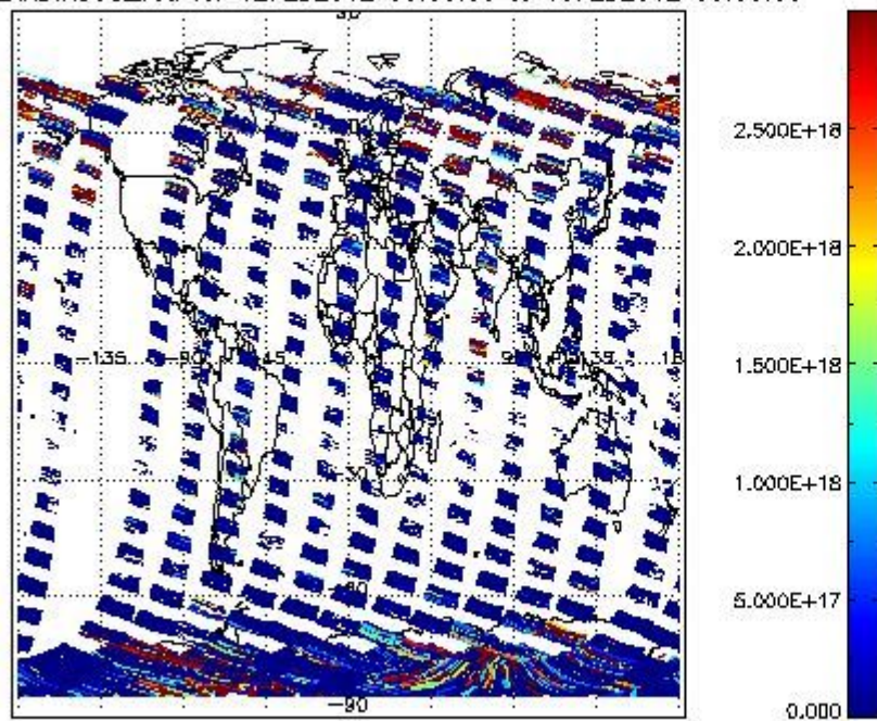
SCIDL2P_NADIR3CO_vcd for 12FEB2012 00:00:00 to 13FEB2012 00:00:00
