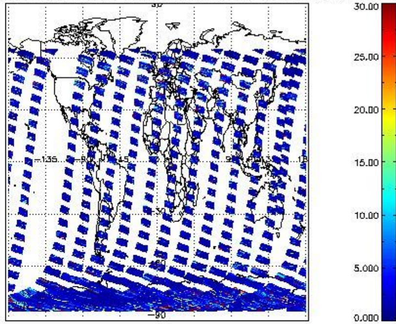
SCIOL2P_NADUV5S02_vcd_err for 12FEB2012 00:00:00 to 13FEB2012 00:00:00
