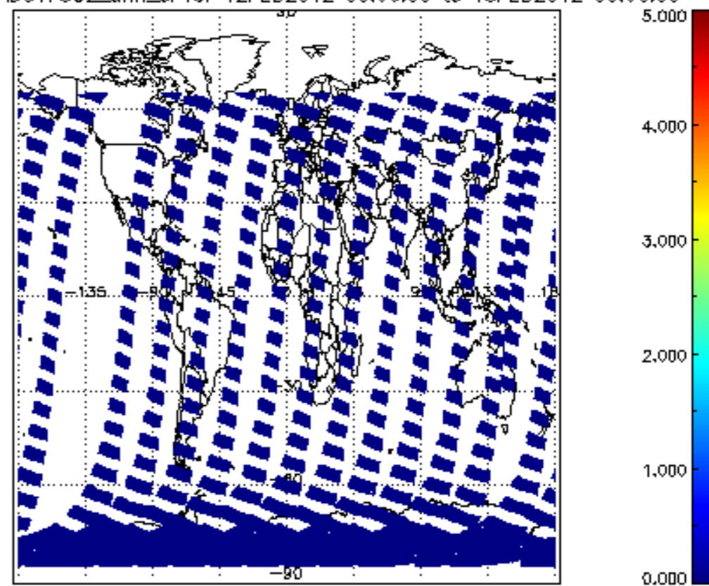
SCIOL2P_NADUV7S02_amf_cl for 12FEB2012 00:00:00 to 13FEB2012 00:00:00
