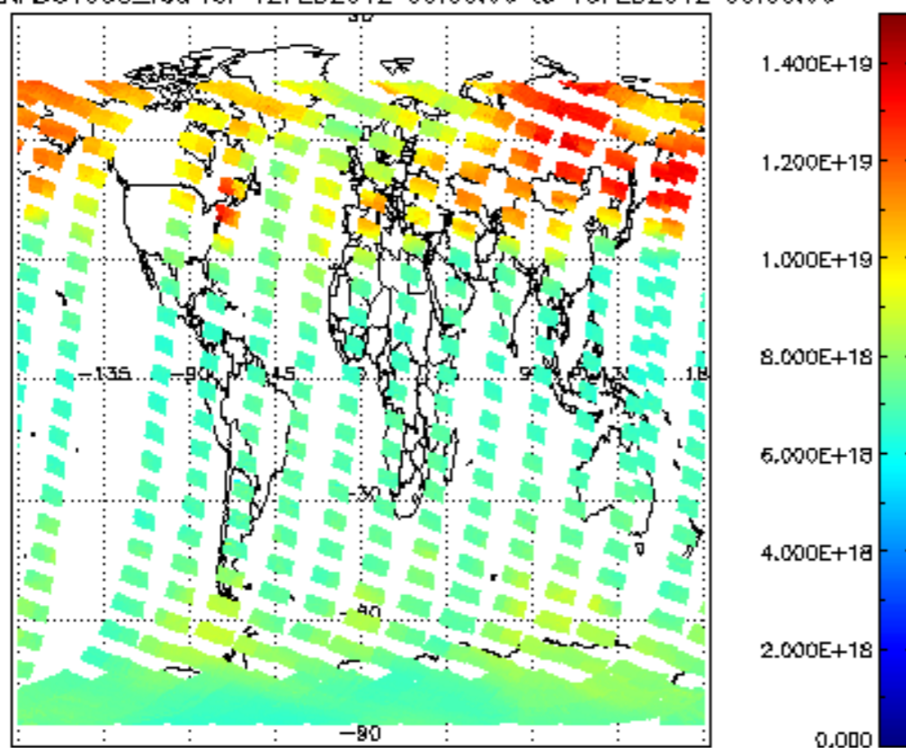
SCIOL2P_NADUV003_vcd for 12FEB2012 00:00:00 to 13FEB2012 00:00:00
