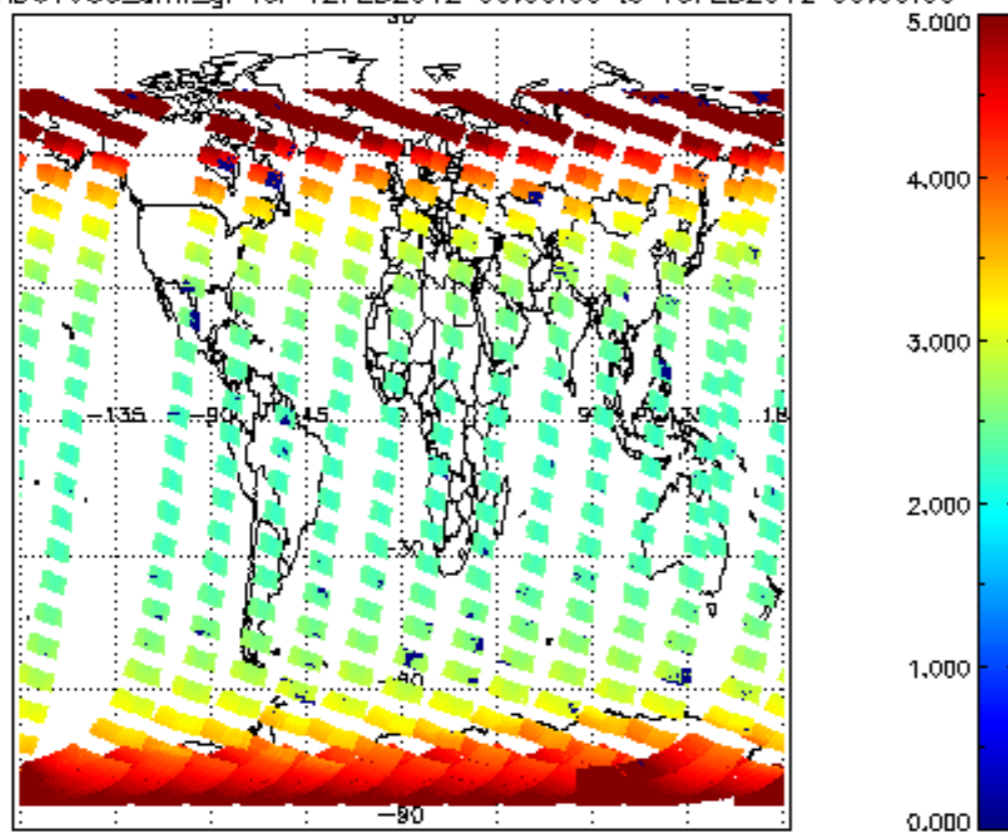
SCIOL2P_NADUV003_amf_gr for 12FEB2012 00:00:00 to 13FEB2012 00:00:00
