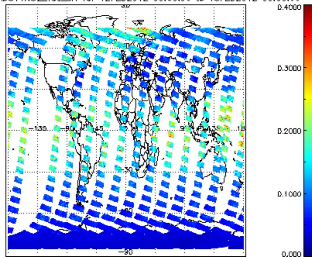
SCIOL2P_NADUV1N02_vcd_err for 12FEB2012 00:00:00 to 13FEB2012 00:00:00
