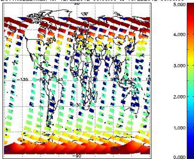
SCIOL2P_NADUV1N02_amf_cl for 12FEB2012 00:00:00 to 13FEB2012 00:00:00
