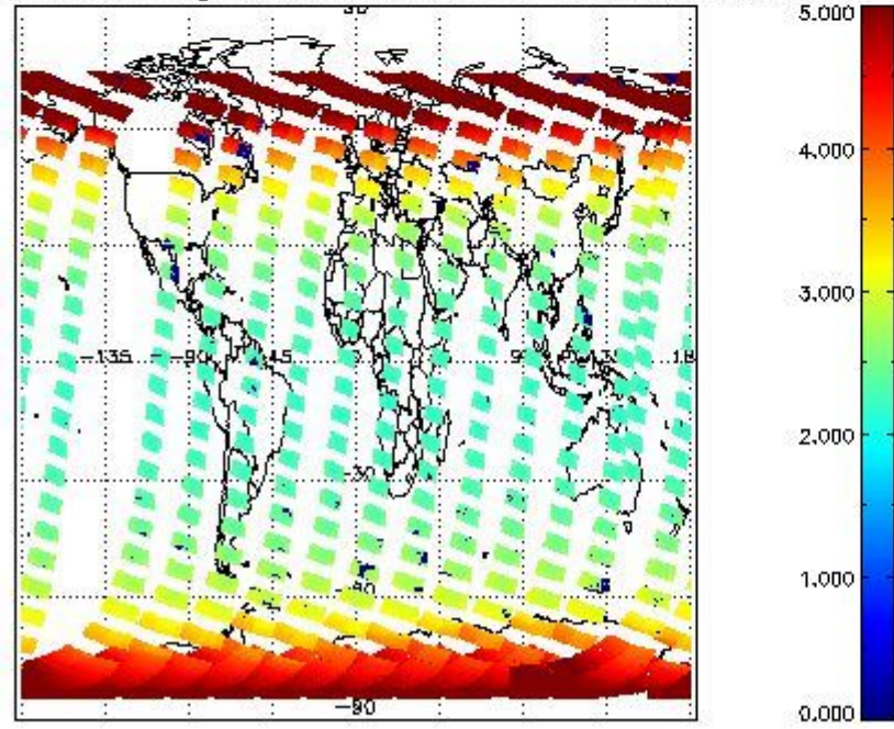
SCIOL2P_NADUV3BRO_amf_gr for 12FEB2012 00:00:00 to 13FEB2012 00:00:00
