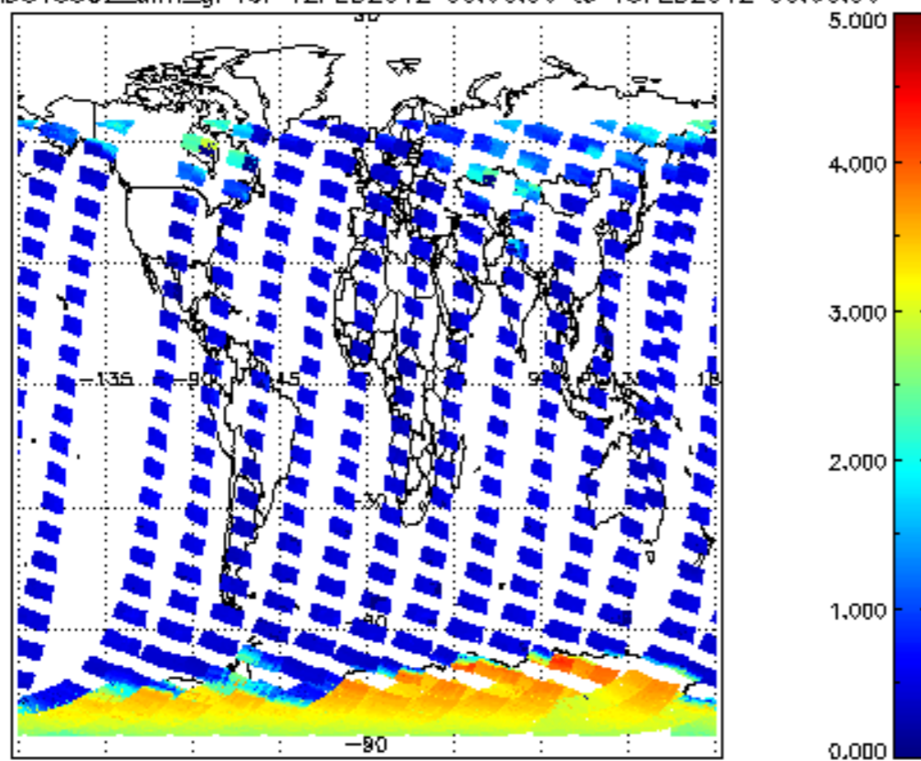
SCIOL2P_NADUV5S02_amf_gr for 12FEB2012 00:00:00 to 13FEB2012 00:00:00
