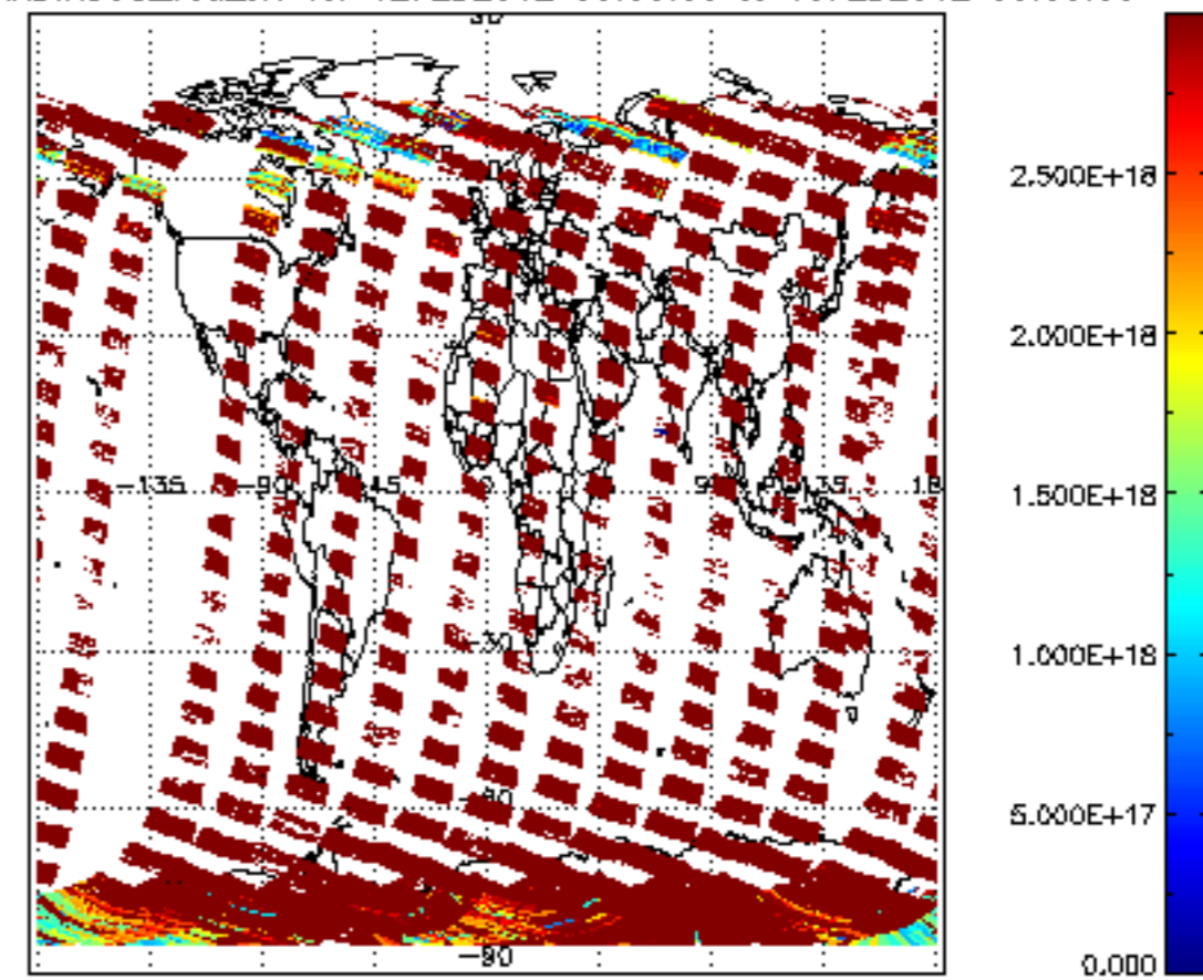
SCIOL2P_NADIR3CO_vcd_err for 12FEB2012 00:00:00 to 13FEB2012 00:00:00
