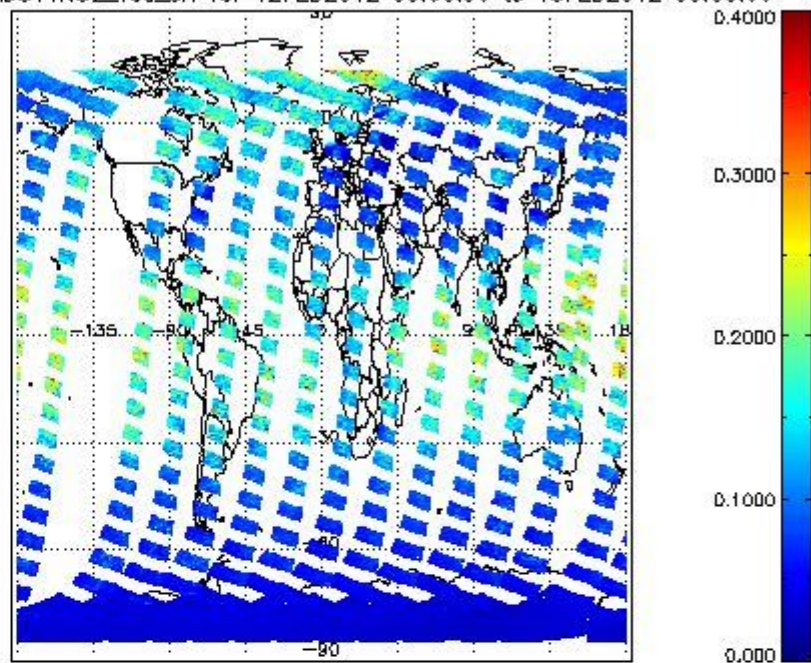
SCIOL2P_NADUV1N02_vcd_err for 12FEB2012 00:00:00 to 13FEB2012 00:00:00
