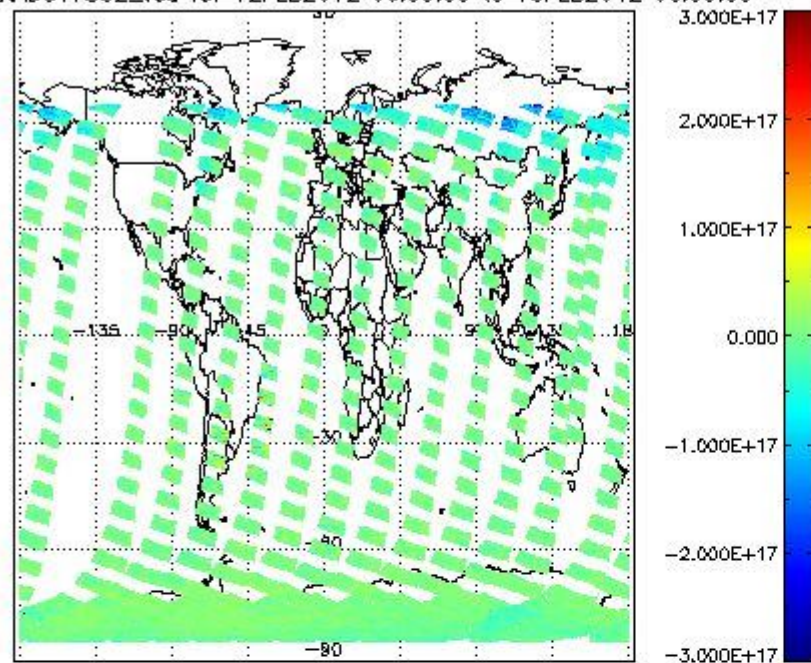
SCIOL2P_NADUV7S02_vcd for 12FEB2012 00:00:00 to 13FEB2012 00:00:00
