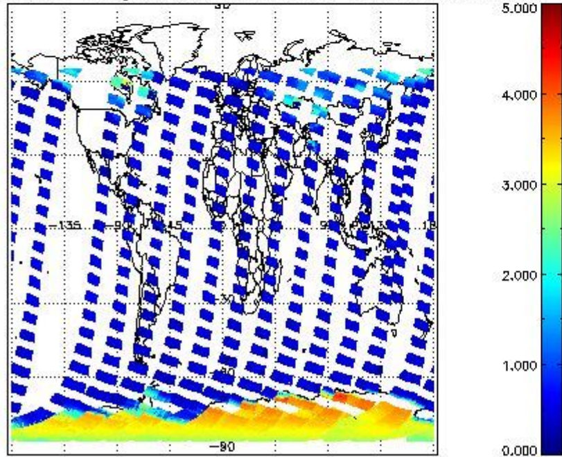
SCIOL2P_NADUV5S02_amf_gr for 12FEB2012 00:00:00 to 13FEB2012 00:00:00
