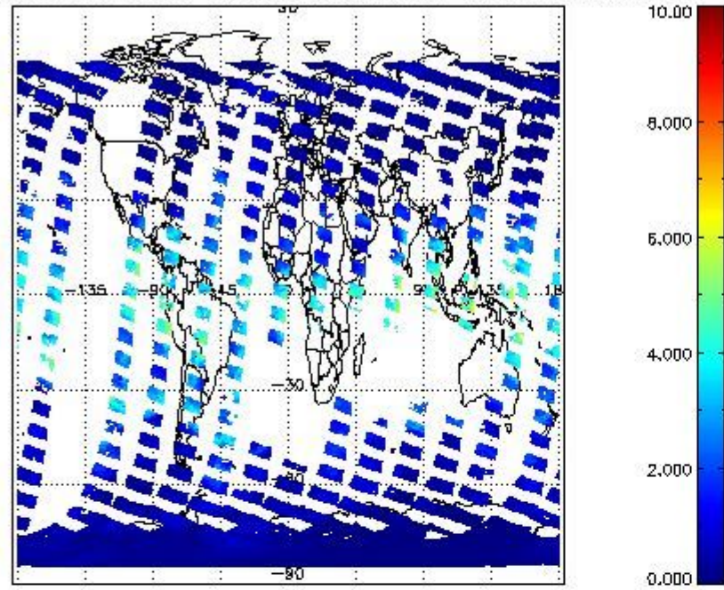
SCIOL2P_NADUV8H2O_vcd for 12FEB2012 00:00:00 to 13FEB2012 00:00:00
