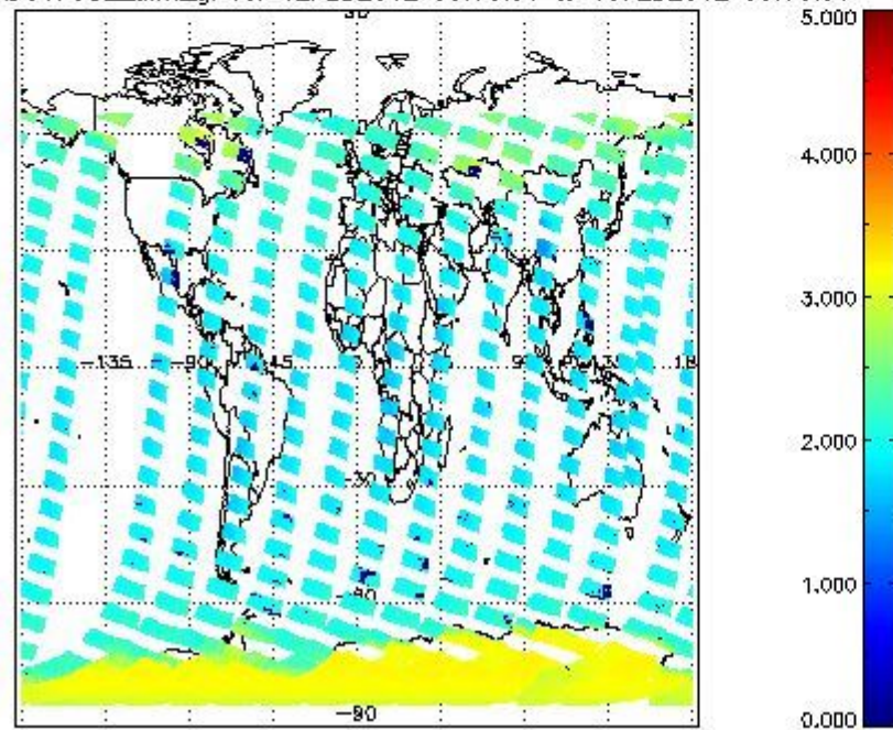
SCIOL2P_NADUV7S02_amf_gr for 12FEB2012 00:00:00 to 13FEB2012 00:00:00
