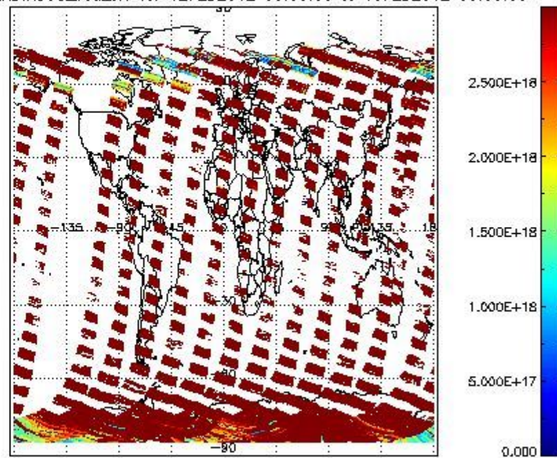
SCIDL2P_NADIR3CO_vcd_err for 12FEB2012 00:00:00 to 13FEB2012 00:00:00
