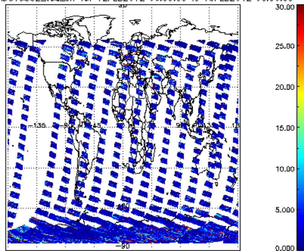
SCIOL2P_NADUV5S02_vcd_err for 12FEB2012 00:00:00 to 13FEB2012 00:00:00
