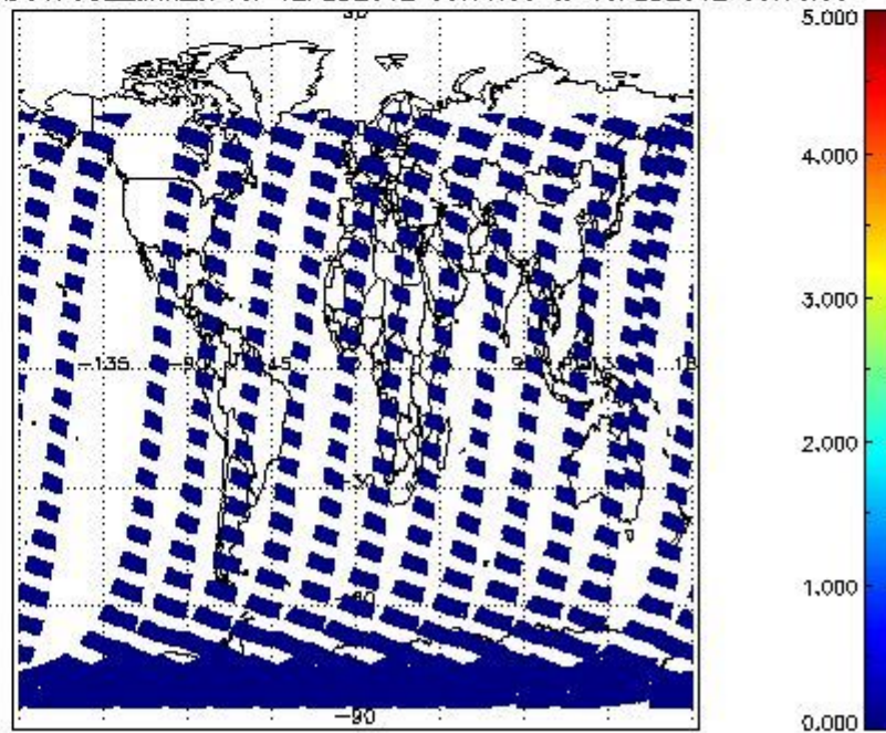
SCIOL2P_NADUV7S02_amf_cl for 12FEB2012 00:00:00 to 13FEB2012 00:00:00
