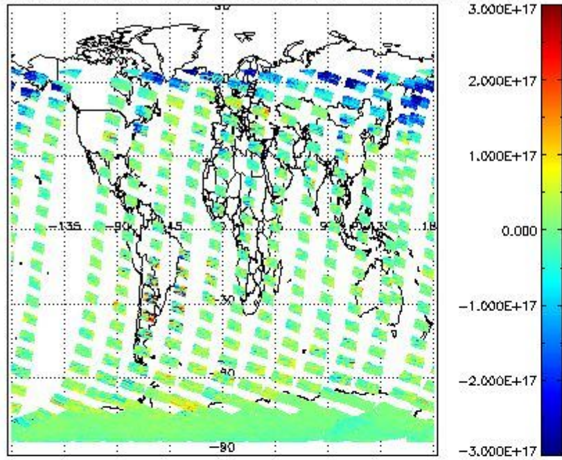
SCIOL2P_NADUV5S02_vcd for 12FEB2012 00:00:00 to 13FEB2012 00:00:00
