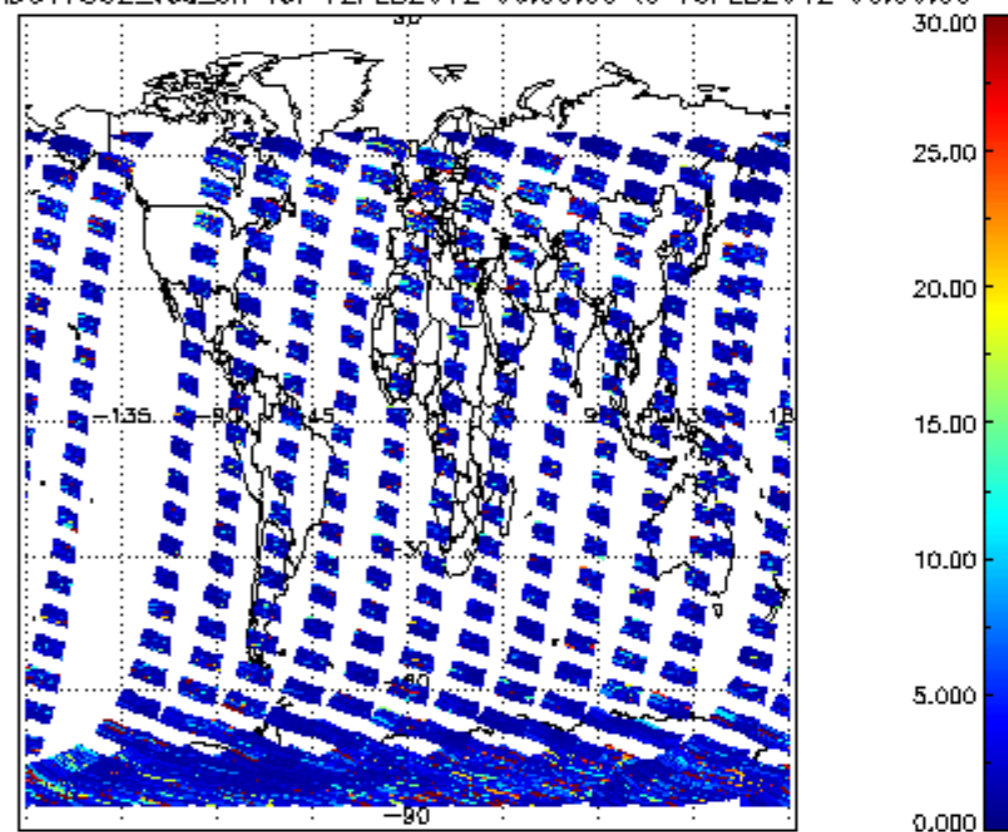
SCIOL2P_NADUV7S02_vcd_err for 12FEB2012 00:00:00 to 13FEB2012 00:00:00
