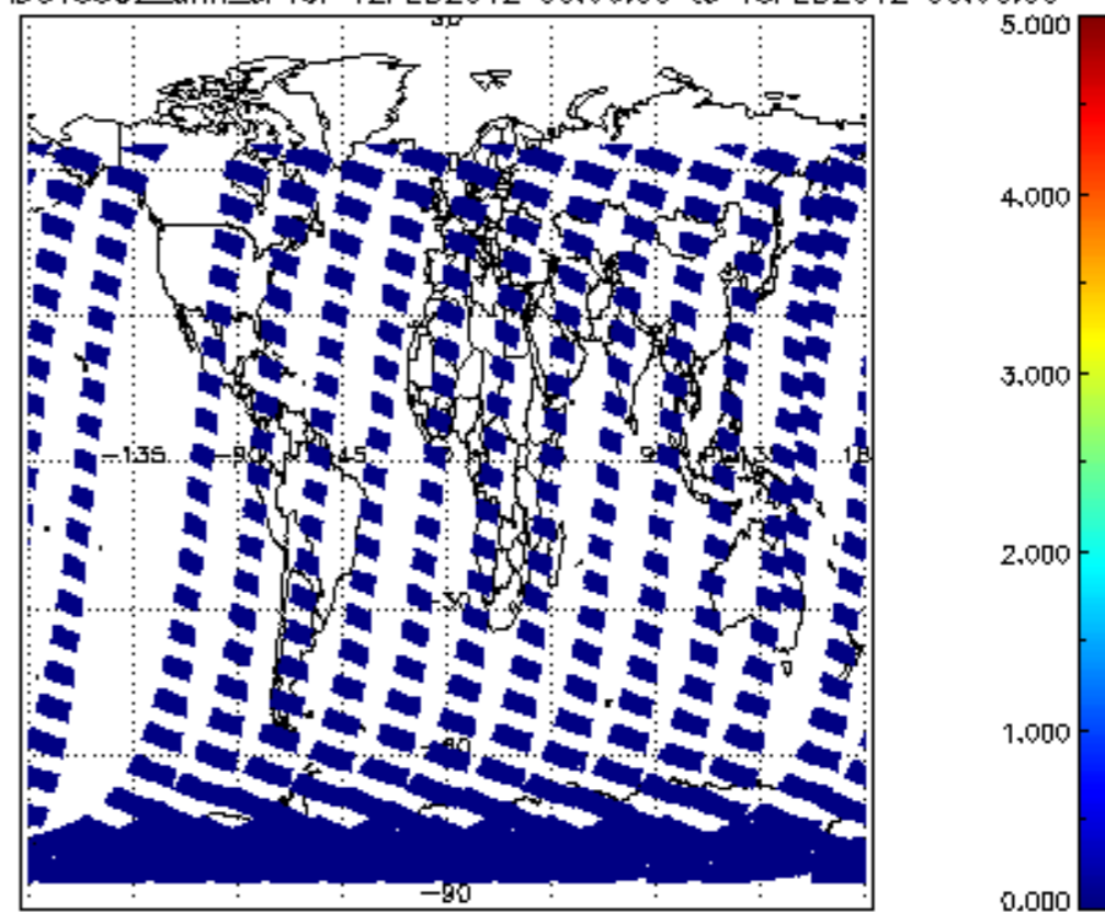
SCIOL2P_NADUV5S02_amf_cl for 12FEB2012 00:00:00 to 13FEB2012 00:00:00
