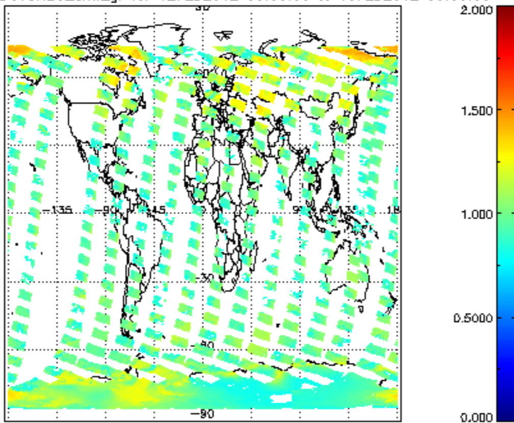
SCIOL2P_NADUV8H2O_amf_gr for 12FEB2012 00:00:00 to 13FEB2012 00:00:00
