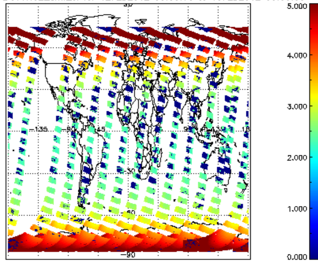
SCIOL2P_NADUV1N02_amf_cl for 12FEB2012 00:00:00 to 13FEB2012 00:00:00
