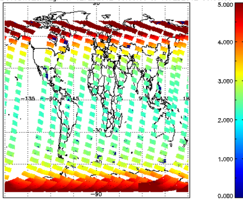
SCIOL2P_NADUV3BRO_amf_gr for 12FEB2012 00:00:00 to 13FEB2012 00:00:00
