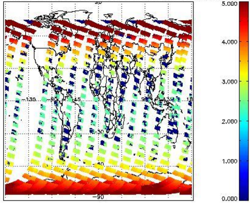
SCIOL2P_NADUV3BRO_amf_cl for 12FEB2012 00:00:00 to 13FEB2012 00:00:00
