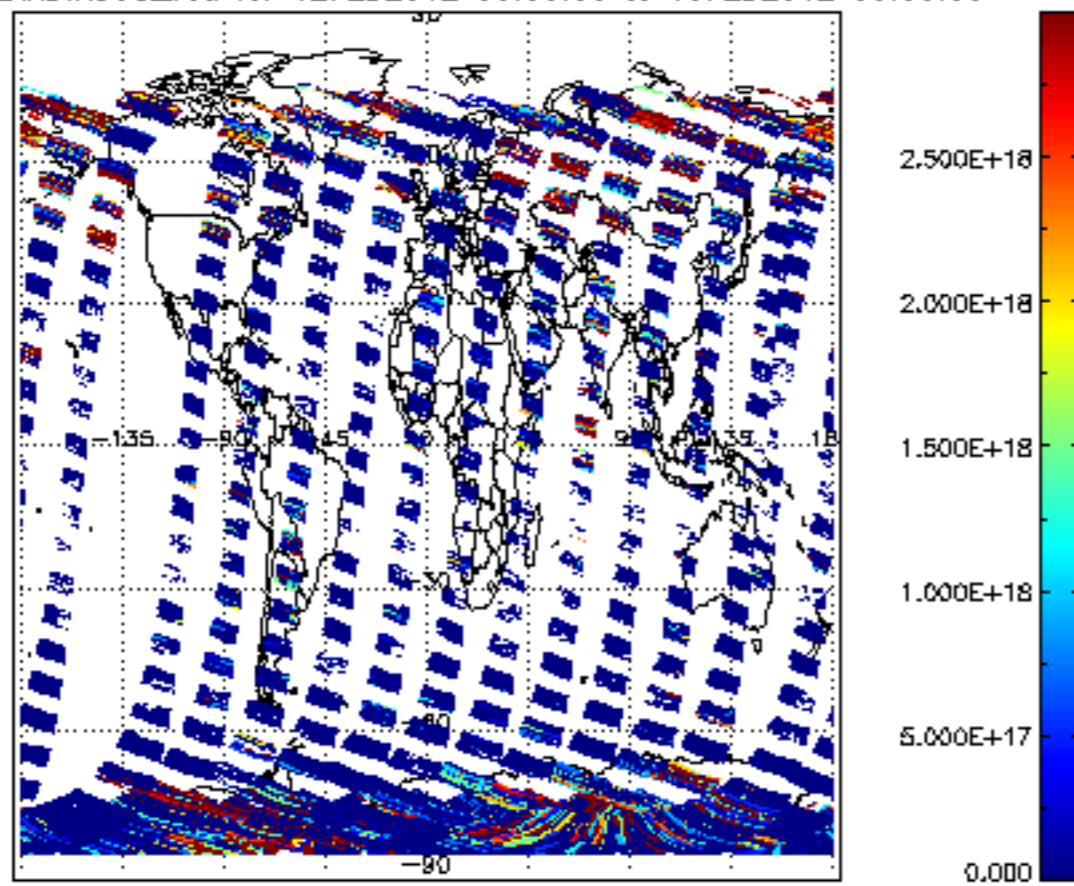
SCIOL2P_NADIR3CO_vcd for 12FEB2012 00:00:00 to 13FEB2012 00:00:00
