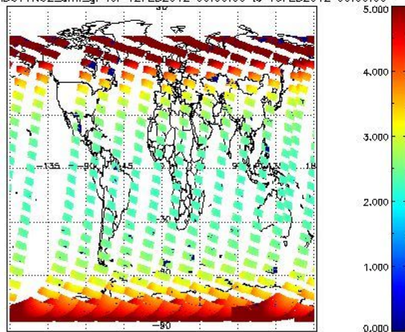
SCIOL2P_NADUV1N02_amf_gr for 12FEB2012 00:00:00 to 13FEB2012 00:00:00
