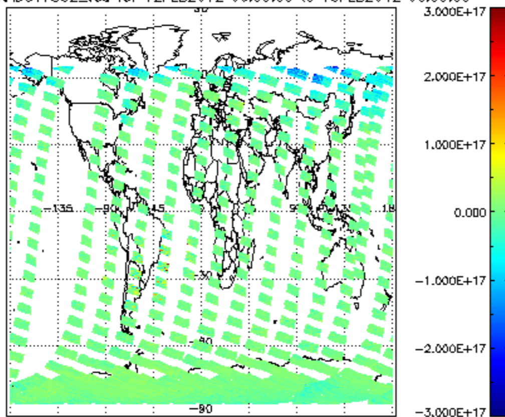
SCIOL2P_NADUV7S02_vcd for 12FEB2012 00:00:00 to 13FEB2012 00:00:00
