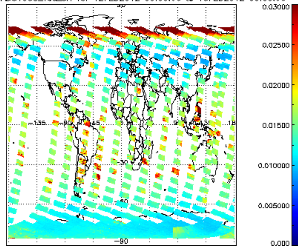
SCIOL2P_NADUV003_vcd_err for 12FEB2012 00:00:00 to 13FEB2012 00:00:00
