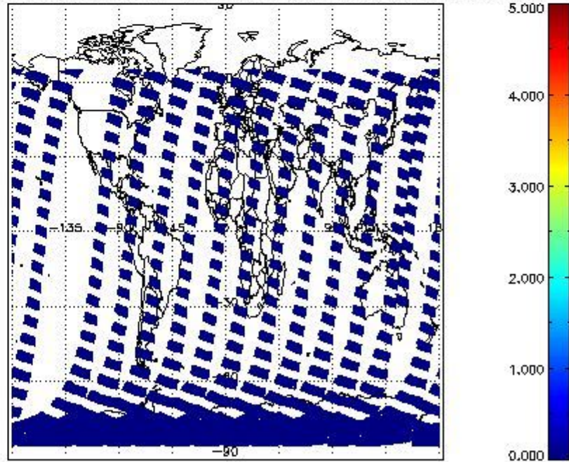
SCIOL2P_NADUV5S02_amf_cl for 12FEB2012 00:00:00 to 13FEB2012 00:00:00
