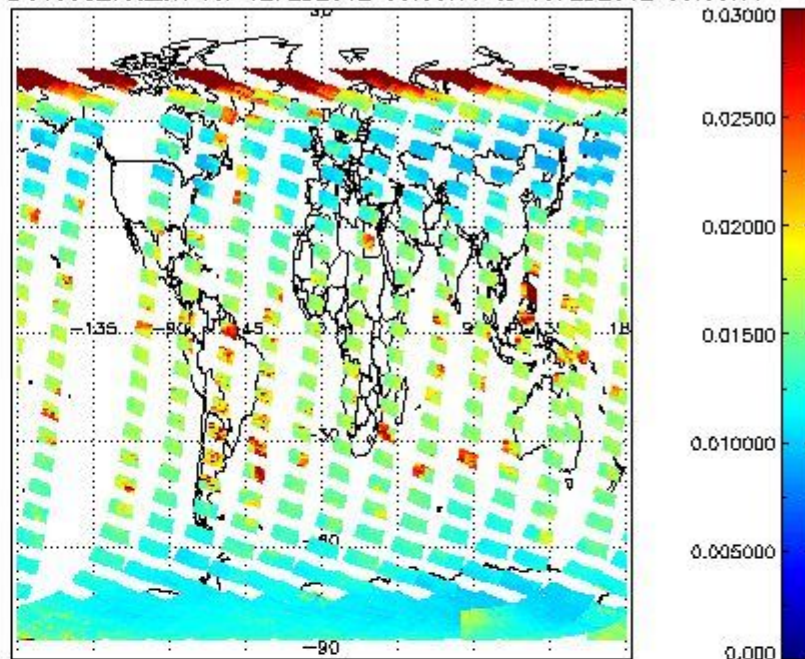
SCIOL2P_NADUV003_vcd_err for 12FEB2012 00:00:00 to 13FEB2012 00:00:00
