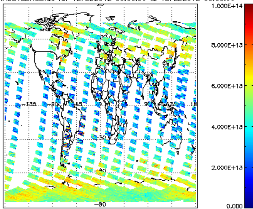
SCIOL2P_NADUV3BRO_vcd for 12FEB2012 00:00:00 to 13FEB2012 00:00:00
