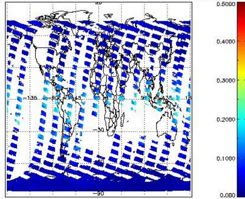
SCIOL2P_NADUV8H2O_vcd_err for 12FEB2012 00:00:00 to 13FEB2012 00:00:00
