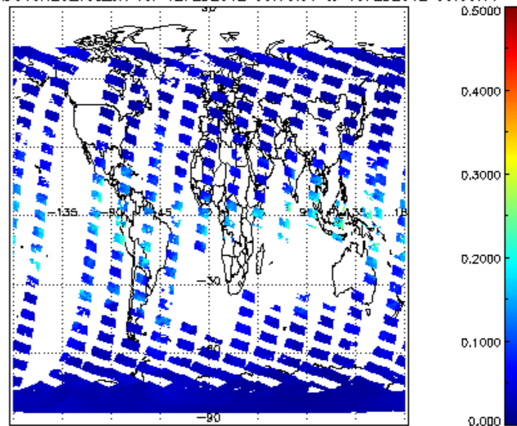
SCIOL2P_NADUV8H2O_vcd_err for 12FEB2012 00:00:00 to 13FEB2012 00:00:00
