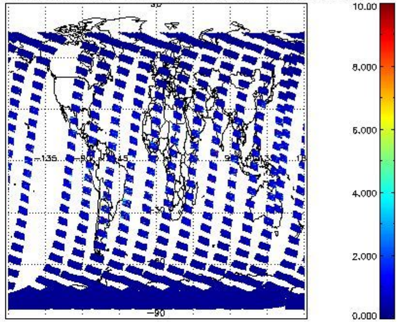
SCIOL2P_NADUV3BRO_vcd_err for 12FEB2012 00:00:00 to 13FEB2012 00:00:00
