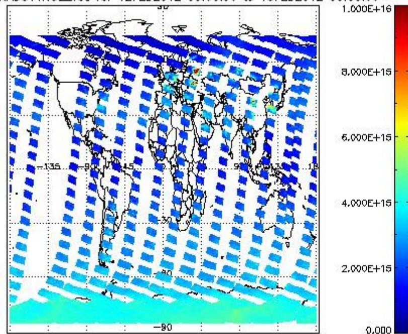
SCIOL2P_NADUV1N02_vcd for 12FEB2012 00:00:00 to 13FEB2012 00:00:00
