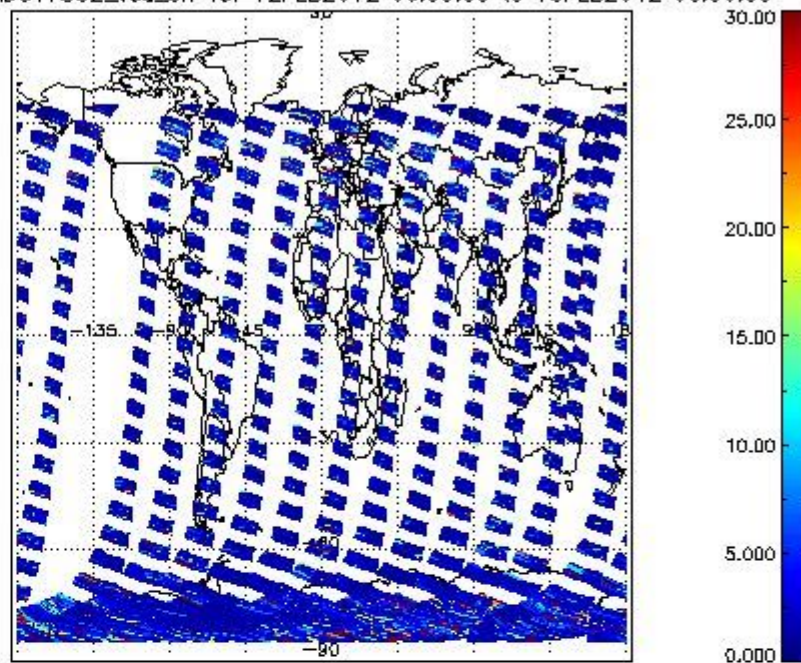
SCIOL2P_NADUV7S02_vcd_err for 12FEB2012 00:00:00 to 13FEB2012 00:00:00
