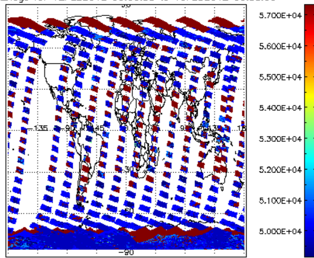
cloud_flags for 12FEB2012 00:00:00 to 13FEB2012 00:00:00
