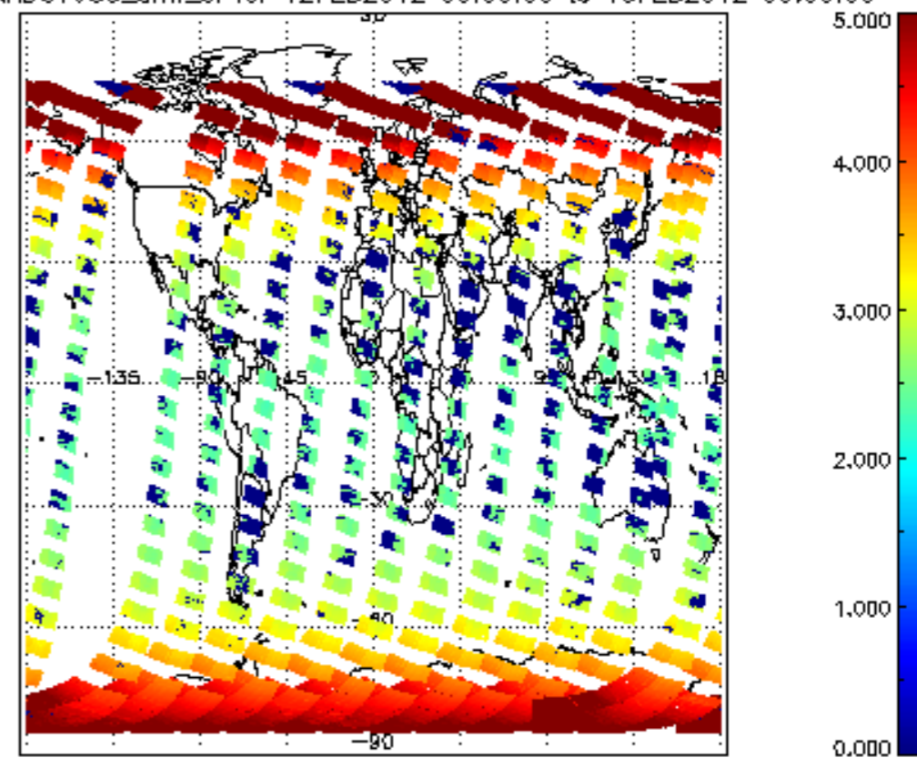
SCIOL2P_NADUV003_amf_cl for 12FEB2012 00:00:00 to 13FEB2012 00:00:00
