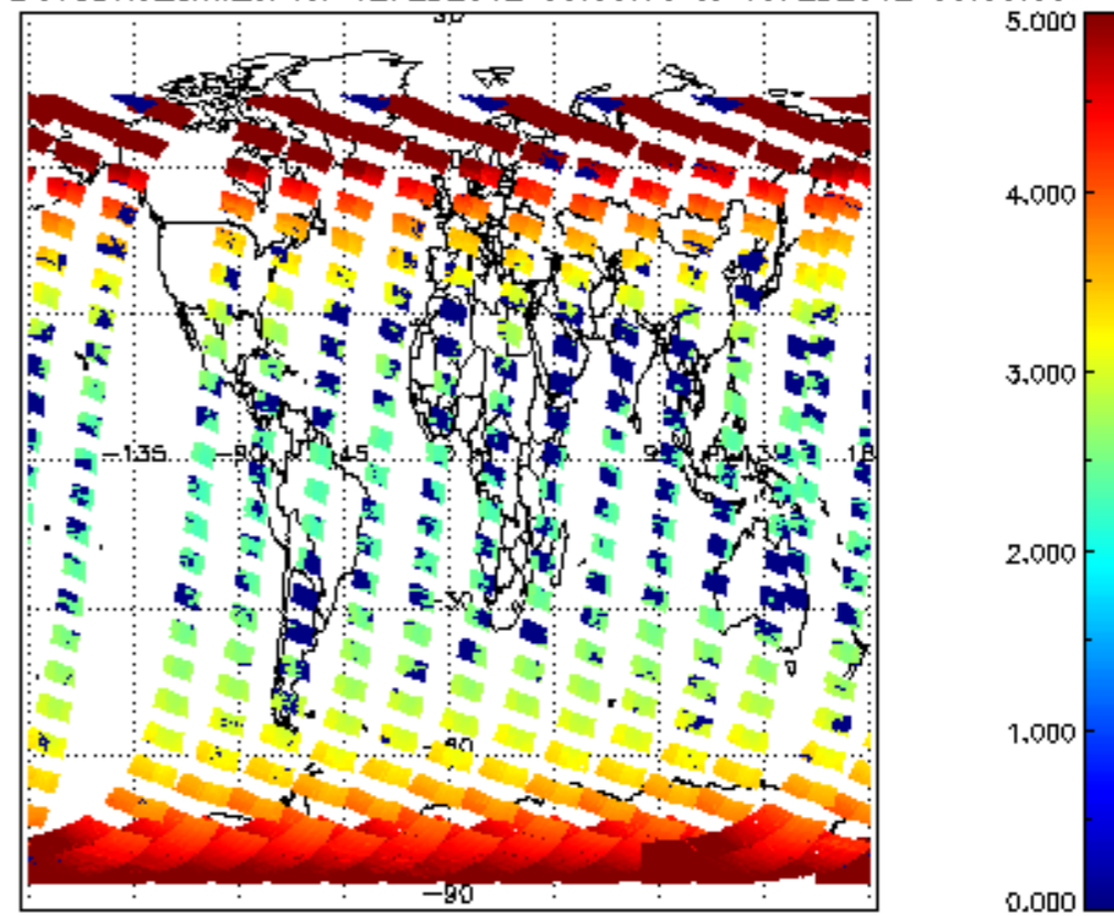
SCIOL2P_NADUV3BRO_amf_cl for 12FEB2012 00:00:00 to 13FEB2012 00:00:00
