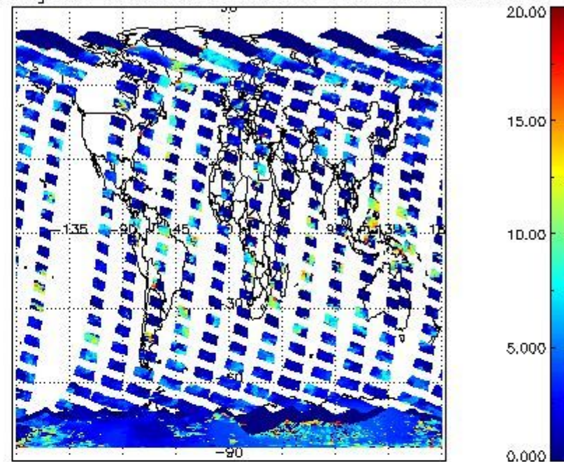
cL_top_height for 12FEB2012 00:00:00 to 13FEB2012 00:00:00
