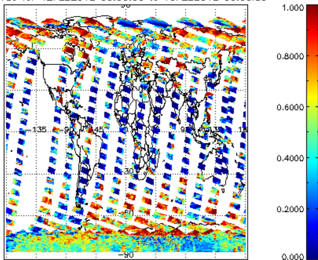
cl_frac for 12FEB2012 00:00:00 to 13FEB2012 00:00:00
