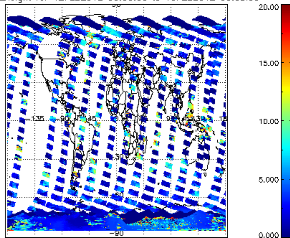
cl_top_height for 12FEB2012 00:00:00 to 13FEB2012 00:00:00
