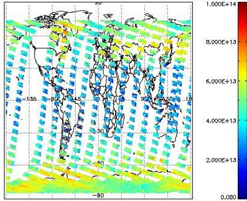
SCIOL2P_NADUV3BRO_vcd for 12FEB2012 00:00:00 to 13FEB2012 00:00:00
