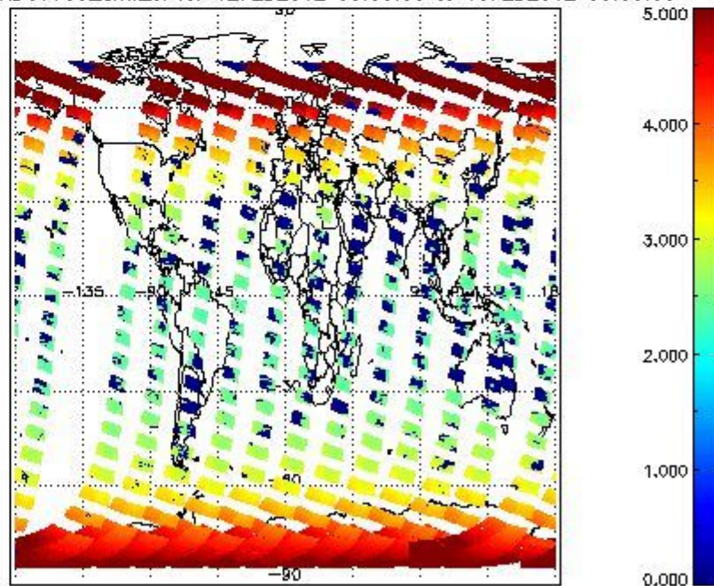
SCIOL2P_NADUV003_amf_cl for 12FEB2012 00:00:00 to 13FEB2012 00:00:00
