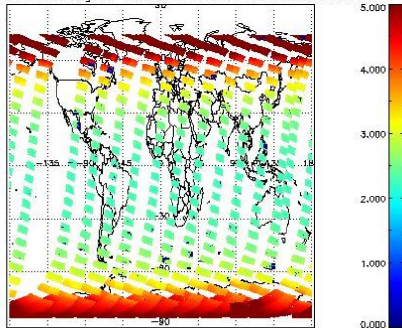
SCIOL2P_NADUV003_amf_gr for 12FEB2012 00:00:00 to 13FEB2012 00:00:00
