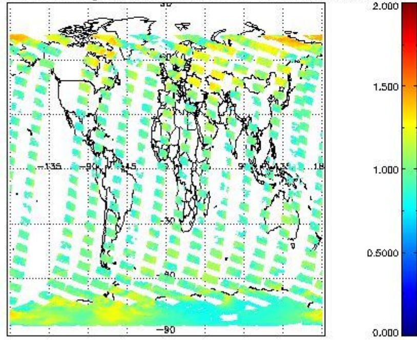
SCIOL2P_NADUV8H2O_amf_gr for 12FEB2012 00:00:00 to 13FEB2012 00:00:00
