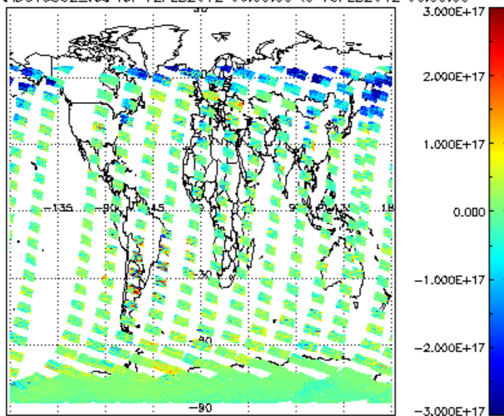
SCIOL2P_NADUV5S02_vcd for 12FEB2012 00:00:00 to 13FEB2012 00:00:00
