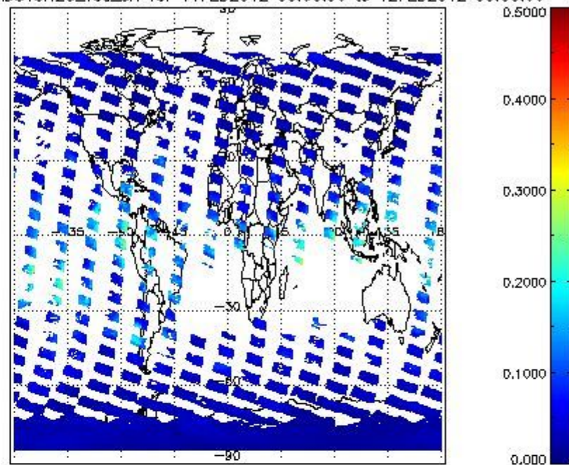
SCIOL2P_NADUV8H2O_vcd_err for 11FEB2012 00:00:00 to 12FEB2012 00:00:00
