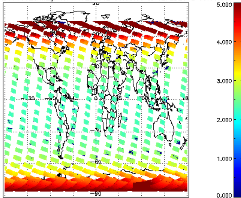
SCIOL2P_NADUV003_amf_gr for 11FEB2012 00:00:00 to 12FEB2012 00:00:00
