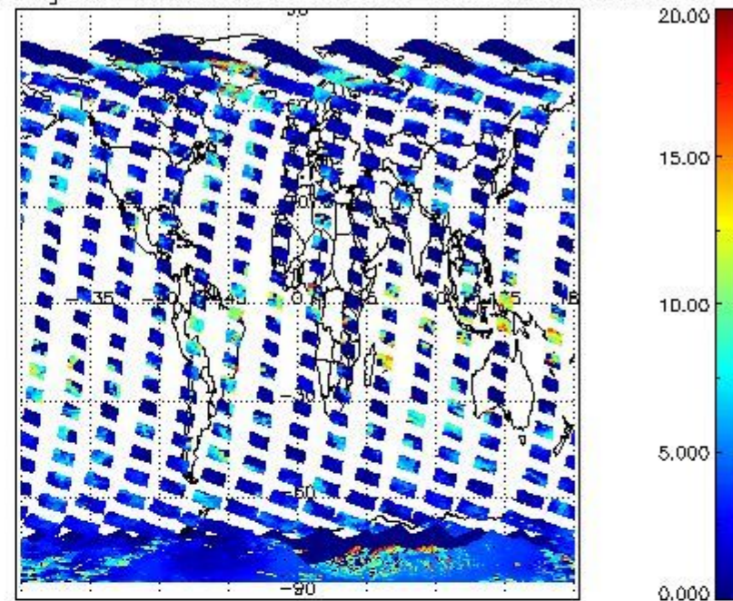
cL_top_height for 11FEB2012 00:00:00 to 12FEB2012 00:00:00
