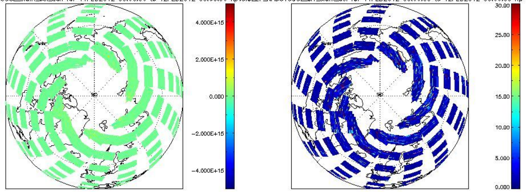
CIOL2P_NADUV6OCL_slant_col_den for 11FEB2012 00:00:00 to 12FEB2012 00:00:00 np; CIOL2P_NADUV6OCL_err_slant_col for 11FEB2012 00:00:00 to 12FEB2012 00:00:00 np
