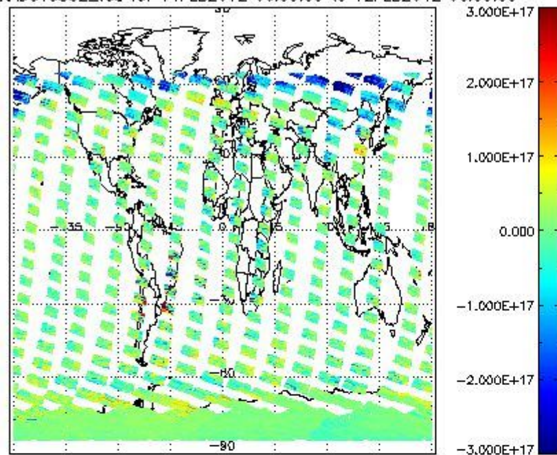
SCIOL2P_NADUV5SO2_vcd for 11FEB2012 00:00:00 to 12FEB2012 00:00:00
