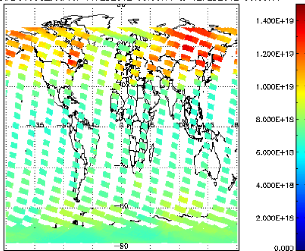
SCIOL2P_NADUV003_vcd for 11FEB2012 00:00:00 to 12FEB2012 00:00:00
