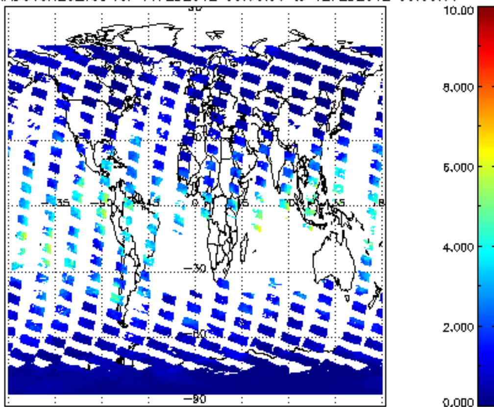
SCIOL2P_NADUV8H2O_vcd for 11FEB2012 00:00:00 to 12FEB2012 00:00:00
