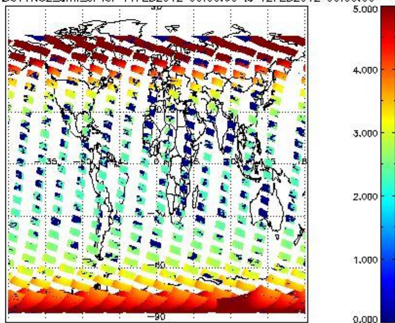
SCIOL2P_NADUV1N02_amf_cl for 11FEB2012 00:00:00 to 12FEB2012 00:00:00
