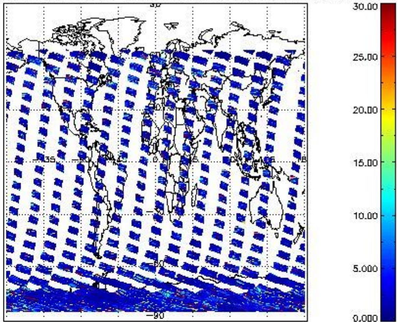
SCIOL2P_NADUV7S02_vcd_err for 11FEB2012 00:00:00 to 12FEB2012 00:00:00
