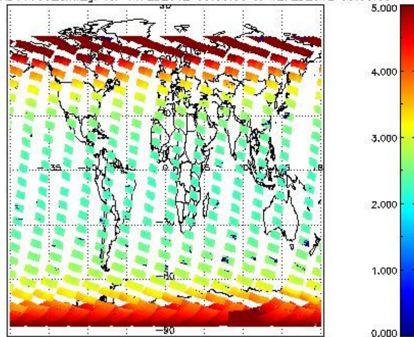
SCIOL2P_NADUV003_amf_gr for 11FEB2012 00:00:00 to 12FEB2012 00:00:00
