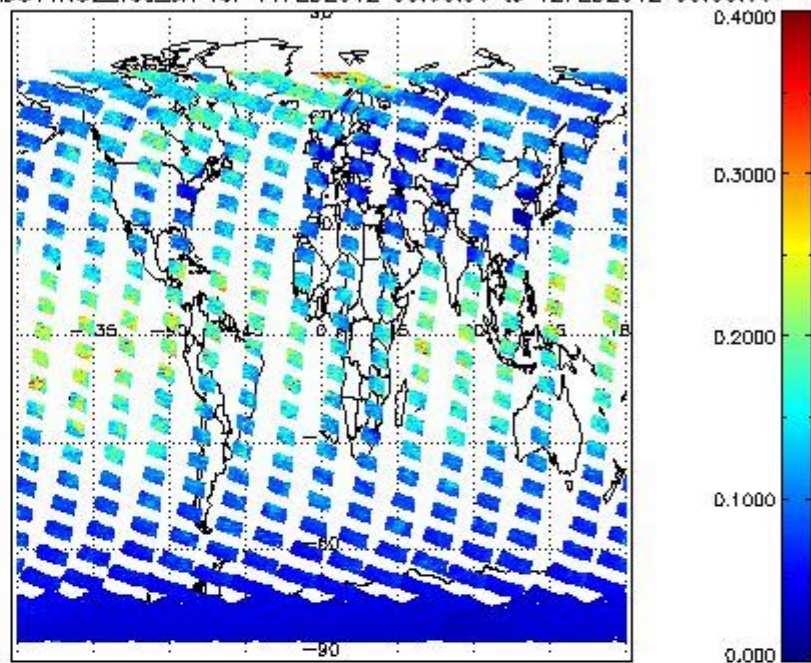
SCIOL2P_NADUV1N02_vcd_err for 11FEB2012 00:00:00 to 12FEB2012 00:00:00
