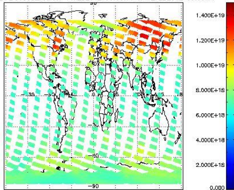
SCIOL2P_NADUV003_vcd for 11FEB2012 00:00:00 to 12FEB2012 00:00:00
