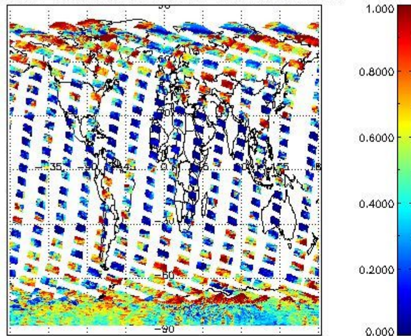
cL_frac for 11FEB2012 00:00:00 to 12FEB2012 00:00:00
