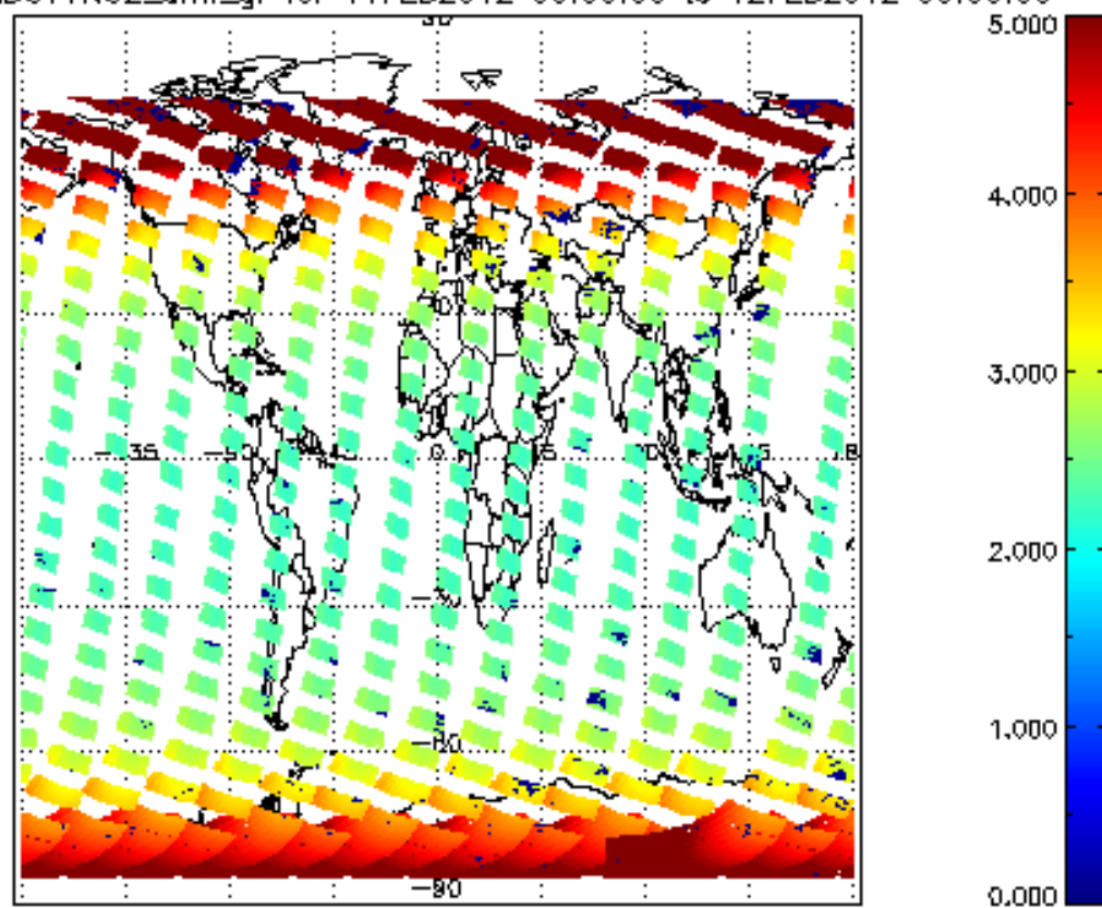
SCIOL2P_NADUV1N02_amf_gr for 11FEB2012 00:00:00 to 12FEB2012 00:00:00
