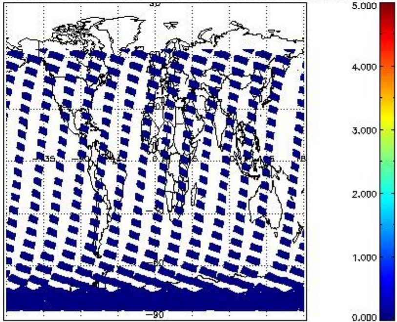
SCIOL2P_NADUV7S02_amf_cl for 11FEB2012 00:00:00 to 12FEB2012 00:00:00
