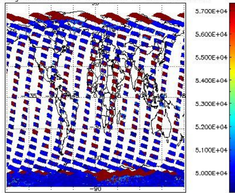
cloud_flags for 11FEB2012 00:00:00 to 12FEB2012 00:00:00
