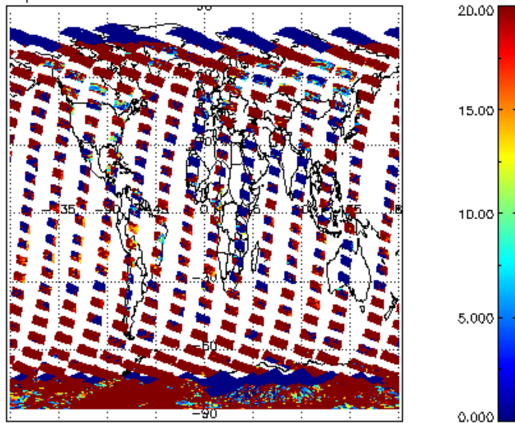
cL_opt_depth for 11FEB2012 00:00:00 to 12FEB2012 00:00:00
