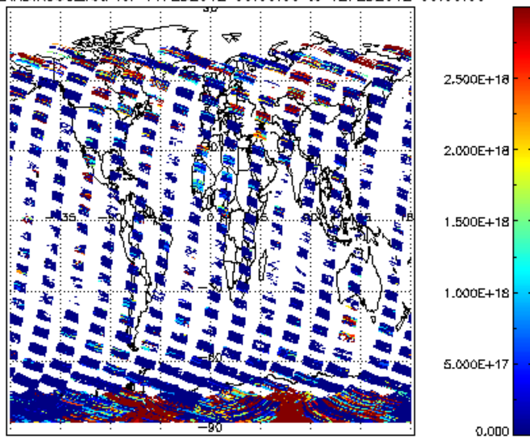
SCIOL2P_NADIR3CO_vcd for 11FEB2012 00:00:00 to 12FEB2012 00:00:00
