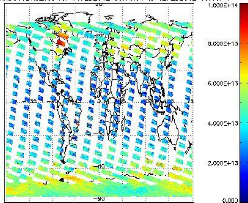
SCIOL2P_NADUV3BRO_vcd for 11FEB2012 00:00:00 to 12FEB2012 00:00:00
