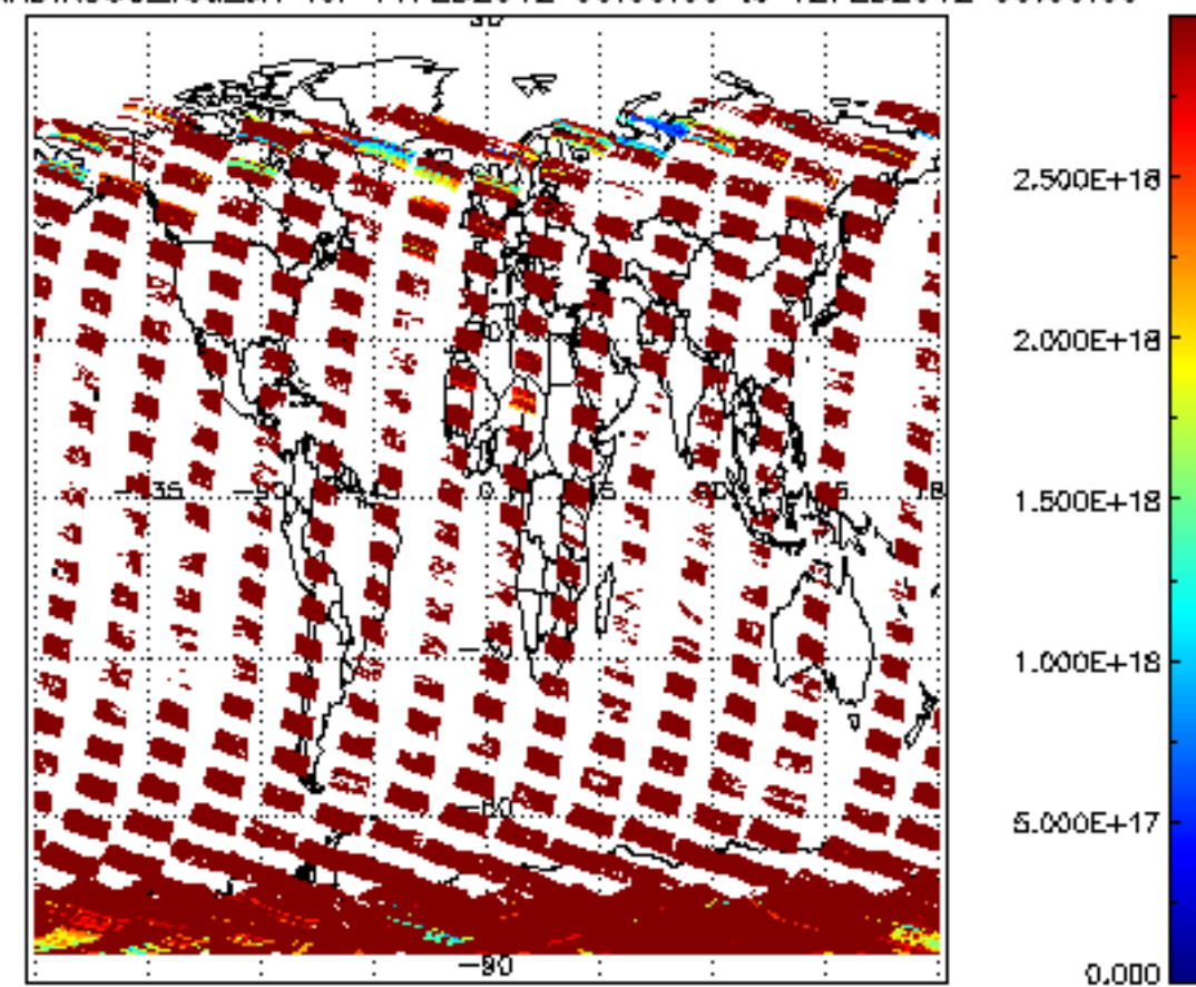
SCIOL2P_NADIR3CO_vcd_err for 11FEB2012 00:00:00 to 12FEB2012 00:00:00
