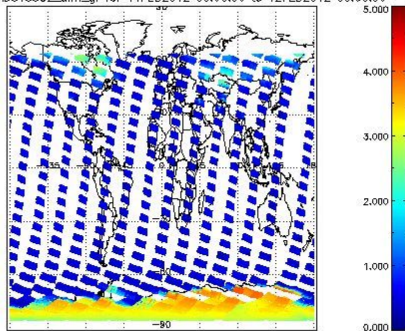
SCIOL2P_NADUV5SO2_amf_gr for 11FEB2012 00:00:00 to 12FEB2012 00:00:00
