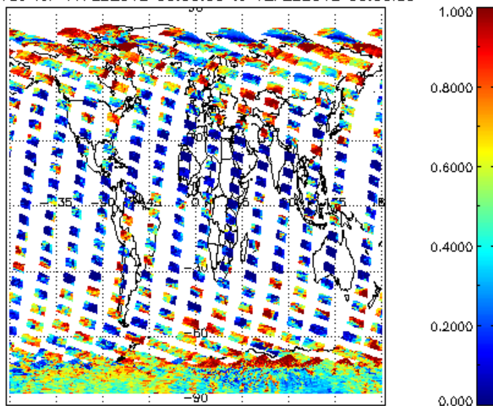
cL_frac for 11FEB2012 00:00:00 to 12FEB2012 00:00:00
