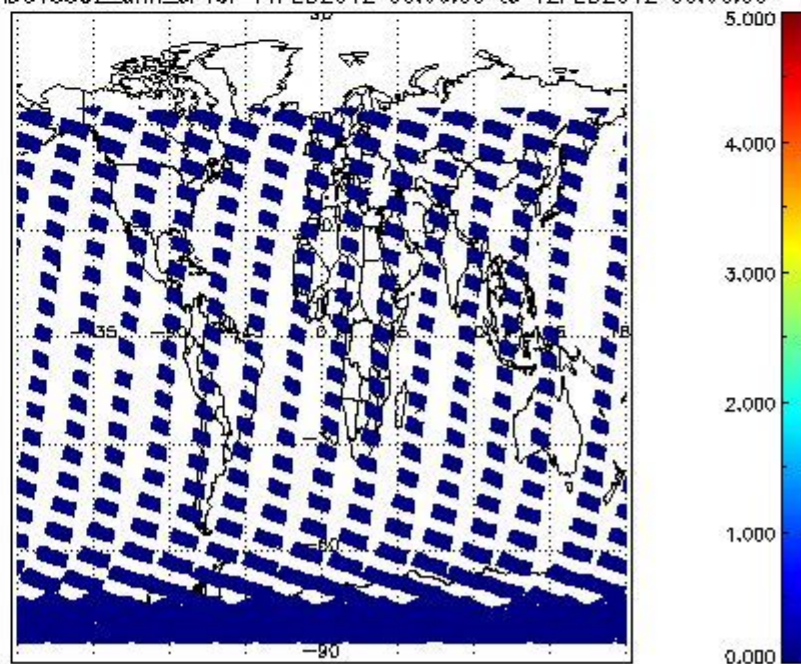
SCIOL2P_NADUV5SO2_amf_cl for 11FEB2012 00:00:00 to 12FEB2012 00:00:00
