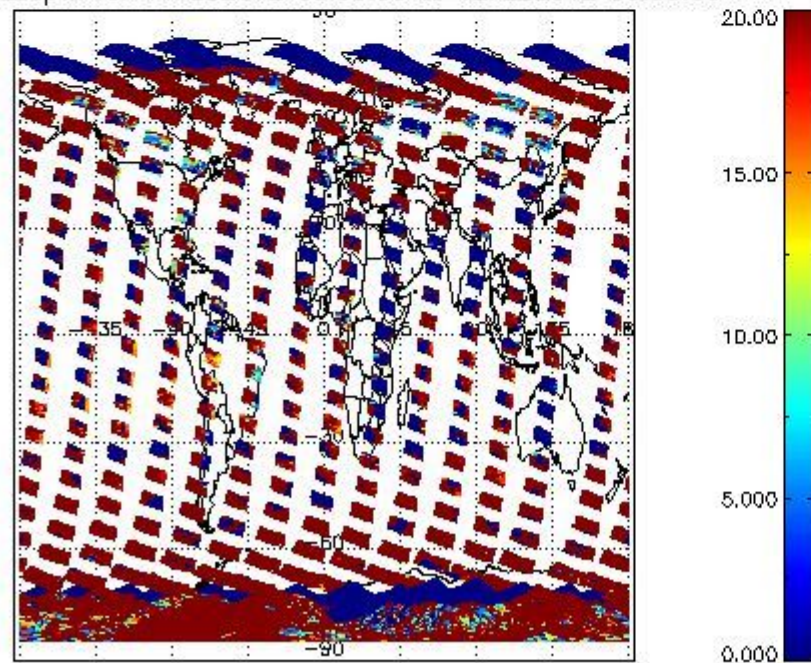
cL_opt_depth for 11FEB2012 00:00:00 to 12FEB2012 00:00:00
