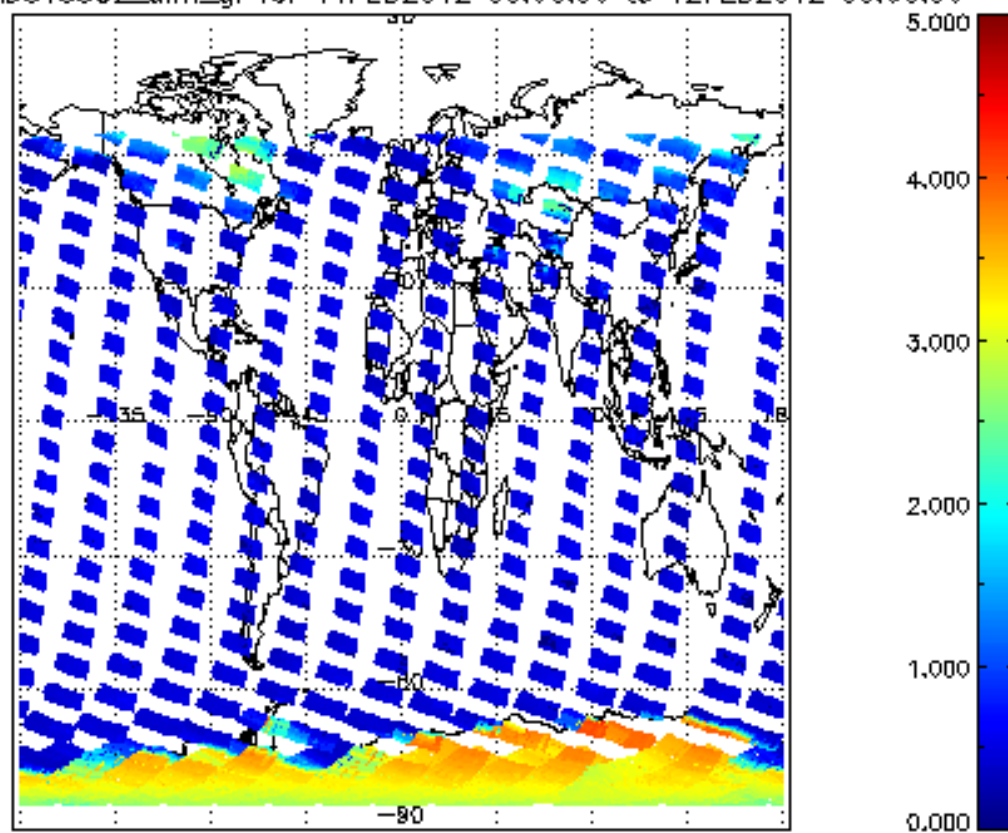
SCIOL2P_NADUV5S02_amf_gr for 11FEB2012 00:00:00 to 12FEB2012 00:00:00
