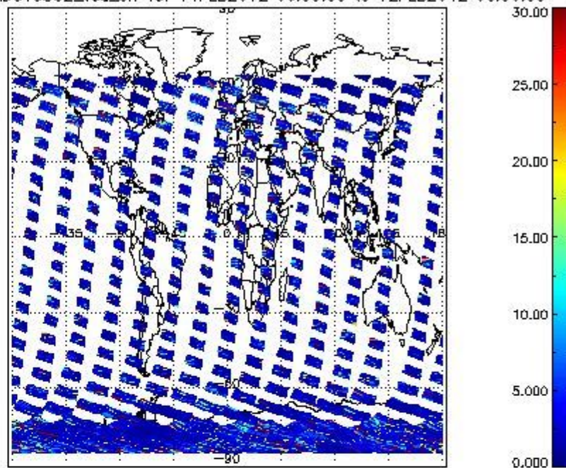
SCIOL2P_NADUV5SO2_vcd_err for 11FEB2012 00:00:00 to 12FEB2012 00:00:00
