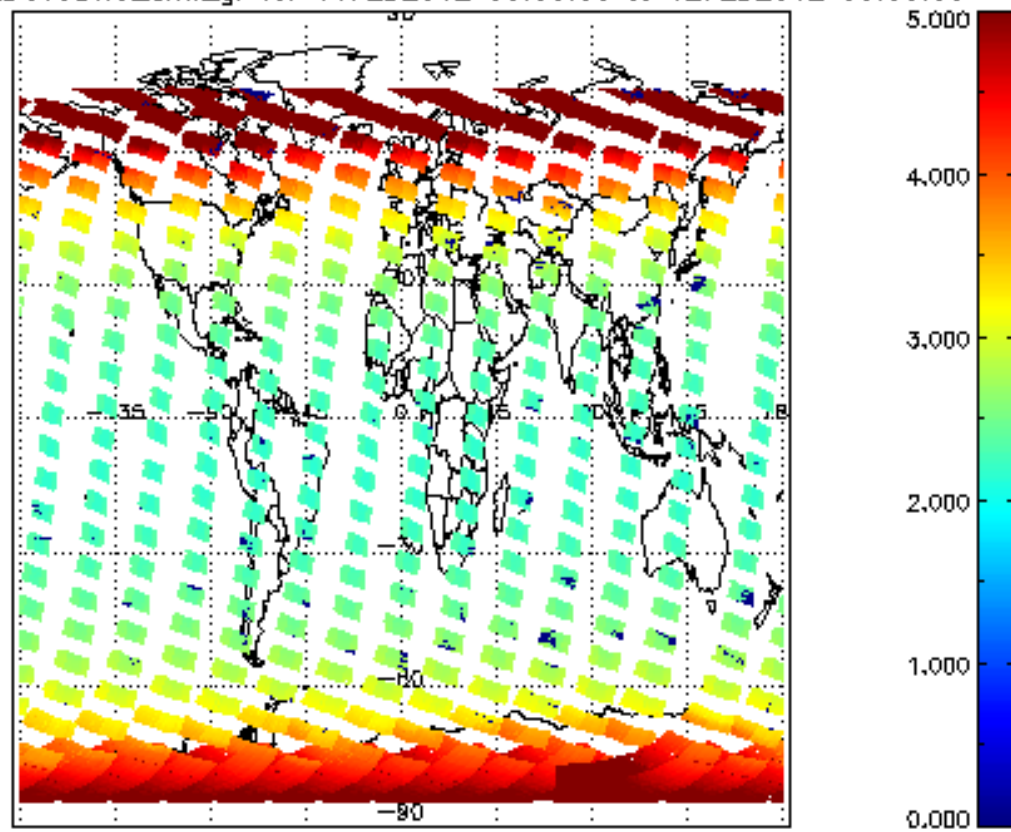
SCIOL2P_NADUV3BRO_amf_gr for 11FEB2012 00:00:00 to 12FEB2012 00:00:00
