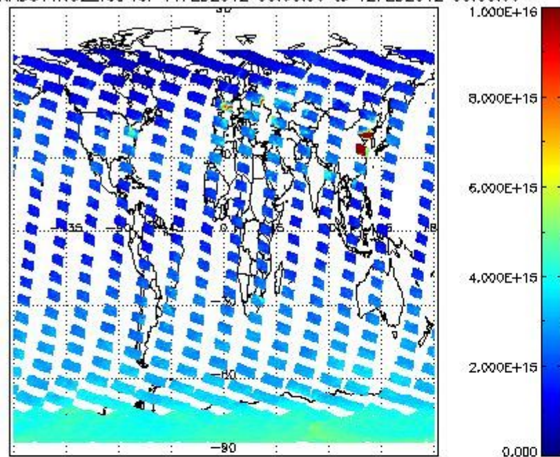
SCIOL2P_NADUV1N02_vcd for 11FEB2012 00:00:00 to 12FEB2012 00:00:00
