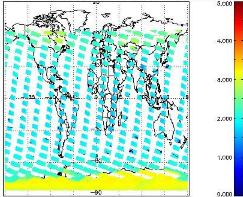
SCIOL2P_NADUV7S02_amf_gr for 11FEB2012 00:00:00 to 12FEB2012 00:00:00
