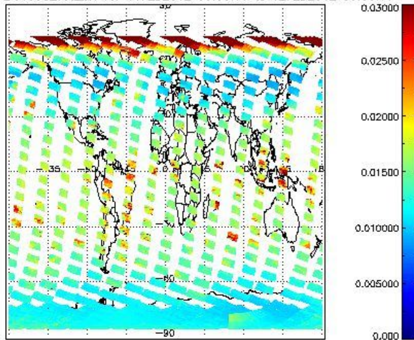
SCIOL2P_NADUV003_vcd_err for 11FEB2012 00:00:00 to 12FEB2012 00:00:00
