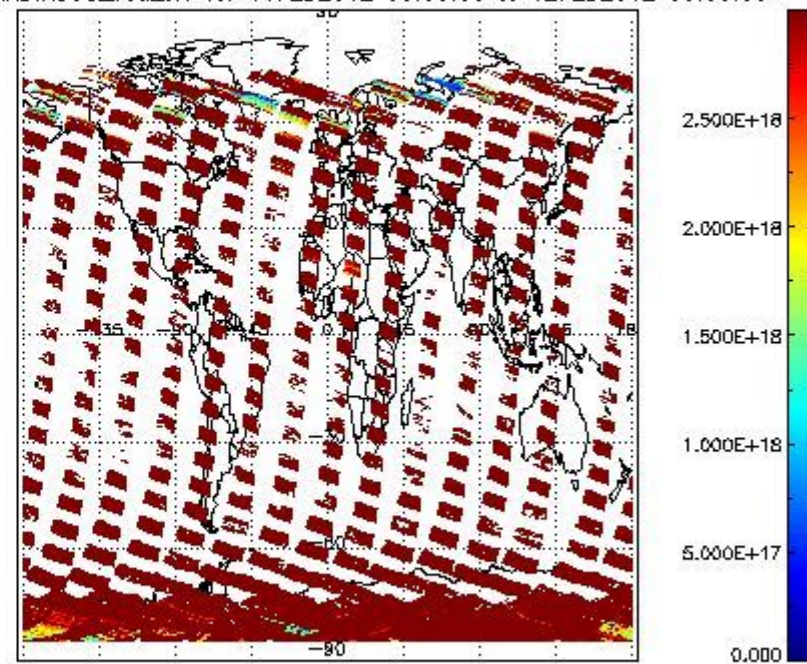
SCIDL2P_NADIR3CO_vcd_err for 11FEB2012 00:00:00 to 12FEB2012 00:00:00
