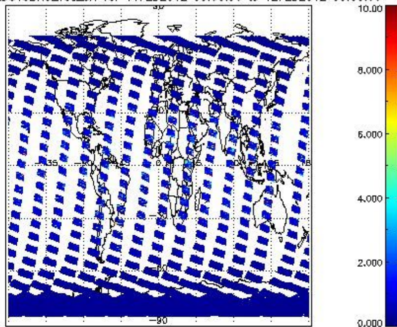
SCIOL2P_NADUV3BRO_vcd_err for 11FEB2012 00:00:00 to 12FEB2012 00:00:00
