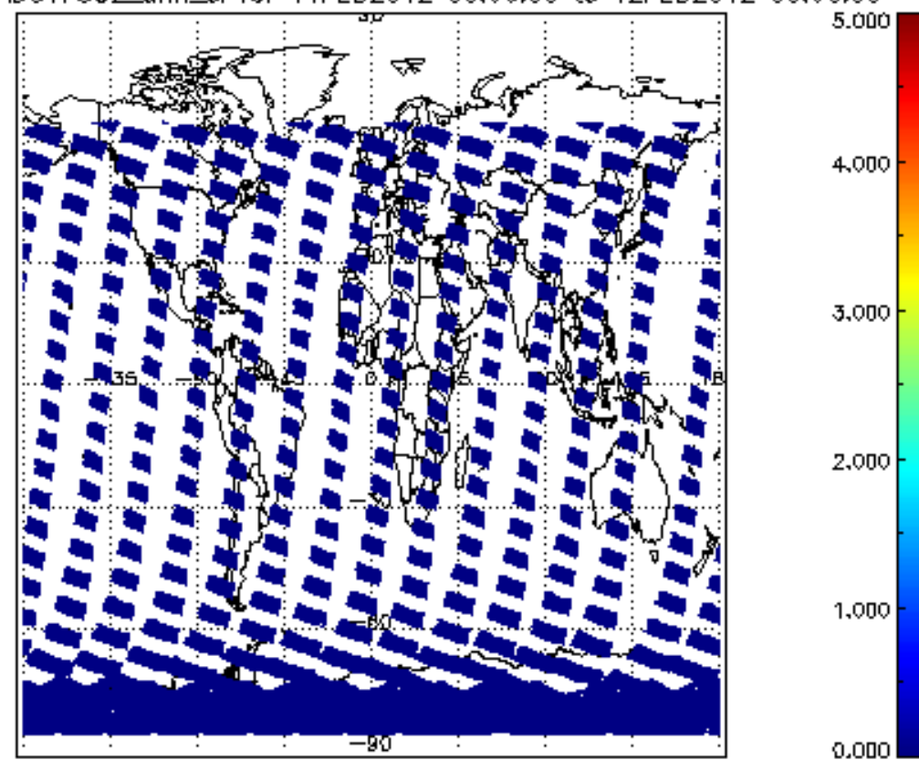
SCIOL2P_NADUV7S02_amf_cl for 11FEB2012 00:00:00 to 12FEB2012 00:00:00
