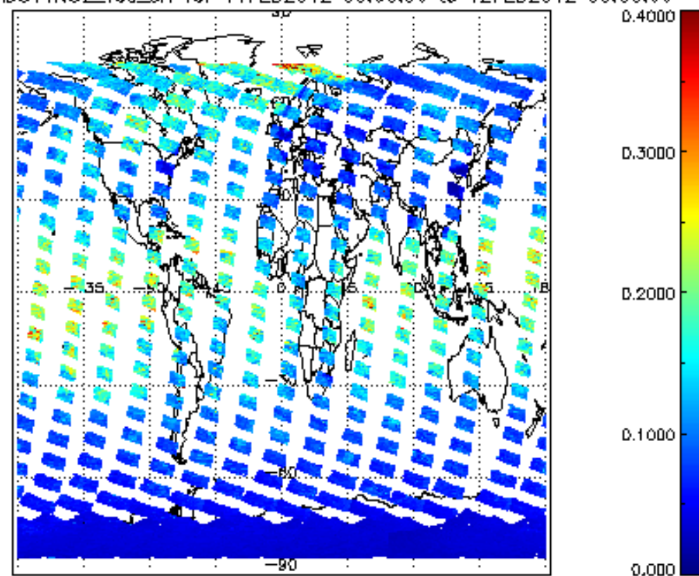
SCIOL2P_NADUV1N02_vcd_err for 11FEB2012 00:00:00 to 12FEB2012 00:00:00
