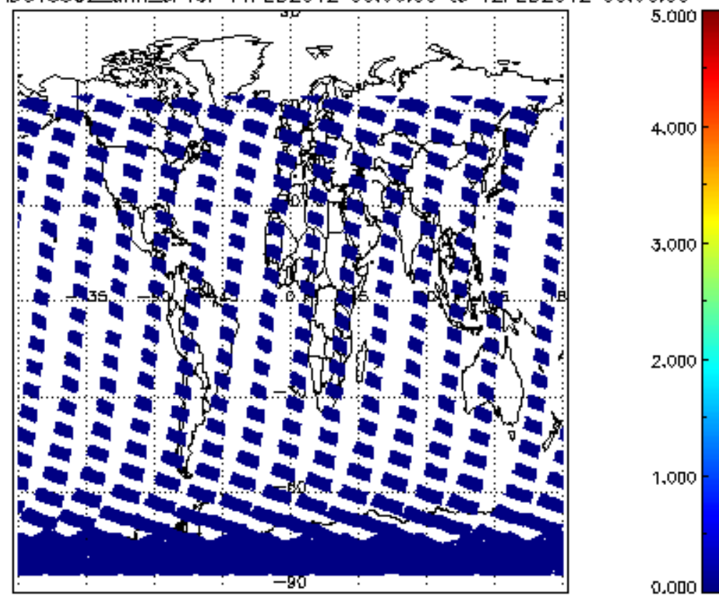
SCIOL2P_NADUV5S02_amf_cl for 11FEB2012 00:00:00 to 12FEB2012 00:00:00
