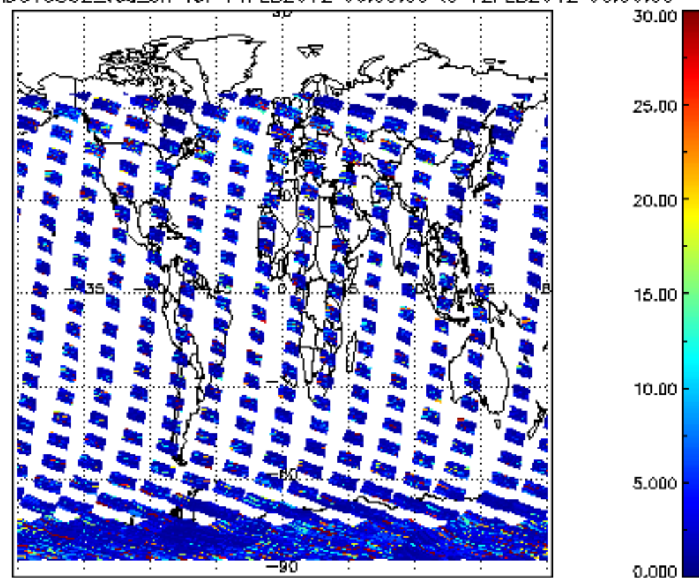
SCIOL2P_NADUV5S02_vcd_err for 11FEB2012 00:00:00 to 12FEB2012 00:00:00
