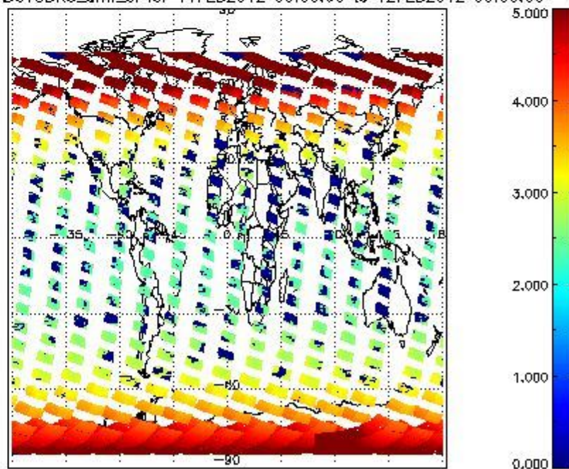
SCIOL2P_NADUV3BRO_amf_cl for 11FEB2012 00:00:00 to 12FEB2012 00:00:00
