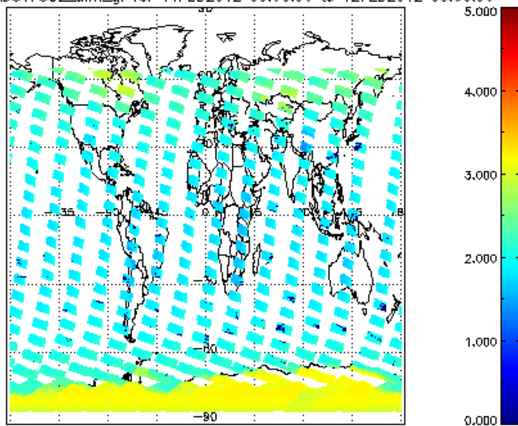
SCIOL2P_NADUV7S02_amf_gr for 11FEB2012 00:00:00 to 12FEB2012 00:00:00
