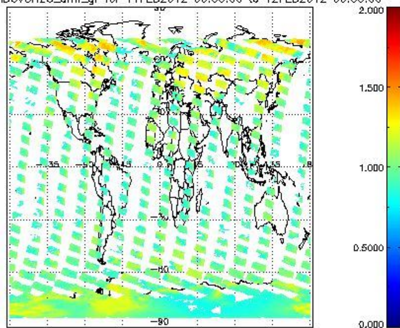
SCIOL2P_NADUV8H2O_amf_gr for 11FEB2012 00:00:00 to 12FEB2012 00:00:00
