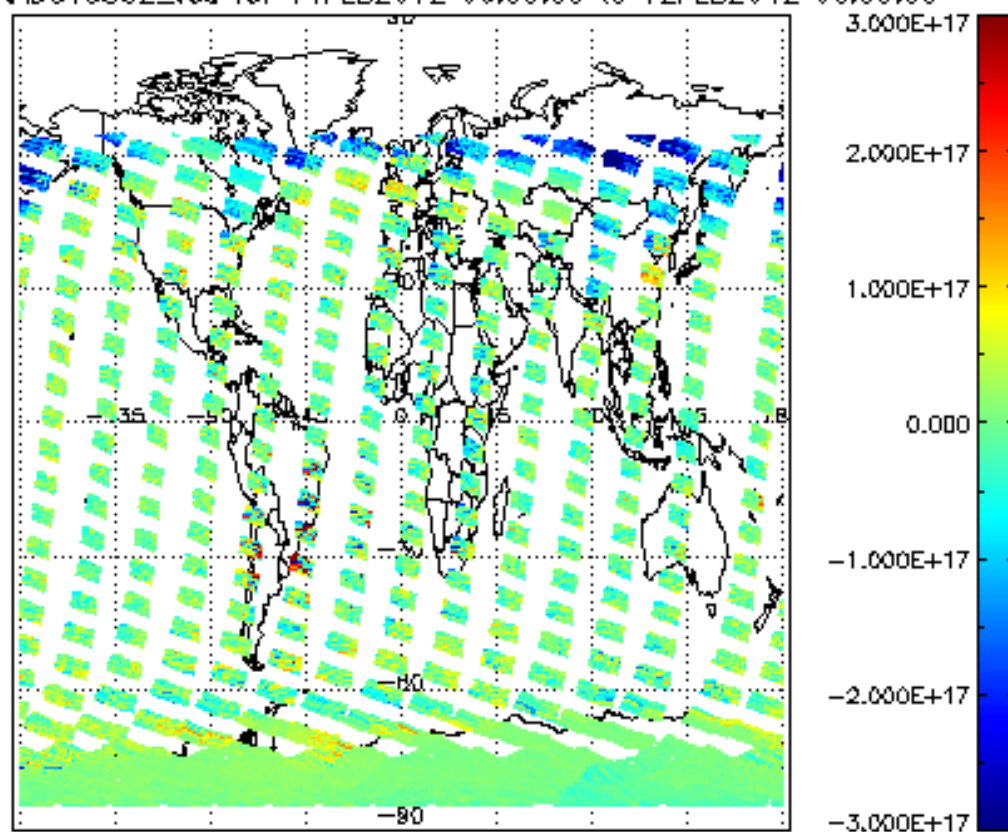
SCIOL2P_NADUV5S02_vcd for 11FEB2012 00:00:00 to 12FEB2012 00:00:00
