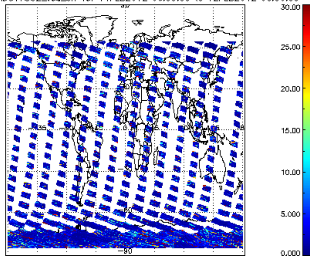
SCIOL2P_NADUV7S02_vcd_err for 11FEB2012 00:00:00 to 12FEB2012 00:00:00
