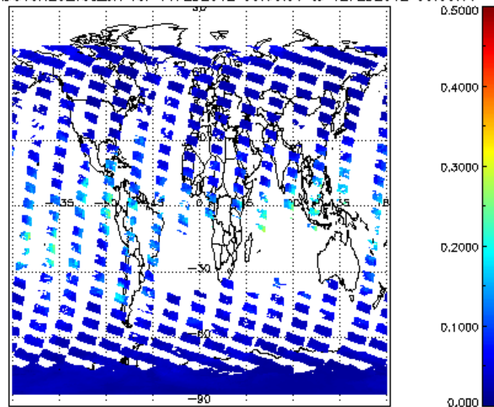
SCIOL2P_NADUV8H2O_vcd_err for 11FEB2012 00:00:00 to 12FEB2012 00:00:00
