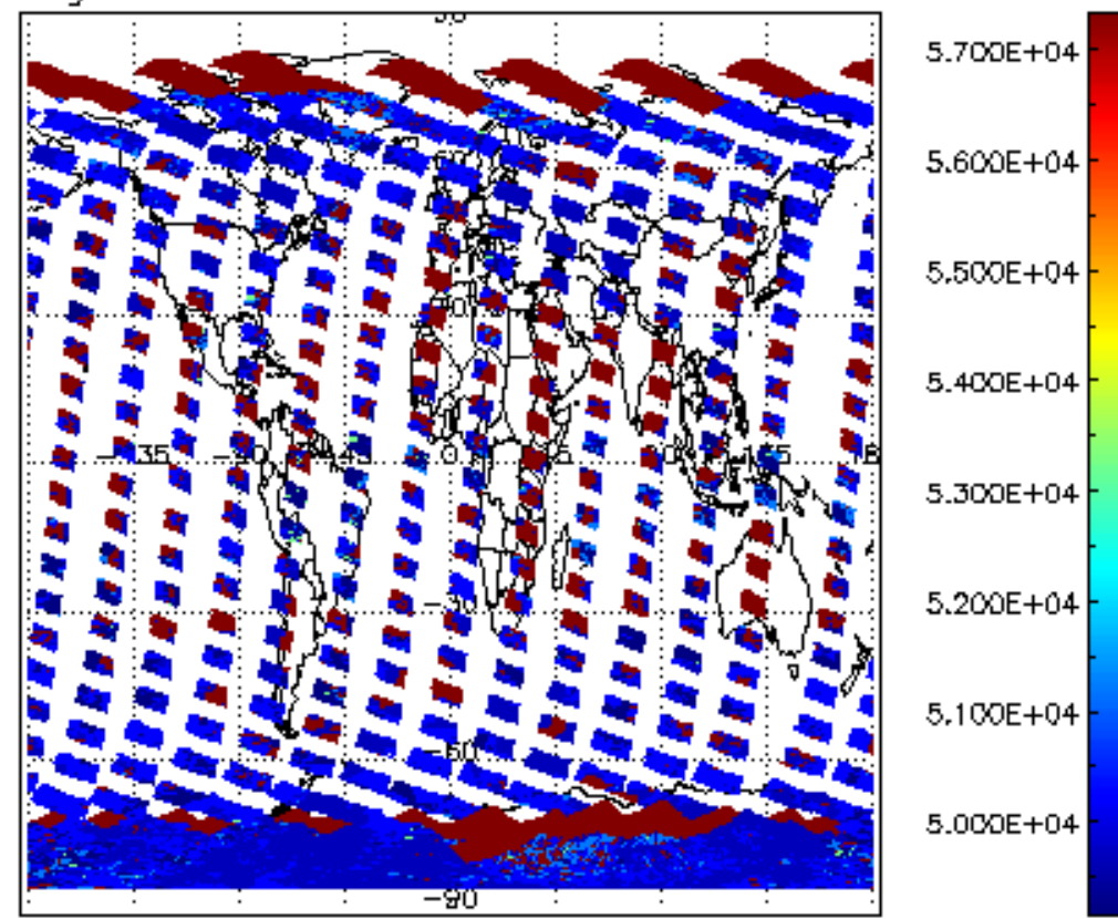
cloud_flags for 11FEB2012 00:00:00 to 12FEB2012 00:00:00
