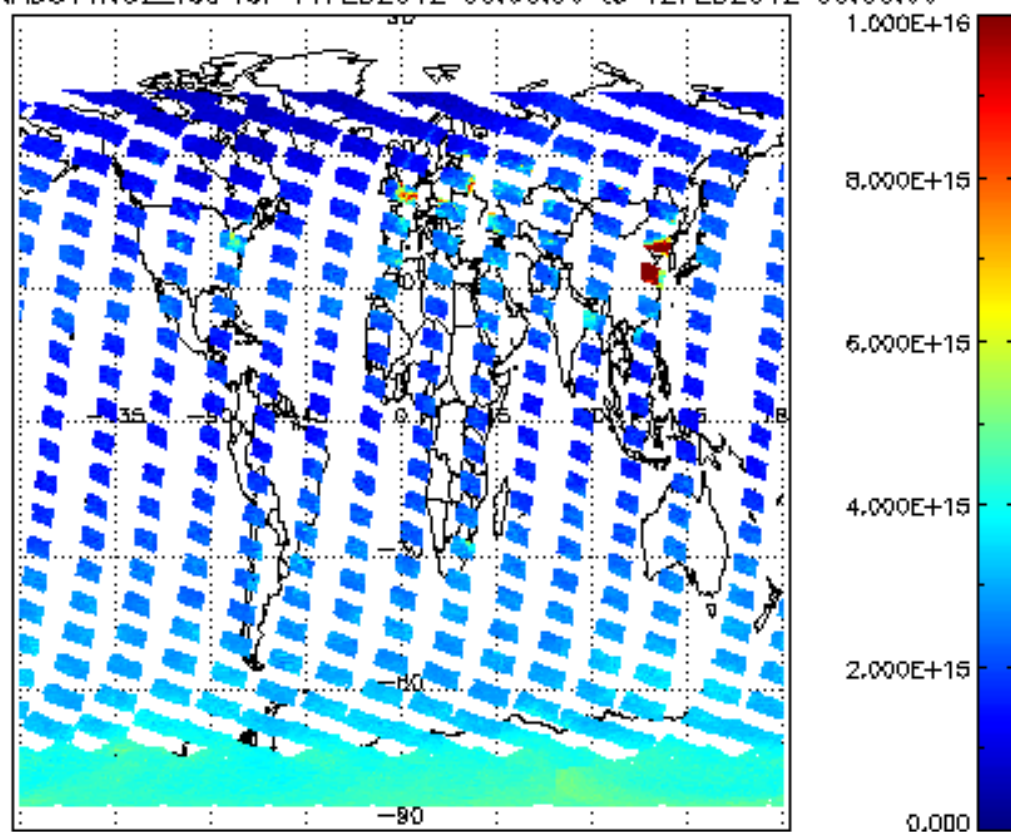
SCIOL2P_NADUV1N02_vcd for 11FEB2012 00:00:00 to 12FEB2012 00:00:00
