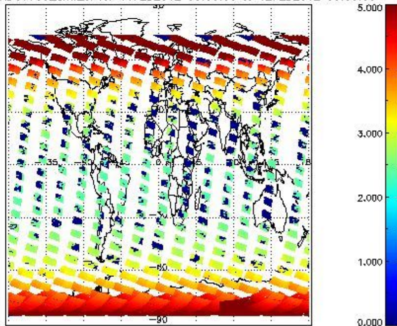
SCIOL2P_NADUV003_amf_cl for 11FEB2012 00:00:00 to 12FEB2012 00:00:00
