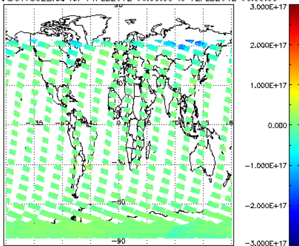
SCIOL2P_NADUV7S02_vcd for 11FEB2012 00:00:00 to 12FEB2012 00:00:00
