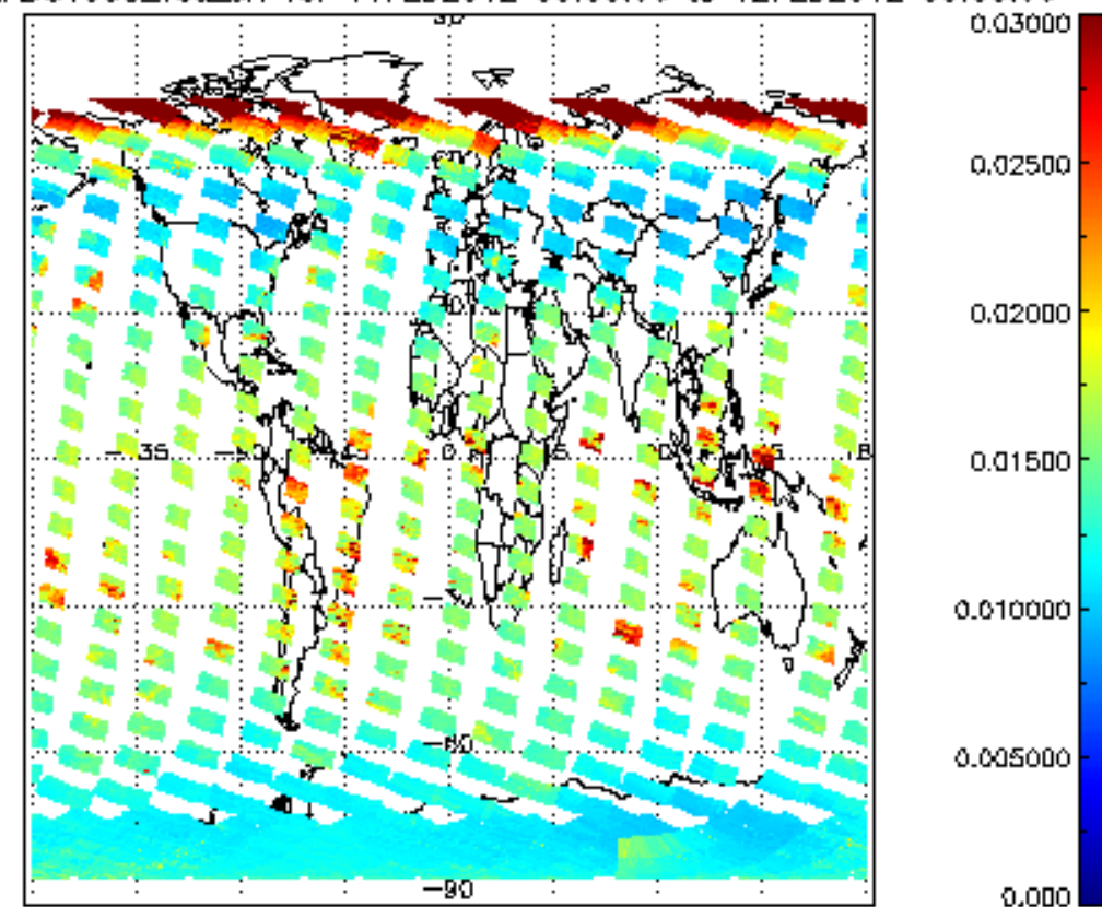
SCIOL2P_NADUV003_vcd_err for 11FEB2012 00:00:00 to 12FEB2012 00:00:00
