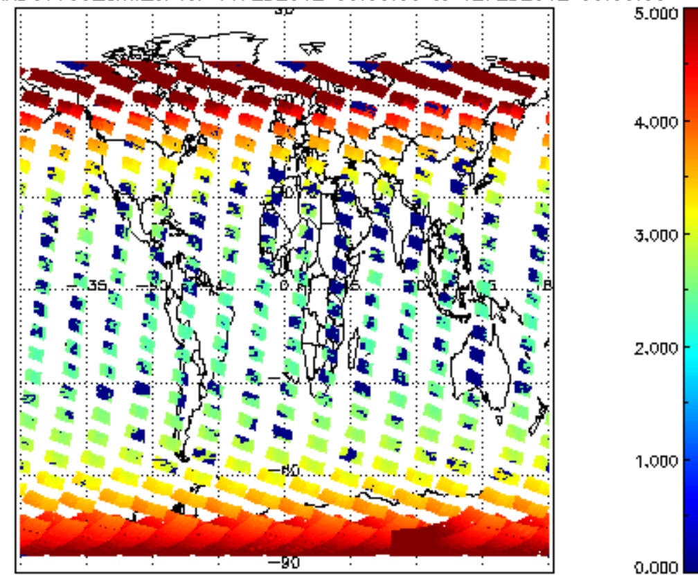
SCIOL2P_NADUV003_amf_cl for 11FEB2012 00:00:00 to 12FEB2012 00:00:00
