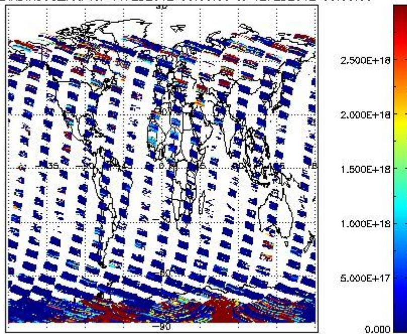
SCIDL2P_NADIR3CO_vcd for 11FEB2012 00:00:00 to 12FEB2012 00:00:00
