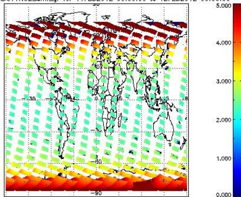
SCIOL2P_NADUV1N02_amf_gr for 11FEB2012 00:00:00 to 12FEB2012 00:00:00
