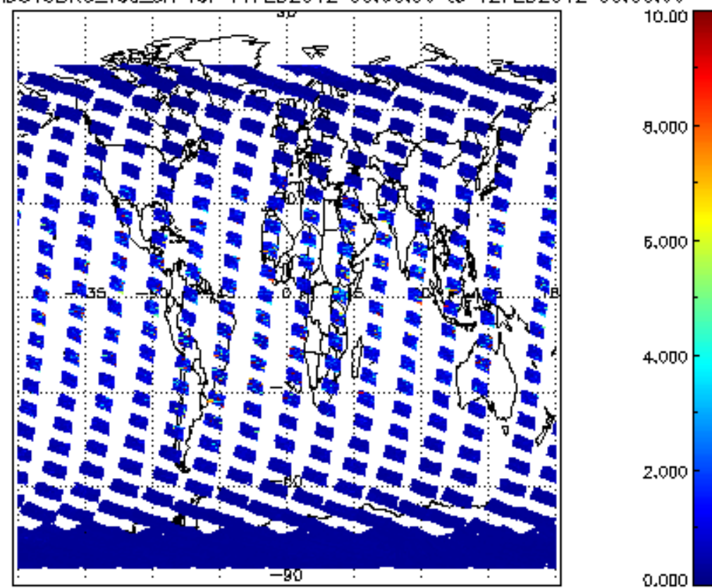
SCIOL2P_NADUV3BRO_vcd_err for 11FEB2012 00:00:00 to 12FEB2012 00:00:00
