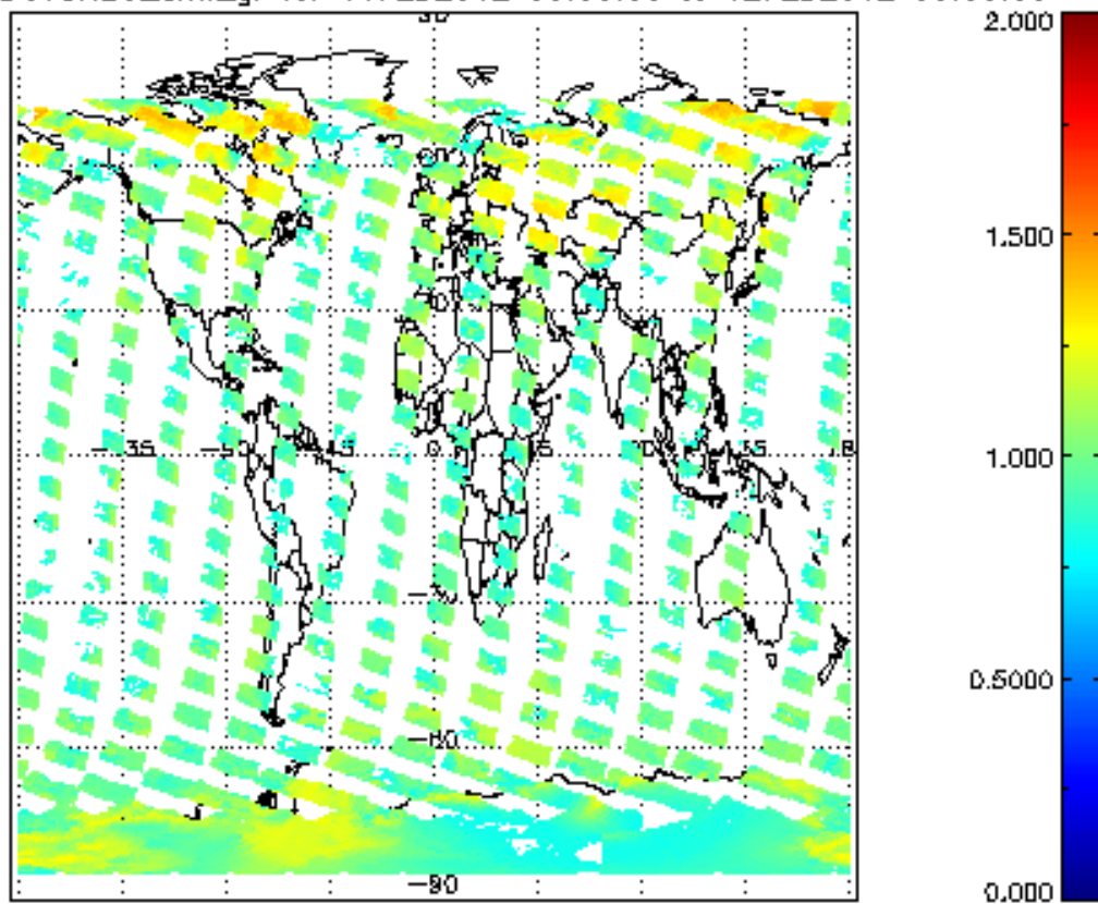
SCIOL2P_NADUV8H2O_amf_gr for 11FEB2012 00:00:00 to 12FEB2012 00:00:00
