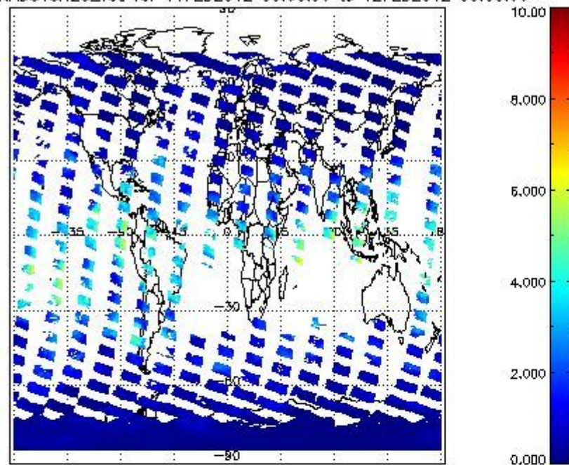
SCIOL2P_NADUV8H2O_vcd for 11FEB2012 00:00:00 to 12FEB2012 00:00:00
