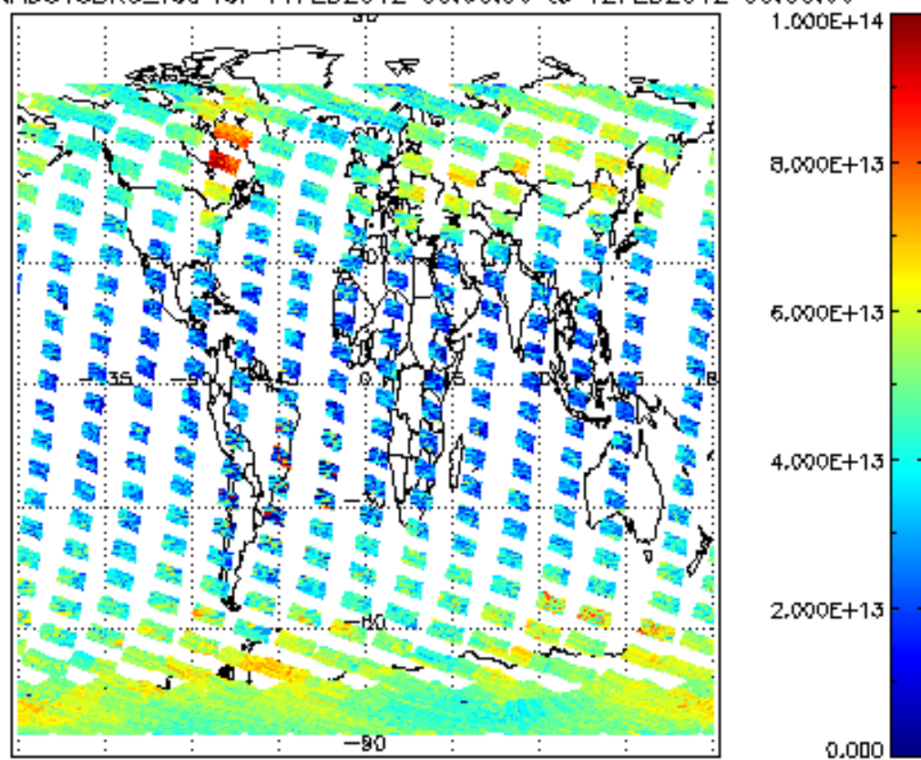
SCIOL2P_NADUV3BRO_vcd for 11FEB2012 00:00:00 to 12FEB2012 00:00:00
