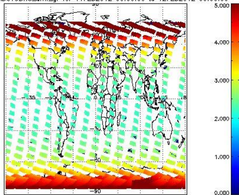
SCIOL2P_NADUV3BRO_amf_gr for 11FEB2012 00:00:00 to 12FEB2012 00:00:00
