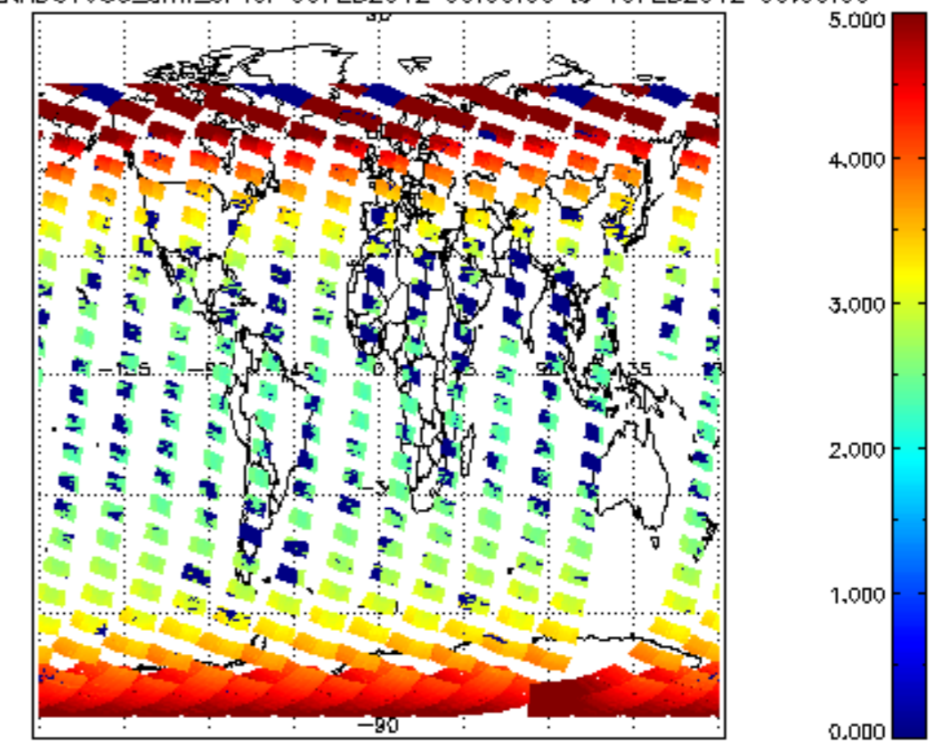
SCIOL2P_NADUV003_amf_cl for 09FEB2012 00:00:00 to 10FEB2012 00:00:00
