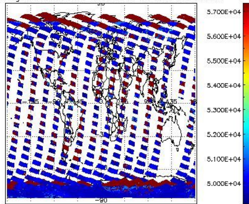
cloud_flags for 09FEB2012 00:00:00 to 10FEB2012 00:00:00
