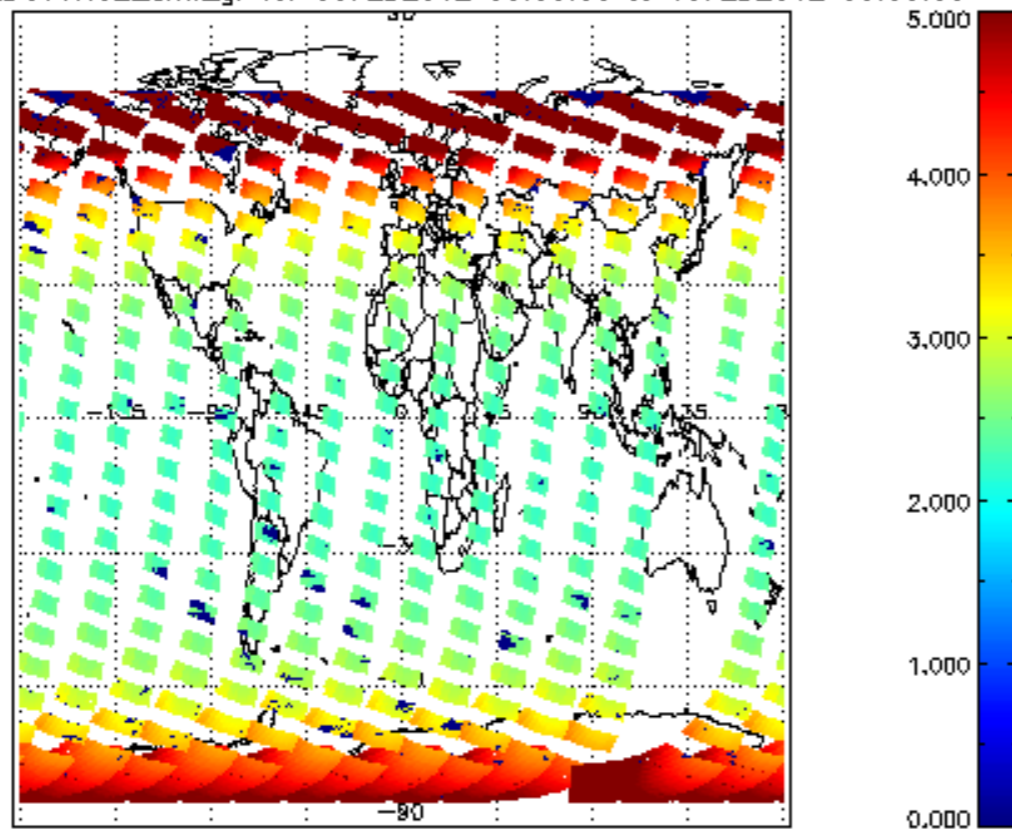
SCIOL2P_NADUV1N02_amf_gr for 09FEB2012 00:00:00 to 10FEB2012 00:00:00
