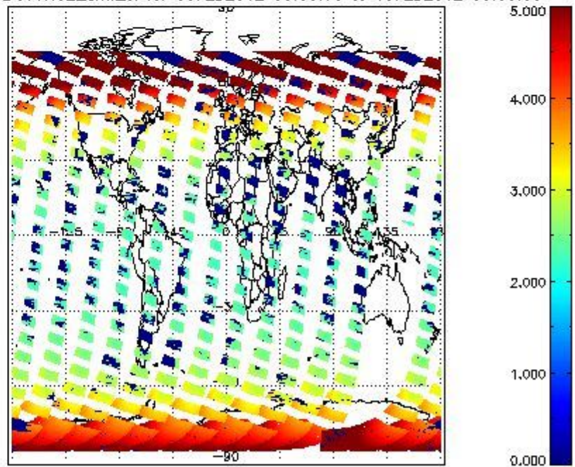
SCIOL2P_NADUV1N02_amf_cl for 09FEB2012 00:00:00 to 10FEB2012 00:00:00
