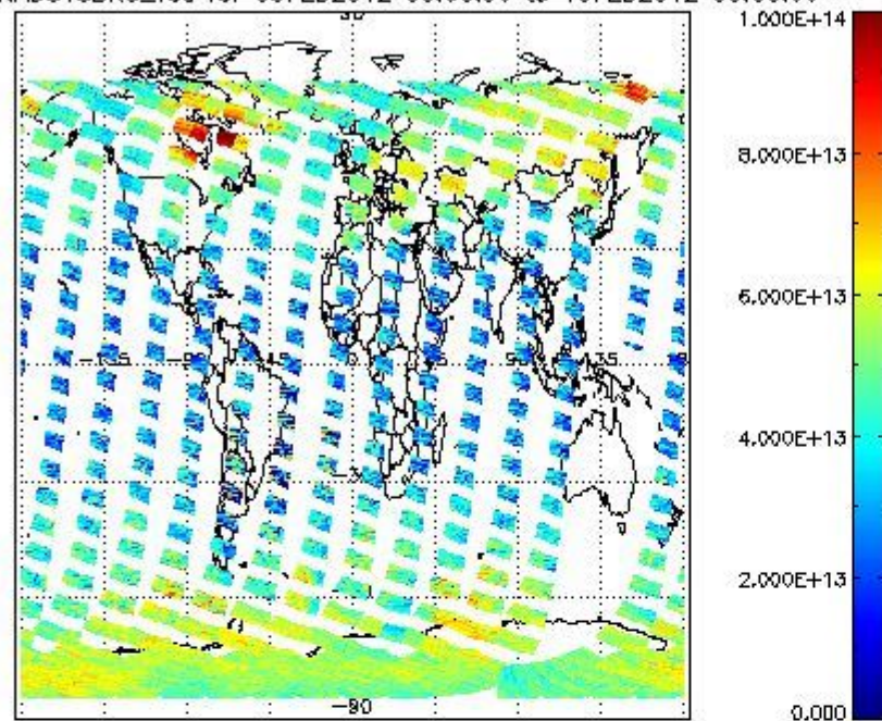
SCIOL2P_NADUV3BRO_vcd for 09FEB2012 00:00:00 to 10FEB2012 00:00:00
