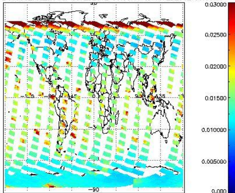
SCIOL2P_NADUV003_vcd_err for 09FEB2012 00:00:00 to 10FEB2012 00:00:00
