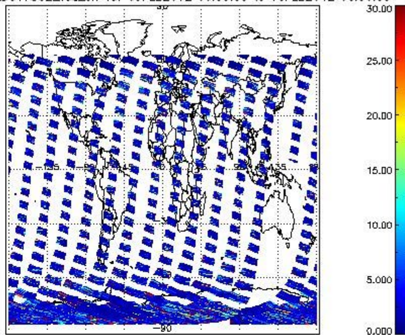
SCIOL2P_NADUV7S02_vcd_err for 09FEB2012 00:00:00 to 10FEB2012 00:00:00
