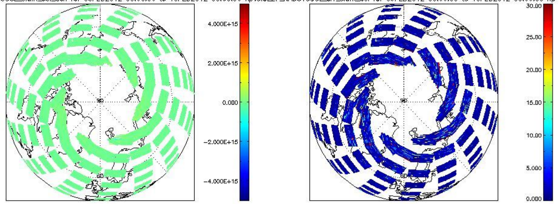
CIOL2P_NADUV6OCL_slant_col_den for 09FEB2012 00:00:00 to 10FEB2012 00:00:00 np; CIOL2P_NADUV6OCL_err_slant_col for 09FEB2012 00:00:00 to 10FEB2012 00:00:00 np
