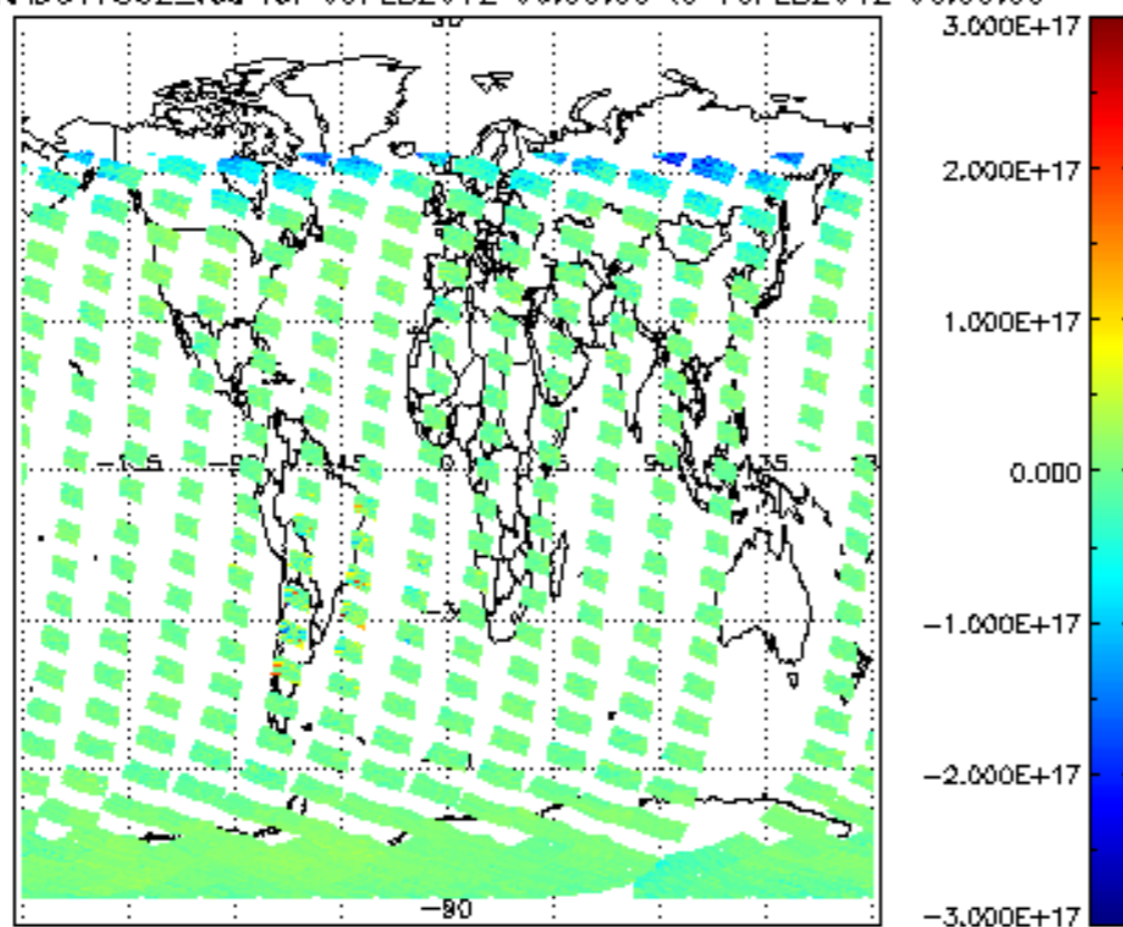
SCIOL2P_NADUV7S02_vcd for 09FEB2012 00:00:00 to 10FEB2012 00:00:00
