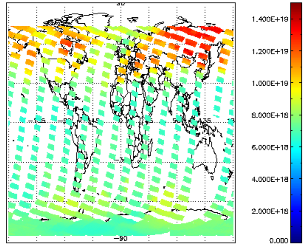
SCIOL2P_NADUV003_vcd for 09FEB2012 00:00:00 to 10FEB2012 00:00:00
