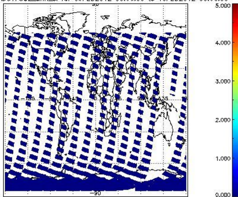
SCIOL2P_NADUV7S02_amf_cl for 09FEB2012 00:00:00 to 10FEB2012 00:00:00
