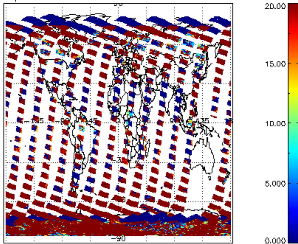
cI_opt_depth for 09FEB2012 00:00:00 to 10FEB2012 00:00:00
