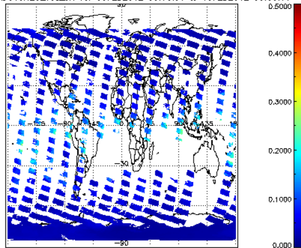
SCIOL2P_NADUV8H20_vcd_err for 09FEB2012 00:00:00 to 10FEB2012 00:00:00
