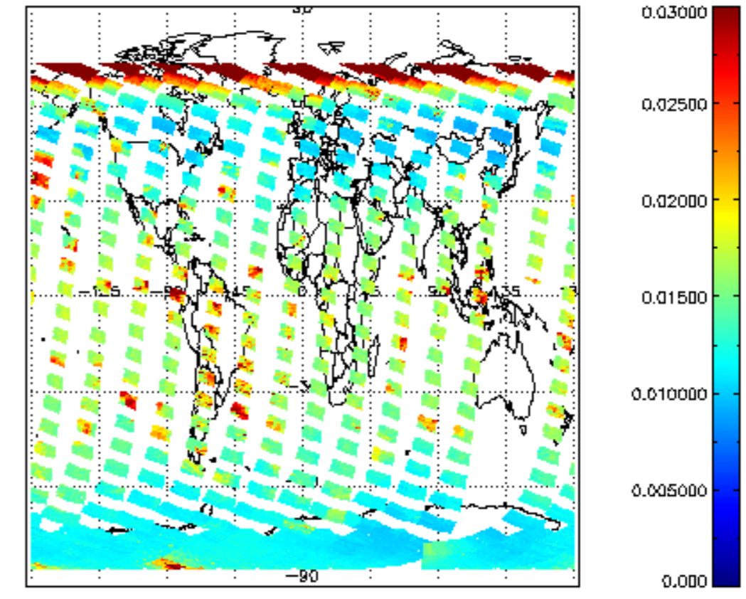
SCIOL2P_NADUV003_vcd_err for 09FEB2012 00:00:00 to 10FEB2012 00:00:00
