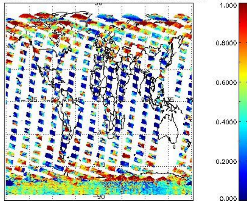
cL_frae for 09FEB2012 00:00:00 to 10FEB2012 00:00:00
