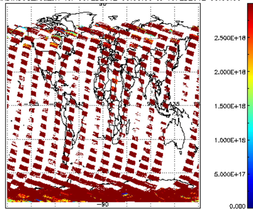
SCIOL2P_NADIR3CO_vcd_err for 09FEB2012 00:00:00 to 10FEB2012 00:00:00
