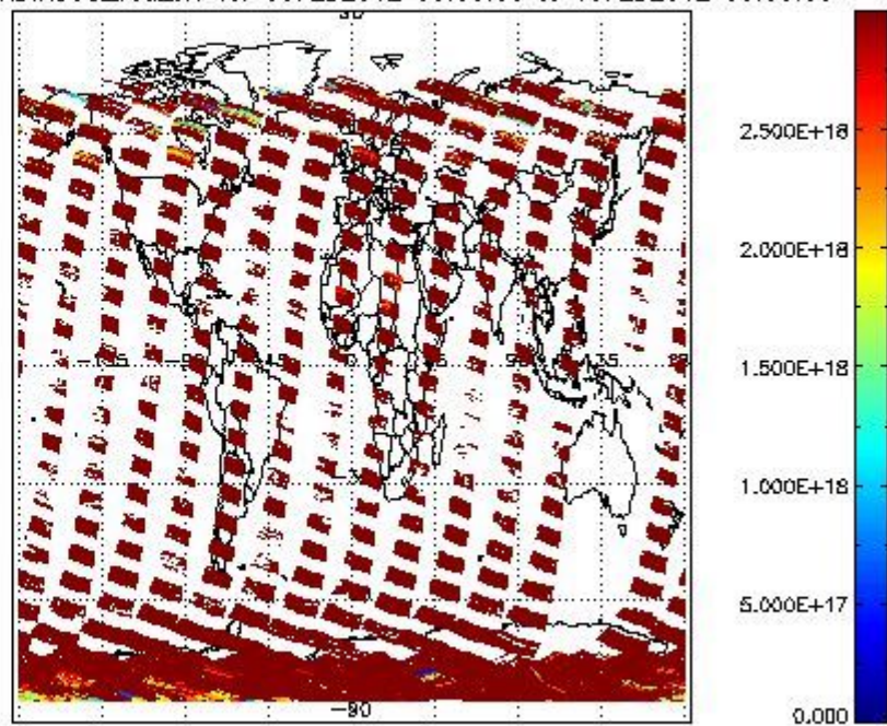
SCIDL2P_NADIR3CO_vcd_err for 09FEB2012 00:00:00 to 10FEB2012 00:00:00
