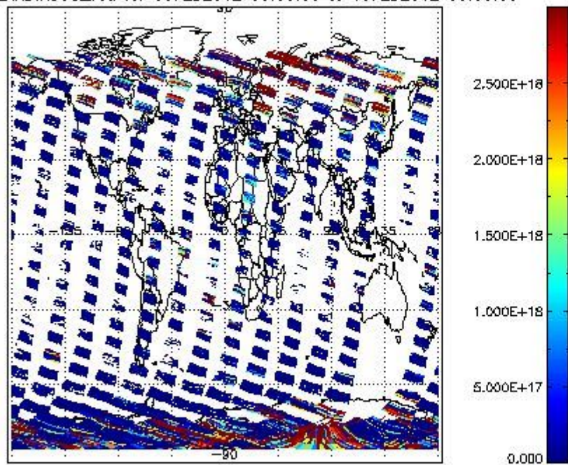
SCIDL2P_NADIR3CO_vcd for 09FEB2012 00:00:00 to 10FEB2012 00:00:00
