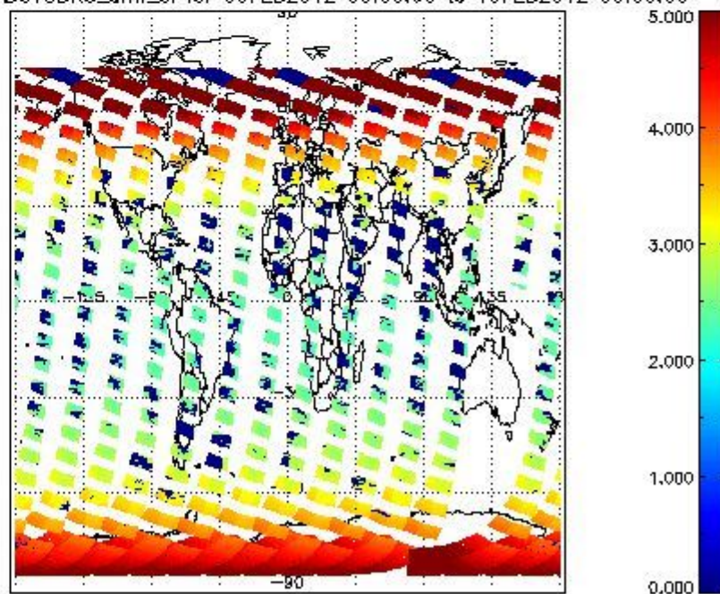
SCIOL2P_NADUV3BRO_amf_cl for 09FEB2012 00:00:00 to 10FEB2012 00:00:00
