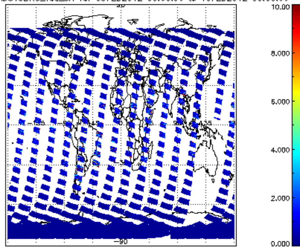
SCIOL2P_NADUV3BRO_vcd_err for 09FEB2012 00:00:00 to 10FEB2012 00:00:00
