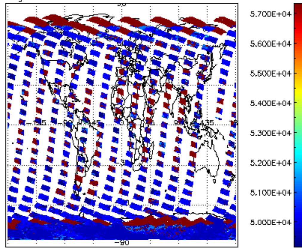
cloud_flags for 09FEB2012 00:00:00 to 10FEB2012 00:00:00
