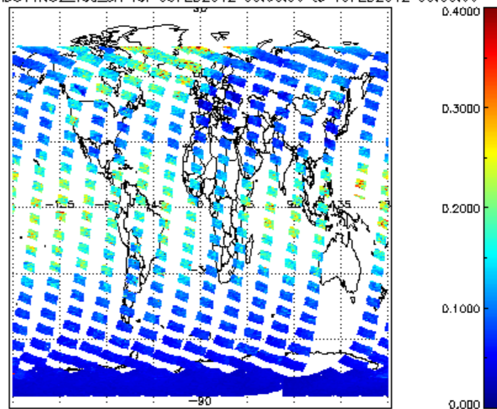
SCIOL2P_NADUV1N02_vcd_err for 09FEB2012 00:00:00 to 10FEB2012 00:00:00
