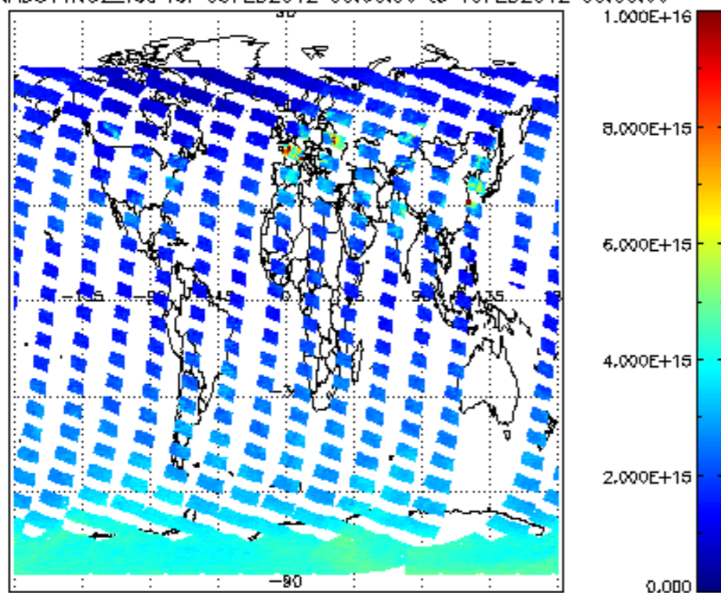
SCIOL2P_NADUV1N02_vcd for 09FEB2012 00:00:00 to 10FEB2012 00:00:00
