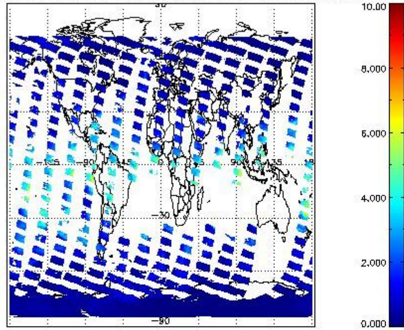
SCIOL2P_NADUV8H2O_vcd for 09FEB2012 00:00:00 to 10FEB2012 00:00:00
