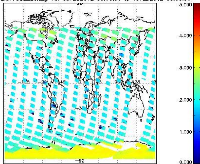
SCIOL2P_NADUV7S02_amf_gr for 09FEB2012 00:00:00 to 10FEB2012 00:00:00
