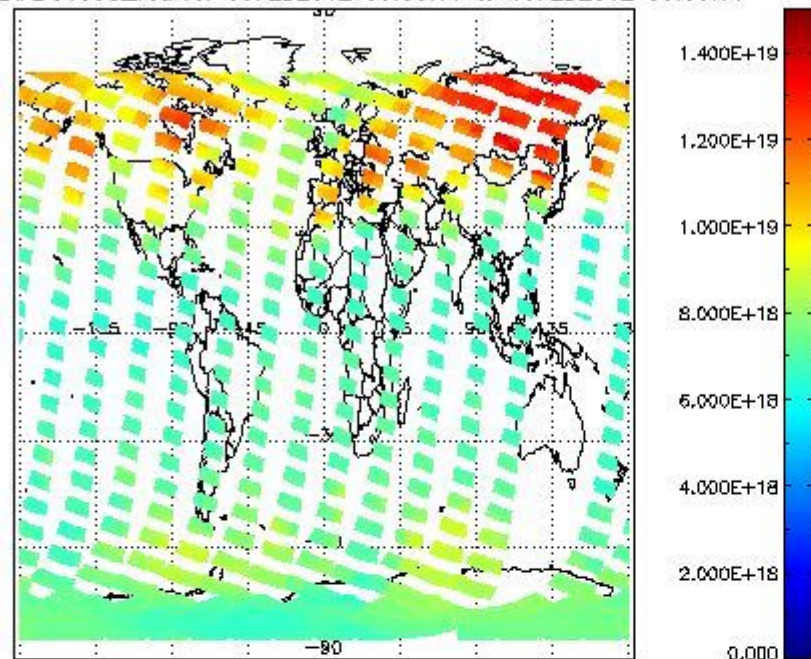
SCIOL2P_NADUV003_vcd for 09FEB2012 00:00:00 to 10FEB2012 00:00:00
