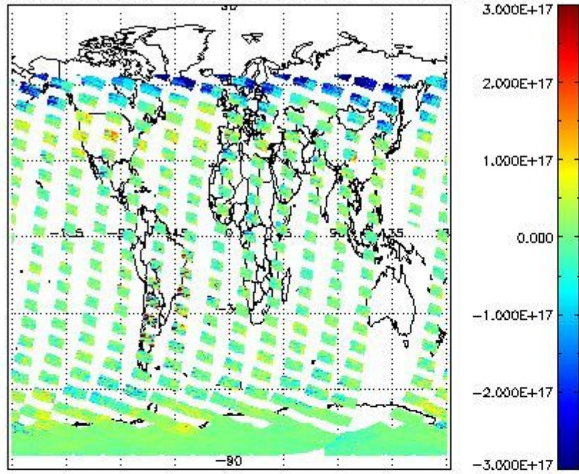
SCIOL2P_NADUV5SO2_vcd for 09FEB2012 00:00:00 to 10FEB2012 00:00:00
