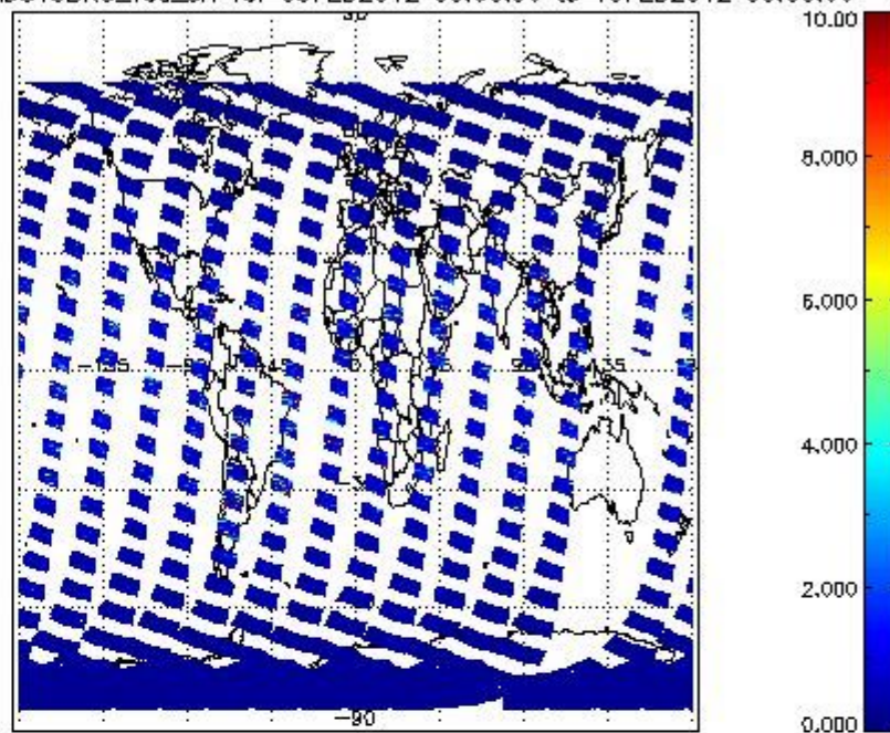
SCIOL2P_NADUV3BRO_vcd_err for 09FEB2012 00:00:00 to 10FEB2012 00:00:00
