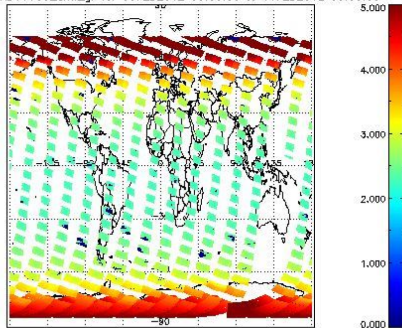
SCIOL2P_NADUV003_amf_gr for 09FEB2012 00:00:00 to 10FEB2012 00:00:00
