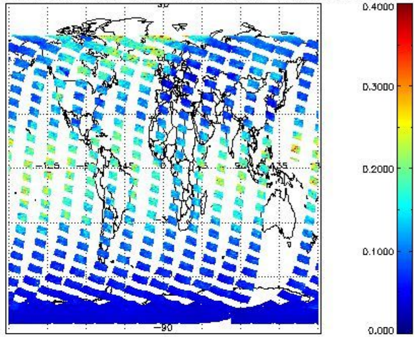
SCIOL2P_NADUV1N02_vcd_err for 09FEB2012 00:00:00 to 10FEB2012 00:00:00
