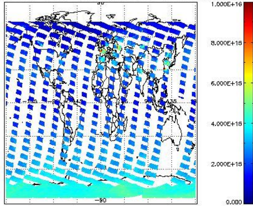
SCIOL2P_NADUV1N02_vcd for 09FEB2012 00:00:00 to 10FEB2012 00:00:00
