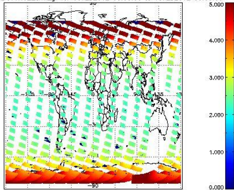
SCIOL2P_NADUV1N02_amf_gr for 09FEB2012 00:00:00 to 10FEB2012 00:00:00
