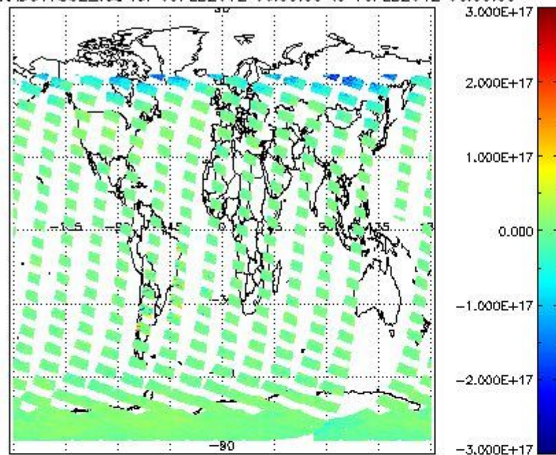
SCIOL2P_NADUV7S02_vcd for 09FEB2012 00:00:00 to 10FEB2012 00:00:00
