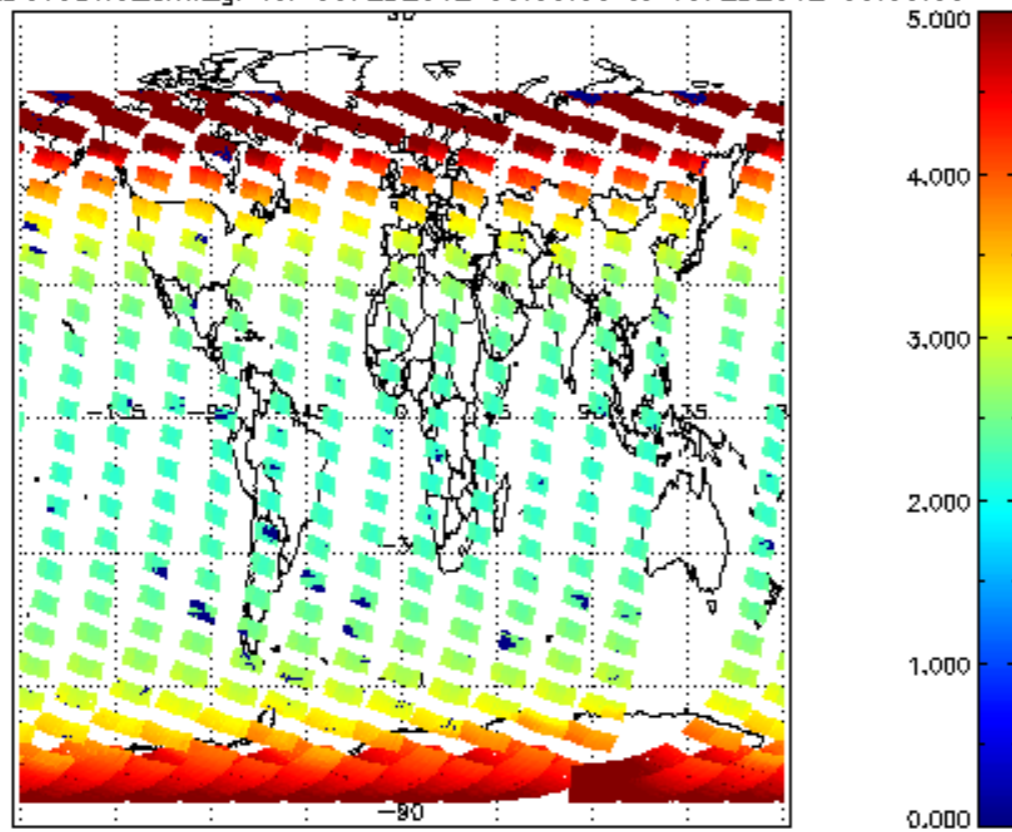
SCIOL2P_NADUV3BRO_amf_gr for 09FEB2012 00:00:00 to 10FEB2012 00:00:00
