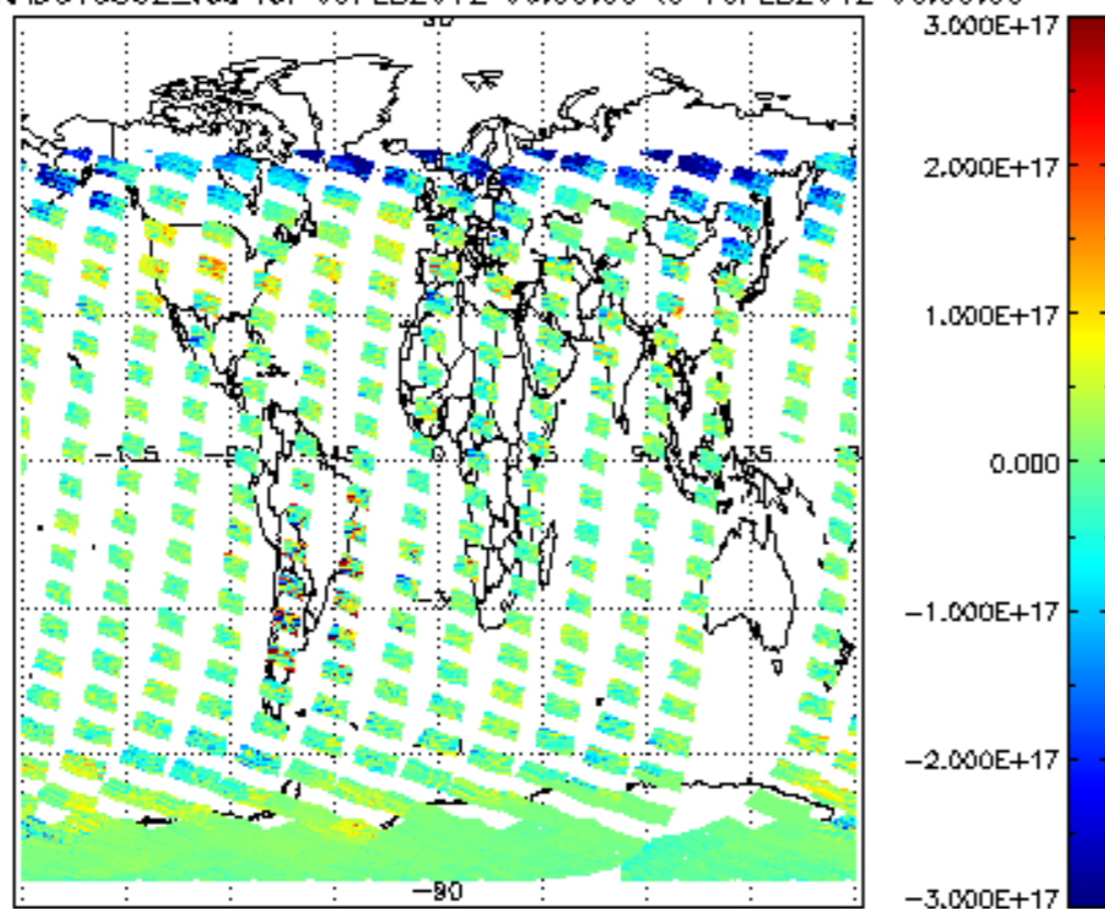
SCIOL2P_NADUV5S02_vcd for 09FEB2012 00:00:00 to 10FEB2012 00:00:00
