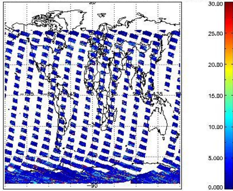
SCIOL2P_NADUV5SO2_vcd_err for 09FEB2012 00:00:00 to 10FEB2012 00:00:00
