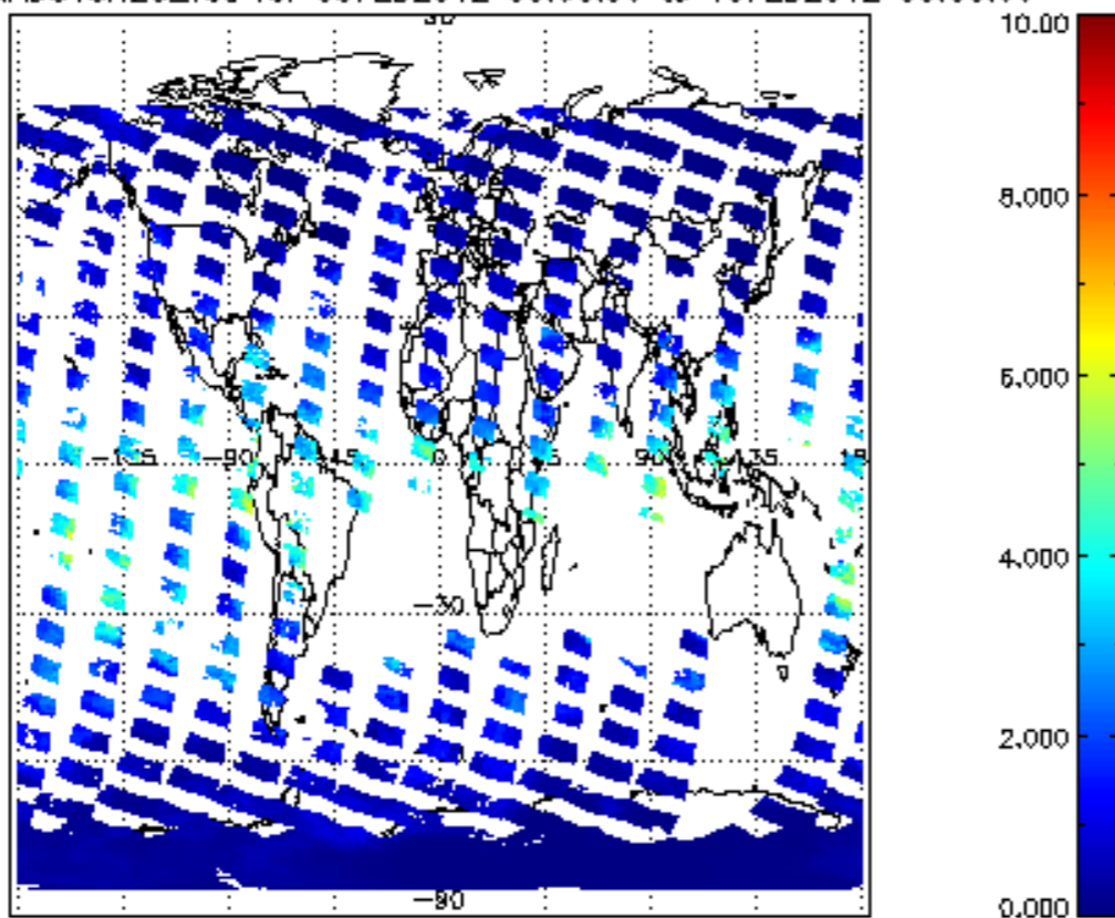
SCIOL2P_NADUV8H20_vcd for 09FEB2012 00:00:00 to 10FEB2012 00:00:00
