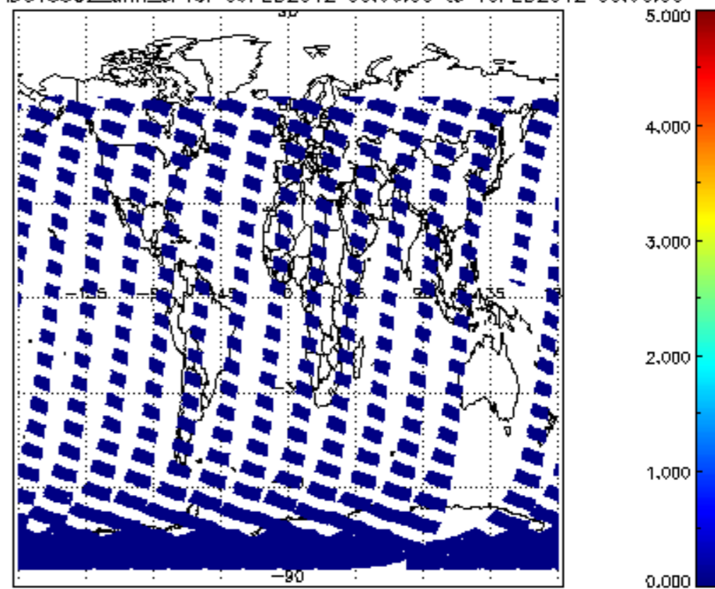
SCIOL2P_NADUV5S02_amf_cl for 09FEB2012 00:00:00 to 10FEB2012 00:00:00
