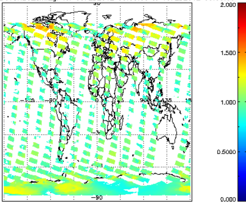
SCIOL2P_NADUV8H20_amf_gr for 09FEB2012 00:00:00 to 10FEB2012 00:00:00
