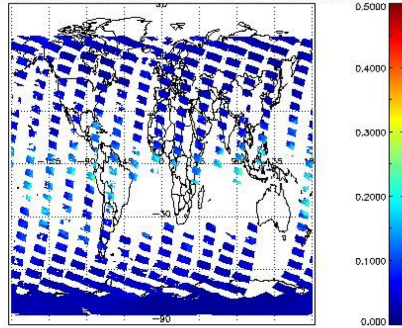
SCIOL2P_NADUV8H2O_vcd_err for 09FEB2012 00:00:00 to 10FEB2012 00:00:00
