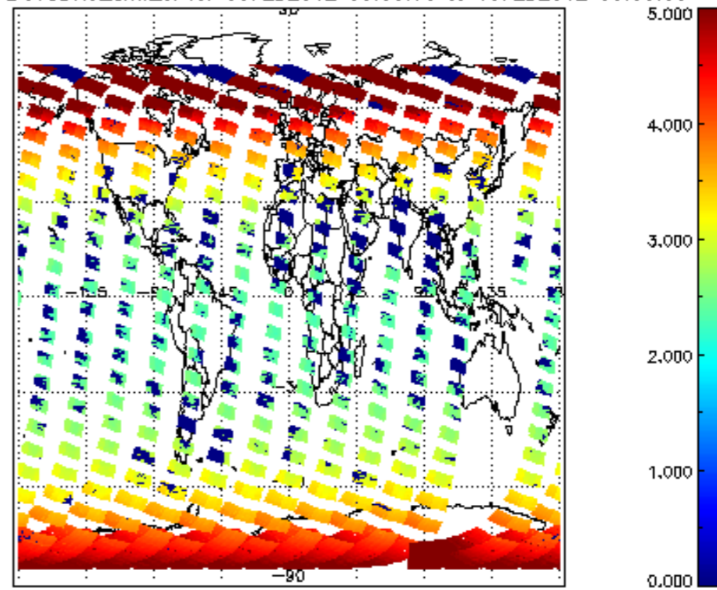
SCIOL2P_NADUV3BRO_amf_cl for 09FEB2012 00:00:00 to 10FEB2012 00:00:00
