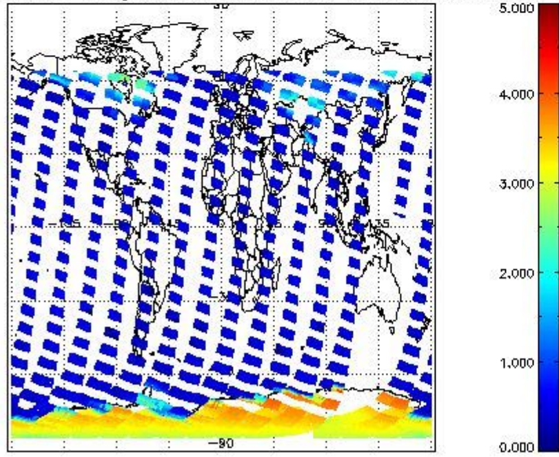
SCIOL2P_NADUV5SO2_amf_gr for 09FEB2012 00:00:00 to 10FEB2012 00:00:00
