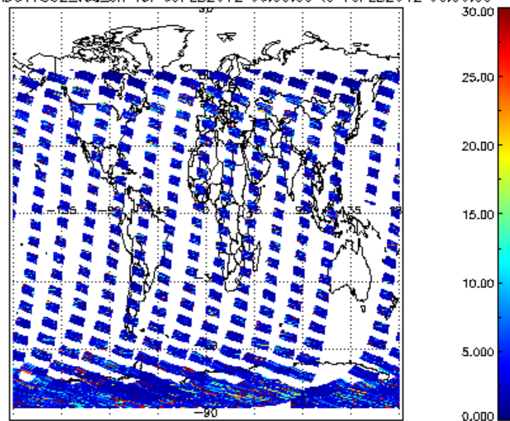
SCIOL2P_NADUV7S02_vcd_err for 09FEB2012 00:00:00 to 10FEB2012 00:00:00
