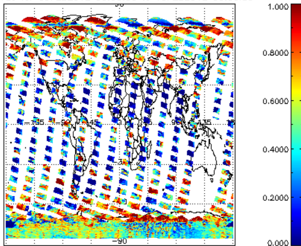
cI_frac for 09FEB2012 00:00:00 to 10FEB2012 00:00:00
