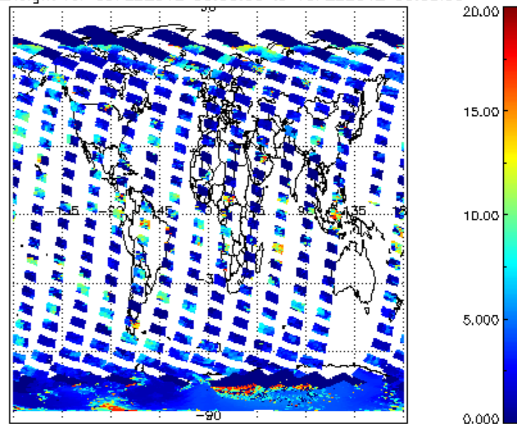
cI_top_height for 09FEB2012 00:00:00 to 10FEB2012 00:00:00
