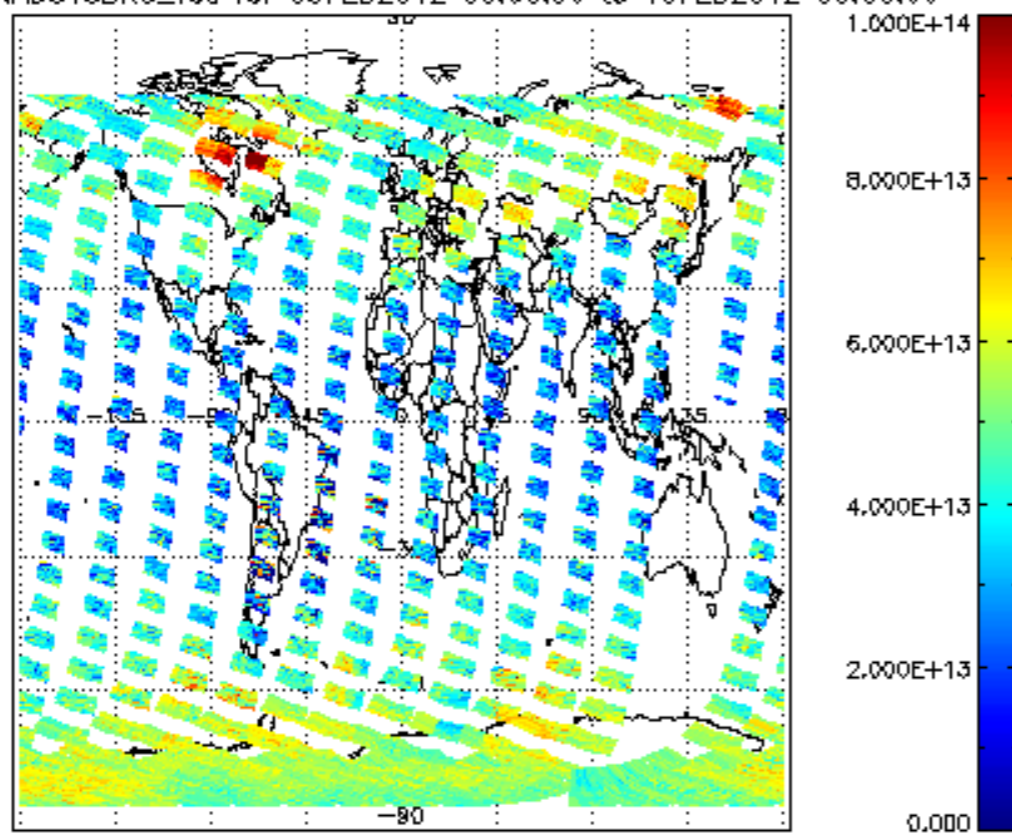
SCIOL2P_NADUV3BRO_vcd for 09FEB2012 00:00:00 to 10FEB2012 00:00:00
