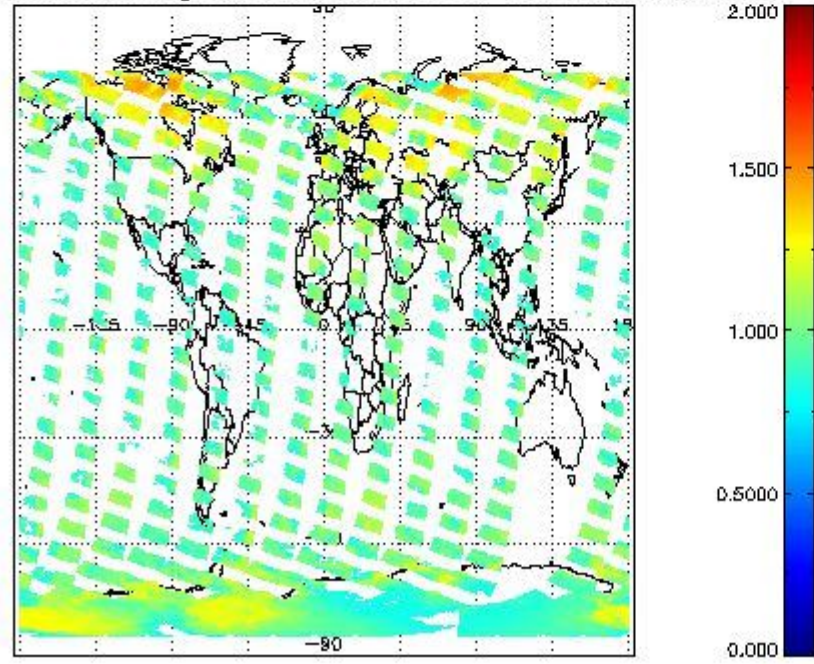
SCIOL2P_NADUV8H2O_amf_gr for 09FEB2012 00:00:00 to 10FEB2012 00:00:00
