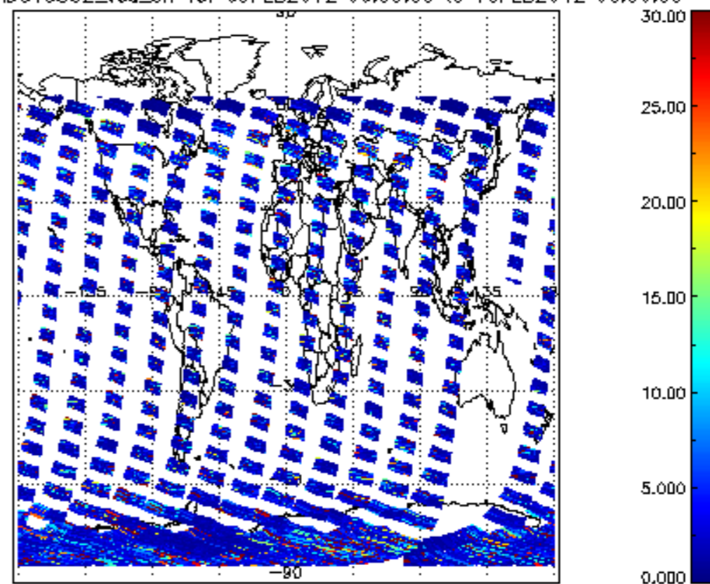
SCIOL2P_NADUV5S02_vcd_err for 09FEB2012 00:00:00 to 10FEB2012 00:00:00
