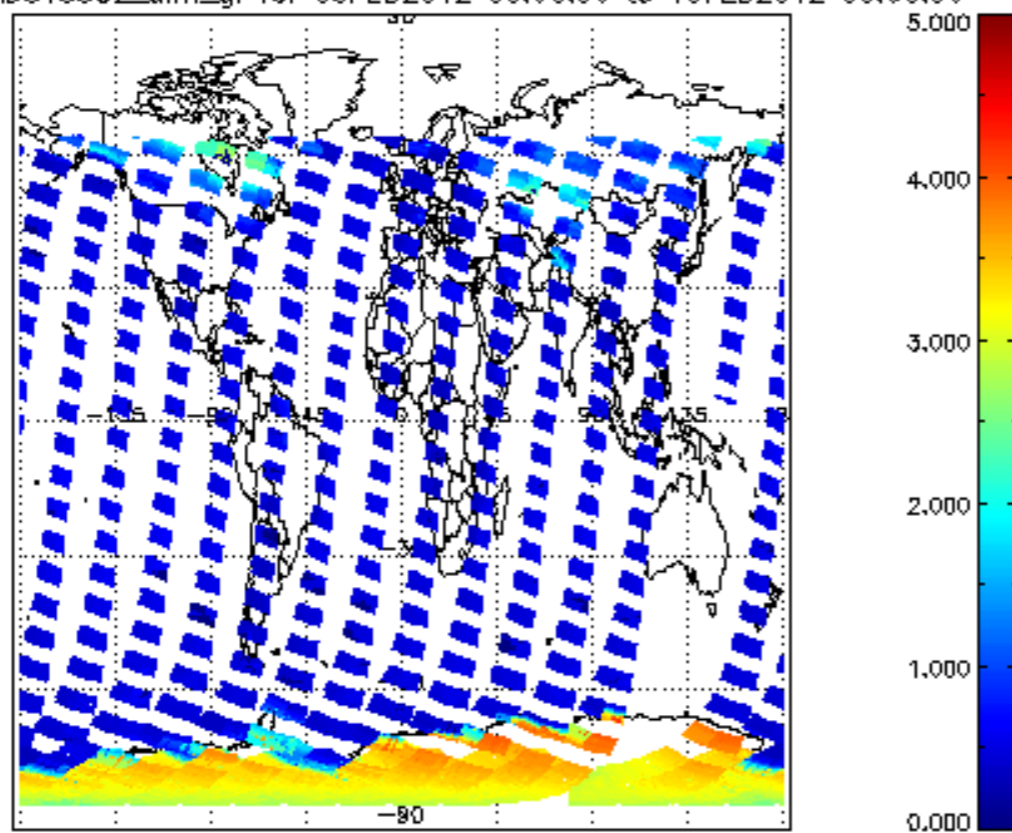
SCIOL2P_NADUV5S02_amf_gr for 09FEB2012 00:00:00 to 10FEB2012 00:00:00
