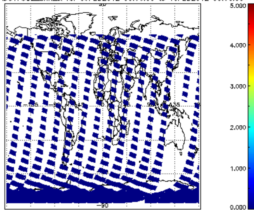
SCIOL2P_NADUV7S02_amf_cl for 09FEB2012 00:00:00 to 10FEB2012 00:00:00
