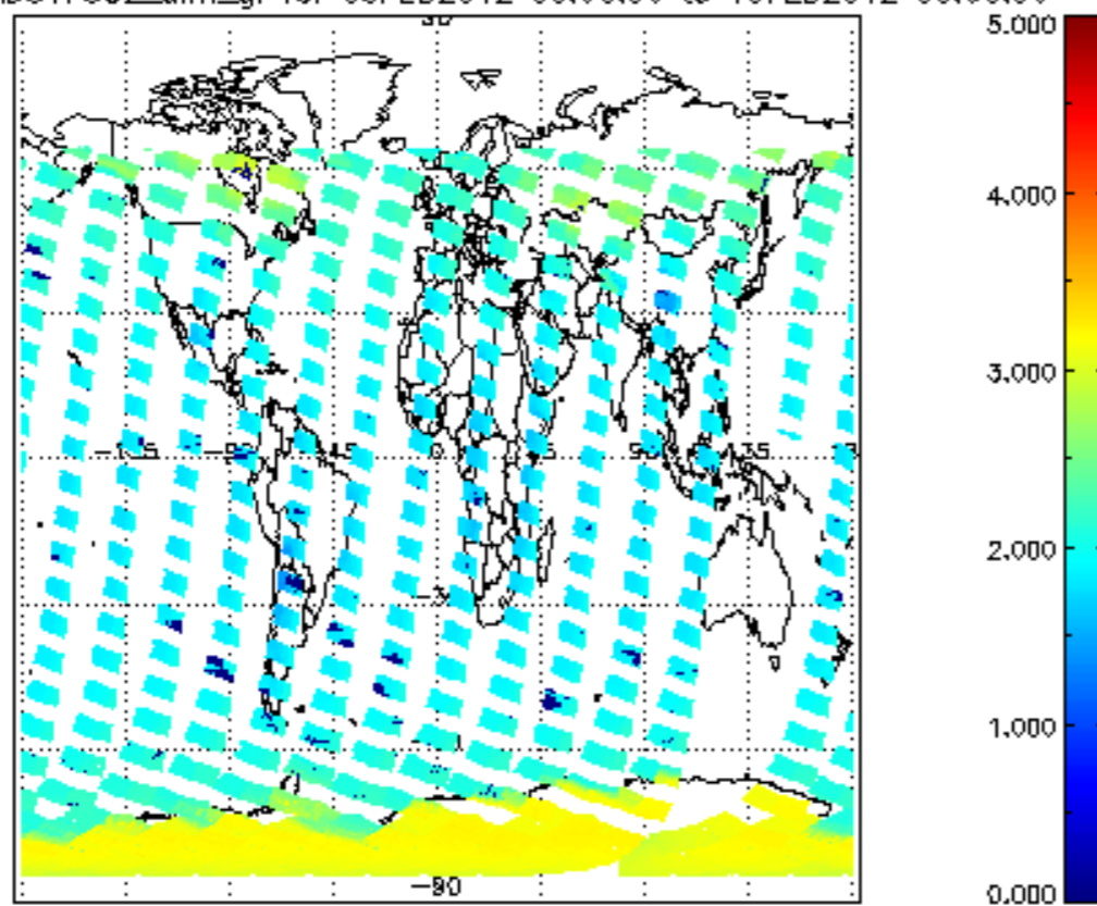
SCIOL2P_NADUV7S02_amf_gr for 09FEB2012 00:00:00 to 10FEB2012 00:00:00
