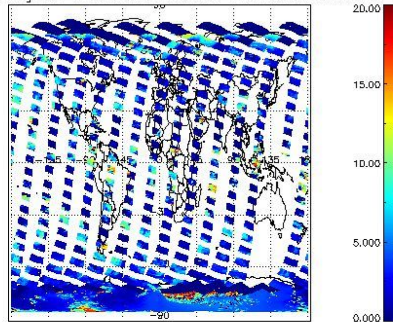
cL_top_height for 09FEB2012 00:00:00 to 10FEB2012 00:00:00
