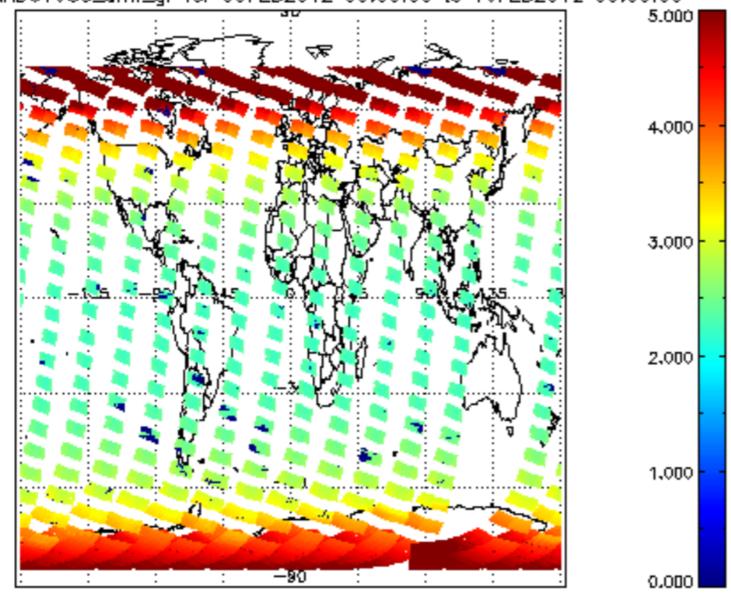
SCIOL2P_NADUV003_amf_gr for 09FEB2012 00:00:00 to 10FEB2012 00:00:00
