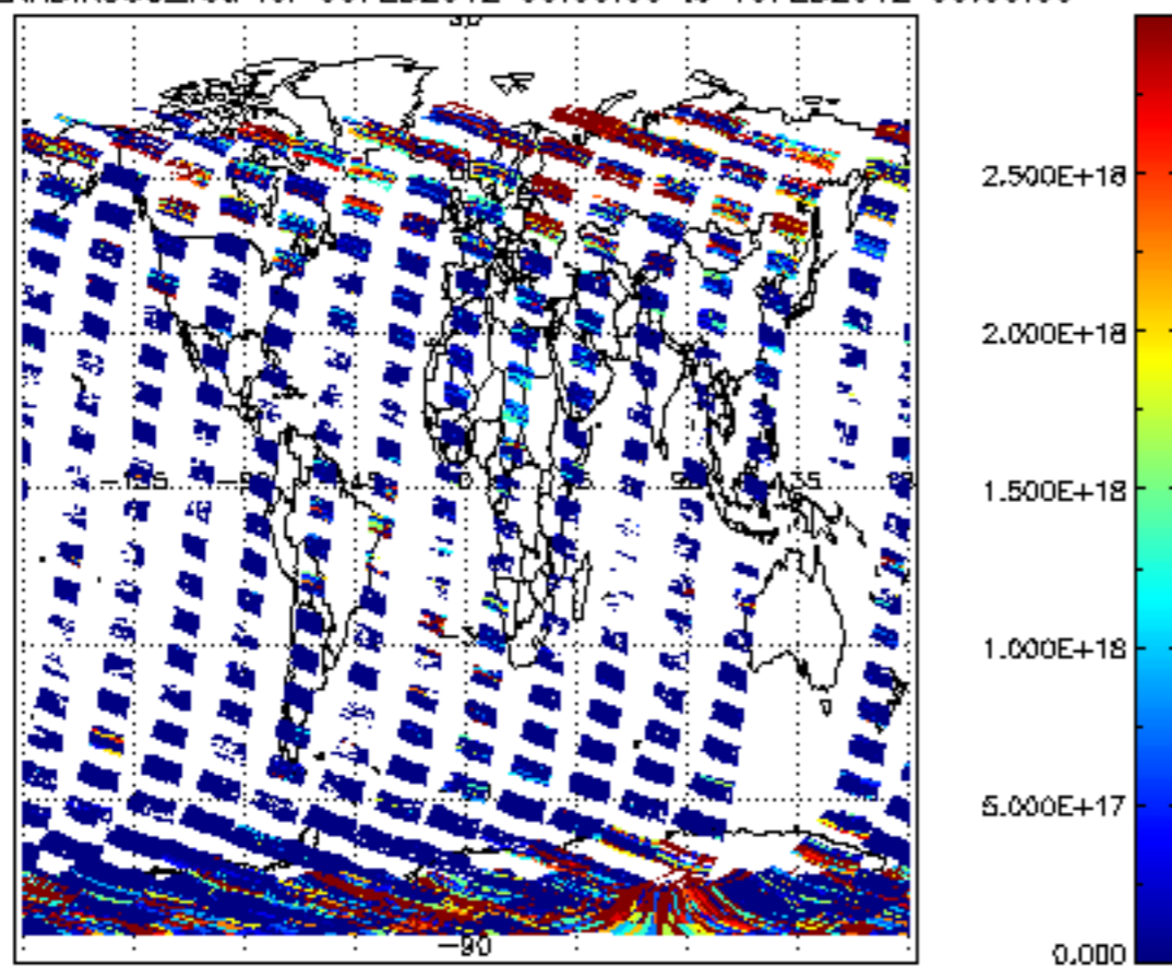
SCIOL2P_NADIR3CO_vcd for 09FEB2012 00:00:00 to 10FEB2012 00:00:00
