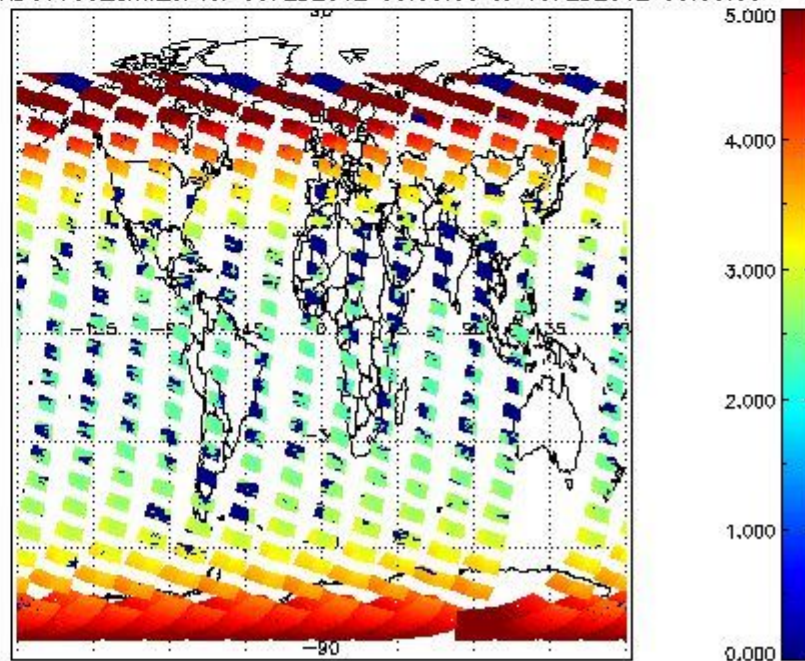
SCIOL2P_NADUV003_amf_cl for 09FEB2012 00:00:00 to 10FEB2012 00:00:00
