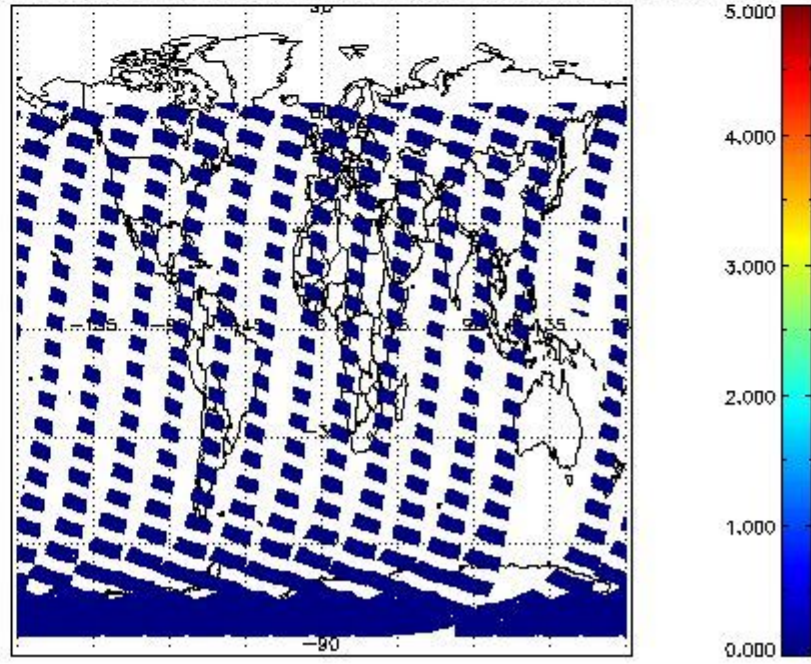
SCIOL2P_NADUV5SO2_amf_cl for 09FEB2012 00:00:00 to 10FEB2012 00:00:00
