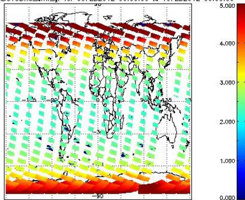
SCIOL2P_NADUV3BRO_amf_gr for 09FEB2012 00:00:00 to 10FEB2012 00:00:00
