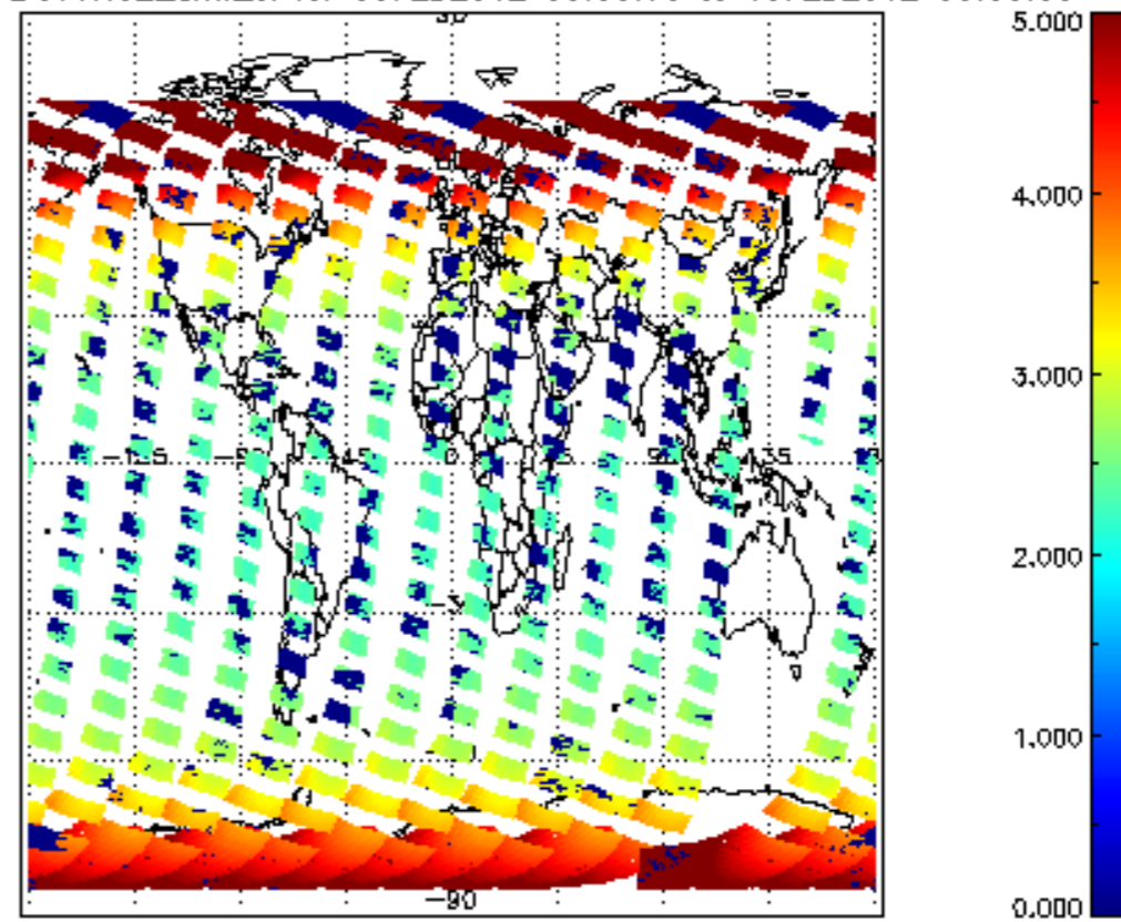
SCIOL2P_NADUV1N02_amf_cl for 09FEB2012 00:00:00 to 10FEB2012 00:00:00
