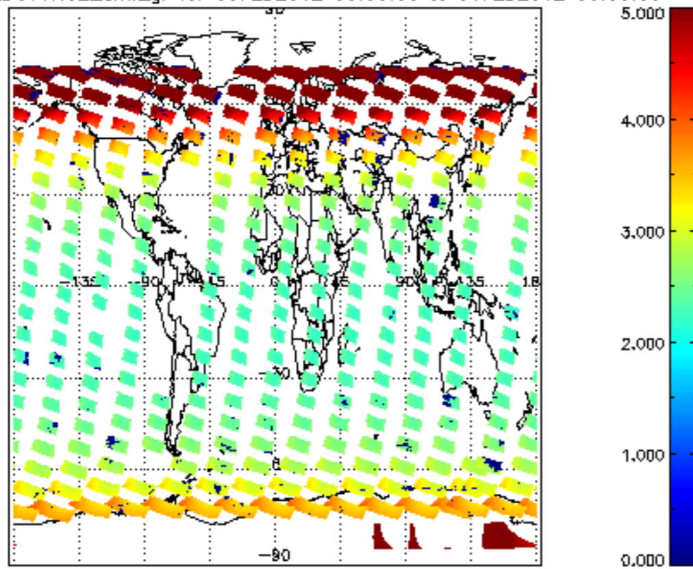
SCIOL2P_NADUV1N02_amf_gr for 05FEB2012 00:00:00 to 06FEB2012 00:00:00
