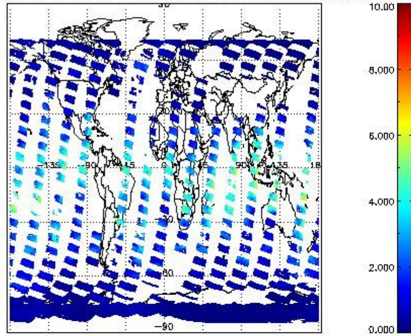
SCIOL2P_NADUV8H2O_vcd for 05FEB2012 00:00:00 to 06FEB2012 00:00:00
