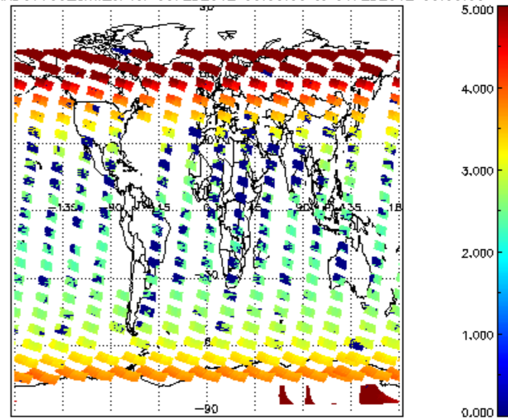
SCIOL2P_NADUV003_amf_cl for 05FEB2012 00:00:00 to 06FEB2012 00:00:00
