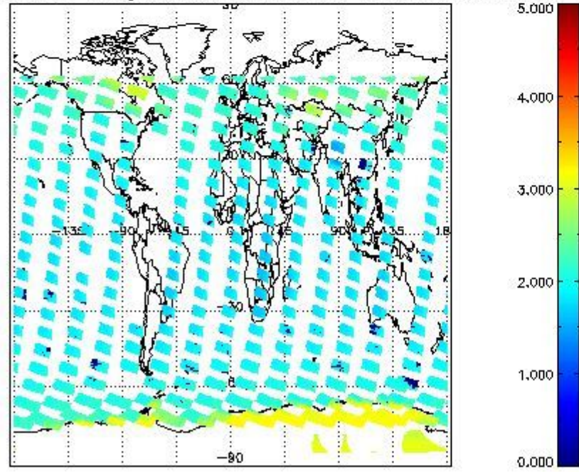
SCIOL2P_NADUV7S02_amf_gr for 05FEB2012 00:00:00 to 06FEB2012 00:00:00
