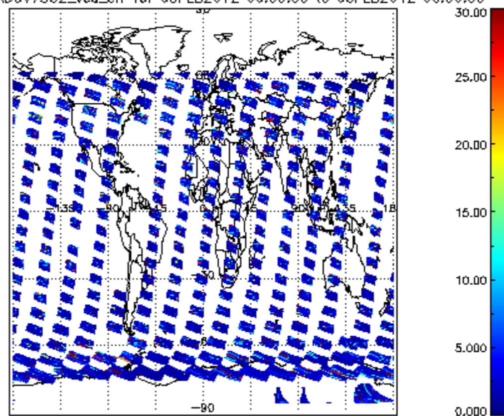
SCIOL2P_NADUV7S02_vcd_err for 05FEB2012 00:00:00 to 06FEB2012 00:00:00
