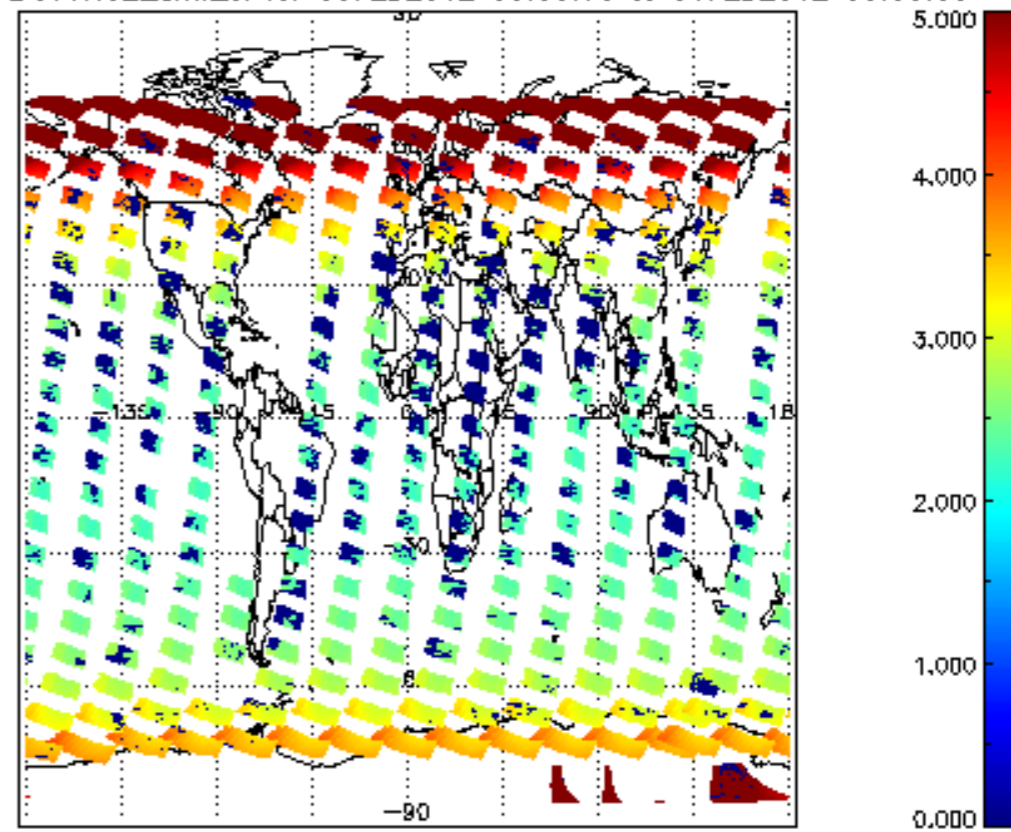
SCIOL2P_NADUV1N02_amf_cl for 05FEB2012 00:00:00 to 06FEB2012 00:00:00
