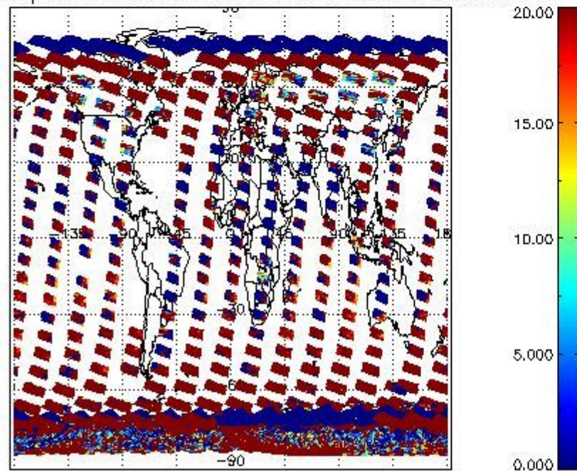
cL_opt_depth for 05FEB2012 00:00:00 to 06FEB2012 00:00:00
