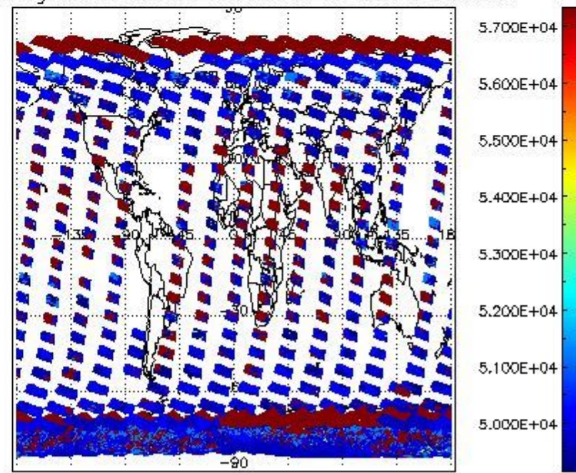
cloud_flags for 05FEB2012 00:00:00 to 06FEB2012 00:00:00
