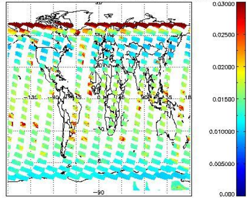
SCIOL2P_NADUV003_vcd_err for 05FEB2012 00:00:00 to 06FEB2012 00:00:00
