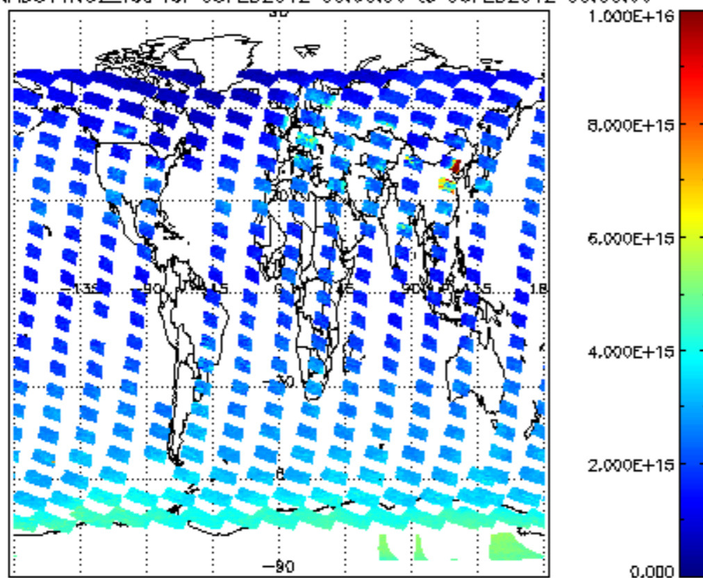
SCIOL2P_NADUV1N02_vcd for 05FEB2012 00:00:00 to 06FEB2012 00:00:00
