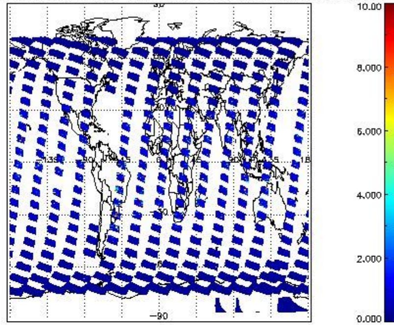
SCIOL2P_NADUV3BRO_vcd_err for 05FEB2012 00:00:00 to 06FEB2012 00:00:00
