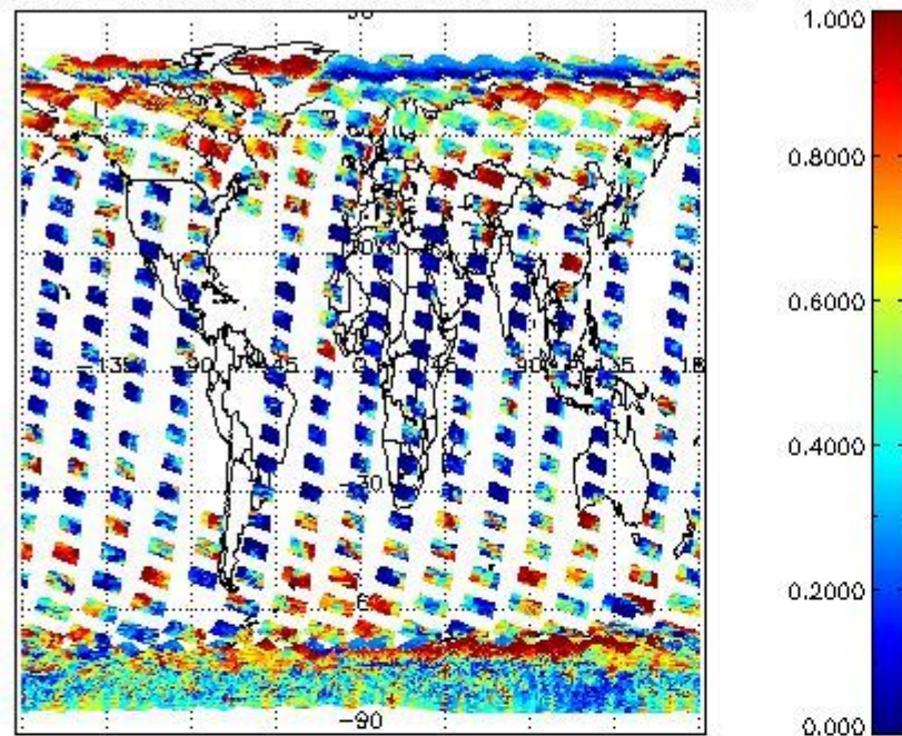
cL_frac for 05FEB2012 00:00:00 to 06FEB2012 00:00:00
