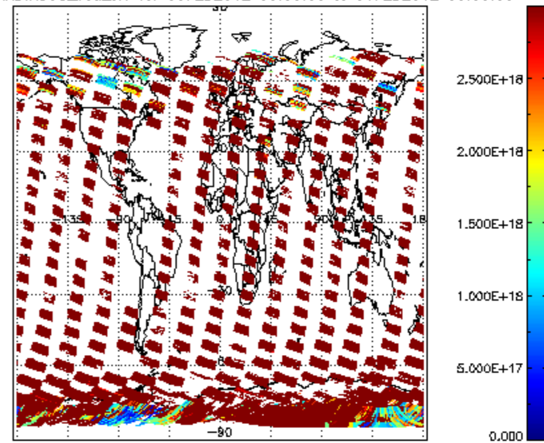
SCIOL2P_NADIR3CO_vcd_err for 05FEB2012 00:00:00 to 06FEB2012 00:00:00
