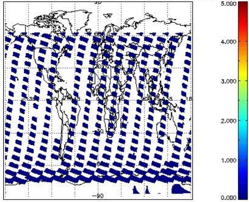
SCIOL2P_NADUV7S02_amf_cl for 05FEB2012 00:00:00 to 06FEB2012 00:00:00
