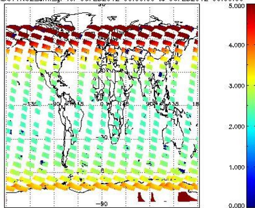
SCIOL2P_NADUV1N02_amf_gr for 05FEB2012 00:00:00 to 06FEB2012 00:00:00
