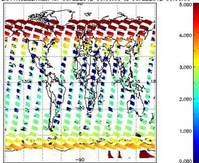
SCIOL2P_NADUV1N02_amf_cl for 05FEB2012 00:00:00 to 06FEB2012 00:00:00
