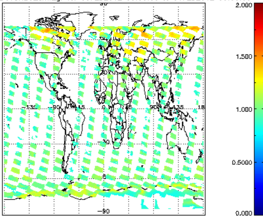
SCIOL2P_NADUV8H20_amf_gr for 05FEB2012 00:00:00 to 06FEB2012 00:00:00
