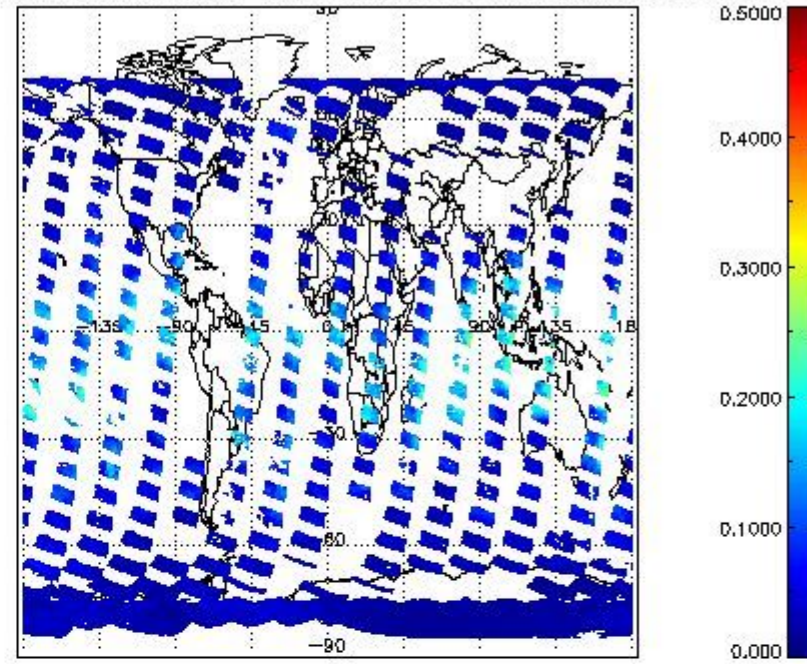
SCIOL2P_NADUV8H2O_vcd_err for 05FEB2012 00:00:00 to 06FEB2012 00:00:00
