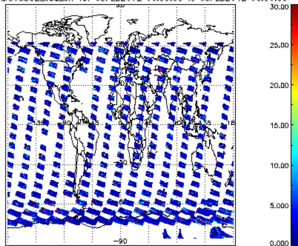
SCIOL2P_NADUV5S02_vcd_err for 05FEB2012 00:00:00 to 06FEB2012 00:00:00
