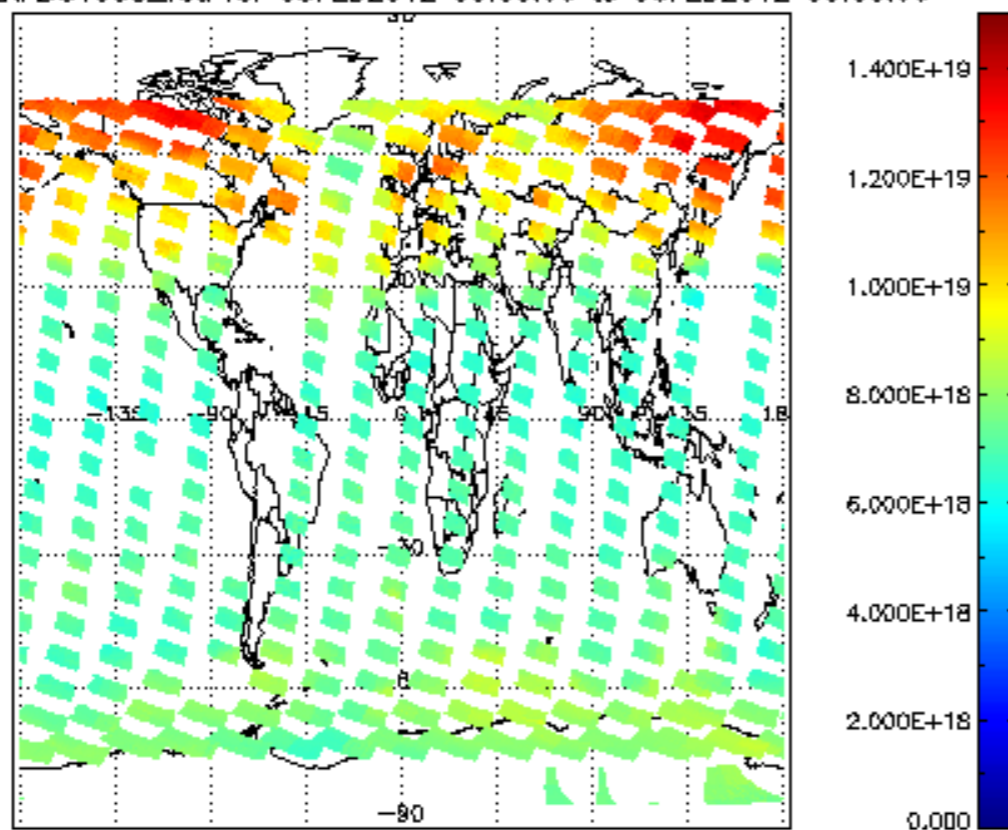
SCIOL2P_NADUV003_vcd for 05FEB2012 00:00:00 to 06FEB2012 00:00:00
