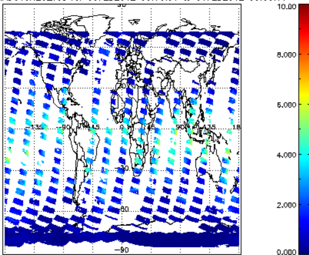
SCIOL2P_NADUV8H20_vcd for 05FEB2012 00:00:00 to 06FEB2012 00:00:00
