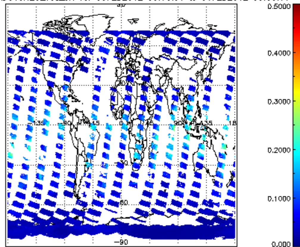
SCIOL2P_NADUV8H20_vcd_err for 05FEB2012 00:00:00 to 06FEB2012 00:00:00
