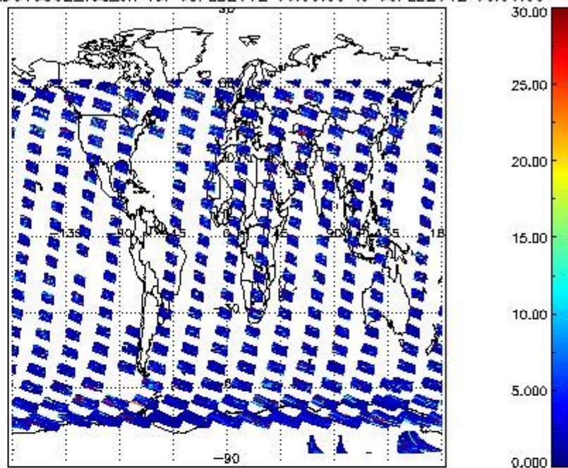
SCIOL2P_NADUV5S02_vcd_err for 05FEB2012 00:00:00 to 06FEB2012 00:00:00
