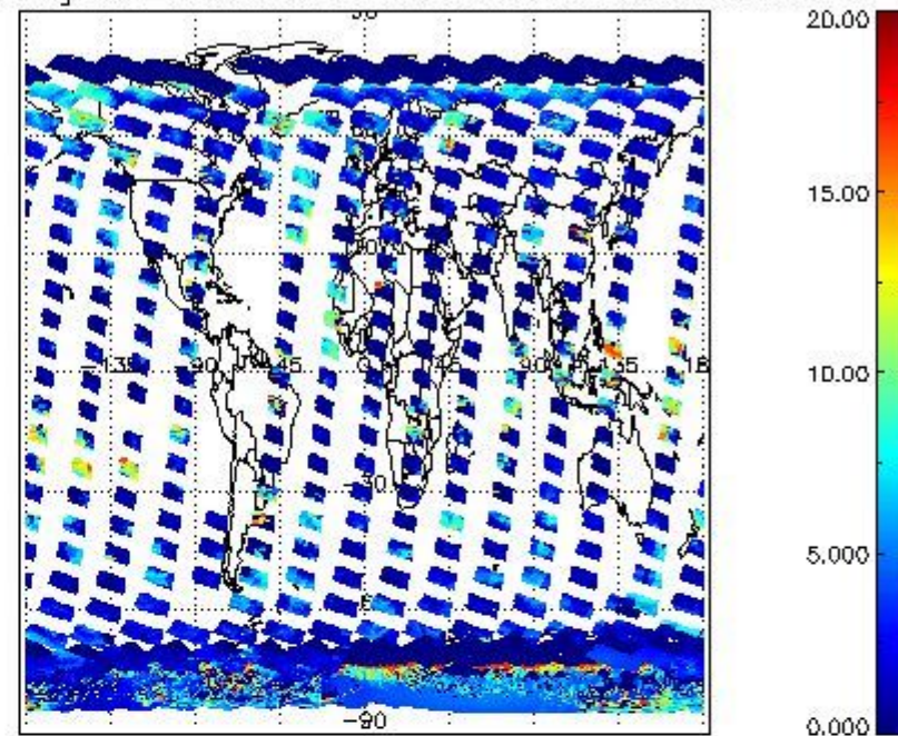
cL_top_height for 05FEB2012 00:00:00 to 06FEB2012 00:00:00
