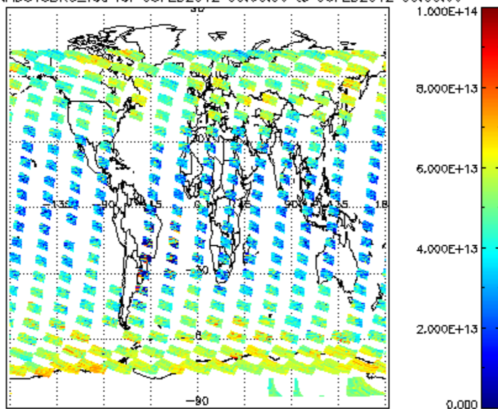
SCIOL2P_NADUV3BRO_vcd for 05FEB2012 00:00:00 to 06FEB2012 00:00:00
