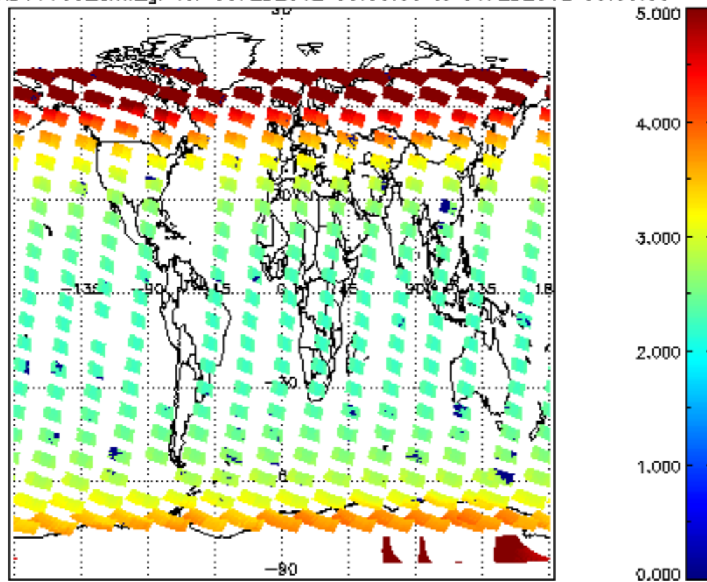
SCIOL2P_NADUV003_amf_gr for 05FEB2012 00:00:00 to 06FEB2012 00:00:00
