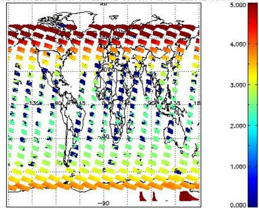
SCIOL2P_NADUV003_amf_cl for 05FEB2012 00:00:00 to 06FEB2012 00:00:00
