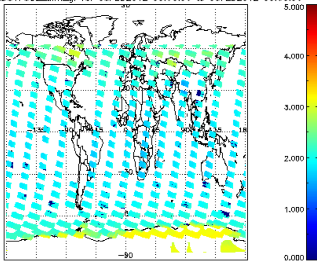
SCIOL2P_NADUV7S02_amf_gr for 05FEB2012 00:00:00 to 06FEB2012 00:00:00
