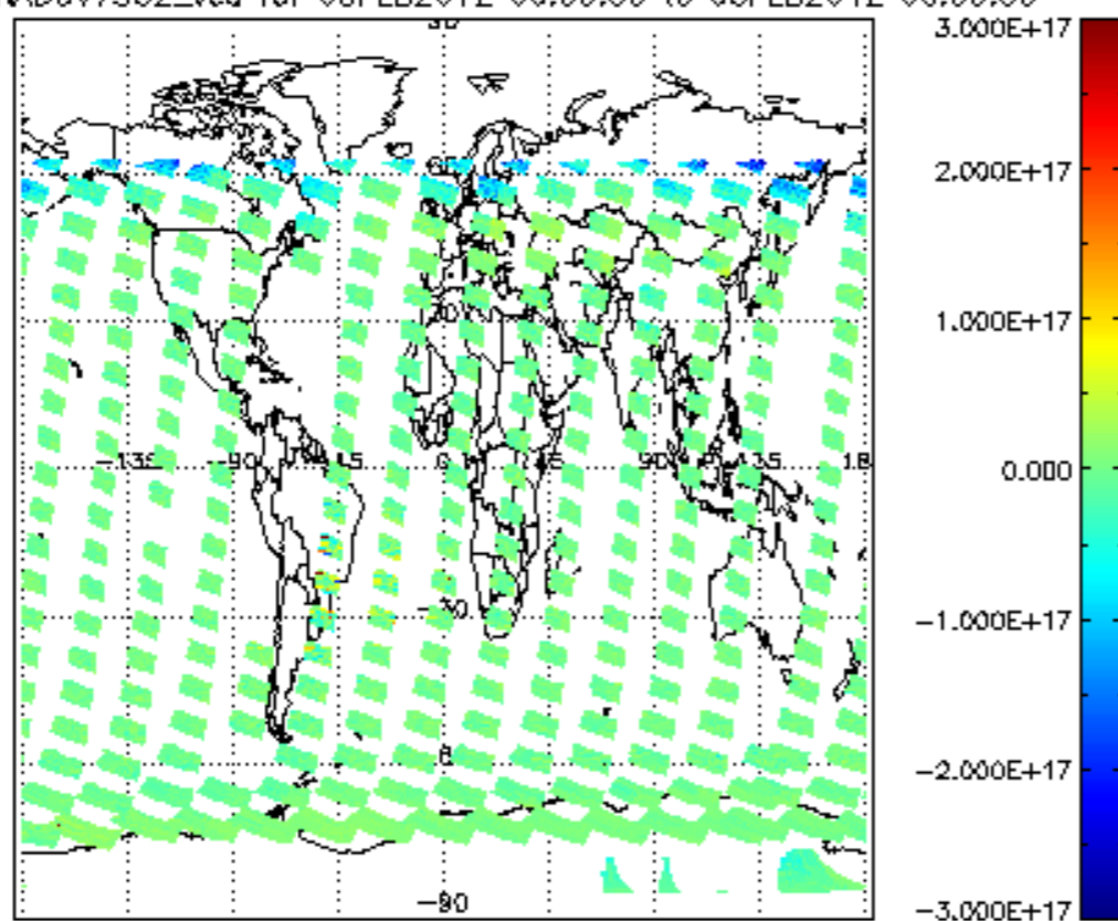
SCIOL2P_NADUV7S02_vcd for 05FEB2012 00:00:00 to 06FEB2012 00:00:00
