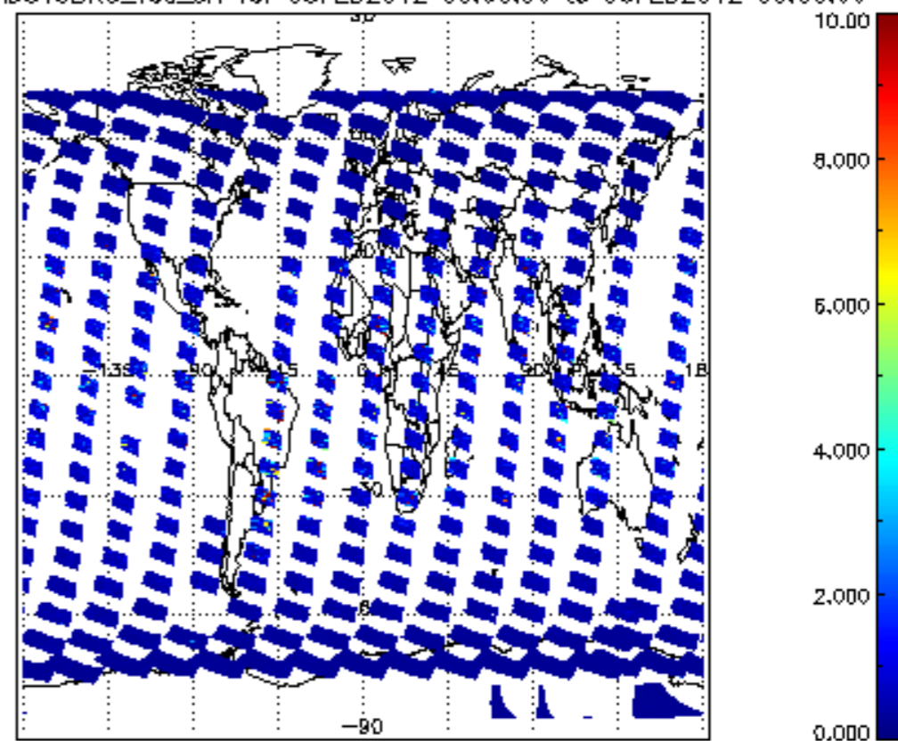
SCIOL2P_NADUV3BRO_vcd_err for 05FEB2012 00:00:00 to 06FEB2012 00:00:00
