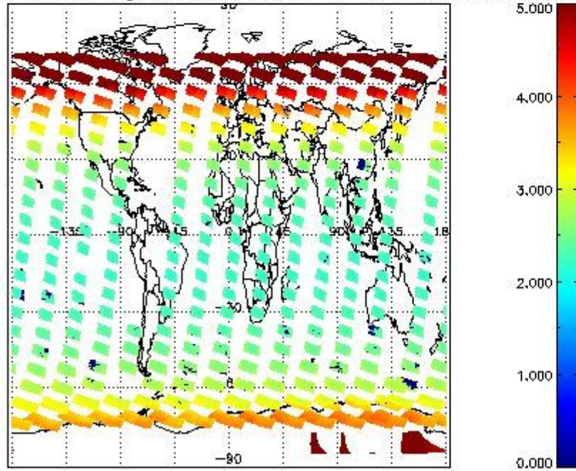
SCIOL2P_NADUV3BRO_amf_gr for 05FEB2012 00:00:00 to 06FEB2012 00:00:00
