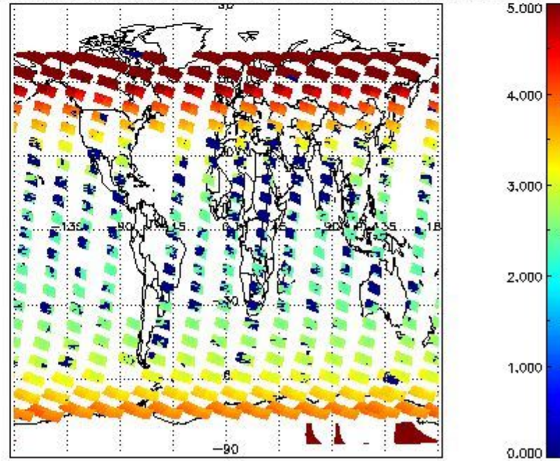
SCIOL2P_NADUV3BRO_amf_cl for 05FEB2012 00:00:00 to 06FEB2012 00:00:00
