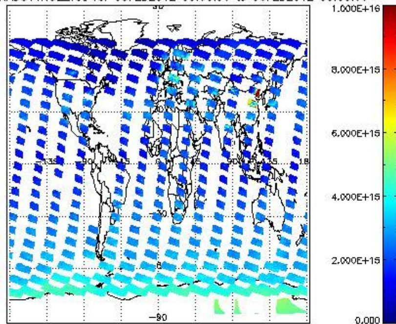
SCIOL2P_NADUV1N02_vcd for 05FEB2012 00:00:00 to 06FEB2012 00:00:00
