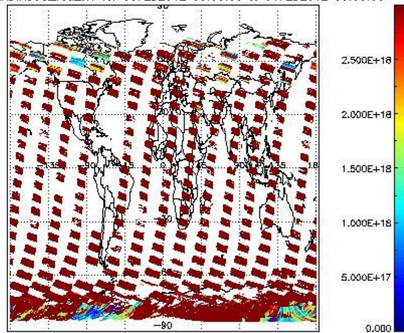
SCIO2P_NADIR3CO_vcd_err for 05FEB2012 00:00:00 to 06FEB2012 00:00:00
