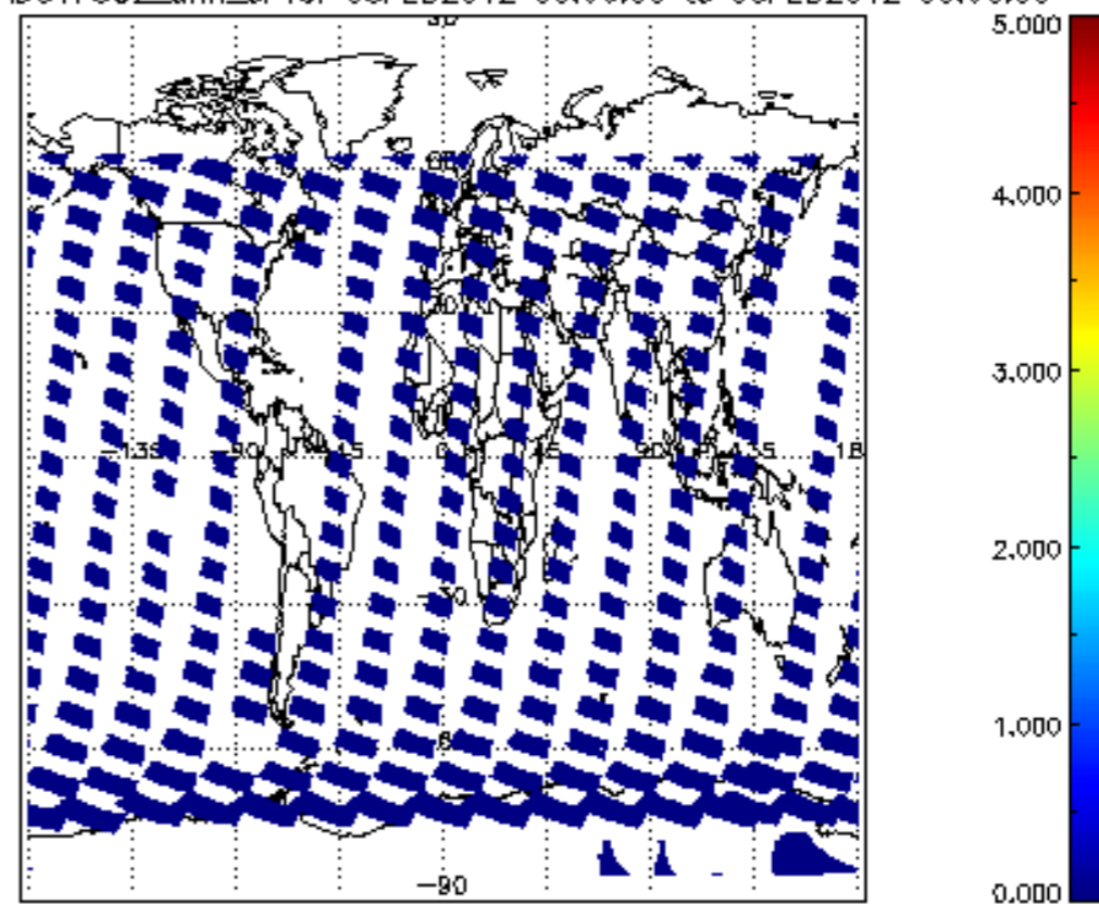
SCIOL2P_NADUV7S02_amf_cl for 05FEB2012 00:00:00 to 06FEB2012 00:00:00
