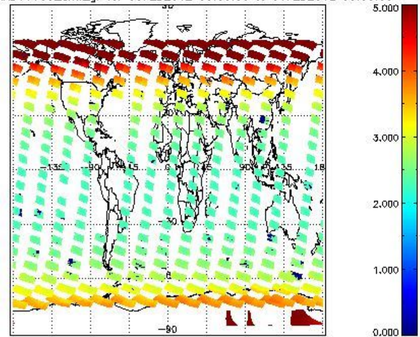
SCIOL2P_NADUV003_amf_gr for 05FEB2012 00:00:00 to 06FEB2012 00:00:00
