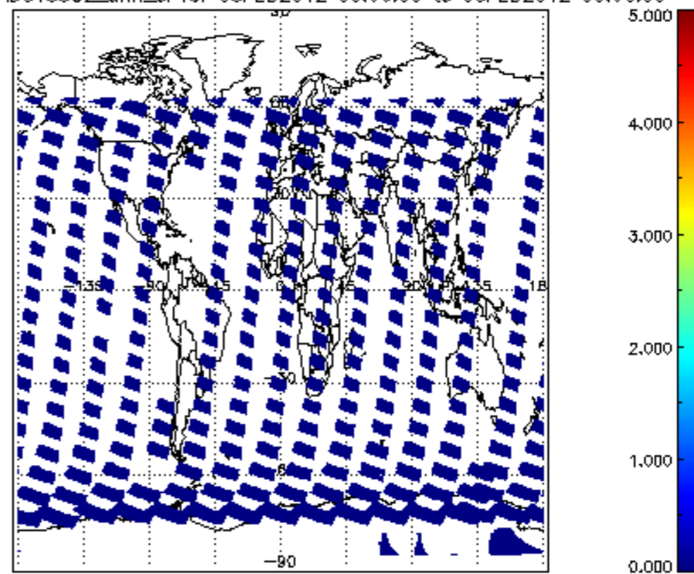
SCIOL2P_NADUV5S02_amf_cl for 05FEB2012 00:00:00 to 06FEB2012 00:00:00
