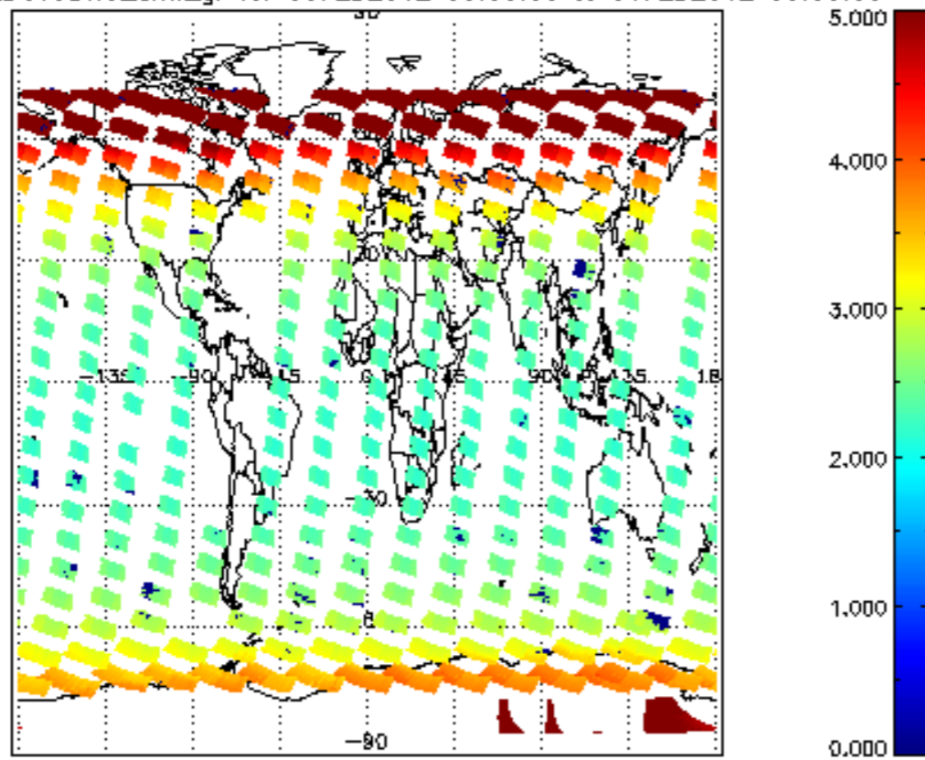
SCIOL2P_NADUV3BRO_amf_gr for 05FEB2012 00:00:00 to 06FEB2012 00:00:00
