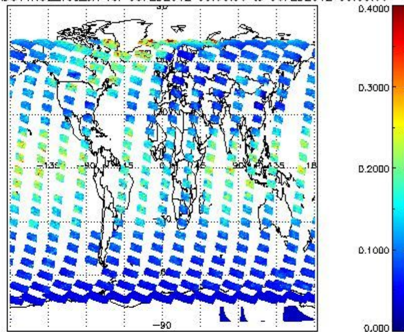
SCIOL2P_NADUV1N02_vcd_err for 05FEB2012 00:00:00 to 06FEB2012 00:00:00
