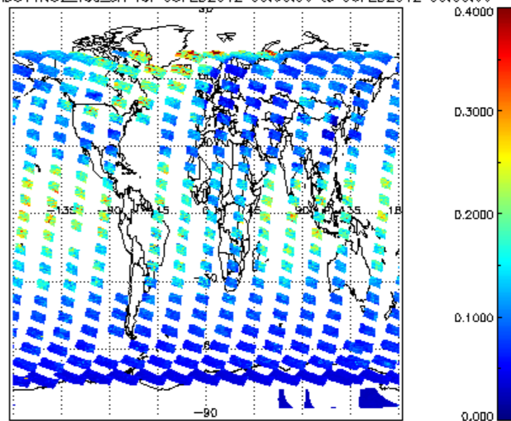
SCIOL2P_NADUV1N02_vcd_err for 05FEB2012 00:00:00 to 06FEB2012 00:00:00
