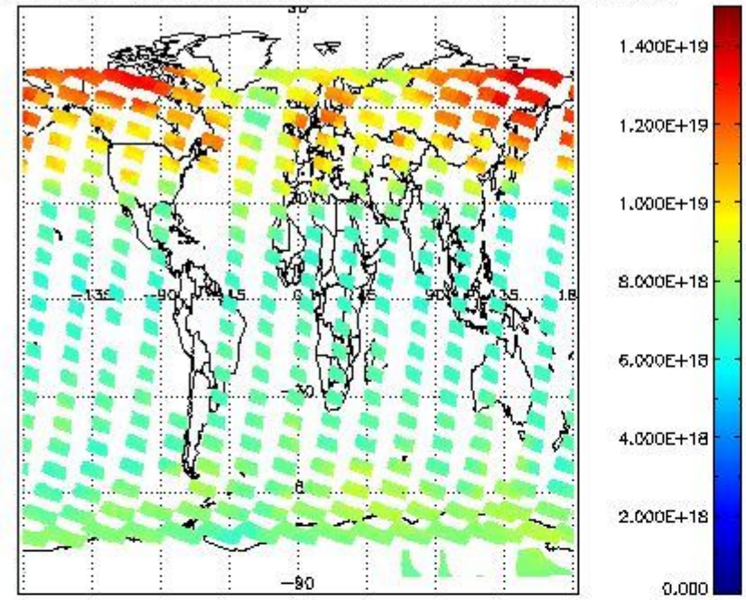
SCIOL2P_NADUV003_vcd for 05FEB2012 00:00:00 to 06FEB2012 00:00:00
