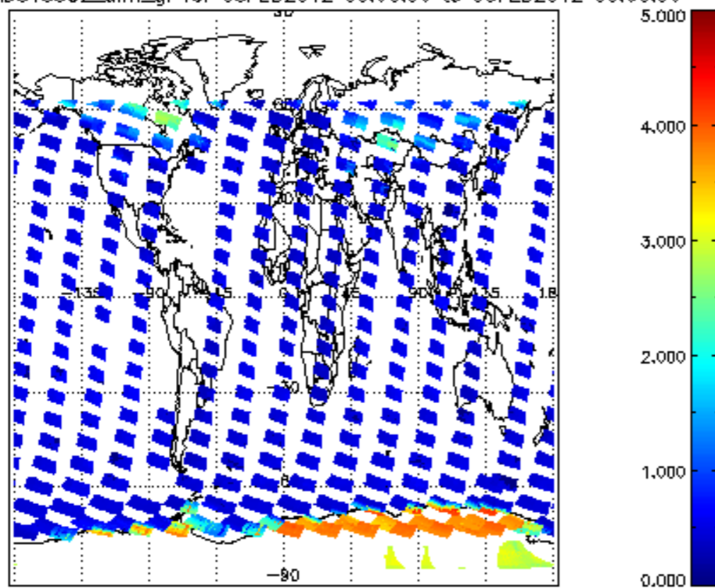
SCIOL2P_NADUV5S02_amf_gr for 05FEB2012 00:00:00 to 06FEB2012 00:00:00
