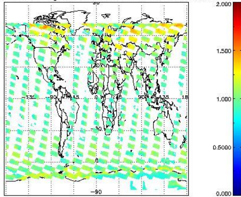
SCIOL2P_NADUV8H2O_arnf_gr for 05FEB2012 00:00:00 to 06FEB2012 00:00:00
