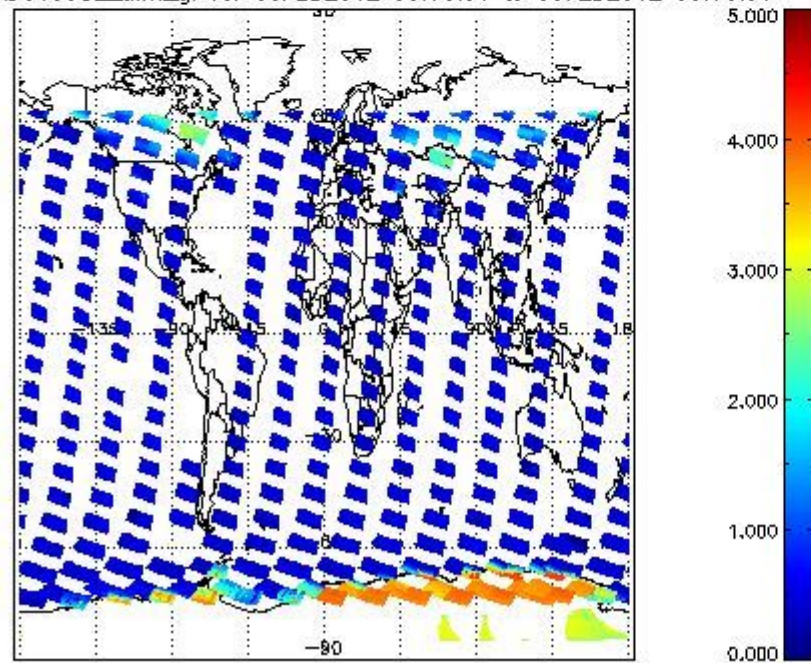
SCIOL2P_NADUV5S02_amf_gr for 05FEB2012 00:00:00 to 06FEB2012 00:00:00
