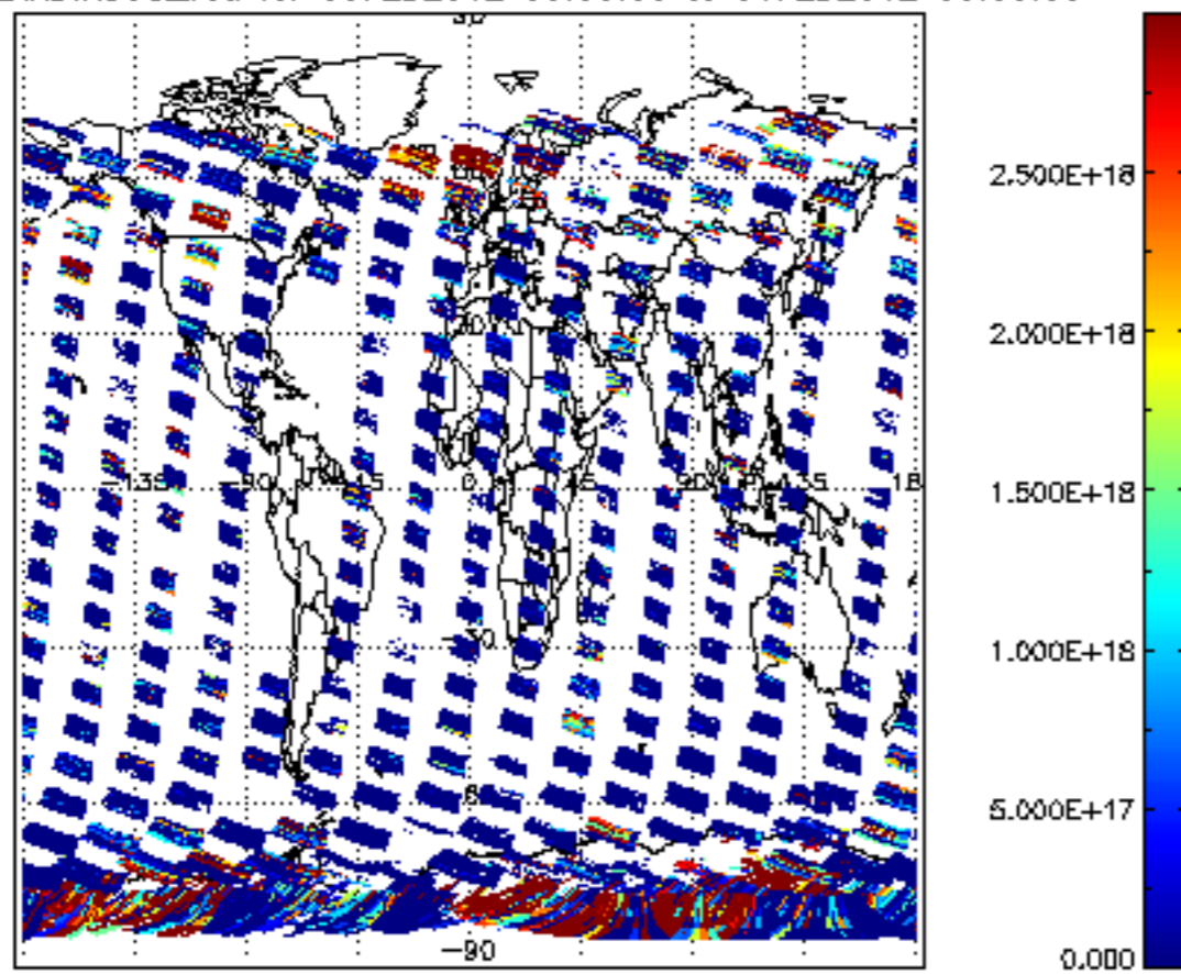
SCIOL2P_NADIR3CO_vcd for 05FEB2012 00:00:00 to 06FEB2012 00:00:00
