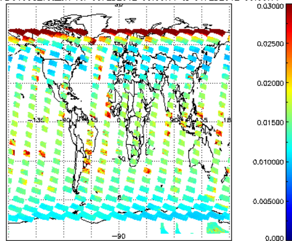
SCIOL2P_NADUV003_vcd_err for 05FEB2012 00:00:00 to 06FEB2012 00:00:00
