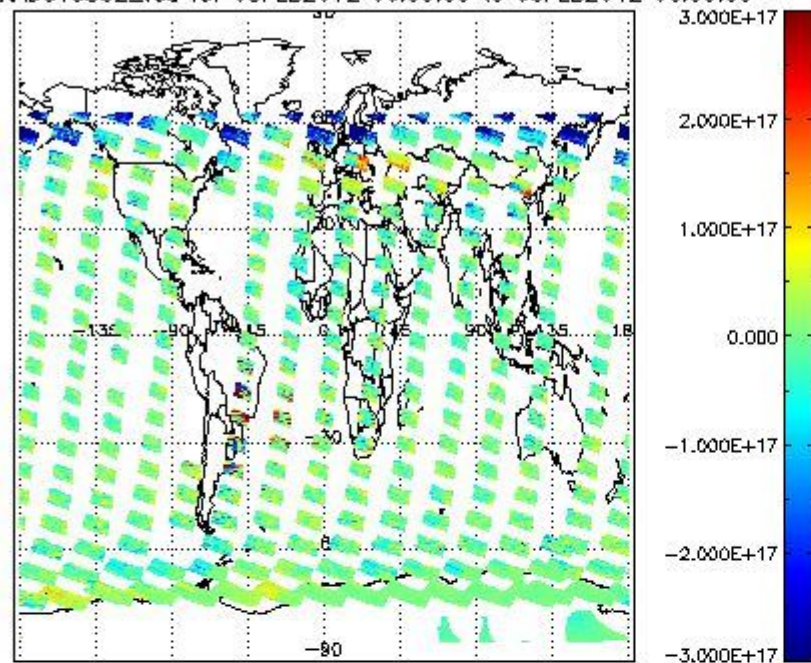
SCIOL2P_NADUV5S02_vcd for 05FEB2012 00:00:00 to 06FEB2012 00:00:00
