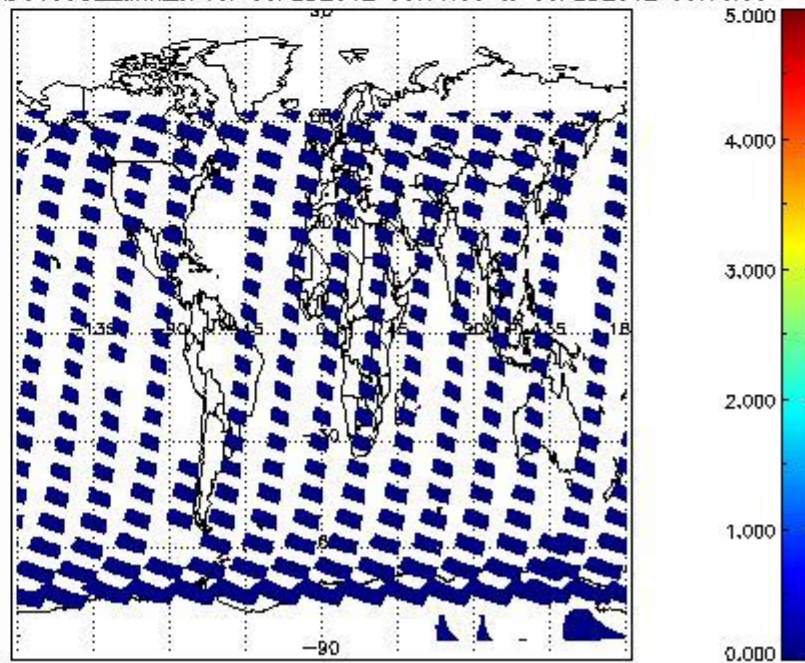
SCIOL2P_NADUV5S02_amf_cl for 05FEB2012 00:00:00 to 06FEB2012 00:00:00
