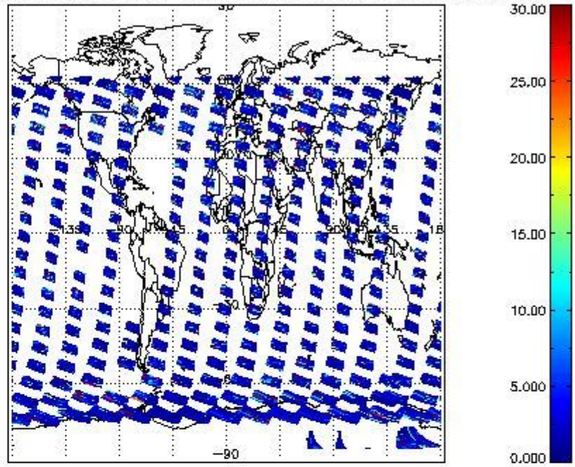
SCIOL2P_NADUV7S02_vcd_err for 05FEB2012 00:00:00 to 06FEB2012 00:00:00
