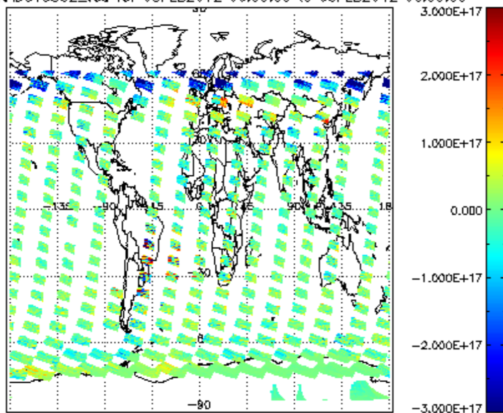
SCIOL2P_NADUV5S02_vcd for 05FEB2012 00:00:00 to 06FEB2012 00:00:00
