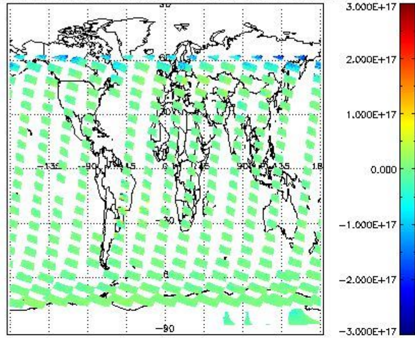
SCIOL2P_NADUV7S02_vcd for 05FEB2012 00:00:00 to 06FEB2012 00:00:00
