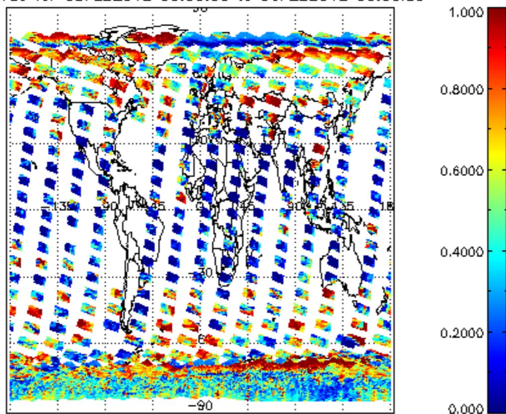
cl_frac for 05FEB2012 00:00:00 to 06FEB2012 00:00:00
