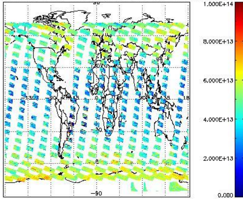
SCIOL2P_NADUV3BRO_vcd for 05FEB2012 00:00:00 to 06FEB2012 00:00:00
