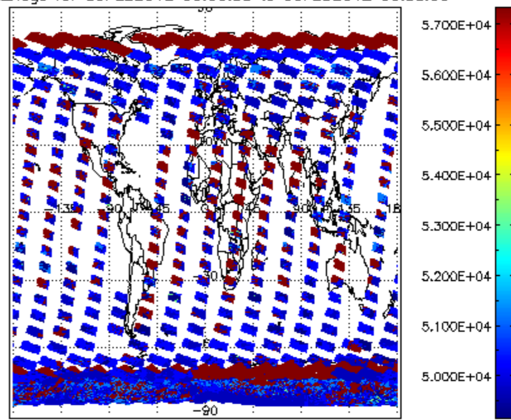
cloud_flags for 05FEB2012 00:00:00 to 06FEB2012 00:00:00
