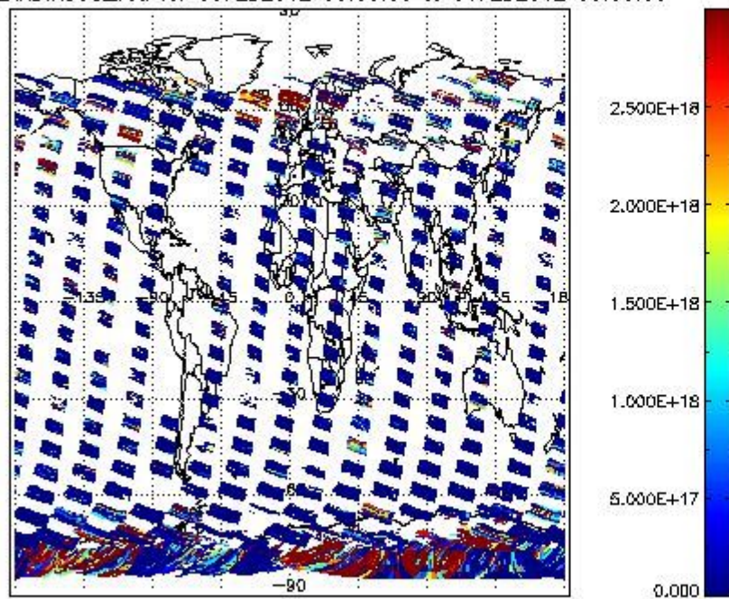
SCIO2P_NADIR3CO_vcd for 05FEB2012 00:00:00 to 06FEB2012 00:00:00
