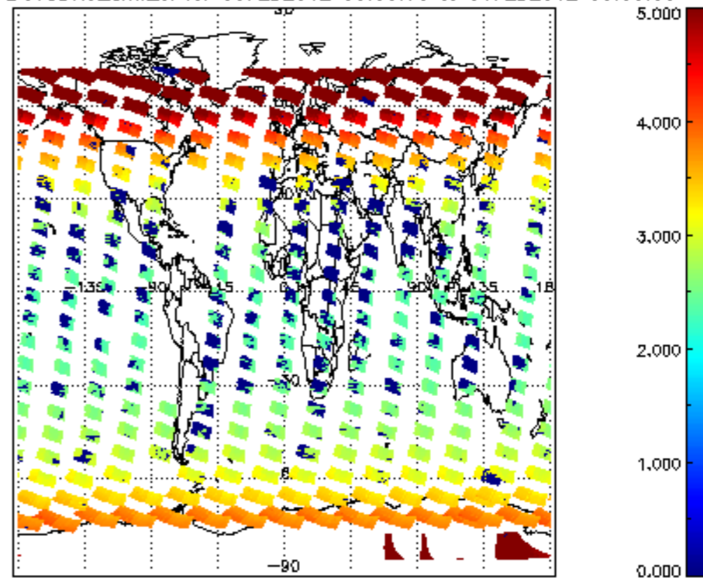
SCIOL2P_NADUV3BRO_amf_cl for 05FEB2012 00:00:00 to 06FEB2012 00:00:00
