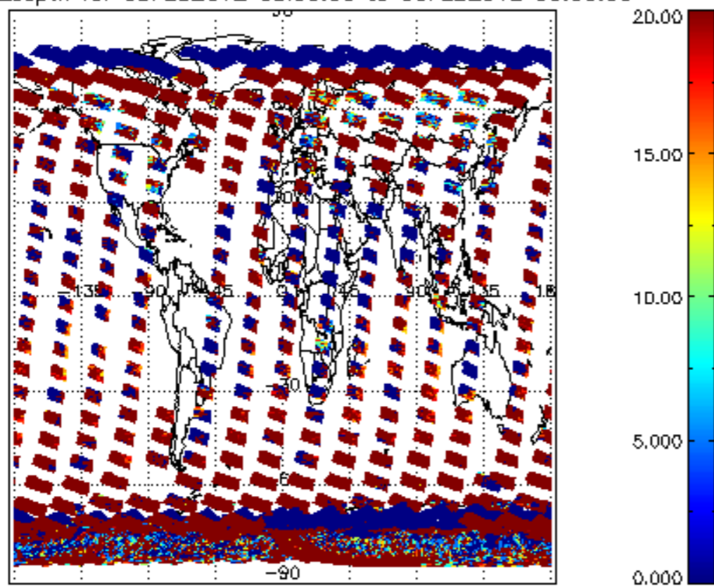
cl_opt_depth for 05FEB2012 00:00:00 to 06FEB2012 00:00:00
