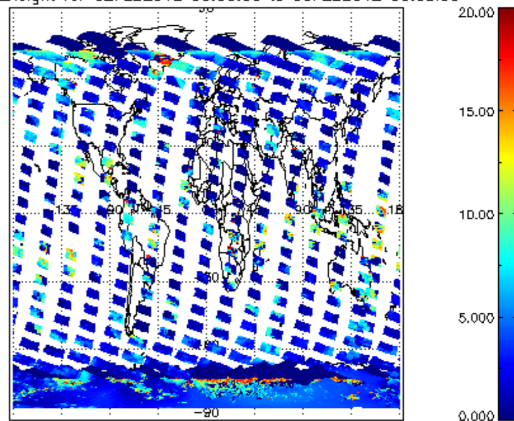
cl_top_height for 02FEB2012 00:00:00 to 03FEB2012 00:00:00
