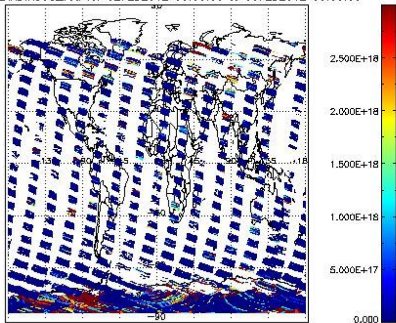
SCIDL2P_NADIR3CO_vcd for 02FEB2012 00:00:00 to 03FEB2012 00:00:00
