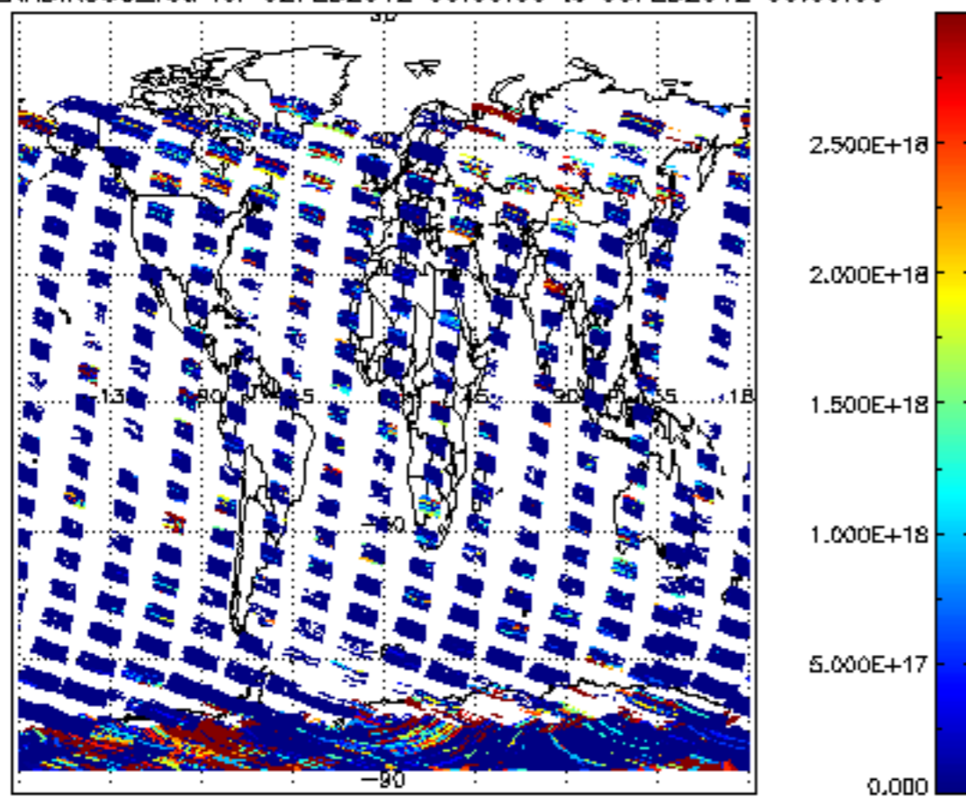
SCIOL2P_NADIR3CO_vcd for 02FEB2012 00:00:00 to 03FEB2012 00:00:00
