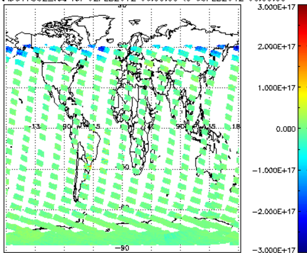
SCIOL2P_NADUV7S02_vcd for 02FEB2012 00:00:00 to 03FEB2012 00:00:00
