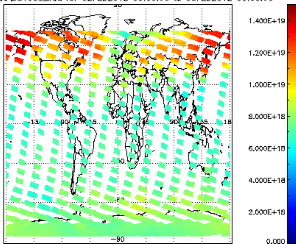
SCIOL2P_NADUV003_vcd for 02FEB2012 00:00:00 to 03FEB2012 00:00:00
