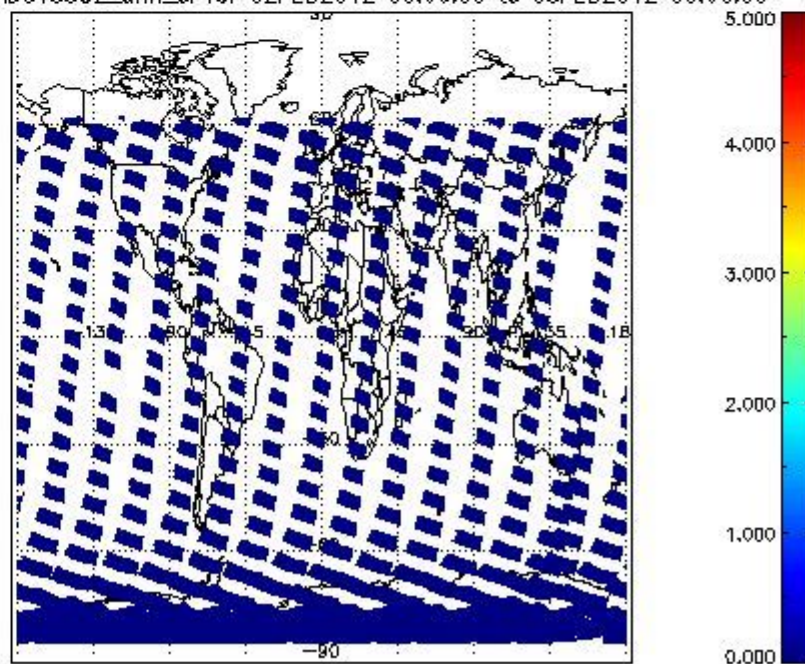
SCIOL2P_NADUV5SO2_amf_cl for 02FEB2012 00:00:00 to 03FEB2012 00:00:00
