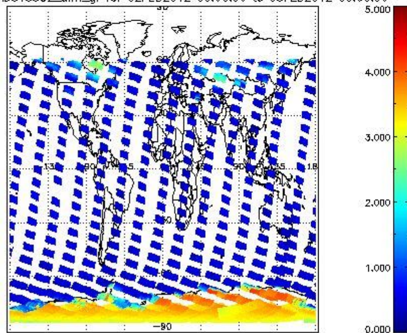
SCIOL2P_NADUV5SO2_amf_gr for 02FEB2012 00:00:00 to 03FEB2012 00:00:00
