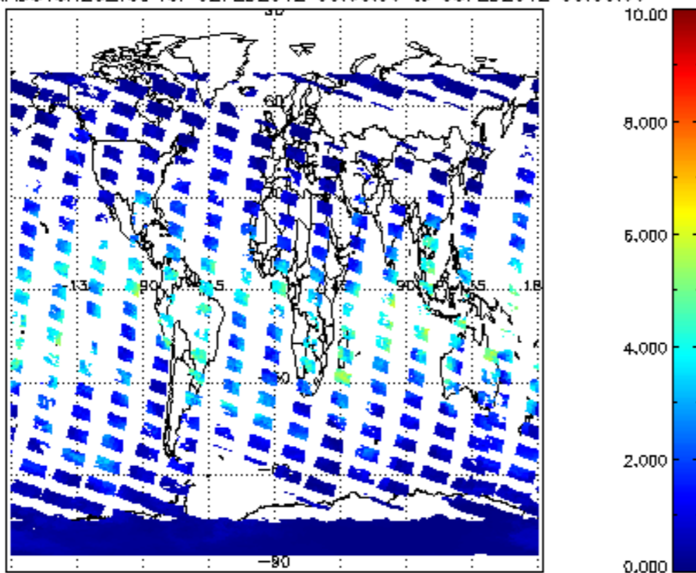
SCIOL2P_NADUV8H20_vcd for 02FEB2012 00:00:00 to 03FEB2012 00:00:00
