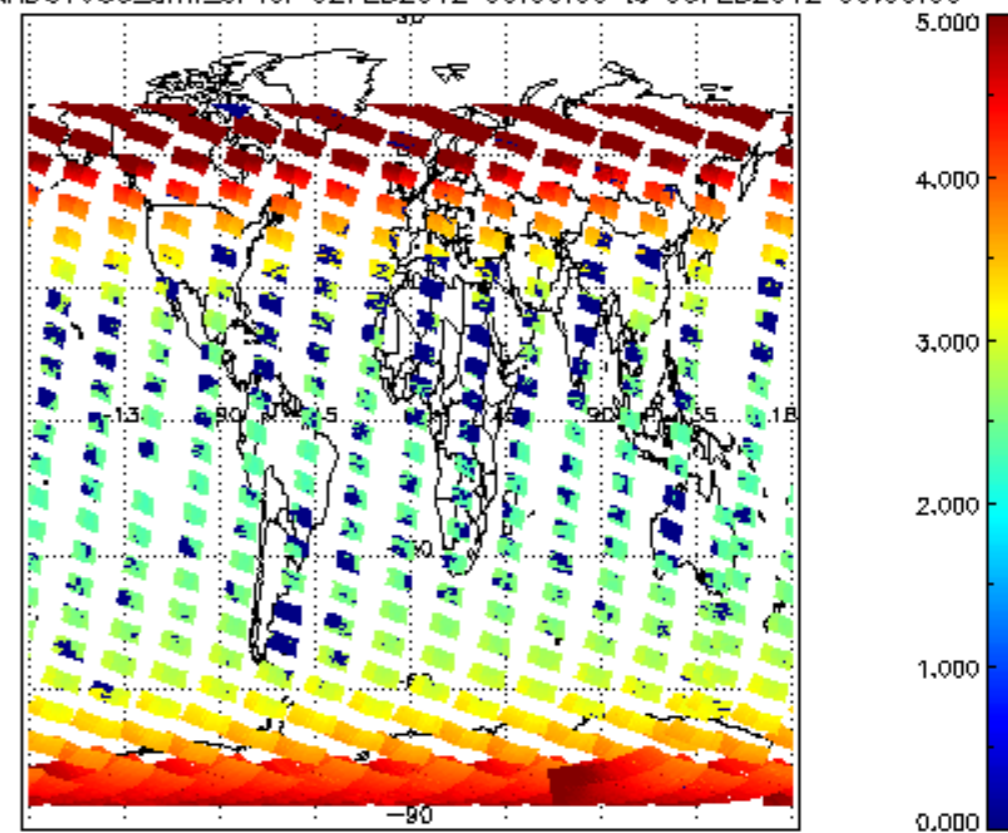
SCIOL2P_NADUV003_amf_cl for 02FEB2012 00:00:00 to 03FEB2012 00:00:00
