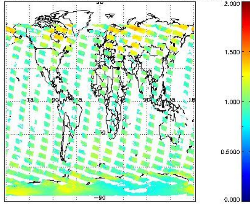
SCIOL2P_NADUV8H2O_amf_gr for 02FEB2012 00:00:00 to 03FEB2012 00:00:00
