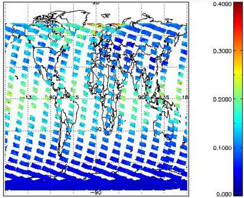
SCIOL2P_NADUV1N02_vcd_err for 02FEB2012 00:00:00 to 03FEB2012 00:00:00
