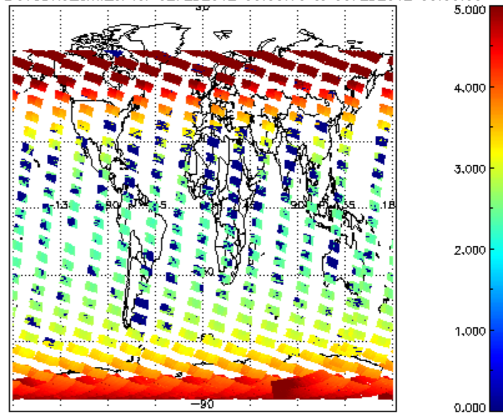
SCIOL2P_NADUV3BRO_amf_cl for 02FEB2012 00:00:00 to 03FEB2012 00:00:00
