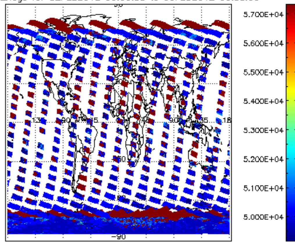
cloud_flags for 02FEB2012 00:00:00 to 03FEB2012 00:00:00
