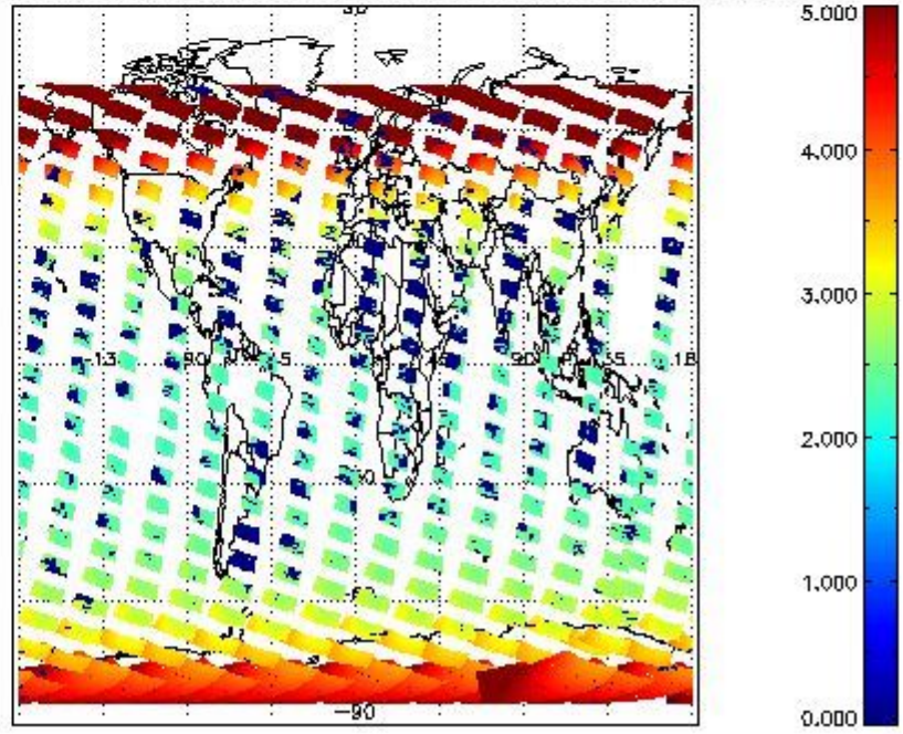
SCIOL2P_NADUV1N02_amf_cl for 02FEB2012 00:00:00 to 03FEB2012 00:00:00
