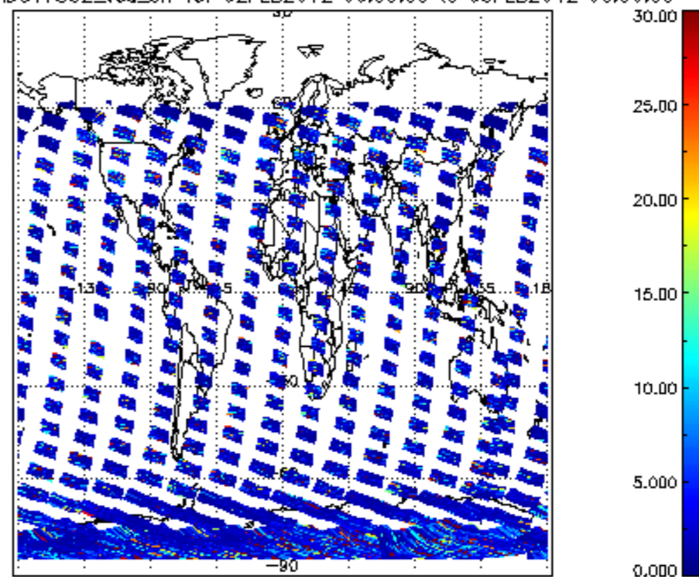
SCIOL2P_NADUV7S02_vcd_err for 02FEB2012 00:00:00 to 03FEB2012 00:00:00
