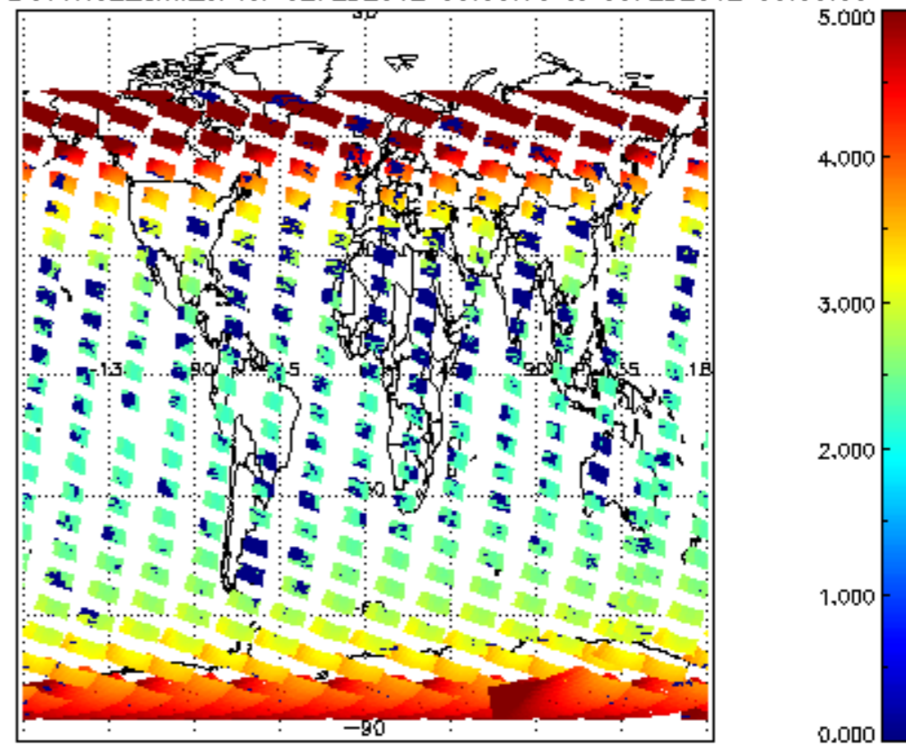
SCIOL2P_NADUV1N02_amf_cl for 02FEB2012 00:00:00 to 03FEB2012 00:00:00
