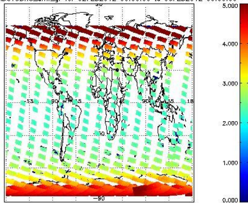
SCIOL2P_NADUV3BRO_amf_gr for 02FEB2012 00:00:00 to 03FEB2012 00:00:00
