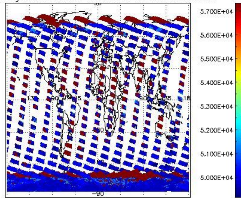
cloud_flags for 02FEB2012 00:00:00 to 03FEB2012 00:00:00
