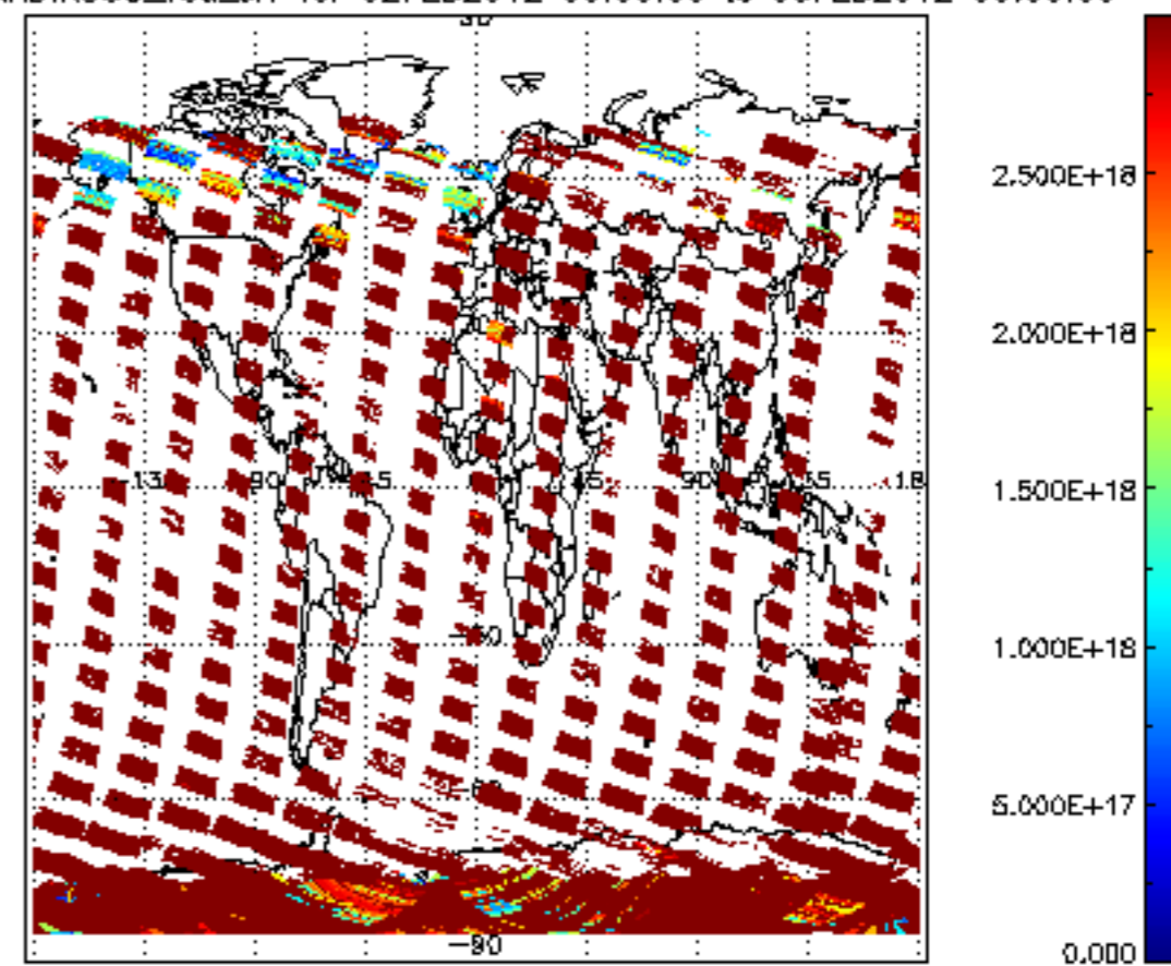
SCIOL2P_NADIR3CO_vcd_err for 02FEB2012 00:00:00 to 03FEB2012 00:00:00
