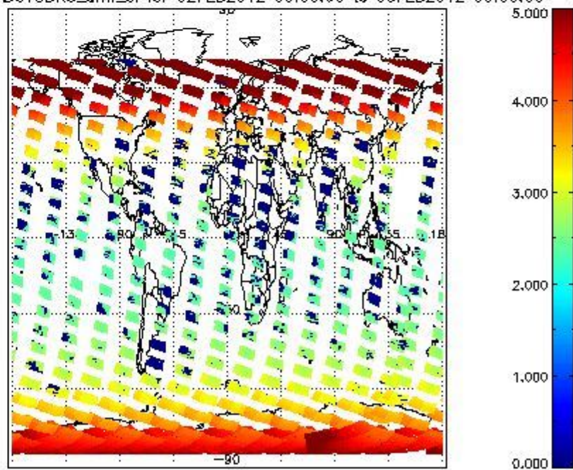
SCIOL2P_NADUV3BRO_amf_cl for 02FEB2012 00:00:00 to 03FEB2012 00:00:00
