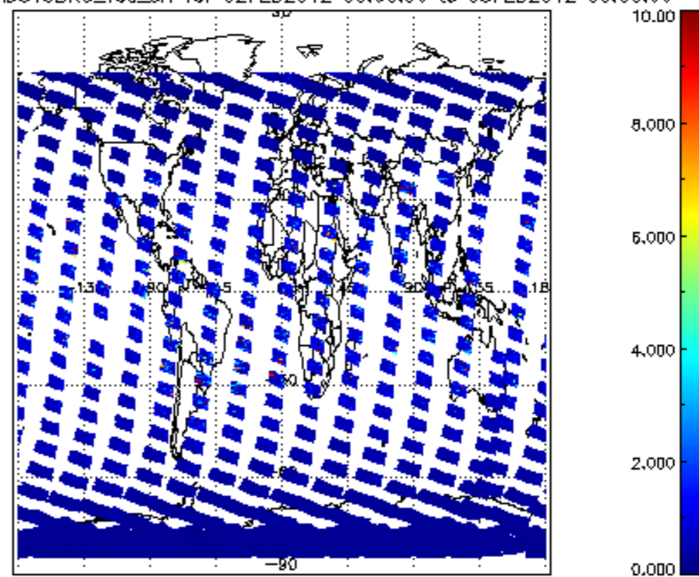
SCIOL2P_NADUV3BRO_vcd_err for 02FEB2012 00:00:00 to 03FEB2012 00:00:00
