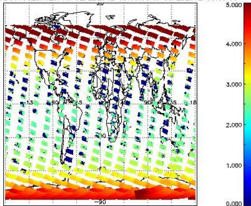
SCIOL2P_NADUV003_amf_cl for 02FEB2012 00:00:00 to 03FEB2012 00:00:00
