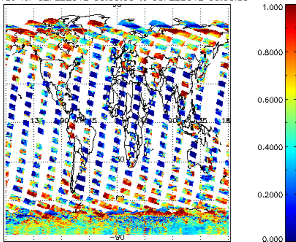
cl_frac for 02FEB2012 00:00:00 to 03FEB2012 00:00:00
