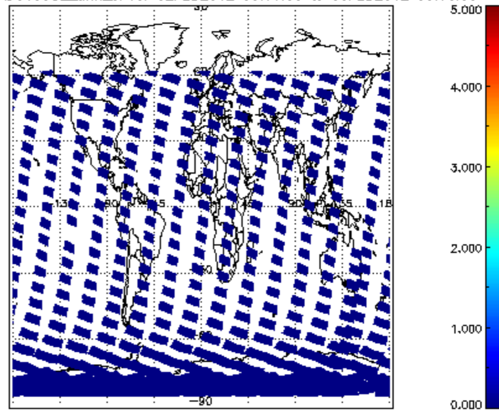
SCIOL2P_NADUV5S02_amf_cl for 02FEB2012 00:00:00 to 03FEB2012 00:00:00
