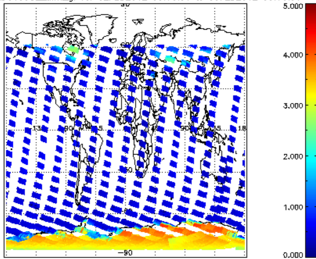
SCIOL2P_NADUV5S02_amf_gr for 02FEB2012 00:00:00 to 03FEB2012 00:00:00
