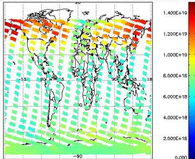
SCIOL2P_NADUV003_vcd for 02FEB2012 00:00:00 to 03FEB2012 00:00:00
