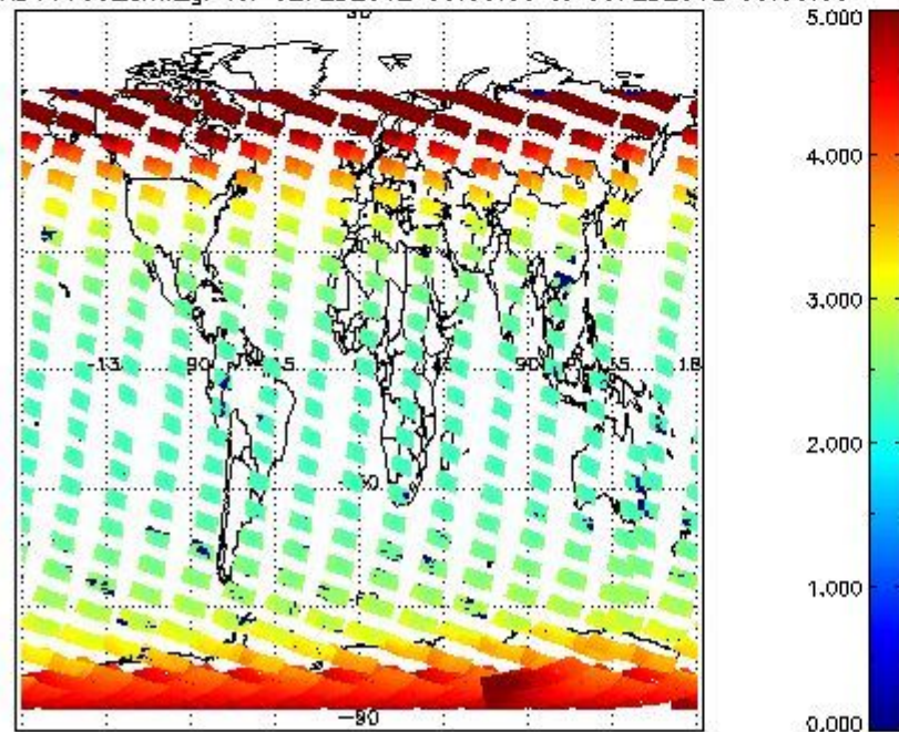
SCIOL2P_NADUV003_amf_gr for 02FEB2012 00:00:00 to 03FEB2012 00:00:00
