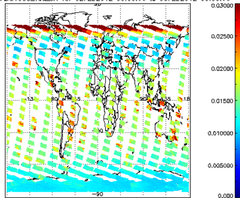
SCIOL2P_NADUV003_vcd_err for 02FEB2012 00:00:00 to 03FEB2012 00:00:00
