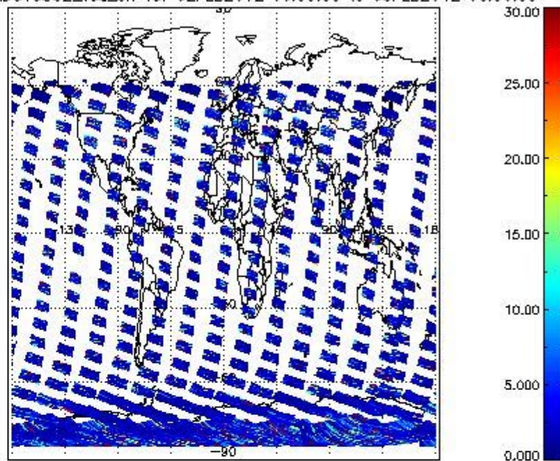
SCIOL2P_NADUV5SO2_vcd_err for 02FEB2012 00:00:00 to 03FEB2012 00:00:00
