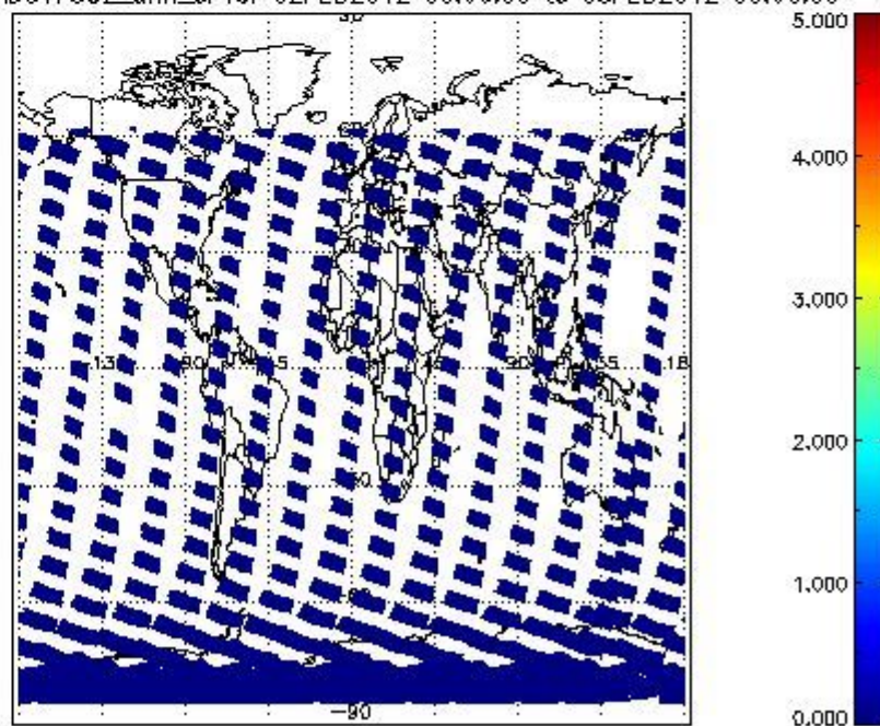
SCIOL2P_NADUV7S02_amf_cl for 02FEB2012 00:00:00 to 03FEB2012 00:00:00
