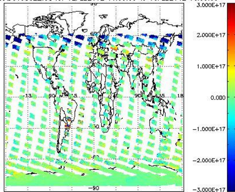
SCIOL2P_NADUV5SO2_vcd for 02FEB2012 00:00:00 to 03FEB2012 00:00:00
