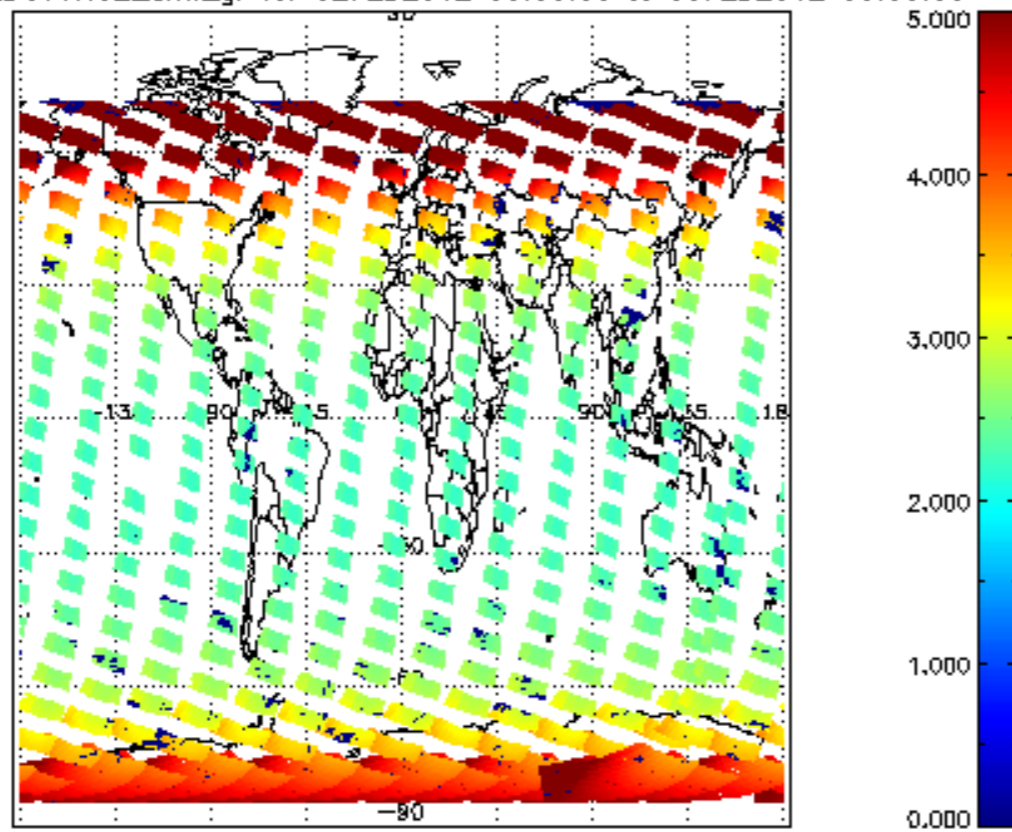
SCIOL2P_NADUV1N02_amf_gr for 02FEB2012 00:00:00 to 03FEB2012 00:00:00
