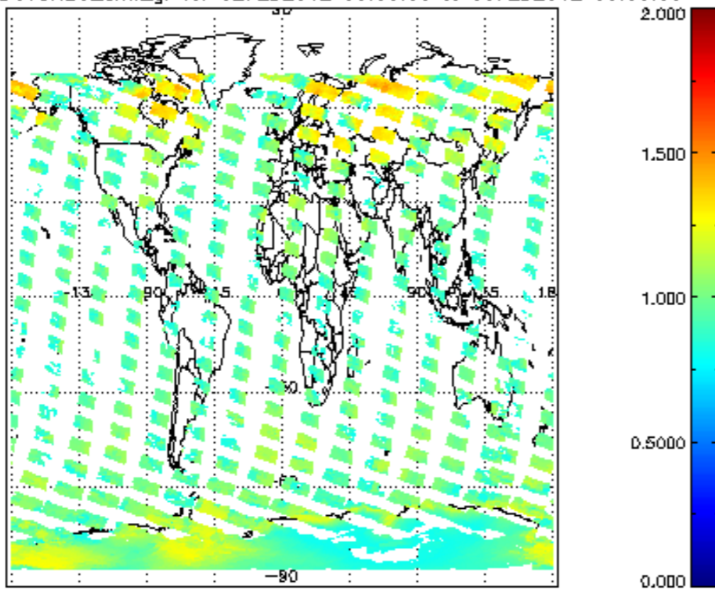
SCIOL2P_NADUV8H20_amf_gr for 02FEB2012 00:00:00 to 03FEB2012 00:00:00
