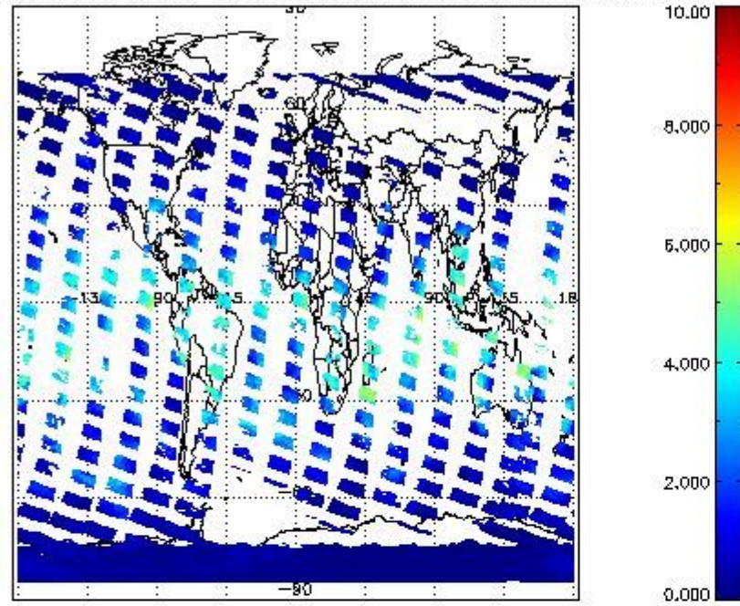
SCIOL2P_NADUV8H2O_vcd for 02FEB2012 00:00:00 to 03FEB2012 00:00:00
