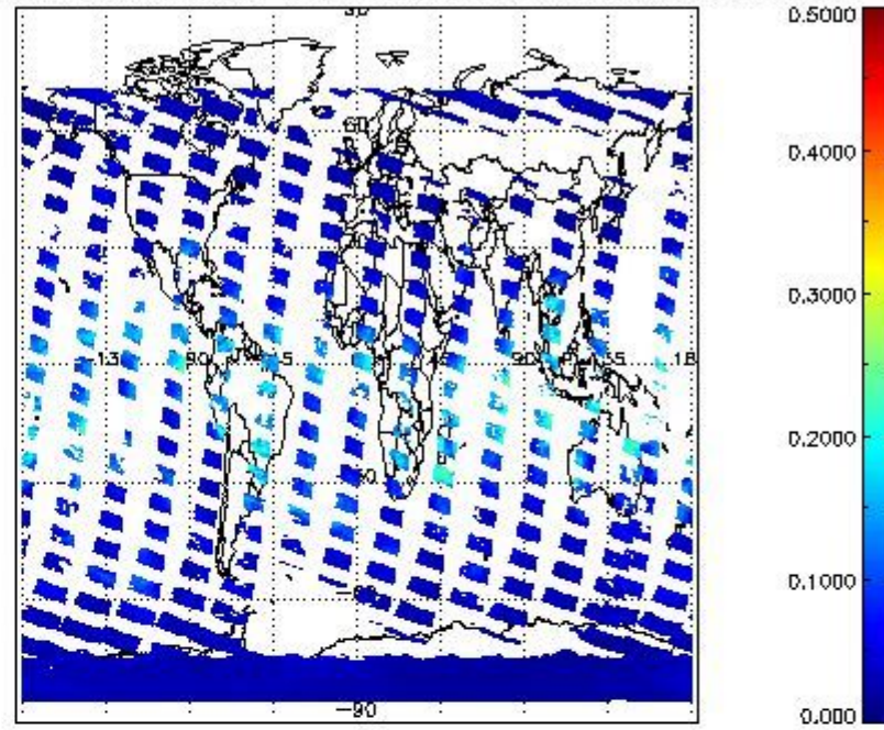
SCIOL2P_NADUV8H2O_vcd_err for 02FEB2012 00:00:00 to 03FEB2012 00:00:00
