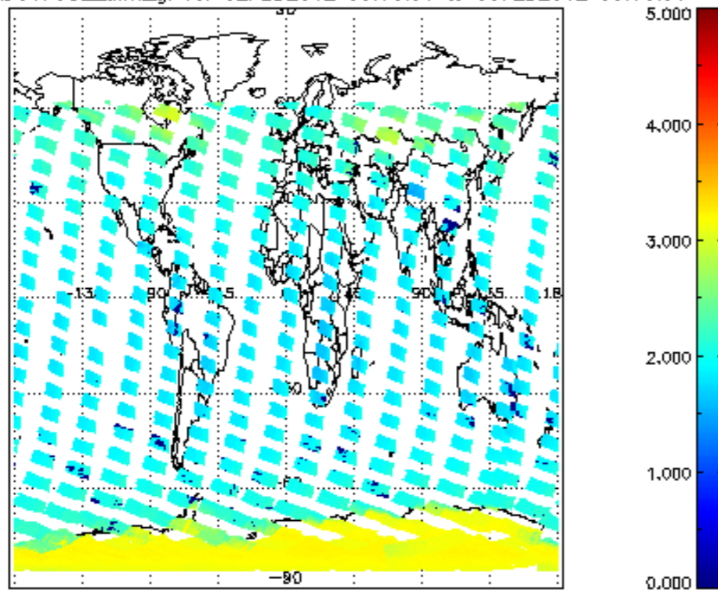
SCIOL2P_NADUV7S02_amf_gr for 02FEB2012 00:00:00 to 03FEB2012 00:00:00
