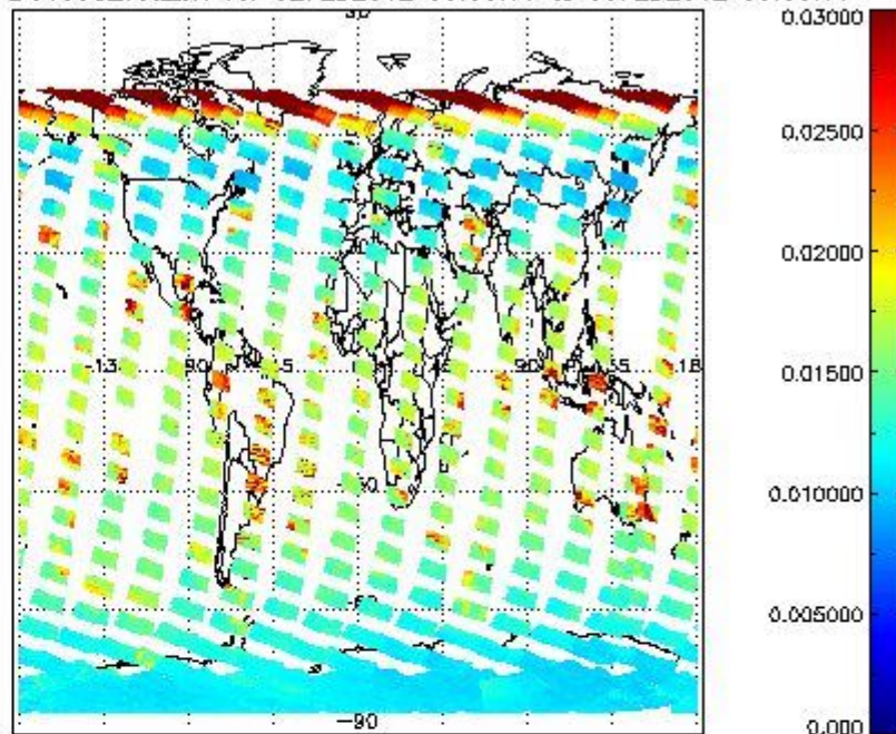
SCIOL2P_NADUV003_vcd_err for 02FEB2012 00:00:00 to 03FEB2012 00:00:00
