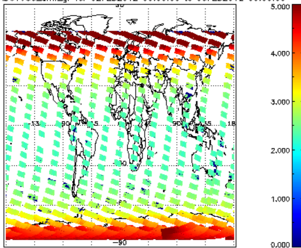
SCIOL2P_NADUV003_amf_gr for 02FEB2012 00:00:00 to 03FEB2012 00:00:00
