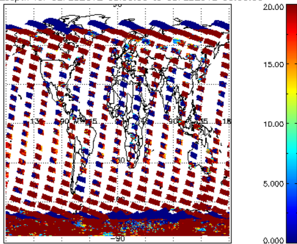
cl_opt_depth for 02FEB2012 00:00:00 to 03FEB2012 00:00:00
