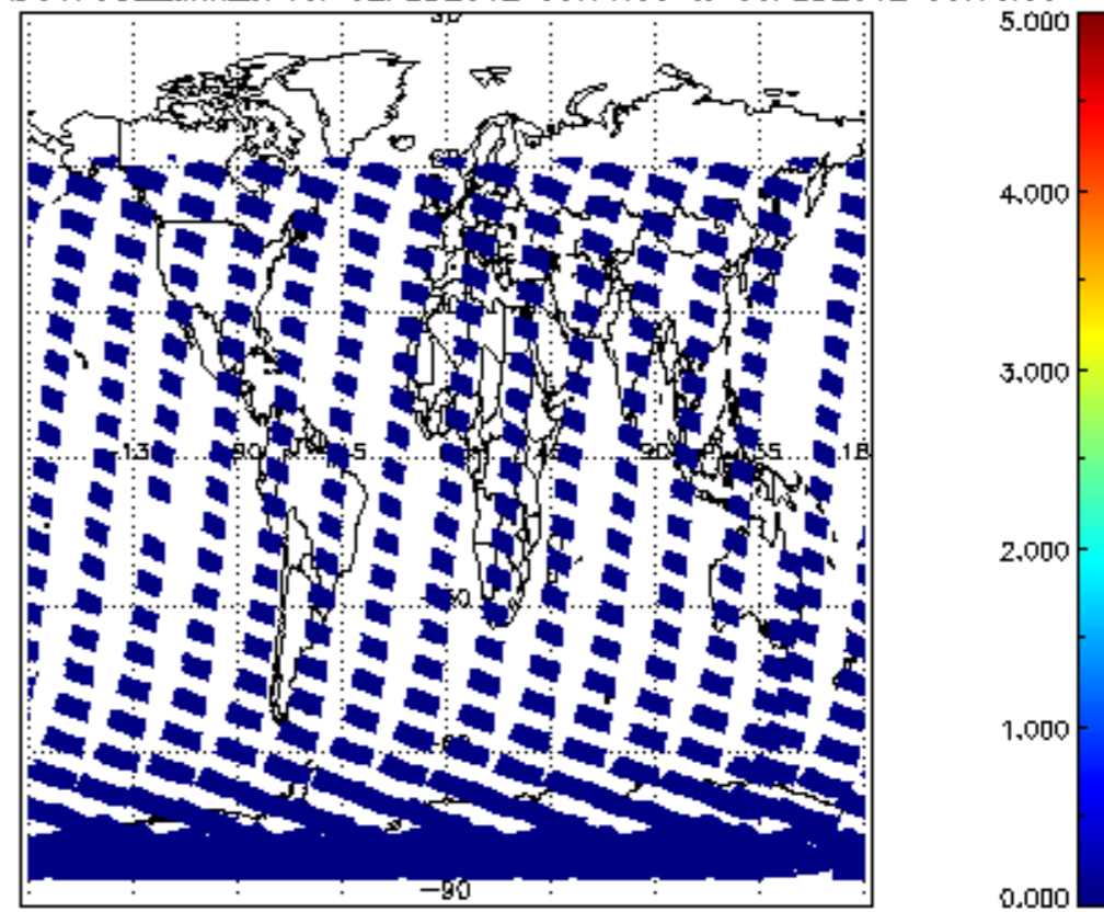
SCIOL2P_NADUV7S02_amf_cl for 02FEB2012 00:00:00 to 03FEB2012 00:00:00
