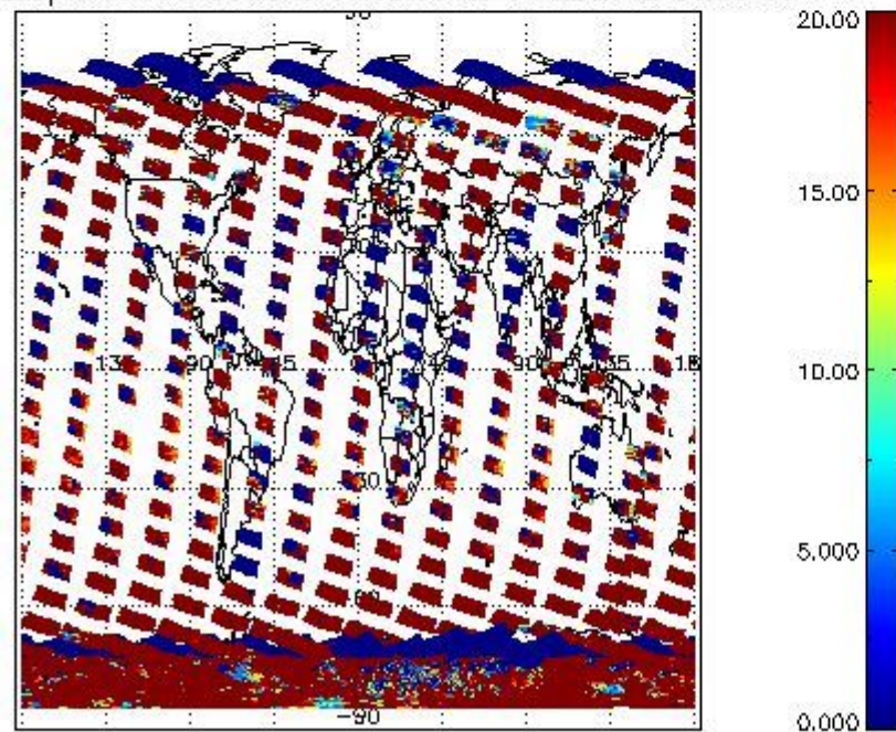
cL_opt_depth for 02FEB2012 00:00:00 to 03FEB2012 00:00:00
