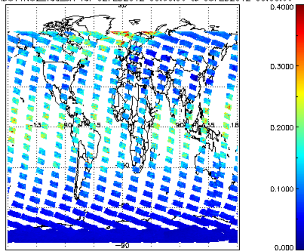
SCIOL2P_NADUV1N02_vcd_err for 02FEB2012 00:00:00 to 03FEB2012 00:00:00
