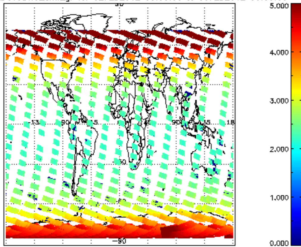
SCIOL2P_NADUV3BRO_amf_gr for 02FEB2012 00:00:00 to 03FEB2012 00:00:00
