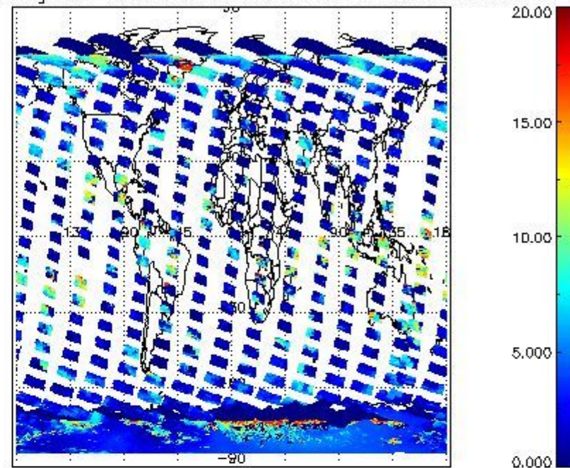
cL_top_height for 02FEB2012 00:00:00 to 03FEB2012 00:00:00
