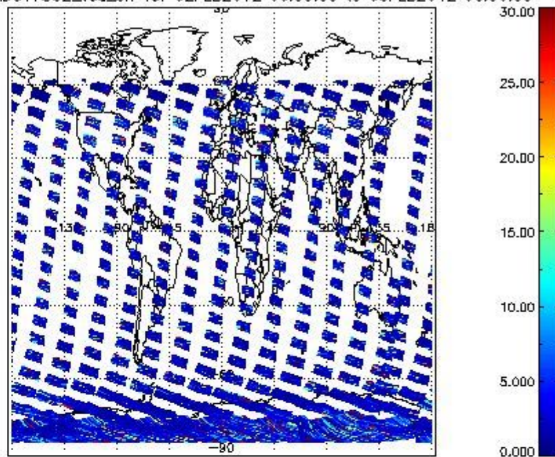
SCIOL2P_NADUV7S02_vcd_err for 02FEB2012 00:00:00 to 03FEB2012 00:00:00
