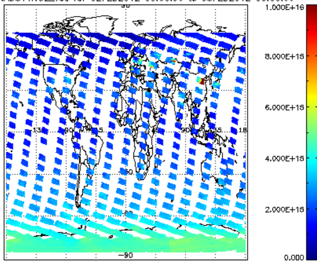
SCIOL2P_NADUV1N02_vcd for 02FEB2012 00:00:00 to 03FEB2012 00:00:00
