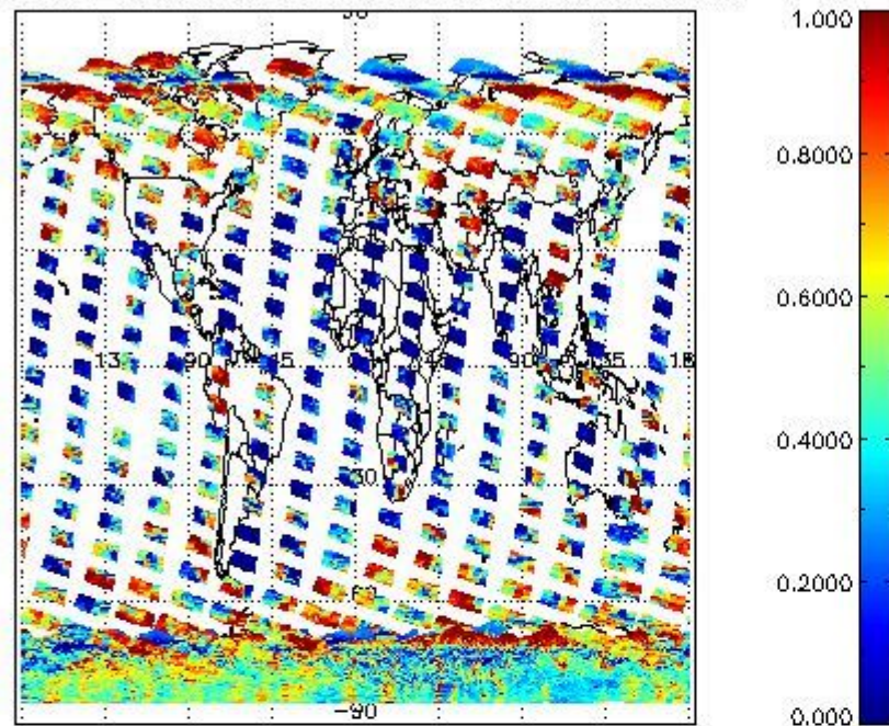
cL_frae for 02FEB2012 00:00:00 to 03FEB2012 00:00:00
