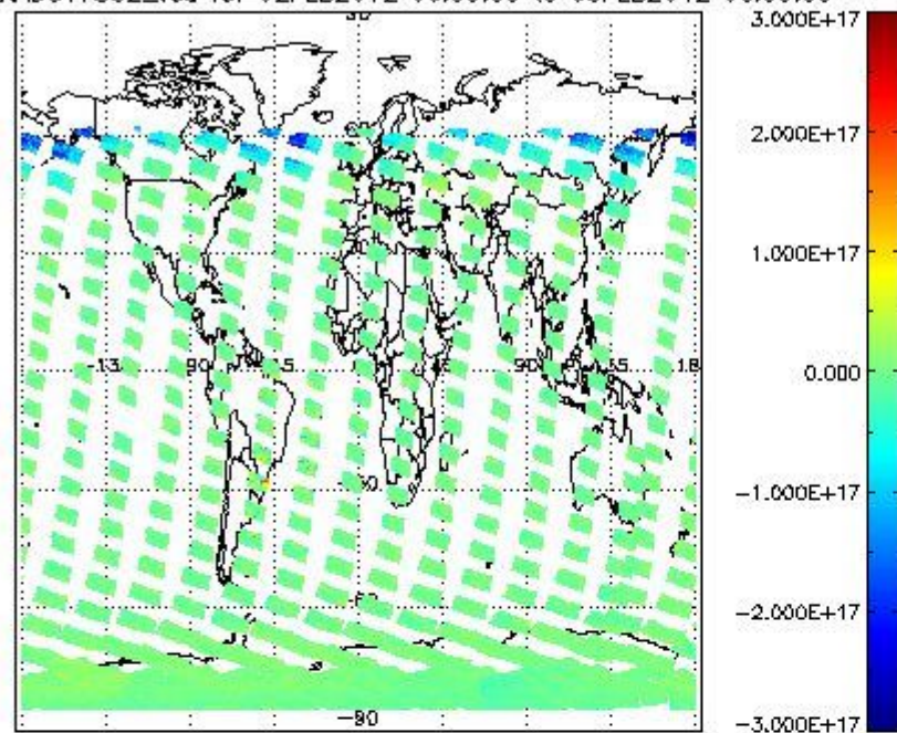
SCIOL2P_NADUV7S02_vcd for 02FEB2012 00:00:00 to 03FEB2012 00:00:00
