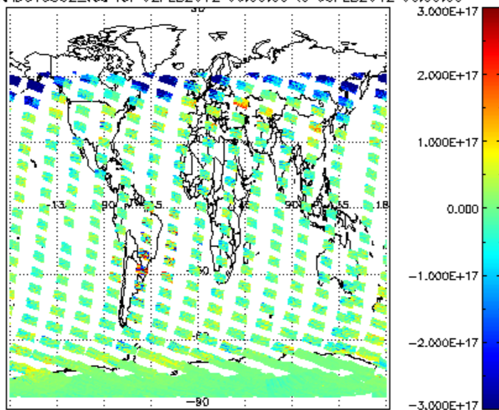
SCIOL2P_NADUV5S02_vcd for 02FEB2012 00:00:00 to 03FEB2012 00:00:00
