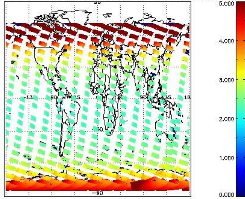
SCIOL2P_NADUV1N02_amf_gr for 02FEB2012 00:00:00 to 03FEB2012 00:00:00
