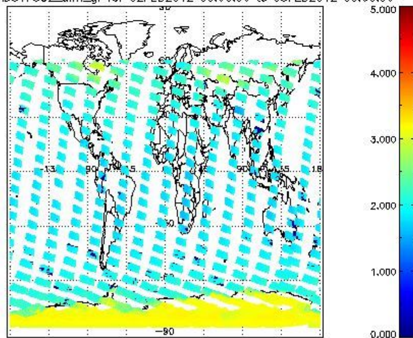
SCIOL2P_NADUV7S02_amf_gr for 02FEB2012 00:00:00 to 03FEB2012 00:00:00
