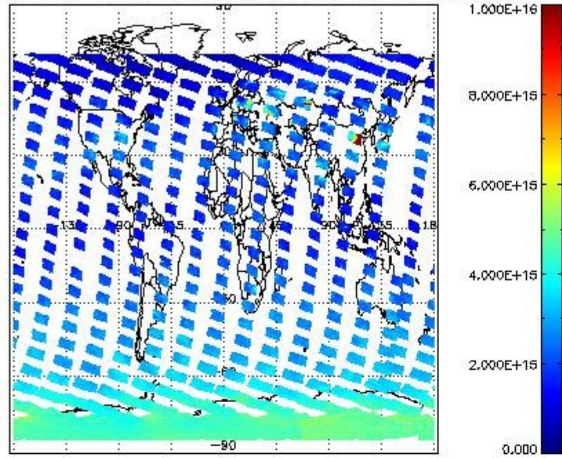
SCIOL2P_NADUV1N02_vcd for 02FEB2012 00:00:00 to 03FEB2012 00:00:00
