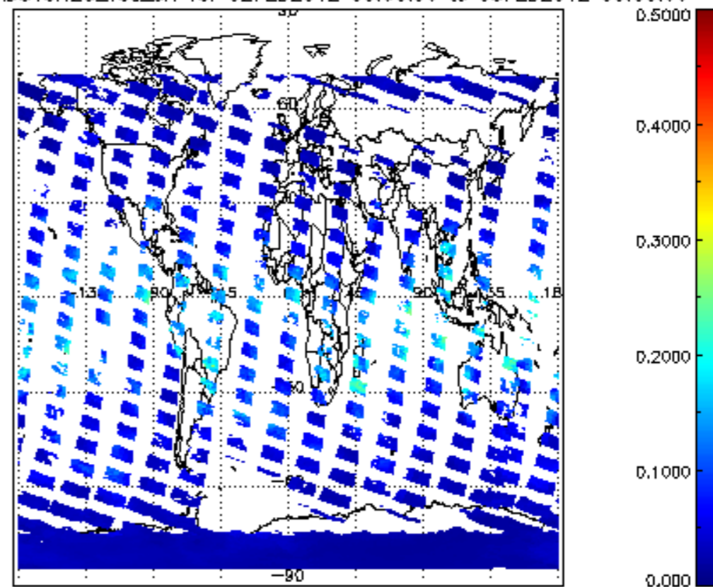
SCIOL2P_NADUV8H20_vcd_err for 02FEB2012 00:00:00 to 03FEB2012 00:00:00
