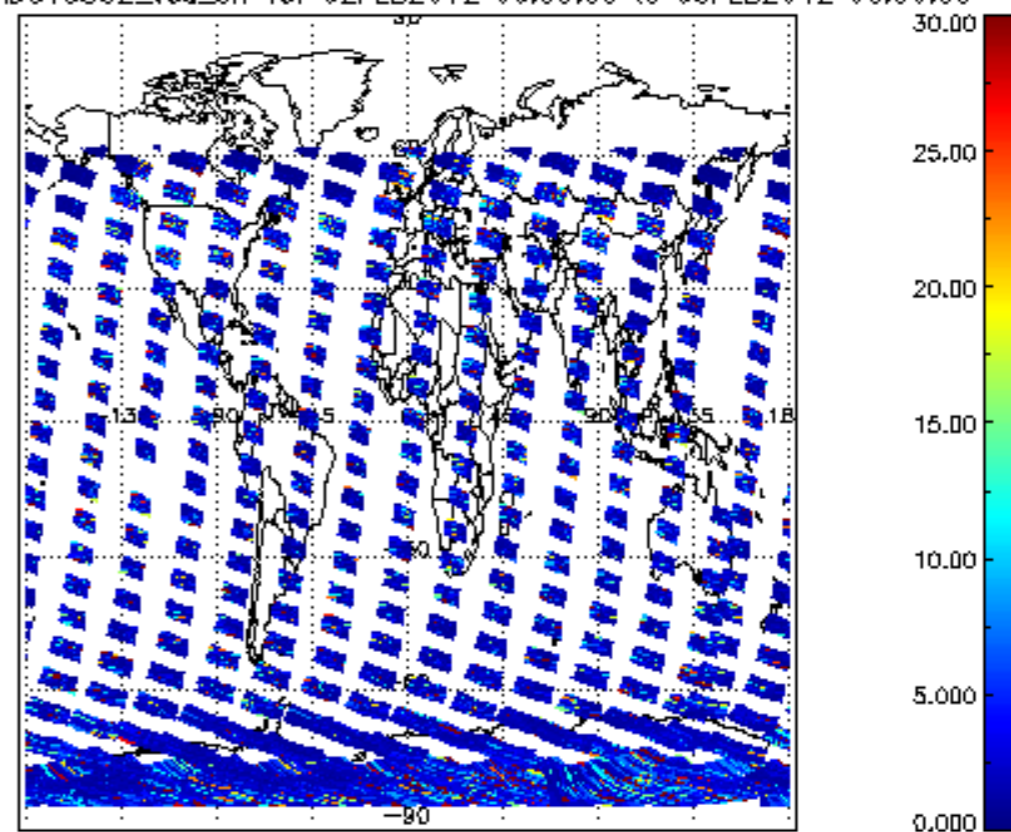
SCIOL2P_NADUV5S02_vcd_err for 02FEB2012 00:00:00 to 03FEB2012 00:00:00
