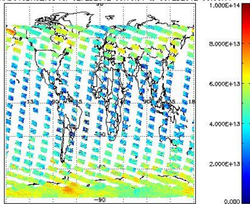
SCIOL2P_NADUV3BRO_vcd for 02FEB2012 00:00:00 to 03FEB2012 00:00:00
