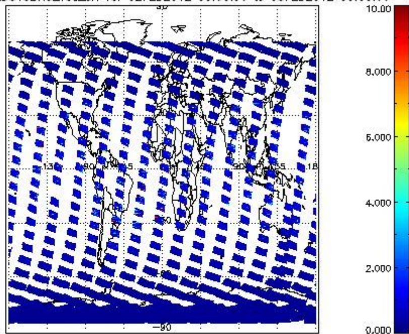
SCIOL2P_NADUV3BRO_vcd_err for 02FEB2012 00:00:00 to 03FEB2012 00:00:00
