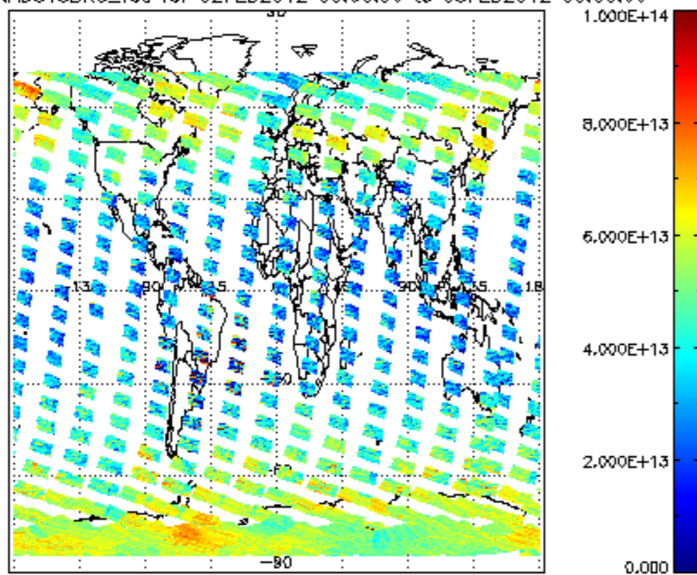
SCIOL2P_NADUV3BRO_vcd for 02FEB2012 00:00:00 to 03FEB2012 00:00:00
