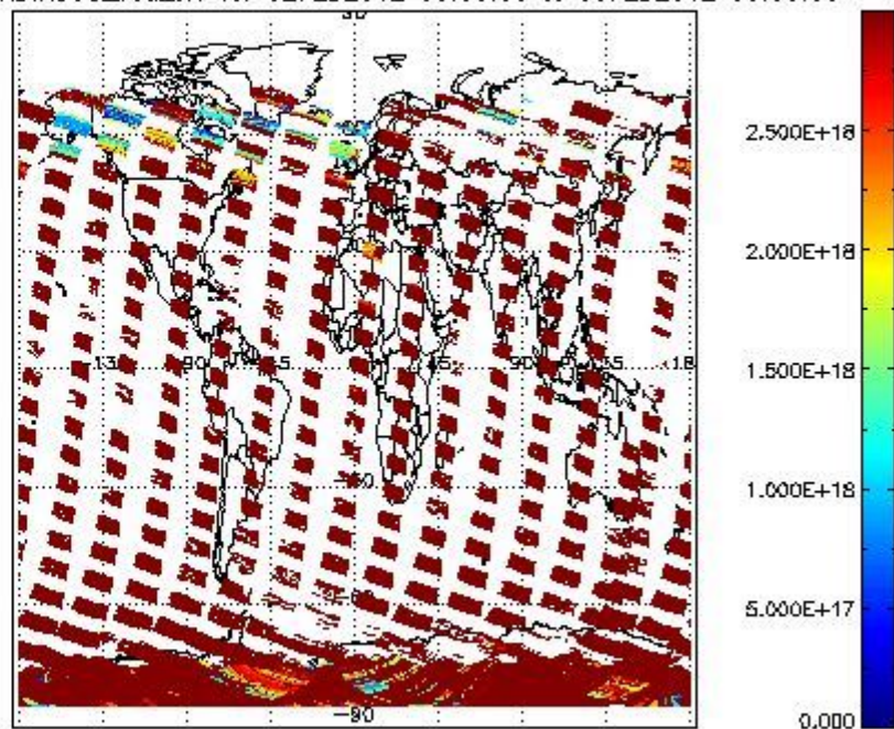
SCIDL2P_NADIR3CO_vcd_err for 02FEB2012 00:00:00 to 03FEB2012 00:00:00
