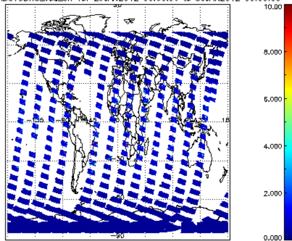
SCIOL2P_NADUV3BRO_vcd_err for 29JAN2012 00:00:00 to 30JAN2012 00:00:00
