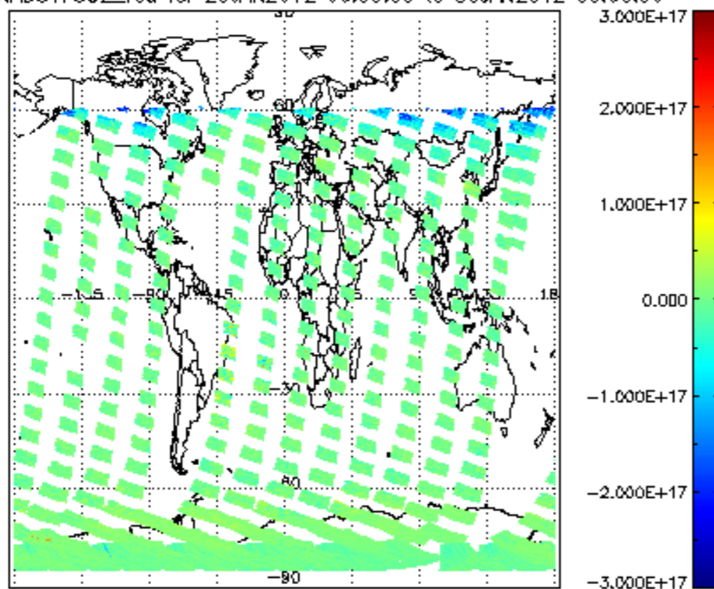
SCIOL2P_NADUV7S02_vcd for 29JAN2012 00:00:00 to 30JAN2012 00:00:00
