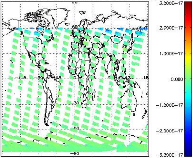
SCIOL2P_NADUV7S02_vcd for 29JAN2012 00:00:00 to 30JAN2012 00:00:00
