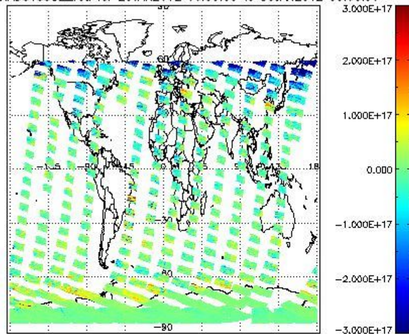
SCIOL2P_NADUV5SO2_vcd for 29JAN2012 00:00:00 to 30JAN2012 00:00:00
