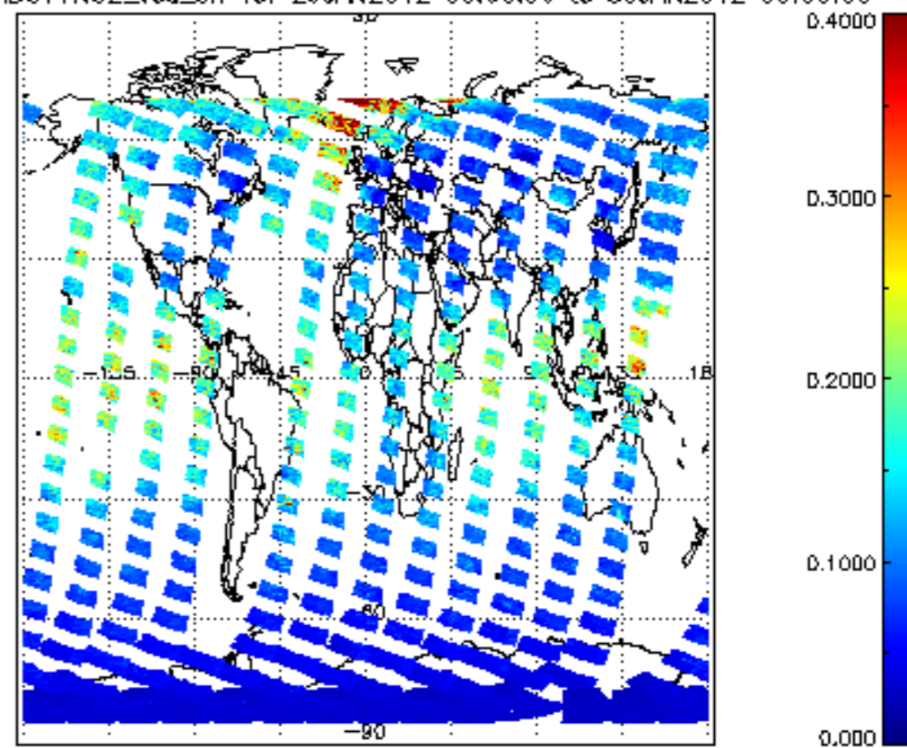
SCIOL2P_NADUV1NO2_vcd_err for 29JAN2012 00:00:00 to 30JAN2012 00:00:00
