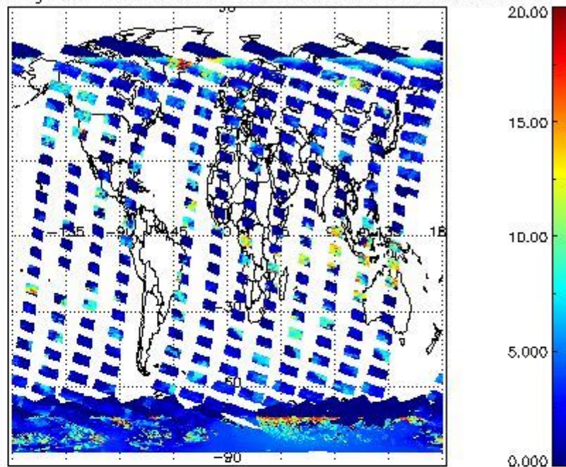
cL_top_height for 29JAN2012 00:00:00 to 30JAN2012 00:00:00
