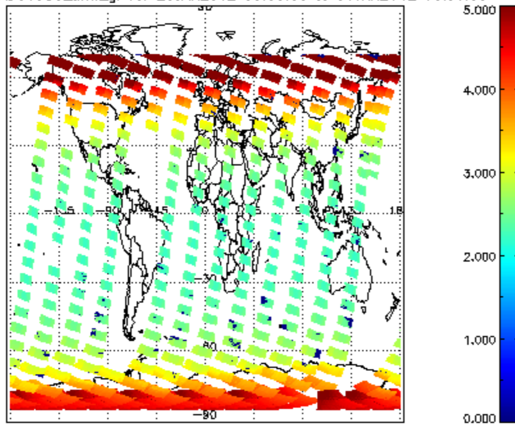
SCIOL2P_NADUV003_amf_gr for 29JAN2012 00:00:00 to 30JAN2012 00:00:00
