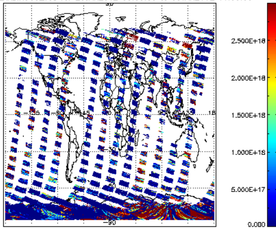
SCIOL2P_NADIR3CO_vcd for 29JAN2012 00:00:00 to 30JAN2012 00:00:00
