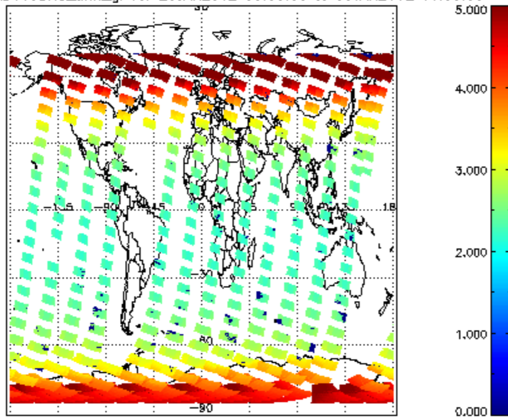
SCIOL2P_NADUV3BRO_amf_gr for 29JAN2012 00:00:00 to 30JAN2012 00:00:00
