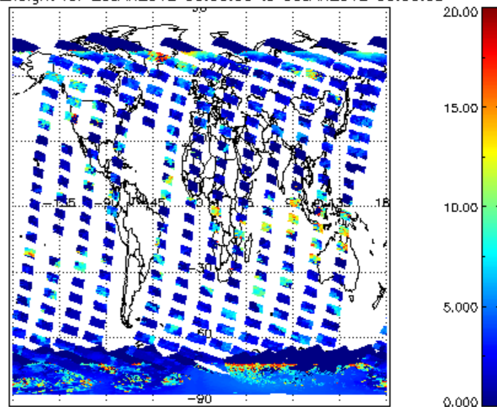
cL_top_height for 29JAN2012 00:00:00 to 30JAN2012 00:00:00
