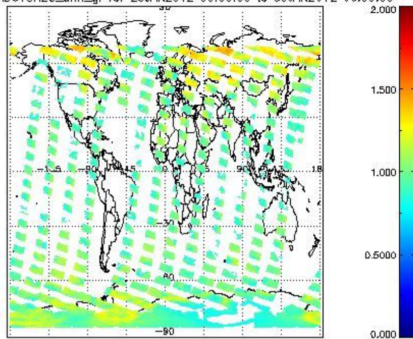
SCIOL2P_NADUV8H20_amf_gr for 29JAN2012 00:00:00 to 30JAN2012 00:00:00
