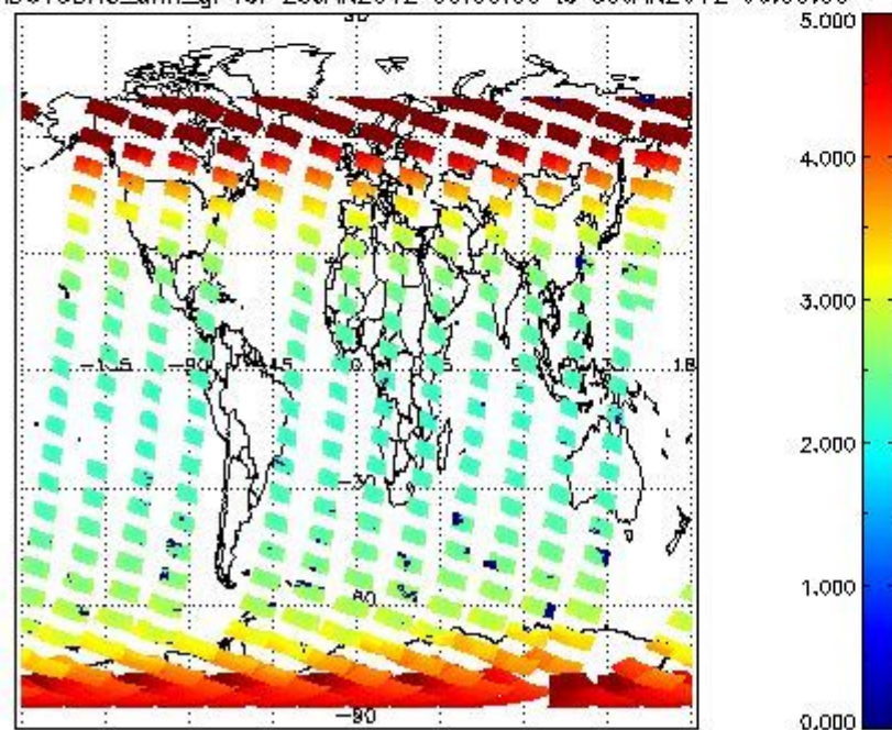
SCIOL2P_NADUV3BRO_amf_gr for 29JAN2012 00:00:00 to 30JAN2012 00:00:00
