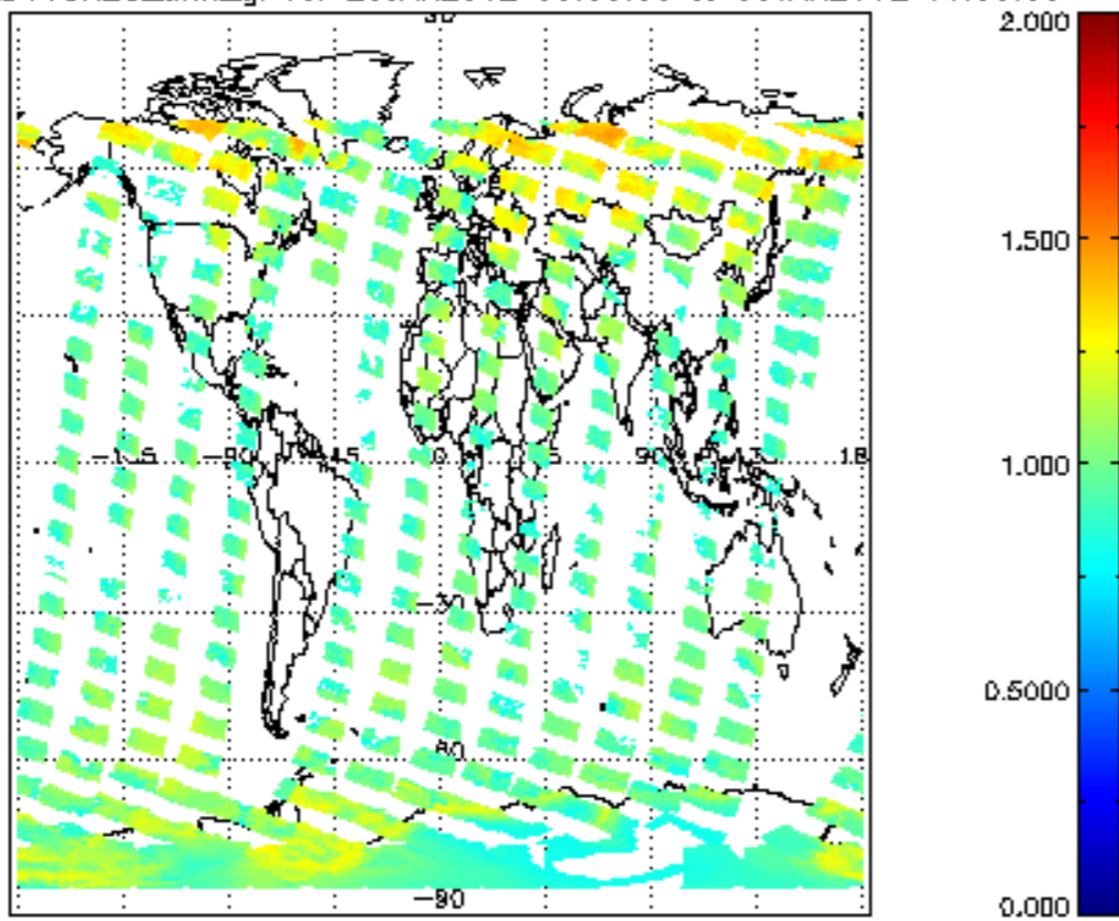
SCIOL2P_NADUV8H20_amf_gr for 29JAN2012 00:00:00 to 30JAN2012 00:00:00
