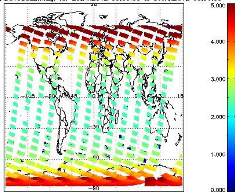
SCIOL2P_NADUV003_amf_gr for 29JAN2012 00:00:00 to 30JAN2012 00:00:00
