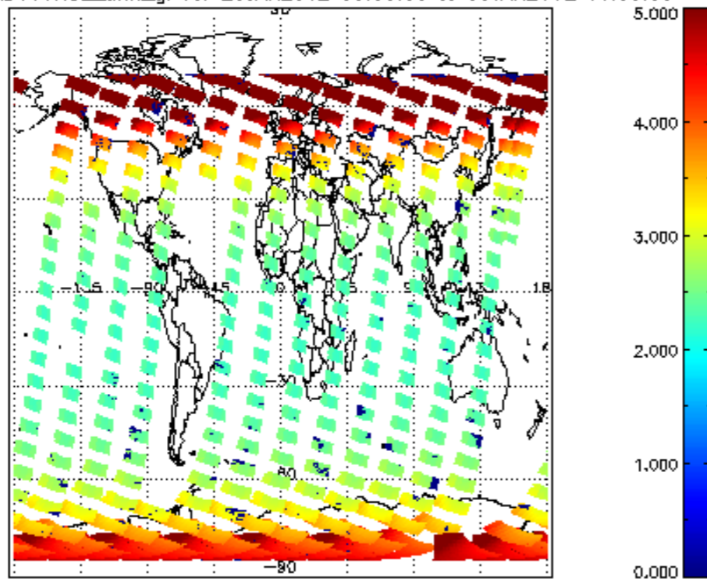
SCIOL2P_NADUV1NO2_amf_gr for 29JAN2012 00:00:00 to 30JAN2012 00:00:00
