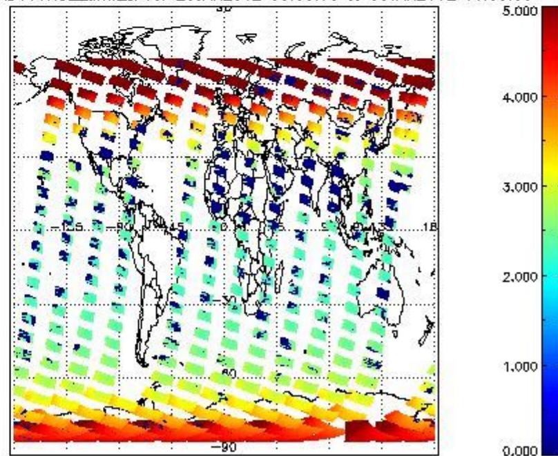
SCIOL2P_NADUV1NO2_amf_cl for 29JAN2012 00:00:00 to 30JAN2012 00:00:00
