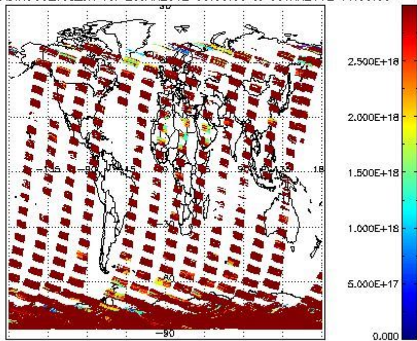
SCIDL2P_NADIR3CO_vcd_err for 29JAN2012 00:00:00 to 30JAN2012 00:00:00
