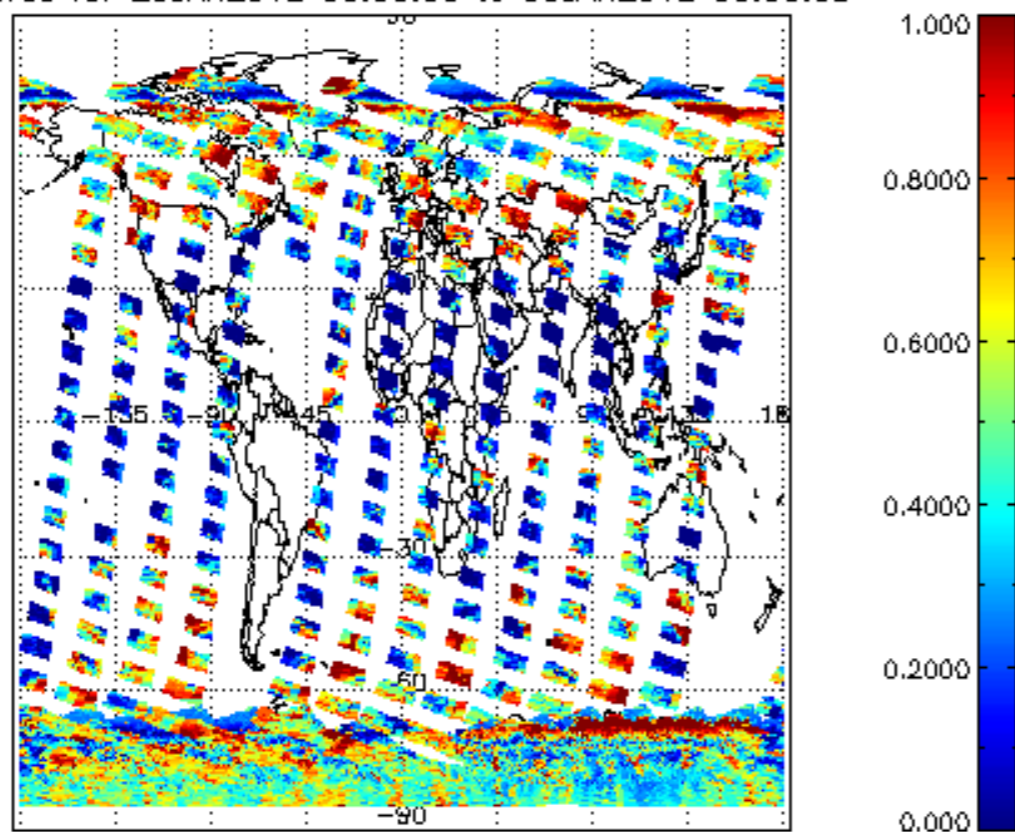
cL_frac for 29JAN2012 00:00:00 to 30JAN2012 00:00:00
