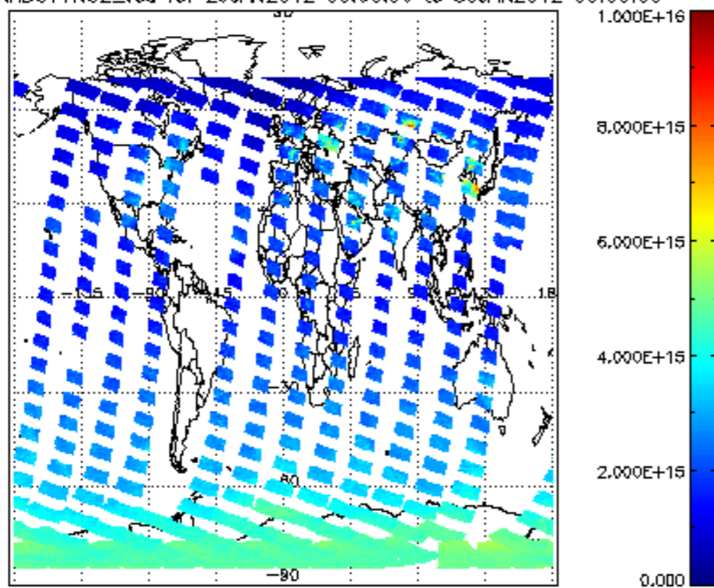
SCIOL2P_NADUV1NO2_vcd for 29JAN2012 00:00:00 to 30JAN2012 00:00:00
