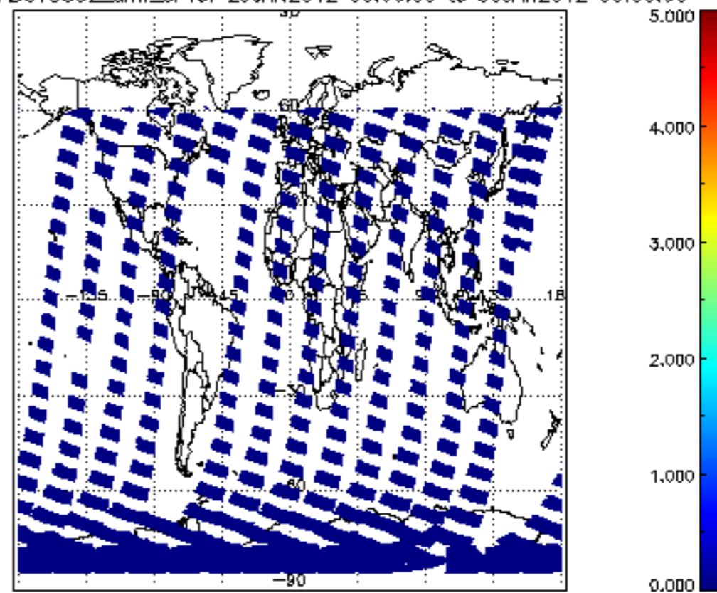
SCIOL2P_NADUV5S02_amf_cl for 29JAN2012 00:00:00 to 30JAN2012 00:00:00
