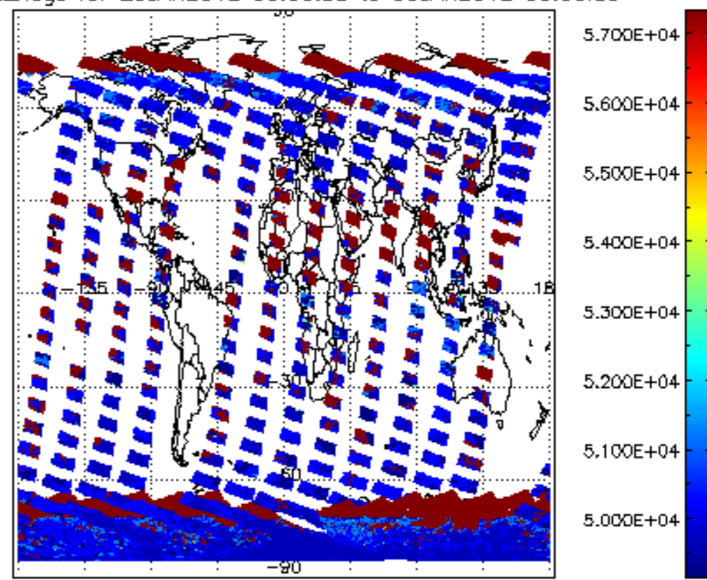
cloud_flags for 29JAN2012 00:00:00 to 30JAN2012 00:00:00
