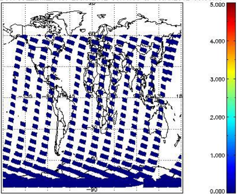
SCIOL2P_NADUV7S02_amf_cl for 29JAN2012 00:00:00 to 30JAN2012 00:00:00
