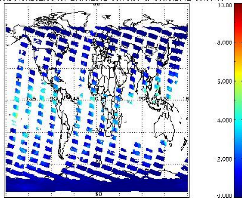
SCIOL2P_NADUV8H20_vcd for 29JAN2012 00:00:00 to 30JAN2012 00:00:00
