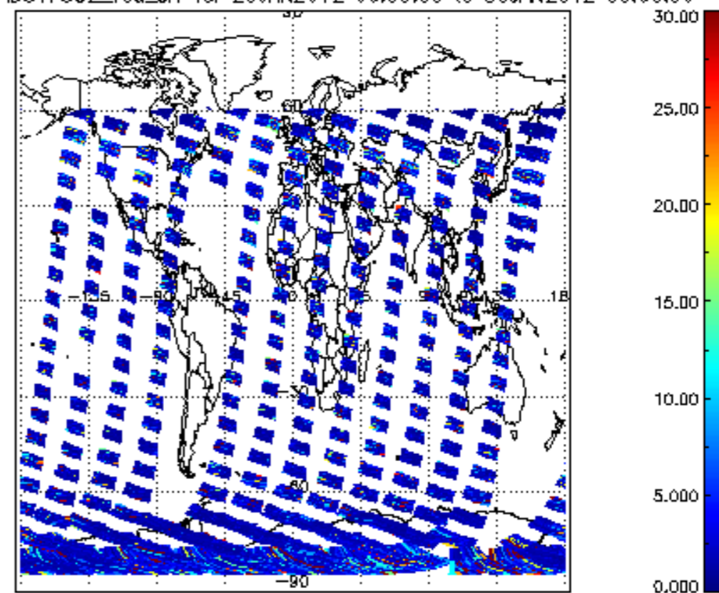
SCIOL2P_NADUV7S02_vcd_err for 29JAN2012 00:00:00 to 30JAN2012 00:00:00
