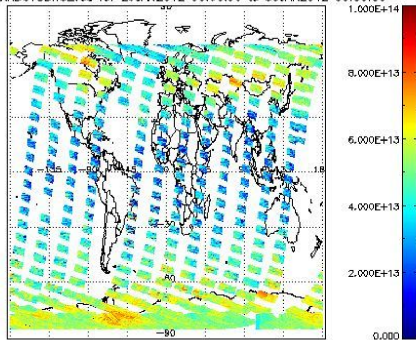
SCIOL2P_NADUV3BRO_vcd for 29JAN2012 00:00:00 to 30JAN2012 00:00:00
