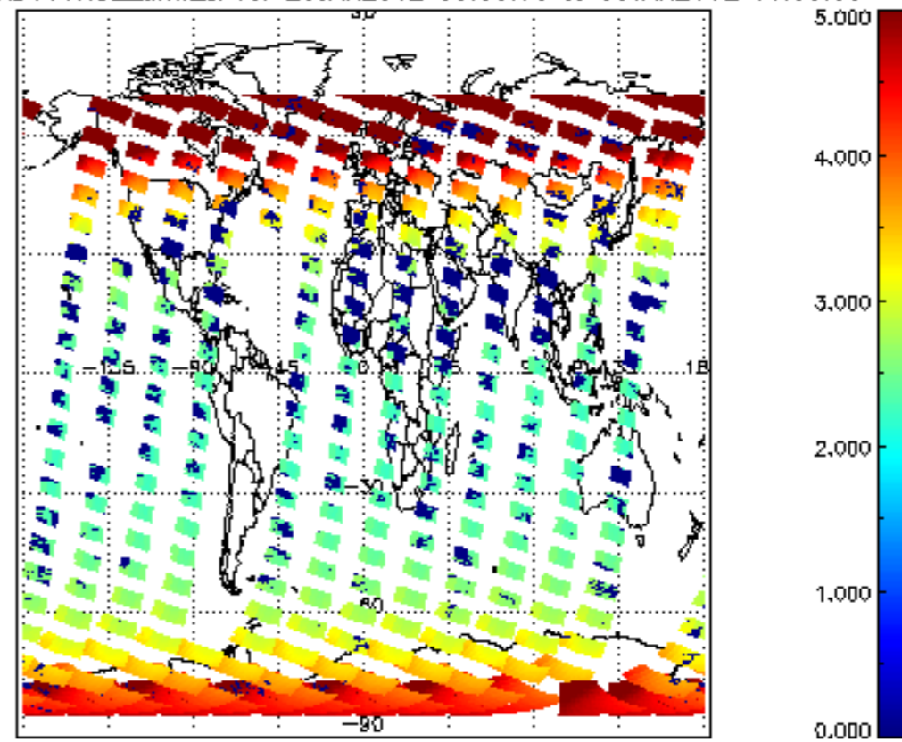
SCIOL2P_NADUV1NO2_amf_cl for 29JAN2012 00:00:00 to 30JAN2012 00:00:00
