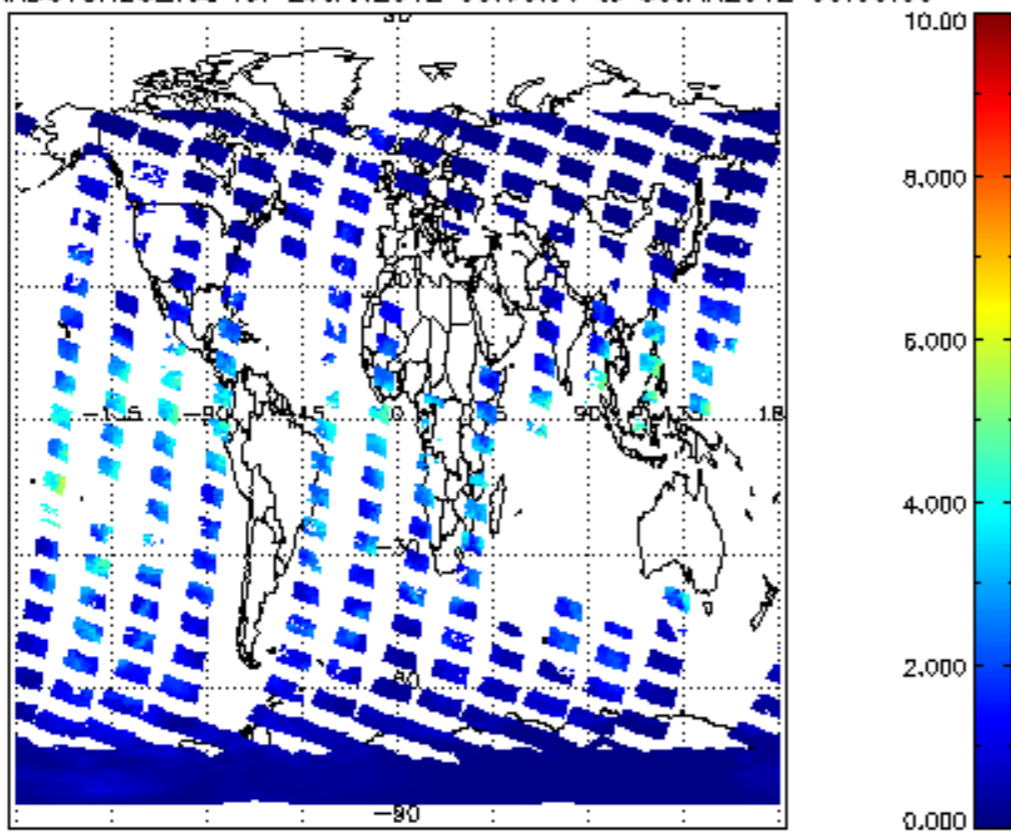
SCIOL2P_NADUV8H20_vcd for 29JAN2012 00:00:00 to 30JAN2012 00:00:00
