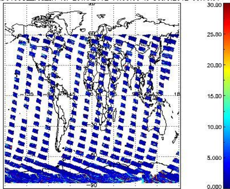
SCIOL2P_NADUV5SO2_vcd_err for 29JAN2012 00:00:00 to 30JAN2012 00:00:00
