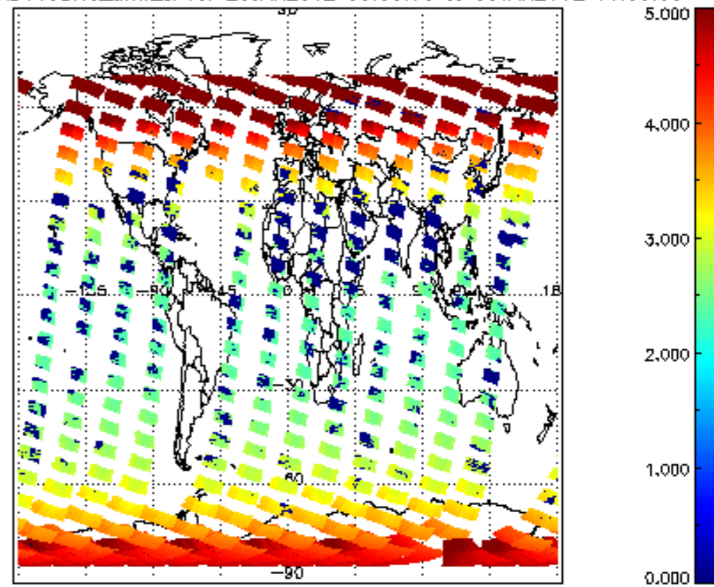
SCIOL2P_NADUV3BRO_amf_cl for 29JAN2012 00:00:00 to 30JAN2012 00:00:00
