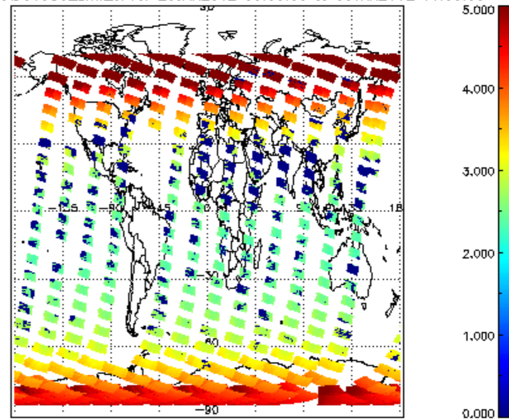
SCIOL2P_NADUV003_amf_cl for 29JAN2012 00:00:00 to 30JAN2012 00:00:00
