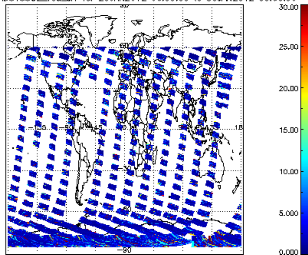
SCIOL2P_NADUV5S02_vcd_err for 29JAN2012 00:00:00 to 30JAN2012 00:00:00
