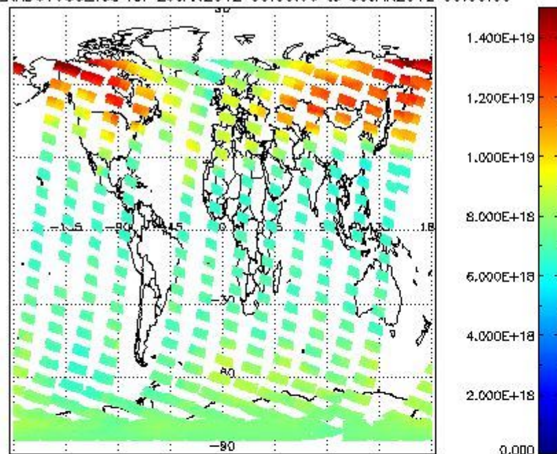
SCIOL2P_NADUV003_vcd for 29JAN2012 00:00:00 to 30JAN2012 00:00:00
