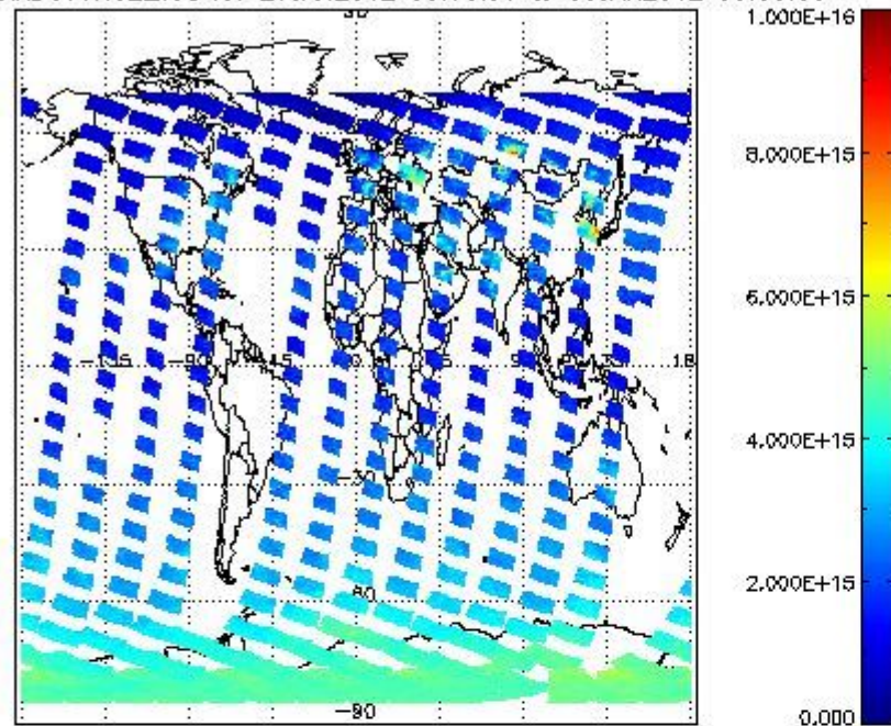
SCIOL2P_NADUV1NO2_vcd for 29JAN2012 00:00:00 to 30JAN2012 00:00:00
