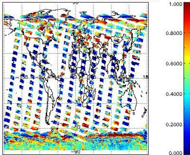
cL_frac for 29JAN2012 00:00:00 to 30JAN2012 00:00:00
