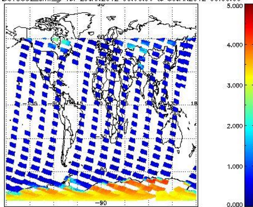
SCIOL2P_NADUV5SO2_amf_gr for 29JAN2012 00:00:00 to 30JAN2012 00:00:00
