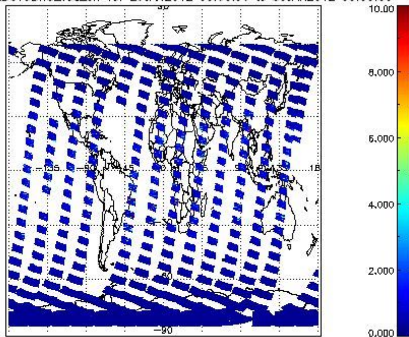
SCIOL2P_NADUV3BRO_vcd_err for 29JAN2012 00:00:00 to 30JAN2012 00:00:00
