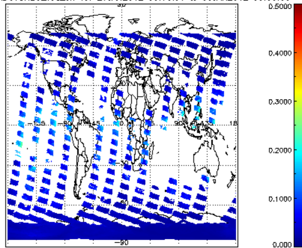
SCIOL2P_NADUV8H20_vcd_err for 29JAN2012 00:00:00 to 30JAN2012 00:00:00
