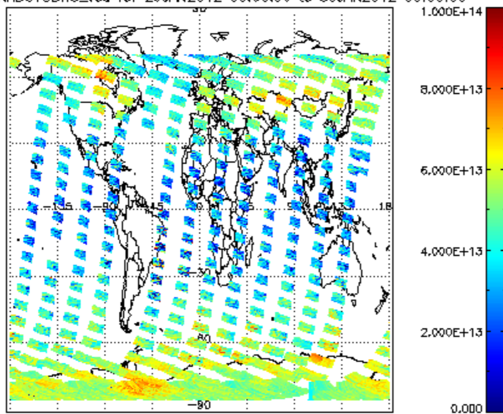
SCIOL2P_NADUV3BRO_vcd for 29JAN2012 00:00:00 to 30JAN2012 00:00:00
