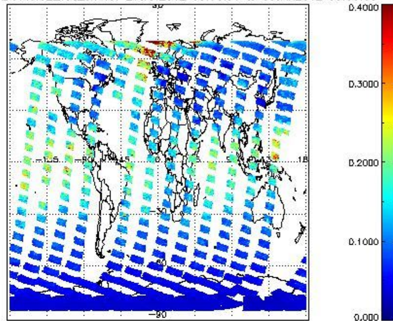
SCIOL2P_NADUV1NO2_vcd_err for 29JAN2012 00:00:00 to 30JAN2012 00:00:00
