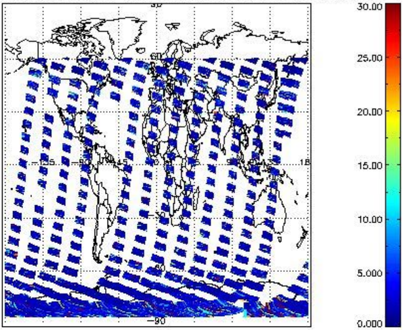
SCIOL2P_NADUV7S02_vcd_err for 29JAN2012 00:00:00 to 30JAN2012 00:00:00
