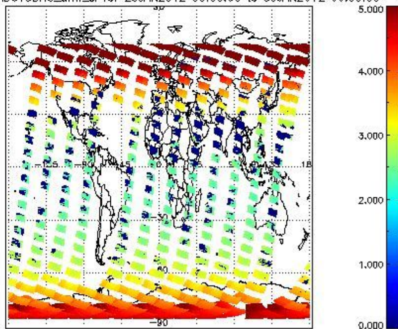
SCIOL2P_NADUV3BRO_amf_cl for 29JAN2012 00:00:00 to 30JAN2012 00:00:00
