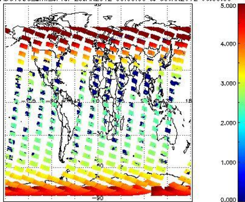
SCIOL2P_NADUV003_amf_cl for 29JAN2012 00:00:00 to 30JAN2012 00:00:00
