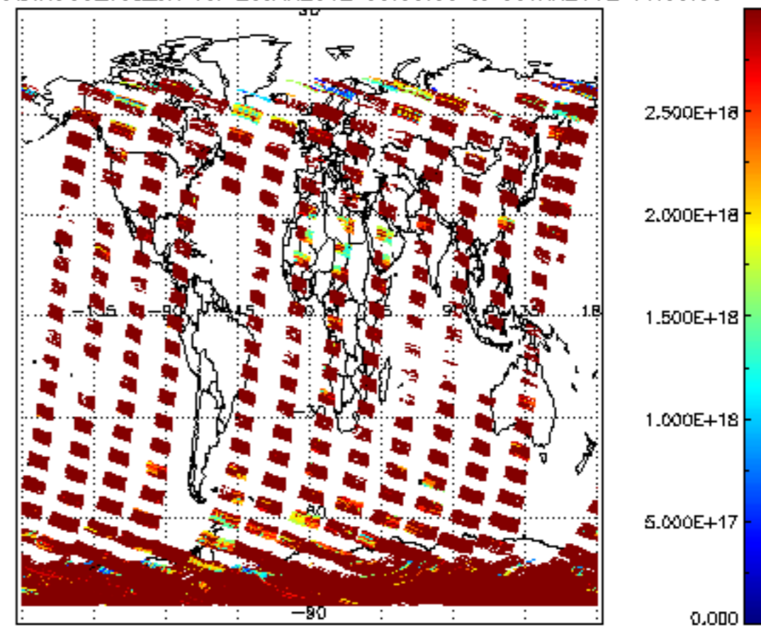
SCIOL2P_NADIR3CO_vcd_err for 29JAN2012 00:00:00 to 30JAN2012 00:00:00
