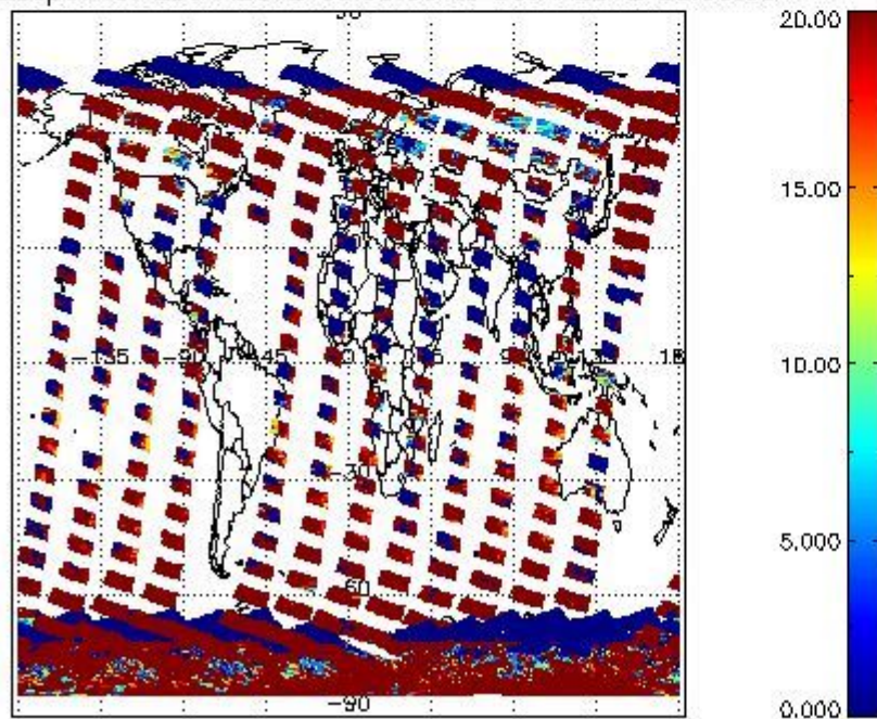
cLopt_depth for 29JAN2012 00:00:00 to 30JAN2012 00:00:00
