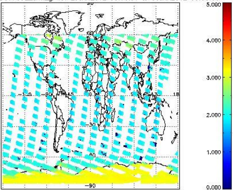
SCIOL2P_NADUV7S02_amf_gr for 29JAN2012 00:00:00 to 30JAN2012 00:00:00
