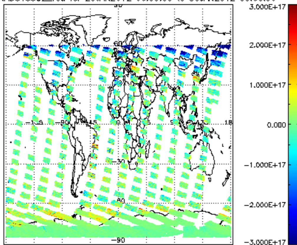
SCIOL2P_NADUV5S02_vcd for 29JAN2012 00:00:00 to 30JAN2012 00:00:00
