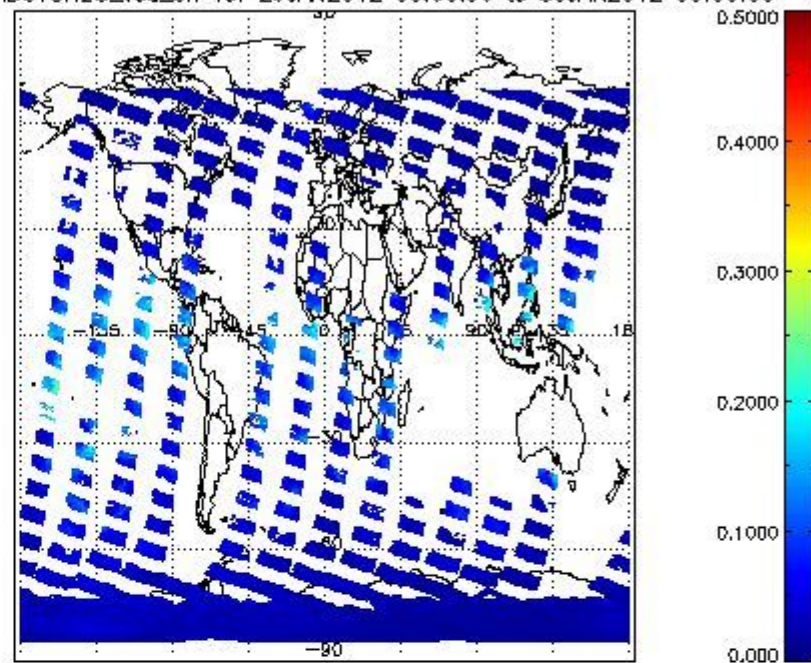
SCIOL2P_NADUV8H20_vcd_err for 29JAN2012 00:00:00 to 30JAN2012 00:00:00
