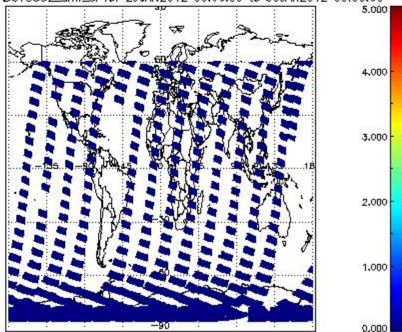
SCIOL2P_NADUV5SO2_amf_cl for 29JAN2012 00:00:00 to 30JAN2012 00:00:00
