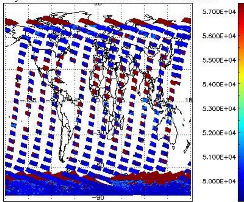
cloud_flags for 29JAN2012 00:00:00 to 30JAN2012 00:00:00
