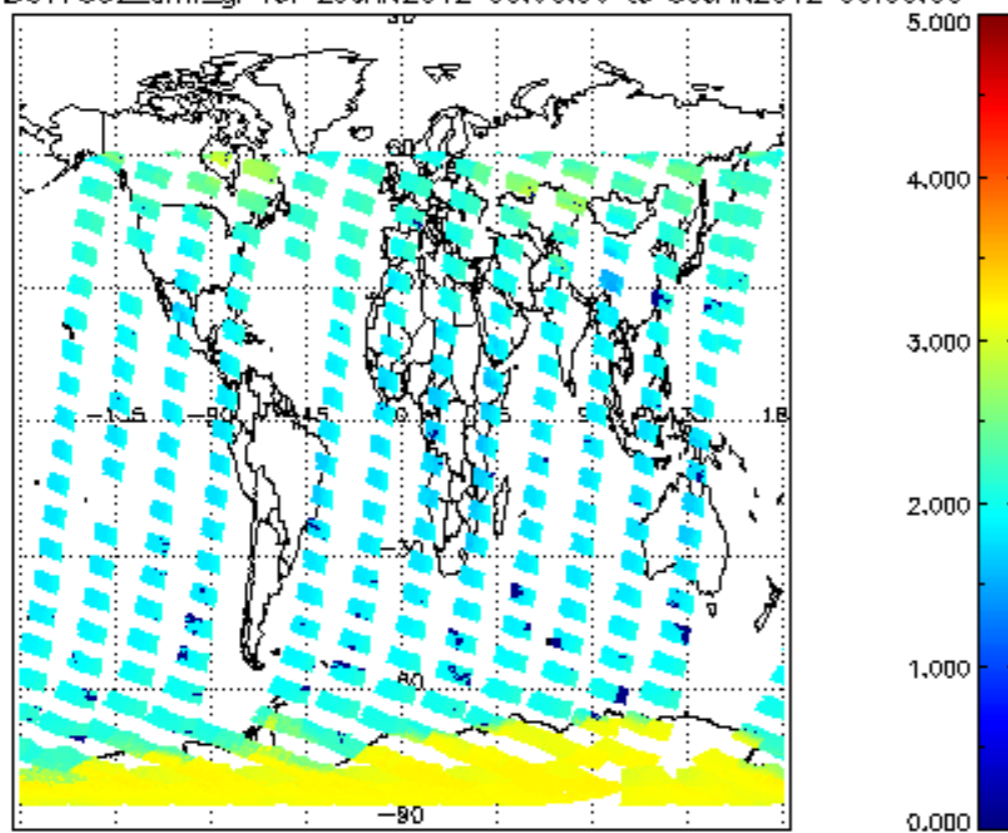
SCIOL2P_NADUV7S02_amf_gr for 29JAN2012 00:00:00 to 30JAN2012 00:00:00
