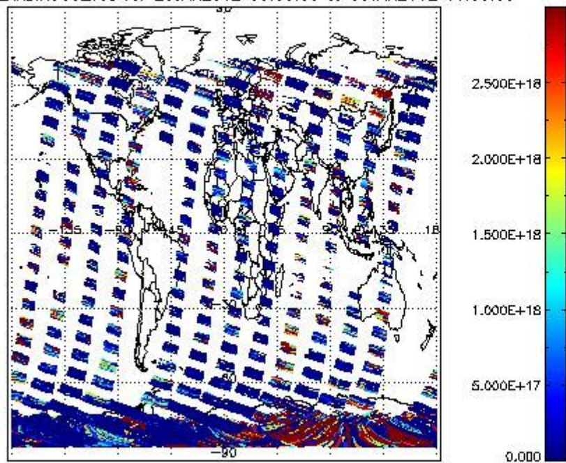
SCIDL2P_NADIR3CO_vcd for 29JAN2012 00:00:00 to 30JAN2012 00:00:00
