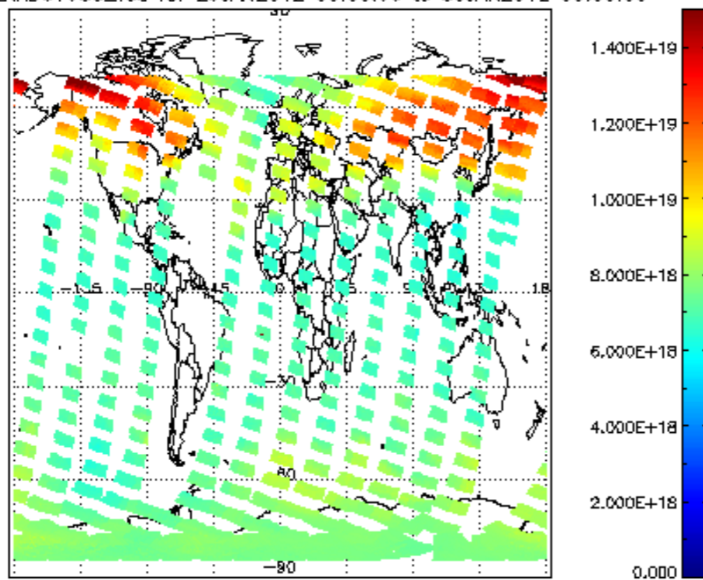
SCIOL2P_NADUV003_vcd for 29JAN2012 00:00:00 to 30JAN2012 00:00:00
