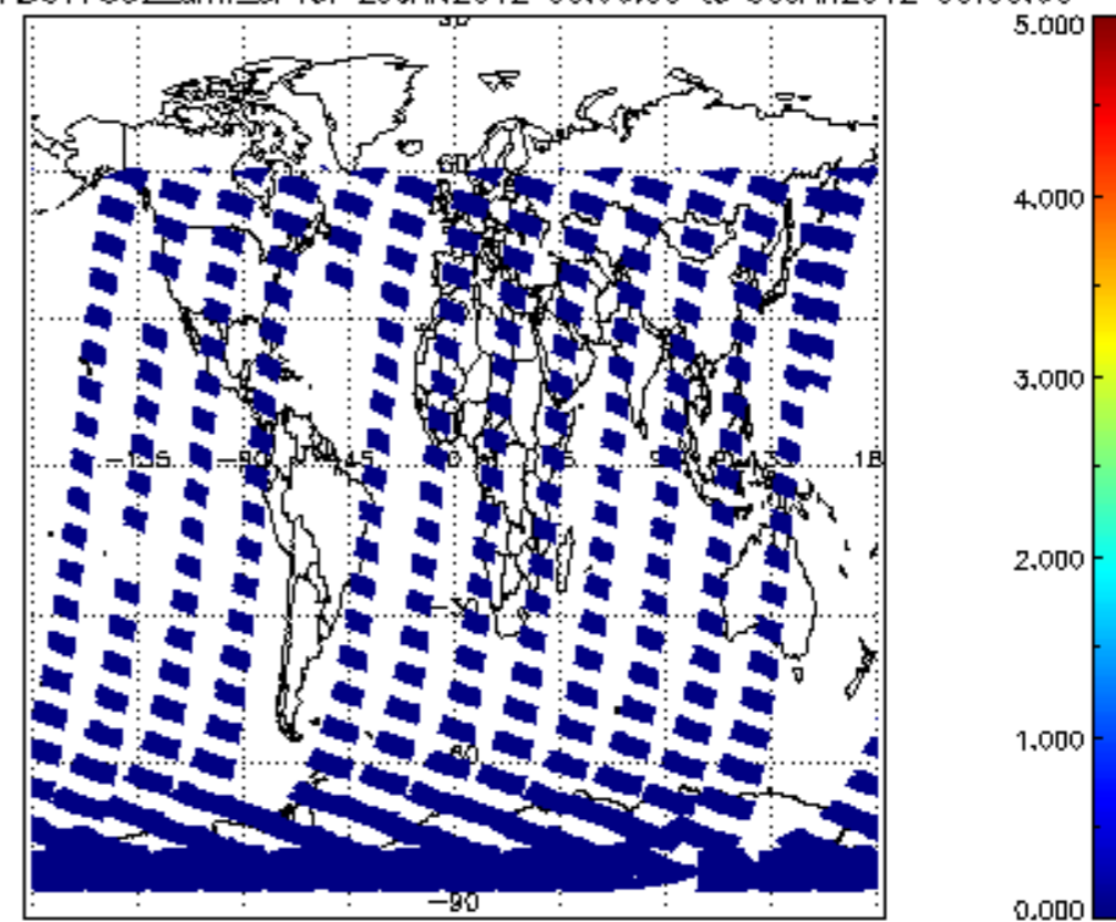
SCIOL2P_NADUV7S02_amf_cl for 29JAN2012 00:00:00 to 30JAN2012 00:00:00
