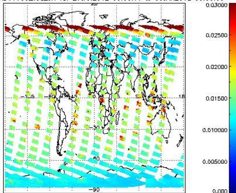
SCIOL2P_NADUV003_vcd_err for 29JAN2012 00:00:00 to 30JAN2012 00:00:00
