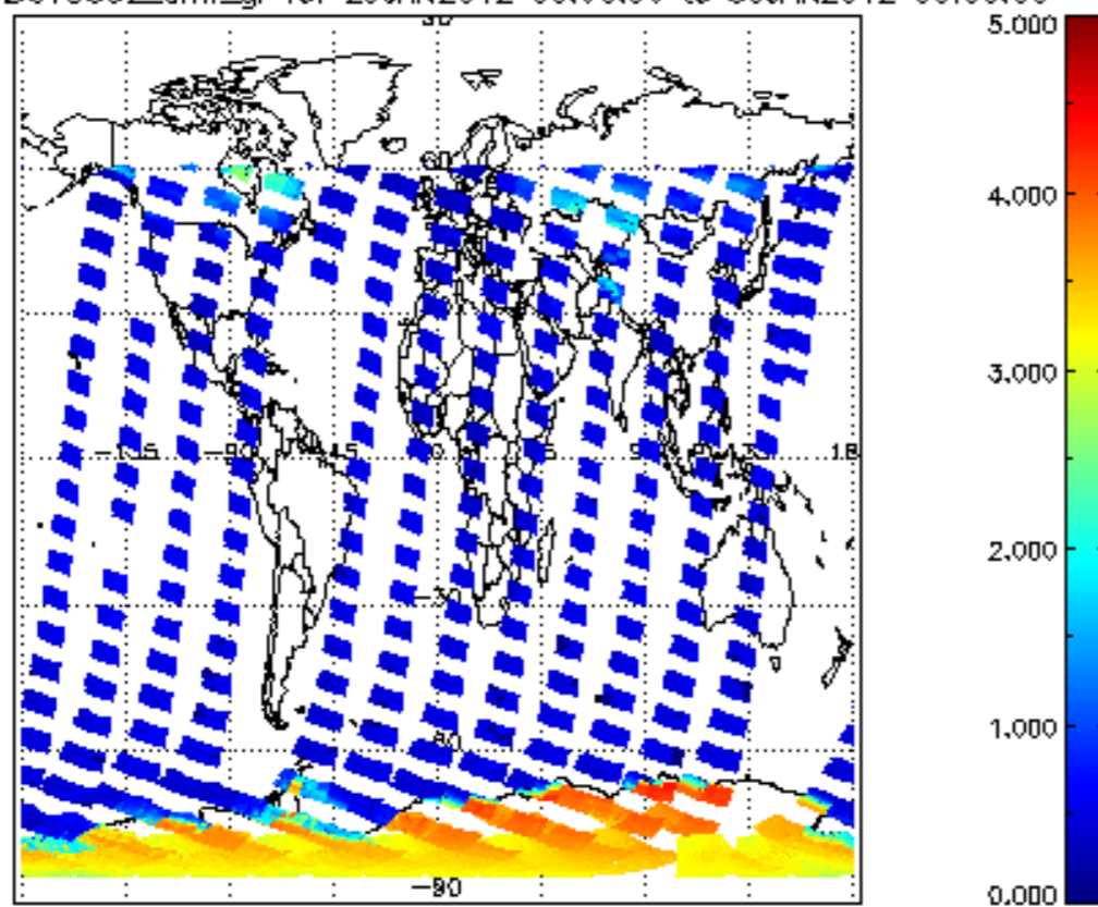
SCIOL2P_NADUV5S02_amf_gr for 29JAN2012 00:00:00 to 30JAN2012 00:00:00
