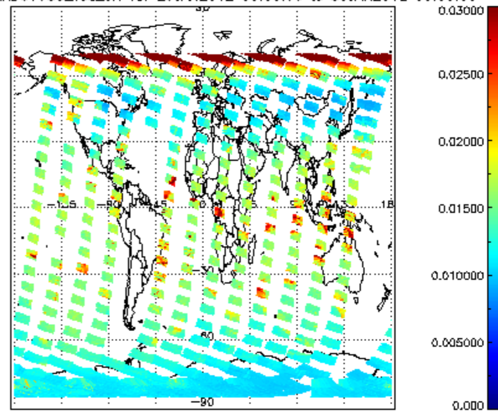
SCIOL2P_NADUV003_vcd_err for 29JAN2012 00:00:00 to 30JAN2012 00:00:00
