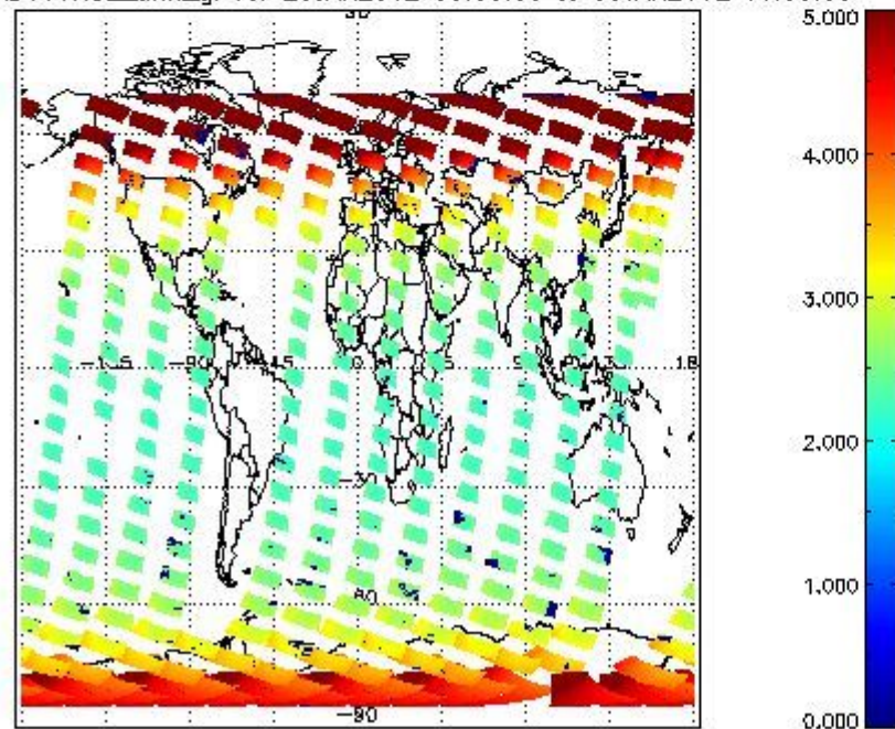
SCIOL2P_NADUV1NO2_amf_gr for 29JAN2012 00:00:00 to 30JAN2012 00:00:00
