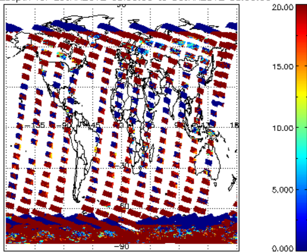
cLopt_depth for 29JAN2012 00:00:00 to 30JAN2012 00:00:00
