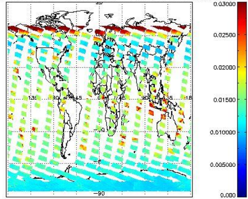
SCIOL2P_NADUV003_vcd_err for 25JAN2012 00:00:00 to 26JAN2012 00:00:00
