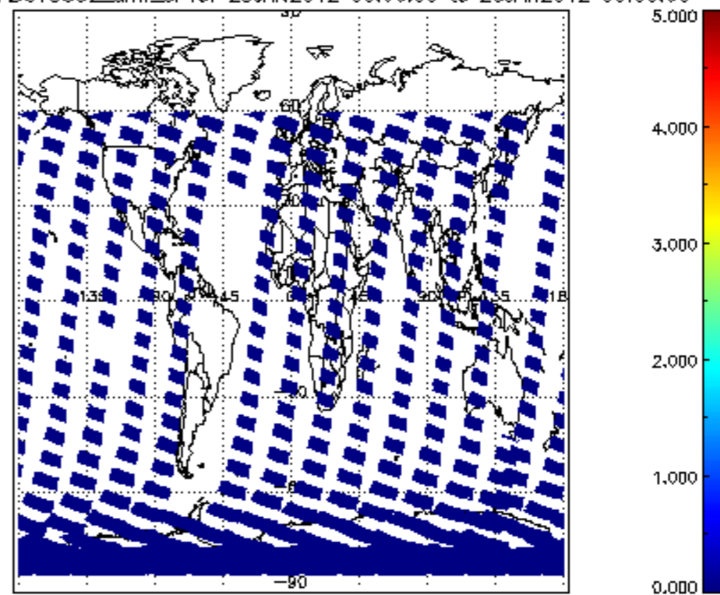
SCIOL2P_NADUV5S02_amf_cl for 25JAN2012 00:00:00 to 26JAN2012 00:00:00
