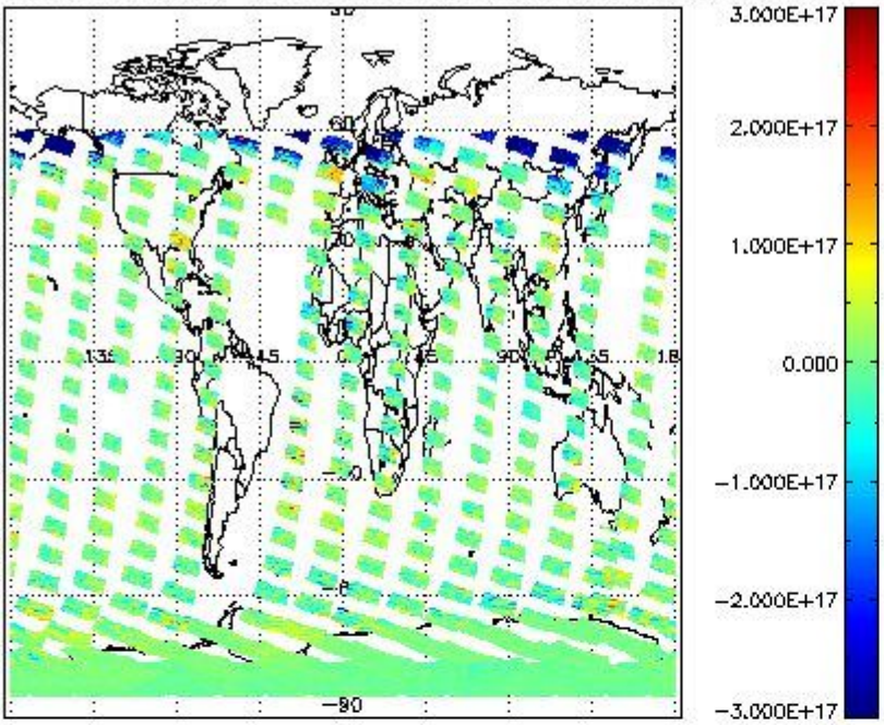
SCIOL2P_NADUV5SO2_vcd for 25JAN2012 00:00:00 to 26JAN2012 00:00:00
