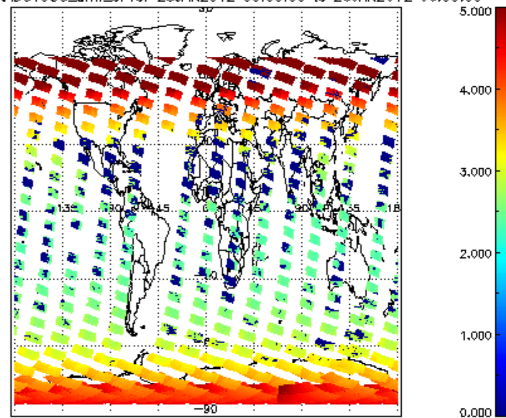
SCIOL2P_NADUV003_amf_cl for 25JAN2012 00:00:00 to 26JAN2012 00:00:00
