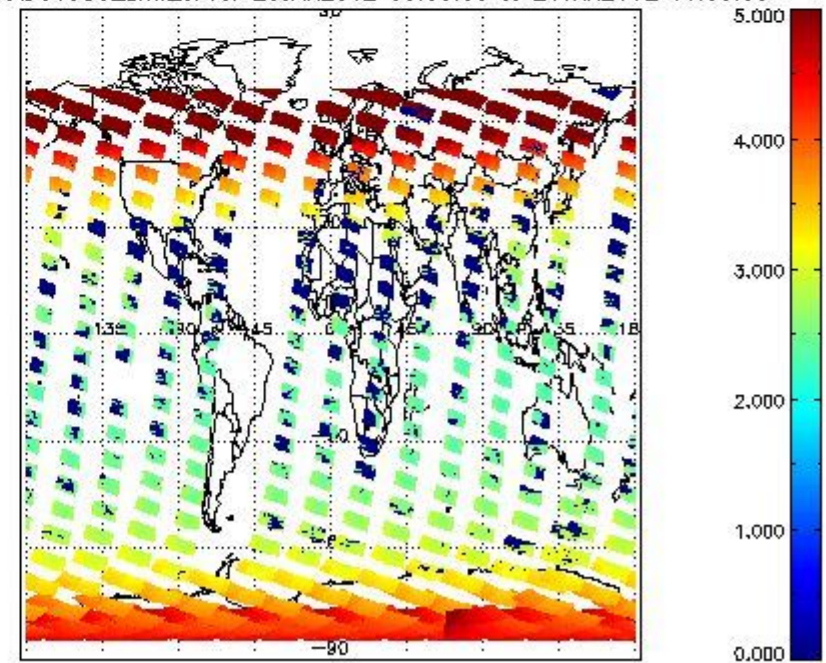
SCIOL2P_NADUV003_amf_cl for 25JAN2012 00:00:00 to 26JAN2012 00:00:00
