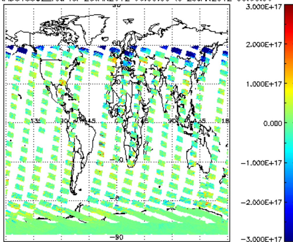
SCIOL2P_NADUV5S02_vcd for 25JAN2012 00:00:00 to 26JAN2012 00:00:00
