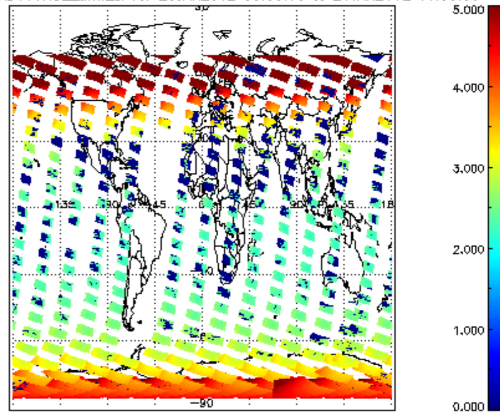
SCIOL2P_NADUV1NO2_amf_cl for 25JAN2012 00:00:00 to 26JAN2012 00:00:00
