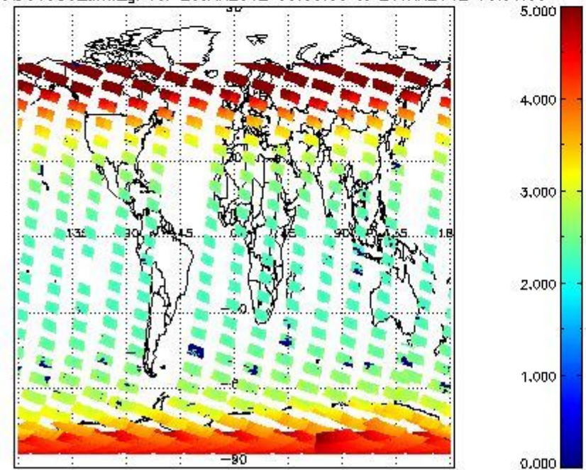
SCIOL2P_NADUV003_amf_gr for 25JAN2012 00:00:00 to 26JAN2012 00:00:00
