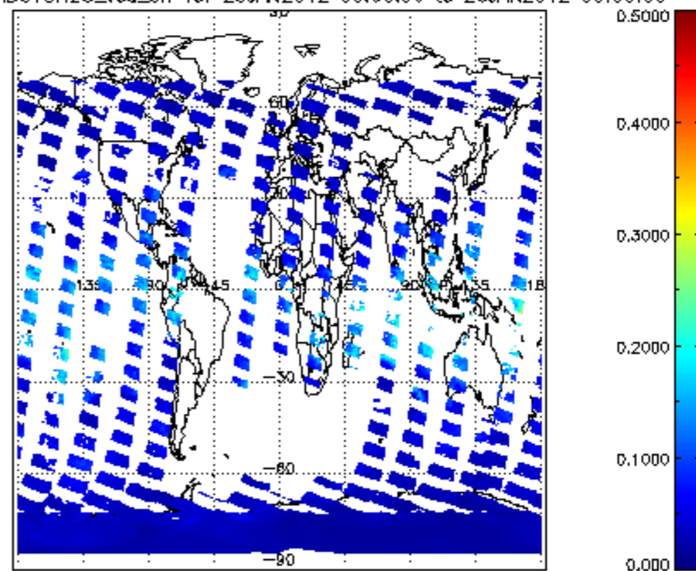
SCIOL2P_NADUV8H20_vcd_err for 25JAN2012 00:00:00 to 26JAN2012 00:00:00
