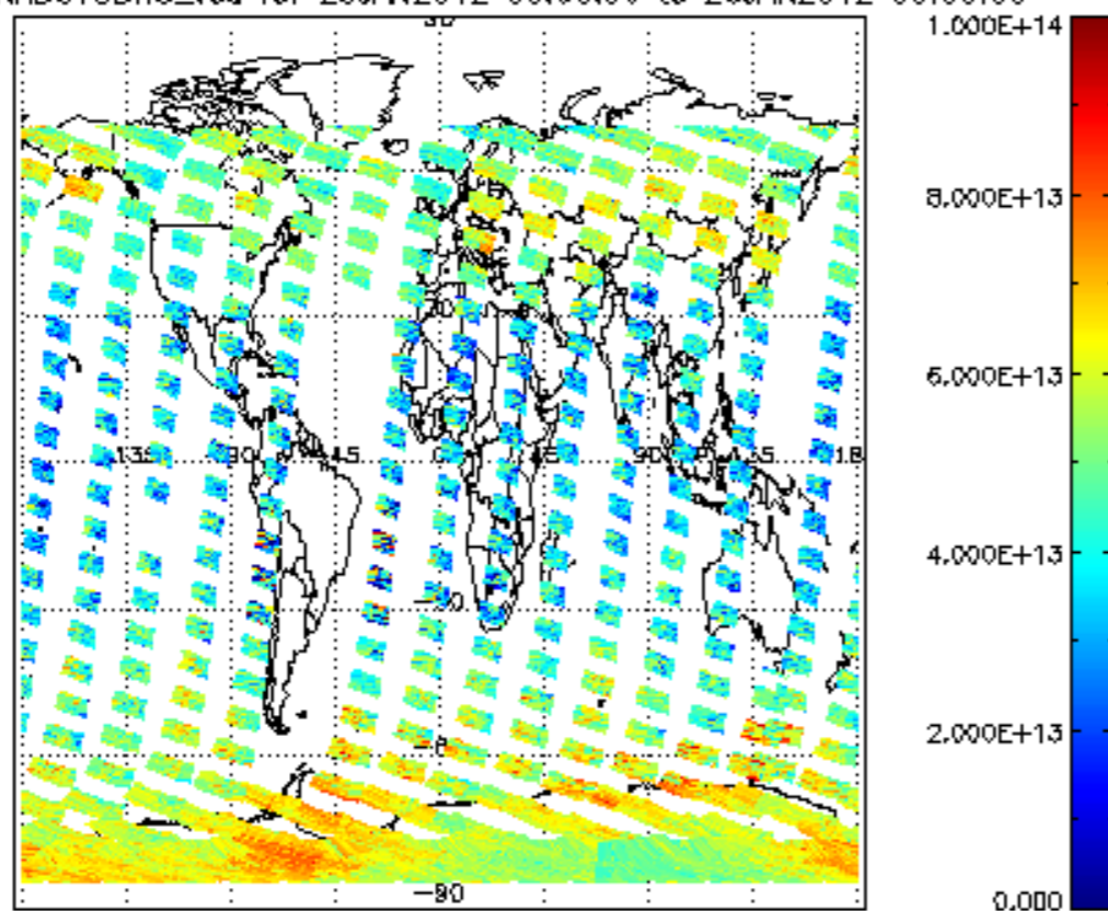
SCIOL2P_NADUV3BRO_vcd for 25JAN2012 00:00:00 to 26JAN2012 00:00:00
