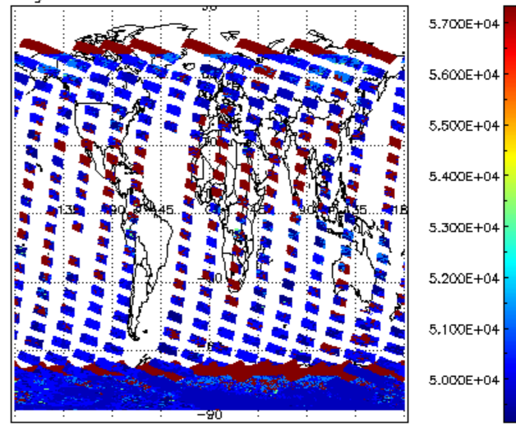
cloud_flags for 25JAN2012 00:00:00 to 26JAN2012 00:00:00
