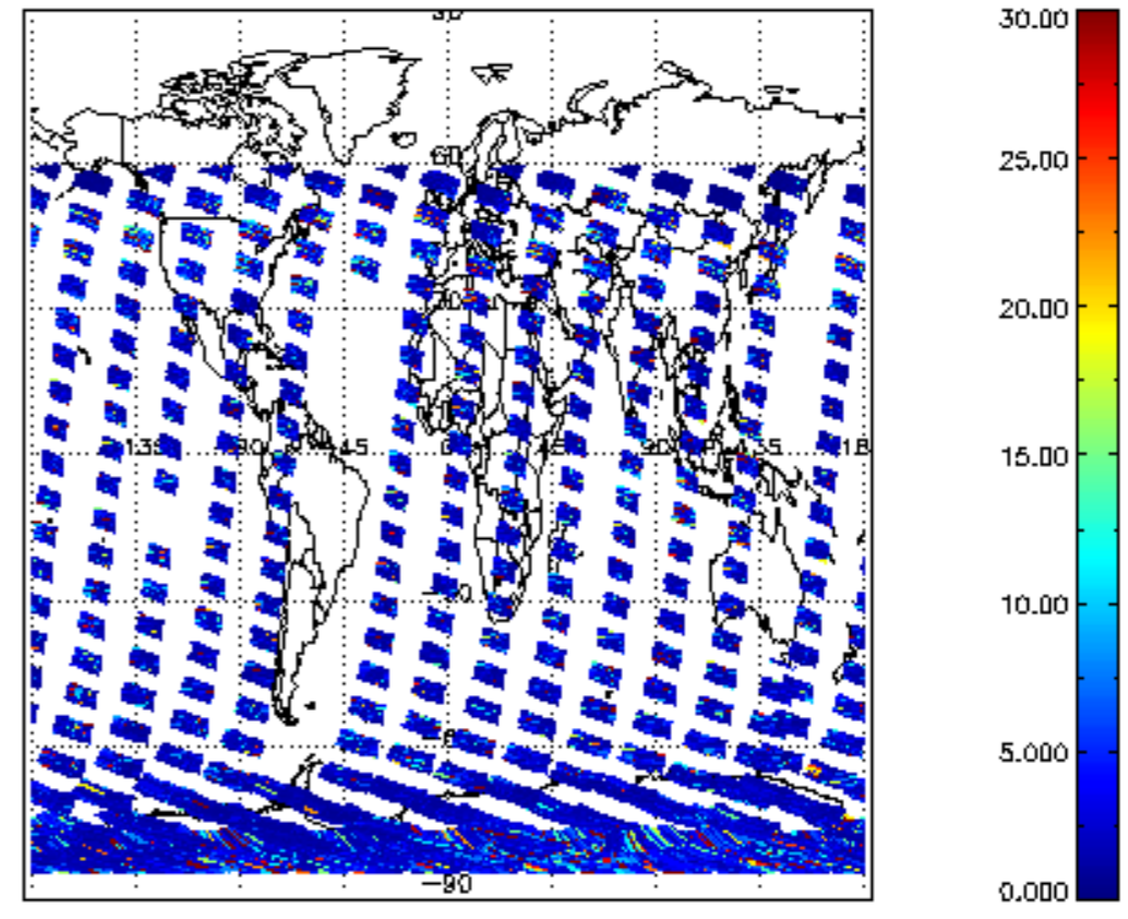
SCIOL2P_NADUV7S02_vcd_err for 25JAN2012 00:00:00 to 26JAN2012 00:00:00
