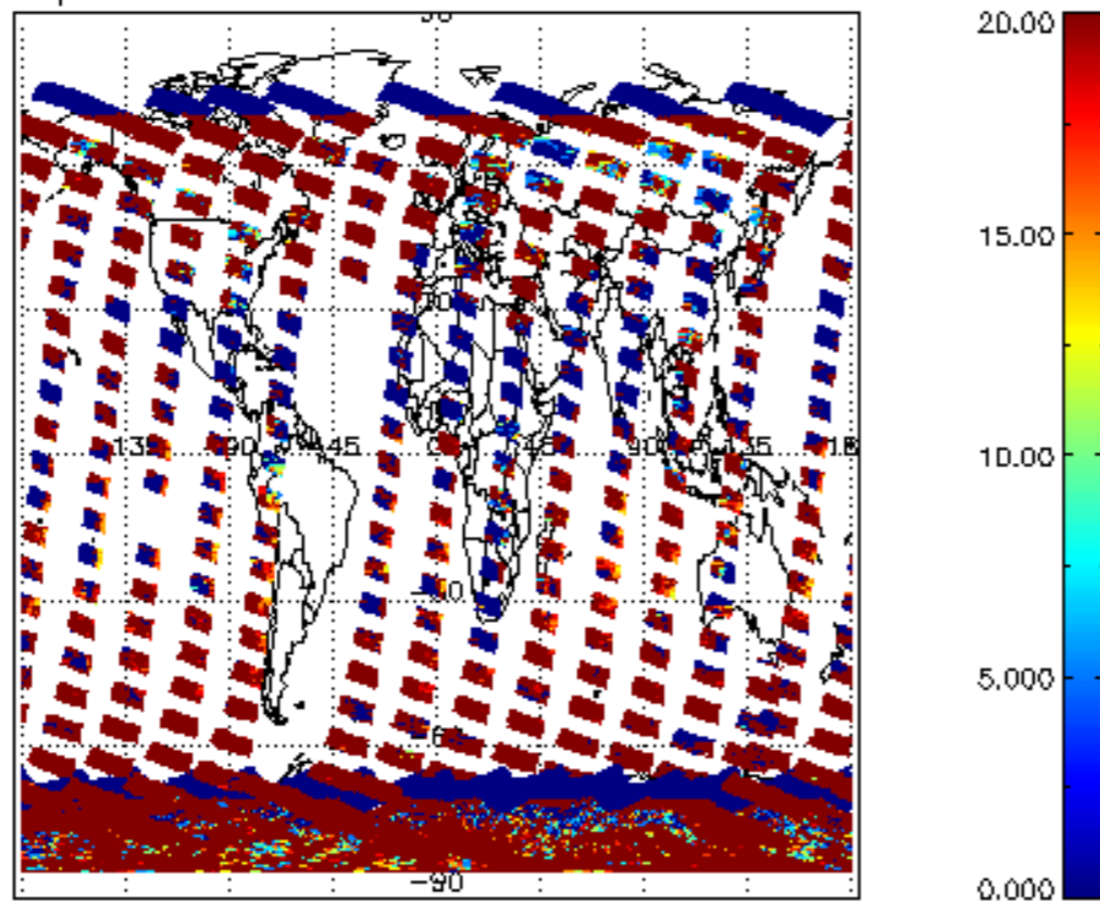
cLopt_depth for 25JAN2012 00:00:00 to 26JAN2012 00:00:00
