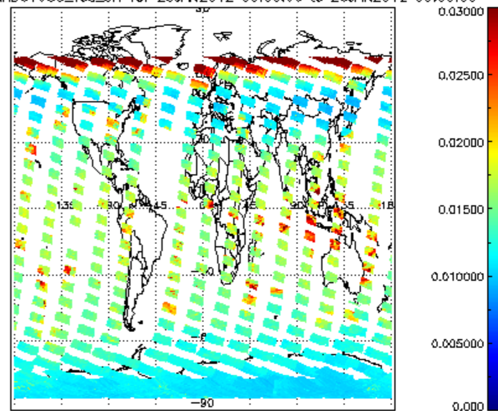
SCIOL2P_NADUV003_vcd_err for 25JAN2012 00:00:00 to 26JAN2012 00:00:00
