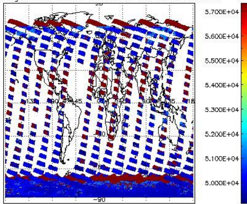
cloud_flags for 25JAN2012 00:00:00 to 26JAN2012 00:00:00
