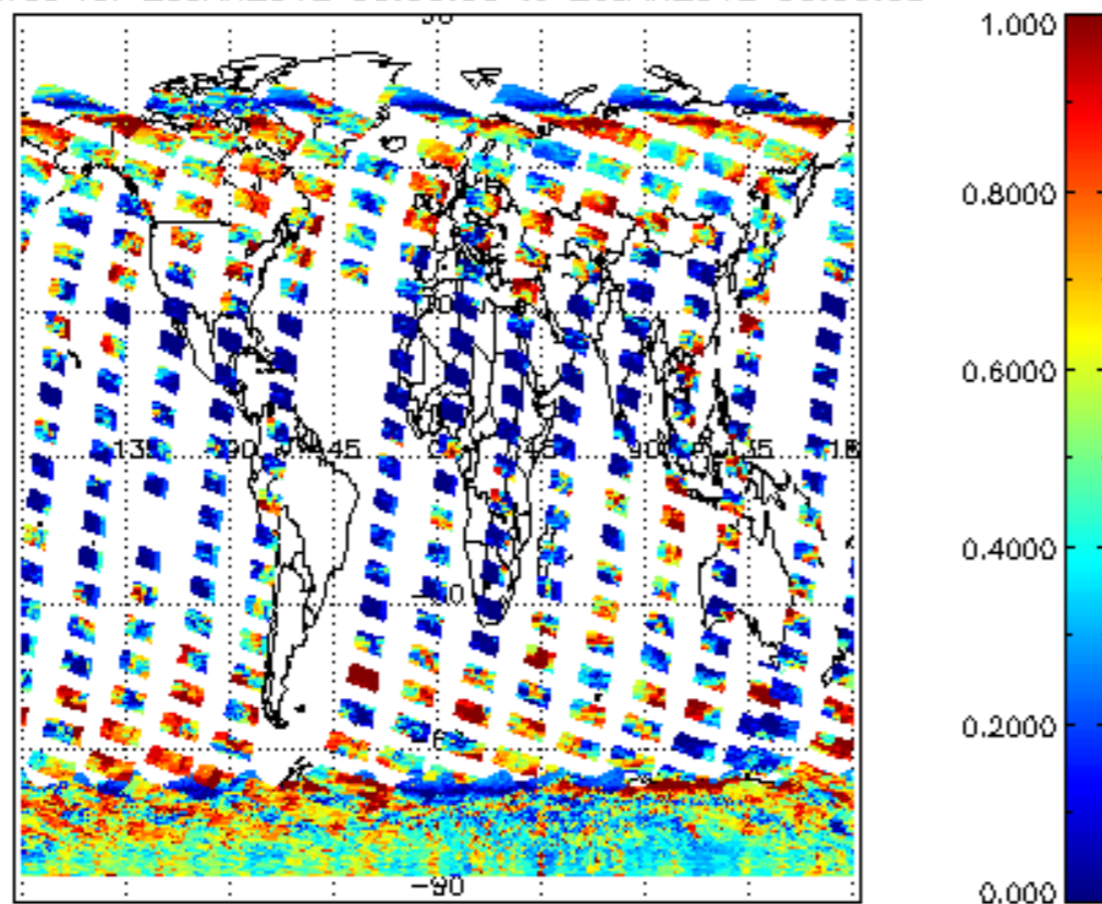
cL_frac for 25JAN2012 00:00:00 to 26JAN2012 00:00:00
