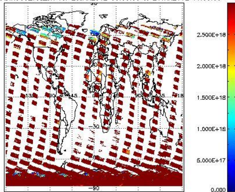
SCIDL2P_NADIR3CO_vcd_err for 25JAN2012 00:00:00 to 26JAN2012 00:00:00
