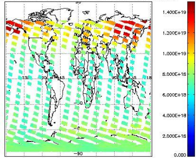
SCIOL2P_NADUV003_vcd for 25JAN2012 00:00:00 to 26JAN2012 00:00:00
