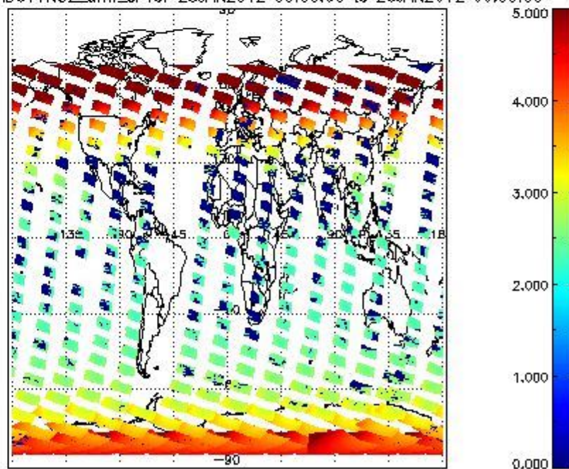
SCIOL2P_NADUV1NO2_amf_cl for 25JAN2012 00:00:00 to 26JAN2012 00:00:00
