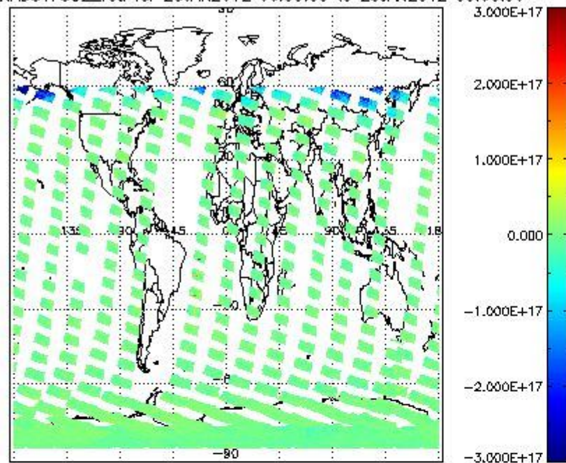
SCIOL2P_NADUV7S02_vcd for 25JAN2012 00:00:00 to 26JAN2012 00:00:00
