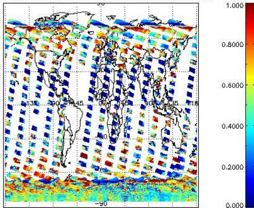
cL_frac for 25JAN2012 00:00:00 to 26JAN2012 00:00:00
