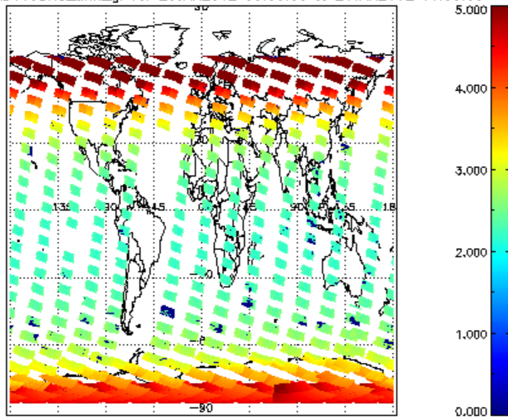
SCIOL2P_NADUV3BRO_amf_gr for 25JAN2012 00:00:00 to 26JAN2012 00:00:00
