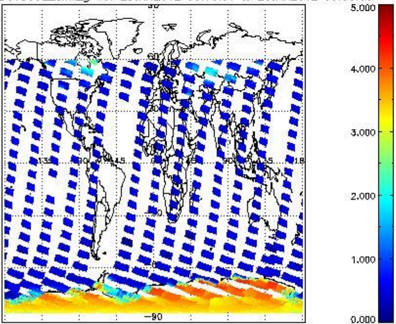
SCIOL2P_NADUV5SO2_amf_gr for 25JAN2012 00:00:00 to 26JAN2012 00:00:00
