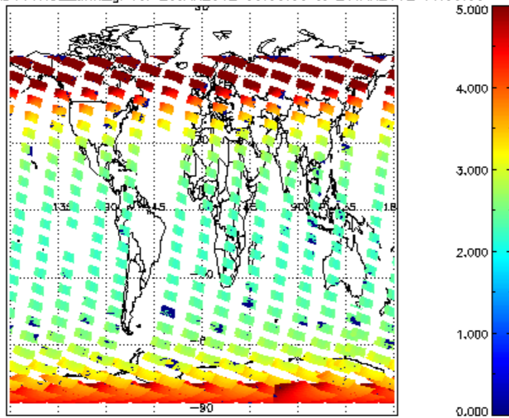
SCIOL2P_NADUV1NO2_amf_gr for 25JAN2012 00:00:00 to 26JAN2012 00:00:00
