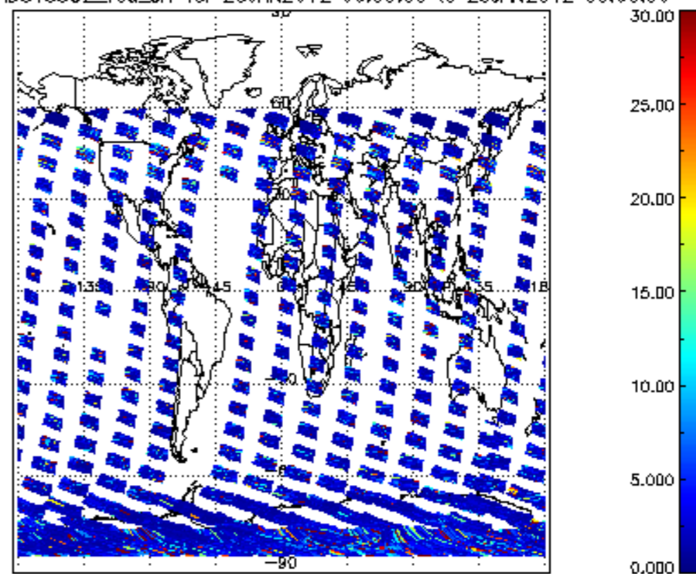
SCIOL2P_NADUV5S02_vcd_err for 25JAN2012 00:00:00 to 26JAN2012 00:00:00
