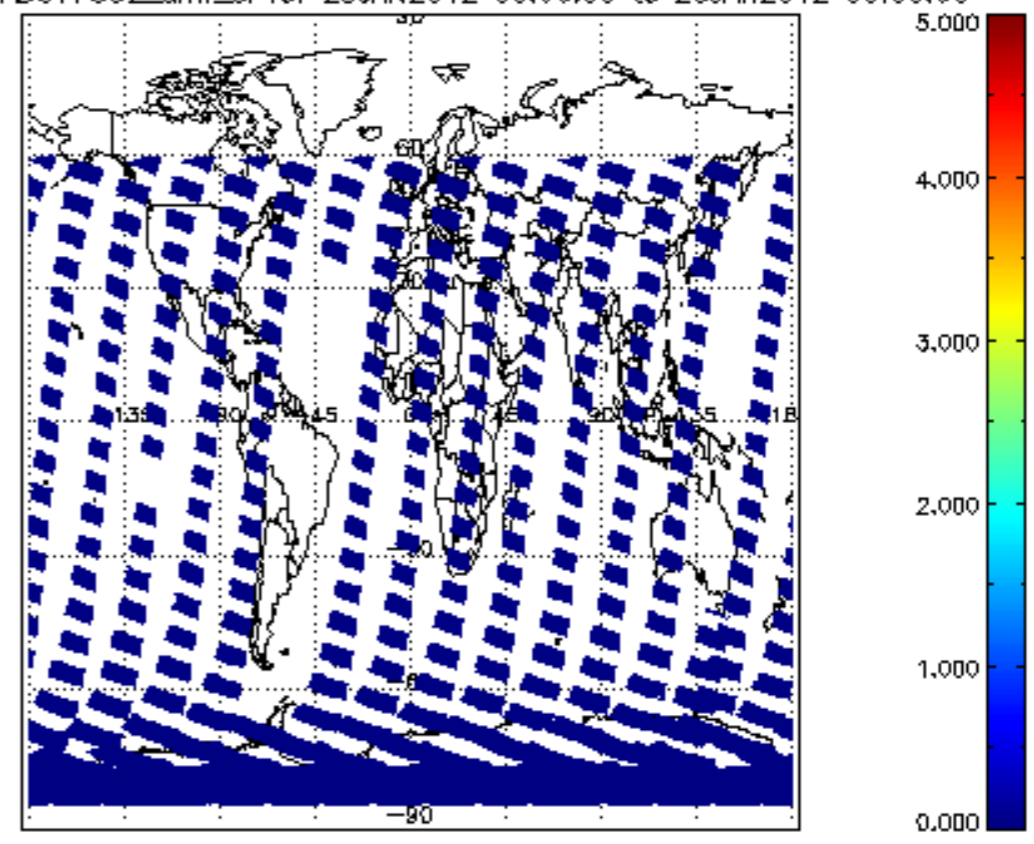
SCIOL2P_NADUV7S02_amf_cl for 25JAN2012 00:00:00 to 26JAN2012 00:00:00
