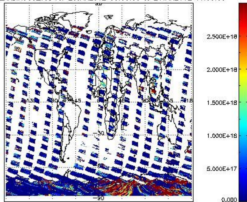
SCIDL2P_NADIR3CO_vcd for 25JAN2012 00:00:00 to 26JAN2012 00:00:00
