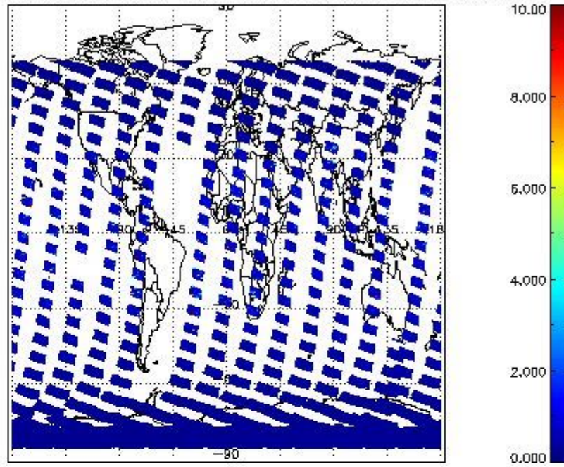
SCIOL2P_NADUV3BRO_vcd_err for 25JAN2012 00:00:00 to 26JAN2012 00:00:00
