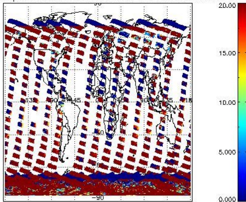
cLopt_depth for 25JAN2012 00:00:00 to 26JAN2012 00:00:00
