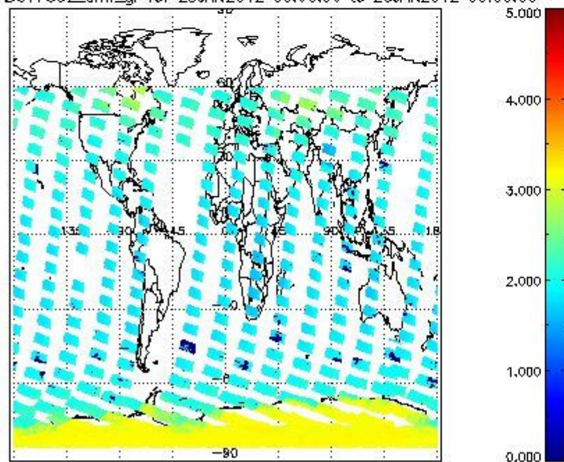
SCIOL2P_NADUV7S02_amf_gr for 25JAN2012 00:00:00 to 26JAN2012 00:00:00
