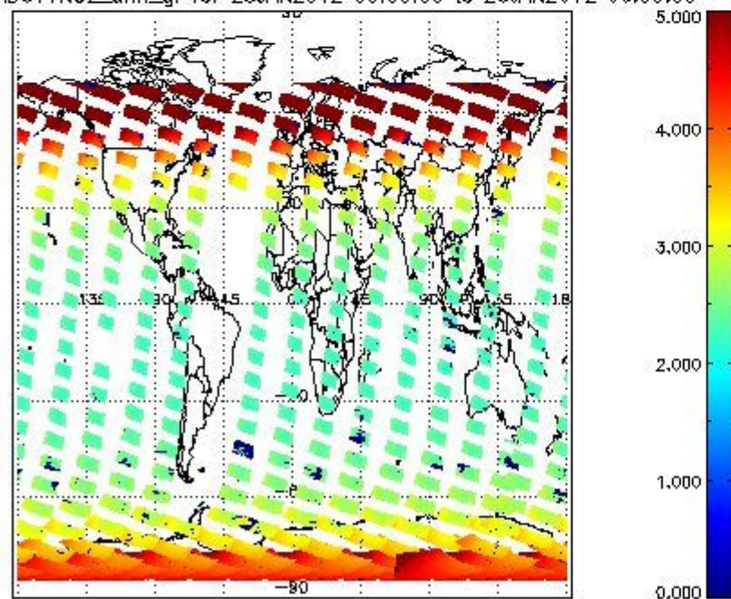
SCIOL2P_NADUV1NO2_amf_gr for 25JAN2012 00:00:00 to 26JAN2012 00:00:00
