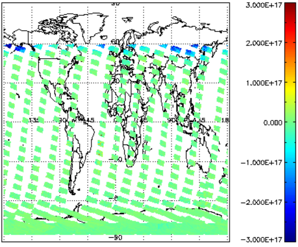
SCIOL2P_NADUV7S02_vcd for 25JAN2012 00:00:00 to 26JAN2012 00:00:00
