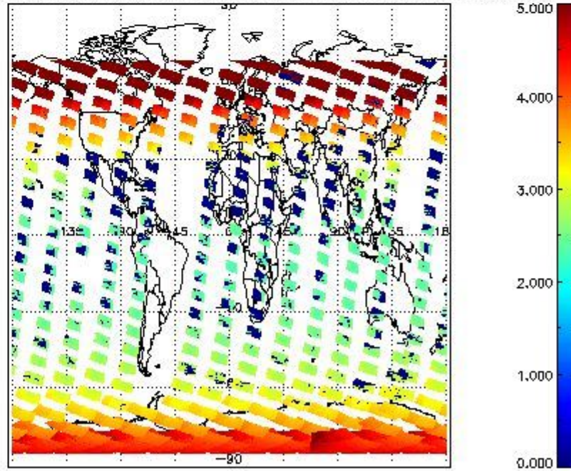
SCIOL2P_NADUV3BRO_amf_cl for 25JAN2012 00:00:00 to 26JAN2012 00:00:00
