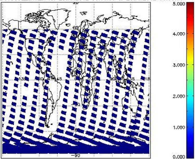
SCIOL2P_NADUV5SO2_amf_cl for 25JAN2012 00:00:00 to 26JAN2012 00:00:00
