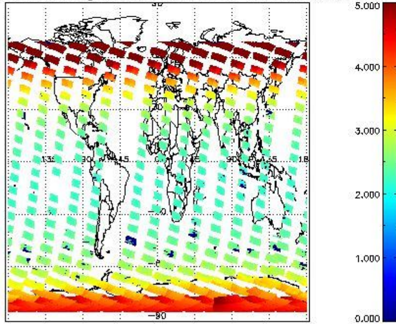
SCIOL2P_NADUV3BRO_amf_gr for 25JAN2012 00:00:00 to 26JAN2012 00:00:00
