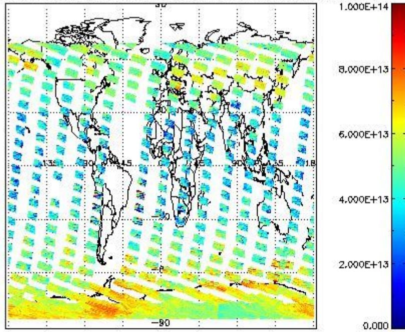
SCIOL2P_NADUV3BRO_vcd for 25JAN2012 00:00:00 to 26JAN2012 00:00:00
