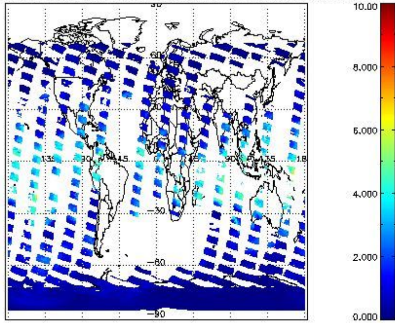
SCIOL2P_NADUV8H20_vcd for 25JAN2012 00:00:00 to 26JAN2012 00:00:00
