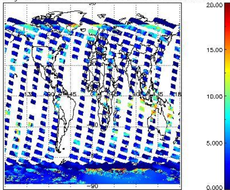
cL_top_height for 25JAN2012 00:00:00 to 26JAN2012 00:00:00
