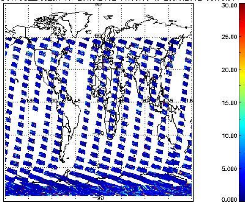
SCIOL2P_NADUV7S02_vcd_err for 25JAN2012 00:00:00 to 26JAN2012 00:00:00
