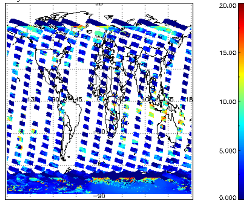
cL_top_height for 25JAN2012 00:00:00 to 26JAN2012 00:00:00
