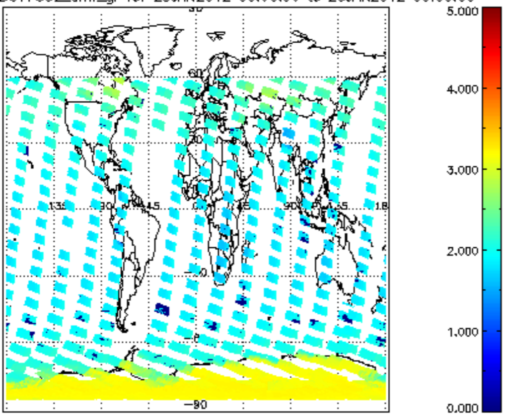
SCIOL2P_NADUV7S02_amf_gr for 25JAN2012 00:00:00 to 26JAN2012 00:00:00
