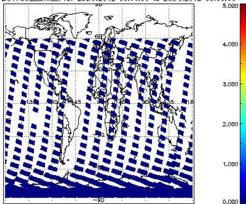
SCIOL2P_NADUV7S02_amf_cl for 25JAN2012 00:00:00 to 26JAN2012 00:00:00
