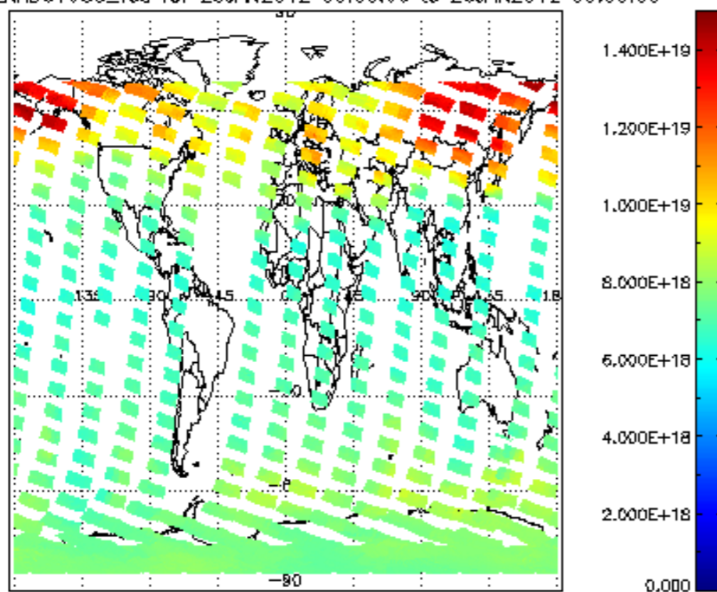
SCIOL2P_NADUV003_vcd for 25JAN2012 00:00:00 to 26JAN2012 00:00:00
