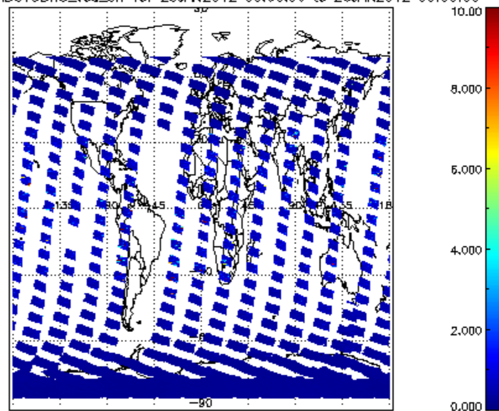
SCIOL2P_NADUV3BRO_vcd_err for 25JAN2012 00:00:00 to 26JAN2012 00:00:00
