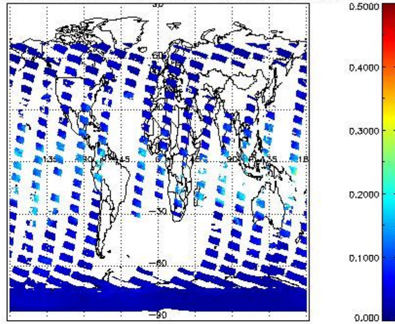
SCIOL2P_NADUV8H20_vcd_err for 25JAN2012 00:00:00 to 26JAN2012 00:00:00
