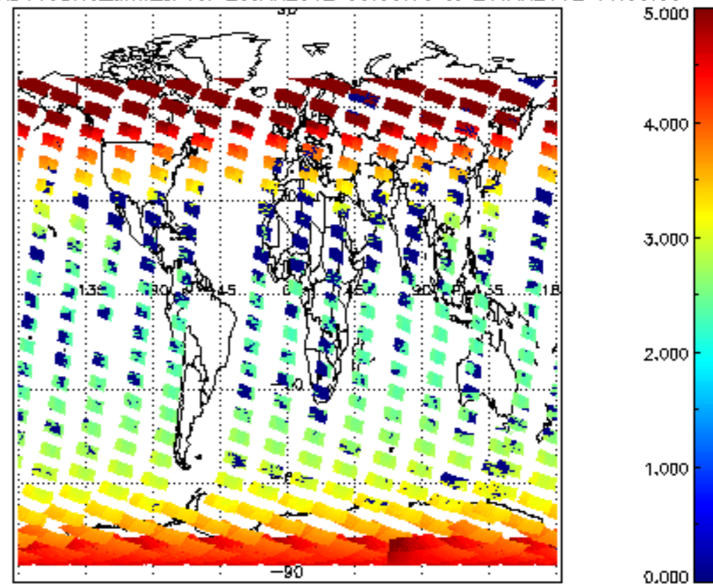
SCIOL2P_NADUV3BRO_amf_cl for 25JAN2012 00:00:00 to 26JAN2012 00:00:00
