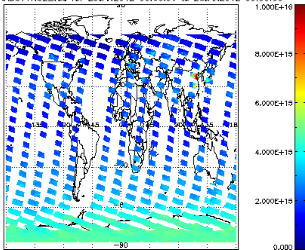
SCIOL2P_NADUV1NO2_vcd for 25JAN2012 00:00:00 to 26JAN2012 00:00:00
