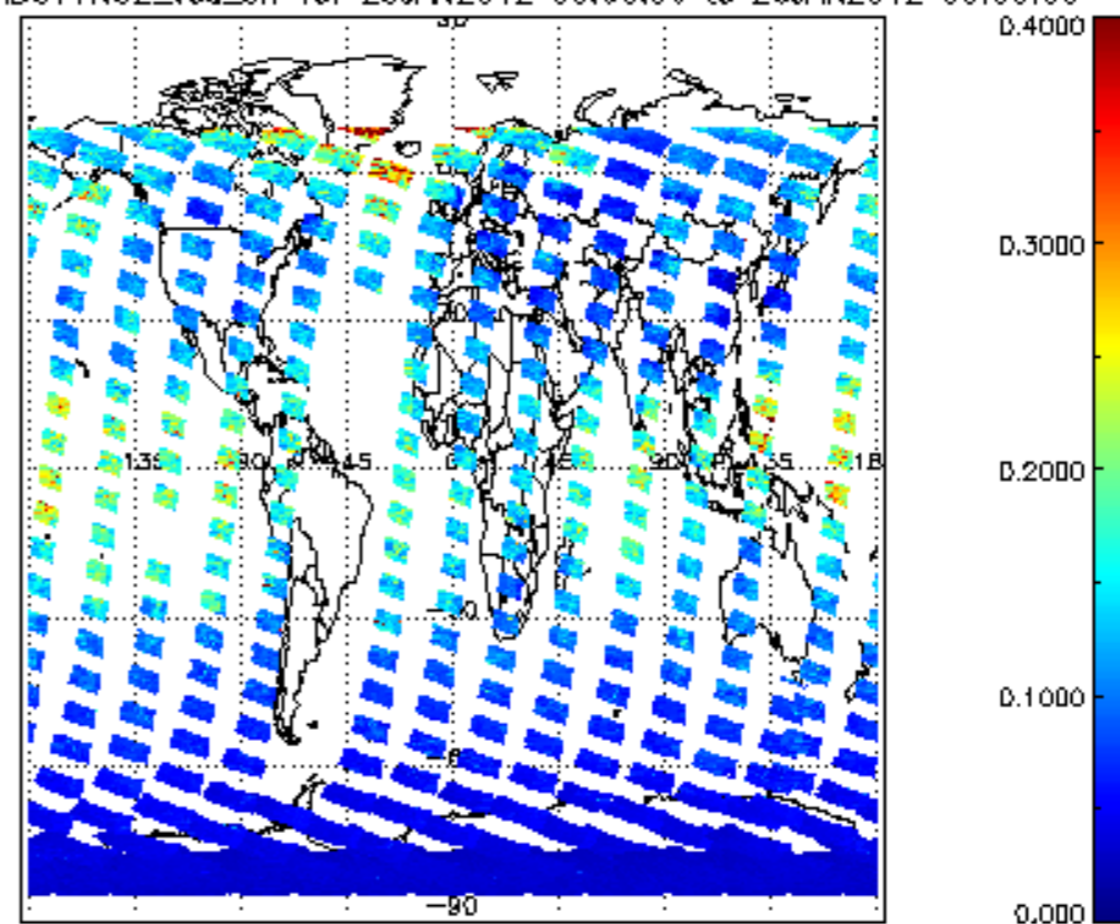
SCIOL2P_NADUV1NO2_vcd_err for 25JAN2012 00:00:00 to 26JAN2012 00:00:00
