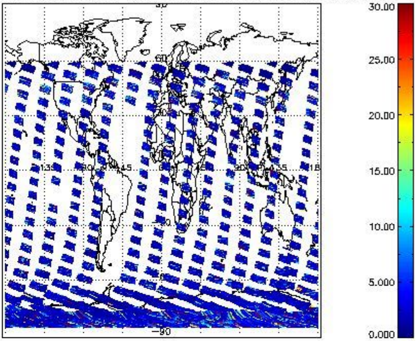
SCIOL2P_NADUV5SO2_vcd_err for 25JAN2012 00:00:00 to 26JAN2012 00:00:00
