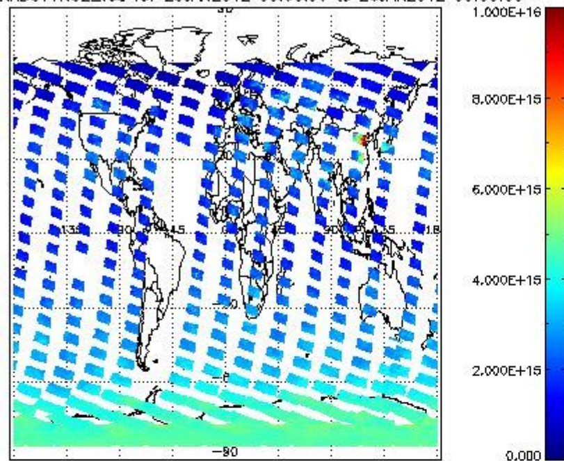
SCIOL2P_NADUV1NO2_vcd for 25JAN2012 00:00:00 to 26JAN2012 00:00:00
