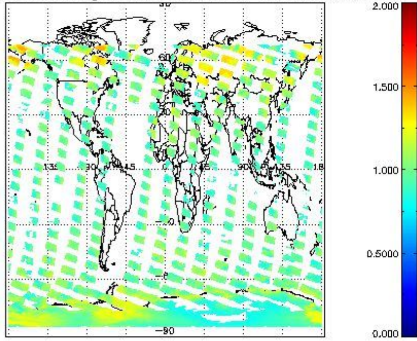
SCIOL2P_NADUV8H20_amf_gr for 25JAN2012 00:00:00 to 26JAN2012 00:00:00
