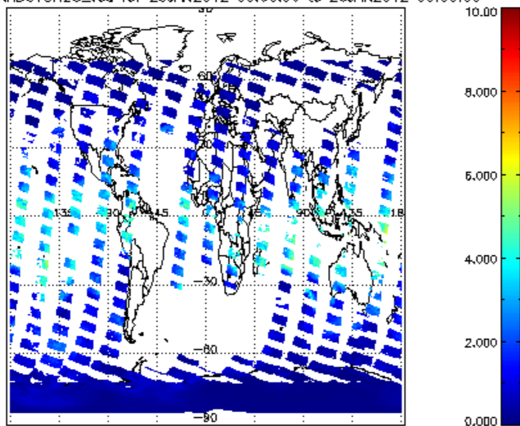
SCIOL2P_NADUV8H20_vcd for 25JAN2012 00:00:00 to 26JAN2012 00:00:00
