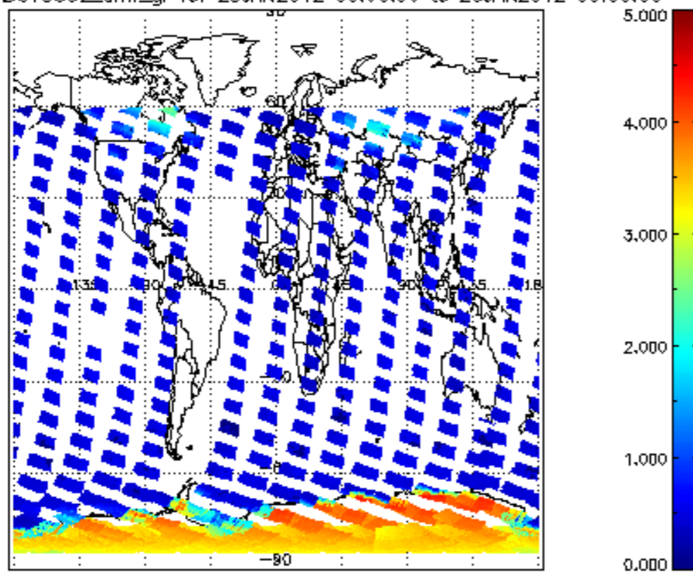
SCIOL2P_NADUV5S02_amf_gr for 25JAN2012 00:00:00 to 26JAN2012 00:00:00
