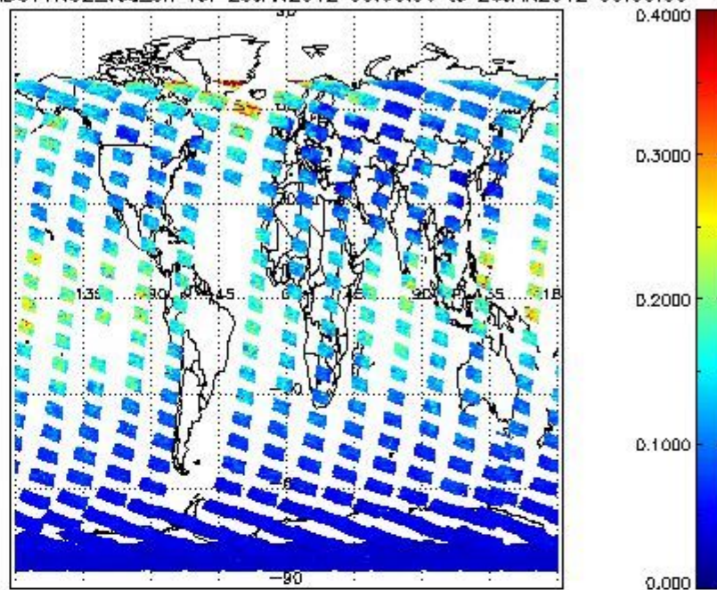
SCIOL2P_NADUV1NO2_vcd_err for 25JAN2012 00:00:00 to 26JAN2012 00:00:00
