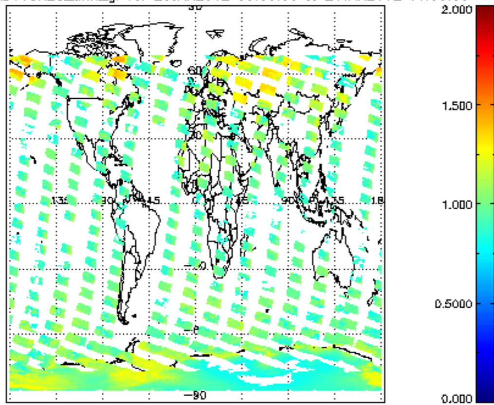
SCIOL2P_NADUV8H20_amf_gr for 25JAN2012 00:00:00 to 26JAN2012 00:00:00
