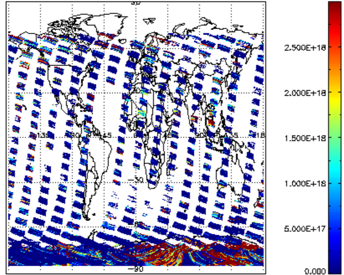
SCIOL2P_NADIR3CO_vcd for 25JAN2012 00:00:00 to 26JAN2012 00:00:00
