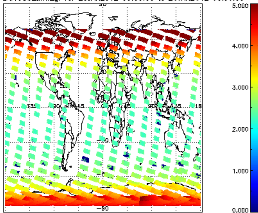
SCIOL2P_NADUV003_amf_gr for 25JAN2012 00:00:00 to 26JAN2012 00:00:00
