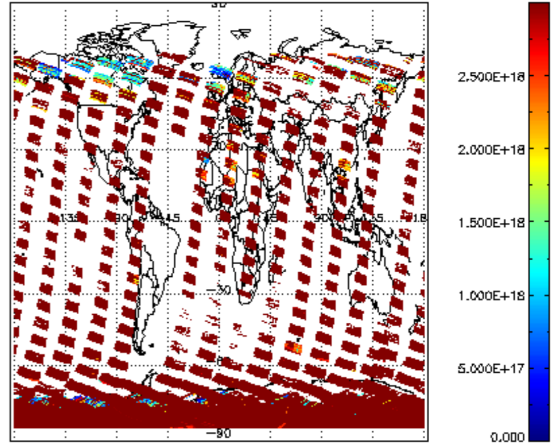
SCIOL2P_NADIR3CO_vcd_err for 25JAN2012 00:00:00 to 26JAN2012 00:00:00
