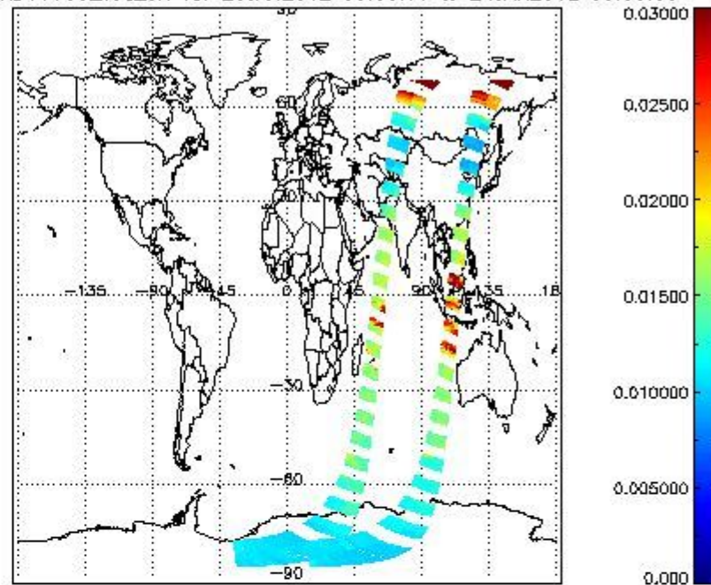
SCIOL2P_NADUV003_vcd_err for 23JAN2012 00:00:00 to 24JAN2012 00:00:00
