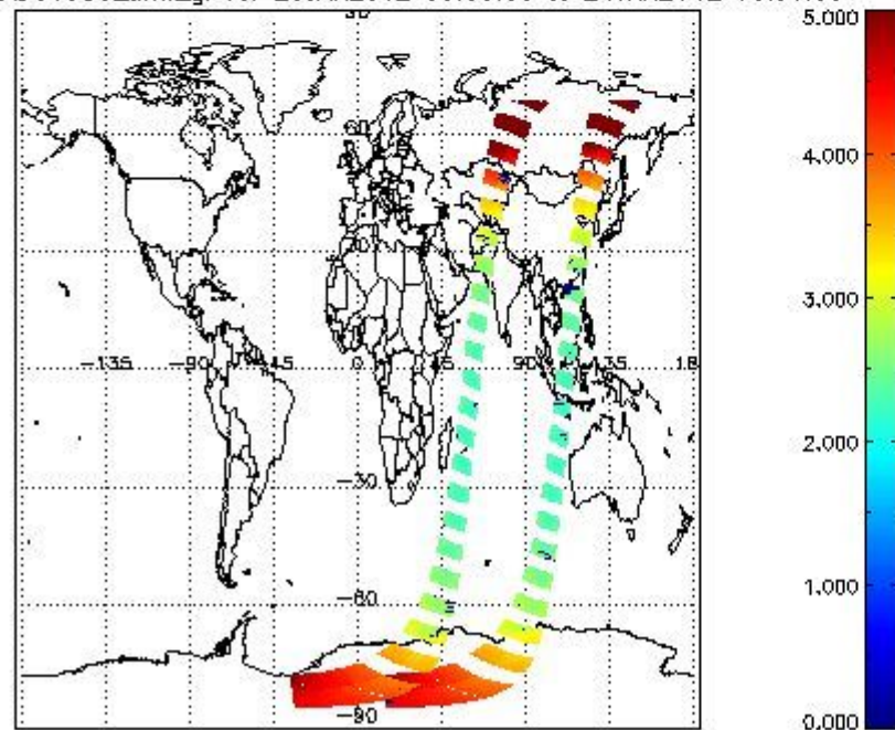
SCIOL2P_NADUV003_amf_gr for 23JAN2012 00:00:00 to 24JAN2012 00:00:00
