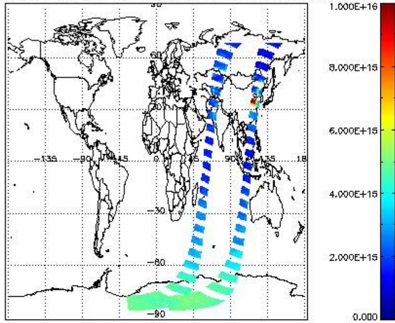
SCIOL2P_NADUV1NO2_vcd for 23JAN2012 00:00:00 to 24JAN2012 00:00:00
