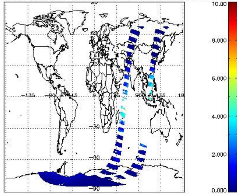
SCIOL2P_NADUV8H2O_vcd for 23JAN2012 00:00:00 to 24JAN2012 00:00:00
