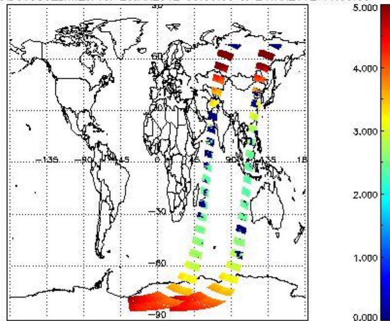
SCIOL2P_NADUV003_amf_cl for 23JAN2012 00:00:00 to 24JAN2012 00:00:00
