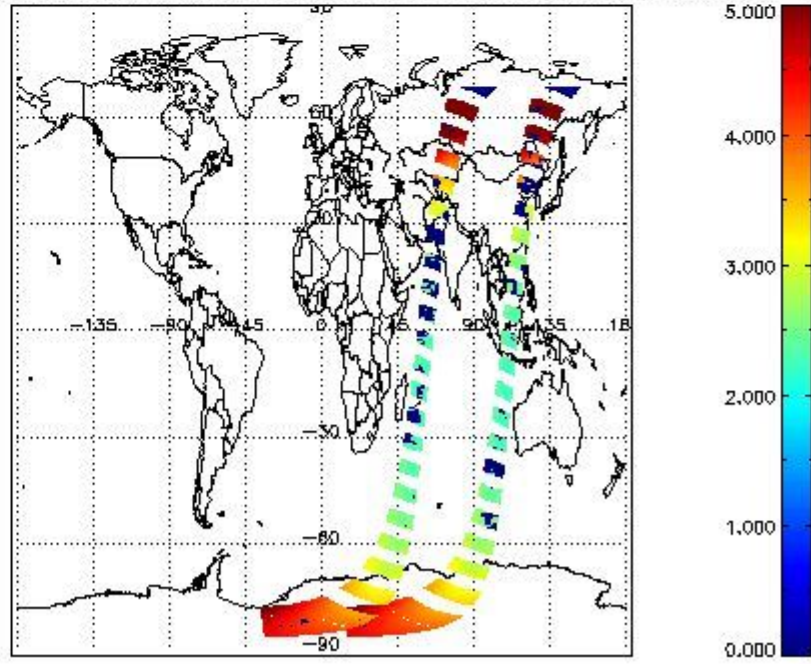
SCIOL2P_NADUV1NO2_amf_cl for 23JAN2012 00:00:00 to 24JAN2012 00:00:00
