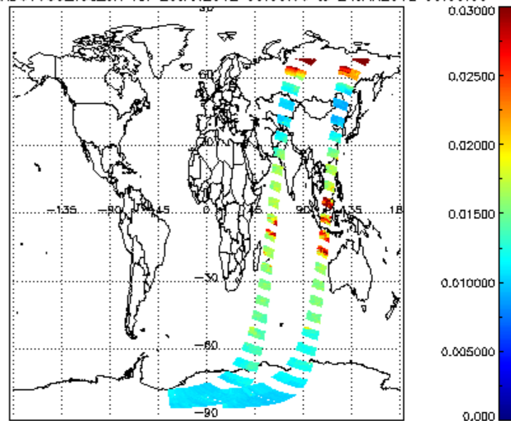
SCIOL2P_NADUV003_vcd_err for 23JAN2012 00:00:00 to 24JAN2012 00:00:00
