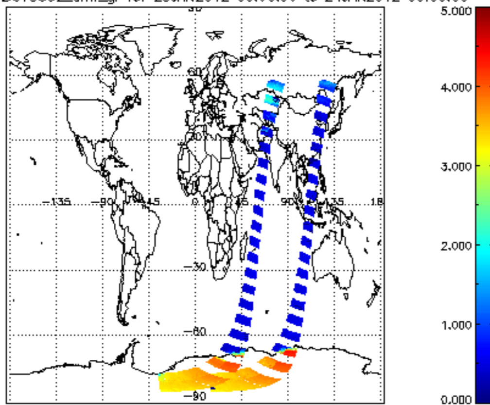
SCIOL2P_NADUV5S02_amf_gr for 23JAN2012 00:00:00 to 24JAN2012 00:00:00
