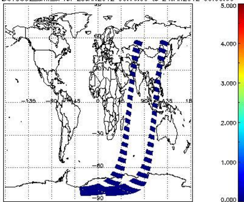
SCIOL2P_NADUV5SO2_amf_cl for 23JAN2012 00:00:00 to 24JAN2012 00:00:00
