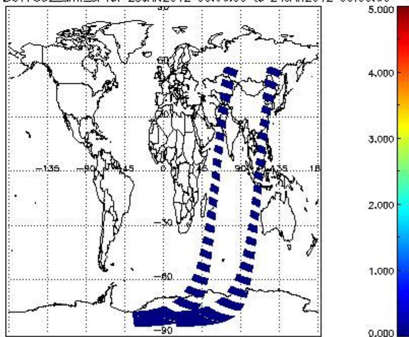
SCIOL2P_NADUV7S02_amf_cl for 23JAN2012 00:00:00 to 24JAN2012 00:00:00
