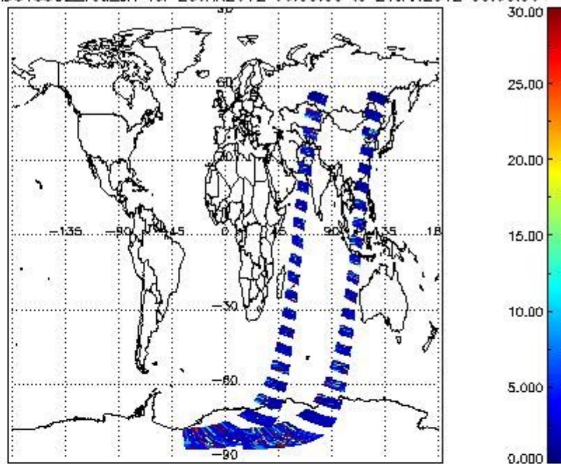
SCIOL2P_NADUV5SO2_vcd_err for 23JAN2012 00:00:00 to 24JAN2012 00:00:00
