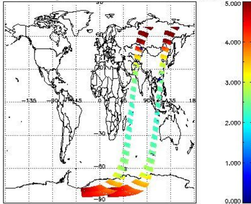
SCIOL2P_NADUV3BRO_amf_gr for 23JAN2012 00:00:00 to 24JAN2012 00:00:00
