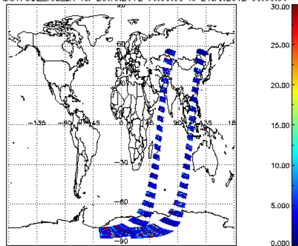
SCIOL2P_NADUV7S02_vcd_err for 23JAN2012 00:00:00 to 24JAN2012 00:00:00
