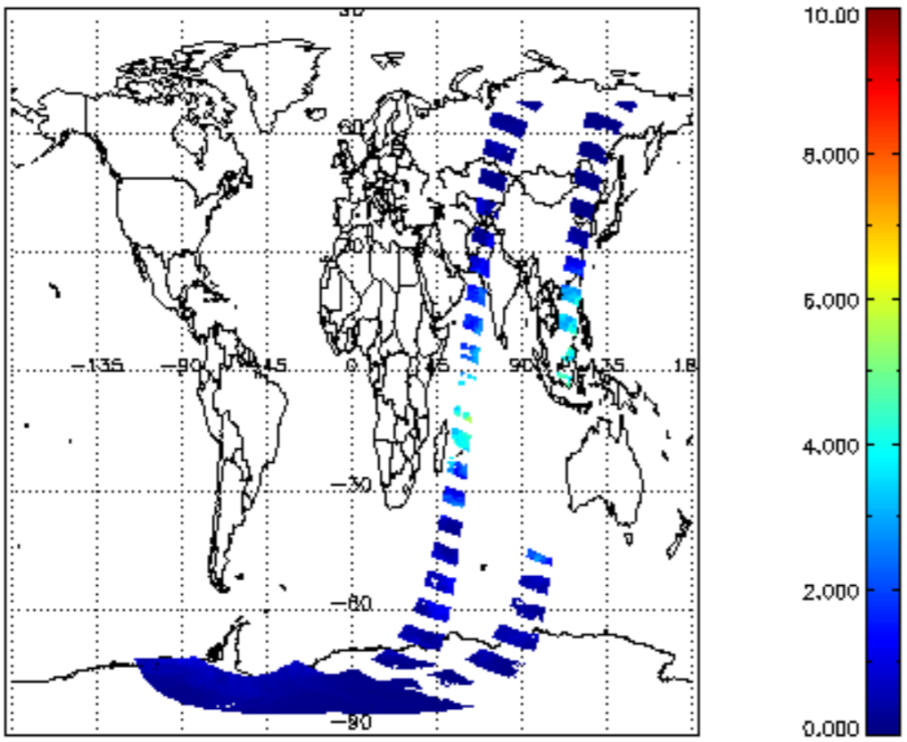
SCIOL2P_NADUVBH20_vcd for 23JAN2012 00:00:00 to 24JAN2012 00:00:00
