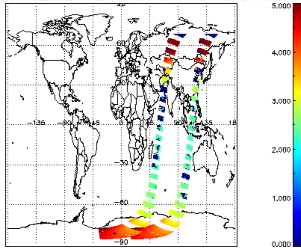
SCIOL2P_NADUV1NO2_amf_cl for 23JAN2012 00:00:00 to 24JAN2012 00:00:00
