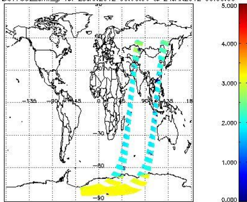
SCIOL2P_NADUV7S02_amf_gr for 23JAN2012 00:00:00 to 24JAN2012 00:00:00
