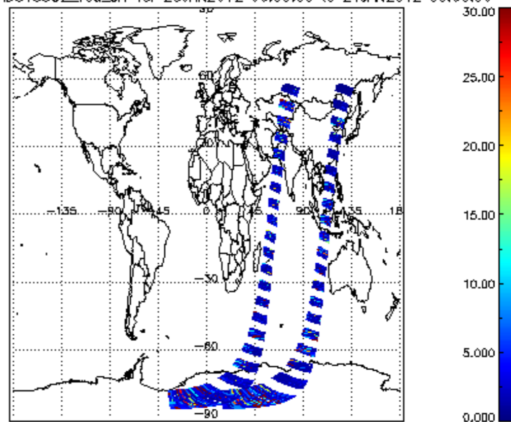
SCIOL2P_NADUV5S02_vcd_err for 23JAN2012 00:00:00 to 24JAN2012 00:00:00
