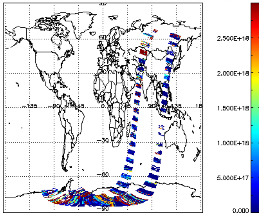
SCIOL2P_NADIR3CO_vcd for 23JAN2012 00:00:00 to 24JAN2012 00:00:00
