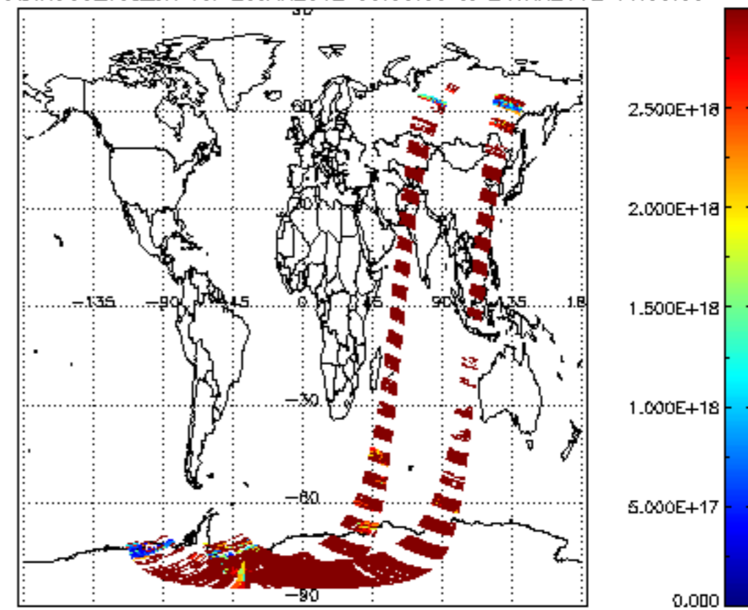
SCIOL2P_NADIR3CO_vcd_err for 23JAN2012 00:00:00 to 24JAN2012 00:00:00
