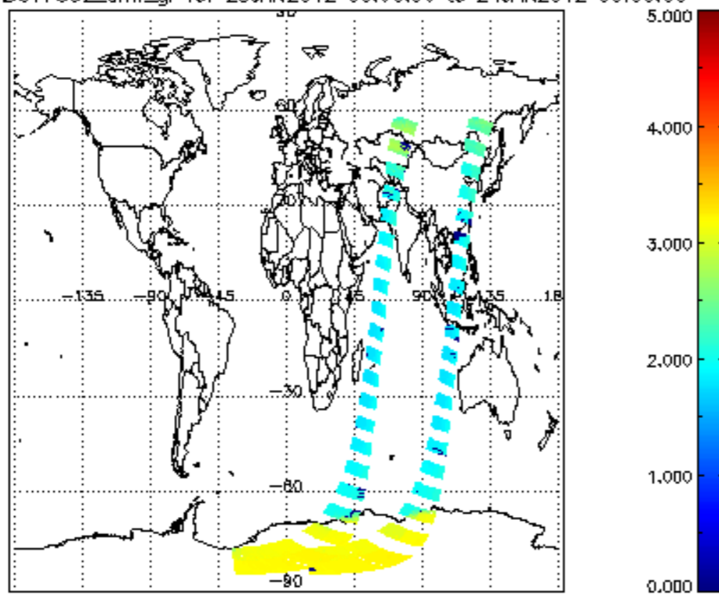
SCIOL2P_NADUV7S02_amf_gr for 23JAN2012 00:00:00 to 24JAN2012 00:00:00
