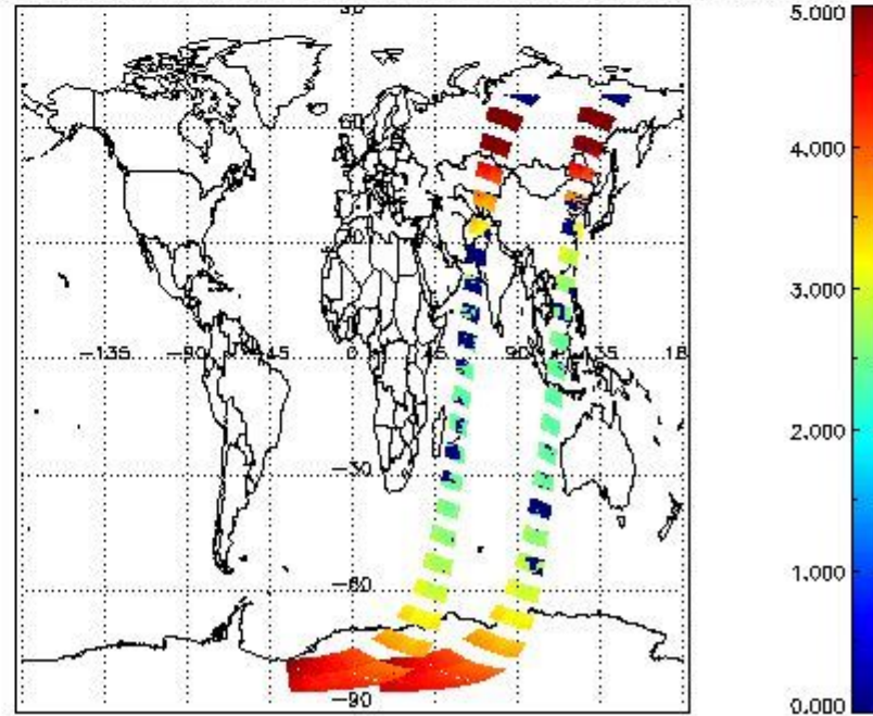
SCIOL2P_NADUV3BRO_amf_cl for 23JAN2012 00:00:00 to 24JAN2012 00:00:00
