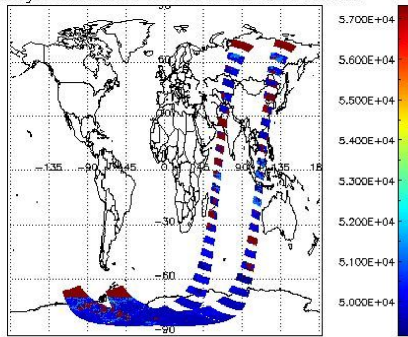
cloud_flags for 23JAN2012 00:00:00 to 24JAN2012 00:00:00
