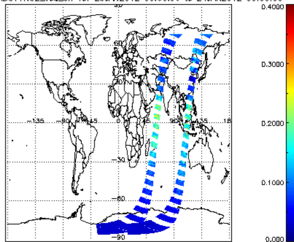
SCIOL2P_NADUV1NO2_vcd_err for 23JAN2012 00:00:00 to 24JAN2012 00:00:00
