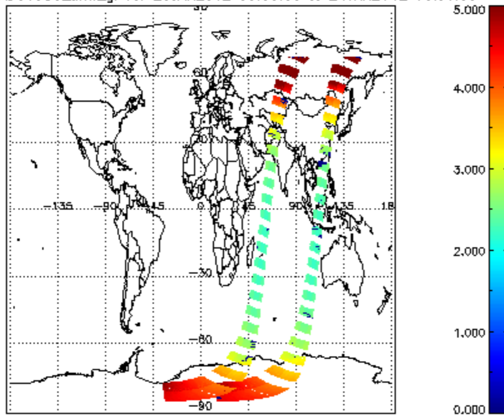
SCIOL2P_NADUV003_amf_gr for 23JAN2012 00:00:00 to 24JAN2012 00:00:00
