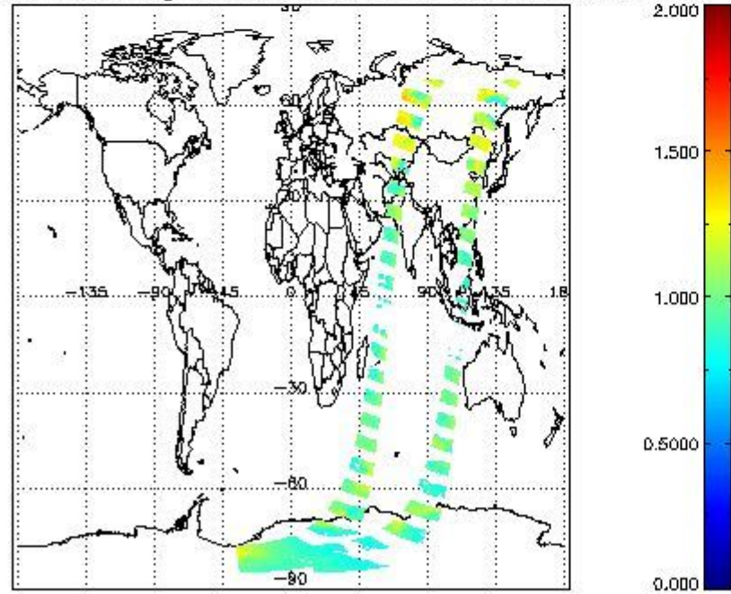
SCIOL2P_NADUV8H2O_amf_gr for 23JAN2012 00:00:00 to 24JAN2012 00:00:00
