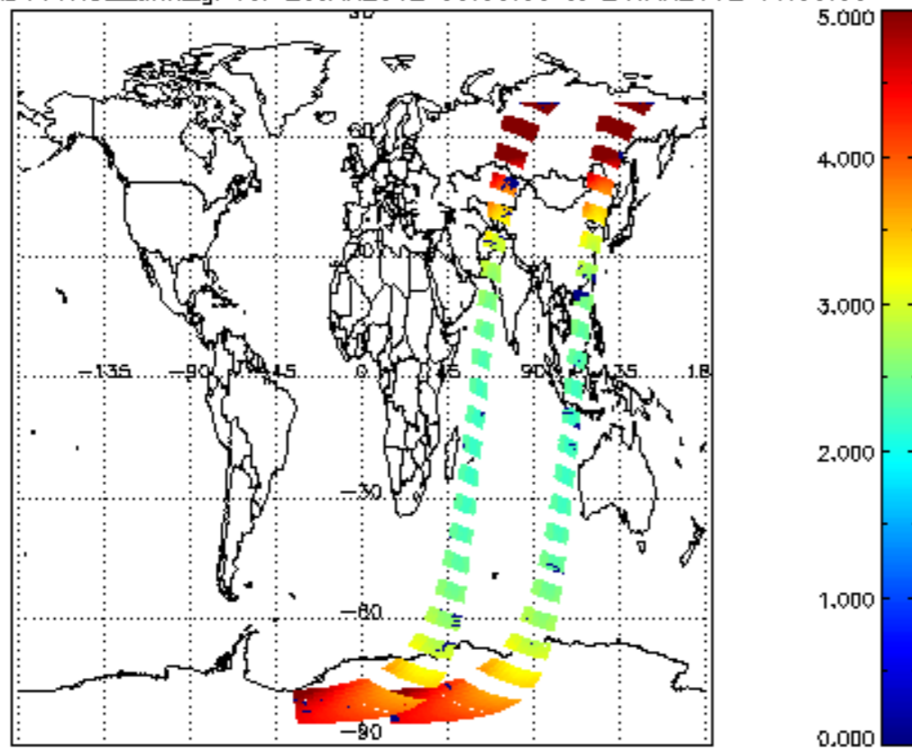
SCIOL2P_NADUV1NO2_amf_gr for 23JAN2012 00:00:00 to 24JAN2012 00:00:00
