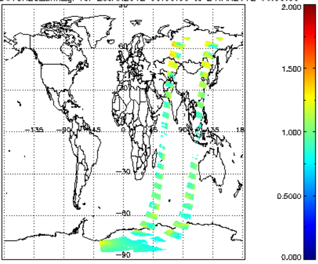
SCIOL2P_NADUVBH20_amf_gr for 23JAN2012 00:00:00 to 24JAN2012 00:00:00
