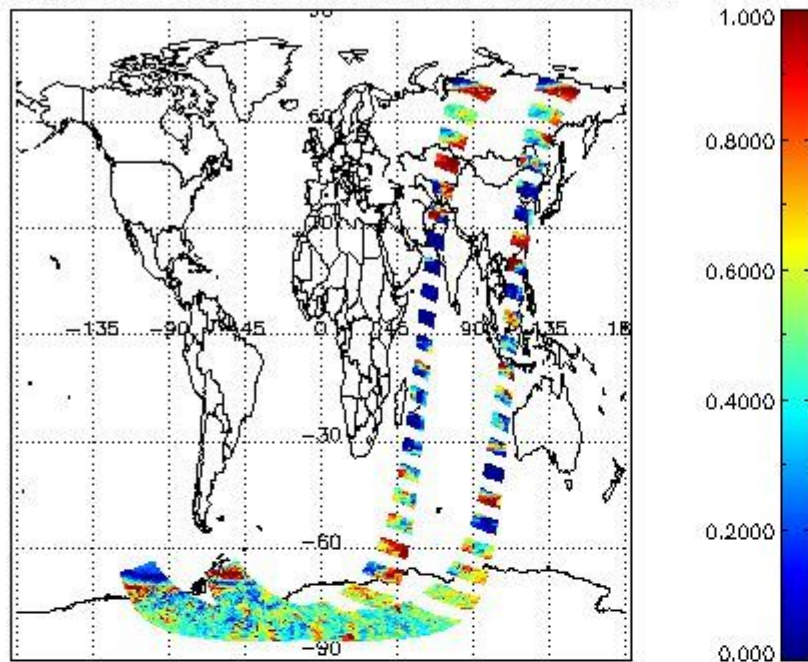
cL_frac for 23JAN2012 00:00:00 to 24JAN2012 00:00:00
