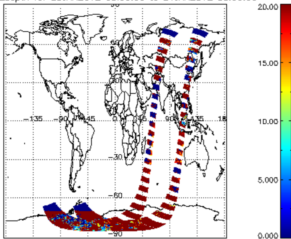
cL_opt_depth for 23JAN2012 00:00:00 to 24JAN2012 00:00:00
