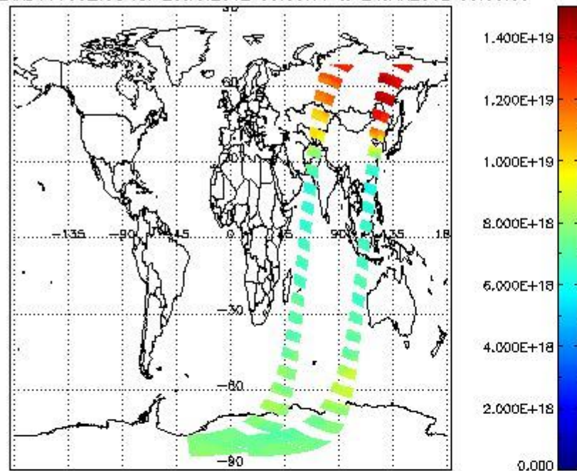
SCIOL2P_NADUV003_vcd for 23JAN2012 00:00:00 to 24JAN2012 00:00:00
