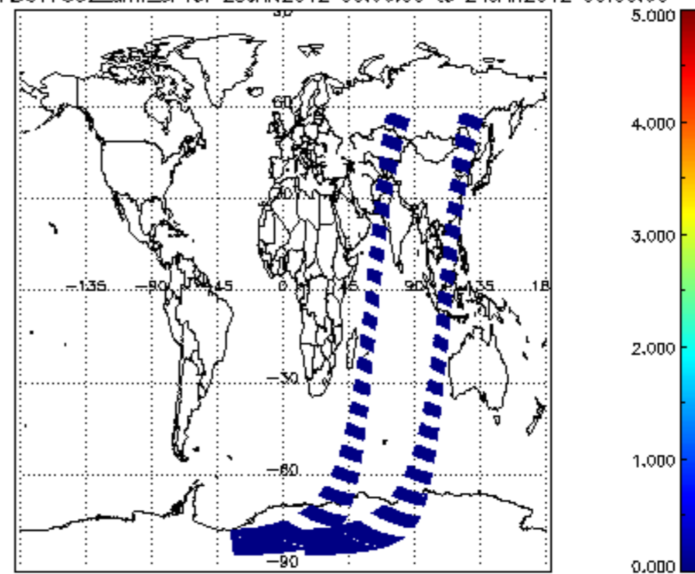
SCIOL2P_NADUV7S02_amf_cl for 23JAN2012 00:00:00 to 24JAN2012 00:00:00
