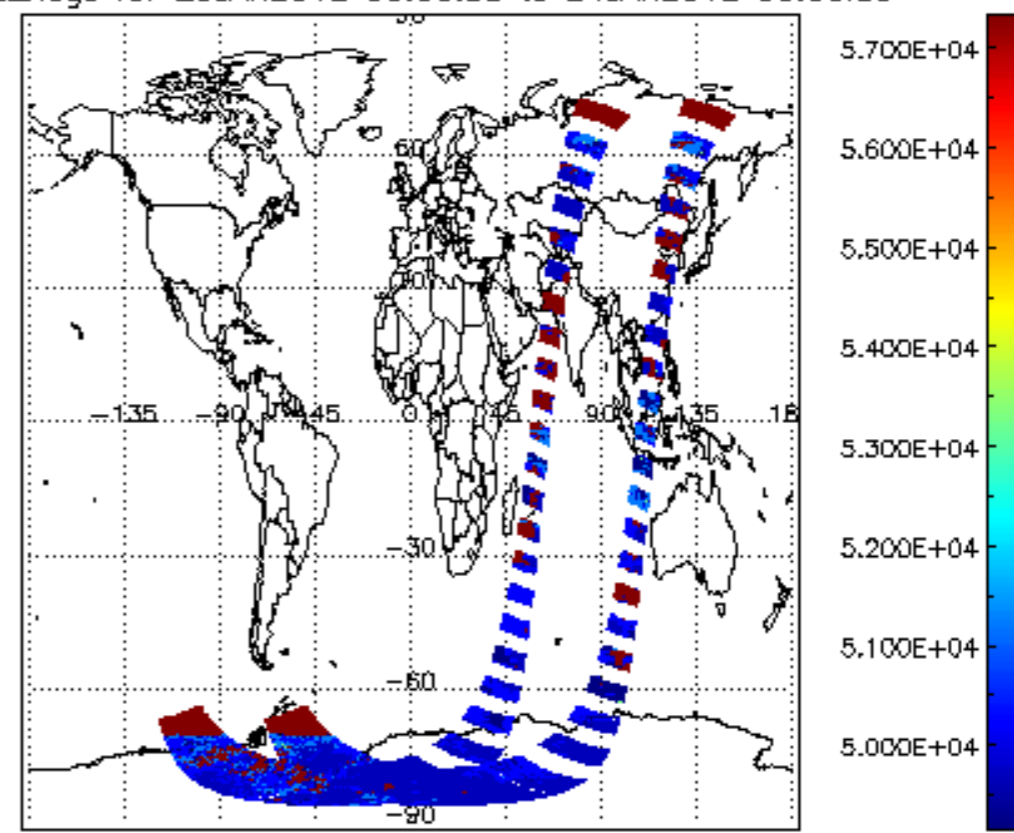
cloud_flags for 23JAN2012 00:00:00 to 24JAN2012 00:00:00
