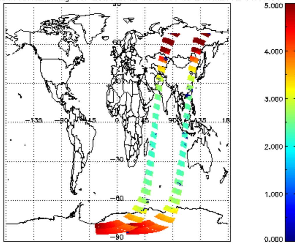
SCIOL2P_NADUV3BRO_amf_gr for 23JAN2012 00:00:00 to 24JAN2012 00:00:00
