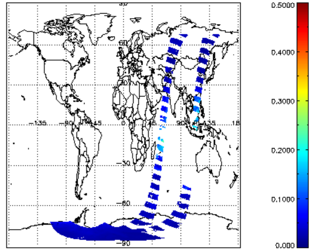
SCIOL2P_NADUVBH20_vcd_err for 23JAN2012 00:00:00 to 24JAN2012 00:00:00
