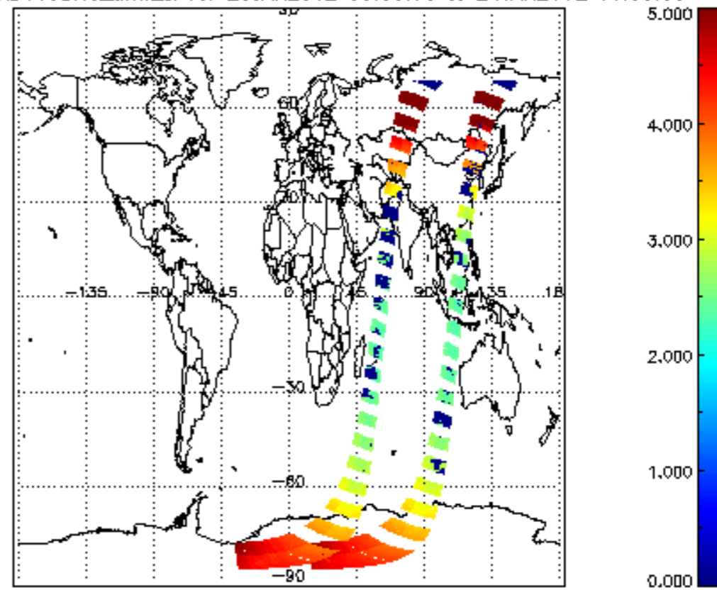
SCIOL2P_NADUV3BRO_amf_cl for 23JAN2012 00:00:00 to 24JAN2012 00:00:00
