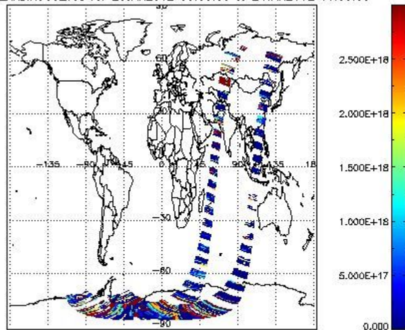
SCIDL2P_NADIR3CO_vcd for 23JAN2012 00:00:00 to 24JAN2012 00:00:00
