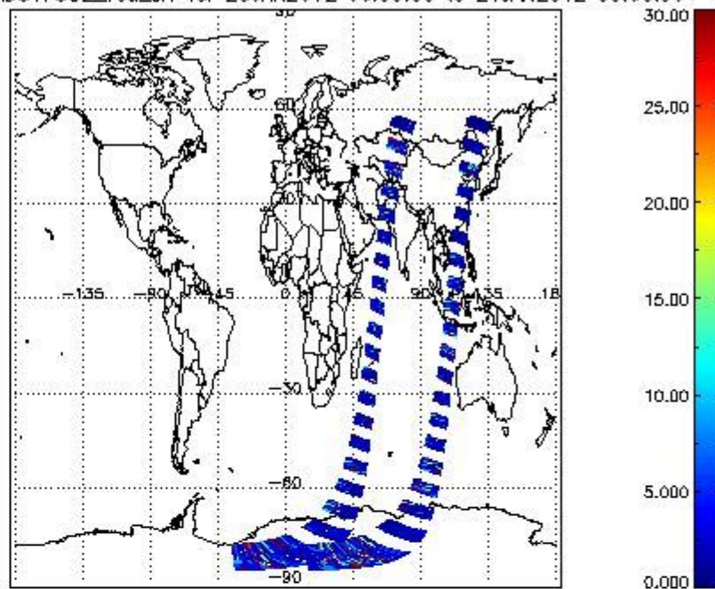
SCIOL2P_NADUV7S02_vcd_err for 23JAN2012 00:00:00 to 24JAN2012 00:00:00
