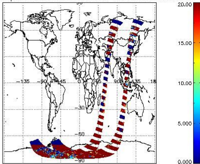
cLopt_depth for 23JAN2012 00:00:00 to 24JAN2012 00:00:00
