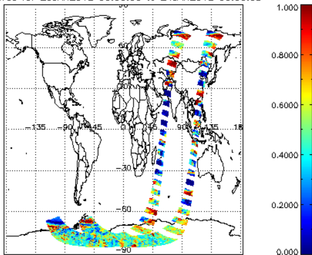
cL_frac for 23JAN2012 00:00:00 to 24JAN2012 00:00:00
