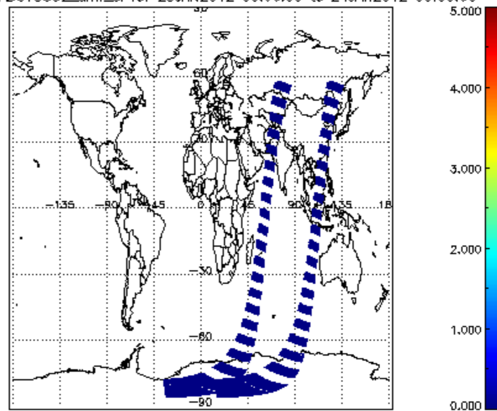
SCIOL2P_NADUV5S02_amf_cl for 23JAN2012 00:00:00 to 24JAN2012 00:00:00
