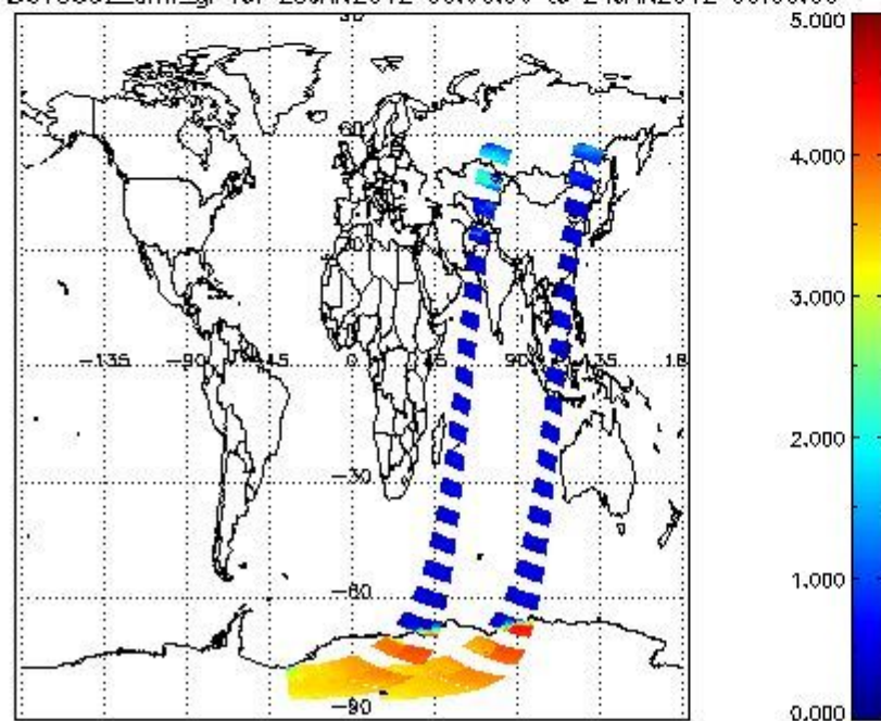
SCIOL2P_NADUV5SO2_amf_gr for 23JAN2012 00:00:00 to 24JAN2012 00:00:00
