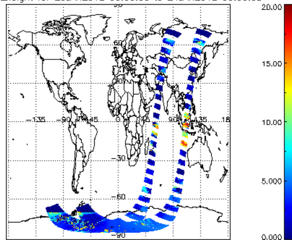
cL_top_height for 23JAN2012 00:00:00 to 24JAN2012 00:00:00
