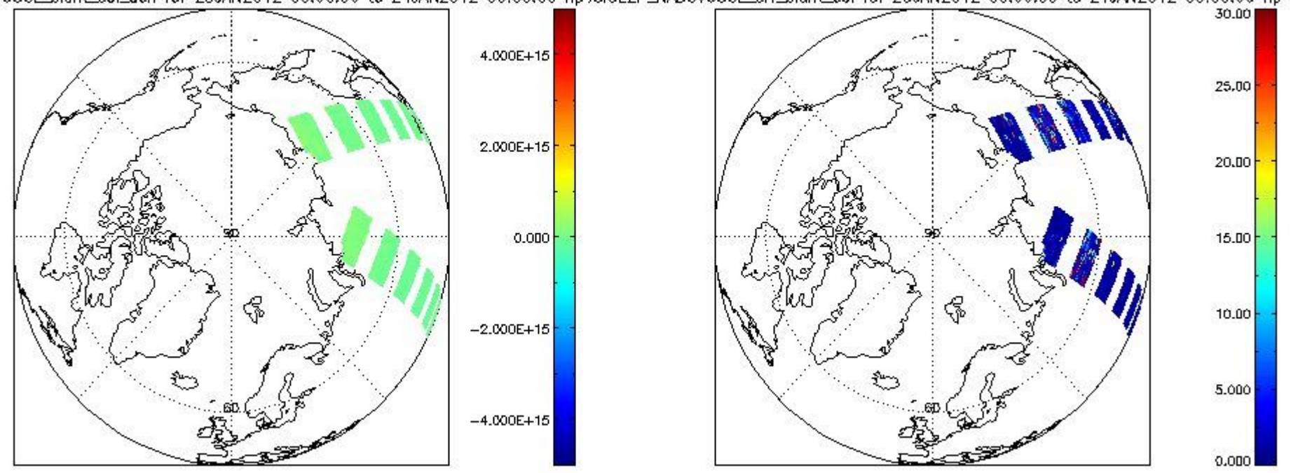
SCIDL2P_NADUV60CL_slant_col_den for 23JAN2012 00:00:00 to 24JAN2012 00:00:00 np; SCIDL2P_NADUV60CL_err_slant_col for 23JAN2012 00:00:00 to 24JAN2012 00:00:00 np
