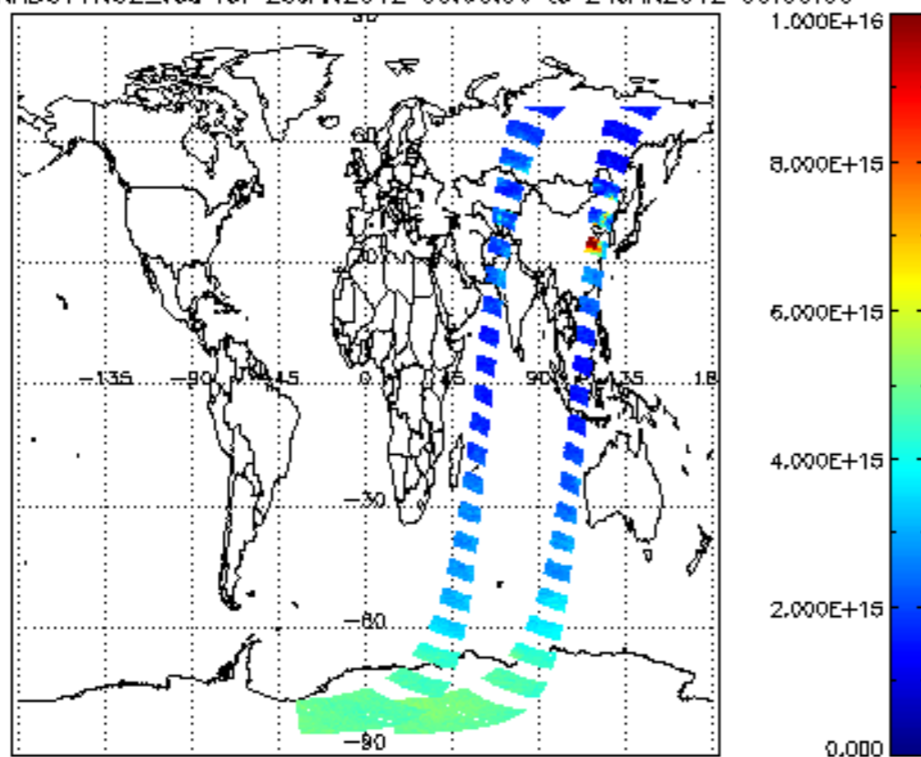
SCIOL2P_NADUV1NO2_vcd for 23JAN2012 00:00:00 to 24JAN2012 00:00:00
