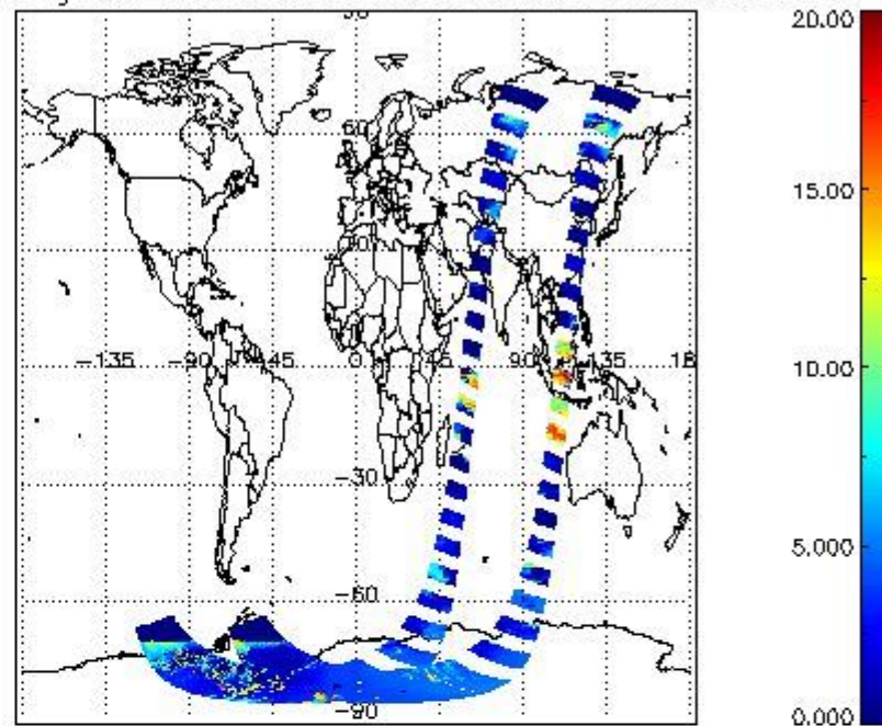
cL_top_height for 23JAN2012 00:00:00 to 24JAN2012 00:00:00
