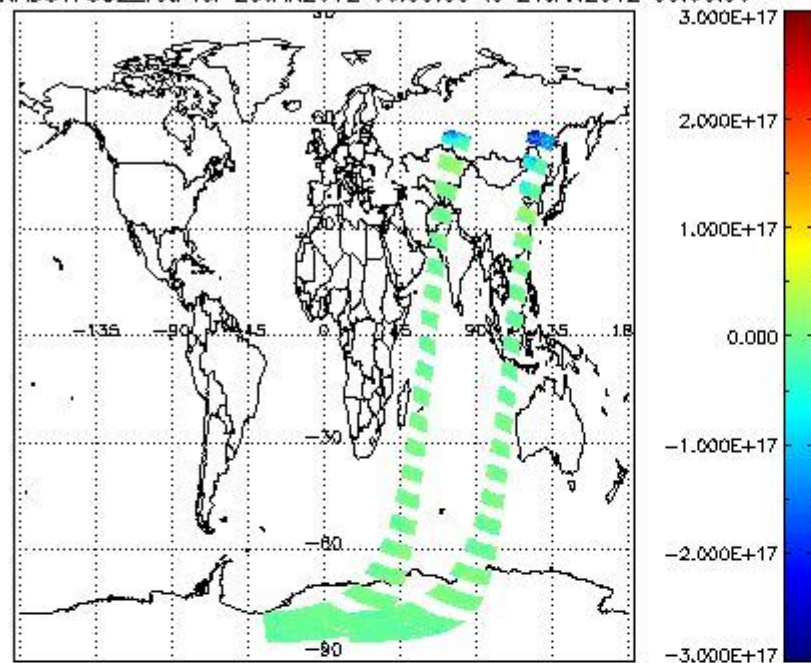
SCIOL2P_NADUV7S02_vcd for 23JAN2012 00:00:00 to 24JAN2012 00:00:00
