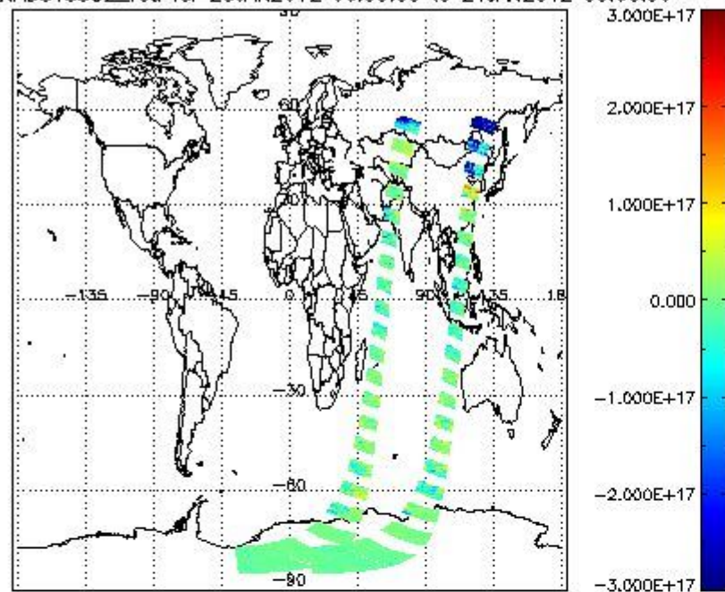
SCIOL2P_NADUV5SO2_vcd for 23JAN2012 00:00:00 to 24JAN2012 00:00:00
