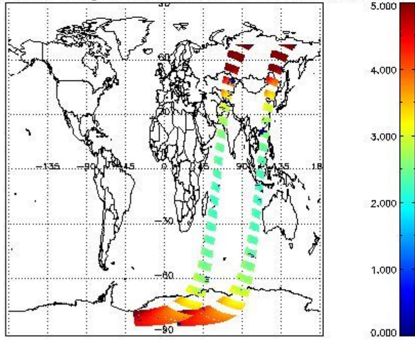
SCIOL2P_NADUV1NO2_amf_gr for 23JAN2012 00:00:00 to 24JAN2012 00:00:00
