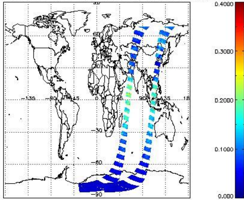
SCIOL2P_NADUV1NO2_vcd_err for 23JAN2012 00:00:00 to 24JAN2012 00:00:00
