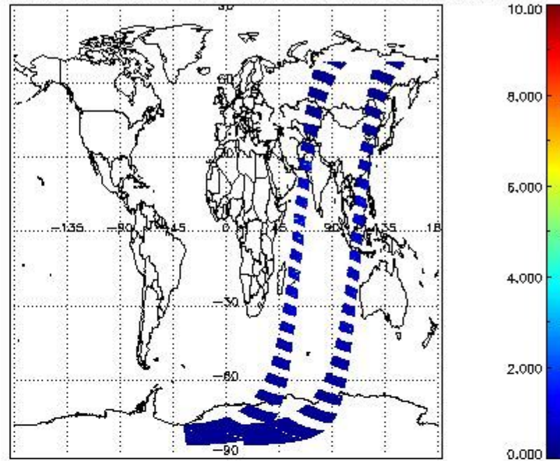
SCIOL2P_NADUV3BRO_vcd_err for 23JAN2012 00:00:00 to 24JAN2012 00:00:00
