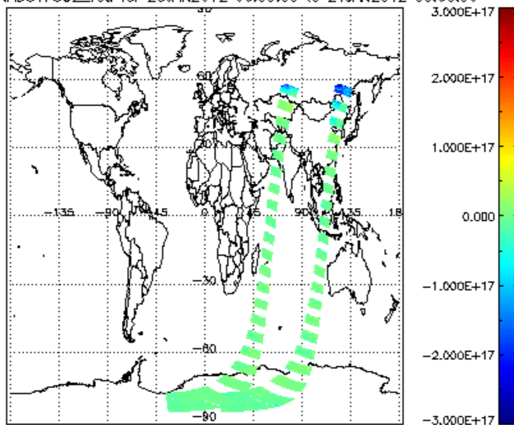
SCIOL2P_NADUV7S02_vcd for 23JAN2012 00:00:00 to 24JAN2012 00:00:00
