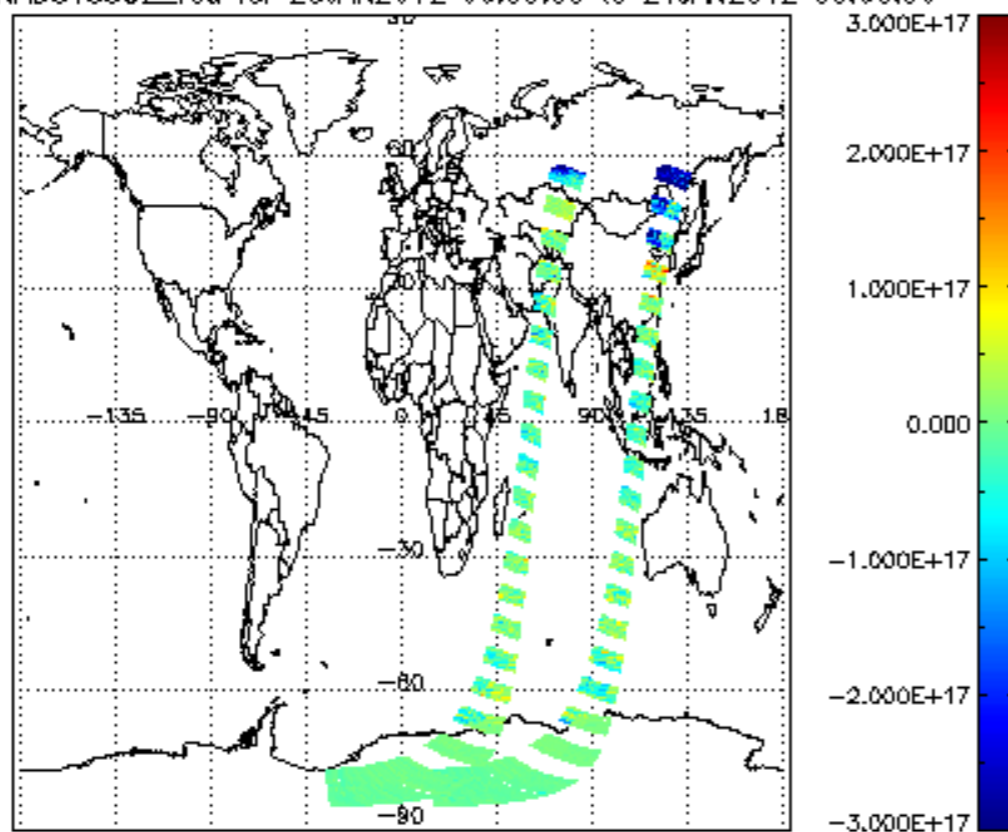
SCIOL2P_NADUV5S02_vcd for 23JAN2012 00:00:00 to 24JAN2012 00:00:00
