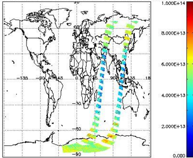
SCIOL2P_NADUV3BRO_vcd for 23JAN2012 00:00:00 to 24JAN2012 00:00:00
