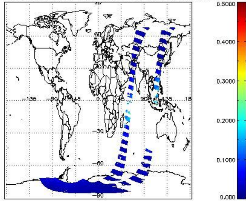
SCIOL2P_NADUV8H2O_vcd_err for 23JAN2012 00:00:00 to 24JAN2012 00:00:00
