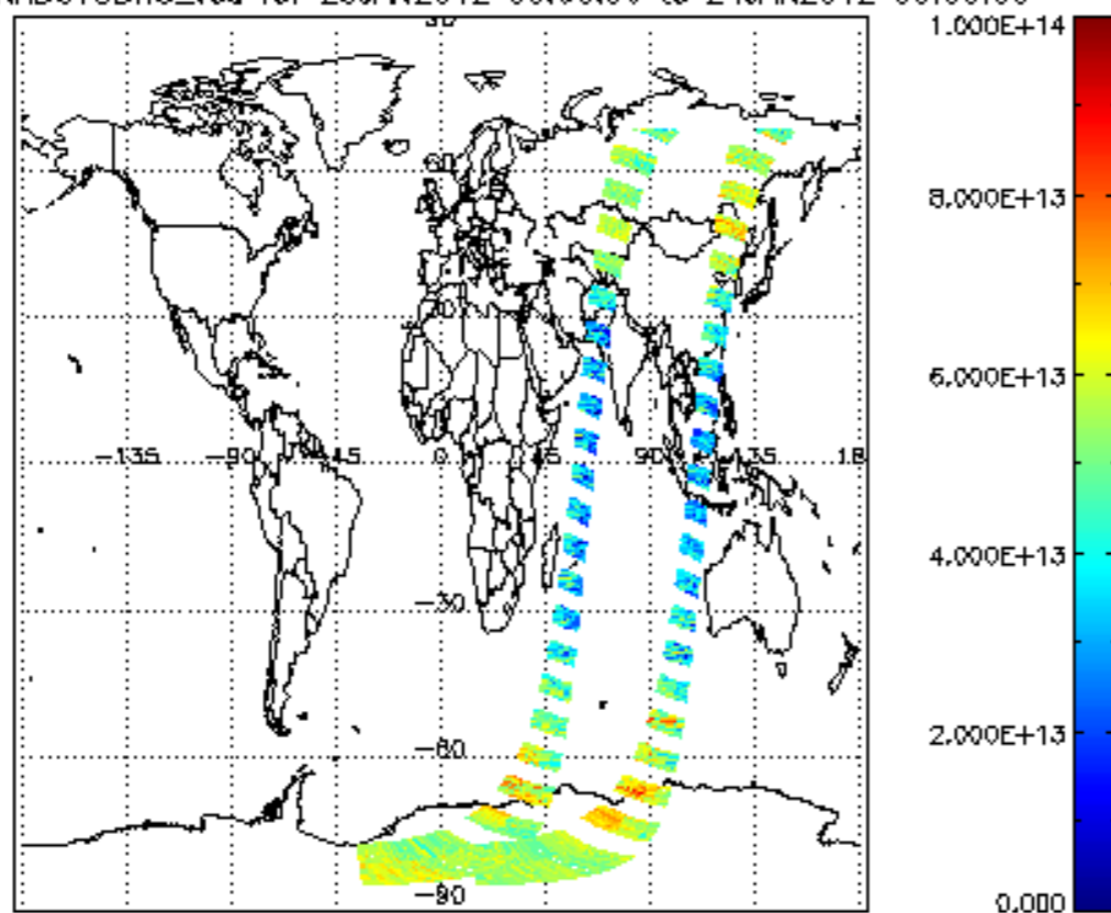
SCIOL2P_NADUV3BRO_vcd for 23JAN2012 00:00:00 to 24JAN2012 00:00:00
