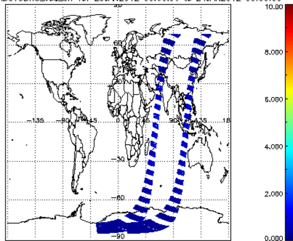
SCIOL2P_NADUV3BRO_vcd_err for 23JAN2012 00:00:00 to 24JAN2012 00:00:00
