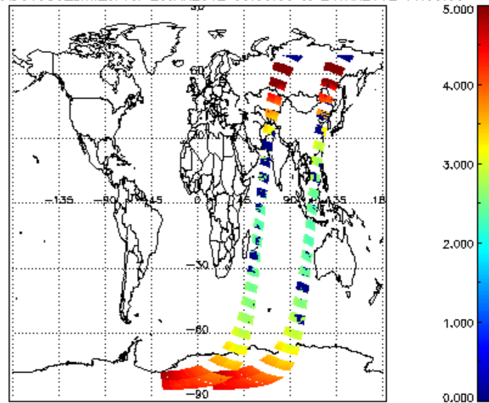
SCIOL2P_NADUV003_amf_cl for 23JAN2012 00:00:00 to 24JAN2012 00:00:00
