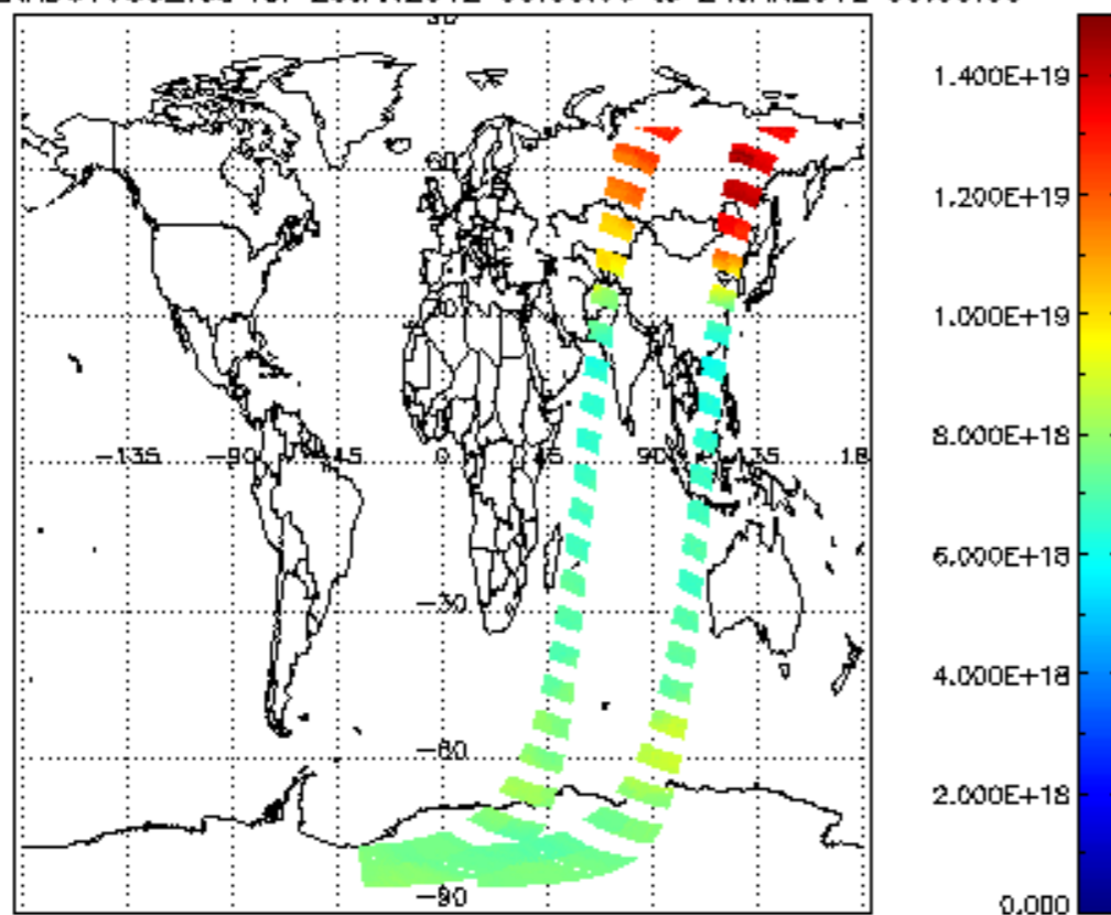
SCIOL2P_NADUV003_vcd for 23JAN2012 00:00:00 to 24JAN2012 00:00:00
