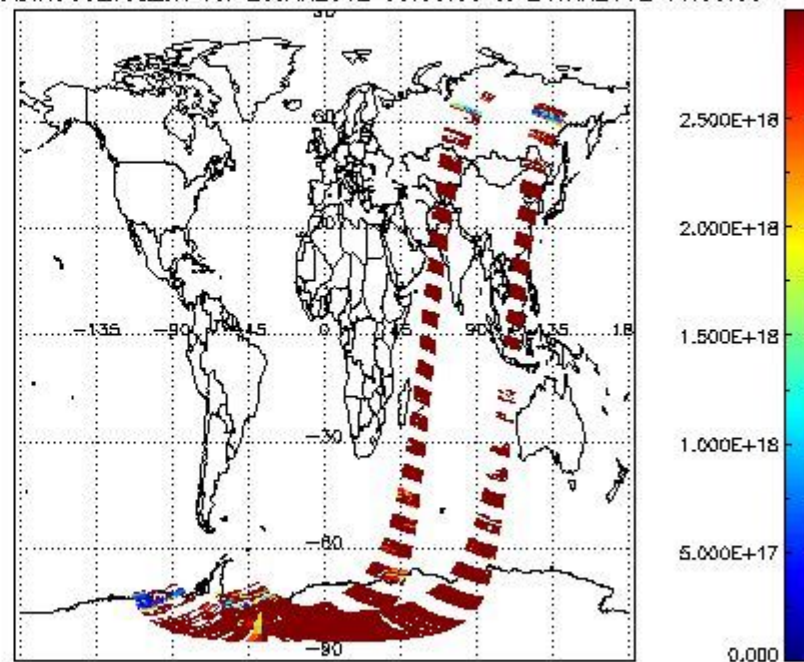
SCIDL2P_NADIR3CO_vcd_err for 23JAN2012 00:00:00 to 24JAN2012 00:00:00
