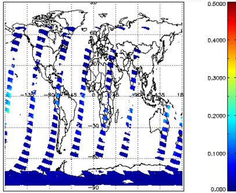
SCIOL2P_NADUV8H2O_vcd_err for 22JAN2012 00:00:00 to 23JAN2012 00:00:00
