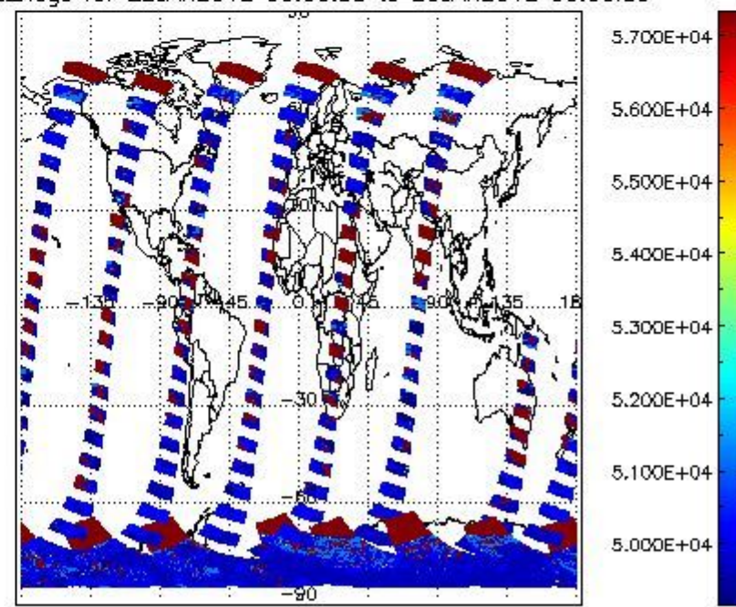
cloud_flags for 22JAN2012 00:00:00 to 23JAN2012 00:00:00
