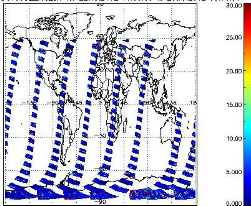
SCIOL2P_NADUV5SO2_vcd_err for 22JAN2012 00:00:00 to 23JAN2012 00:00:00
