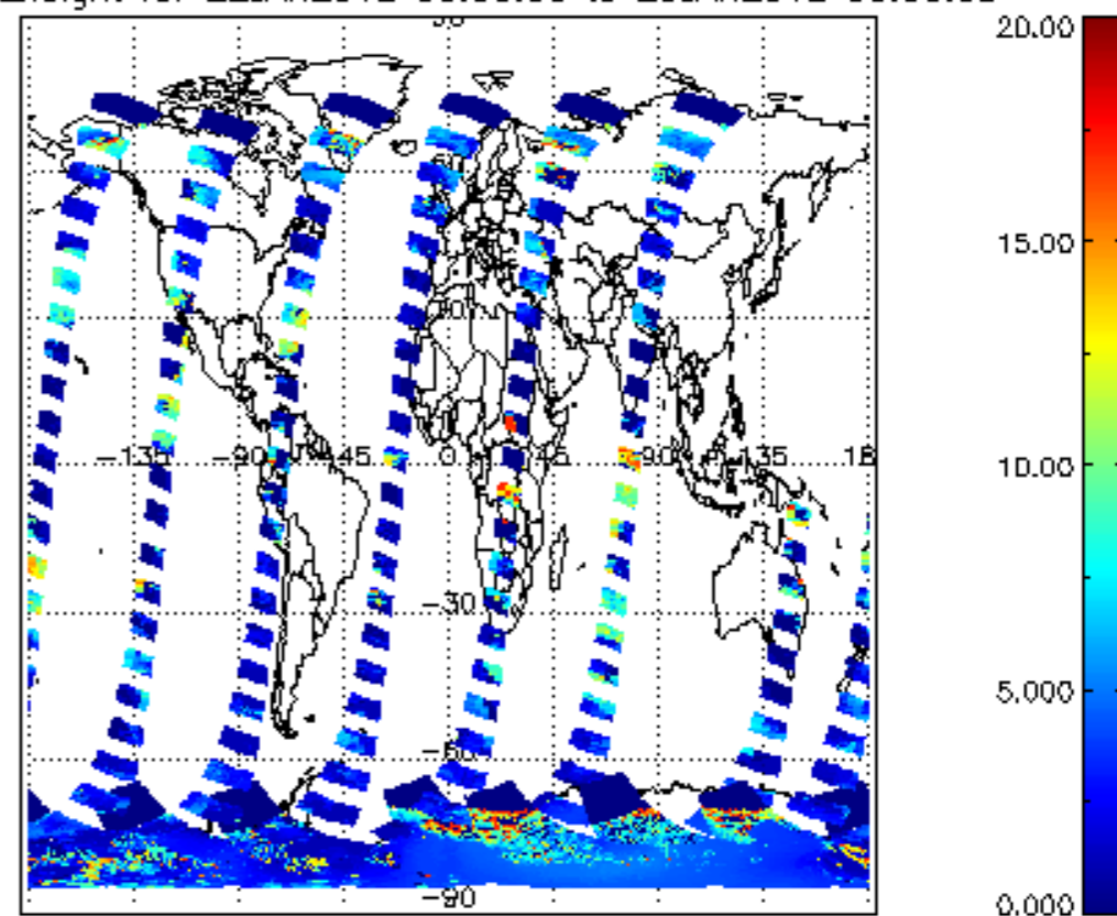
cL_top_height for 22JAN2012 00:00:00 to 23JAN2012 00:00:00
