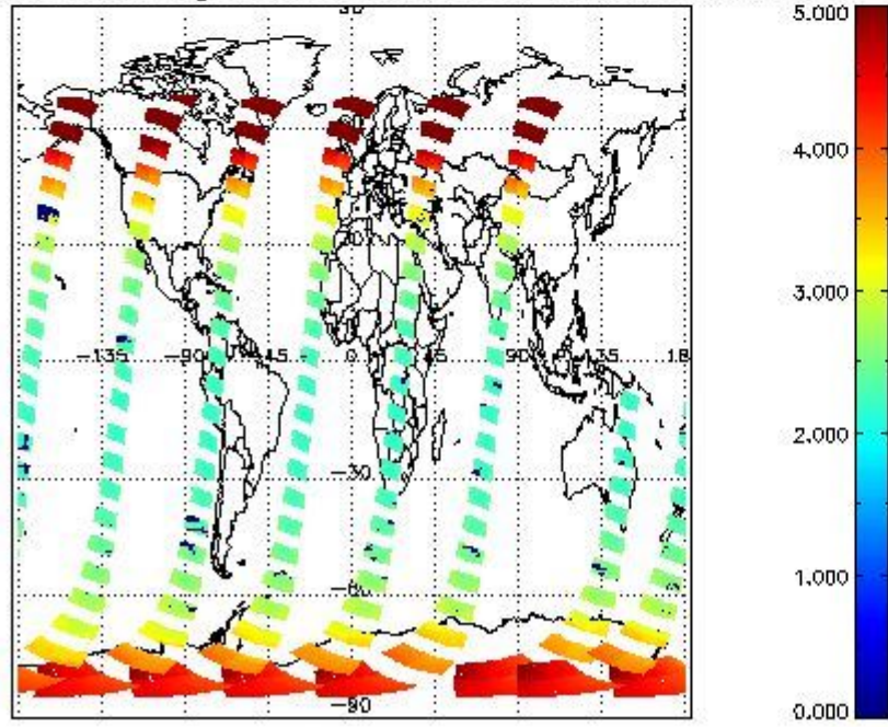
SCIOL2P_NADUV3BRO_amf_gr for 22JAN2012 00:00:00 to 23JAN2012 00:00:00
