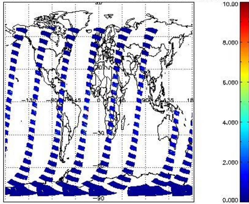
SCIOL2P_NADUV3BRO_vcd_err for 22JAN2012 00:00:00 to 23JAN2012 00:00:00
