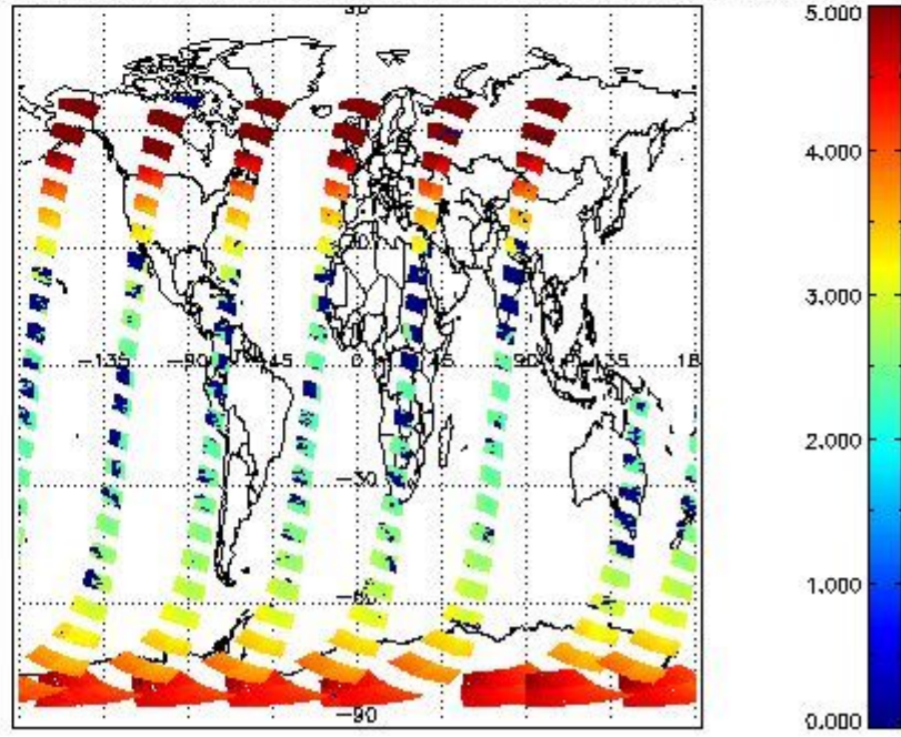
SCIOL2P_NADUV3BRO_amf_cl for 22JAN2012 00:00:00 to 23JAN2012 00:00:00
