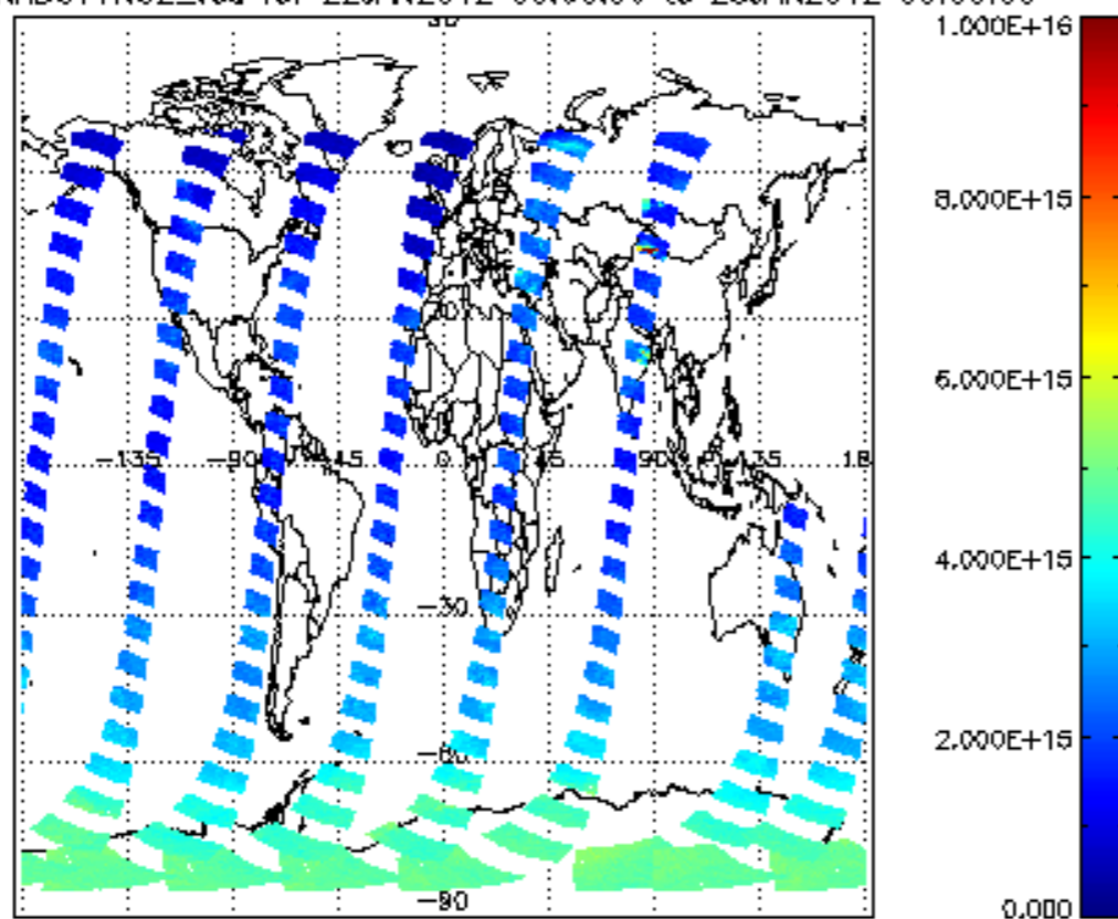
SCIOL2P_NADUV1NO2_vcd for 22JAN2012 00:00:00 to 23JAN2012 00:00:00
