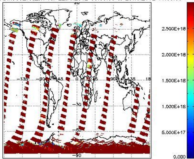
SCIDL2P_NADIR3CO_vcd_err for 22JAN2012 00:00:00 to 23JAN2012 00:00:00
