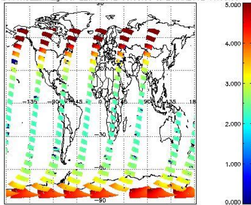
SCIOL2P_NADUV1NO2_amf_gr for 22JAN2012 00:00:00 to 23JAN2012 00:00:00
