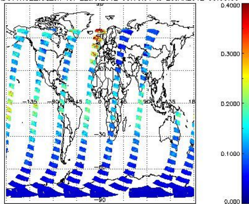
SCIOL2P_NADUV1NO2_vcd_err for 22JAN2012 00:00:00 to 23JAN2012 00:00:00
