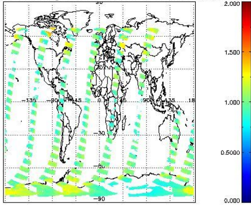
SCIOL2P_NADUV8H2O_amf_gr for 22JAN2012 00:00:00 to 23JAN2012 00:00:00
