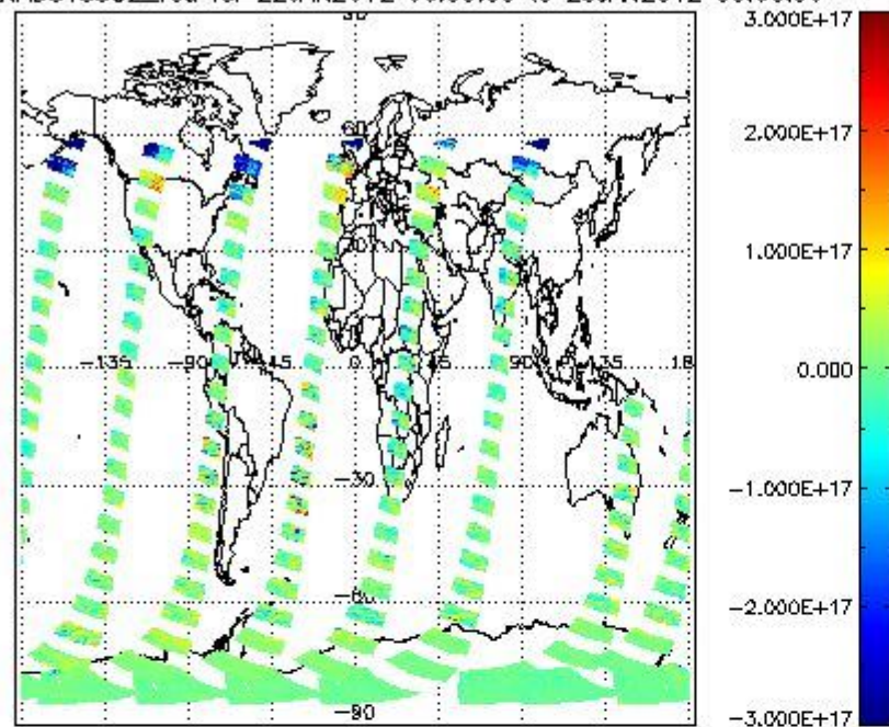
SCIOL2P_NADUV5SO2_vcd for 22JAN2012 00:00:00 to 23JAN2012 00:00:00
