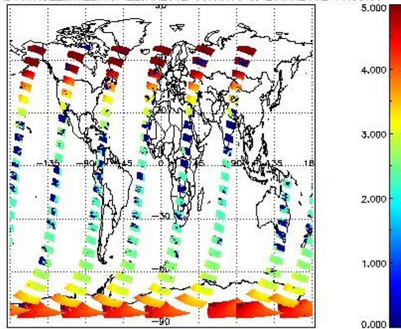
SCIOL2P_NADUV1NO2_amf_cl for 22JAN2012 00:00:00 to 23JAN2012 00:00:00
