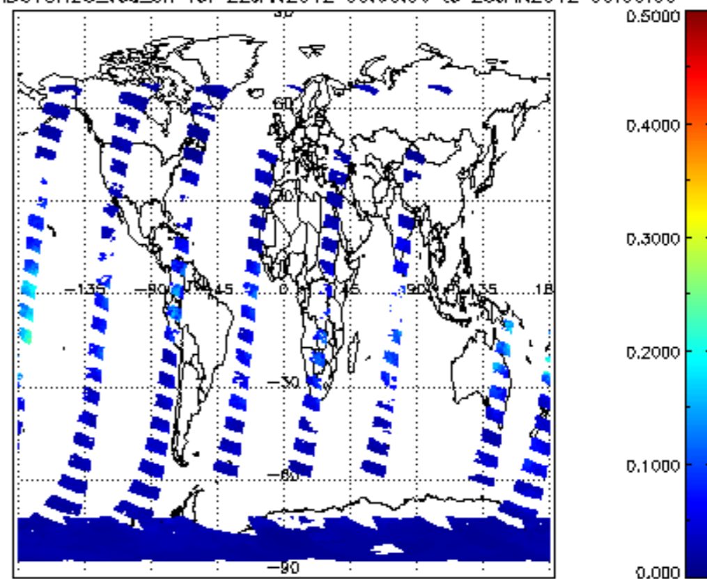
SCIOL2P_NADUV8H20_vcd_err for 22JAN2012 00:00:00 to 23JAN2012 00:00:00
