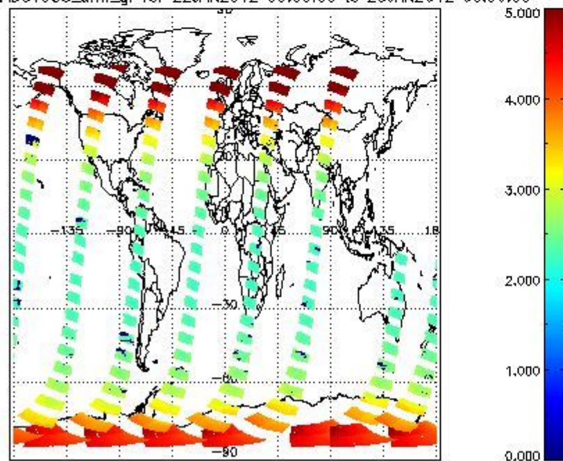
SCIOL2P_NADUV003_amf_gr for 22JAN2012 00:00:00 to 23JAN2012 00:00:00
