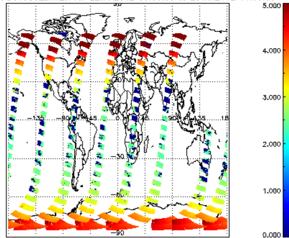
SCIOL2P_NADUV003_amf_cl for 22JAN2012 00:00:00 to 23JAN2012 00:00:00
