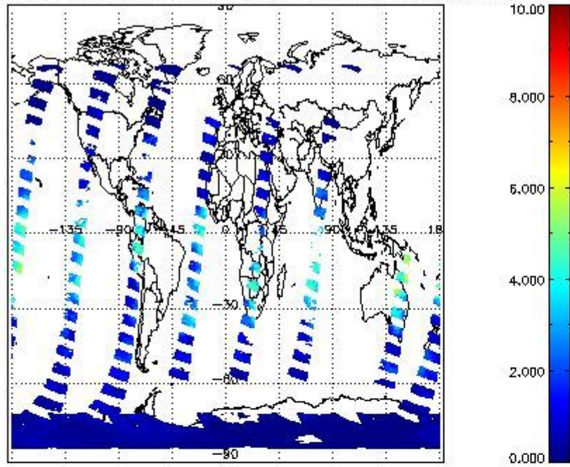
SCIOL2P_NADUV8H2O_vcd for 22JAN2012 00:00:00 to 23JAN2012 00:00:00
