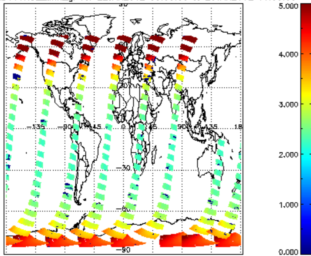
SCIOL2P_NADUV1NO2_amf_gr for 22JAN2012 00:00:00 to 23JAN2012 00:00:00
