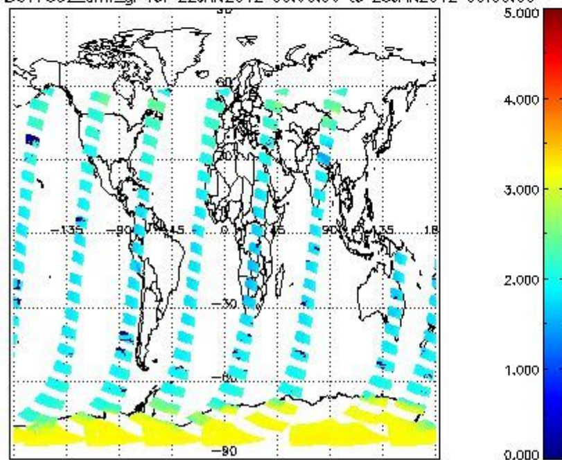
SCIOL2P_NADUV7S02_amf_gr for 22JAN2012 00:00:00 to 23JAN2012 00:00:00
