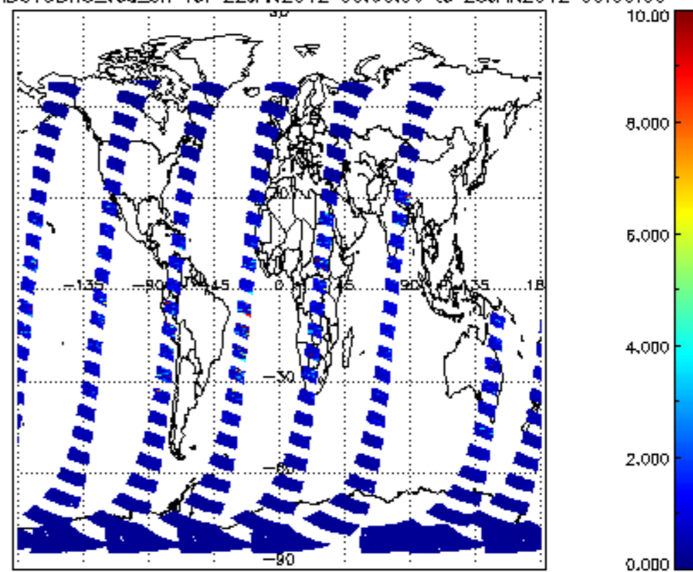
SCIOL2P_NADUV3BRO_vcd_err for 22JAN2012 00:00:00 to 23JAN2012 00:00:00
