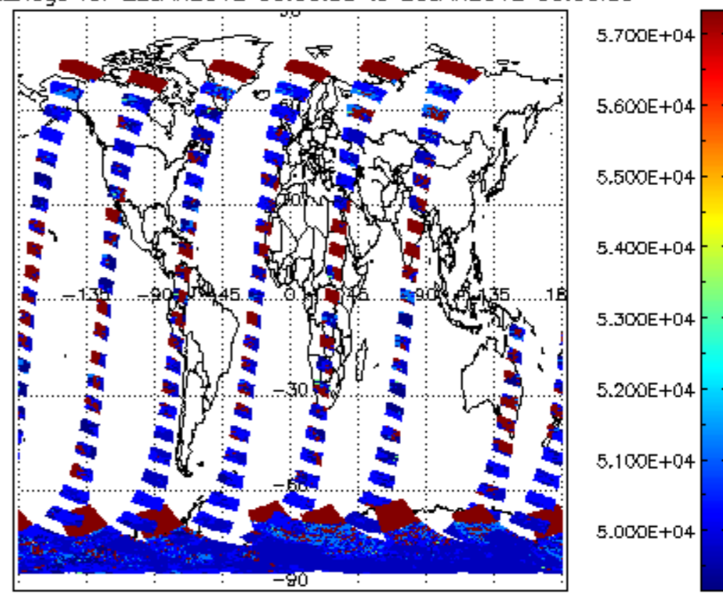
cloud_flags for 22JAN2012 00:00:00 to 23JAN2012 00:00:00
