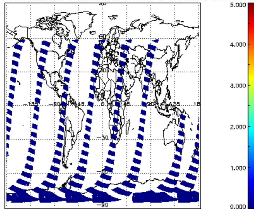
SCIOL2P_NADUV5S02_amf_sl for 22JAN2012 00:00:00 to 23JAN2012 00:00:00
