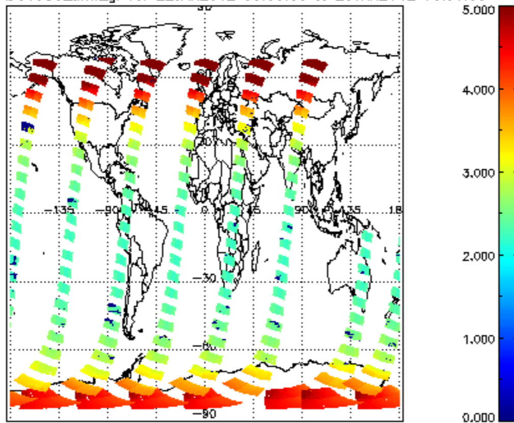
SCIOL2P_NADUV003_amf_gr for 22JAN2012 00:00:00 to 23JAN2012 00:00:00
