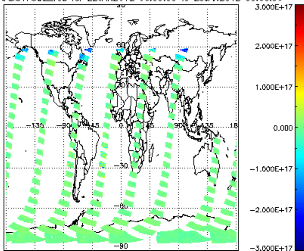
SCIOL2P_NADUV7S02_vcd for 22JAN2012 00:00:00 to 23JAN2012 00:00:00
