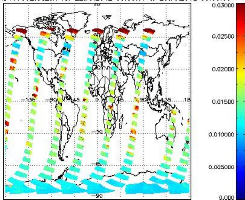
SCIOL2P_NADUV003_vcd_err for 22JAN2012 00:00:00 to 23JAN2012 00:00:00
