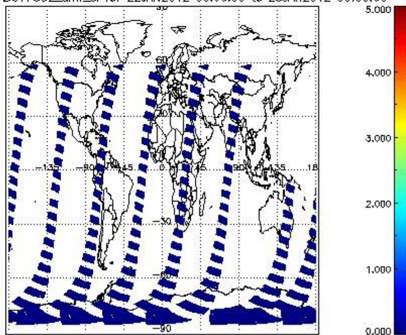
SCIOL2P_NADUV7S02_amf_cl for 22JAN2012 00:00:00 to 23JAN2012 00:00:00
