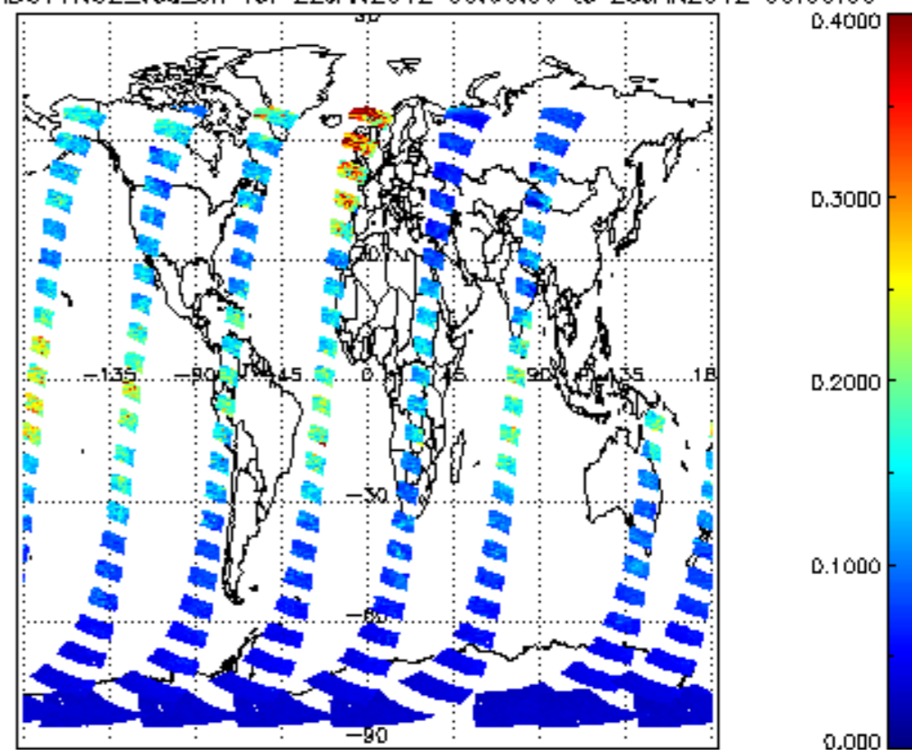
SCIOL2P_NADUV1NO2_vcd_err for 22JAN2012 00:00:00 to 23JAN2012 00:00:00
