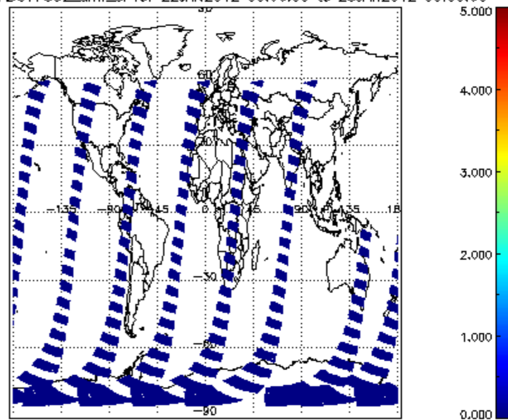
SCIOL2P_NADUV7S02_amf_sl for 22JAN2012 00:00:00 to 23JAN2012 00:00:00
