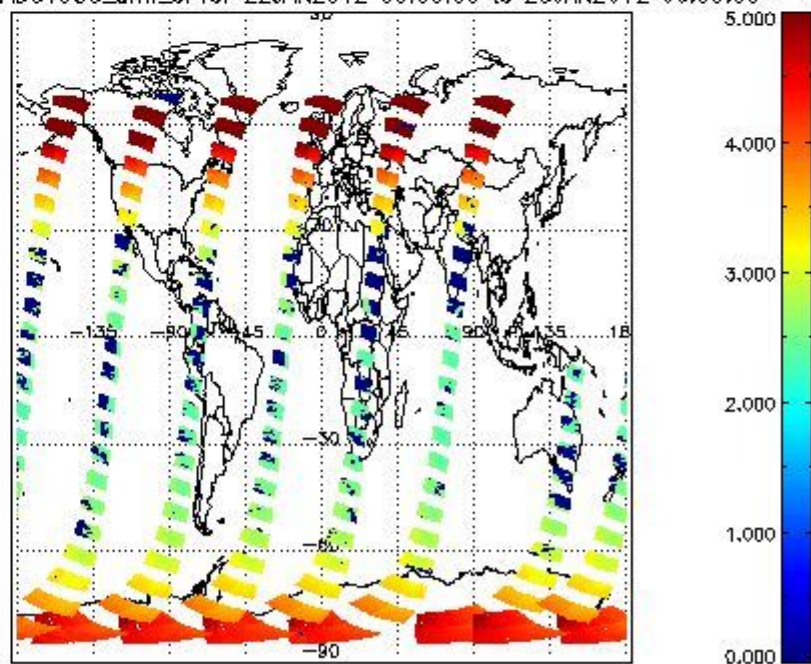
SCIOL2P_NADUV003_amf_cl for 22JAN2012 00:00:00 to 23JAN2012 00:00:00
