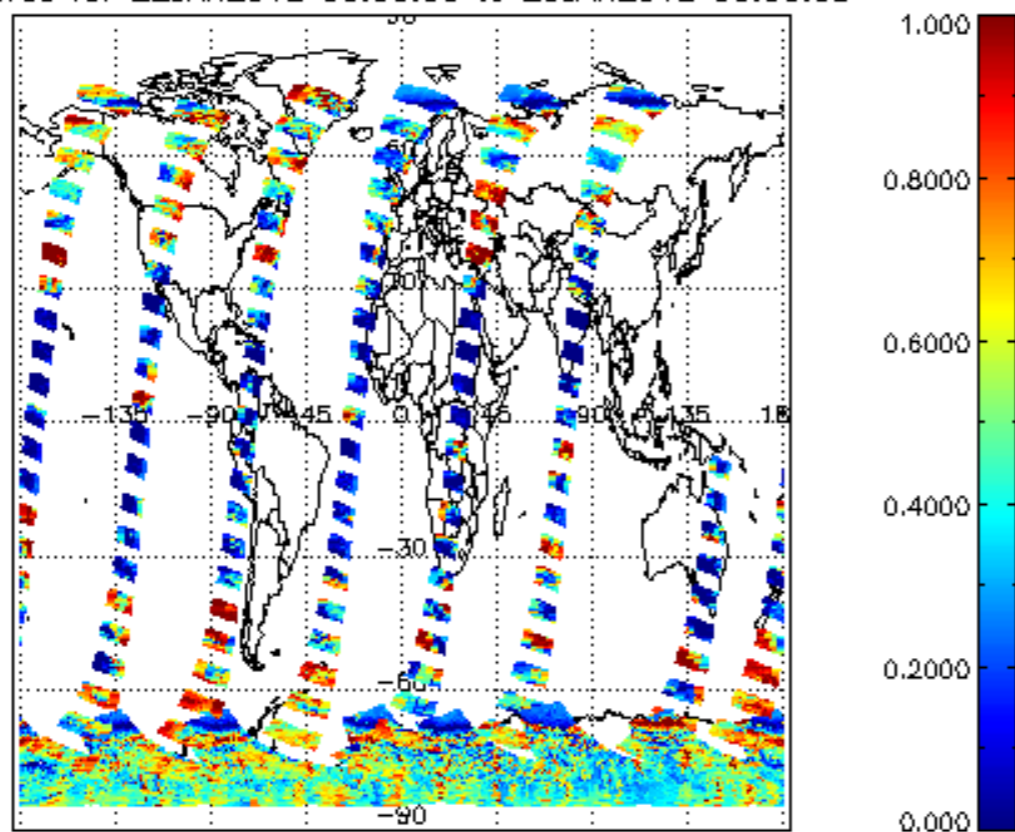
cL_frac for 22JAN2012 00:00:00 to 23JAN2012 00:00:00
