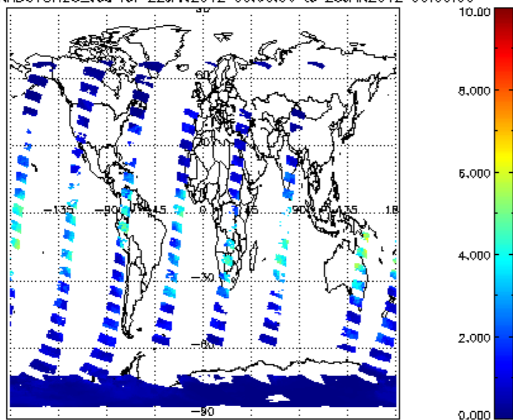
SCIOL2P_NADUV8H20_vcd for 22JAN2012 00:00:00 to 23JAN2012 00:00:00
