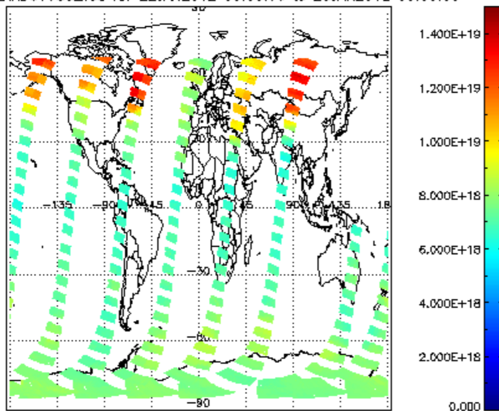
SCIOL2P_NADUV003_vcd for 22JAN2012 00:00:00 to 23JAN2012 00:00:00
