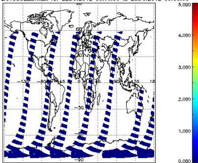
SCIOL2P_NADUV5SO2_amf_cl for 22JAN2012 00:00:00 to 23JAN2012 00:00:00
