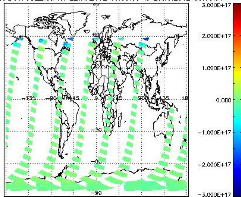
SCIOL2P_NADUV7S02_vcd for 22JAN2012 00:00:00 to 23JAN2012 00:00:00
