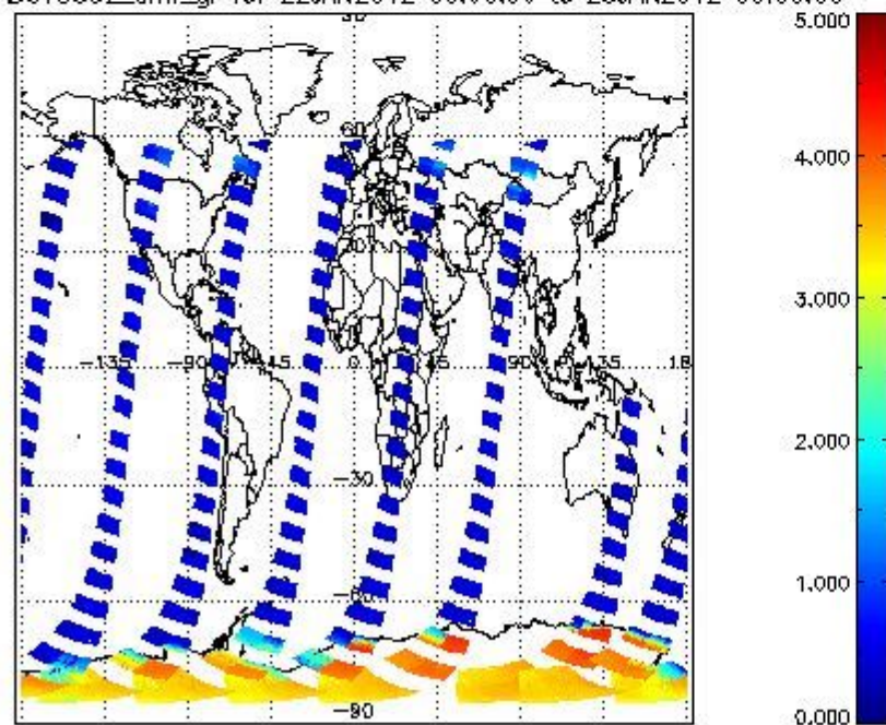
SCIOL2P_NADUV5SO2_amf_gr for 22JAN2012 00:00:00 to 23JAN2012 00:00:00
