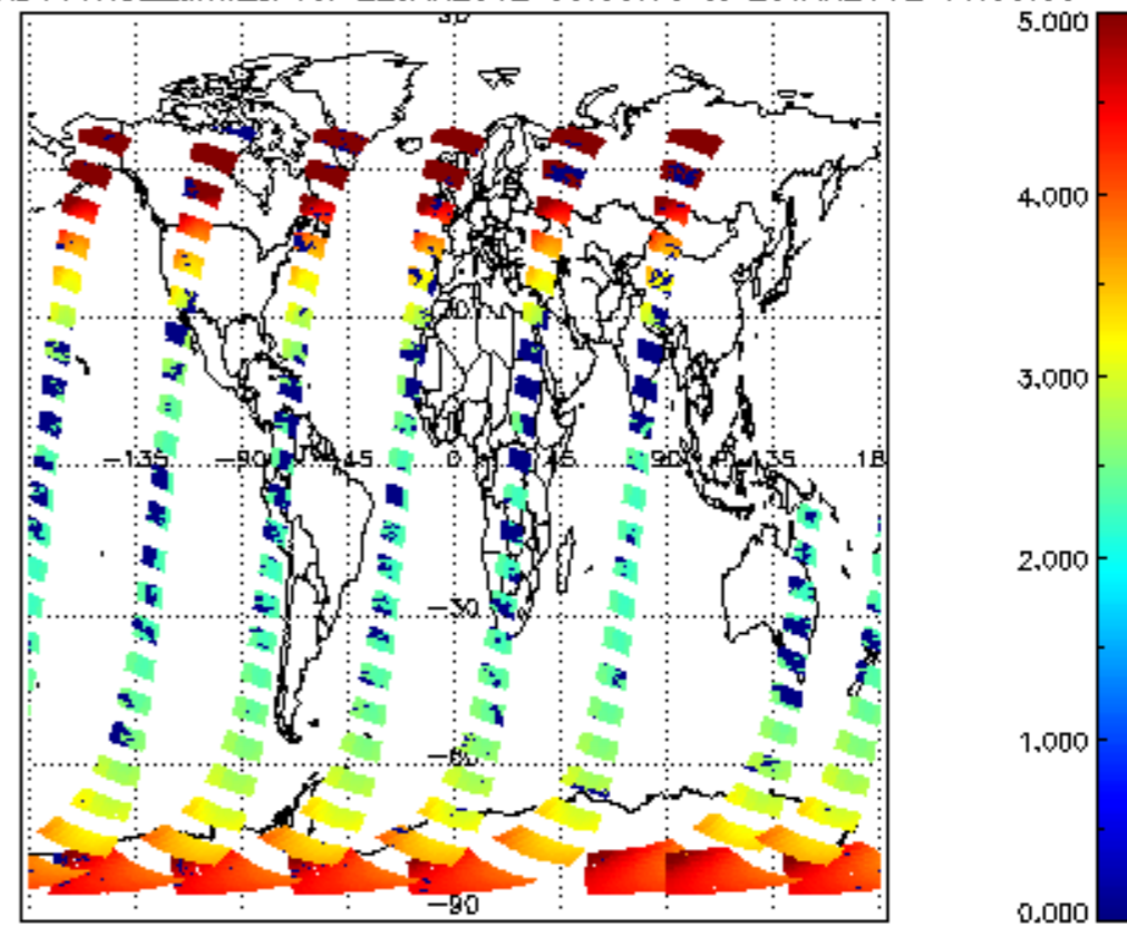
SCIOL2P_NADUV1NO2_amf_cl for 22JAN2012 00:00:00 to 23JAN2012 00:00:00
