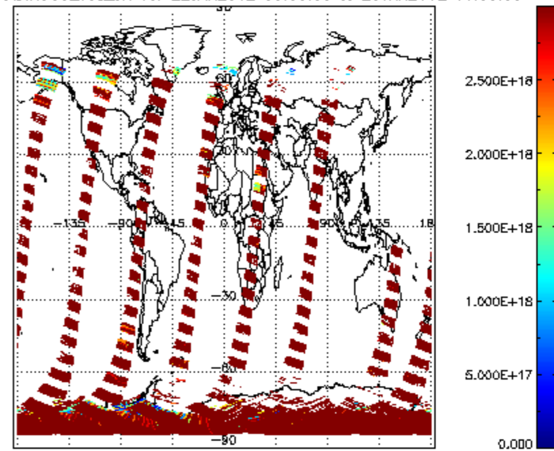
SCIOL2P_NADIR3CO_vcd_err for 22JAN2012 00:00:00 to 23JAN2012 00:00:00
