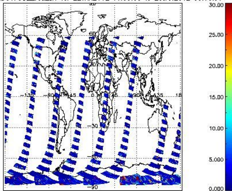
SCIOL2P_NADUV7S02_vcd_err for 22JAN2012 00:00:00 to 23JAN2012 00:00:00
