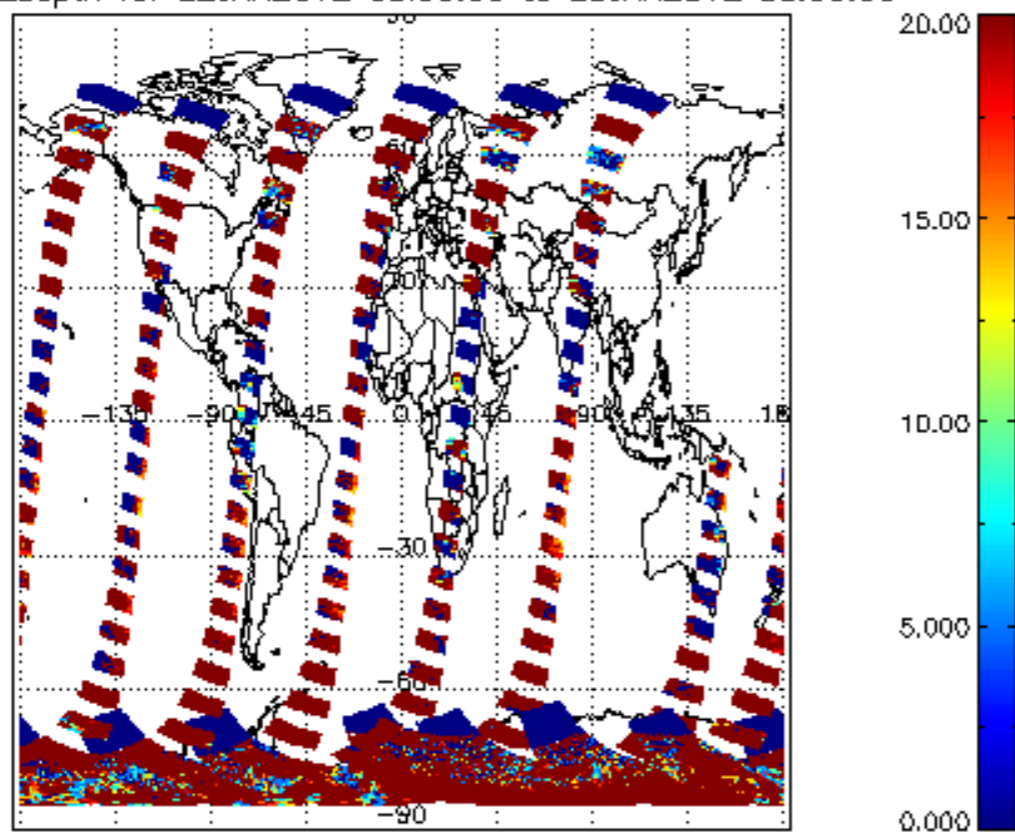
cLopt_depth for 22JAN2012 00:00:00 to 23JAN2012 00:00:00
