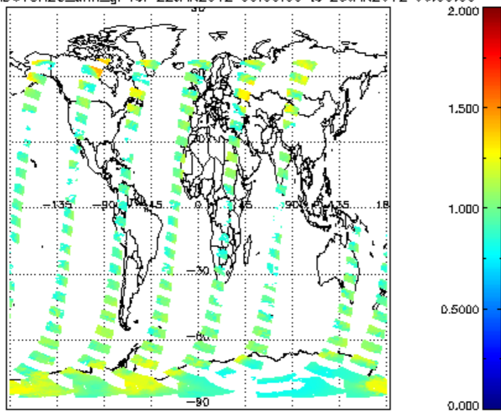
SCIOL2P_NADUV8H20_amf_gr for 22JAN2012 00:00:00 to 23JAN2012 00:00:00
