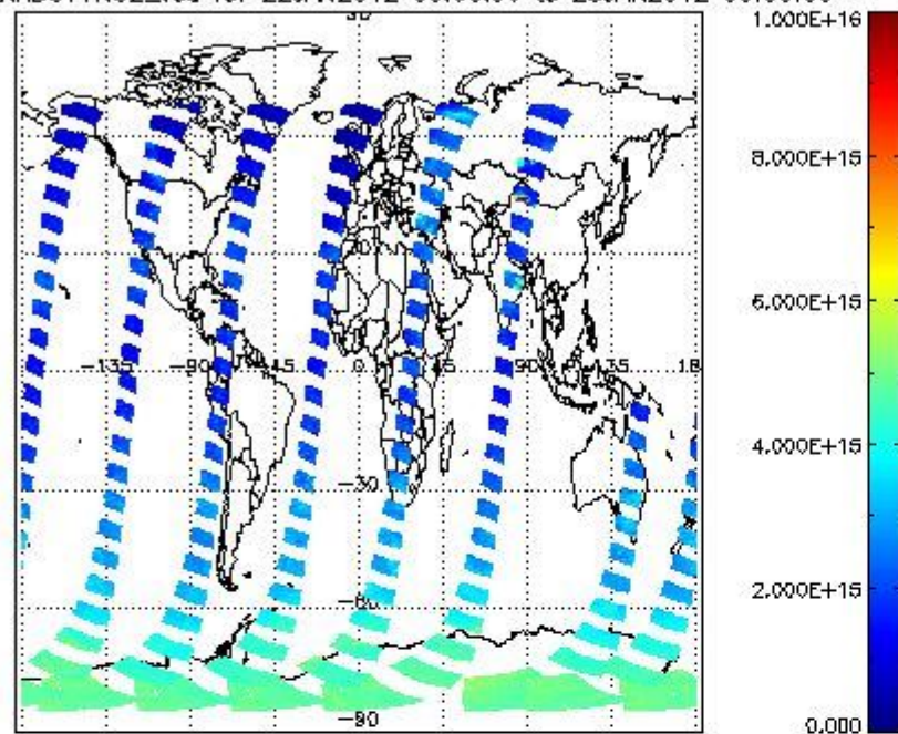
SCIOL2P_NADUV1NO2_vcd for 22JAN2012 00:00:00 to 23JAN2012 00:00:00
