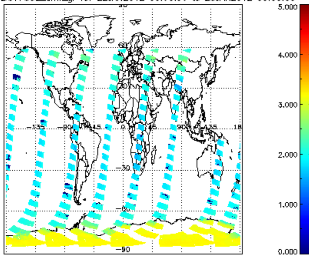
SCIOL2P_NADUV7S02_amf_gr for 22JAN2012 00:00:00 to 23JAN2012 00:00:00
