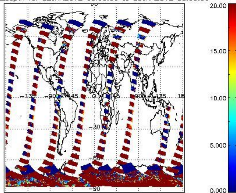
cLopt_depth for 22JAN2012 00:00:00 to 23JAN2012 00:00:00
