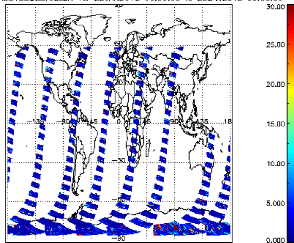
SCIOL2P_NADUV5S02_vcd_err for 22JAN2012 00:00:00 to 23JAN2012 00:00:00
