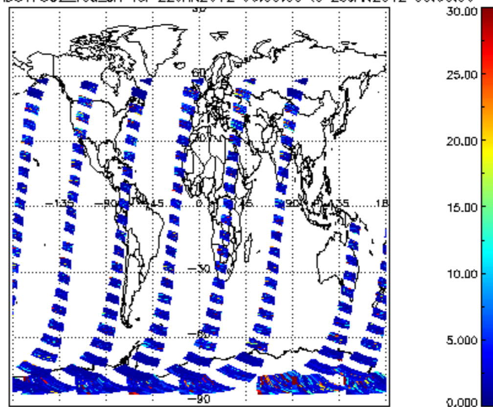
SCIOL2P_NADUV7S02_vcd_err for 22JAN2012 00:00:00 to 23JAN2012 00:00:00
