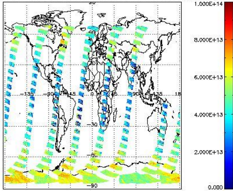
SCIOL2P_NADUV3BRO_vcd for 22JAN2012 00:00:00 to 23JAN2012 00:00:00
