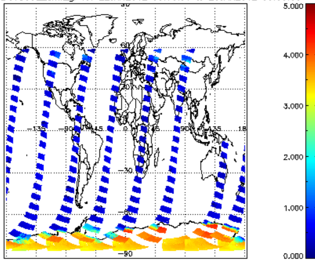
SCIOL2P_NADUV5S02_amf_gr for 22JAN2012 00:00:00 to 23JAN2012 00:00:00
