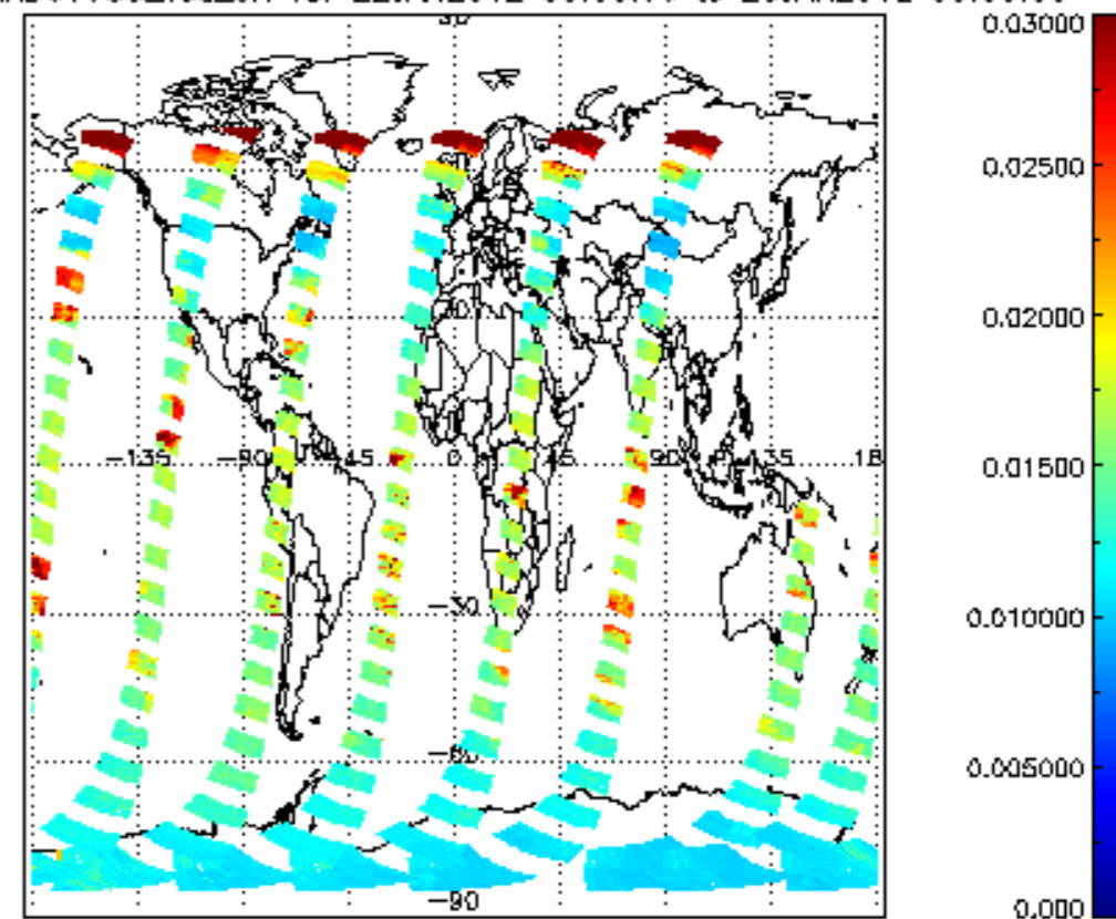
SCIOL2P_NADUV003_vcd_err for 22JAN2012 00:00:00 to 23JAN2012 00:00:00
