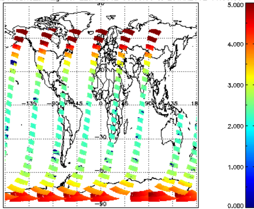
SCIOL2P_NADUV3BRO_amf_gr for 22JAN2012 00:00:00 to 23JAN2012 00:00:00
