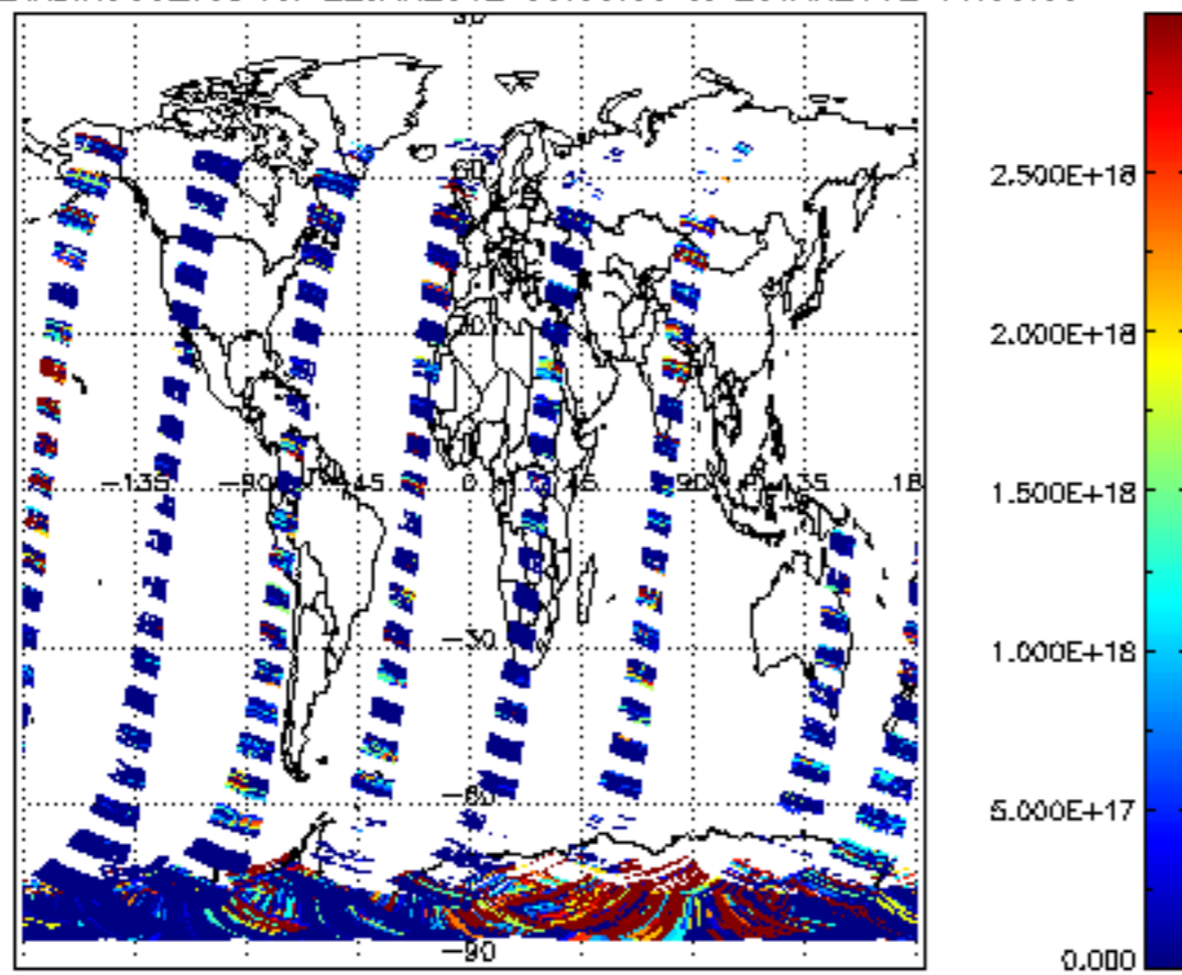
SCIOL2P_NADIR3CO_vcd for 22JAN2012 00:00:00 to 23JAN2012 00:00:00
