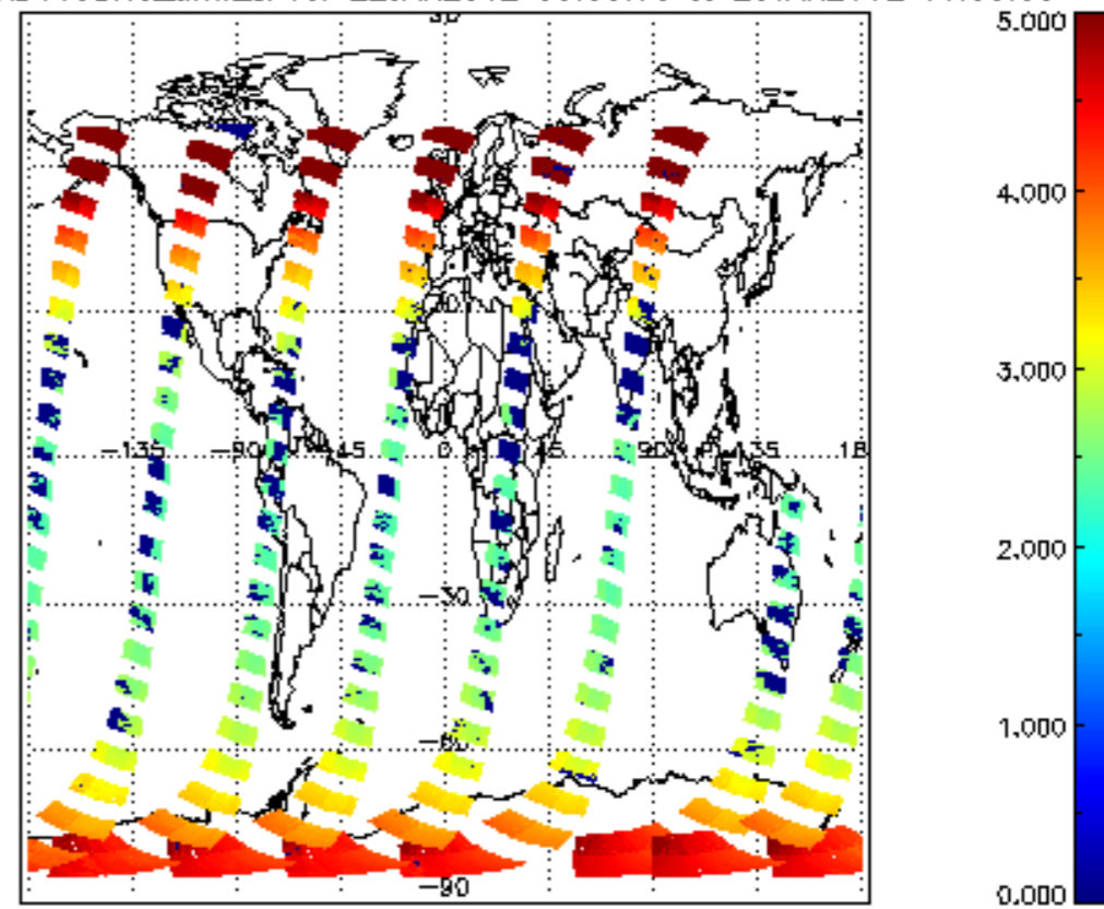
SCIOL2P_NADUV3BRO_amf_cl for 22JAN2012 00:00:00 to 23JAN2012 00:00:00
