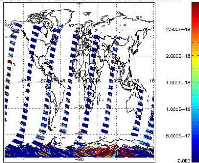
SCIDL2P_NADIR3CO_vcd for 22JAN2012 00:00:00 to 23JAN2012 00:00:00
