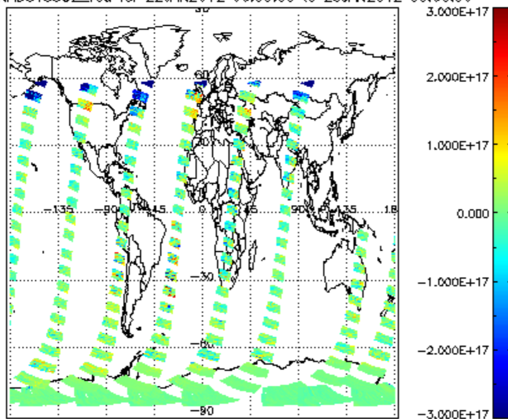
SCIOL2P_NADUV5S02_vcd for 22JAN2012 00:00:00 to 23JAN2012 00:00:00
