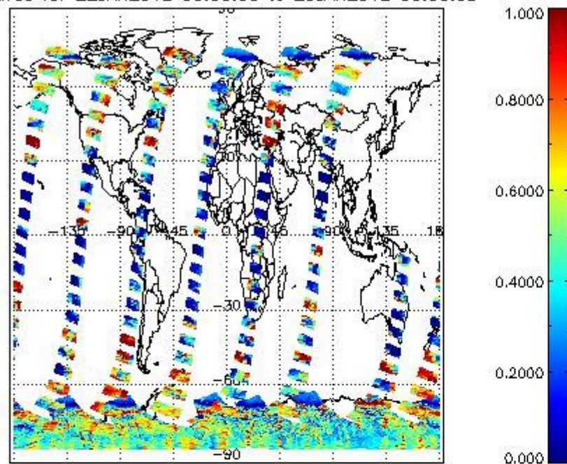
cL_frac for 22JAN2012 00:00:00 to 23JAN2012 00:00:00
