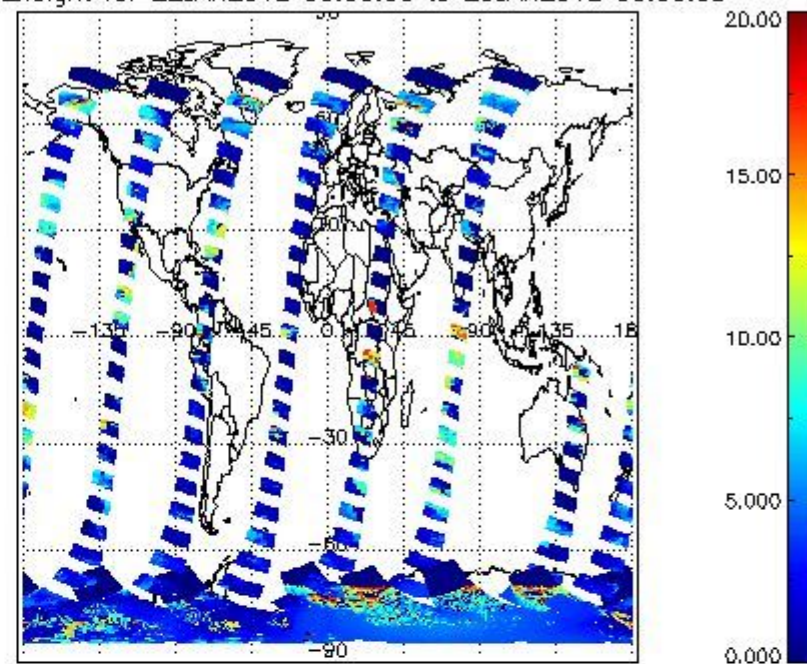
cL_top_height for 22JAN2012 00:00:00 to 23JAN2012 00:00:00
