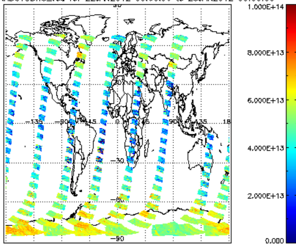
SCIOL2P_NADUV3BRO_vcd for 22JAN2012 00:00:00 to 23JAN2012 00:00:00
