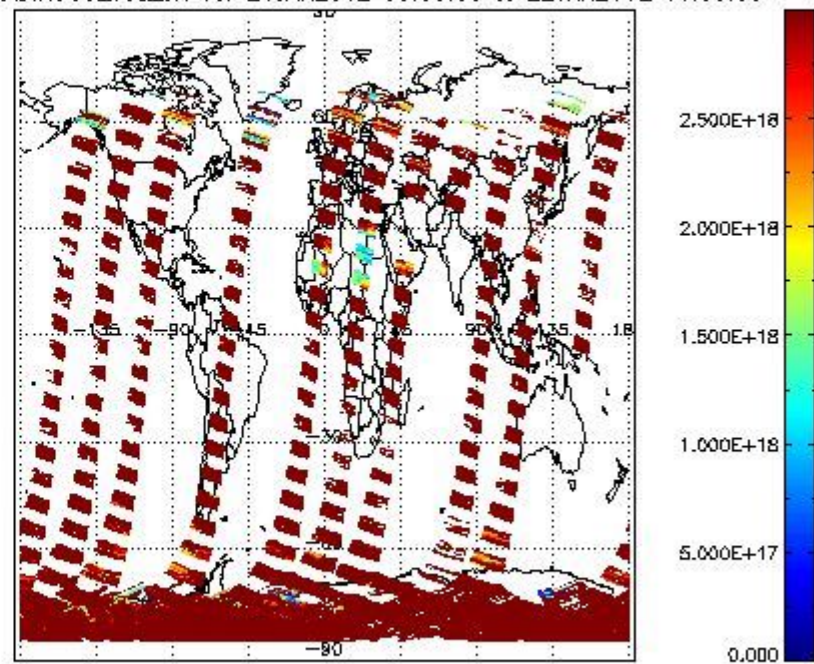
SCIDL2P_NADIR3CO_vcd_err for 21JAN2012 00:00:00 to 22JAN2012 00:00:00
