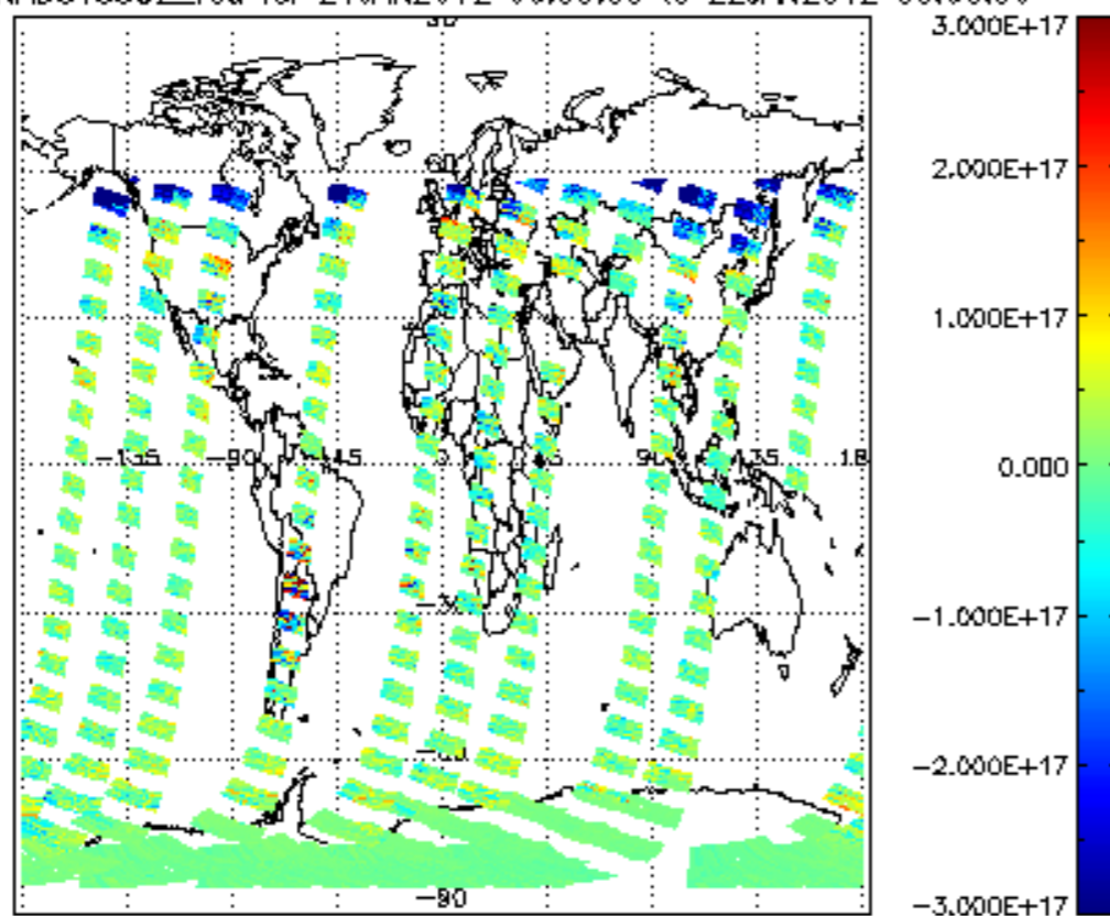
SCIOL2P_NADUV5S02_vcd for 21JAN2012 00:00:00 to 22JAN2012 00:00:00
