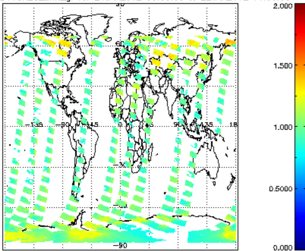
SCIOL2P_NADUVB20_amf_gr for 21JAN2012 00:00:00 to 22JAN2012 00:00:00
