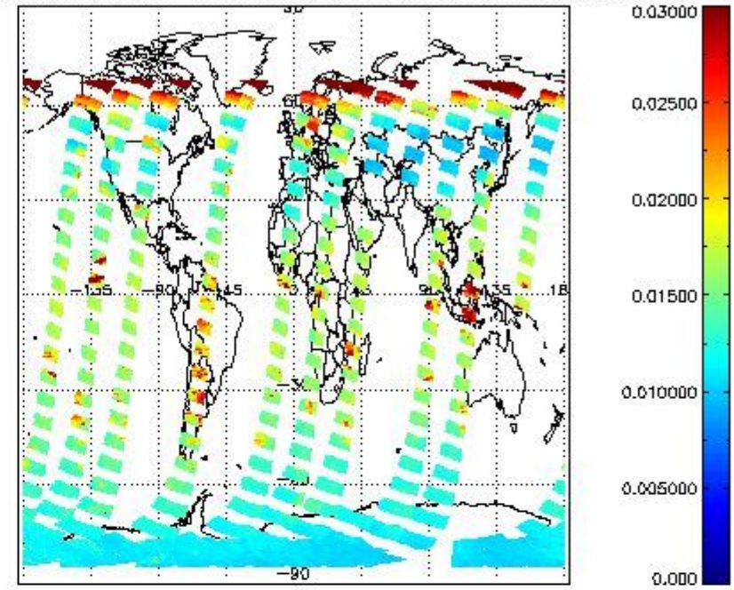
SCIOL2P_NADUV003_vcd_err for 21JAN2012 00:00:00 to 22JAN2012 00:00:00
