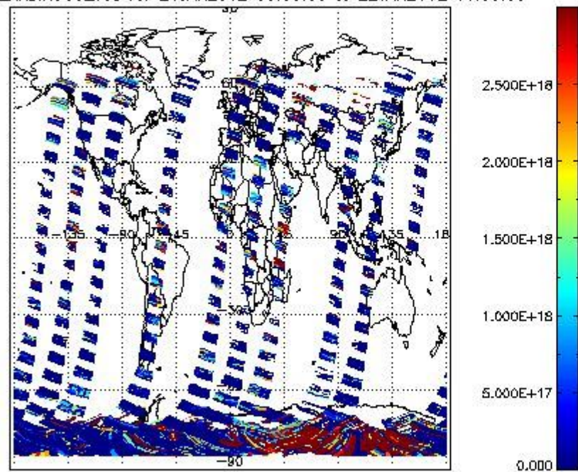
SCIDL2P_NADIR3CO_vcd for 21JAN2012 00:00:00 to 22JAN2012 00:00:00
