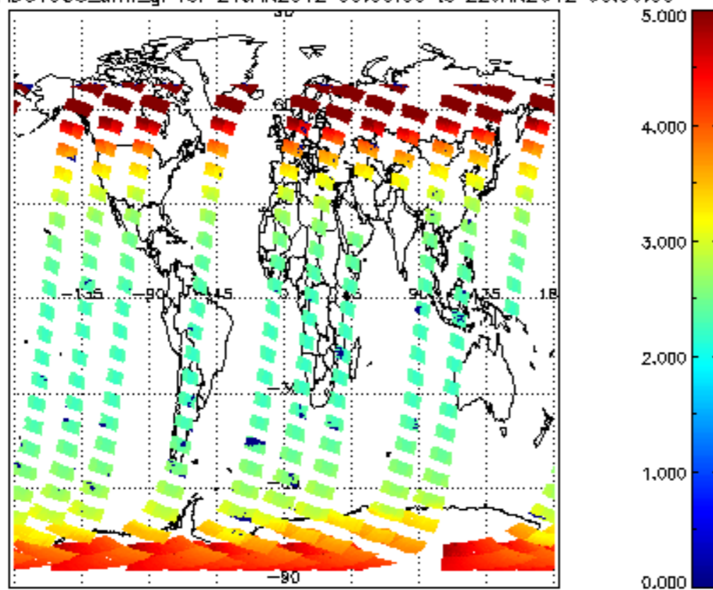
SCIOL2P_NADUV003_amf_gr for 21JAN2012 00:00:00 to 22JAN2012 00:00:00
