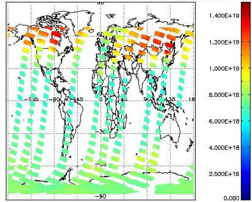
SCIOL2P_NADUV003_vcd for 21JAN2012 00:00:00 to 22JAN2012 00:00:00
