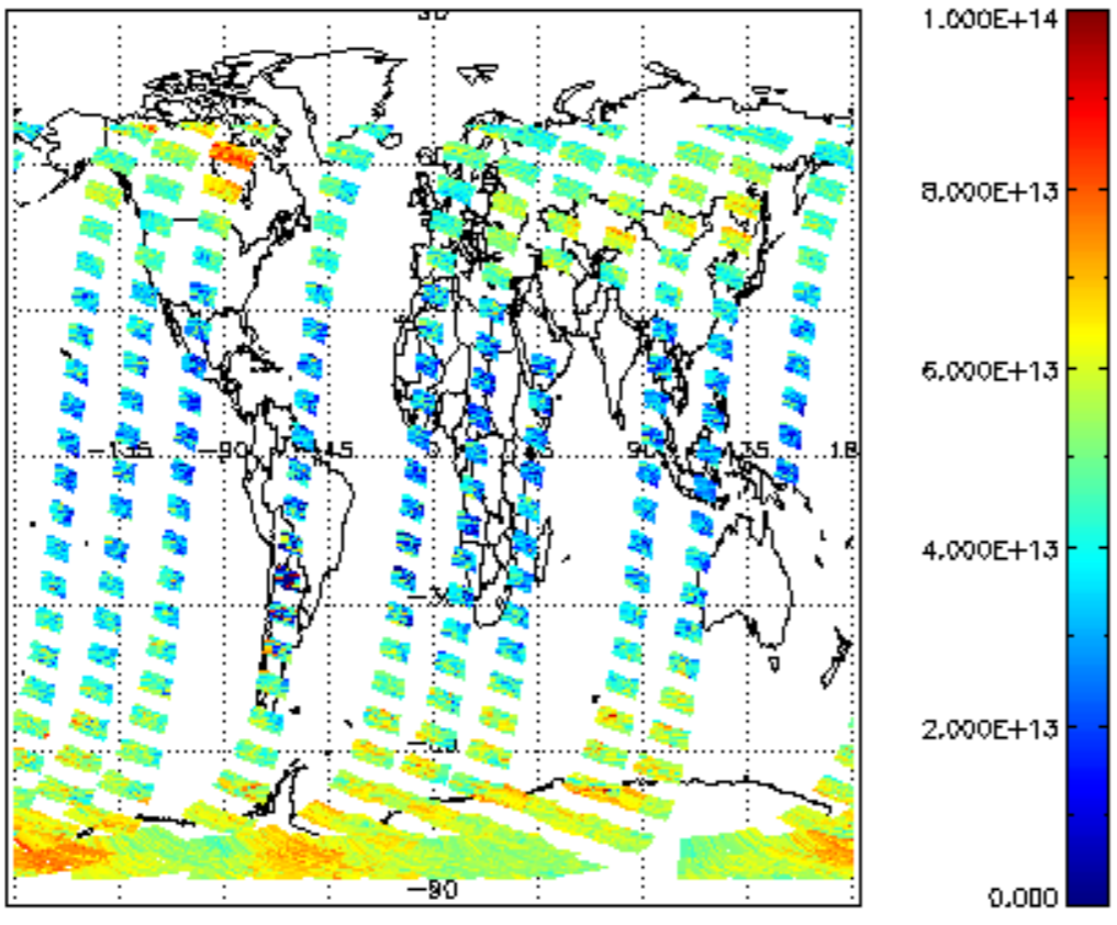
SCIOL2P_NADUV3BRO_vcd for 21JAN2012 00:00:00 to 22JAN2012 00:00:00
