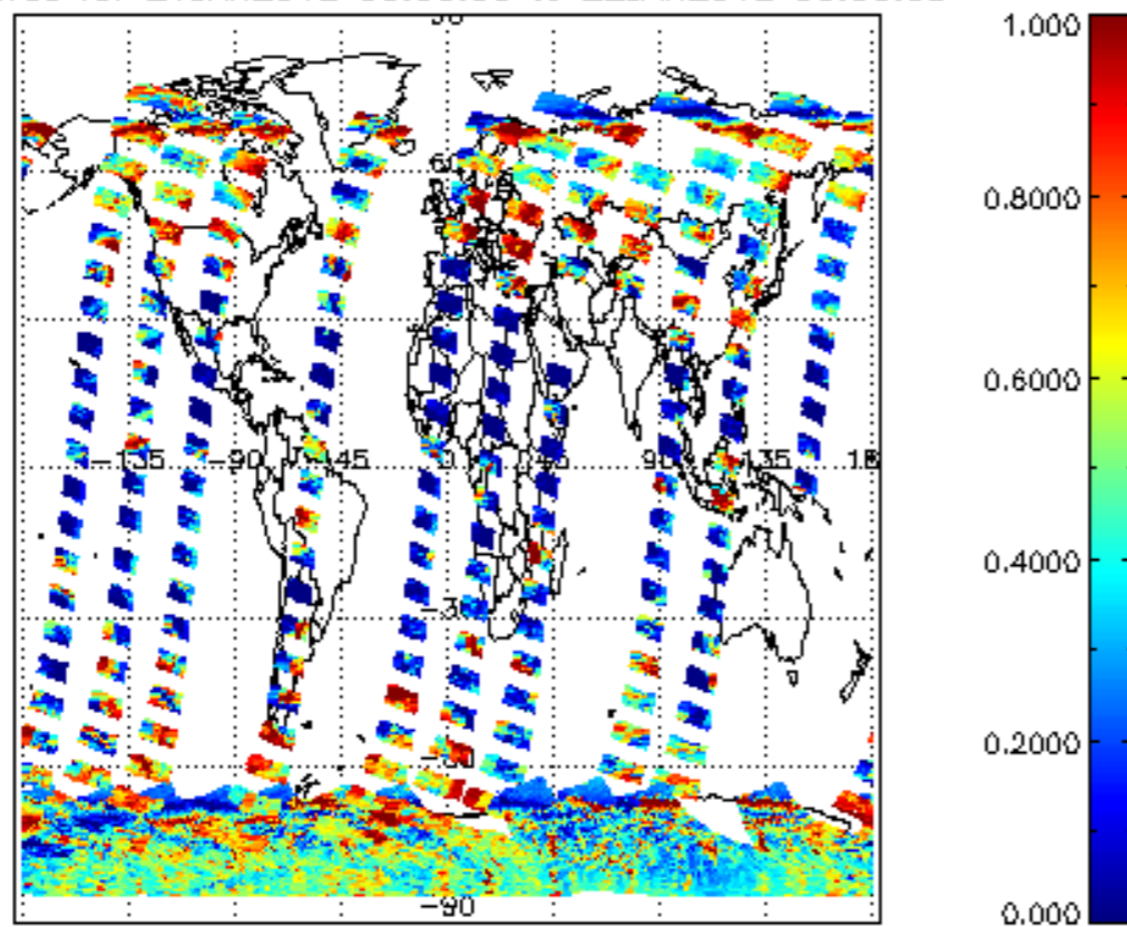
cL_frac for 21JAN2012 00:00:00 to 22JAN2012 00:00:00
