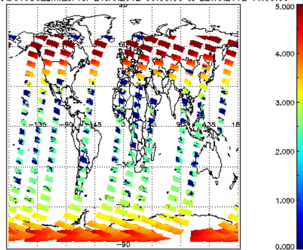
SCIOL2P_NADUV003_amf_cl for 21JAN2012 00:00:00 to 22JAN2012 00:00:00
