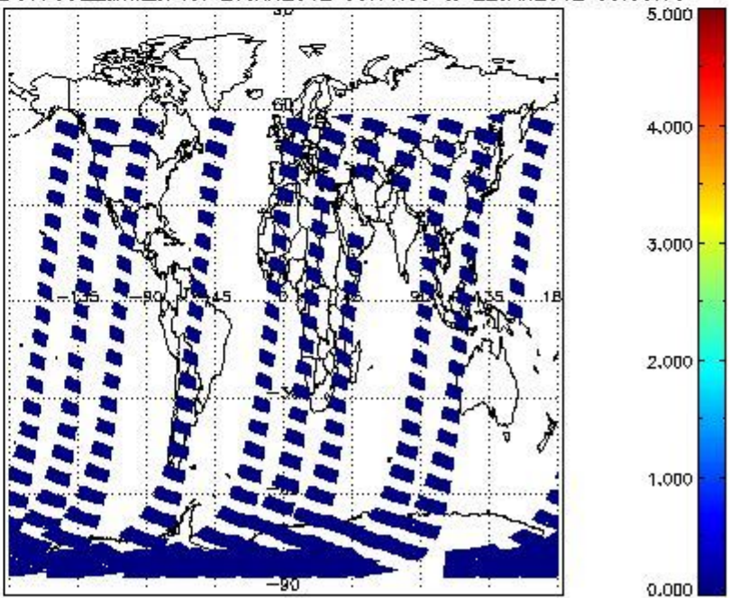
SCIOL2P_NADUV7S02_amf_cl for 21JAN2012 00:00:00 to 22JAN2012 00:00:00
