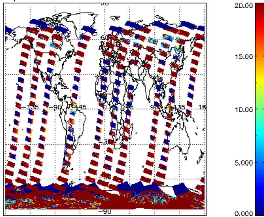
cLopt_depth for 21JAN2012 00:00:00 to 22JAN2012 00:00:00
