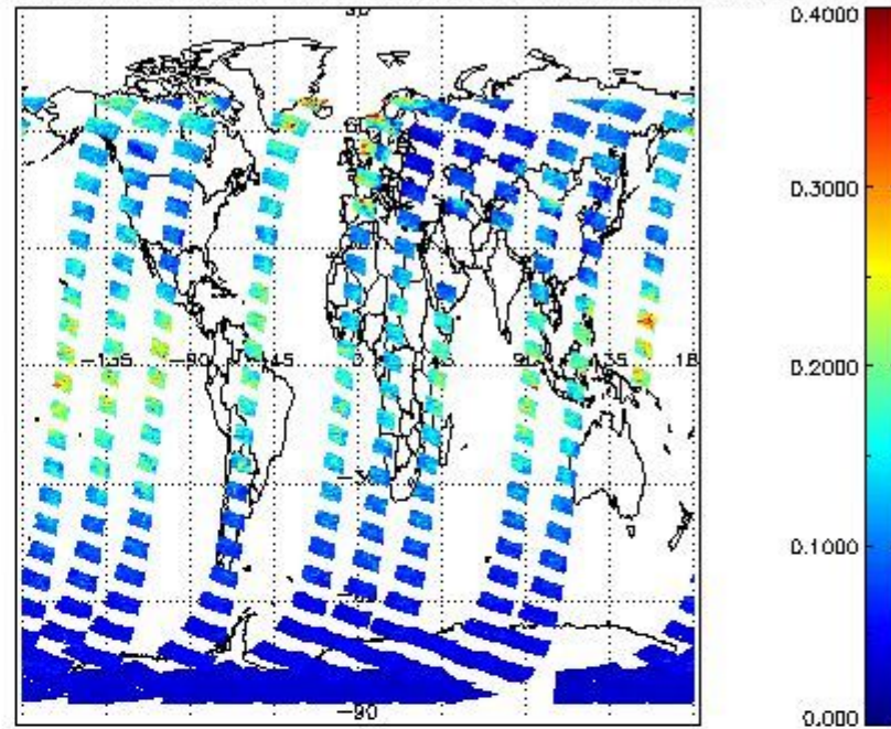
SCIOL2P_NADUV1NO2_vcd_err for 21JAN2012 00:00:00 to 22JAN2012 00:00:00
