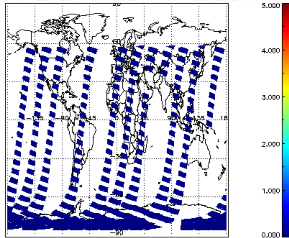
SCIOL2P_NADUV5S02_amf_cl for 21JAN2012 00:00:00 to 22JAN2012 00:00:00
