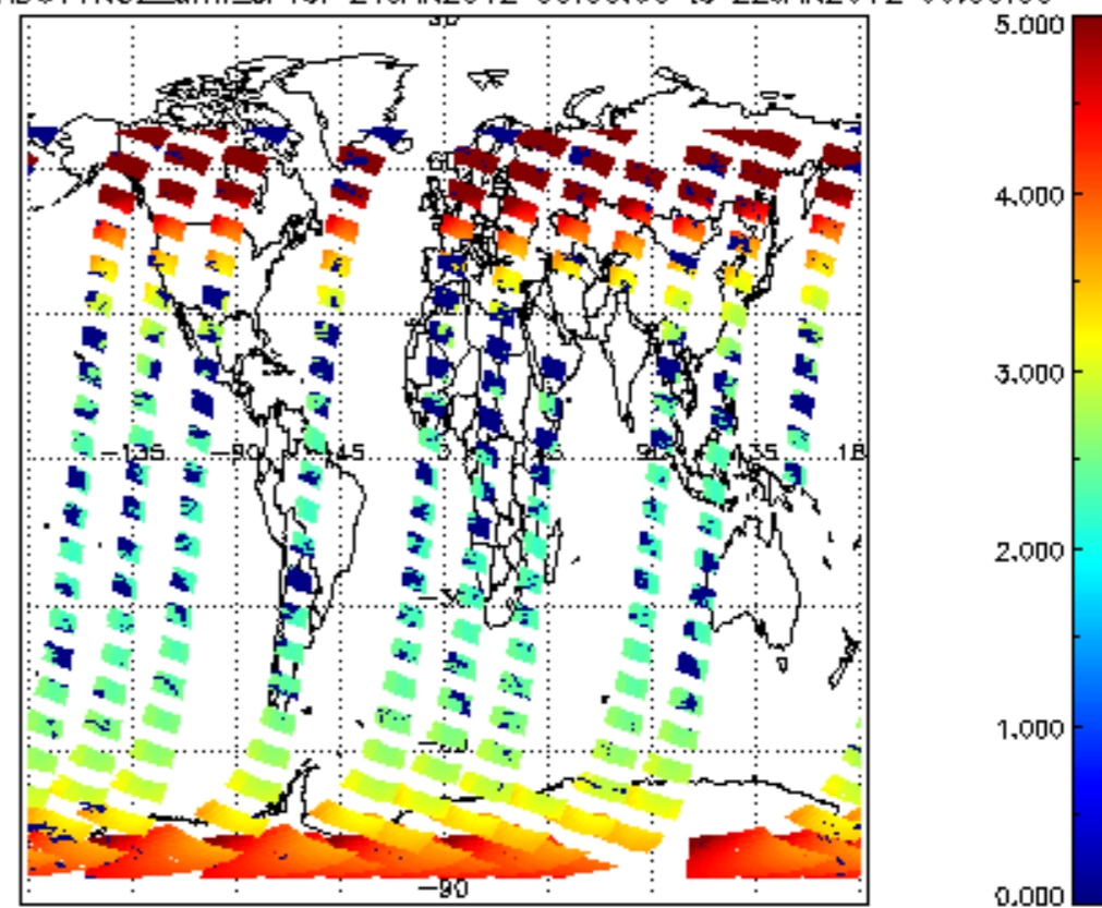
SCIOL2P_NADUV1NO2_amf_cl for 21JAN2012 00:00:00 to 22JAN2012 00:00:00
