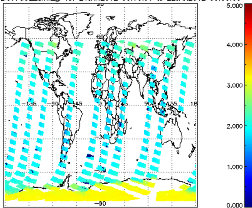
SCIOL2P_NADUV7S02_amf_gr for 21JAN2012 00:00:00 to 22JAN2012 00:00:00
