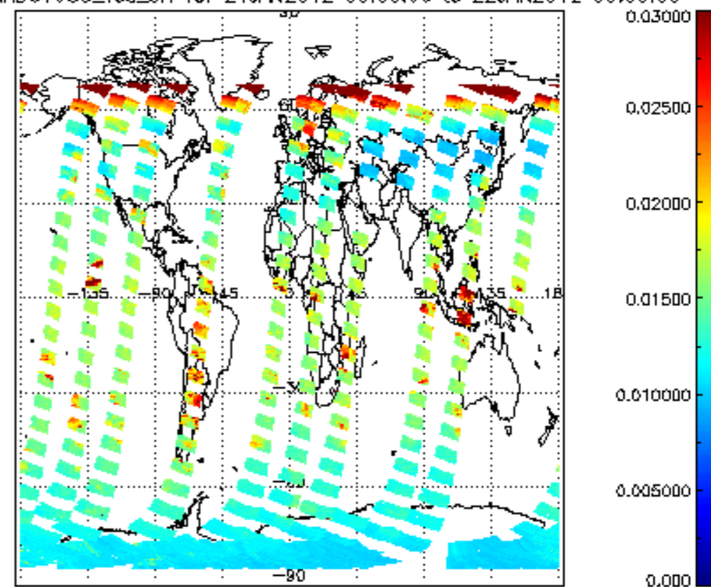
SCIOL2P_NADUV003_vcd_err for 21JAN2012 00:00:00 to 22JAN2012 00:00:00
