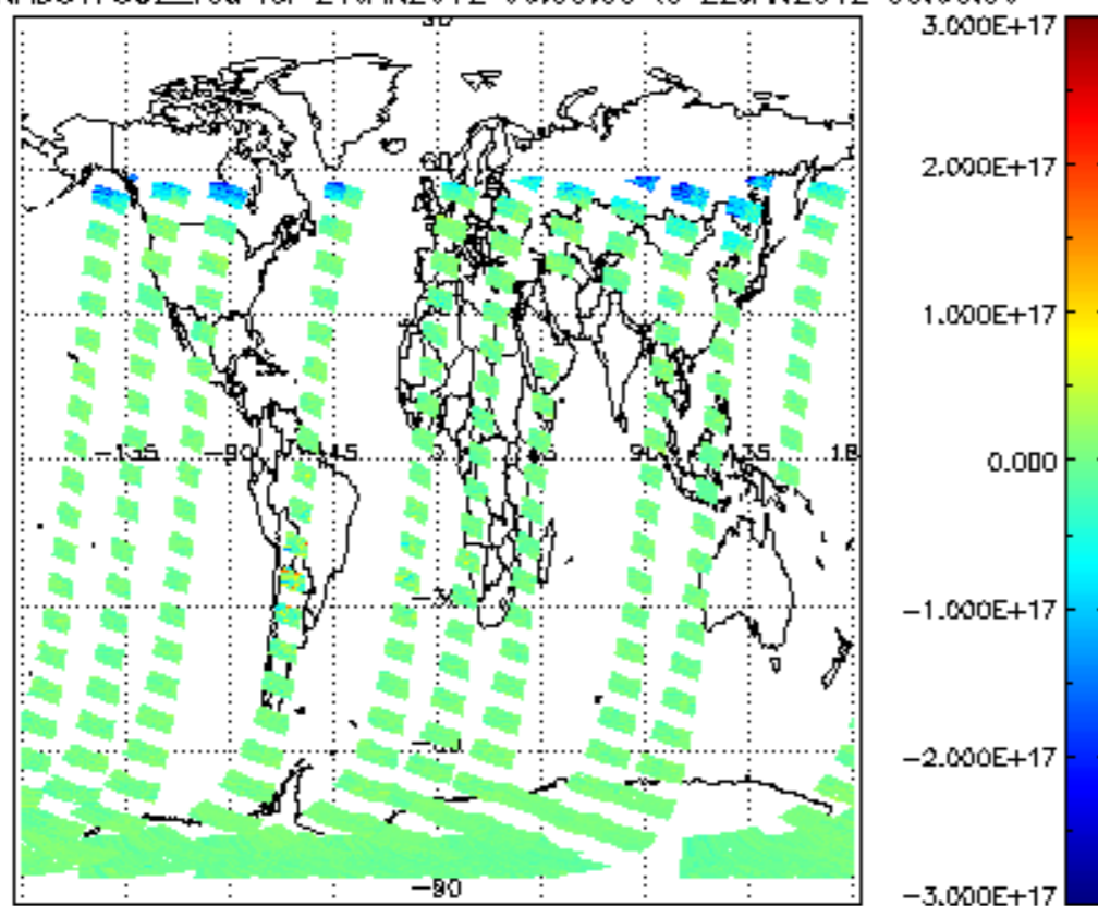
SCIOL2P_NADUV7S02_vcd for 21JAN2012 00:00:00 to 22JAN2012 00:00:00
