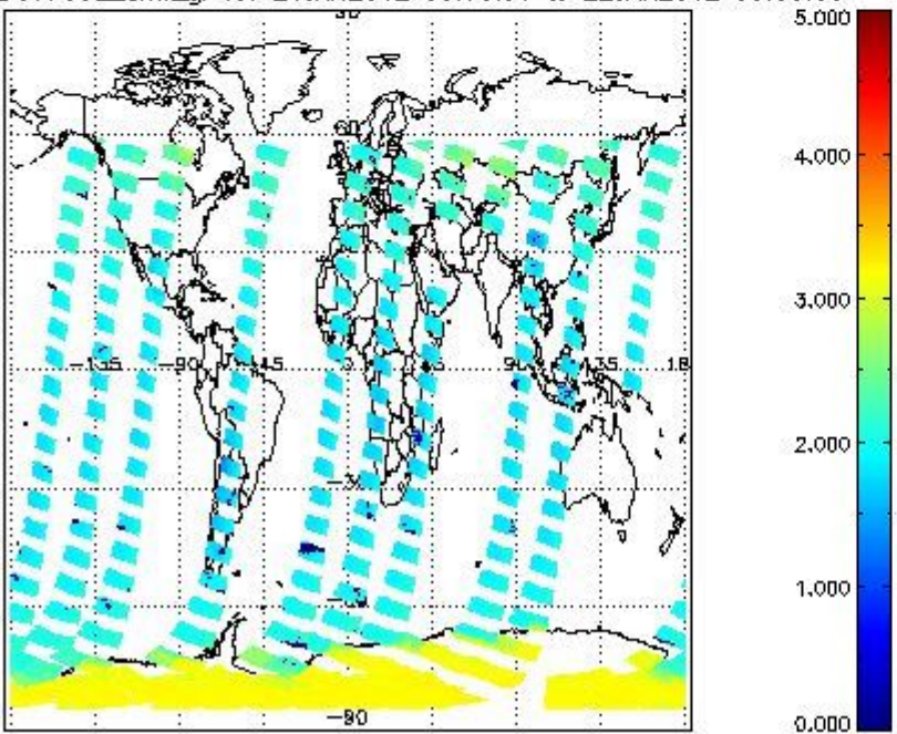
SCIOL2P_NADUV7S02_amf_gr for 21JAN2012 00:00:00 to 22JAN2012 00:00:00
