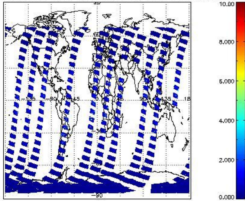
SCIOL2P_NADUV3BRO_vcd_err for 21JAN2012 00:00:00 to 22JAN2012 00:00:00
