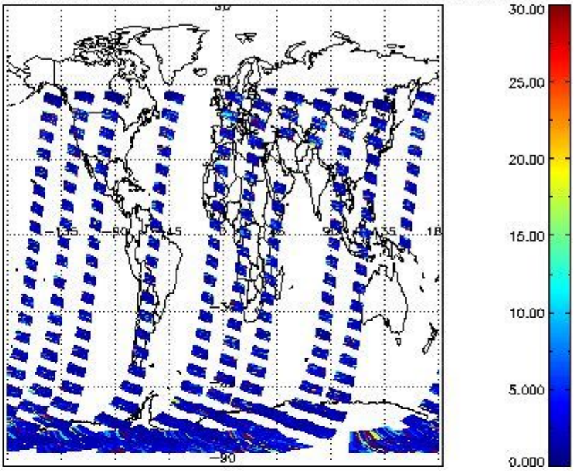
SCIOL2P_NADUV7S02_vcd_err for 21JAN2012 00:00:00 to 22JAN2012 00:00:00
