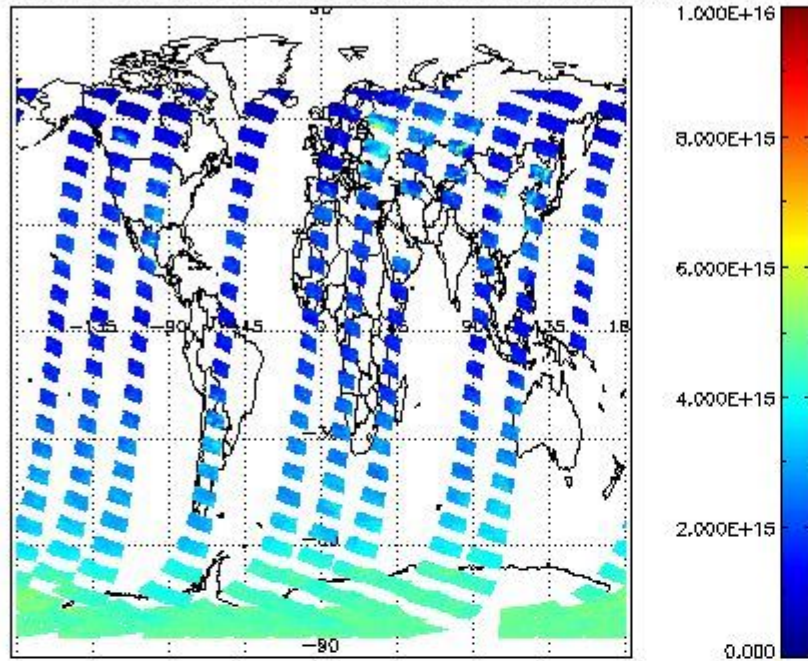
SCIOL2P_NADUV1NO2_vcd for 21JAN2012 00:00:00 to 22JAN2012 00:00:00
