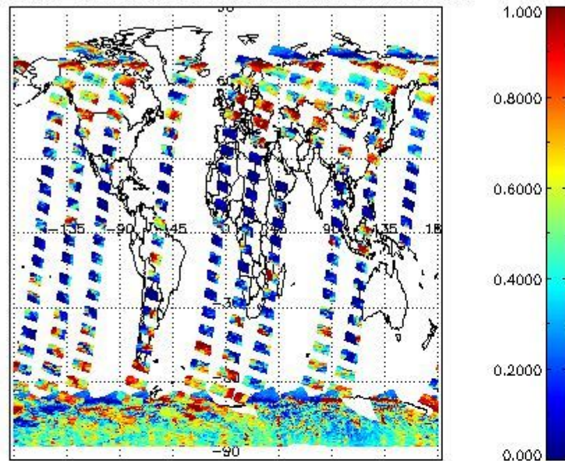
cL_frac for 21JAN2012 00:00:00 to 22JAN2012 00:00:00
