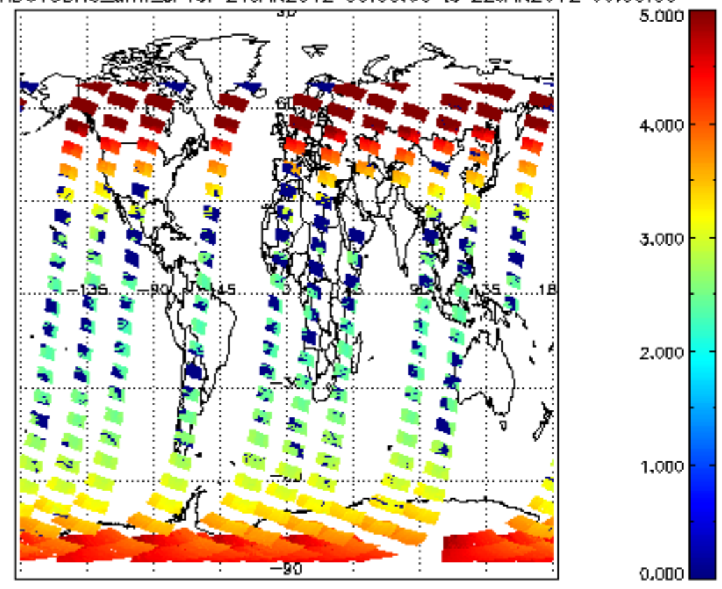
SCIOL2P_NADUV3BRO_amf_cl for 21JAN2012 00:00:00 to 22JAN2012 00:00:00
