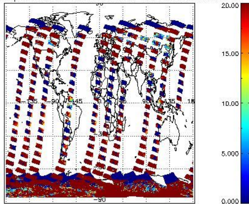
cLopt_depth for 21JAN2012 00:00:00 to 22JAN2012 00:00:00
