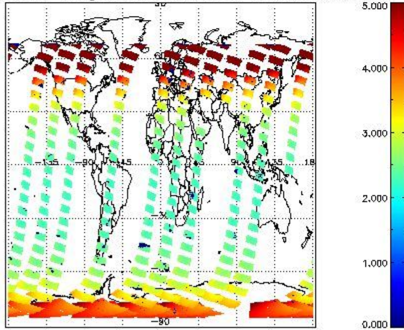
SCIOL2P_NADUV1NO2_amf_gr for 21JAN2012 00:00:00 to 22JAN2012 00:00:00
