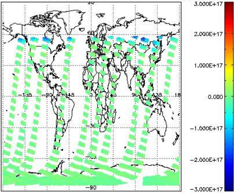
SCIOL2P_NADUV7S02_vcd for 21JAN2012 00:00:00 to 22JAN2012 00:00:00
