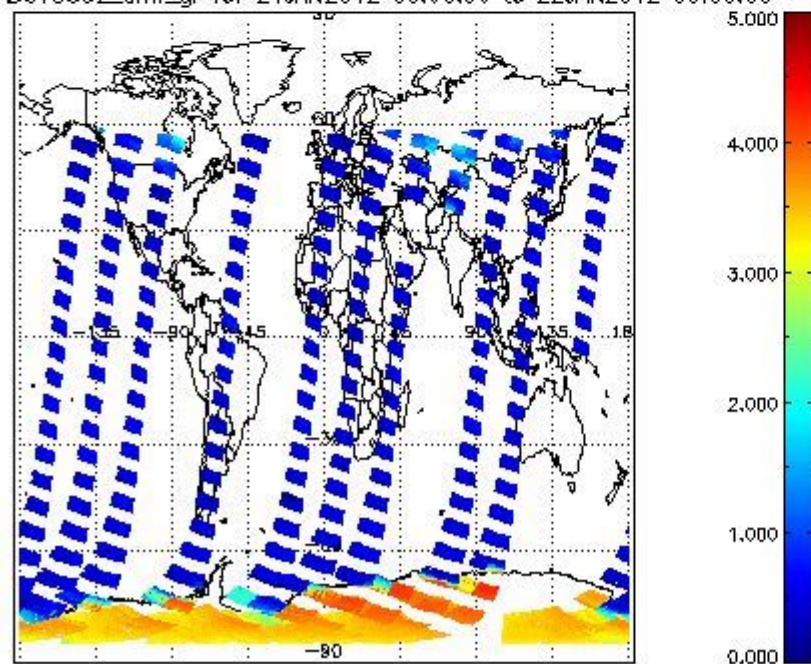
SCIOL2P_NADUV5S02_amf_gr for 21JAN2012 00:00:00 to 22JAN2012 00:00:00
