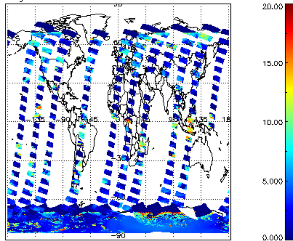
cL_top_height for 21JAN2012 00:00:00 to 22JAN2012 00:00:00
