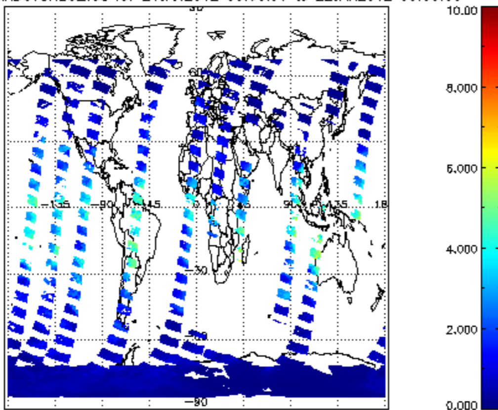
SCIOL2P_NADUVB20_vcd for 21JAN2012 00:00:00 to 22JAN2012 00:00:00
