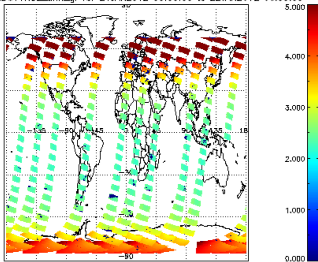
SCIOL2P_NADUV1NO2_amf_gr for 21JAN2012 00:00:00 to 22JAN2012 00:00:00
