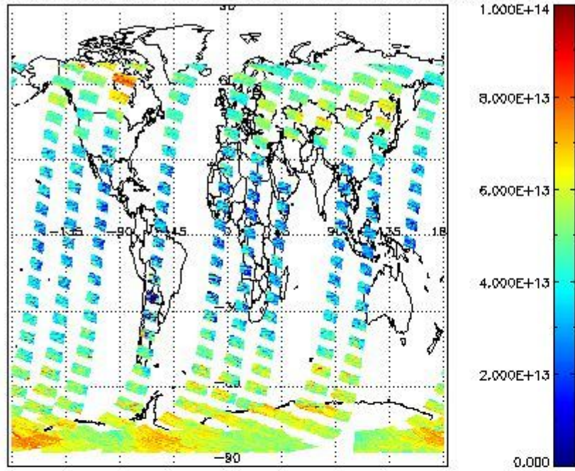
SCIOL2P_NADUV3BRO_vcd for 21JAN2012 00:00:00 to 22JAN2012 00:00:00
