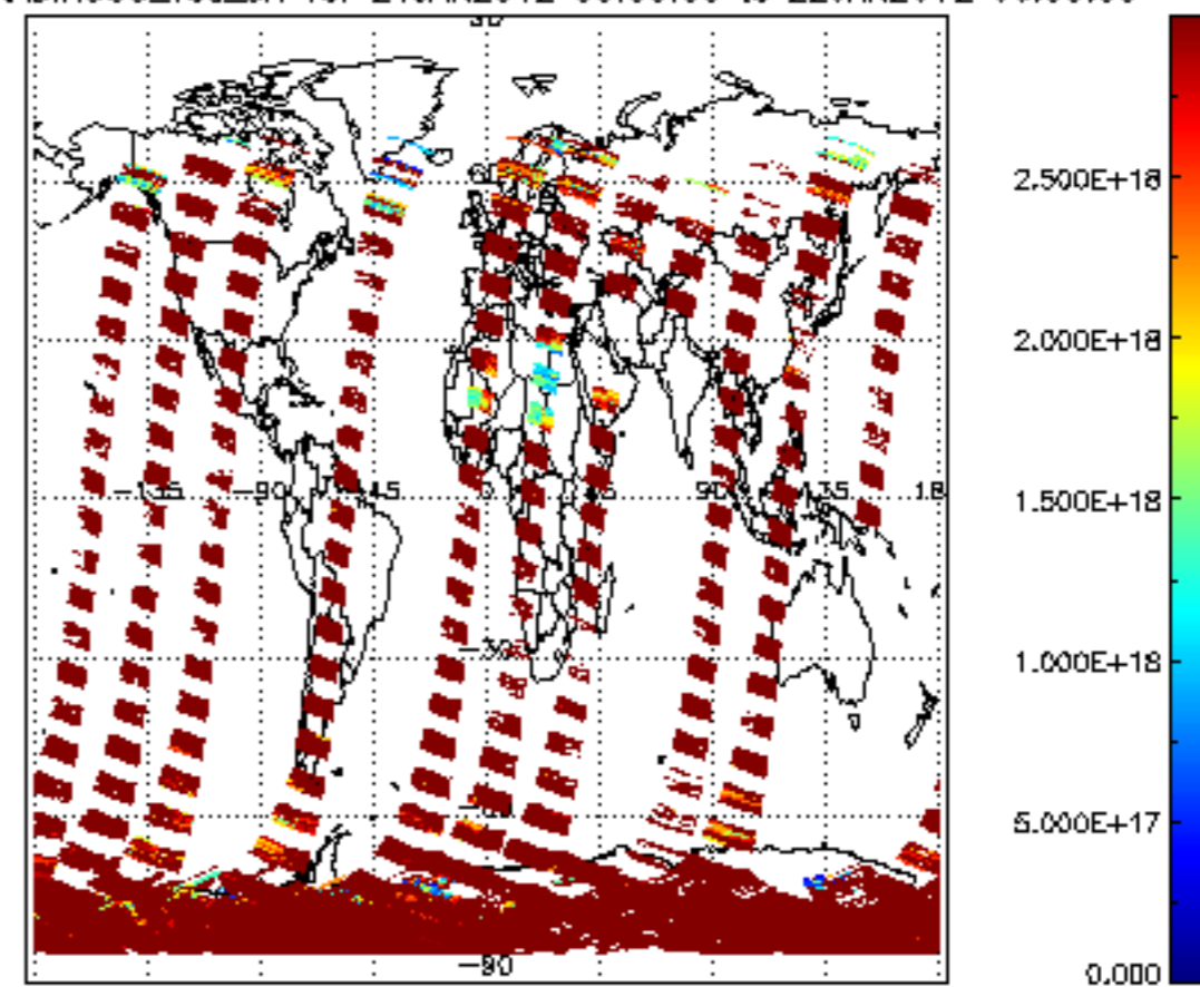
SCIOL2P_NADIR3CO_vcd_err for 21JAN2012 00:00:00 to 22JAN2012 00:00:00
