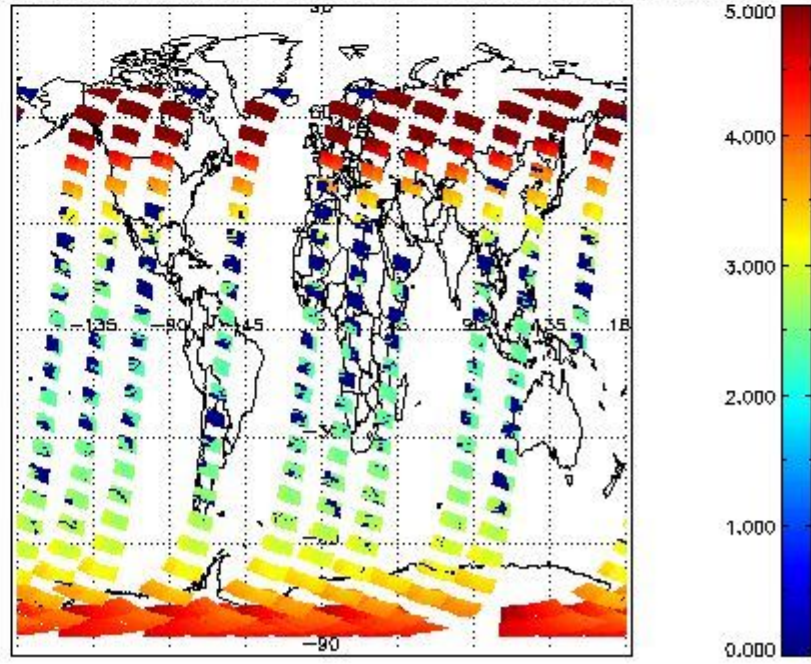
SCIOL2P_NADUV3BRO_amf_cl for 21JAN2012 00:00:00 to 22JAN2012 00:00:00
