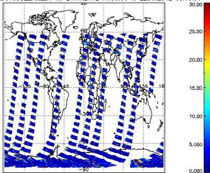
SCIOL2P_NADUV5S02_vcd_err for 21JAN2012 00:00:00 to 22JAN2012 00:00:00
