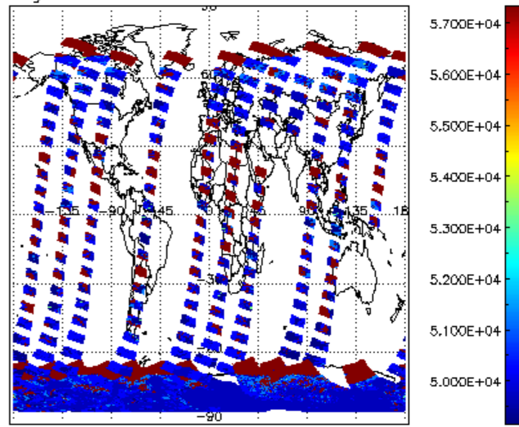
cloud_flags for 21JAN2012 00:00:00 to 22JAN2012 00:00:00
