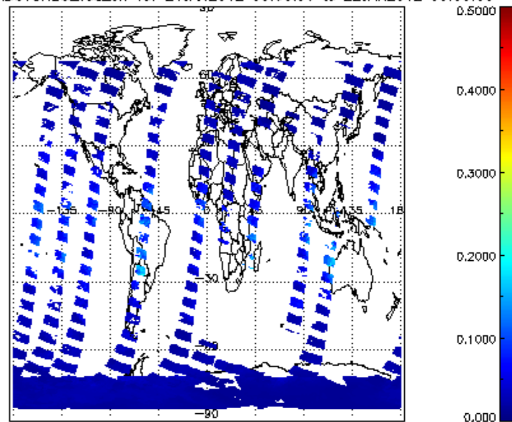
SCIOL2P_NADUVB20_vcd_err for 21JAN2012 00:00:00 to 22JAN2012 00:00:00
