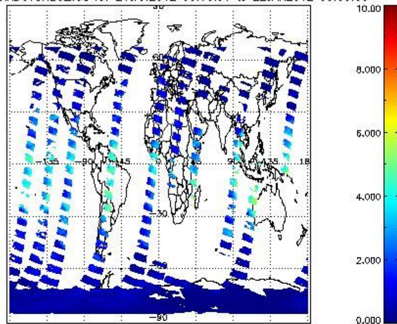
SCIOL2P_NADUV8H20_vcd for 21JAN2012 00:00:00 to 22JAN2012 00:00:00
