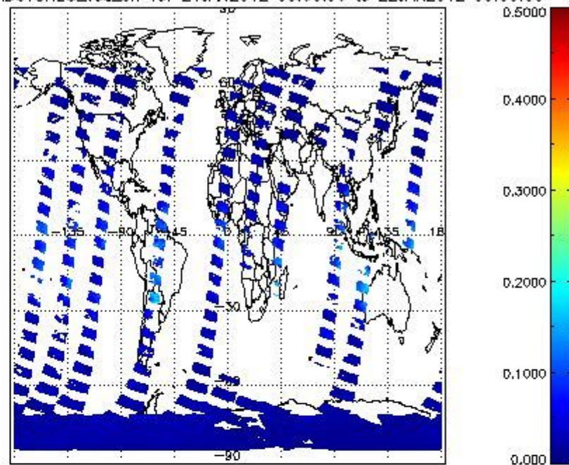
SCIOL2P_NADUV8H20_vcd_err for 21JAN2012 00:00:00 to 22JAN2012 00:00:00
