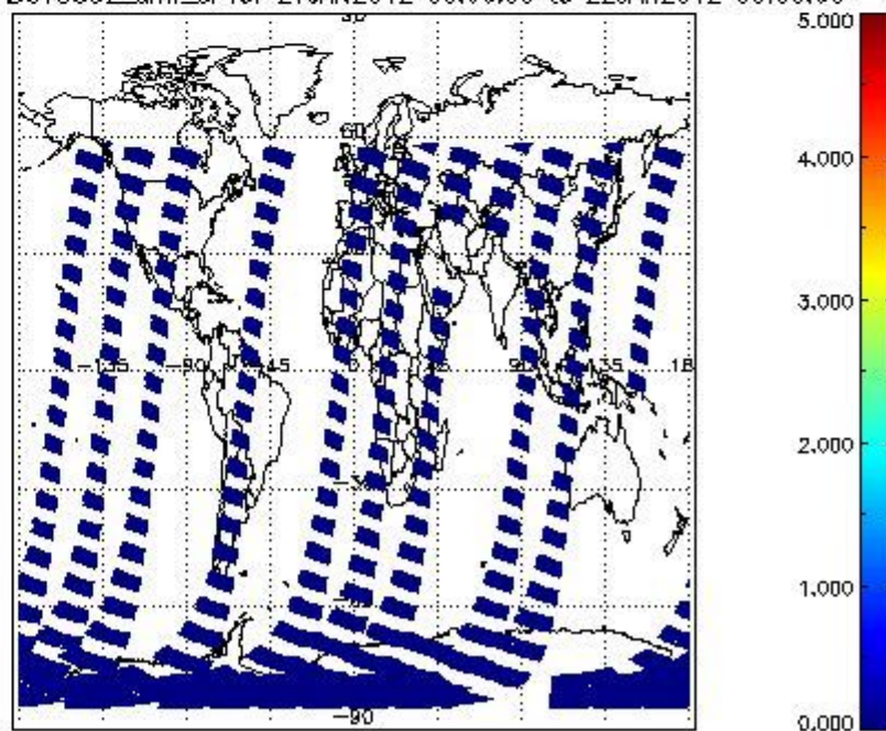
SCIOL2P_NADUV5S02_amf_cl for 21JAN2012 00:00:00 to 22JAN2012 00:00:00
