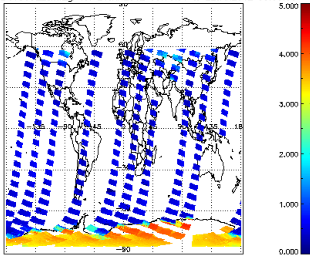
SCIOL2P_NADUV5S02_amf_gr for 21JAN2012 00:00:00 to 22JAN2012 00:00:00
