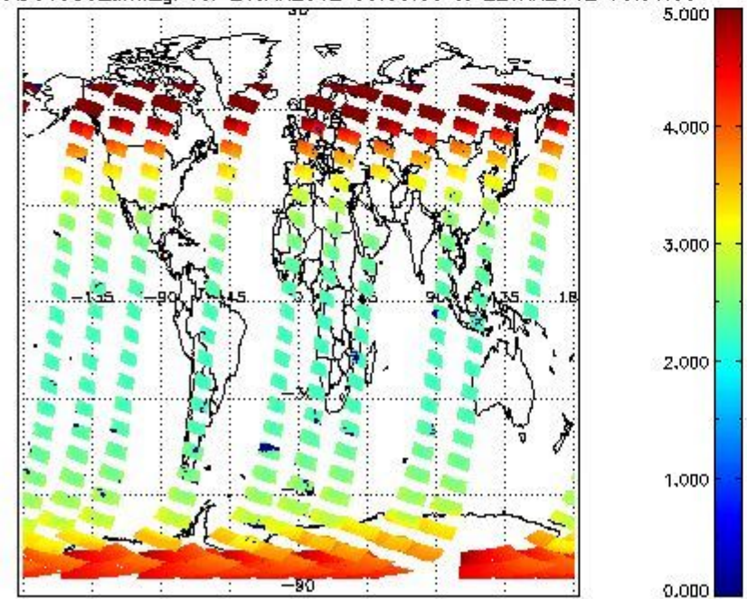
SCIOL2P_NADUV003_amf_gr for 21JAN2012 00:00:00 to 22JAN2012 00:00:00
