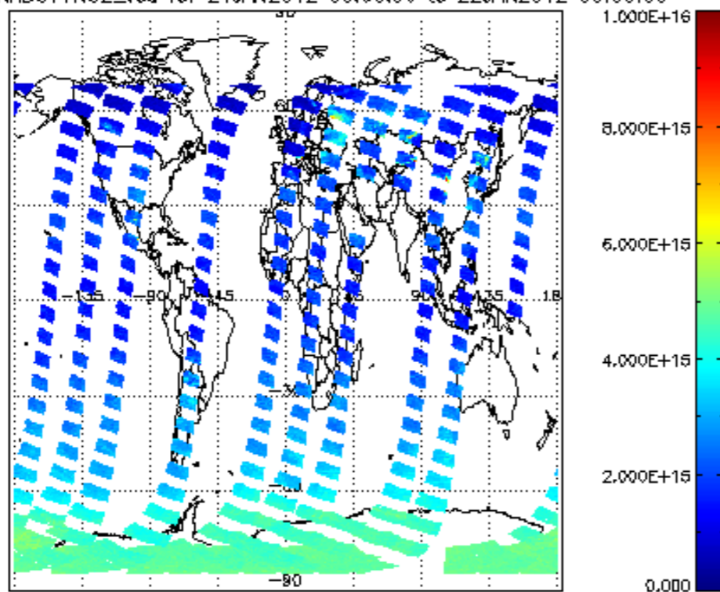
SCIOL2P_NADUV1NO2_vcd for 21JAN2012 00:00:00 to 22JAN2012 00:00:00
