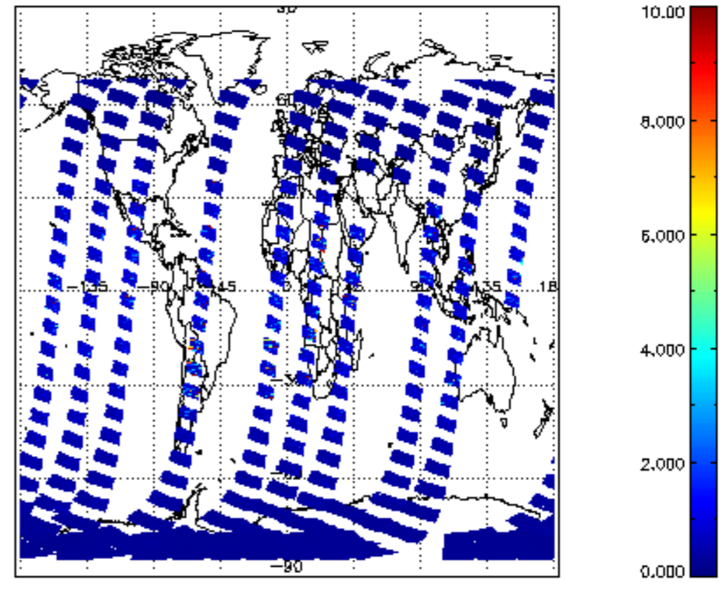
SCIOL2P_NADUV3BRO_vcd_err for 21JAN2012 00:00:00 to 22JAN2012 00:00:00
