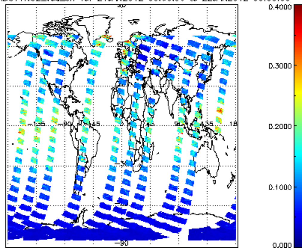
SCIOL2P_NADUV1NO2_vcd_err for 21JAN2012 00:00:00 to 22JAN2012 00:00:00
