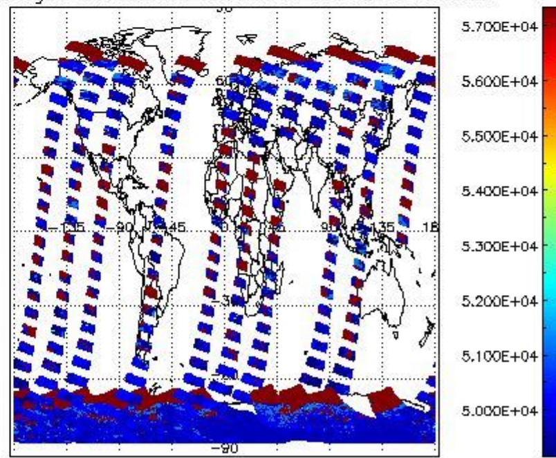
cloud_flags for 21JAN2012 00:00:00 to 22JAN2012 00:00:00
