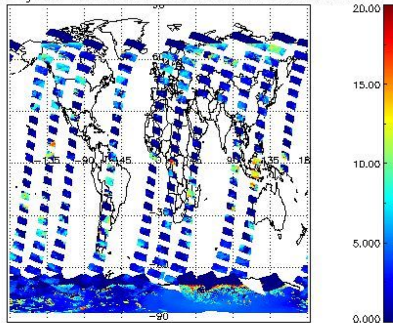
cL_top_height for 21JAN2012 00:00:00 to 22JAN2012 00:00:00
