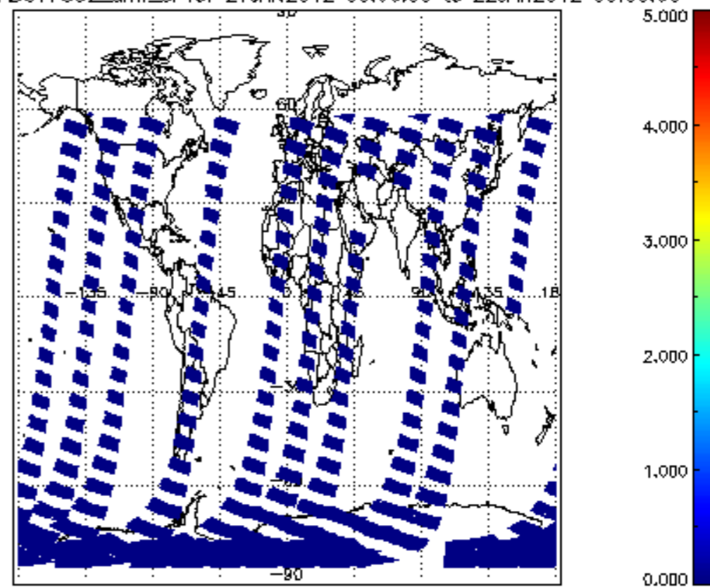
SCIOL2P_NADUV7S02_amf_cl for 21JAN2012 00:00:00 to 22JAN2012 00:00:00
