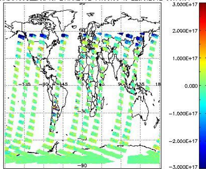
SCIOL2P_NADUV5S02_vcd for 21JAN2012 00:00:00 to 22JAN2012 00:00:00
