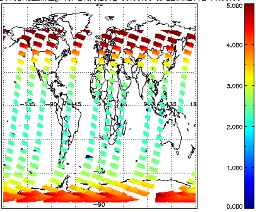
SCIOL2P_NADUV3BRO_amf_gr for 21JAN2012 00:00:00 to 22JAN2012 00:00:00
