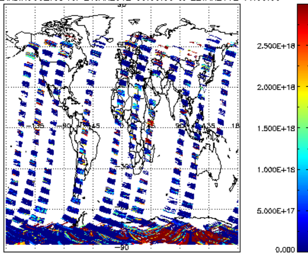
SCIOL2P_NADIR3CO_vcd for 21JAN2012 00:00:00 to 22JAN2012 00:00:00
