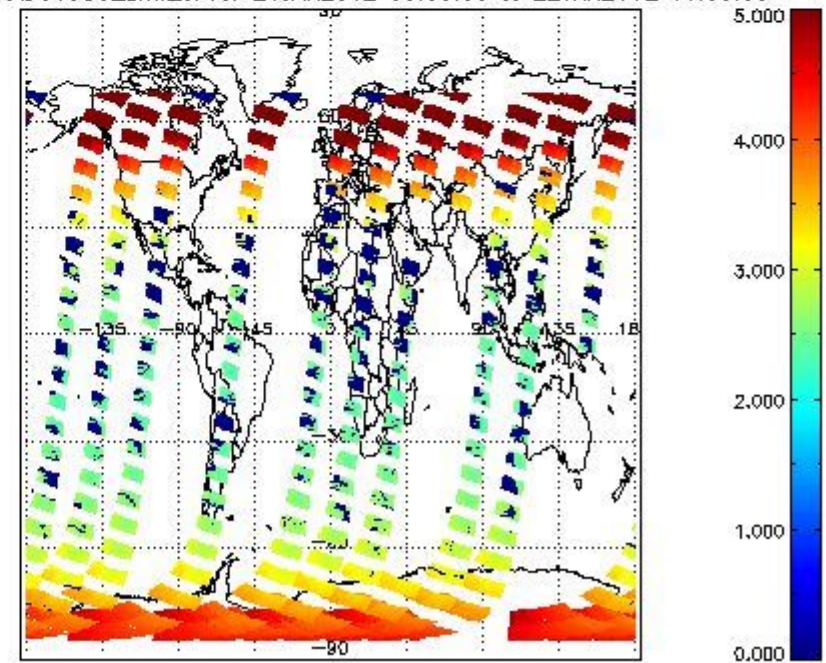
SCIOL2P_NADUV003_amf_cl for 21JAN2012 00:00:00 to 22JAN2012 00:00:00
