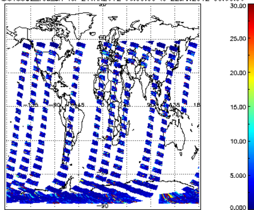
SCIOL2P_NADUV5S02_vcd_err for 21JAN2012 00:00:00 to 22JAN2012 00:00:00
