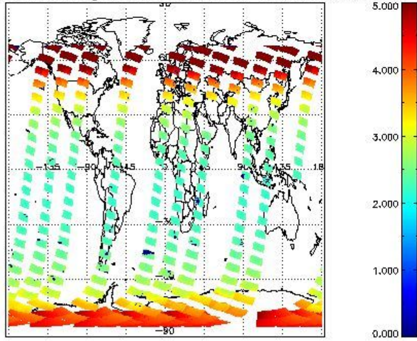
SCIOL2P_NADUV3BRO_amf_gr for 21JAN2012 00:00:00 to 22JAN2012 00:00:00
