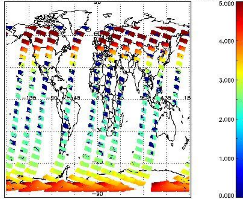
SCIOL2P_NADUV1NO2_amf_cl for 21JAN2012 00:00:00 to 22JAN2012 00:00:00
