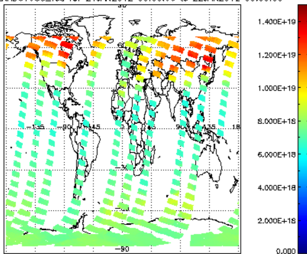
SCIOL2P_NADUV003_vcd for 21JAN2012 00:00:00 to 22JAN2012 00:00:00
