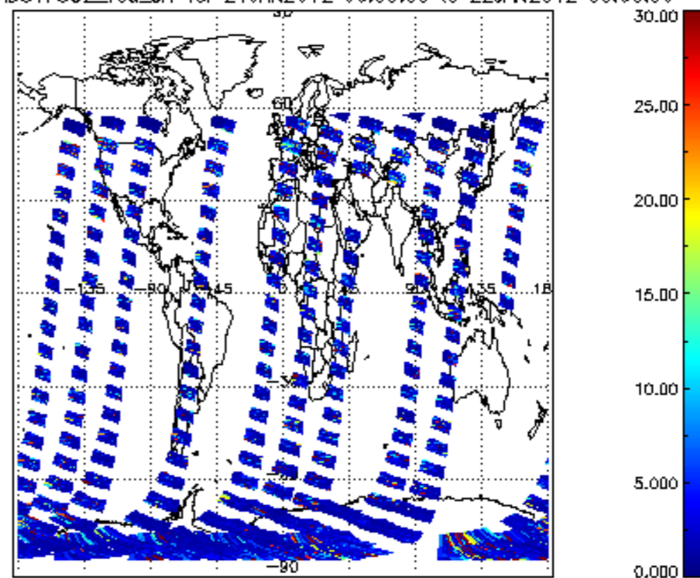
SCIOL2P_NADUV7S02_vcd_err for 21JAN2012 00:00:00 to 22JAN2012 00:00:00
