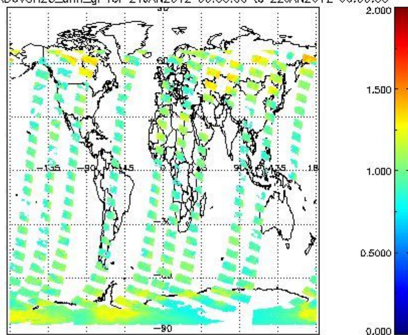
SCIOL2P_NADUV8H20_amf_gr for 21JAN2012 00:00:00 to 22JAN2012 00:00:00
