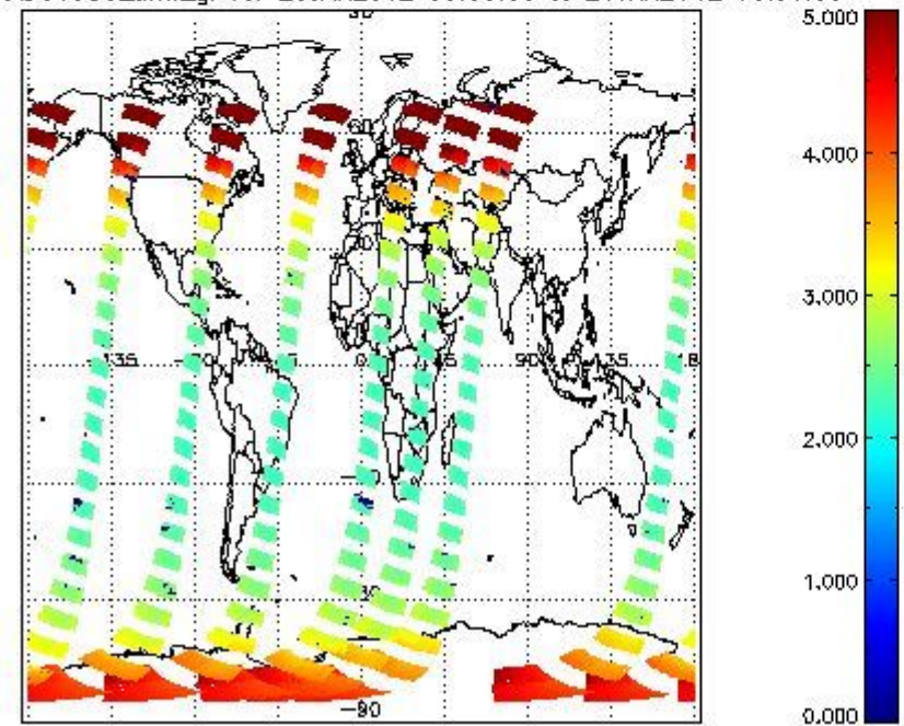
SCIOL2P_NADUV003_amf_gr for 20JAN2012 00:00:00 to 21JAN2012 00:00:00
