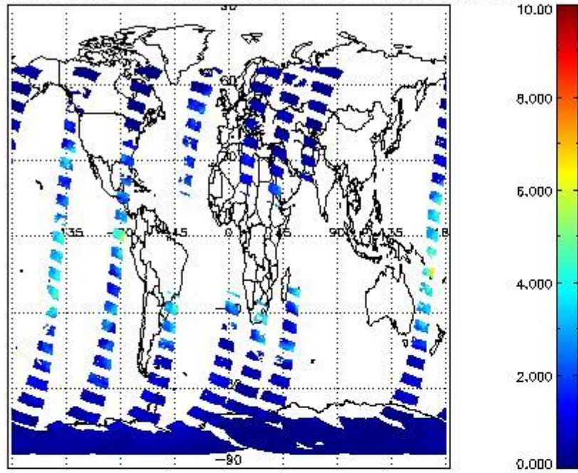
SCIOL2P_NADUV8H20_vcd for 20JAN2012 00:00:00 to 21JAN2012 00:00:00
