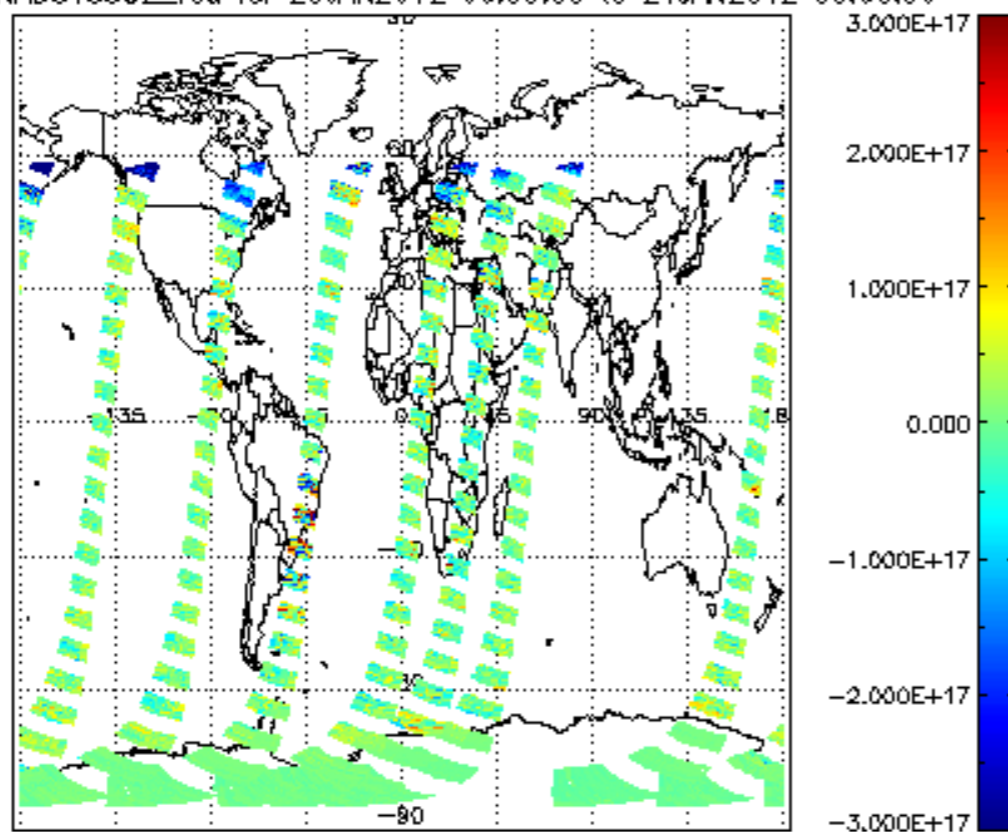
SCIOL2P_NADUV5S02_vcd for 20JAN2012 00:00:00 to 21JAN2012 00:00:00
