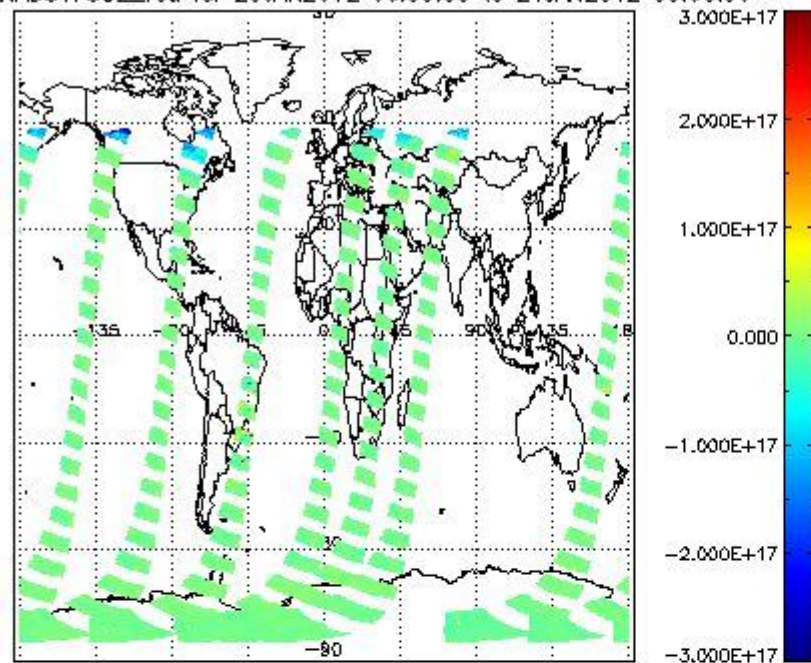
SCIOL2P_NADUV7S02_vcd for 20JAN2012 00:00:00 to 21JAN2012 00:00:00
