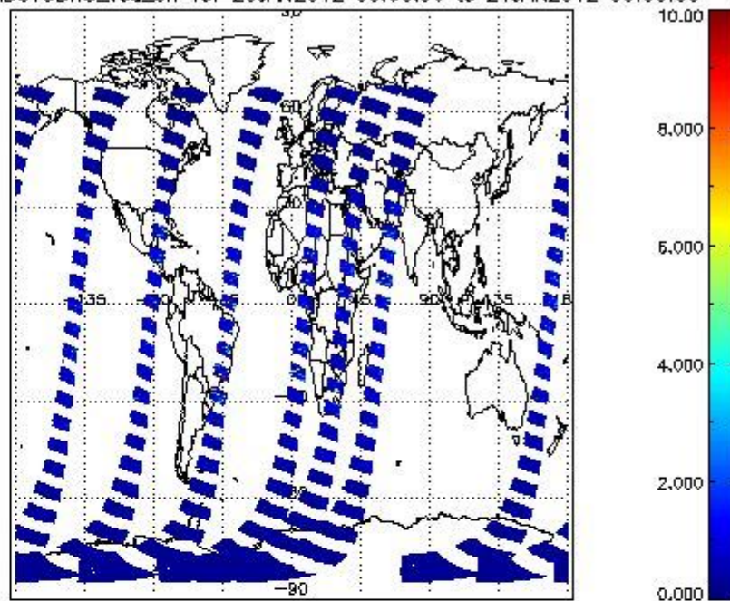
SCIOL2P_NADUV3BRO_vcd_err for 20JAN2012 00:00:00 to 21JAN2012 00:00:00
