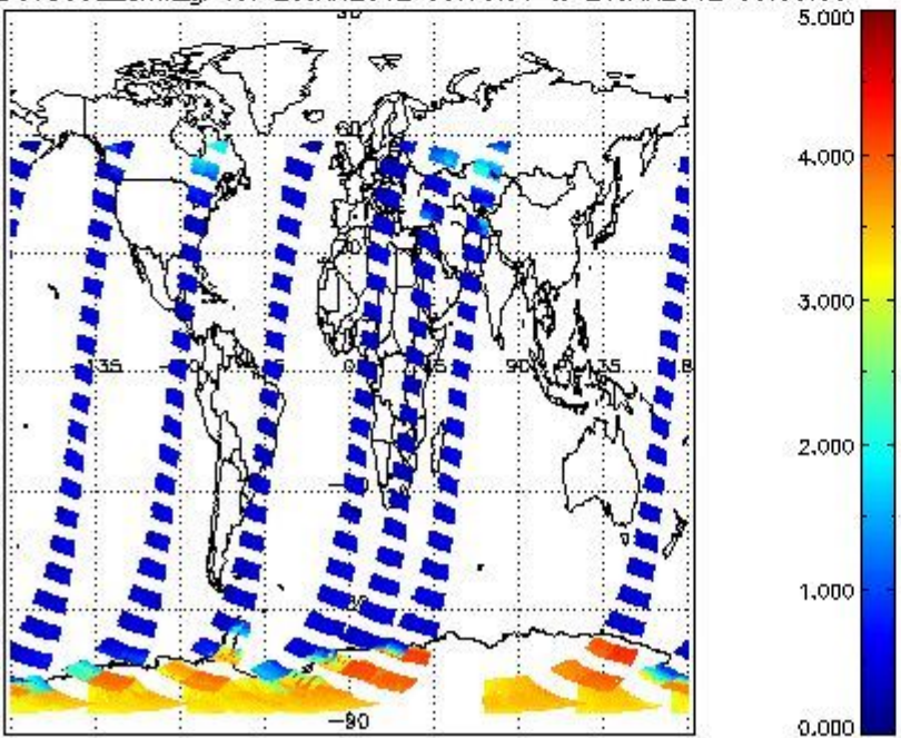
SCIOL2P_NADUV5SO2_amf_gr for 20JAN2012 00:00:00 to 21JAN2012 00:00:00
