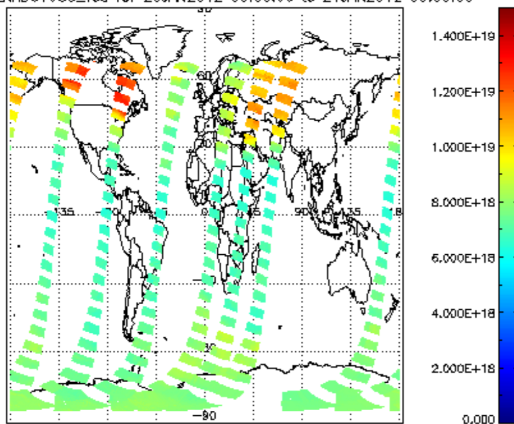
SCIOL2P_NADUV003_vcd for 20JAN2012 00:00:00 to 21JAN2012 00:00:00
