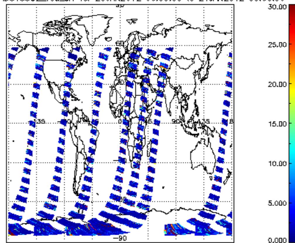
SCIOL2P_NADUV5S02_vcd_err for 20JAN2012 00:00:00 to 21JAN2012 00:00:00
