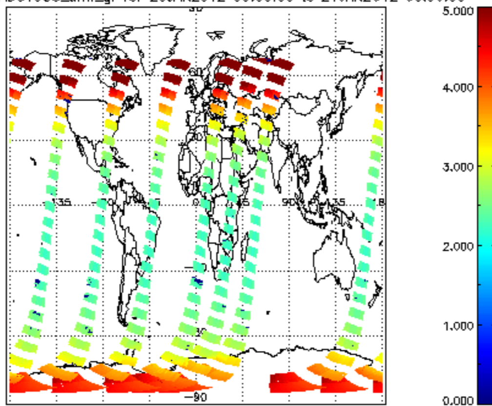
SCIOL2P_NADUV003_amf_gr for 20JAN2012 00:00:00 to 21JAN2012 00:00:00
