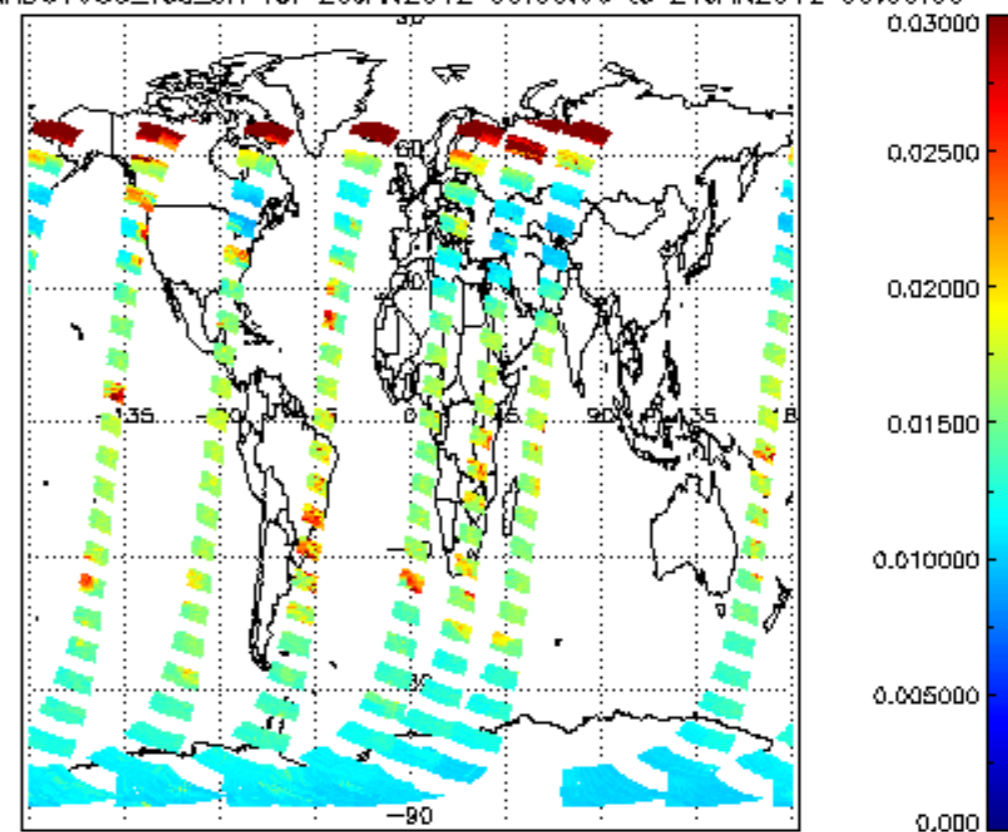
SCIOL2P_NADUV003_vcd_err for 20JAN2012 00:00:00 to 21JAN2012 00:00:00
