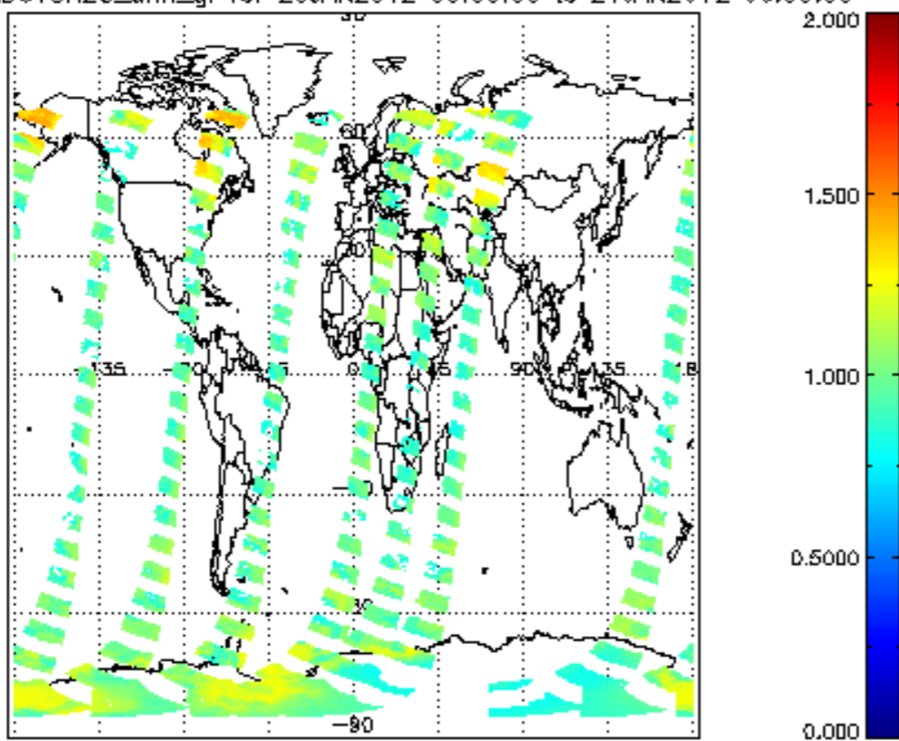
SCIOL2P_NADUV8H20_amf_gr for 20JAN2012 00:00:00 to 21JAN2012 00:00:00
