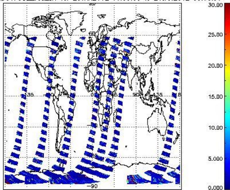
SCIOL2P_NADUV7S02_vcd_err for 20JAN2012 00:00:00 to 21JAN2012 00:00:00
