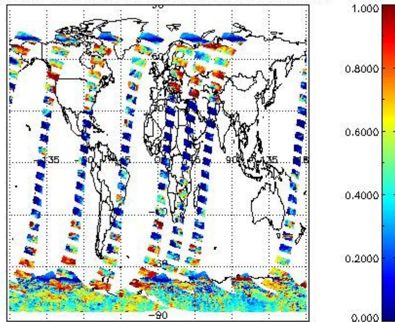
cL_frac for 20JAN2012 00:00:00 to 21JAN2012 00:00:00
