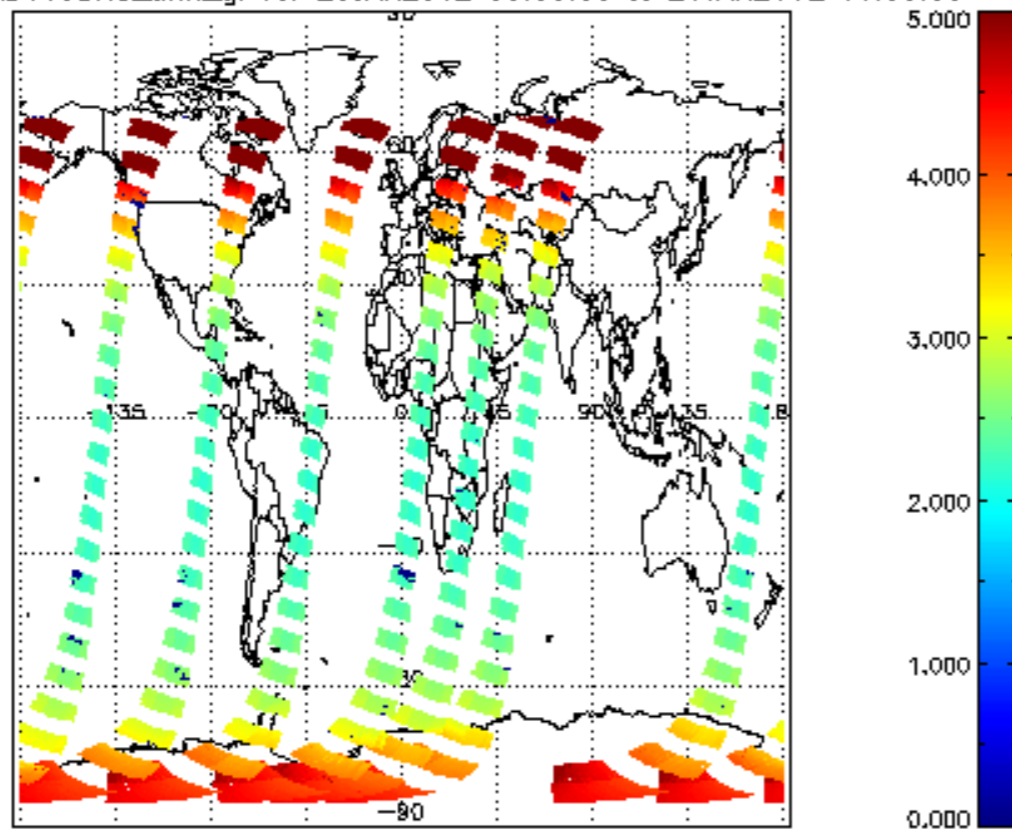
SCIOL2P_NADUV3BRO_amf_gr for 20JAN2012 00:00:00 to 21JAN2012 00:00:00
