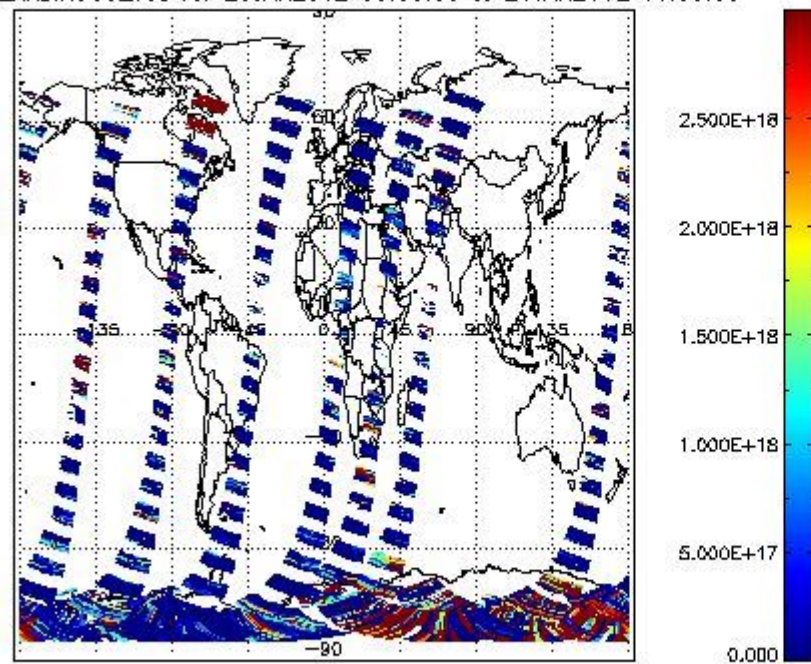
SCIDL2P_NADIR3CO_vcd for 20JAN2012 00:00:00 to 21JAN2012 00:00:00
