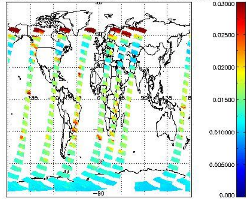
SCIOL2P_NADUV003_vcd_err for 20JAN2012 00:00:00 to 21JAN2012 00:00:00
