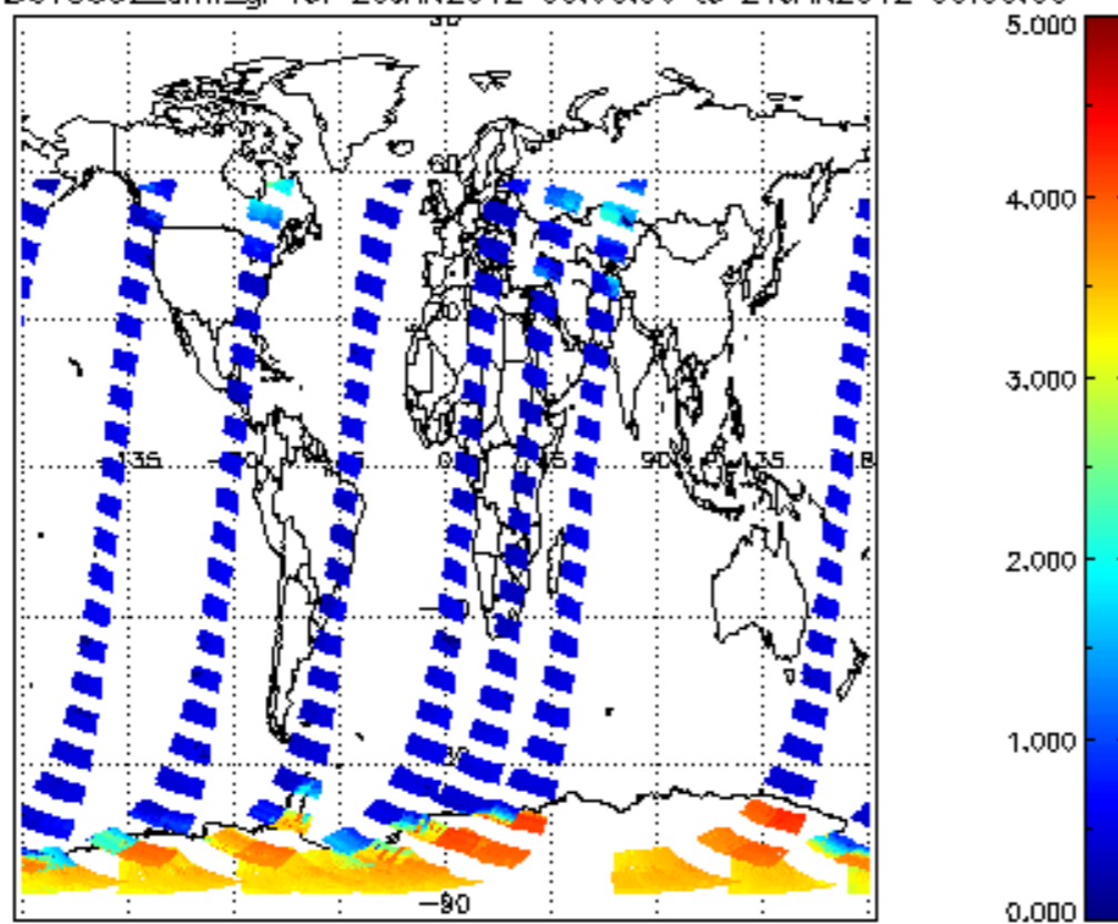
SCIOL2P_NADUV5S02_amf_gr for 20JAN2012 00:00:00 to 21JAN2012 00:00:00
