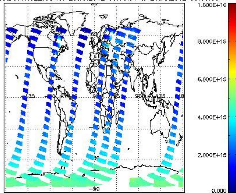
SCIOL2P_NADUV1NO2_vcd for 20JAN2012 00:00:00 to 21JAN2012 00:00:00
