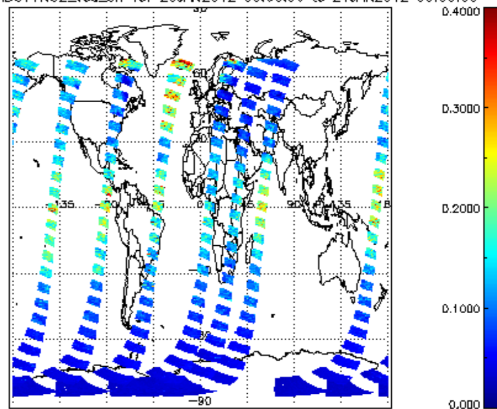
SCIOL2P_NADUV1NO2_vcd_err for 20JAN2012 00:00:00 to 21JAN2012 00:00:00
