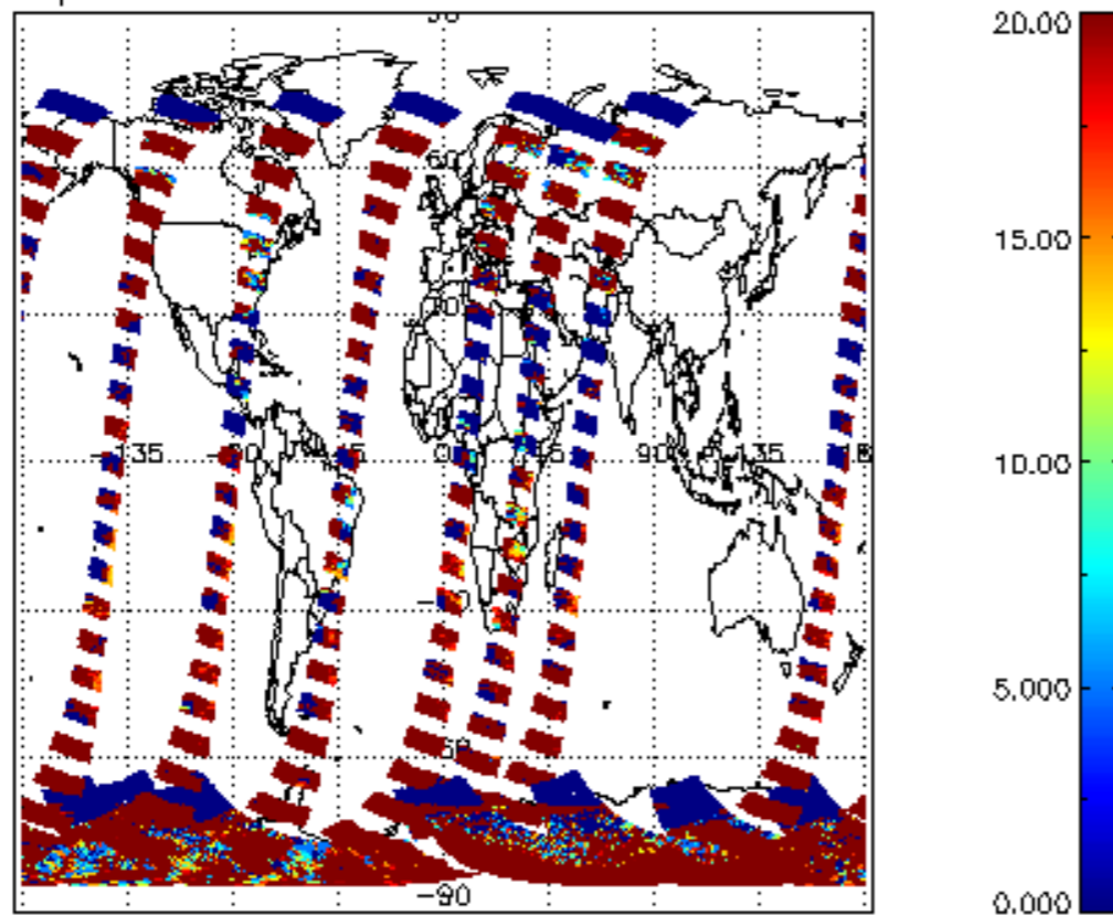
cLopt_depth for 20JAN2012 00:00:00 to 21JAN2012 00:00:00
