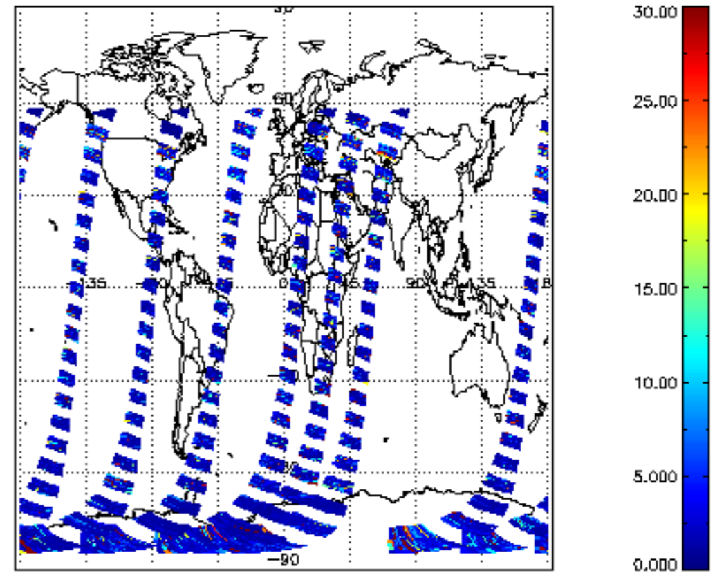
SCIOL2P_NADUV7S02_vcd_err for 20JAN2012 00:00:00 to 21JAN2012 00:00:00
