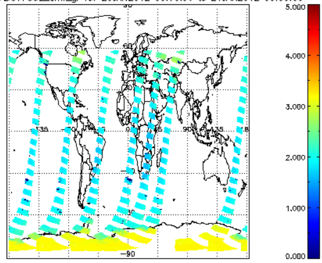
SCIOL2P_NADUV7S02_amf_gr for 20JAN2012 00:00:00 to 21JAN2012 00:00:00
