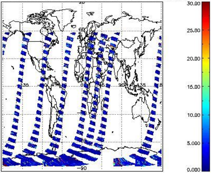
SCIOL2P_NADUV5SO2_vcd_err for 20JAN2012 00:00:00 to 21JAN2012 00:00:00
