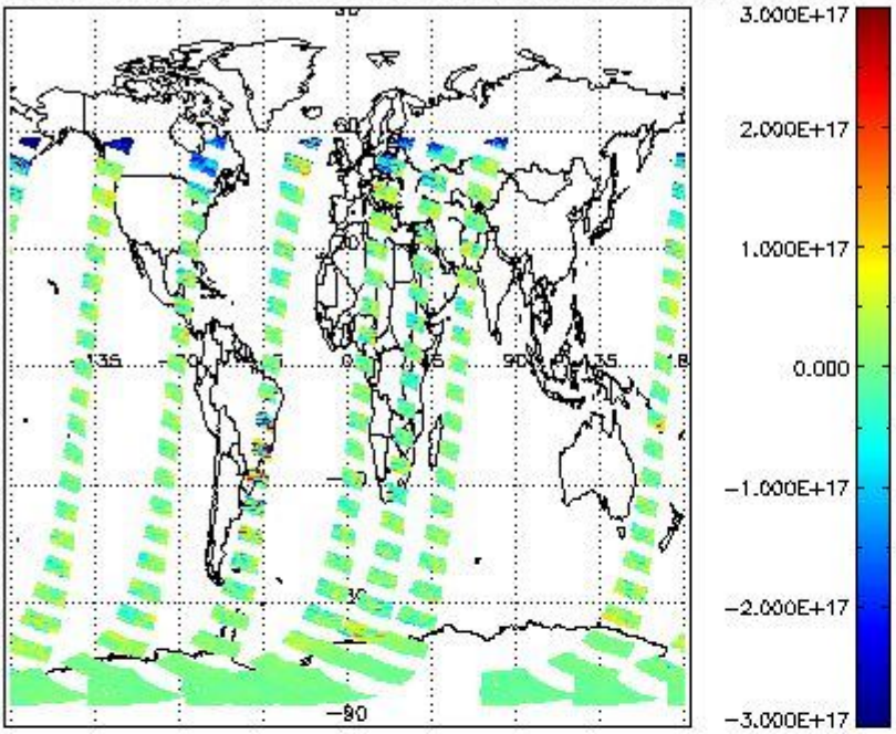
SCIOL2P_NADUV5SO2_vcd for 20JAN2012 00:00:00 to 21JAN2012 00:00:00
