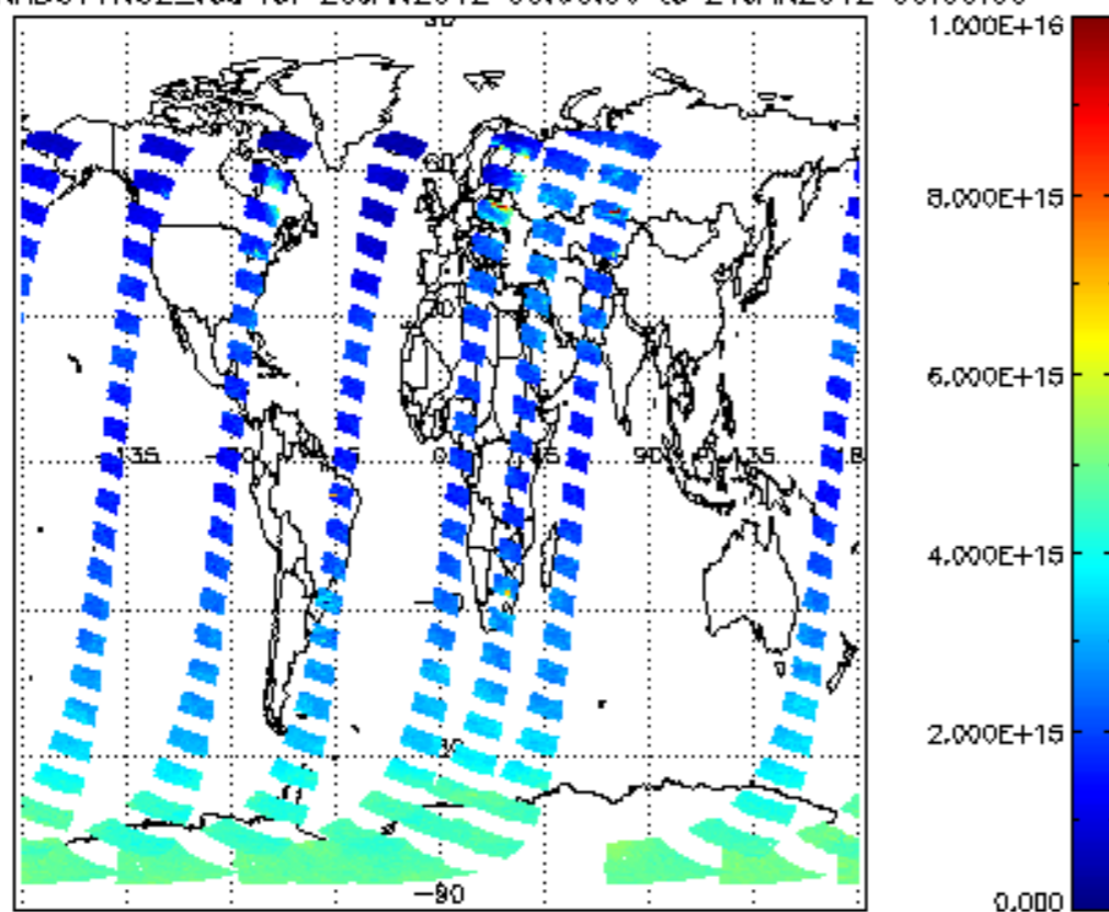
SCIOL2P_NADUV1NO2_vcd for 20JAN2012 00:00:00 to 21JAN2012 00:00:00
