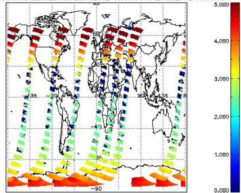
SCIOL2P_NADUV003_amf_cl for 20JAN2012 00:00:00 to 21JAN2012 00:00:00
