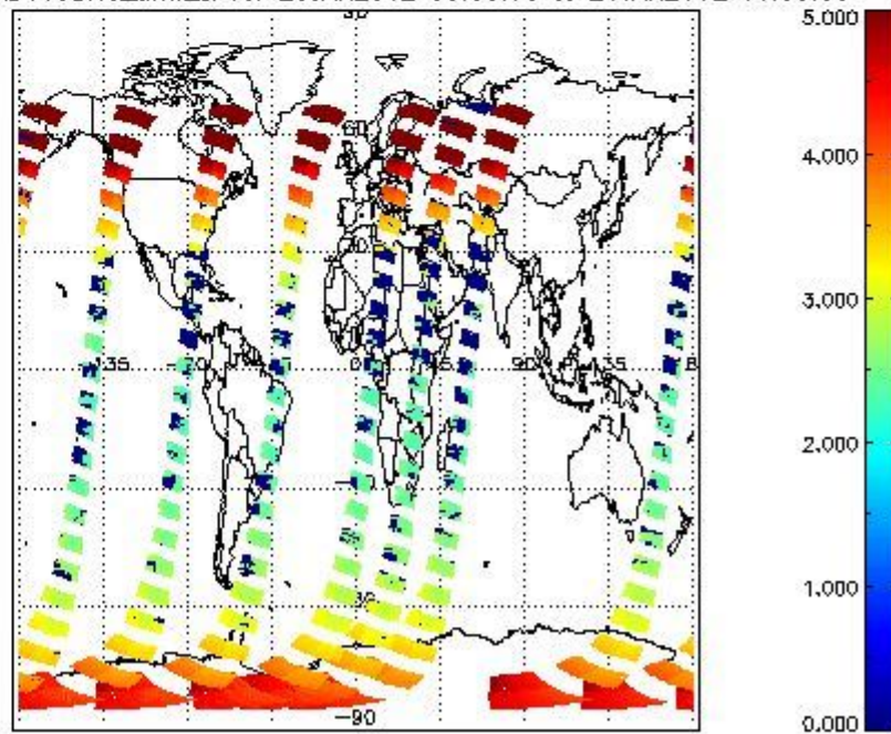
SCIOL2P_NADUV3BRO_amf_cl for 20JAN2012 00:00:00 to 21JAN2012 00:00:00
