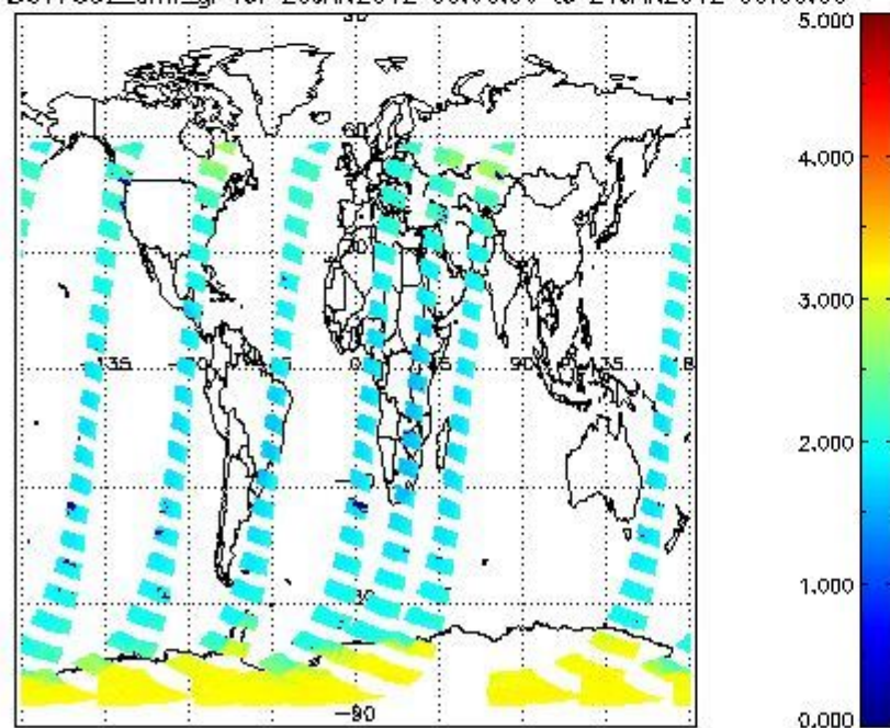
SCIOL2P_NADUV7S02_amf_gr for 20JAN2012 00:00:00 to 21JAN2012 00:00:00
