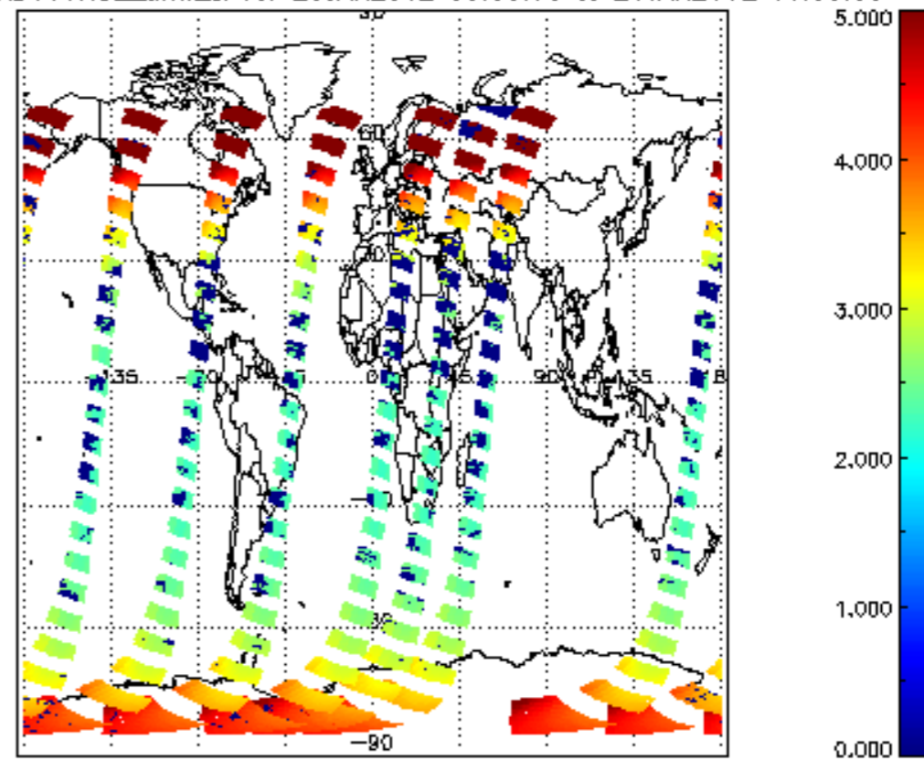
SCIOL2P_NADUV1NO2_amf_cl for 20JAN2012 00:00:00 to 21JAN2012 00:00:00
