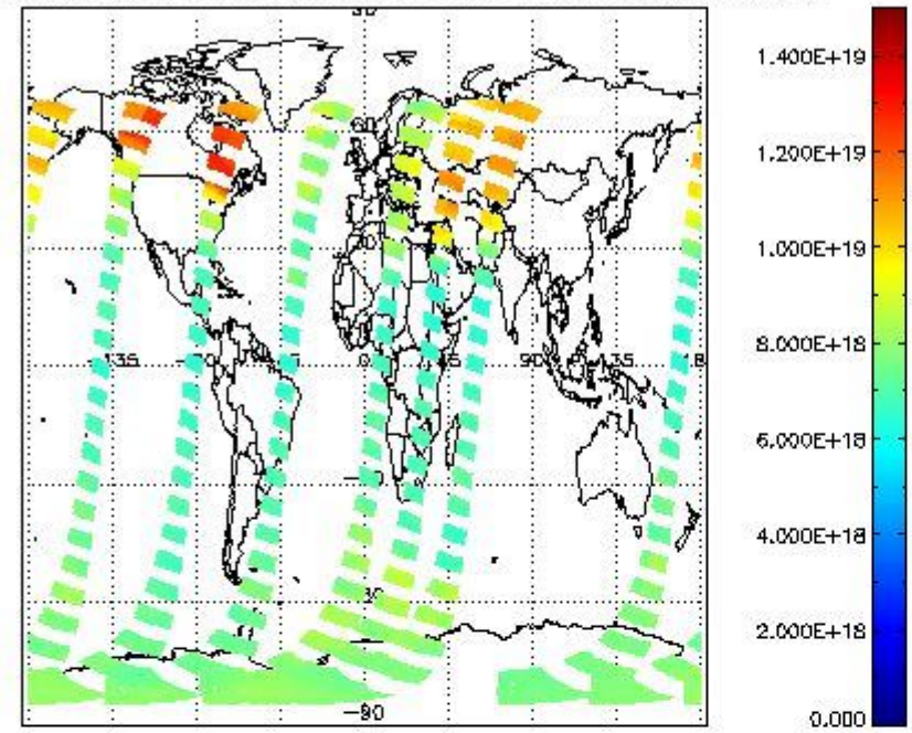
SCIOL2P_NADUV003_vcd for 20JAN2012 00:00:00 to 21JAN2012 00:00:00
