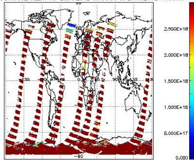
SCIDL2P_NADIR3CO_vcd_err for 20JAN2012 00:00:00 to 21JAN2012 00:00:00
