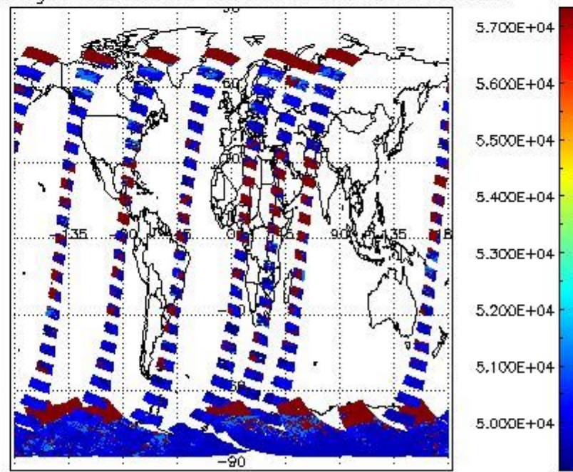
cloud_flags for 20JAN2012 00:00:00 to 21JAN2012 00:00:00
