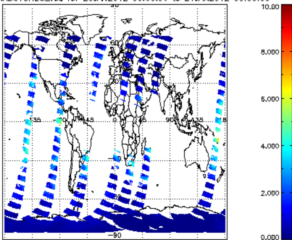
SCIOL2P_NADUV8H20_vcd for 20JAN2012 00:00:00 to 21JAN2012 00:00:00
