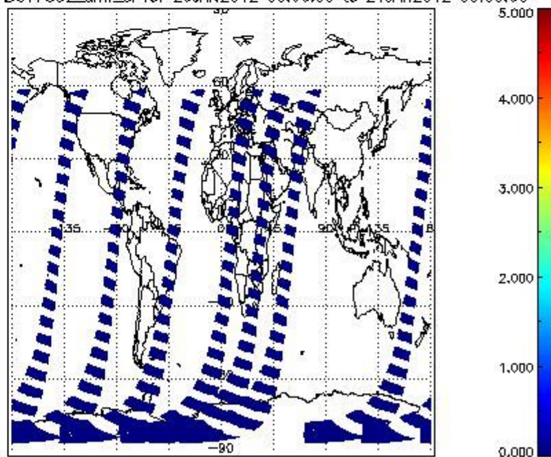
SCIOL2P_NADUV7S02_amf_cl for 20JAN2012 00:00:00 to 21JAN2012 00:00:00
