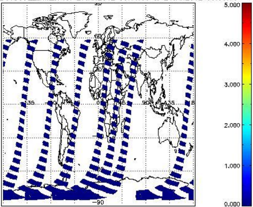
SCIOL2P_NADUV5SO2_amf_cl for 20JAN2012 00:00:00 to 21JAN2012 00:00:00
