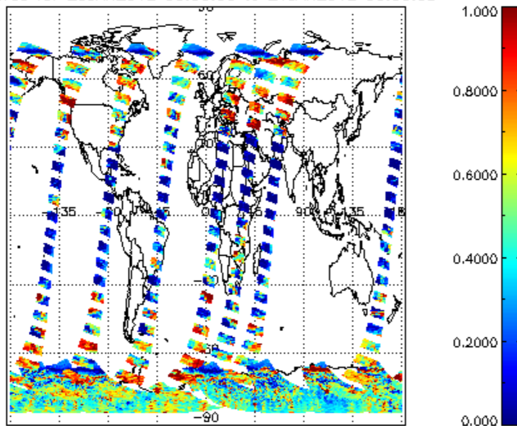
cL_frac for 20JAN2012 00:00:00 to 21JAN2012 00:00:00
