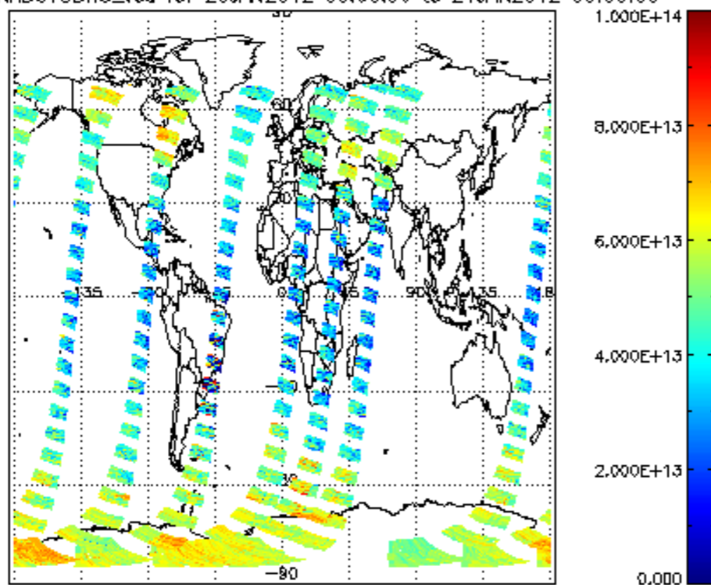
SCIOL2P_NADUV3BRO_vcd for 20JAN2012 00:00:00 to 21JAN2012 00:00:00
