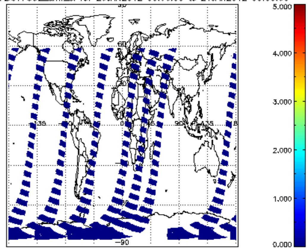
SCIOL2P_NADUV7S02_amf_sl for 20JAN2012 00:00:00 to 21JAN2012 00:00:00
