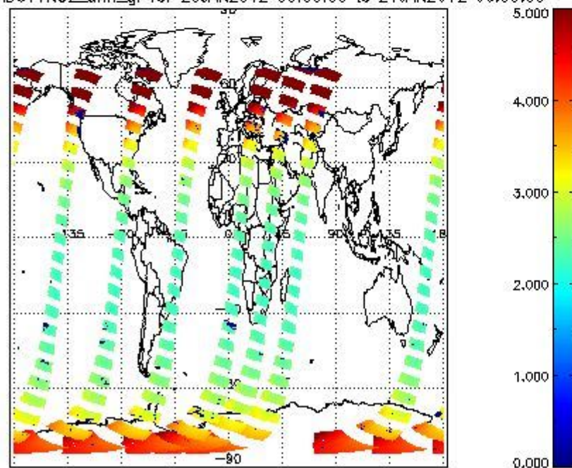
SCIOL2P_NADUV1NO2_amf_gr for 20JAN2012 00:00:00 to 21JAN2012 00:00:00
