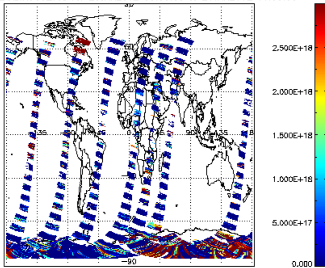
SCIOL2P_NADIR3CO_vcd for 20JAN2012 00:00:00 to 21JAN2012 00:00:00
