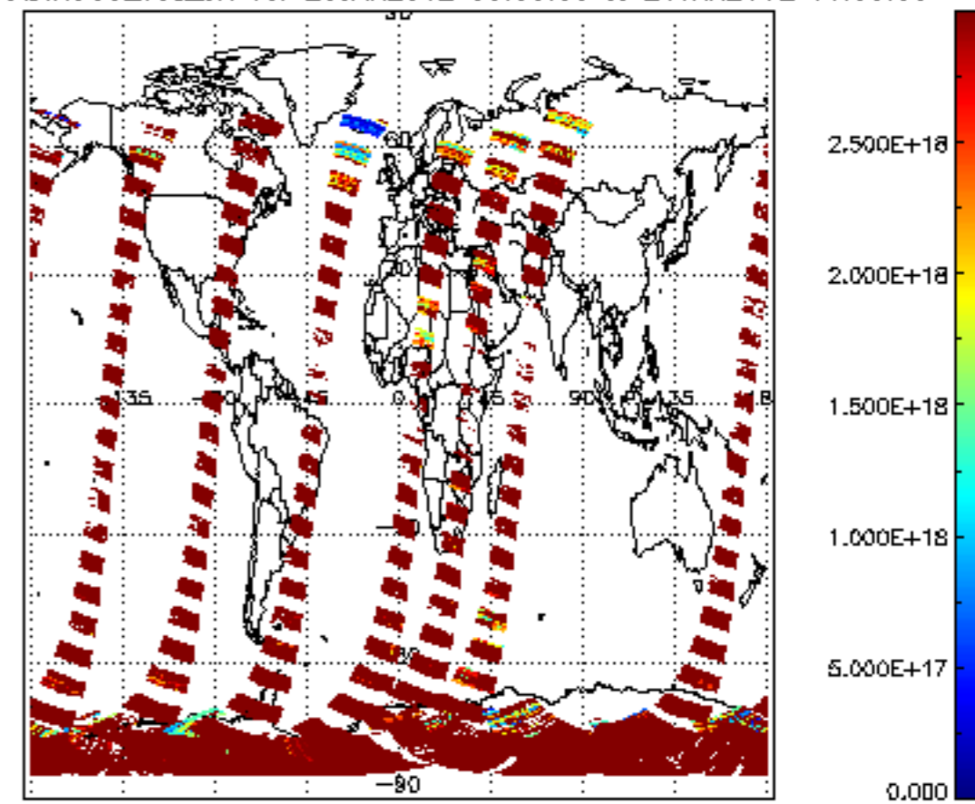
SCIOL2P_NADIR3CO_vcd_err for 20JAN2012 00:00:00 to 21JAN2012 00:00:00
