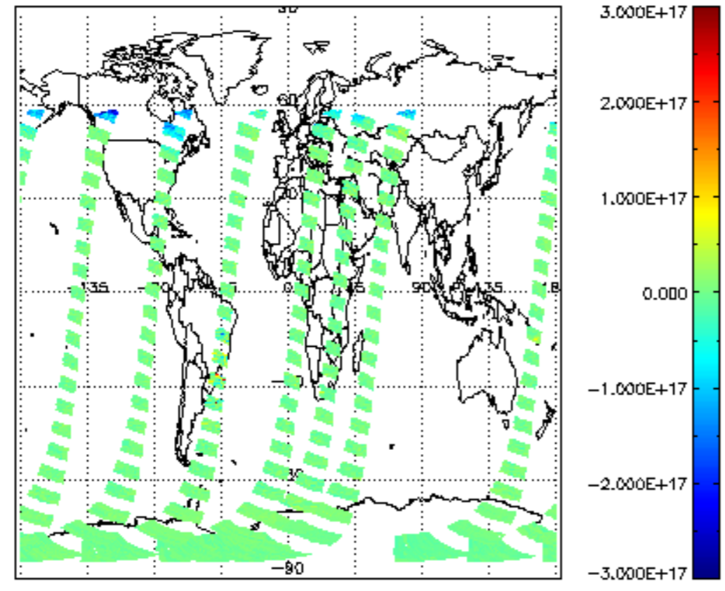
SCIOL2P_NADUV7S02_vcd for 20JAN2012 00:00:00 to 21JAN2012 00:00:00
