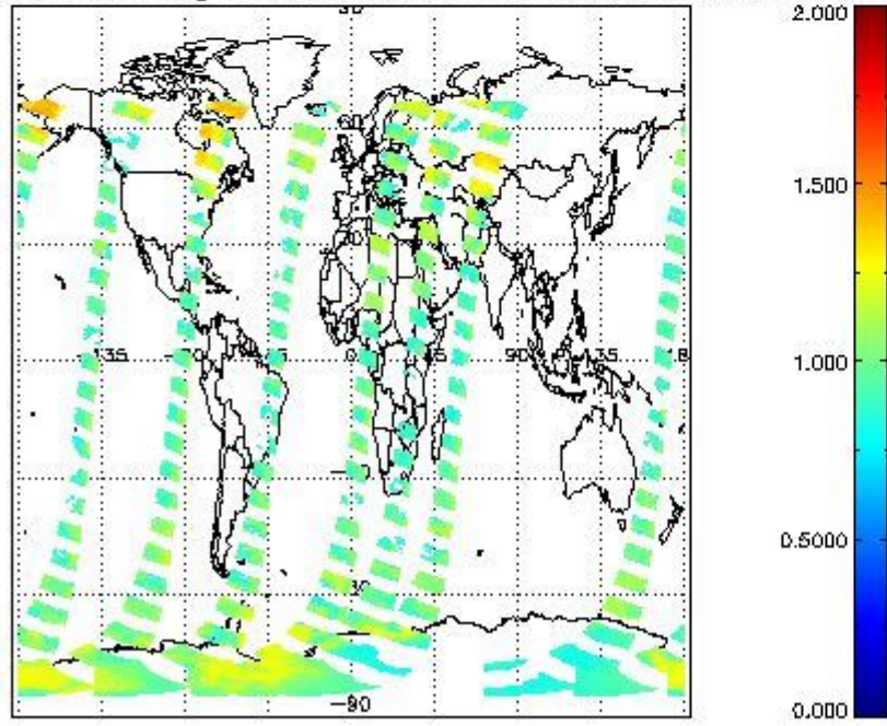
SCIOL2P_NADUV8H20_amf_gr for 20JAN2012 00:00:00 to 21JAN2012 00:00:00
