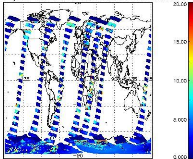
cL_top_height for 20JAN2012 00:00:00 to 21JAN2012 00:00:00
