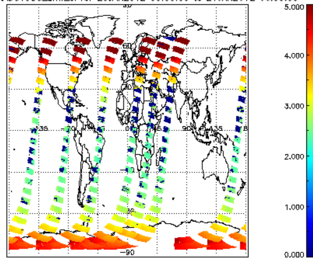
SCIOL2P_NADUV003_amf_cl for 20JAN2012 00:00:00 to 21JAN2012 00:00:00
