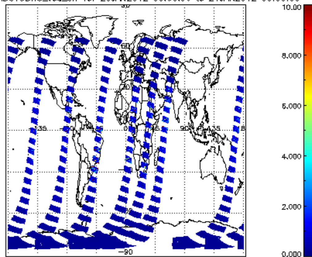
SCIOL2P_NADUV3BRO_vcd_err for 20JAN2012 00:00:00 to 21JAN2012 00:00:00
