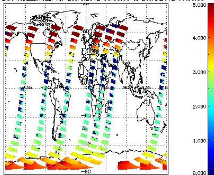
SCIOL2P_NADUV1NO2_amf_cl for 20JAN2012 00:00:00 to 21JAN2012 00:00:00
