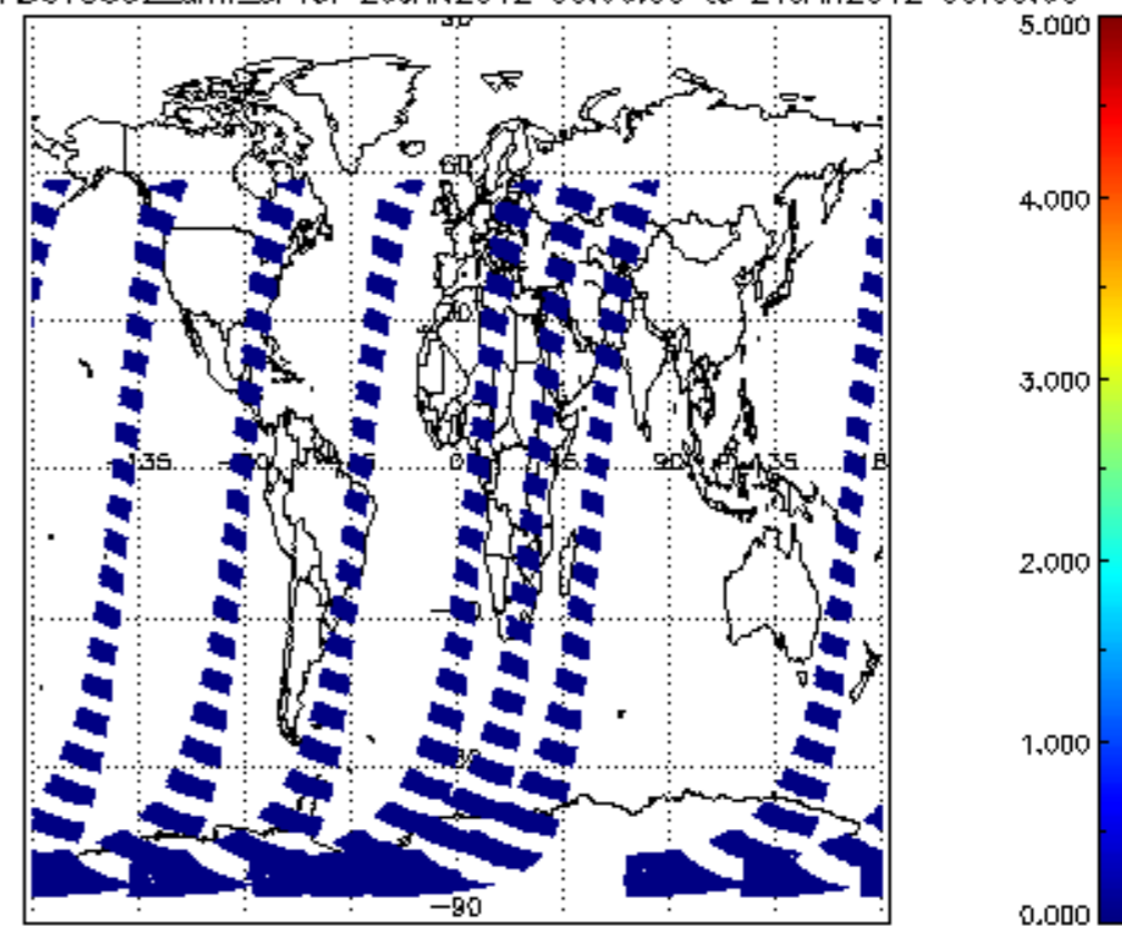
SCIOL2P_NADUV5S02_amf_sl for 20JAN2012 00:00:00 to 21JAN2012 00:00:00
