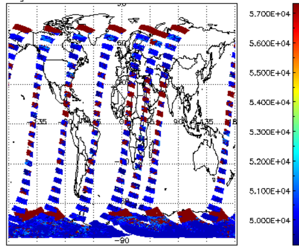
cloud_flags for 20JAN2012 00:00:00 to 21JAN2012 00:00:00
