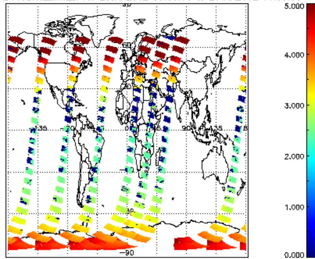
SCIOL2P_NADUV3BRO_amf_cl for 20JAN2012 00:00:00 to 21JAN2012 00:00:00
