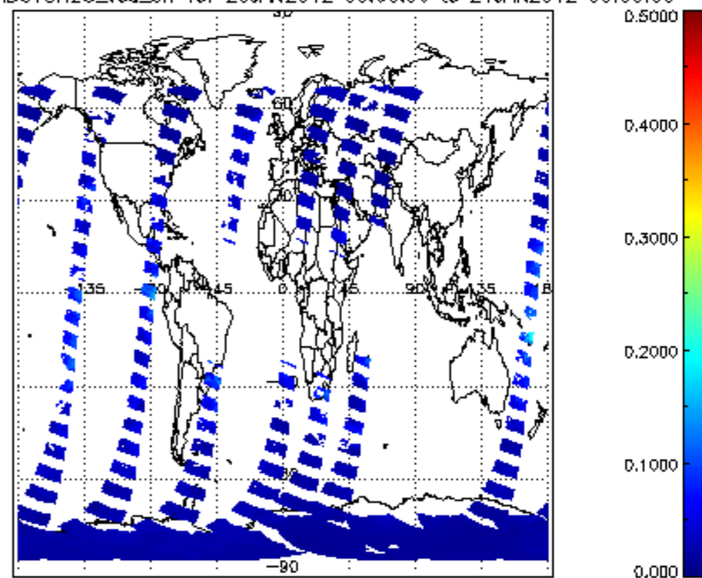
SCIOL2P_NADUV8H20_vcd_err for 20JAN2012 00:00:00 to 21JAN2012 00:00:00
