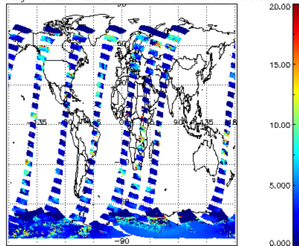
cL_top_height for 20JAN2012 00:00:00 to 21JAN2012 00:00:00
