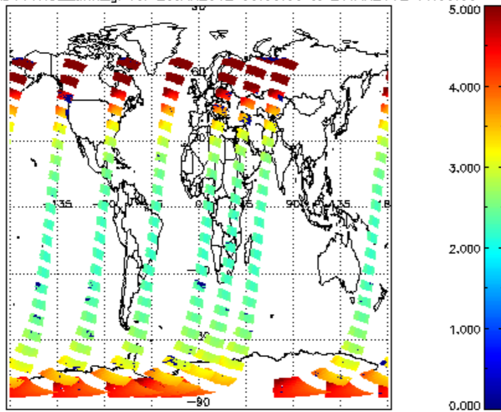
SCIOL2P_NADUV1NO2_amf_gr for 20JAN2012 00:00:00 to 21JAN2012 00:00:00
