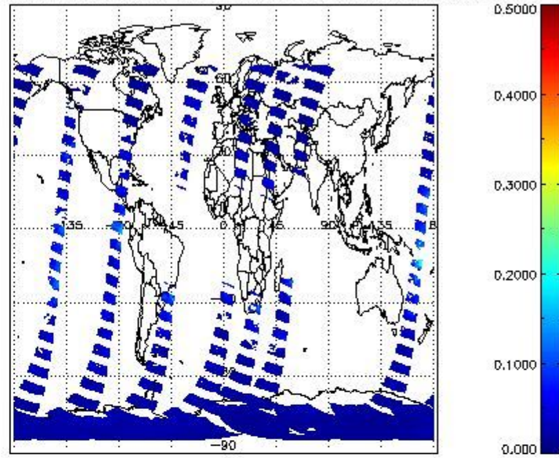
SCIOL2P_NADUV8H20_vcd_err for 20JAN2012 00:00:00 to 21JAN2012 00:00:00
