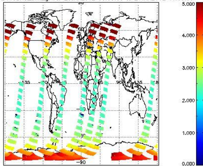
SCIOL2P_NADUV3BRO_amf_gr for 20JAN2012 00:00:00 to 21JAN2012 00:00:00
