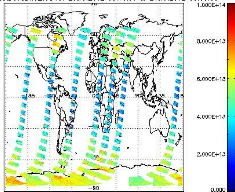
SCIOL2P_NADUV3BRO_vcd for 20JAN2012 00:00:00 to 21JAN2012 00:00:00
