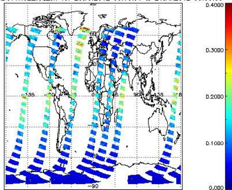
SCIOL2P_NADUV1NO2_vcd_err for 20JAN2012 00:00:00 to 21JAN2012 00:00:00
