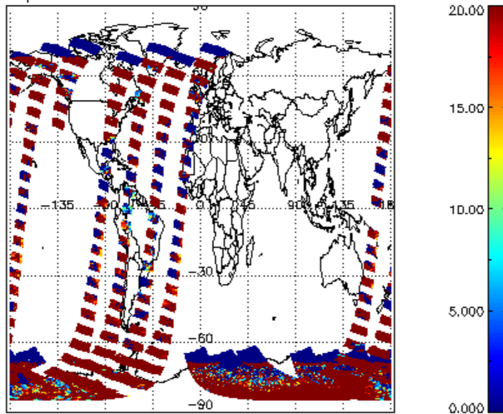
cLopt_depth for 17JAN2012 00:00:00 to 18JAN2012 00:00:00
