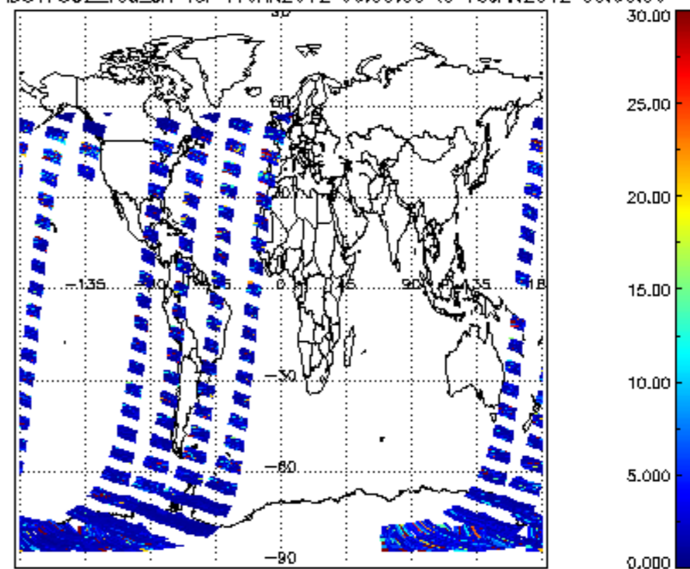
SCIOL2P_NADUV7S02_vcd_err for 17JAN2012 00:00:00 to 18JAN2012 00:00:00
