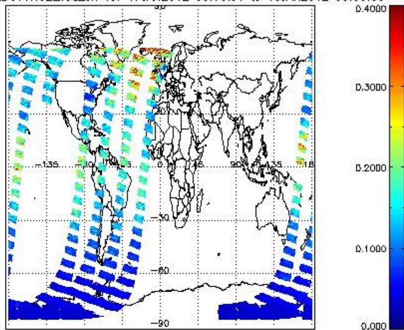
SCIOL2P_NADUV1NO2_vcd_err for 17JAN2012 00:00:00 to 18JAN2012 00:00:00
