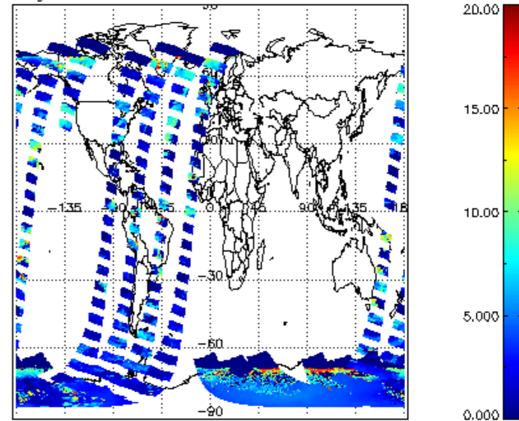
cL_top_height for 17JAN2012 00:00:00 to 18JAN2012 00:00:00
