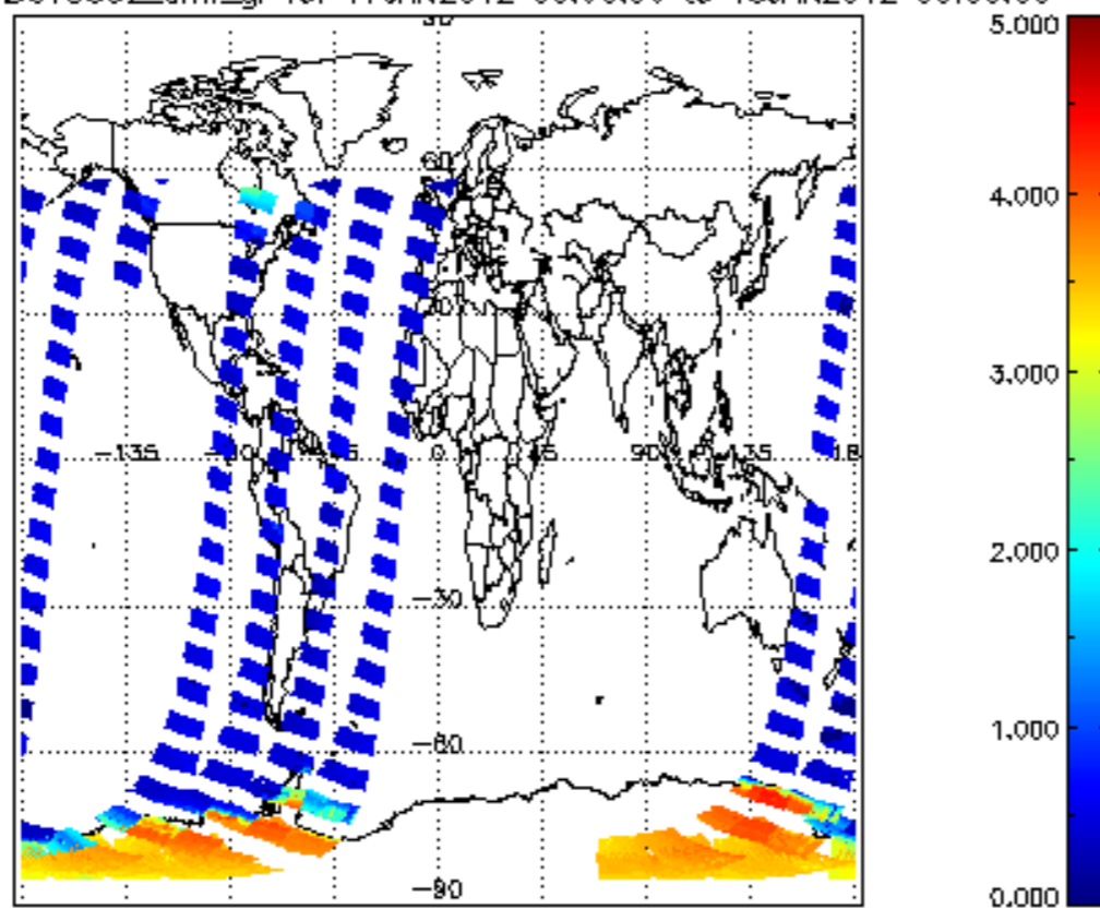
SCIOL2P_NADUV5S02_amf_gr for 17JAN2012 00:00:00 to 18JAN2012 00:00:00
