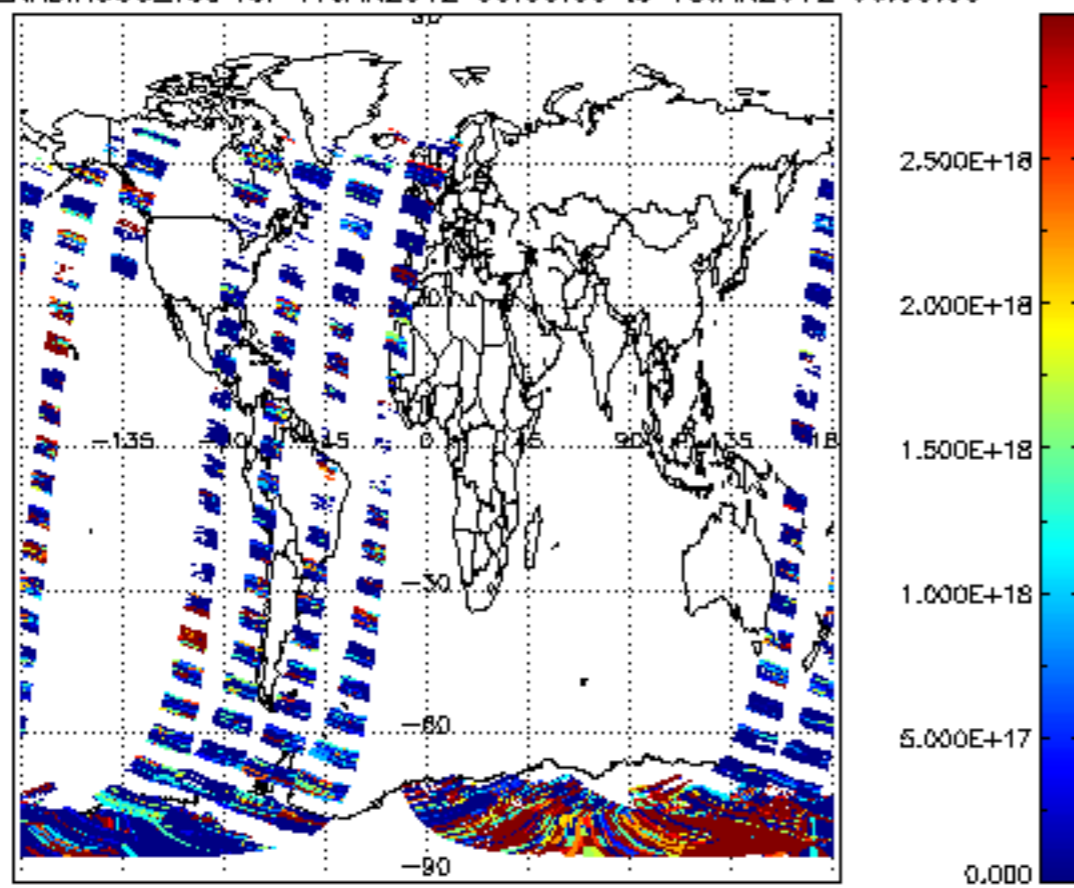
SCIOL2P_NADIR3CO_vcd for 17JAN2012 00:00:00 to 18JAN2012 00:00:00
