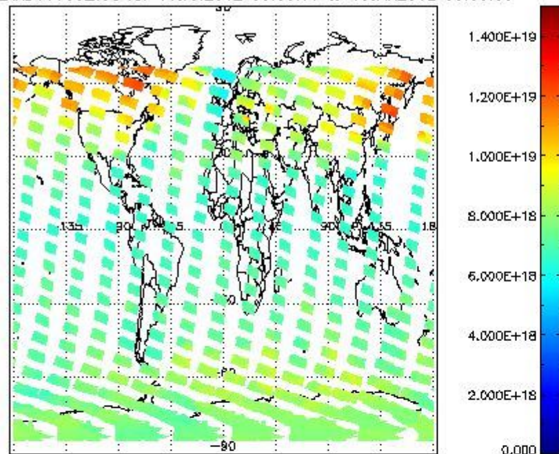
SCIOL2P_NADUV003_vcd for 14JAN2012 00:00:00 to 15JAN2012 00:00:00
