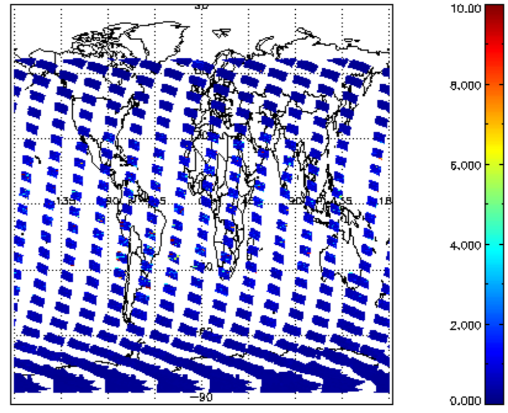
SCIOL2P_NADUV3BRO_vcd_err for 14JAN2012 00:00:00 to 15JAN2012 00:00:00
