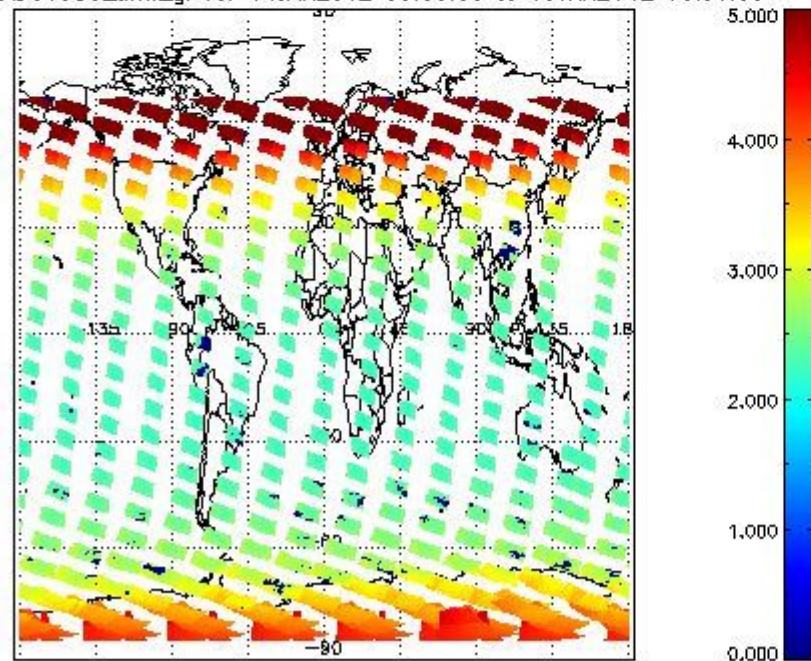
SCIOL2P_NADUV003_amf_gr for 14JAN2012 00:00:00 to 15JAN2012 00:00:00
