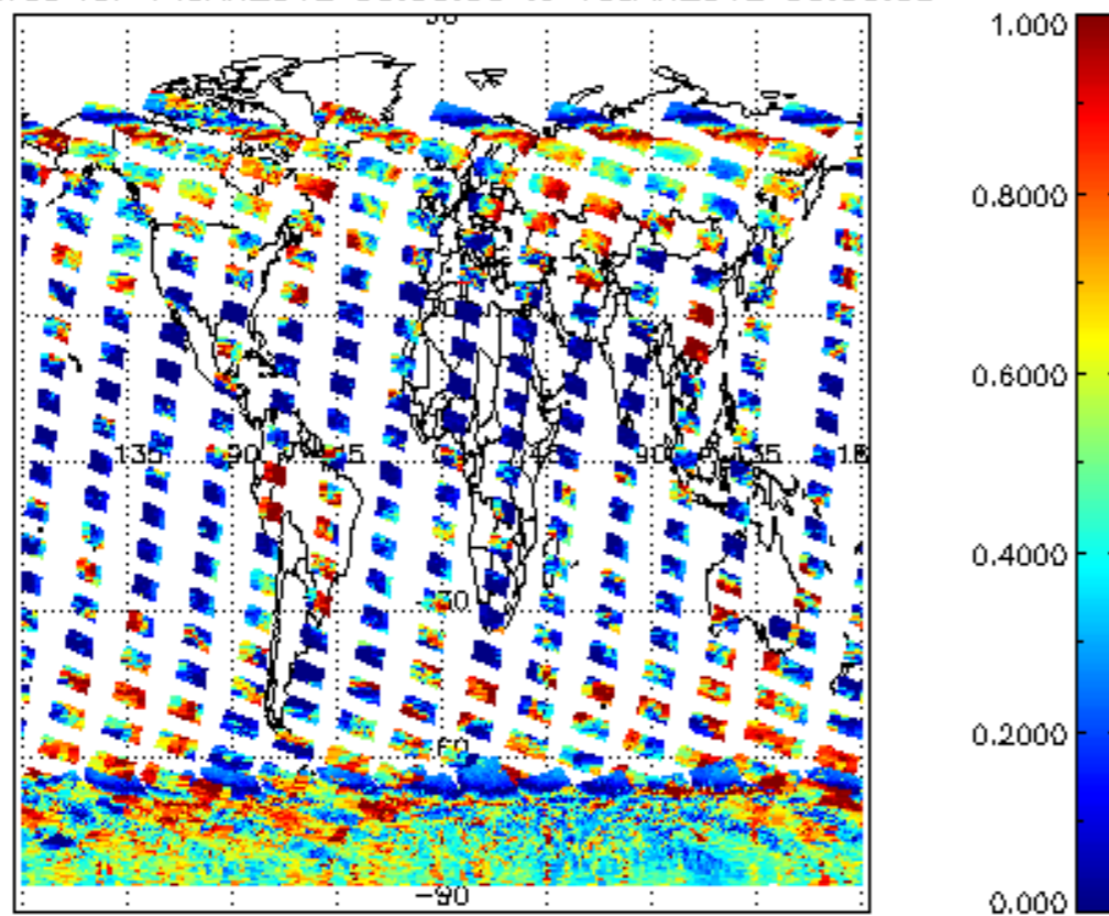
cL_frac for 14JAN2012 00:00:00 to 15JAN2012 00:00:00
