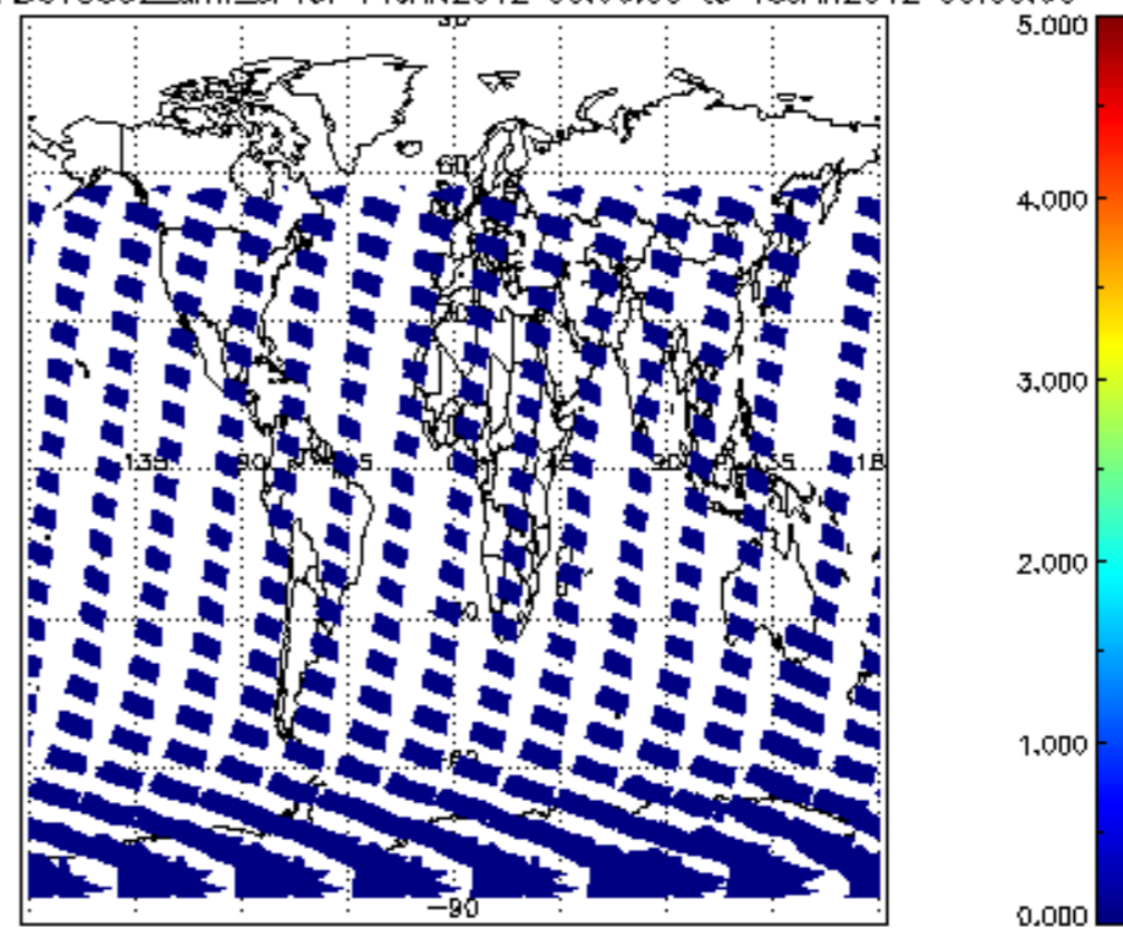
SCIOL2P_NADUV5S02_amf_sl for 14JAN2012 00:00:00 to 15JAN2012 00:00:00
