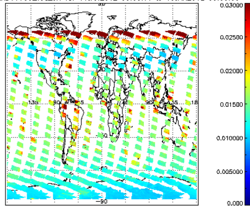
SCIOL2P_NADUV003_vcd_err for 14JAN2012 00:00:00 to 15JAN2012 00:00:00
