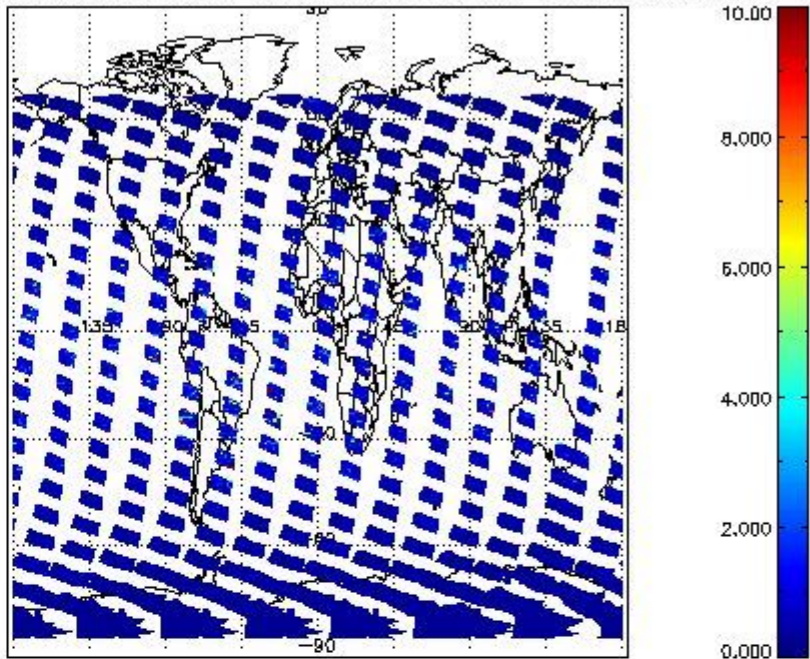
SCIOL2P_NADUV3BRO_vcd_err for 14JAN2012 00:00:00 to 15JAN2012 00:00:00
