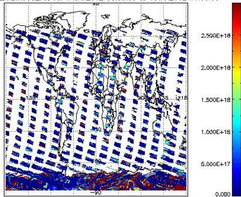
SCIOL2P_NADIR3CO_vcd for 14JAN2012 00:00:00 to 15JAN2012 00:00:00
