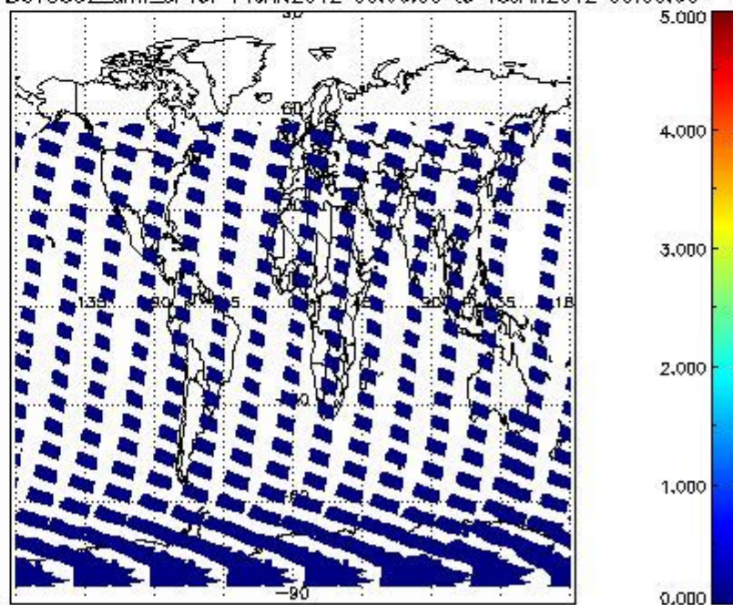
SCIOL2P_NADUV5SO2_amf_cl for 14JAN2012 00:00:00 to 15JAN2012 00:00:00
