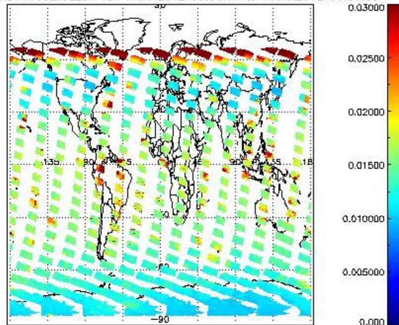
SCIOL2P_NADUV003_vcd_err for 14JAN2012 00:00:00 to 15JAN2012 00:00:00
