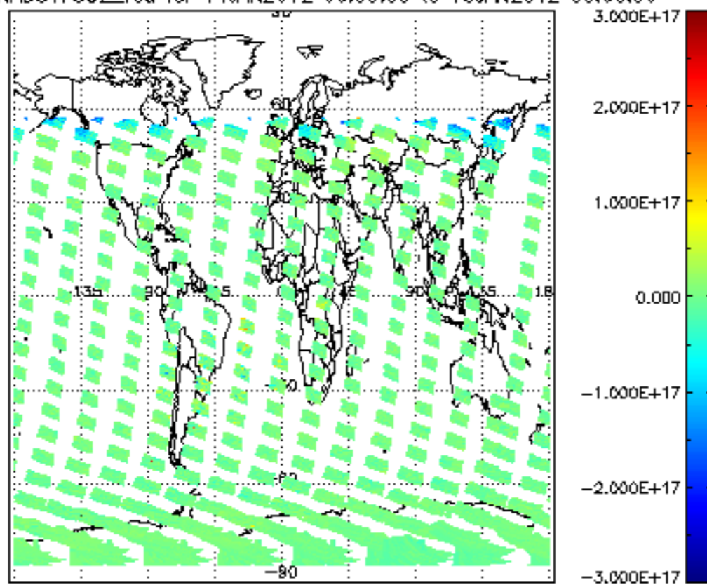
SCIOL2P_NADUV7S02_vcd for 14JAN2012 00:00:00 to 15JAN2012 00:00:00
