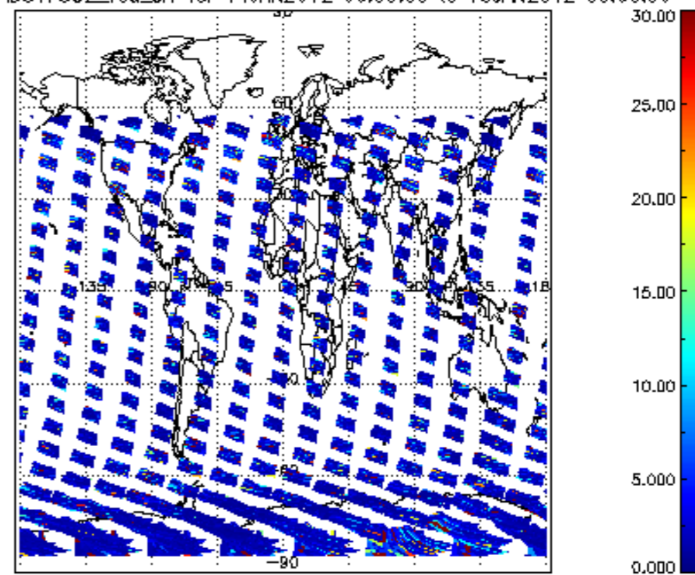
SCIOL2P_NADUV7S02_vcd_err for 14JAN2012 00:00:00 to 15JAN2012 00:00:00
