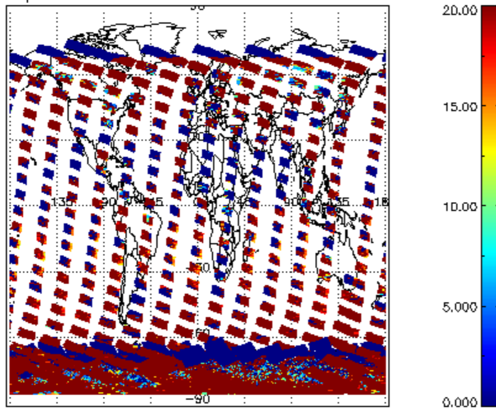
cLopt_depth for 14JAN2012 00:00:00 to 15JAN2012 00:00:00
