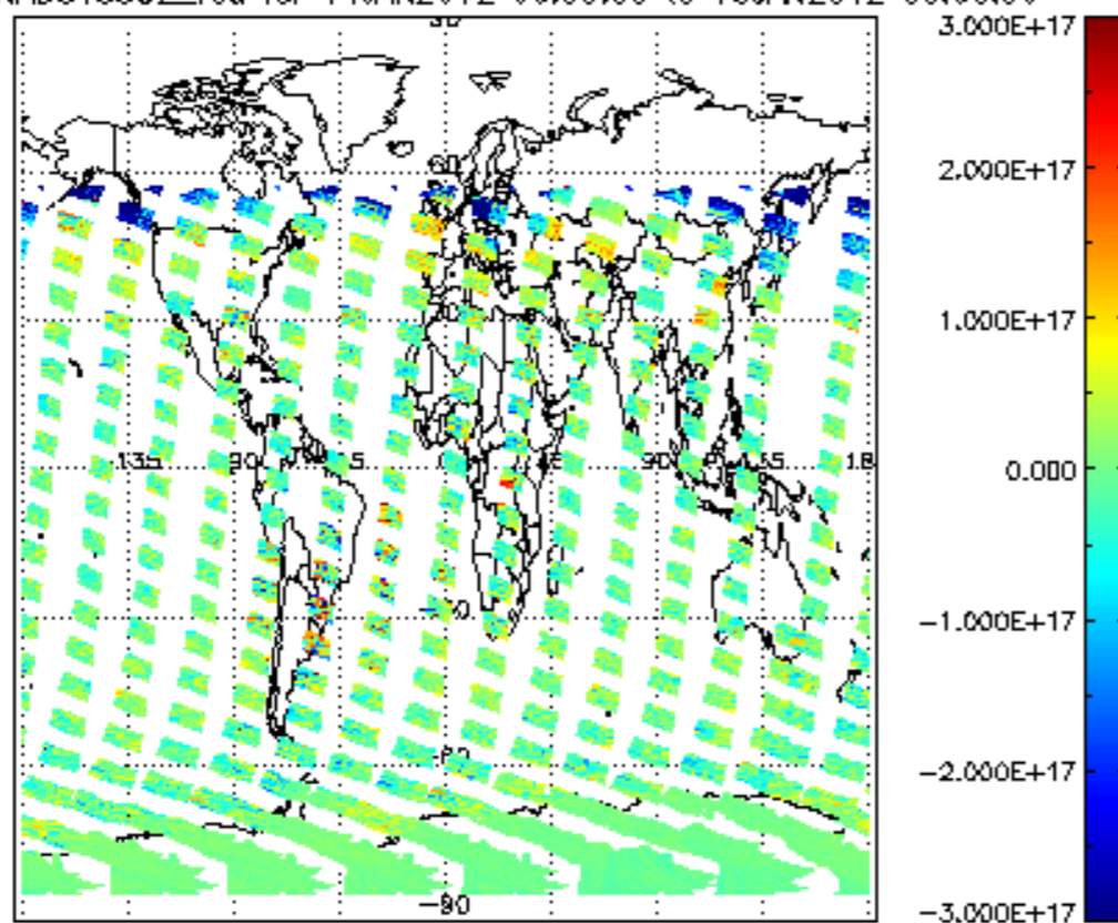
SCIOL2P_NADUV5S02_vcd for 14JAN2012 00:00:00 to 15JAN2012 00:00:00
