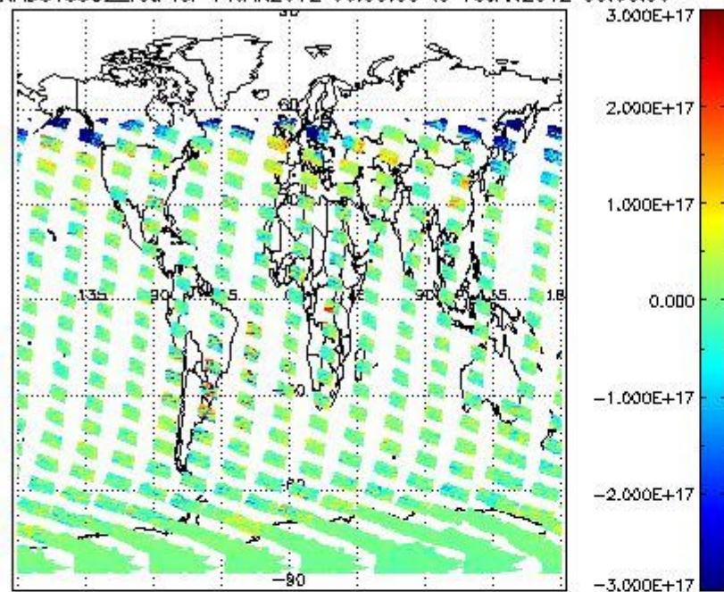
SCIOL2P_NADUV5SO2_vcd for 14JAN2012 00:00:00 to 15JAN2012 00:00:00
