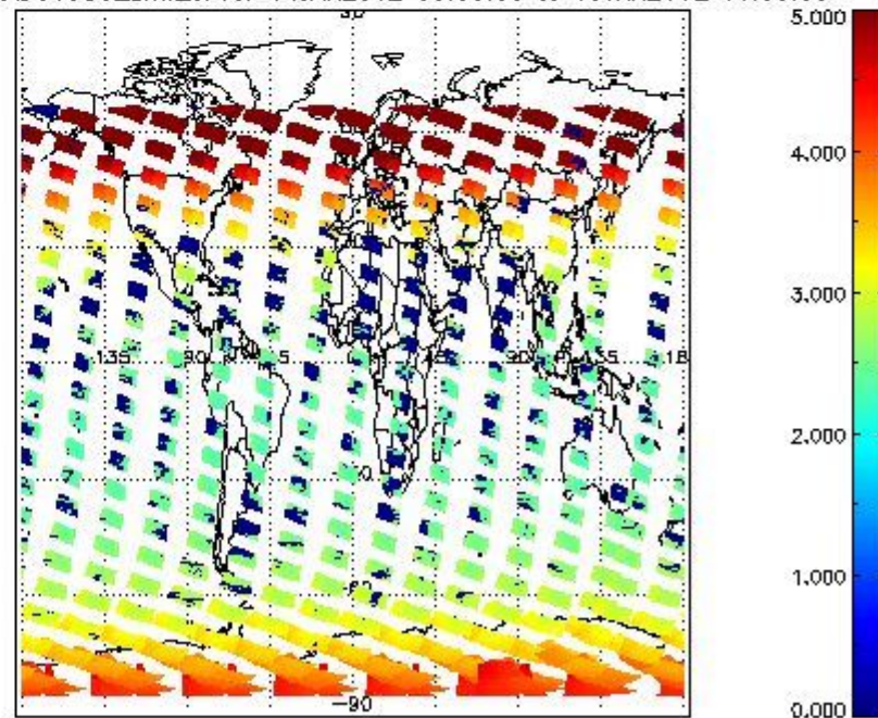
SCIOL2P_NADUV003_amf_cl for 14JAN2012 00:00:00 to 15JAN2012 00:00:00
