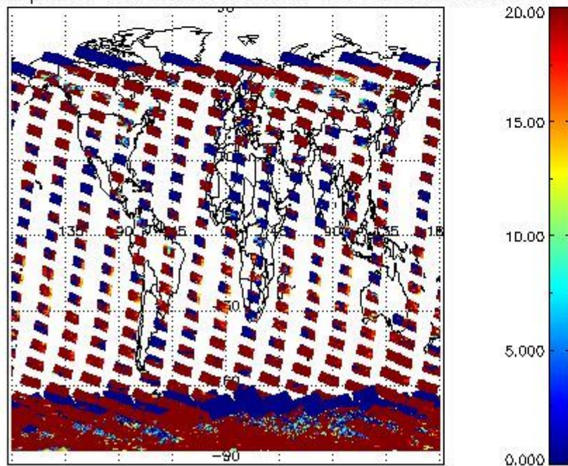
cLopt_depth for 14JAN2012 00:00:00 to 15JAN2012 00:00:00
