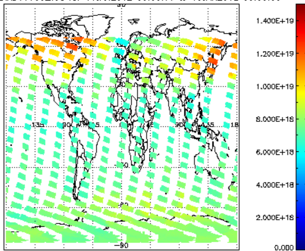
SCIOL2P_NADUV003_vcd for 14JAN2012 00:00:00 to 15JAN2012 00:00:00
