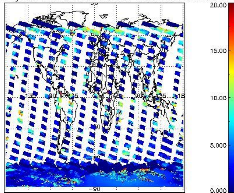
cL_top_height for 14JAN2012 00:00:00 to 15JAN2012 00:00:00
