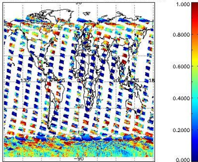
cL_frac for 14JAN2012 00:00:00 to 15JAN2012 00:00:00
