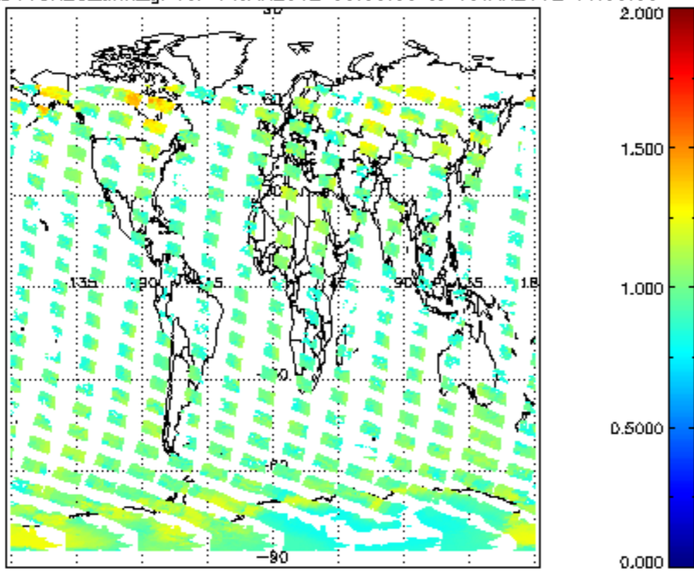
SCIOL2P_NADUV8H20_amf_gr for 14JAN2012 00:00:00 to 15JAN2012 00:00:00
