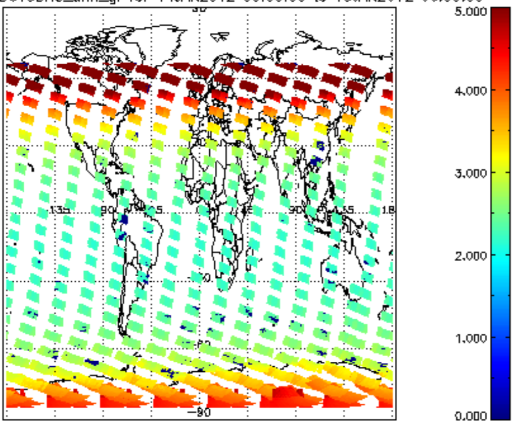
SCIOL2P_NADUV3BRO_amf_gr for 14JAN2012 00:00:00 to 15JAN2012 00:00:00
