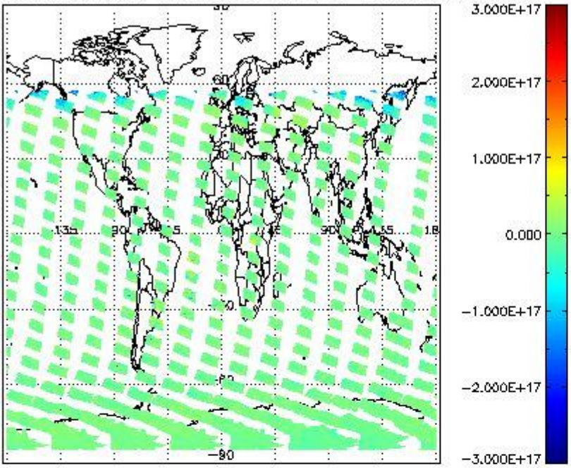
SCIOL2P_NADUV7S02_vcd for 14JAN2012 00:00:00 to 15JAN2012 00:00:00
