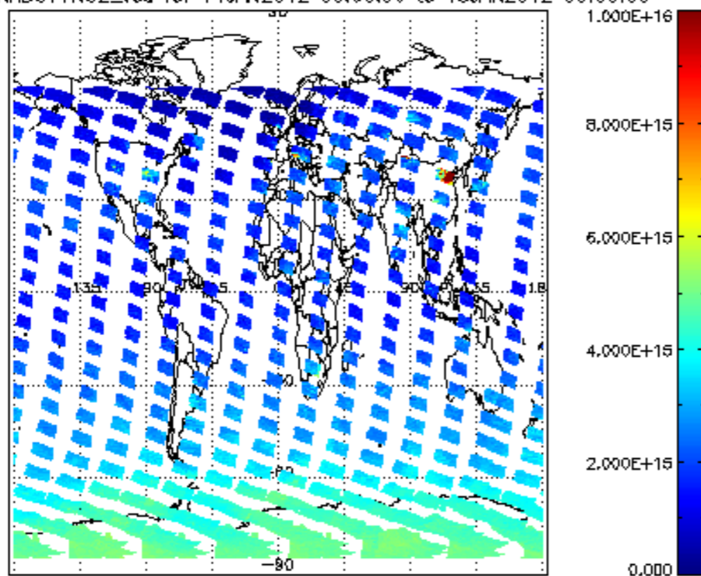
SCIOL2P_NADUV1NO2_vcd for 14JAN2012 00:00:00 to 15JAN2012 00:00:00
