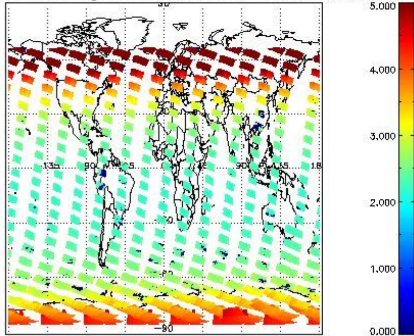
SCIOL2P_NADUV3BRO_amf_gr for 14JAN2012 00:00:00 to 15JAN2012 00:00:00
