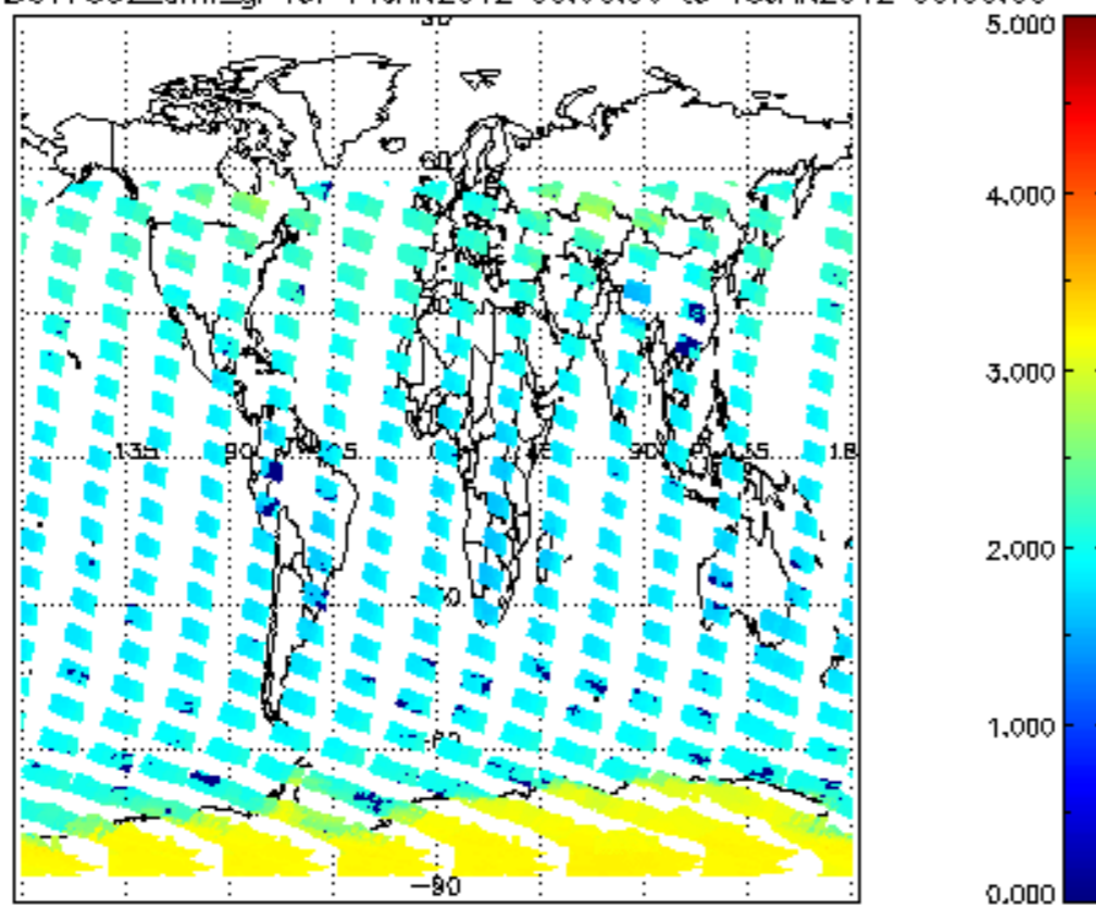
SCIOL2P_NADUV7S02_amf_gr for 14JAN2012 00:00:00 to 15JAN2012 00:00:00
