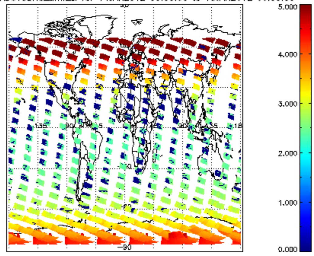
SCIOL2P_NADUV3BRO_amf_cl for 14JAN2012 00:00:00 to 15JAN2012 00:00:00
