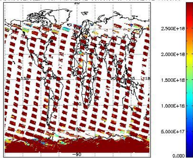
SCIOL2P_NADIR3CO_vcd_err for 14JAN2012 00:00:00 to 15JAN2012 00:00:00
