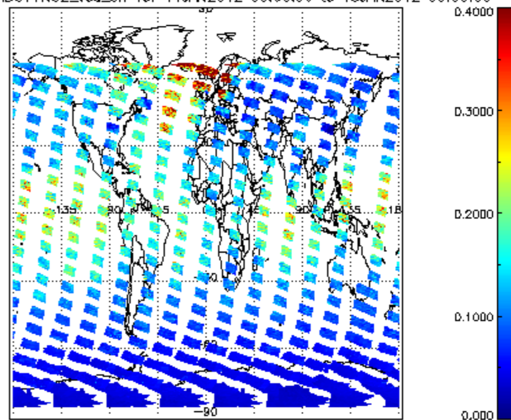
SCIOL2P_NADUV1NO2_vcd_err for 14JAN2012 00:00:00 to 15JAN2012 00:00:00
