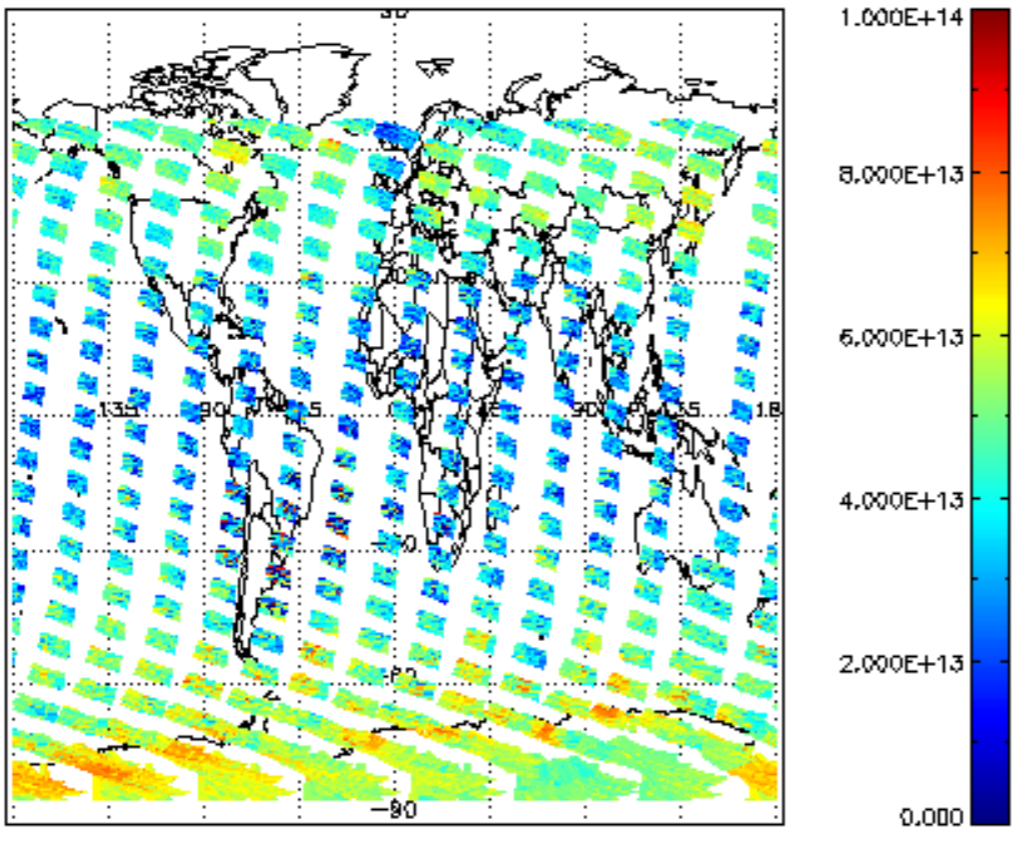
SCIOL2P_NADUV3BRO_vcd for 14JAN2012 00:00:00 to 15JAN2012 00:00:00
