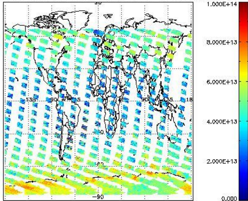
SCIOL2P_NADUV3BRO_vcd for 14JAN2012 00:00:00 to 15JAN2012 00:00:00
