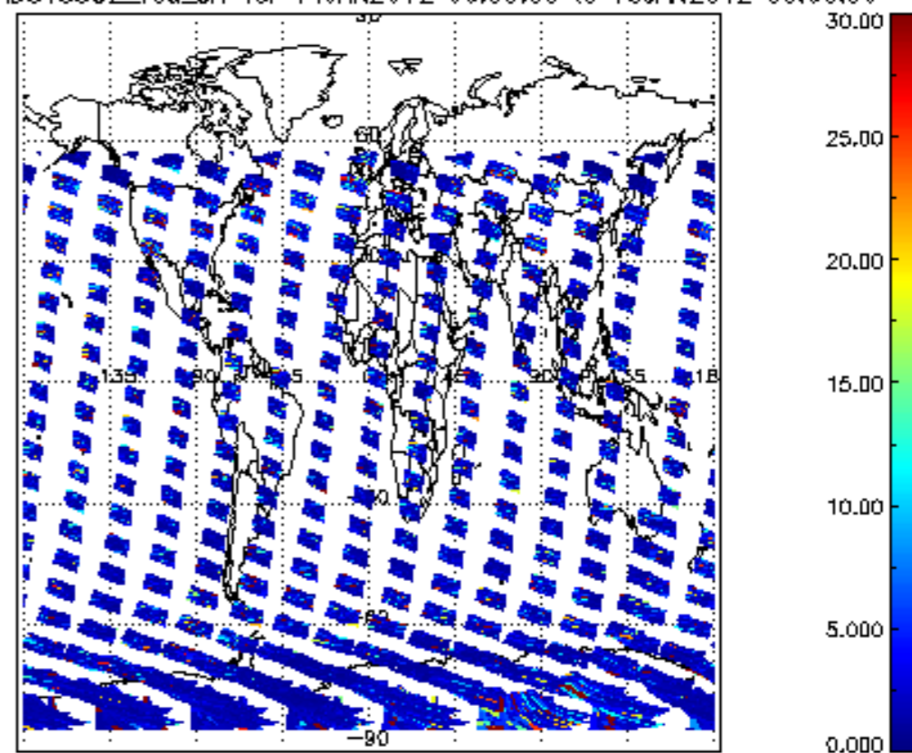
SCIOL2P_NADUV5S02_vcd_err for 14JAN2012 00:00:00 to 15JAN2012 00:00:00
