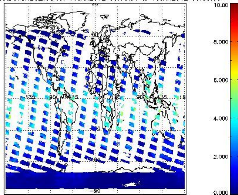
SCIOL2P_NADUV8H20_vcd for 14JAN2012 00:00:00 to 15JAN2012 00:00:00
