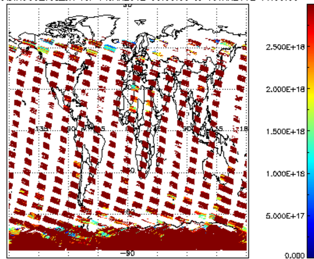
SCIOL2P_NADIR3CO_vcd_err for 14JAN2012 00:00:00 to 15JAN2012 00:00:00
