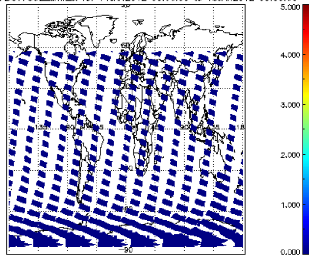
SCIOL2P_NADUV7S02_amf_cl for 14JAN2012 00:00:00 to 15JAN2012 00:00:00
