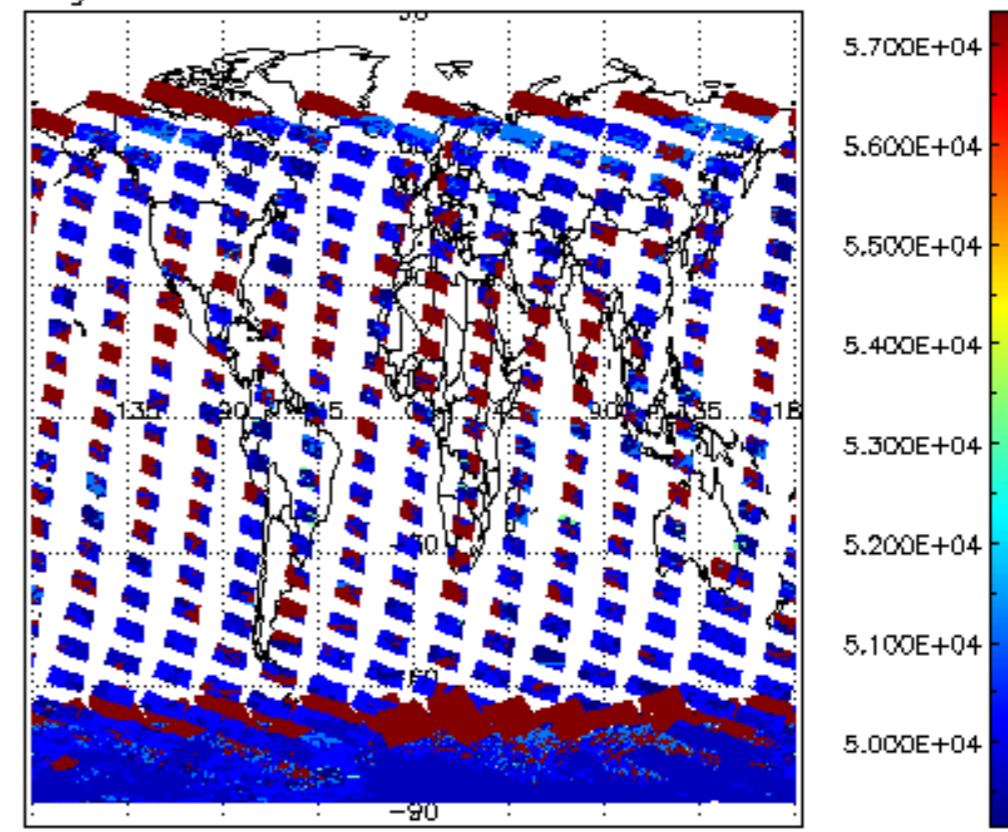
cloud_flags for 14JAN2012 00:00:00 to 15JAN2012 00:00:00
