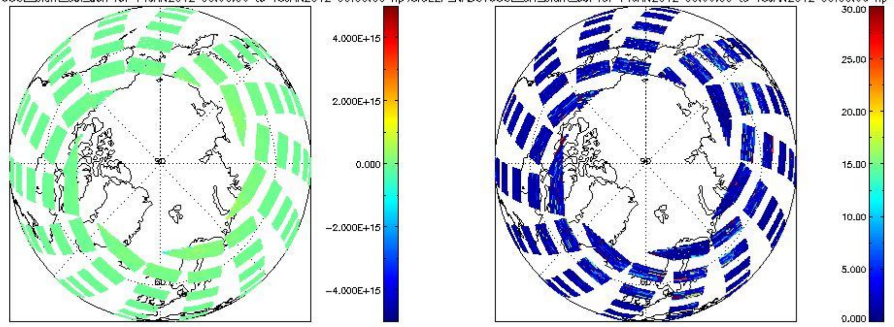
SCIOI2P_NADUV60CL_slant_col_den for 14JAN2012 00:00:00 to 15JAN2012 00:00:00 np; SCIOI2P_NADUV60CL_err_slant_col for 14JAN2012 00:00:00 to 15JAN2012 00:00:00 np
