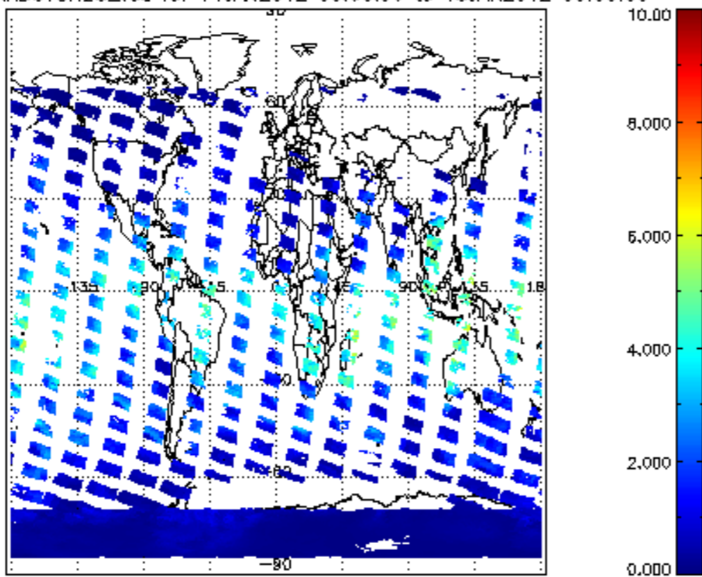
SCIOL2P_NADUV8H20_vcd for 14JAN2012 00:00:00 to 15JAN2012 00:00:00
