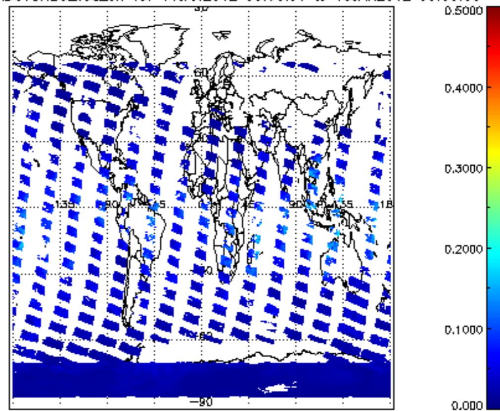
SCIOL2P_NADUV8H20_vcd_err for 14JAN2012 00:00:00 to 15JAN2012 00:00:00
