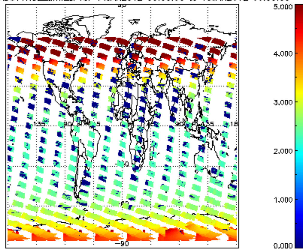
SCIOL2P_NADUV1NO2_amf_cl for 14JAN2012 00:00:00 to 15JAN2012 00:00:00
