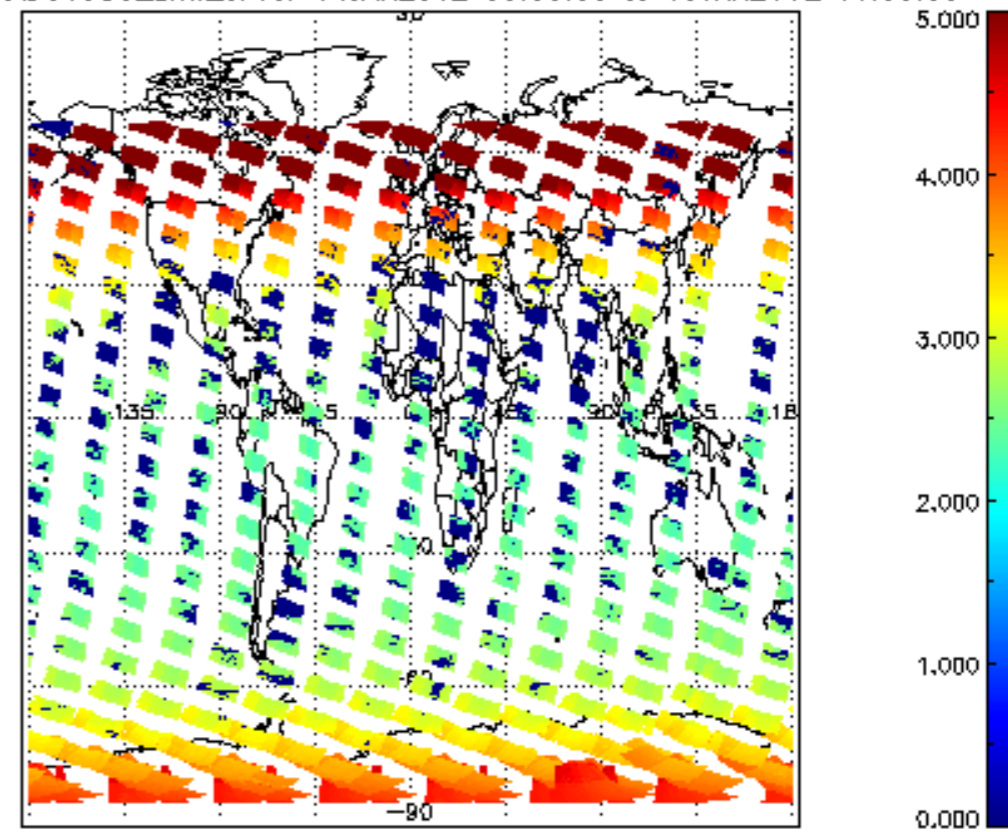
SCIOL2P_NADUV003_amf_cl for 14JAN2012 00:00:00 to 15JAN2012 00:00:00
