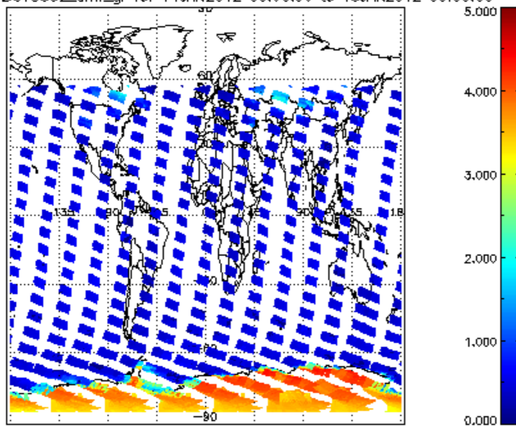
SCIOL2P_NADUV5S02_amf_gr for 14JAN2012 00:00:00 to 15JAN2012 00:00:00
