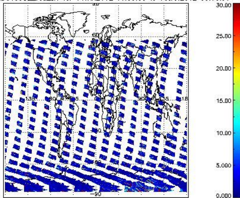
SCIOL2P_NADUV5SO2_vcd_err for 14JAN2012 00:00:00 to 15JAN2012 00:00:00
