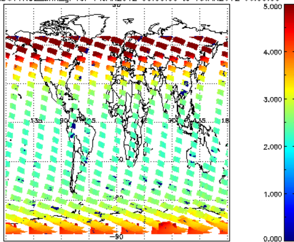
SCIOL2P_NADUV1NO2_amf_gr for 14JAN2012 00:00:00 to 15JAN2012 00:00:00
