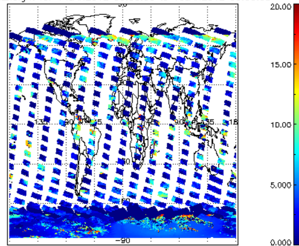
cL_top_height for 14JAN2012 00:00:00 to 15JAN2012 00:00:00
