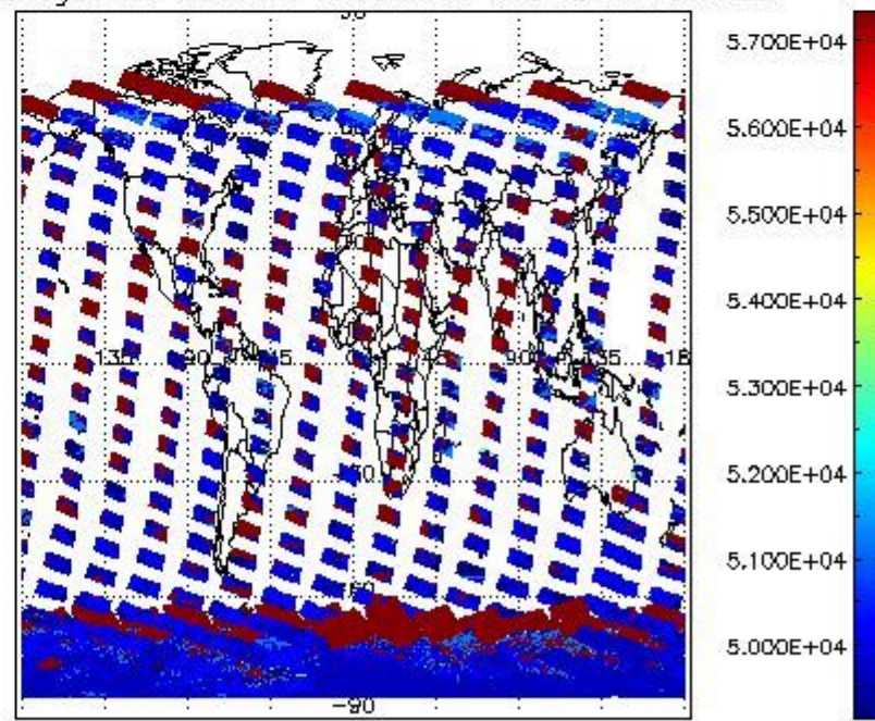
cloud_flags for 14JAN2012 00:00:00 to 15JAN2012 00:00:00
