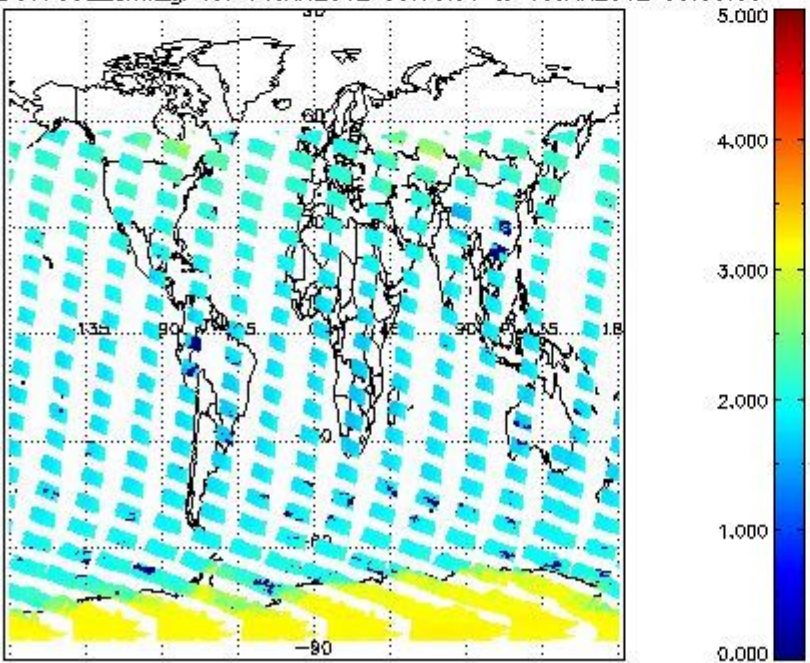
SCIOL2P_NADUV7S02_amf_gr for 14JAN2012 00:00:00 to 15JAN2012 00:00:00
