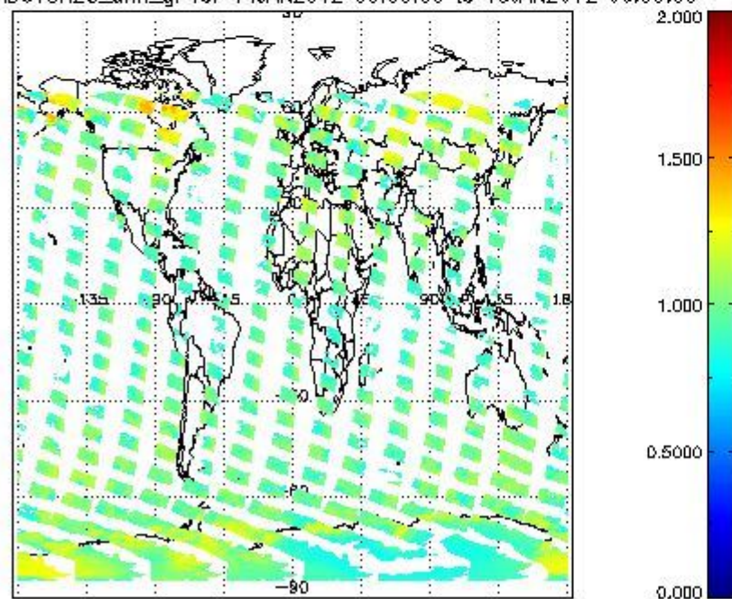
SCIOL2P_NADUV8H20_amf_gr for 14JAN2012 00:00:00 to 15JAN2012 00:00:00
