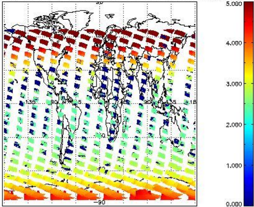
SCIOL2P_NADUV3BRO_amf_cl for 14JAN2012 00:00:00 to 15JAN2012 00:00:00
