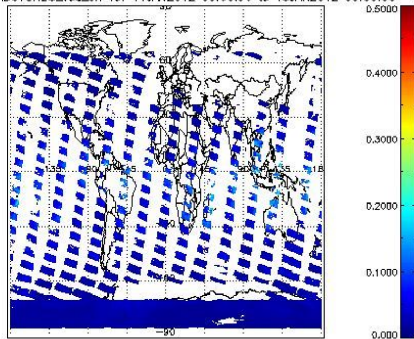
SCIOL2P_NADUV8H20_vcd_err for 14JAN2012 00:00:00 to 15JAN2012 00:00:00
