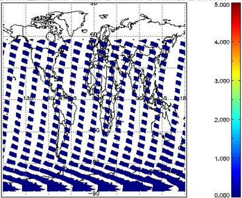
SCIOL2P_NADUV7S02_amf_cl for 14JAN2012 00:00:00 to 15JAN2012 00:00:00
