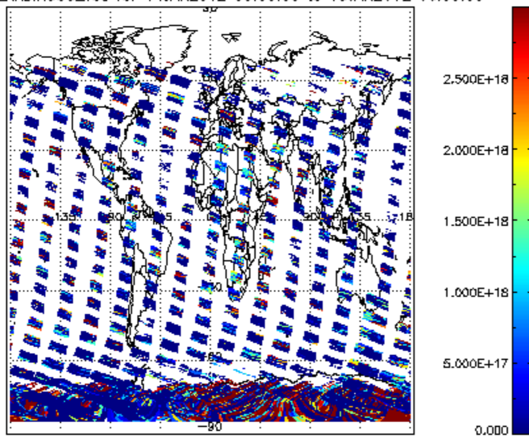
SCIOL2P_NADIR3CO_vcd for 14JAN2012 00:00:00 to 15JAN2012 00:00:00
