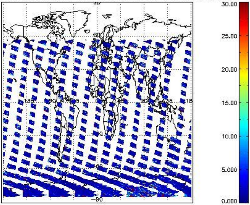
SCIOL2P_NADUV7S02_vcd_err for 14JAN2012 00:00:00 to 15JAN2012 00:00:00
