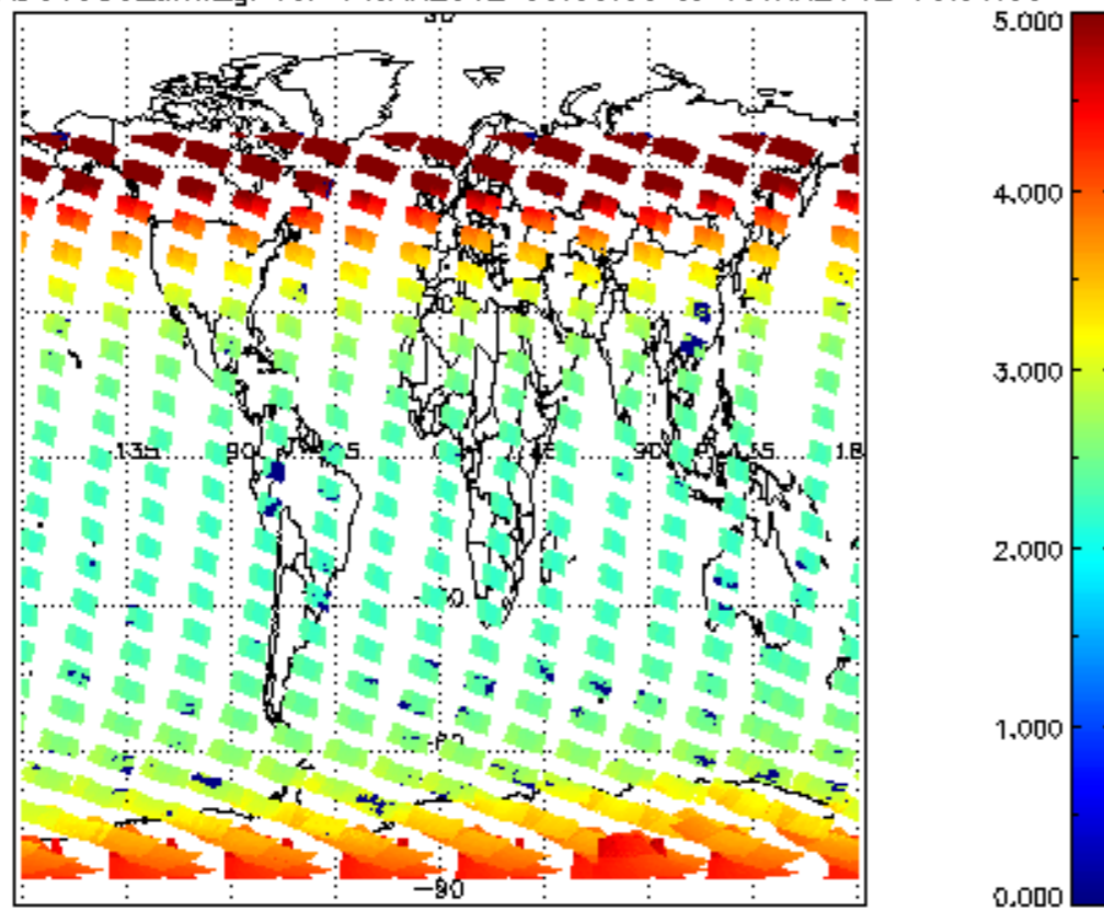
SCIOL2P_NADUV003_amf_gr for 14JAN2012 00:00:00 to 15JAN2012 00:00:00
