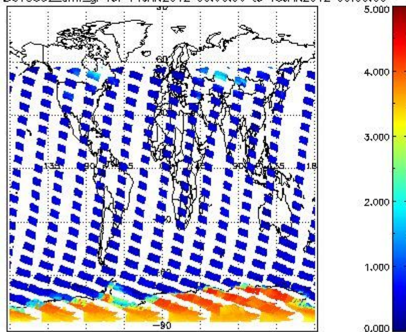
SCIOL2P_NADUV5SO2_amf_gr for 14JAN2012 00:00:00 to 15JAN2012 00:00:00
