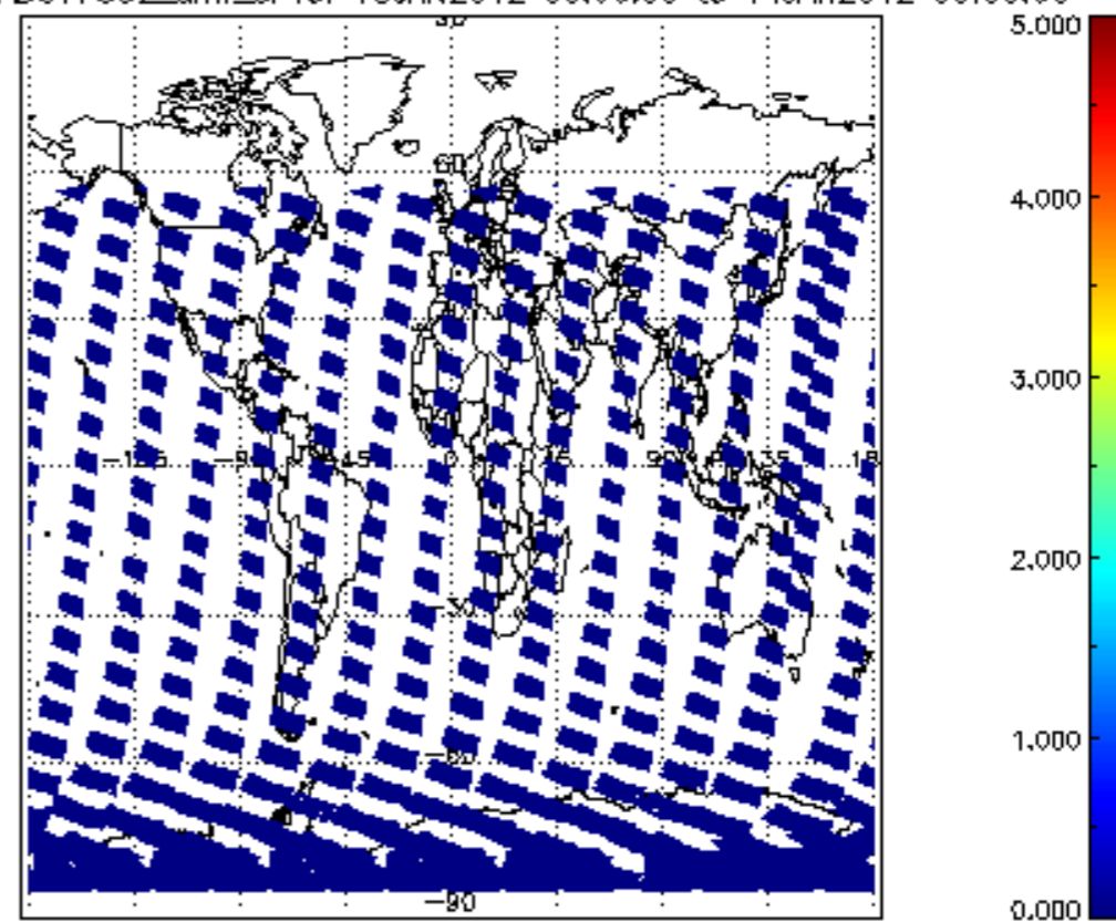
SCIOL2P_NADUV7S02_amf_sl for 13JAN2012 00:00:00 to 14JAN2012 00:00:00
