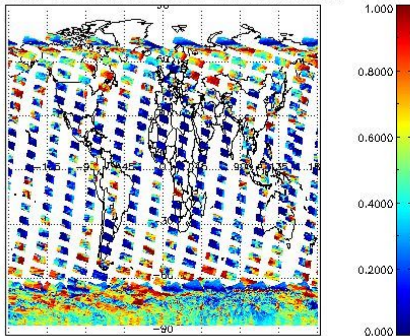
cL_frac for 13JAN2012 00:00:00 to 14JAN2012 00:00:00
