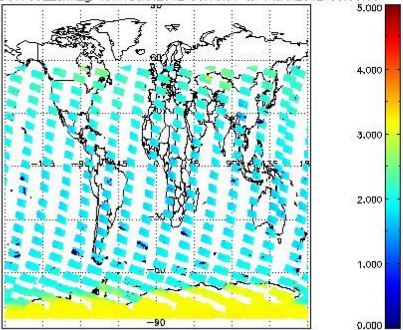
SCIOL2P_NADUV7S02_amf_gr for 13JAN2012 00:00:00 to 14JAN2012 00:00:00
