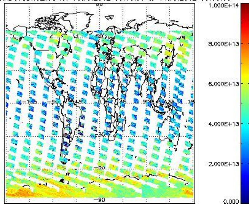
SCIOL2P_NADUV3BRO_vcd for 13JAN2012 00:00:00 to 14JAN2012 00:00:00
