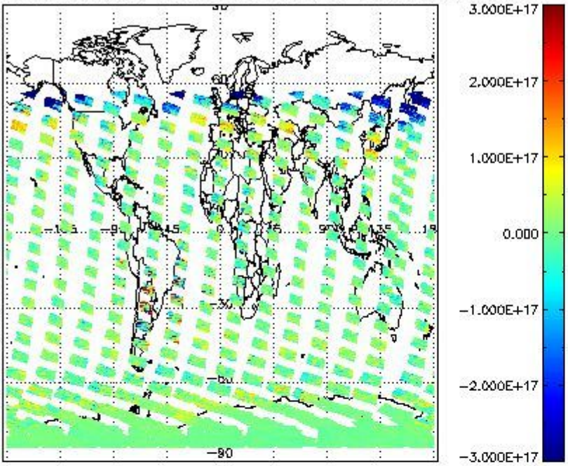
SCIOL2P_NADUV5S02_vcd for 13JAN2012 00:00:00 to 14JAN2012 00:00:00
