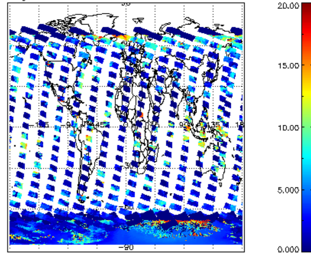
cL_top_height for 13JAN2012 00:00:00 to 14JAN2012 00:00:00
