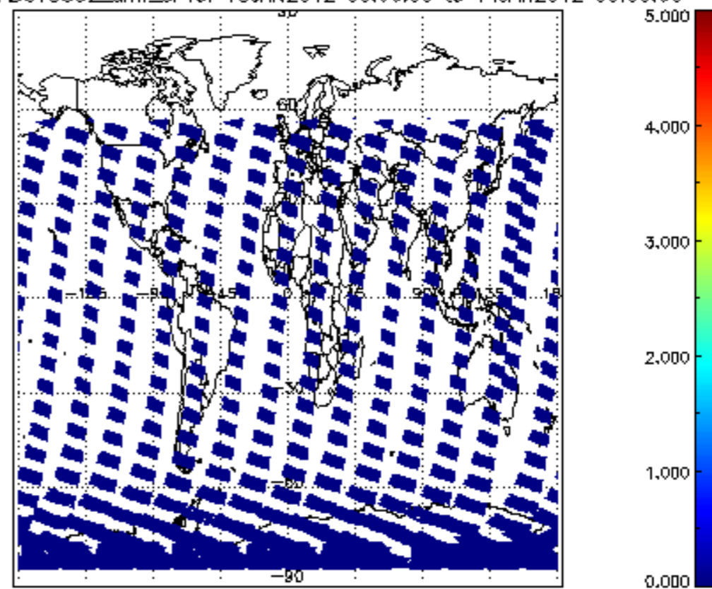
SCIOL2P_NADUV5S02_amf_cl for 13JAN2012 00:00:00 to 14JAN2012 00:00:00
