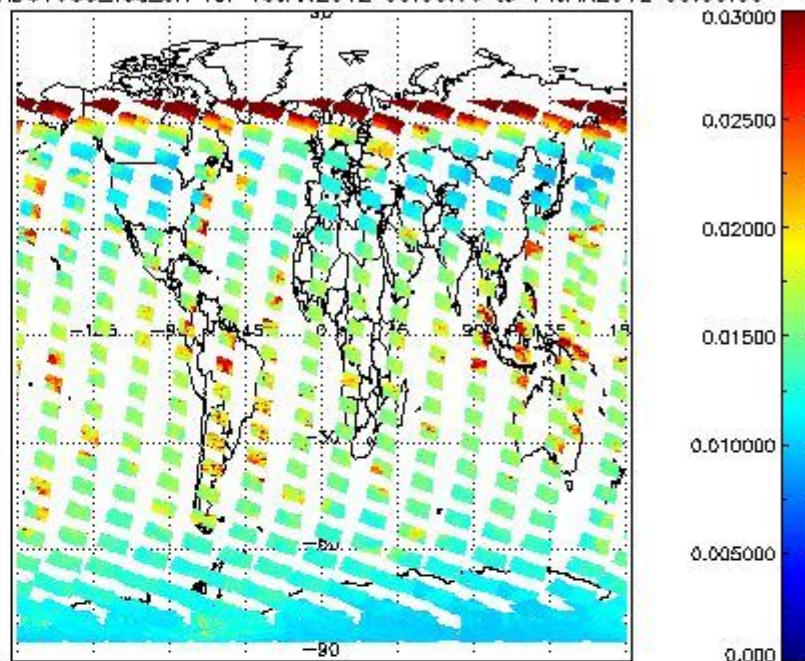
SCIOL2P_NADUV003_vcd_err for 13JAN2012 00:00:00 to 14JAN2012 00:00:00
