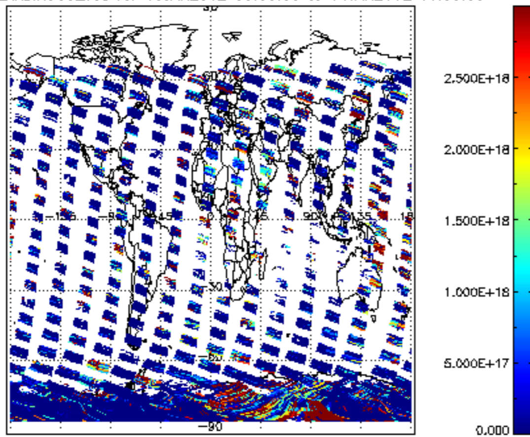
SCIOL2P_NADIR3CO_vcd for 13JAN2012 00:00:00 to 14JAN2012 00:00:00
