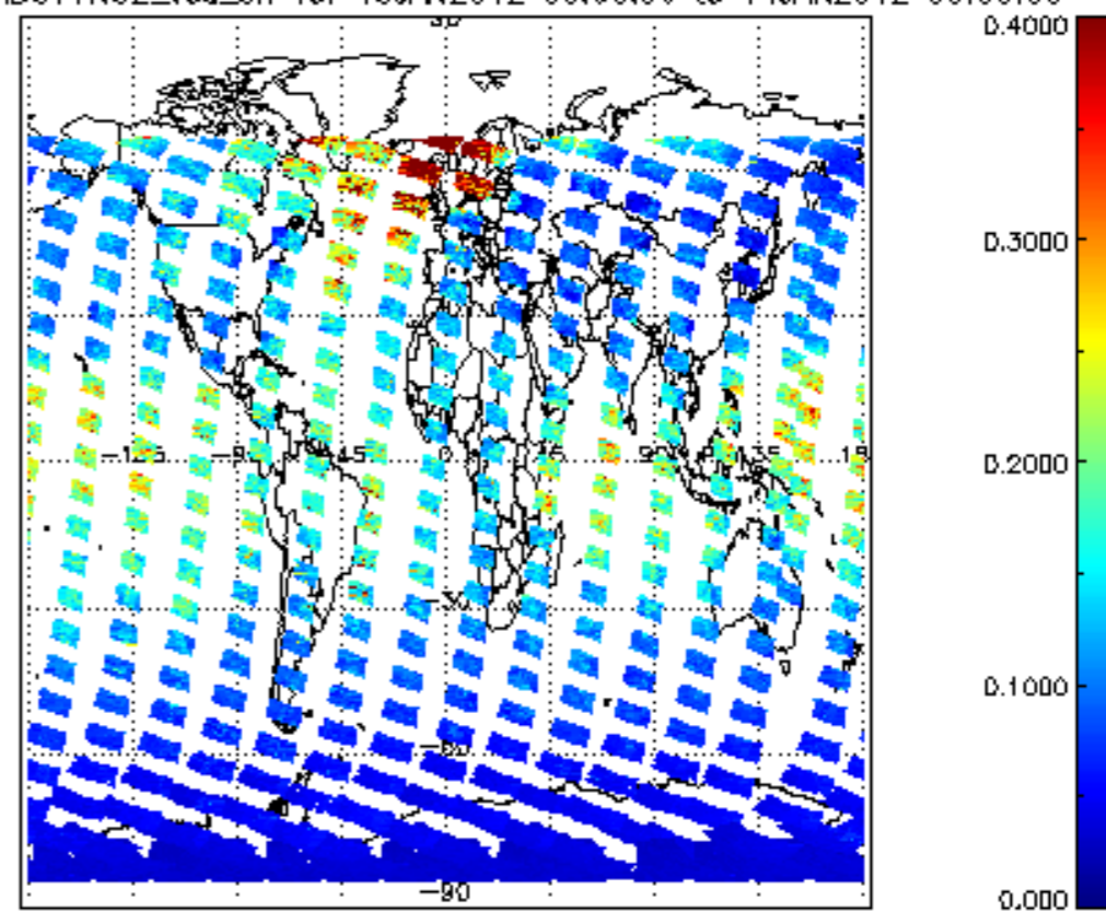
SCIOL2P_NADUV1NO2_vcd_err for 13JAN2012 00:00:00 to 14JAN2012 00:00:00
