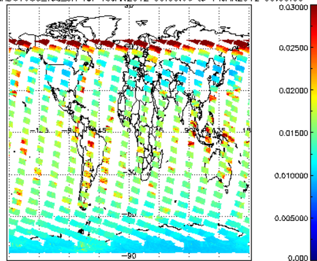
SCIOL2P_NADUV003_vcd_err for 13JAN2012 00:00:00 to 14JAN2012 00:00:00
