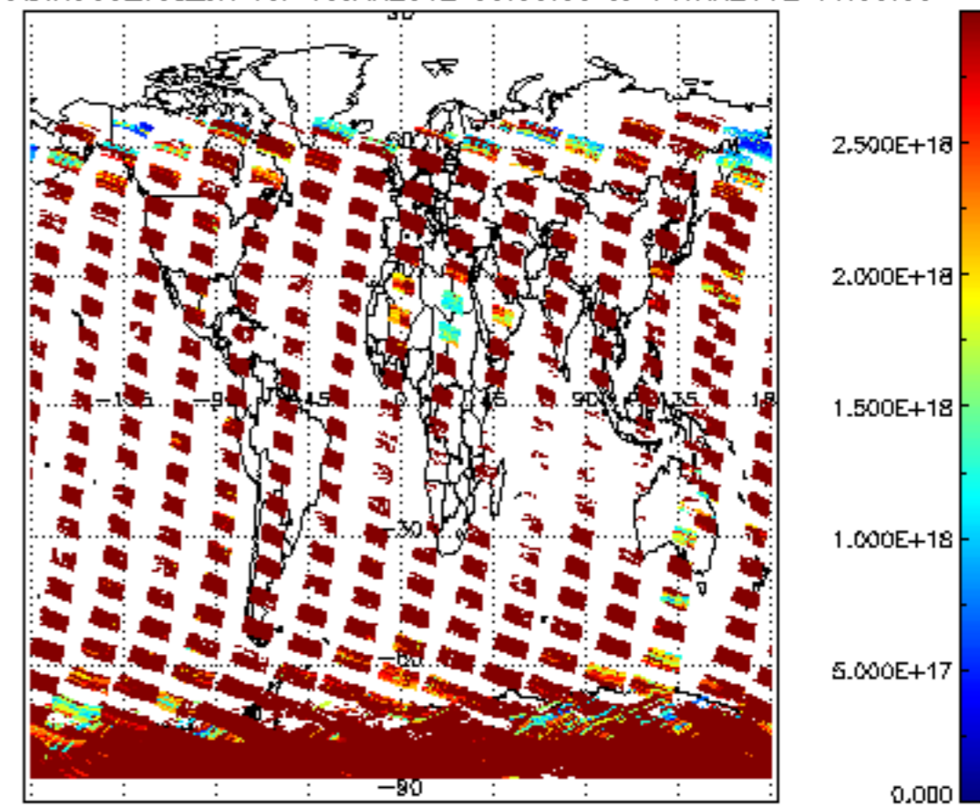
SCIOL2P_NADIR3CO_vcd_err for 13JAN2012 00:00:00 to 14JAN2012 00:00:00
