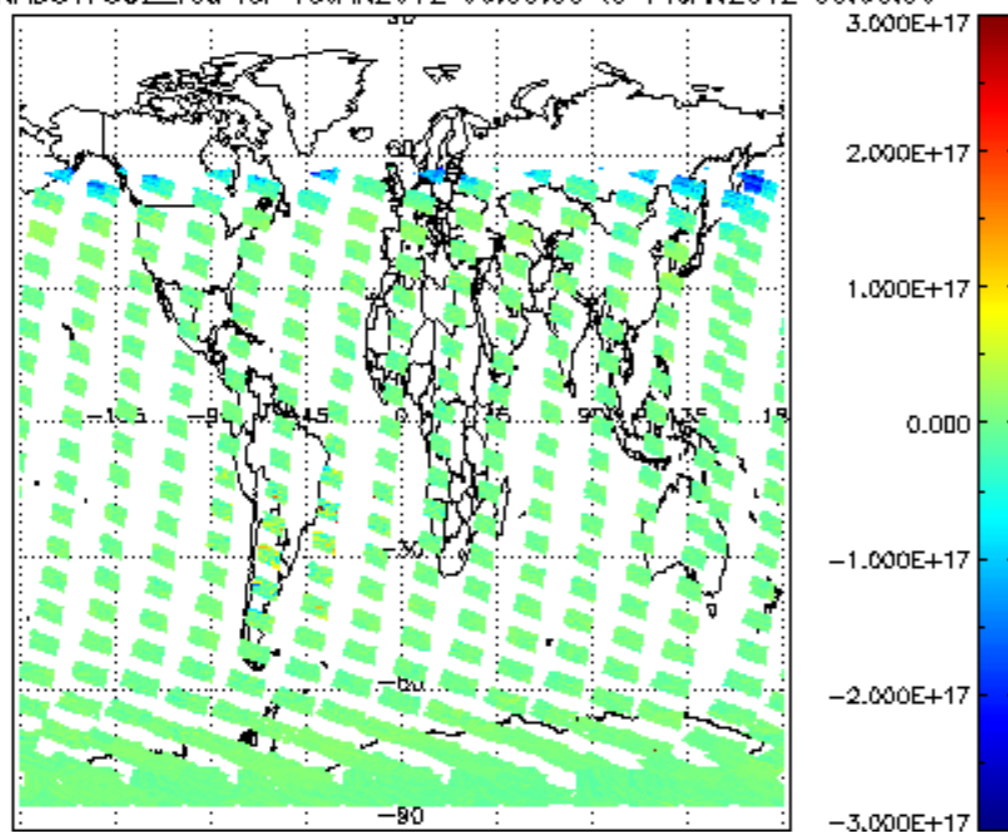
SCIOL2P_NADUV7S02_vcd for 13JAN2012 00:00:00 to 14JAN2012 00:00:00
