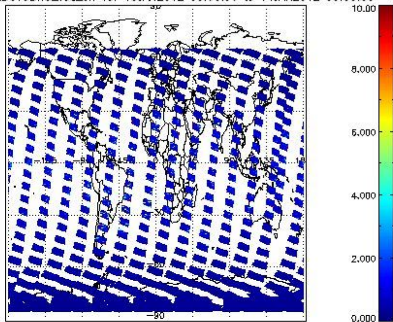
SCIOL2P_NADUV3BRO_vcd_err for 13JAN2012 00:00:00 to 14JAN2012 00:00:00
