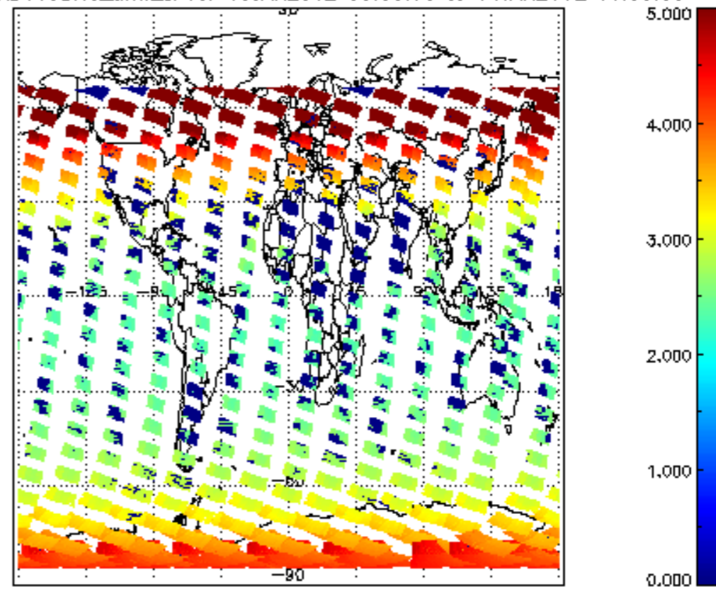
SCIOL2P_NADUV3BRO_amf_cl for 13JAN2012 00:00:00 to 14JAN2012 00:00:00
