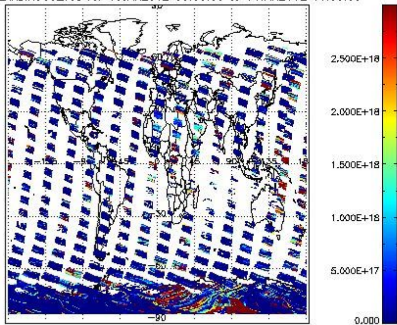
SCIDL2P_NADIR3CO_vcd for 13JAN2012 00:00:00 to 14JAN2012 00:00:00
