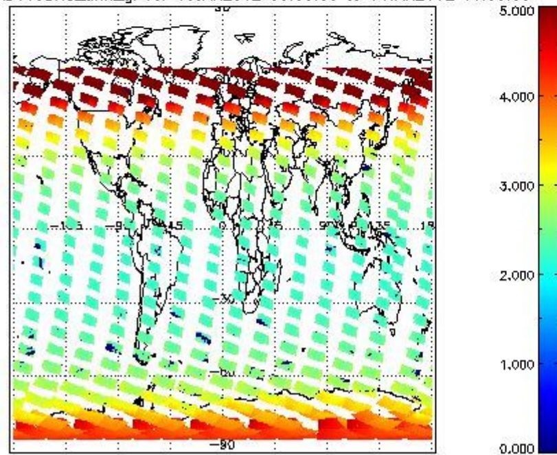
SCIOL2P_NADUV3BRO_amf_gr for 13JAN2012 00:00:00 to 14JAN2012 00:00:00
