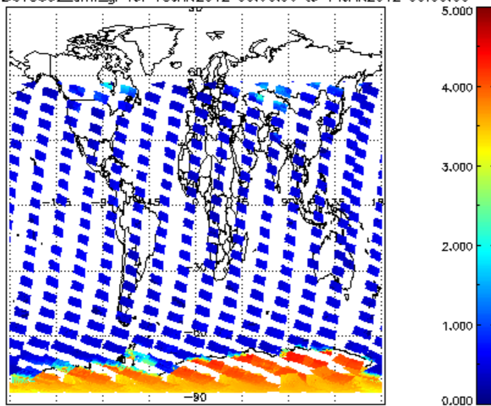
SCIOL2P_NADUV5S02_amf_gr for 13JAN2012 00:00:00 to 14JAN2012 00:00:00
