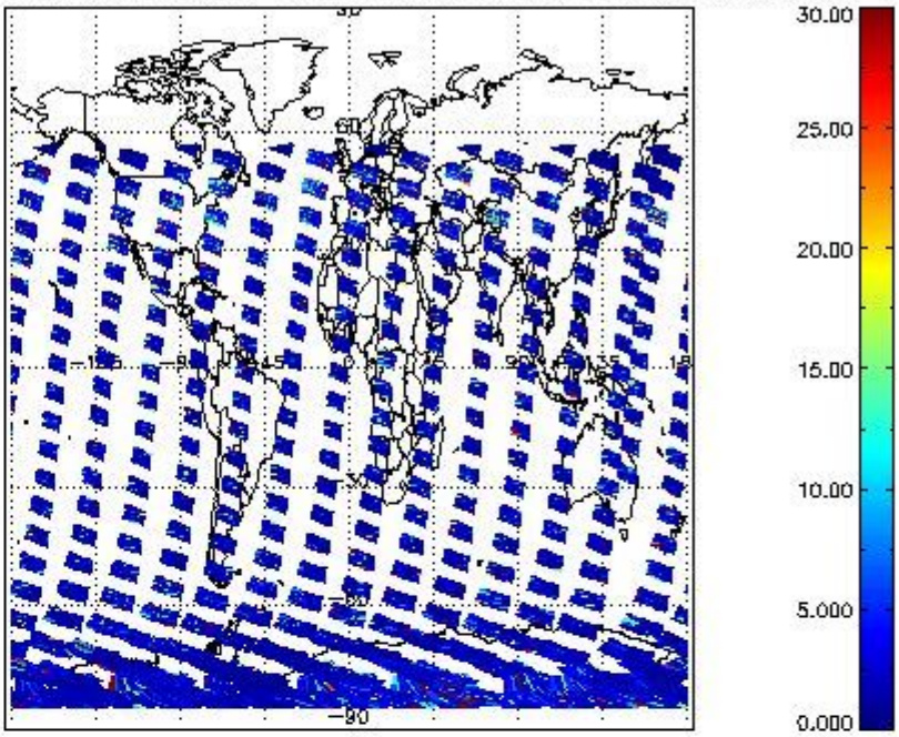
SCIOL2P_NADUV7S02_vcd_err for 13JAN2012 00:00:00 to 14JAN2012 00:00:00
