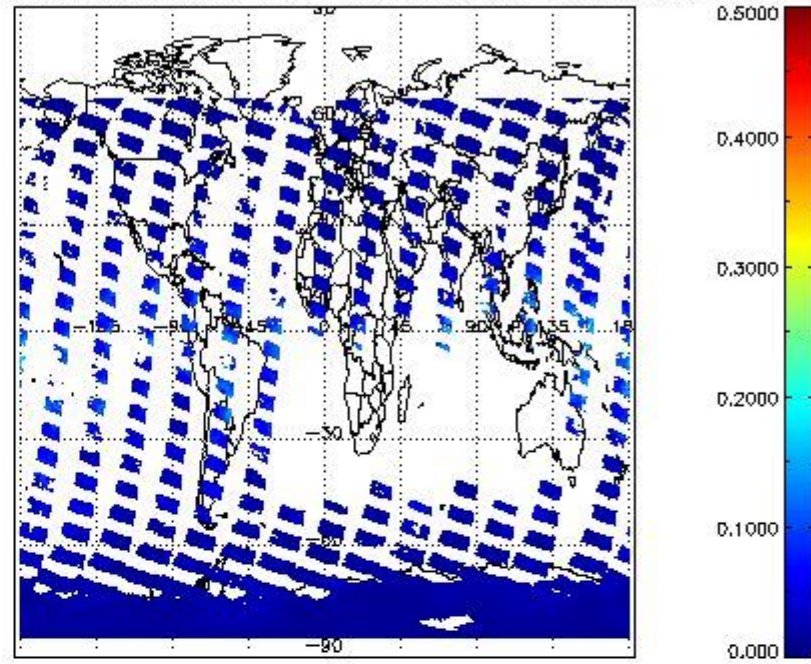
SCIOL2P_NADUV8H20_vcd_err for 13JAN2012 00:00:00 to 14JAN2012 00:00:00
