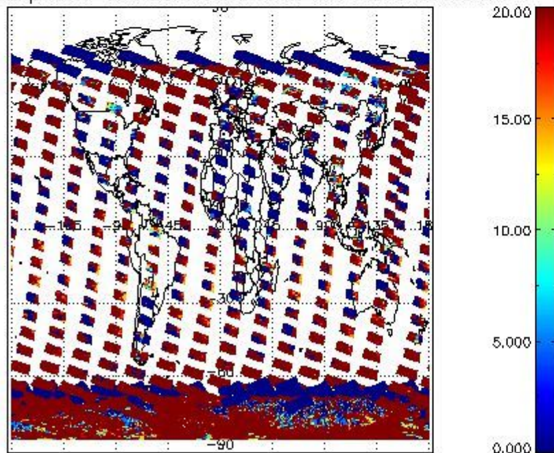
cLopt_depth for 13JAN2012 00:00:00 to 14JAN2012 00:00:00
