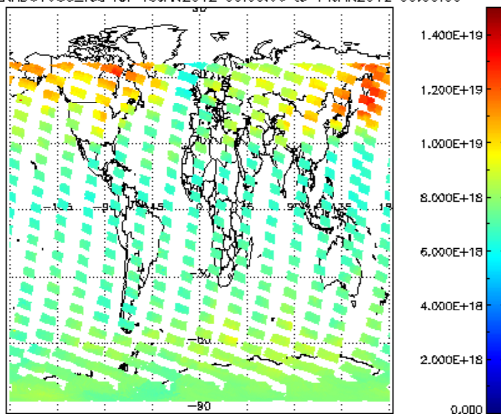
SCIOL2P_NADUV003_vcd for 13JAN2012 00:00:00 to 14JAN2012 00:00:00
