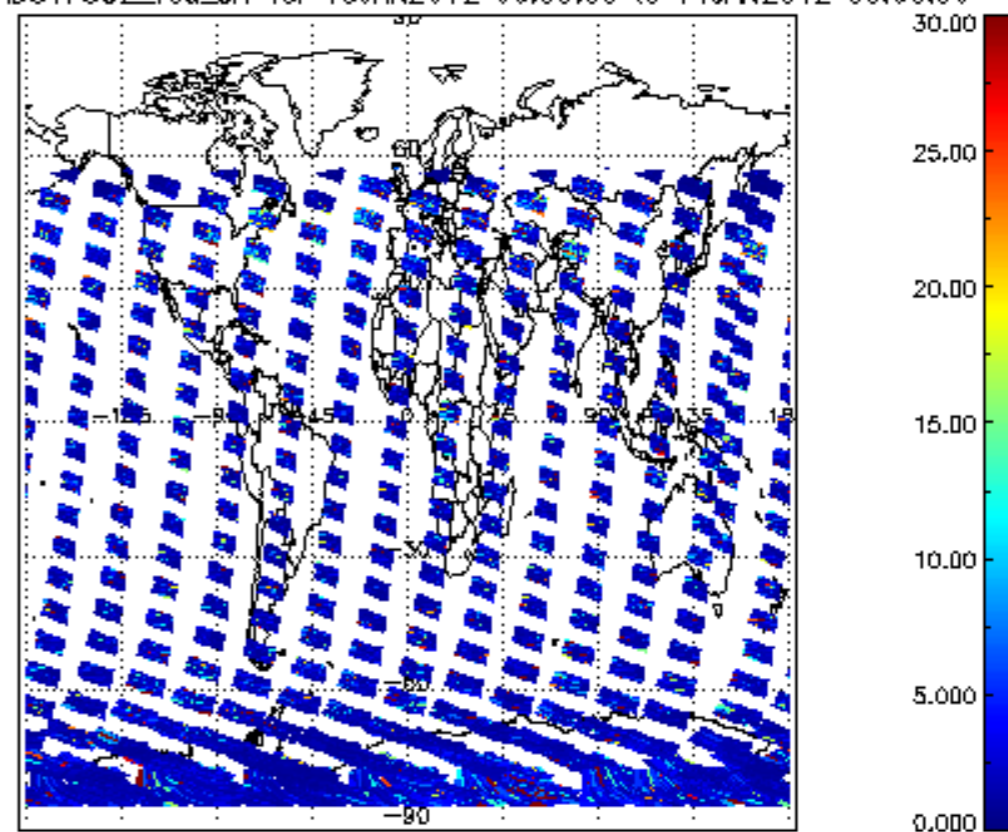
SCIOL2P_NADUV7S02_vcd_err for 13JAN2012 00:00:00 to 14JAN2012 00:00:00
