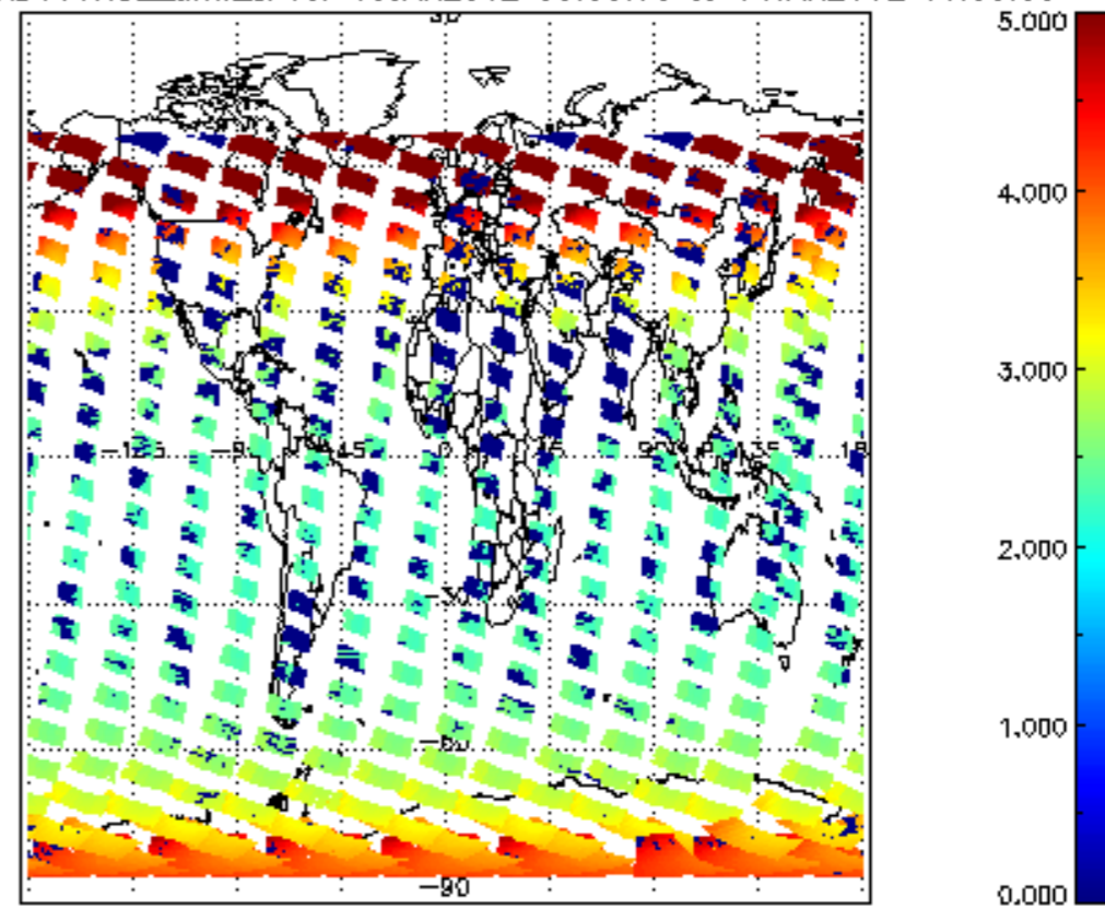
SCIOL2P_NADUV1NO2_amf_cl for 13JAN2012 00:00:00 to 14JAN2012 00:00:00
