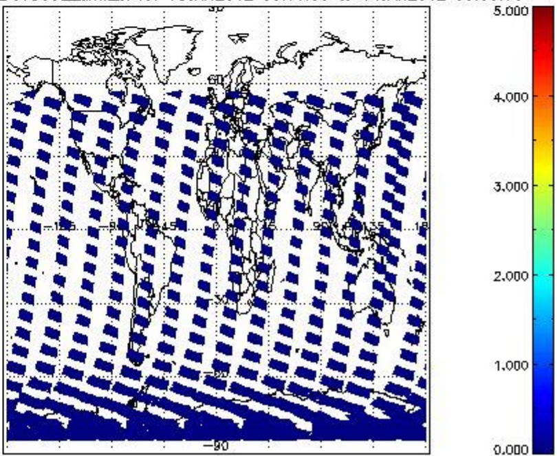
SCIOL2P_NADUV5S02_amf_cl for 13JAN2012 00:00:00 to 14JAN2012 00:00:00
