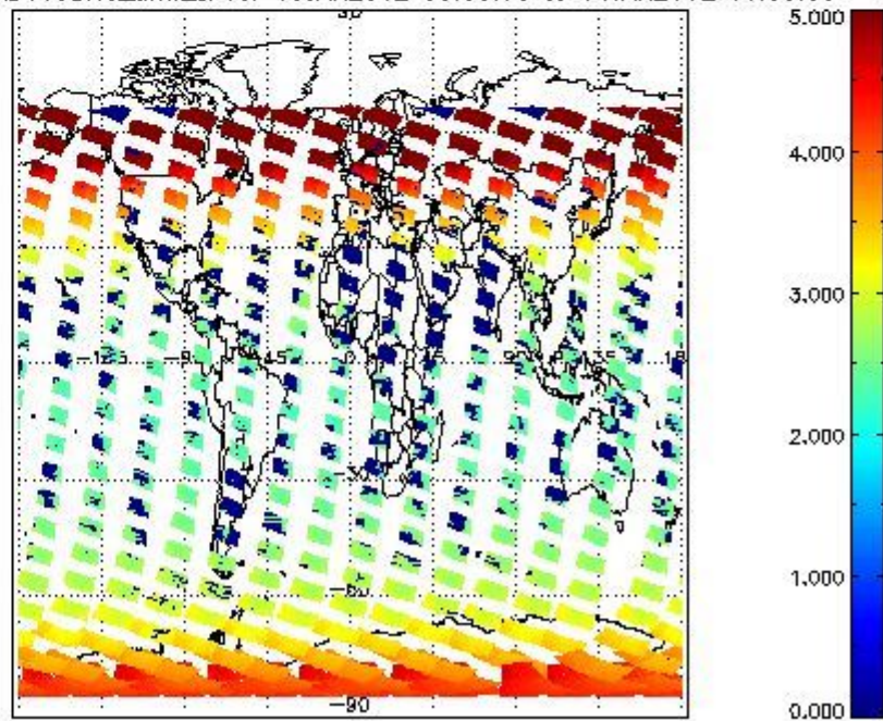
SCIOL2P_NADUV3BRO_amf_cl for 13JAN2012 00:00:00 to 14JAN2012 00:00:00
