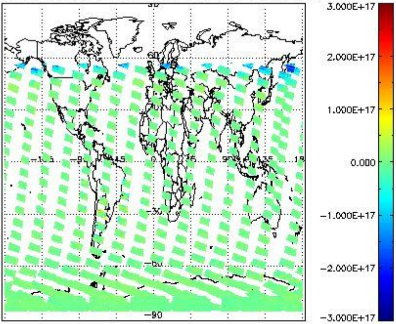
SCIOL2P_NADUV7S02_vcd for 13JAN2012 00:00:00 to 14JAN2012 00:00:00
