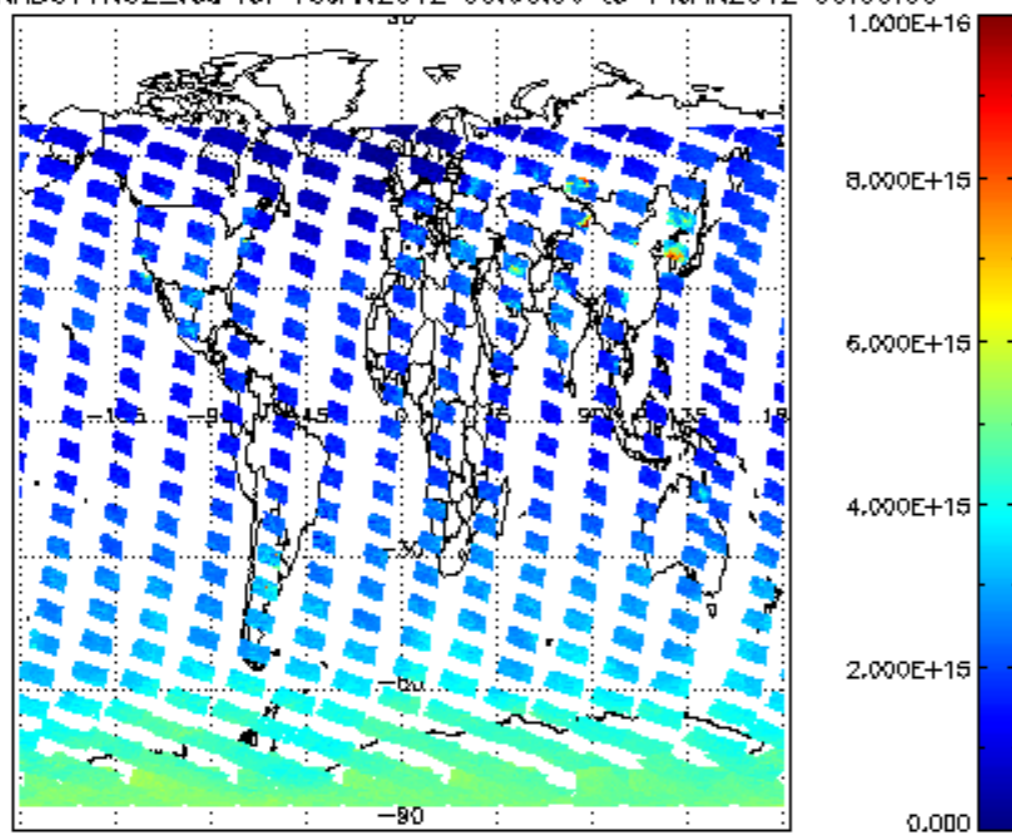
SCIOL2P_NADUV1NO2_vcd for 13JAN2012 00:00:00 to 14JAN2012 00:00:00
