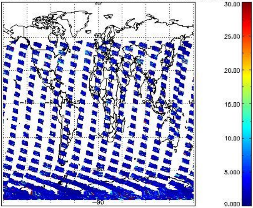
SCIOL2P_NADUV5S02_vcd_err for 13JAN2012 00:00:00 to 14JAN2012 00:00:00
