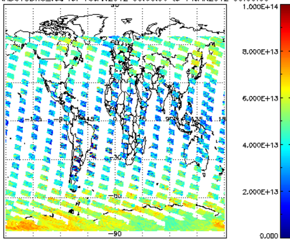
SCIOL2P_NADUV3BRO_vcd for 13JAN2012 00:00:00 to 14JAN2012 00:00:00
