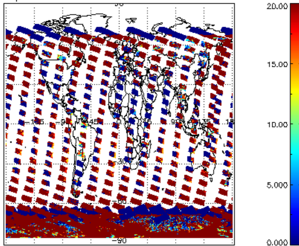
cL_opt_depth for 13JAN2012 00:00:00 to 14JAN2012 00:00:00
