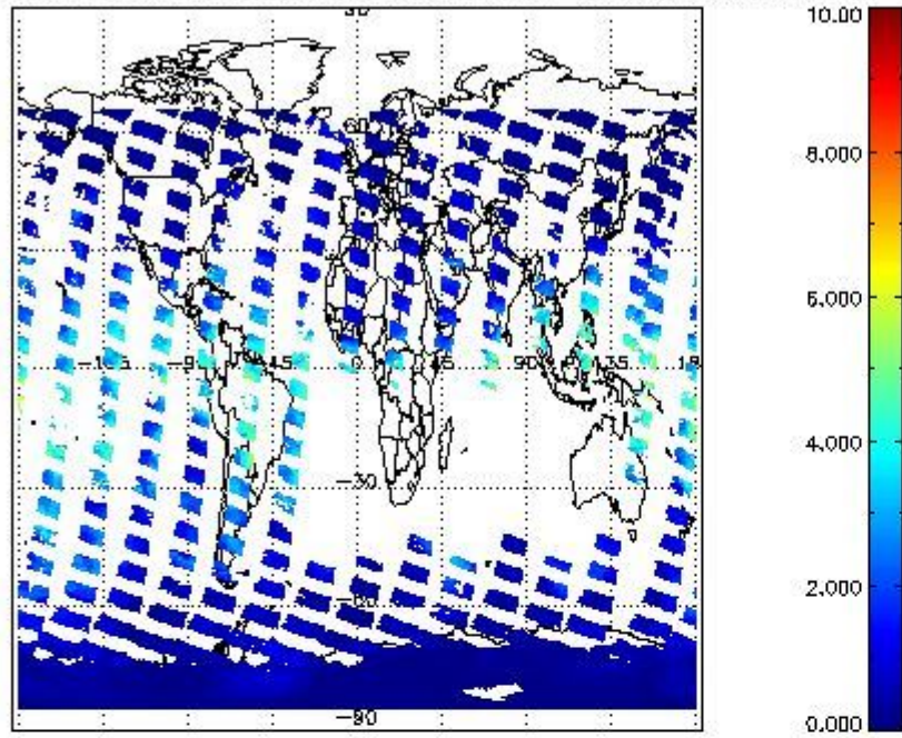
SCIOL2P_NADUV8H20_vcd for 13JAN2012 00:00:00 to 14JAN2012 00:00:00
