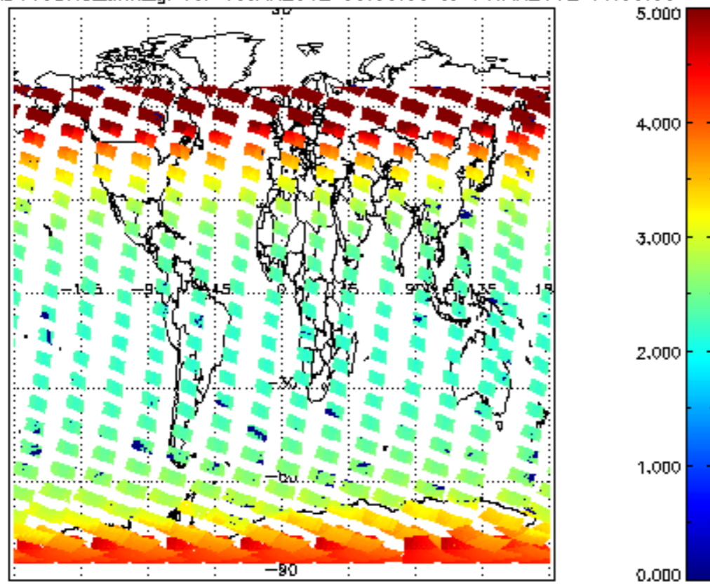
SCIOL2P_NADUV3BRO_amf_gr for 13JAN2012 00:00:00 to 14JAN2012 00:00:00
