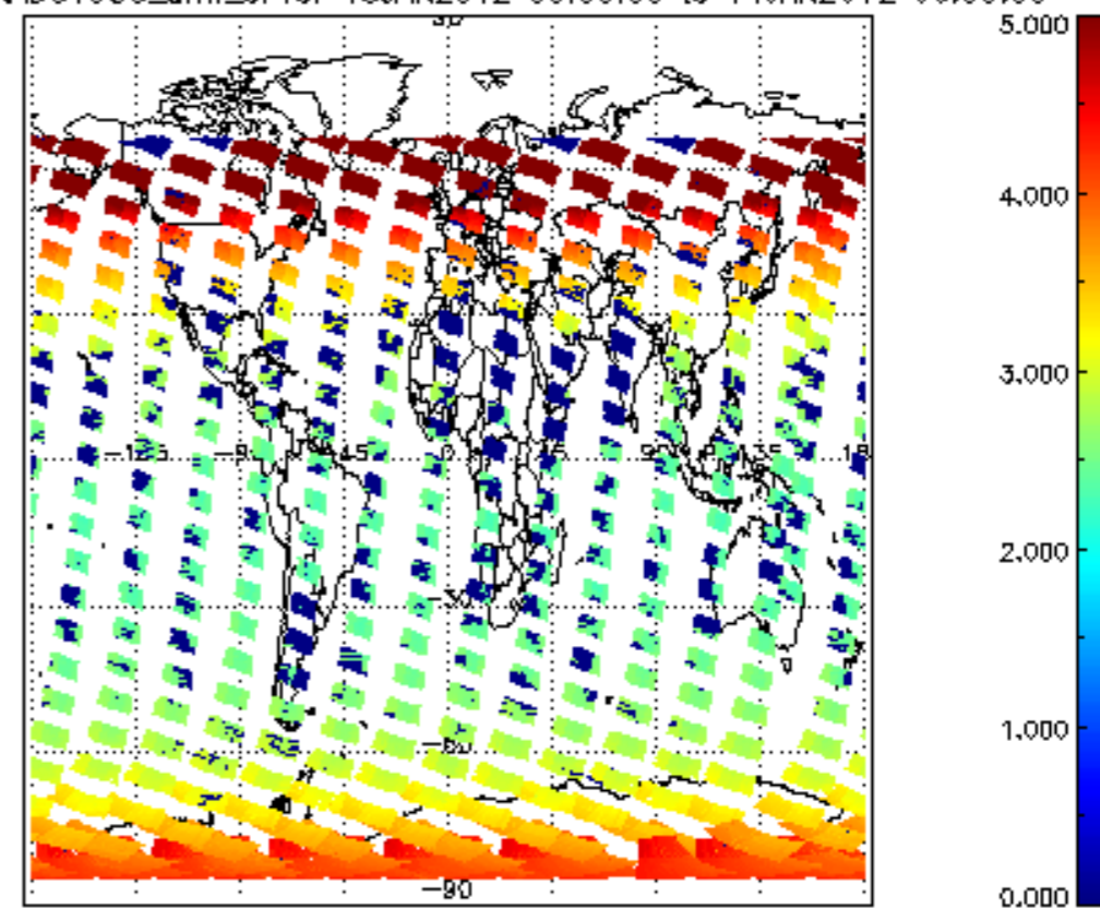
SCIOL2P_NADUV003_amf_cl for 13JAN2012 00:00:00 to 14JAN2012 00:00:00
