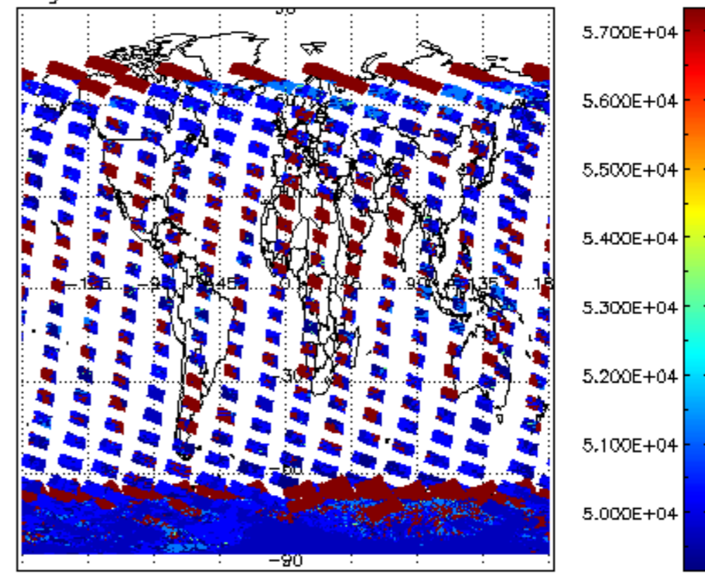
cloud_flags for 13JAN2012 00:00:00 to 14JAN2012 00:00:00
