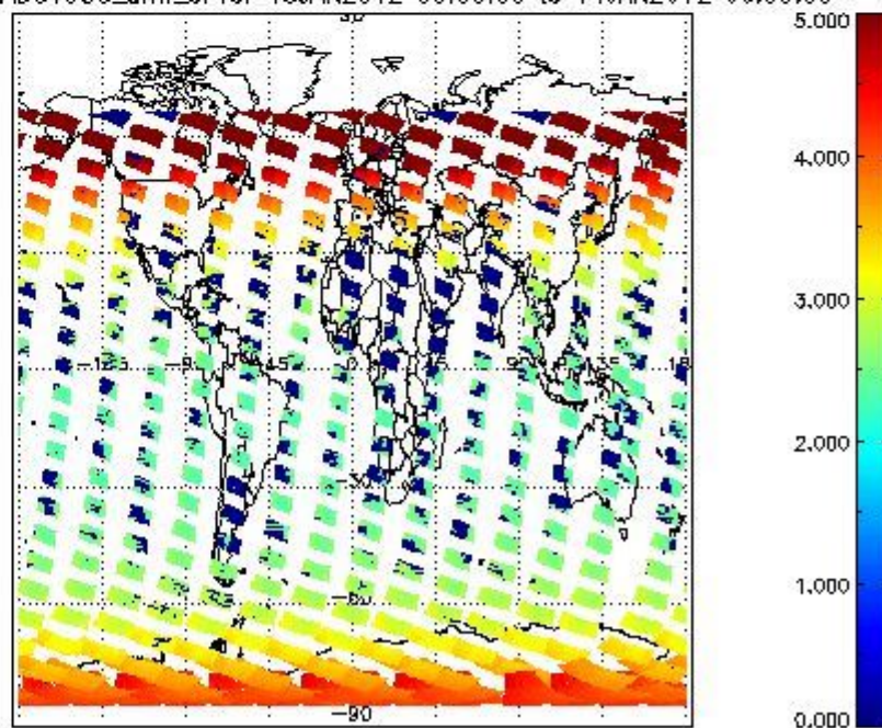
SCIOL2P_NADUV003_amf_cl for 13JAN2012 00:00:00 to 14JAN2012 00:00:00
