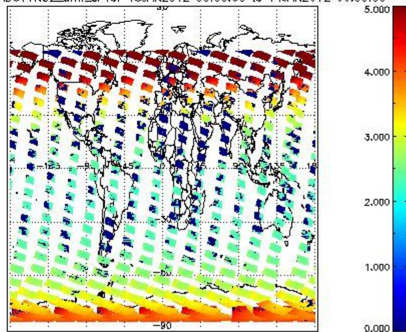
SCIOL2P_NADUV1NO2_amf_cl for 13JAN2012 00:00:00 to 14JAN2012 00:00:00
