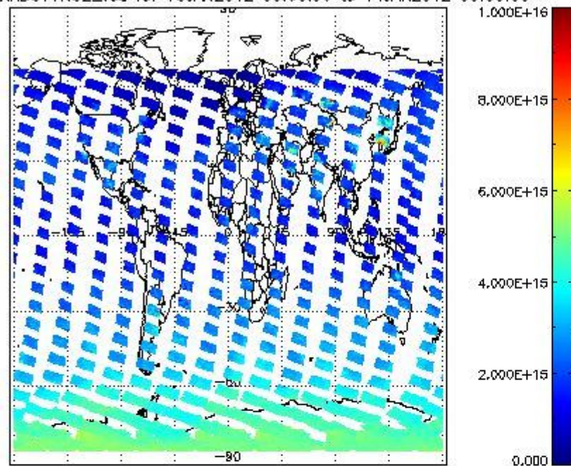
SCIOL2P_NADUV1NO2_vcd for 13JAN2012 00:00:00 to 14JAN2012 00:00:00
