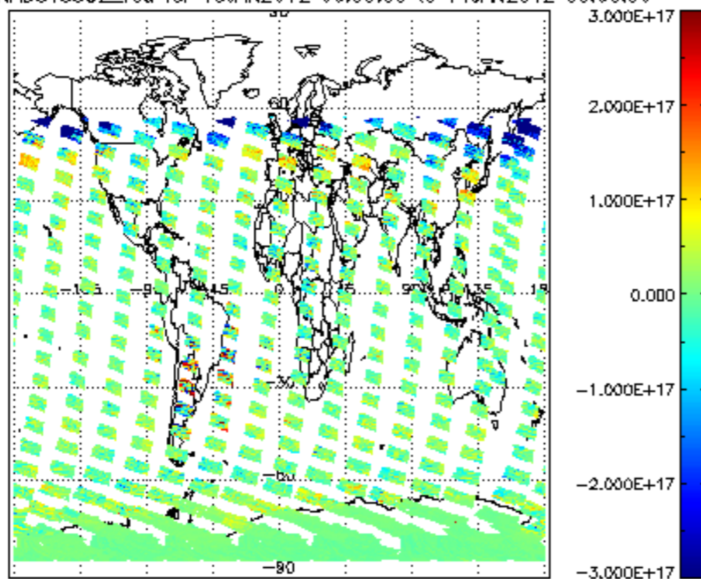
SCIOL2P_NADUV5S02_vcd for 13JAN2012 00:00:00 to 14JAN2012 00:00:00
