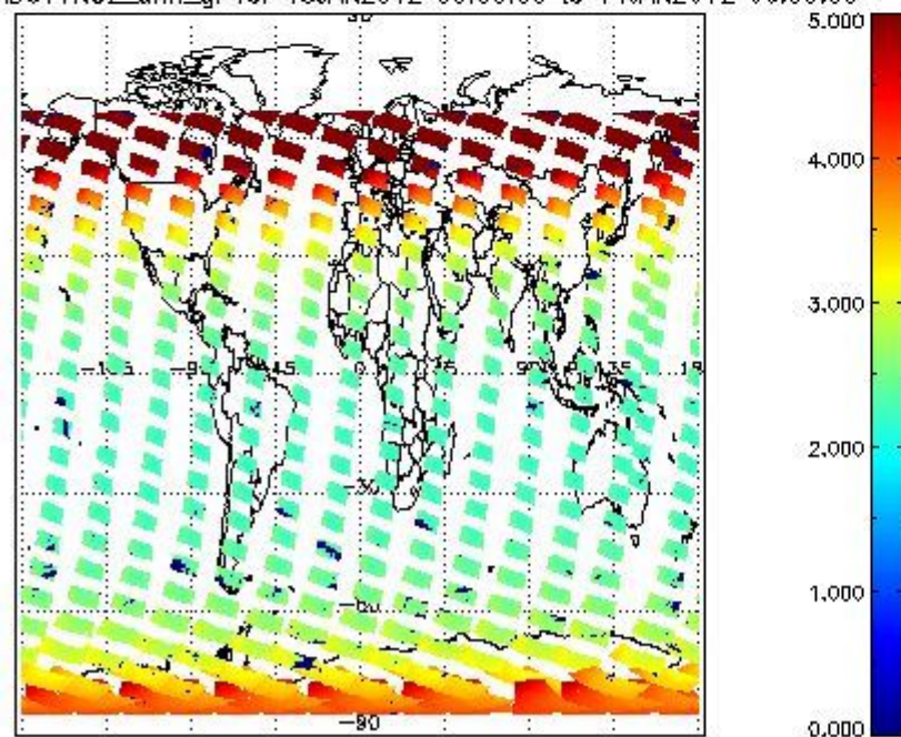
SCIOL2P_NADUV1NO2_amf_gr for 13JAN2012 00:00:00 to 14JAN2012 00:00:00
