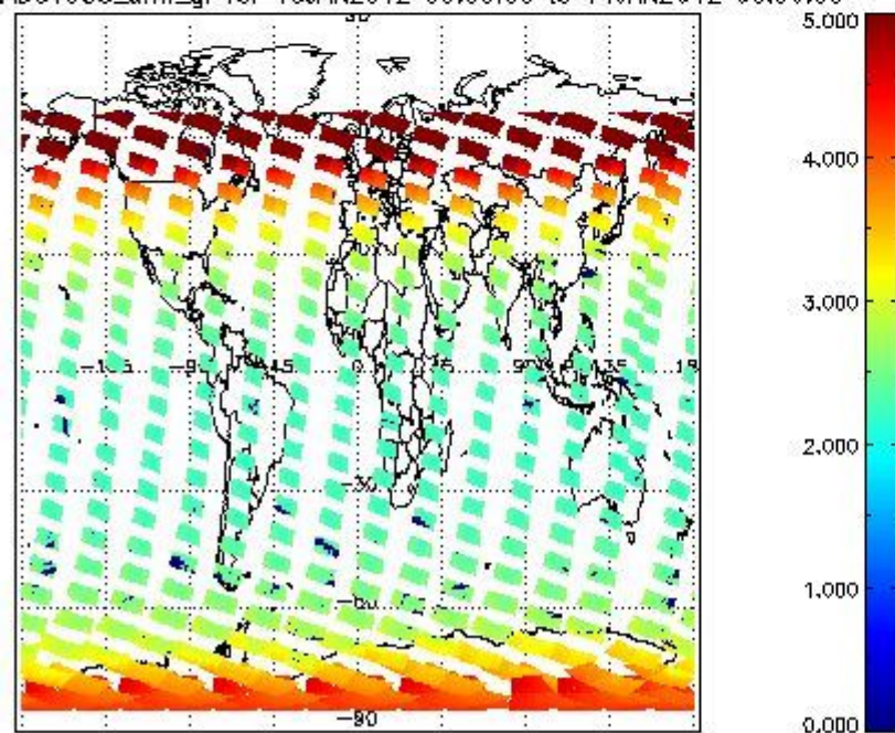
SCIOL2P_NADUV003_amf_gr for 13JAN2012 00:00:00 to 14JAN2012 00:00:00
