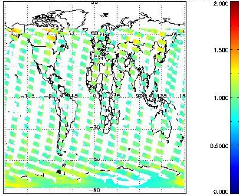
SCIOL2P_NADUV8H20_amf_gr for 13JAN2012 00:00:00 to 14JAN2012 00:00:00
