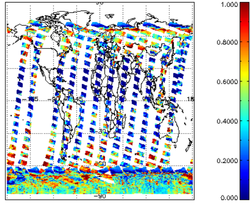
cL_frac for 10JAN2012 00:00:00 to 11JAN2012 00:00:00
