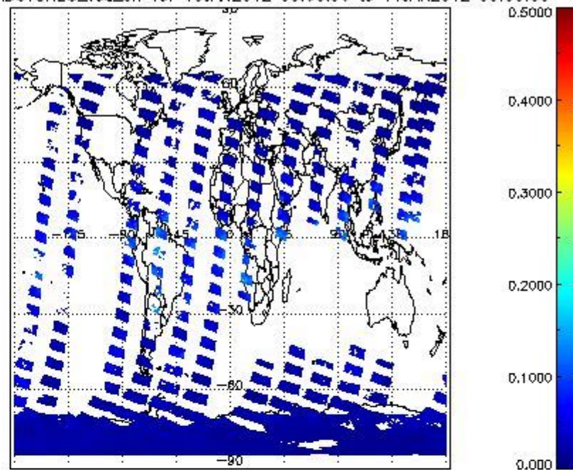
SCIOL2P_NADUV8H20_vcd_err for 10JAN2012 00:00:00 to 11JAN2012 00:00:00
