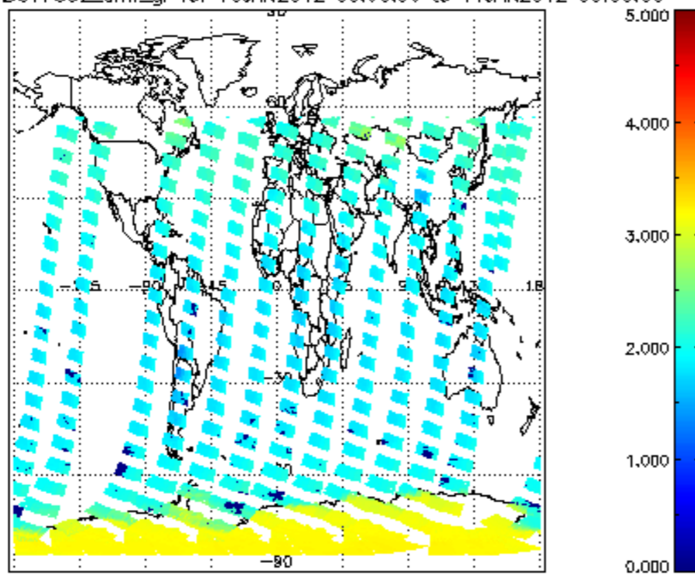
SCIOL2P_NADUV7S02_amf_gr for 10JAN2012 00:00:00 to 11JAN2012 00:00:00
