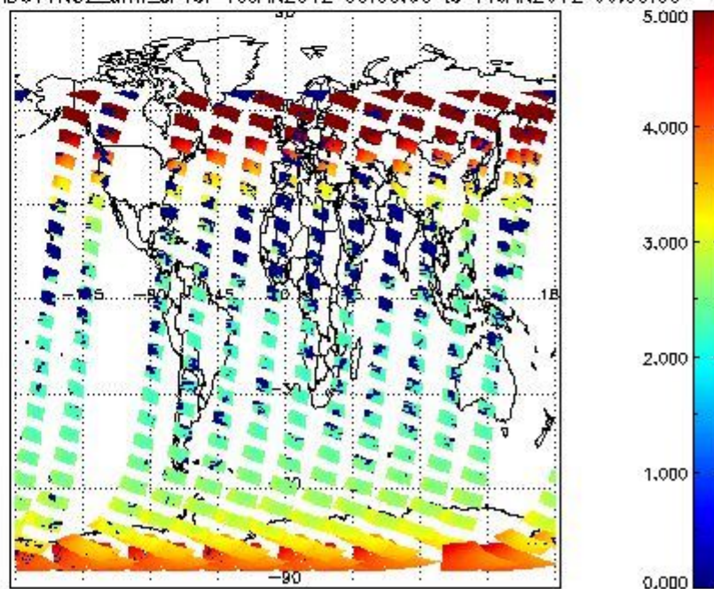
SCIOL2P_NADUV1NO2_amf_cl for 10JAN2012 00:00:00 to 11JAN2012 00:00:00
