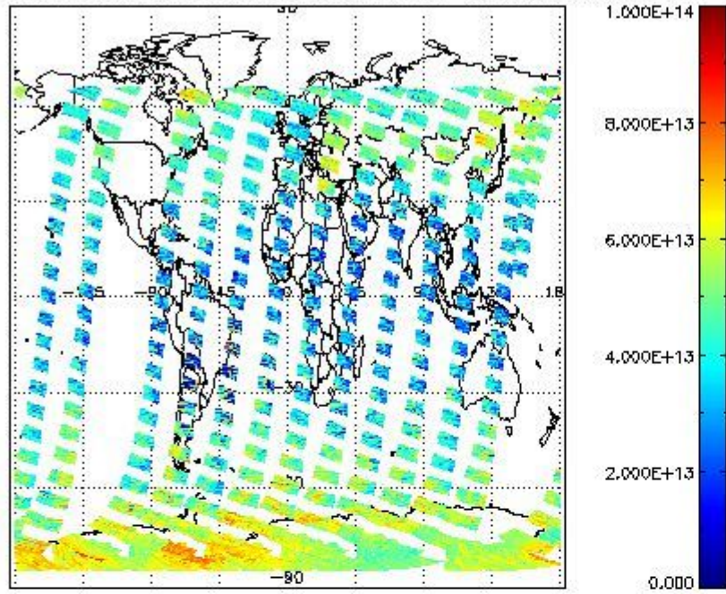
SCIOL2P_NADUV3BRO_vcd for 10JAN2012 00:00:00 to 11JAN2012 00:00:00
