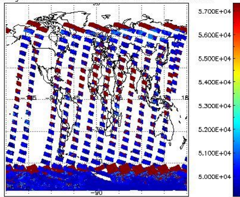
cloud_flags for 10JAN2012 00:00:00 to 11JAN2012 00:00:00
