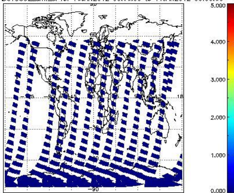
SCIOL2P_NADUV5SO2_amf_cl for 10JAN2012 00:00:00 to 11JAN2012 00:00:00
