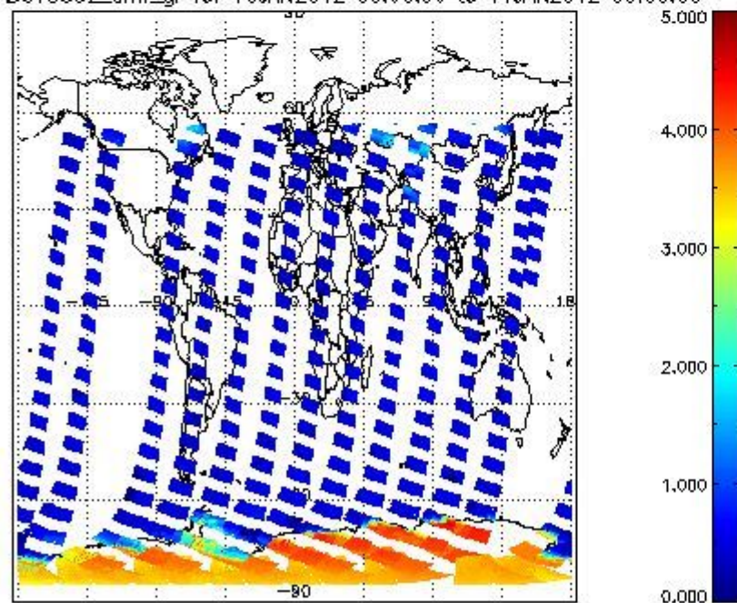
SCIOL2P_NADUV5SO2_amf_gr for 10JAN2012 00:00:00 to 11JAN2012 00:00:00
