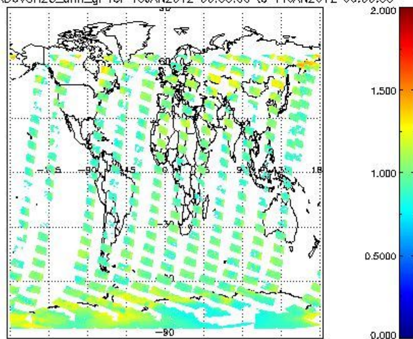
SCIOL2P_NADUV8H20_amf_gr for 10JAN2012 00:00:00 to 11JAN2012 00:00:00
