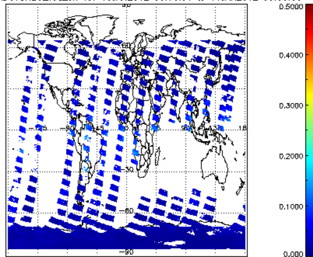
SCIOL2P_NADUV8H20_vcd_err for 10JAN2012 00:00:00 to 11JAN2012 00:00:00
