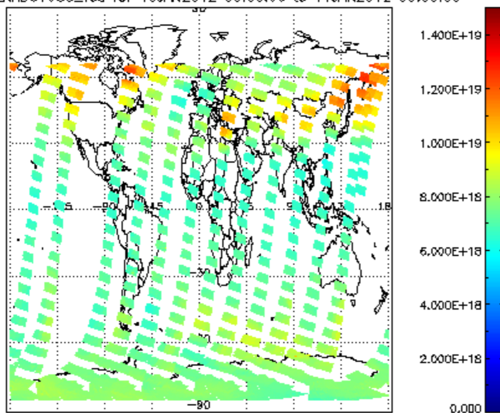
SCIOL2P_NADUV003_vcd for 10JAN2012 00:00:00 to 11JAN2012 00:00:00
