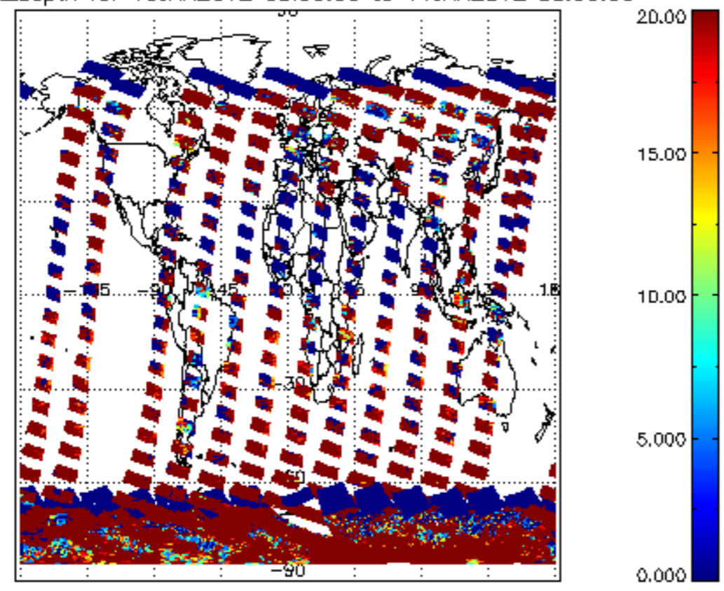
cL_opt_depth for 10JAN2012 00:00:00 to 11JAN2012 00:00:00
