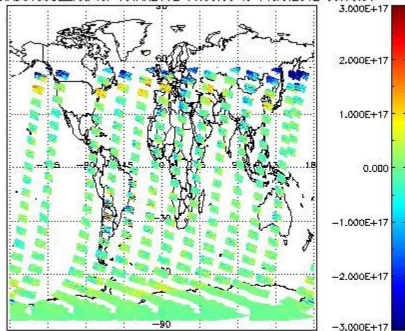
SCIOL2P_NADUV5SO2_vcd for 10JAN2012 00:00:00 to 11JAN2012 00:00:00
