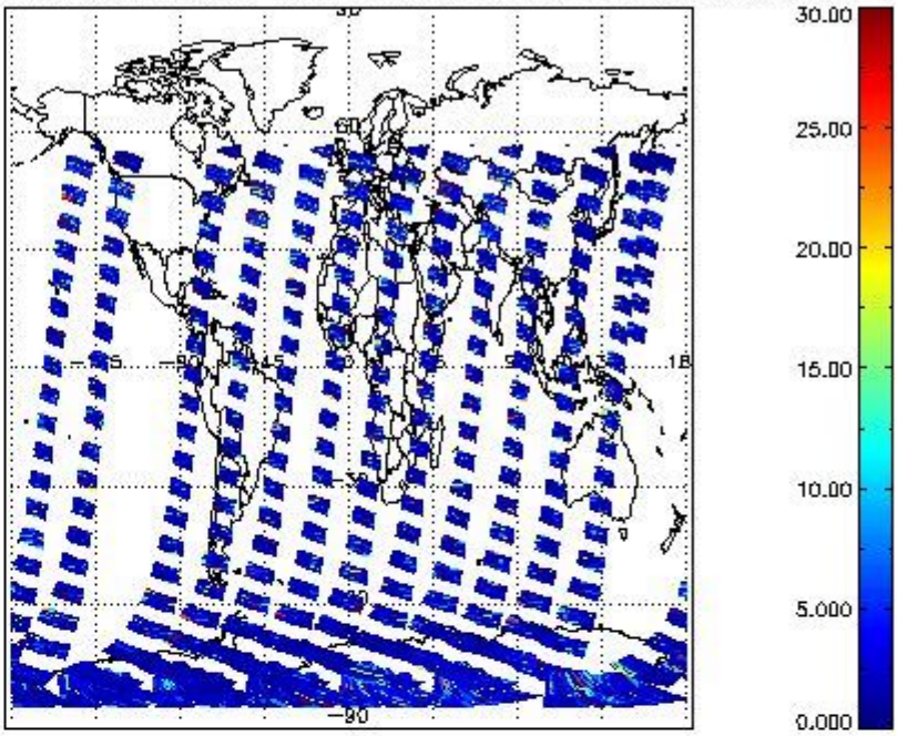
SCIOL2P_NADUV7S02_vcd_err for 10JAN2012 00:00:00 to 11JAN2012 00:00:00
