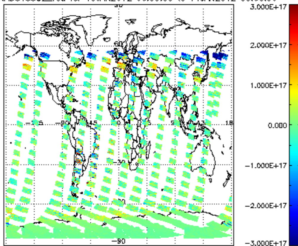
SCIOL2P_NADUV5S02_vcd for 10JAN2012 00:00:00 to 11JAN2012 00:00:00
