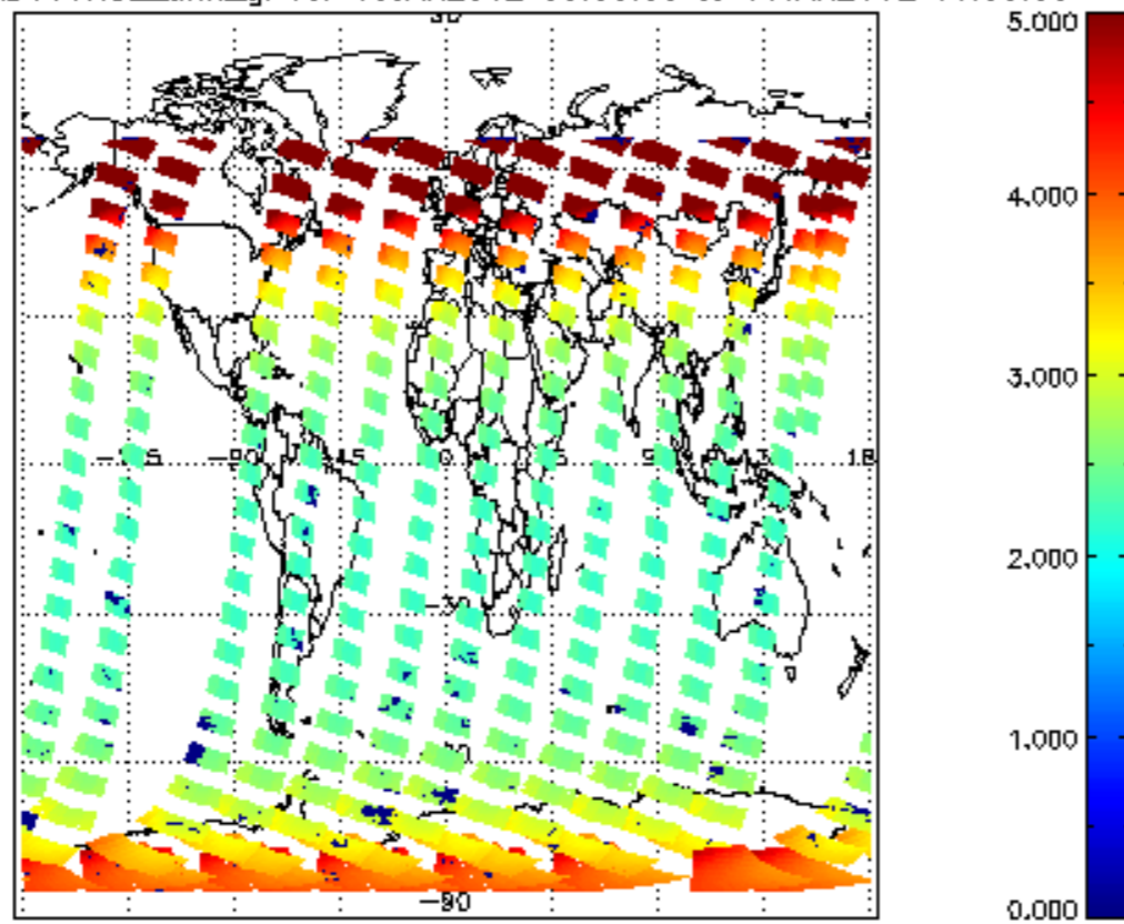
SCIOL2P_NADUV1NO2_amf_gr for 10JAN2012 00:00:00 to 11JAN2012 00:00:00
