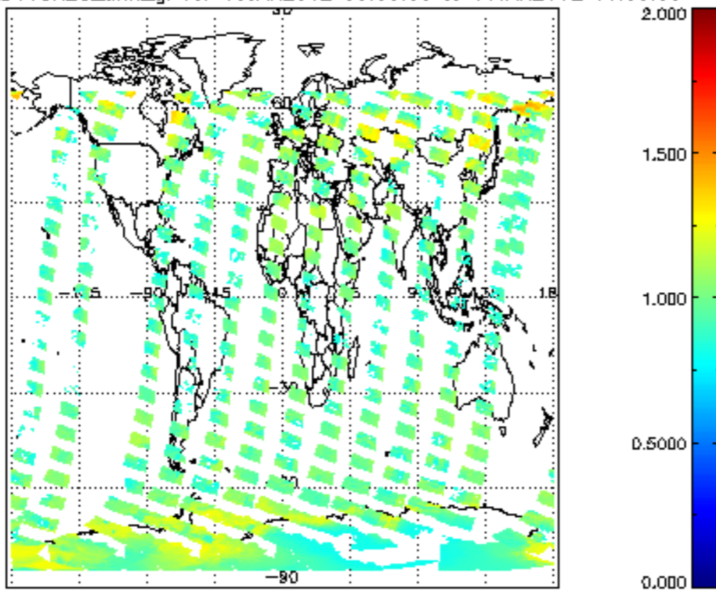
SCIOL2P_NADUV8H20_amf_gr for 10JAN2012 00:00:00 to 11JAN2012 00:00:00
