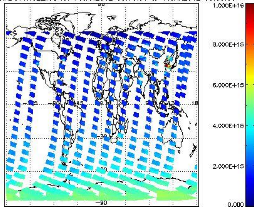
SCIOL2P_NADUV1NO2_vcd for 10JAN2012 00:00:00 to 11JAN2012 00:00:00
