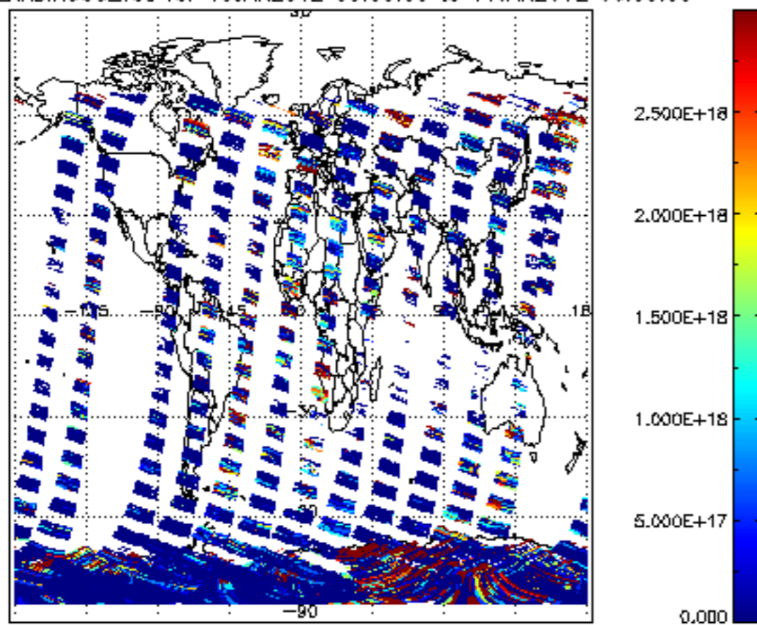
SCIOL2P_NADIR3CO_vcd for 10JAN2012 00:00:00 to 11JAN2012 00:00:00
