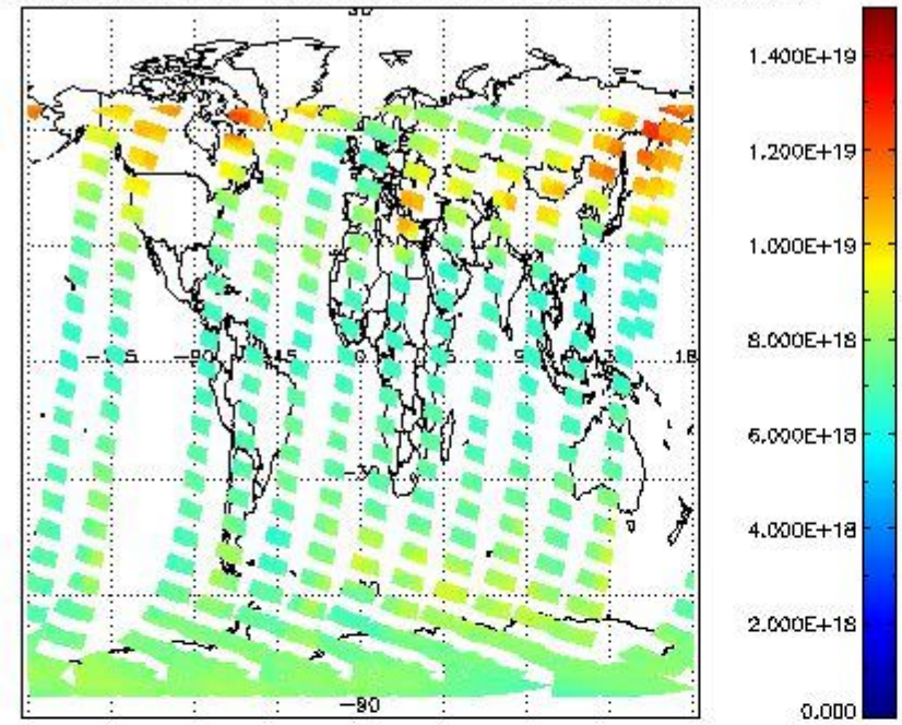
SCIOL2P_NADUV003_vcd for 10JAN2012 00:00:00 to 11JAN2012 00:00:00
