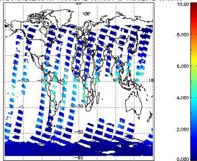
SCIOL2P_NADUV8H20_vcd for 10JAN2012 00:00:00 to 11JAN2012 00:00:00
