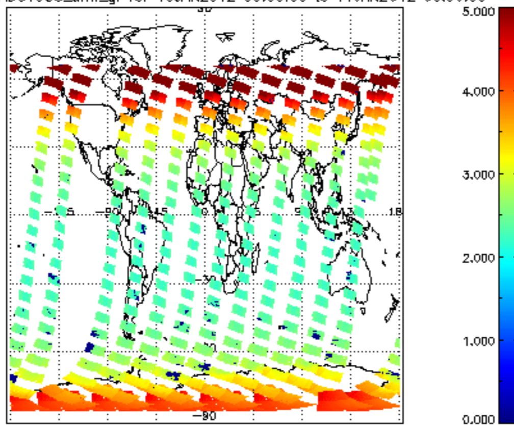
SCIOL2P_NADUV003_amf_gr for 10JAN2012 00:00:00 to 11JAN2012 00:00:00
