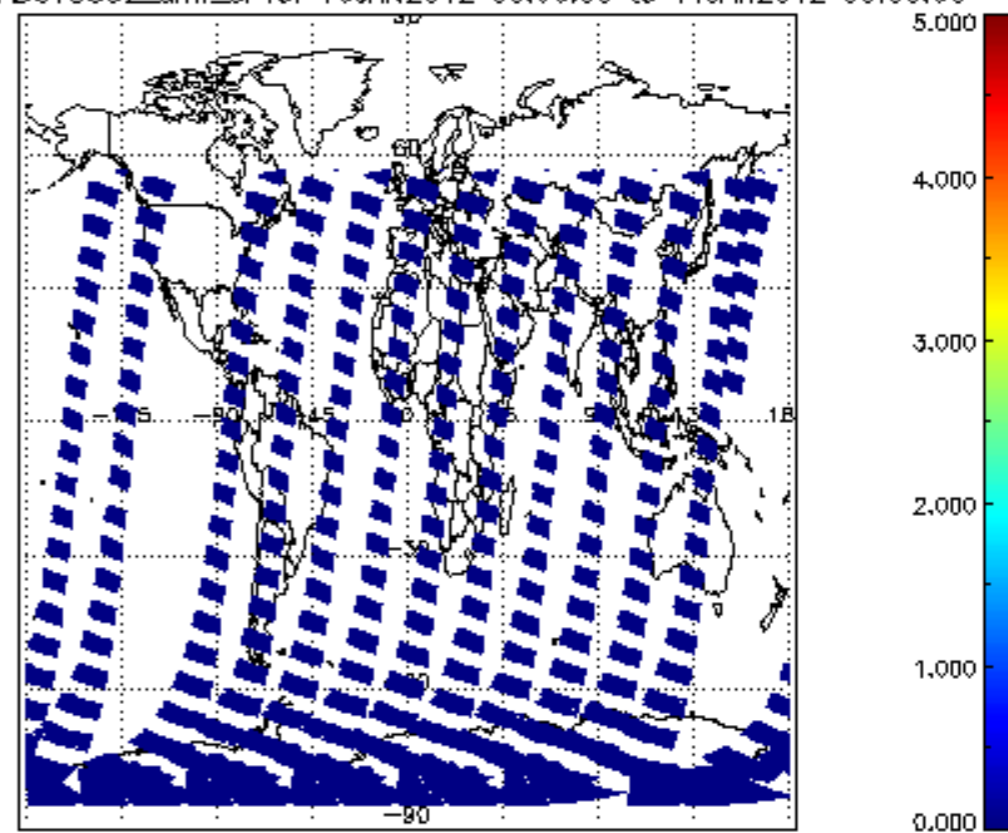
SCIOL2P_NADUV5S02_amf_cl for 10JAN2012 00:00:00 to 11JAN2012 00:00:00
