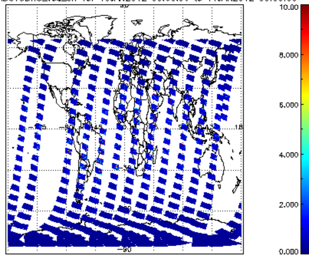
SCIOL2P_NADUV3BRO_vcd_err for 10JAN2012 00:00:00 to 11JAN2012 00:00:00
