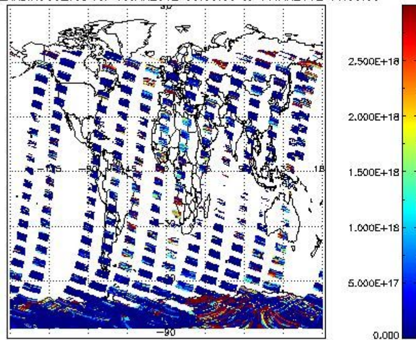
SCIDL2P_NADIR3CO_vcd for 10JAN2012 00:00:00 to 11JAN2012 00:00:00
