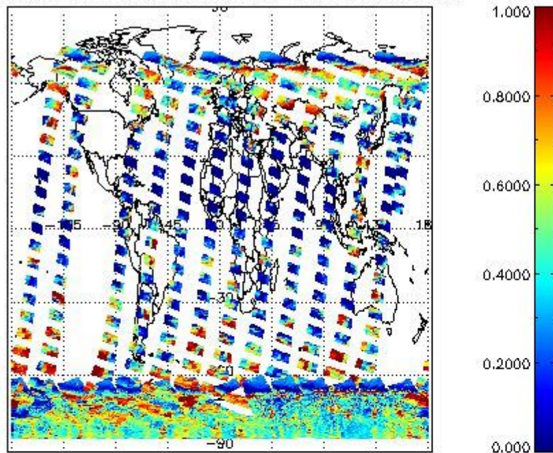
cL_frac for 10JAN2012 00:00:00 to 11JAN2012 00:00:00
