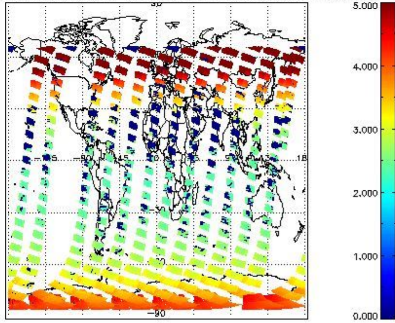
SCIOL2P_NADUV3BRO_amf_cl for 10JAN2012 00:00:00 to 11JAN2012 00:00:00
