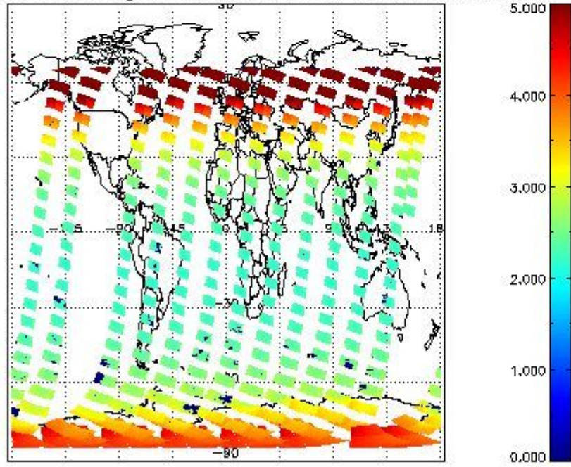
SCIOL2P_NADUV3BRO_amf_gr for 10JAN2012 00:00:00 to 11JAN2012 00:00:00
