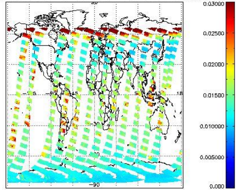
SCIOL2P_NADUV003_vcd_err for 10JAN2012 00:00:00 to 11JAN2012 00:00:00
