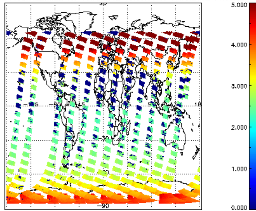
SCIOL2P_NADUV3BRO_amf_cl for 10JAN2012 00:00:00 to 11JAN2012 00:00:00
