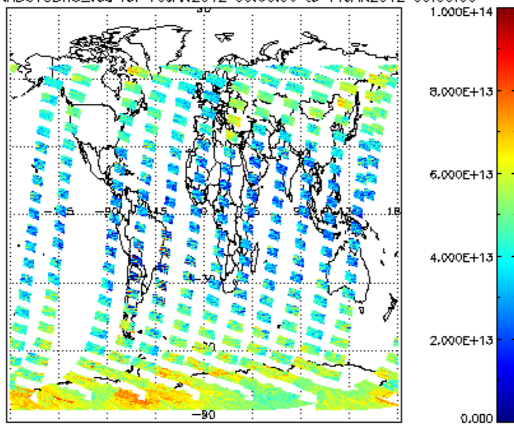
SCIOL2P_NADUV3BRO_vcd for 10JAN2012 00:00:00 to 11JAN2012 00:00:00
