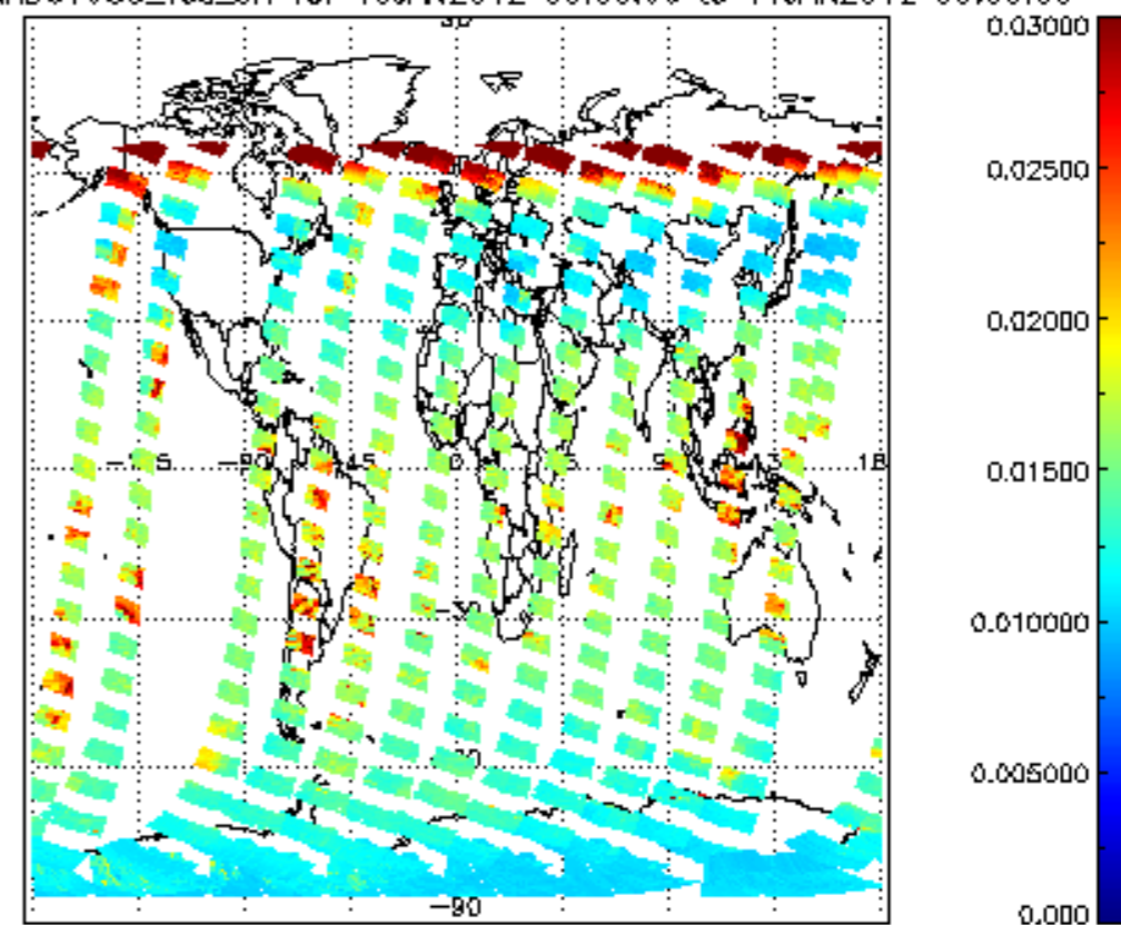
SCIOL2P_NADUV003_vcd_err for 10JAN2012 00:00:00 to 11JAN2012 00:00:00
