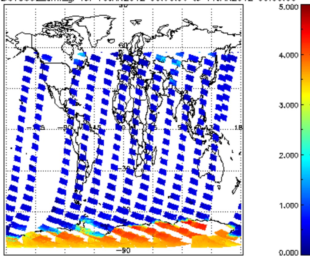
SCIOL2P_NADUV5S02_amf_gr for 10JAN2012 00:00:00 to 11JAN2012 00:00:00
