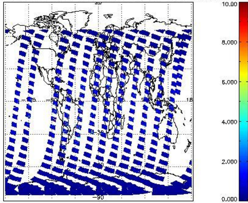
SCIOL2P_NADUV3BRO_vcd_err for 10JAN2012 00:00:00 to 11JAN2012 00:00:00
