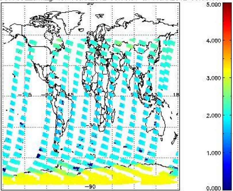
SCIOL2P_NADUV7S02_amf_gr for 10JAN2012 00:00:00 to 11JAN2012 00:00:00
