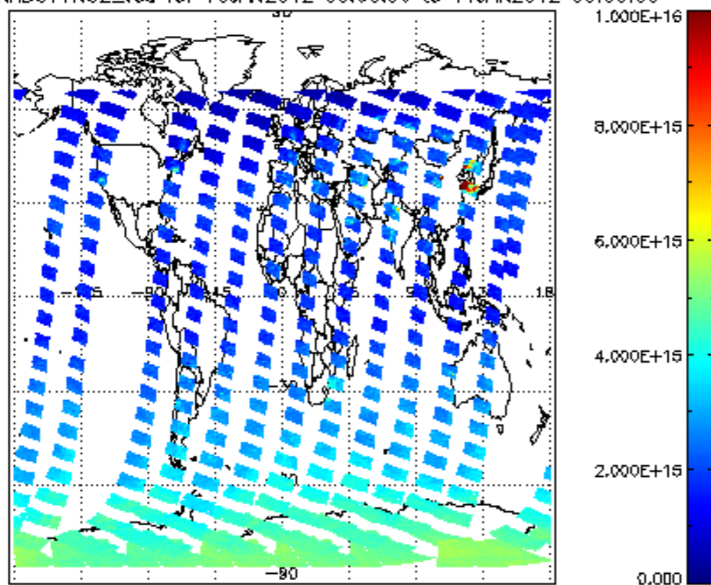
SCIOL2P_NADUV1NO2_vcd for 10JAN2012 00:00:00 to 11JAN2012 00:00:00
