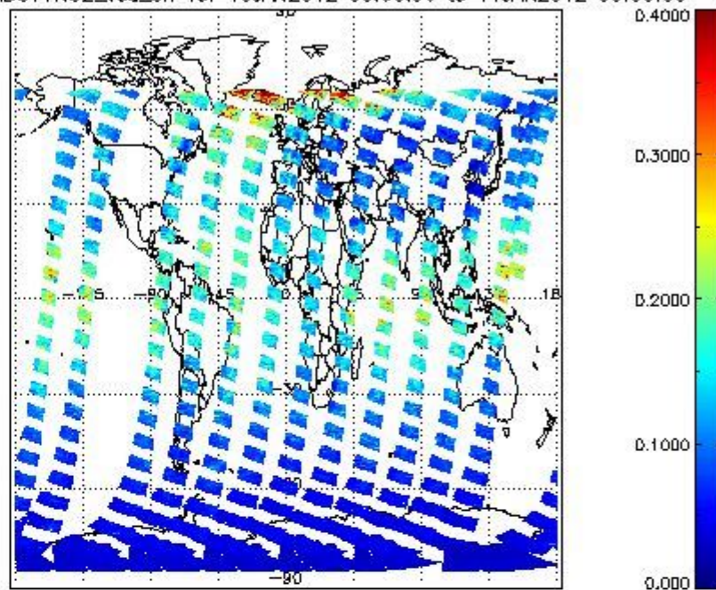
SCIOL2P_NADUV1NO2_vcd_err for 10JAN2012 00:00:00 to 11JAN2012 00:00:00
