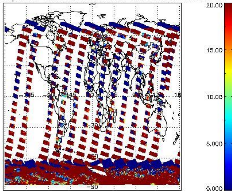
cLopt_depth for 10JAN2012 00:00:00 to 11JAN2012 00:00:00
