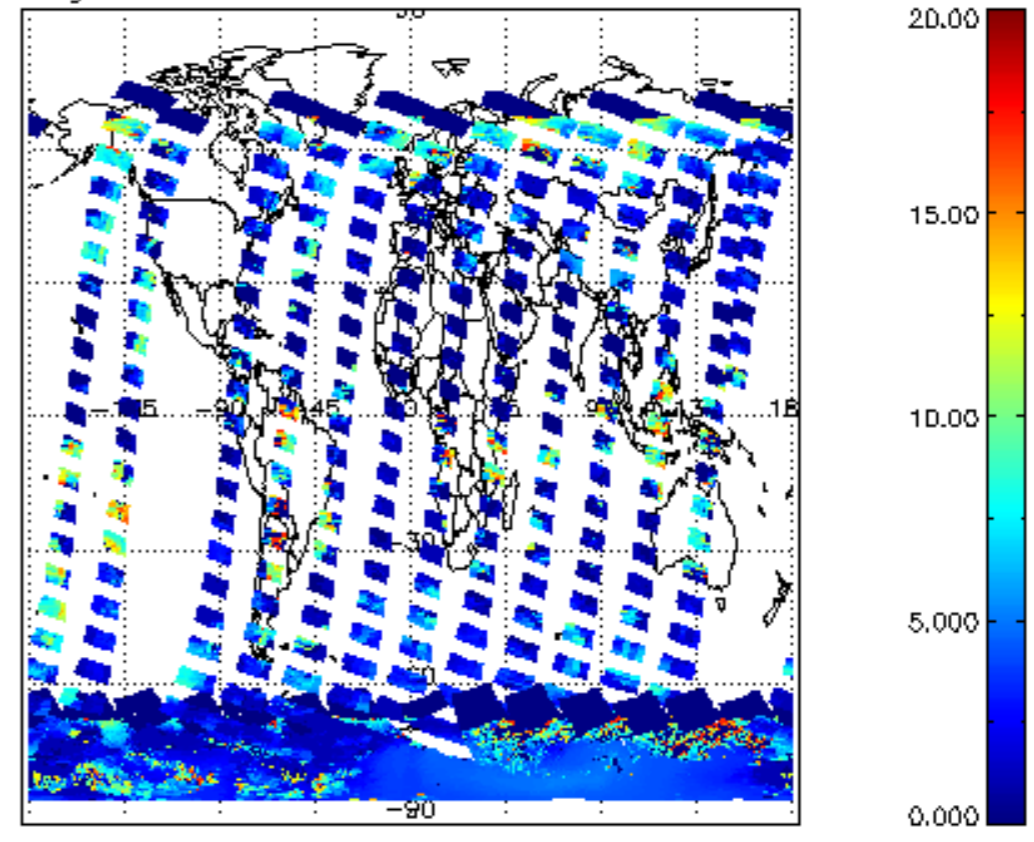
cL_top_height for 10JAN2012 00:00:00 to 11JAN2012 00:00:00
