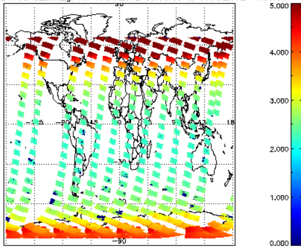
SCIOL2P_NADUV3BRO_amf_gr for 10JAN2012 00:00:00 to 11JAN2012 00:00:00
