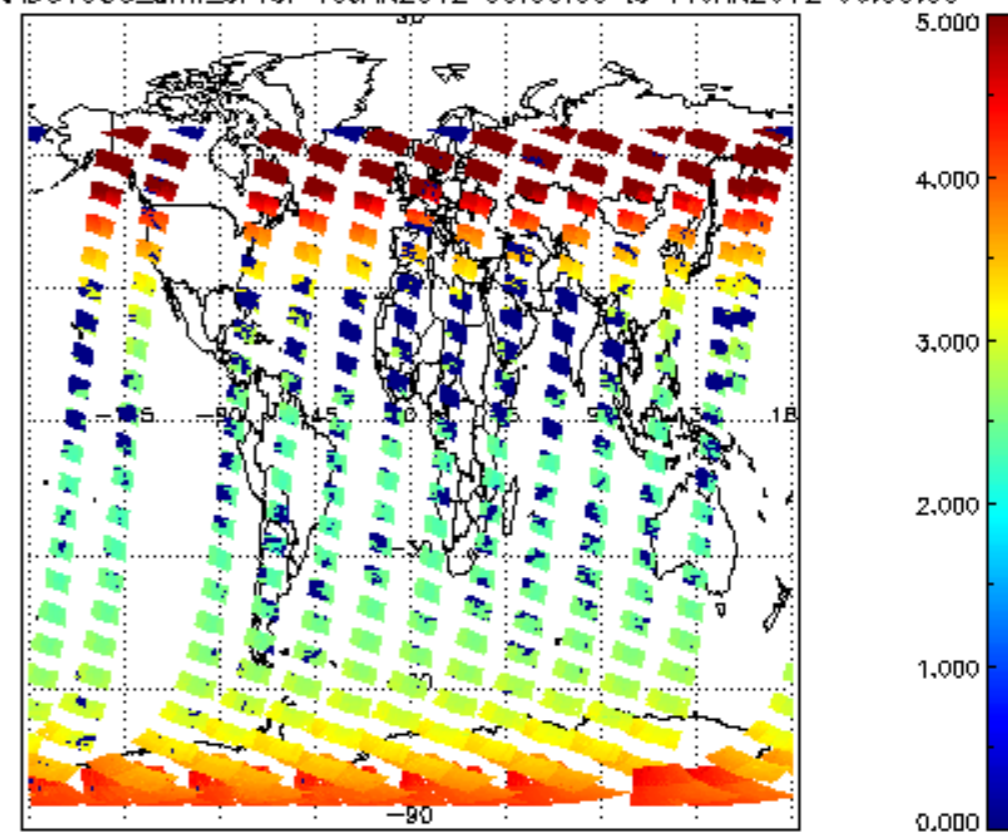
SCIOL2P_NADUV003_amf_cl for 10JAN2012 00:00:00 to 11JAN2012 00:00:00
