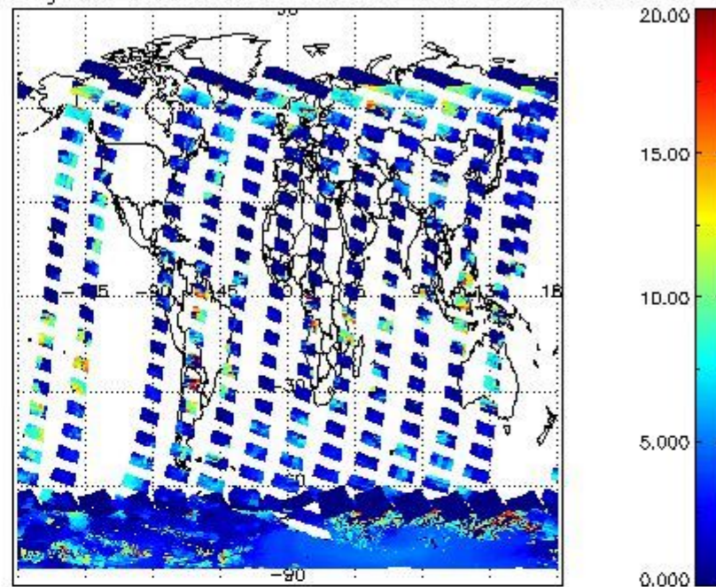
cL_top_height for 10JAN2012 00:00:00 to 11JAN2012 00:00:00
