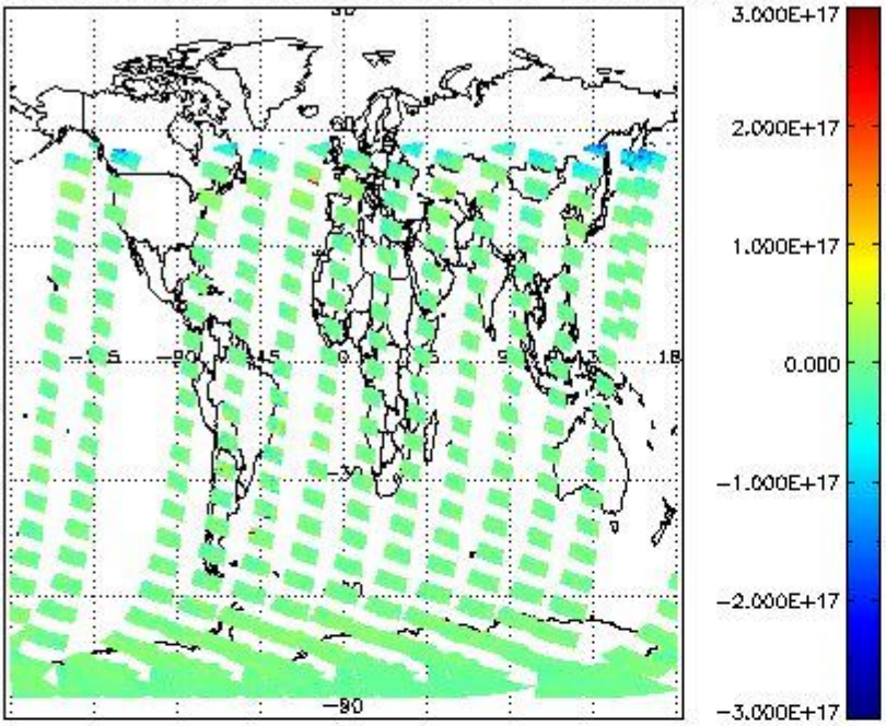
SCIOL2P_NADUV7S02_vcd for 10JAN2012 00:00:00 to 11JAN2012 00:00:00
