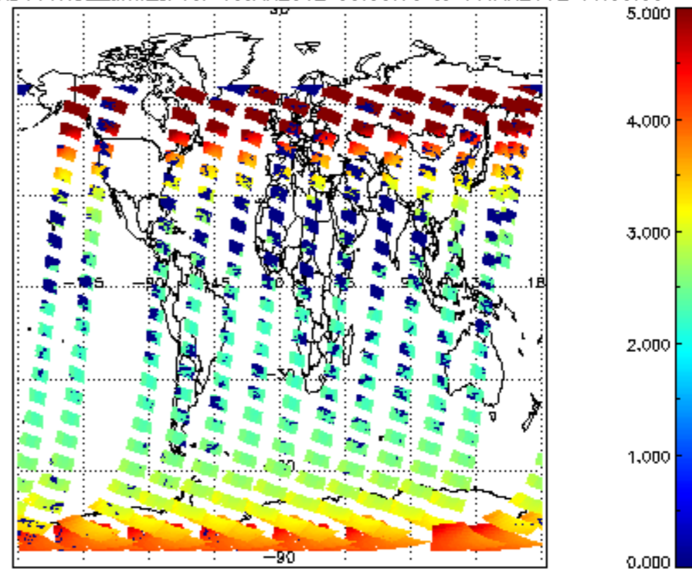
SCIOL2P_NADUV1NO2_amf_cl for 10JAN2012 00:00:00 to 11JAN2012 00:00:00
