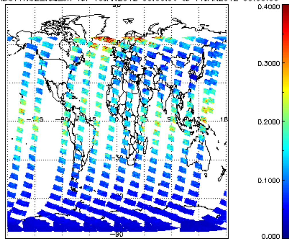
SCIOL2P_NADUV1NO2_vcd_err for 10JAN2012 00:00:00 to 11JAN2012 00:00:00
