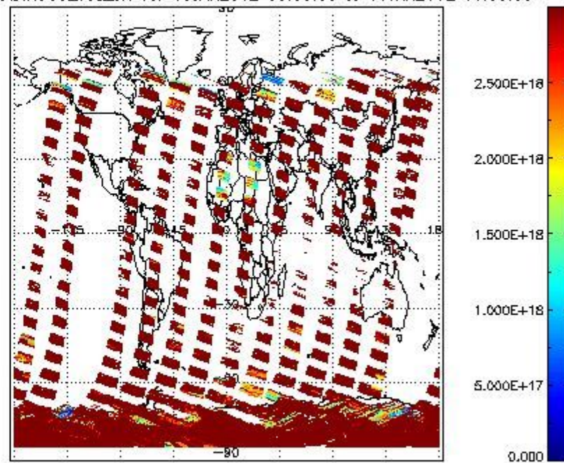
SCIDL2P_NADIR3CO_vcd_err for 10JAN2012 00:00:00 to 11JAN2012 00:00:00
