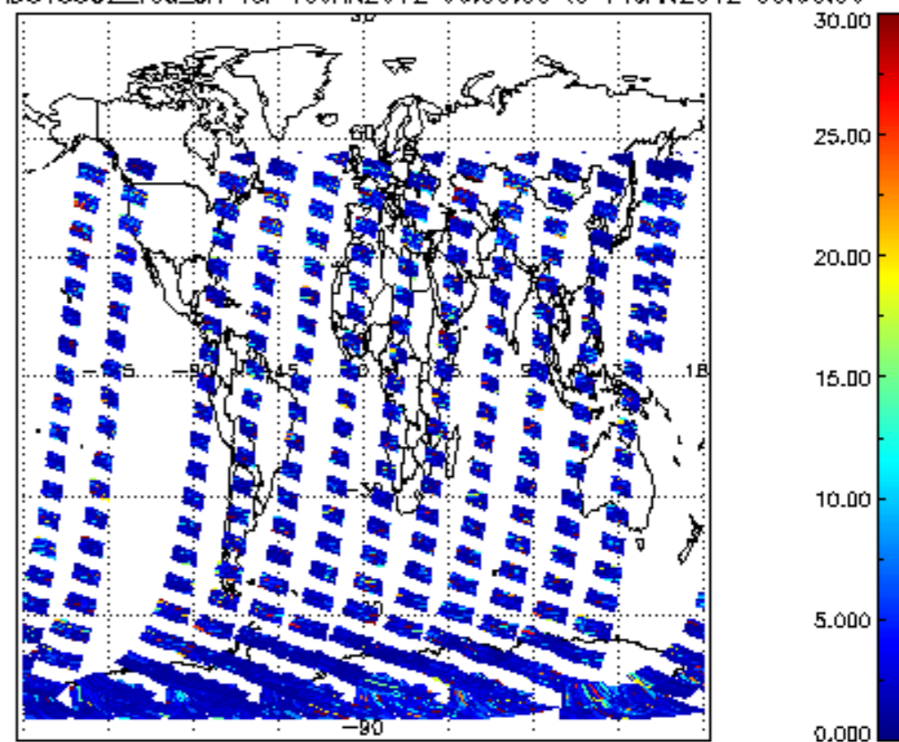
SCIOL2P_NADUV5S02_vcd_err for 10JAN2012 00:00:00 to 11JAN2012 00:00:00
