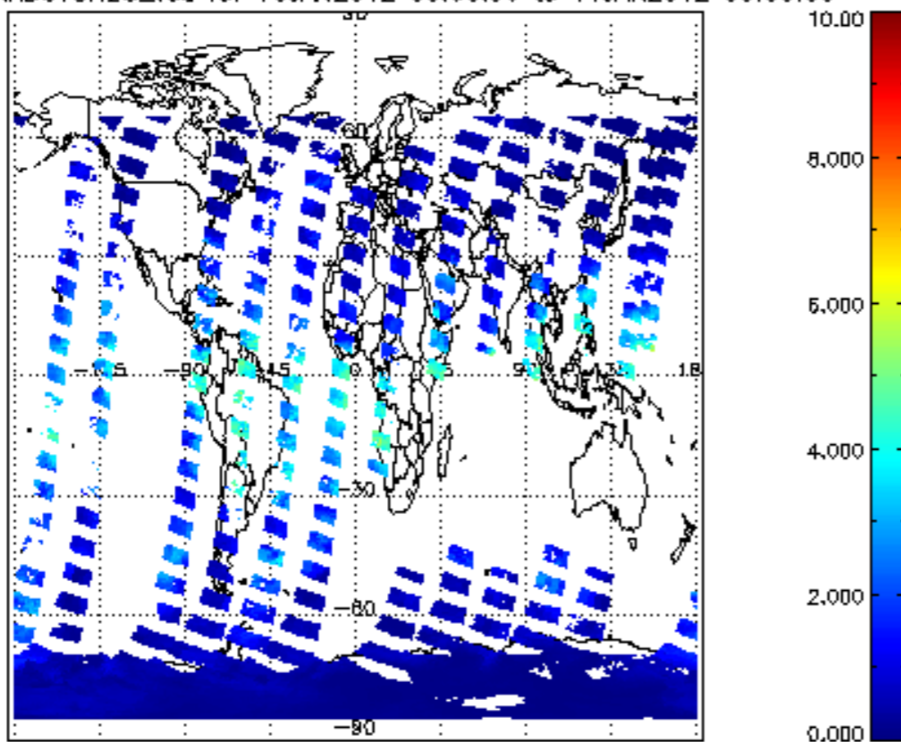
SCIOL2P_NADUV8H20_vcd for 10JAN2012 00:00:00 to 11JAN2012 00:00:00
