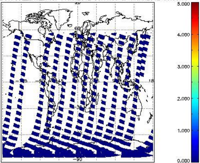
SCIOL2P_NADUV7S02_amf_cl for 10JAN2012 00:00:00 to 11JAN2012 00:00:00
