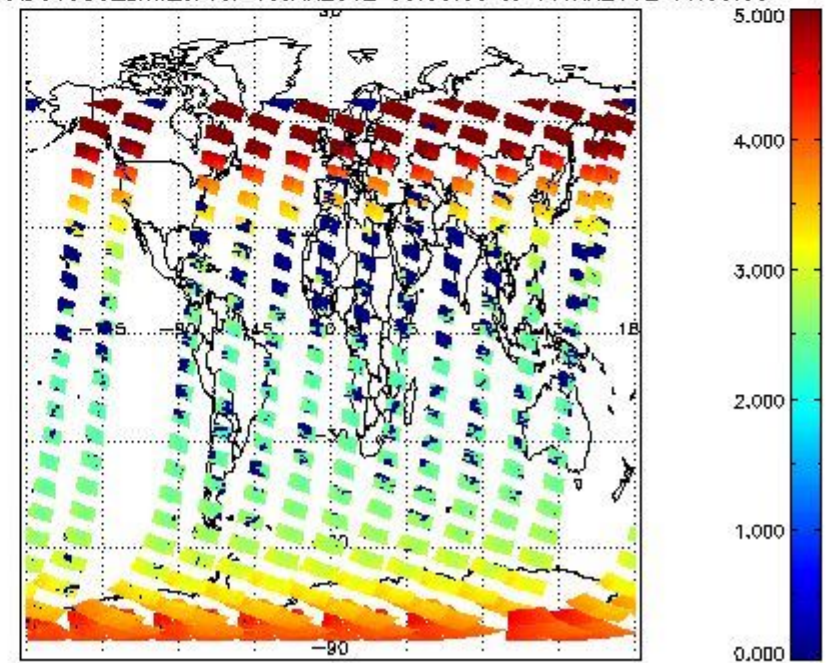
SCIOL2P_NADUV003_amf_cl for 10JAN2012 00:00:00 to 11JAN2012 00:00:00
