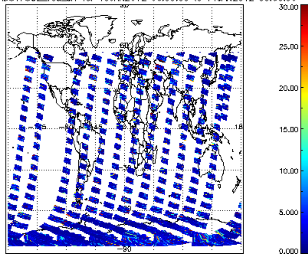
SCIOL2P_NADUV7S02_vcd_err for 10JAN2012 00:00:00 to 11JAN2012 00:00:00
