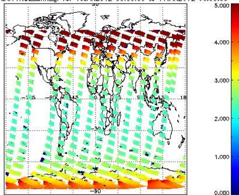
SCIOL2P_NADUV1NO2_amf_gr for 10JAN2012 00:00:00 to 11JAN2012 00:00:00
