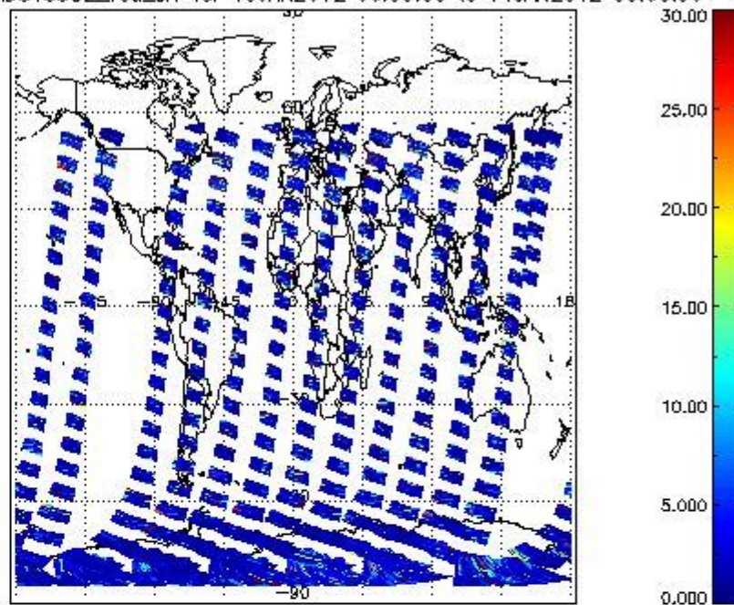
SCIOL2P_NADUV5SO2_vcd_err for 10JAN2012 00:00:00 to 11JAN2012 00:00:00
