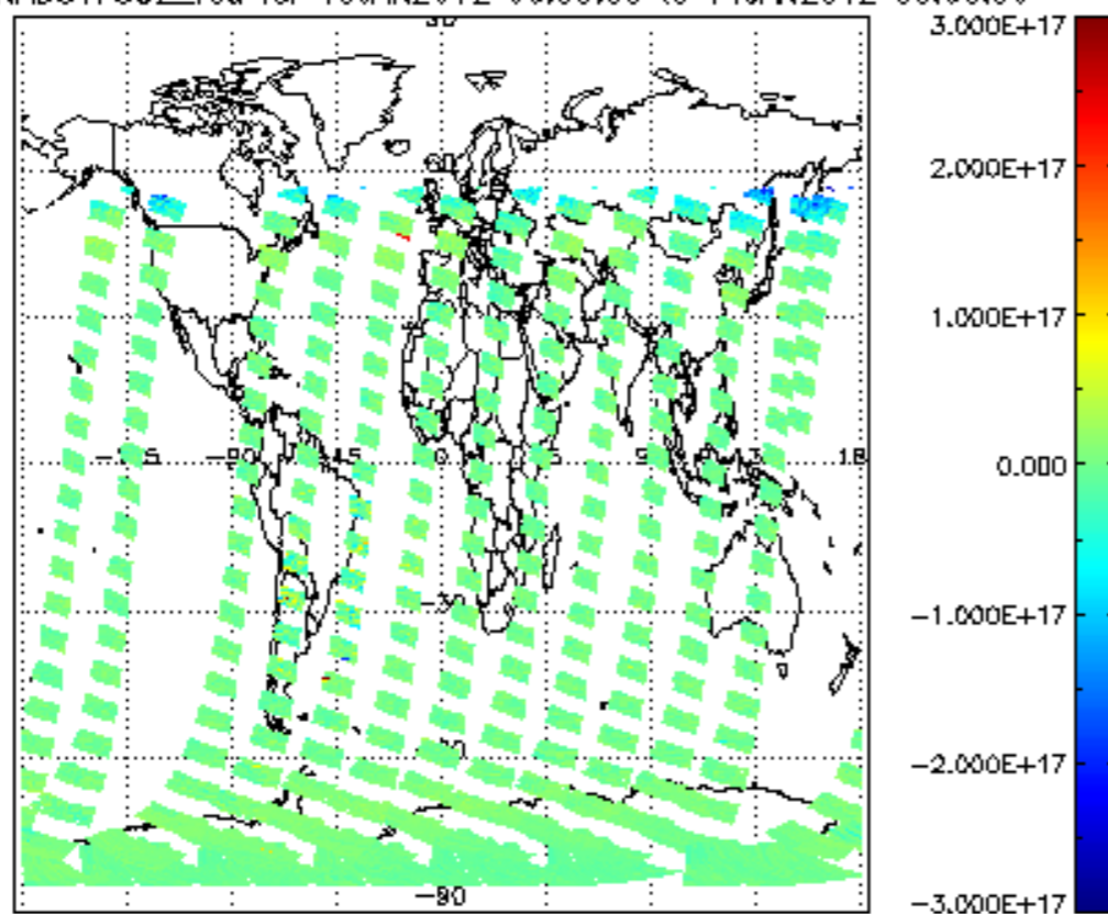
SCIOL2P_NADUV7S02_vcd for 10JAN2012 00:00:00 to 11JAN2012 00:00:00
