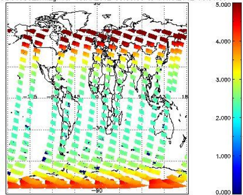
SCIOL2P_NADUV003_amf_gr for 10JAN2012 00:00:00 to 11JAN2012 00:00:00
