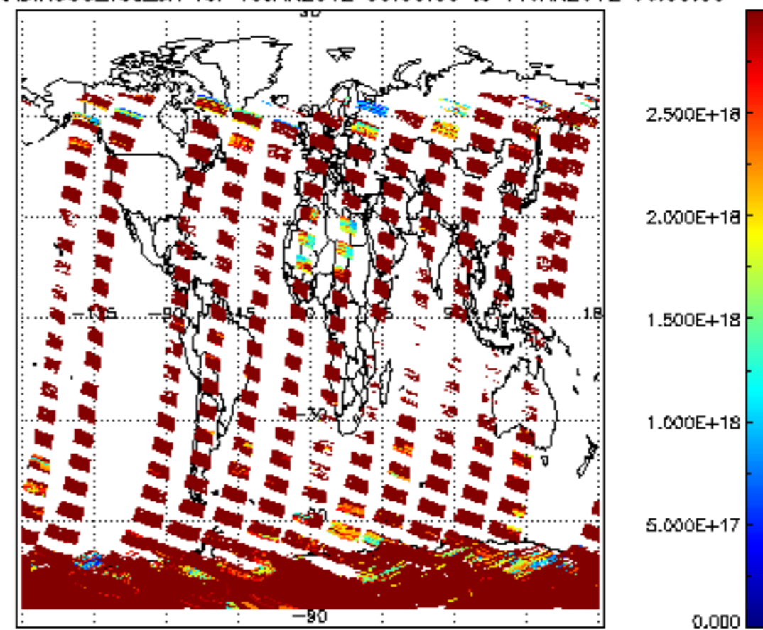
SCIOL2P_NADIR3CO_vcd_err for 10JAN2012 00:00:00 to 11JAN2012 00:00:00
