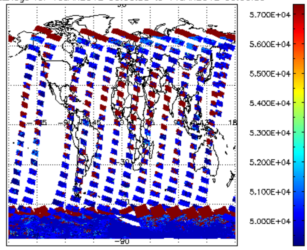
cloud_flags for 10JAN2012 00:00:00 to 11JAN2012 00:00:00
