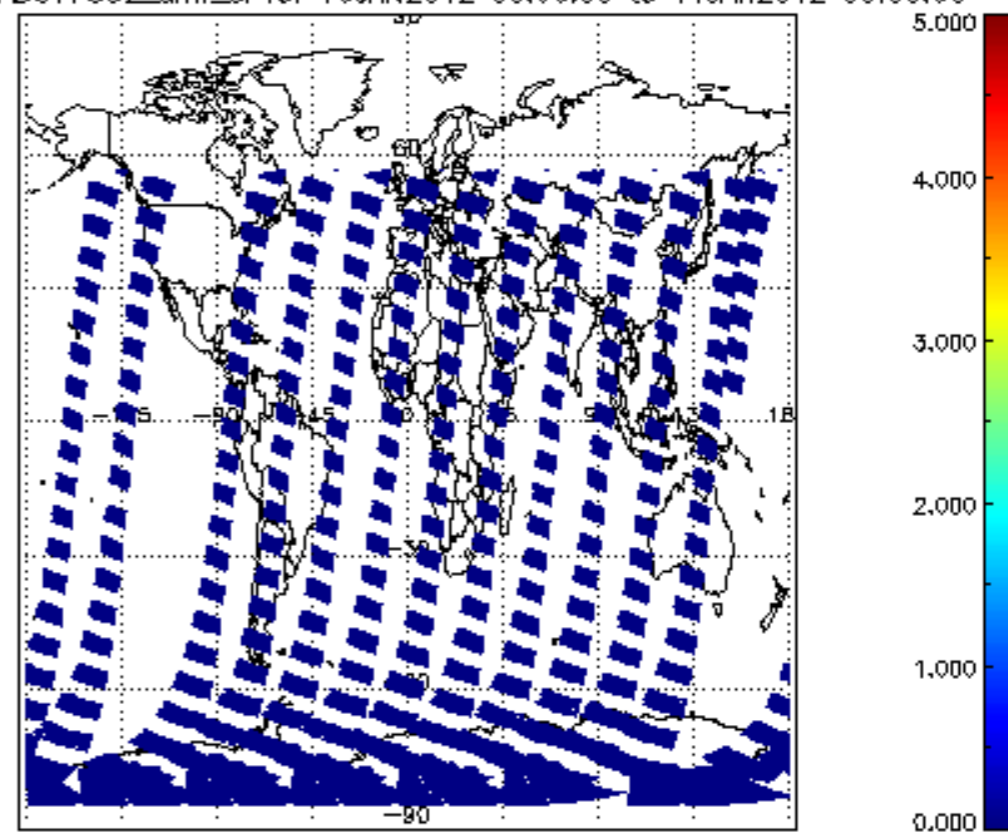
SCIOL2P_NADUV7S02_amf_cl for 10JAN2012 00:00:00 to 11JAN2012 00:00:00
