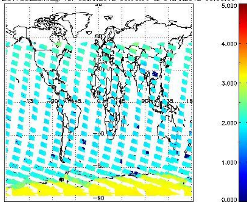
SCIOL2P_NADUV7S02_amf_gr for 03JAN2012 00:00:00 to 04JAN2012 00:00:00
