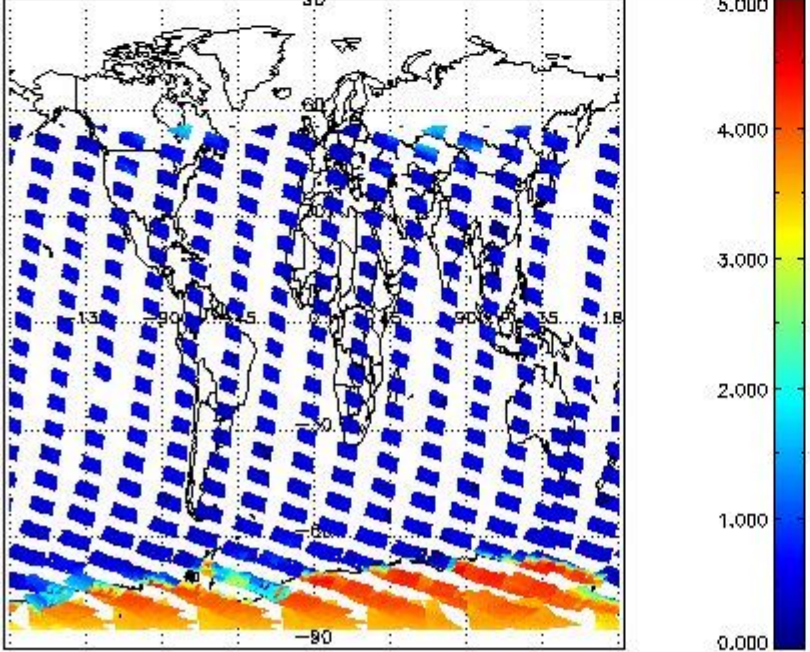
SCIOL2P_NADUV5SO2_amf_gr for 03JAN2012 00:00:00 to 04JAN2012 00:00:00
