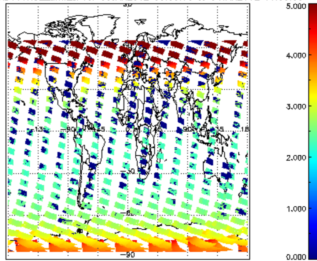
SCIOL2P_NADUV1NO2_amf_cl for 03JAN2012 00:00:00 to 04JAN2012 00:00:00
