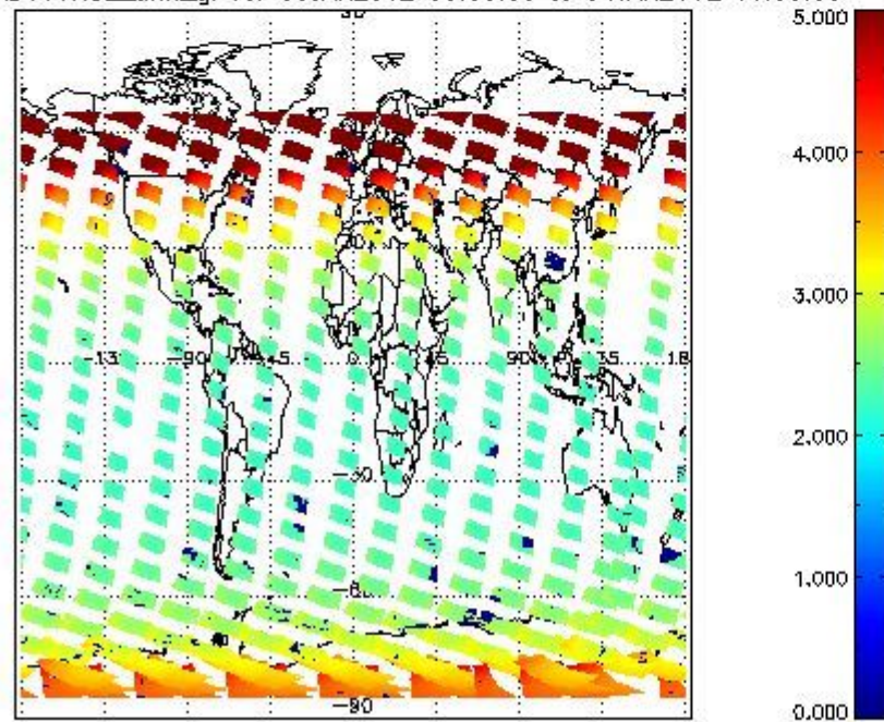
SCIOL2P_NADUV1N02_amf_gr for 03JAN2012 00:00:00 to 04JAN2012 00:00:00
