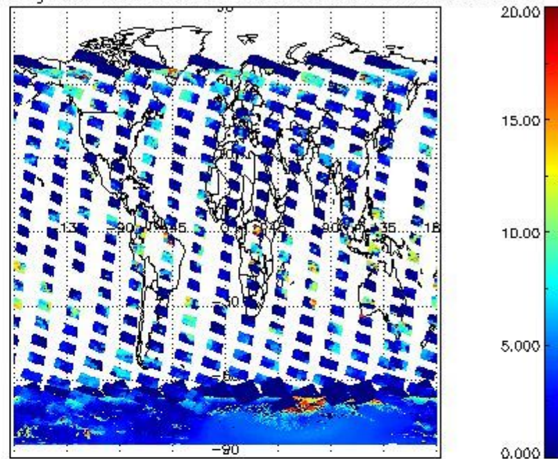
cL_top_height for 03JAN2012 00:00:00 to 04JAN2012 00:00:00
