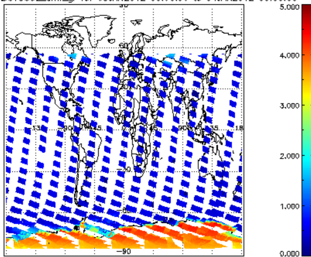
SCIOL2P_NADUV5S02_amf_gr for 03JAN2012 00:00:00 to 04JAN2012 00:00:00
