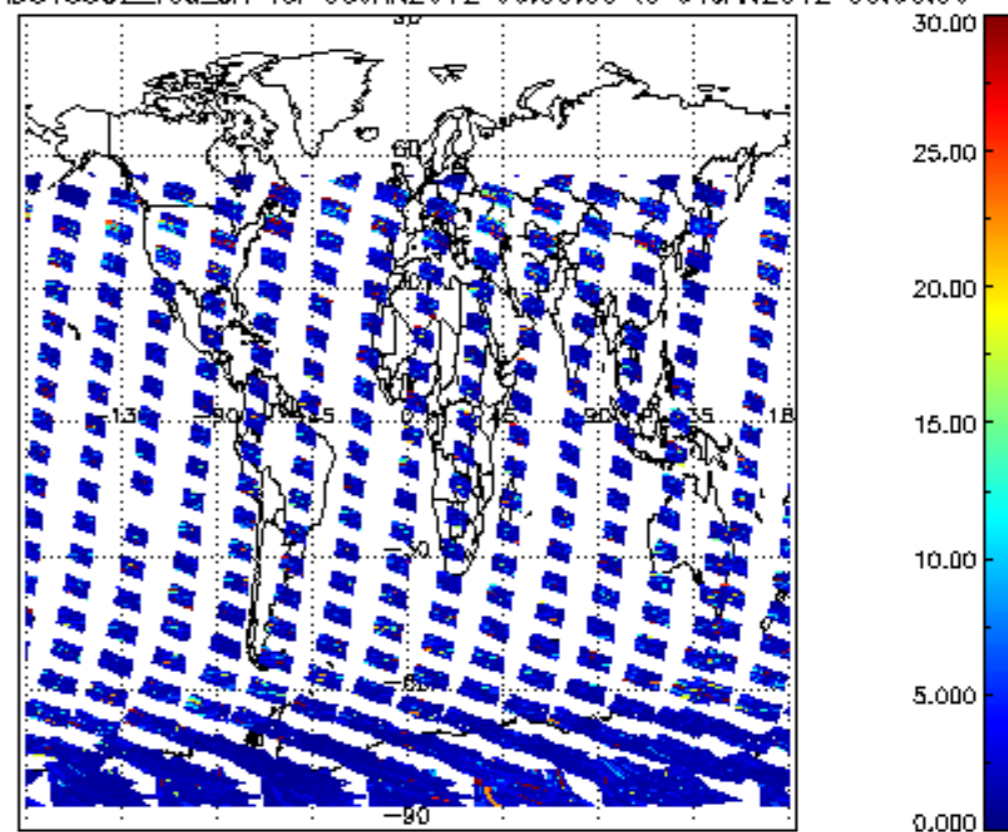
SCIOL2P_NADUV5S02_vcd_err for 03JAN2012 00:00:00 to 04JAN2012 00:00:00
