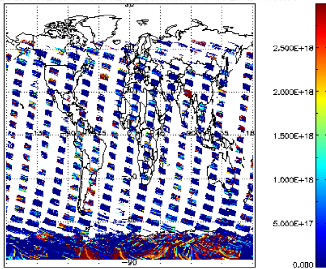
SCIOL2P_NADIR3CO_vcd for 03JAN2012 00:00:00 to 04JAN2012 00:00:00
