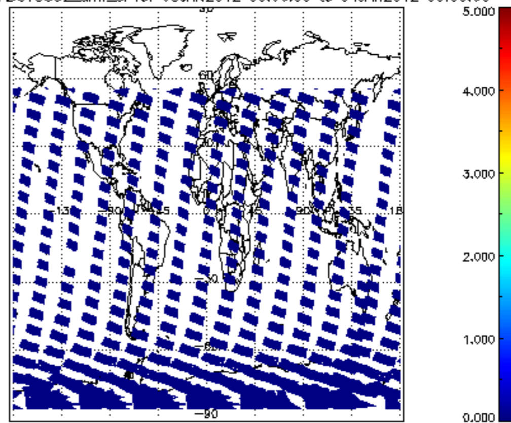
SCIOL2P_NADUV5S02_amf_cl for 03JAN2012 00:00:00 to 04JAN2012 00:00:00
