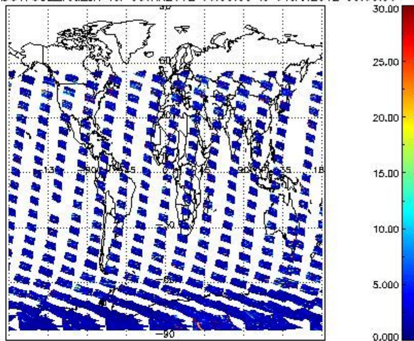
SCIOL2P_NADUV7S02_vcd_err for 03JAN2012 00:00:00 to 04JAN2012 00:00:00
