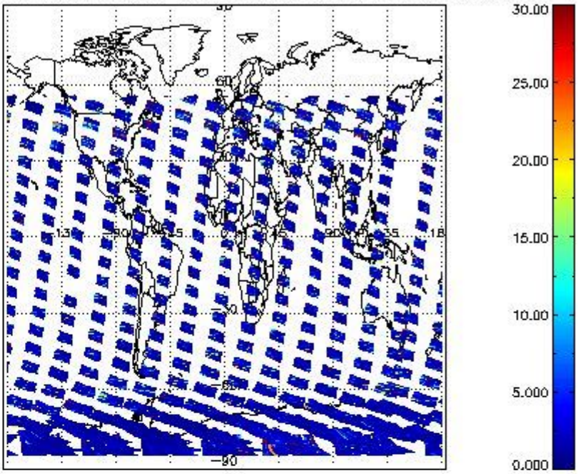
SCIOL2P_NADUV5SO2_vcd_err for 03JAN2012 00:00:00 to 04JAN2012 00:00:00
