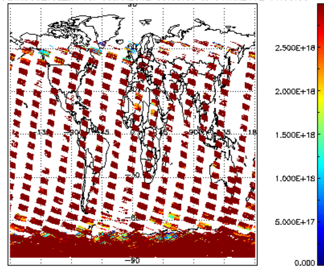
SCIOL2P_NADIR3CO_vcd_err for 03JAN2012 00:00:00 to 04JAN2012 00:00:00
