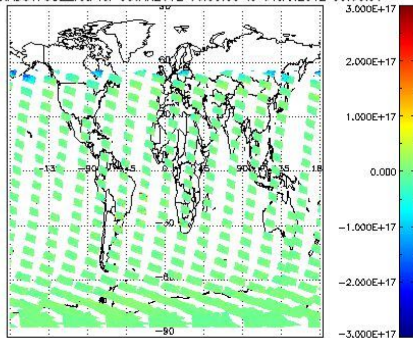
SCIOL2P_NADUV7S02_vcd for 03JAN2012 00:00:00 to 04JAN2012 00:00:00
