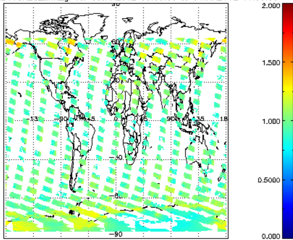
SCIOL2P_NADUV8H20_amf_gr for 03JAN2012 00:00:00 to 04JAN2012 00:00:00
