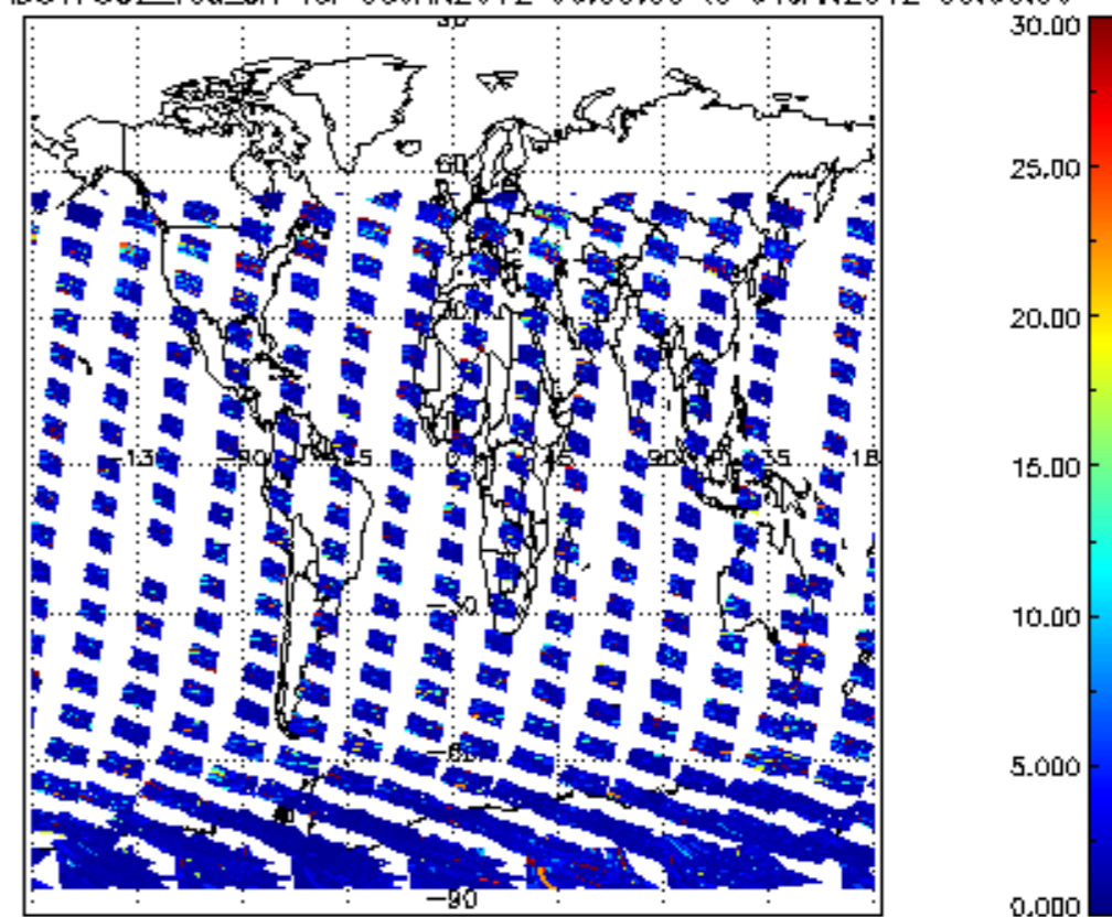
SCIOL2P_NADUV7S02_vcd_err for 03JAN2012 00:00:00 to 04JAN2012 00:00:00
