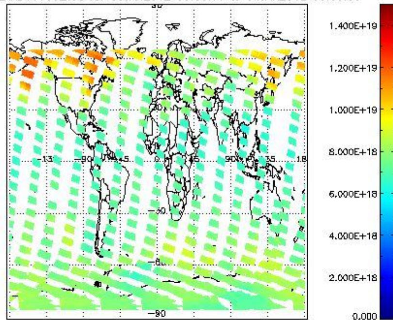
SCIOL2P_NADUV003_vcd for 03JAN2012 00:00:00 to 04JAN2012 00:00:00
