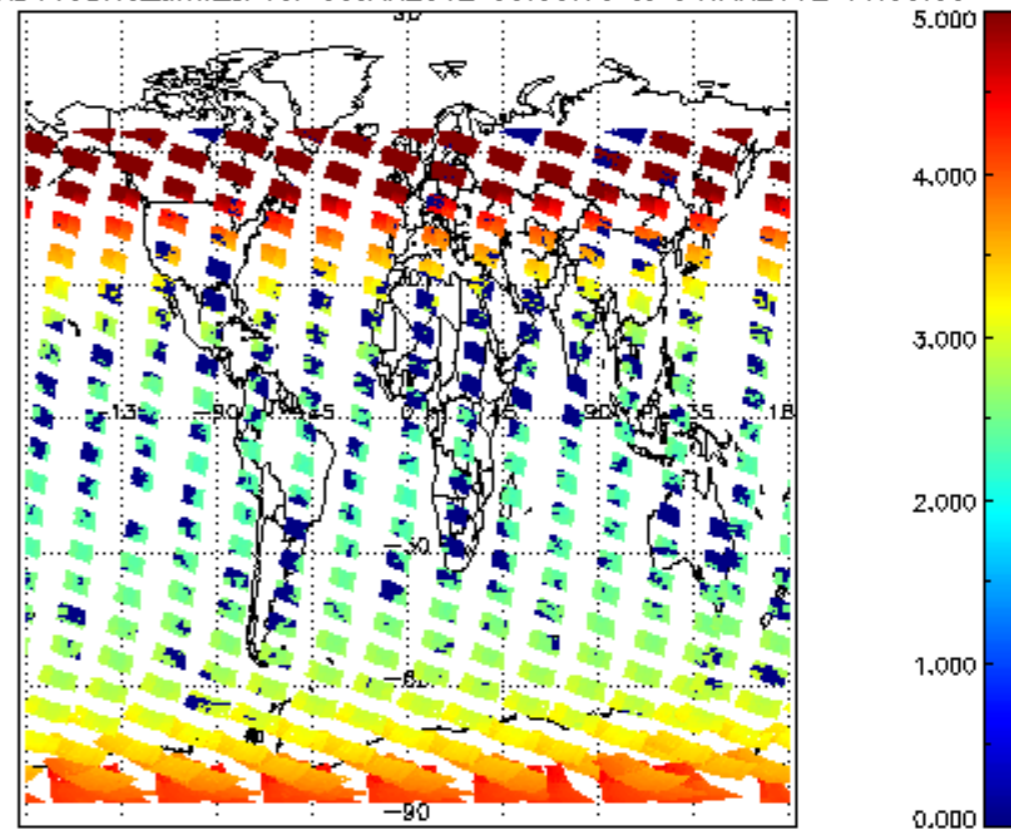
SCIOL2P_NADUV3BRO_amf_cl for 03JAN2012 00:00:00 to 04JAN2012 00:00:00
