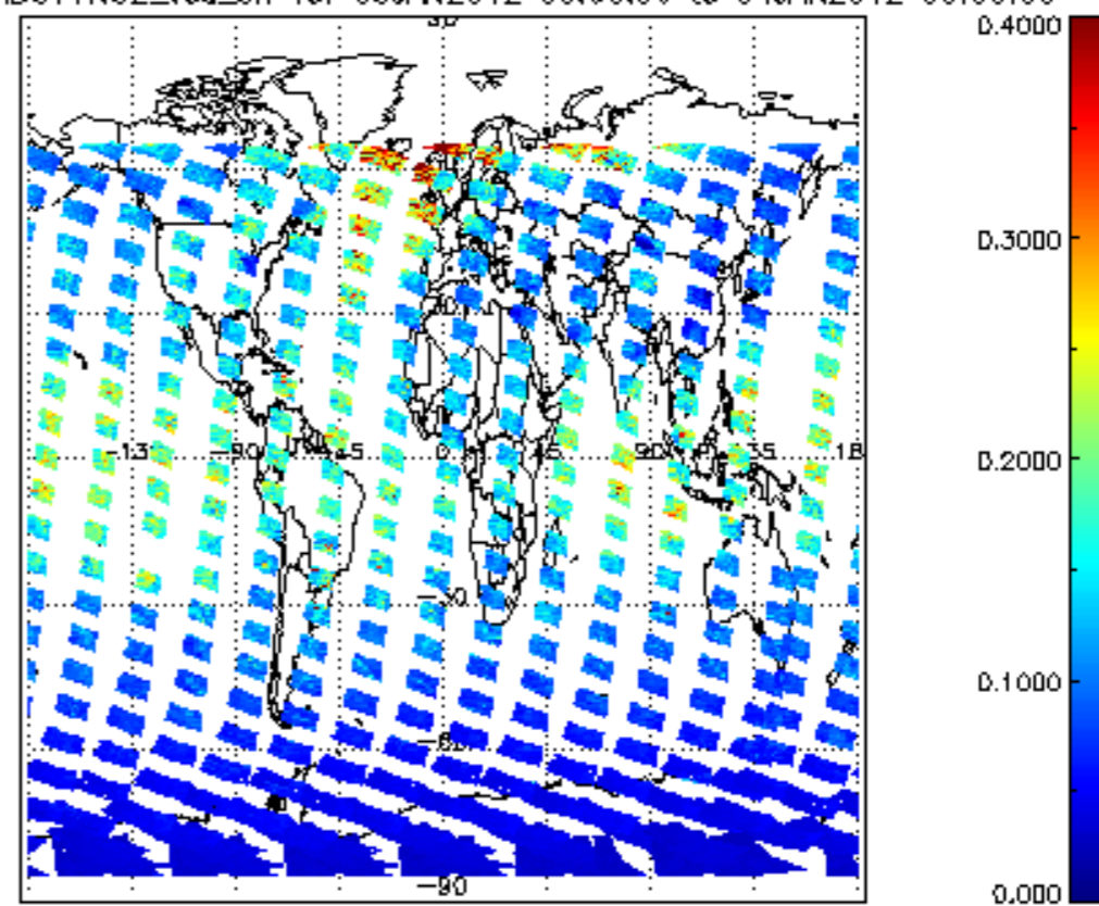
SCIOL2P_NADUV1NO2_vcd_err for 03JAN2012 00:00:00 to 04JAN2012 00:00:00
