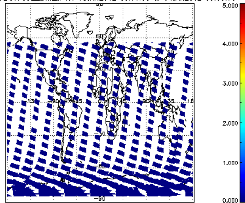
SCIOL2P_NADUV7S02_amf_sl for 03JAN2012 00:00:00 to 04JAN2012 00:00:00
