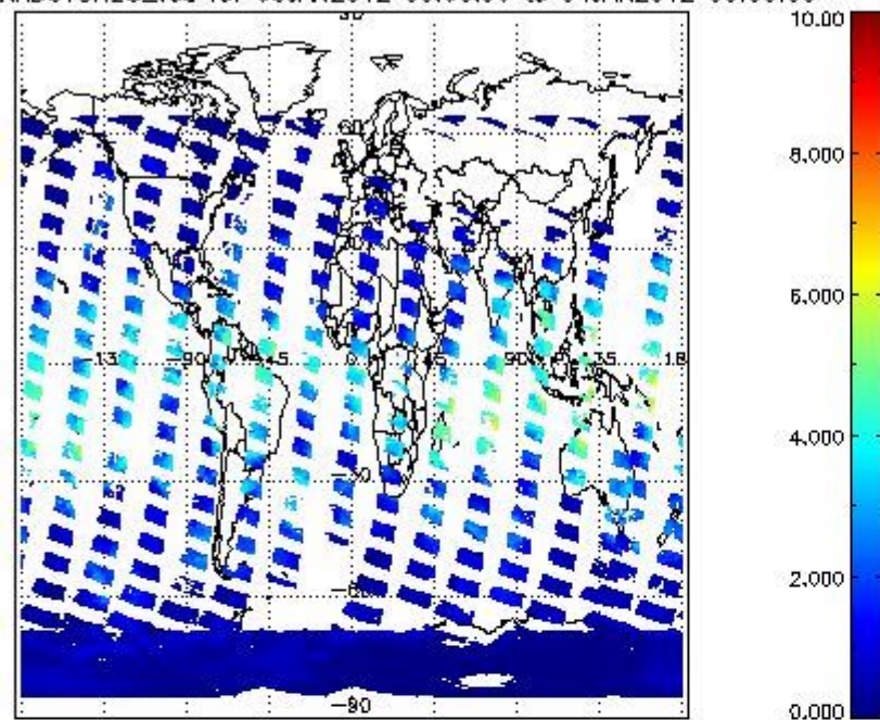
SCIOL2P_NADUV8H20_vcd for 03JAN2012 00:00:00 to 04JAN2012 00:00:00
