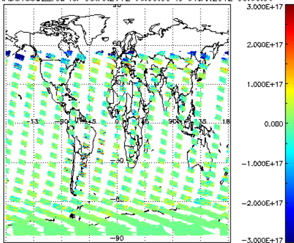
SCIOL2P_NADUV5S02_vcd for 03JAN2012 00:00:00 to 04JAN2012 00:00:00
