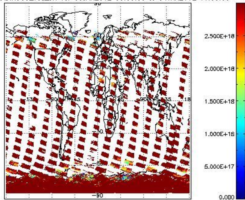
SCIDL2P_NADIR3CO_vcd_err for 03JAN2012 00:00:00 to 04JAN2012 00:00:00
