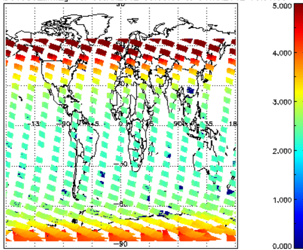
SCIOL2P_NADUV003_amf_gr for 03JAN2012 00:00:00 to 04JAN2012 00:00:00
