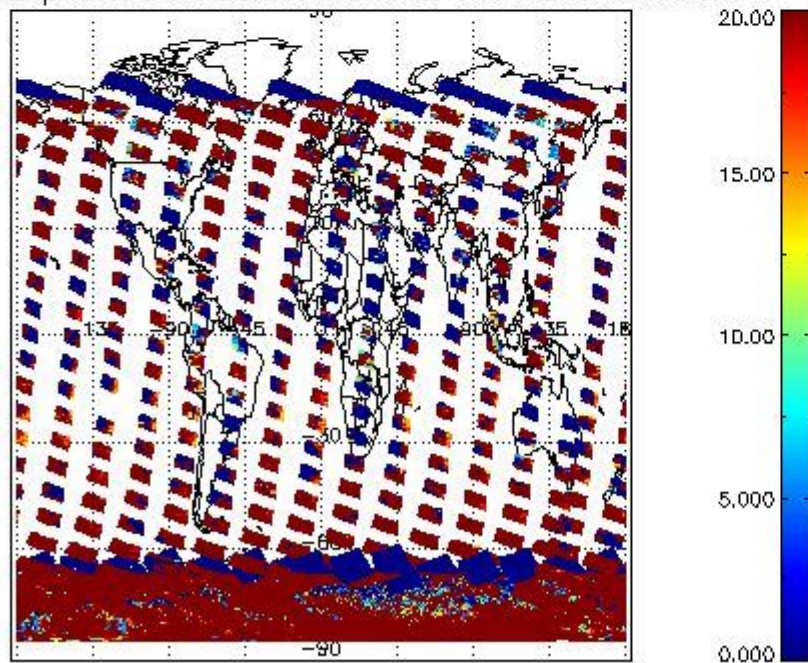
cLopt_depth for 03JAN2012 00:00:00 to 04JAN2012 00:00:00
