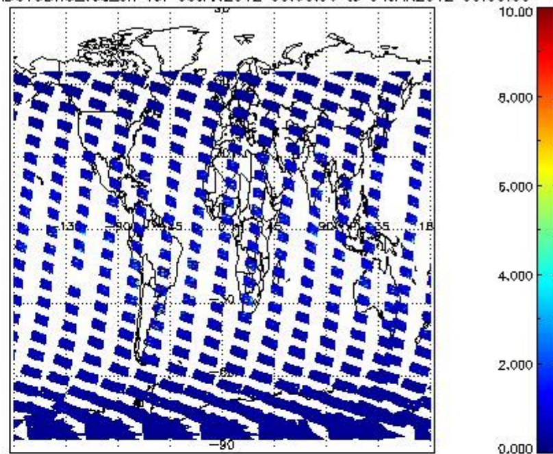
SCIOL2P_NADUV3BRO_vcd_err for 03JAN2012 00:00:00 to 04JAN2012 00:00:00
