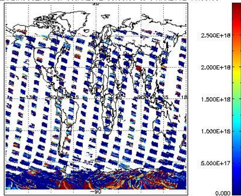
SCIDL2P_NADIR3CO_vcd for 03JAN2012 00:00:00 to 04JAN2012 00:00:00
