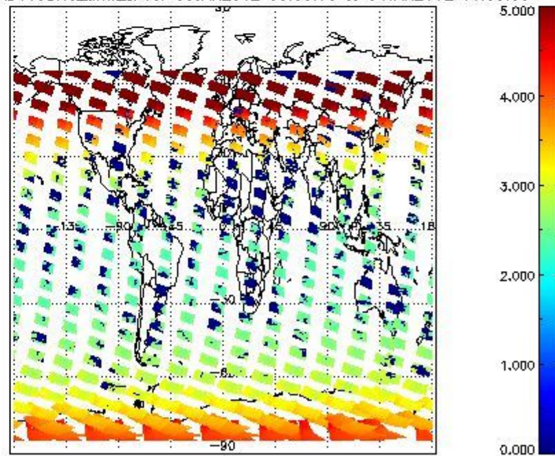
SCIOL2P_NADUV3BRO_amf_cl for 03JAN2012 00:00:00 to 04JAN2012 00:00:00
