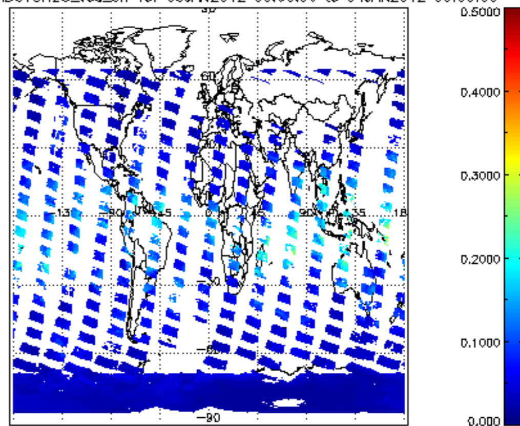
SCIOL2P_NADUV8H20_vcd_err for 03JAN2012 00:00:00 to 04JAN2012 00:00:00
