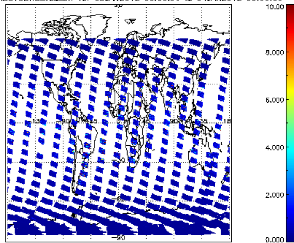
SCIOL2P_NADUV3BRO_vcd_err for 03JAN2012 00:00:00 to 04JAN2012 00:00:00
