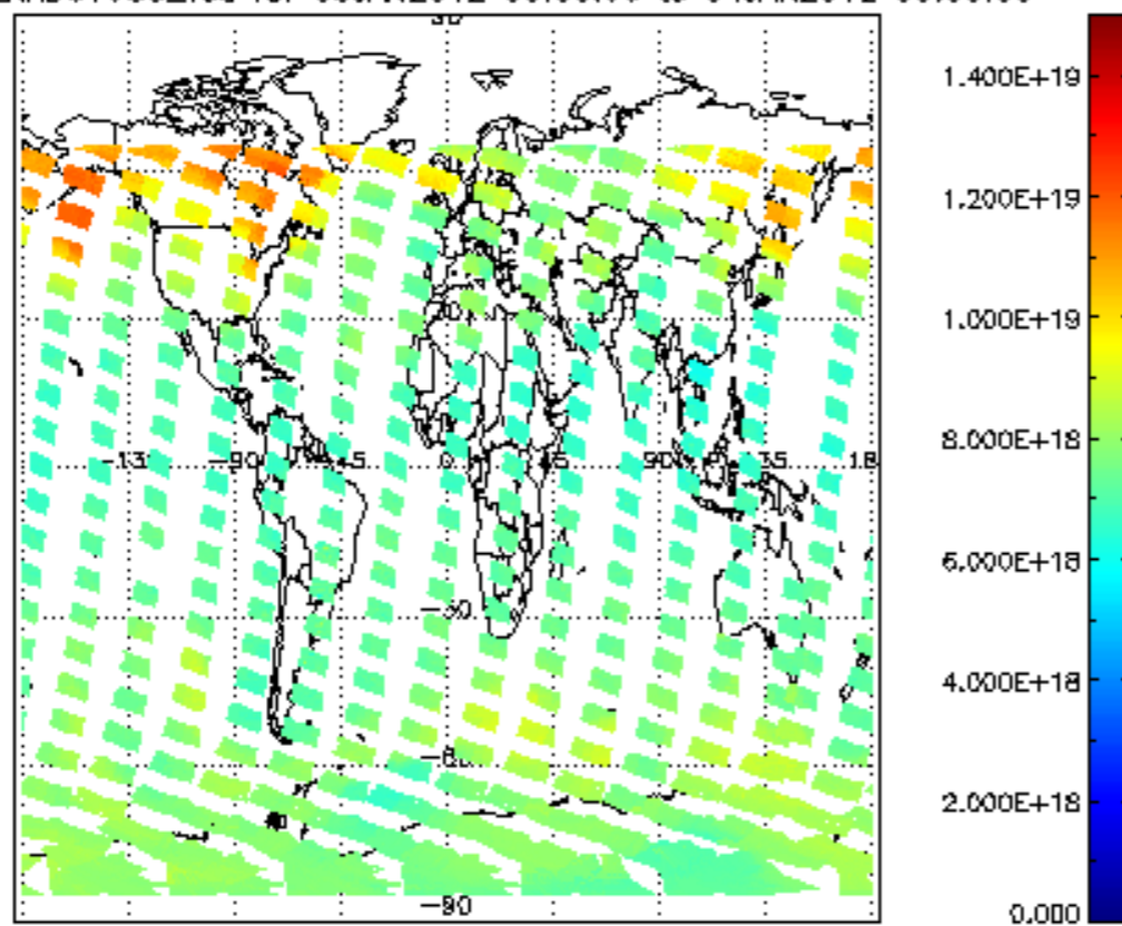
SCIOL2P_NADUV003_vcd for 03JAN2012 00:00:00 to 04JAN2012 00:00:00
