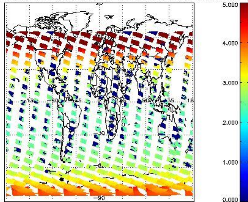
SCIOL2P_NADUV003_amf_cl for 03JAN2012 00:00:00 to 04JAN2012 00:00:00
