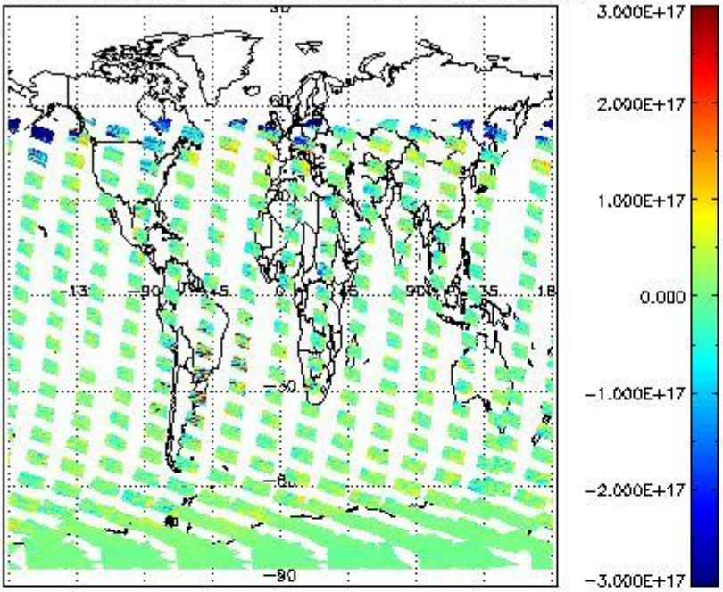
SCIOL2P_NADUV5SO2_vcd for 03JAN2012 00:00:00 to 04JAN2012 00:00:00
