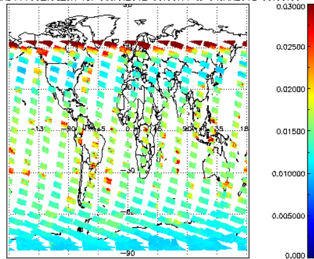
SCIOL2P_NADUV003_vcd_err for 03JAN2012 00:00:00 to 04JAN2012 00:00:00
