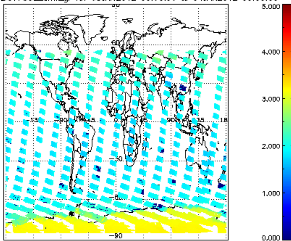
SCIOL2P_NADUV7S02_amf_gr for 03JAN2012 00:00:00 to 04JAN2012 00:00:00
