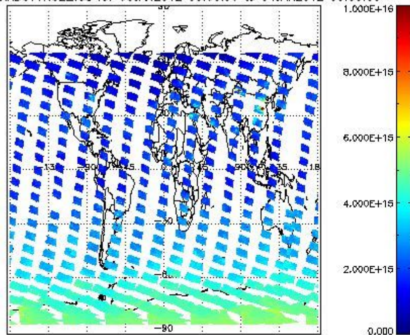
SCIOL2P_NADUV1N02_vcd for 03JAN2012 00:00:00 to 04JAN2012 00:00:00
