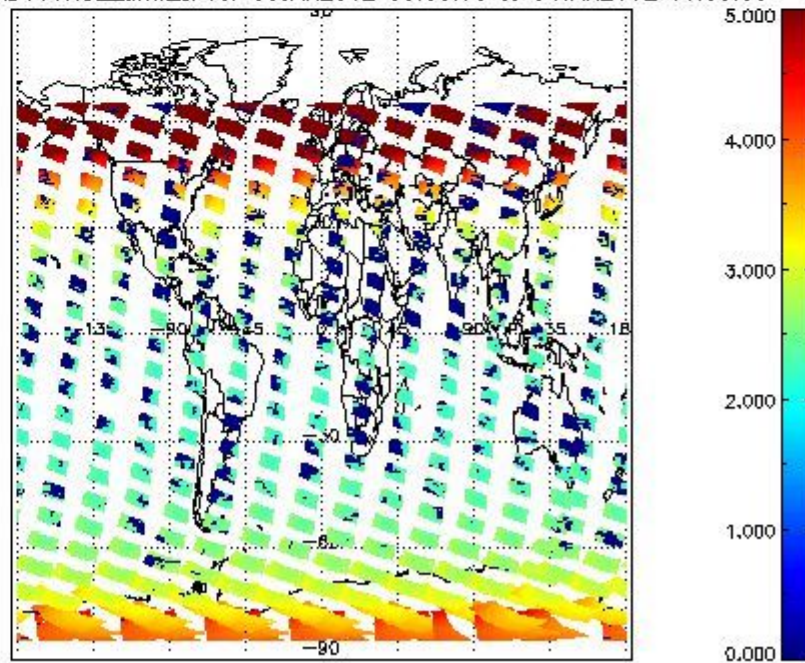
SCIOL2P_NADUV1N02_amf_cl for 03JAN2012 00:00:00 to 04JAN2012 00:00:00
