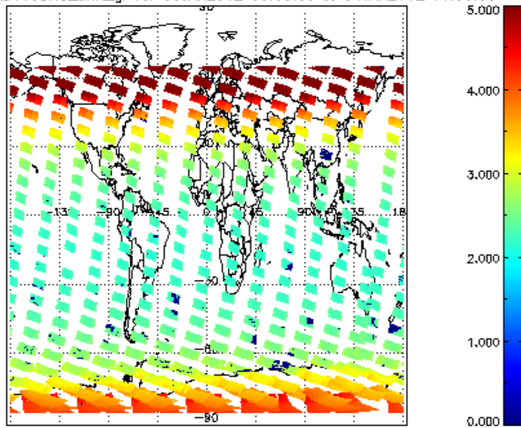
SCIOL2P_NADUV3BRO_amf_gr for 03JAN2012 00:00:00 to 04JAN2012 00:00:00
