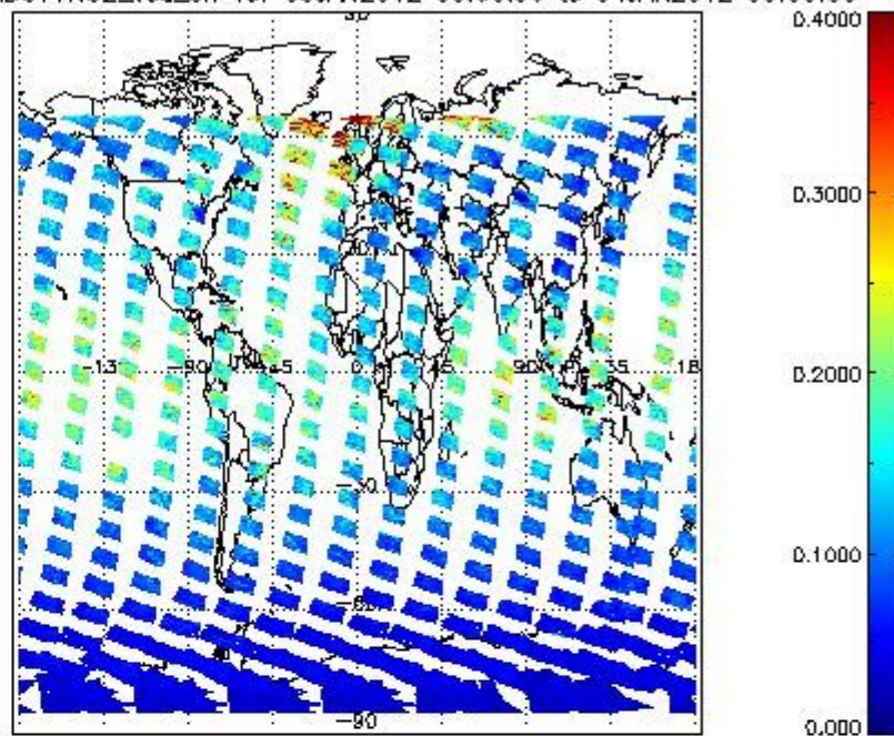
SCIOL2P_NADUV1N02_vcd_err for 03JAN2012 00:00:00 to 04JAN2012 00:00:00
