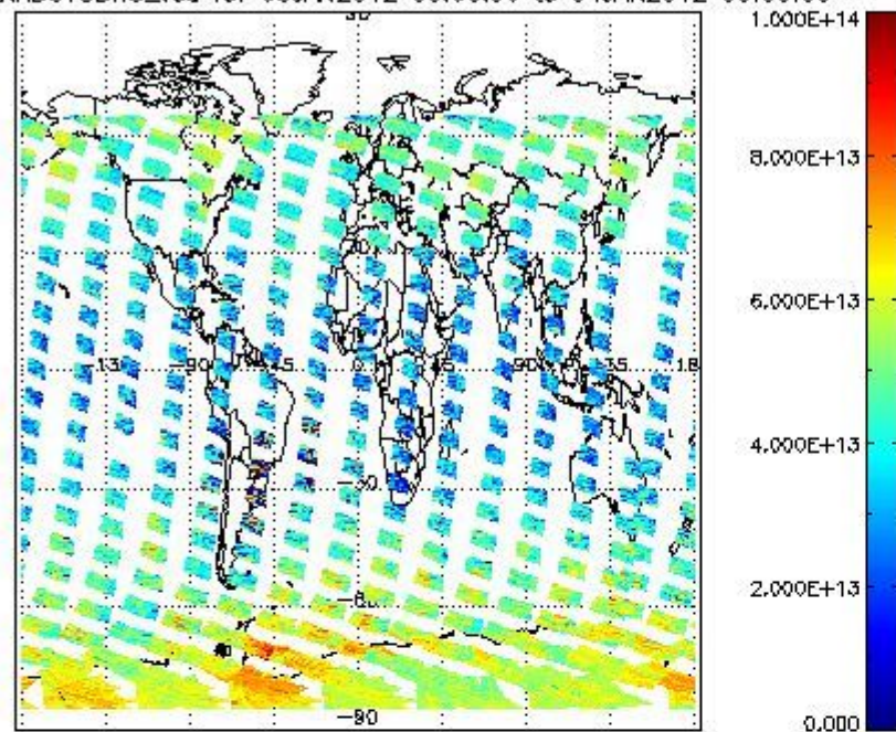
SCIOL2P_NADUV3BRO_vcd for 03JAN2012 00:00:00 to 04JAN2012 00:00:00
