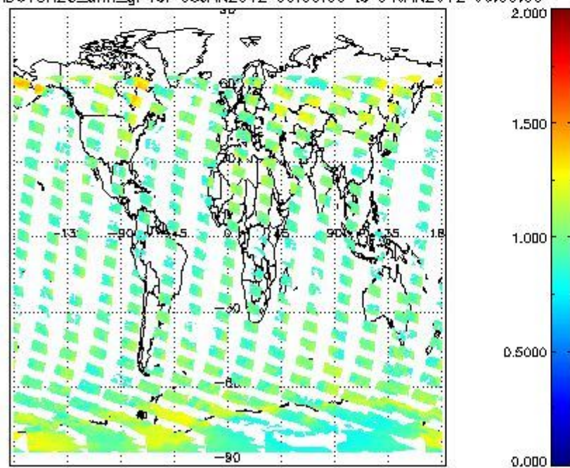
SCIOL2P_NADUV8H20_amf_gr for 03JAN2012 00:00:00 to 04JAN2012 00:00:00
