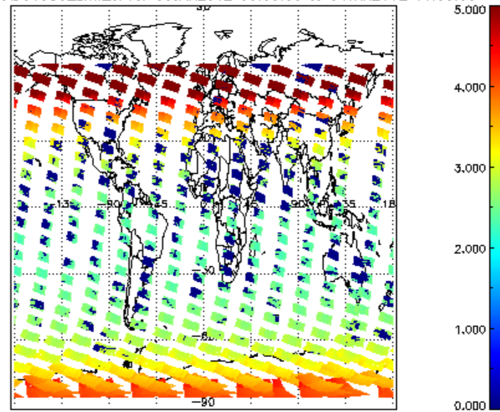
SCIOL2P_NADUV003_amf_cl for 03JAN2012 00:00:00 to 04JAN2012 00:00:00
