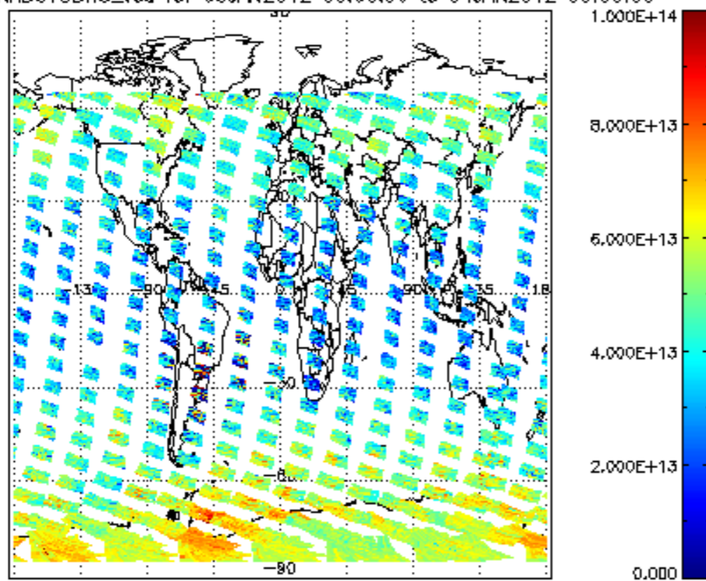
SCIOL2P_NADUV3BRO_vcd for 03JAN2012 00:00:00 to 04JAN2012 00:00:00
