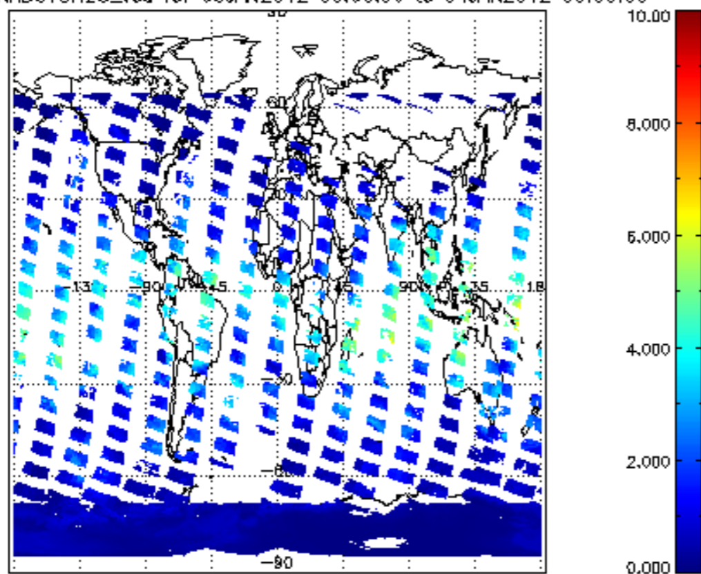
SCIOL2P_NADUV8H20_vcd for 03JAN2012 00:00:00 to 04JAN2012 00:00:00
