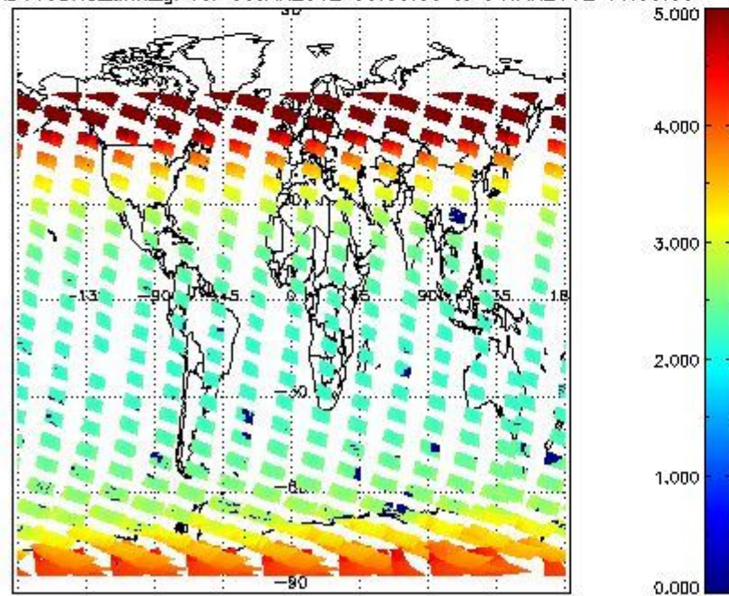
SCIOL2P_NADUV3BRO_amf_gr for 03JAN2012 00:00:00 to 04JAN2012 00:00:00
