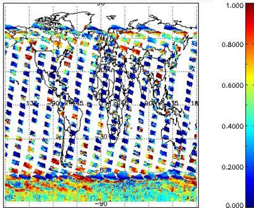
cL_frac for 03JAN2012 00:00:00 to 04JAN2012 00:00:00
