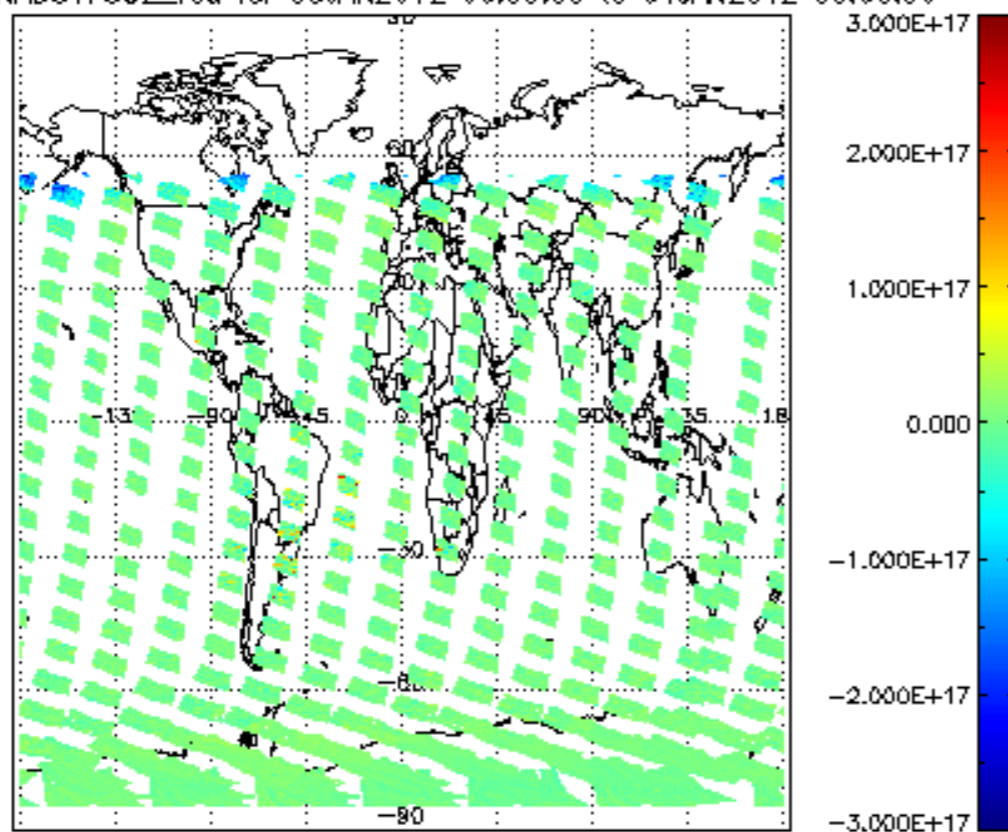
SCIOL2P_NADUV7S02_vcd for 03JAN2012 00:00:00 to 04JAN2012 00:00:00
