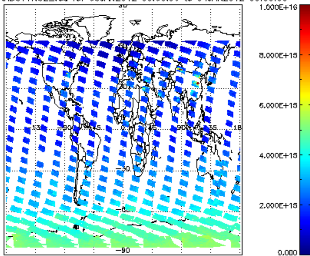
SCIOL2P_NADUV1NO2_vcd for 03JAN2012 00:00:00 to 04JAN2012 00:00:00
