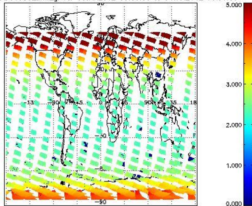
SCIOL2P_NADUV003_amf_gr for 03JAN2012 00:00:00 to 04JAN2012 00:00:00
