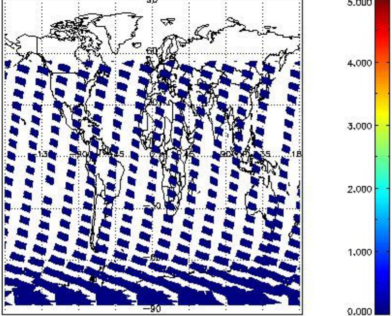
SCIOL2P_NADUV5SO2_amf_cl for 03JAN2012 00:00:00 to 04JAN2012 00:00:00
