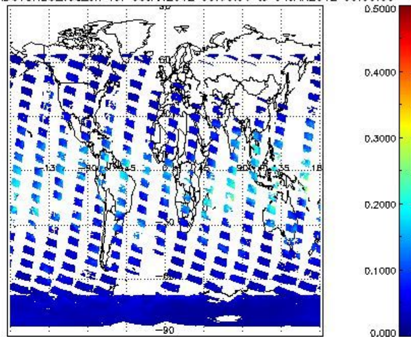
SCIOL2P_NADUV8H20_vcd_err for 03JAN2012 00:00:00 to 04JAN2012 00:00:00
