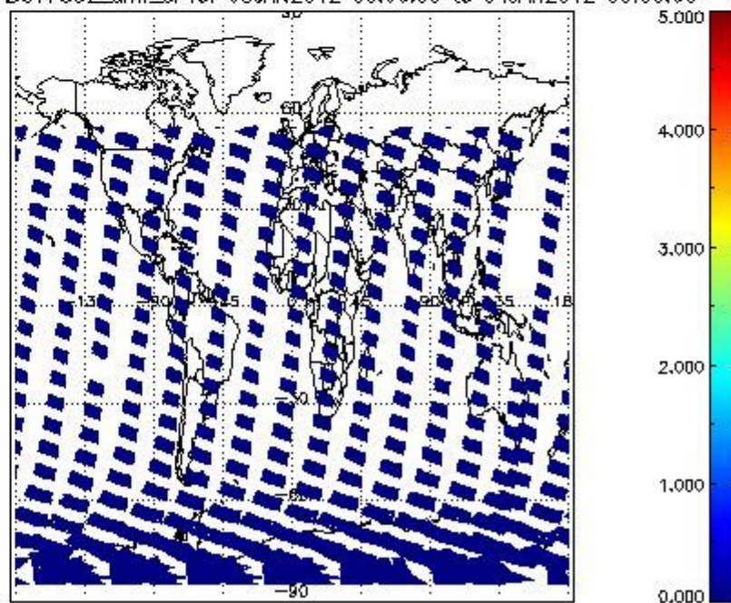
SCIOL2P_NADUV7S02_amf_cl for 03JAN2012 00:00:00 to 04JAN2012 00:00:00
