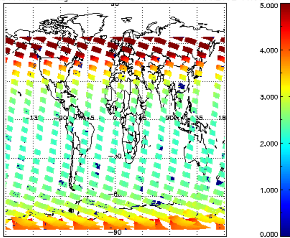
SCIOL2P_NADUV1NO2_amf_gr for 03JAN2012 00:00:00 to 04JAN2012 00:00:00
