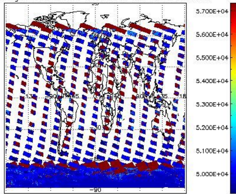
cloud_flags for 03JAN2012 00:00:00 to 04JAN2012 00:00:00
