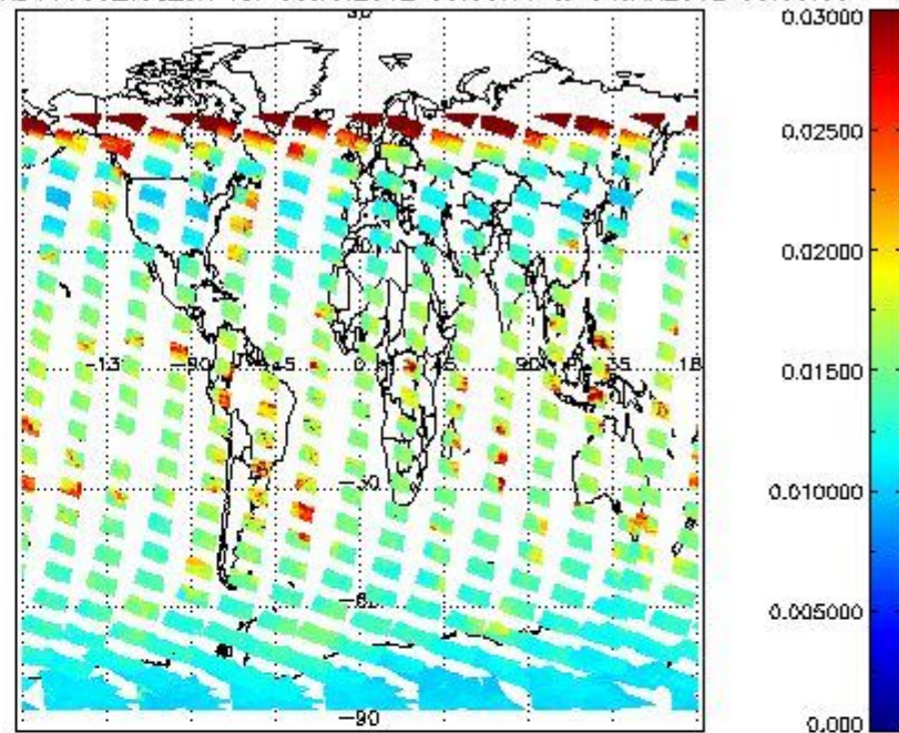
SCIOL2P_NADUV003_vcd_err for 03JAN2012 00:00:00 to 04JAN2012 00:00:00
