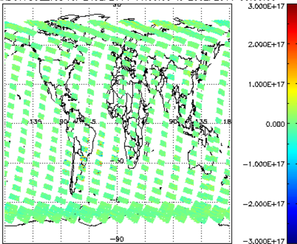
SCIOL2P_NADUV7S02_vcd for 24SEP2011 00:00:00 to 25SEP2011 00:00:00
