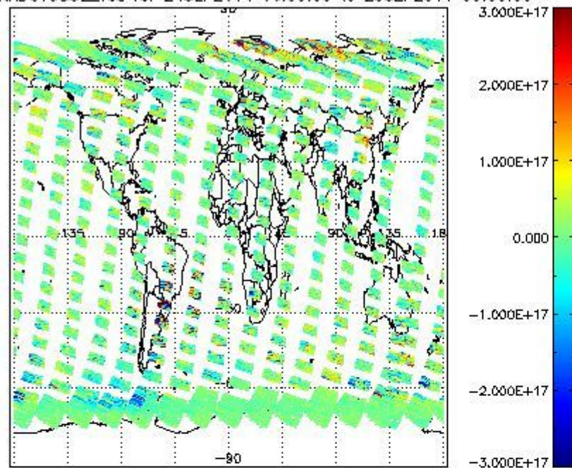
SCIOL2P_NADUV5S02_vcd for 24SEP2011 00:00:00 to 25SEP2011 00:00:00
