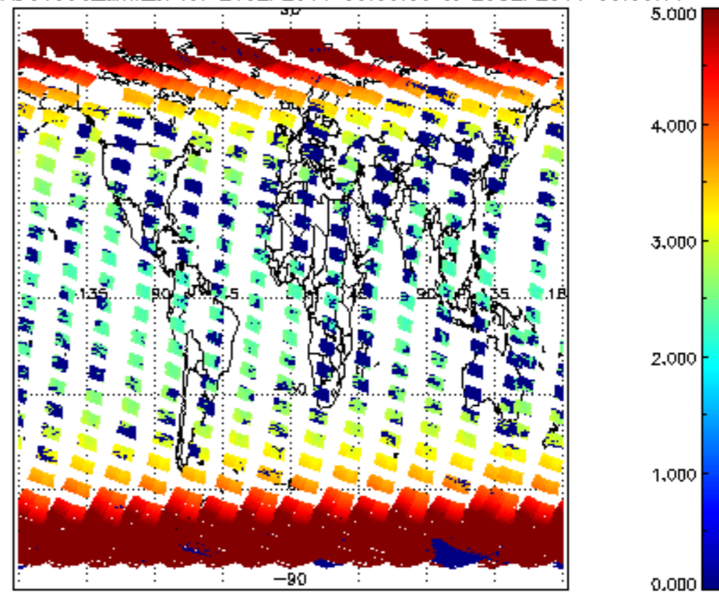
SCIOL2P_NADUV003_amf_cl for 24SEP2011 00:00:00 to 25SEP2011 00:00:00
