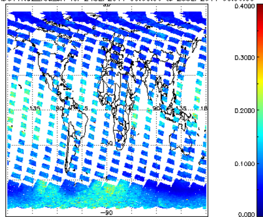
SCIOL2P_NADUV1NO2_vcd_err for 24SEP2011 00:00:00 to 25SEP2011 00:00:00
