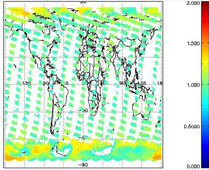
SCIOL2P_NADUV8H2O_arnf_gr for 24SEP2011 00:00:00 to 25SEP2011 00:00:00
