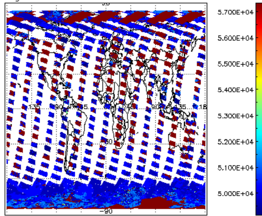
cloud_flags for 24SEP2011 00:00:00 to 25SEP2011 00:00:00
