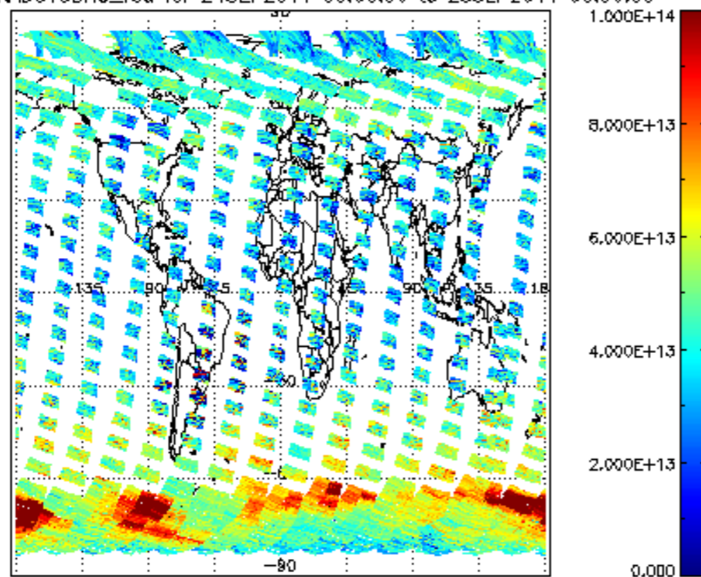
SCIOL2P_NADUV3BRO_vcd for 24SEP2011 00:00:00 to 25SEP2011 00:00:00
