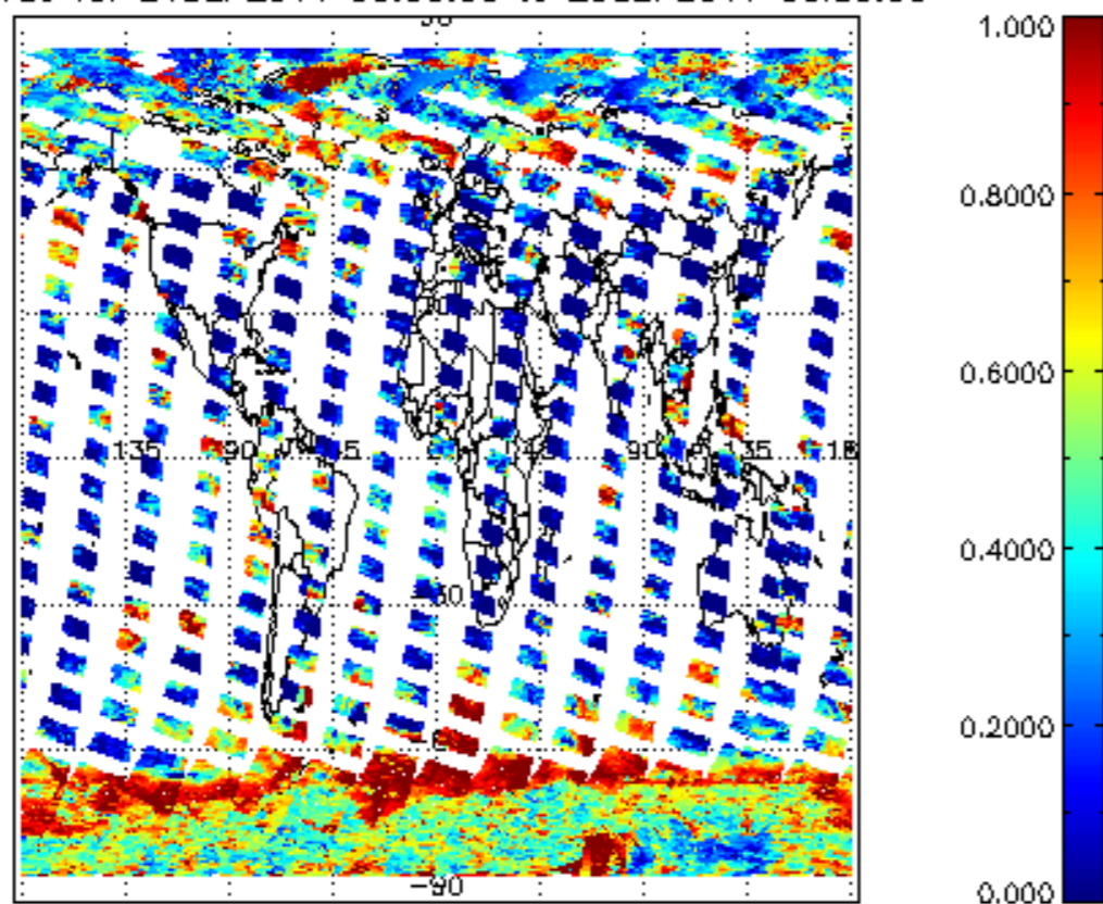
cl_frac for 24SEP2011 00:00:00 to 25SEP2011 00:00:00
