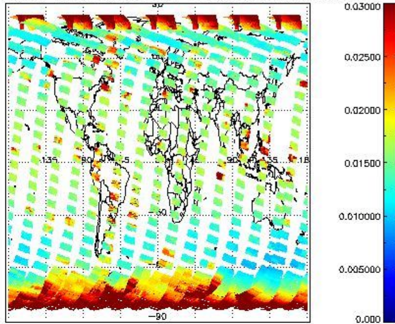
SCIOL2P_NADUV003_vcd_err for 24SEP2011 00:00:00 to 25SEP2011 00:00:00
