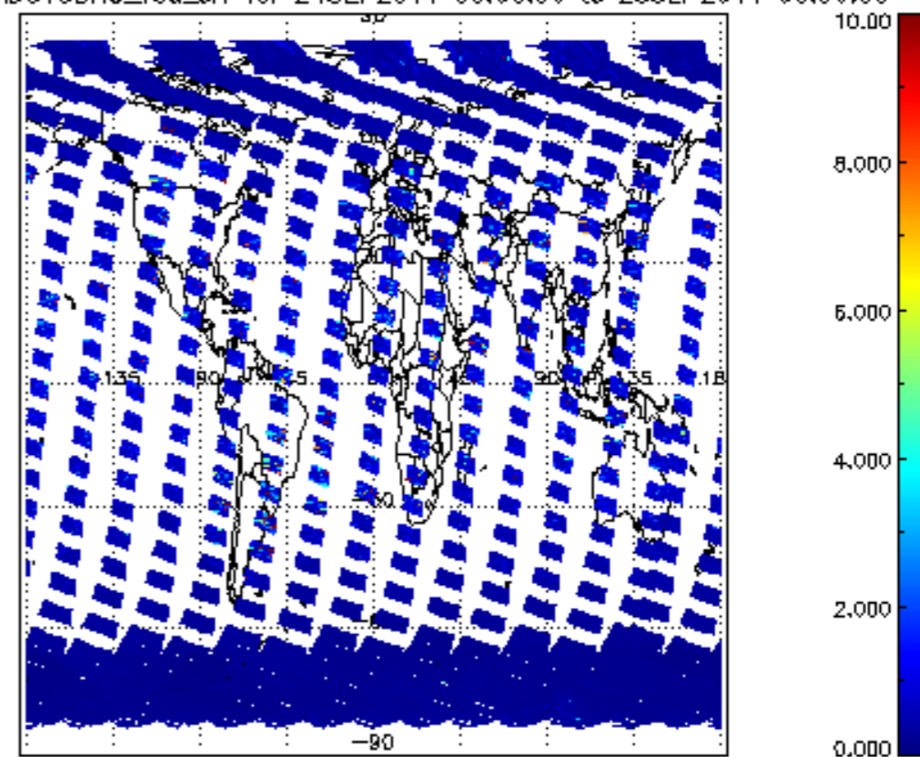
SCIOL2P_NADUV3BRO_vcd_err for 24SEP2011 00:00:00 to 25SEP2011 00:00:00
