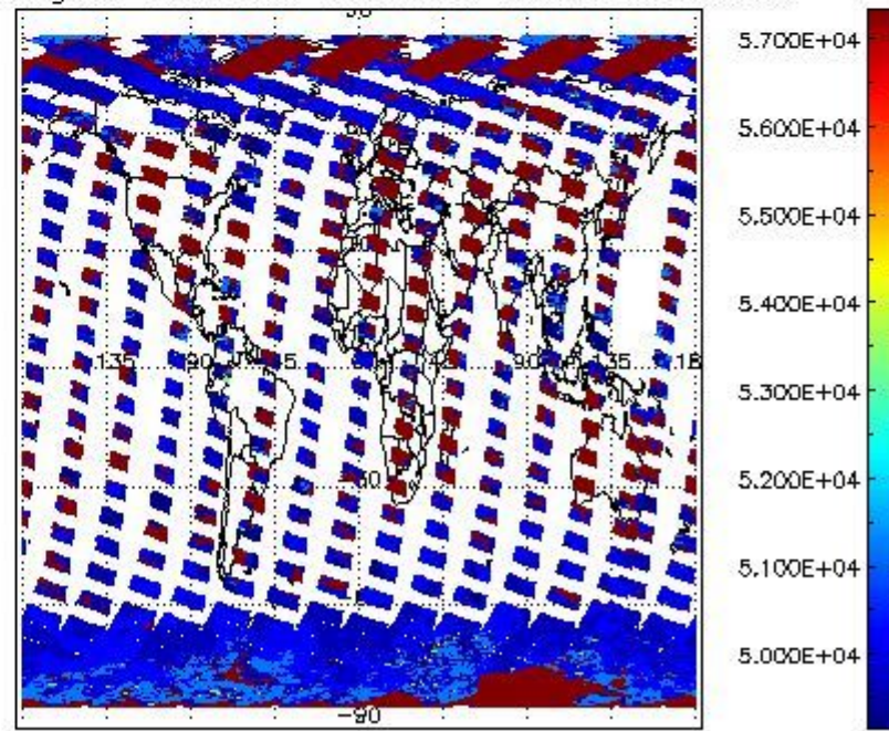
cloud_flags for 24SEP2011 00:00:00 to 25SEP2011 00:00:00
