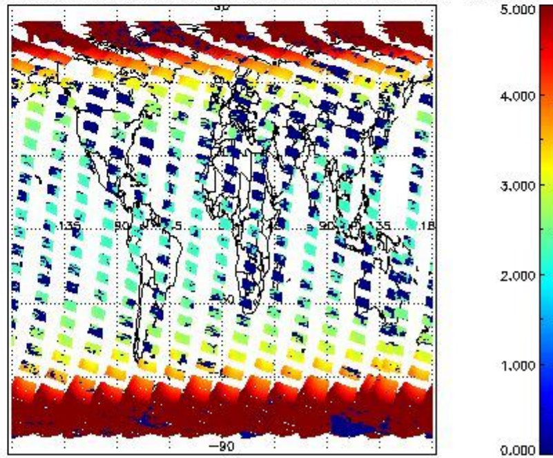
SCIOL2P_NADUV1N02_amf_cl for 24SEP2011 00:00:00 to 25SEP2011 00:00:00
