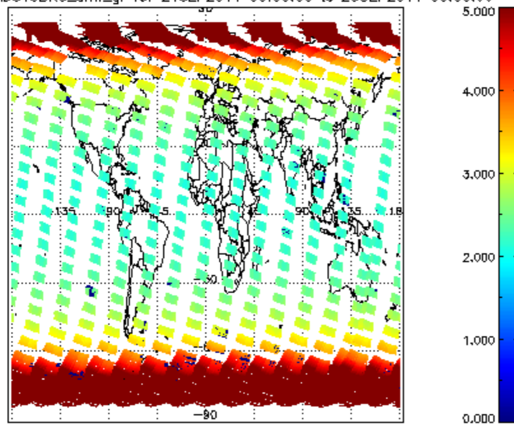
SCIOL2P_NADUV3BRO_amf_gr for 24SEP2011 00:00:00 to 25SEP2011 00:00:00
