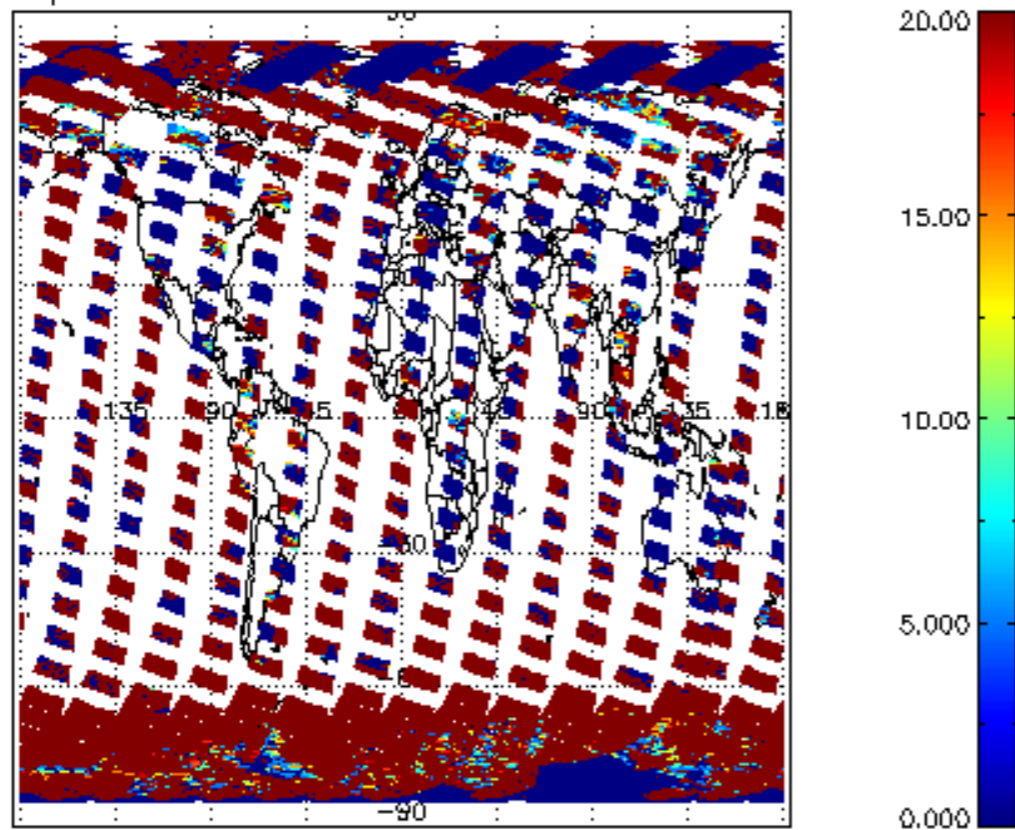
cl_opt_depth for 24SEP2011 00:00:00 to 25SEP2011 00:00:00
