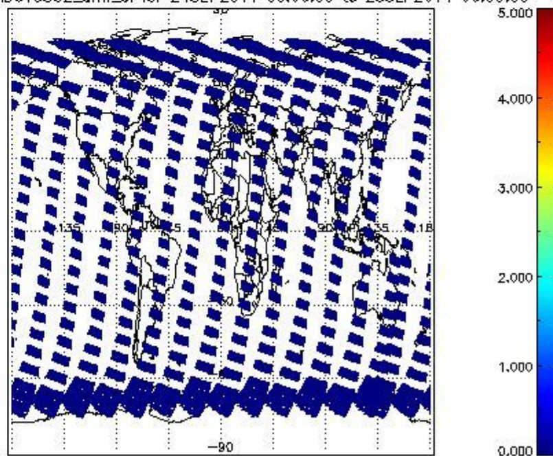
SCIOL2P_NADUV5S02_amf_cl for 24SEP2011 00:00:00 to 25SEP2011 00:00:00
