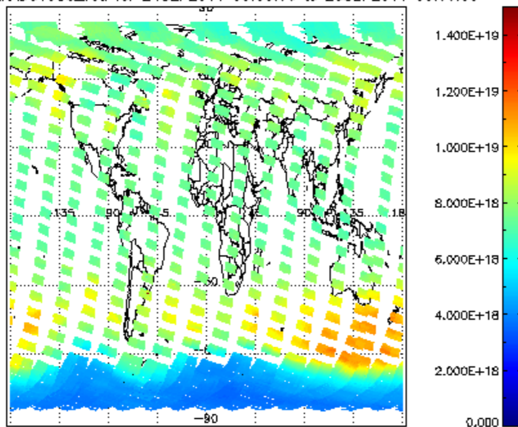
SCIOL2P_NADUV003_vcd for 24SEP2011 00:00:00 to 25SEP2011 00:00:00
