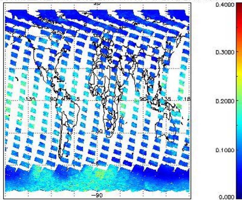
SCIOL2P_NADUV1N02_vcd_err for 24SEP2011 00:00:00 to 25SEP2011 00:00:00
