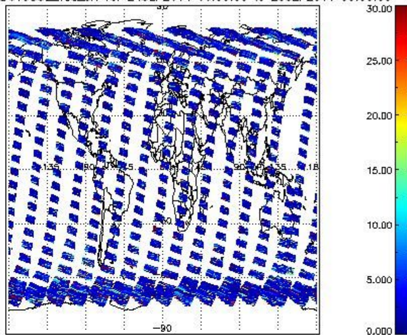
SCIOL2P_NADUV5S02_vcd_err for 24SEP2011 00:00:00 to 25SEP2011 00:00:00
