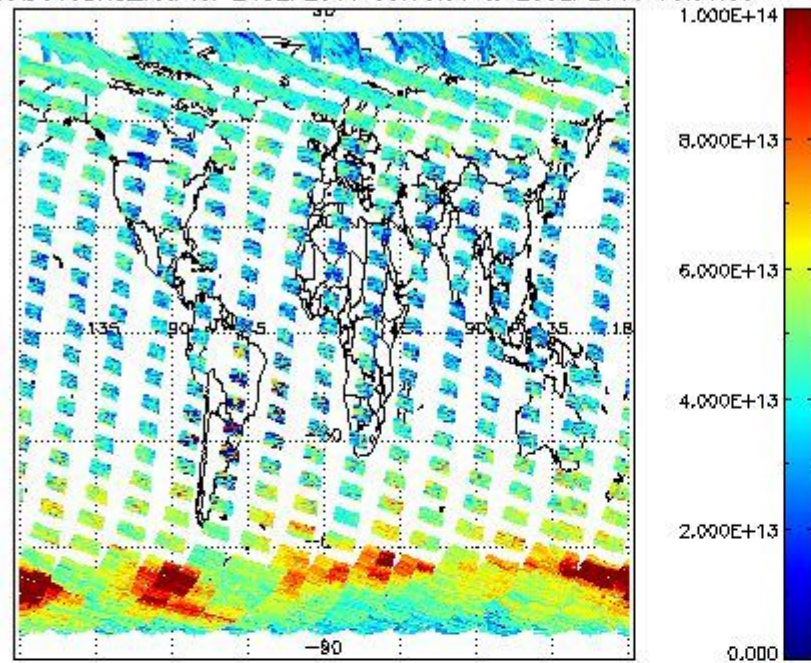
SCIOL2P_NADUV3BRO_vcd for 24SEP2011 00:00:00 to 25SEP2011 00:00:00
