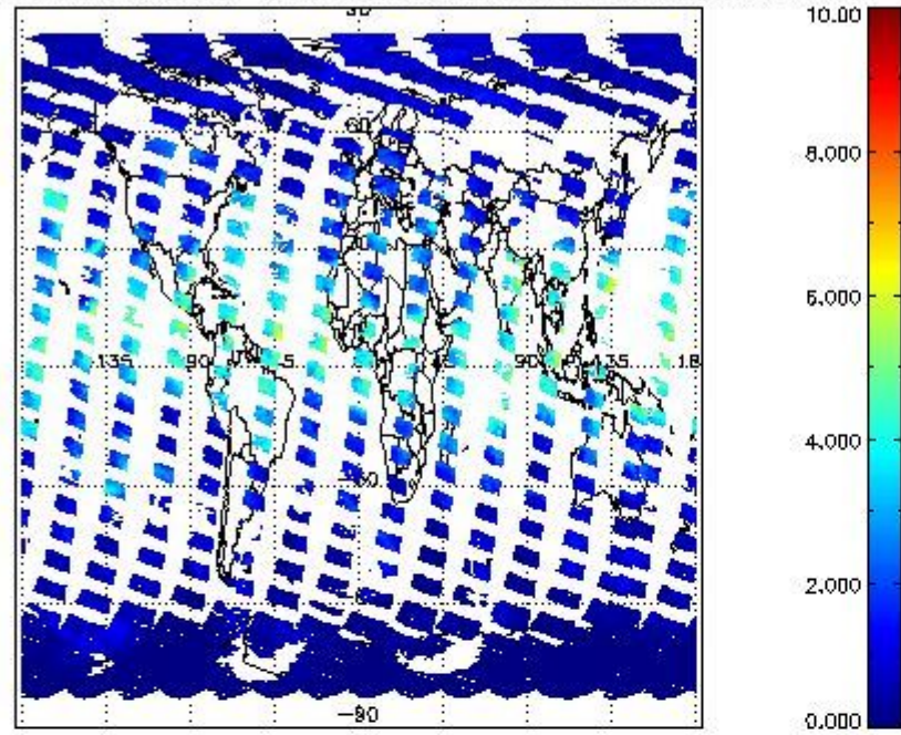
SCIOL2P_NADUV8H2O_vcd for 24SEP2011 00:00:00 to 25SEP2011 00:00:00
