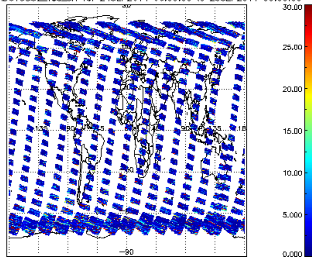
SCIOL2P_NADUV5S02_vcd_err for 24SEP2011 00:00:00 to 25SEP2011 00:00:00
