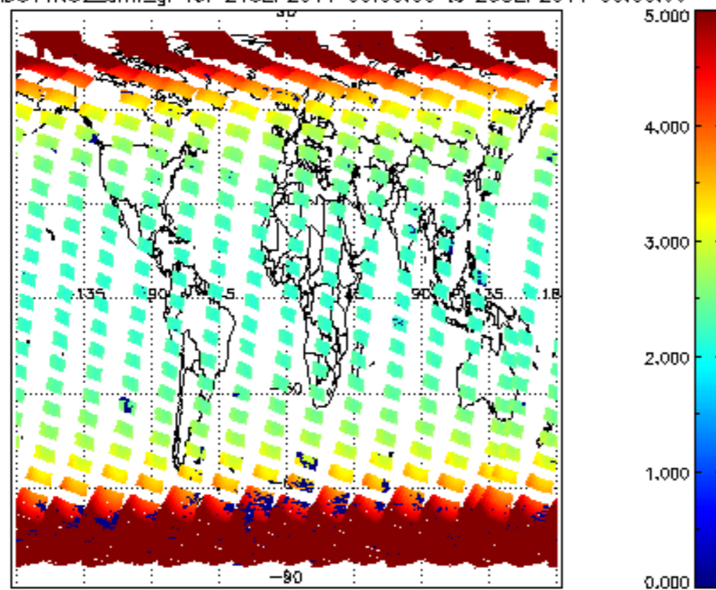
SCIOL2P_NADUV1NO2_amf_gr for 24SEP2011 00:00:00 to 25SEP2011 00:00:00
