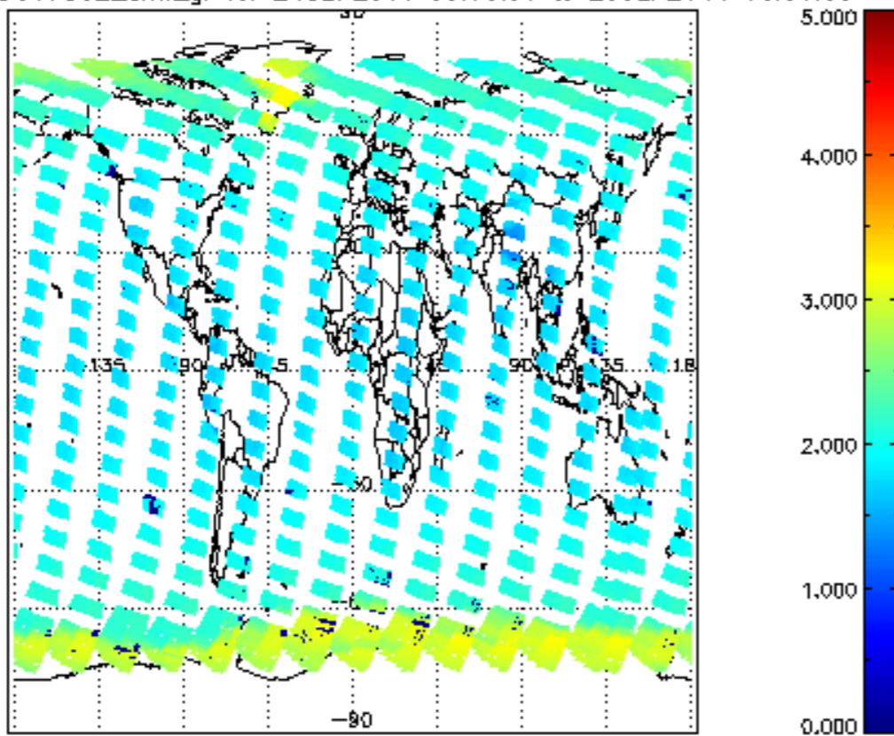
SCIOL2P_NADUV7S02_amf_gr for 24SEP2011 00:00:00 to 25SEP2011 00:00:00
