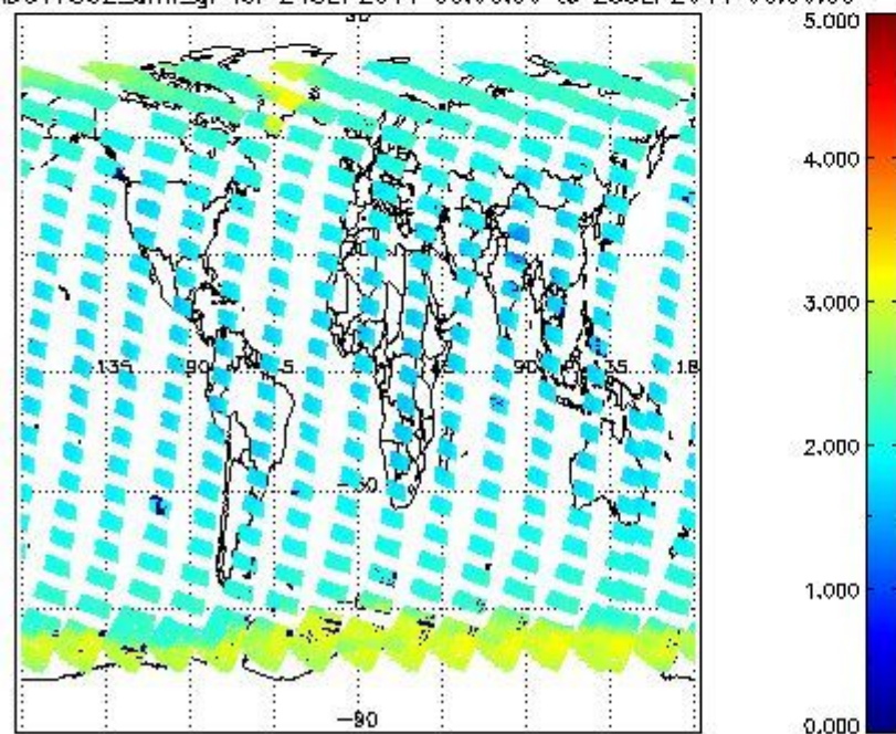
SCIOL2P_NADUV7S02_amf_gr for 24SEP2011 00:00:00 to 25SEP2011 00:00:00
