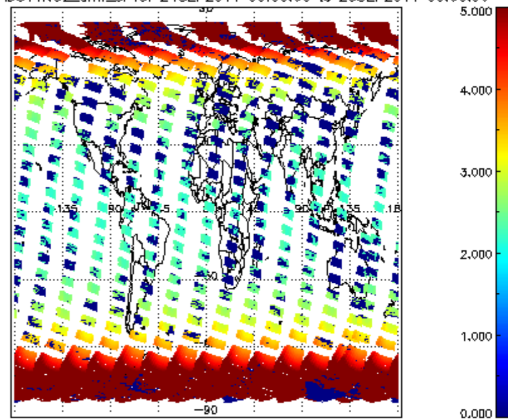
SCIOL2P_NADUV1NO2_amf_sl for 24SEP2011 00:00:00 to 25SEP2011 00:00:00
