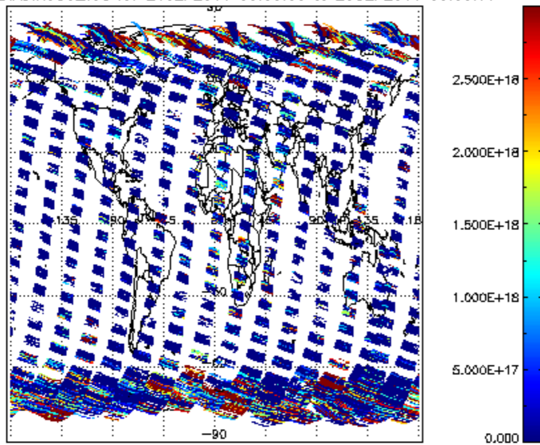
SCIOL2P_NADIR3CO_vcd for 24SEP2011 00:00:00 to 25SEP2011 00:00:00
