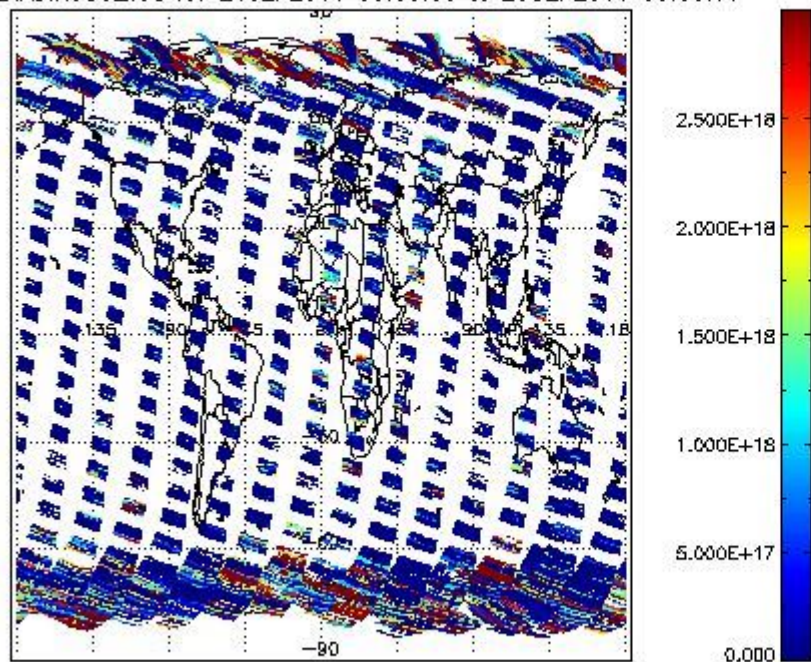
SCIOL2P_NADIR3CO_vcd for 24SEP2011 00:00:00 to 25SEP2011 00:00:00
