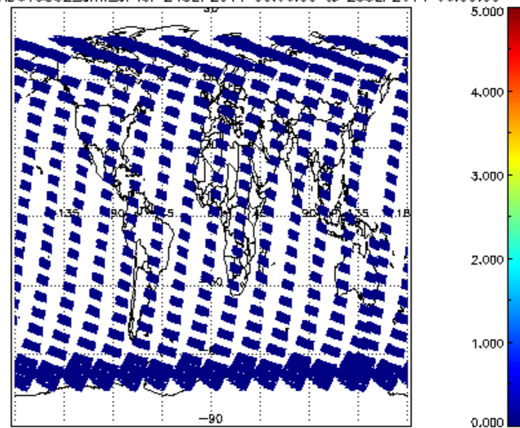
SCIOL2P_NADUV5S02_amf_cl for 24SEP2011 00:00:00 to 25SEP2011 00:00:00
