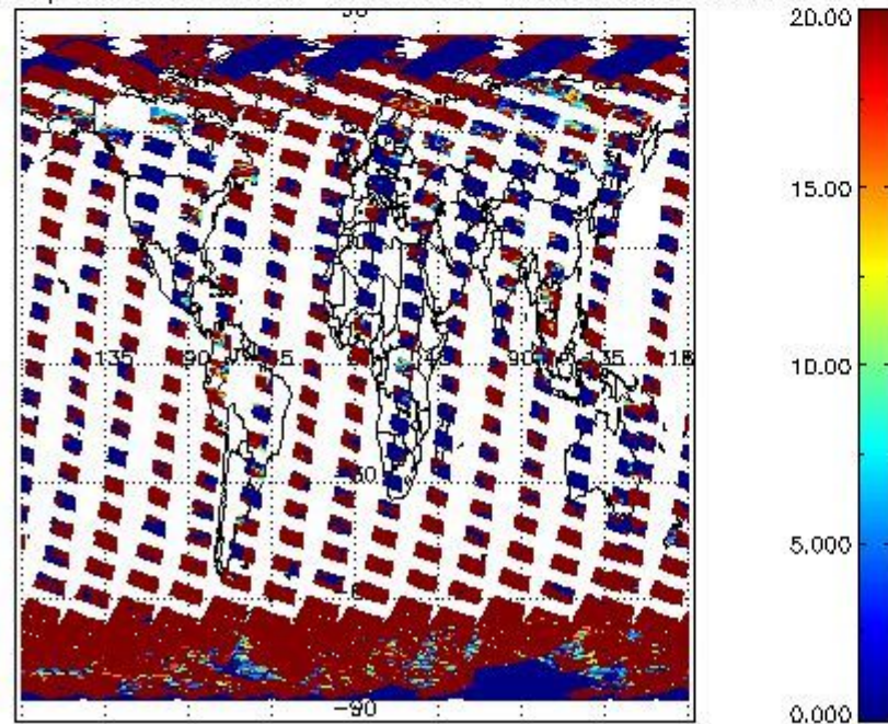
cL_opt_depth for 24SEP2011 00:00:00 to 25SEP2011 00:00:00
