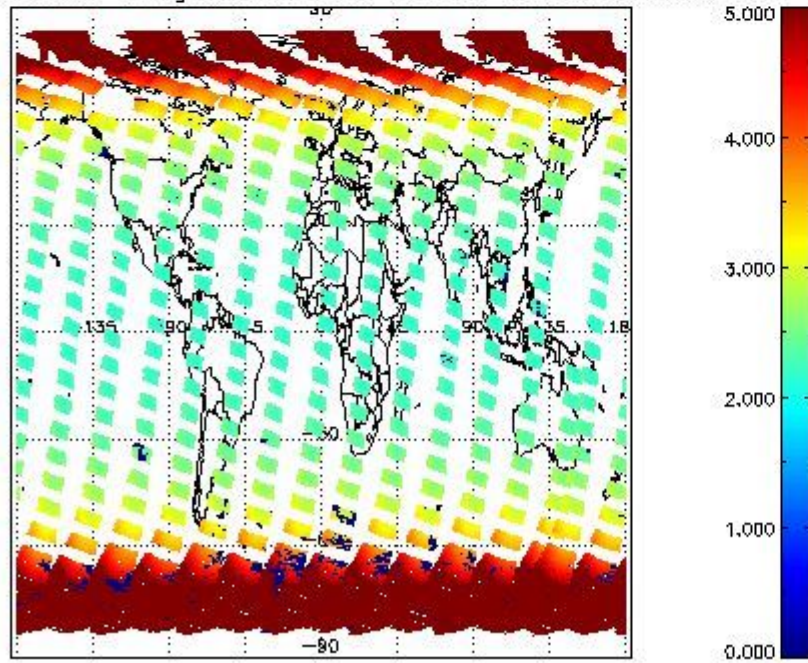
SCIOL2P_NADUV1N02_amf_gr for 24SEP2011 00:00:00 to 25SEP2011 00:00:00
