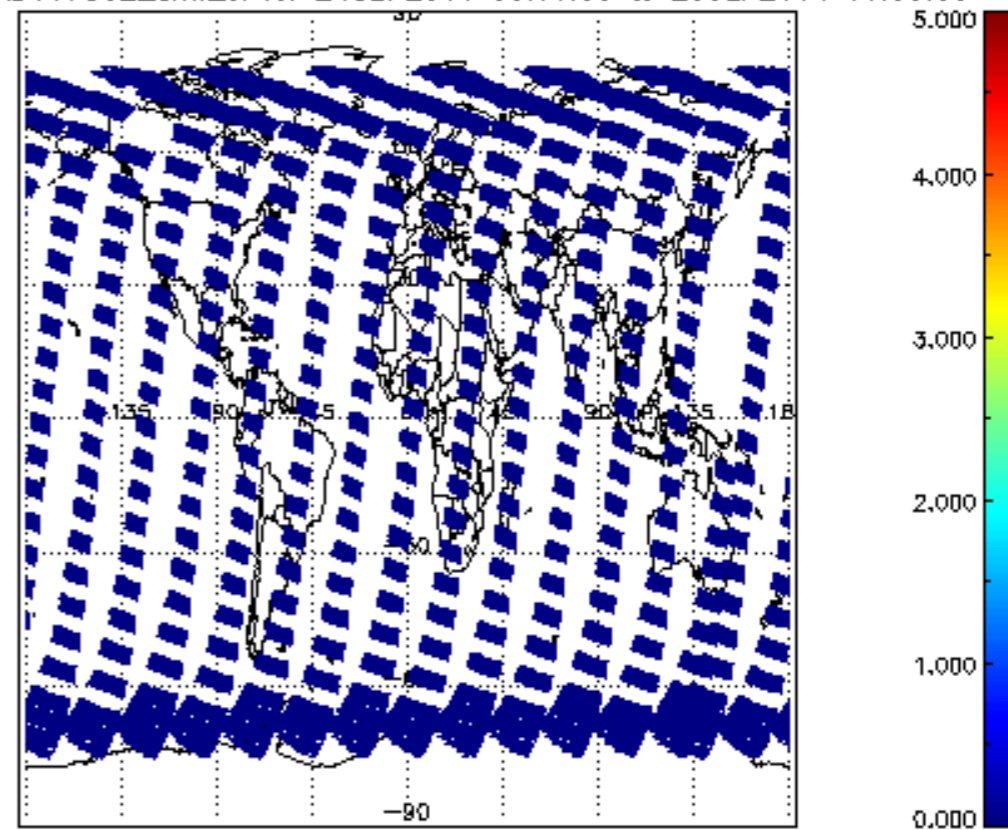
SCIOL2P_NADUV7S02_amf_cl for 24SEP2011 00:00:00 to 25SEP2011 00:00:00
