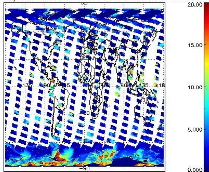
cL_top_height for 24SEP2011 00:00:00 to 25SEP2011 00:00:00
