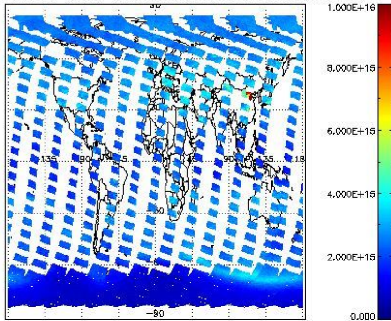
SCIOL2P_NADUV1N02_vcd for 24SEP2011 00:00:00 to 25SEP2011 00:00:00
