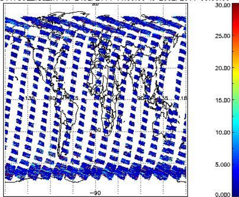
SCIOL2P_NADUV7S02_vcd_err for 24SEP2011 00:00:00 to 25SEP2011 00:00:00
