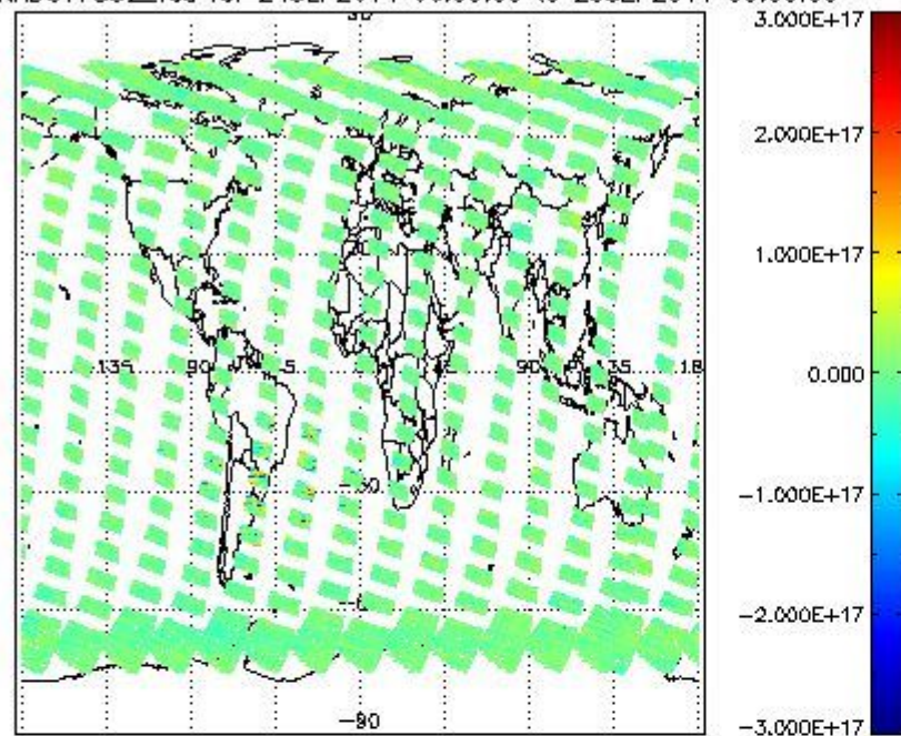
SCIOL2P_NADUV7S02_vcd for 24SEP2011 00:00:00 to 25SEP2011 00:00:00
