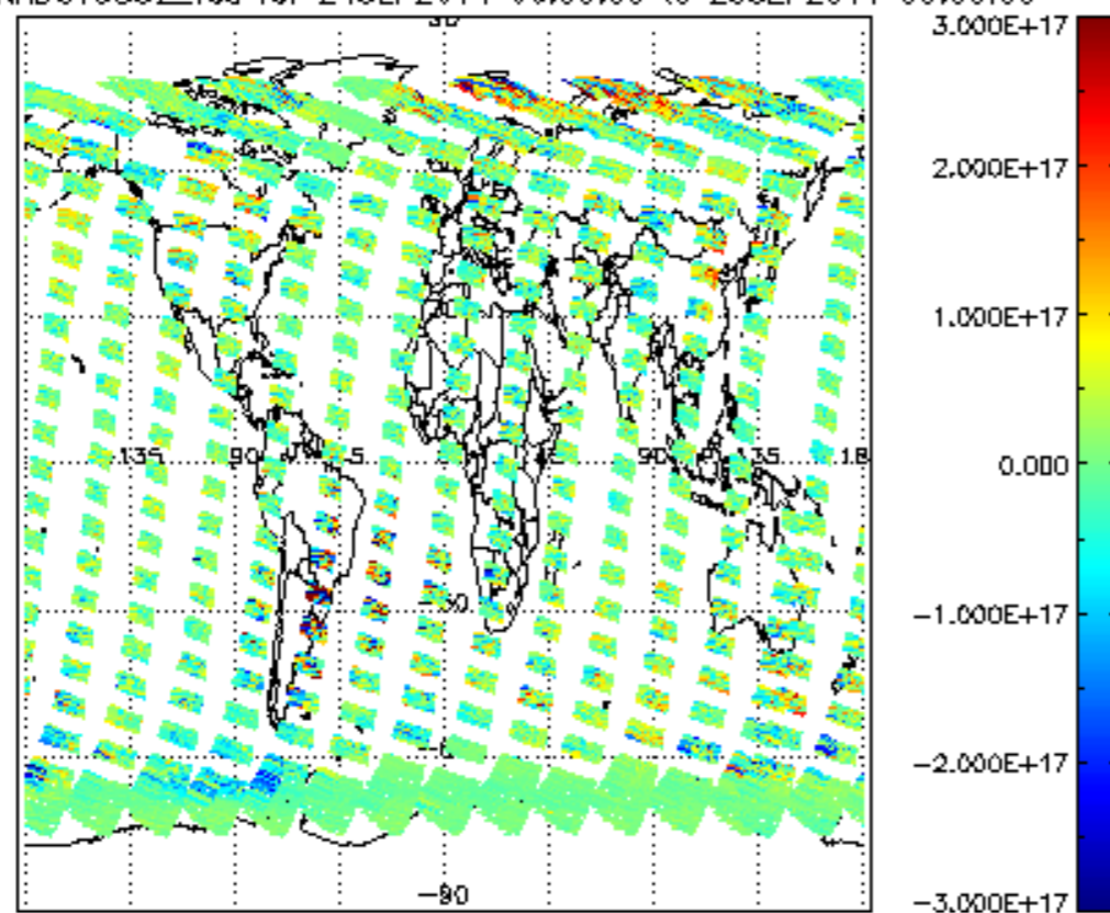
SCIOL2P_NADUV5S02_vcd for 24SEP2011 00:00:00 to 25SEP2011 00:00:00
