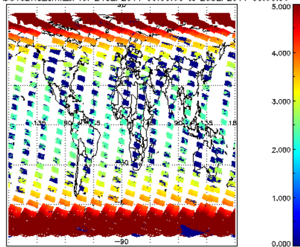
SCIOL2P_NADUV3BRO_amf_sl for 24SEP2011 00:00:00 to 25SEP2011 00:00:00
