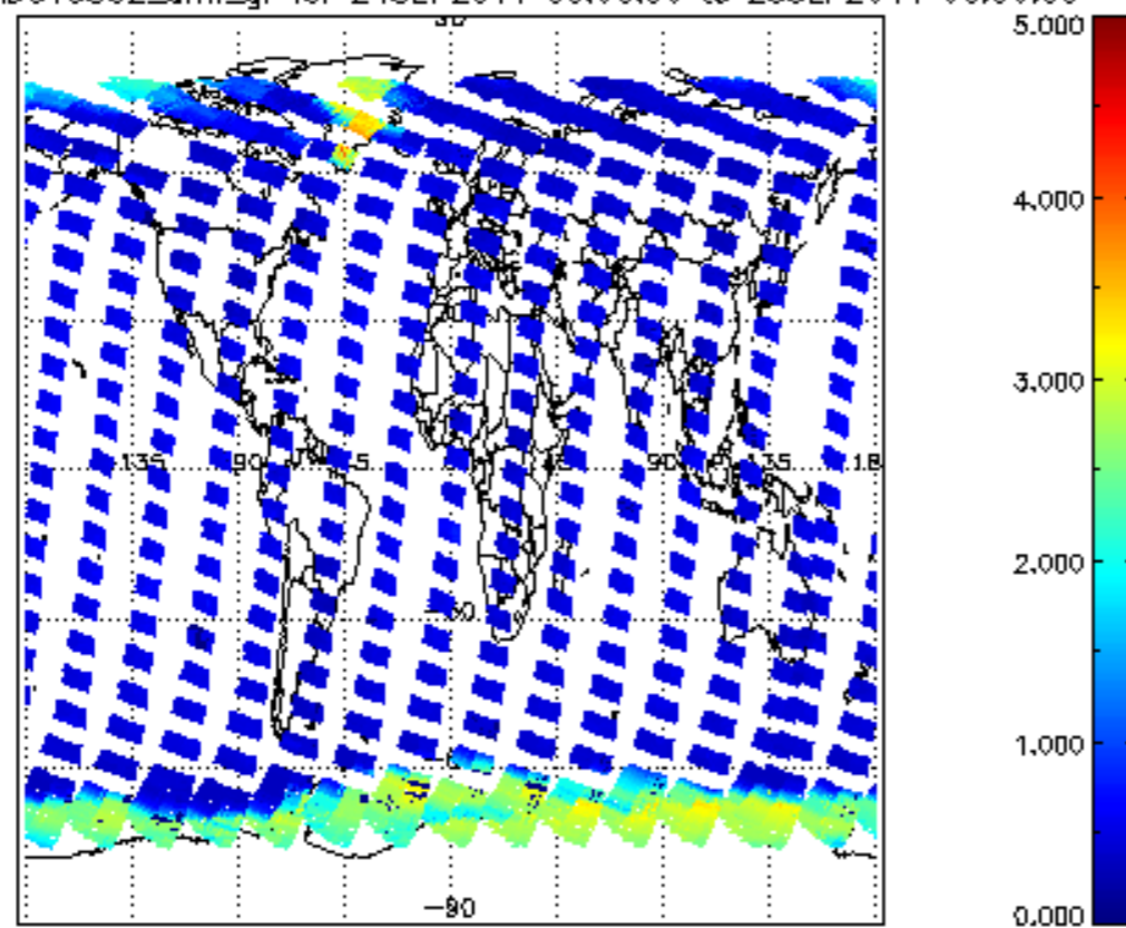
SCIOL2P_NADUV5S02_amf_gr for 24SEP2011 00:00:00 to 25SEP2011 00:00:00
