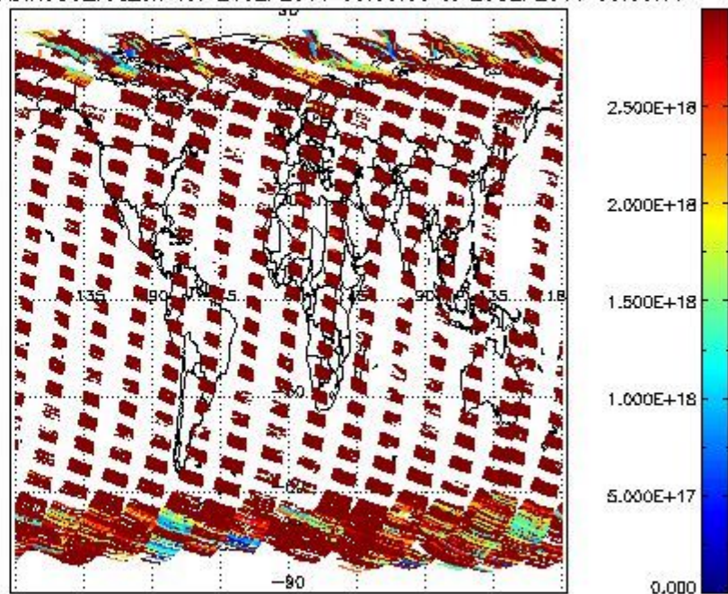
SCIOL2P_NADIR3CO_vcd_err for 24SEP2011 00:00:00 to 25SEP2011 00:00:00
