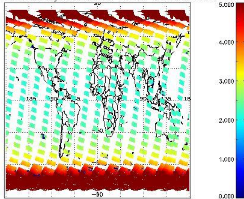
SCIOL2P_NADUV3BRO_amf_gr for 24SEP2011 00:00:00 to 25SEP2011 00:00:00
