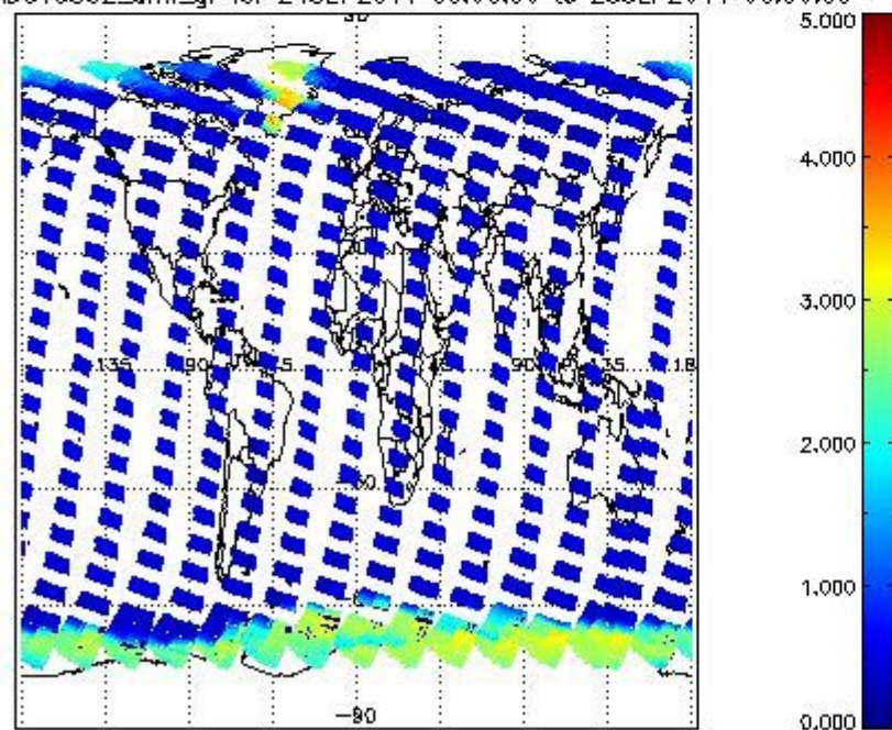
SCIOL2P_NADUV5S02_amf_gr for 24SEP2011 00:00:00 to 25SEP2011 00:00:00
