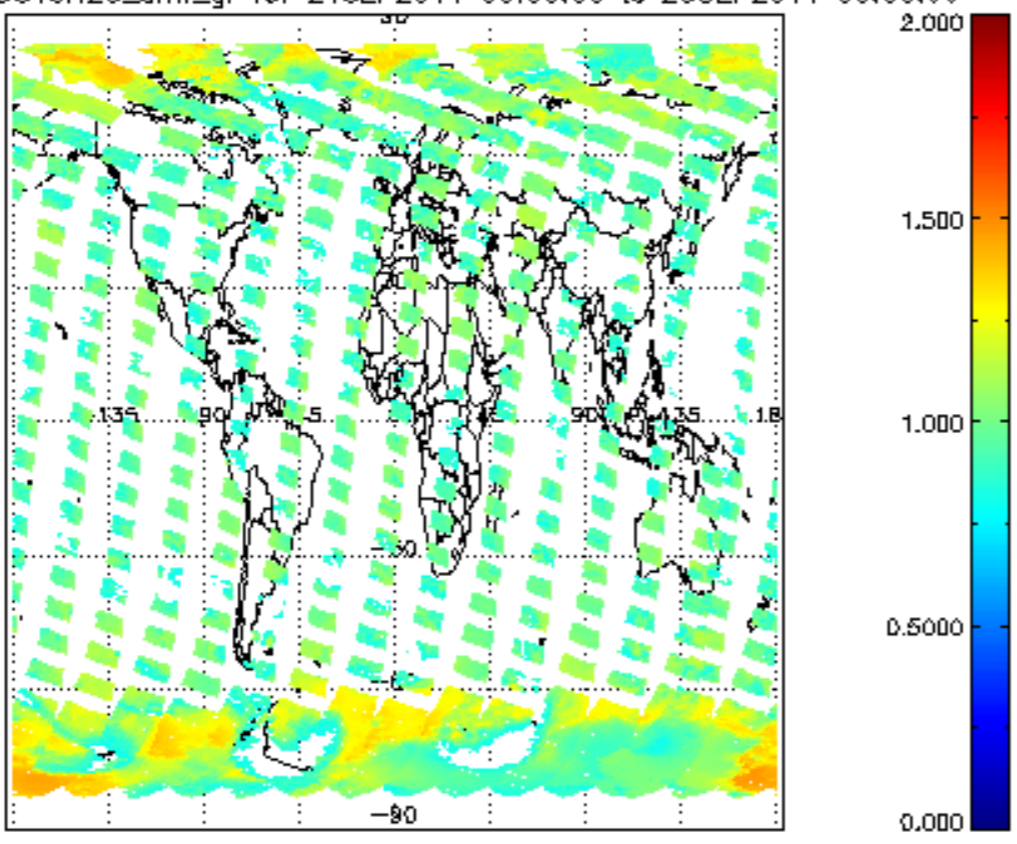
SCIOL2P_NADUV8H20_amf_gr for 24SEP2011 00:00:00 to 25SEP2011 00:00:00
