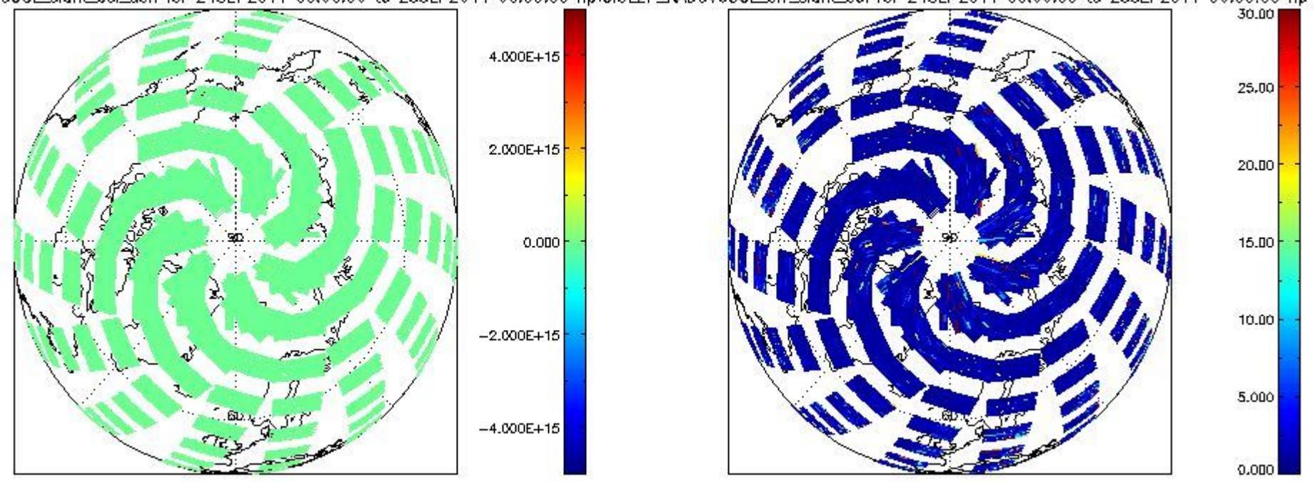
CIOL2P_NADUV60CLslant_col_den for 24SEP2011 00:00:00 to 25SEP2011 00:00:00 np; CIOL2P_NADUV60CLerr_slant_col for 24SEP2011 00:00:00 to 25SEP2011 00:00:00 np
