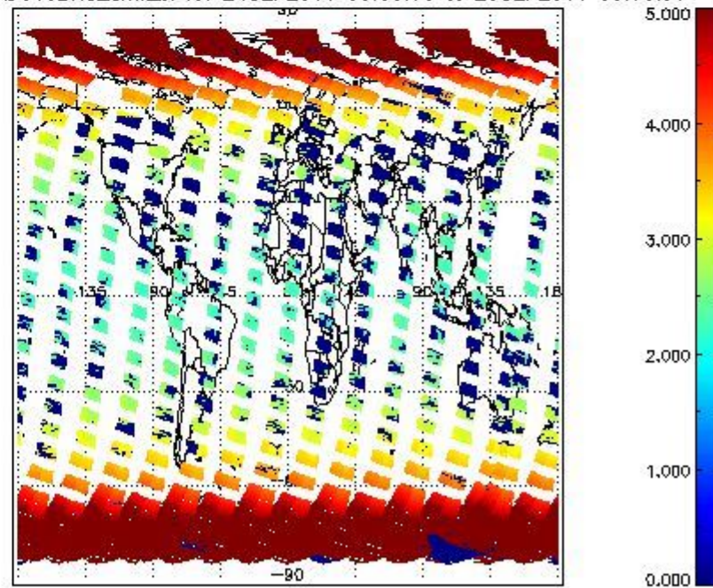
SCIOL2P_NADUV3BRO_amf_cl for 24SEP2011 00:00:00 to 25SEP2011 00:00:00
