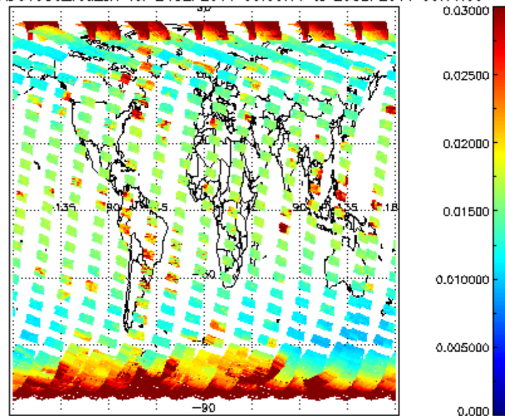
SCIOL2P_NADUV003_vcd_err for 24SEP2011 00:00:00 to 25SEP2011 00:00:00
