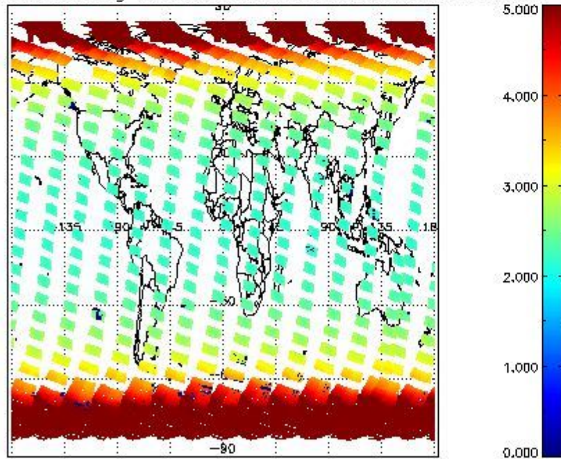
SCIOL2P_NADUV003_amf_gr for 24SEP2011 00:00:00 to 25SEP2011 00:00:00
