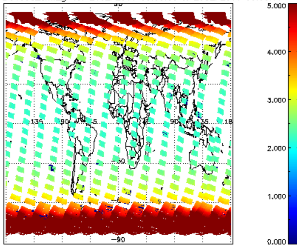
SCIOL2P_NADUV003_amf_gr for 24SEP2011 00:00:00 to 25SEP2011 00:00:00
