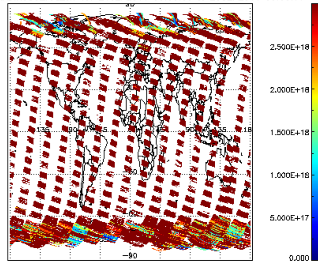
SCIOL2P_NADIR3CO_vcd_err for 24SEP2011 00:00:00 to 25SEP2011 00:00:00
