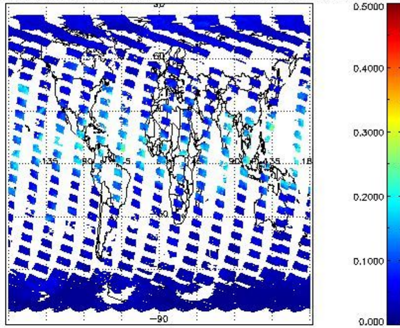
SCIOL2P_NADUV8H2O_vcd_err for 24SEP2011 00:00:00 to 25SEP2011 00:00:00
