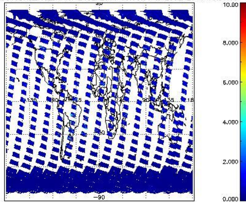
SCIOL2P_NADUV3BRO_vcd_err for 24SEP2011 00:00:00 to 25SEP2011 00:00:00
