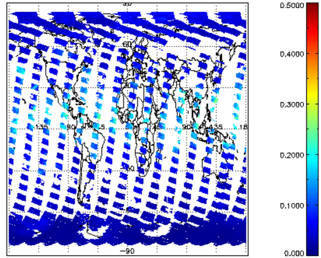
SCIOL2P_NADUV8H20_vcd_err for 24SEP2011 00:00:00 to 25SEP2011 00:00:00
