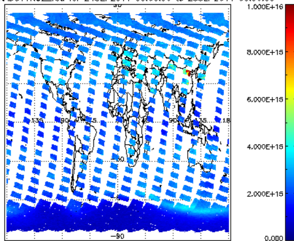
SCIOL2P_NADUV1NO2_vcd for 24SEP2011 00:00:00 to 25SEP2011 00:00:00
