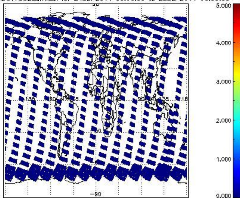
SCIOL2P_NADUV7S02_amf_cl for 24SEP2011 00:00:00 to 25SEP2011 00:00:00
