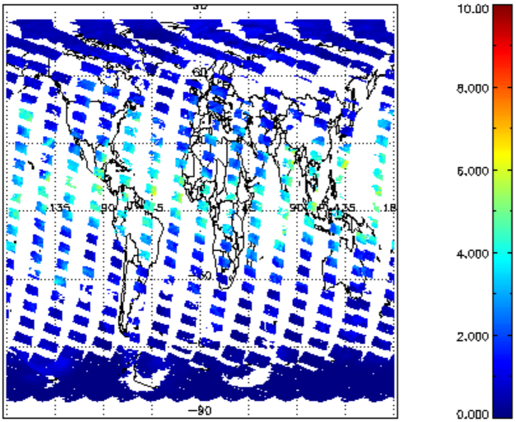
SCIOL2P_NADUV8H20_vcd for 24SEP2011 00:00:00 to 25SEP2011 00:00:00
