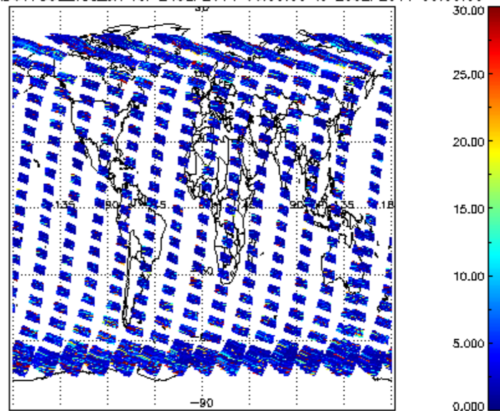
SCIOL2P_NADUV7S02_vcd_err for 24SEP2011 00:00:00 to 25SEP2011 00:00:00
