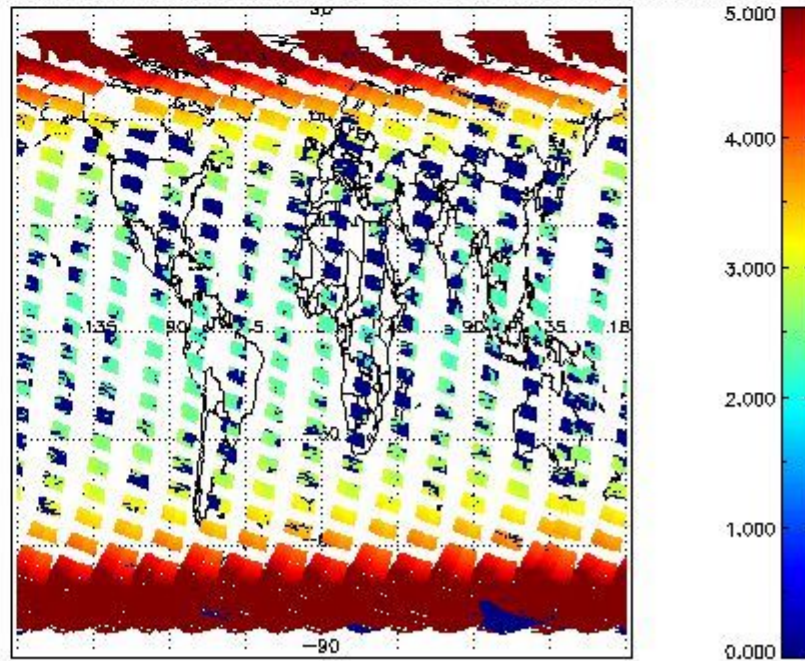
SCIOL2P_NADUV003_amf_cl for 24SEP2011 00:00:00 to 25SEP2011 00:00:00
