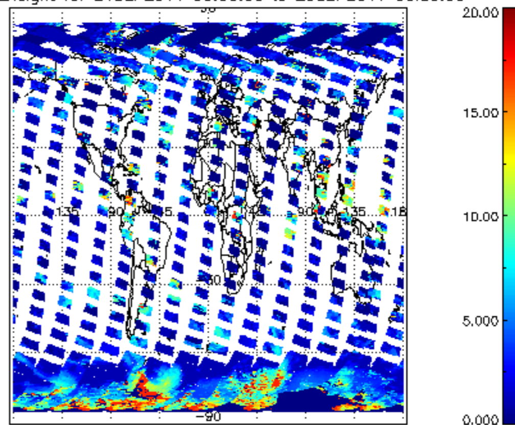
cl_top_height for 24SEP2011 00:00:00 to 25SEP2011 00:00:00
