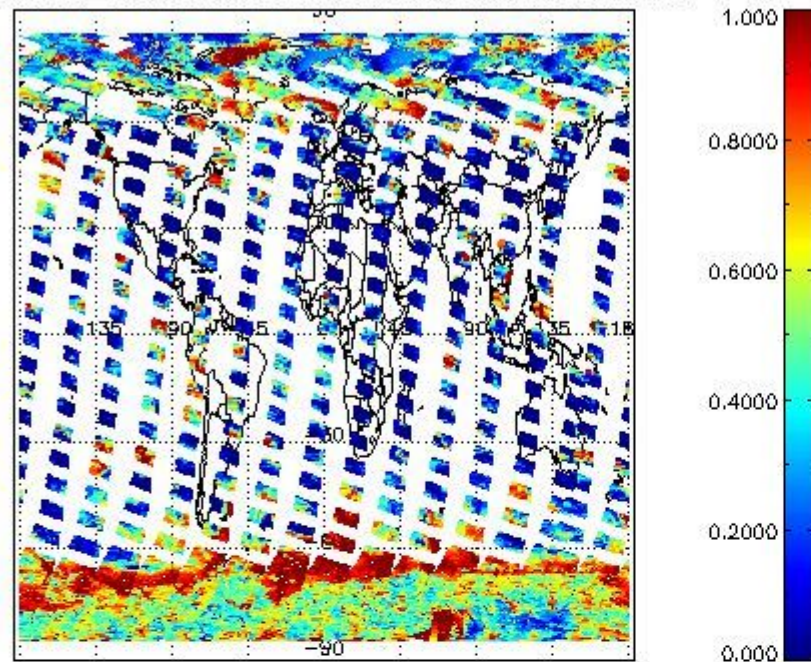
cL_frac for 24SEP2011 00:00:00 to 25SEP2011 00:00:00
