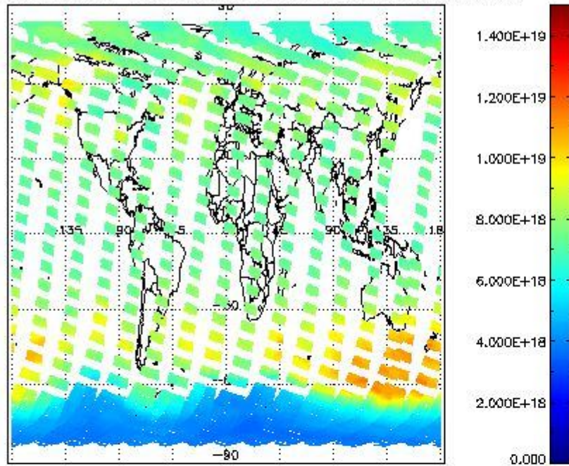
SCIOL2P_NADUV003_vcd for 24SEP2011 00:00:00 to 25SEP2011 00:00:00
