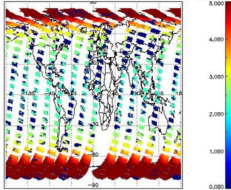
SCIOL2P_NADUV1N02_amf_cl for 19SEP2011 00:00:00 to 20SEP2011 00:00:00
