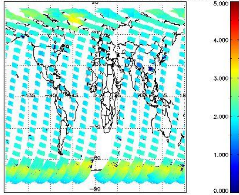
SCIOL2P_NADUV7S02_amf_gr for 19SEP2011 00:00:00 to 20SEP2011 00:00:00
