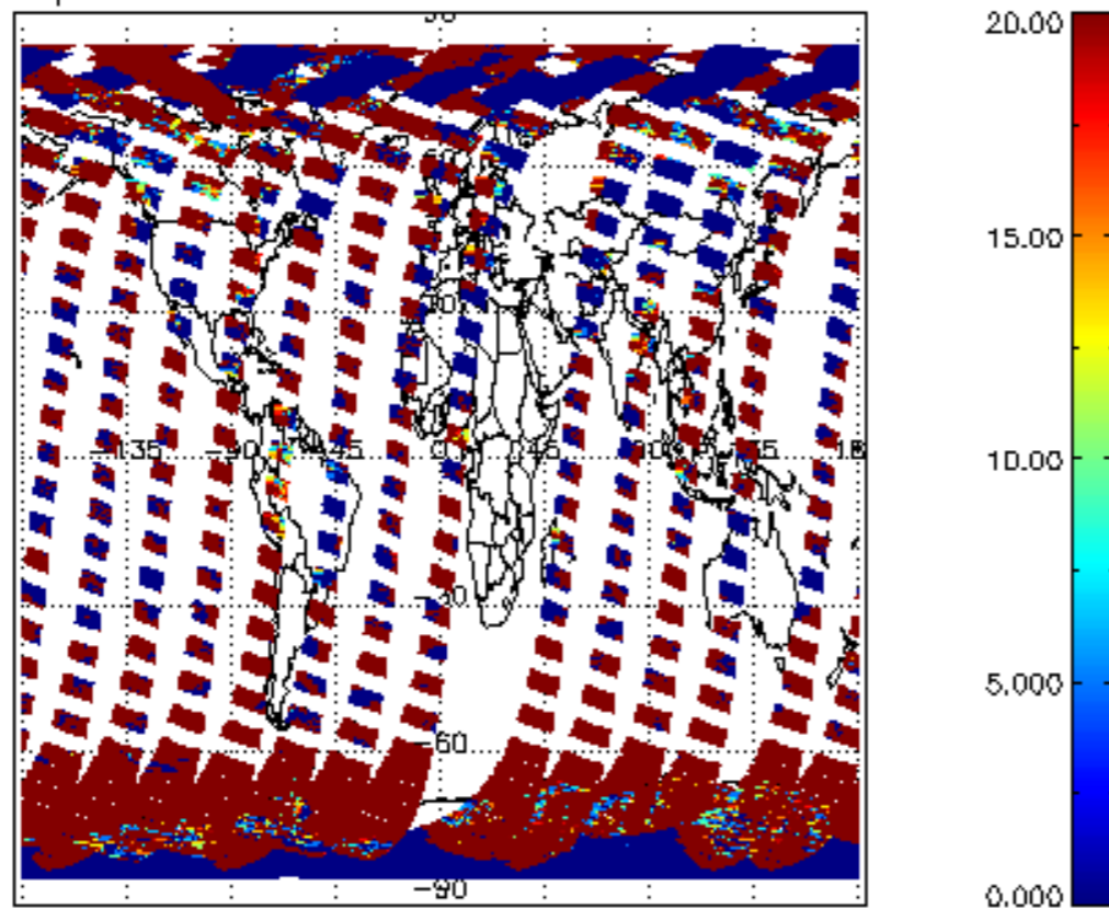
cl_opt_depth for 19SEP2011 00:00:00 to 20SEP2011 00:00:00
