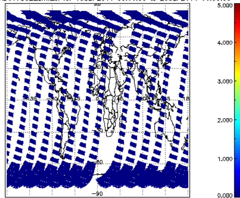
SCIOL2P_NADUV7S02_amf_cl for 19SEP2011 00:00:00 to 20SEP2011 00:00:00
