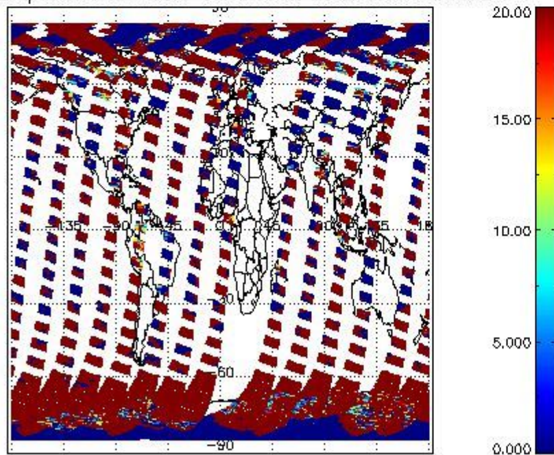
cL_opt_depth for 19SEP2011 00:00:00 to 20SEP2011 00:00:00
