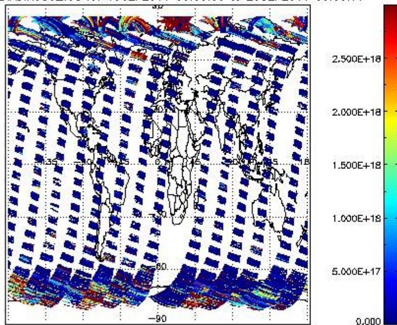
SCIDL2P_NADIR3CO_vcd for 19SEP2011 00:00:00 to 20SEP2011 00:00:00
