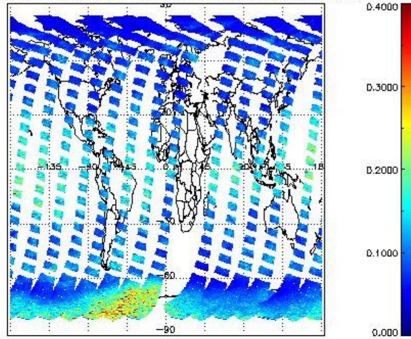
SCIOL2P_NADUV1N02_vcd_err for 19SEP2011 00:00:00 to 20SEP2011 00:00:00
