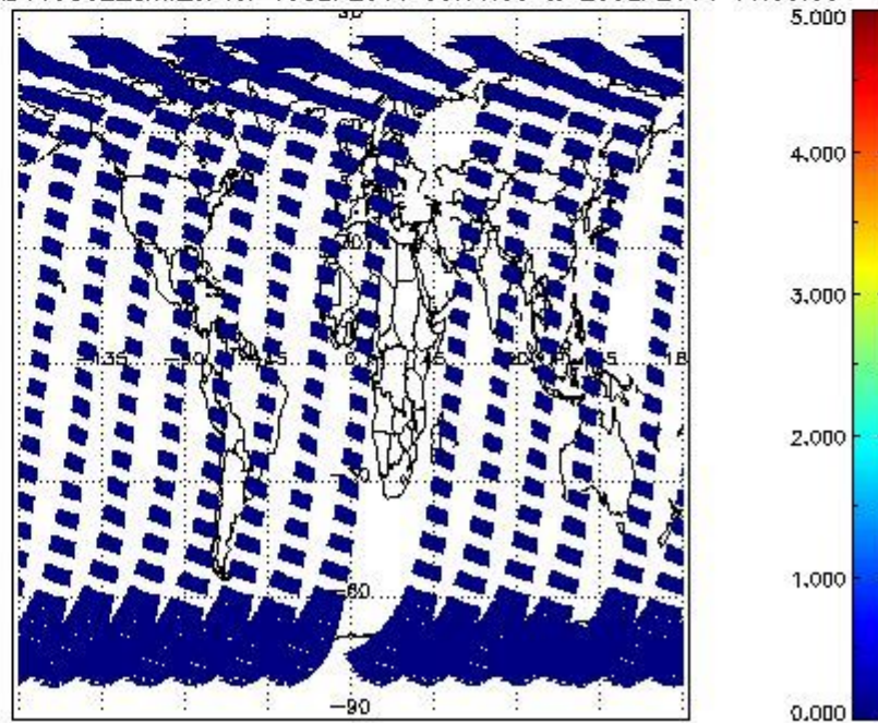
SCIOL2P_NADUV5S02_amf_cl for 19SEP2011 00:00:00 to 20SEP2011 00:00:00
