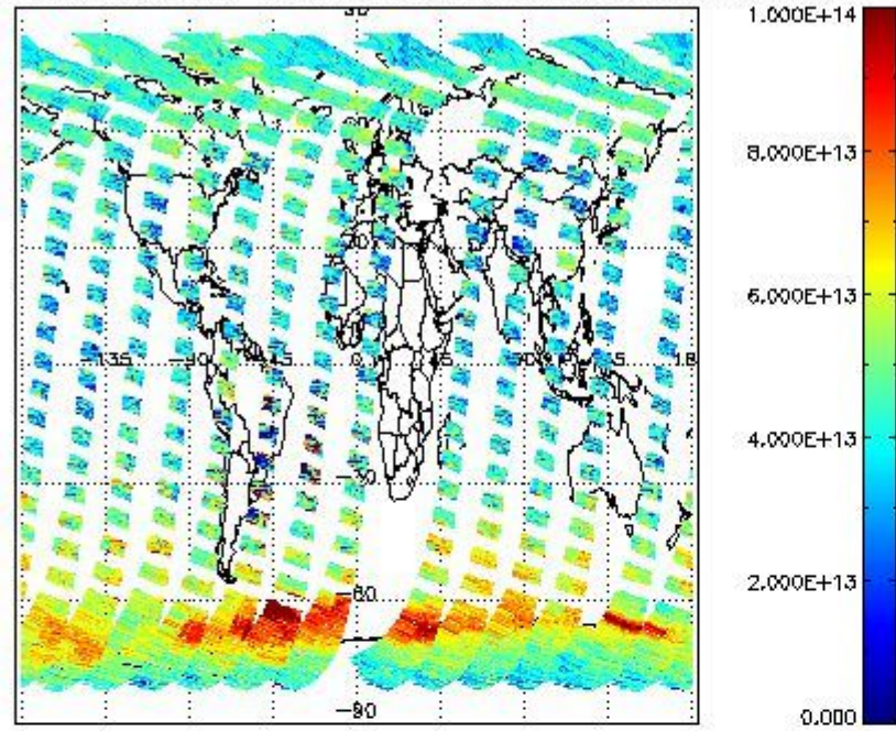
SCIOL2P_NADUV3BRO_vcd for 19SEP2011 00:00:00 to 20SEP2011 00:00:00
