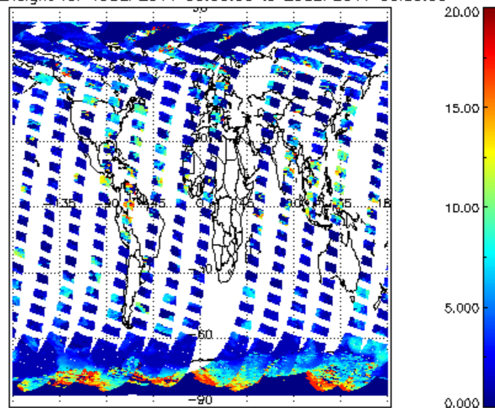
cl_top_height for 19SEP2011 00:00:00 to 20SEP2011 00:00:00
