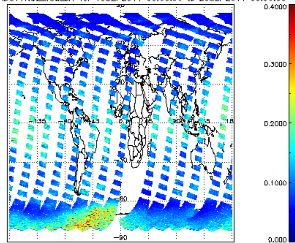
SCIOL2P_NADUV1N02_vcd_err for 19SEP2011 00:00:00 to 20SEP2011 00:00:00
