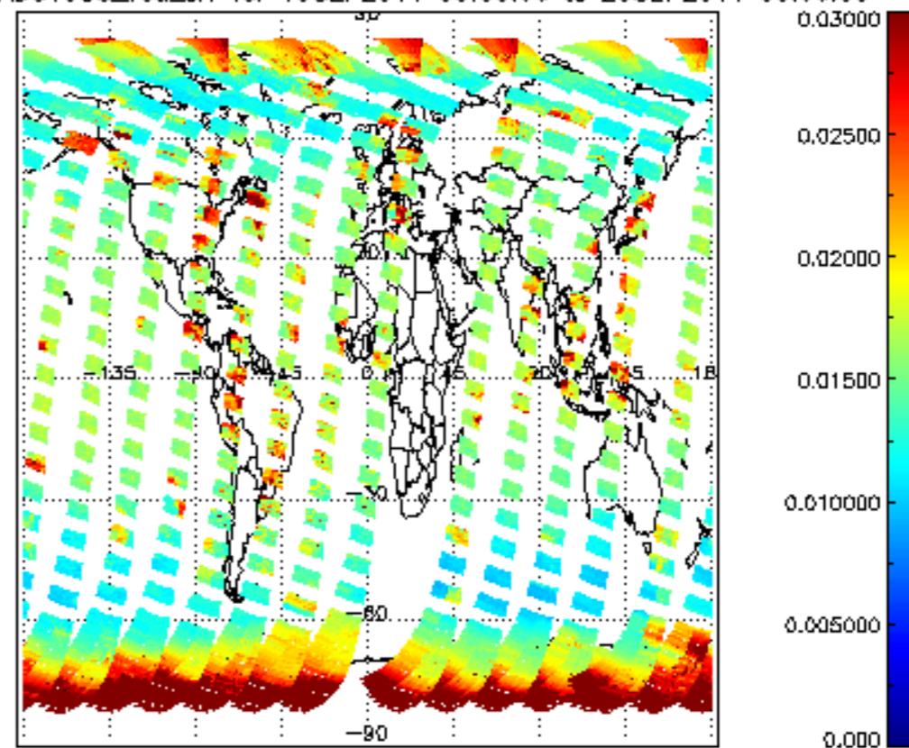
SCIOL2P_NADUV003_vcd_err for 19SEP2011 00:00:00 to 20SEP2011 00:00:00
