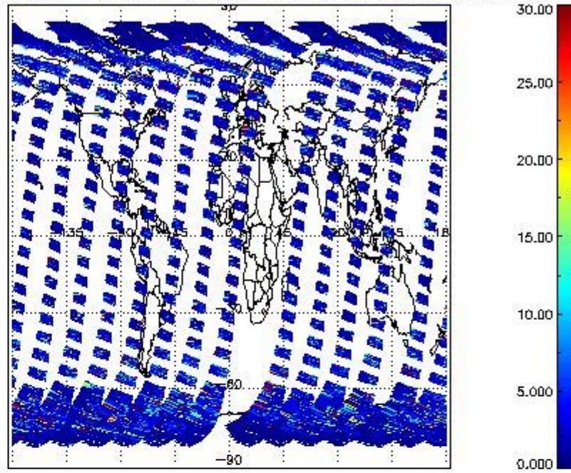
SCIOL2P_NADUV7S02_vcd_err for 19SEP2011 00:00:00 to 20SEP2011 00:00:00
