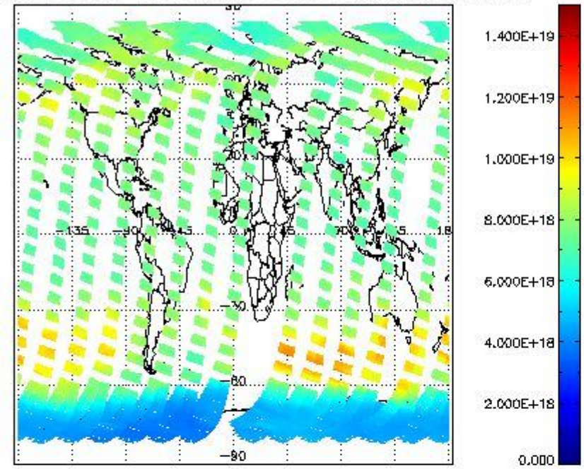
SCIOL2P_NADUV003_vcd for 19SEP2011 00:00:00 to 20SEP2011 00:00:00
