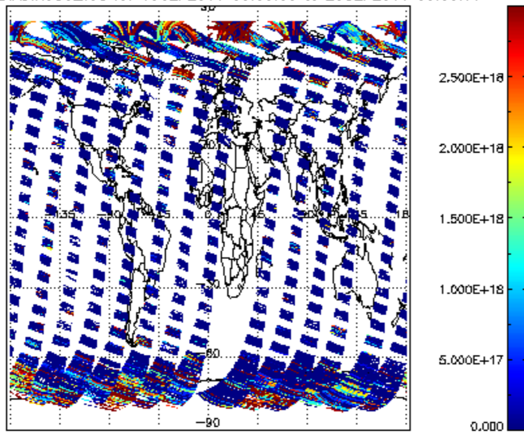
SCIOL2P_NADIR3CO_vcd for 19SEP2011 00:00:00 to 20SEP2011 00:00:00
