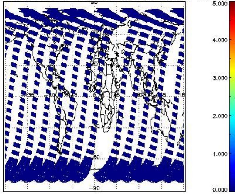
SCIOL2P_NADUV7S02_amf_cl for 19SEP2011 00:00:00 to 20SEP2011 00:00:00
