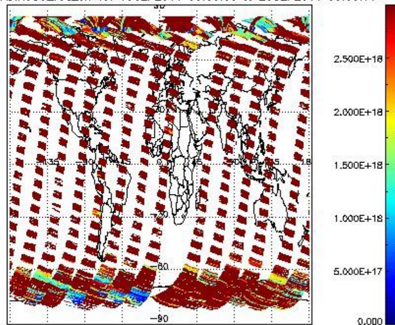
SCIDL2P_NADIR3CO_vcd_err for 19SEP2011 00:00:00 to 20SEP2011 00:00:00
