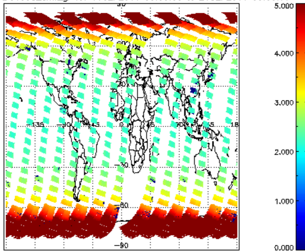
SCIOL2P_NADUV003_amf_gr for 19SEP2011 00:00:00 to 20SEP2011 00:00:00
