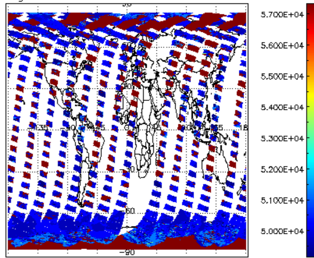
cloud_flags for 19SEP2011 00:00:00 to 20SEP2011 00:00:00
