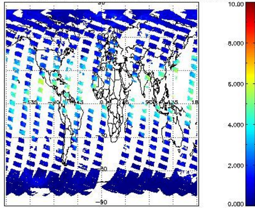
SCIOL2P_NADUV8H2O_vcd for 19SEP2011 00:00:00 to 20SEP2011 00:00:00
