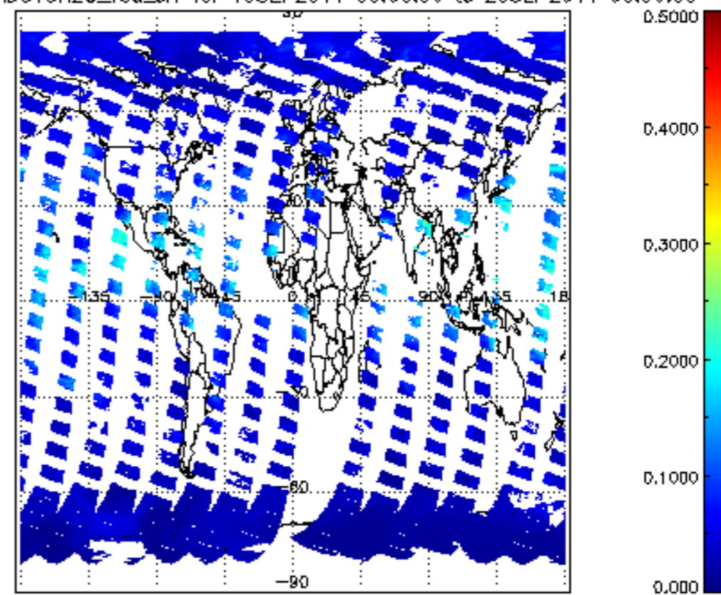
SCIOL2P_NADUV8H2O_vcd_err for 19SEP2011 00:00:00 to 20SEP2011 00:00:00
