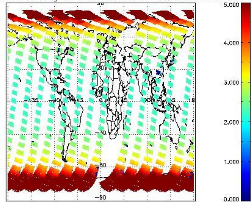
SCIOL2P_NADUV003_amf_gr for 19SEP2011 00:00:00 to 20SEP2011 00:00:00
