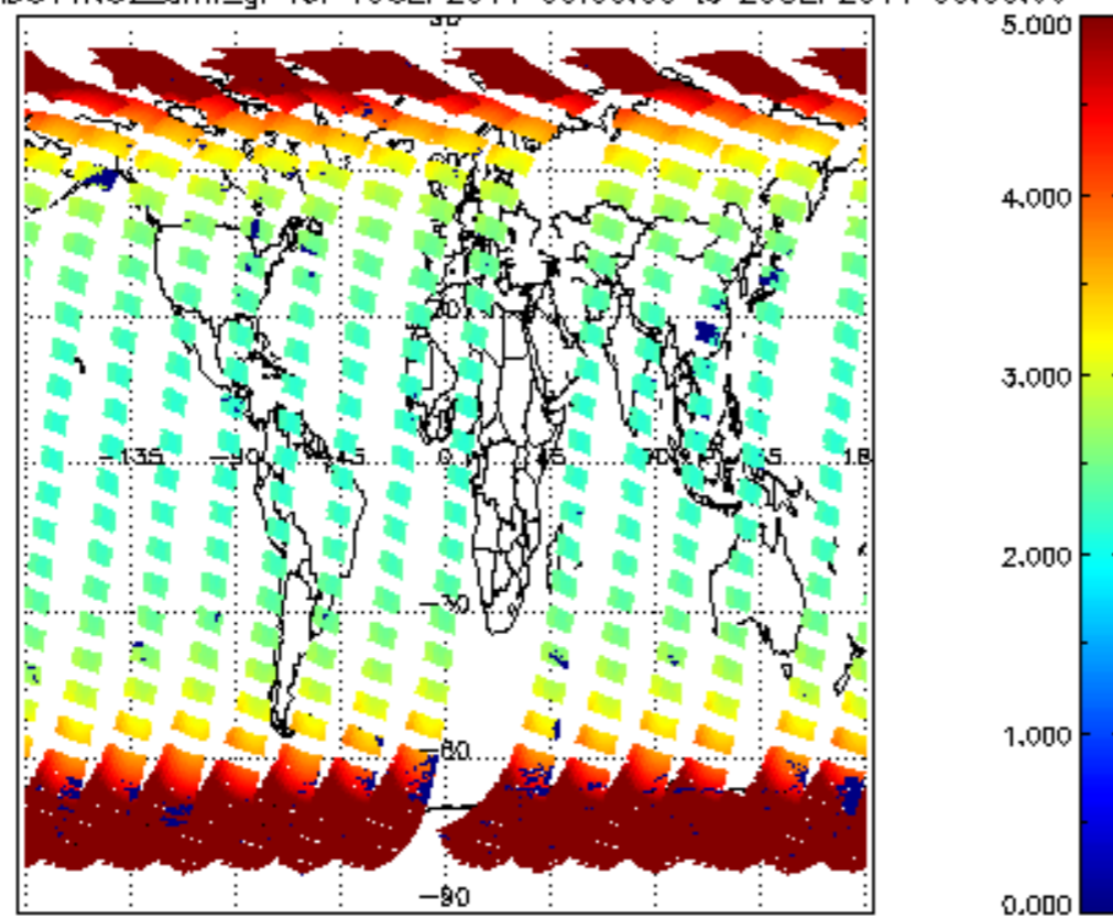
SCIOL2P_NADUV1N02_amf_gr for 19SEP2011 00:00:00 to 20SEP2011 00:00:00
