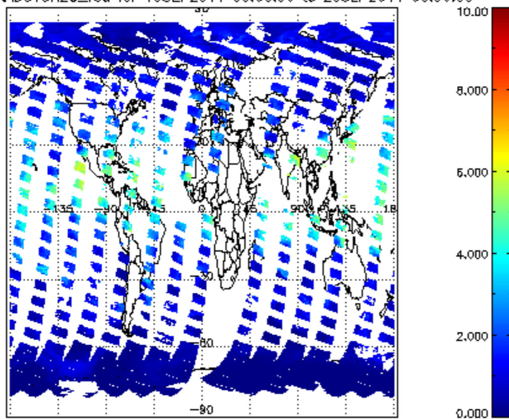
SCIOL2P_NADUV8H2O_vcd for 19SEP2011 00:00:00 to 20SEP2011 00:00:00
