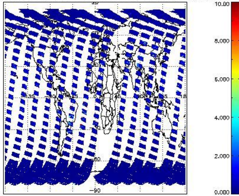
SCIOL2P_NADUV3BRO_vcd_err for 19SEP2011 00:00:00 to 20SEP2011 00:00:00
