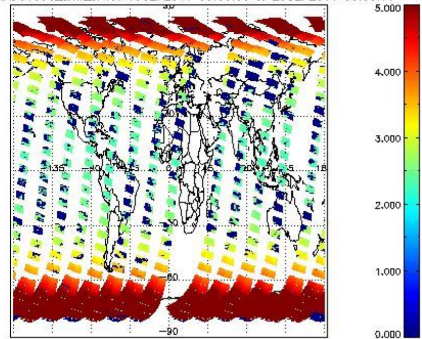
SCIOL2P_NADUV003_amf_cl for 19SEP2011 00:00:00 to 20SEP2011 00:00:00
