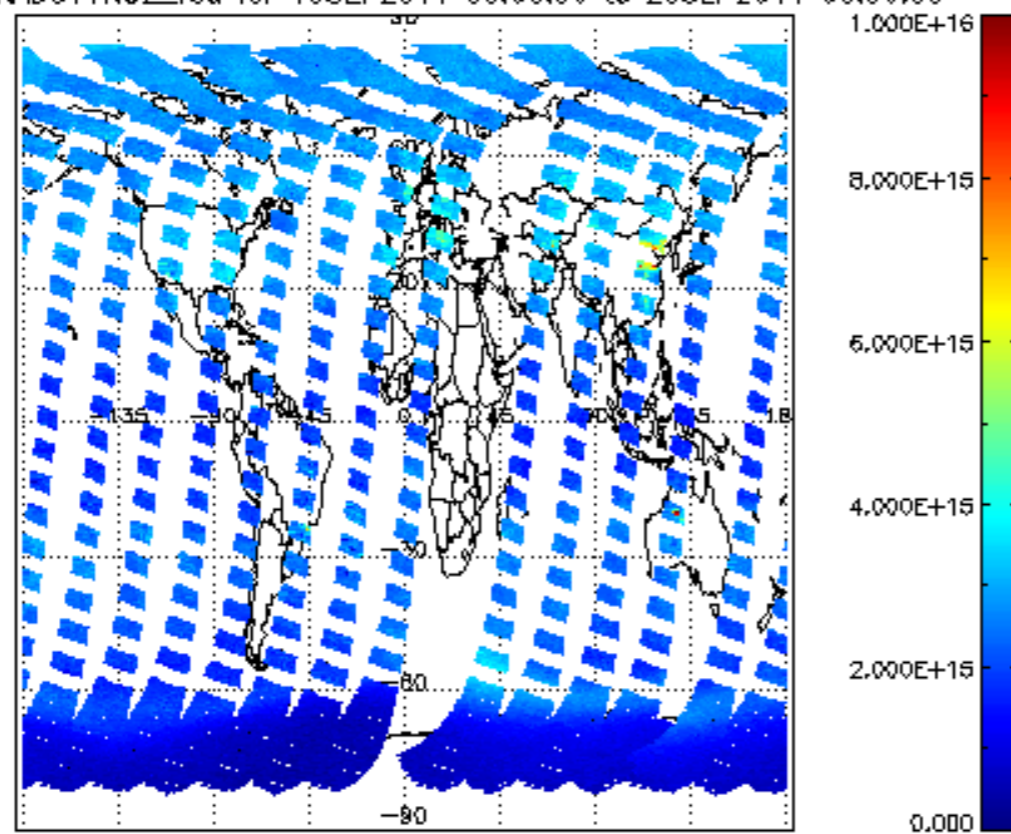
SCIOL2P_NADUV1N02_vcd for 19SEP2011 00:00:00 to 20SEP2011 00:00:00
