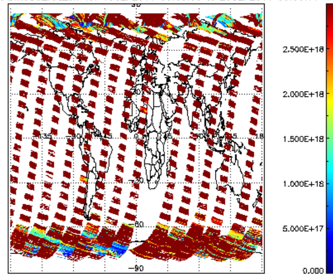
SCIOL2P_NADIR3CO_vcd_err for 19SEP2011 00:00:00 to 20SEP2011 00:00:00
