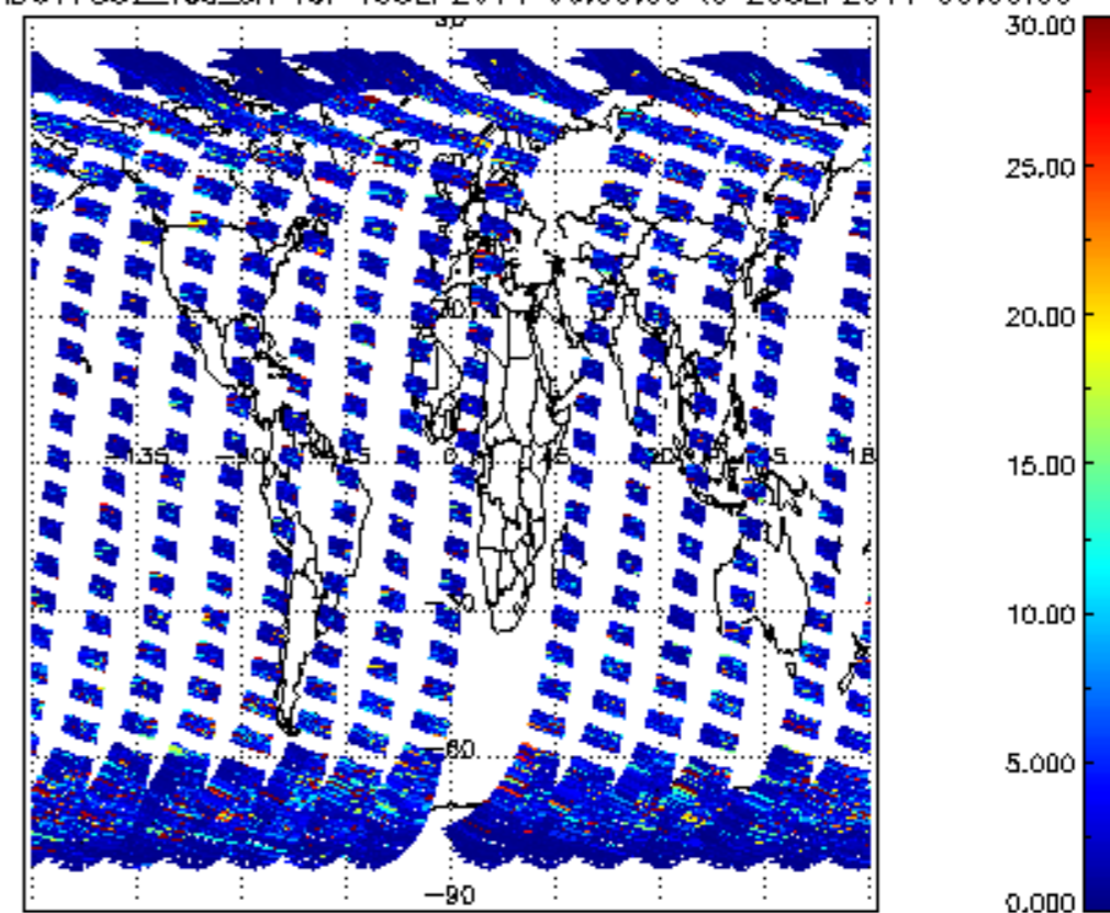
SCIOL2P_NADUV7S02_vcd_err for 19SEP2011 00:00:00 to 20SEP2011 00:00:00
