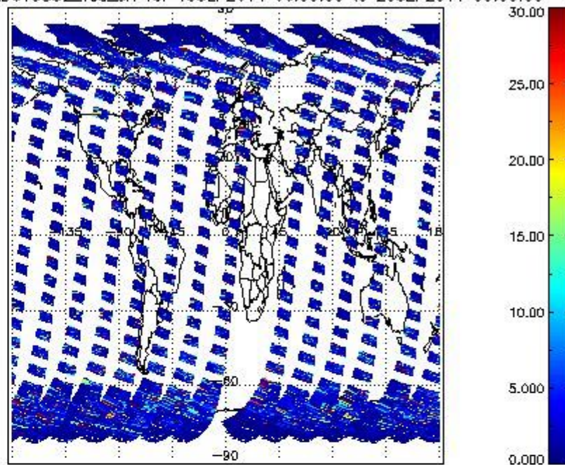
SCIOL2P_NADUV5S02_vcd_err for 19SEP2011 00:00:00 to 20SEP2011 00:00:00
