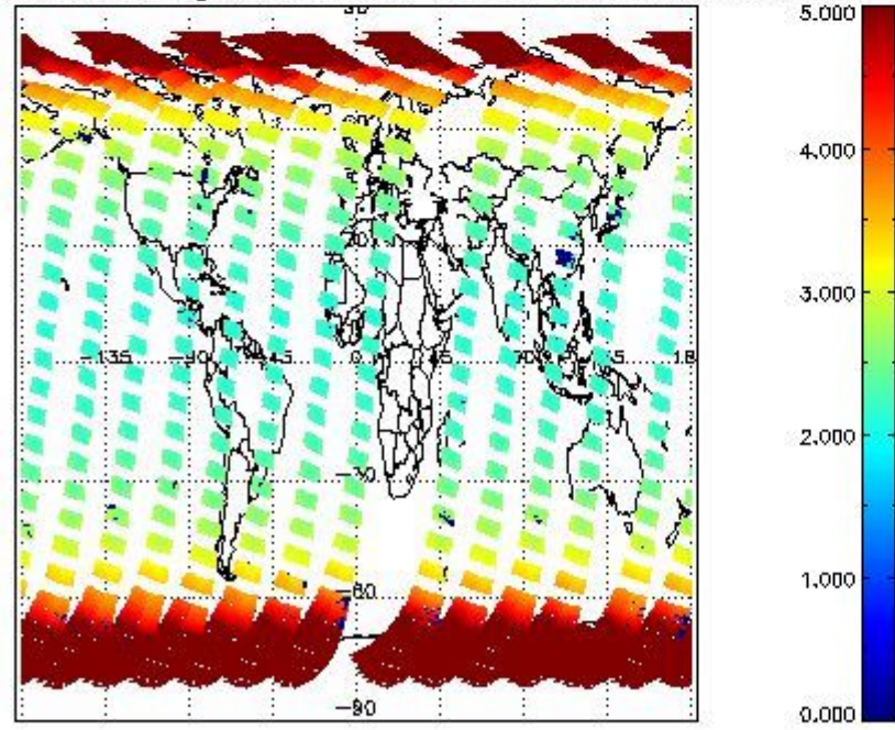
SCIOL2P_NADUV3BRO_amf_gr for 19SEP2011 00:00:00 to 20SEP2011 00:00:00
