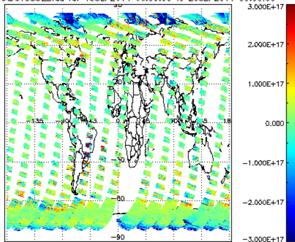
SCIOL2P_NADUV5S02_vcd for 19SEP2011 00:00:00 to 20SEP2011 00:00:00
