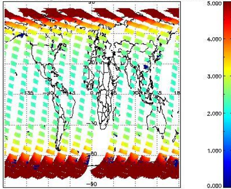
SCIOL2P_NADUV1N02_amf_gr for 19SEP2011 00:00:00 to 20SEP2011 00:00:00
