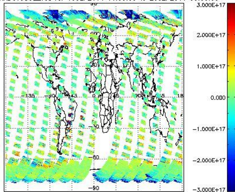
SCIOL2P_NADUV5S02_vcd for 19SEP2011 00:00:00 to 20SEP2011 00:00:00
