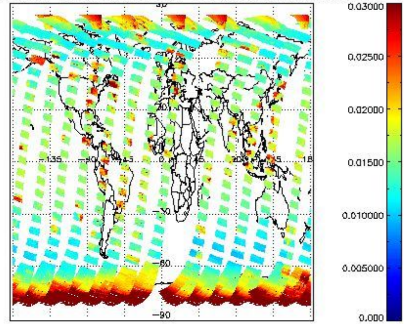
SCIOL2P_NADUV003_vcd_err for 19SEP2011 00:00:00 to 20SEP2011 00:00:00
