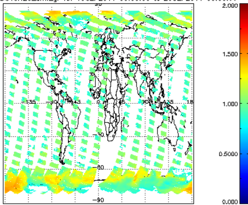
SCIOL2P_NADUV8H2O_amf_gr for 19SEP2011 00:00:00 to 20SEP2011 00:00:00
