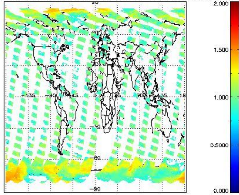
SCIOL2P_NADUV8H2O_arnf_gr for 19SEP2011 00:00:00 to 20SEP2011 00:00:00
