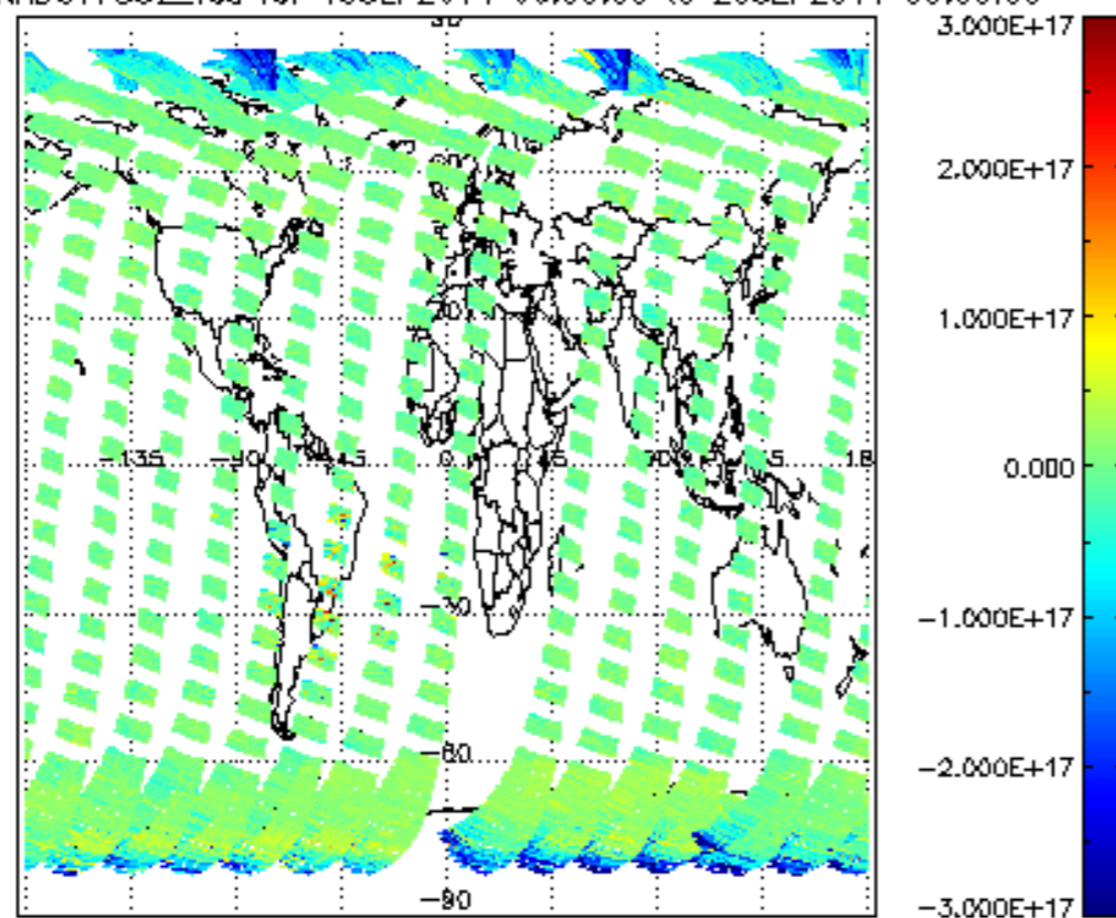
SCIOL2P_NADUV7S02_vcd for 19SEP2011 00:00:00 to 20SEP2011 00:00:00
