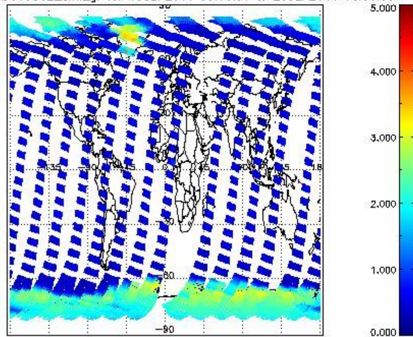
SCIOL2P_NADUV5S02_amf_gr for 19SEP2011 00:00:00 to 20SEP2011 00:00:00
