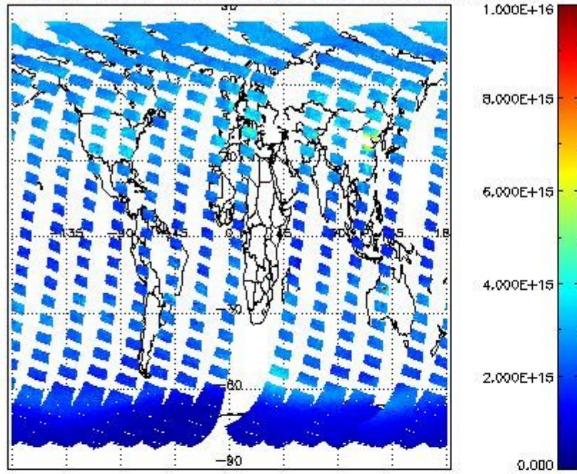
SCIOL2P_NADUV1N02_vcd for 19SEP2011 00:00:00 to 20SEP2011 00:00:00
