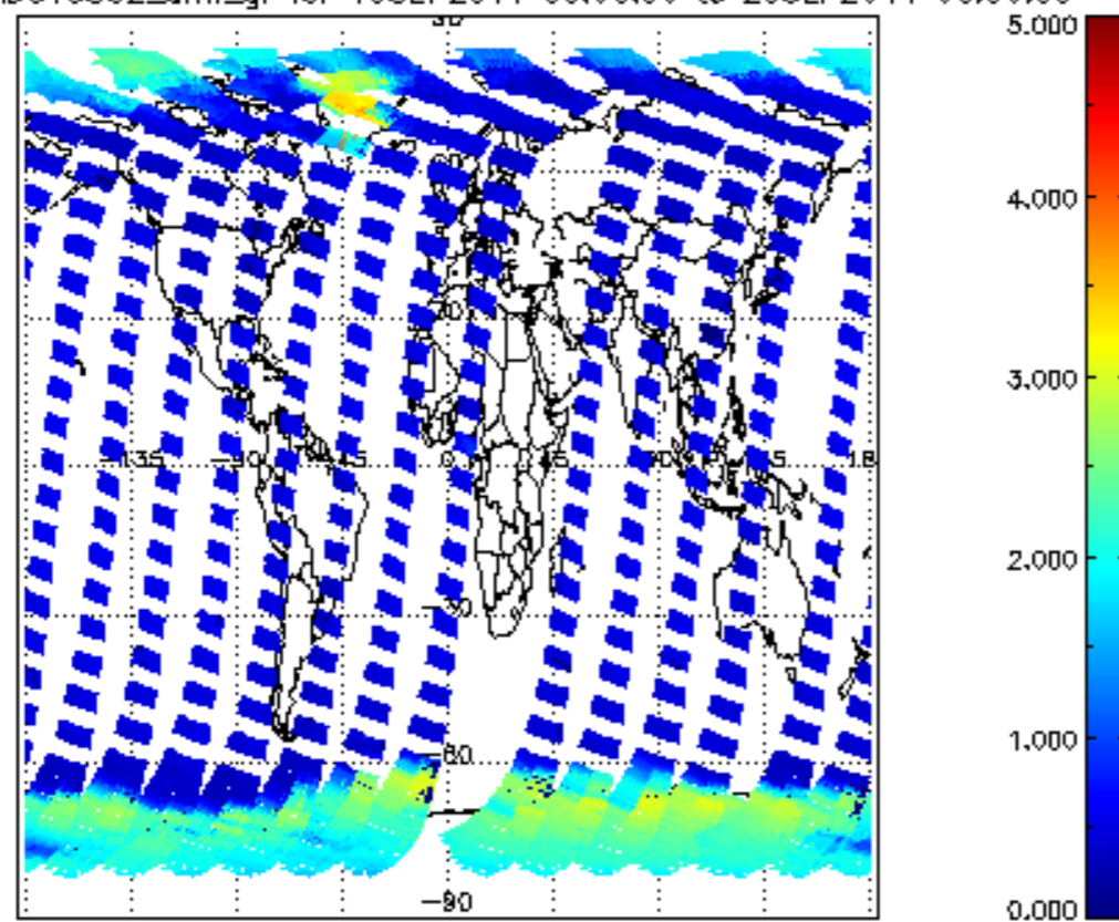
SCIOL2P_NADUV5S02_amf_gr for 19SEP2011 00:00:00 to 20SEP2011 00:00:00
