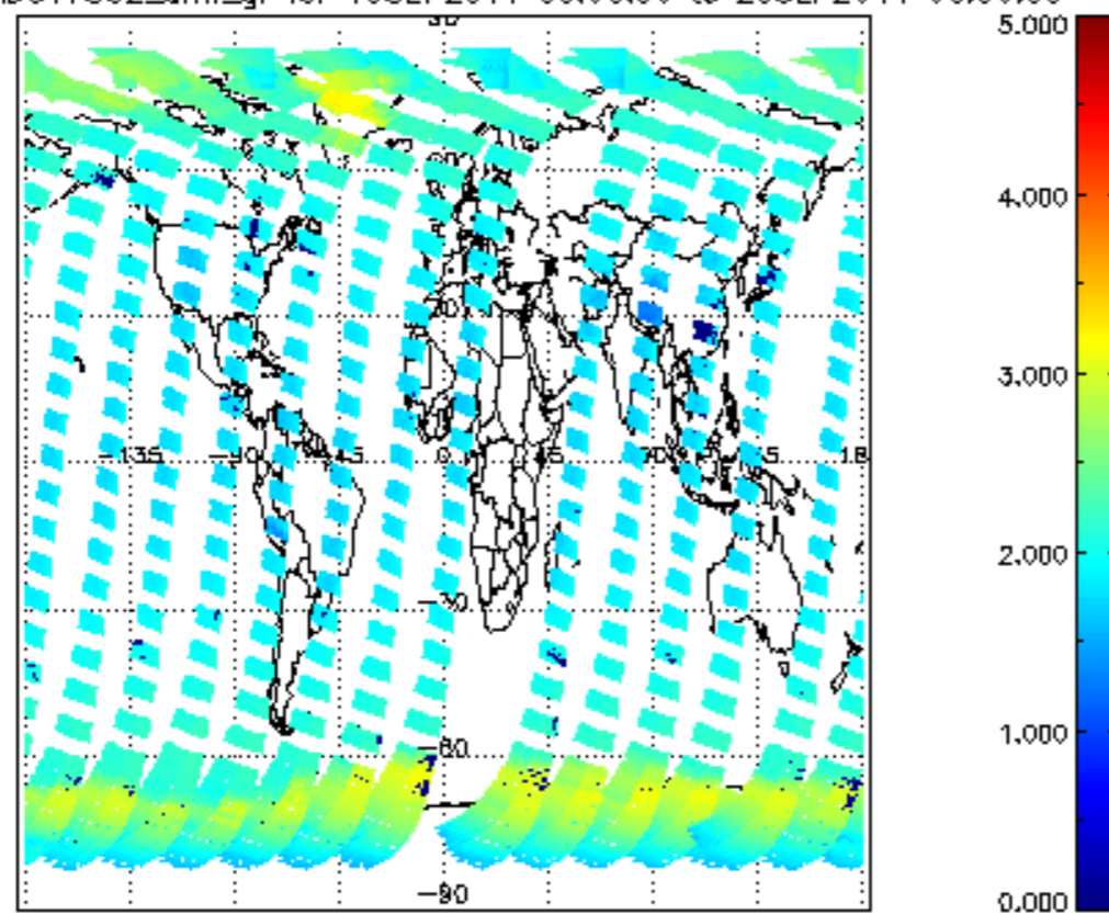
SCIOL2P_NADUV7S02_amf_gr for 19SEP2011 00:00:00 to 20SEP2011 00:00:00
