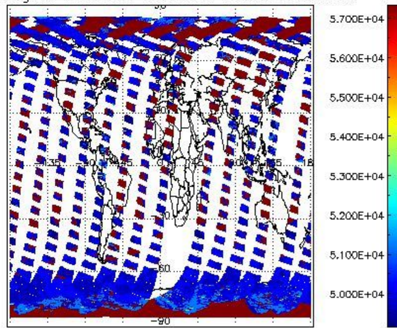
cloud_flags for 19SEP2011 00:00:00 to 20SEP2011 00:00:00
