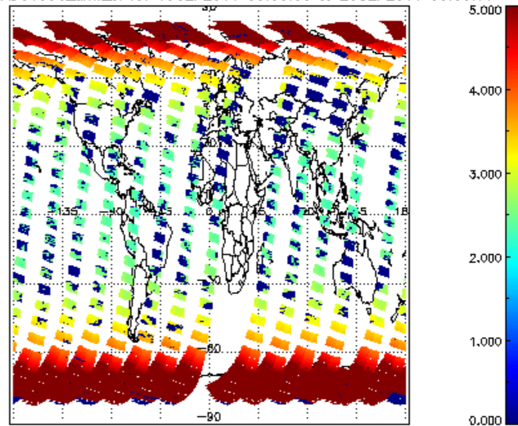
SCIOL2P_NADUV003_amf_cl for 19SEP2011 00:00:00 to 20SEP2011 00:00:00
