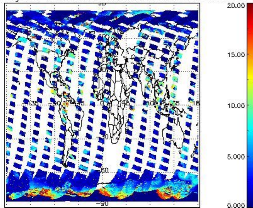
cL_top_height for 19SEP2011 00:00:00 to 20SEP2011 00:00:00
