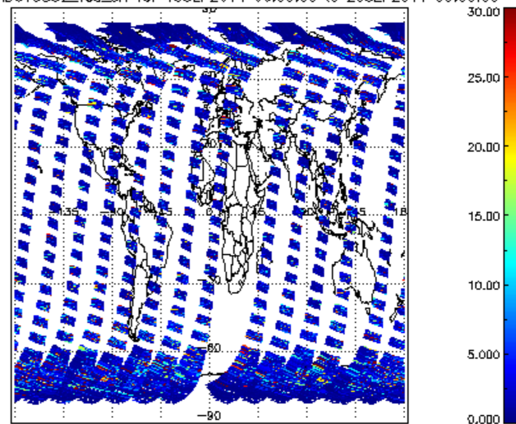
SCIOL2P_NADUV5S02_vcd_err for 19SEP2011 00:00:00 to 20SEP2011 00:00:00
