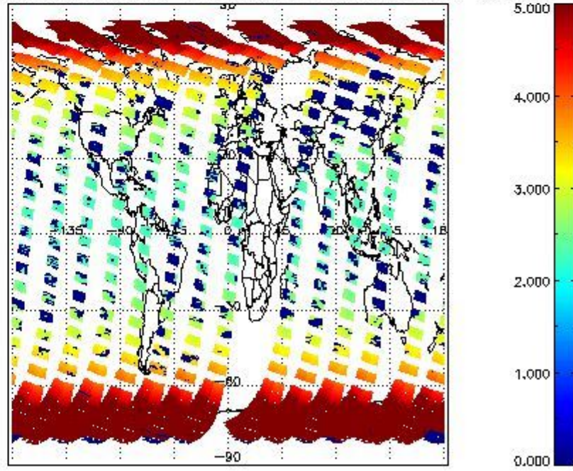
SCIOL2P_NADUV3BRO_amf_cl for 19SEP2011 00:00:00 to 20SEP2011 00:00:00
