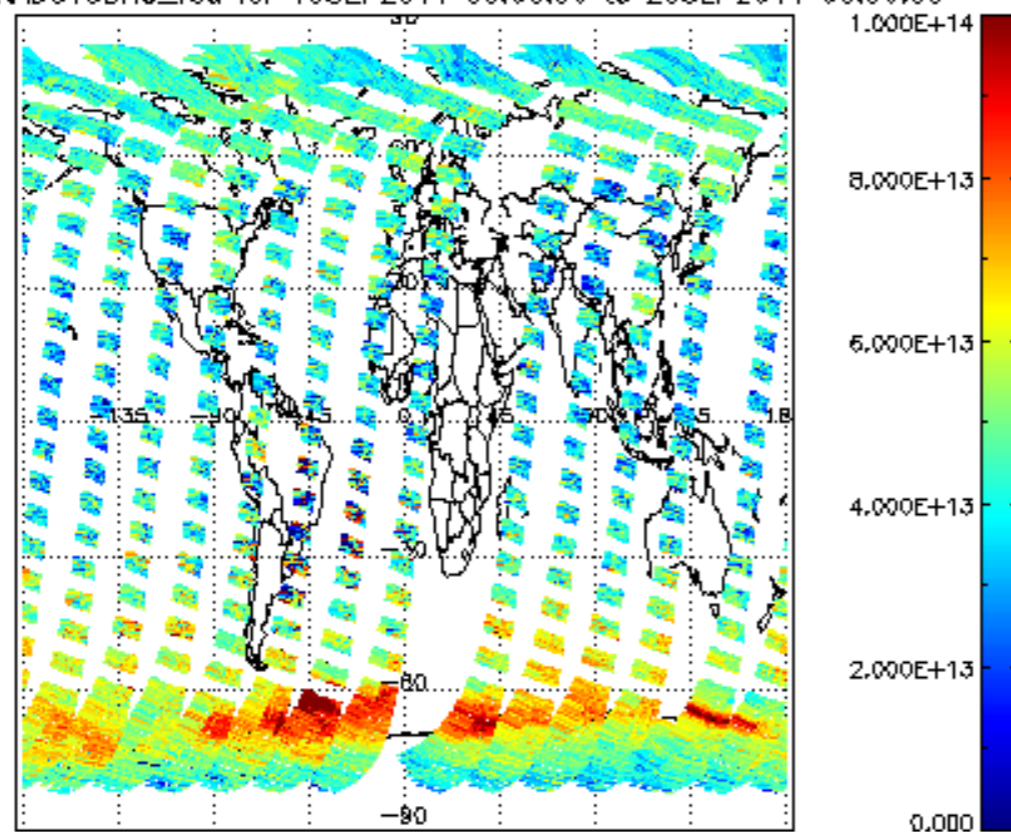
SCIOL2P_NADUV3BRO_vcd for 19SEP2011 00:00:00 to 20SEP2011 00:00:00
