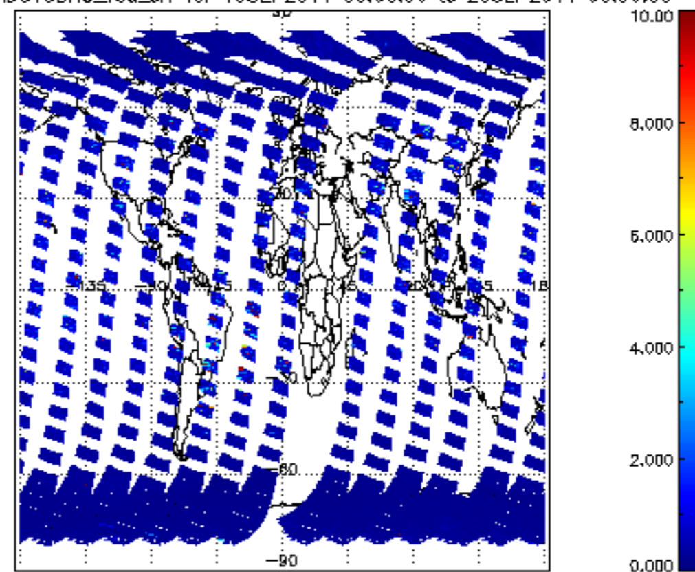
SCIOL2P_NADUV3BRO_vcd_err for 19SEP2011 00:00:00 to 20SEP2011 00:00:00
