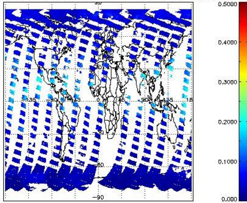
SCIOL2P_NADUV8H2O_vcd_err for 19SEP2011 00:00:00 to 20SEP2011 00:00:00
