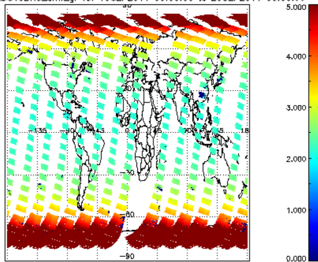
SCIOL2P_NADUV3BRO_amf_gr for 19SEP2011 00:00:00 to 20SEP2011 00:00:00
