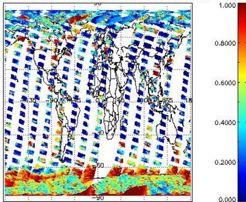
cL_frac for 19SEP2011 00:00:00 to 20SEP2011 00:00:00
