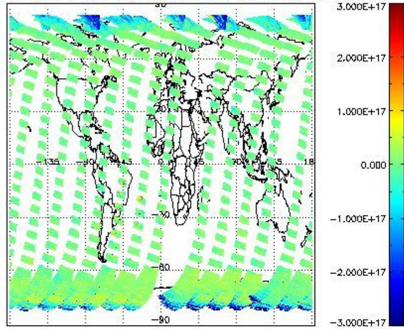
SCIOL2P_NADUV7S02_vcd for 19SEP2011 00:00:00 to 20SEP2011 00:00:00
