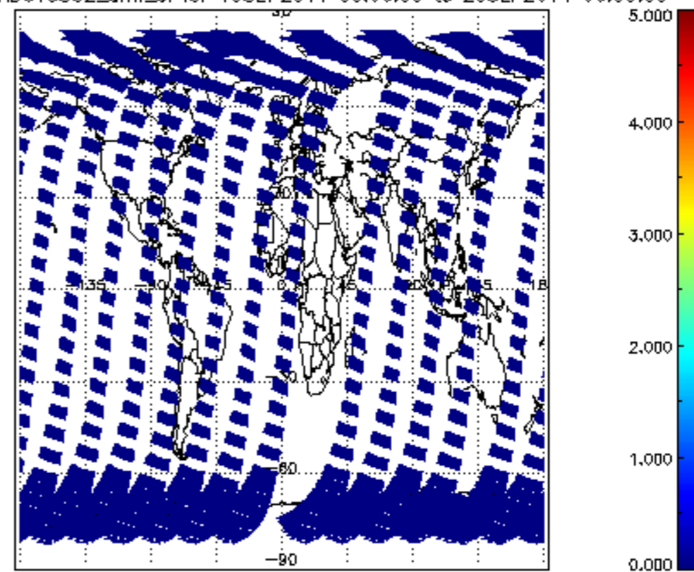
SCIOL2P_NADUV5S02_amf_cl for 19SEP2011 00:00:00 to 20SEP2011 00:00:00
