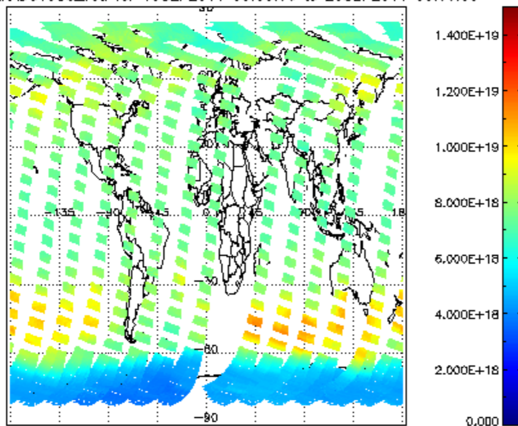
SCIOL2P_NADUV003_vcd for 19SEP2011 00:00:00 to 20SEP2011 00:00:00
