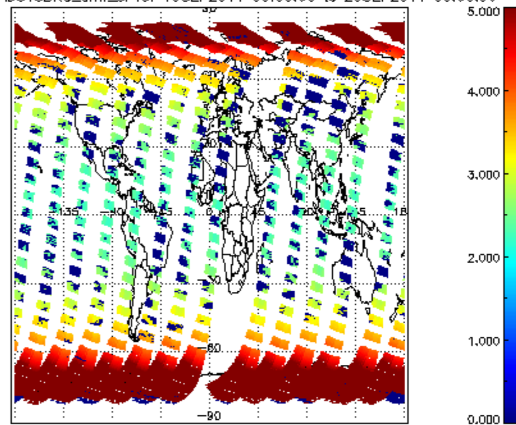
SCIOL2P_NADUV3BRO_amf_sl for 19SEP2011 00:00:00 to 20SEP2011 00:00:00
