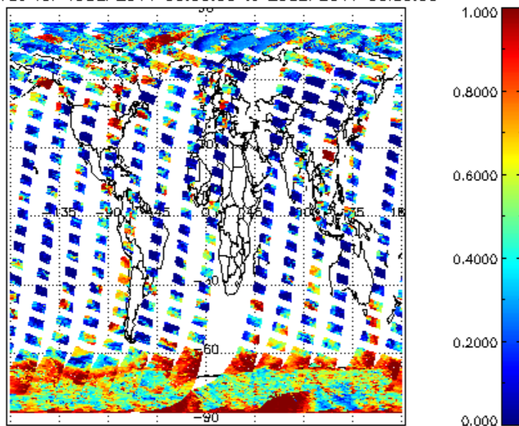
cl_frac for 19SEP2011 00:00:00 to 20SEP2011 00:00:00
