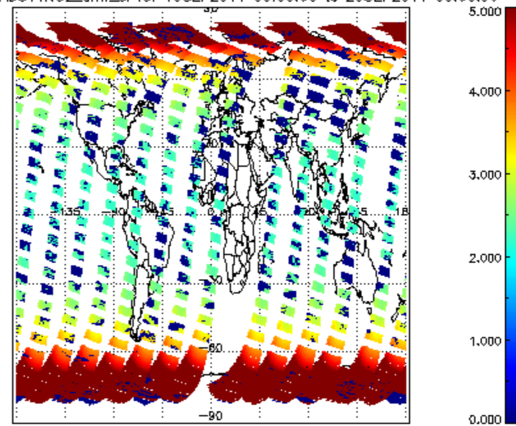
SCIOL2P_NADUV1N02_amf_sl for 19SEP2011 00:00:00 to 20SEP2011 00:00:00
