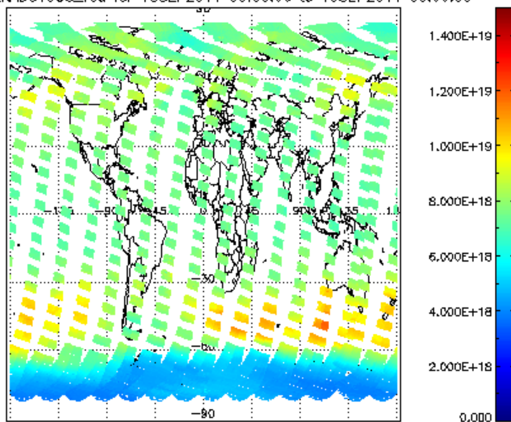
SCIOL2P_NADUV003_vcd for 18SEP2011 00:00:00 to 19SEP2011 00:00:00
