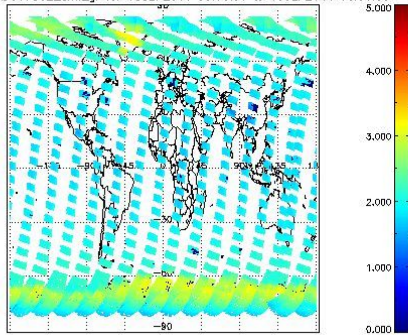
SCIOL2P_NADUV7S02_amf_gr for 18SEP2011 00:00:00 to 19SEP2011 00:00:00
