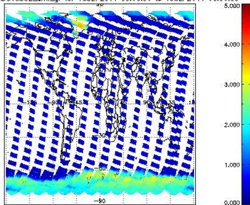
SCIOL2P_NADUV5S02_amf_gr for 18SEP2011 00:00:00 to 19SEP2011 00:00:00
