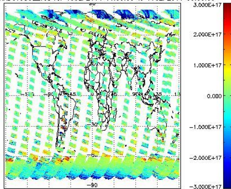
SCIOL2P_NADUV5S02_vcd for 18SEP2011 00:00:00 to 19SEP2011 00:00:00
