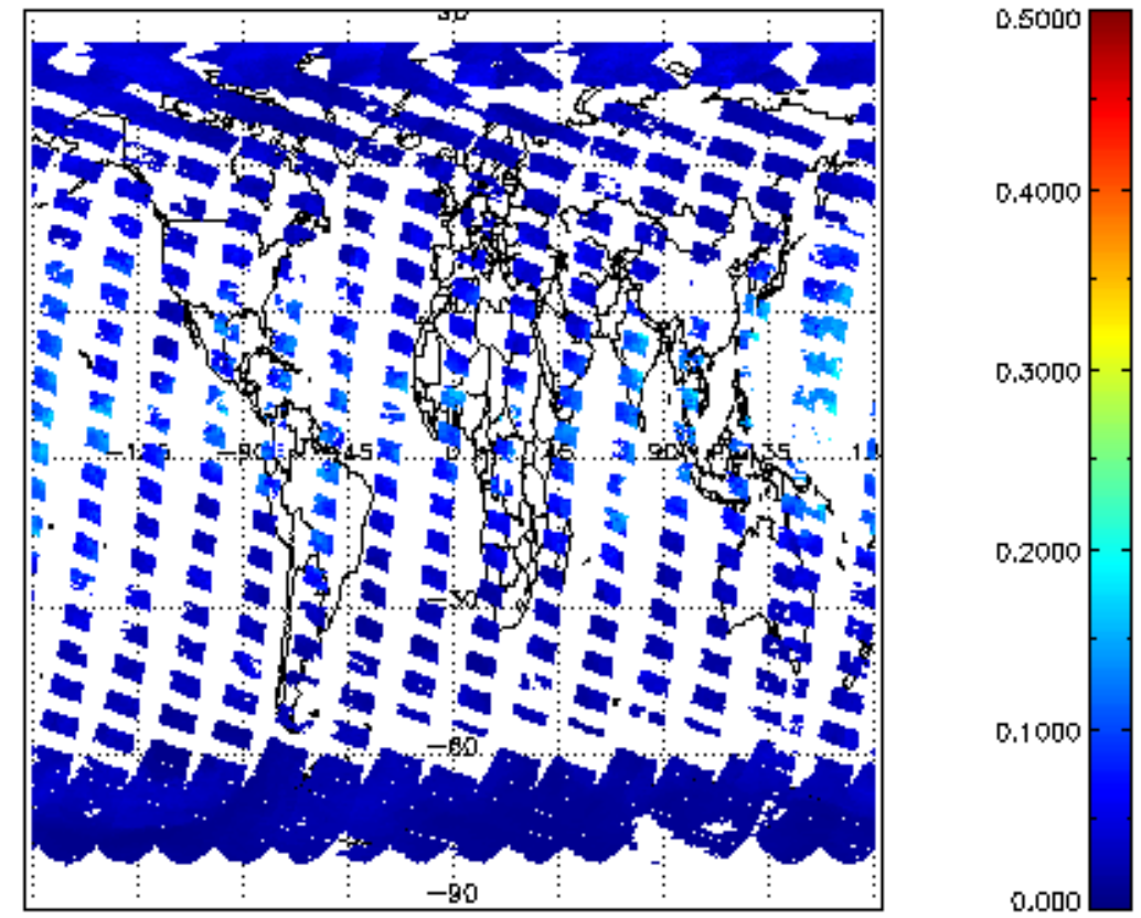
SCIOL2P_NADUV8H20_vcd_err for 18SEP2011 00:00:00 to 19SEP2011 00:00:00
