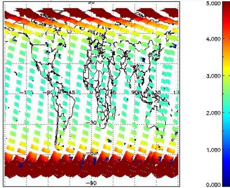
SCIOL2P_NADUV1N02_amf_gr for 18SEP2011 00:00:00 to 19SEP2011 00:00:00
