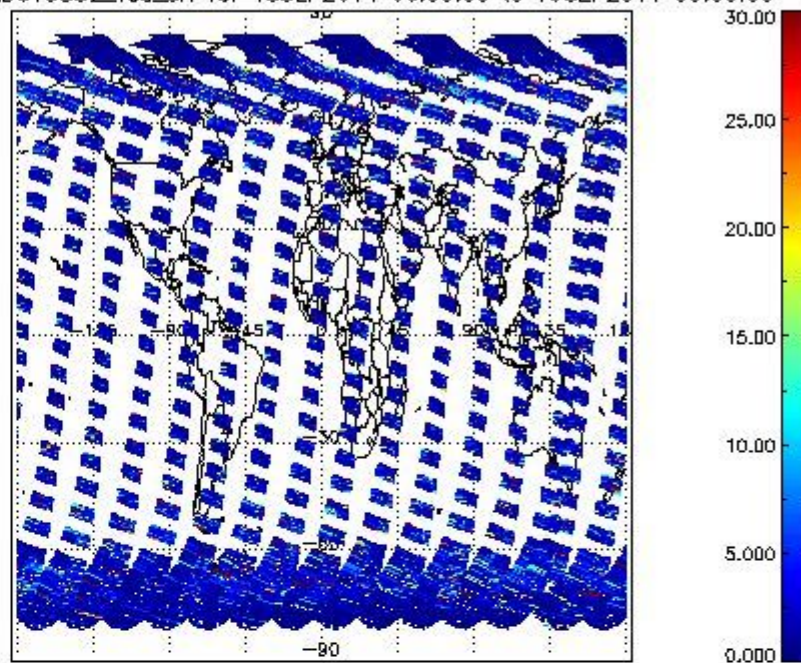
SCIOL2P_NADUV5S02_vcd_err for 18SEP2011 00:00:00 to 19SEP2011 00:00:00
