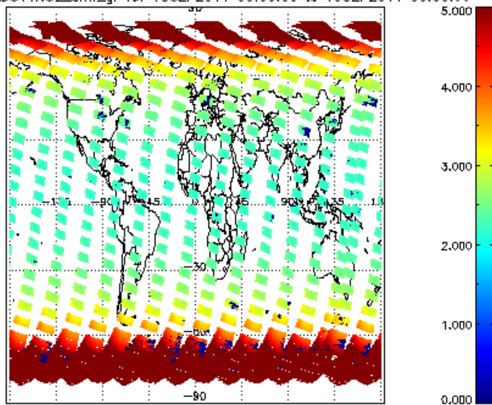
SCIOL2P_NADUV1NO2_amf_gr for 18SEP2011 00:00:00 to 19SEP2011 00:00:00
