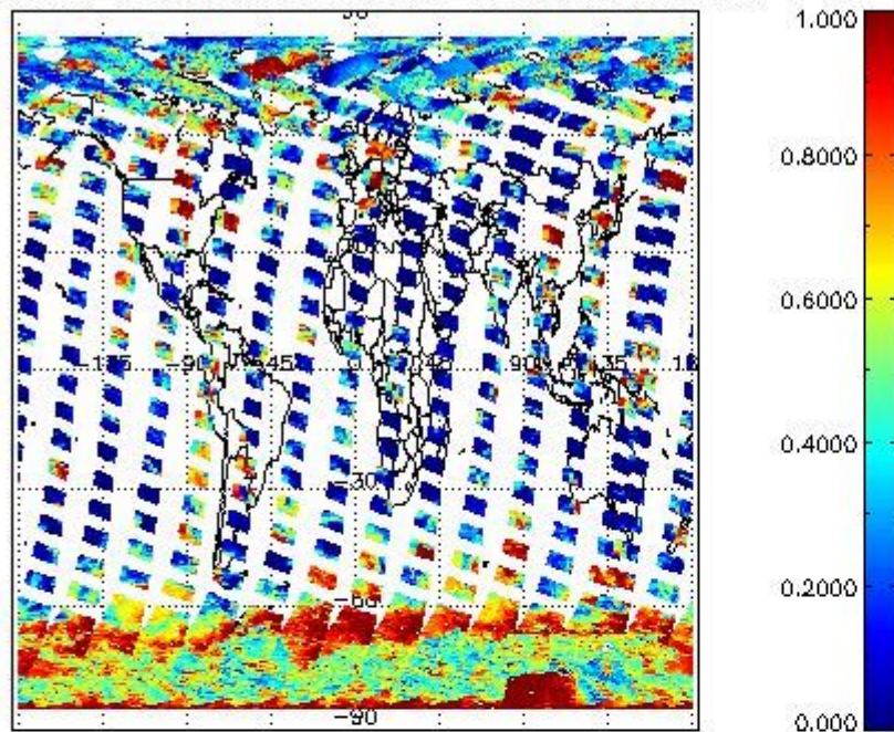
cL_frac for 18SEP2011 00:00:00 to 19SEP2011 00:00:00
