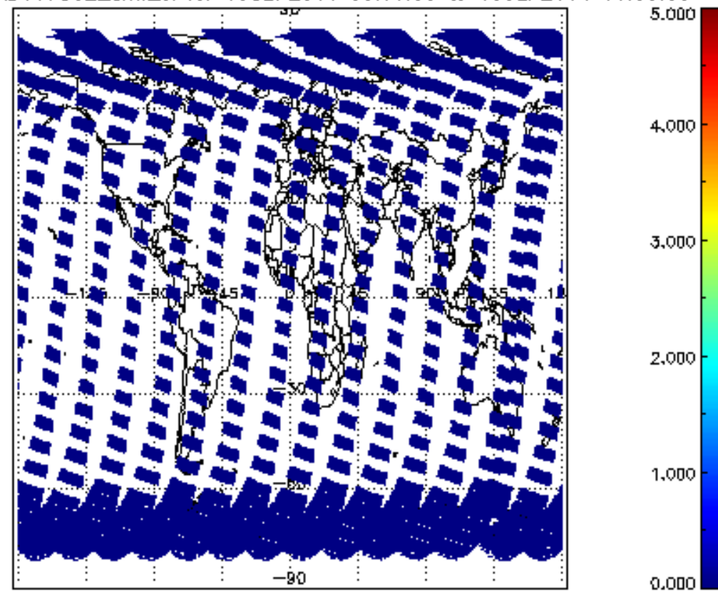
SCIOL2P_NADUV7S02_amf_cl for 18SEP2011 00:00:00 to 19SEP2011 00:00:00
