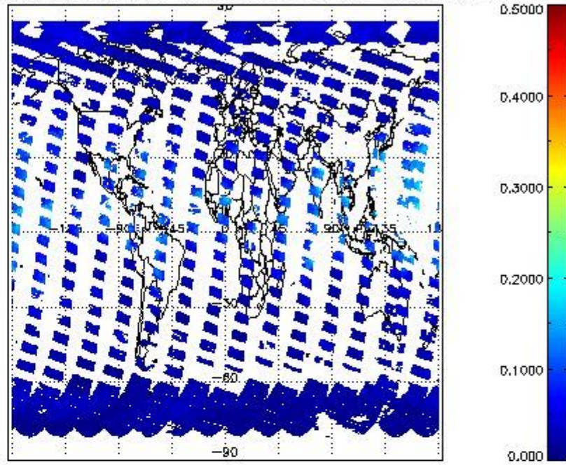
SCIOL2P_NADUV8H2O_vcd_err for 18SEP2011 00:00:00 to 19SEP2011 00:00:00
