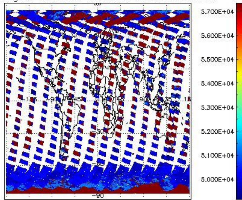
cloud_flags for 18SEP2011 00:00:00 to 19SEP2011 00:00:00
