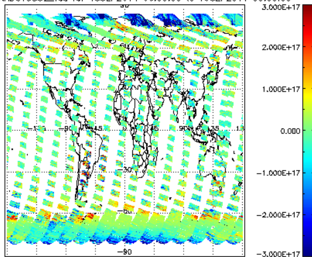
SCIOL2P_NADUV5S02_vcd for 18SEP2011 00:00:00 to 19SEP2011 00:00:00
