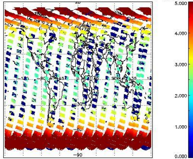
SCIOL2P_NADUV3BRO_amf_cl for 18SEP2011 00:00:00 to 19SEP2011 00:00:00
