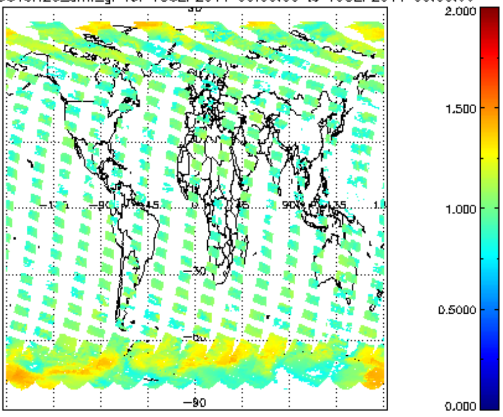
SCIOL2P_NADUV8H20_amf_gr for 18SEP2011 00:00:00 to 19SEP2011 00:00:00
