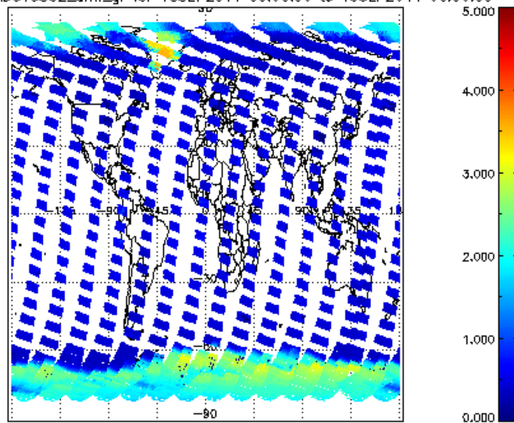
SCIOL2P_NADUV5S02_amf_gr for 18SEP2011 00:00:00 to 19SEP2011 00:00:00
