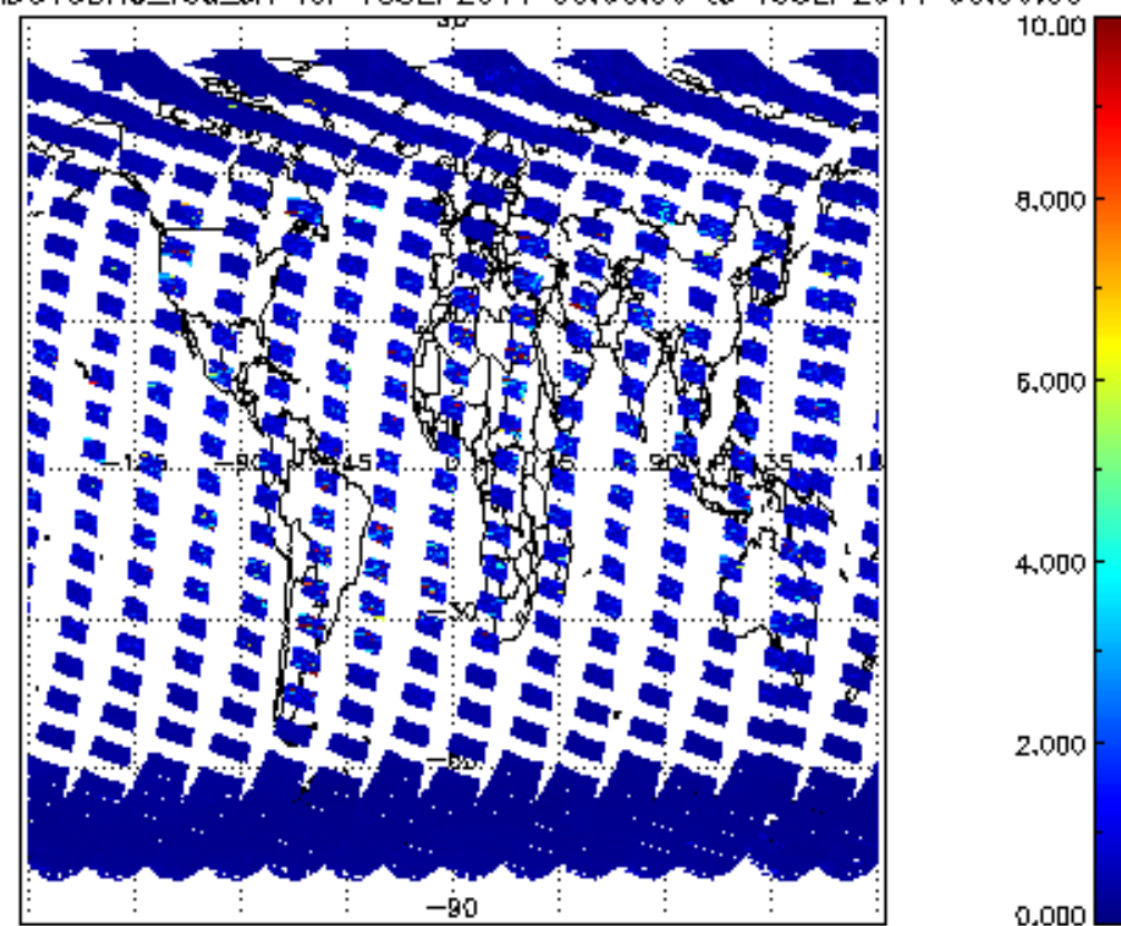
SCIOL2P_NADUV3BRO_vcd_err for 18SEP2011 00:00:00 to 19SEP2011 00:00:00
