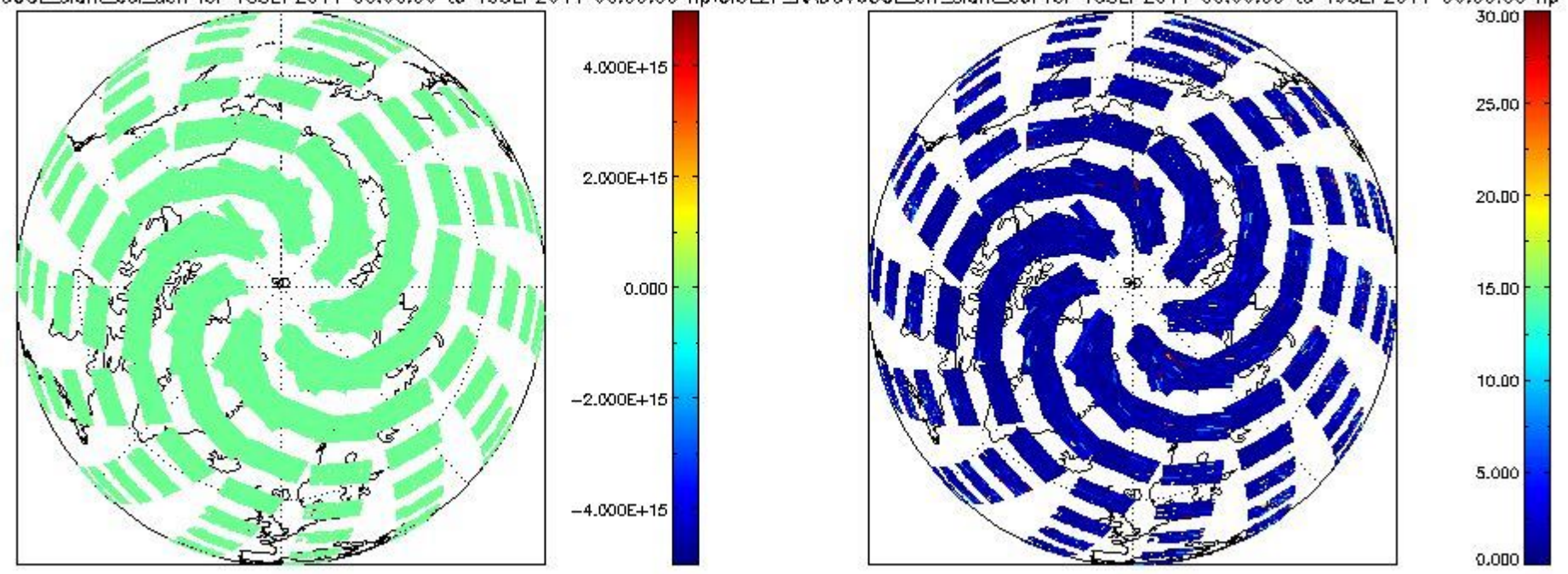
CIOL2P_NADUV60CLslant_col_den for 18SEP2011 00:00:00 to 19SEP2011 00:00:00 np; CIOL2P_NADUV60CLarr_slant_col for 18SEP2011 00:00:00 to 19SEP2011 00:00:00 np
