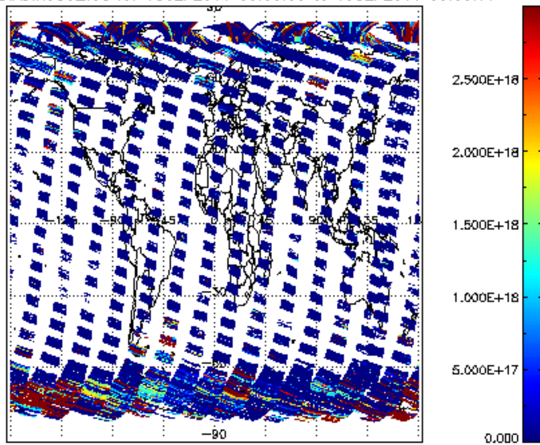
SCIOL2P_NADIR3CO_vcd for 18SEP2011 00:00:00 to 19SEP2011 00:00:00
