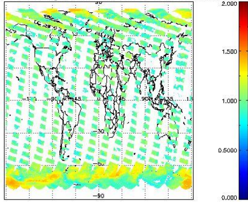
SCIOL2P_NADUV8H2O_arnf_gr for 18SEP2011 00:00:00 to 19SEP2011 00:00:00
