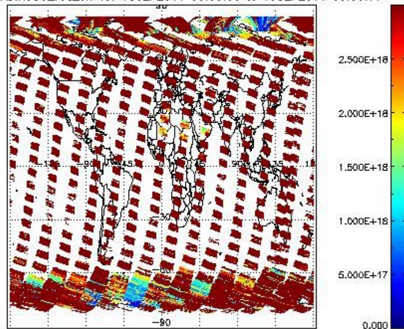
SCIDL2P_NADIR3CO_vcd_err for 18SEP2011 00:00:00 to 19SEP2011 00:00:00
