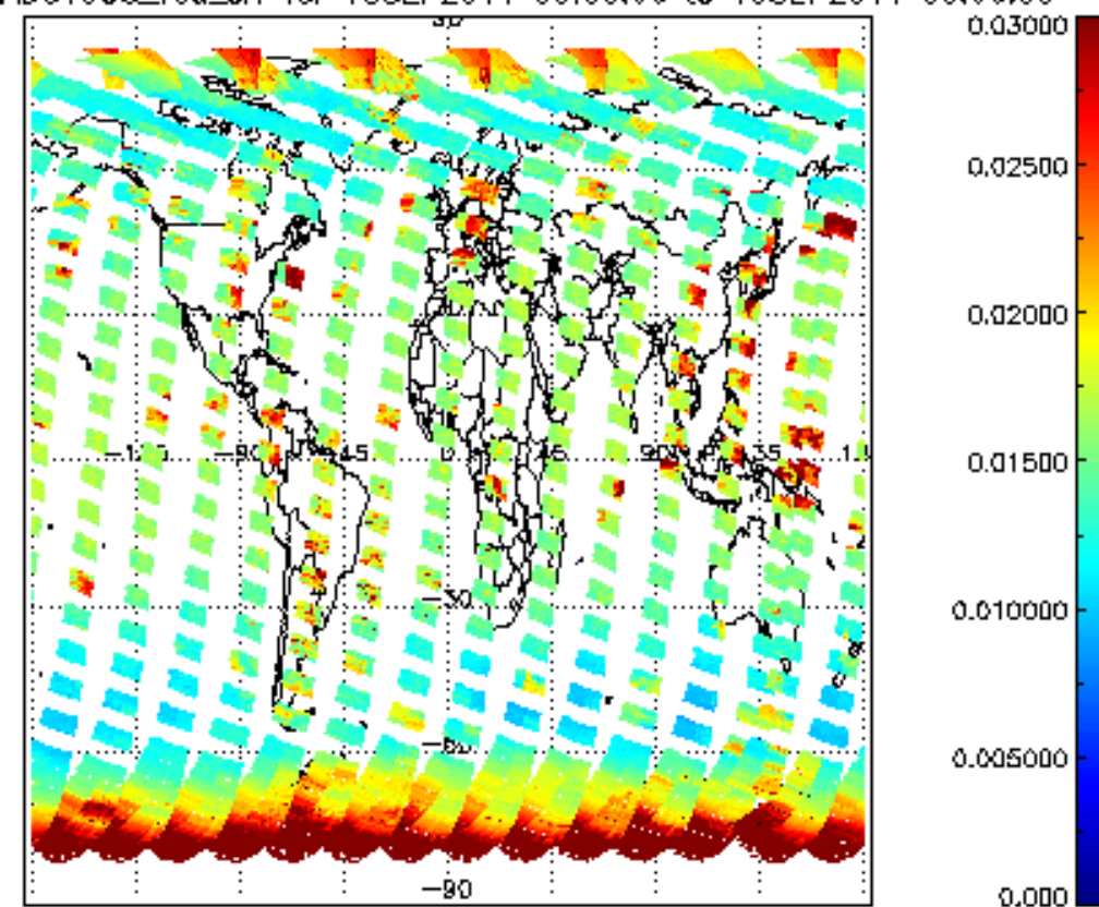
SCIOL2P_NADUV003_vcd_err for 18SEP2011 00:00:00 to 19SEP2011 00:00:00
