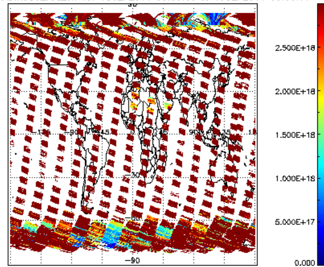
SCIOL2P_NADIR3CO_vcd_err for 18SEP2011 00:00:00 to 19SEP2011 00:00:00
