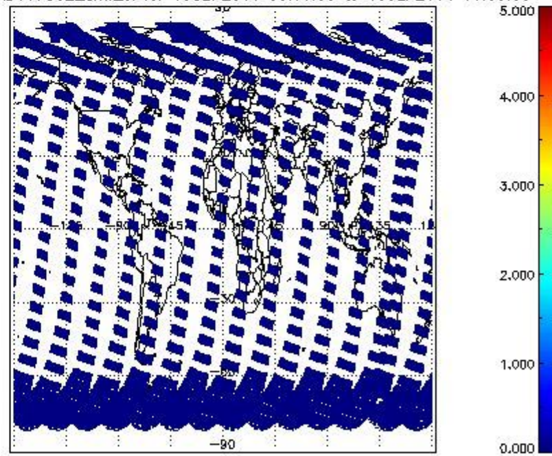
SCIOL2P_NADUV7S02_amf_cl for 18SEP2011 00:00:00 to 19SEP2011 00:00:00
