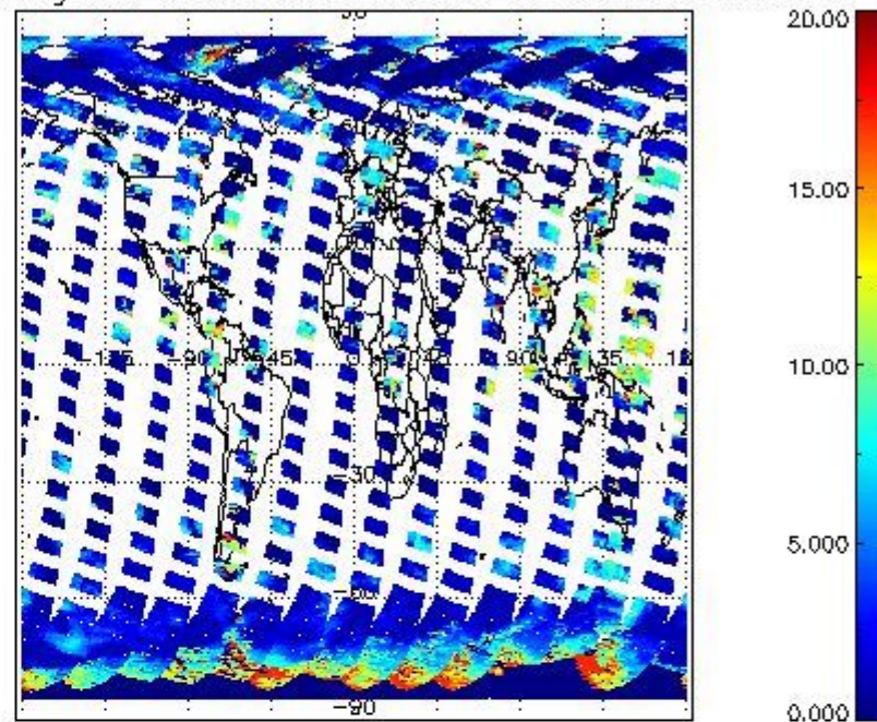
cL_top_height for 18SEP2011 00:00:00 to 19SEP2011 00:00:00
