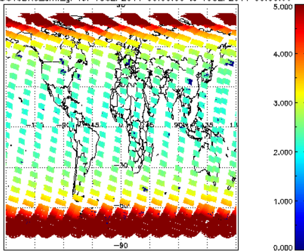
SCIOL2P_NADUV3BRO_amf_gr for 18SEP2011 00:00:00 to 19SEP2011 00:00:00
