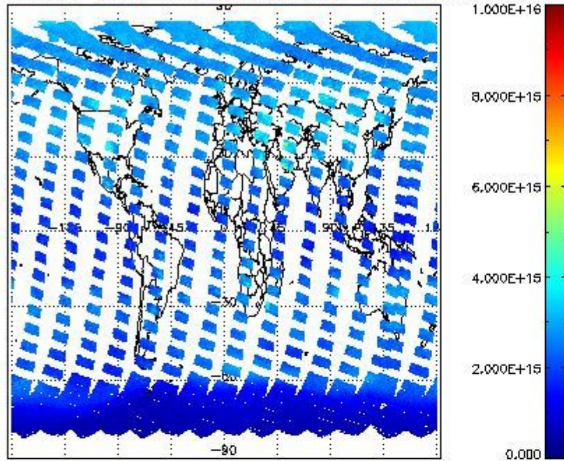
SCIOL2P_NADUV1N02_vcd for 18SEP2011 00:00:00 to 19SEP2011 00:00:00
