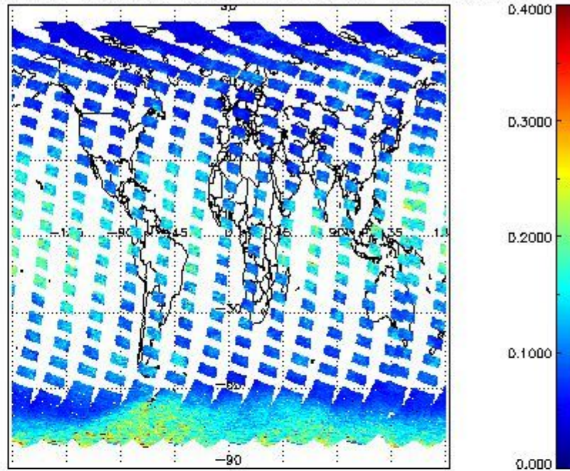
SCIOL2P_NADUV1N02_vcd_err for 18SEP2011 00:00:00 to 19SEP2011 00:00:00
