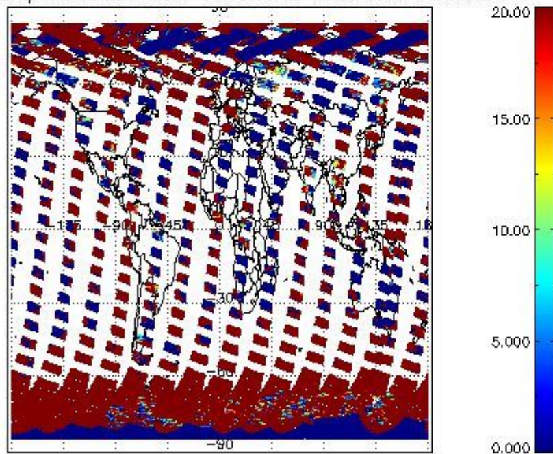
cL_opt_depth for 18SEP2011 00:00:00 to 19SEP2011 00:00:00
