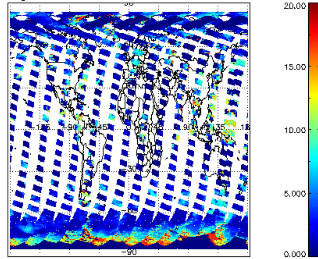
cl_top_height for 18SEP2011 00:00:00 to 19SEP2011 00:00:00
