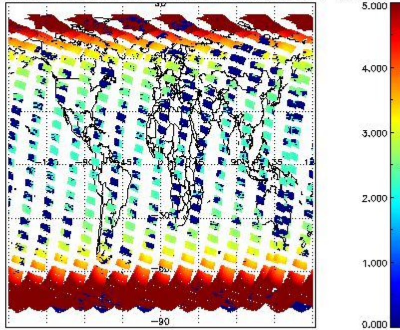
SCIOL2P_NADUV1N02_amf_cl for 18SEP2011 00:00:00 to 19SEP2011 00:00:00
