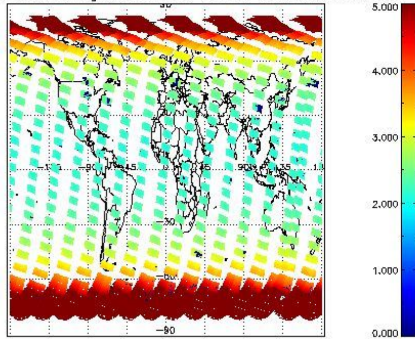
SCIOL2P_NADUV3BRO_amf_gr for 18SEP2011 00:00:00 to 19SEP2011 00:00:00
