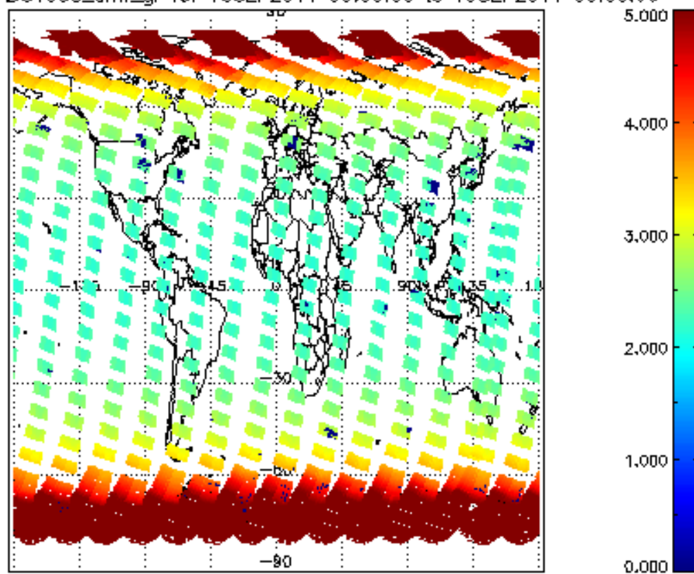
SCIOL2P_NADUV003_amf_gr for 18SEP2011 00:00:00 to 19SEP2011 00:00:00
