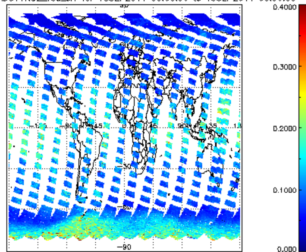
SCIOL2P_NADUV1NO2_vcd_err for 18SEP2011 00:00:00 to 19SEP2011 00:00:00
