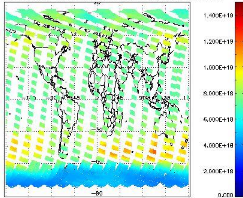
SCIOL2P_NADUV003_vcd for 18SEP2011 00:00:00 to 19SEP2011 00:00:00
