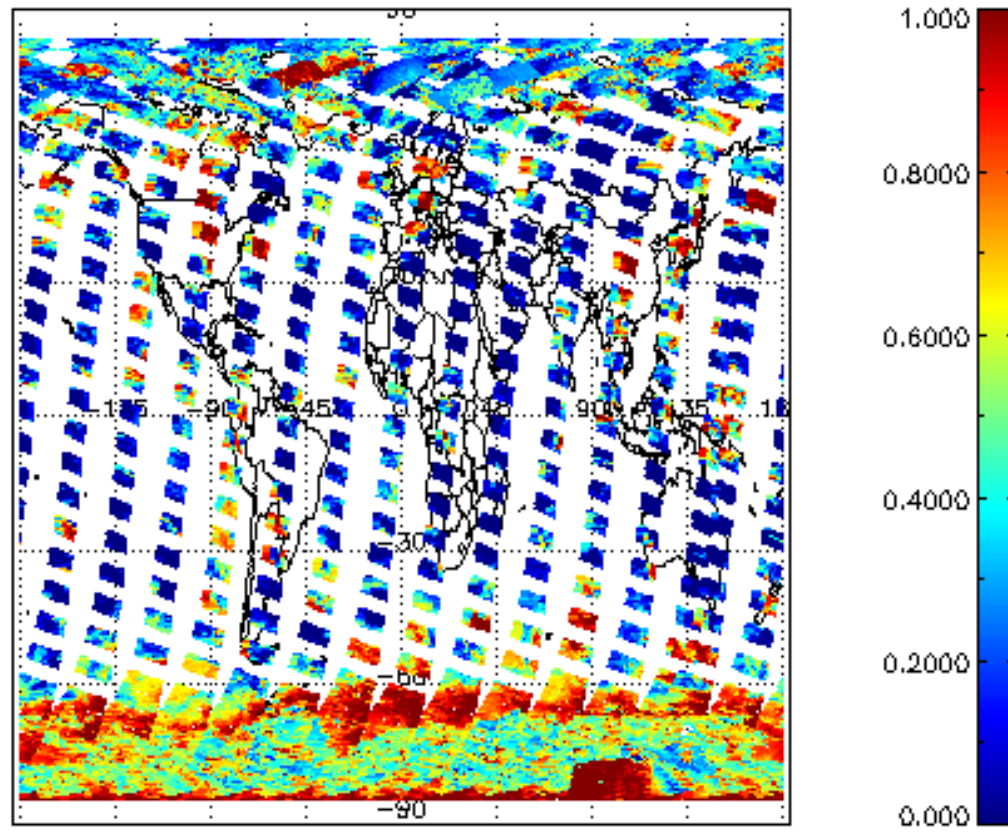
cl_frac for 18SEP2011 00:00:00 to 19SEP2011 00:00:00
