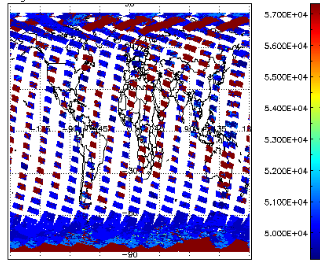
cloud_flags for 18SEP2011 00:00:00 to 19SEP2011 00:00:00
