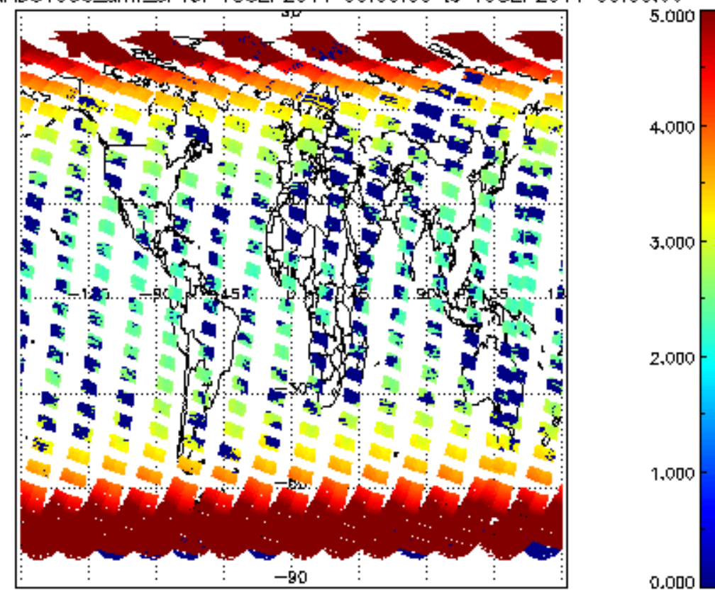
SCIOL2P_NADUV003_amf_cl for 18SEP2011 00:00:00 to 19SEP2011 00:00:00
