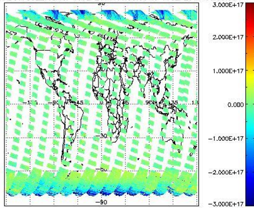
SCIOL2P_NADUV7S02_vcd for 18SEP2011 00:00:00 to 19SEP2011 00:00:00
