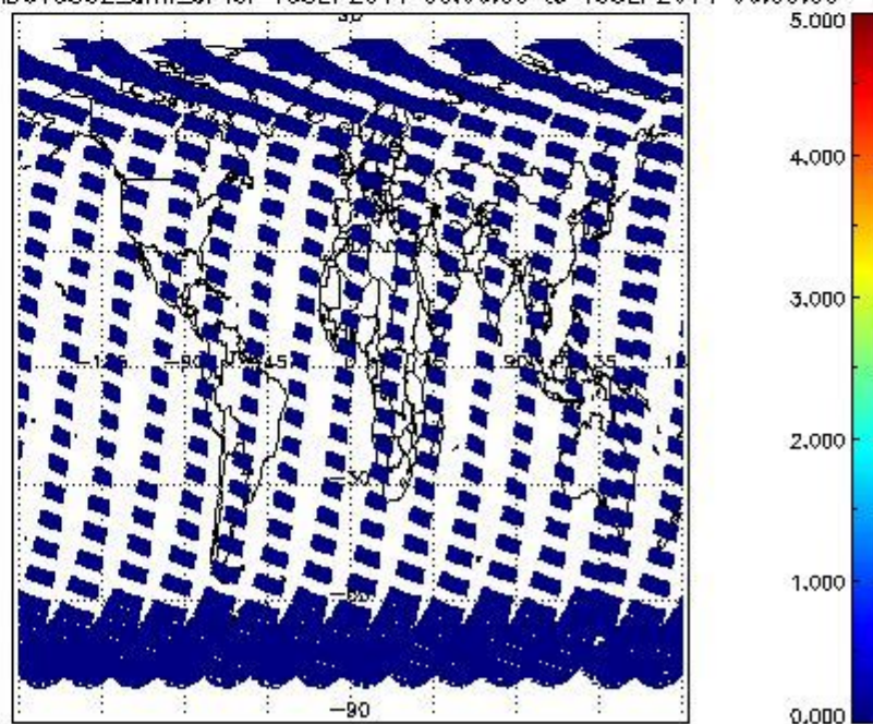
SCIOL2P_NADUV5S02_amf_cl for 18SEP2011 00:00:00 to 19SEP2011 00:00:00
