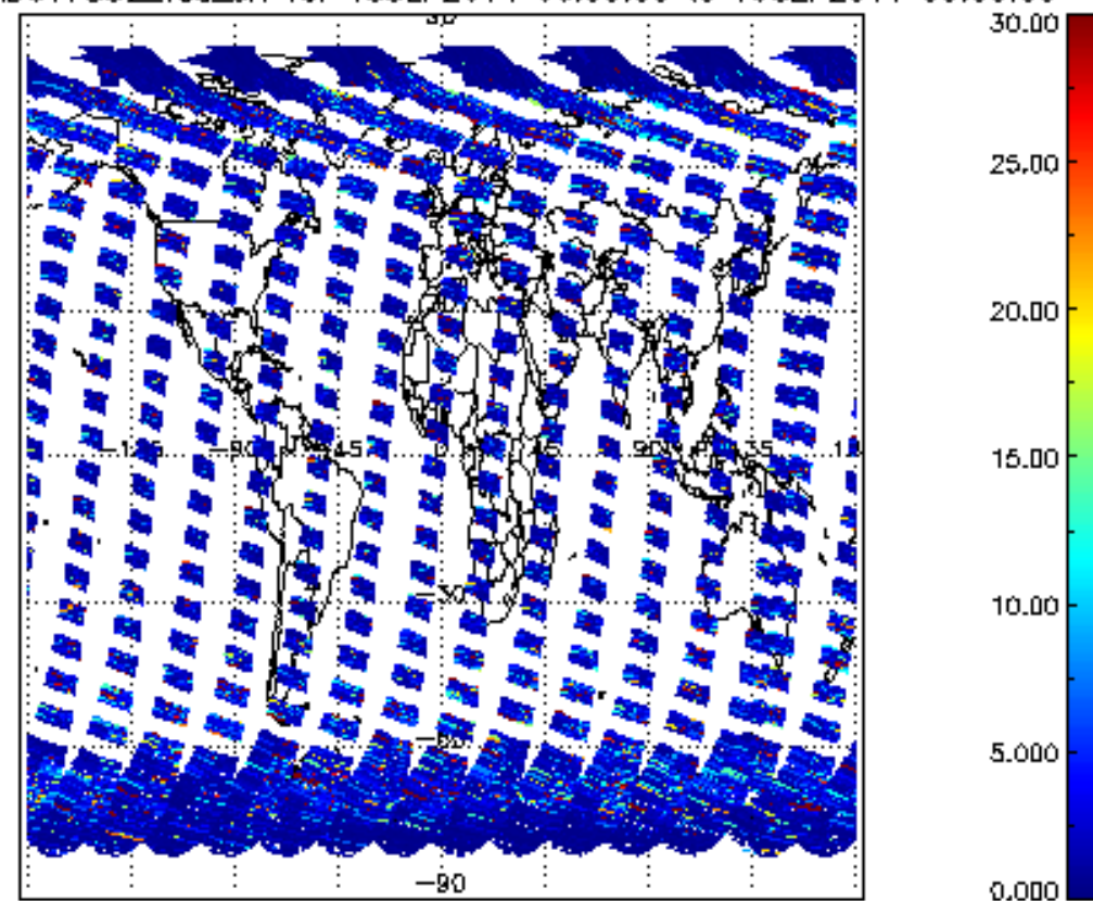
SCIOL2P_NADUV7S02_vcd_err for 18SEP2011 00:00:00 to 19SEP2011 00:00:00
