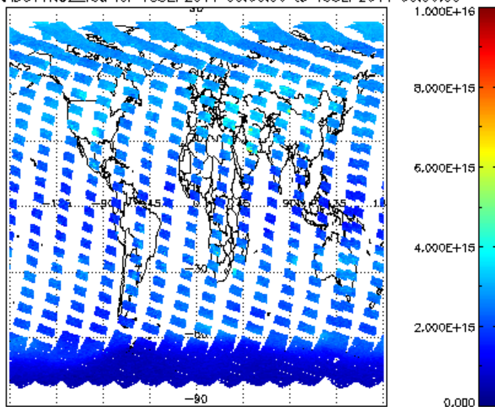
SCIOL2P_NADUV1NO2_vcd for 18SEP2011 00:00:00 to 19SEP2011 00:00:00
