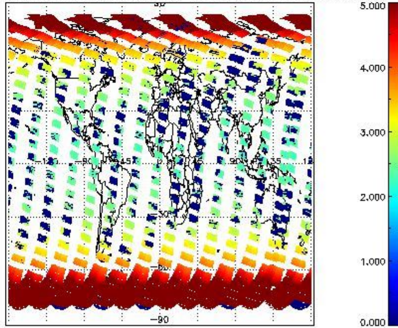
SCIOL2P_NADUV003_amf_cl for 18SEP2011 00:00:00 to 19SEP2011 00:00:00
