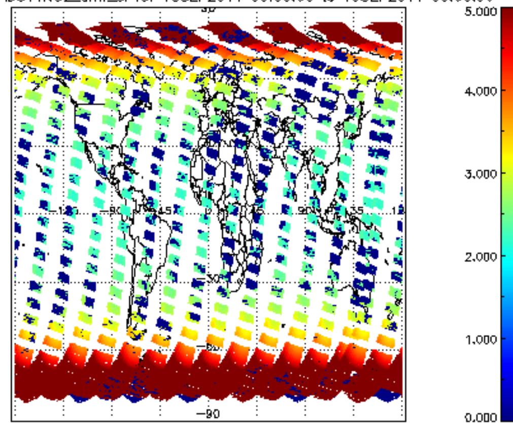
SCIOL2P_NADUV1NO2_amf_cl for 18SEP2011 00:00:00 to 19SEP2011 00:00:00
