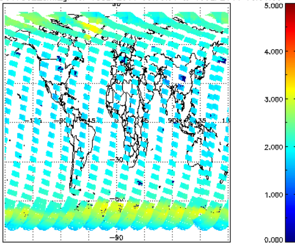
SCIOL2P_NADUV7S02_amf_gr for 18SEP2011 00:00:00 to 19SEP2011 00:00:00
