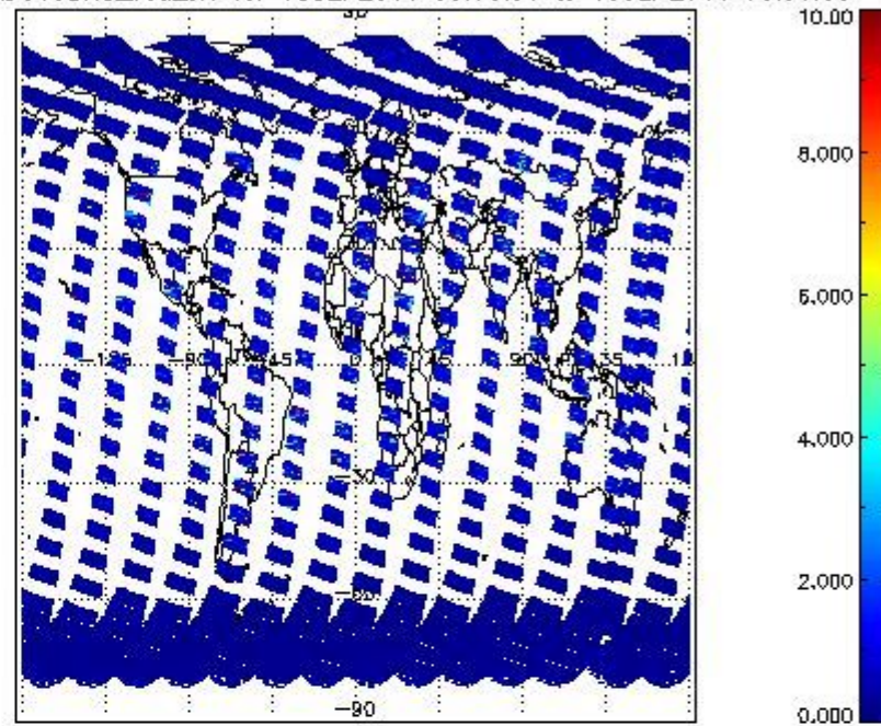
SCIOL2P_NADUV3BRO_vcd_err for 18SEP2011 00:00:00 to 19SEP2011 00:00:00
