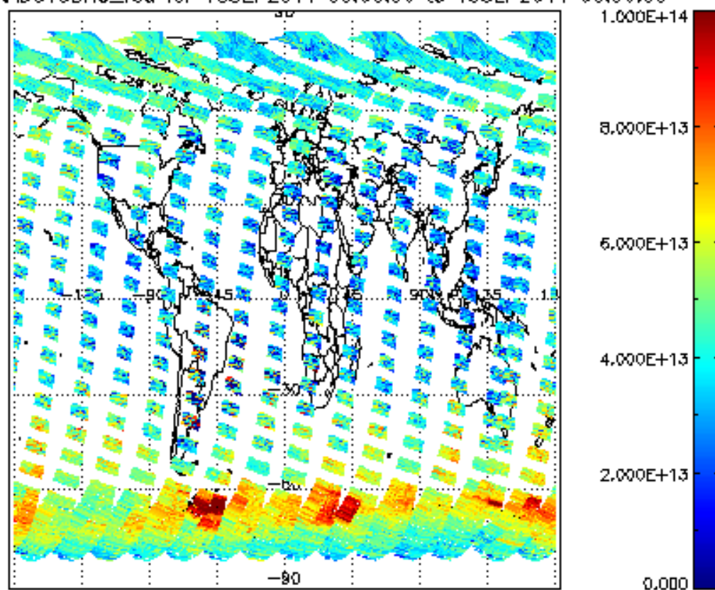
SCIOL2P_NADUV3BRO_vcd for 18SEP2011 00:00:00 to 19SEP2011 00:00:00
