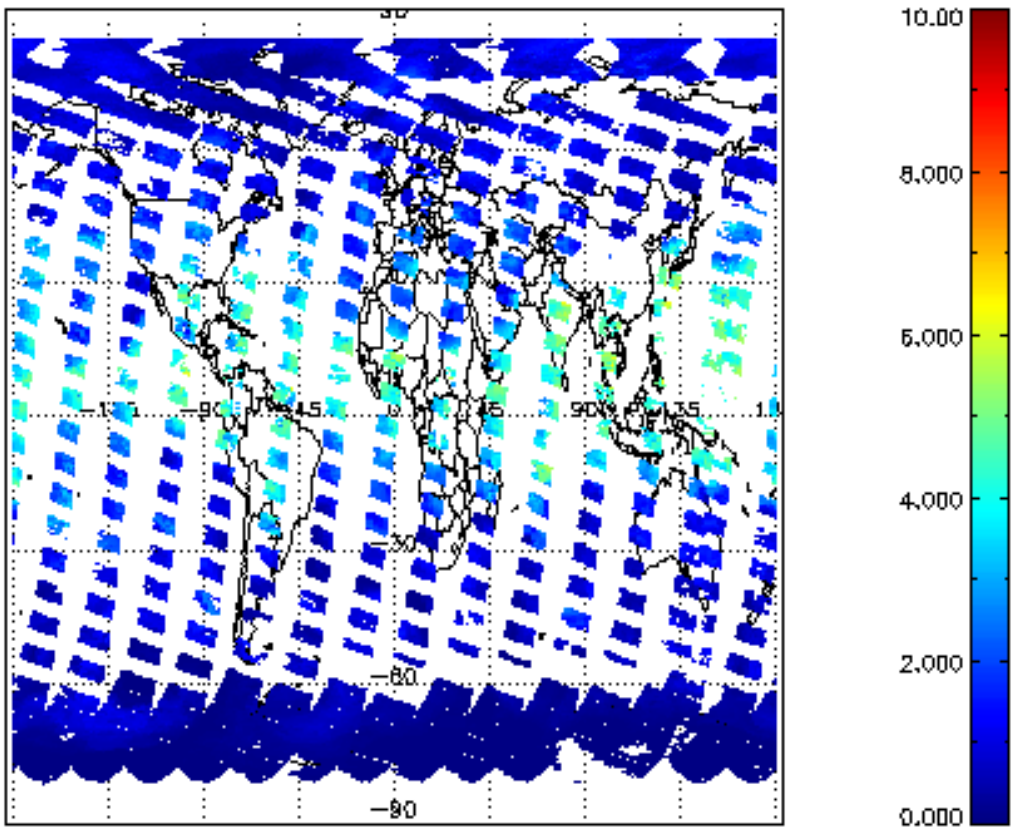
SCIOL2P_NADUV8H20_vcd for 18SEP2011 00:00:00 to 19SEP2011 00:00:00
