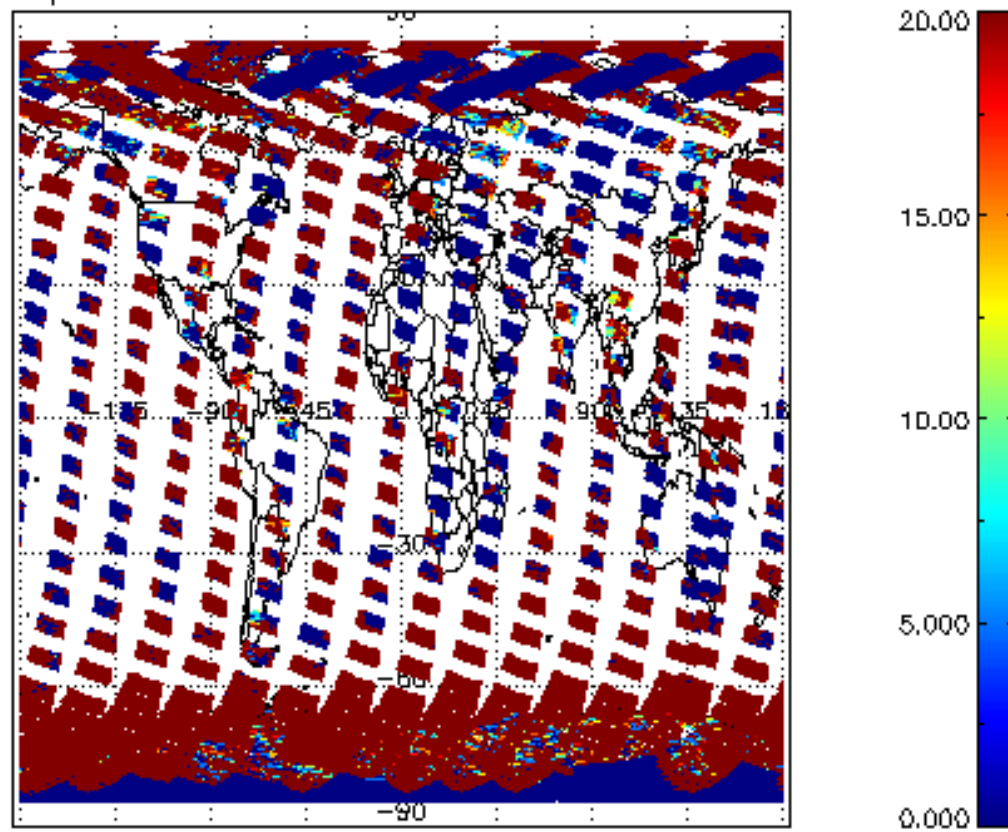
cl_opt_depth for 18SEP2011 00:00:00 to 19SEP2011 00:00:00
