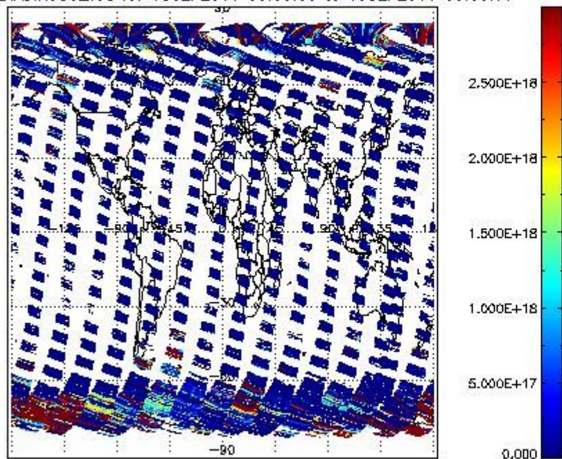
SCIDL2P_NADIR3CO_vcd for 18SEP2011 00:00:00 to 19SEP2011 00:00:00
