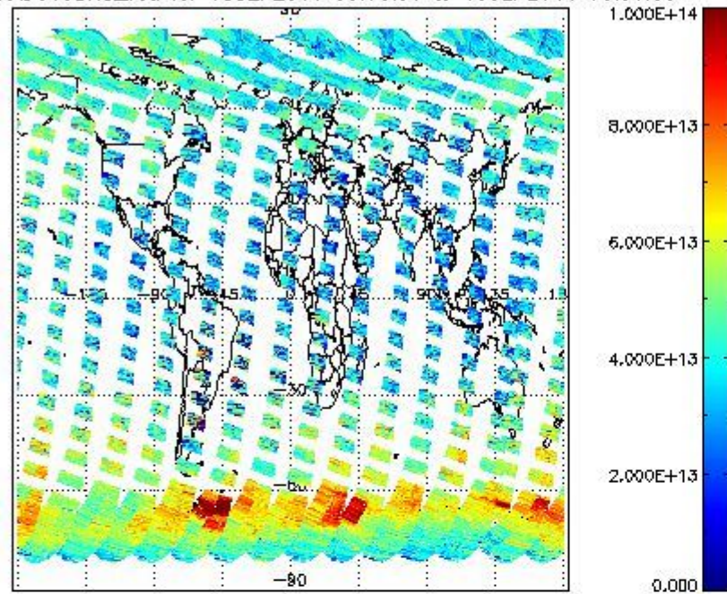
SCIOL2P_NADUV3BRO_vcd for 18SEP2011 00:00:00 to 19SEP2011 00:00:00
