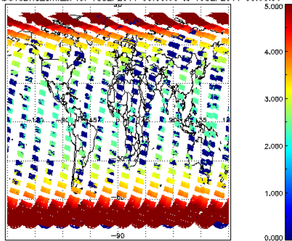
SCIOL2P_NADUV3BRO_amf_sl for 18SEP2011 00:00:00 to 19SEP2011 00:00:00
