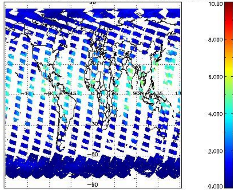
SCIOL2P_NADUV8H2O_vcd for 18SEP2011 00:00:00 to 19SEP2011 00:00:00
