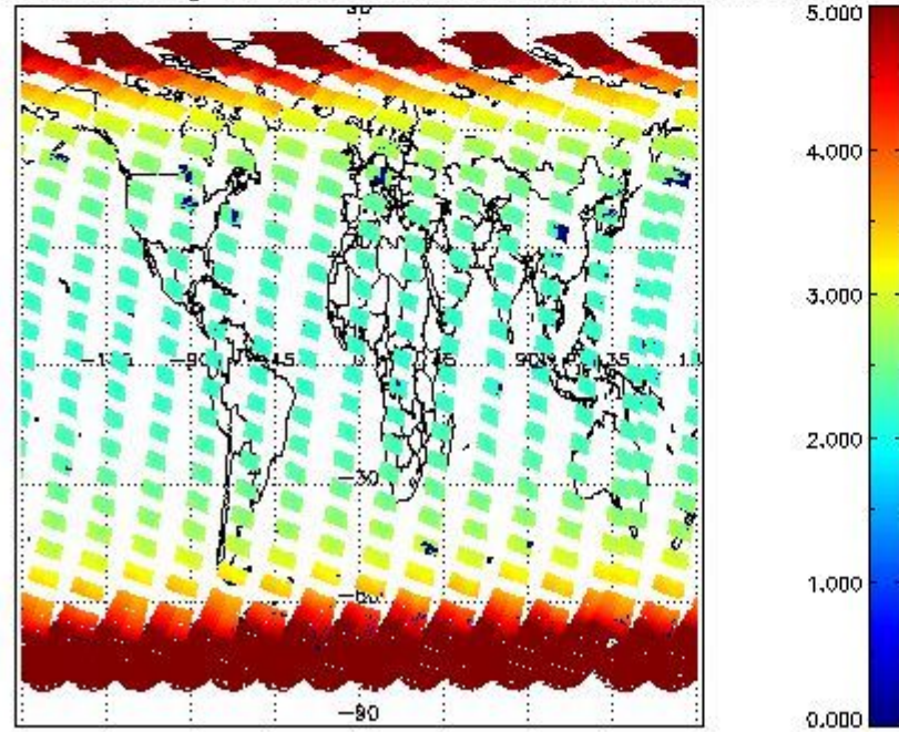
SCIOL2P_NADUV003_amf_gr for 18SEP2011 00:00:00 to 19SEP2011 00:00:00
