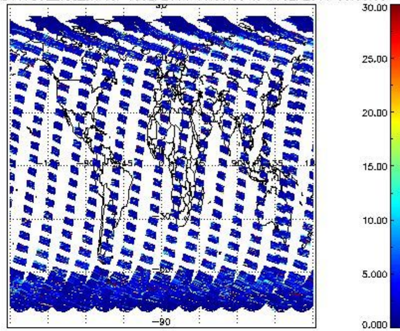
SCIOL2P_NADUV7S02_vcd_err for 18SEP2011 00:00:00 to 19SEP2011 00:00:00
