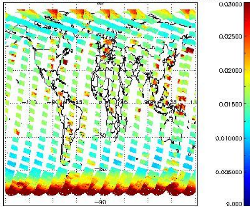
SCIOL2P_NADUV003_vcd_err for 18SEP2011 00:00:00 to 19SEP2011 00:00:00
