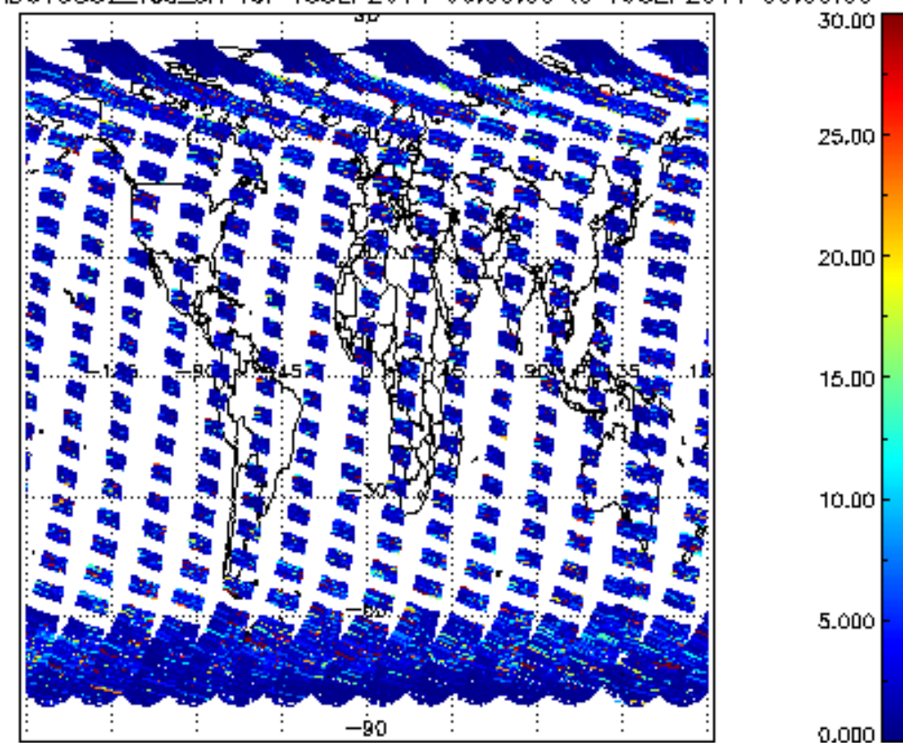
SCIOL2P_NADUV5S02_vcd_err for 18SEP2011 00:00:00 to 19SEP2011 00:00:00
