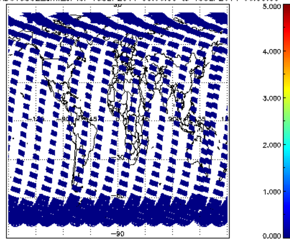
SCIOL2P_NADUV5S02_amf_cl for 18SEP2011 00:00:00 to 19SEP2011 00:00:00
