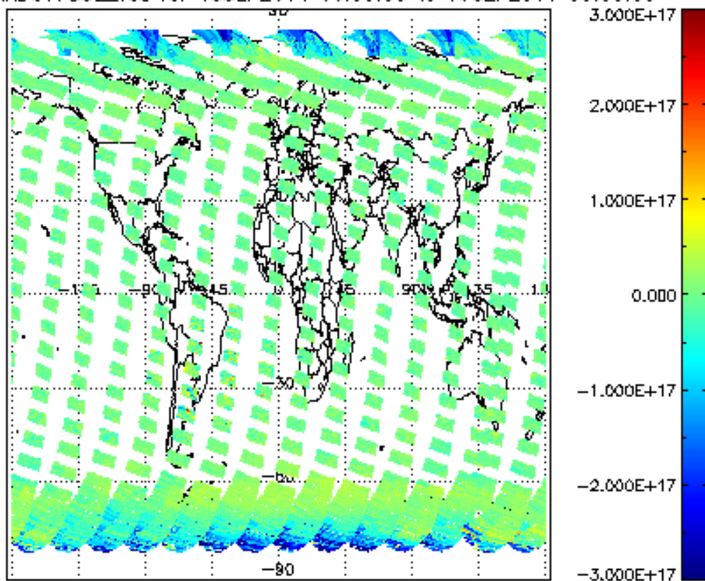
SCIOL2P_NADUV7S02_vcd for 18SEP2011 00:00:00 to 19SEP2011 00:00:00
