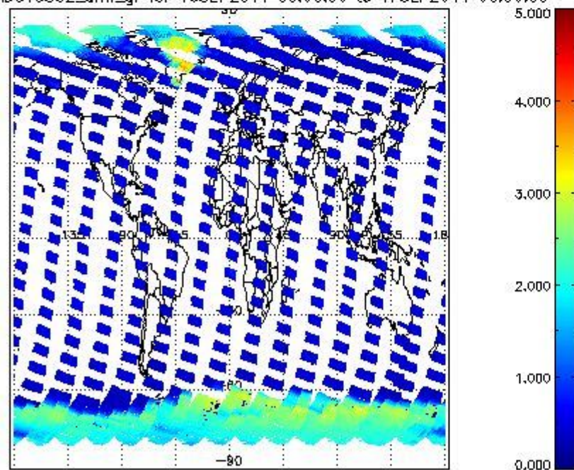
SCIOL2P_NADUV5S02_amf_gr for 16SEP2011 00:00:00 to 17SEP2011 00:00:00
