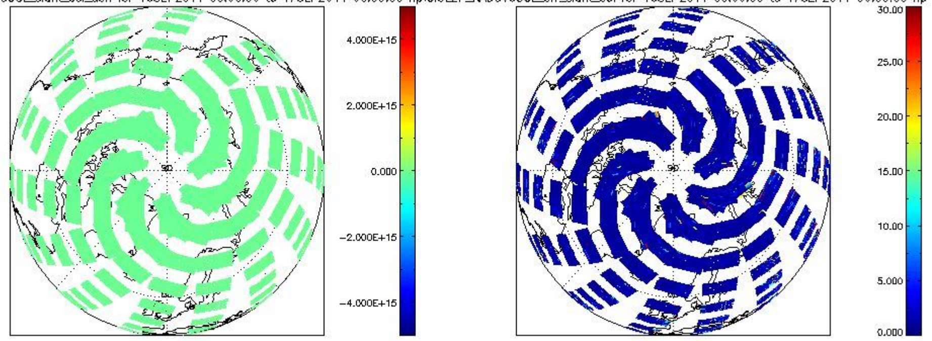
CIOL2P_NADUV6OCLslant_col_den for 16SEP2011 00:00:00 to 17SEP2011 00:00:00 np; CIOL2P_NADUV6OCLerr_slant_col for 16SEP2011 00:00:00 to 17SEP2011 00:00:00 np
