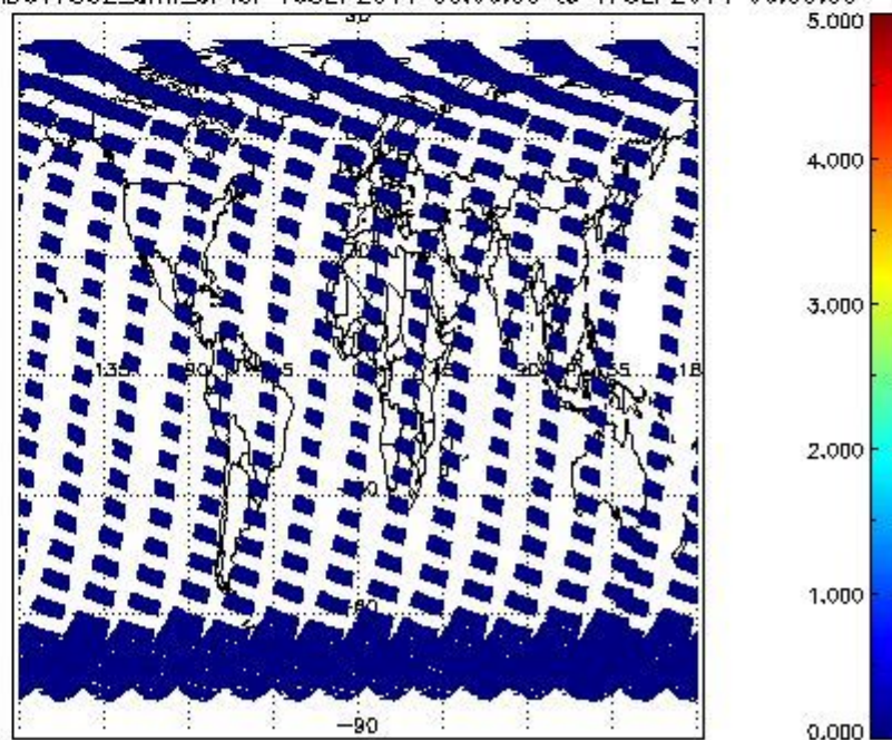
SCIOL2P_NADUV7S02_amf_cl for 16SEP2011 00:00:00 to 17SEP2011 00:00:00
