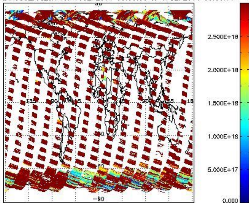
SCIOL2P_NADIR3CO_vcd_err for 16SEP2011 00:00:00 to 17SEP2011 00:00:00
