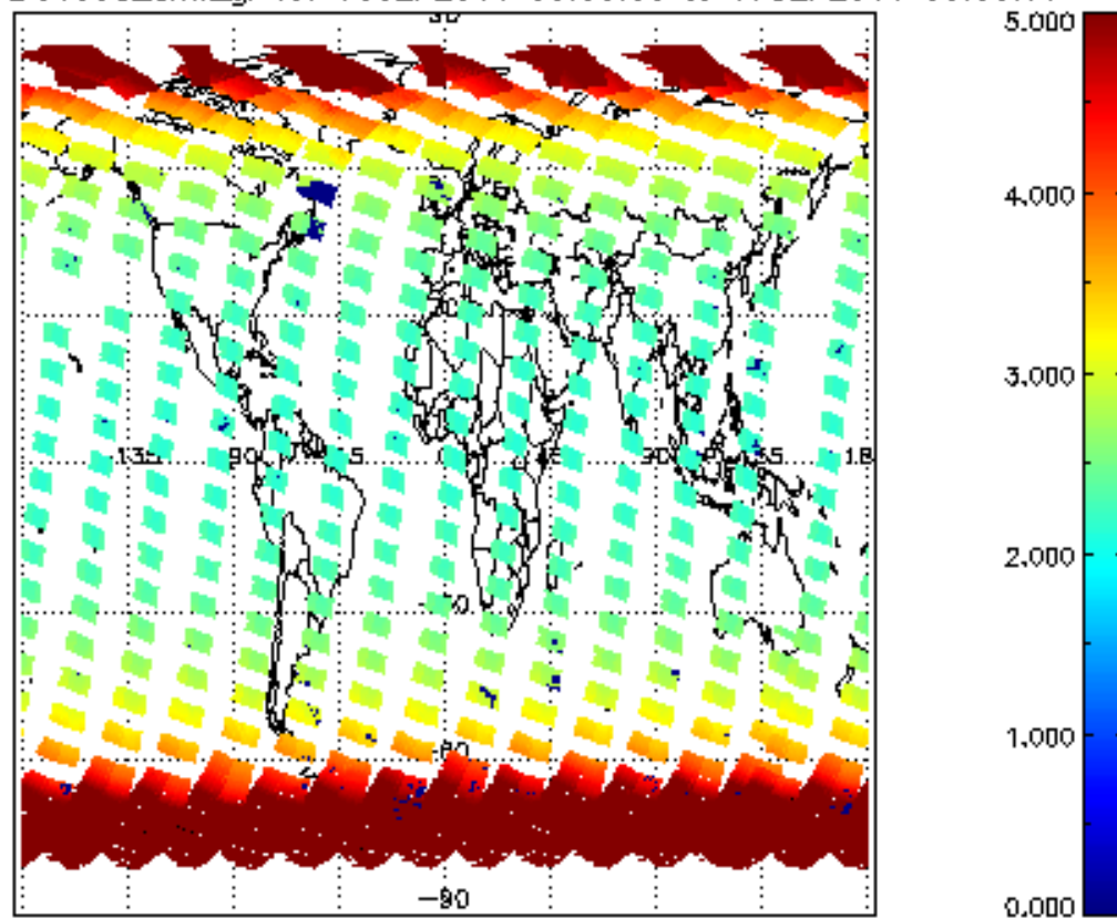
SCIOL2P_NADUV003_amf_gr for 16SEP2011 00:00:00 to 17SEP2011 00:00:00
