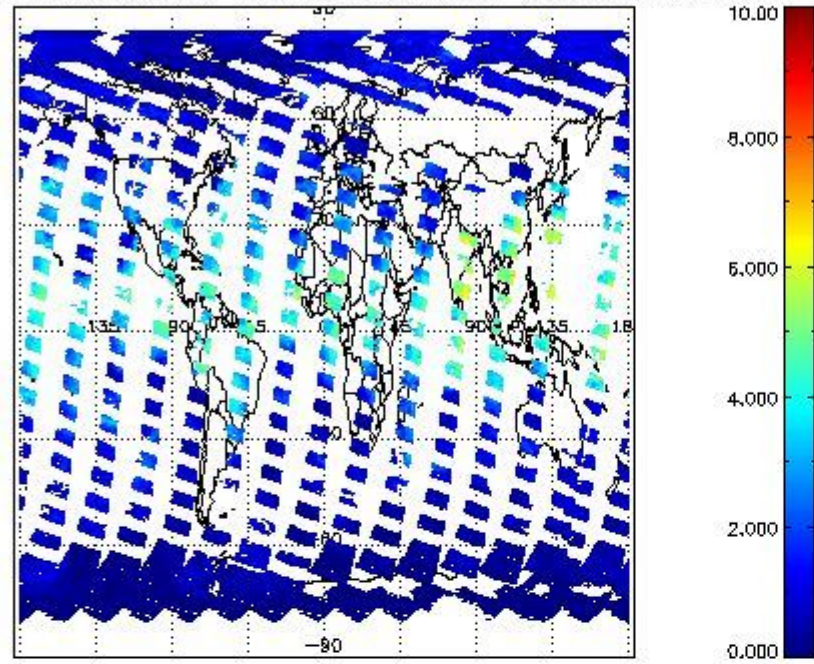
SCIOL2P_NADUV8H2O_vcd for 16SEP2011 00:00:00 to 17SEP2011 00:00:00
