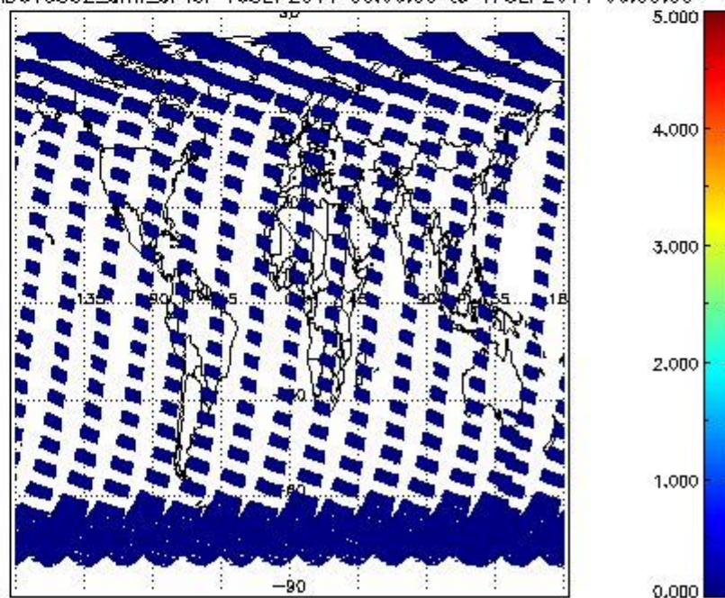
SCIOL2P_NADUV5S02_amf_cl for 16SEP2011 00:00:00 to 17SEP2011 00:00:00
