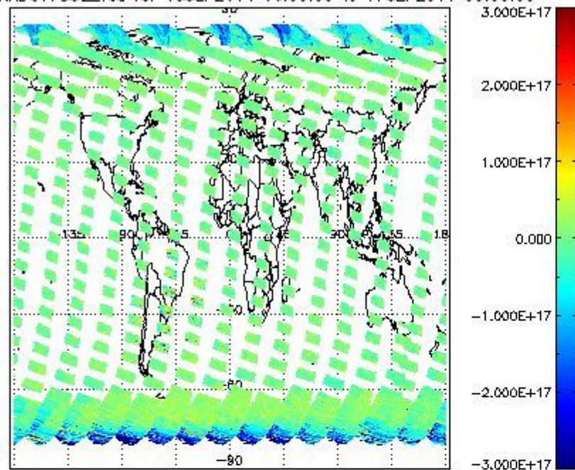
SCIOL2P_NADUV7S02_vcd for 16SEP2011 00:00:00 to 17SEP2011 00:00:00
