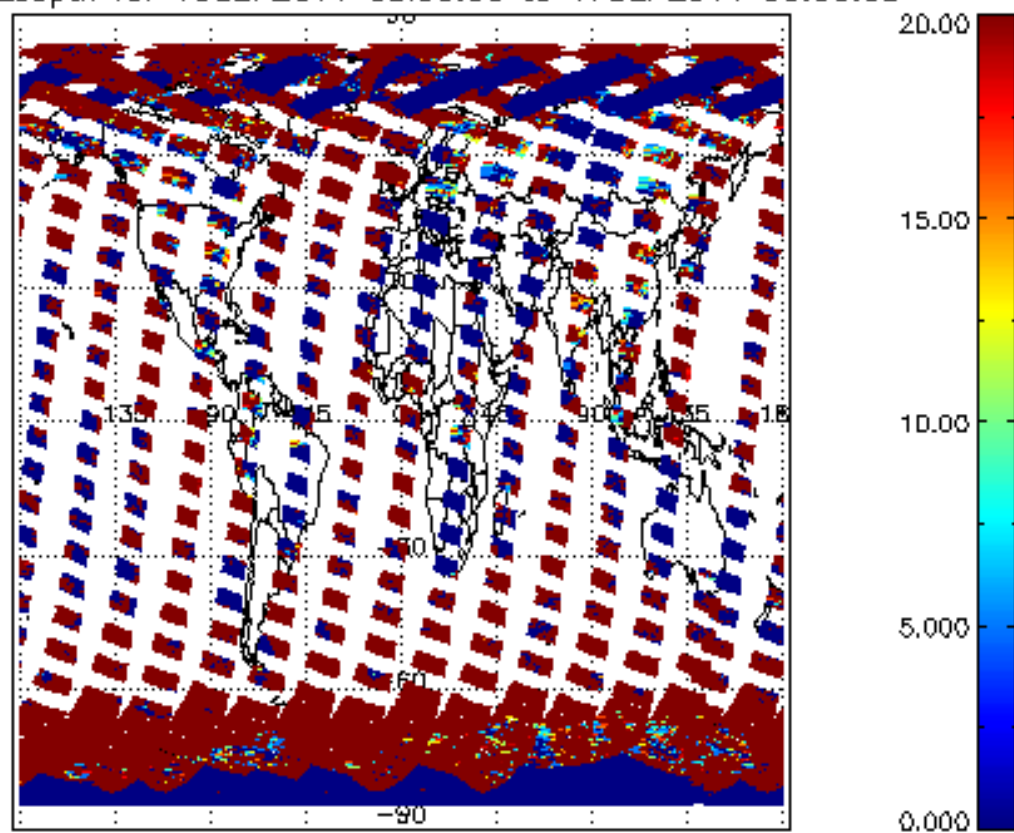
cL_opt_depth for 16SEP2011 00:00:00 to 17SEP2011 00:00:00
