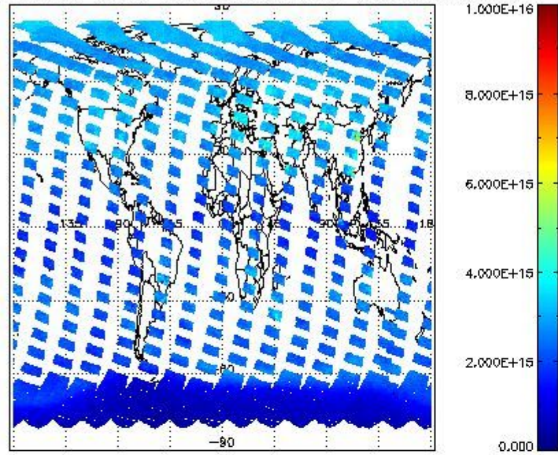
SCIOL2P_NADUV1N02_vcd for 16SEP2011 00:00:00 to 17SEP2011 00:00:00
