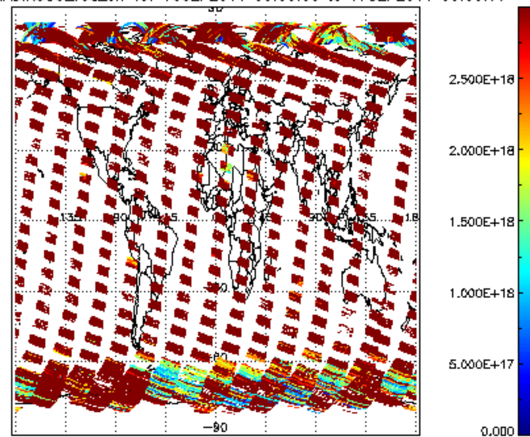
SCIOL2P_NADIR3CO_vcd_err for 16SEP2011 00:00:00 to 17SEP2011 00:00:00
