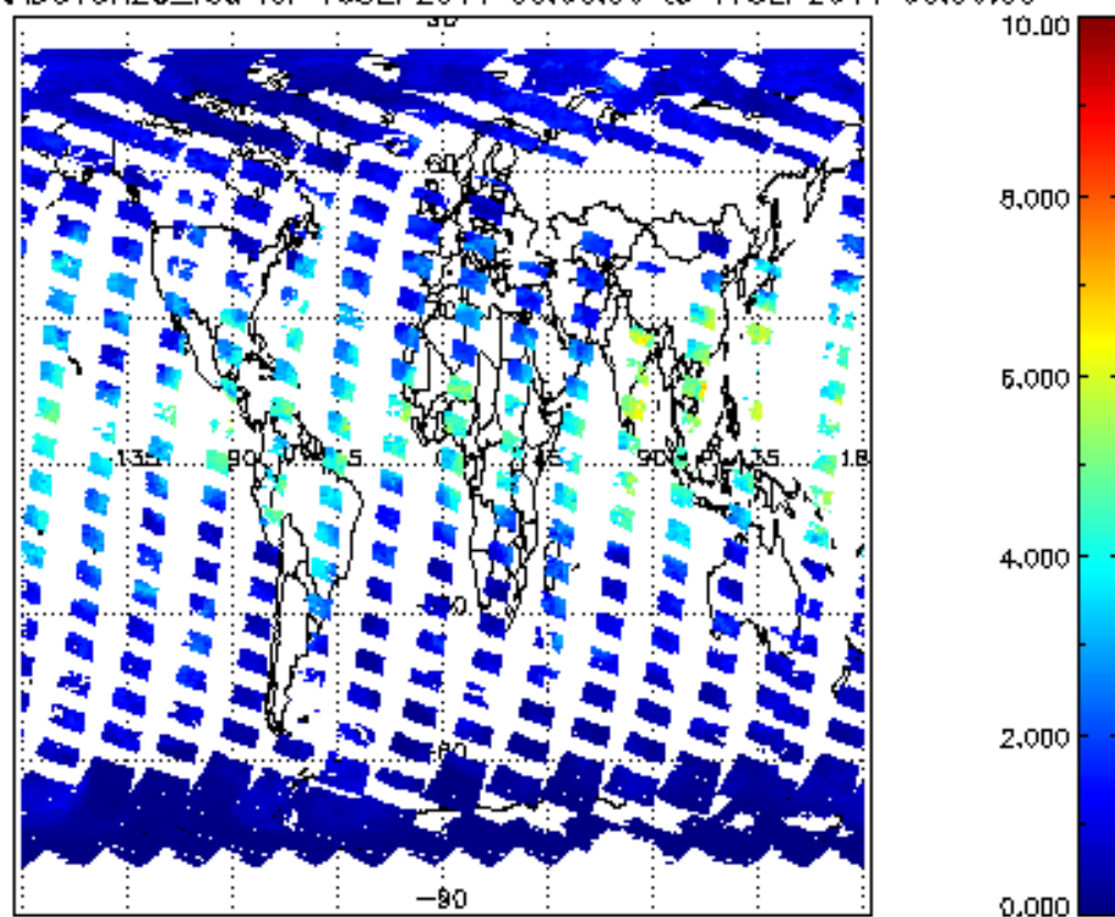
SCIOL2P_NADUV8H2O_vcd for 16SEP2011 00:00:00 to 17SEP2011 00:00:00
