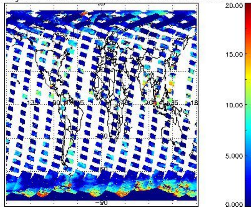
cL_top_height for 16SEP2011 00:00:00 to 17SEP2011 00:00:00
