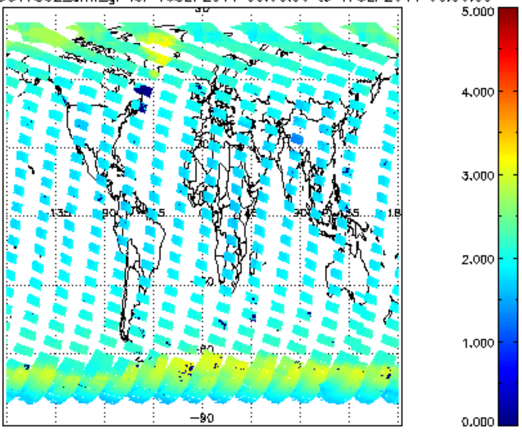
SCIOL2P_NADUV7S02_amf_gr for 16SEP2011 00:00:00 to 17SEP2011 00:00:00
