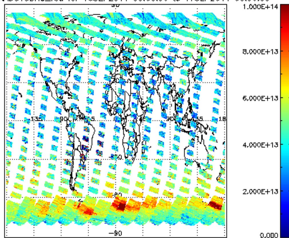
SCIOL2P_NADUV3BRO_vcd for 16SEP2011 00:00:00 to 17SEP2011 00:00:00
