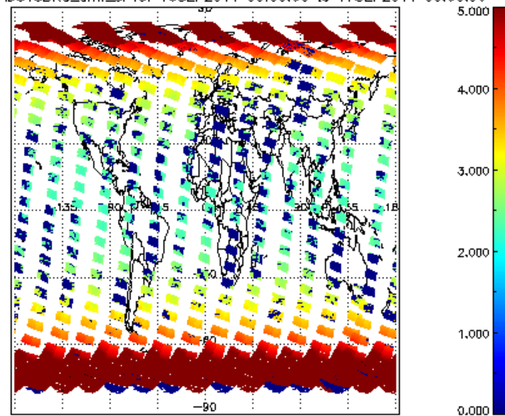
SCIOL2P_NADUV3BRO_amf_sl for 16SEP2011 00:00:00 to 17SEP2011 00:00:00
