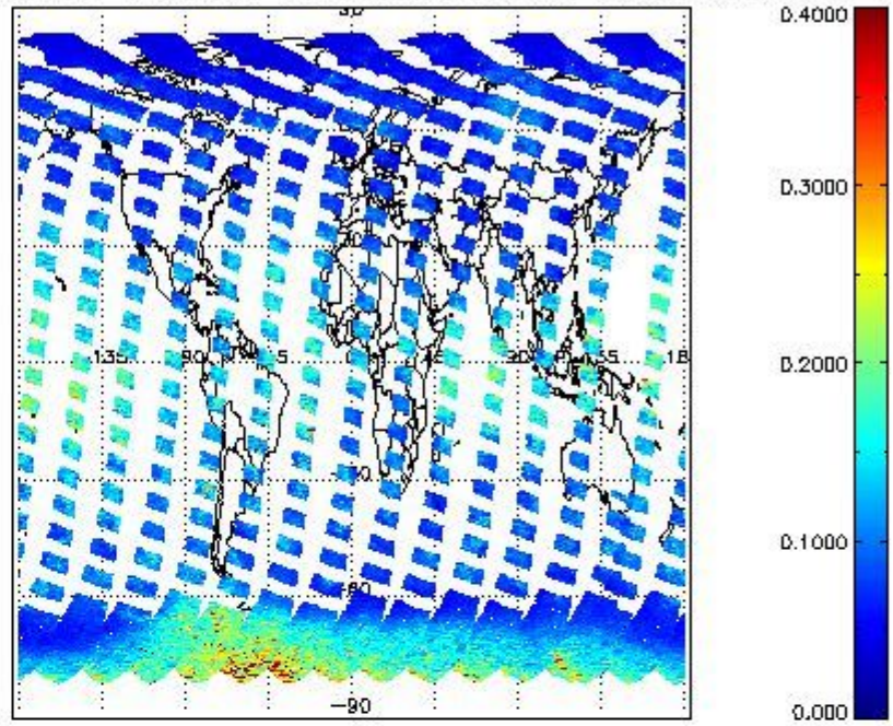
SCIOL2P_NADUV1N02_vcd_err for 16SEP2011 00:00:00 to 17SEP2011 00:00:00
