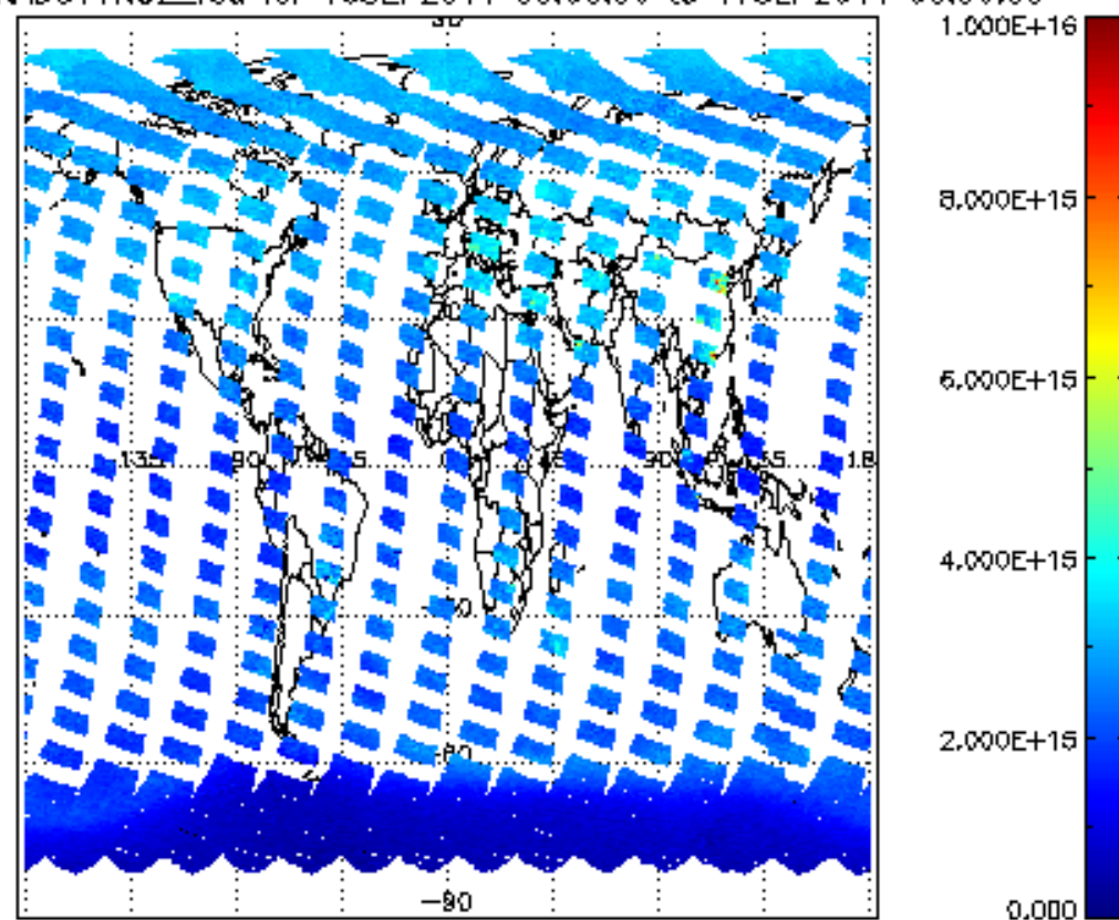
SCIOL2P_NADUV1NO2_vcd for 16SEP2011 00:00:00 to 17SEP2011 00:00:00
