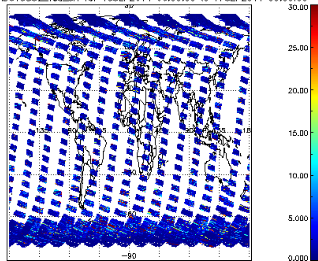
SCIOL2P_NADUV5S02_vcd_err for 16SEP2011 00:00:00 to 17SEP2011 00:00:00
