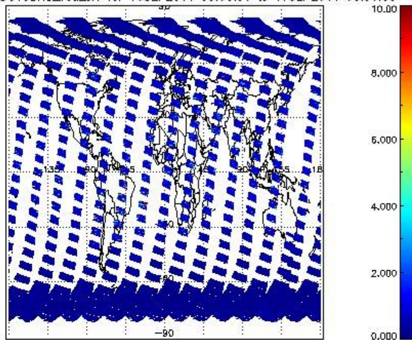
SCIOL2P_NADUV3BRO_vcd_err for 16SEP2011 00:00:00 to 17SEP2011 00:00:00
