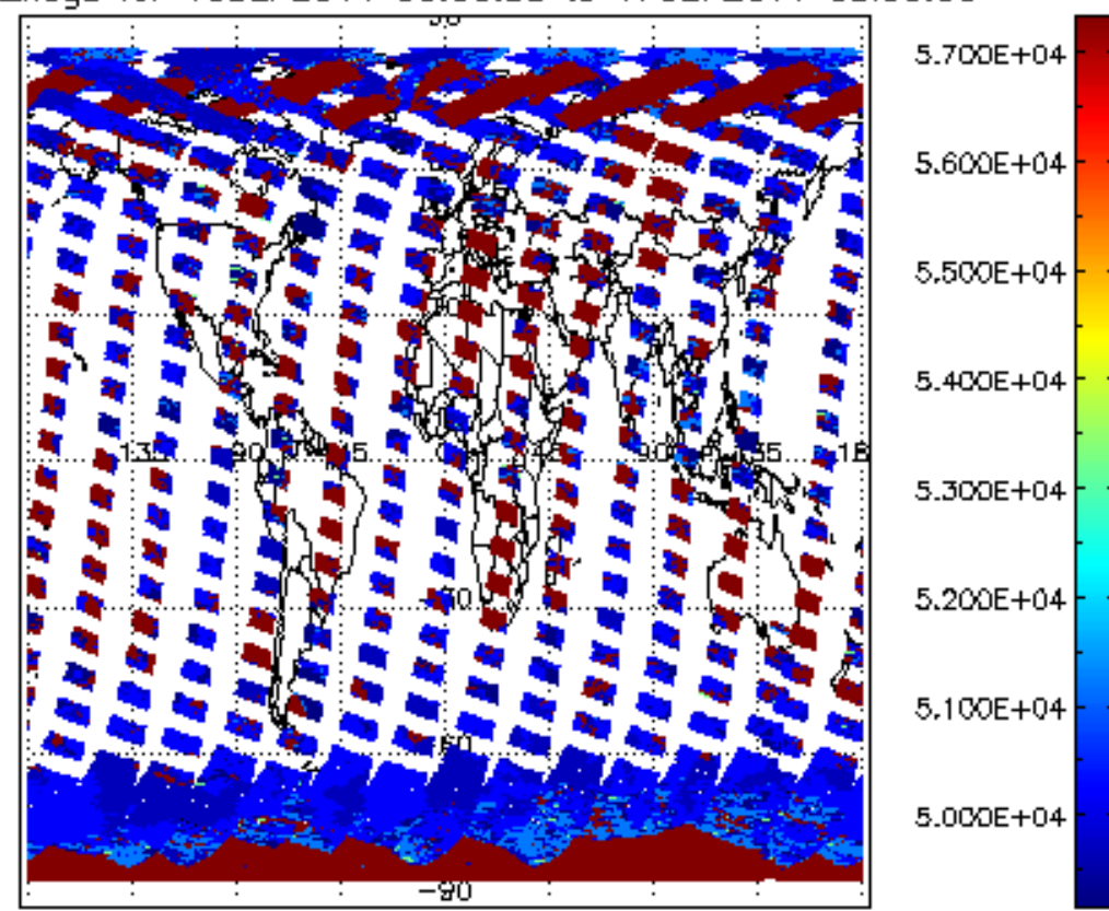
cloud_flags for 16SEP2011 00:00:00 to 17SEP2011 00:00:00
