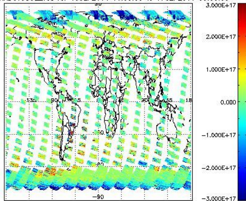
SCIOL2P_NADUV5S02_vcd for 16SEP2011 00:00:00 to 17SEP2011 00:00:00
