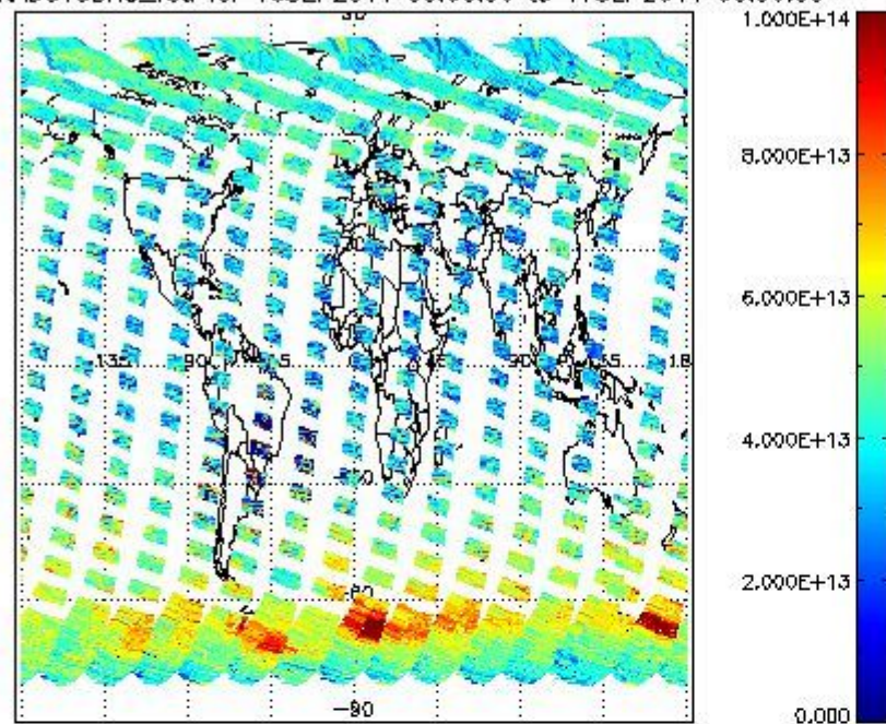
SCIOL2P_NADUV3BRO_vcd for 16SEP2011 00:00:00 to 17SEP2011 00:00:00
