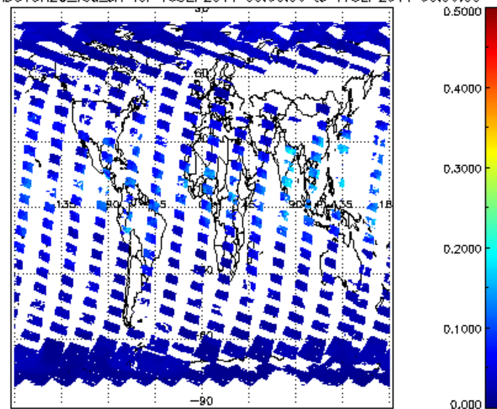
SCIOL2P_NADUV8H2O_vcd_err for 16SEP2011 00:00:00 to 17SEP2011 00:00:00
