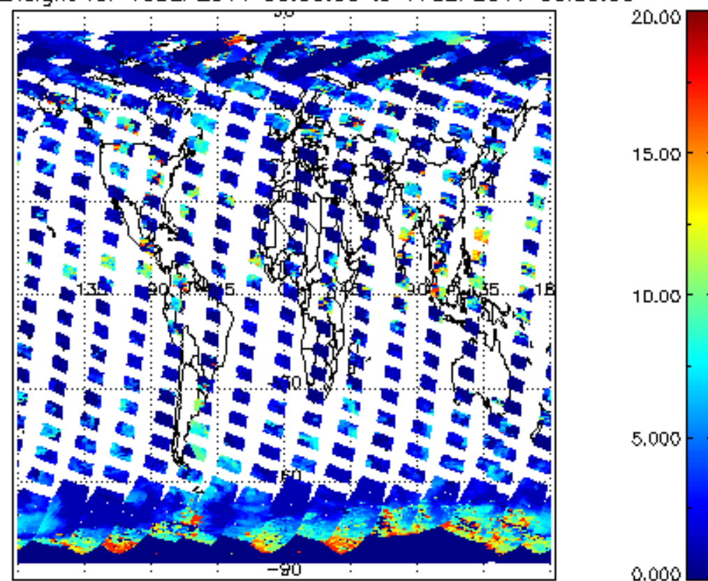
cL_top_height for 16SEP2011 00:00:00 to 17SEP2011 00:00:00
