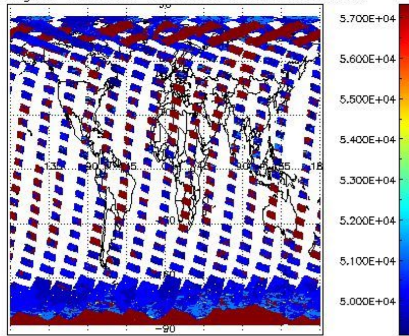
cloud_flags for 16SEP2011 00:00:00 to 17SEP2011 00:00:00
