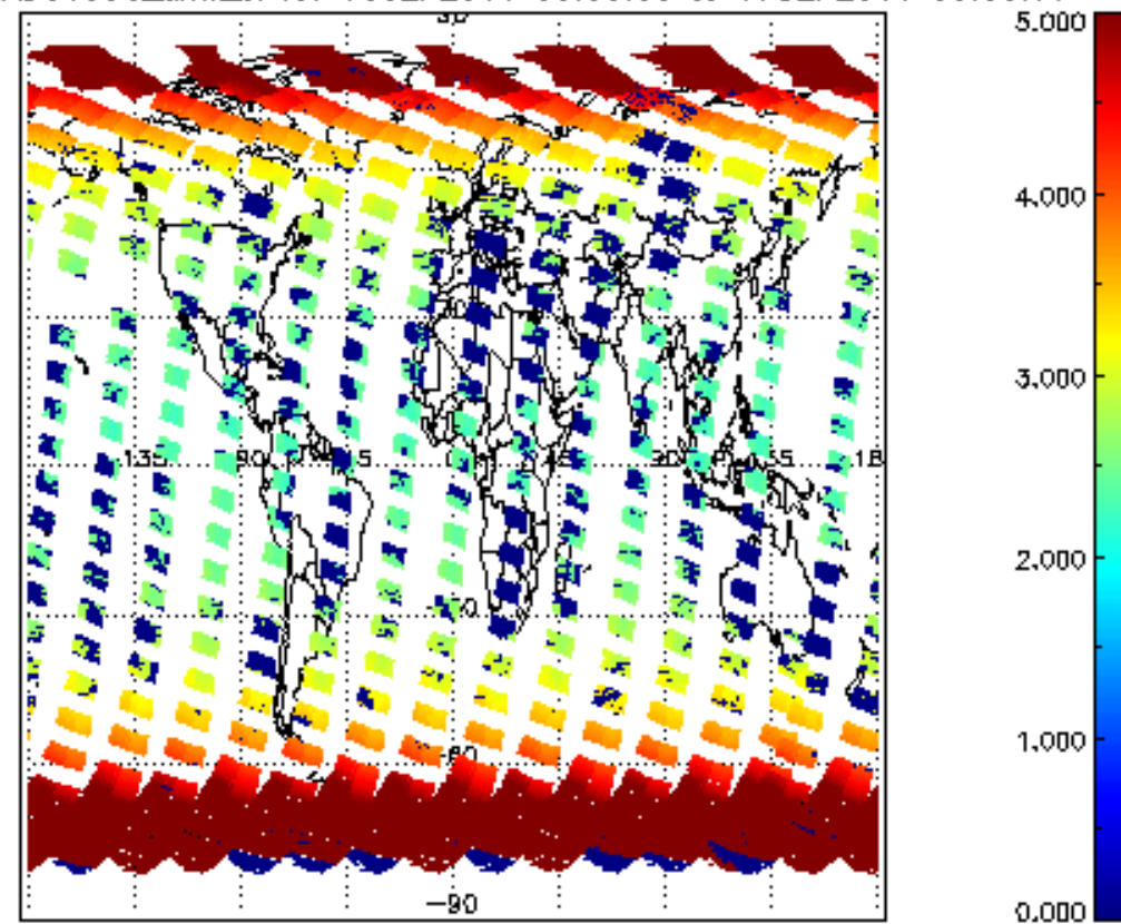
SCIOL2P_NADUV003_amf_cl for 16SEP2011 00:00:00 to 17SEP2011 00:00:00
