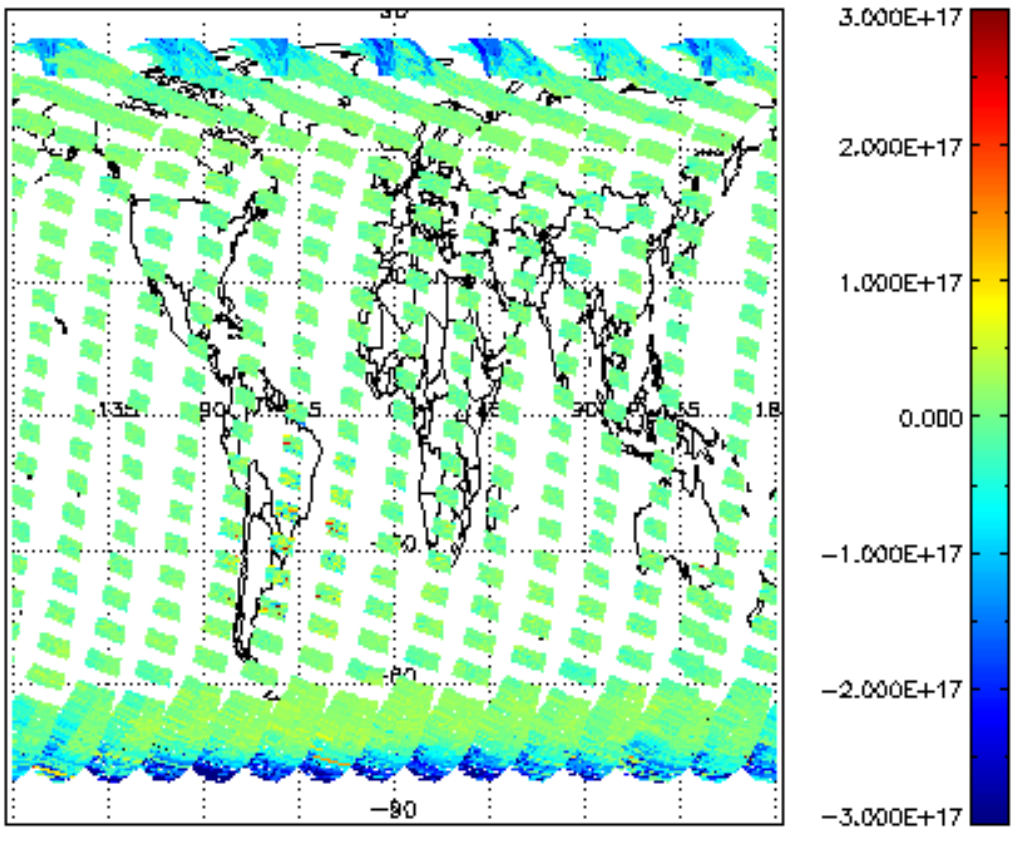
SCIOL2P_NADUV7S02_vcd for 16SEP2011 00:00:00 to 17SEP2011 00:00:00
