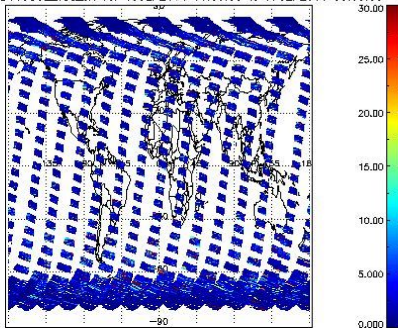
SCIOL2P_NADUV5S02_vcd_err for 16SEP2011 00:00:00 to 17SEP2011 00:00:00
