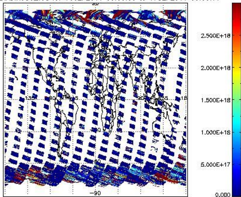
SCIOL2P_NADIR3CO_vcd for 16SEP2011 00:00:00 to 17SEP2011 00:00:00
