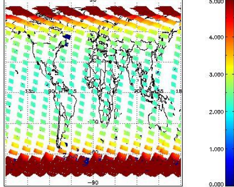
SCIOL2P_NADUV1N02_amf_gr for 16SEP2011 00:00:00 to 17SEP2011 00:00:00
