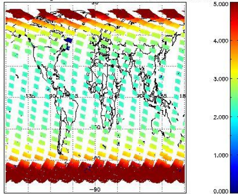
SCIOL2P_NADUV003_amf_gr for 16SEP2011 00:00:00 to 17SEP2011 00:00:00
