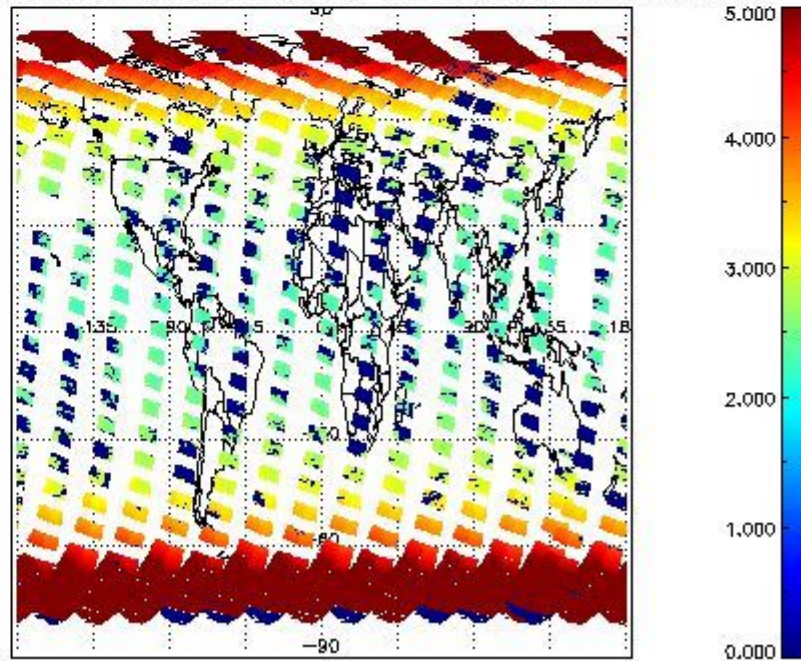
SCIOL2P_NADUV003_amf_cl for 16SEP2011 00:00:00 to 17SEP2011 00:00:00
