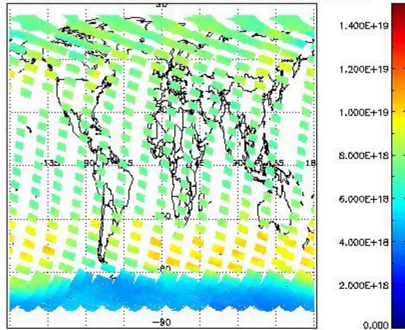
SCIOL2P_NADUV003_vcd for 16SEP2011 00:00:00 to 17SEP2011 00:00:00
