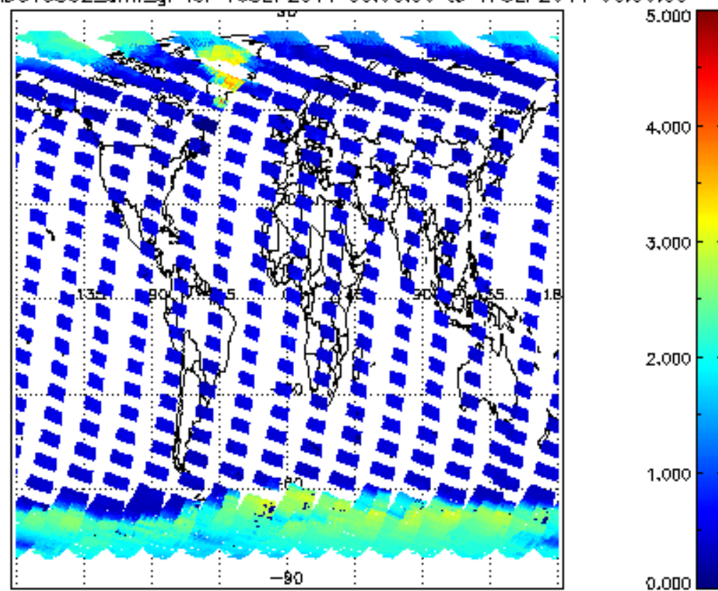
SCIOL2P_NADUV5S02_amf_gr for 16SEP2011 00:00:00 to 17SEP2011 00:00:00
