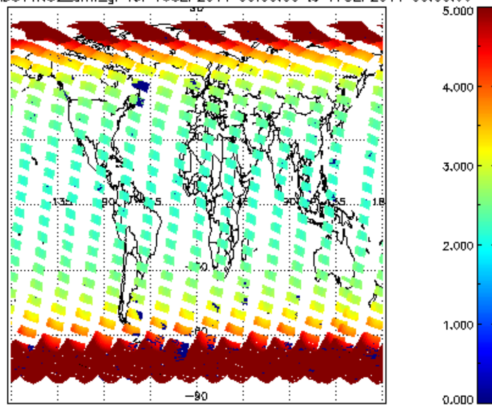
SCIOL2P_NADUV1NO2_amf_gr for 16SEP2011 00:00:00 to 17SEP2011 00:00:00
