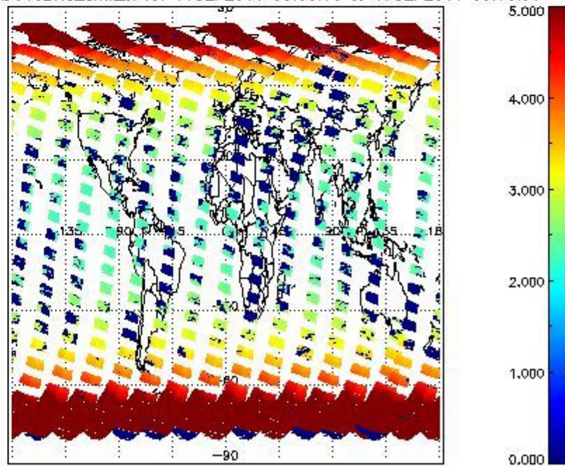
SCIOL2P_NADUV3BRO_amf_cl for 16SEP2011 00:00:00 to 17SEP2011 00:00:00
