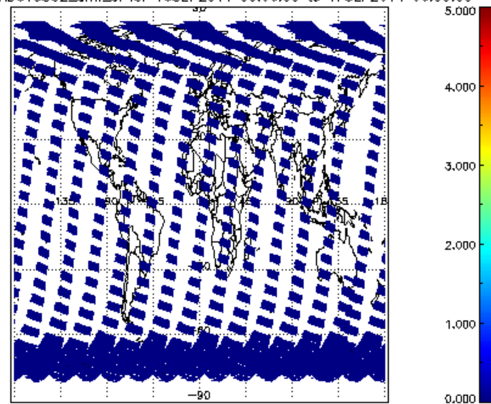
SCIOL2P_NADUV5S02_amf_cl for 16SEP2011 00:00:00 to 17SEP2011 00:00:00
