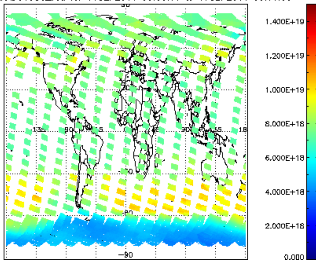
SCIOL2P_NADUV003_vcd for 16SEP2011 00:00:00 to 17SEP2011 00:00:00
