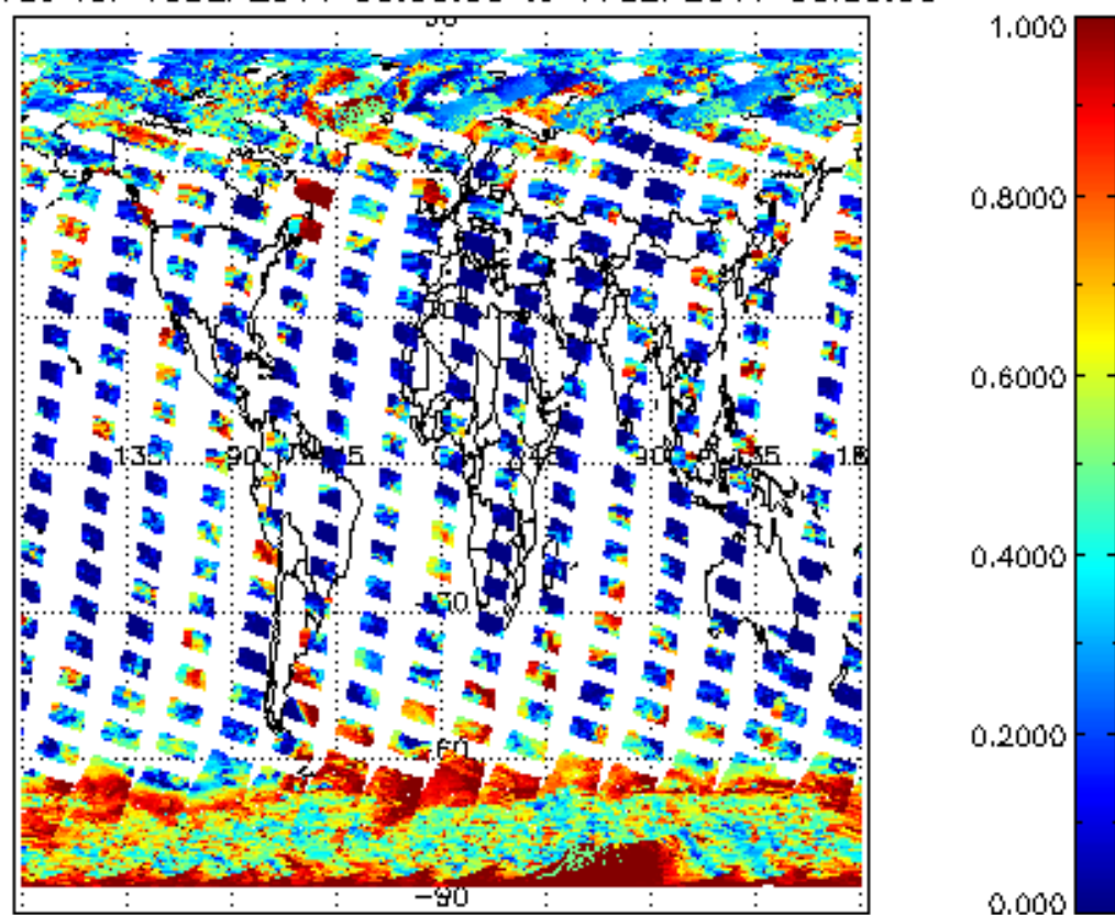
cL_frac for 16SEP2011 00:00:00 to 17SEP2011 00:00:00
