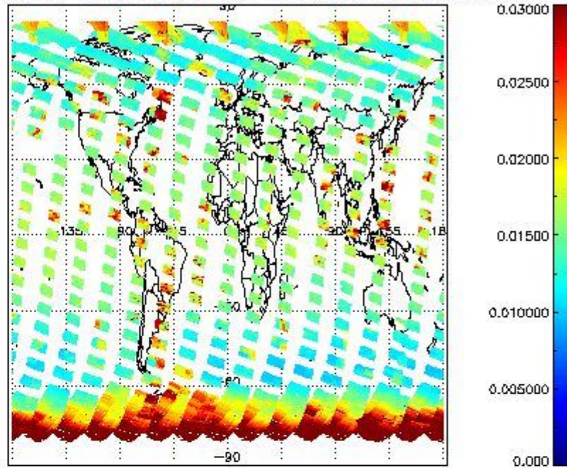
SCIOL2P_NADUV003_vcd_err for 16SEP2011 00:00:00 to 17SEP2011 00:00:00
