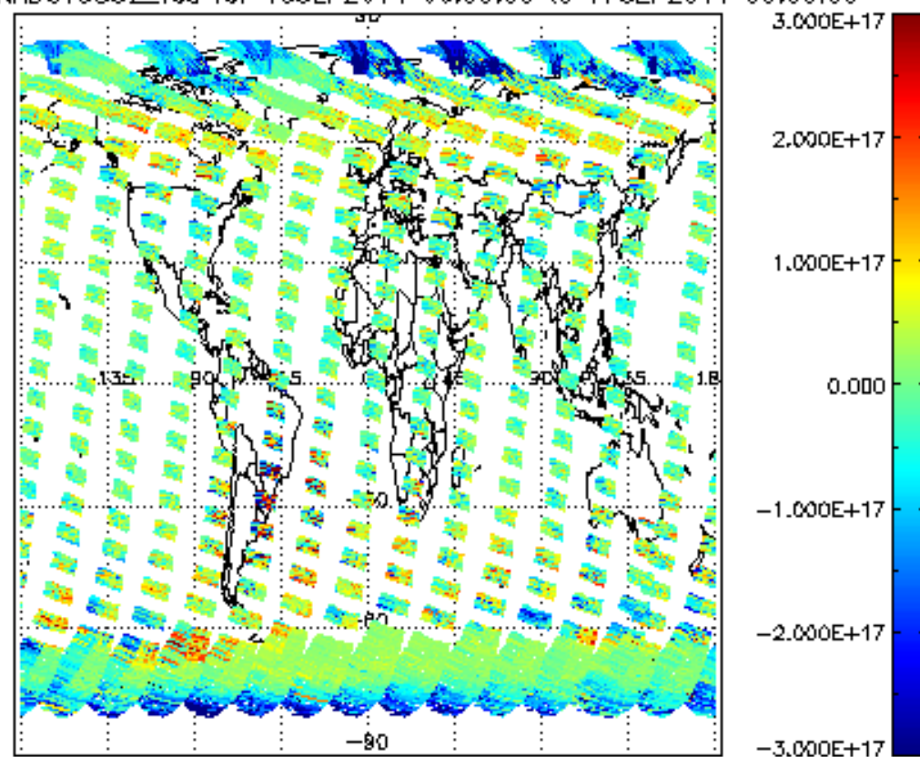
SCIOL2P_NADUV5S02_vcd for 16SEP2011 00:00:00 to 17SEP2011 00:00:00
