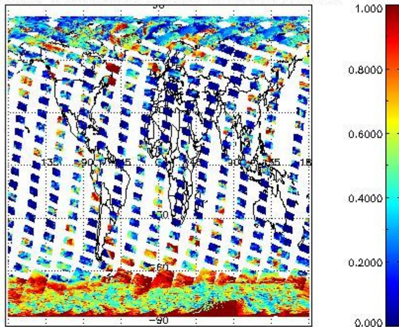
cL_frac for 16SEP2011 00:00:00 to 17SEP2011 00:00:00
