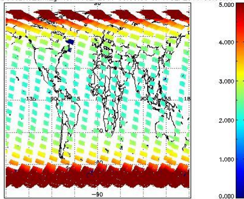
SCIOL2P_NADUV3BRO_amf_gr for 16SEP2011 00:00:00 to 17SEP2011 00:00:00
