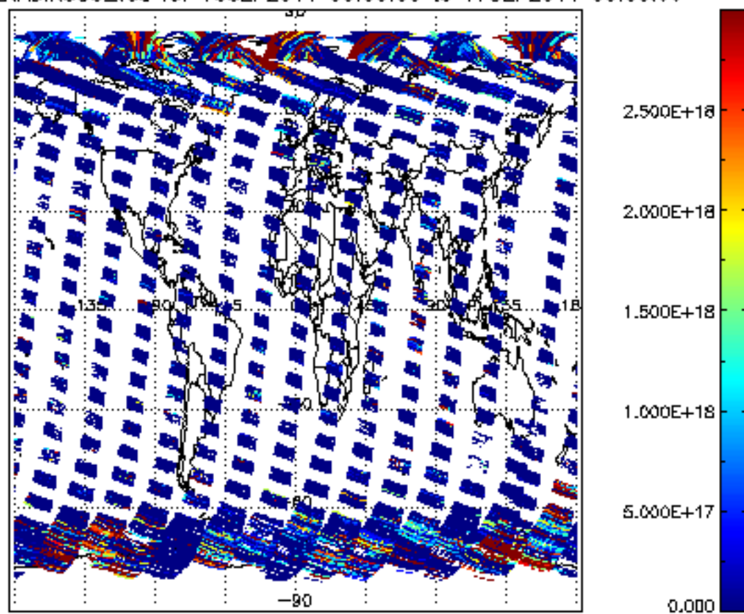
SCIOL2P_NADIR3CO_vcd for 16SEP2011 00:00:00 to 17SEP2011 00:00:00
