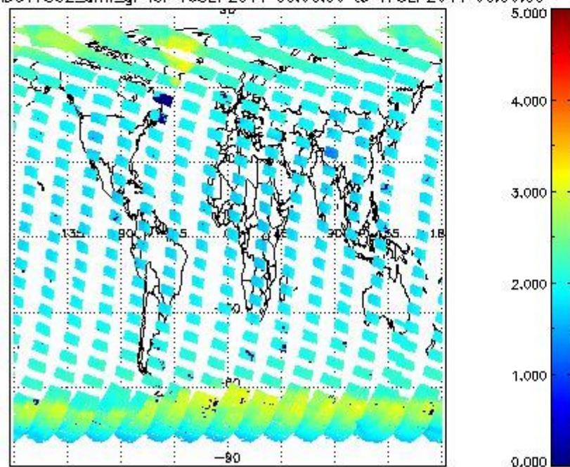
SCIOL2P_NADUV7S02_amf_gr for 16SEP2011 00:00:00 to 17SEP2011 00:00:00
