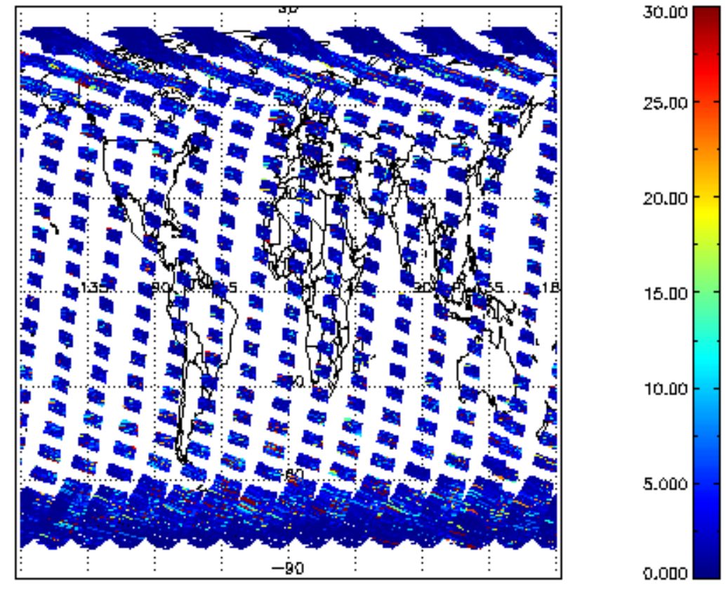
SCIOL2P_NADUV7S02_vcd_err for 16SEP2011 00:00:00 to 17SEP2011 00:00:00
