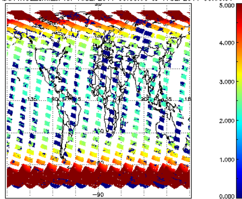
SCIOL2P_NADUV1NO2_amf_sl for 16SEP2011 00:00:00 to 17SEP2011 00:00:00
