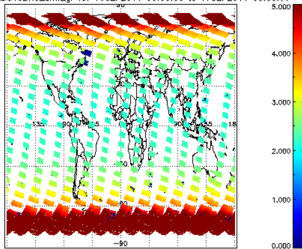
SCIOL2P_NADUV3BRO_amf_gr for 16SEP2011 00:00:00 to 17SEP2011 00:00:00
