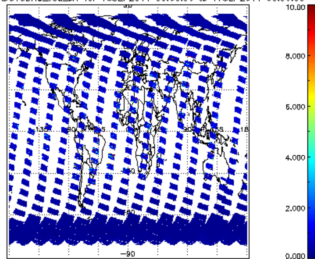
SCIOL2P_NADUV3BRO_vcd_err for 16SEP2011 00:00:00 to 17SEP2011 00:00:00
