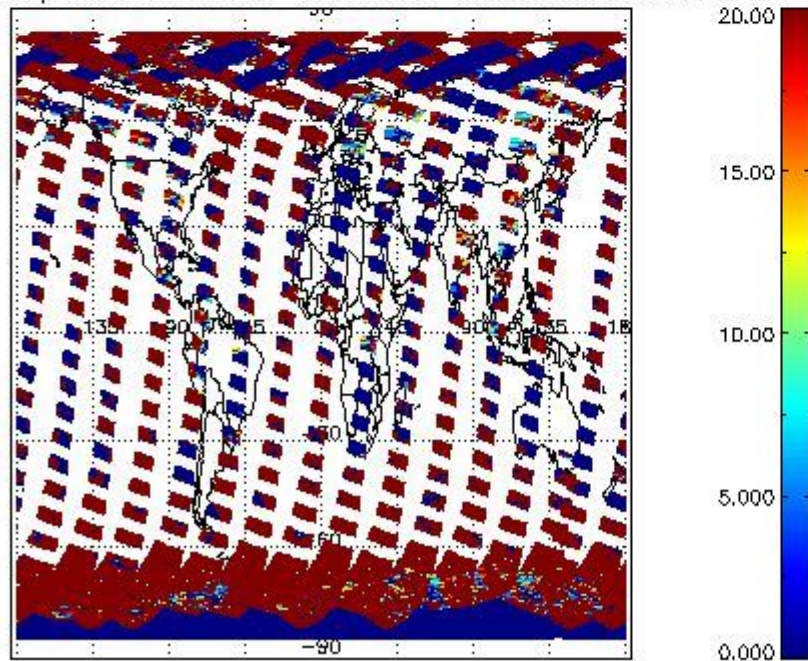
cL_opt_depth for 16SEP2011 00:00:00 to 17SEP2011 00:00:00
