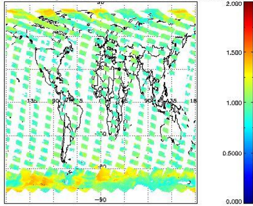
SCIOL2P_NADUV8H2O_arnf_gr for 16SEP2011 00:00:00 to 17SEP2011 00:00:00
