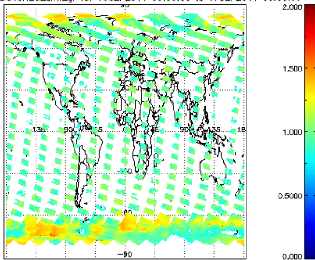
SCIOL2P_NADUV8H2O_amf_gr for 16SEP2011 00:00:00 to 17SEP2011 00:00:00
