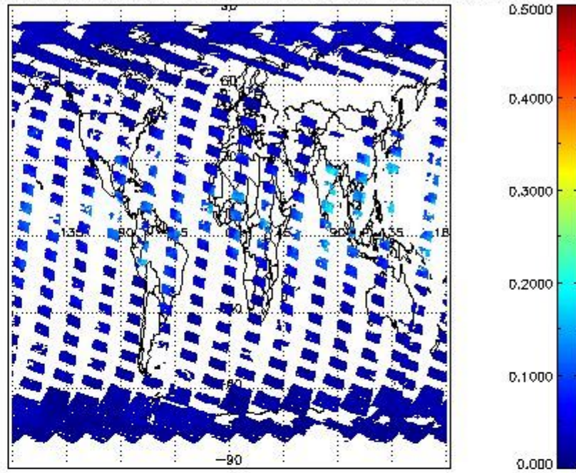
SCIOL2P_NADUV8H2O_vcd_err for 16SEP2011 00:00:00 to 17SEP2011 00:00:00
