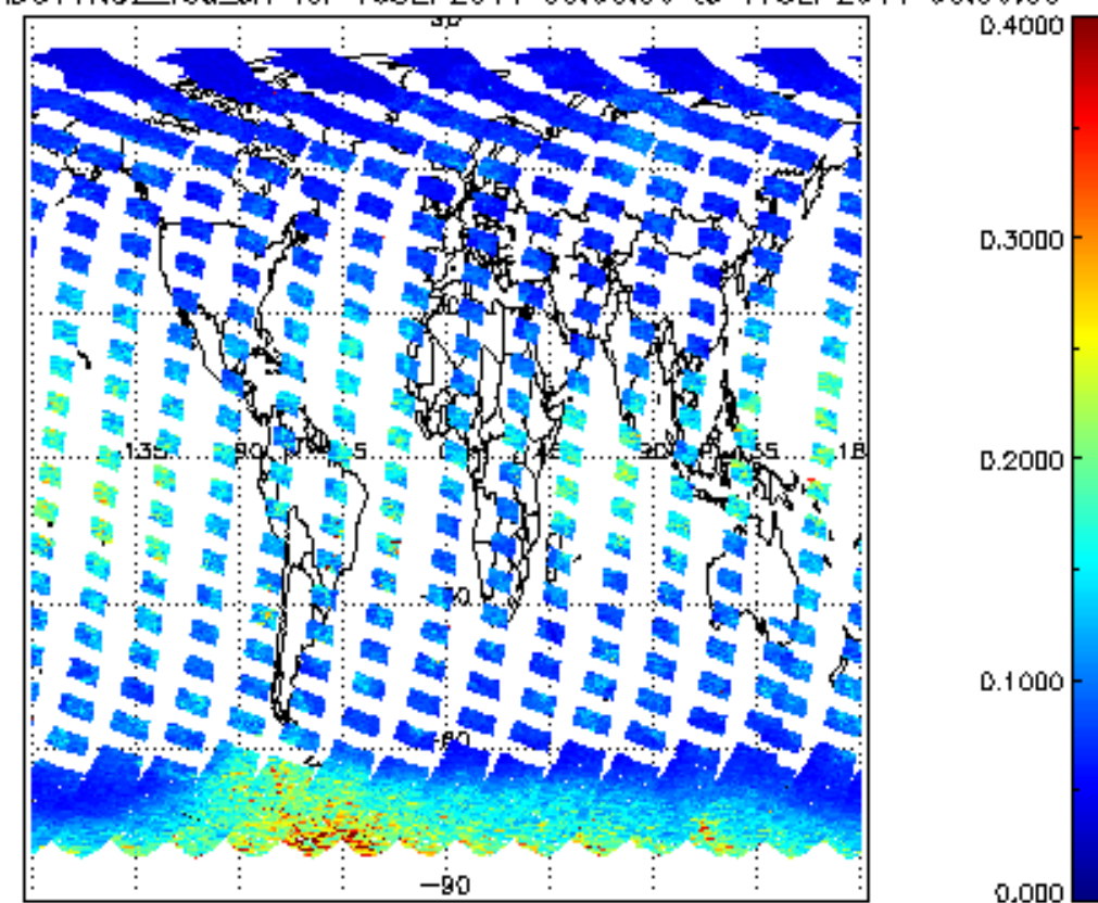
SCIOL2P_NADUV1NO2_vcd_err for 16SEP2011 00:00:00 to 17SEP2011 00:00:00
