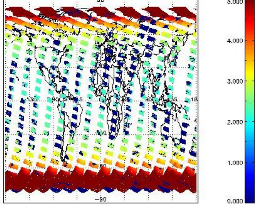
SCIOL2P_NADUV1N02_amf_cl for 16SEP2011 00:00:00 to 17SEP2011 00:00:00
