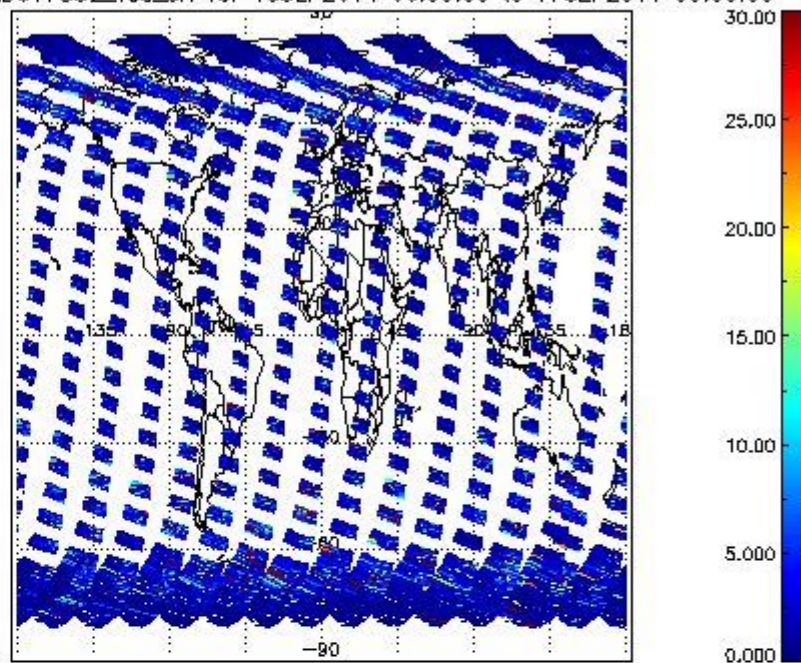
SCIOL2P_NADUV7S02_vcd_err for 16SEP2011 00:00:00 to 17SEP2011 00:00:00
