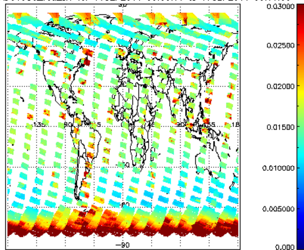
SCIOL2P_NADUV003_vcd_err for 16SEP2011 00:00:00 to 17SEP2011 00:00:00
