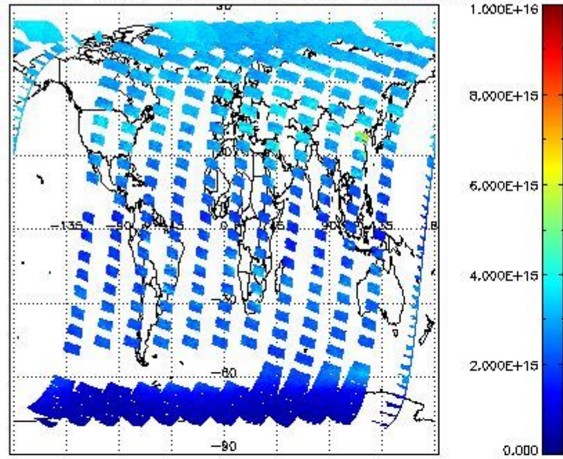
SCIOL2P_NADUV1NO2_vcd for 11SEP2011 00:00:00 to 12SEP2011 00:00:00
