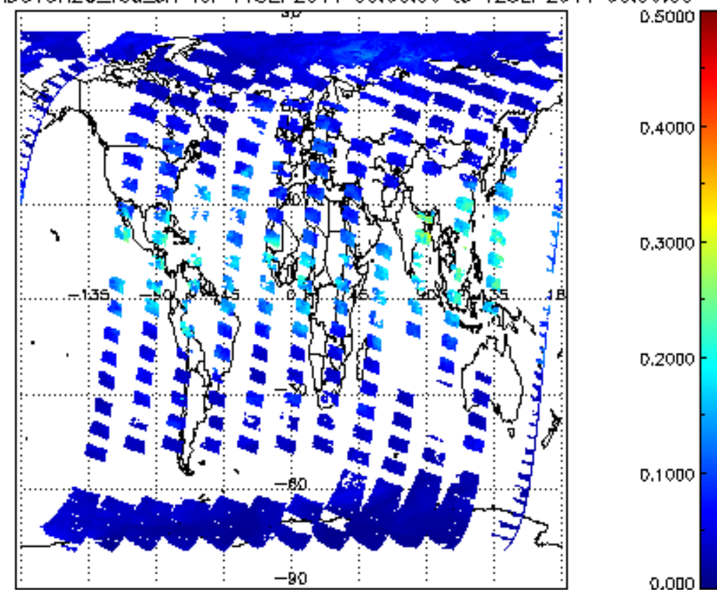
SCIOL2P_NADUV8H2O_vcd_err for 11SEP2011 00:00:00 to 12SEP2011 00:00:00
