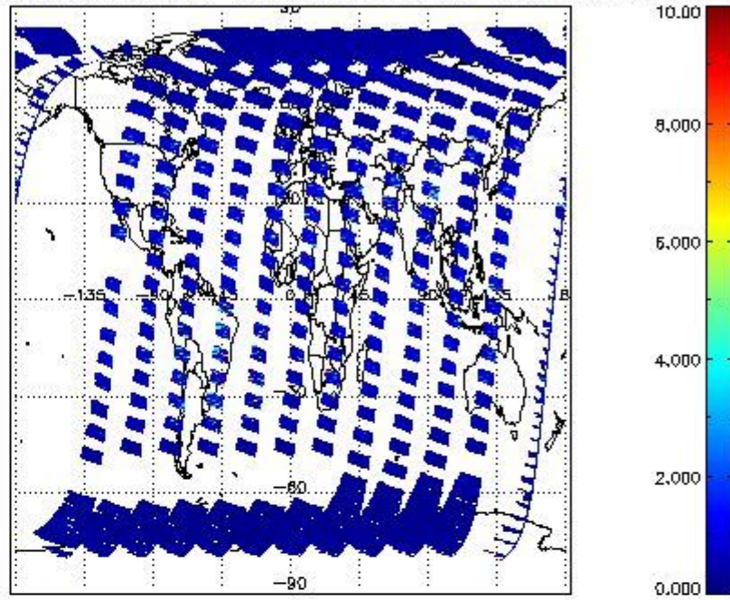
SCIOL2P_NADUV3BRO_vcd_err for 11SEP2011 00:00:00 to 12SEP2011 00:00:00
