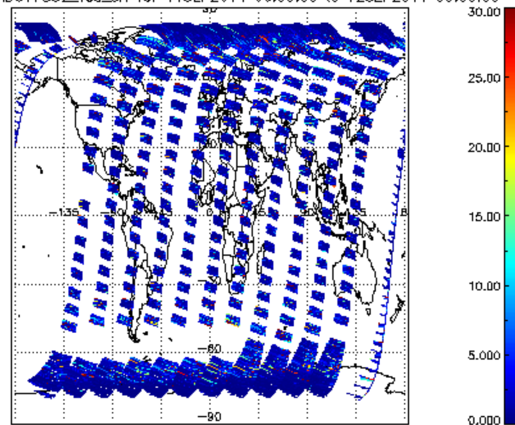
SCIOL2P_NADUV7S02_vcd_err for 11SEP2011 00:00:00 to 12SEP2011 00:00:00
