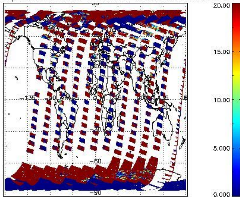
cL_opt_depth for 11SEP2011 00:00:00 to 12SEP2011 00:00:00
