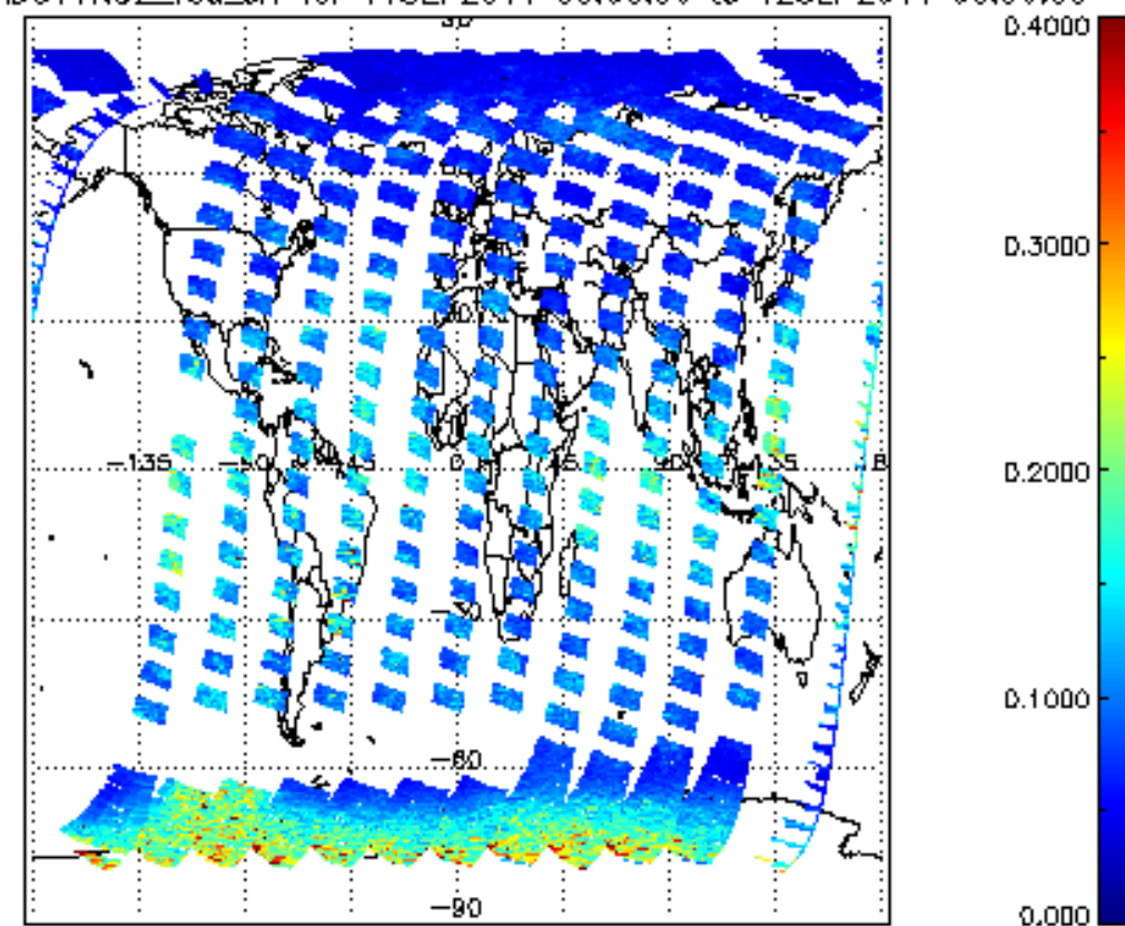
SCIOL2P_NADUV1N02_vcd_err for 11SEP2011 00:00:00 to 12SEP2011 00:00:00
