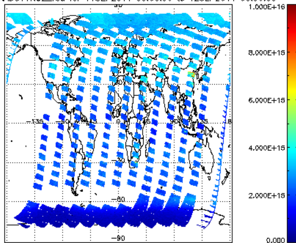
SCIOL2P_NADUV1N02_vcd for 11SEP2011 00:00:00 to 12SEP2011 00:00:00
