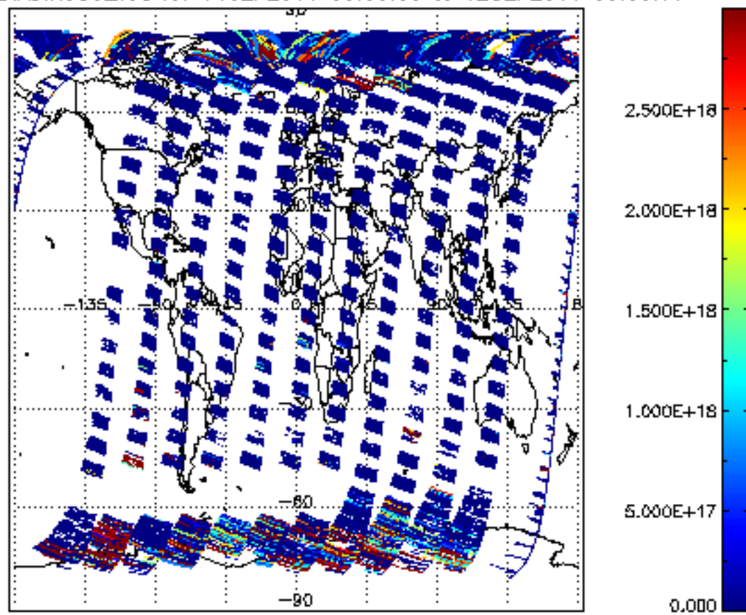
SCIOL2P_NADIR3CO_vcd for 11SEP2011 00:00:00 to 12SEP2011 00:00:00
