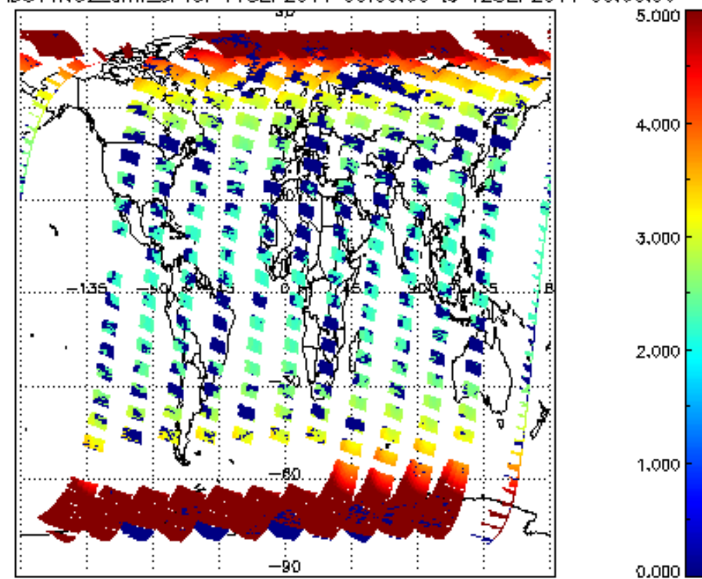
SCIOL2P_NADUV1N02_amf_cl for 11SEP2011 00:00:00 to 12SEP2011 00:00:00
