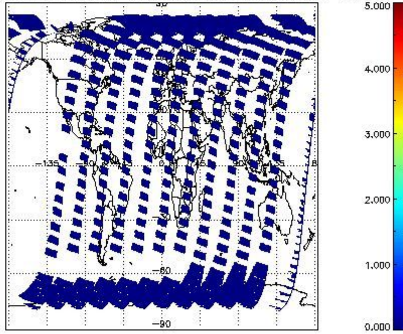
SCIOL2P_NADUV5S02_amf_cl for 11SEP2011 00:00:00 to 12SEP2011 00:00:00
