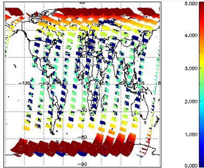
SCIOL2P_NADUV003_amf_cl for 11SEP2011 00:00:00 to 12SEP2011 00:00:00
