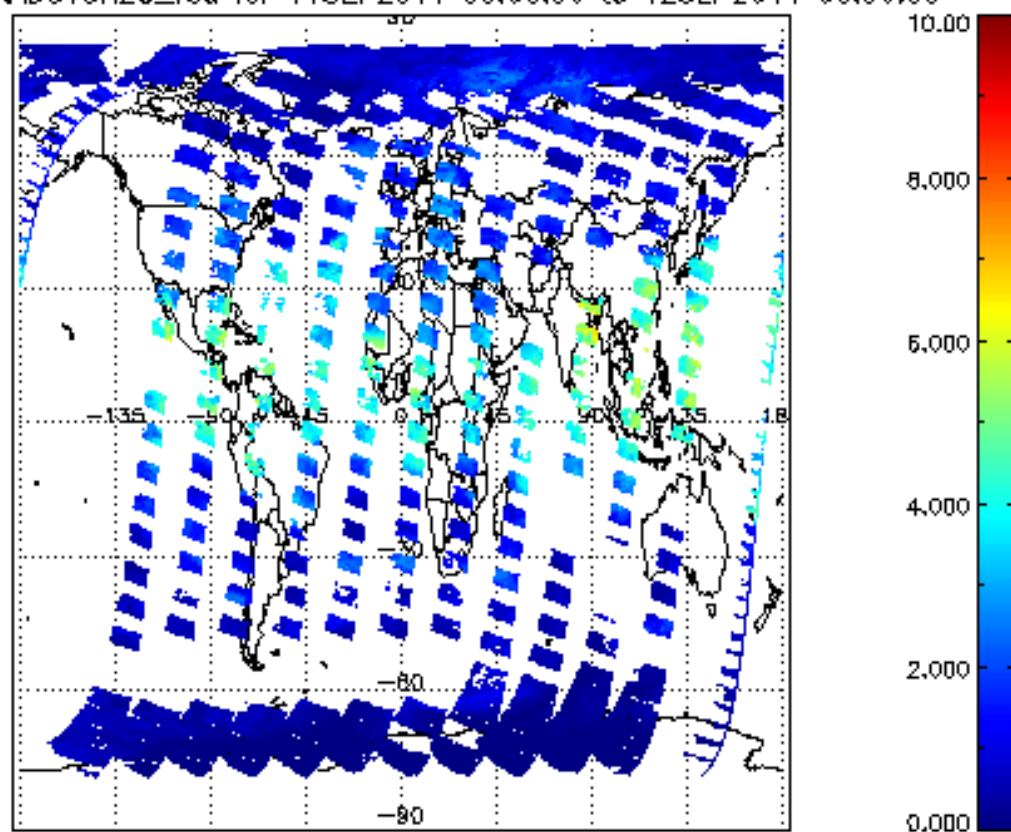
SCIOL2P_NADUV8H2O_vcd for 11SEP2011 00:00:00 to 12SEP2011 00:00:00
