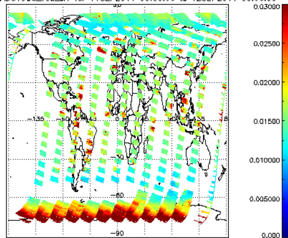
SCIOL2P_NADUV003_vcd_err for 11SEP2011 00:00:00 to 12SEP2011 00:00:00
