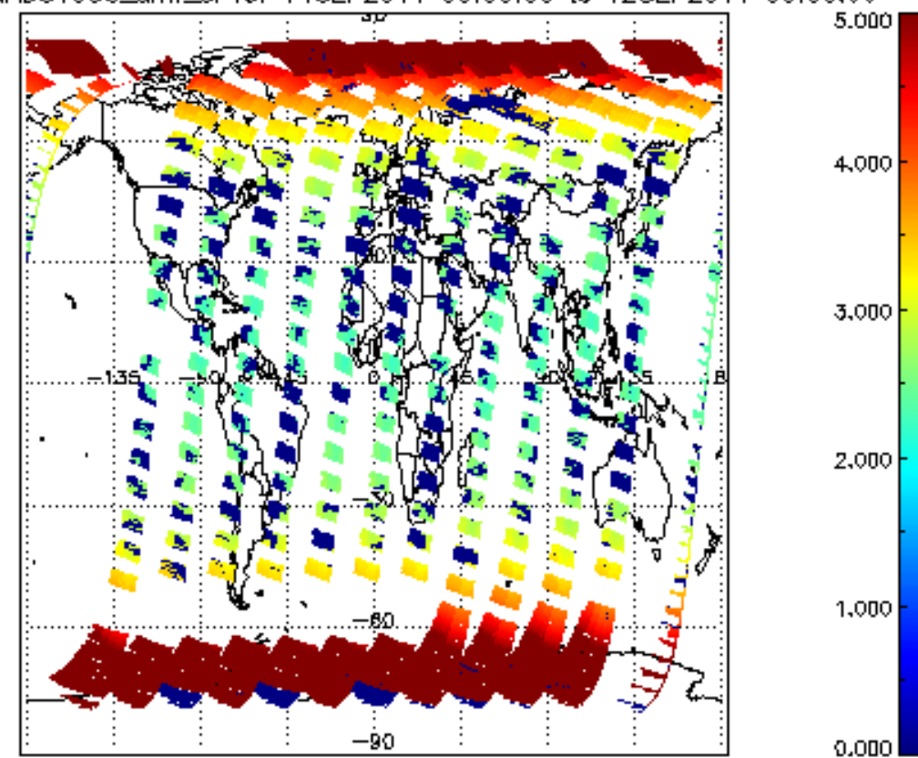
SCIOL2P_NADUV003_amf_cl for 11SEP2011 00:00:00 to 12SEP2011 00:00:00
