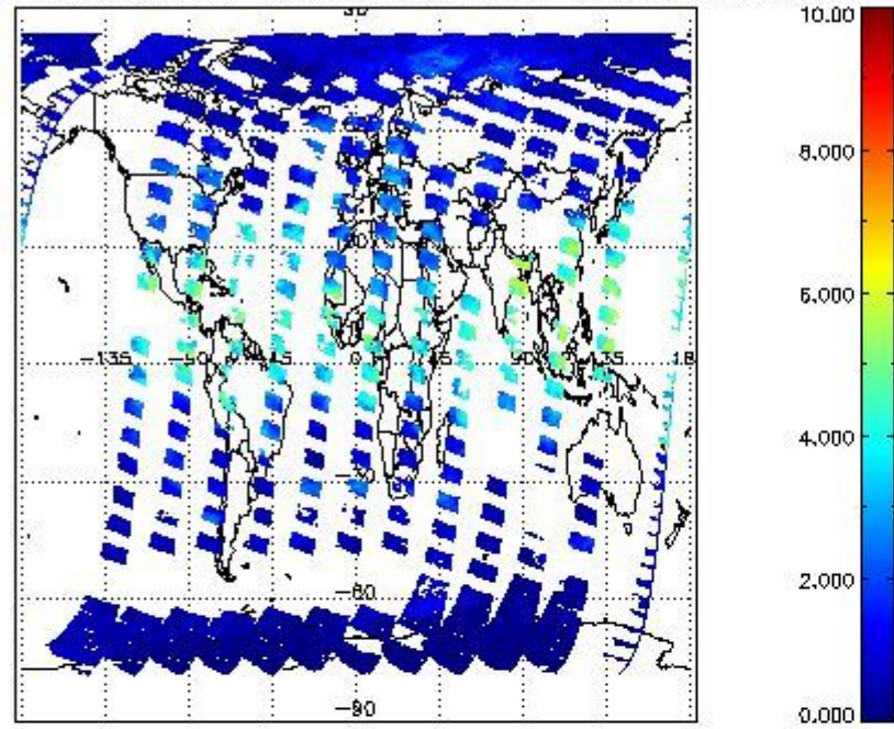
SCIOL2P_NADUV8H2O_vcd for 11SEP2011 00:00:00 to 12SEP2011 00:00:00
