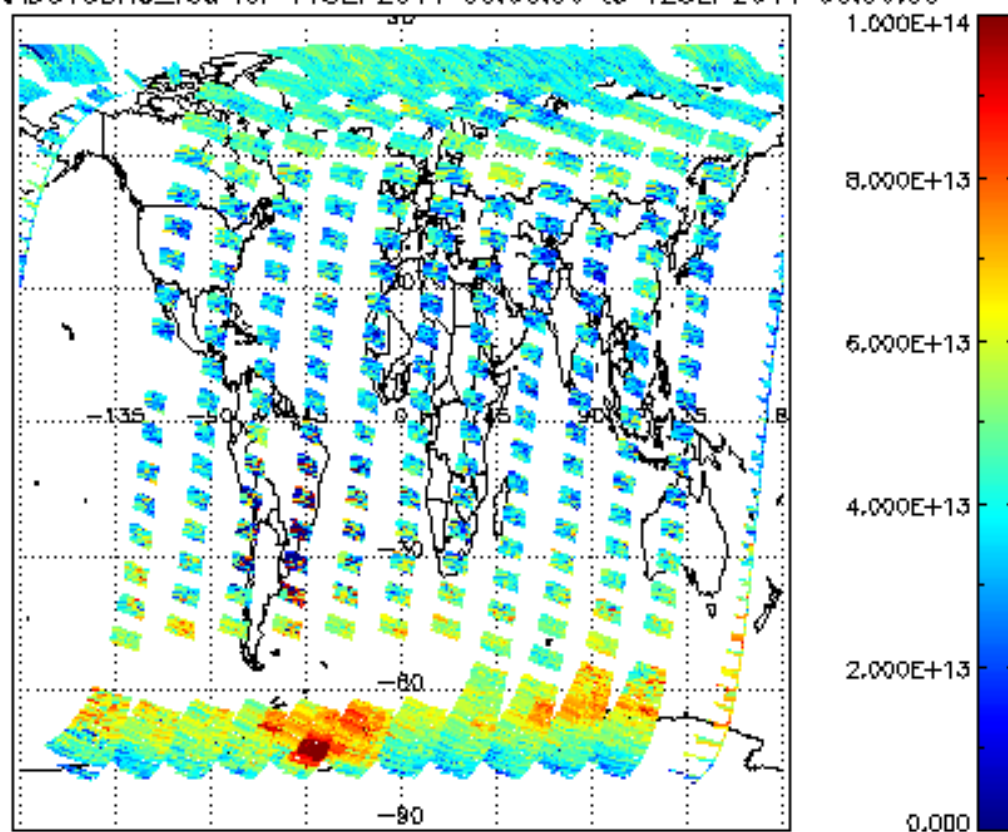
SCIOL2P_NADUV3BRO_vcd for 11SEP2011 00:00:00 to 12SEP2011 00:00:00
