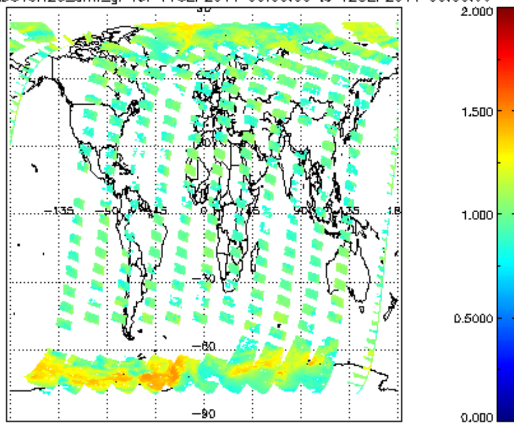
SCIOL2P_NADUV8H2O_amf_gr for 11SEP2011 00:00:00 to 12SEP2011 00:00:00
