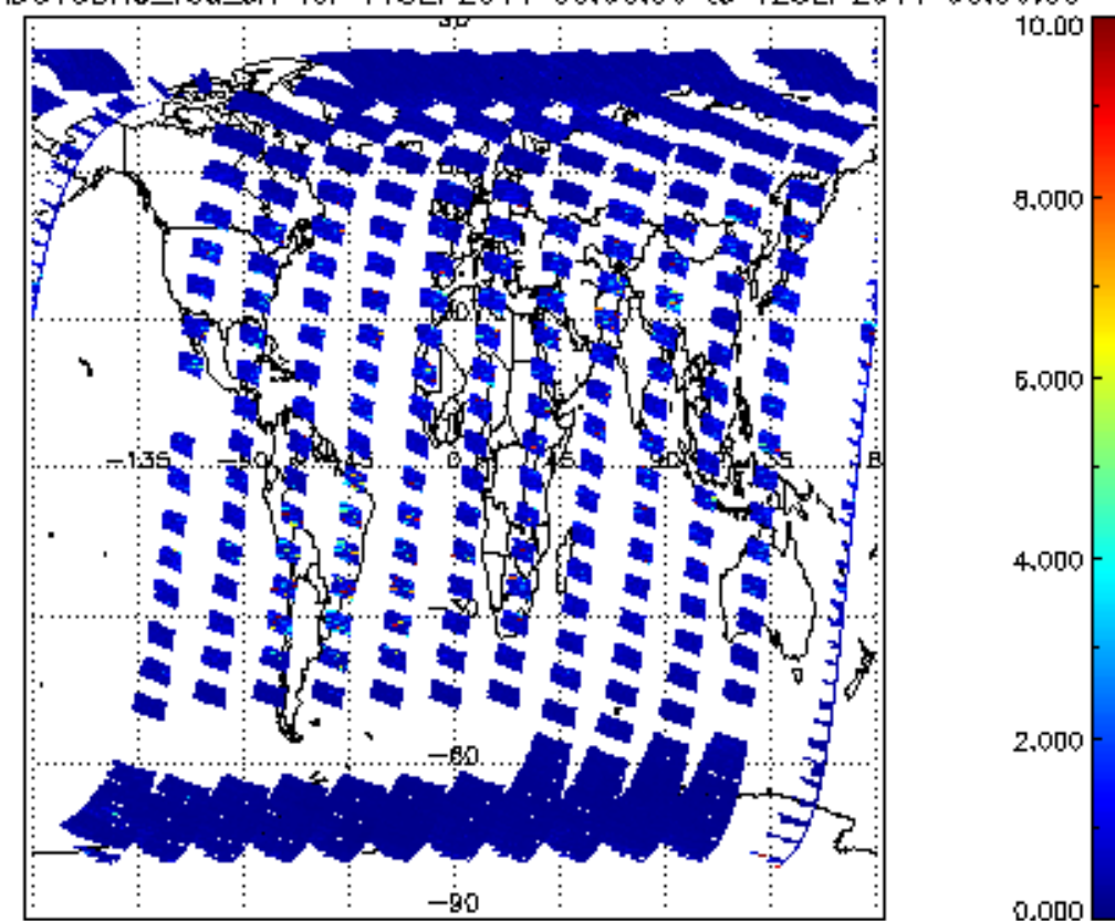
SCIOL2P_NADUV3BRO_vcd_err for 11SEP2011 00:00:00 to 12SEP2011 00:00:00
