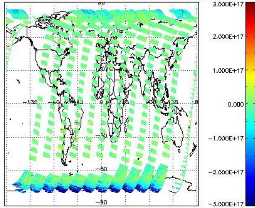
SCIOL2P_NADUV7S02_vcd for 11SEP2011 00:00:00 to 12SEP2011 00:00:00
