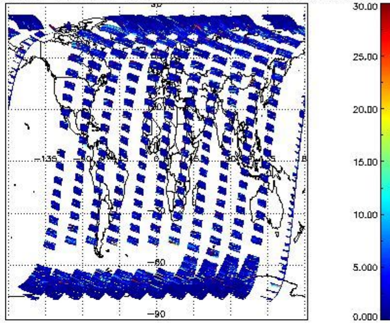
SCIOL2P_NADUV7S02_vcd_err for 11SEP2011 00:00:00 to 12SEP2011 00:00:00
