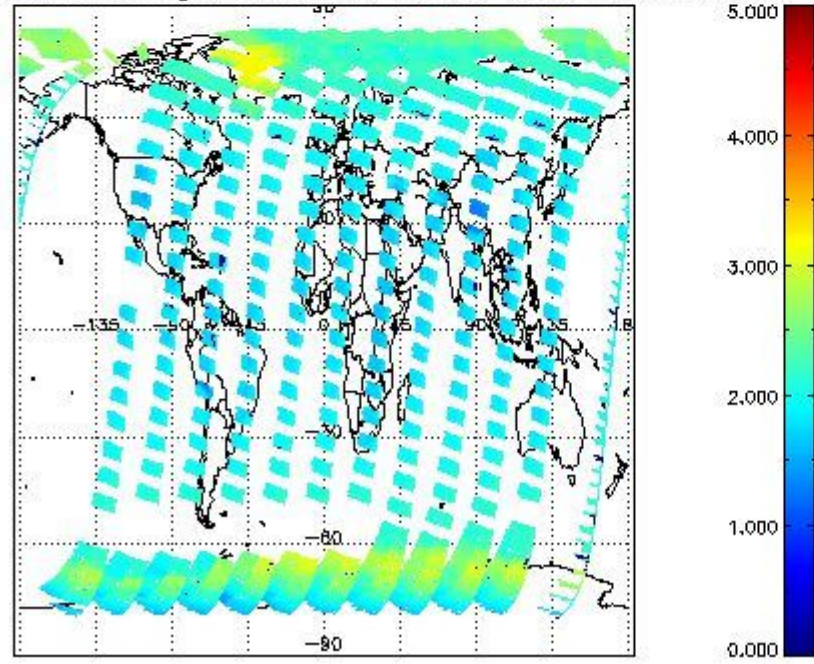
SCIOL2P_NADUV7S02_amf_gr for 11SEP2011 00:00:00 to 12SEP2011 00:00:00
