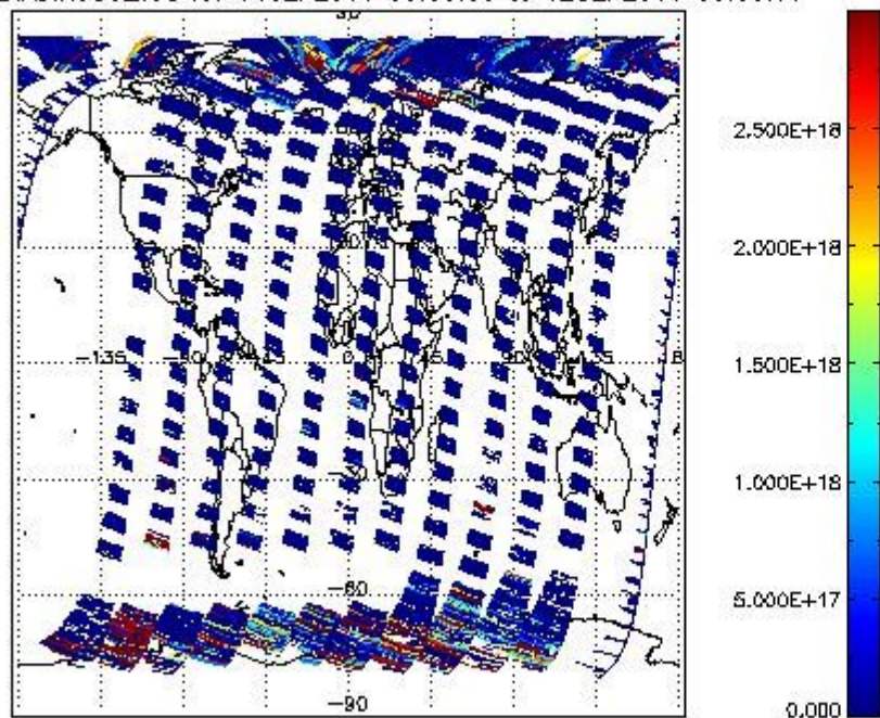
SCIO2P_NADIR3CO_vcd for 11SEP2011 00:00:00 to 12SEP2011 00:00:00
