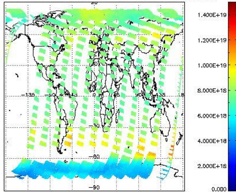
SCIOL2P_NADUV003_vcd for 11SEP2011 00:00:00 to 12SEP2011 00:00:00
