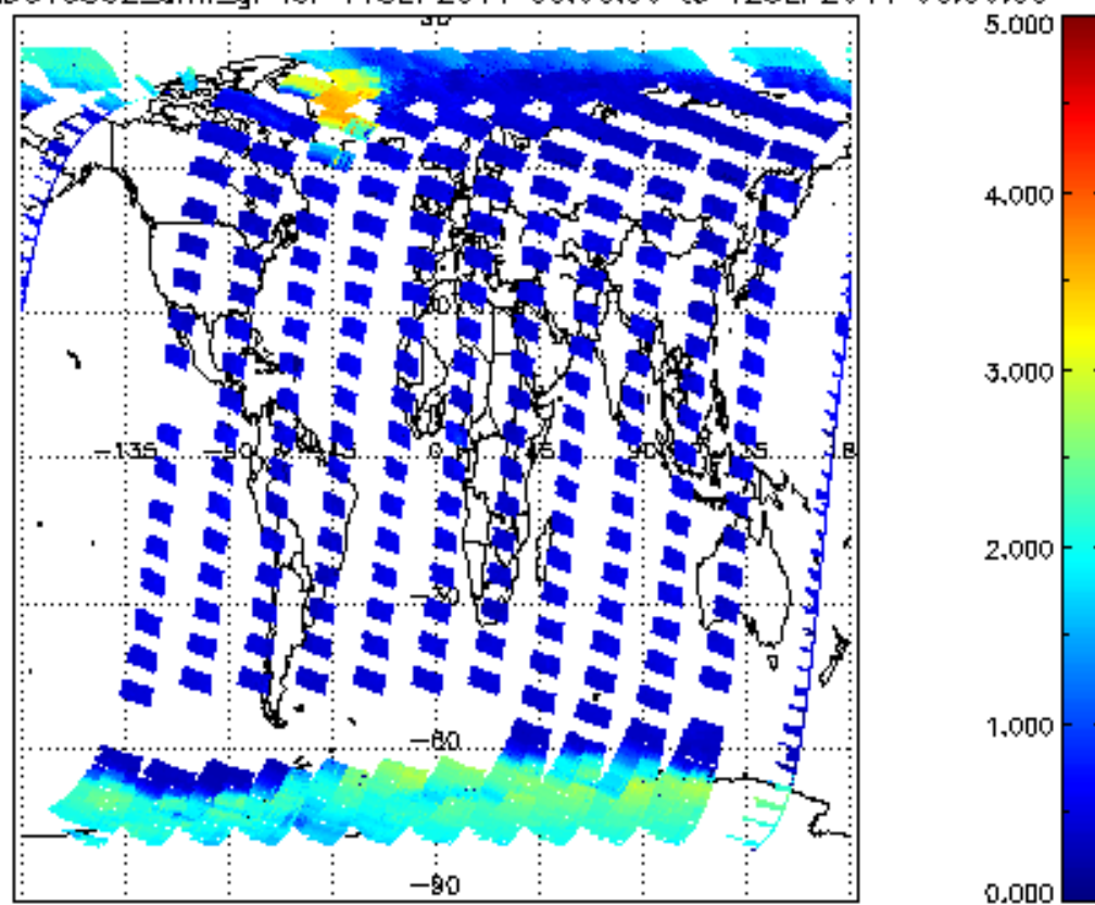
SCIOL2P_NADUV5S02_amf_gr for 11SEP2011 00:00:00 to 12SEP2011 00:00:00
