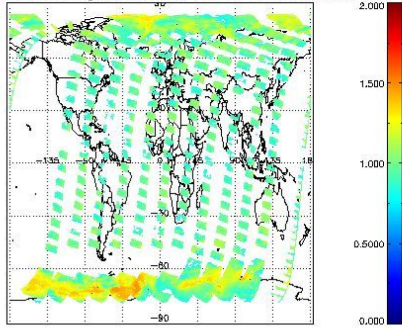
SCIOL2P_NADUV8H2O_arnf_gr for 11SEP2011 00:00:00 to 12SEP2011 00:00:00
