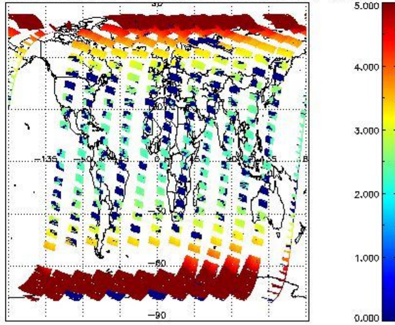
SCIOL2P_NADUV3BRO_amf_cl for 11SEP2011 00:00:00 to 12SEP2011 00:00:00
