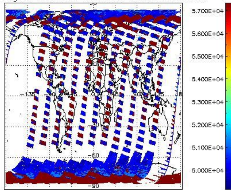
cloud_flags for 11SEP2011 00:00:00 to 12SEP2011 00:00:00
