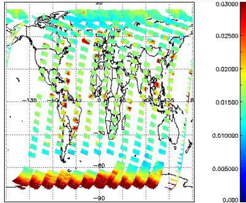
SCIOL2P_NADUV003_vcd_err for 11SEP2011 00:00:00 to 12SEP2011 00:00:00
