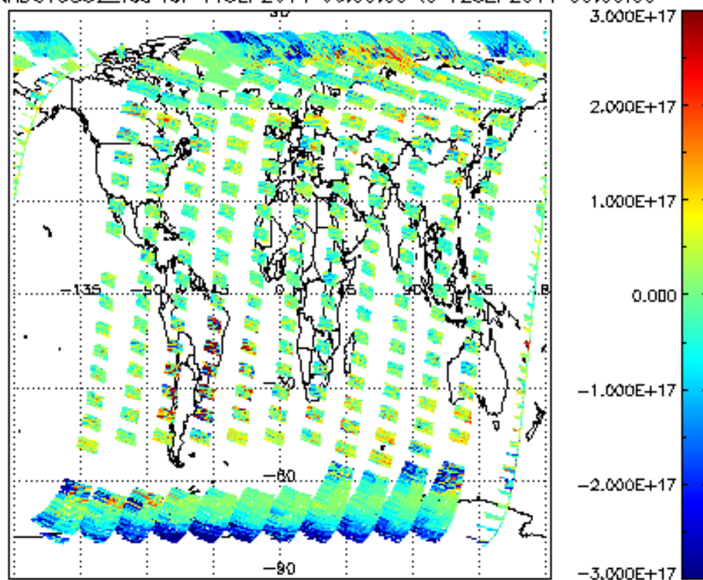
SCIOL2P_NADUV5S02_vcd for 11SEP2011 00:00:00 to 12SEP2011 00:00:00
