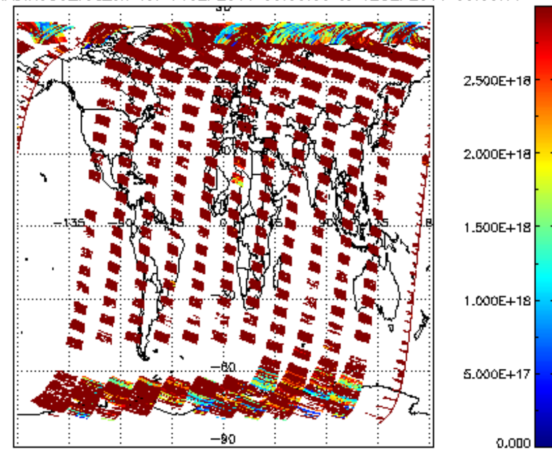
SCIOL2P_NADIR3CO_vcd_err for 11SEP2011 00:00:00 to 12SEP2011 00:00:00
