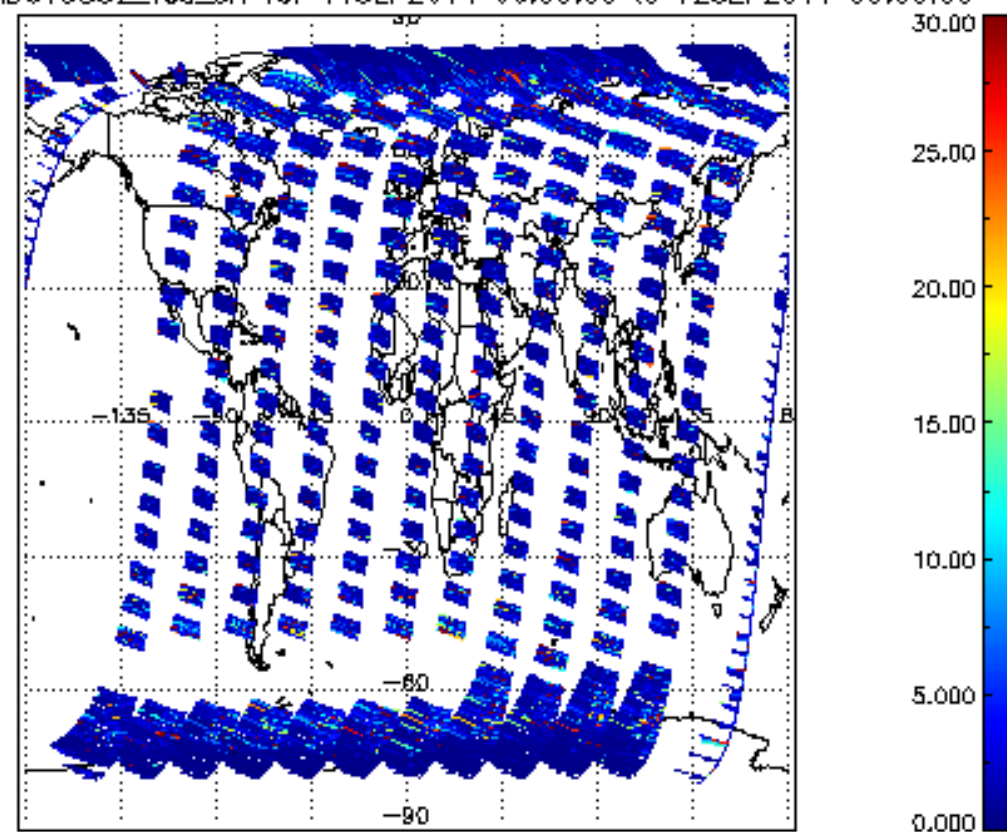
SCIOL2P_NADUV5S02_vcd_err for 11SEP2011 00:00:00 to 12SEP2011 00:00:00
