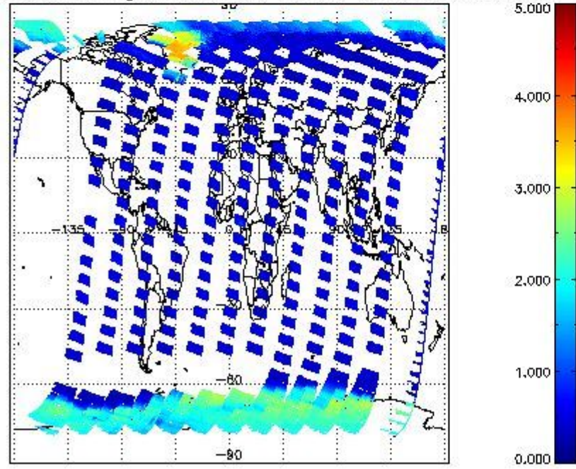
SCIOL2P_NADUV5S02_amf_gr for 11SEP2011 00:00:00 to 12SEP2011 00:00:00
