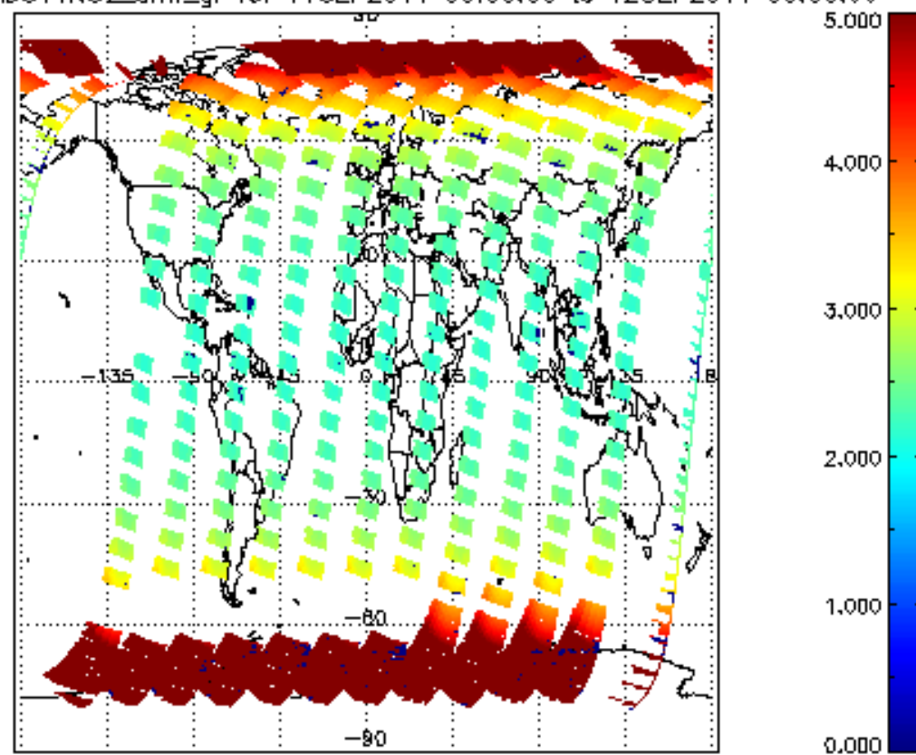
SCIOL2P_NADUV1N02_amf_gr for 11SEP2011 00:00:00 to 12SEP2011 00:00:00
