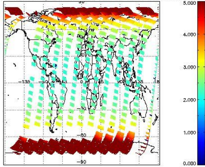
SCIOL2P_NADUV3BRO_amf_gr for 11SEP2011 00:00:00 to 12SEP2011 00:00:00
