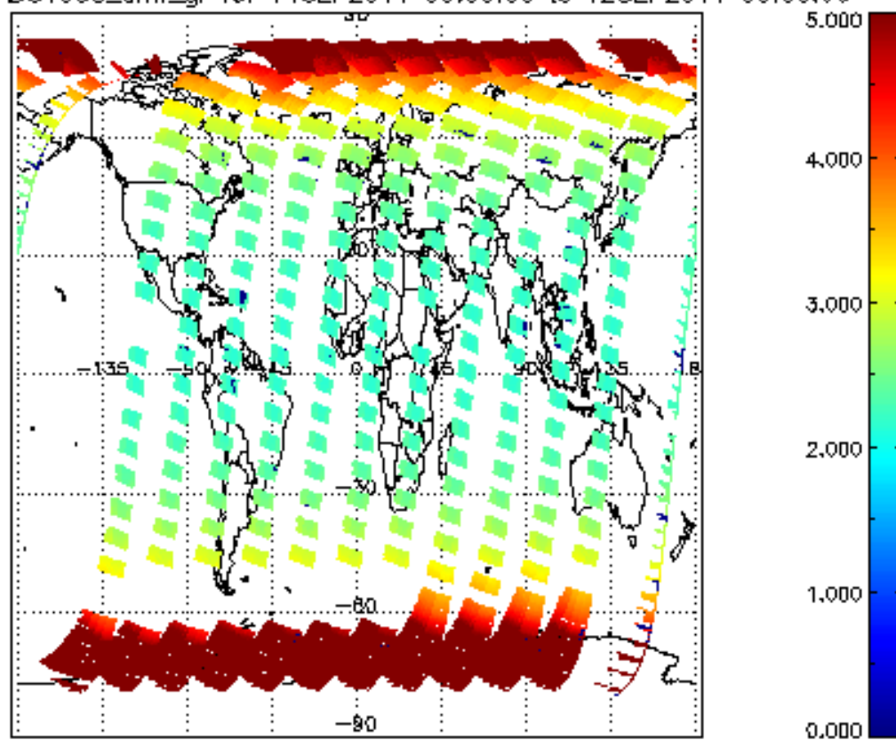
SCIOL2P_NADUV003_amf_gr for 11SEP2011 00:00:00 to 12SEP2011 00:00:00
