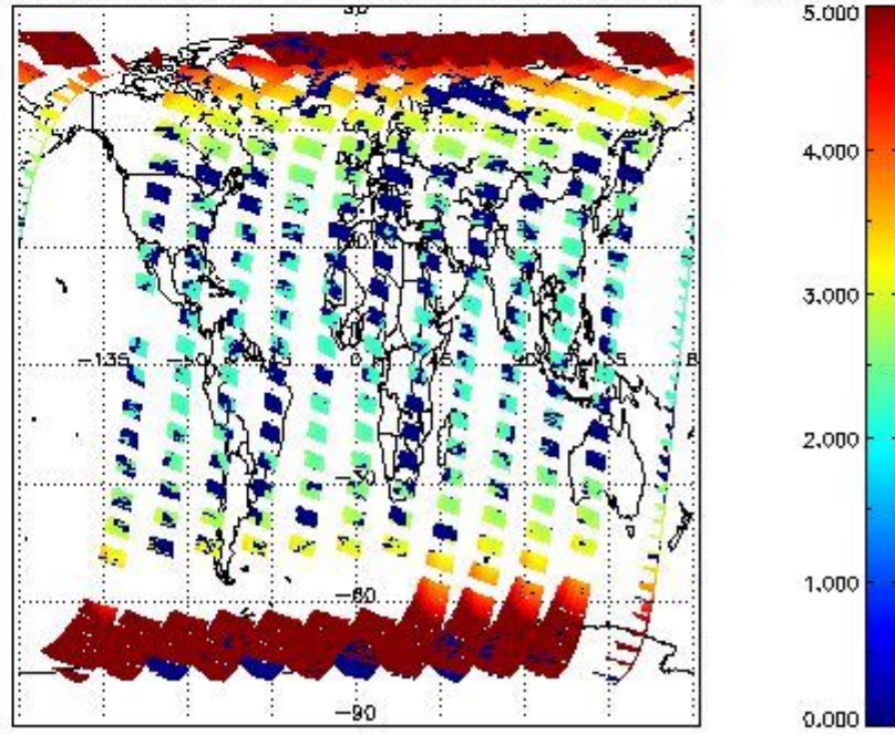
SCIOL2P_NADUV1NO2_amf_cl for 11SEP2011 00:00:00 to 12SEP2011 00:00:00
