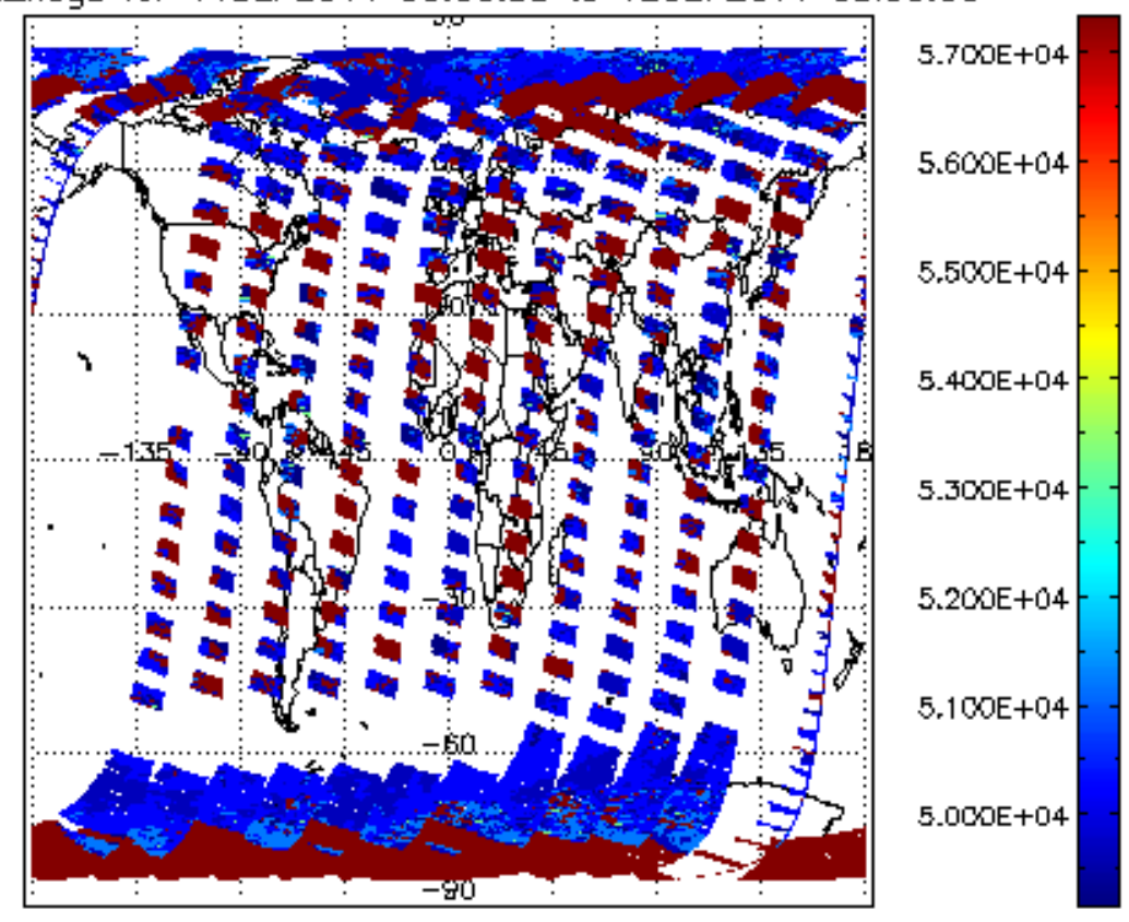
cloud_flags for 11SEP2011 00:00:00 to 12SEP2011 00:00:00
