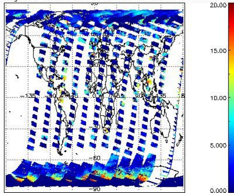
cL_top_height for 11SEP2011 00:00:00 to 12SEP2011 00:00:00
