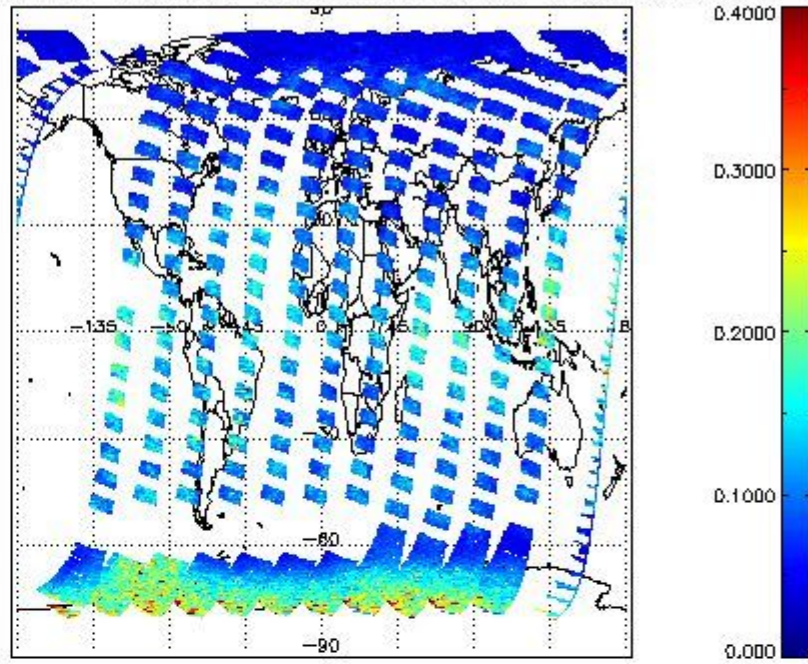
SCIOL2P_NADUV1NO2_vcd_err for 11SEP2011 00:00:00 to 12SEP2011 00:00:00
