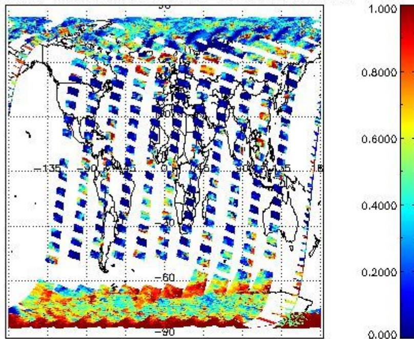
cL_frac for 11SEP2011 00:00:00 to 12SEP2011 00:00:00
