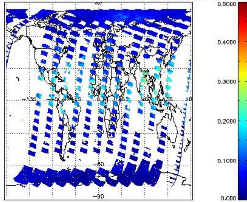
SCIOL2P_NADUV8H2O_vcd_err for 11SEP2011 00:00:00 to 12SEP2011 00:00:00
