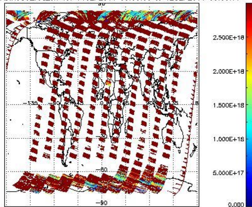
SCIO2P_NADIR3CO_vcd_err for 11SEP2011 00:00:00 to 12SEP2011 00:00:00
