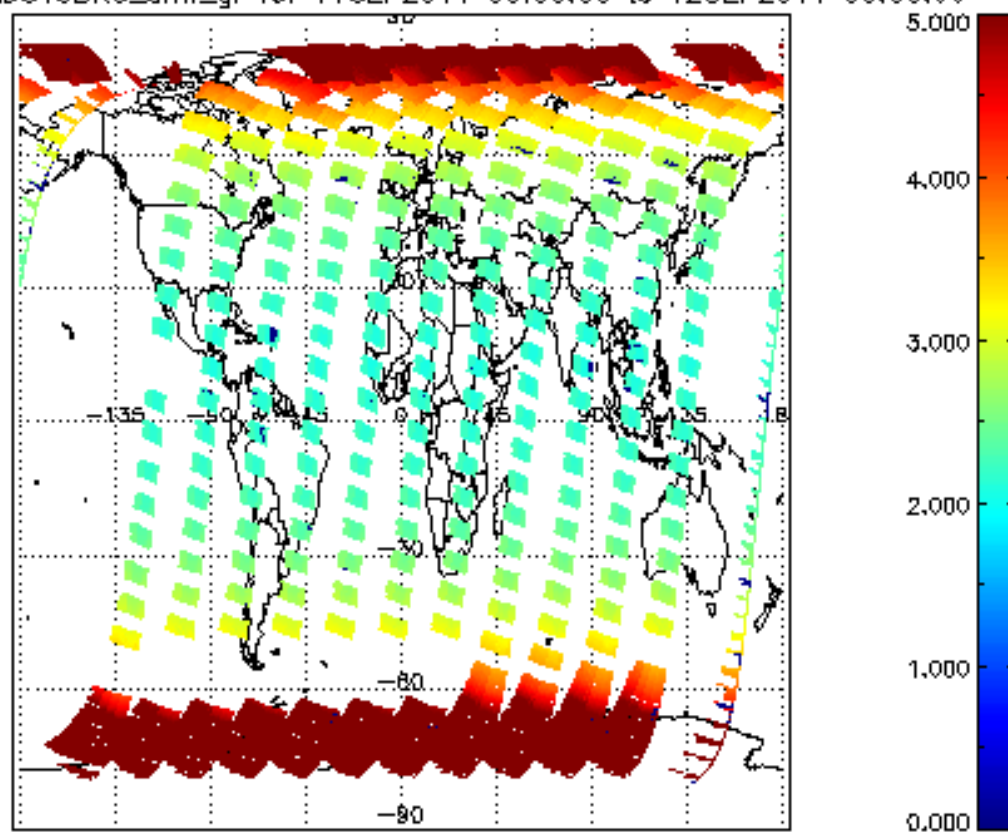
SCIOL2P_NADUV3BRO_amf_gr for 11SEP2011 00:00:00 to 12SEP2011 00:00:00
