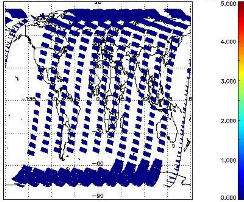
SCIOL2P_NADUV7S02_amf_cl for 11SEP2011 00:00:00 to 12SEP2011 00:00:00
