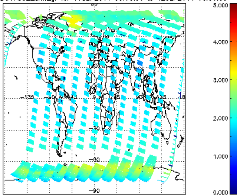
SCIOL2P_NADUV7S02_amf_gr for 11SEP2011 00:00:00 to 12SEP2011 00:00:00
