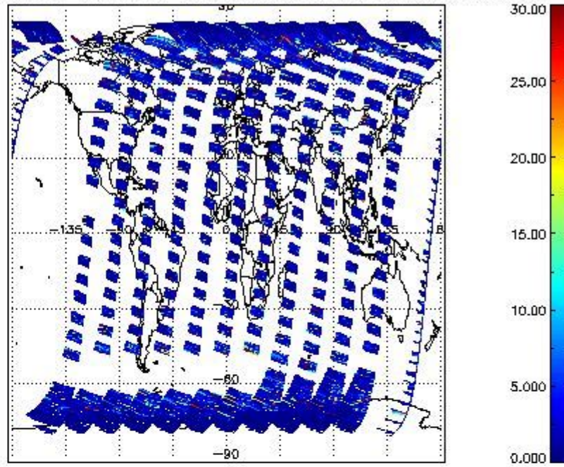
SCIOL2P_NADUV5S02_vcd_err for 11SEP2011 00:00:00 to 12SEP2011 00:00:00
