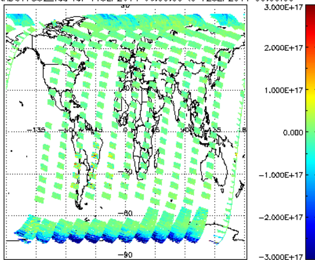
SCIOL2P_NADUV7S02_vcd for 11SEP2011 00:00:00 to 12SEP2011 00:00:00
