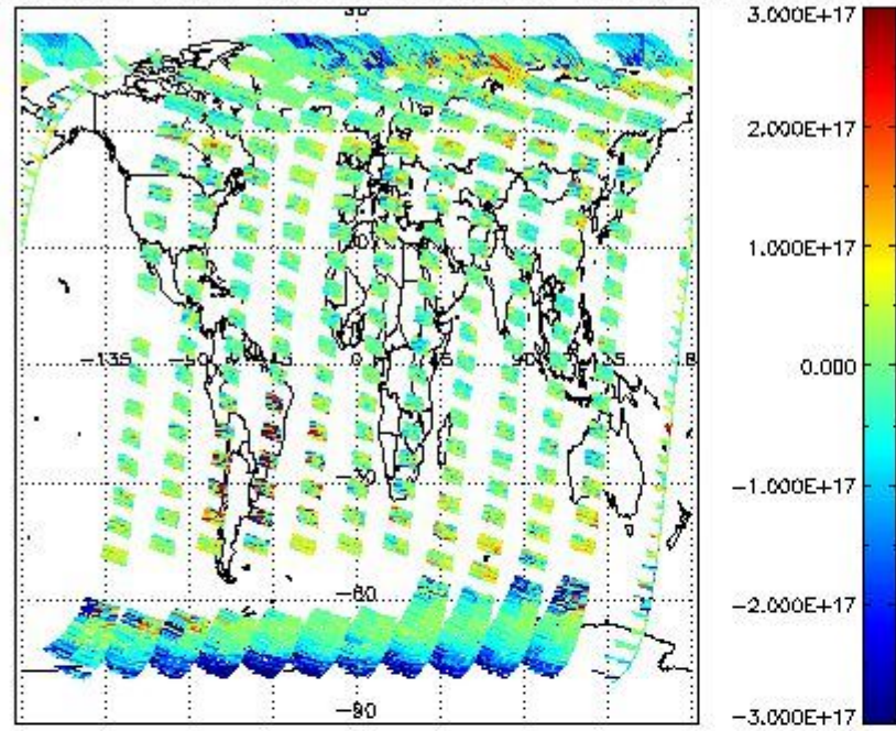
SCIOL2P_NADUV5S02_vcd for 11SEP2011 00:00:00 to 12SEP2011 00:00:00
