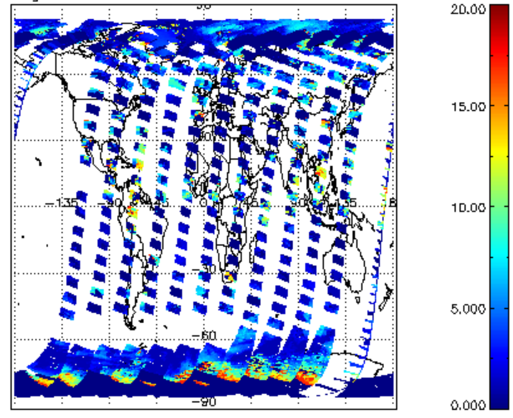
cL_top_height for 11SEP2011 00:00:00 to 12SEP2011 00:00:00
