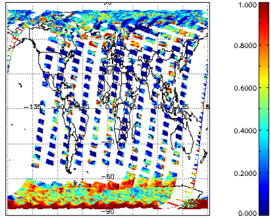
cL_frac for 11SEP2011 00:00:00 to 12SEP2011 00:00:00
