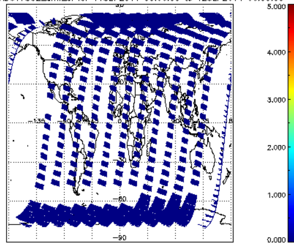
SCIOL2P_NADUV7S02_amf_cl for 11SEP2011 00:00:00 to 12SEP2011 00:00:00
