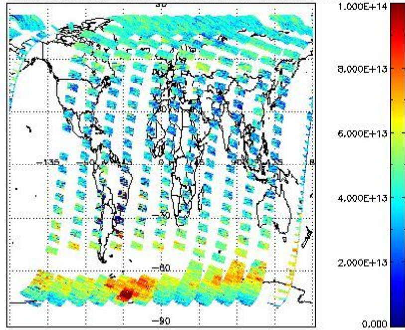
SCIOL2P_NADUV3BRO_vcd for 11SEP2011 00:00:00 to 12SEP2011 00:00:00
