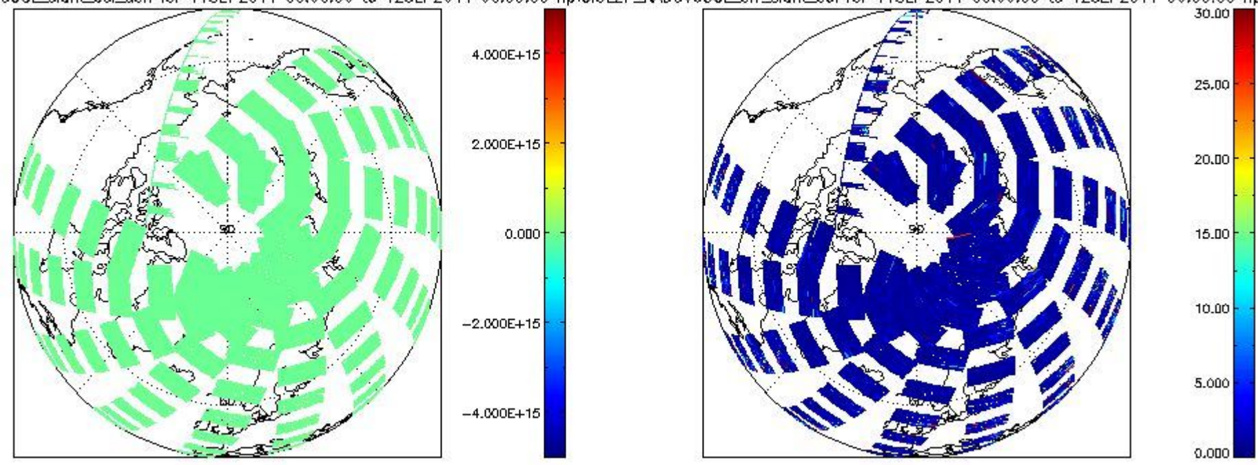
CIOL2P_NADUV60CLslant_col_den for 11SEP2011 00:00:00 to 12SEP2011 00:00:00 np; CIOL2P_NADUV60CLerr_slant_col for 11SEP2011 00:00:00 to 12SEP2011 00:00:00 np
