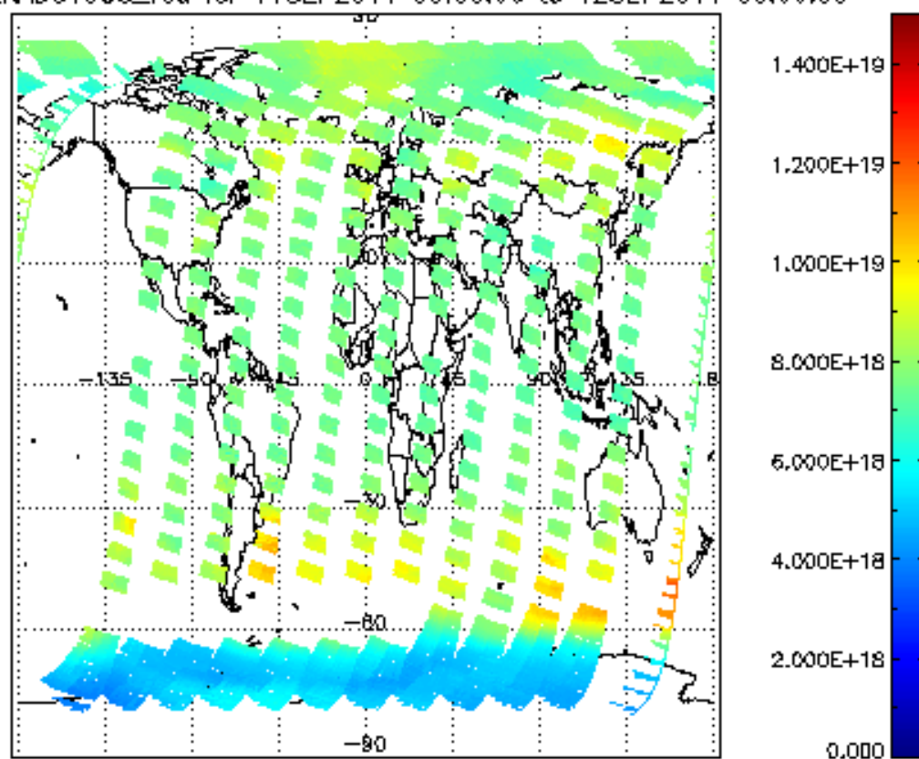
SCIOL2P_NADUV003_vcd for 11SEP2011 00:00:00 to 12SEP2011 00:00:00
