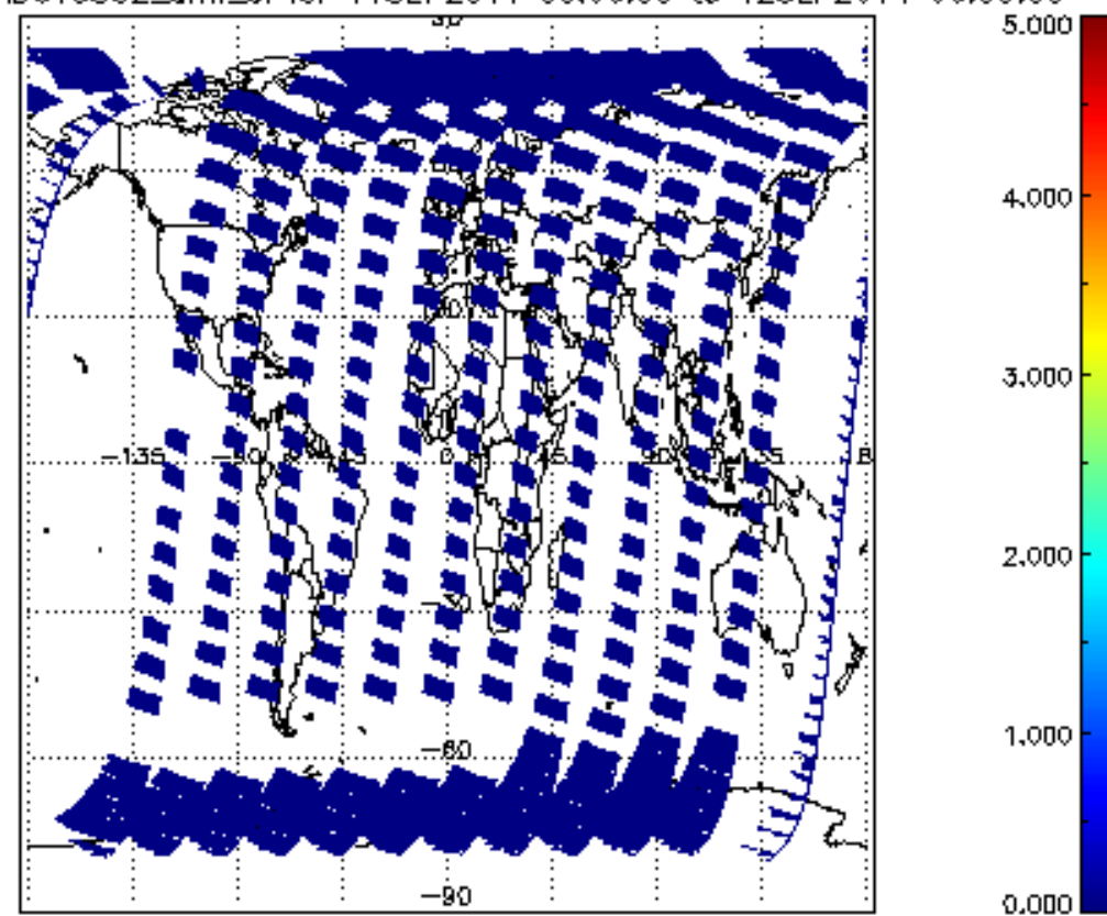
SCIOL2P_NADUV5S02_amf_cl for 11SEP2011 00:00:00 to 12SEP2011 00:00:00
