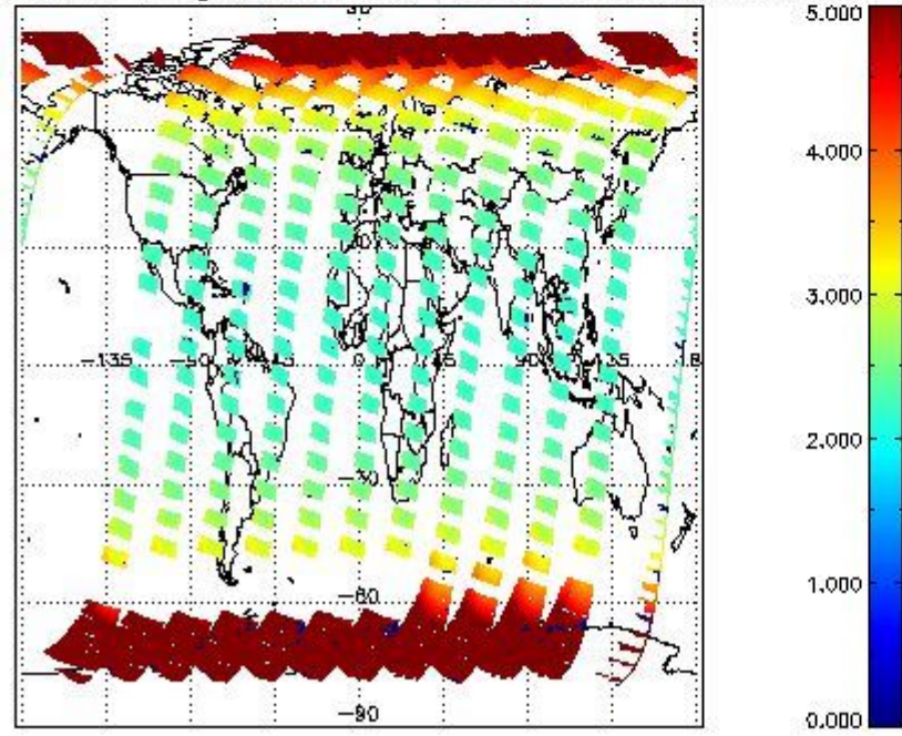
SCIOL2P_NADUV1NO2_amf_gr for 11SEP2011 00:00:00 to 12SEP2011 00:00:00
