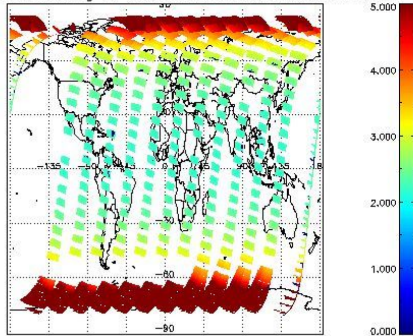
SCIOL2P_NADUV003_amf_gr for 11SEP2011 00:00:00 to 12SEP2011 00:00:00
