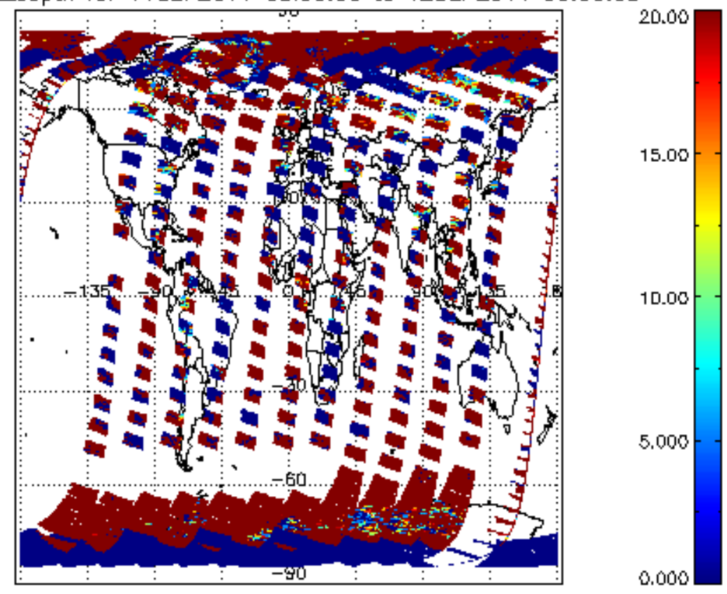
cL_opt_depth for 11SEP2011 00:00:00 to 12SEP2011 00:00:00
