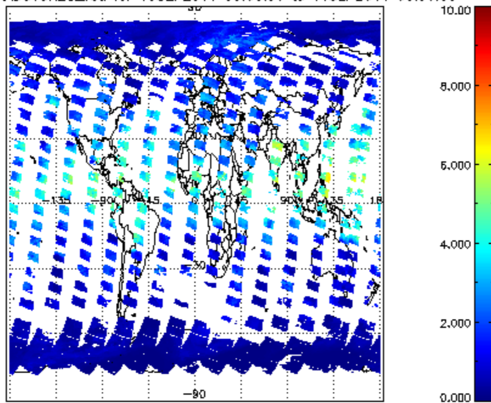
SCIOL2P_NADUV8H20_vcd for 10SEP2011 00:00:00 to 11SEP2011 00:00:00
