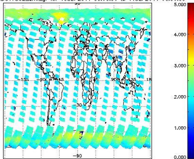
SCIOL2P_NADUV7S02_amf_gr for 10SEP2011 00:00:00 to 11SEP2011 00:00:00
