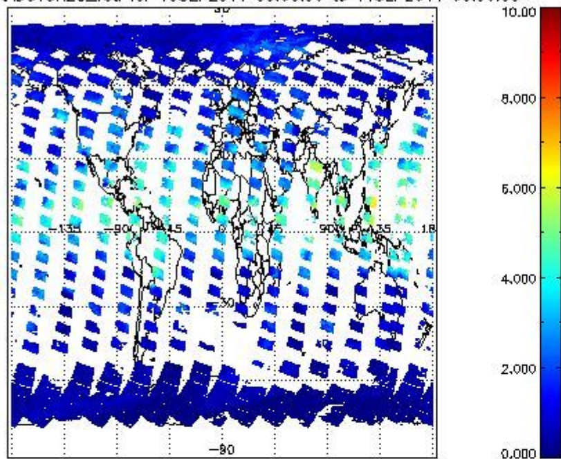
SCIOL2P_NADUV8H2O_vcd for 10SEP2011 00:00:00 to 11SEP2011 00:00:00
