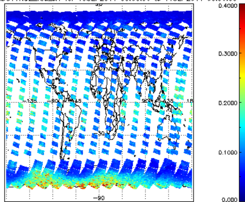
SCIOL2P_NADUV1NO2_vcd_err for 10SEP2011 00:00:00 to 11SEP2011 00:00:00
