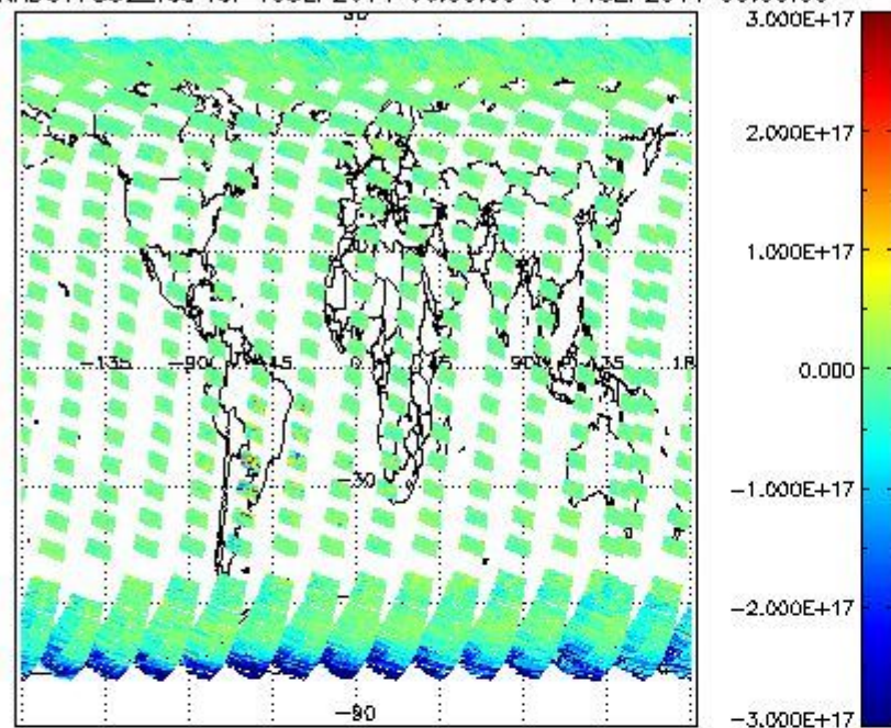
SCIOL2P_NADUV7S02_vcd for 10SEP2011 00:00:00 to 11SEP2011 00:00:00
