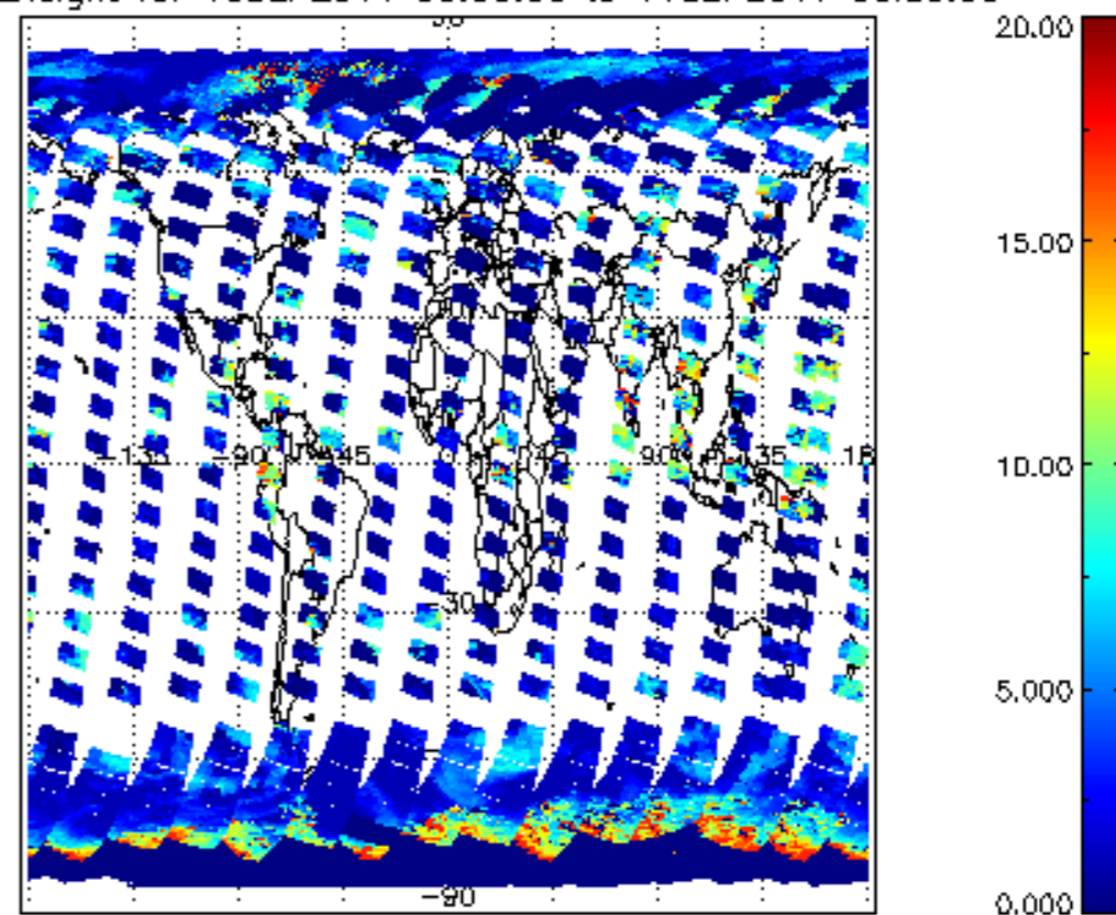
cL_top_height for 10SEP2011 00:00:00 to 11SEP2011 00:00:00
