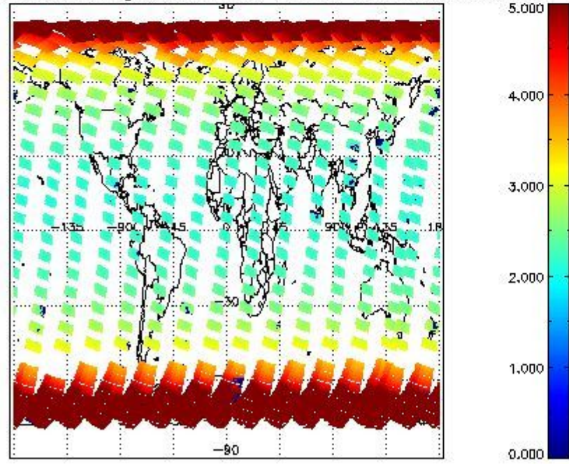
SCIOL2P_NADUV3BRO_amf_gr for 10SEP2011 00:00:00 to 11SEP2011 00:00:00
