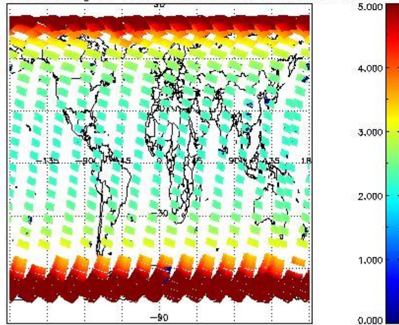
SCIOL2P_NADUV003_amf_gr for 10SEP2011 00:00:00 to 11SEP2011 00:00:00
