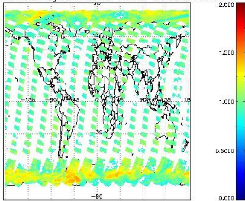
SCIOL2P_NADUV8H2O_arnf_gr for 10SEP2011 00:00:00 to 11SEP2011 00:00:00
