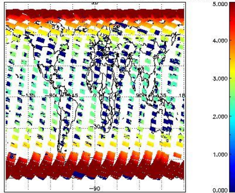
SCIOL2P_NADUV003_amf_cl for 10SEP2011 00:00:00 to 11SEP2011 00:00:00
