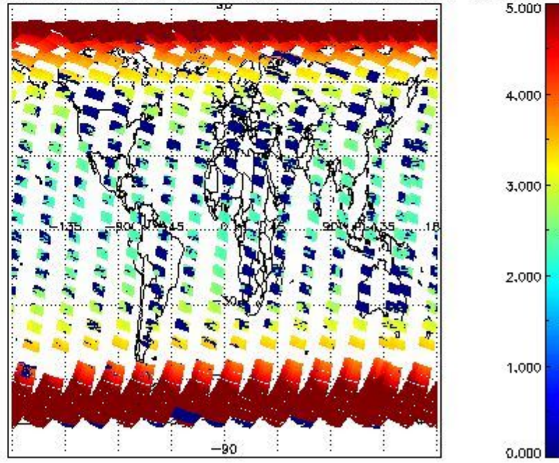
SCIOL2P_NADUV3BRO_amf_cl for 10SEP2011 00:00:00 to 11SEP2011 00:00:00
