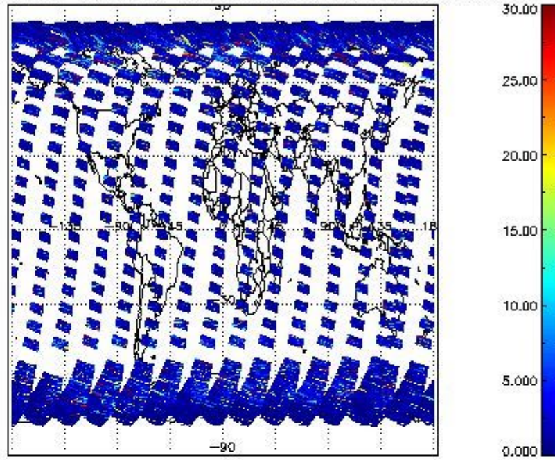
SCIOL2P_NADUV5S02_vcd_err for 10SEP2011 00:00:00 to 11SEP2011 00:00:00
