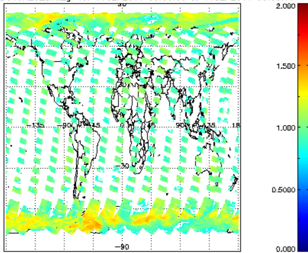
SCIOL2P_NADUV8H20_amf_gr for 10SEP2011 00:00:00 to 11SEP2011 00:00:00
