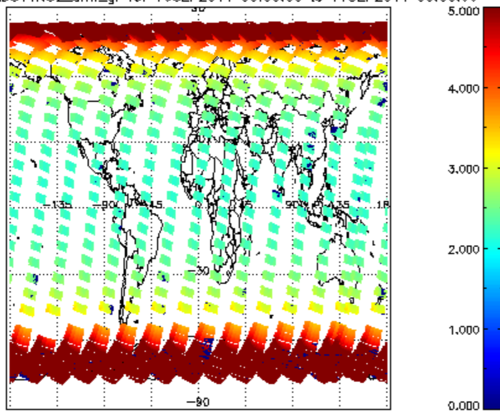
SCIOL2P_NADUV1NO2_amf_gr for 10SEP2011 00:00:00 to 11SEP2011 00:00:00
