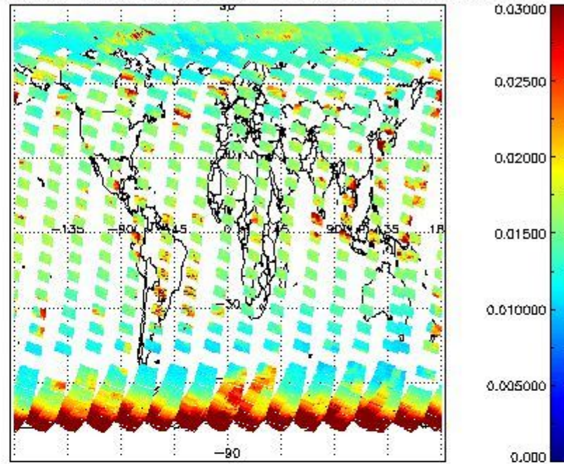
SCIOL2P_NADUV003_vcd_err for 10SEP2011 00:00:00 to 11SEP2011 00:00:00
