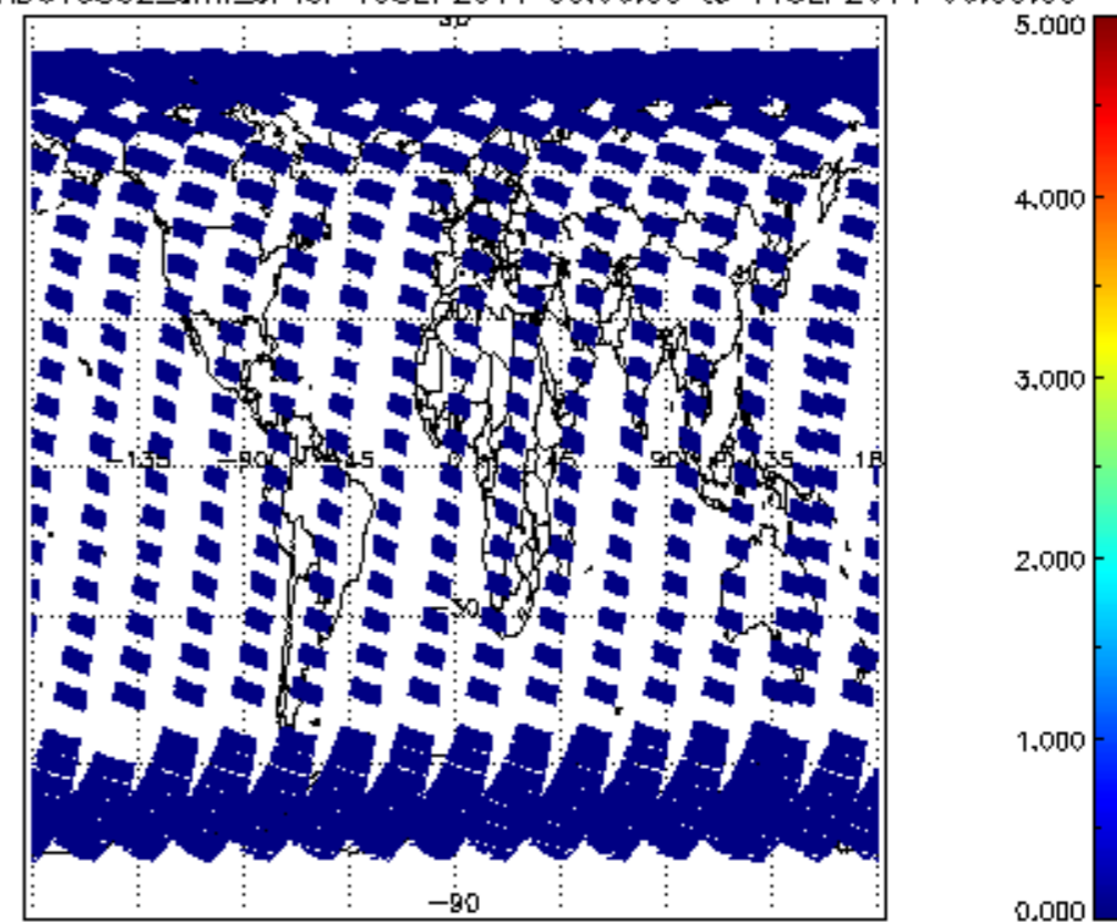
SCIOL2P_NADUV5S02_amf_cl for 10SEP2011 00:00:00 to 11SEP2011 00:00:00
