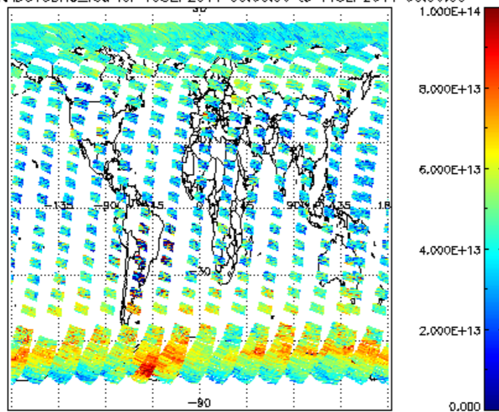
SCIOL2P_NADUV3BRO_vcd for 10SEP2011 00:00:00 to 11SEP2011 00:00:00
