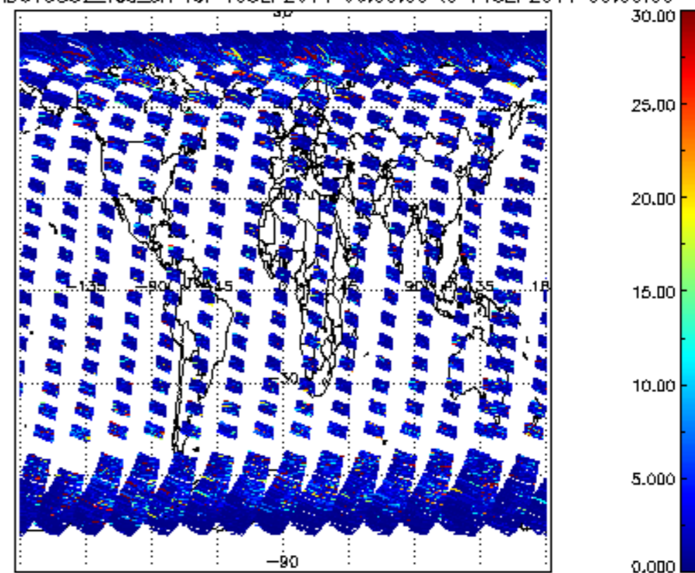
SCIOL2P_NADUV5S02_vcd_err for 10SEP2011 00:00:00 to 11SEP2011 00:00:00
