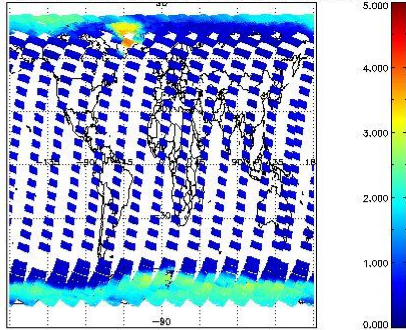
SCIOL2P_NADUV5S02_amf_gr for 10SEP2011 00:00:00 to 11SEP2011 00:00:00
