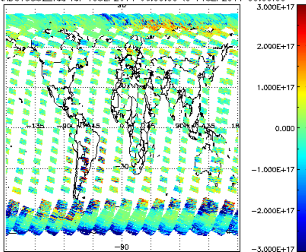
SCIOL2P_NADUV5S02_vcd for 10SEP2011 00:00:00 to 11SEP2011 00:00:00
