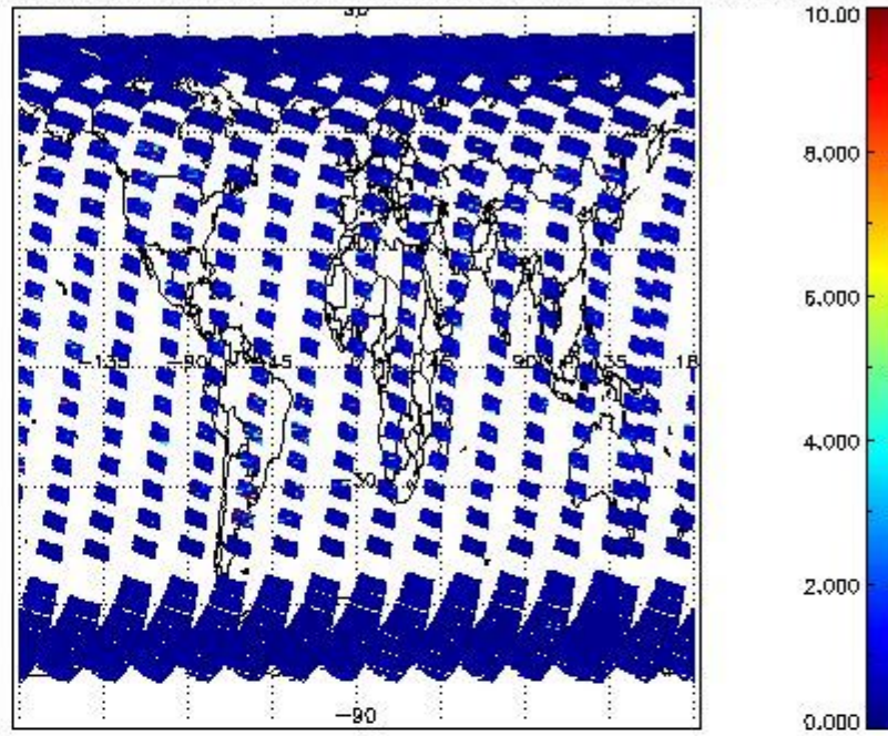
SCIOL2P_NADUV3BRO_vcd_err for 10SEP2011 00:00:00 to 11SEP2011 00:00:00
