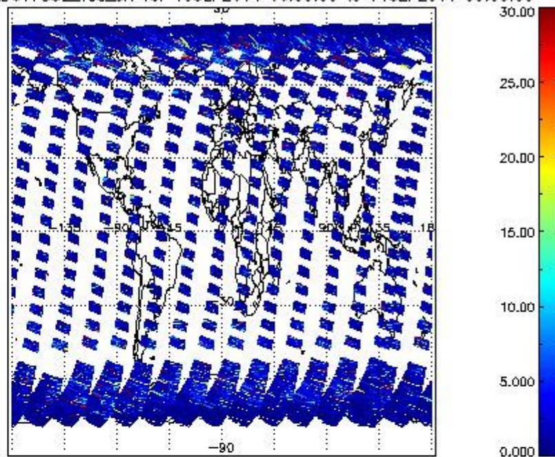
SCIOL2P_NADUV7S02_vcd_err for 10SEP2011 00:00:00 to 11SEP2011 00:00:00
