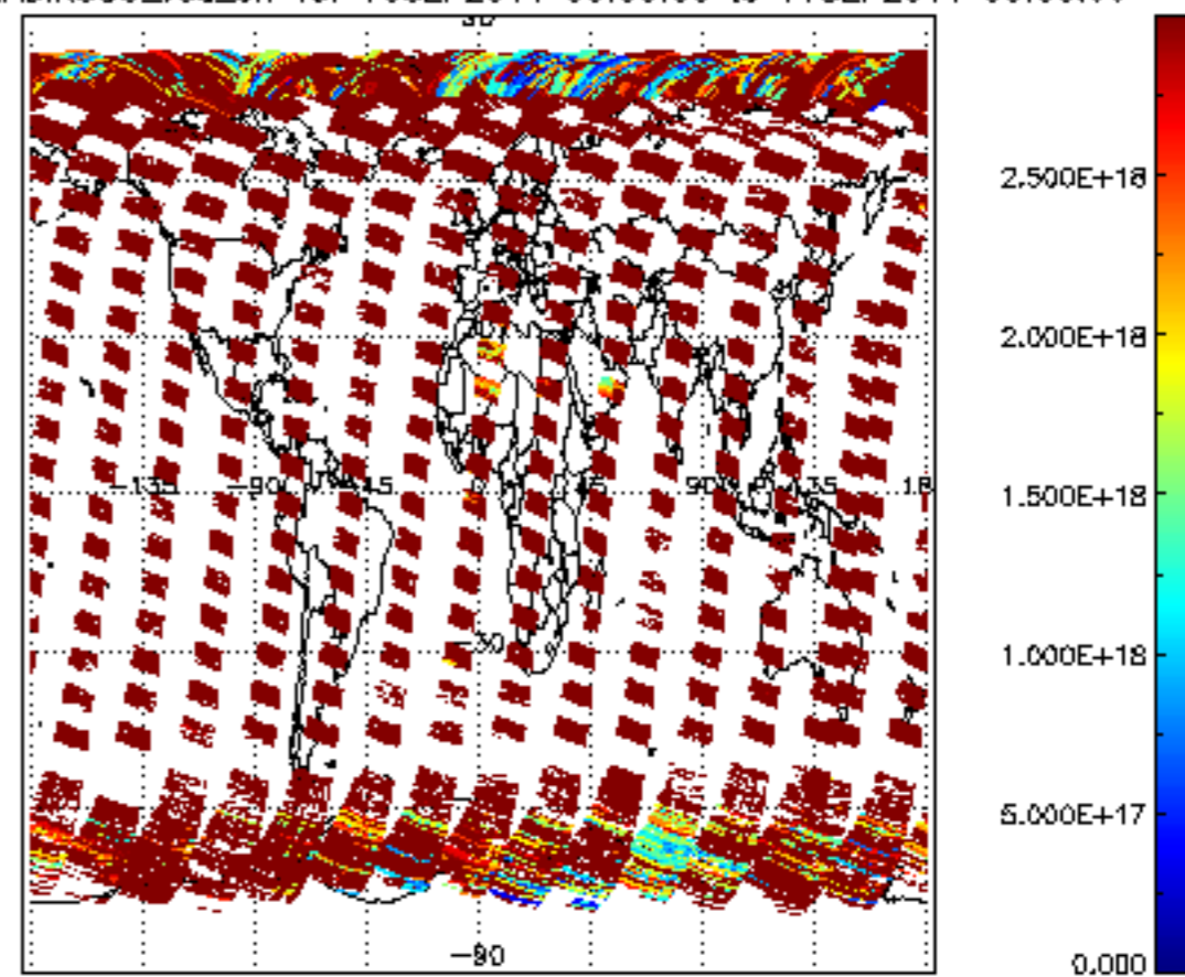
SCIOL2P_NADIR3CO_vcd_err for 10SEP2011 00:00:00 to 11SEP2011 00:00:00
