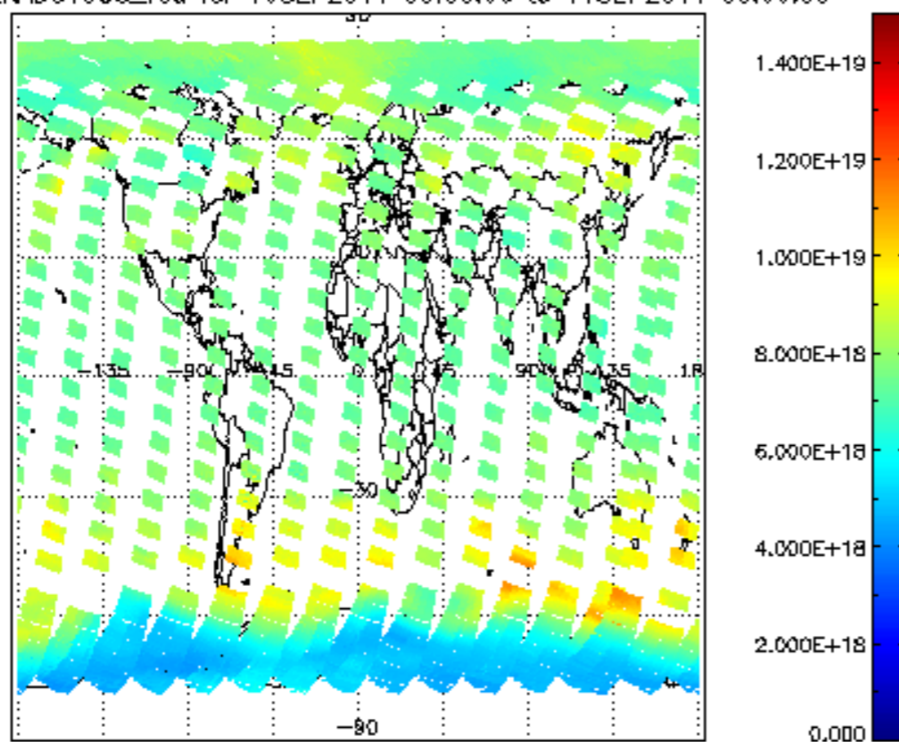
SCIOL2P_NADUV003_vcd for 10SEP2011 00:00:00 to 11SEP2011 00:00:00
