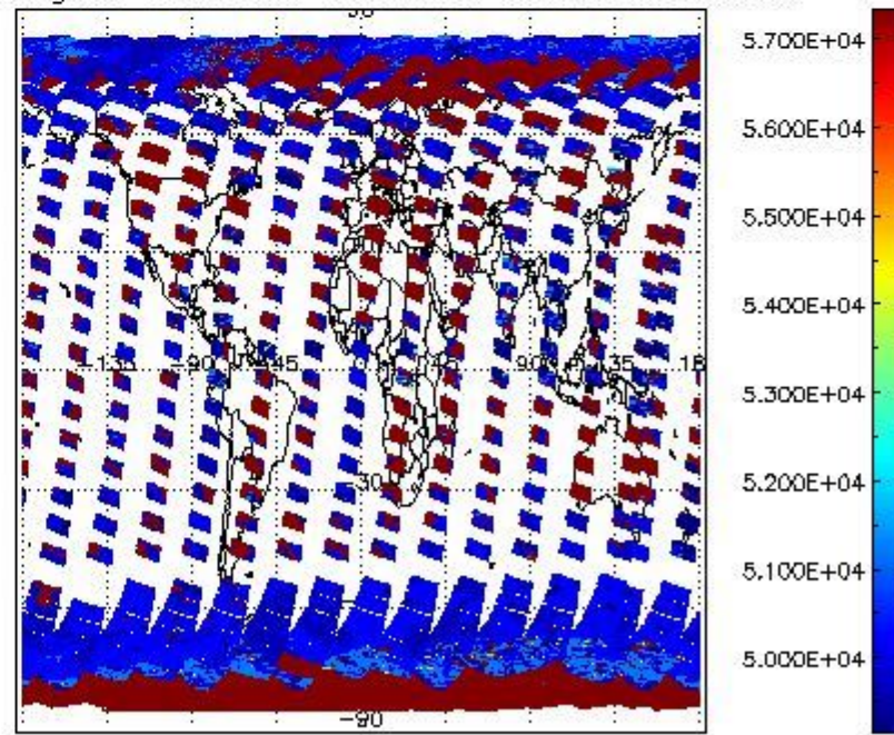
cloud_flags for 10SEP2011 00:00:00 to 11SEP2011 00:00:00
