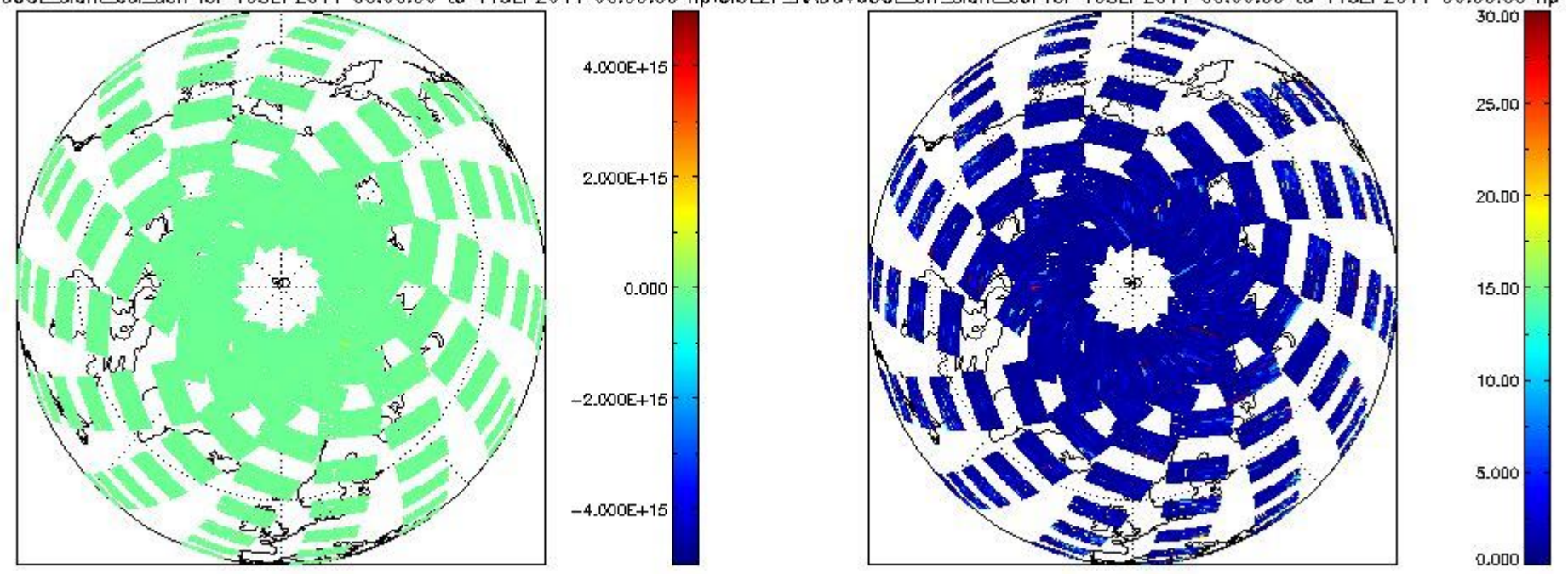
CIOL2P_NADUV60CLslant_col_den for 10SEP2011 00:00:00 to 11SEP2011 00:00:00 np; CIOL2P_NADUV60CLerr_slant_col for 10SEP2011 00:00:00 to 11SEP2011 00:00:00 np
