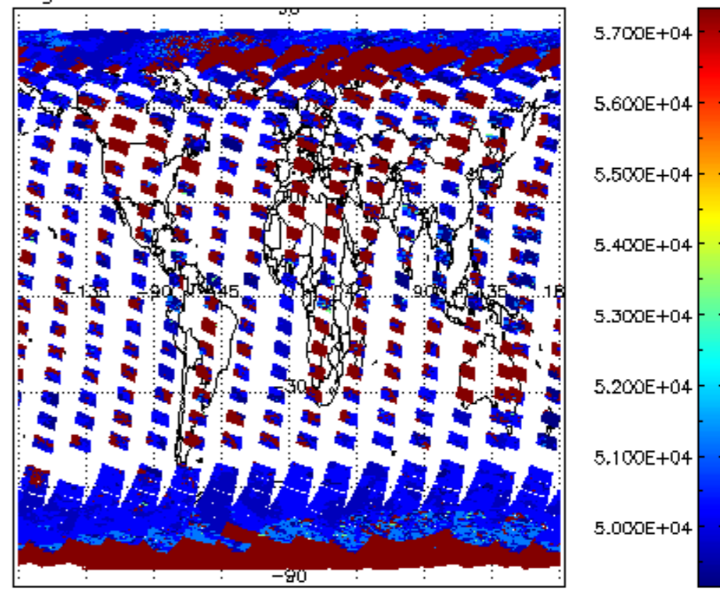
cloud_flags for 10SEP2011 00:00:00 to 11SEP2011 00:00:00
