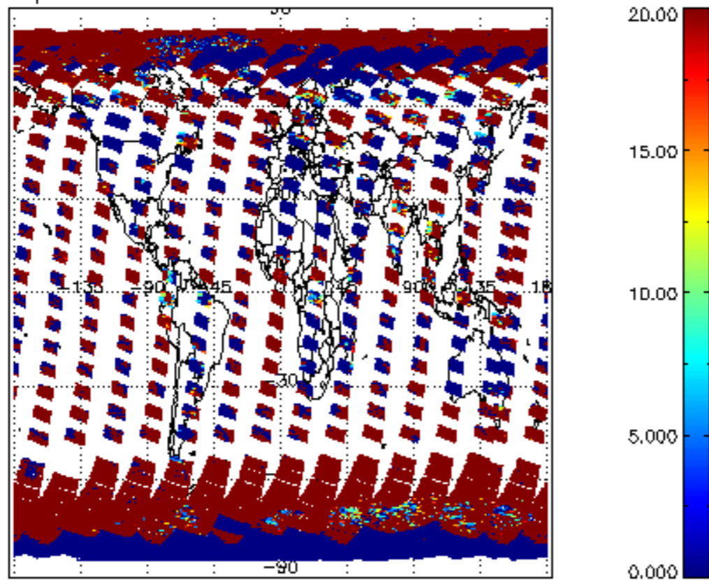
cL_opt_depth for 10SEP2011 00:00:00 to 11SEP2011 00:00:00
