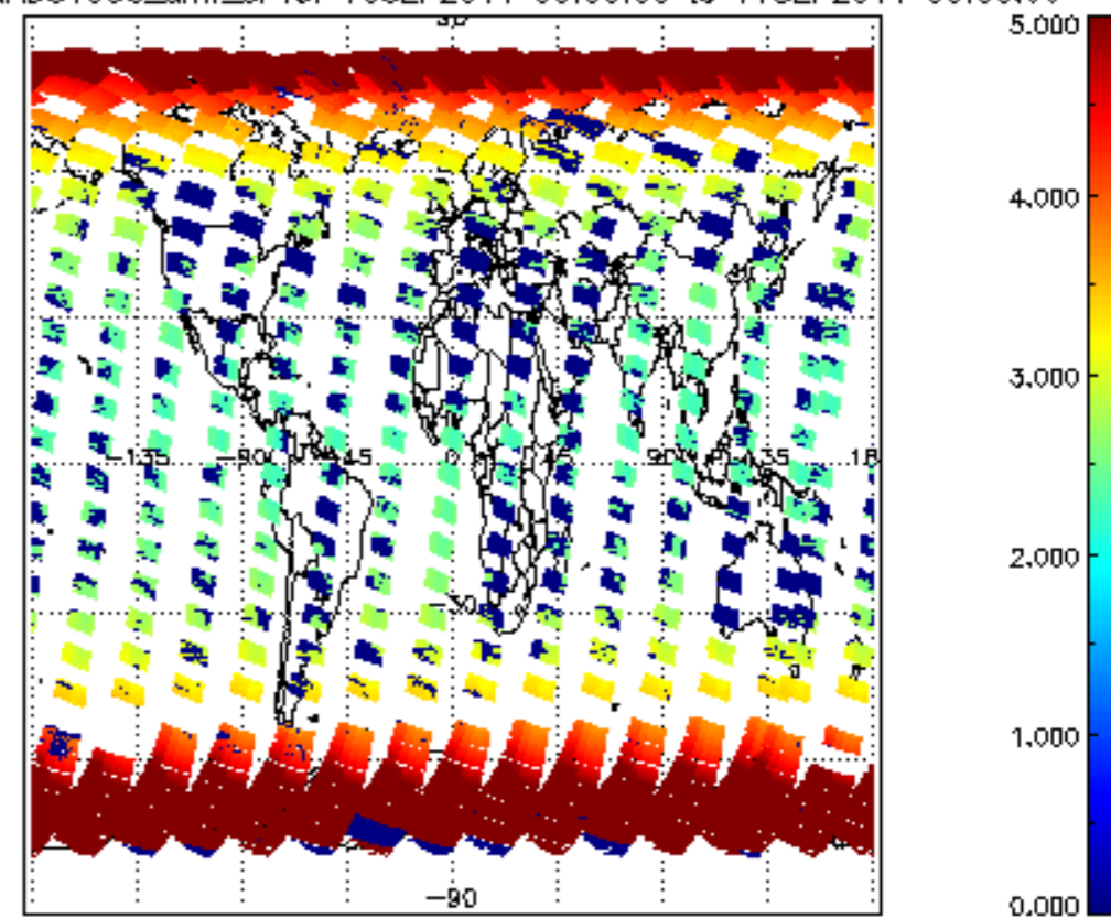
SCIOL2P_NADUV003_amf_cl for 10SEP2011 00:00:00 to 11SEP2011 00:00:00
