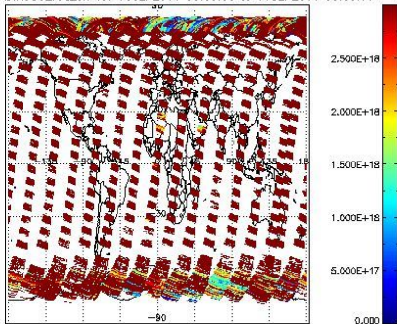
SCIDL2P_NADIR3CO_vcd_err for 10SEP2011 00:00:00 to 11SEP2011 00:00:00
