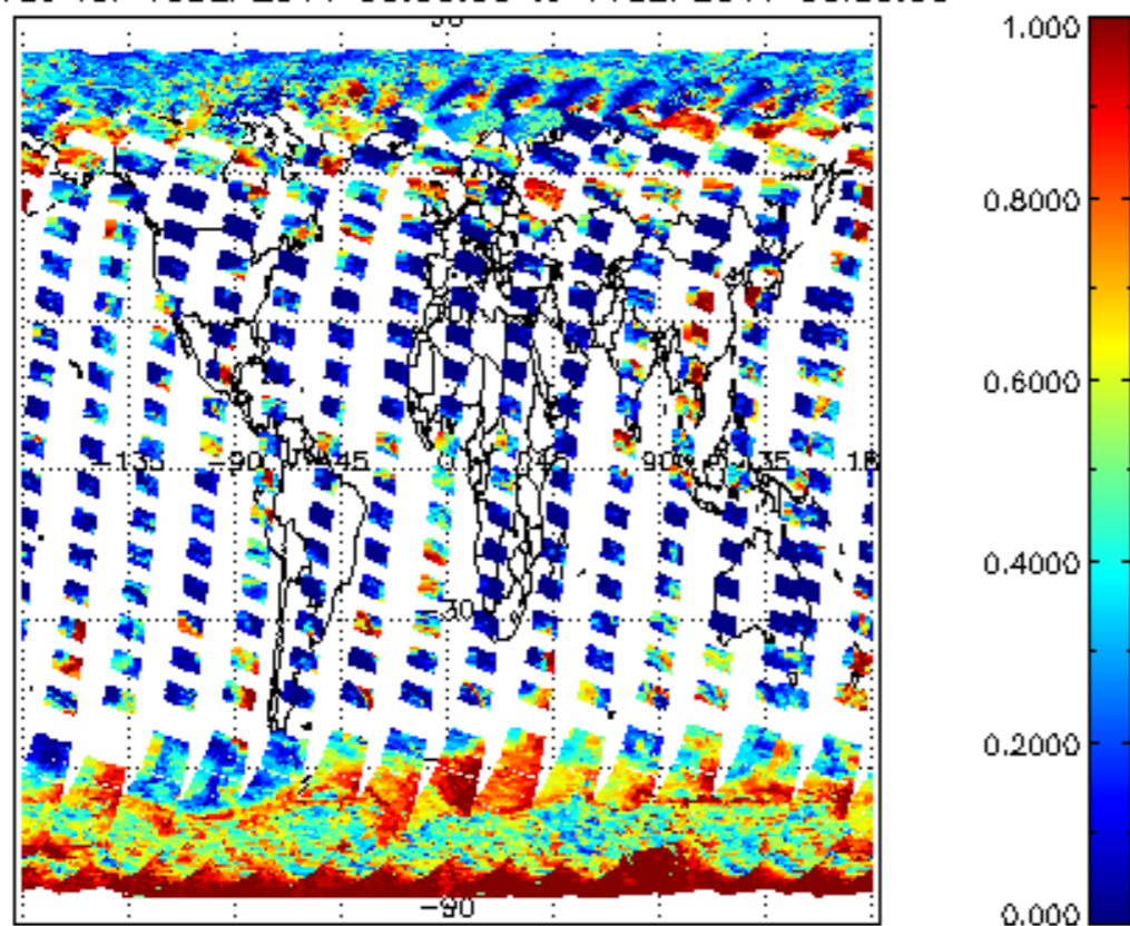
cL_frac for 10SEP2011 00:00:00 to 11SEP2011 00:00:00
