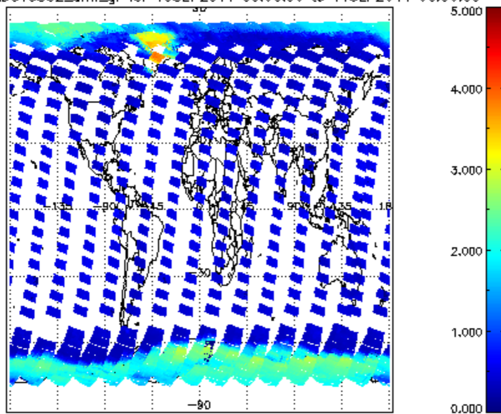
SCIOL2P_NADUV5S02_amf_gr for 10SEP2011 00:00:00 to 11SEP2011 00:00:00
