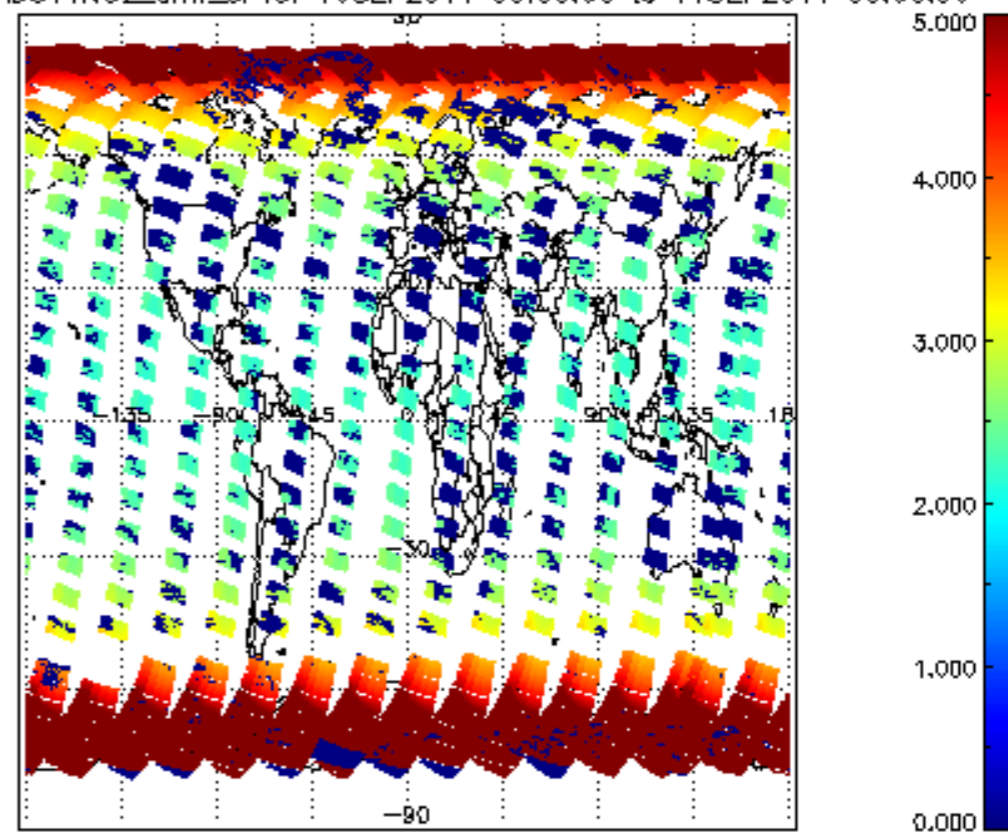
SCIOL2P_NADUV1NO2_amf_sl for 10SEP2011 00:00:00 to 11SEP2011 00:00:00
