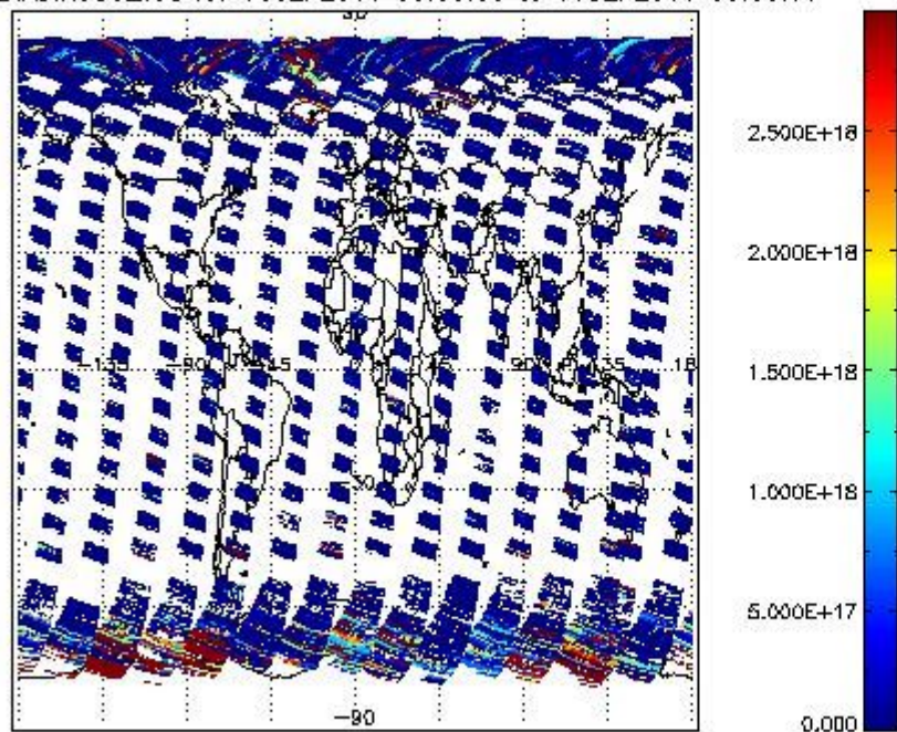
SCIDL2P_NADIR3CO_vcd for 10SEP2011 00:00:00 to 11SEP2011 00:00:00
