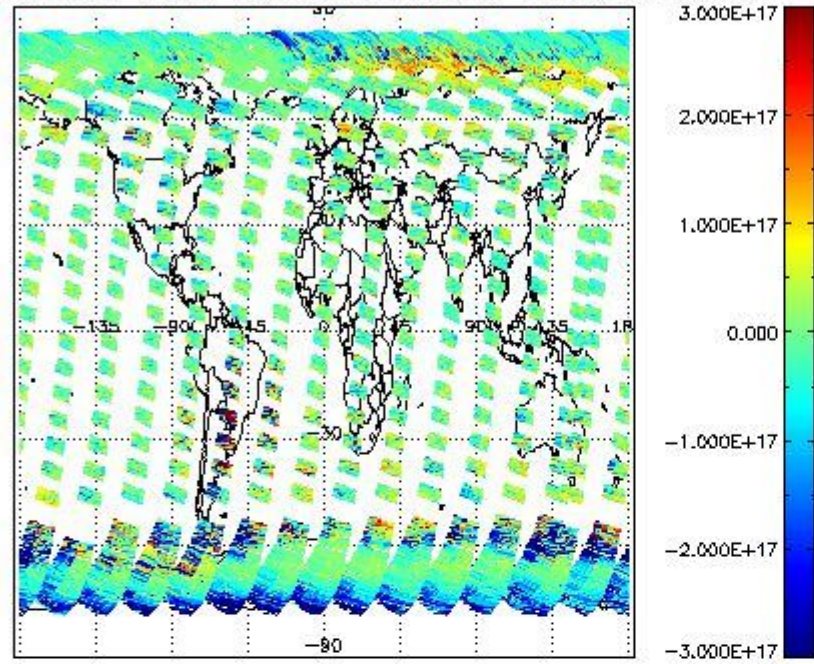
SCIOL2P_NADUV5S02_vcd for 10SEP2011 00:00:00 to 11SEP2011 00:00:00
