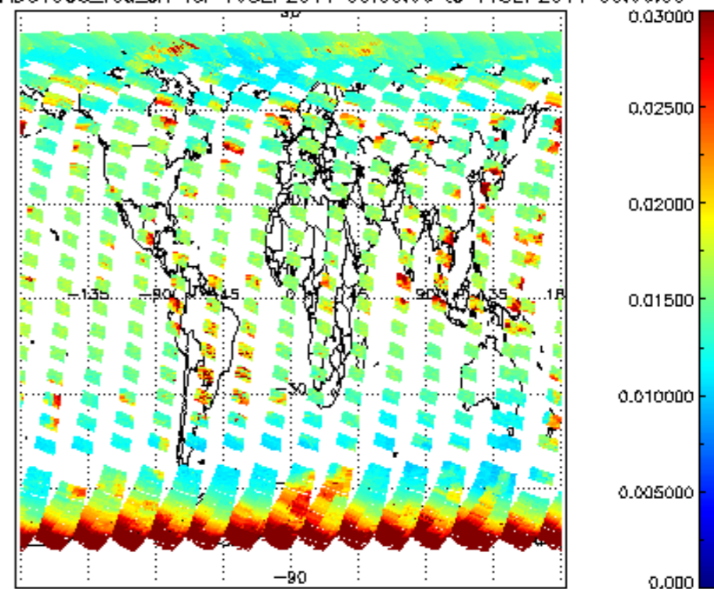
SCIOL2P_NADUV003_vcd_err for 10SEP2011 00:00:00 to 11SEP2011 00:00:00
