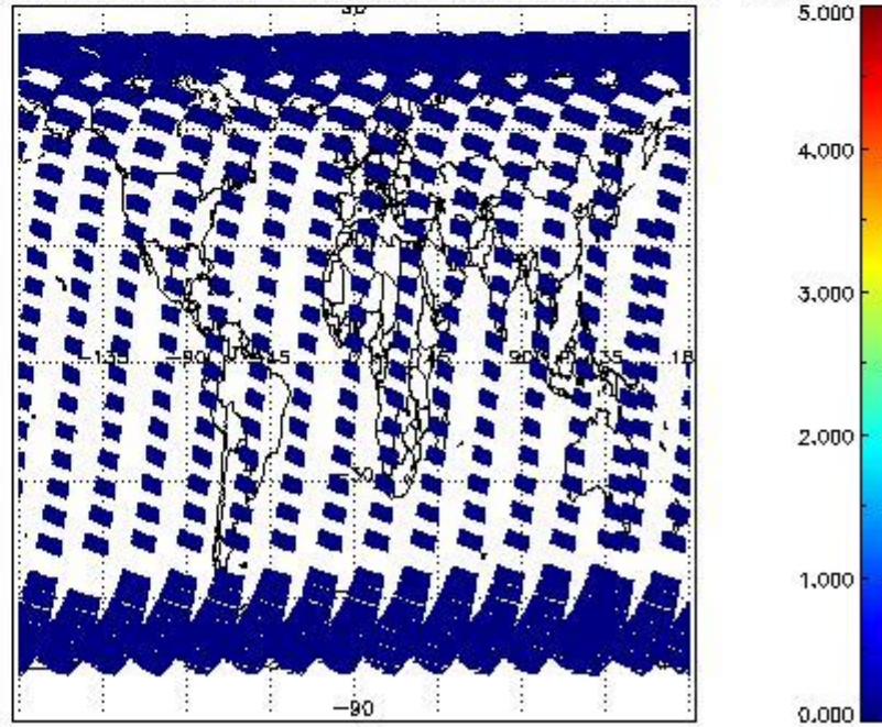
SCIOL2P_NADUV5S02_amf_cl for 10SEP2011 00:00:00 to 11SEP2011 00:00:00
