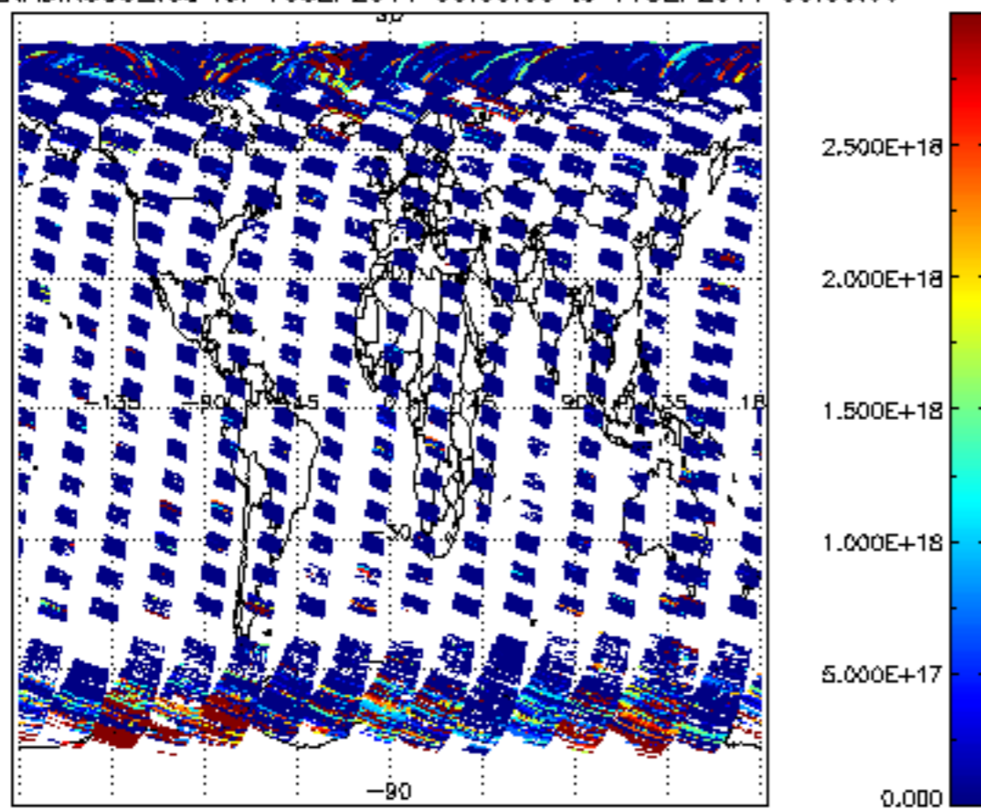
SCIOL2P_NADIR3CO_vcd for 10SEP2011 00:00:00 to 11SEP2011 00:00:00
