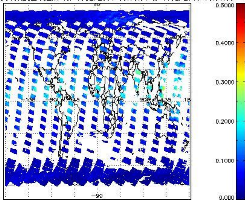
SCIOL2P_NADUV8H2O_vcd_err for 10SEP2011 00:00:00 to 11SEP2011 00:00:00
