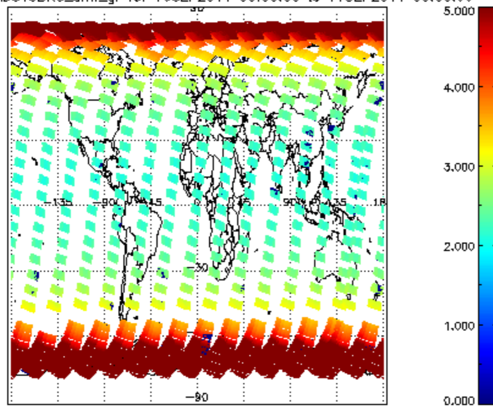
SCIOL2P_NADUV3BRO_amf_gr for 10SEP2011 00:00:00 to 11SEP2011 00:00:00
