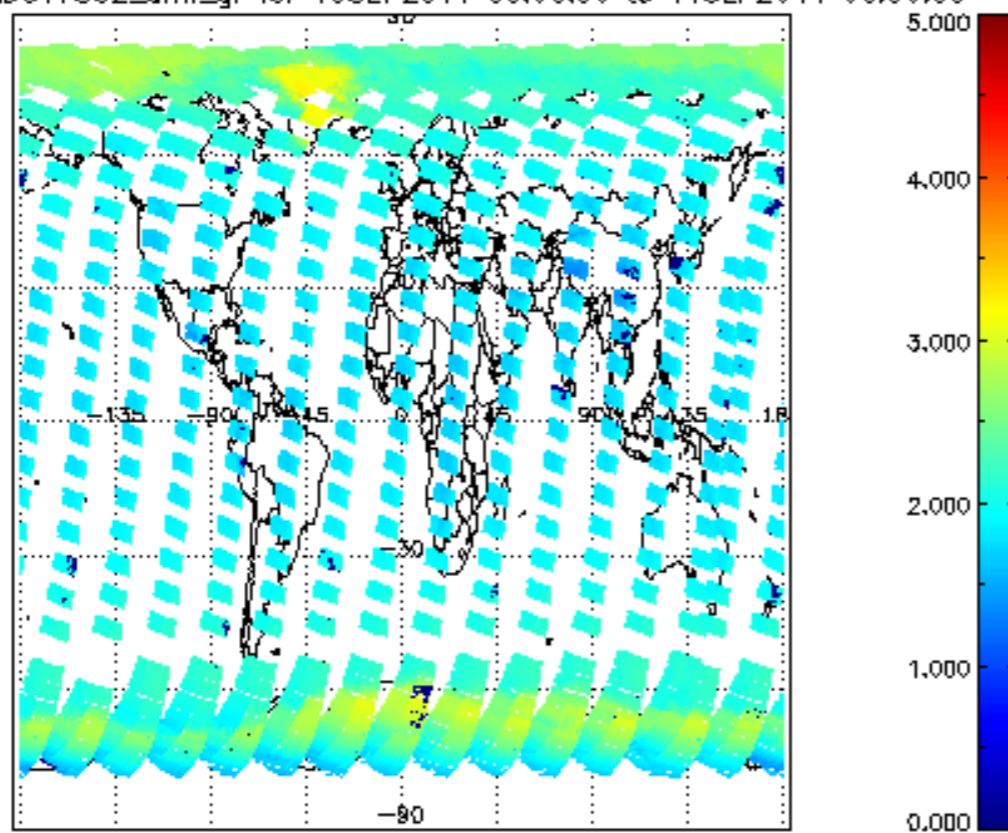
SCIOL2P_NADUV7S02_amf_gr for 10SEP2011 00:00:00 to 11SEP2011 00:00:00
