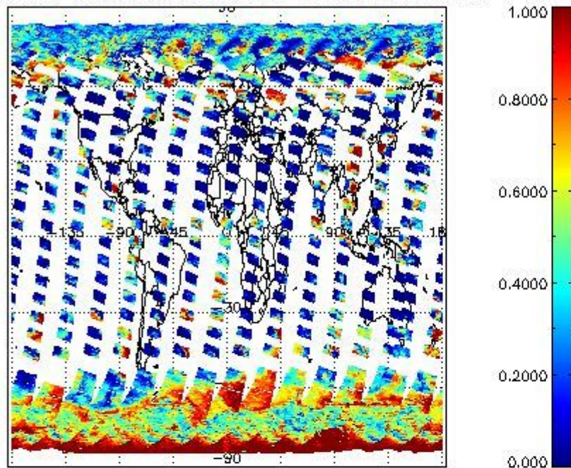
cL_frac for 10SEP2011 00:00:00 to 11SEP2011 00:00:00
