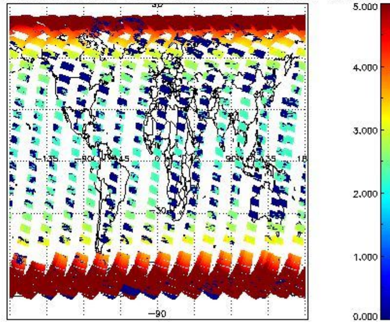
SCIOL2P_NADUV1NO2_amf_cl for 10SEP2011 00:00:00 to 11SEP2011 00:00:00
