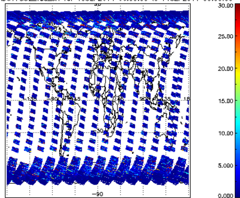
SCIOL2P_NADUV7S02_vcd_err for 10SEP2011 00:00:00 to 11SEP2011 00:00:00
