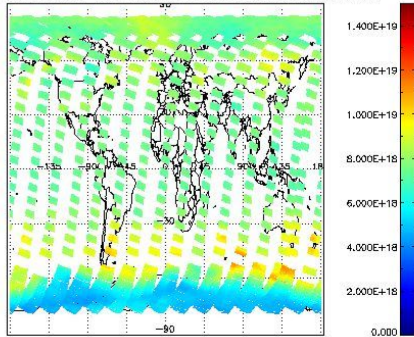
SCIOL2P_NADUV003_vcd for 10SEP2011 00:00:00 to 11SEP2011 00:00:00
