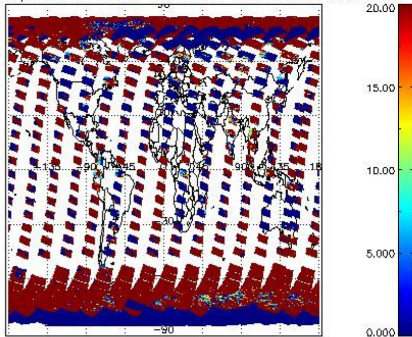
cL_opt_depth for 10SEP2011 00:00:00 to 11SEP2011 00:00:00
