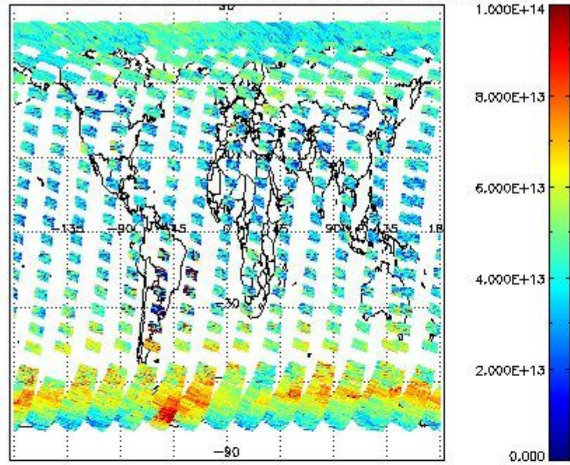
SCIOL2P_NADUV3BRO_vcd for 10SEP2011 00:00:00 to 11SEP2011 00:00:00
