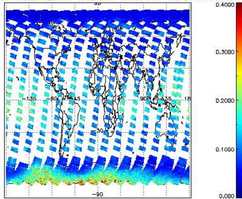
SCIOL2P_NADUV1NO2_vcd_err for 10SEP2011 00:00:00 to 11SEP2011 00:00:00
