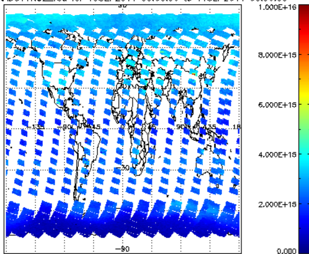
SCIOL2P_NADUV1NO2_vcd for 10SEP2011 00:00:00 to 11SEP2011 00:00:00
