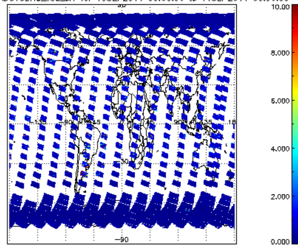
SCIOL2P_NADUV3BRO_vcd_err for 10SEP2011 00:00:00 to 11SEP2011 00:00:00
