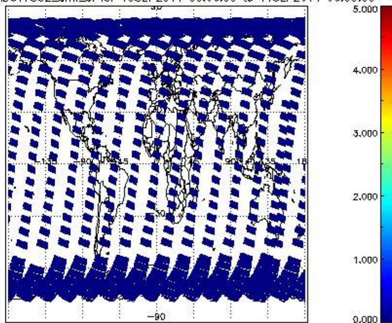
SCIOL2P_NADUV7S02_amf_cl for 10SEP2011 00:00:00 to 11SEP2011 00:00:00
