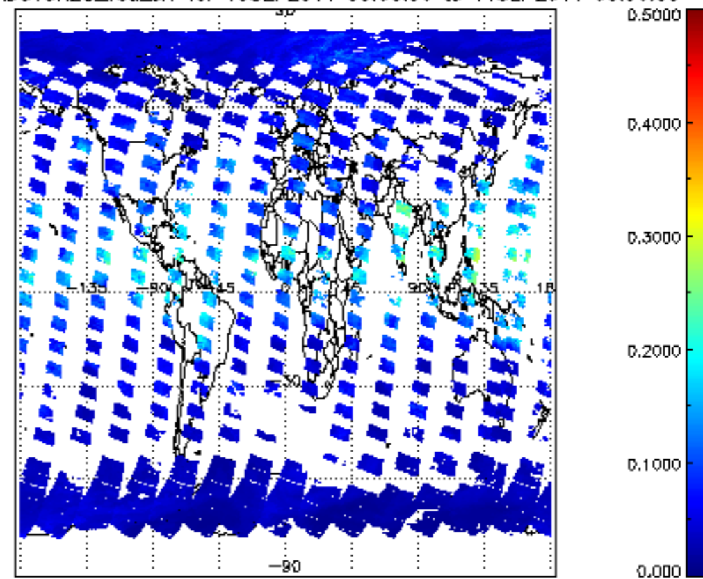
SCIOL2P_NADUV8H20_vcd_err for 10SEP2011 00:00:00 to 11SEP2011 00:00:00
