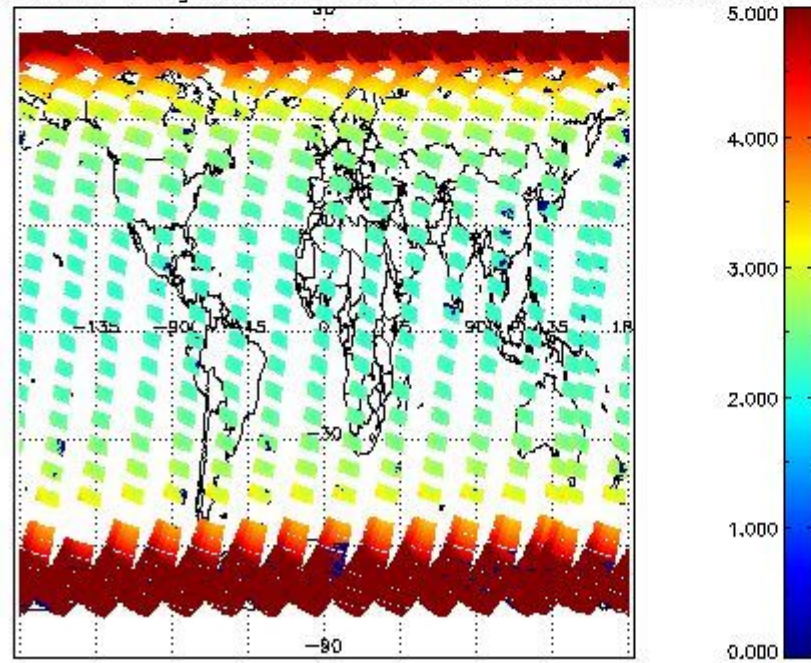
SCIOL2P_NADUV1NO2_amf_gr for 10SEP2011 00:00:00 to 11SEP2011 00:00:00
