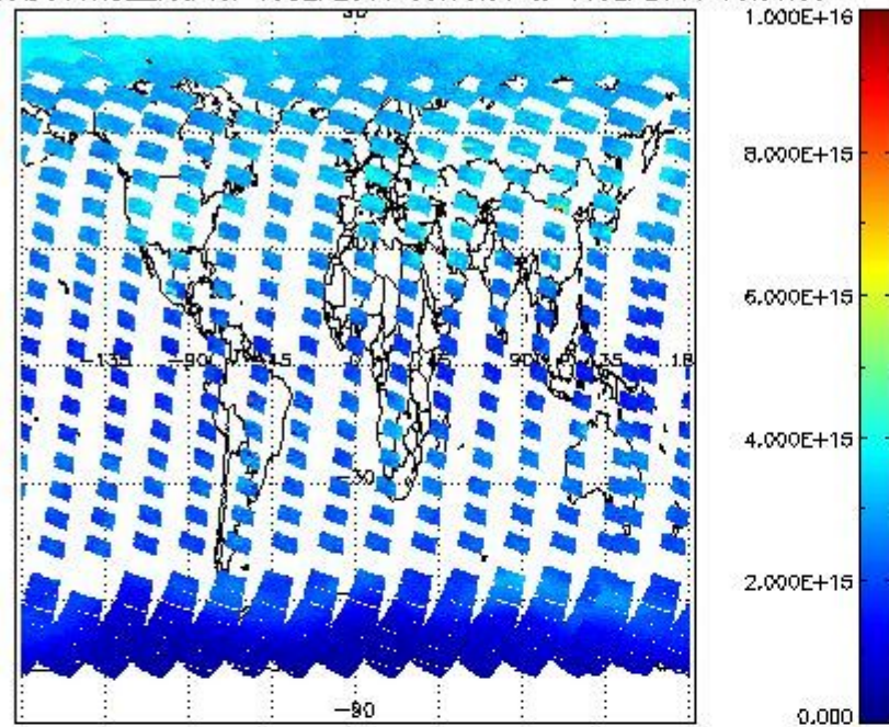
SCIOL2P_NADUV1NO2_vcd for 10SEP2011 00:00:00 to 11SEP2011 00:00:00
