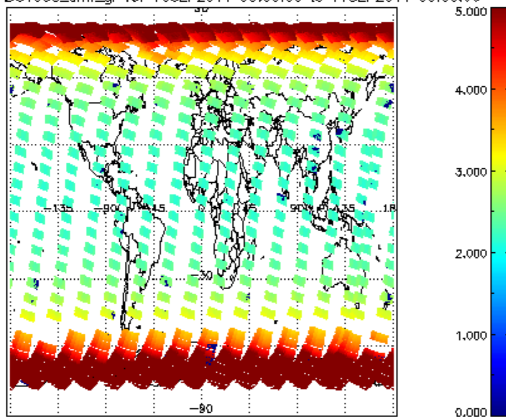
SCIOL2P_NADUV003_amf_gr for 10SEP2011 00:00:00 to 11SEP2011 00:00:00
