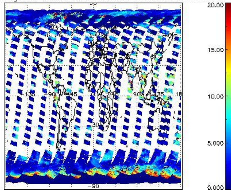
cL_top_height for 10SEP2011 00:00:00 to 11SEP2011 00:00:00
