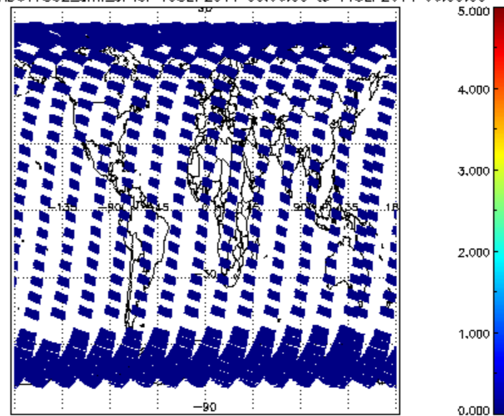
SCIOL2P_NADUV7S02_amf_cl for 10SEP2011 00:00:00 to 11SEP2011 00:00:00
