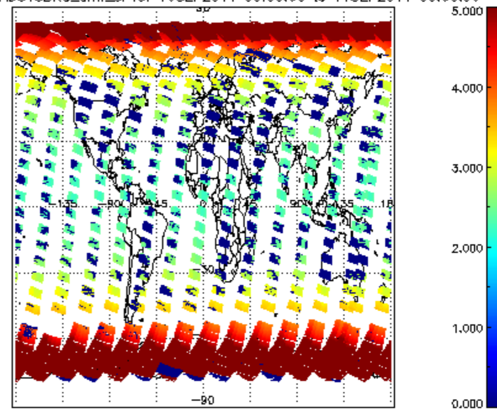
SCIOL2P_NADUV3BRO_amf_cl for 10SEP2011 00:00:00 to 11SEP2011 00:00:00
