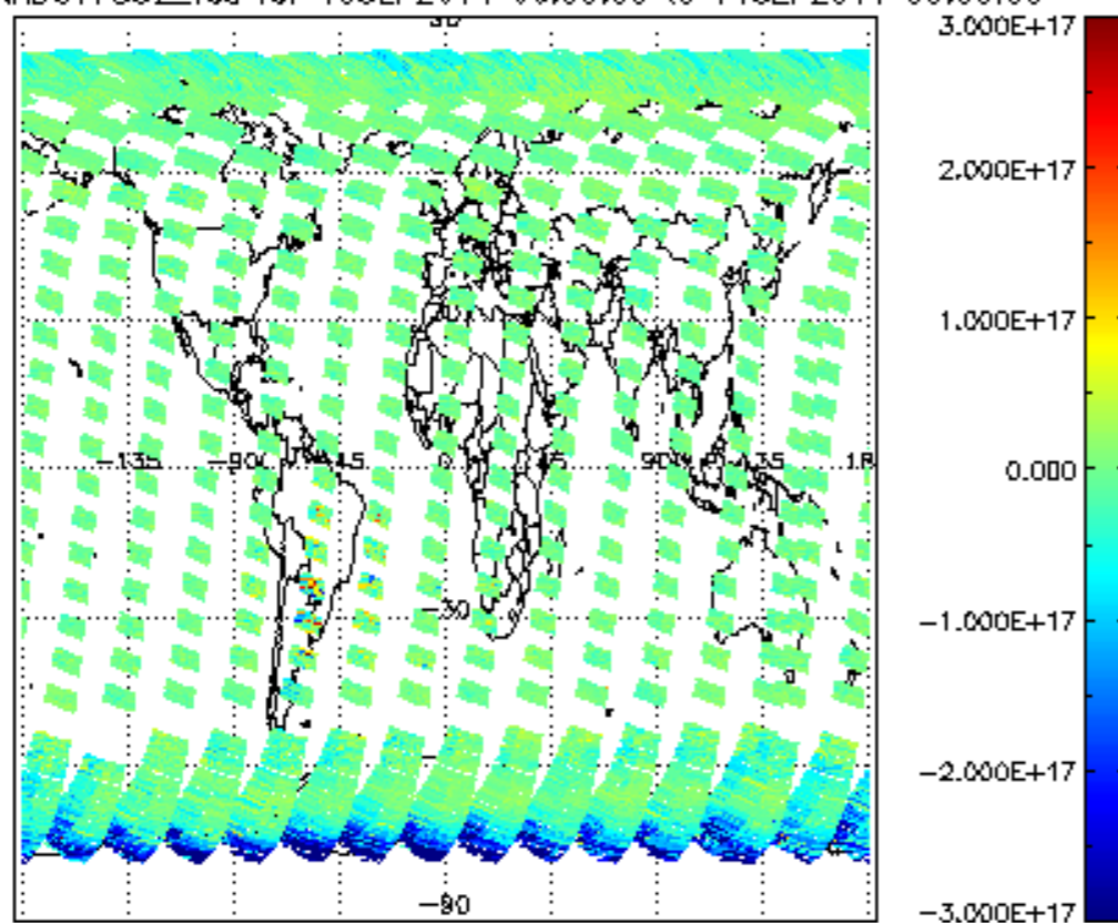
SCIOL2P_NADUV7S02_vcd for 10SEP2011 00:00:00 to 11SEP2011 00:00:00
