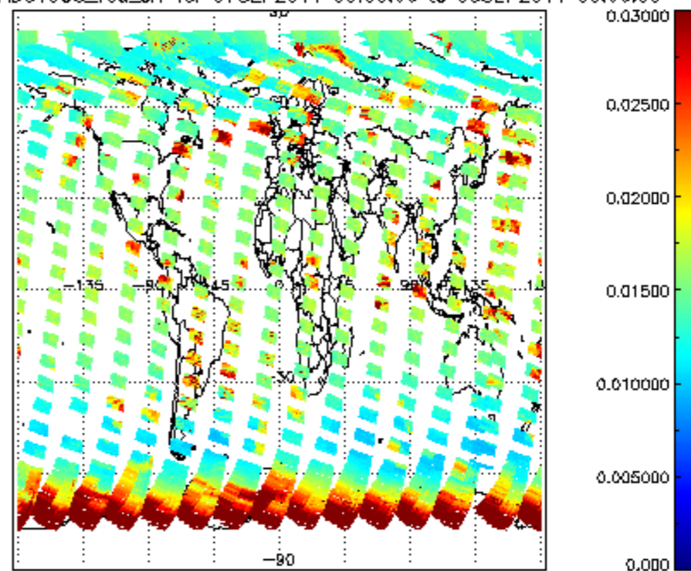
SCIOL2P_NADUV003_vcd_err for 07SEP2011 00:00:00 to 08SEP2011 00:00:00
