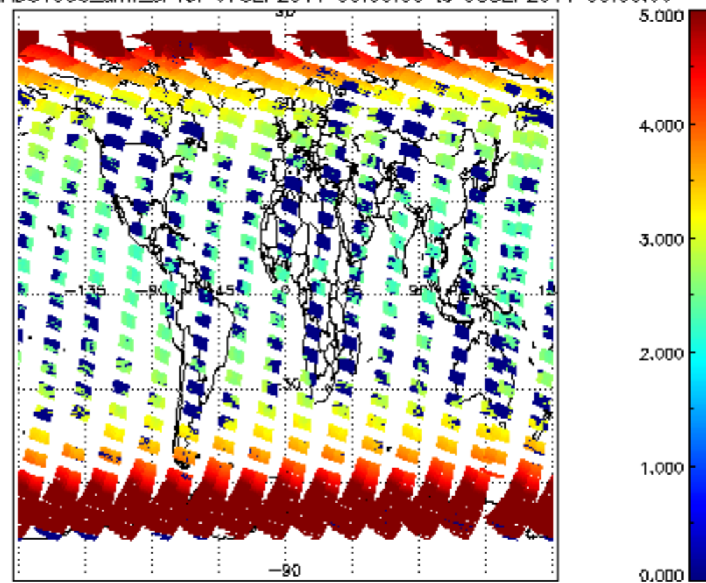
SCIOL2P_NADUV003_amf_cl for 07SEP2011 00:00:00 to 08SEP2011 00:00:00
