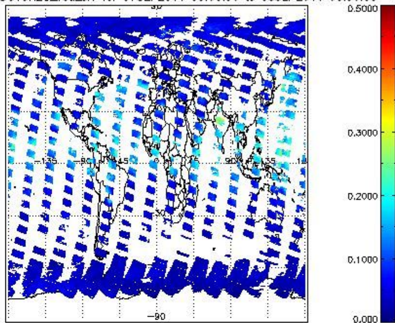
SCIOL2P_NADUV8H2O_vcd_err for 07SEP2011 00:00:00 to 08SEP2011 00:00:00
