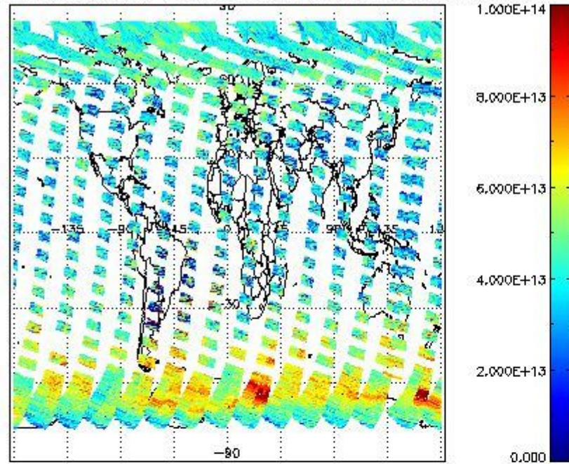
SCIOL2P_NADUV3BRO_vcd for 07SEP2011 00:00:00 to 06SEP2011 00:00:00
