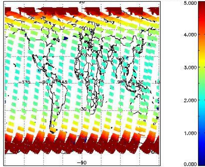
SCIOL2P_NADUV3BRO_amf_gr for 07SEP2011 00:00:00 to 08SEP2011 00:00:00
