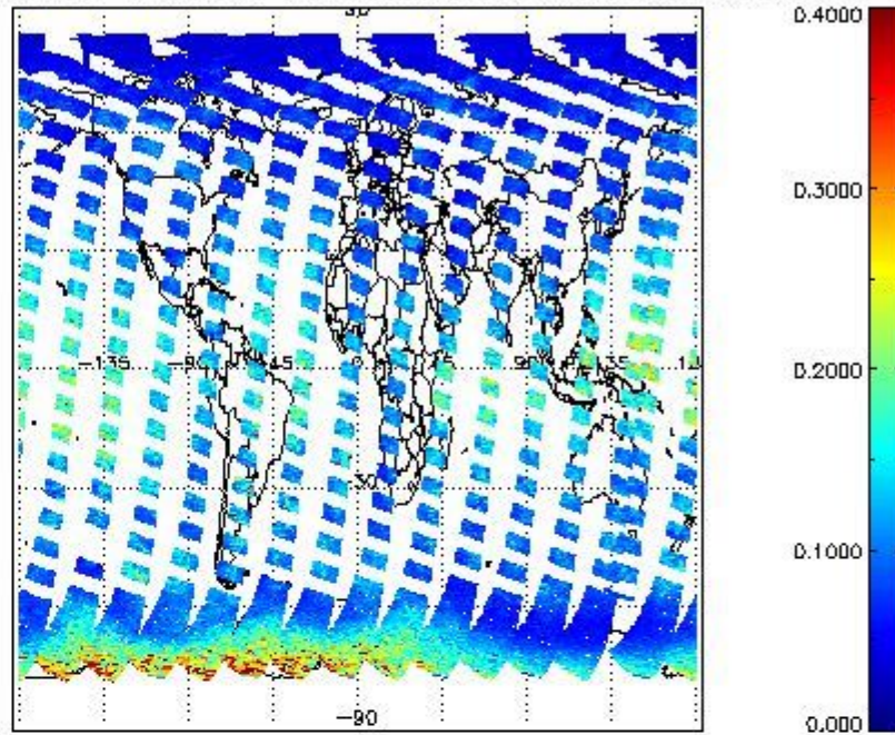
SCIOL2P_NADUV1N02_vcd_err for 07SEP2011 00:00:00 to 08SEP2011 00:00:00
