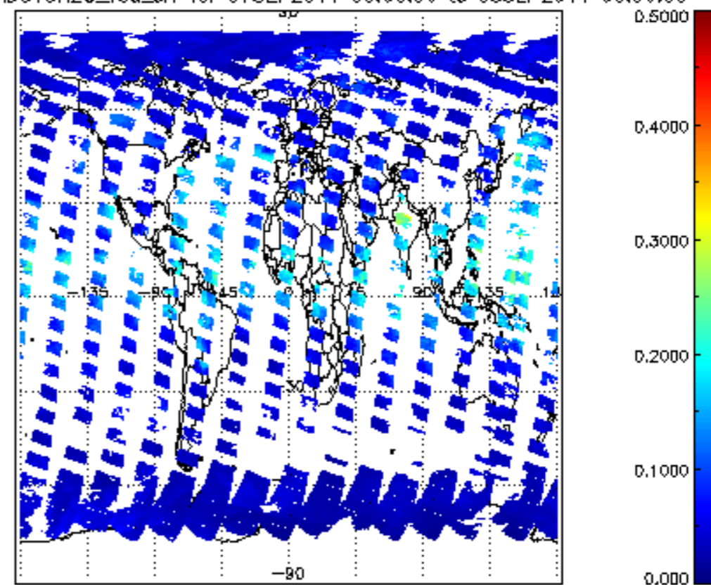
SCIOL2P_NADUV8H20_vcd_err for 07SEP2011 00:00:00 to 08SEP2011 00:00:00
