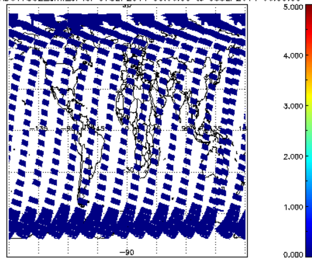
SCIOL2P_NADUV7S02_amf_cl for 07SEP2011 00:00:00 to 08SEP2011 00:00:00
