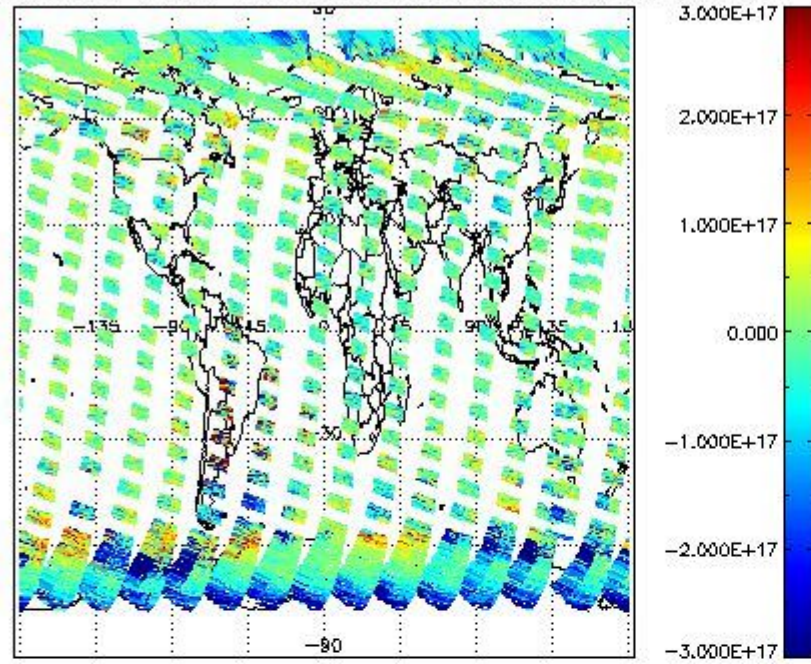
SCIOL2P_NADUV5S02_vcd for 07SEP2011 00:00:00 to 08SEP2011 00:00:00
