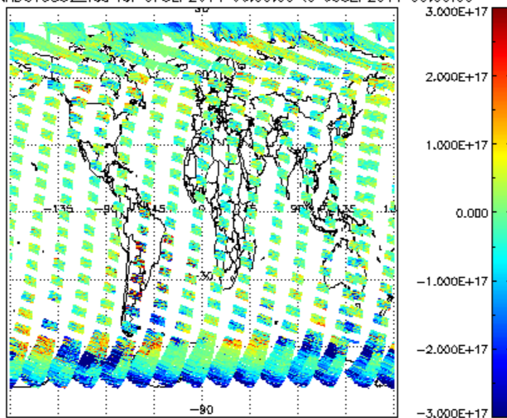
SCIOL2P_NADUV5S02_vcd for 07SEP2011 00:00:00 to 08SEP2011 00:00:00
