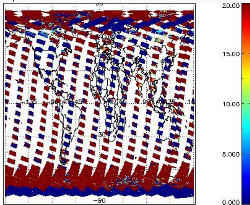
cL_opt_depth for 07SEP2011 00:00:00 to 08SEP2011 00:00:00
