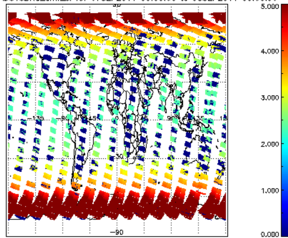
SCIOL2P_NADUV3BRO_amf_cl for 07SEP2011 00:00:00 to 08SEP2011 00:00:00
