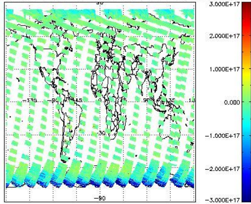
SCIOL2P_NADUV7S02_vcd for 07SEP2011 00:00:00 to 08SEP2011 00:00:00
