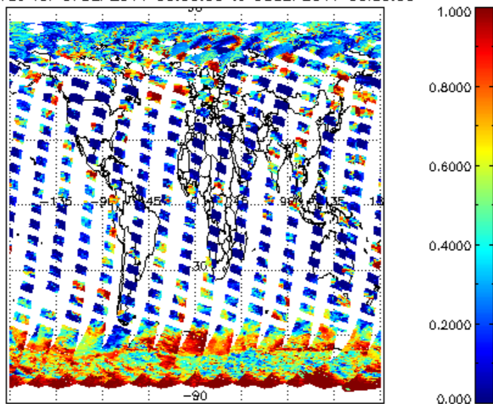
cL_frac for 07SEP2011 00:00:00 to 08SEP2011 00:00:00
