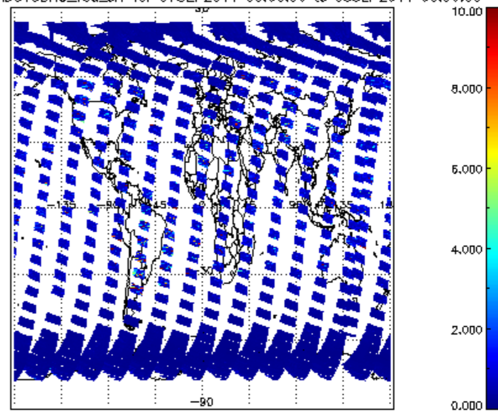
SCIOL2P_NADUV3BRO_vcd_err for 07SEP2011 00:00:00 to 08SEP2011 00:00:00
