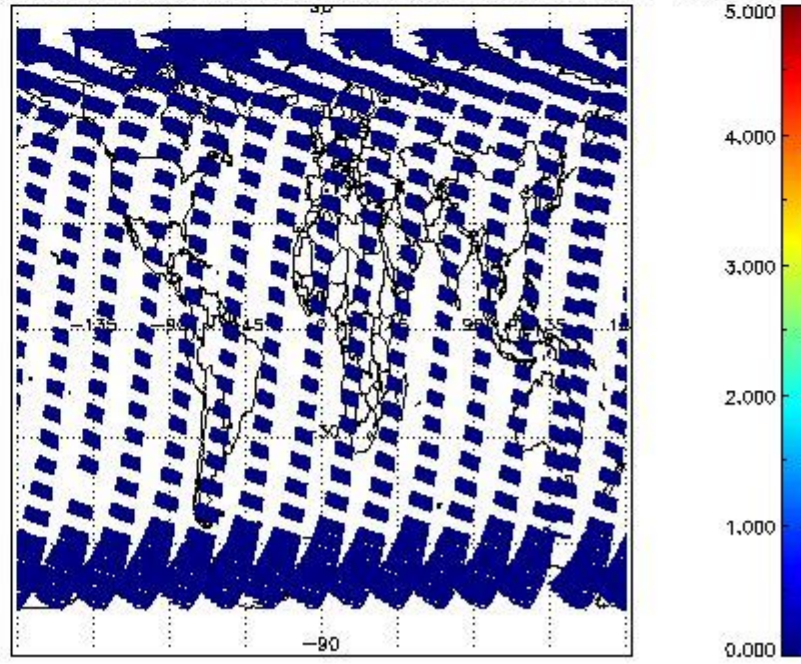
SCIOL2P_NADUV7S02_amf_cl for 07SEP2011 00:00:00 to 08SEP2011 00:00:00
