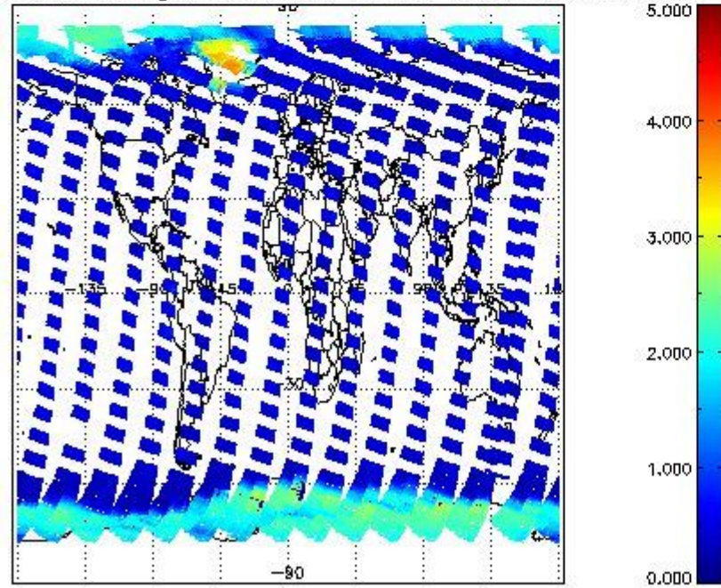
SCIOL2P_NADUV5S02_amf_gr for 07SEP2011 00:00:00 to 08SEP2011 00:00:00
