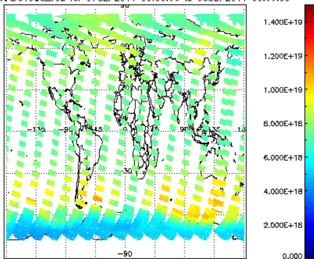
SCIOL2P_NADUV003_vcd for 07SEP2011 00:00:00 to 08SEP2011 00:00:00
