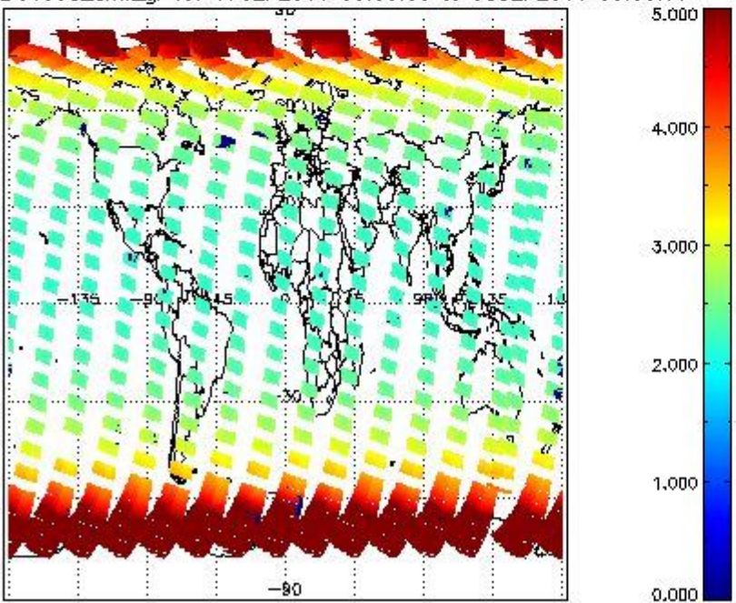
SCIOL2P_NADUV003_amf_gr for 07SEP2011 00:00:00 to 08SEP2011 00:00:00
