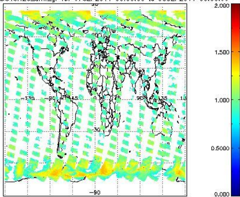
SCIOL2P_NADUV8H2O_arnf_gr for 07SEP2011 00:00:00 to 08SEP2011 00:00:00
