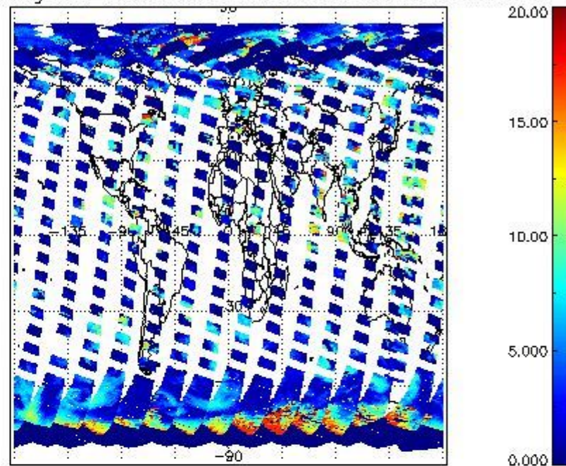
cL_top_height for 07SEP2011 00:00:00 to 08SEP2011 00:00:00
