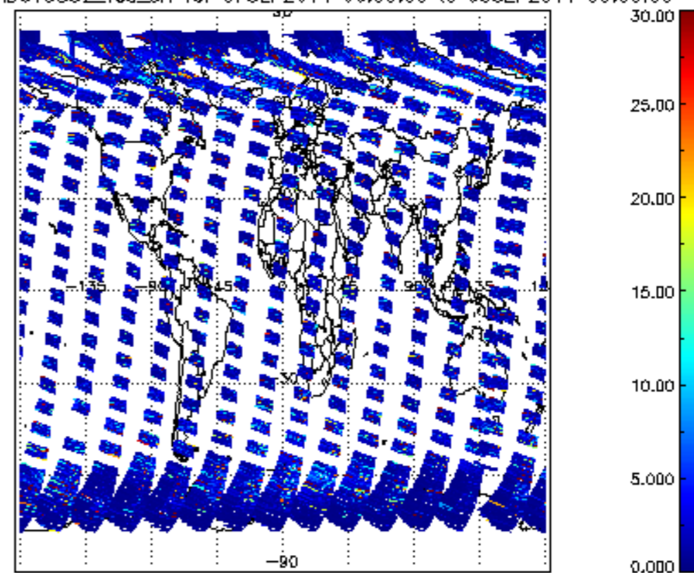
SCIOL2P_NADUV5S02_vcd_err for 07SEP2011 00:00:00 to 08SEP2011 00:00:00
