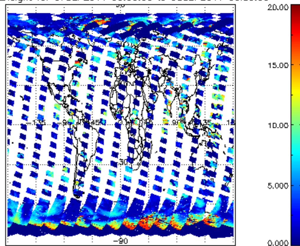
cL_top_height for 07SEP2011 00:00:00 to 08SEP2011 00:00:00
