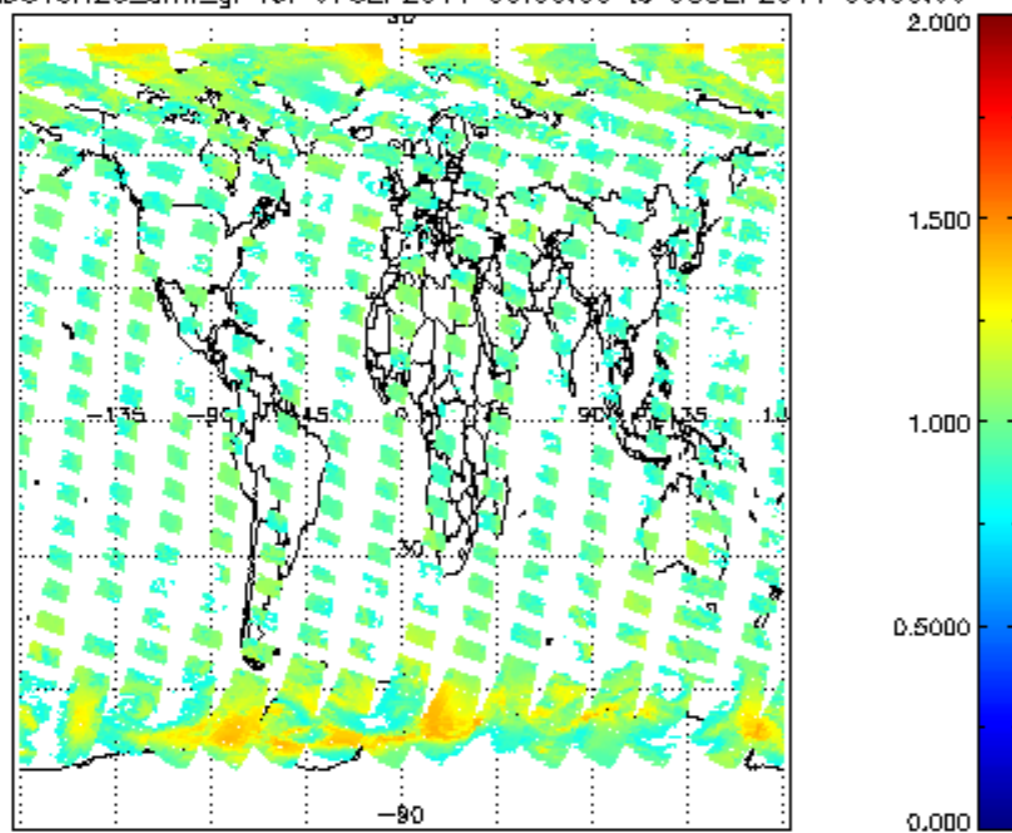
SCIOL2P_NADUV8H20_amf_gr for 07SEP2011 00:00:00 to 08SEP2011 00:00:00
