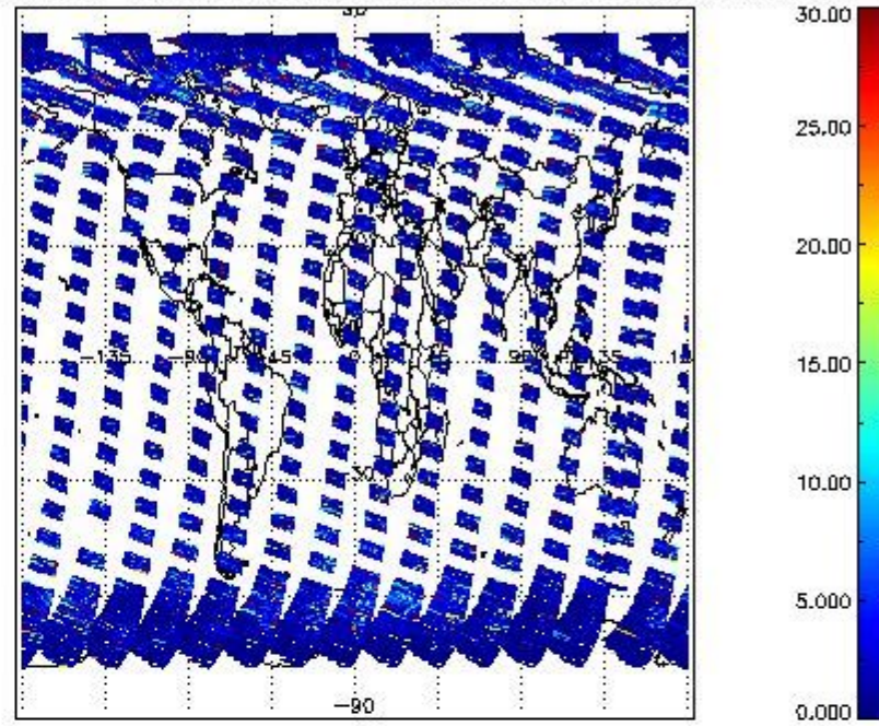
SCIOL2P_NADUV5S02_vcd_err for 07SEP2011 00:00:00 to 08SEP2011 00:00:00
