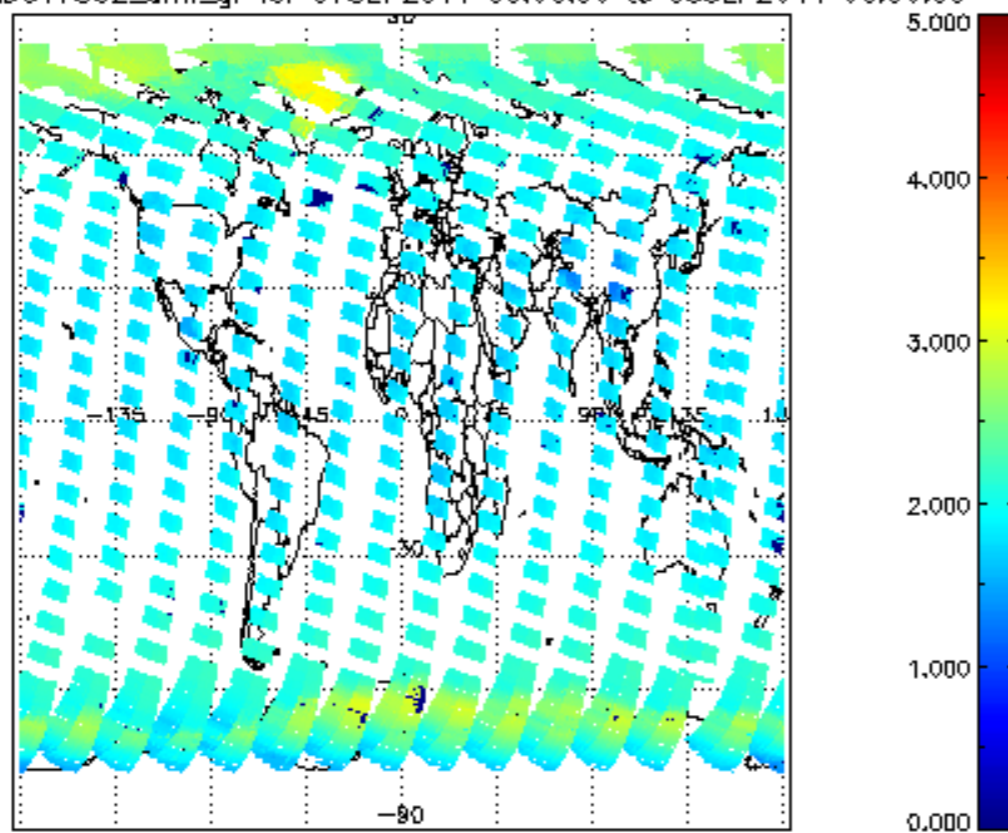
SCIOL2P_NADUV7S02_amf_gr for 07SEP2011 00:00:00 to 08SEP2011 00:00:00
