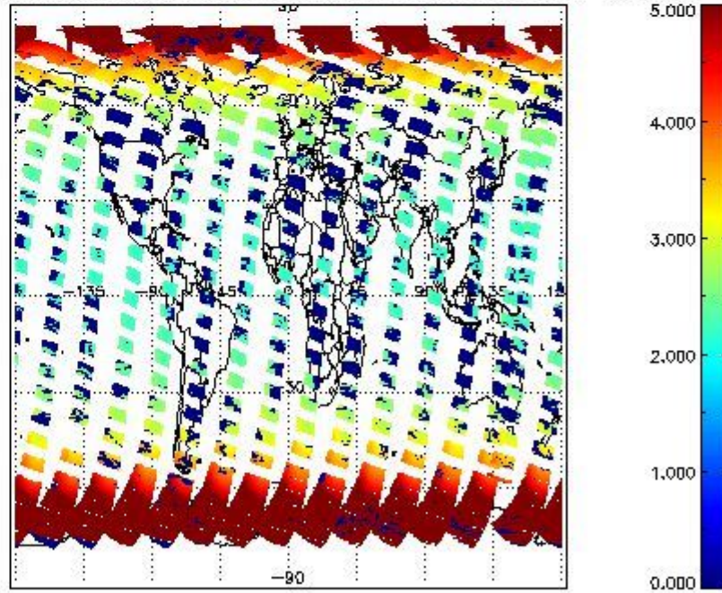
SCIOL2P_NADUV1N02_amf_cl for 07SEP2011 00:00:00 to 08SEP2011 00:00:00
