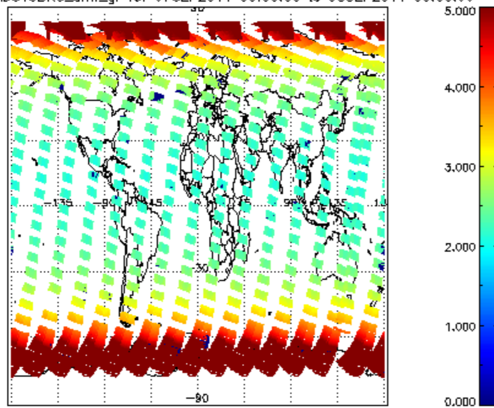
SCIOL2P_NADUV3BRO_amf_gr for 07SEP2011 00:00:00 to 08SEP2011 00:00:00
