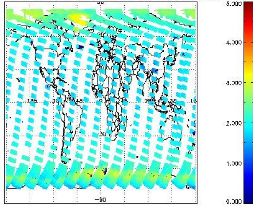
SCIOL2P_NADUV7S02_amf_gr for 07SEP2011 00:00:00 to 08SEP2011 00:00:00
