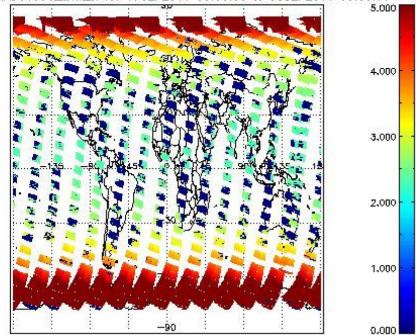
SCIOL2P_NADUV003_amf_cl for 07SEP2011 00:00:00 to 08SEP2011 00:00:00
