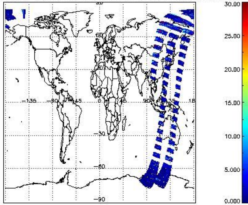
SCIOL2P_NADUV7S02_vcd_err for 07SEP2011 00:00:00 to 08SEP2011 00:00:00
