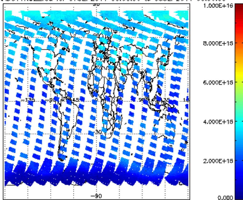
SCIOL2P_NADUV1NO2_vcd for 07SEP2011 00:00:00 to 08SEP2011 00:00:00
