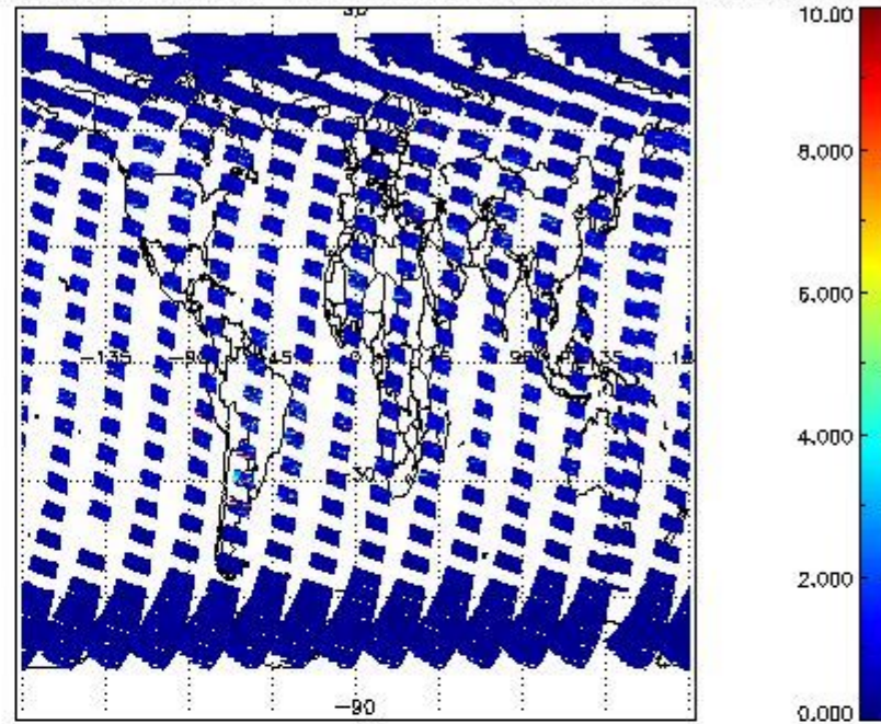
SCIOL2P_NADUV3BRO_vcd_err for 07SEP2011 00:00:00 to 06SEP2011 00:00:00
