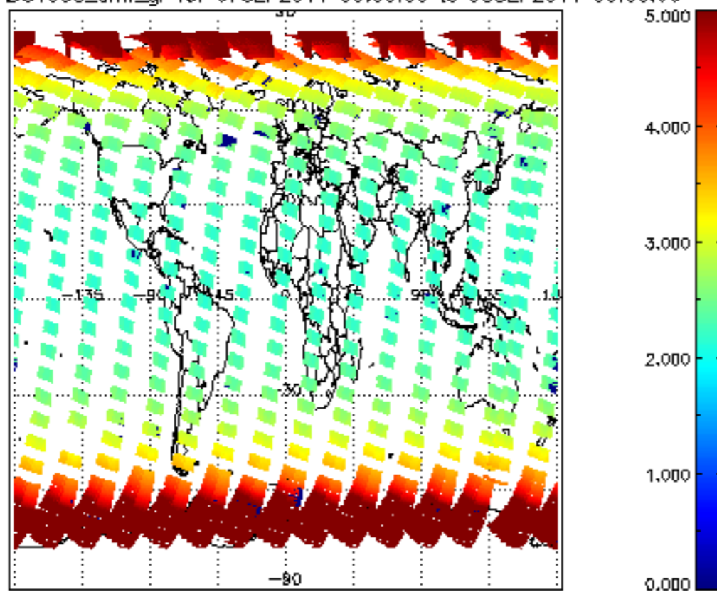
SCIOL2P_NADUV003_amf_gr for 07SEP2011 00:00:00 to 08SEP2011 00:00:00
