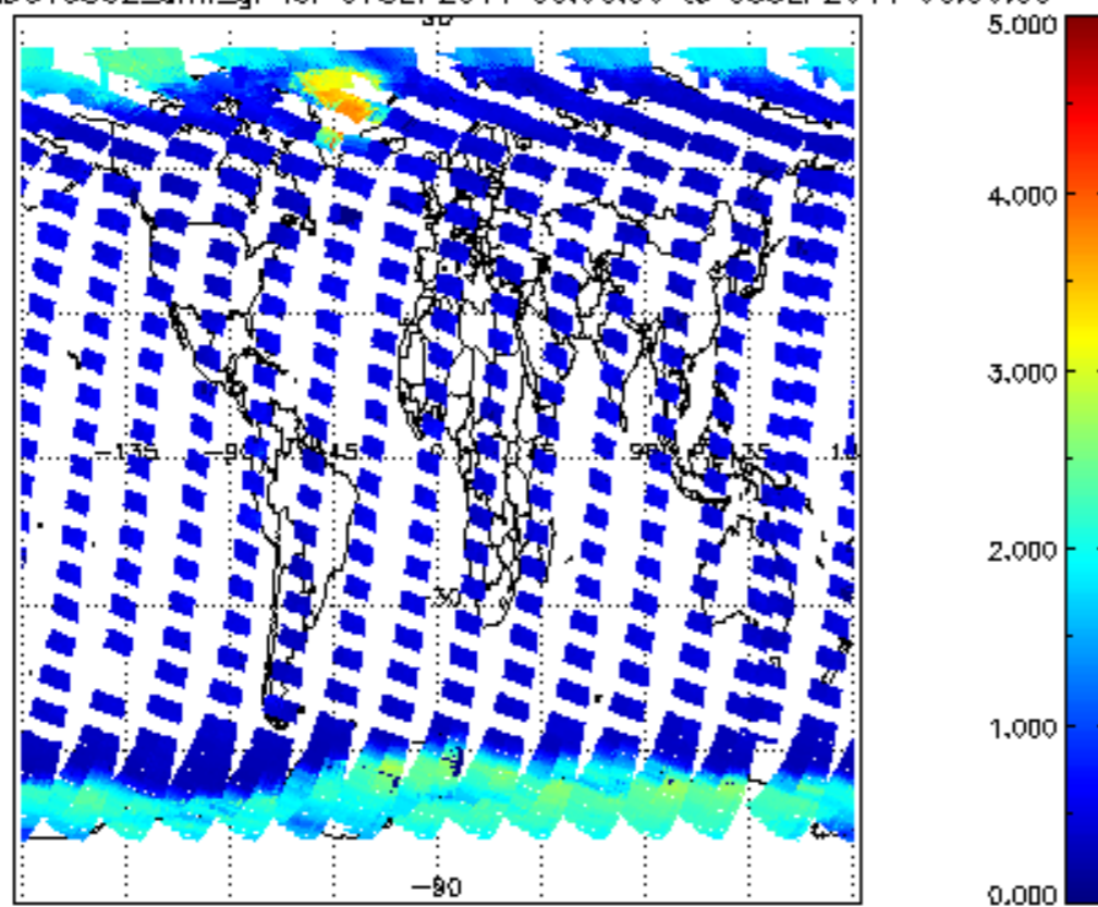
SCIOL2P_NADUV5S02_amf_gr for 07SEP2011 00:00:00 to 08SEP2011 00:00:00
