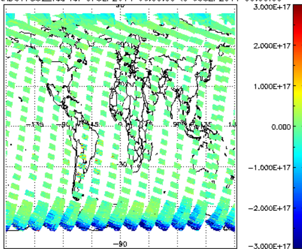
SCIOL2P_NADUV7S02_vcd for 07SEP2011 00:00:00 to 08SEP2011 00:00:00
