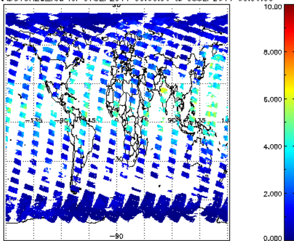
SCIOL2P_NADUV8H20_vcd for 07SEP2011 00:00:00 to 08SEP2011 00:00:00
