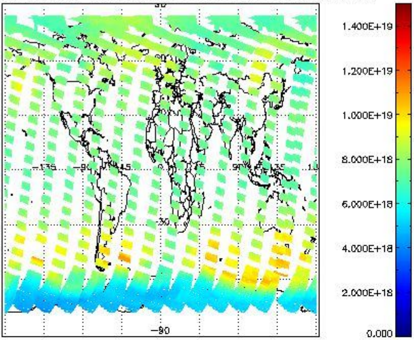
SCIOL2P_NADUV003_vcd for 07SEP2011 00:00:00 to 08SEP2011 00:00:00
