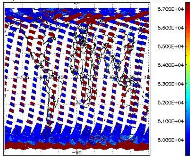
cloud_flags for 07SEP2011 00:00:00 to 08SEP2011 00:00:00
