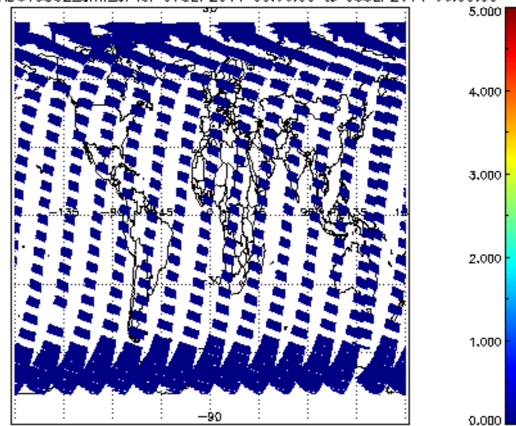
SCIOL2P_NADUV5S02_amf_cl for 07SEP2011 00:00:00 to 08SEP2011 00:00:00
