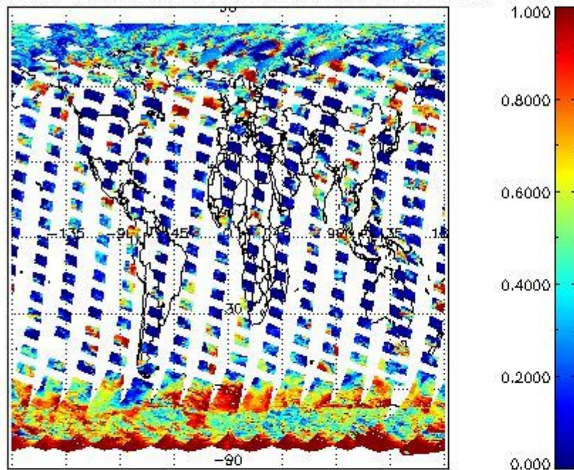
cL_frac for 07SEP2011 00:00:00 to 08SEP2011 00:00:00
