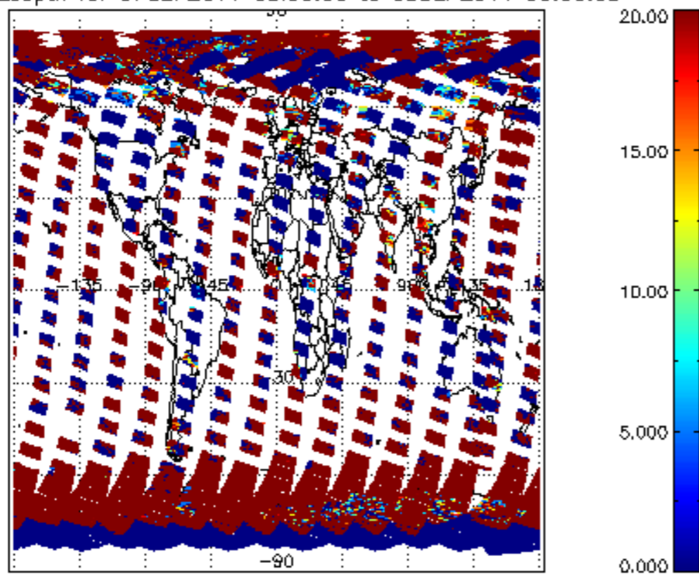
cL_opt_depth for 07SEP2011 00:00:00 to 08SEP2011 00:00:00
