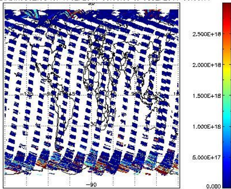
SCIDL2P_NADIR3CO_vcd for 07SEP2011 00:00:00 to 08SEP2011 00:00:00
