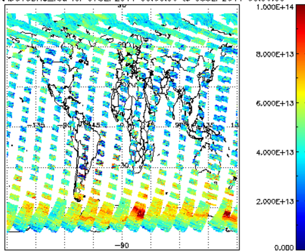
SCIOL2P_NADUV3BRO_vcd for 07SEP2011 00:00:00 to 08SEP2011 00:00:00
