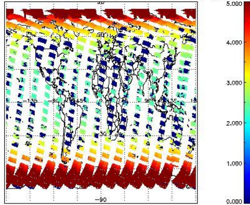
SCIOL2P_NADUV3BRO_amf_cl for 07SEP2011 00:00:00 to 08SEP2011 00:00:00
