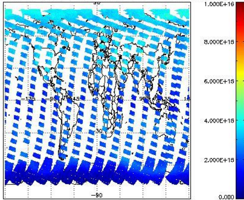
SCIOL2P_NADUV1N02_vcd for 07SEP2011 00:00:00 to 08SEP2011 00:00:00
