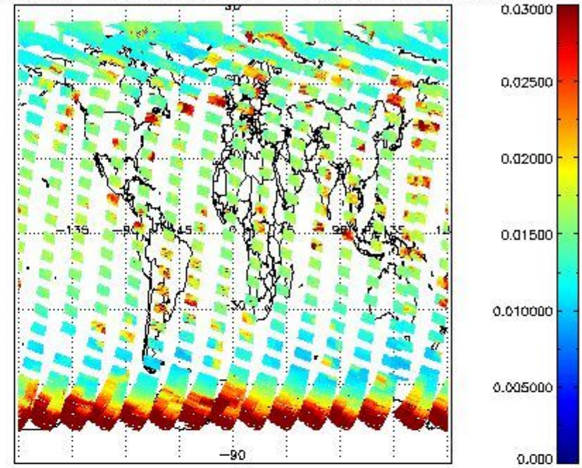
SCIOL2P_NADUV003_vcd_err for 07SEP2011 00:00:00 to 08SEP2011 00:00:00
