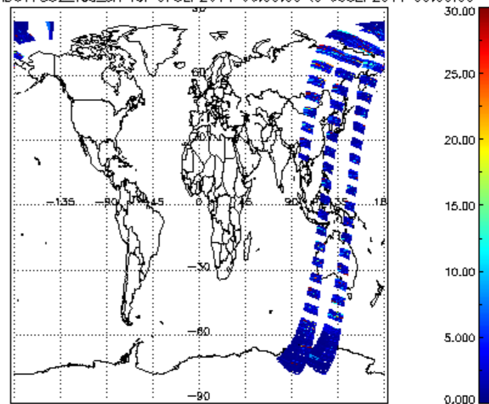
SCIOL2P_NADUV7S02_vcd_err for 07SEP2011 00:00:00 to 08SEP2011 00:00:00
