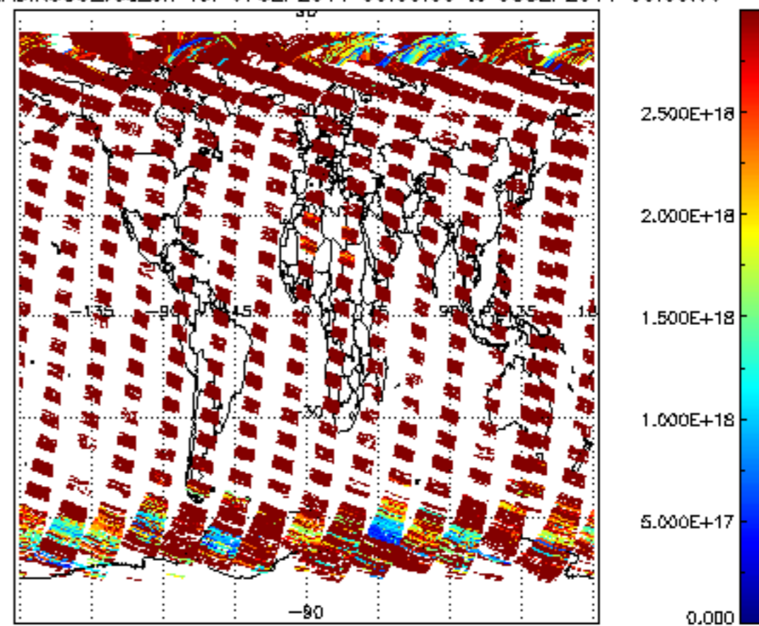
SCIOL2P_NADIR3CO_vcd_err for 07SEP2011 00:00:00 to 08SEP2011 00:00:00
