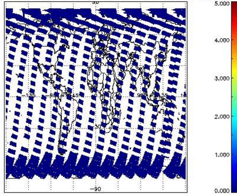
SCIOL2P_NADUV5S02_amf_cl for 07SEP2011 00:00:00 to 08SEP2011 00:00:00
