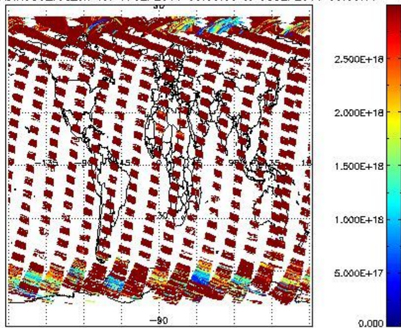
SCIDL2P_NADIR3CO_vcd_err for 07SEP2011 00:00:00 to 08SEP2011 00:00:00
