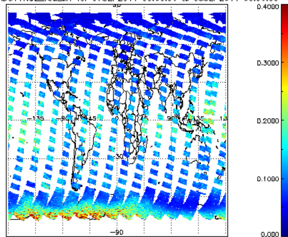
SCIOL2P_NADUV1NO2_vcd_err for 07SEP2011 00:00:00 to 08SEP2011 00:00:00
