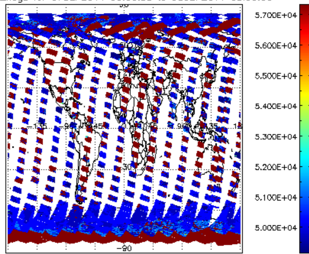
cloud_flags for 07SEP2011 00:00:00 to 08SEP2011 00:00:00
