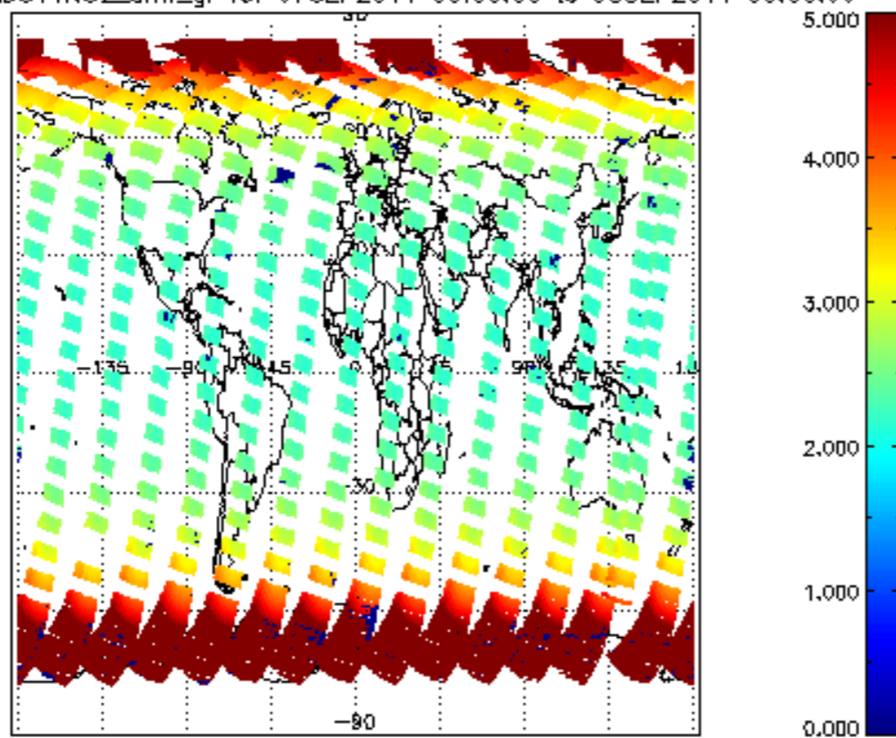
SCIOL2P_NADUV1NO2_amf_gr for 07SEP2011 00:00:00 to 08SEP2011 00:00:00
