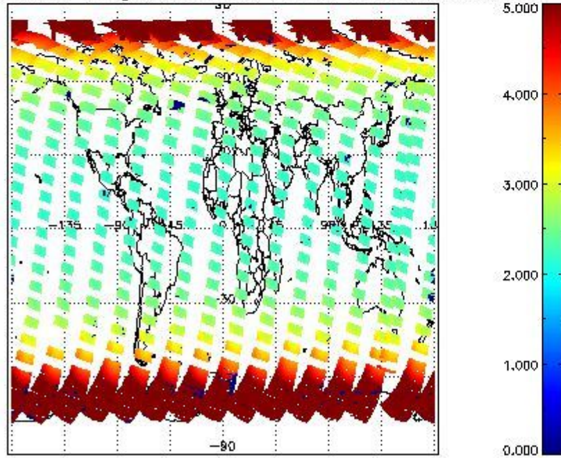
SCIOL2P_NADUV1N02_amf_gr for 07SEP2011 00:00:00 to 08SEP2011 00:00:00
