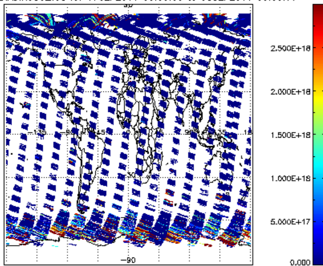
SCIOL2P_NADIR3CO_vcd for 07SEP2011 00:00:00 to 08SEP2011 00:00:00
