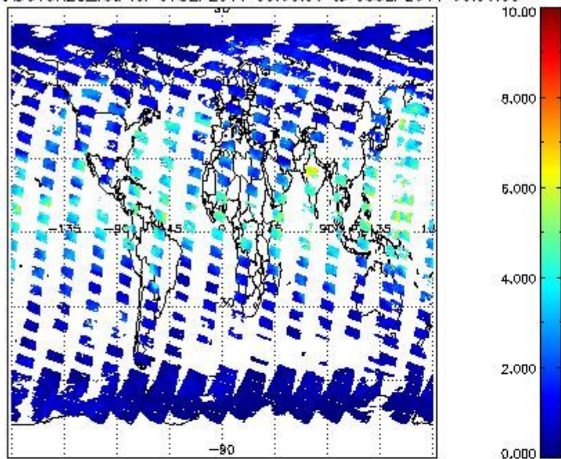
SCIOL2P_NADUV8H2O_vcd for 07SEP2011 00:00:00 to 08SEP2011 00:00:00
