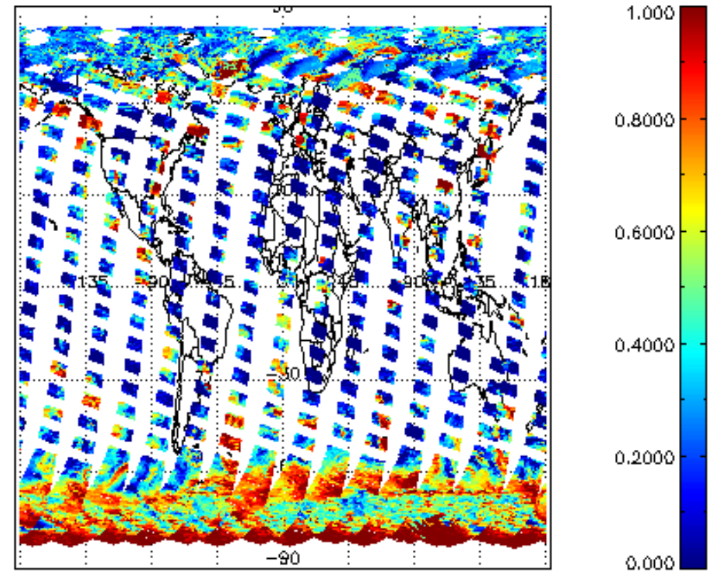
cl_frac for 05SEP2011 00:00:00 to 06SEP2011 00:00:00
