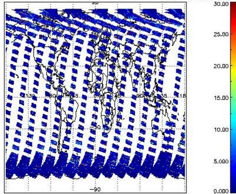
SCIOL2P_NADUV5S02_vcd_err for 05SEP2011 00:00:00 to 06SEP2011 00:00:00
