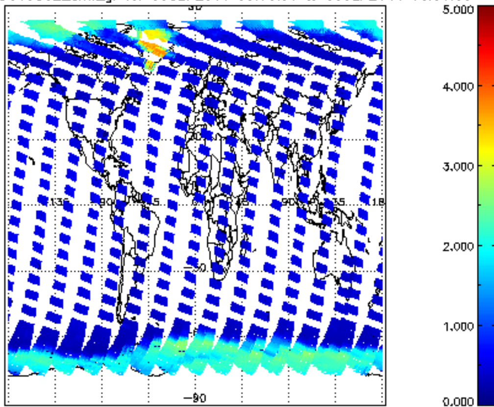
SCIOL2P_NADUV5S02_amf_gr for 05SEP2011 00:00:00 to 06SEP2011 00:00:00
