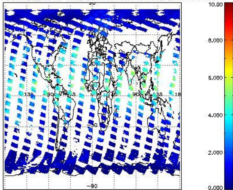
SCIOL2P_NADUV8H2O_vcd for 05SEP2011 00:00:00 to 06SEP2011 00:00:00
