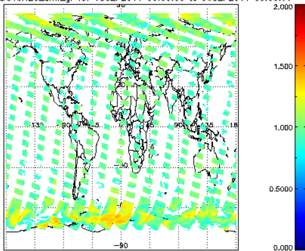
SCIOL2P_NADUV8H20_amf_gr for 05SEP2011 00:00:00 to 06SEP2011 00:00:00
