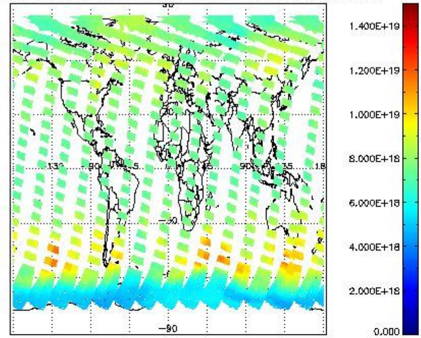
SCIOL2P_NADUV003_vcd for 05SEP2011 00:00:00 to 06SEP2011 00:00:00
