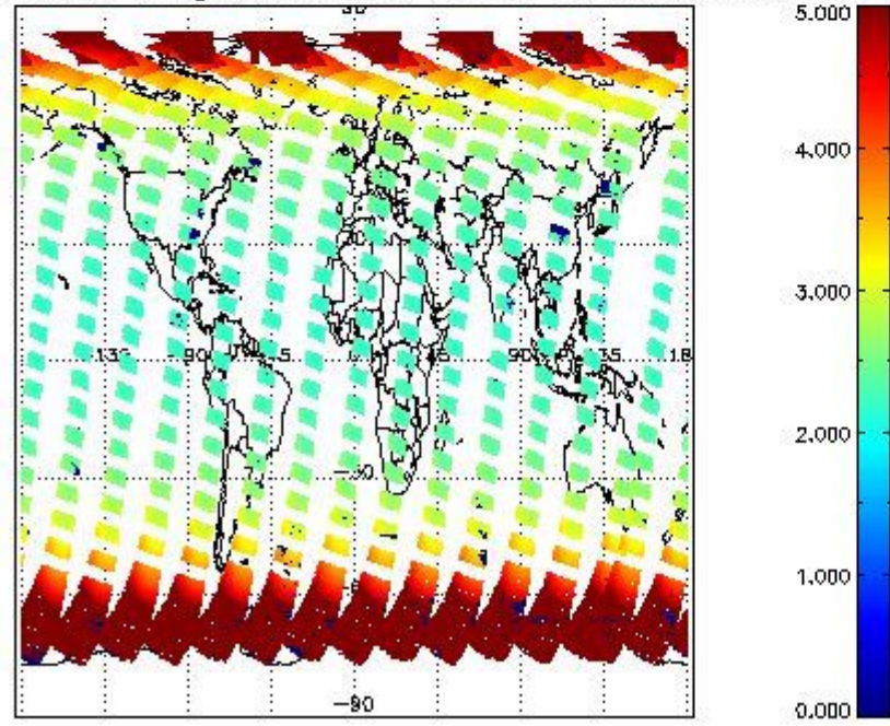
SCIOL2P_NADUV1NO2_amf_gr for 05SEP2011 00:00:00 to 06SEP2011 00:00:00
