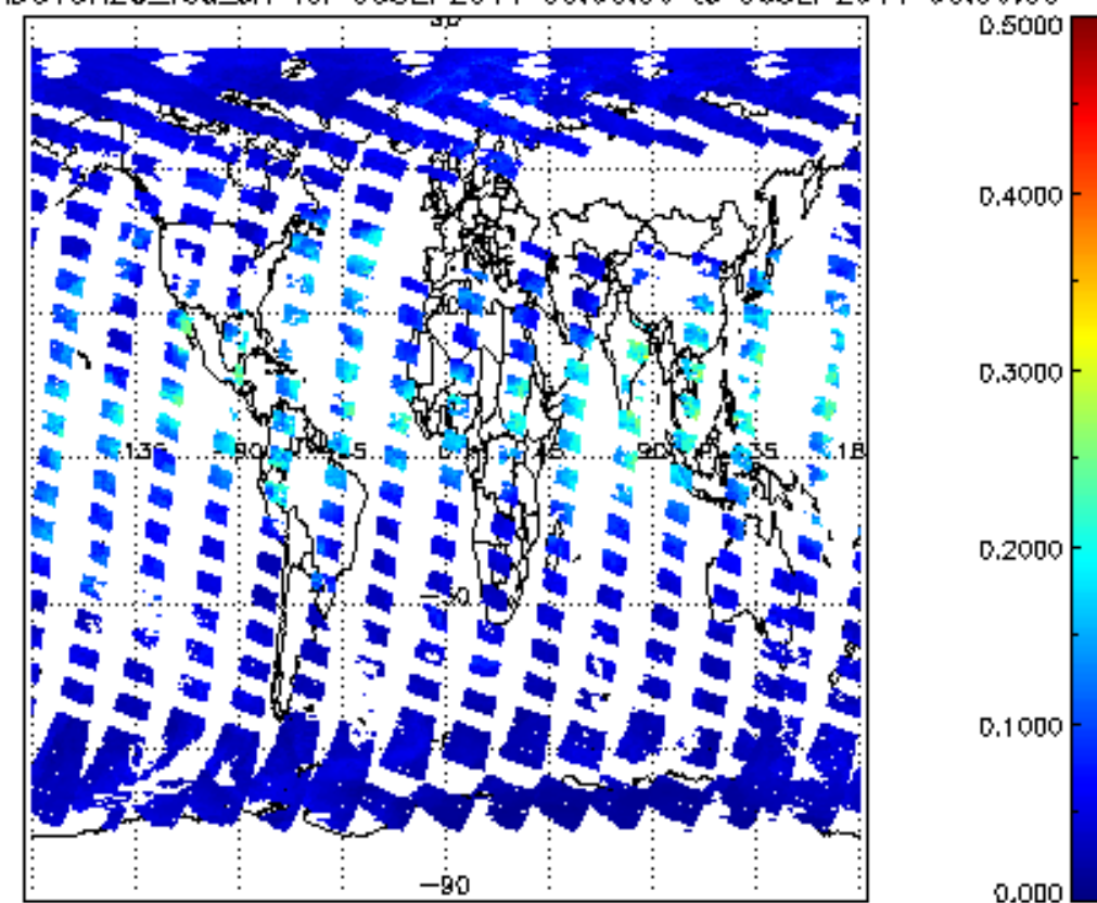
SCIOL2P_NADUV8H20_vcd_err for 05SEP2011 00:00:00 to 06SEP2011 00:00:00
