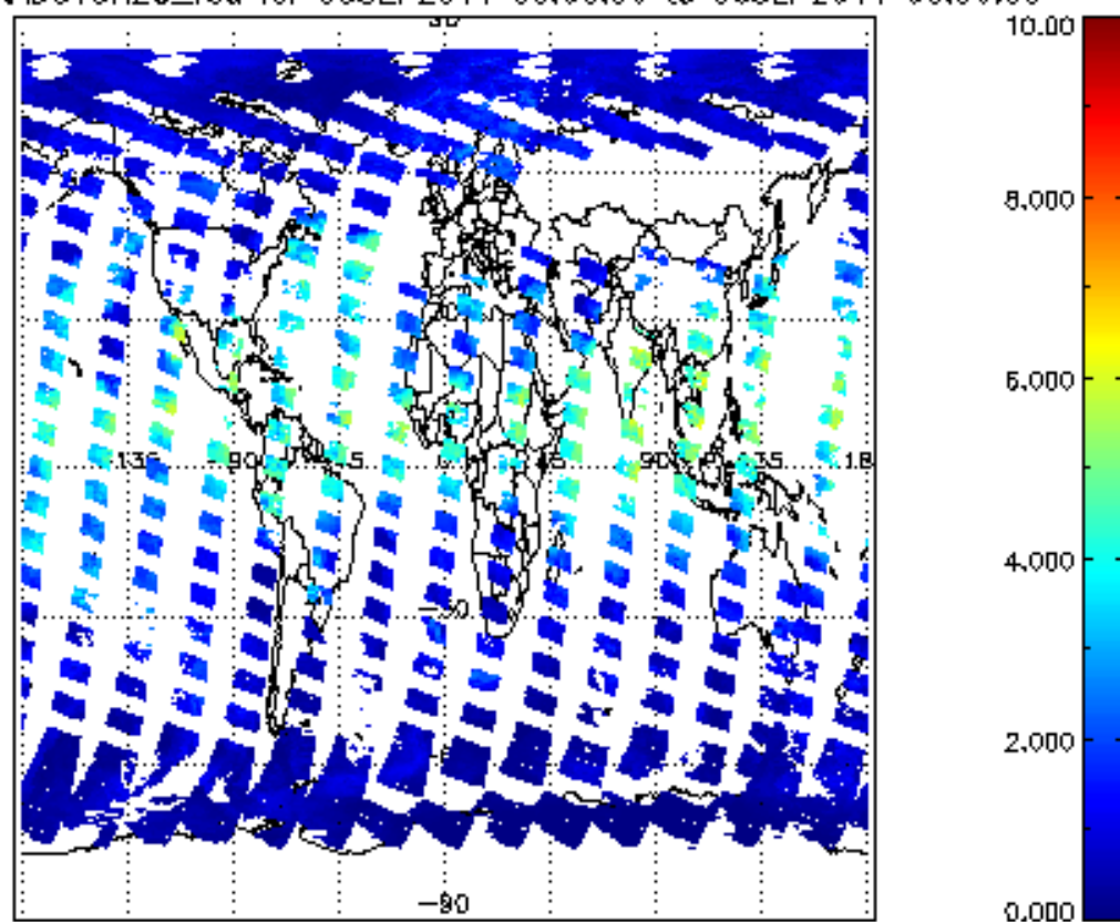
SCIOL2P_NADUV8H20_vcd for 05SEP2011 00:00:00 to 06SEP2011 00:00:00
