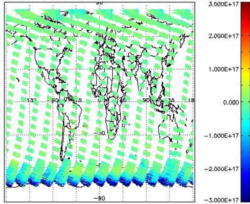
SCIOL2P_NADUV7S02_vcd for 05SEP2011 00:00:00 to 06SEP2011 00:00:00
