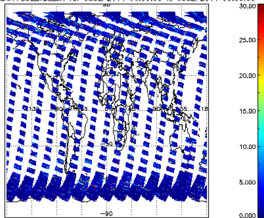
SCIOL2P_NADUV7S02_vcd_err for 05SEP2011 00:00:00 to 06SEP2011 00:00:00
