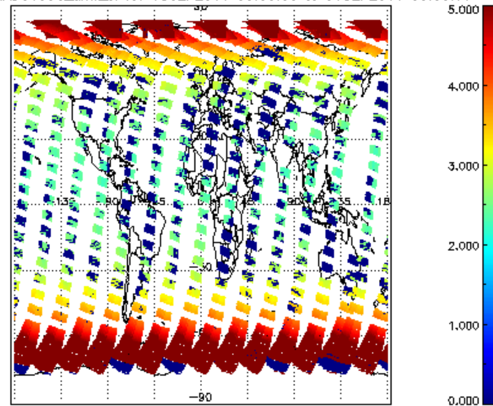
SCIOL2P_NADUV003_amf_cl for 05SEP2011 00:00:00 to 06SEP2011 00:00:00
