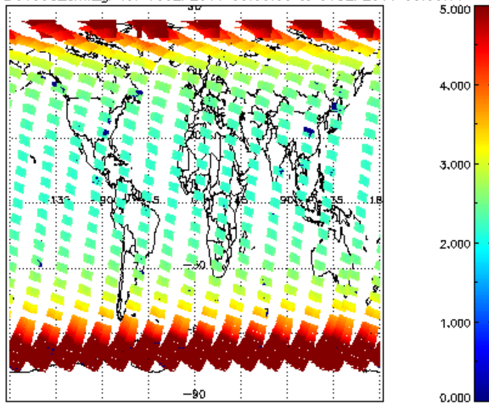
SCIOL2P_NADUV003_amf_gr for 05SEP2011 00:00:00 to 06SEP2011 00:00:00
