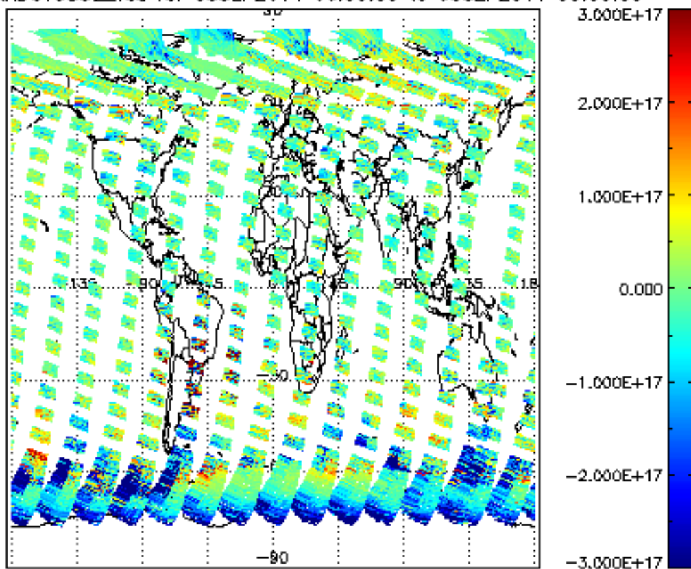
SCIOL2P_NADUV5S02_vcd for 05SEP2011 00:00:00 to 06SEP2011 00:00:00
