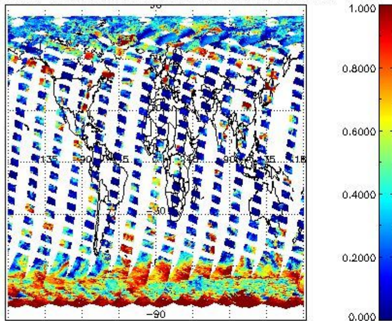
cLfrac for 05SEP2011 00:00:00 to 06SEP2011 00:00:00
