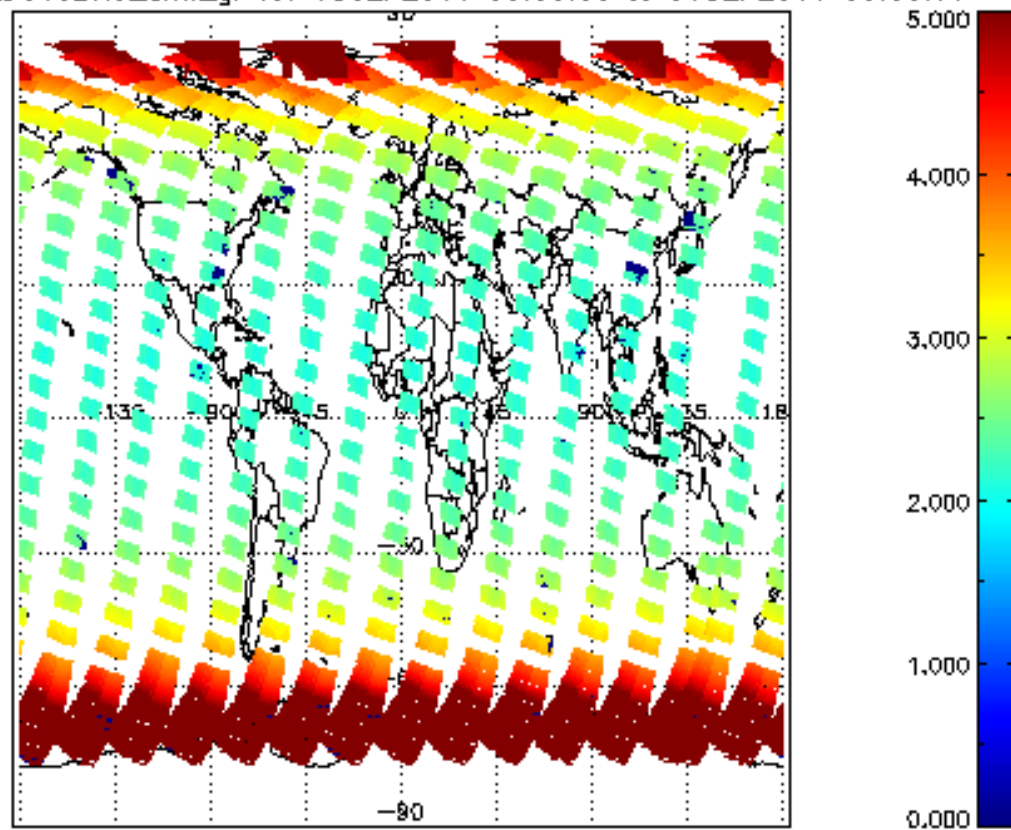
SCIOL2P_NADUV3BRO_amf_gr for 05SEP2011 00:00:00 to 06SEP2011 00:00:00
