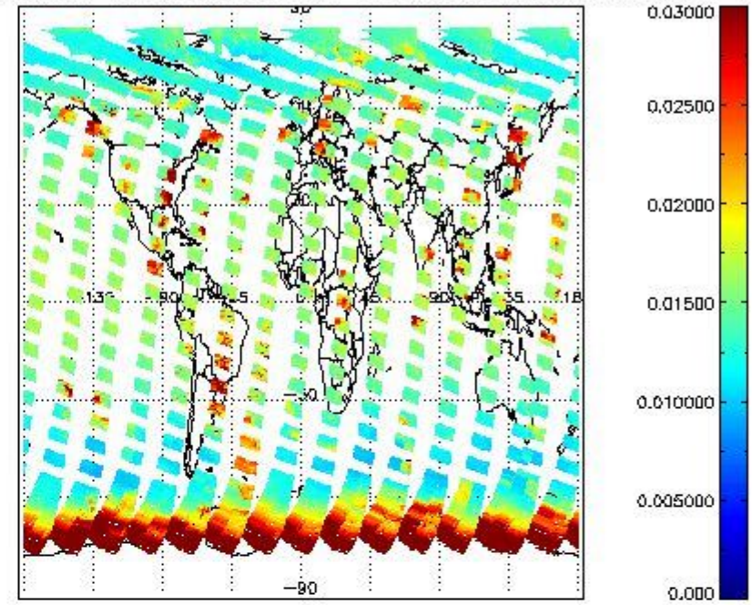
SCIOL2P_NADUV003_vcd_err for 05SEP2011 00:00:00 to 06SEP2011 00:00:00
