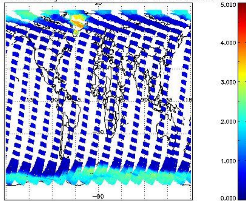
SCIOL2P_NADUV5S02_amf_gr for 05SEP2011 00:00:00 to 06SEP2011 00:00:00
