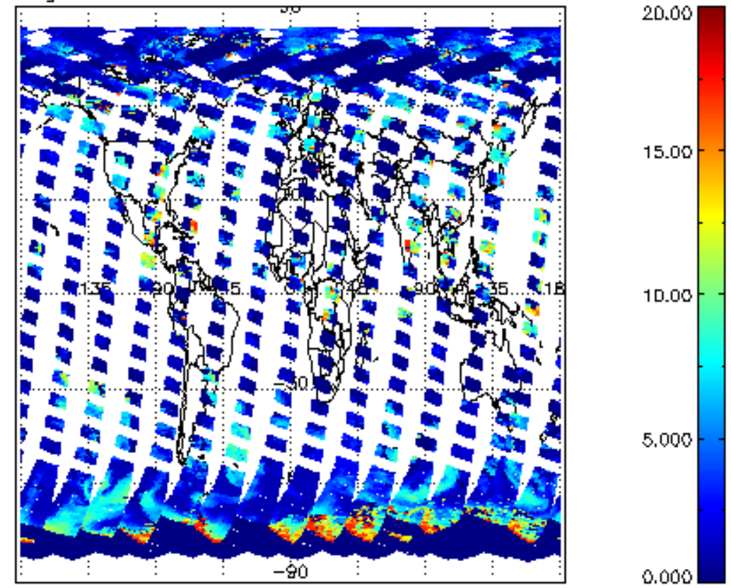
cl_top_height for 05SEP2011 00:00:00 to 06SEP2011 00:00:00
