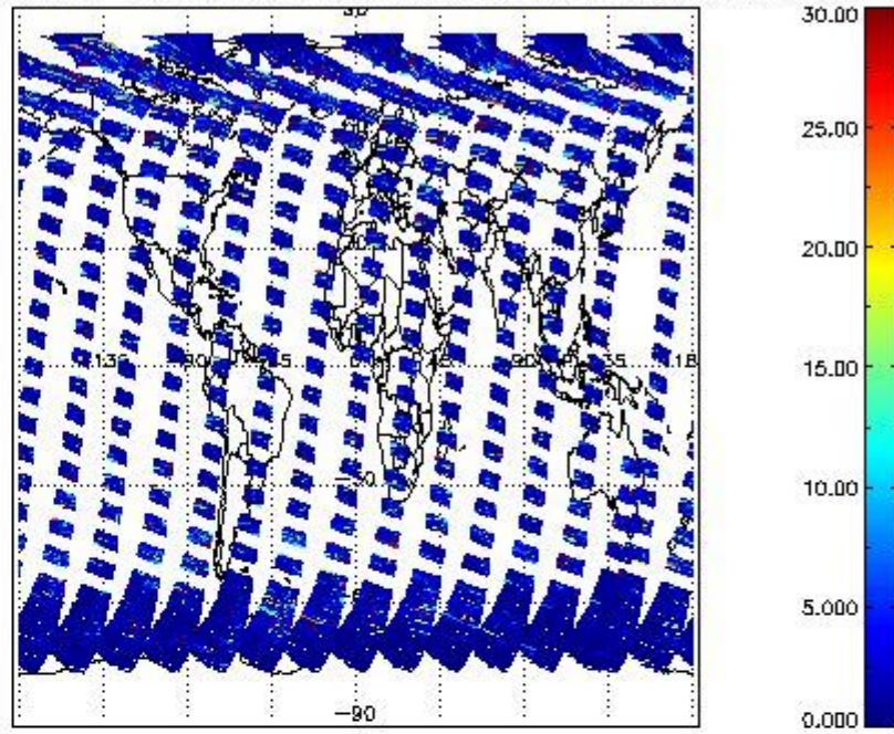
SCIOL2P_NADUV7S02_vcd_err for 05SEP2011 00:00:00 to 06SEP2011 00:00:00
