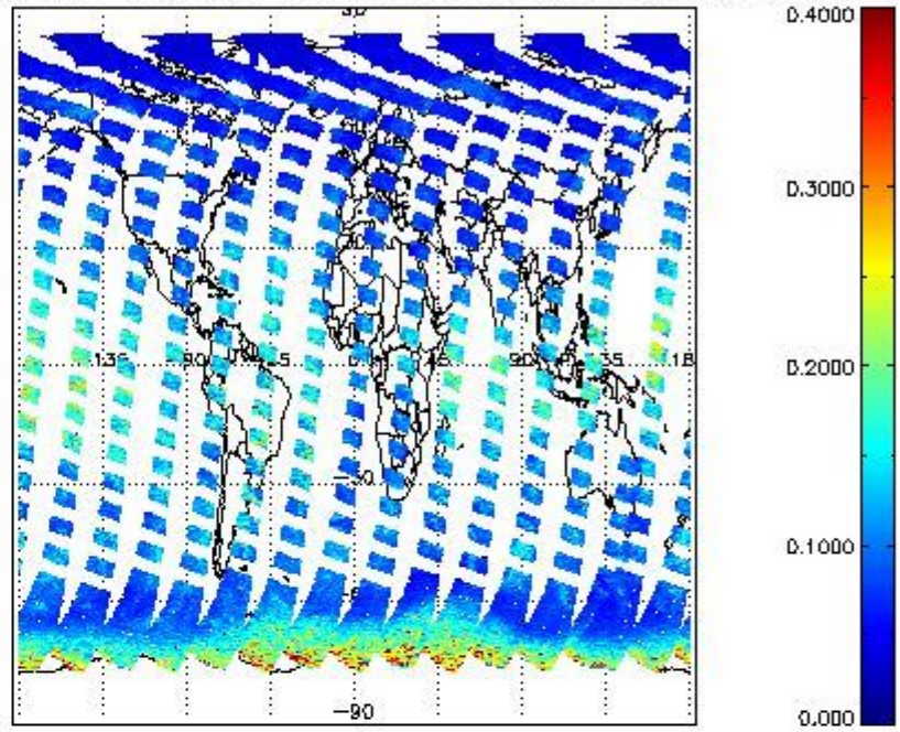
SCIOL2P_NADUV1NO2_vcd_err for 05SEP2011 00:00:00 to 06SEP2011 00:00:00
