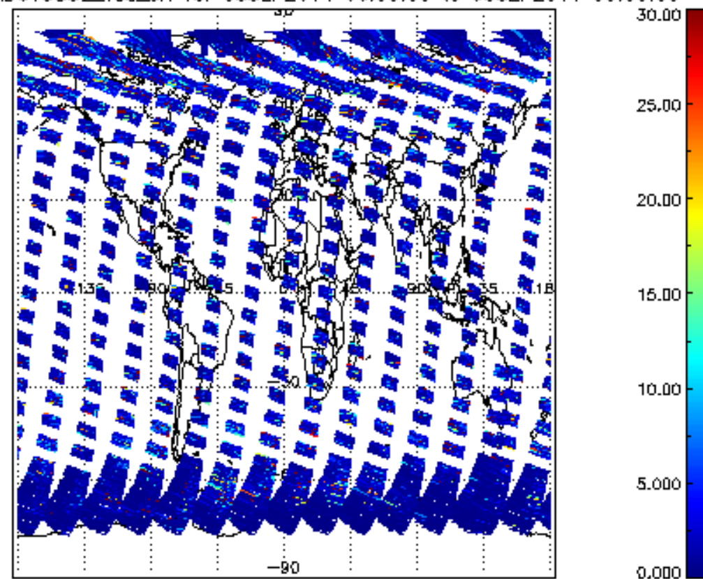
SCIOL2P_NADUV5S02_vcd_err for 05SEP2011 00:00:00 to 06SEP2011 00:00:00
