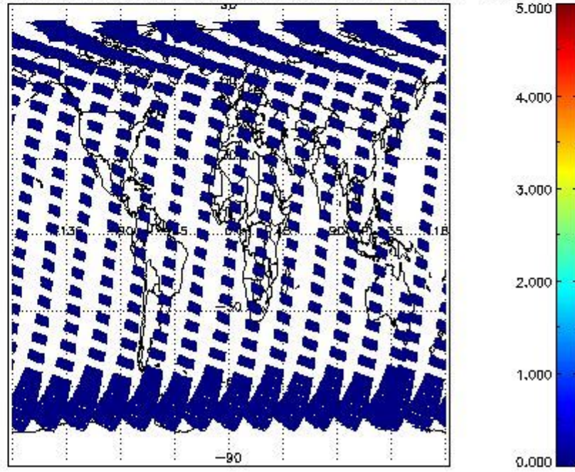
SCIOL2P_NADUV7S02_amf_cl for 05SEP2011 00:00:00 to 06SEP2011 00:00:00
