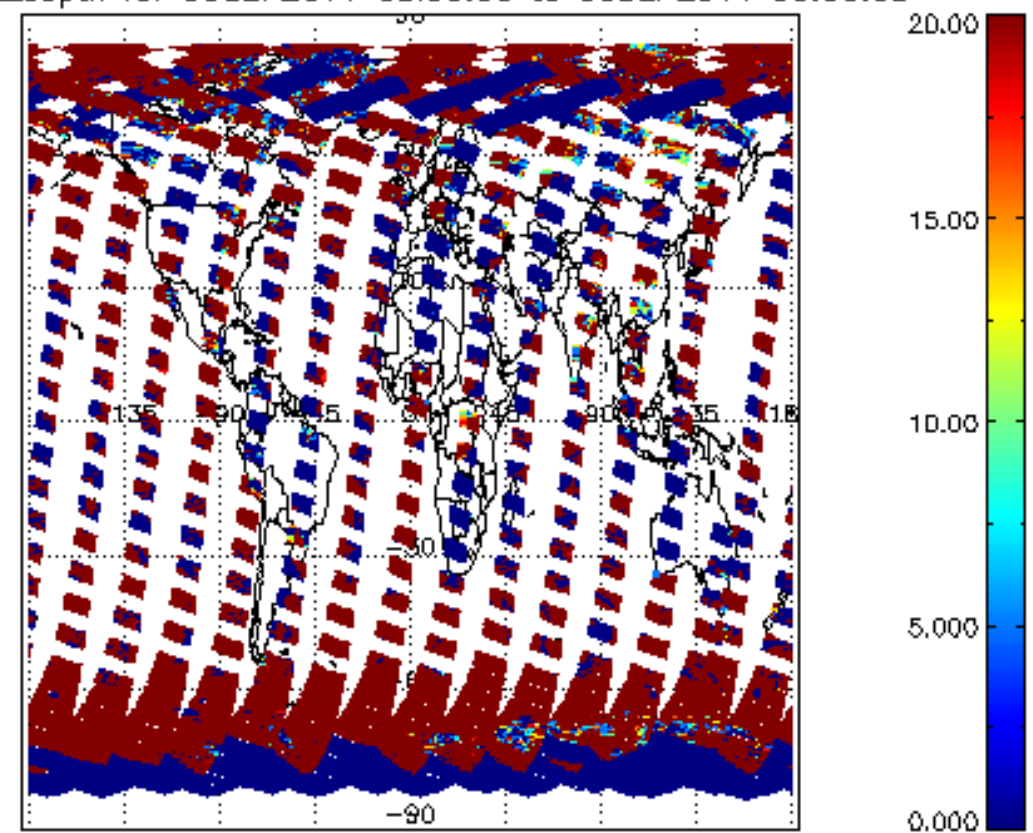
cl_opt_depth for 05SEP2011 00:00:00 to 06SEP2011 00:00:00
