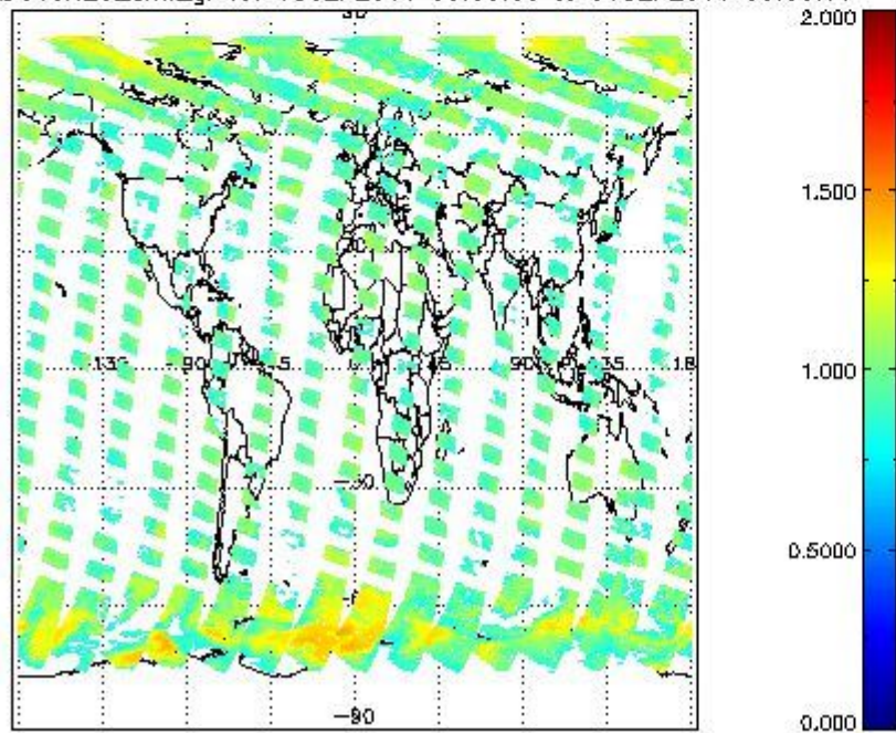
SCIOL2P_NADUV8H2O_arnf_gr for 05SEP2011 00:00:00 to 06SEP2011 00:00:00
