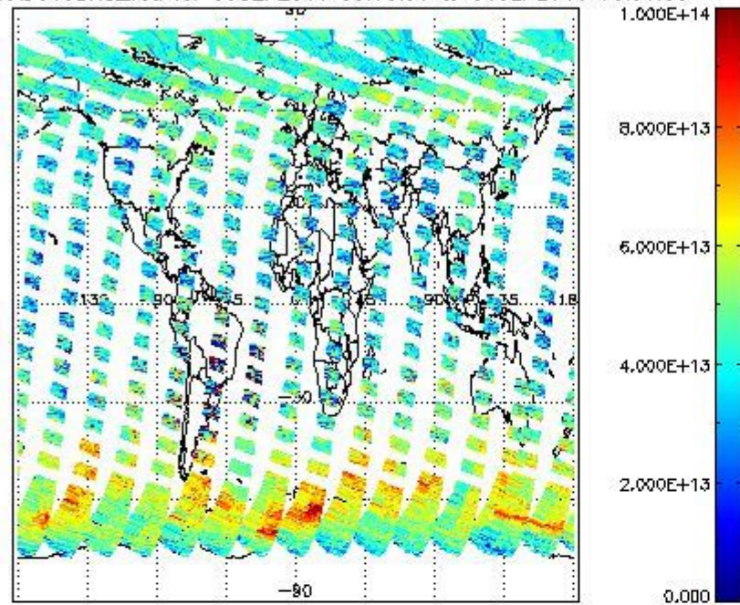
SCIOL2P_NADUV3BRO_vcd for 05SEP2011 00:00:00 to 06SEP2011 00:00:00
