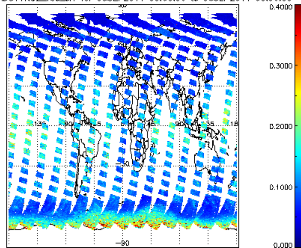
SCIOL2P_NADUV1NO2_vcd_err for 05SEP2011 00:00:00 to 06SEP2011 00:00:00
