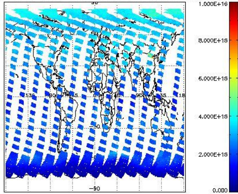
SCIOL2P_NADUV1NO2_vcd for 05SEP2011 00:00:00 to 06SEP2011 00:00:00
