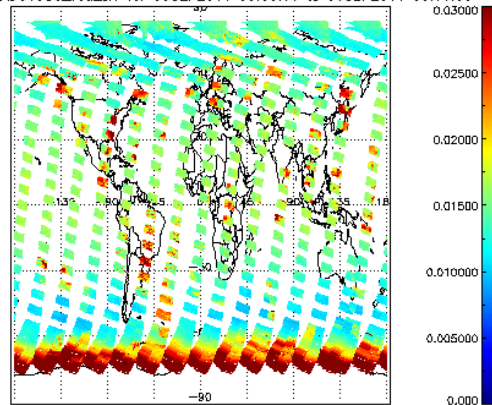
SCIOL2P_NADUV003_vcd_err for 05SEP2011 00:00:00 to 06SEP2011 00:00:00
