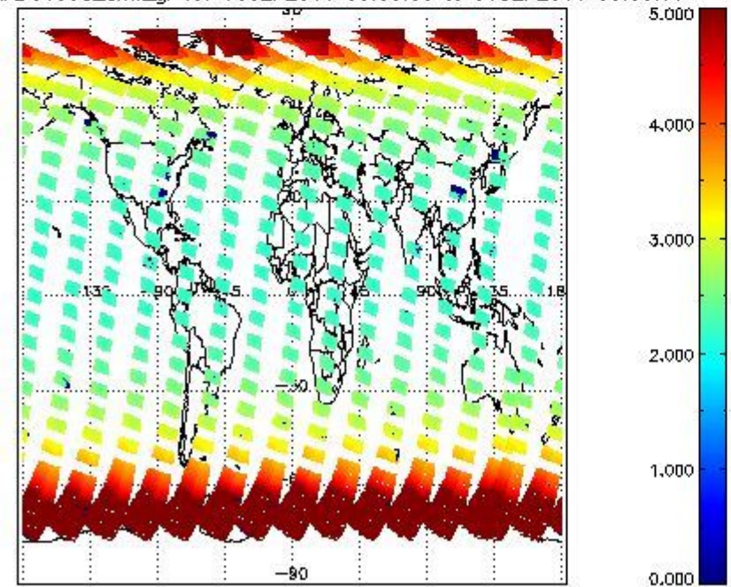
SCIOL2P_NADUV003_amf_gr for 05SEP2011 00:00:00 to 06SEP2011 00:00:00
