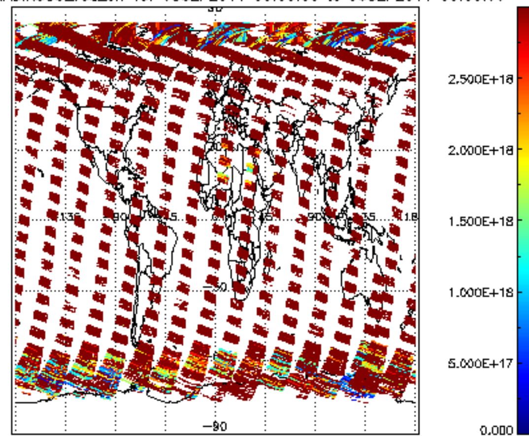
SCIOL2P_NADIR3CO_vcd_err for 05SEP2011 00:00:00 to 06SEP2011 00:00:00
