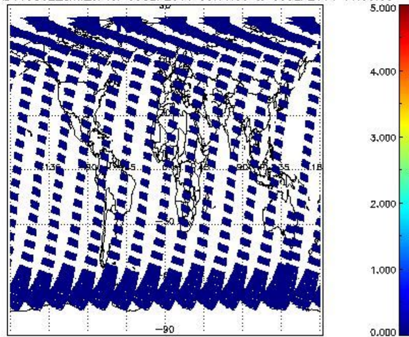
SCIOL2P_NADUV5S02_amf_cl for 05SEP2011 00:00:00 to 06SEP2011 00:00:00
