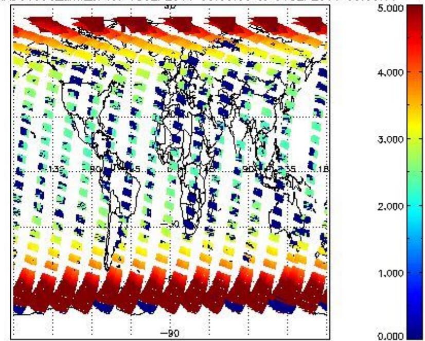
SCIOL2P_NADUV003_amf_cl for 05SEP2011 00:00:00 to 06SEP2011 00:00:00
