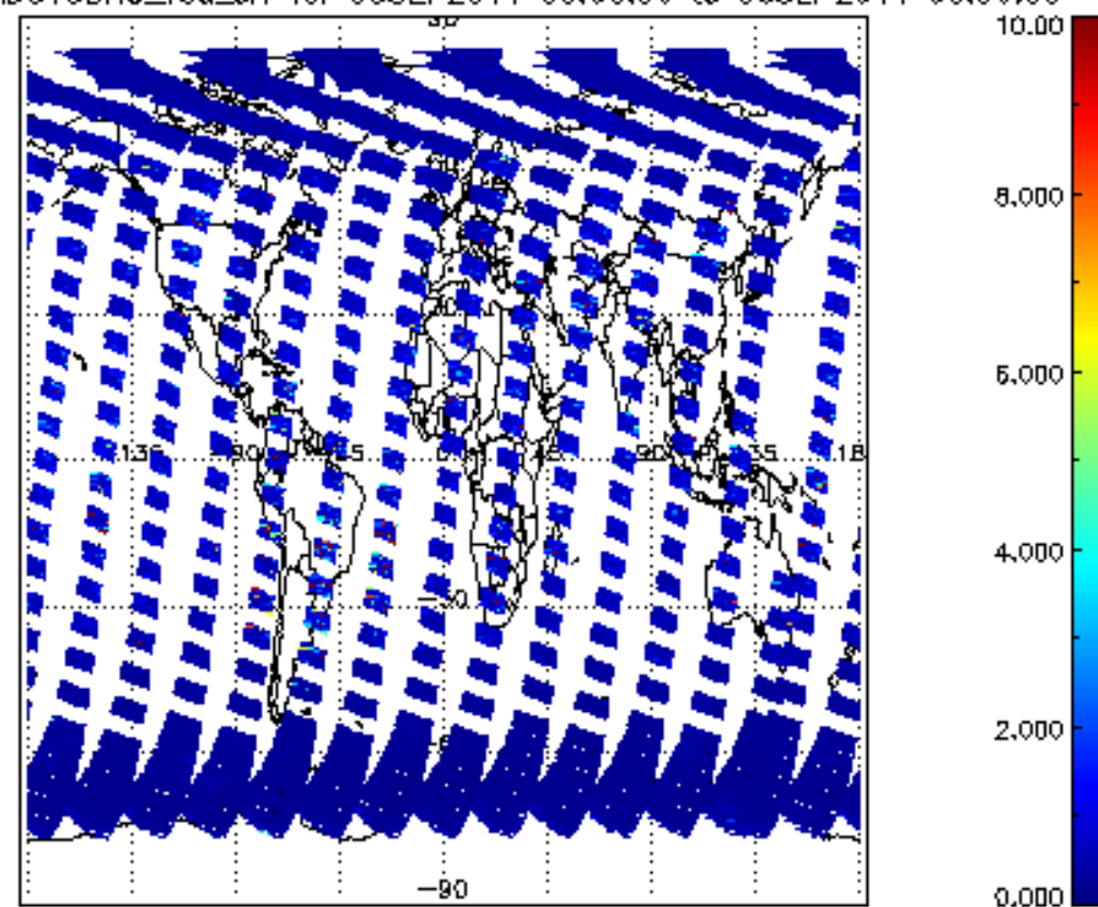
SCIOL2P_NADUV3BRO_vcd_err for 05SEP2011 00:00:00 to 06SEP2011 00:00:00
