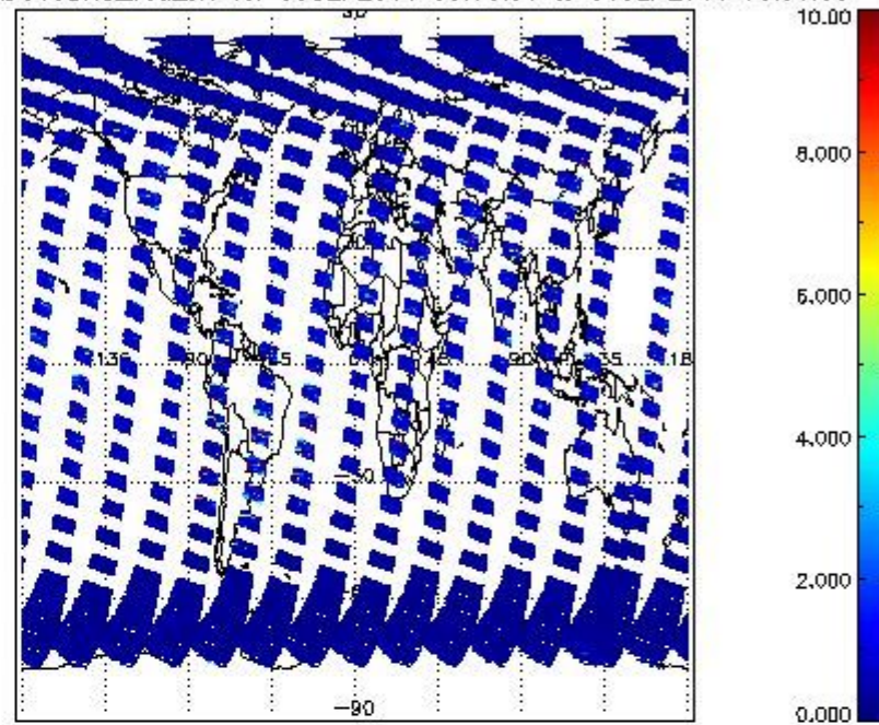
SCIOL2P_NADUV3BRO_vcd_err for 05SEP2011 00:00:00 to 06SEP2011 00:00:00
