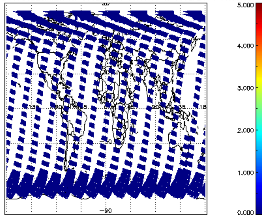
SCIOL2P_NADUV7S02_amf_cl for 05SEP2011 00:00:00 to 06SEP2011 00:00:00
