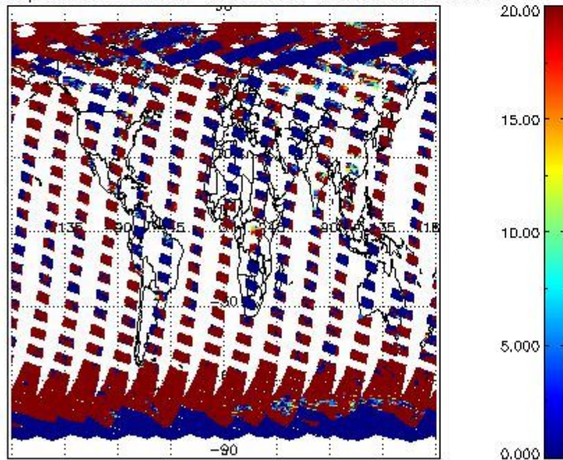
cLopt_depth for 05SEP2011 00:00:00 to 06SEP2011 00:00:00
