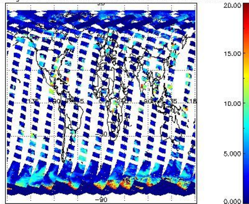
cL_top_height for 05SEP2011 00:00:00 to 06SEP2011 00:00:00
