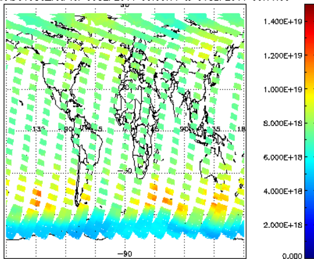
SCIOL2P_NADUV003_vcd for 05SEP2011 00:00:00 to 06SEP2011 00:00:00
