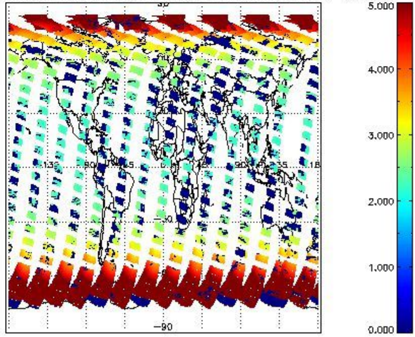
SCIOL2P_NADUV1NO2_amf_cl for 05SEP2011 00:00:00 to 06SEP2011 00:00:00
