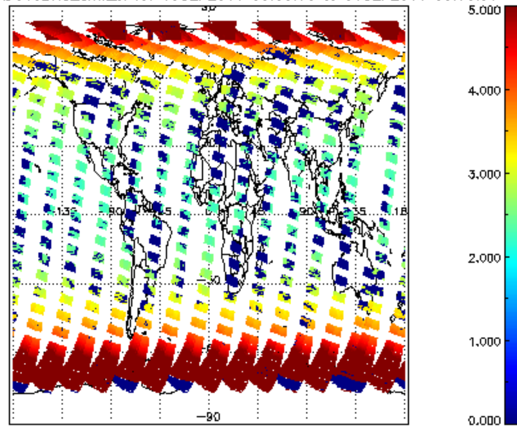
SCIOL2P_NADUV3BRO_amf_cl for 05SEP2011 00:00:00 to 06SEP2011 00:00:00
