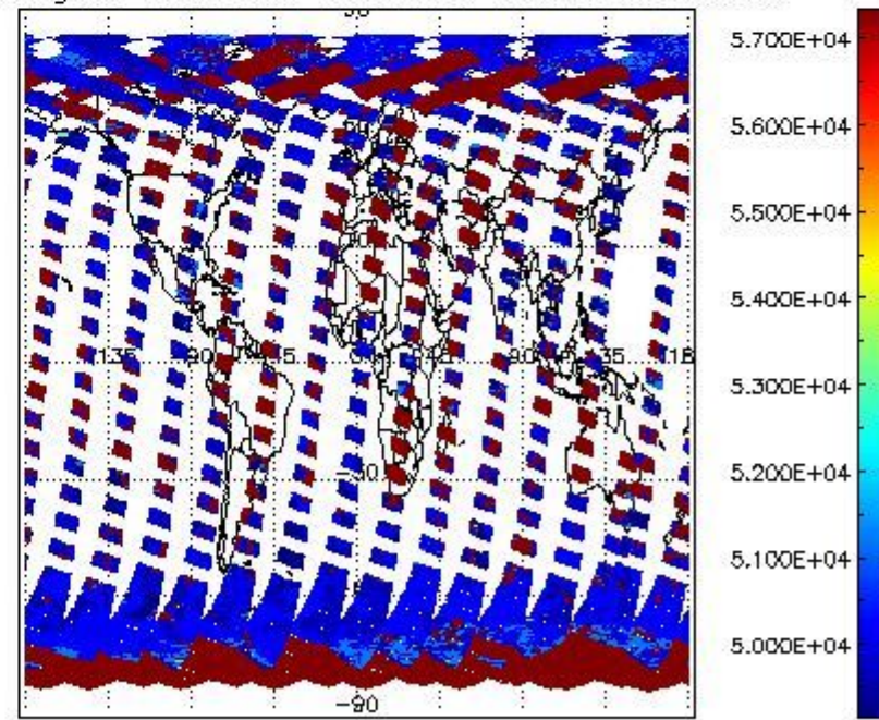
cloud_flags for 05SEP2011 00:00:00 to 06SEP2011 00:00:00
