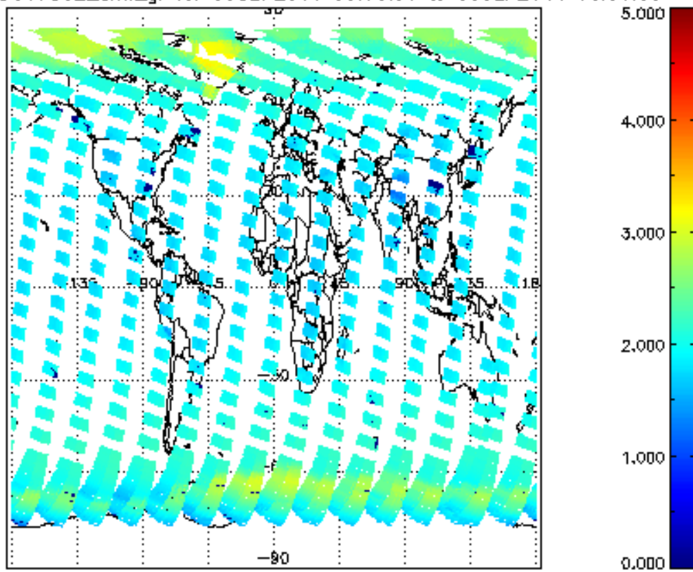
SCIOL2P_NADUV7S02_amf_gr for 05SEP2011 00:00:00 to 06SEP2011 00:00:00
