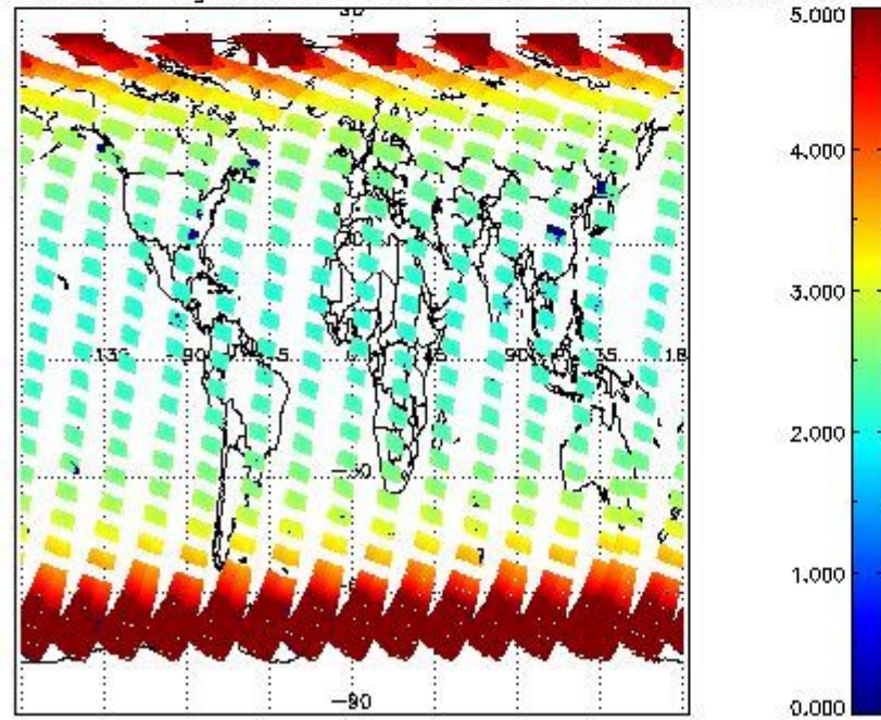
SCIOL2P_NADUV3BRO_amf_gr for 05SEP2011 00:00:00 to 06SEP2011 00:00:00
