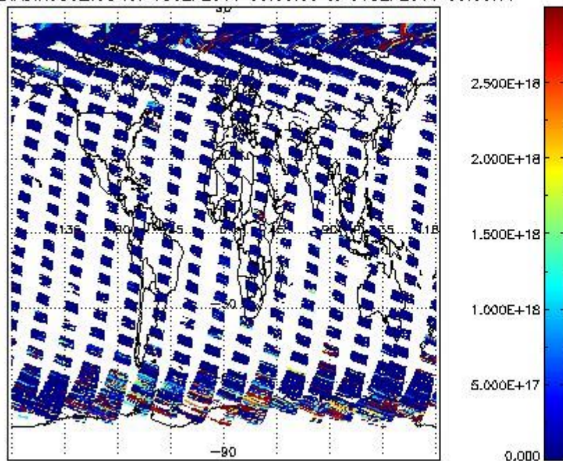
SCIDL2P_NADIR3CO_vcd for 05SEP2011 00:00:00 to 06SEP2011 00:00:00
