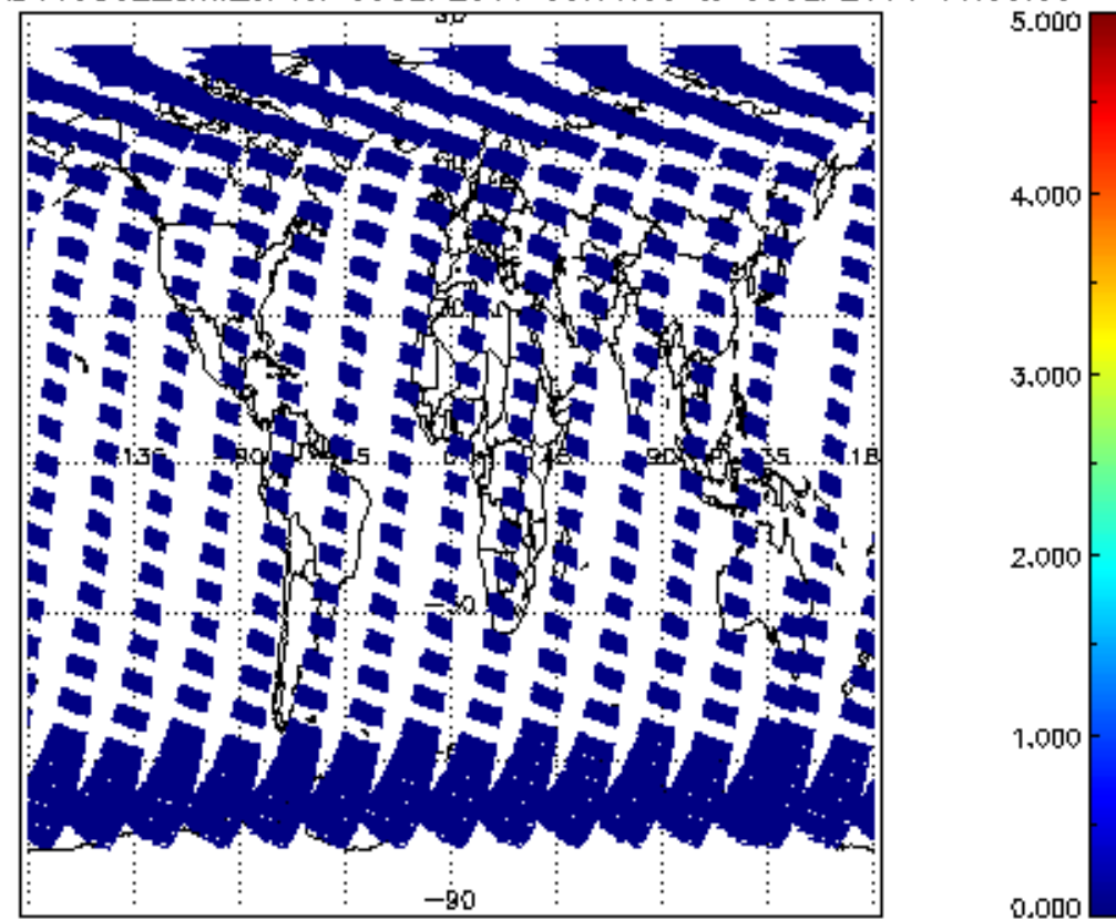
SCIOL2P_NADUV5S02_amf_cl for 05SEP2011 00:00:00 to 06SEP2011 00:00:00
