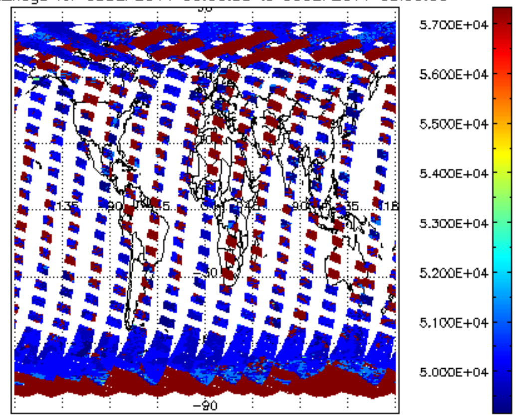
cloud_flags for 05SEP2011 00:00:00 to 06SEP2011 00:00:00
