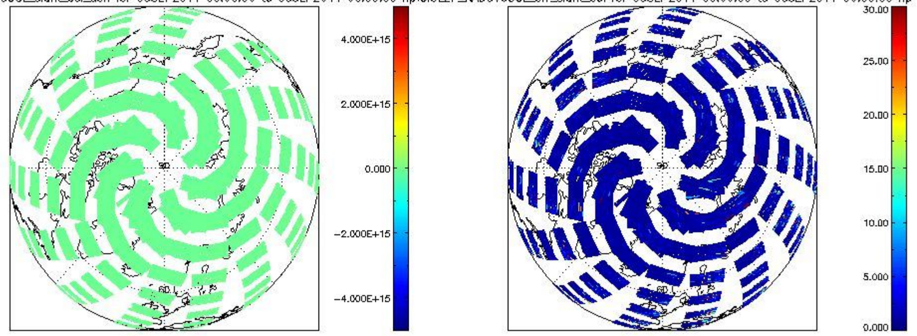
CIOL2P_NADUV60CLslant_col_den for 05SEP2011 00:00:00 to 06SEP2011 00:00:00 np; CIOL2P_NADUV60CLerr_slant_col for 05SEP2011 00:00:00 to 06SEP2011 00:00:00 np
