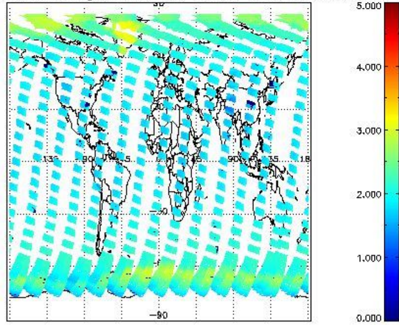
SCIOL2P_NADUV7S02_amf_gr for 05SEP2011 00:00:00 to 06SEP2011 00:00:00
