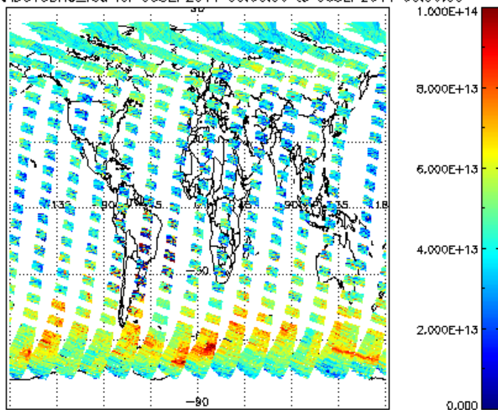
SCIOL2P_NADUV3BRO_vcd for 05SEP2011 00:00:00 to 06SEP2011 00:00:00
