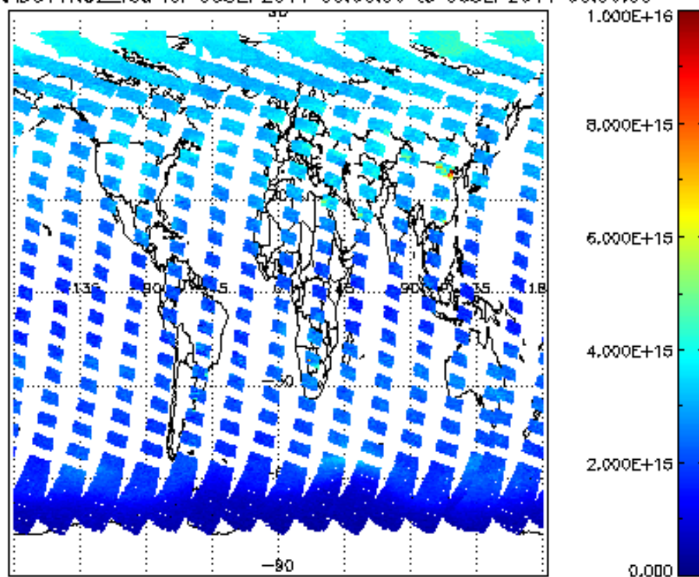
SCIOL2P_NADUV1NO2_vcd for 05SEP2011 00:00:00 to 06SEP2011 00:00:00
