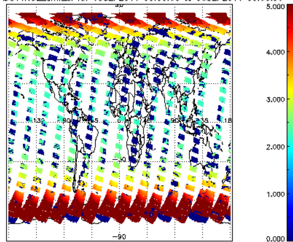
SCIOL2P_NADUV1NO2_amf_sl for 05SEP2011 00:00:00 to 06SEP2011 00:00:00
