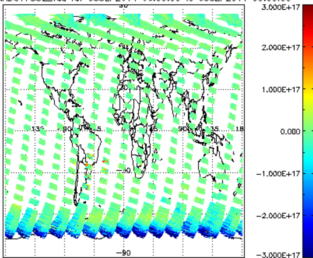
SCIOL2P_NADUV7S02_vcd for 05SEP2011 00:00:00 to 06SEP2011 00:00:00
