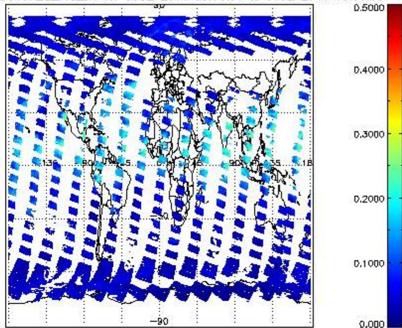
SCIOL2P_NADUV8H2O_vcd_err for 05SEP2011 00:00:00 to 06SEP2011 00:00:00
