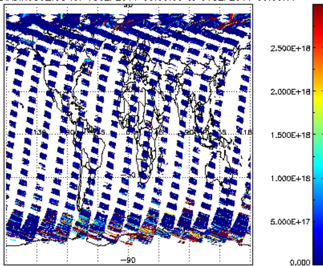
SCIOL2P_NADIR3CO_vcd for 05SEP2011 00:00:00 to 06SEP2011 00:00:00
