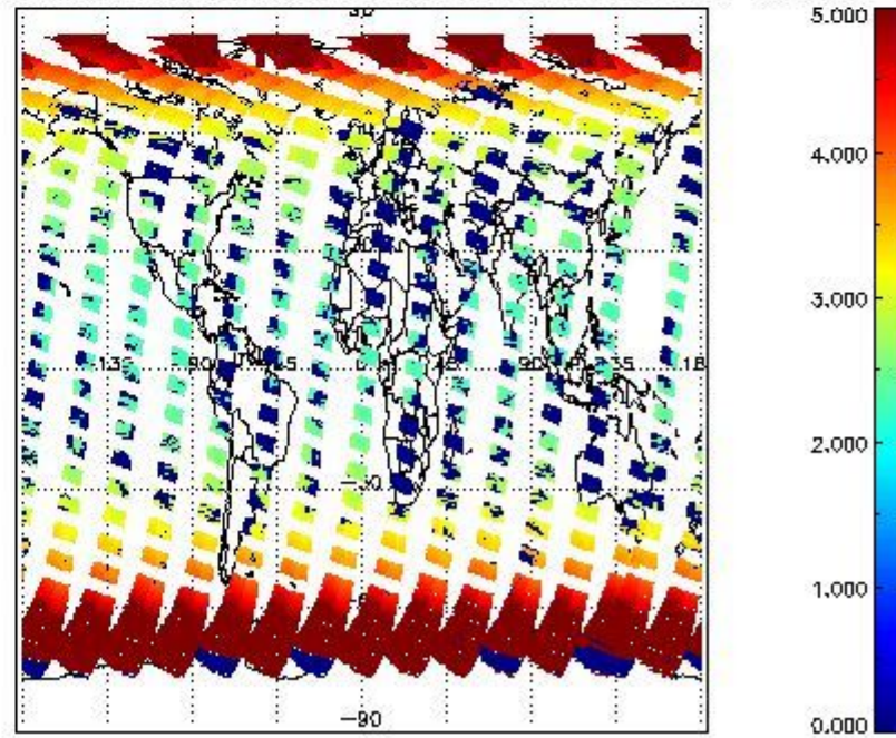
SCIOL2P_NADUV3BRO_amf_cl for 05SEP2011 00:00:00 to 06SEP2011 00:00:00
