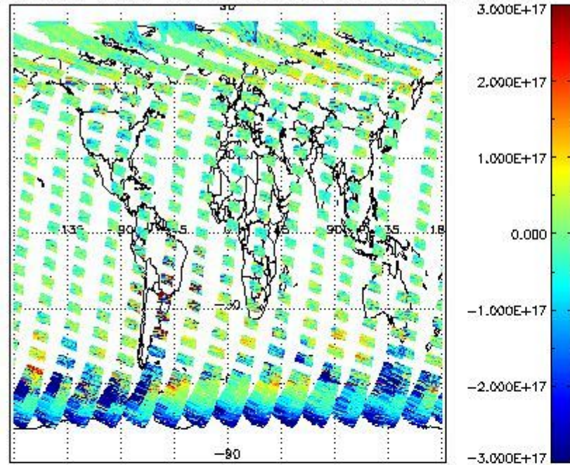
SCIOL2P_NADUV5S02_vcd for 05SEP2011 00:00:00 to 06SEP2011 00:00:00
