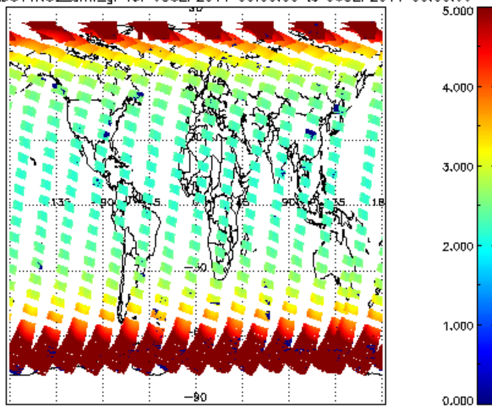
SCIOL2P_NADUV1NO2_amf_gr for 05SEP2011 00:00:00 to 06SEP2011 00:00:00
