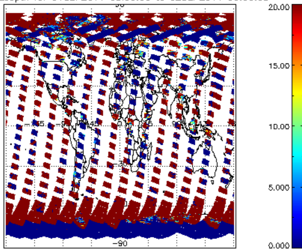
cl_opt_depth for 01SEP2011 00:00:00 to 02SEP2011 00:00:00
