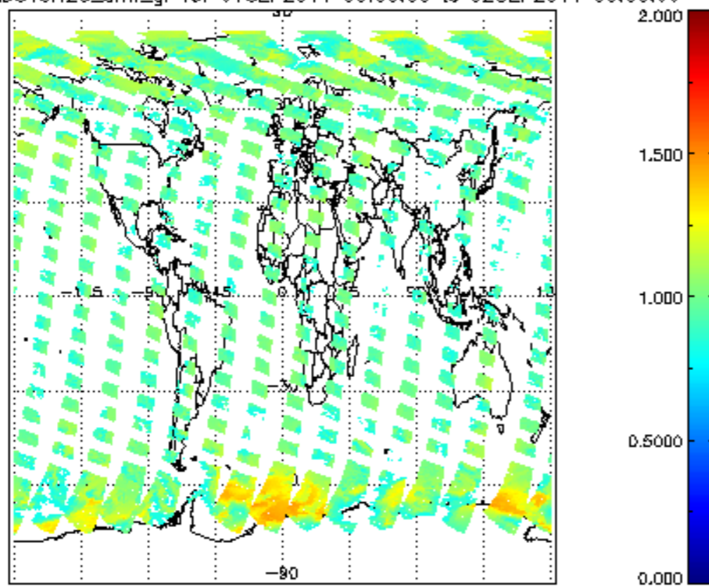
SCIOL2P_NADUV8H2O_amf_gr for 01SEP2011 00:00:00 to 02SEP2011 00:00:00
