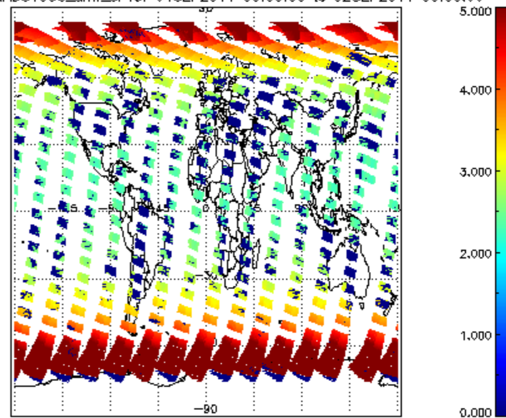
SCIOL2P_NADUV003_amf_cl for 01SEP2011 00:00:00 to 02SEP2011 00:00:00
