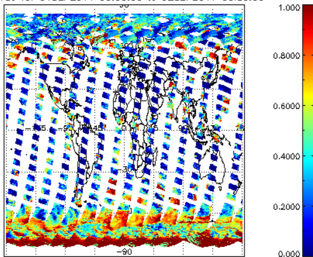
cl_frac for 01SEP2011 00:00:00 to 02SEP2011 00:00:00
