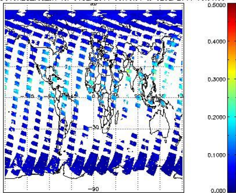
SCIOL2P_NADUV8H2O_vcd_err for 01SEP2011 00:00:00 to 02SEP2011 00:00:00
