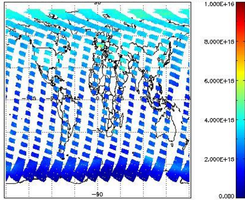
SCIOL2P_NADUV1NO2_vcd for 01SEP2011 00:00:00 to 02SEP2011 00:00:00
