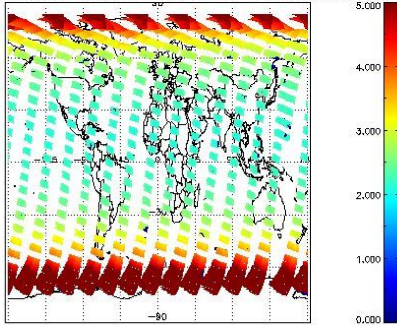
SCIOL2P_NADUV3BRO_amf_gr for 01SEP2011 00:00:00 to 02SEP2011 00:00:00
