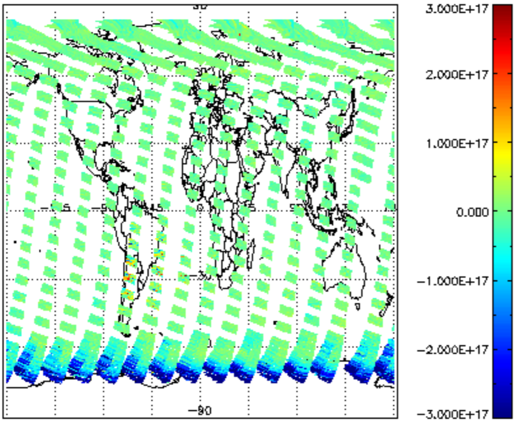
SCIOL2P_NADUV7S02_vcd for 01SEP2011 00:00:00 to 02SEP2011 00:00:00
