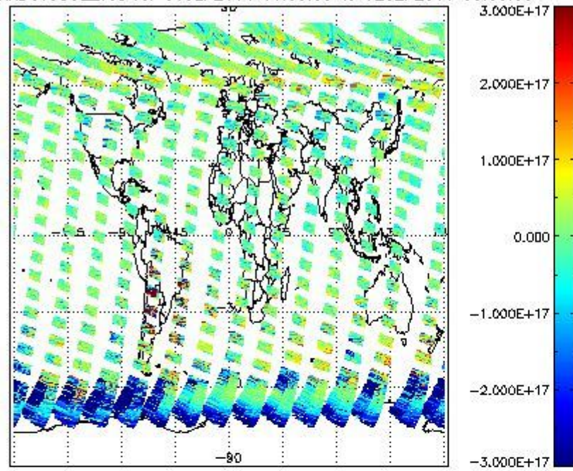
SCIOL2P_NADUV5S02_vcd for 01SEP2011 00:00:00 to 02SEP2011 00:00:00
