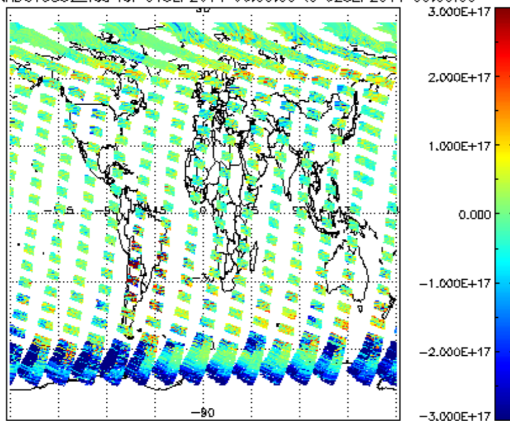
SCIOL2P_NADUV5S02_vcd for 01SEP2011 00:00:00 to 02SEP2011 00:00:00
