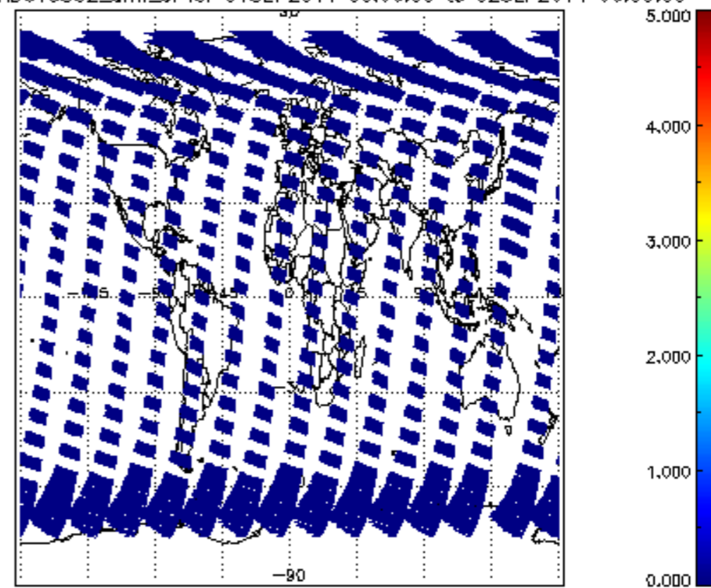
SCIOL2P_NADUV5S02_amf_cl for 01SEP2011 00:00:00 to 02SEP2011 00:00:00
