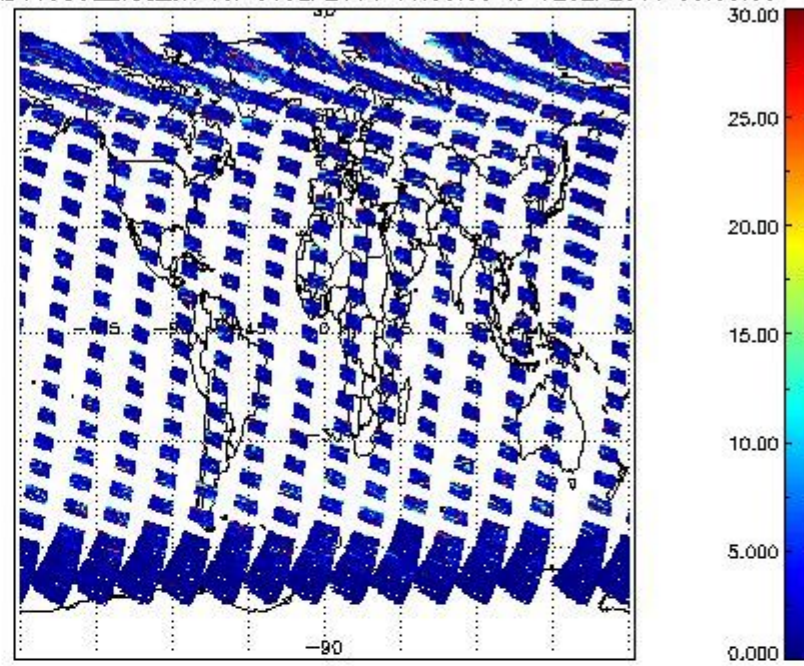
SCIOL2P_NADUV5S02_vcd_err for 01SEP2011 00:00:00 to 02SEP2011 00:00:00
