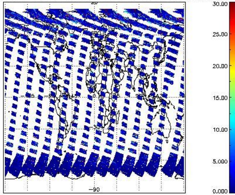
SCIOL2P_NADUV7S02_vcd_err for 01SEP2011 00:00:00 to 02SEP2011 00:00:00
