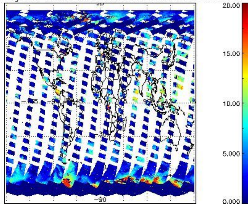
cL_top_height for 01SEP2011 00:00:00 to 02SEP2011 00:00:00
