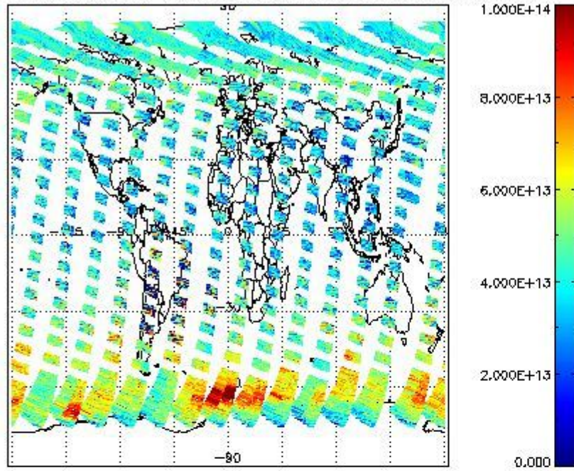
SCIOL2P_NADUV3BRO_vcd for 01SEP2011 00:00:00 to 02SEP2011 00:00:00
