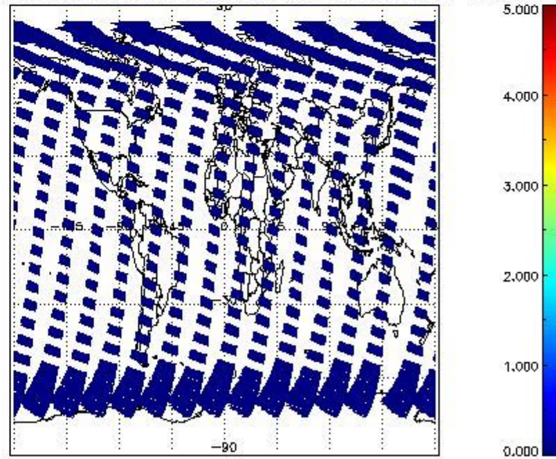
SCIOL2P_NADUV5S02_amf_cl for 01SEP2011 00:00:00 to 02SEP2011 00:00:00
