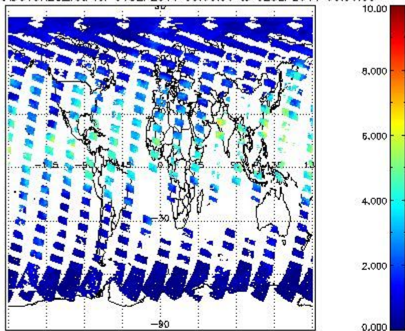
SCIOL2P_NADUV8H2O_vcd for 01SEP2011 00:00:00 to 02SEP2011 00:00:00
