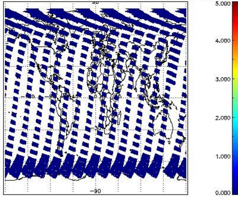
SCIOL2P_NADUV7S02_amf_cl for 01SEP2011 00:00:00 to 02SEP2011 00:00:00
