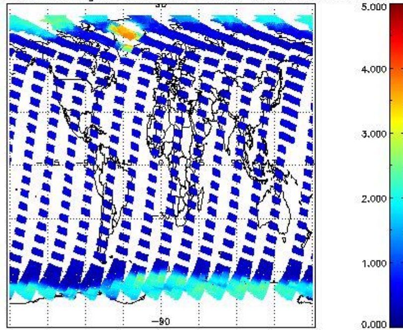
SCIOL2P_NADUV5S02_amf_gr for 01SEP2011 00:00:00 to 02SEP2011 00:00:00
