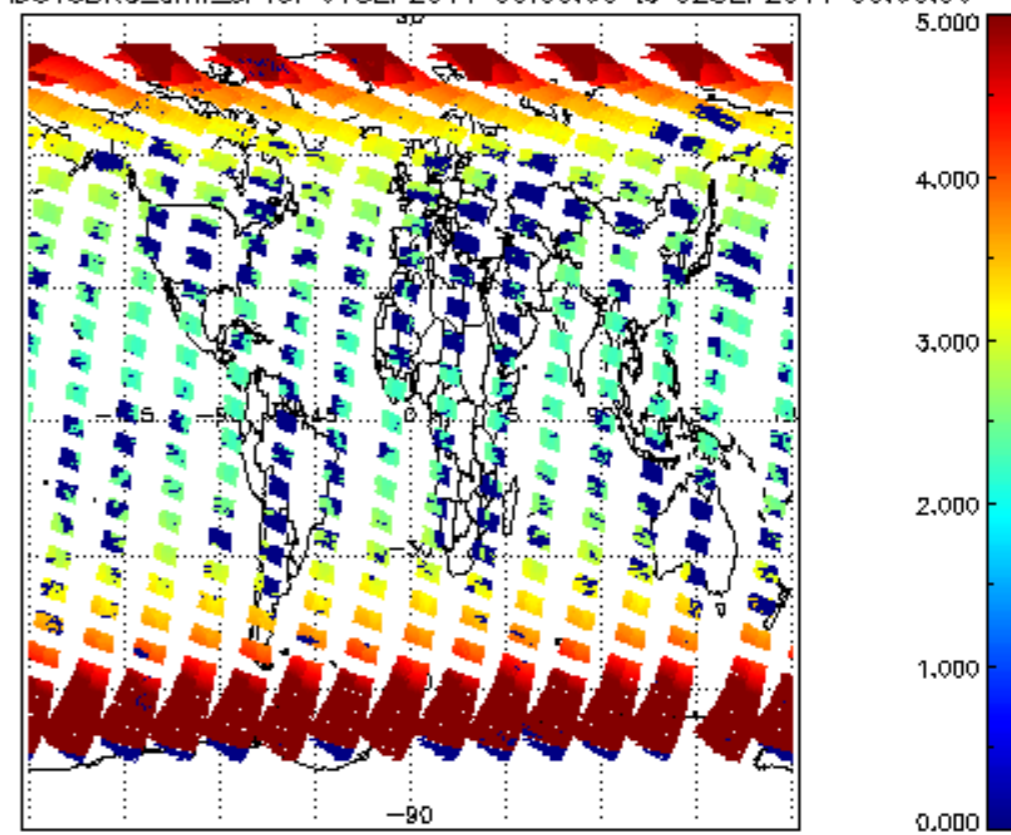
SCIOL2P_NADUV3BRO_amf_sl for 01SEP2011 00:00:00 to 02SEP2011 00:00:00
