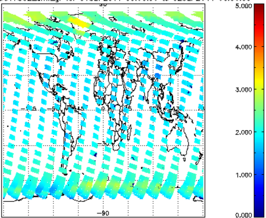
SCIOL2P_NADUV7S02_amf_gr for 01SEP2011 00:00:00 to 02SEP2011 00:00:00
