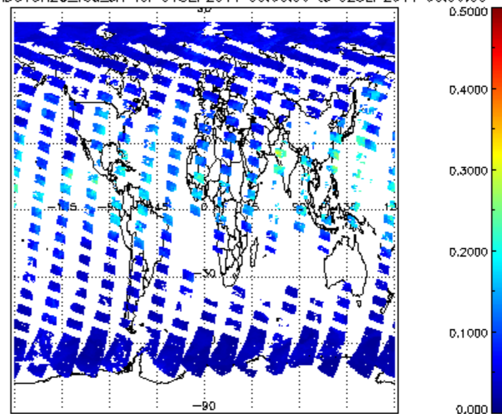
SCIOL2P_NADUV8H2O_vcd_err for 01SEP2011 00:00:00 to 02SEP2011 00:00:00
