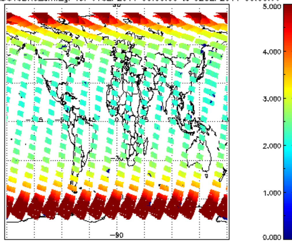
SCIOL2P_NADUV3BRO_amf_gr for 01SEP2011 00:00:00 to 02SEP2011 00:00:00
