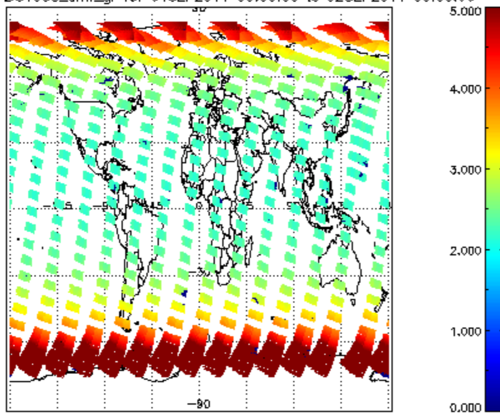
SCIOL2P_NADUV003_amf_gr for 01SEP2011 00:00:00 to 02SEP2011 00:00:00
