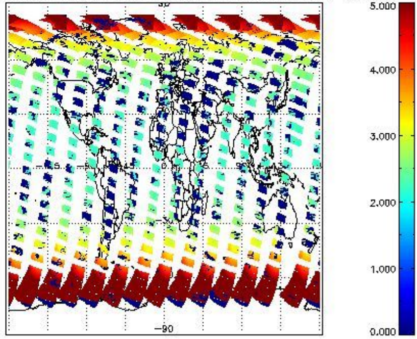
SCIOL2P_NADUV1NO2_amf_cl for 01SEP2011 00:00:00 to 02SEP2011 00:00:00
