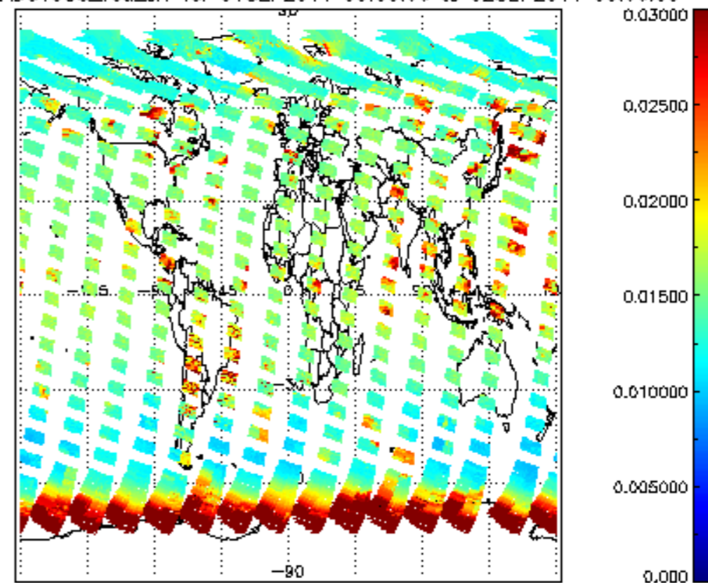
SCIOL2P_NADUV003_vcd_err for 01SEP2011 00:00:00 to 02SEP2011 00:00:00
