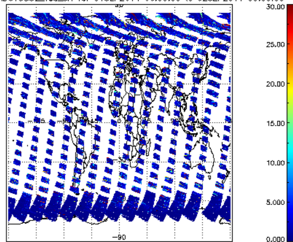
SCIOL2P_NADUV5S02_vcd_err for 01SEP2011 00:00:00 to 02SEP2011 00:00:00
