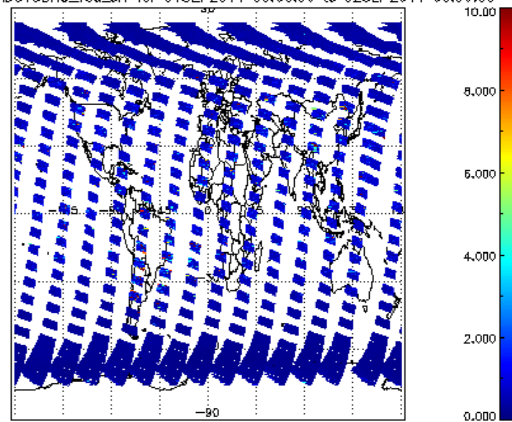
SCIOL2P_NADUV3BRO_vcd_err for 01SEP2011 00:00:00 to 02SEP2011 00:00:00
