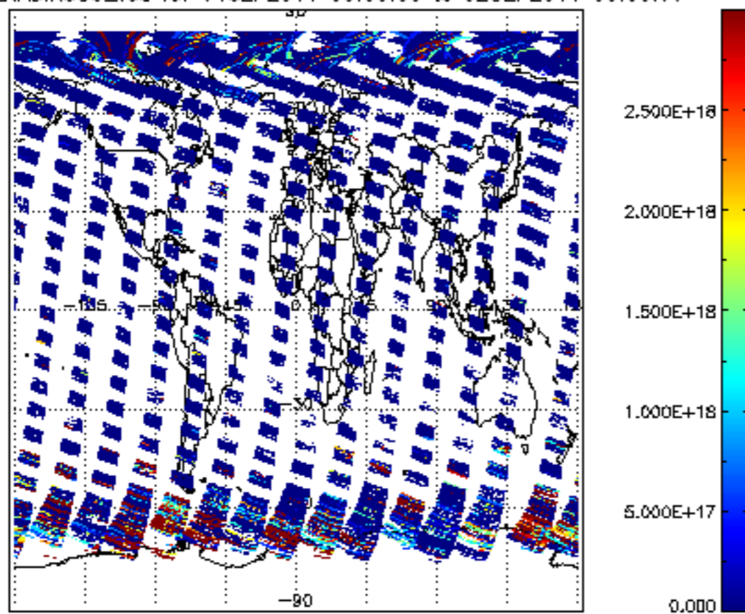
SCIOL2P_NADIR3CO_vcd for 01SEP2011 00:00:00 to 02SEP2011 00:00:00
