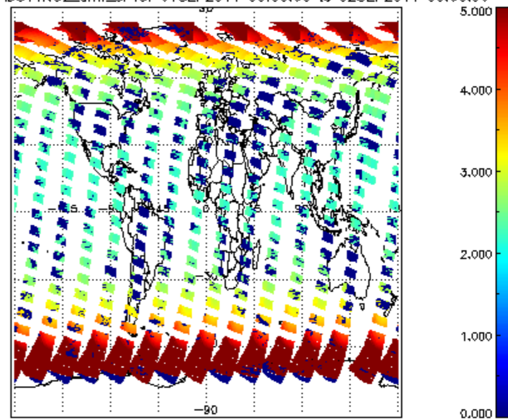
SCIOL2P_NADUV1N02_amf_sl for 01SEP2011 00:00:00 to 02SEP2011 00:00:00
