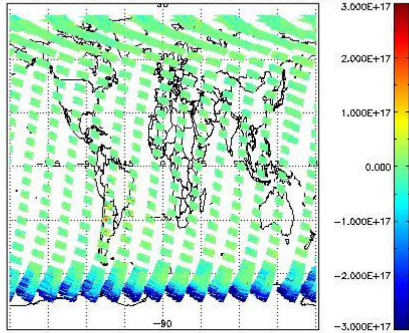
SCIOL2P_NADUV7S02_vcd for 01SEP2011 00:00:00 to 02SEP2011 00:00:00
