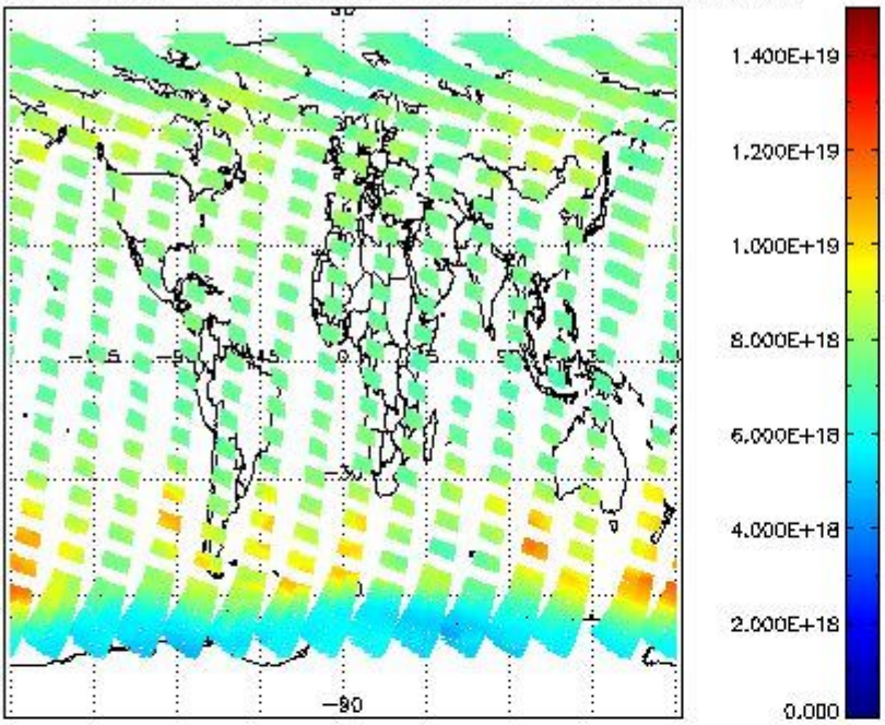
SCIOL2P_NADUV003_vcd for 01SEP2011 00:00:00 to 02SEP2011 00:00:00
