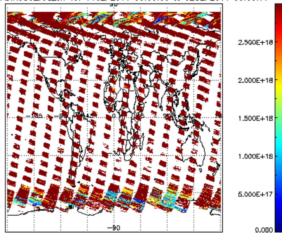
SCIOL2P_NADIR3CO_vcd_err for 01SEP2011 00:00:00 to 02SEP2011 00:00:00
