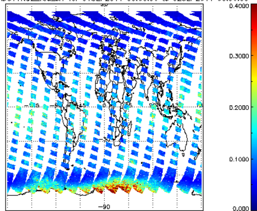
SCIOL2P_NADUV1N02_vcd_err for 01SEP2011 00:00:00 to 02SEP2011 00:00:00
