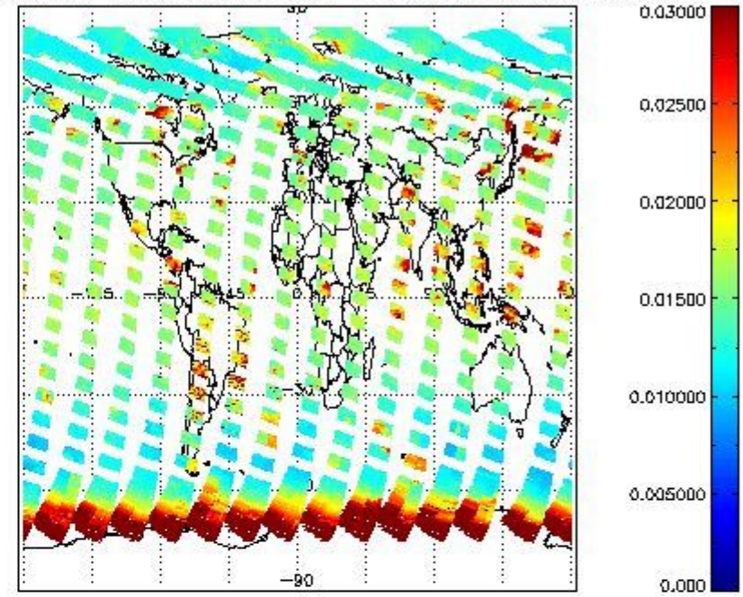
SCIOL2P_NADUV003_vcd_err for 01SEP2011 00:00:00 to 02SEP2011 00:00:00
