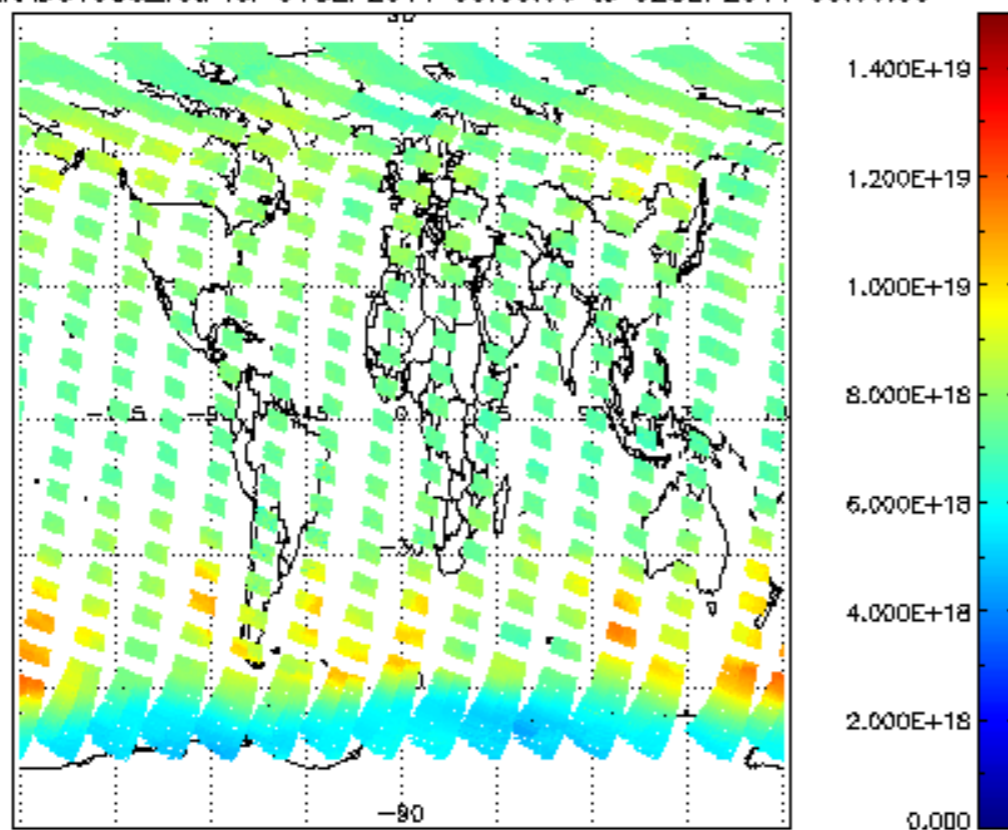
SCIOL2P_NADUV003_vcd for 01SEP2011 00:00:00 to 02SEP2011 00:00:00
