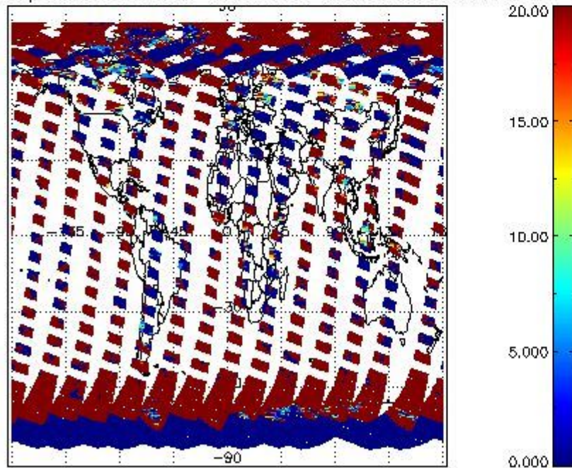
cL_opt_depth for 01SEP2011 00:00:00 to 02SEP2011 00:00:00
