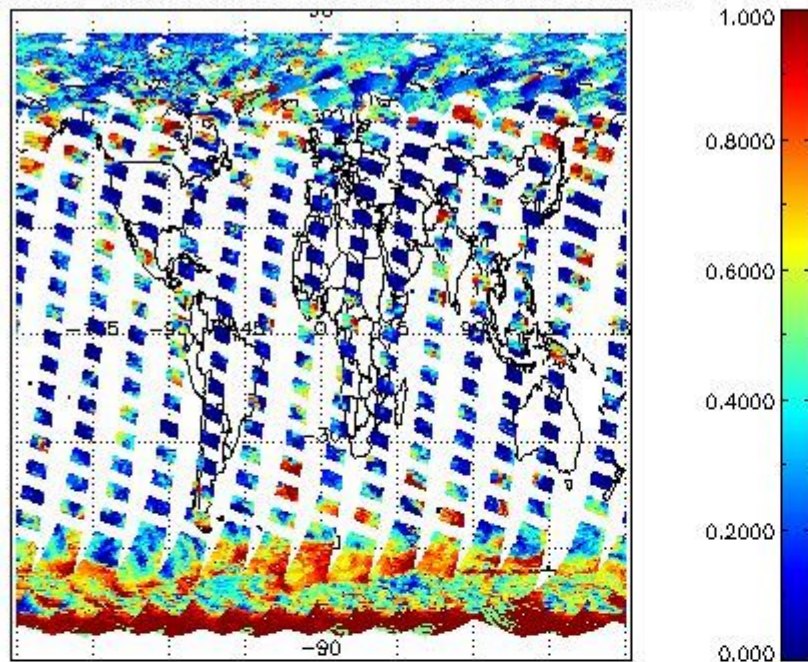
cL_frac for 01SEP2011 00:00:00 to 02SEP2011 00:00:00
