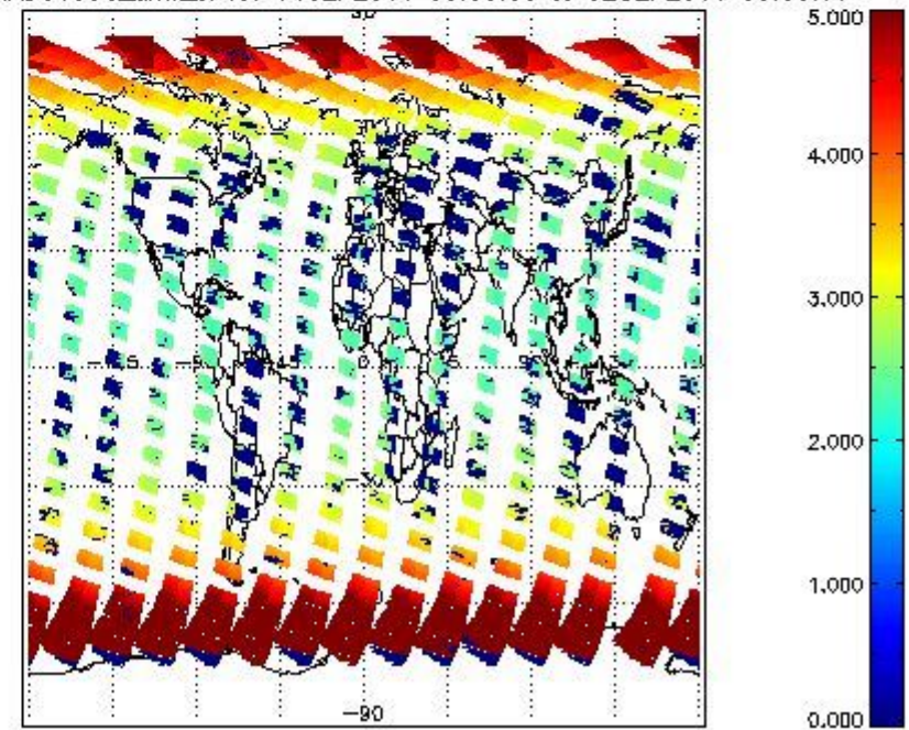
SCIOL2P_NADUV003_amf_cl for 01SEP2011 00:00:00 to 02SEP2011 00:00:00
