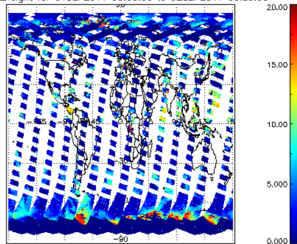
cl_top_height for 01SEP2011 00:00:00 to 02SEP2011 00:00:00
