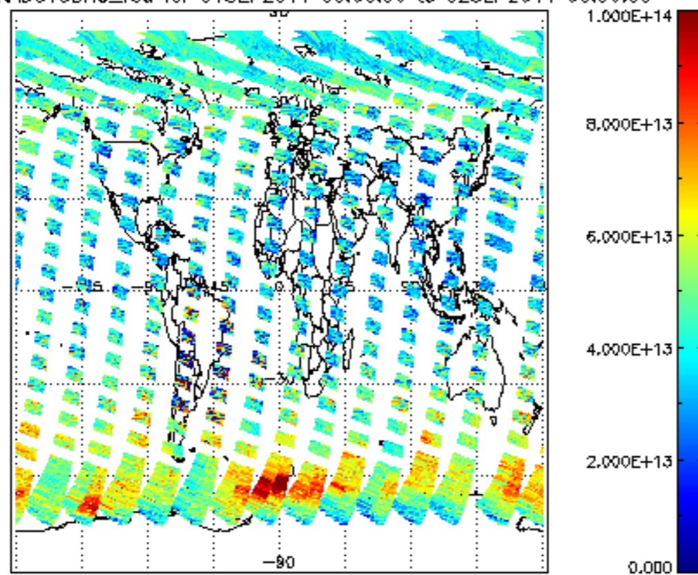
SCIOL2P_NADUV3BRO_vcd for 01SEP2011 00:00:00 to 02SEP2011 00:00:00
