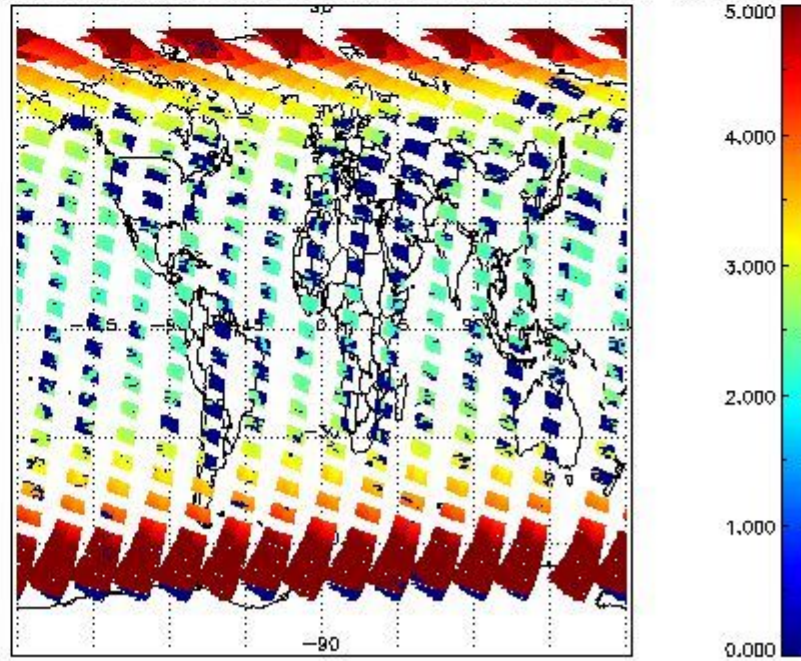
SCIOL2P_NADUV3BRO_amf_cl for 01SEP2011 00:00:00 to 02SEP2011 00:00:00
