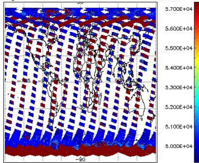
cloud_flags for 01SEP2011 00:00:00 to 02SEP2011 00:00:00
