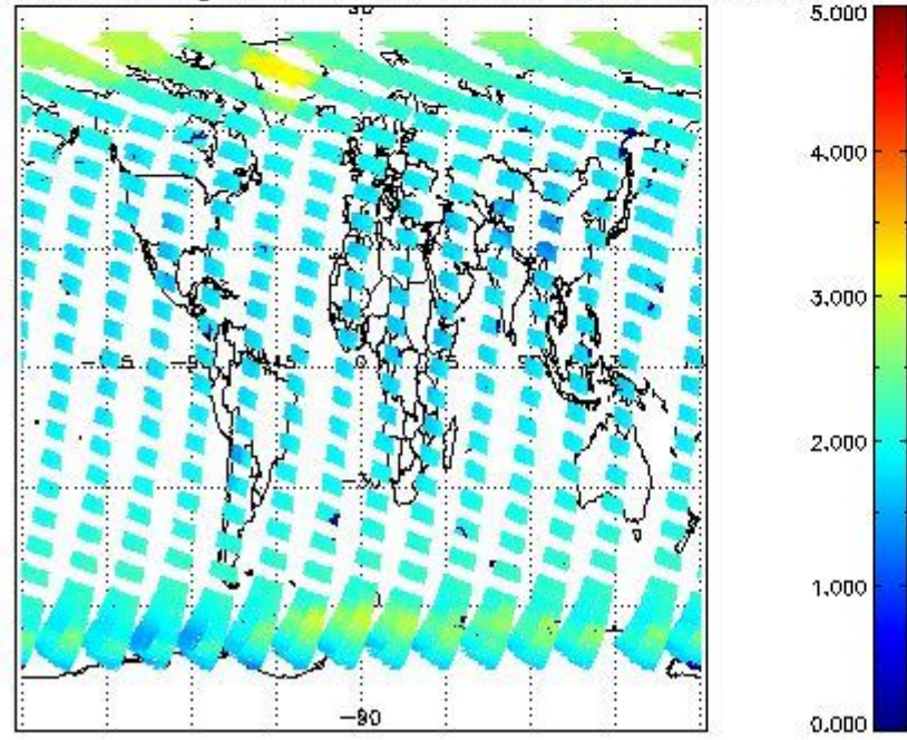
SCIOL2P_NADUV7S02_amf_gr for 01SEP2011 00:00:00 to 02SEP2011 00:00:00
