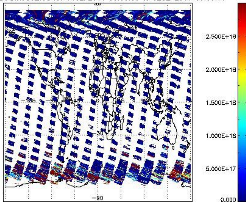
SCIDL2P_NADIR3CO_vcd for 01SEP2011 00:00:00 to 02SEP2011 00:00:00
