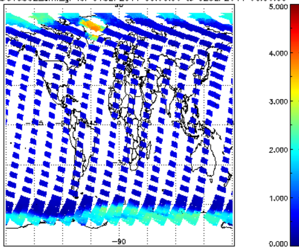
SCIOL2P_NADUV5S02_amf_gr for 01SEP2011 00:00:00 to 02SEP2011 00:00:00
