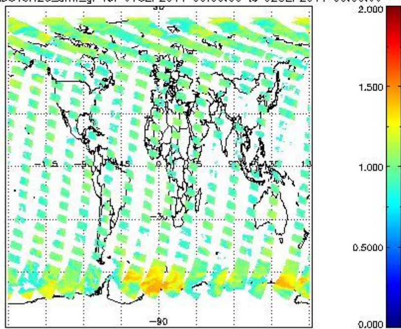
SCIOL2P_NADUV8H2O_arnf_gr for 01SEP2011 00:00:00 to 02SEP2011 00:00:00
