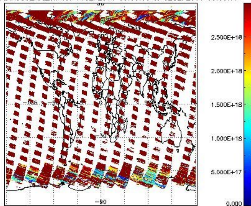
SCIDL2P_NADIR3CO_vcd_err for 01SEP2011 00:00:00 to 02SEP2011 00:00:00
