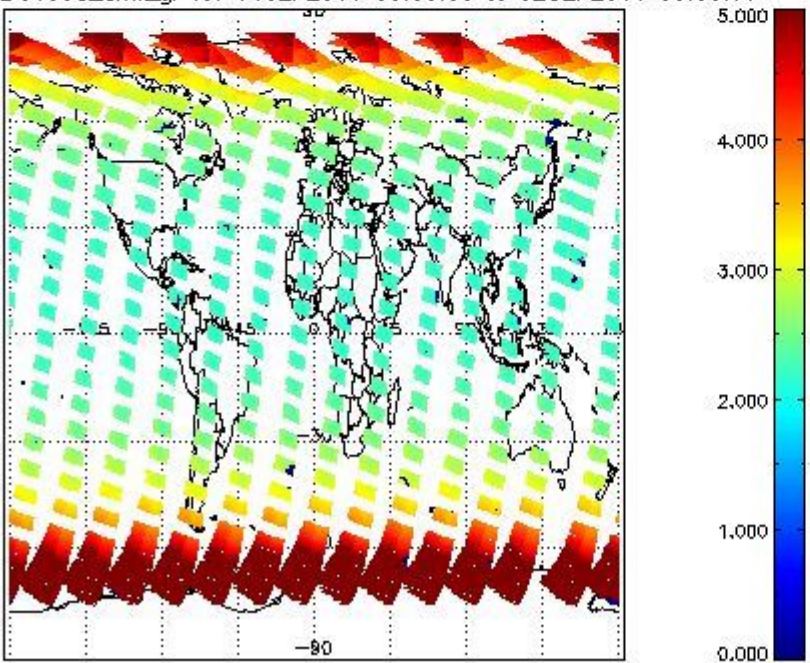
SCIOL2P_NADUV003_amf_gr for 01SEP2011 00:00:00 to 02SEP2011 00:00:00
