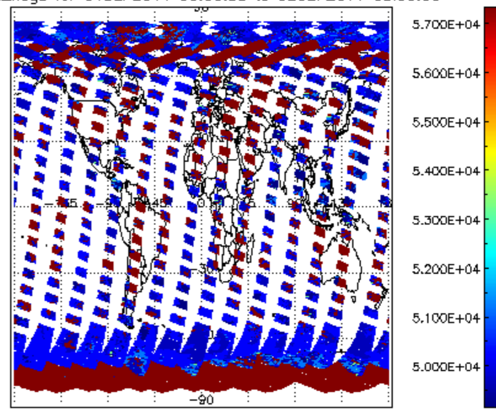
cloud_flags for 01SEP2011 00:00:00 to 02SEP2011 00:00:00
