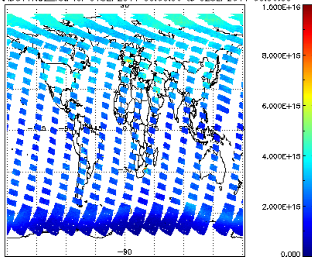
SCIOL2P_NADUV1N02_vcd for 01SEP2011 00:00:00 to 02SEP2011 00:00:00
