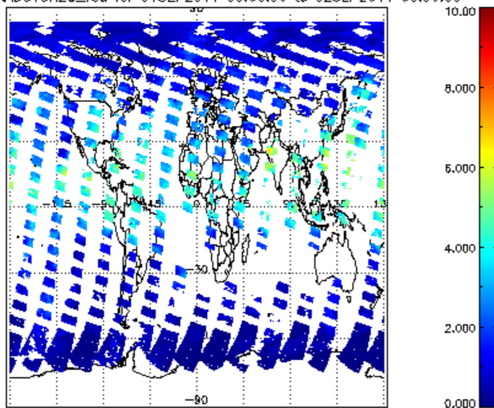
SCIOL2P_NADUV8H2O_vcd for 01SEP2011 00:00:00 to 02SEP2011 00:00:00
