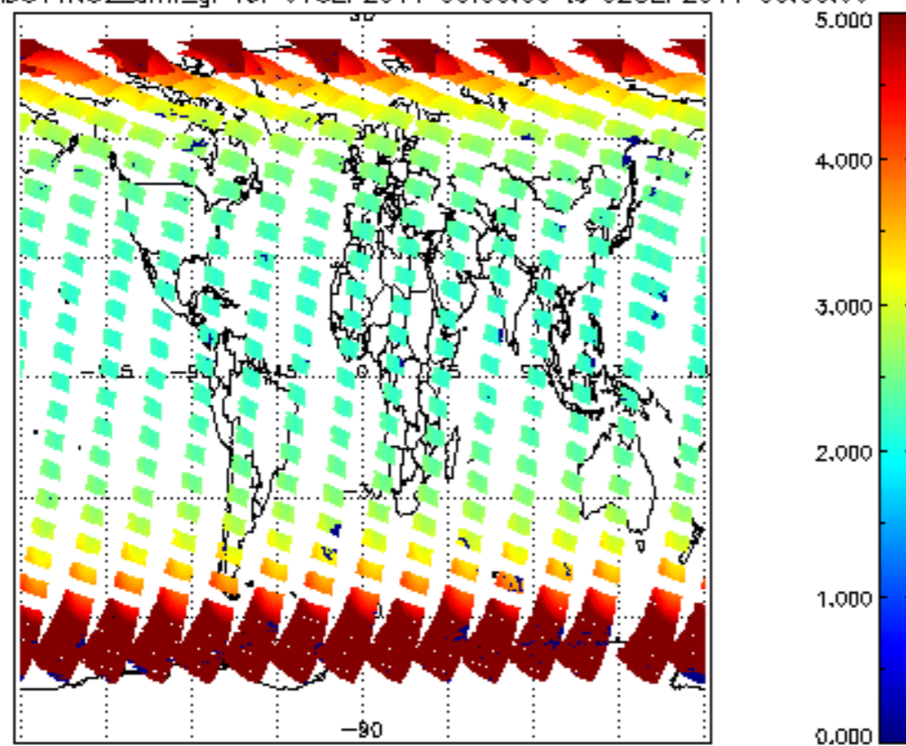
SCIOL2P_NADUV1N02_amf_gr for 01SEP2011 00:00:00 to 02SEP2011 00:00:00
