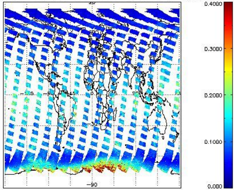
SCIOL2P_NADUV1NO2_vcd_err for 01SEP2011 00:00:00 to 02SEP2011 00:00:00
