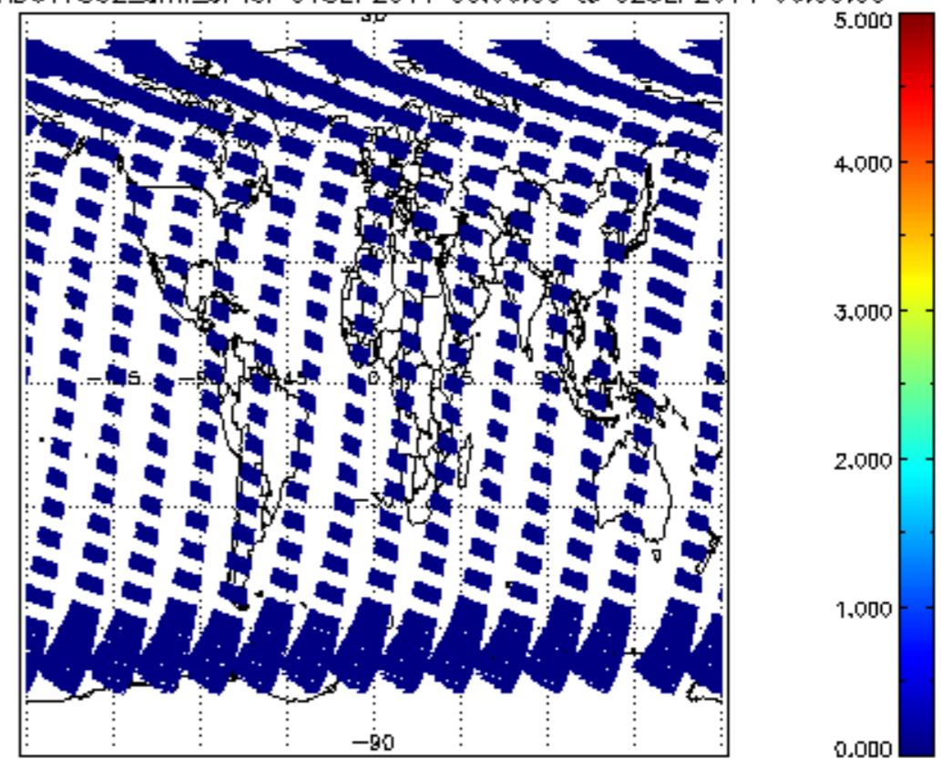
SCIOL2P_NADUV7S02_amf_cl for 01SEP2011 00:00:00 to 02SEP2011 00:00:00
