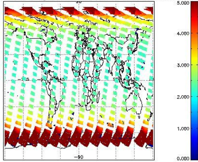
SCIOL2P_NADUV1NO2_amf_gr for 01SEP2011 00:00:00 to 02SEP2011 00:00:00
