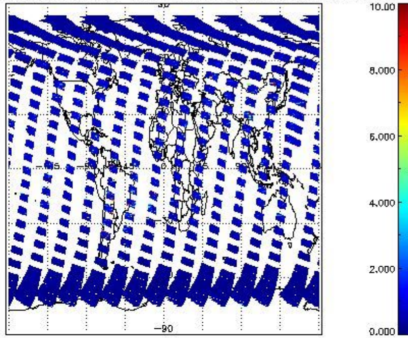
SCIOL2P_NADUV3BRO_vcd_err for 01SEP2011 00:00:00 to 02SEP2011 00:00:00
