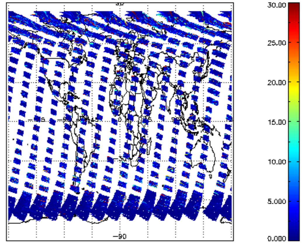
SCIOL2P_NADUV7S02_vcd_err for 01SEP2011 00:00:00 to 02SEP2011 00:00:00
