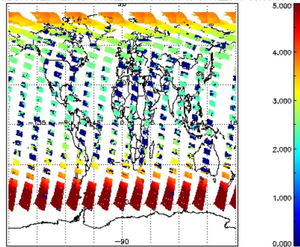
SCIOL2P_NADUV003_amf_cl for 30JUL2011 00:00:00 to 31JUL2011 00:00:00
