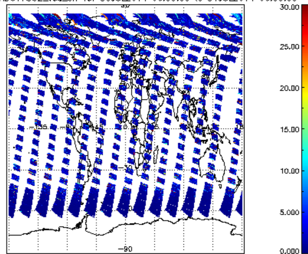
SCIOL2P_NADUV7S02_vcd_err for 30JUL2011 00:00:00 to 31JUL2011 00:00:00
