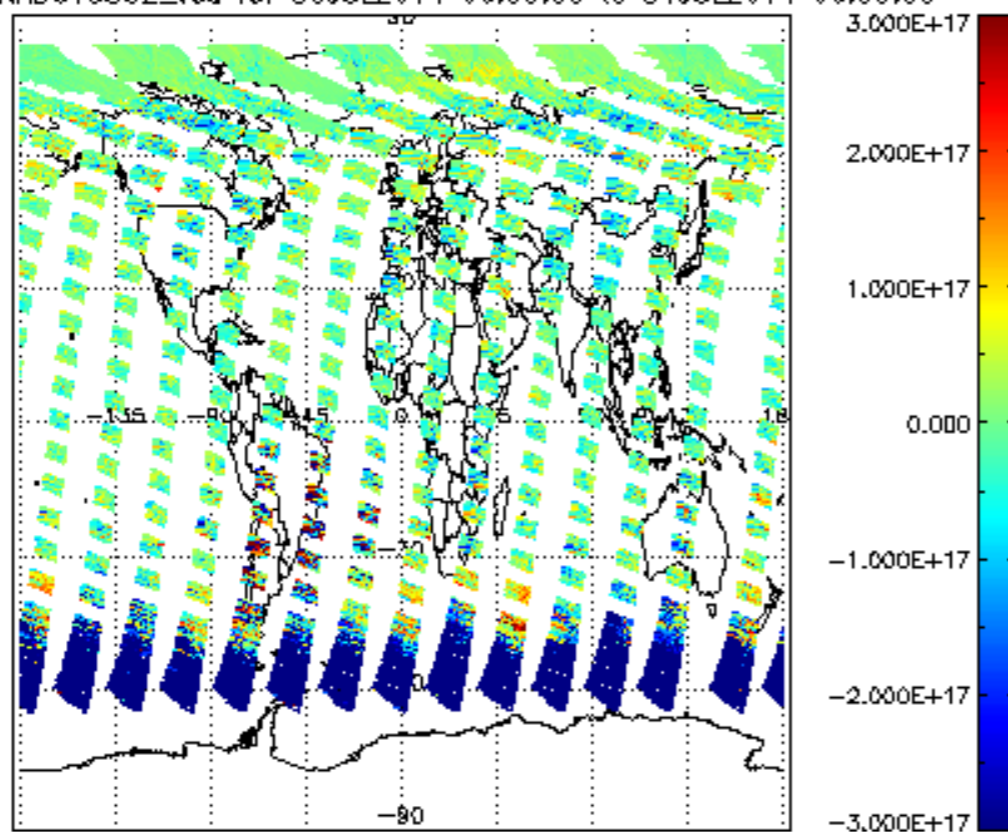
SCIOL2P_NADUV5S02_vcd for 30JUL2011 00:00:00 to 31JUL2011 00:00:00
