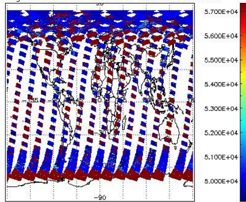
cloud_flags for 30JUL2011 00:00:00 to 31JUL2011 00:00:00
