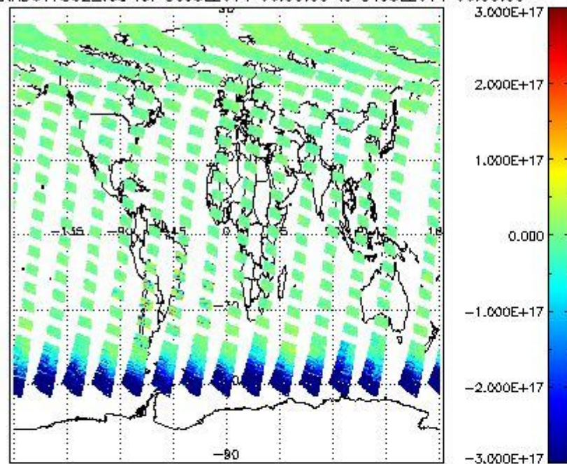
SCIOL2P_NADUV7S02_vcd for 30JUL2011 00:00:00 to 31JUL2011 00:00:00
