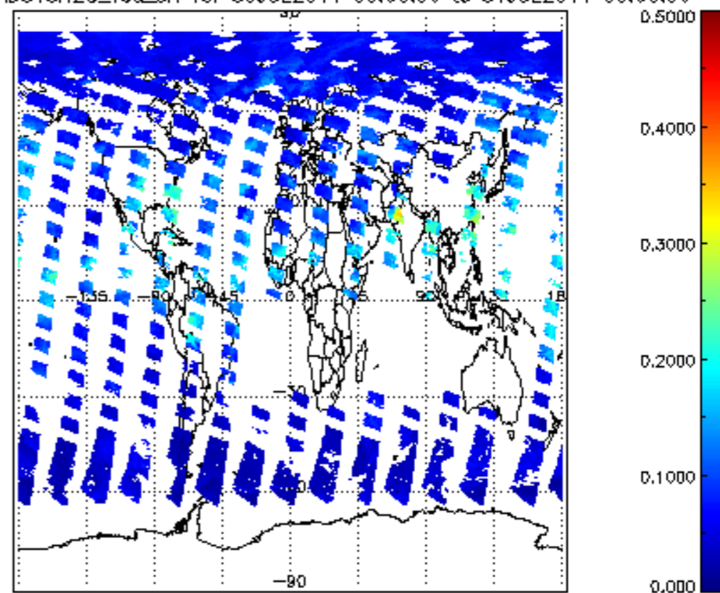
SCIOL2P_NADUV8H20_vcd_err for 30JUL2011 00:00:00 to 31JUL2011 00:00:00
