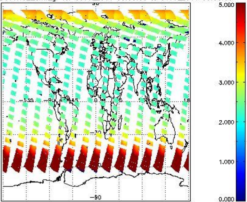
SCIOL2P_NADUV1NO2_amf_gr for 30JUL2011 00:00:00 to 31JUL2011 00:00:00
