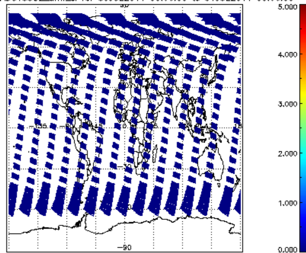
SCIOL2P_NADUV5S02_amf_cl for 30JUL2011 00:00:00 to 31JUL2011 00:00:00
