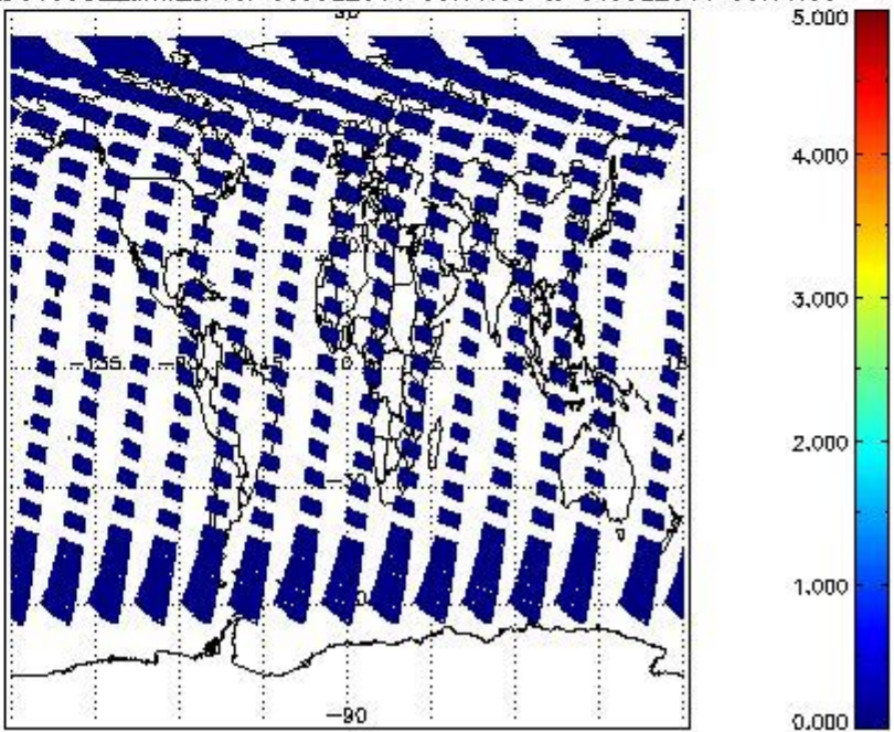
SCIOL2P_NADUV5S02_amf_cl for 30JUL2011 00:00:00 to 31JUL2011 00:00:00
