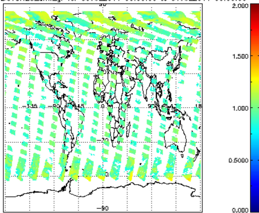
SCIOL2P_NADUV8H20_amf_gr for 30JUL2011 00:00:00 to 31JUL2011 00:00:00
