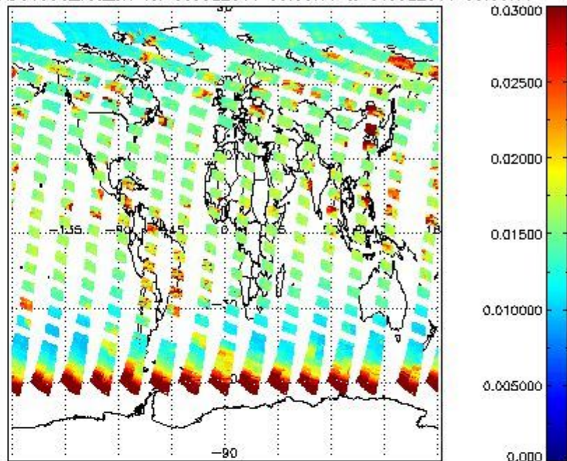
SCIOL2P_NADUV003_vcd_err for 30JUL2011 00:00:00 to 31JUL2011 00:00:00
