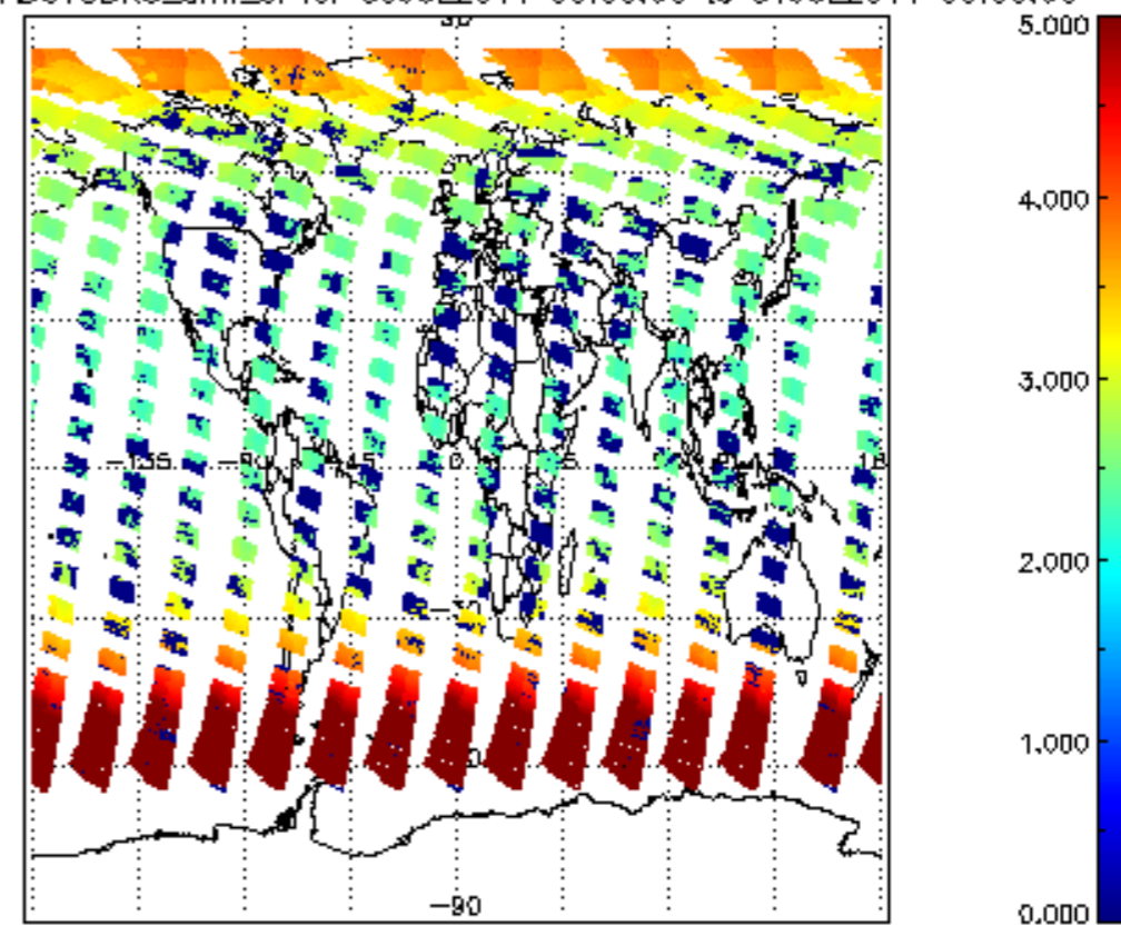
SCIOL2P_NADUV3BRO_amf_cl for 30JUL2011 00:00:00 to 31JUL2011 00:00:00
