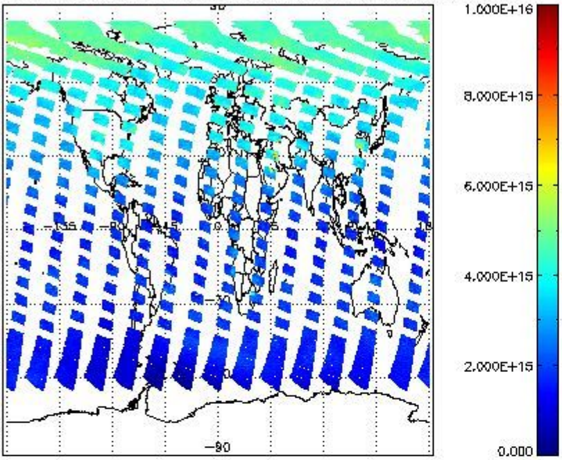
SCIOL2P_NADUV1NO2_vcd for 30JUL2011 00:00:00 to 31JUL2011 00:00:00
