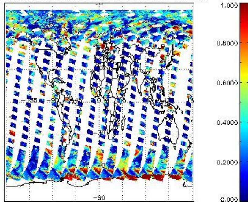
cL_frac for 30JUL2011 00:00:00 to 31JUL2011 00:00:00
