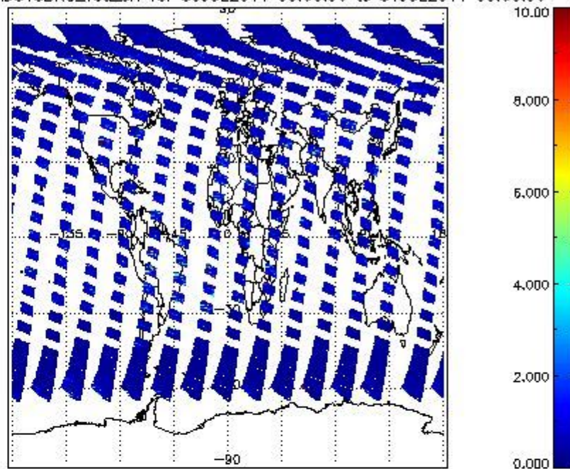
SCIOL2P_NADUV3BRO_vcd_err for 30JUL2011 00:00:00 to 31JUL2011 00:00:00
