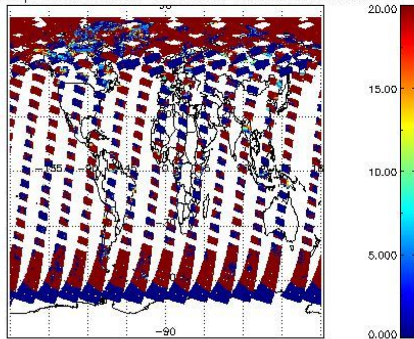
cL_opt_depth for 30JUL2011 00:00:00 to 31JUL2011 00:00:00
