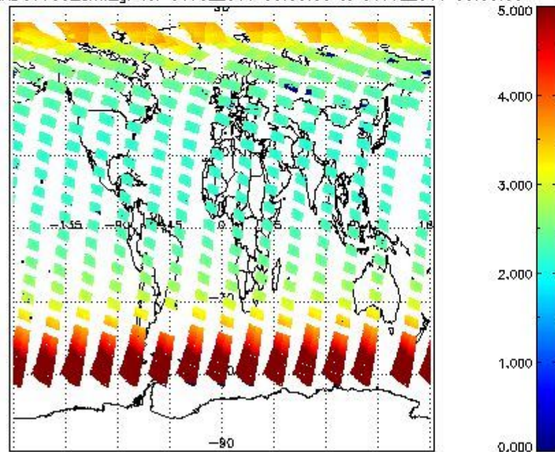
SCIOL2P_NADUV003_amf_gr for 30JUL2011 00:00:00 to 31JUL2011 00:00:00
