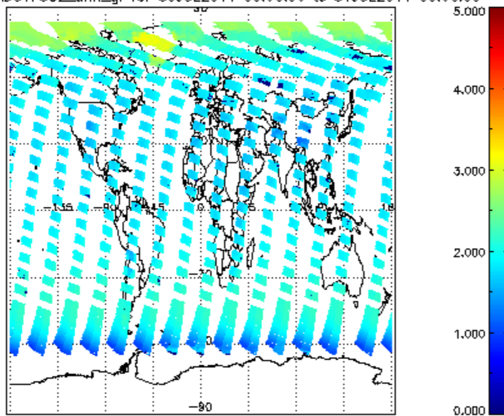
SCIOL2P_NADUV7S02_amf_gr for 30JUL2011 00:00:00 to 31JUL2011 00:00:00
