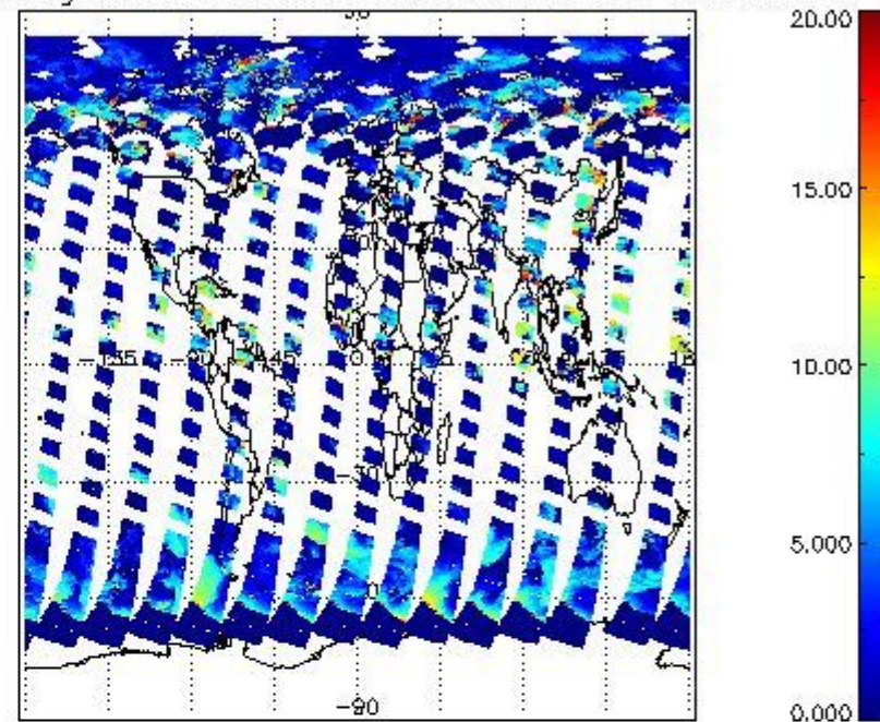
cL_top_height for 30JUL2011 00:00:00 to 31JUL2011 00:00:00
