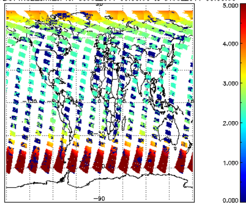
SCIOL2P_NADUV1NO2_amf_cl for 30JUL2011 00:00:00 to 31JUL2011 00:00:00
