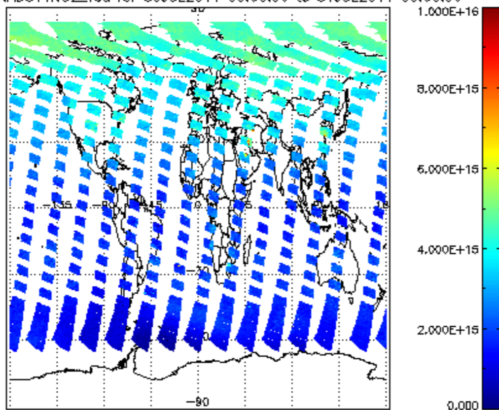
SCIOL2P_NADUV1NO2_vcd for 30JUL2011 00:00:00 to 31JUL2011 00:00:00
