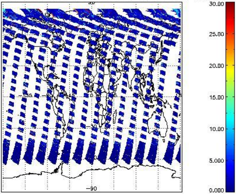
SCIOL2P_NADUV5S02_vcd_err for 30JUL2011 00:00:00 to 31JUL2011 00:00:00
