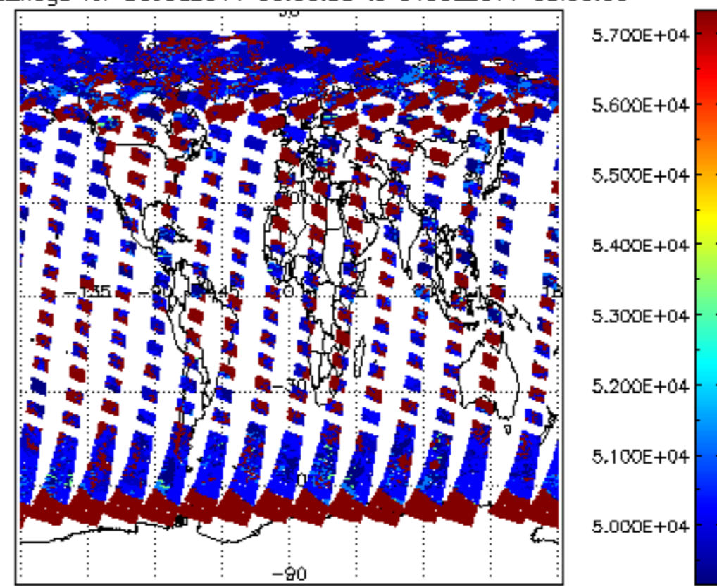
cloud_flags for 30JUL2011 00:00:00 to 31JUL2011 00:00:00
