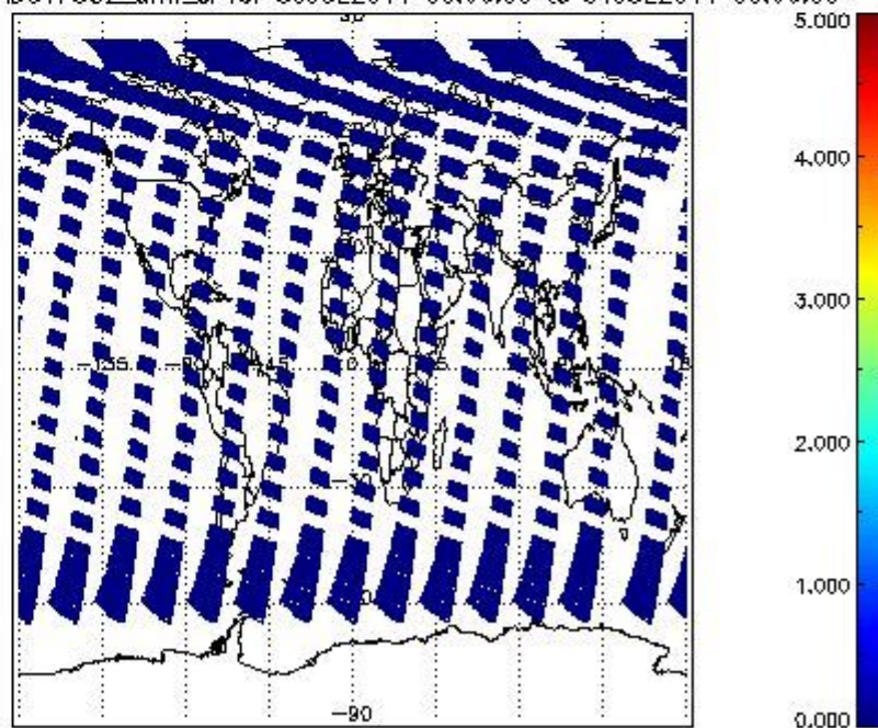
SCIOL2P_NADUV7S02_amf_cl for 30JUL2011 00:00:00 to 31JUL2011 00:00:00
