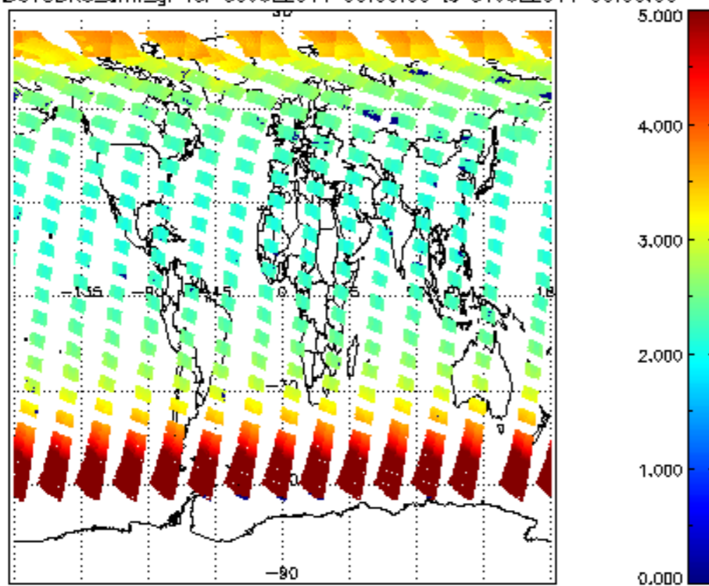
SCIOL2P_NADUV3BRO_amf_gr for 30JUL2011 00:00:00 to 31JUL2011 00:00:00
