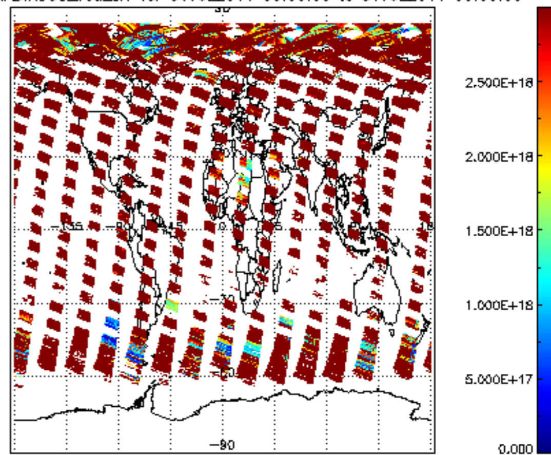
SCIOL2P_NADIR3CO_vcd_err for 30JUL2011 00:00:00 to 31JUL2011 00:00:00
