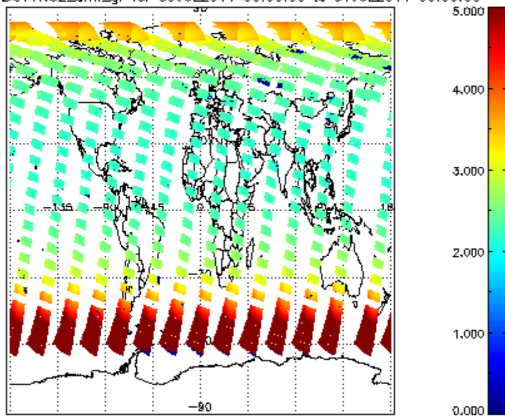
SCIOL2P_NADUV1NO2_amf_gr for 30JUL2011 00:00:00 to 31JUL2011 00:00:00
