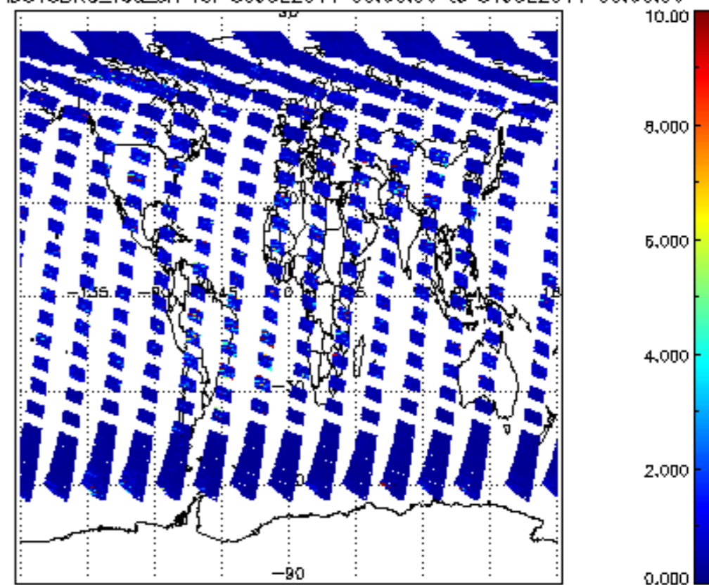
SCIOL2P_NADUV3BRO_vcd_err for 30JUL2011 00:00:00 to 31JUL2011 00:00:00
