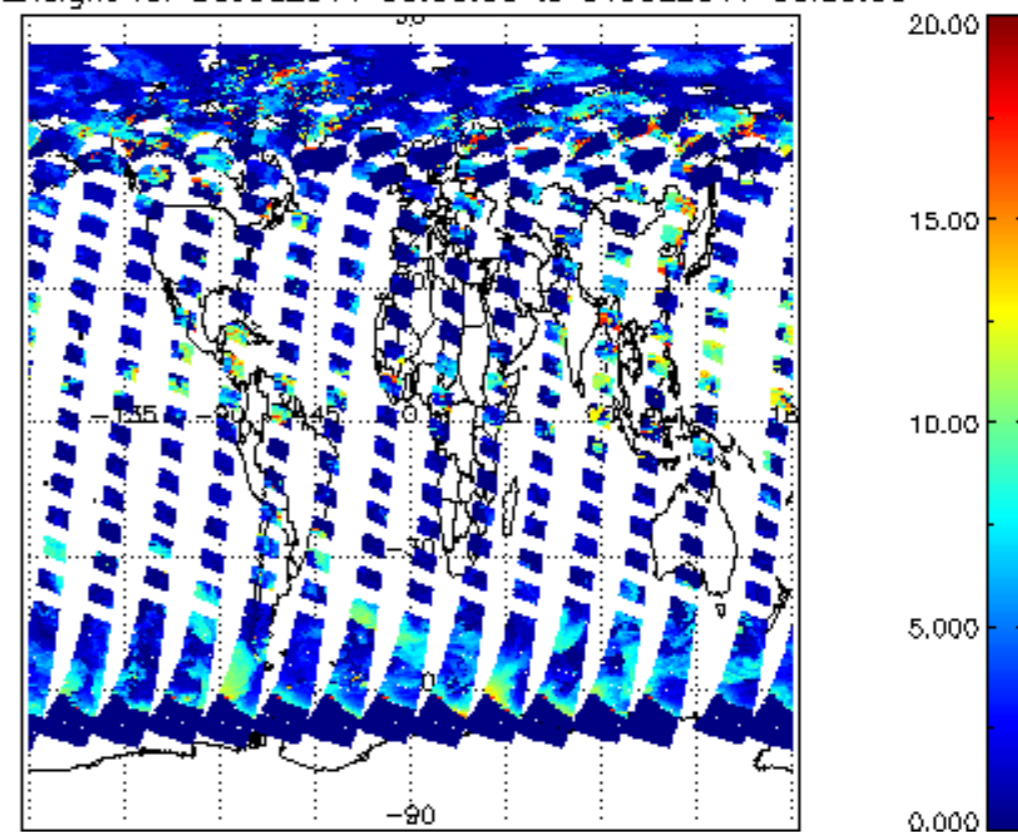
cl_top_height for 30JUL2011 00:00:00 to 31JUL2011 00:00:00
