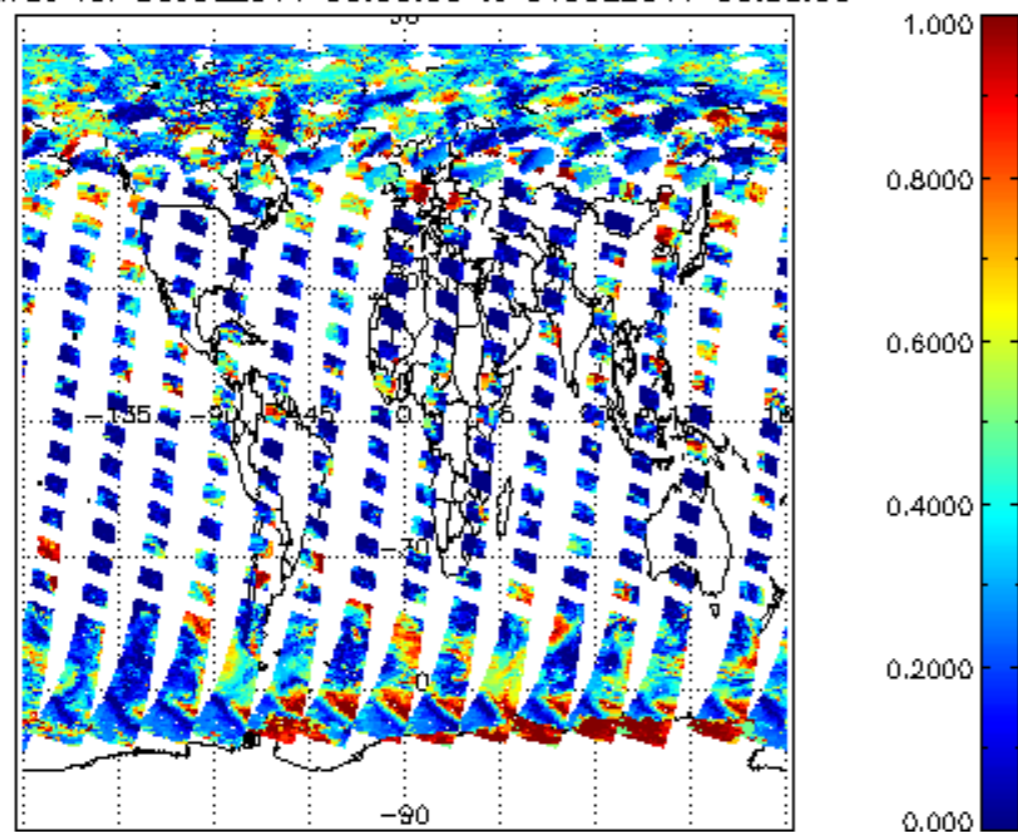
cl_frac for 30JUL2011 00:00:00 to 31JUL2011 00:00:00
