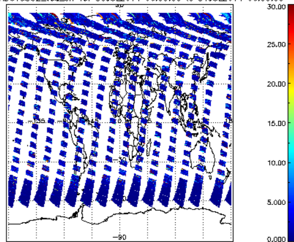
SCIOL2P_NADUV5S02_vcd_err for 30JUL2011 00:00:00 to 31JUL2011 00:00:00
