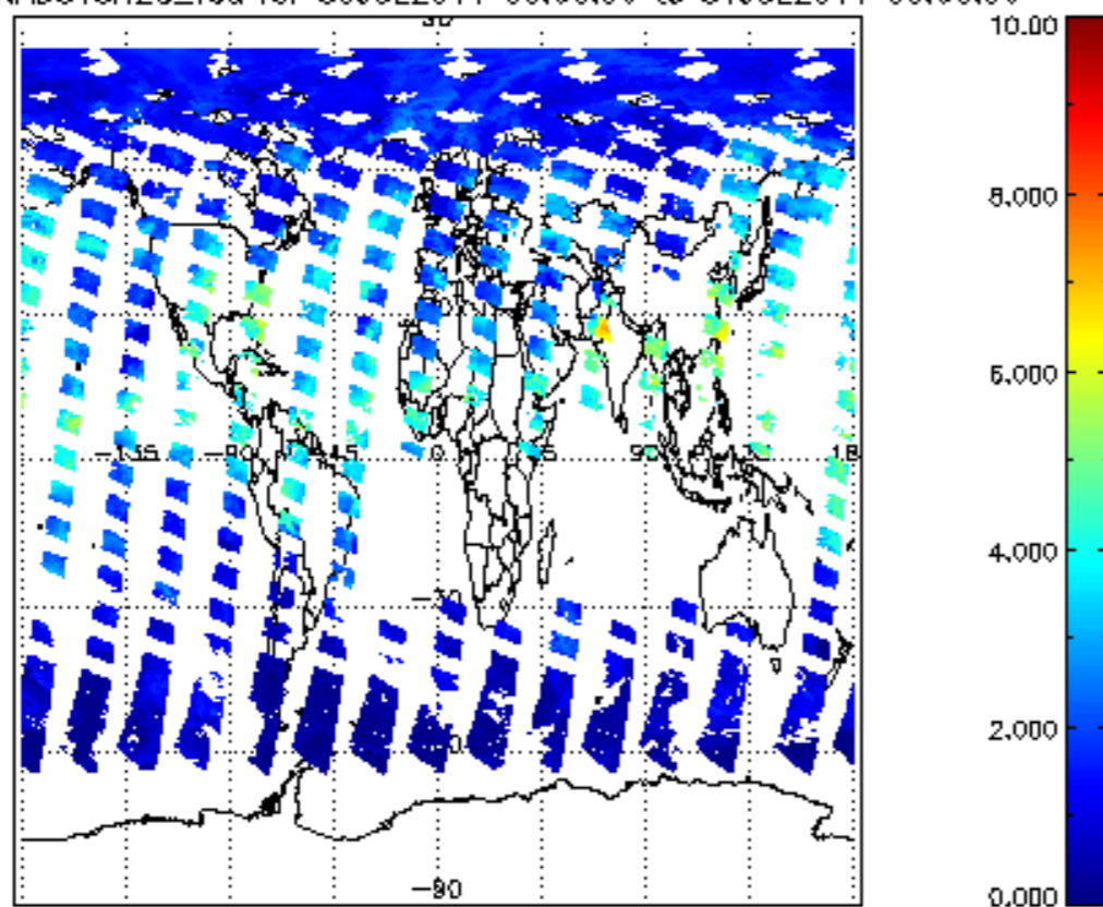
SCIOL2P_NADUV8H20_vcd for 30JUL2011 00:00:00 to 31JUL2011 00:00:00
