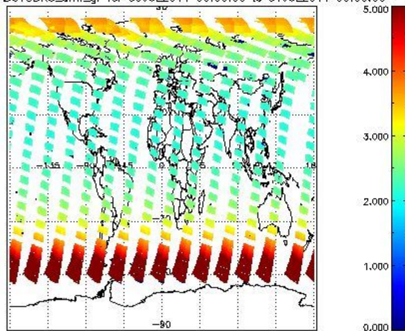
SCIOL2P_NADUV3BRO_amf_gr for 30JUL2011 00:00:00 to 31JUL2011 00:00:00
