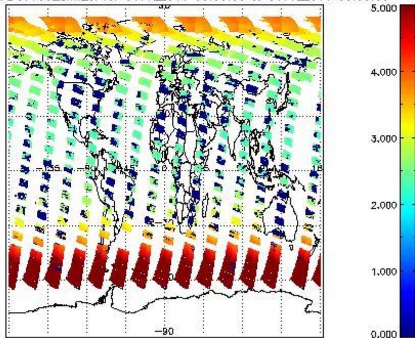
SCIOL2P_NADUV003_amf_cl for 30JUL2011 00:00:00 to 31JUL2011 00:00:00
