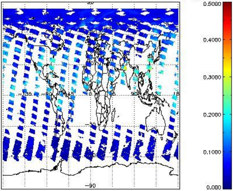
SCIOL2P_NADUV8H2O_vcd_err for 30JUL2011 00:00:00 to 31JUL2011 00:00:00
