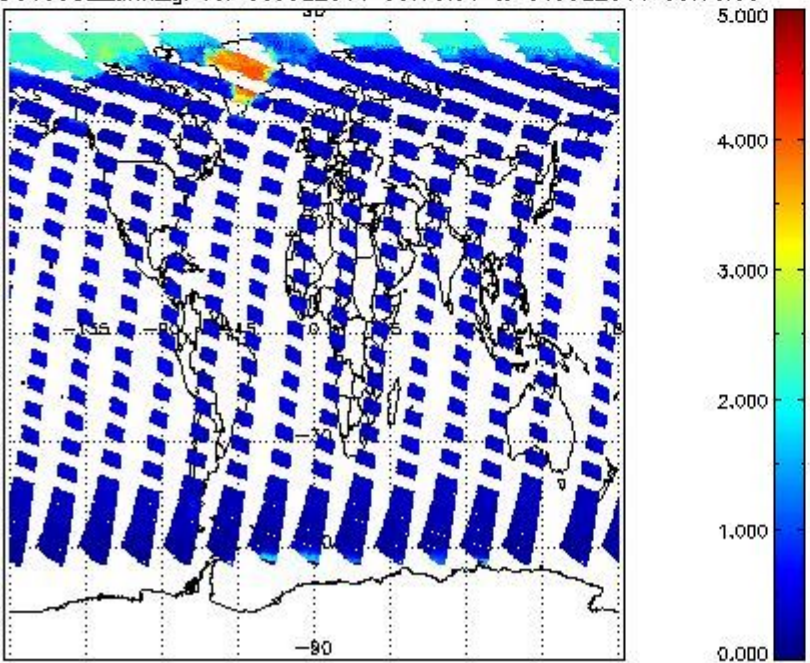
SCIOL2P_NADUV5S02_amf_gr for 30JUL2011 00:00:00 to 31JUL2011 00:00:00
