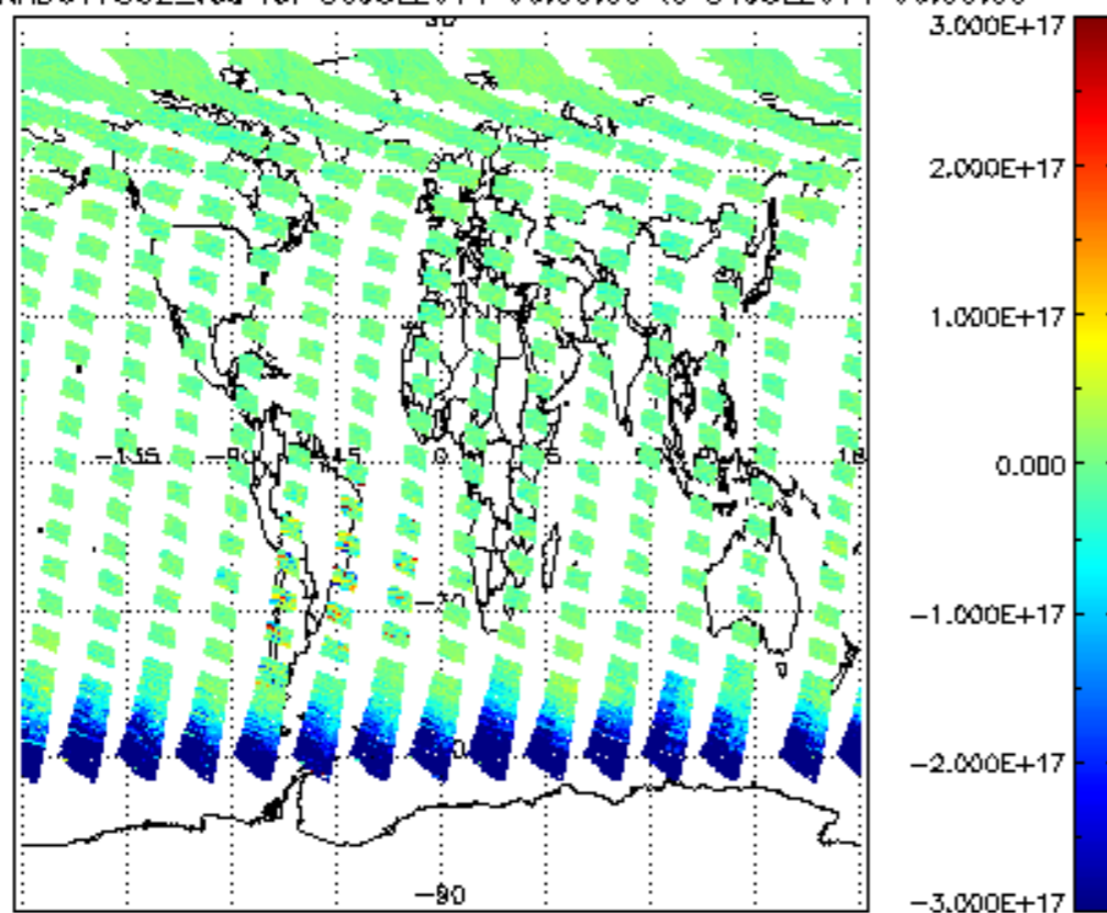
SCIOL2P_NADUV7S02_vcd for 30JUL2011 00:00:00 to 31JUL2011 00:00:00
