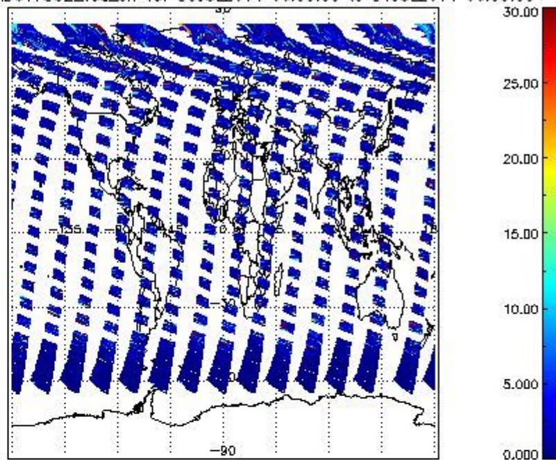
SCIOL2P_NADUV7S02_vcd_err for 30JUL2011 00:00:00 to 31JUL2011 00:00:00
