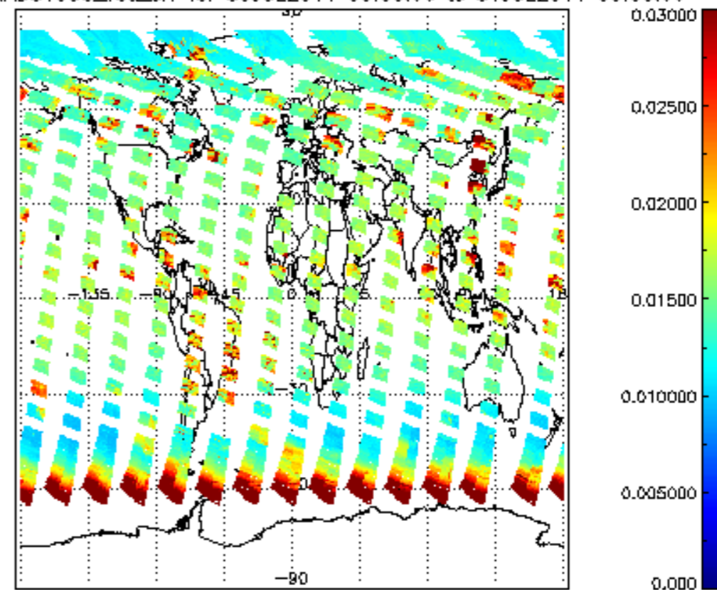
SCIOL2P_NADUV003_vcd_err for 30JUL2011 00:00:00 to 31JUL2011 00:00:00
