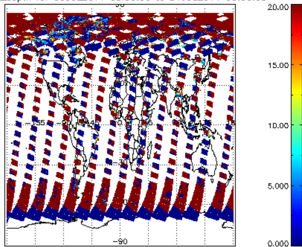
cl_lopt_depth for 30JUL2011 00:00:00 to 31JUL2011 00:00:00
