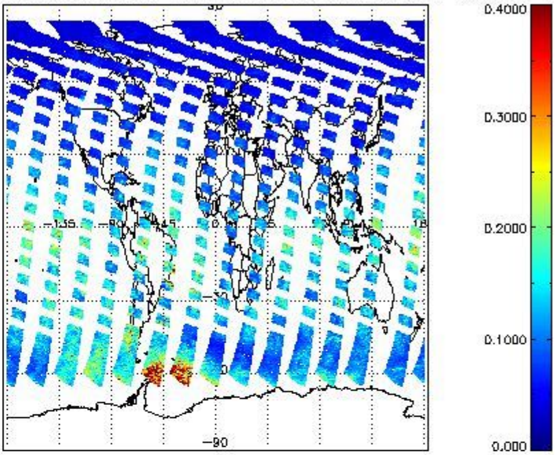
SCIOL2P_NADUV1NO2_vcd_err for 30JUL2011 00:00:00 to 31JUL2011 00:00:00
