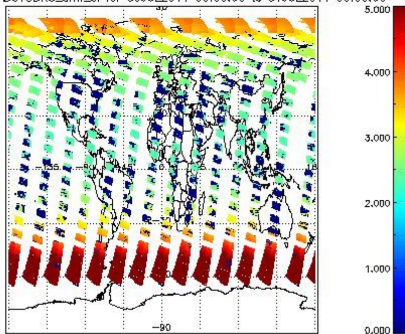
SCIOL2P_NADUV3BRO_amf_cl for 30JUL2011 00:00:00 to 31JUL2011 00:00:00
