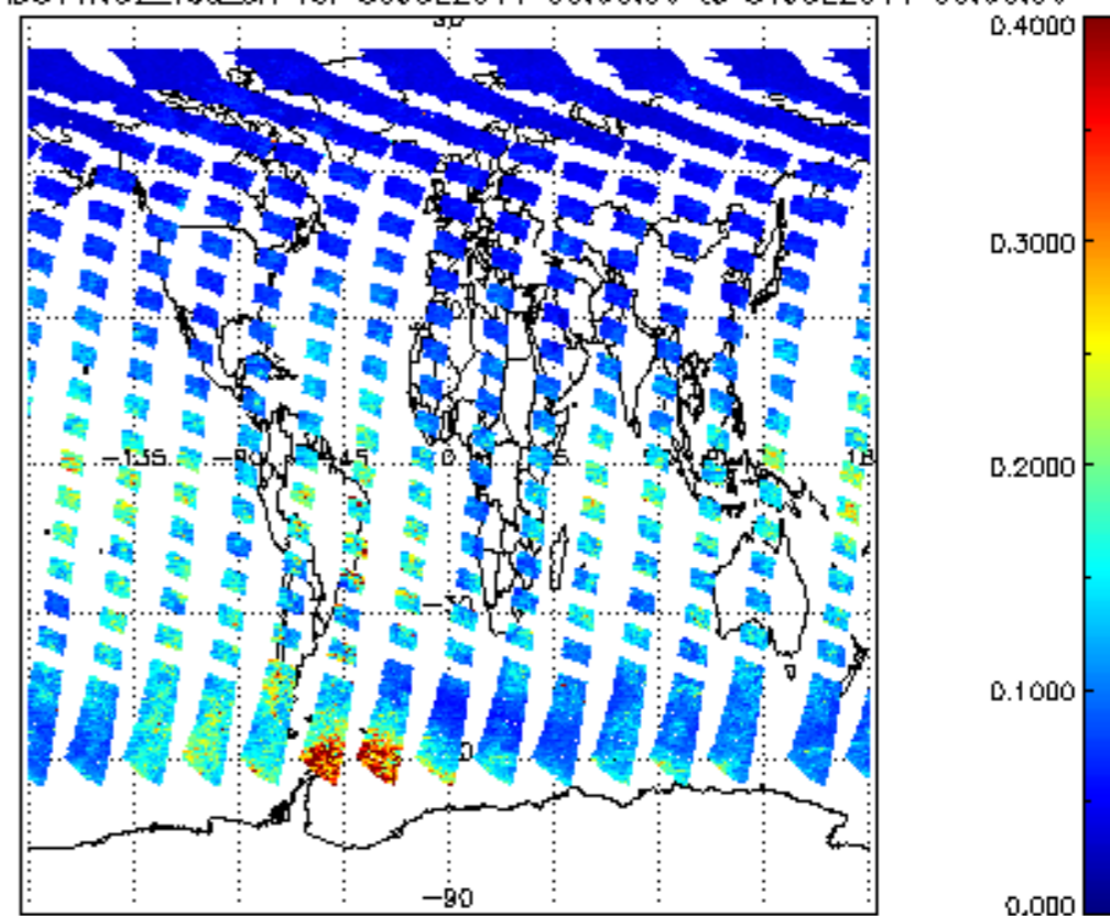
SCIOL2P_NADUV1NO2_vcd_err for 30JUL2011 00:00:00 to 31JUL2011 00:00:00
