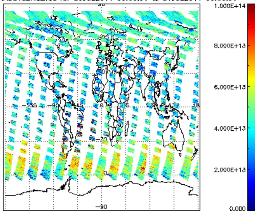
SCIOL2P_NADUV3BRO_vcd for 30JUL2011 00:00:00 to 31JUL2011 00:00:00
