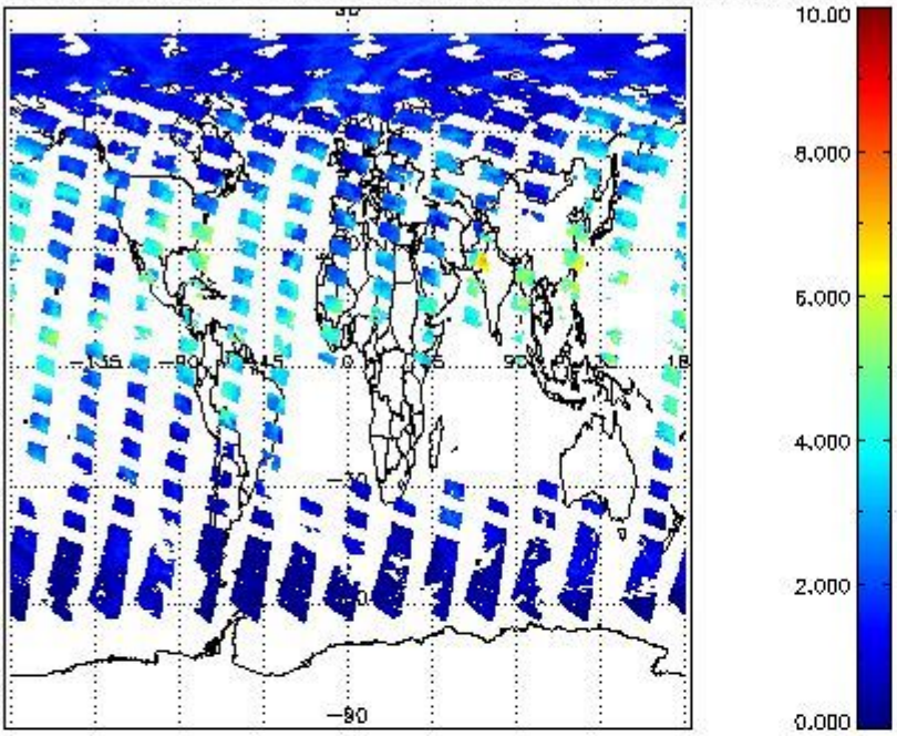
SCIOL2P_NADUV8H2O_vcd for 30JUL2011 00:00:00 to 31JUL2011 00:00:00
