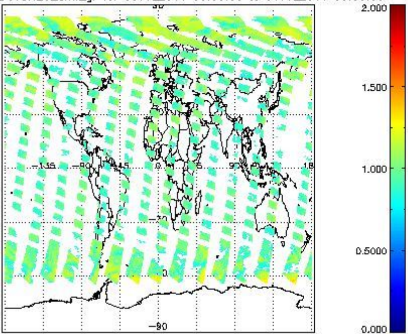
SCIOL2P_NADUV8H2O_amf_gr for 30JUL2011 00:00:00 to 31JUL2011 00:00:00
