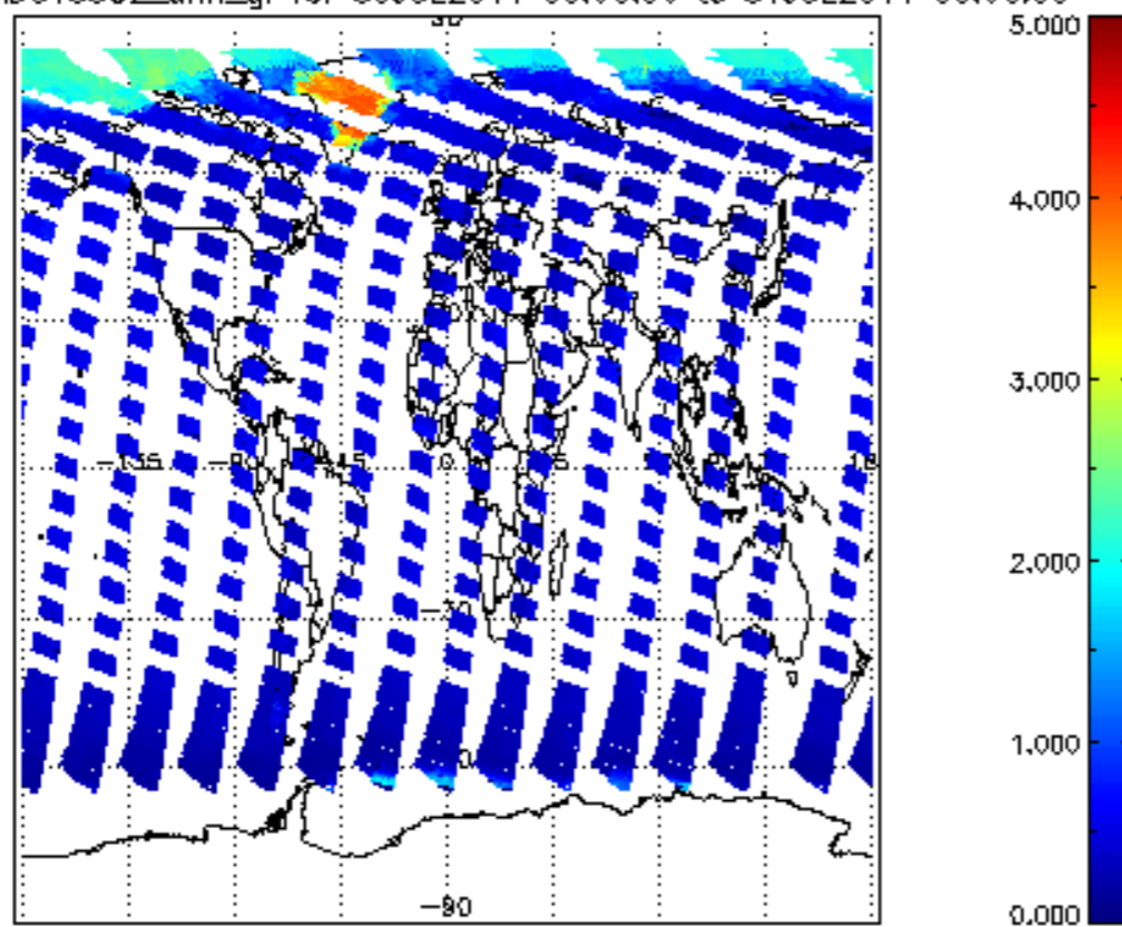
SCIOL2P_NADUV5S02_amf_gr for 30JUL2011 00:00:00 to 31JUL2011 00:00:00
