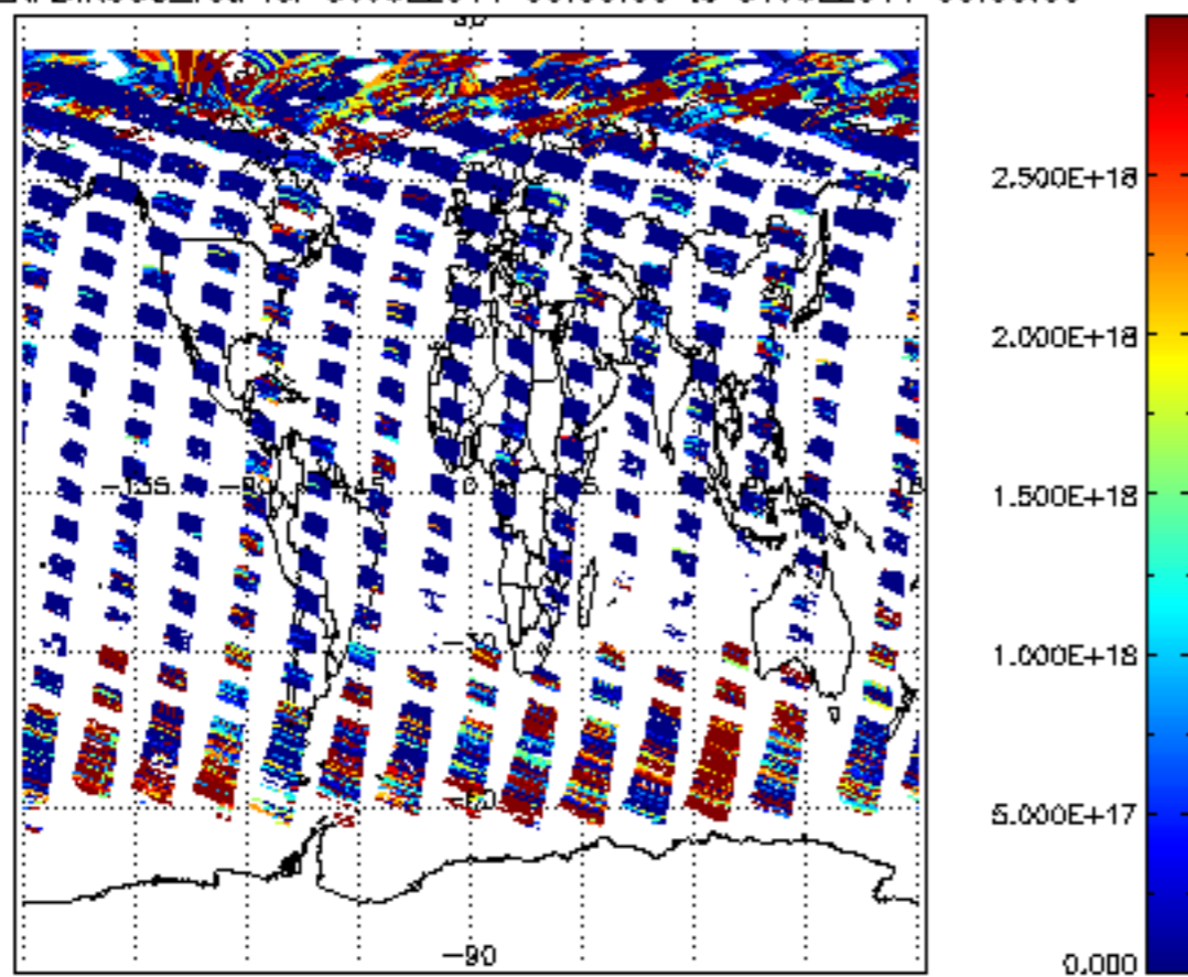
SCIOL2P_NADIR3CO_vcd for 30JUL2011 00:00:00 to 31JUL2011 00:00:00
