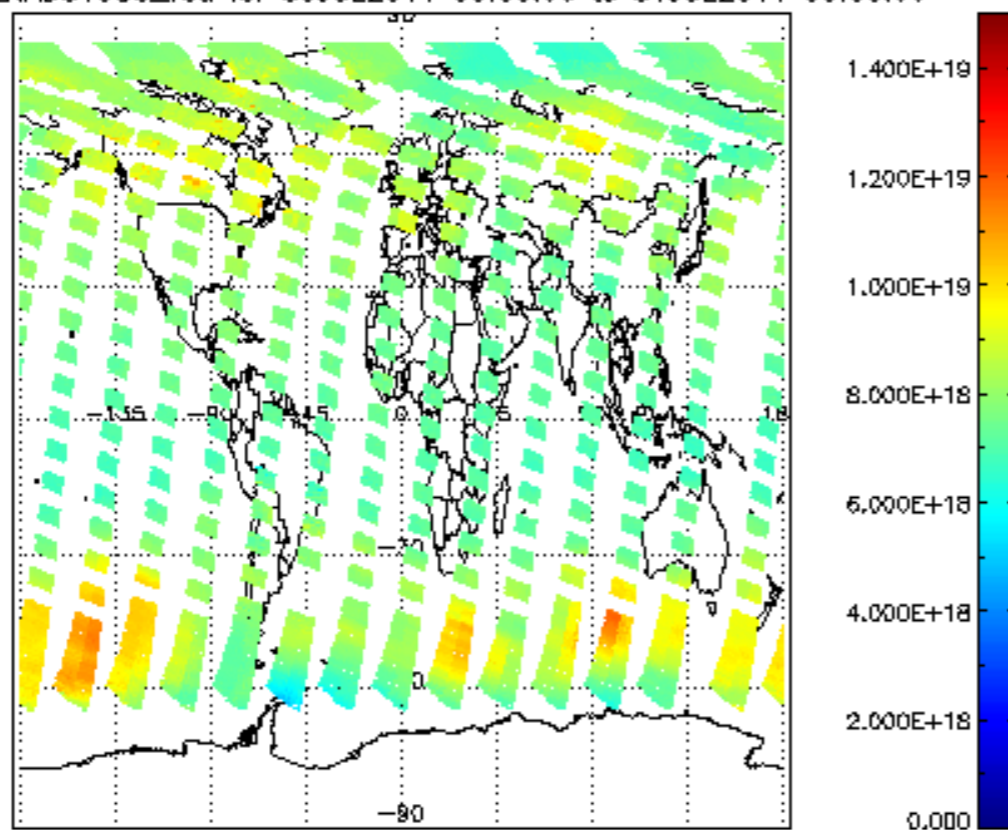
SCIOL2P_NADUV003_vcd for 30JUL2011 00:00:00 to 31JUL2011 00:00:00
