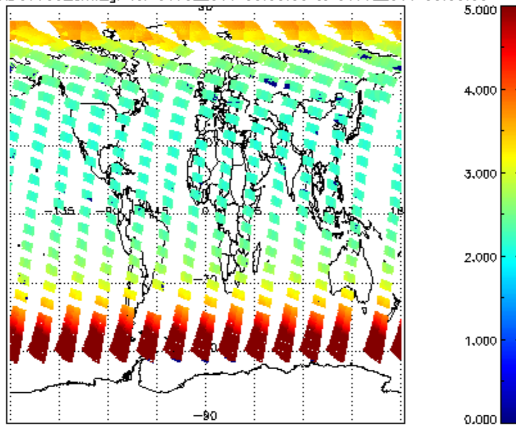
SCIOL2P_NADUV003_amf_gr for 30JUL2011 00:00:00 to 31JUL2011 00:00:00
