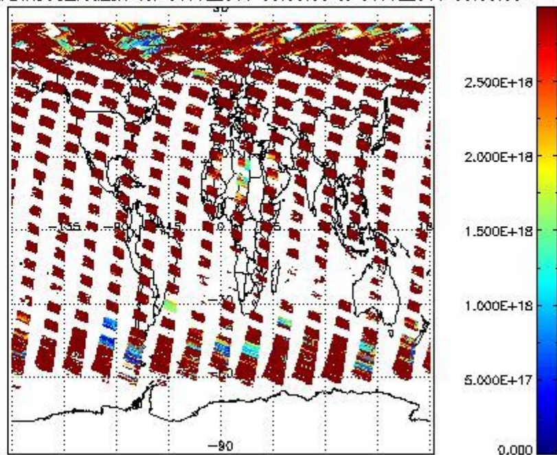
SCIDL2P_NADIR3CO_vcd_err for 30JUL2011 00:00:00 to 31JUL2011 00:00:00
