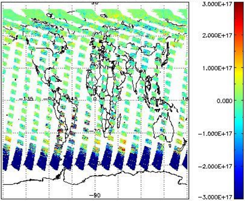
SCIOL2P_NADUV5S02_vcd for 30JUL2011 00:00:00 to 31JUL2011 00:00:00
