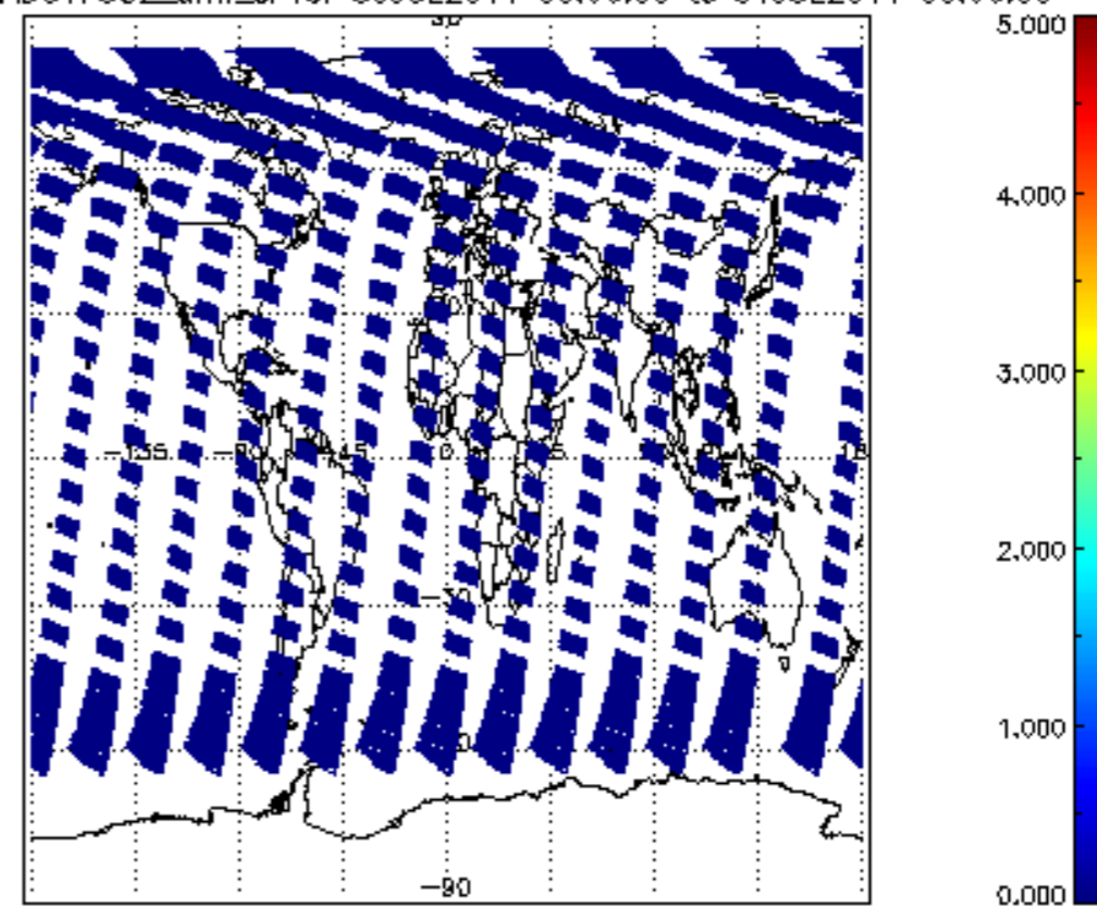
SCIOL2P_NADUV7S02_amf_cl for 30JUL2011 00:00:00 to 31JUL2011 00:00:00
