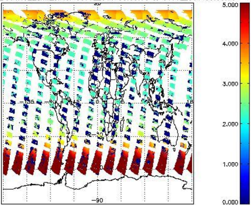
SCIOL2P_NADUV1NO2_amf_cl for 30JUL2011 00:00:00 to 31JUL2011 00:00:00
