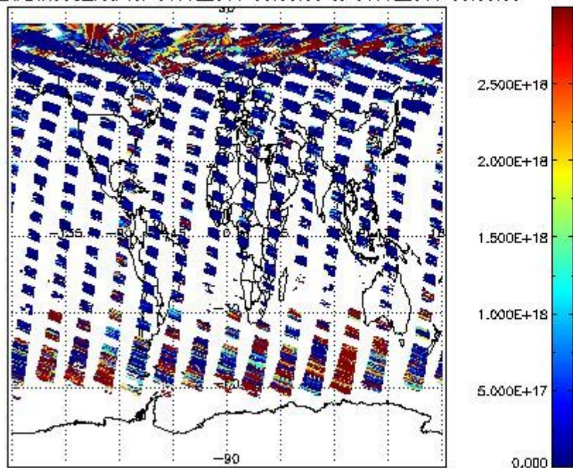
SCIDL2P_NADIR3CO_vcd for 30JUL2011 00:00:00 to 31JUL2011 00:00:00
