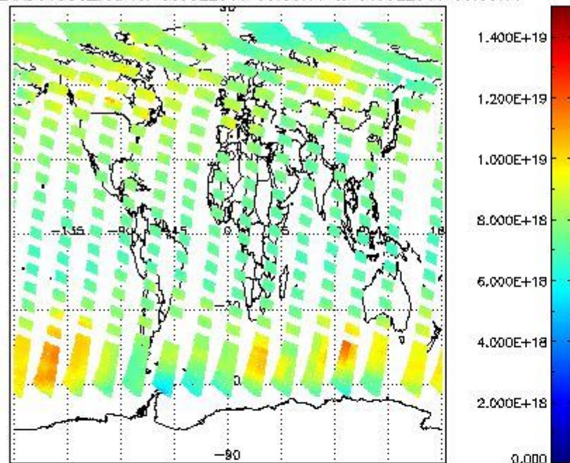
SCIOL2P_NADUV003_vcd for 30JUL2011 00:00:00 to 31JUL2011 00:00:00
