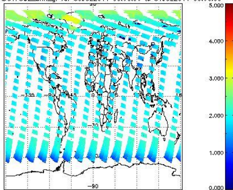
SCIOL2P_NADUV7S02_amf_gr for 30JUL2011 00:00:00 to 31JUL2011 00:00:00
