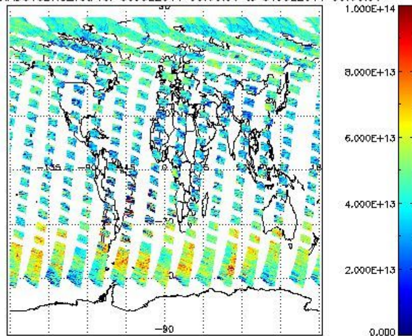
SCIOL2P_NADUV3BRO_vcd for 30JUL2011 00:00:00 to 31JUL2011 00:00:00
