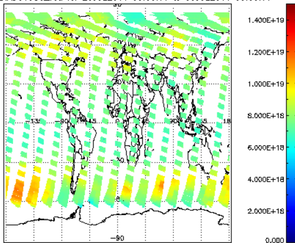
SCIOL2P_NADUV003_vcd for 29JUL2011 00:00:00 to 30JUL2011 00:00:00
