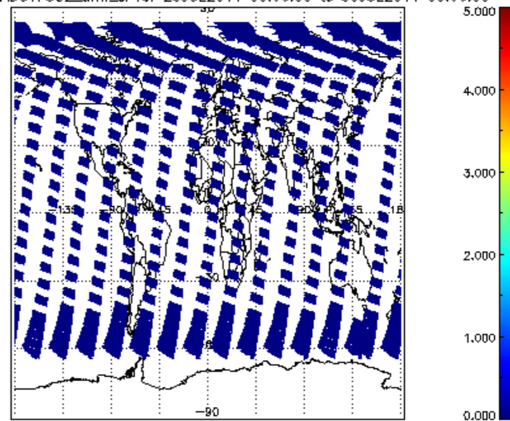
SCIOL2P_NADUV7S02_amf_cl for 29JUL2011 00:00:00 to 30JUL2011 00:00:00
