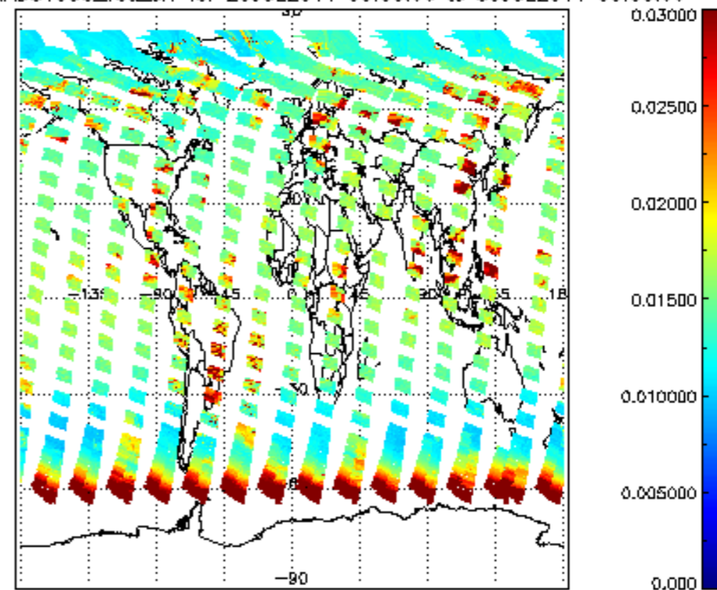
SCIOL2P_NADUV003_vcd_err for 29JUL2011 00:00:00 to 30JUL2011 00:00:00
