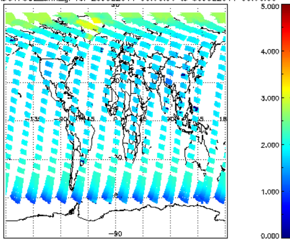
SCIOL2P_NADUV7S02_amf_gr for 29JUL2011 00:00:00 to 30JUL2011 00:00:00
