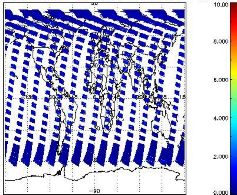
SCIOL2P_NADUV3BRO_vcd_err for 29JUL2011 00:00:00 to 30JUL2011 00:00:00
