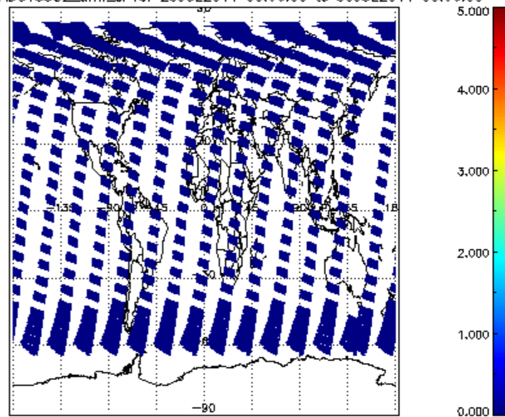
SCIOL2P_NADUV5S02_amf_cl for 29JUL2011 00:00:00 to 30JUL2011 00:00:00
