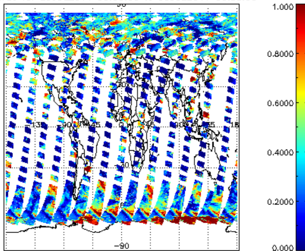
cl_frac for 29JUL2011 00:00:00 to 30JUL2011 00:00:00
