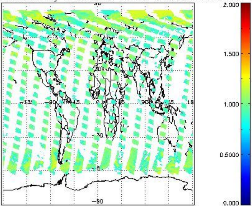
SCIOL2P_NADUV8H2O_amf_gr for 29JUL2011 00:00:00 to 30JUL2011 00:00:00
