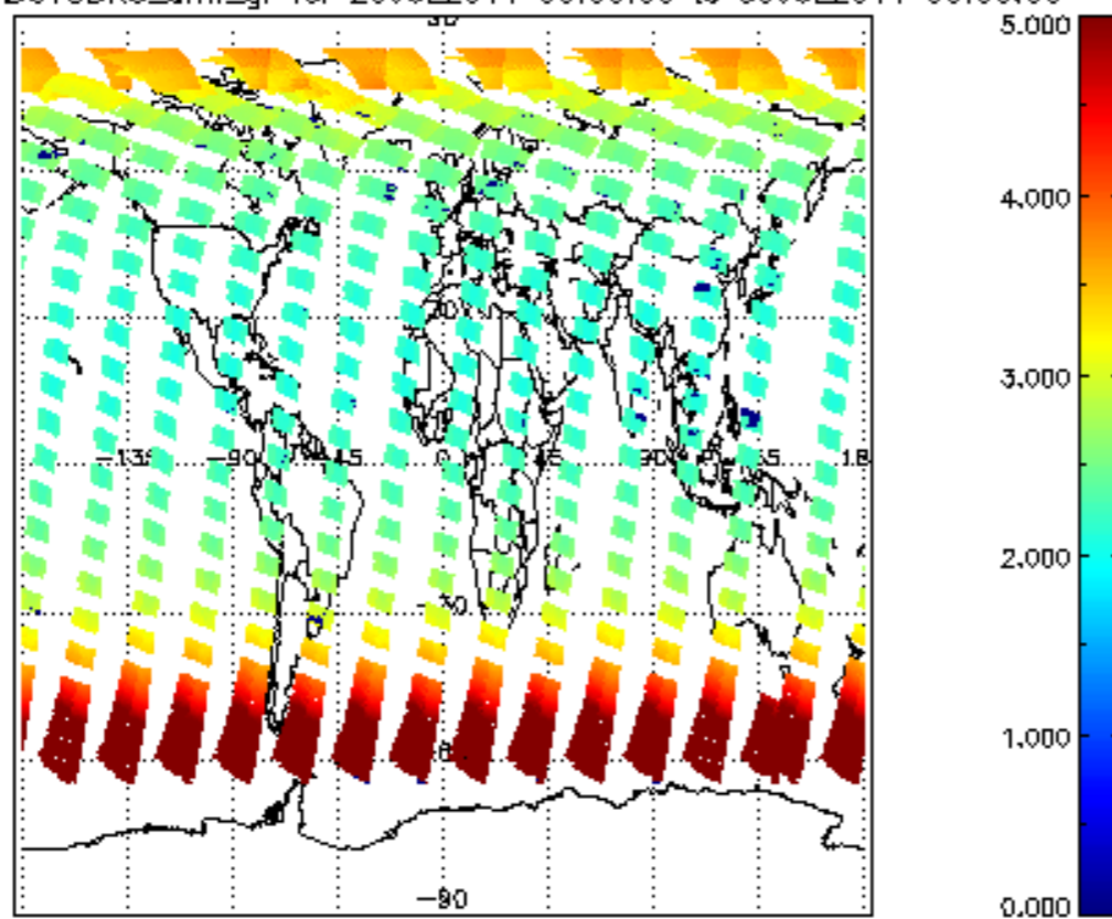
SCIOL2P_NADUV3BRO_arnf_gr for 29JUL2011 00:00:00 to 30JUL2011 00:00:00
