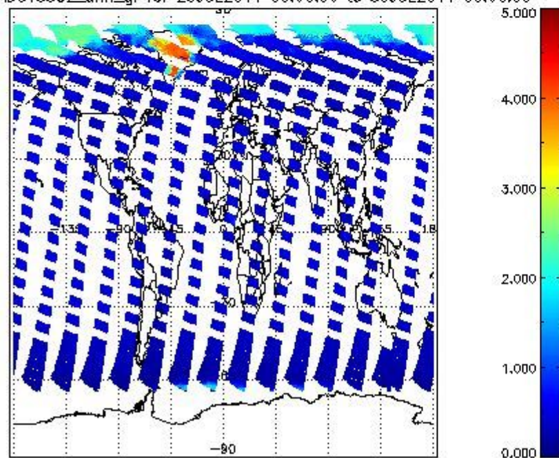
SCIOL2P_NADUV5S02_amf_gr for 29JUL2011 00:00:00 to 30JUL2011 00:00:00
