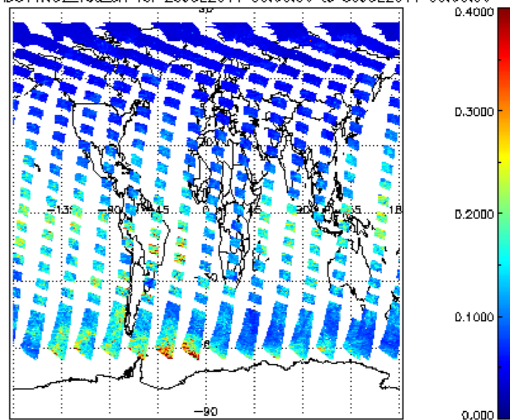
SCIOL2P_NADUV1N02_vcd_err for 29JUL2011 00:00:00 to 30JUL2011 00:00:00
