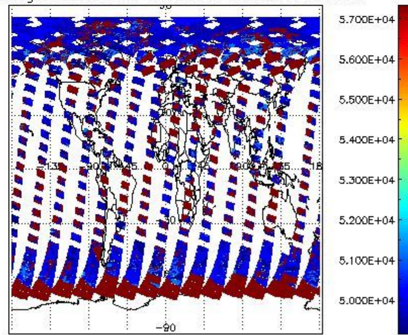
cloud_flags for 29JUL2011 00:00:00 to 30JUL2011 00:00:00
