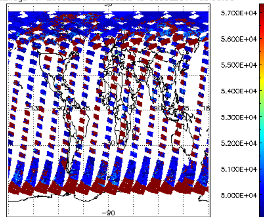
cloud_flags for 29JUL2011 00:00:00 to 30JUL2011 00:00:00
