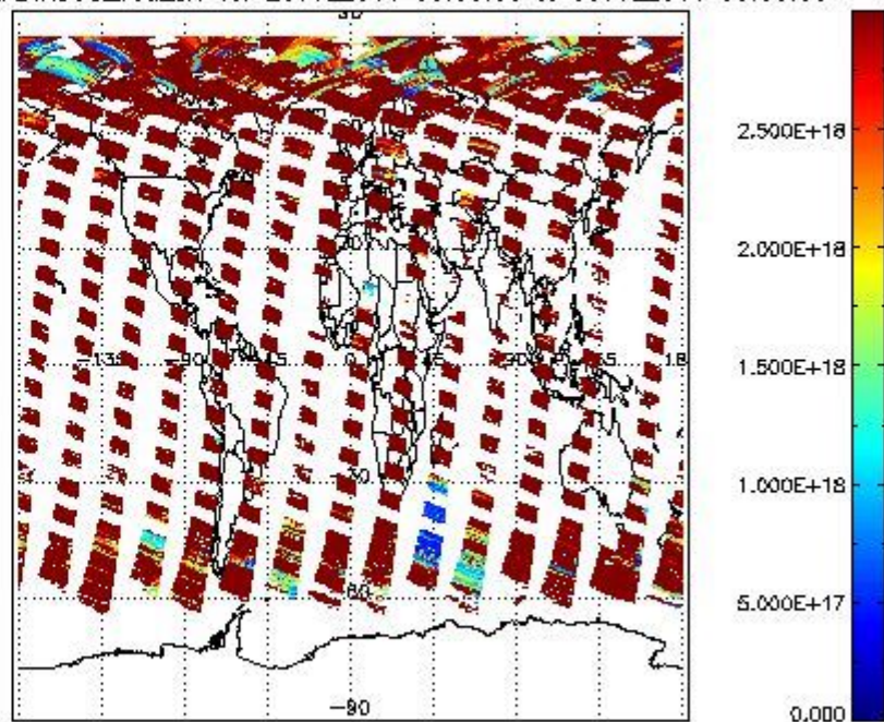
SCIOL2P_NADIR3CO_vcd_err for 29JUL2011 00:00:00 to 30JUL2011 00:00:00
