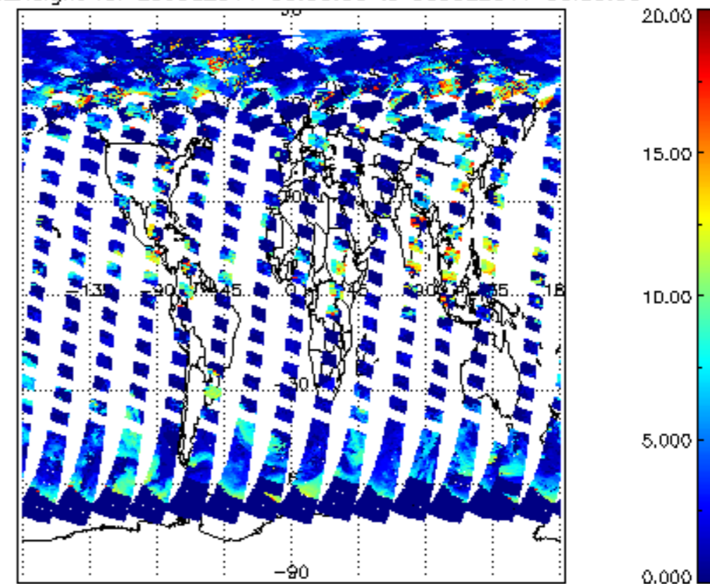
cl_top_height for 29JUL2011 00:00:00 to 30JUL2011 00:00:00
