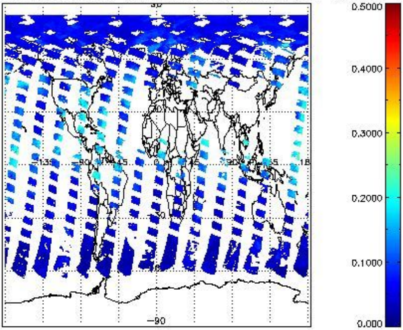
SCIOL2P_NADUV8H2O_vcd_err for 29JUL2011 00:00:00 to 30JUL2011 00:00:00
