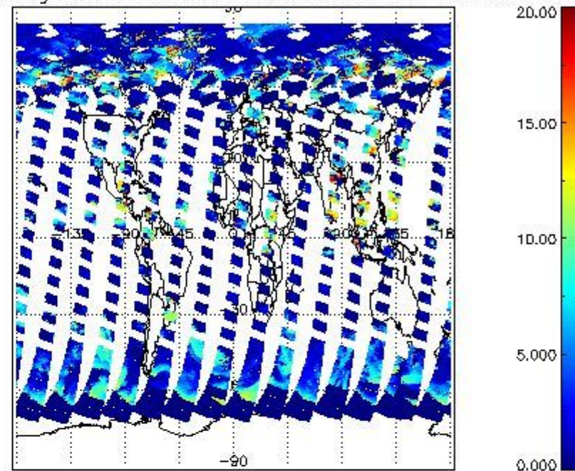
cL_top_height for 29JUL2011 00:00:00 to 30JUL2011 00:00:00
