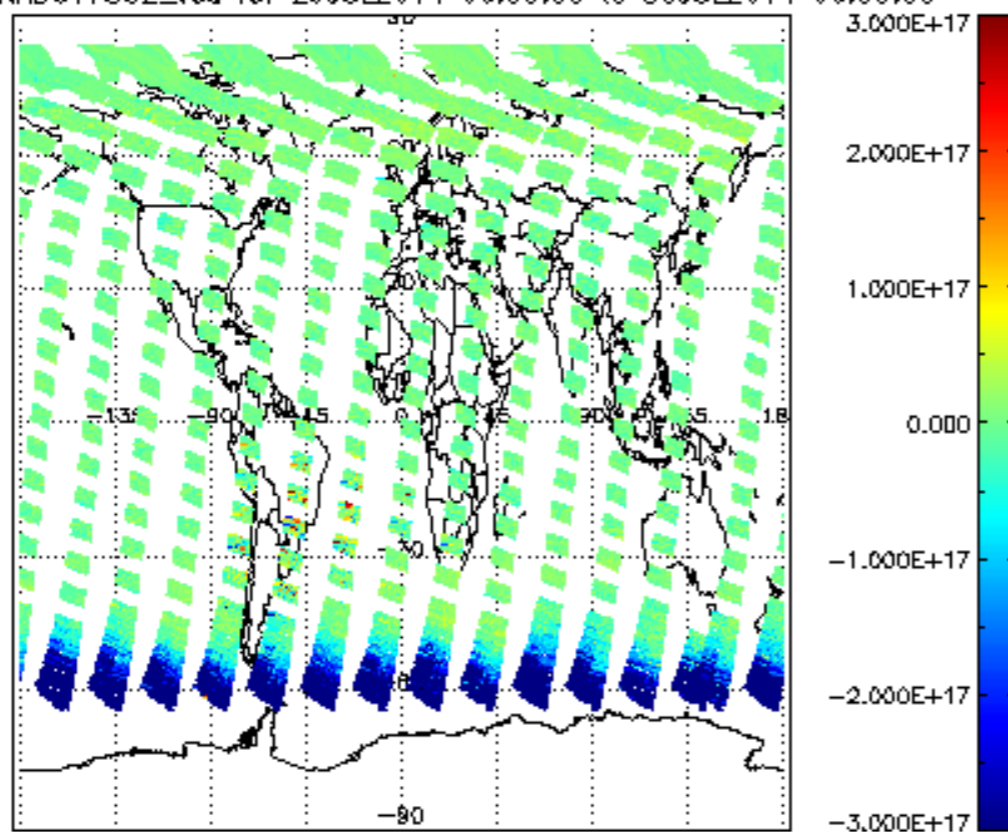
SCIOL2P_NADUV7S02_vcd for 29JUL2011 00:00:00 to 30JUL2011 00:00:00
