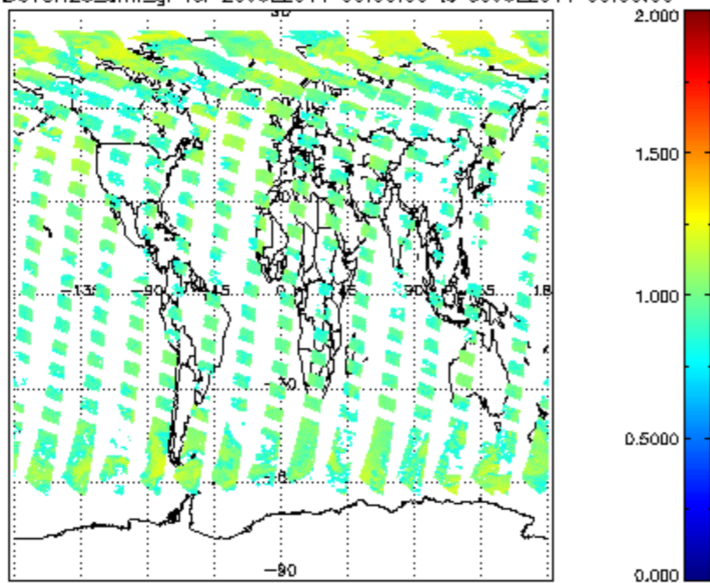
SCIOL2P_NADUV8H2O_amf_gr for 29JUL2011 00:00:00 to 30JUL2011 00:00:00
