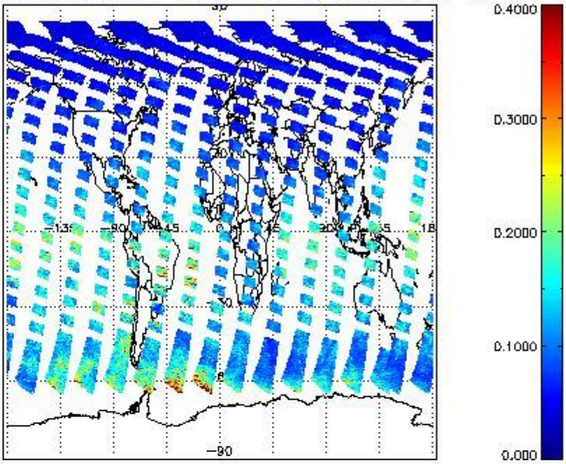
SCIOL2P_NADUV1NO2_vcd_err for 29JUL2011 00:00:00 to 30JUL2011 00:00:00
