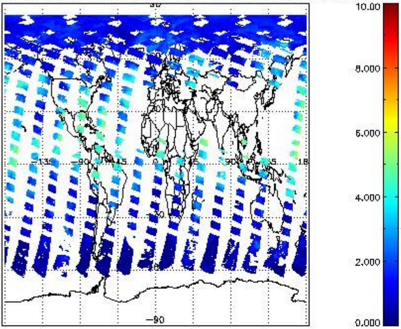
SCIOL2P_NADUV8H2O_vcd for 29JUL2011 00:00:00 to 30JUL2011 00:00:00
