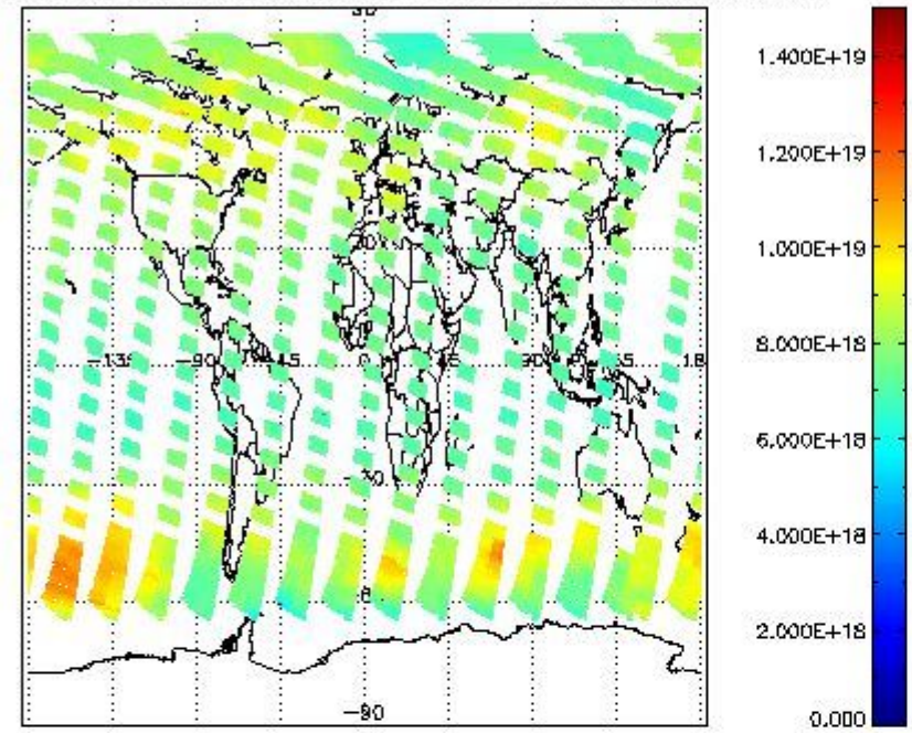
SCIOL2P_NADUV003_vcd for 29JUL2011 00:00:00 to 30JUL2011 00:00:00
