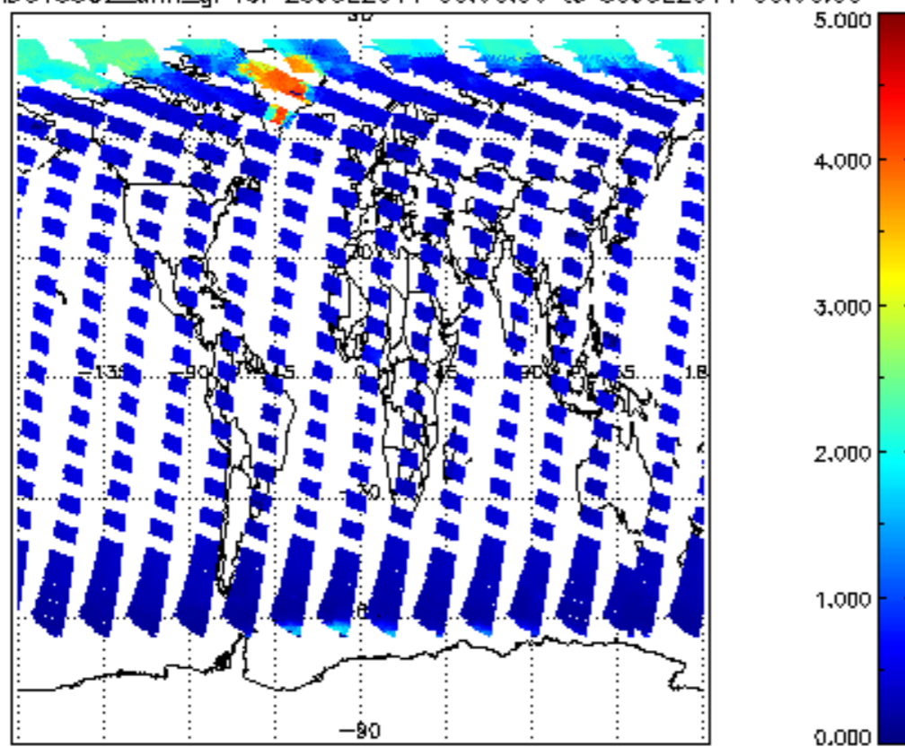
SCIOL2P_NADUV5S02_amf_gr for 29JUL2011 00:00:00 to 30JUL2011 00:00:00
