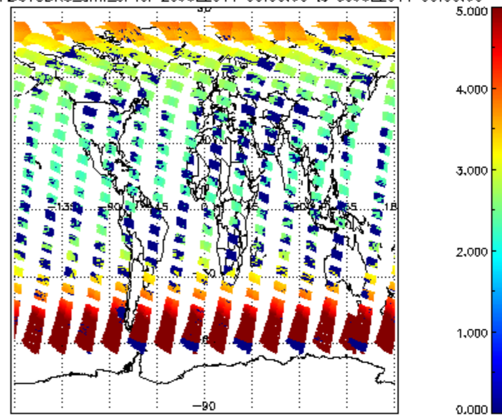
SCIOL2P_NADUV3BRO_arnf_cl for 29JUL2011 00:00:00 to 30JUL2011 00:00:00
