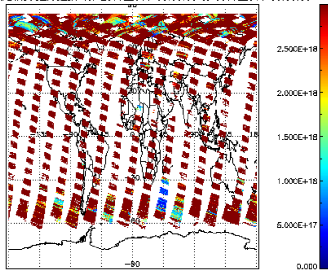
SCIOL2P_NADIR3CO_vcd_err for 29JUL2011 00:00:00 to 30JUL2011 00:00:00
