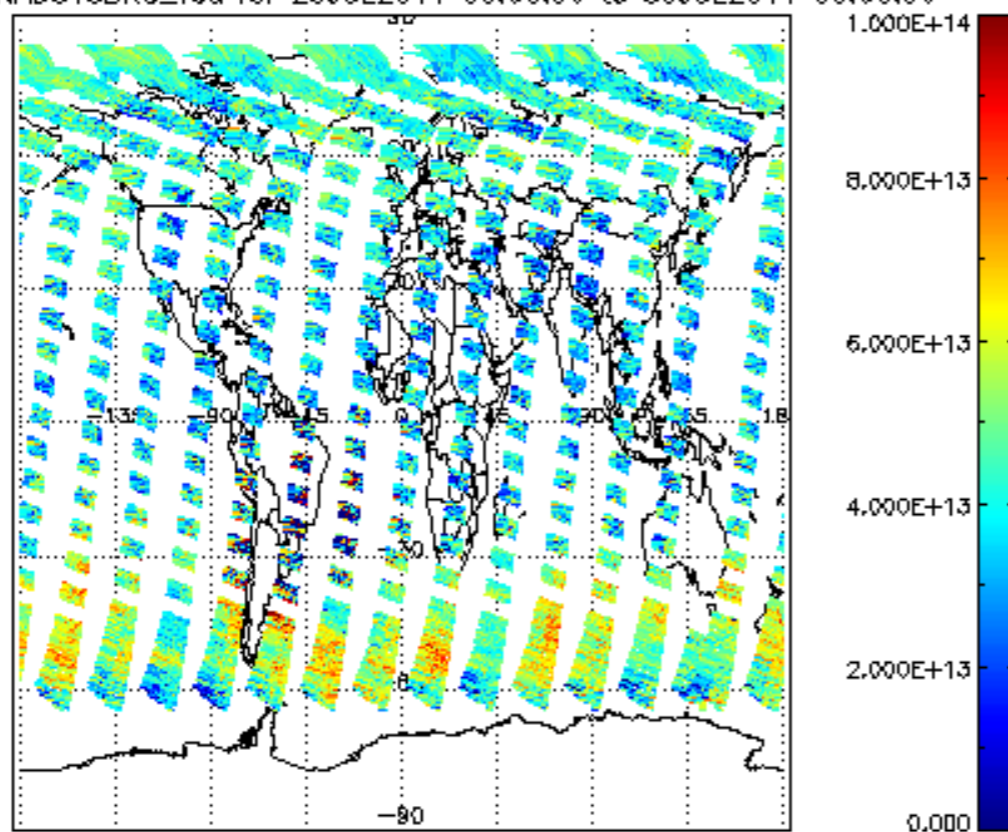
SCIOL2P_NADUV3BRO_vcd for 29JUL2011 00:00:00 to 30JUL2011 00:00:00
