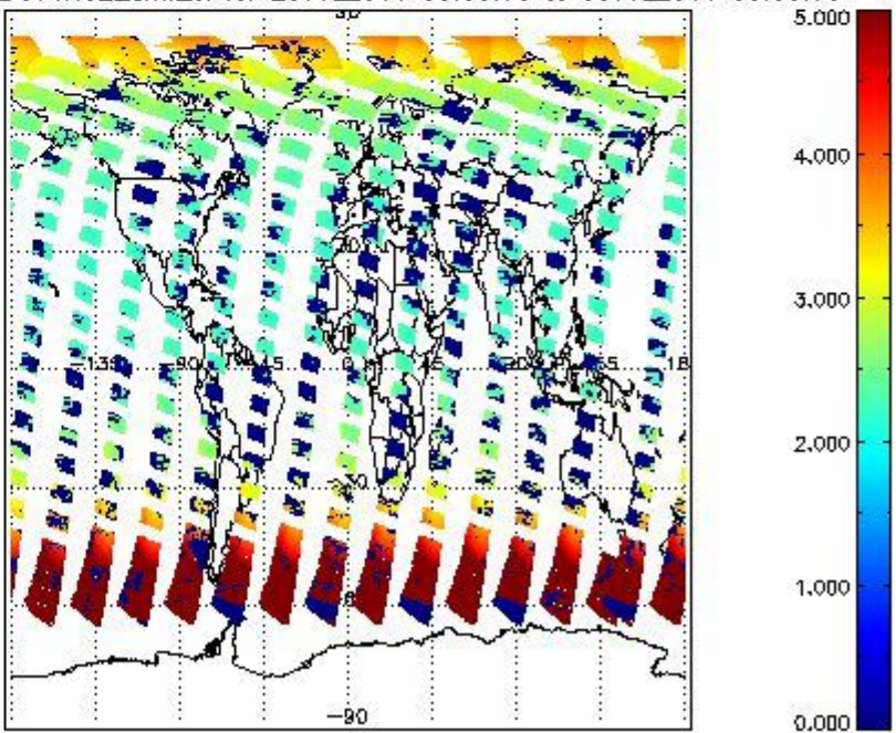
SCIOL2P_NADUV1NO2_amf_cl for 29JUL2011 00:00:00 to 30JUL2011 00:00:00
