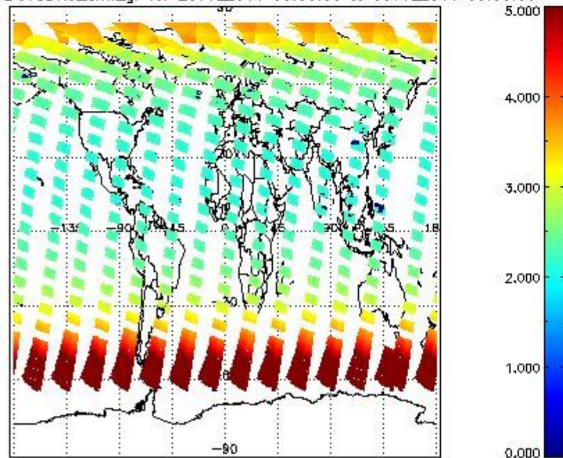
SCIOL2P_NADUV3BRO_amf_gr for 29JUL2011 00:00:00 to 30JUL2011 00:00:00
