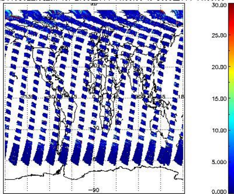
SCIOL2P_NADUV5S02_vcd_err for 29JUL2011 00:00:00 to 30JUL2011 00:00:00
