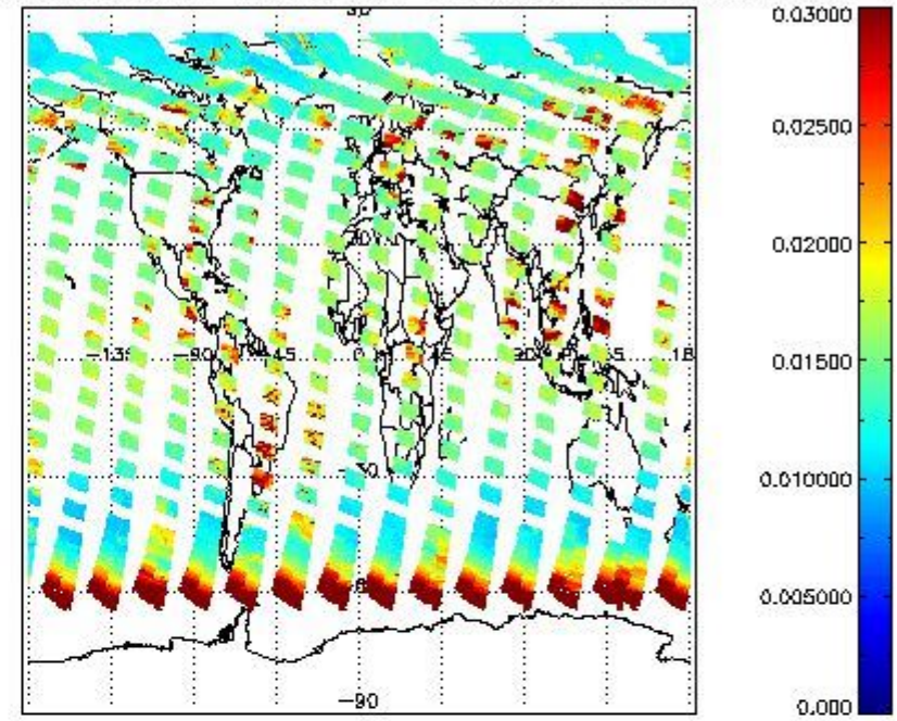
SCIOL2P_NADUV003_vcd_err for 29JUL2011 00:00:00 to 30JUL2011 00:00:00
