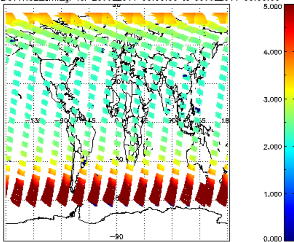
SCIOL2P_NADUV1N02_amf_gr for 29JUL2011 00:00:00 to 30JUL2011 00:00:00
