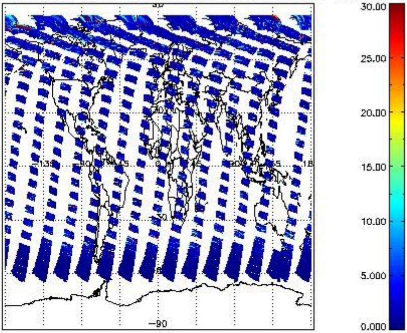
SCIOL2P_NADUV7S02_vcd_err for 29JUL2011 00:00:00 to 30JUL2011 00:00:00
