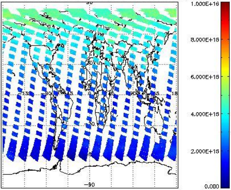
SCIOL2P_NADUV1NO2_vcd for 29JUL2011 00:00:00 to 30JUL2011 00:00:00
