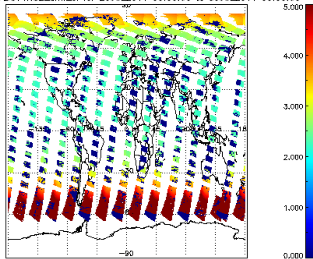
SCIOL2P_NADUV1N02_amf_cl for 29JUL2011 00:00:00 to 30JUL2011 00:00:00
