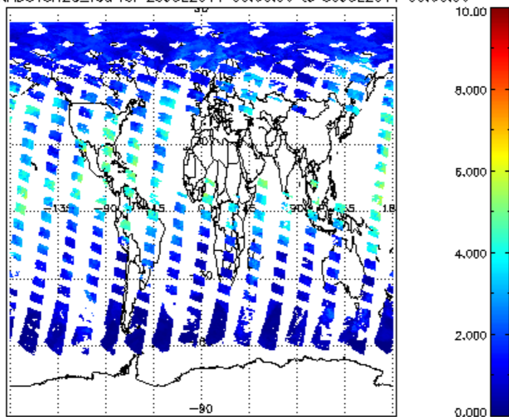
SCIOL2P_NADUV8H2O_vcd for 29JUL2011 00:00:00 to 30JUL2011 00:00:00
