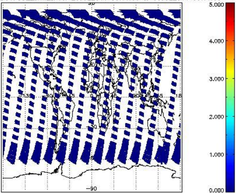
SCIOL2P_NADUV7S02_amf_cl for 29JUL2011 00:00:00 to 30JUL2011 00:00:00
