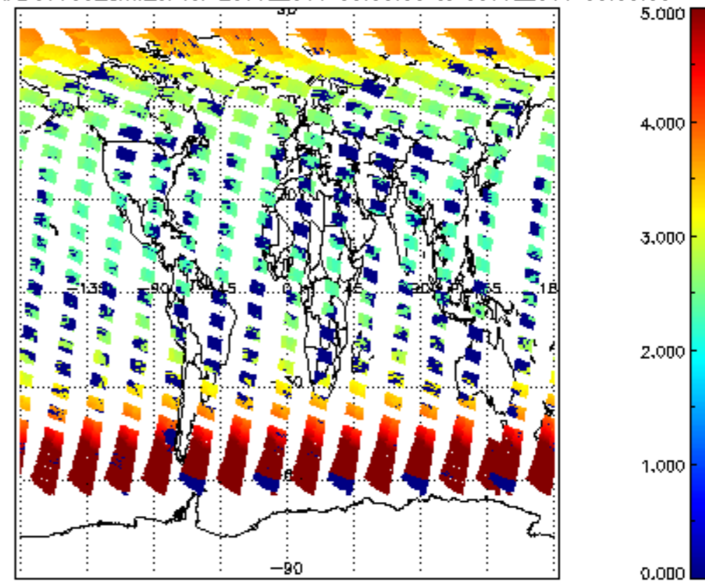
SCIOL2P_NADUV003_amf_cl for 29JUL2011 00:00:00 to 30JUL2011 00:00:00
