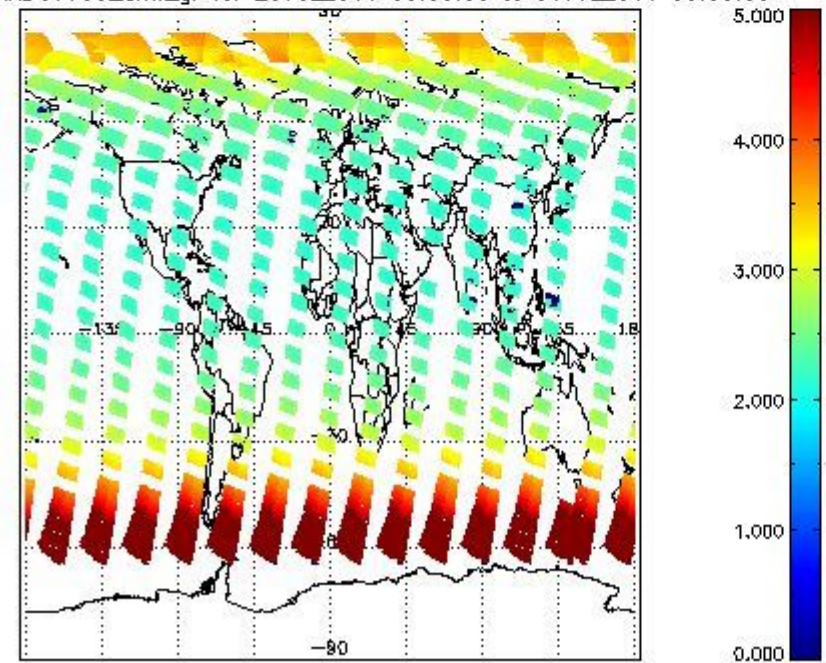
SCIOL2P_NADUV003_amf_gr for 29JUL2011 00:00:00 to 30JUL2011 00:00:00
