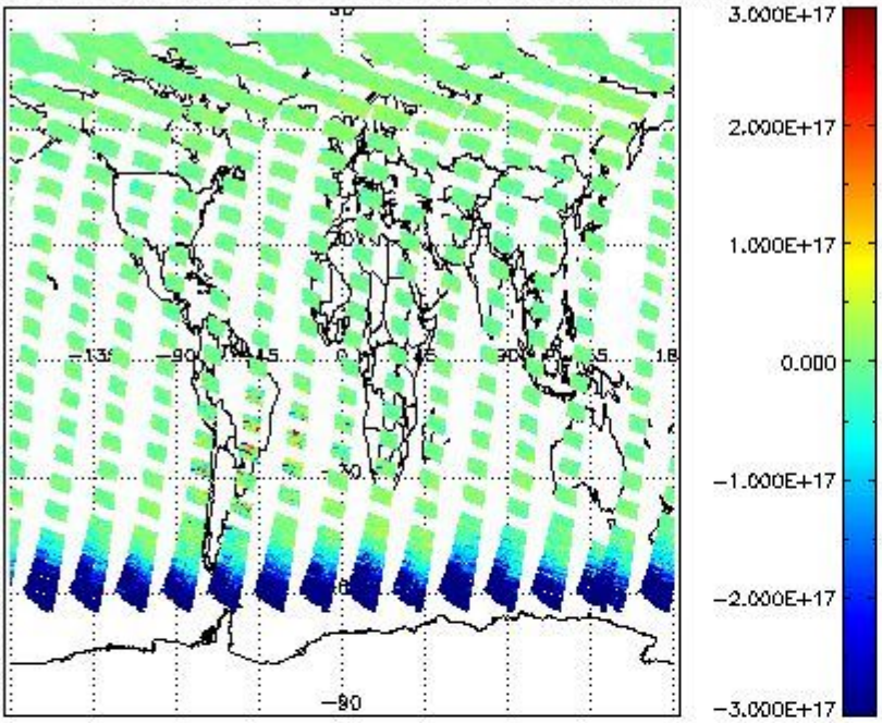
SCIOL2P_NADUV7S02_vcd for 29JUL2011 00:00:00 to 30JUL2011 00:00:00
