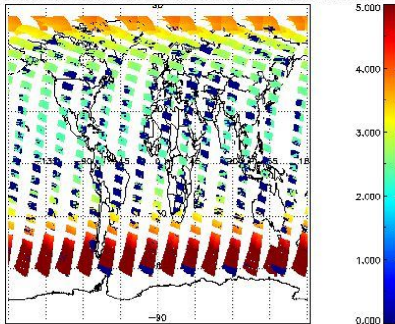
SCIOL2P_NADUV3BRO_amf_cl for 29JUL2011 00:00:00 to 30JUL2011 00:00:00
