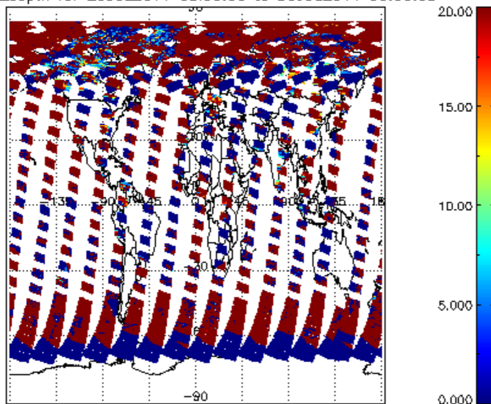
cl_lopt_depth for 29JUL2011 00:00:00 to 30JUL2011 00:00:00
