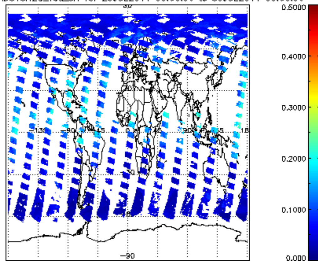
SCIOL2P_NADUV8H2O_vcd_err for 29JUL2011 00:00:00 to 30JUL2011 00:00:00
