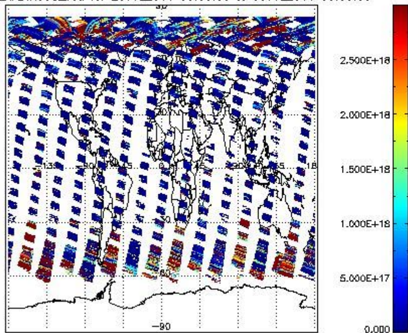
SCIOL2P_NADIR3CO_vcd for 29JUL2011 00:00:00 to 30JUL2011 00:00:00
