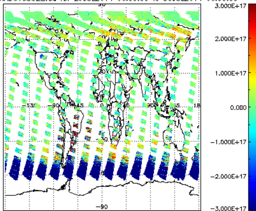
SCIOL2P_NADUV5S02_vcd for 29JUL2011 00:00:00 to 30JUL2011 00:00:00
