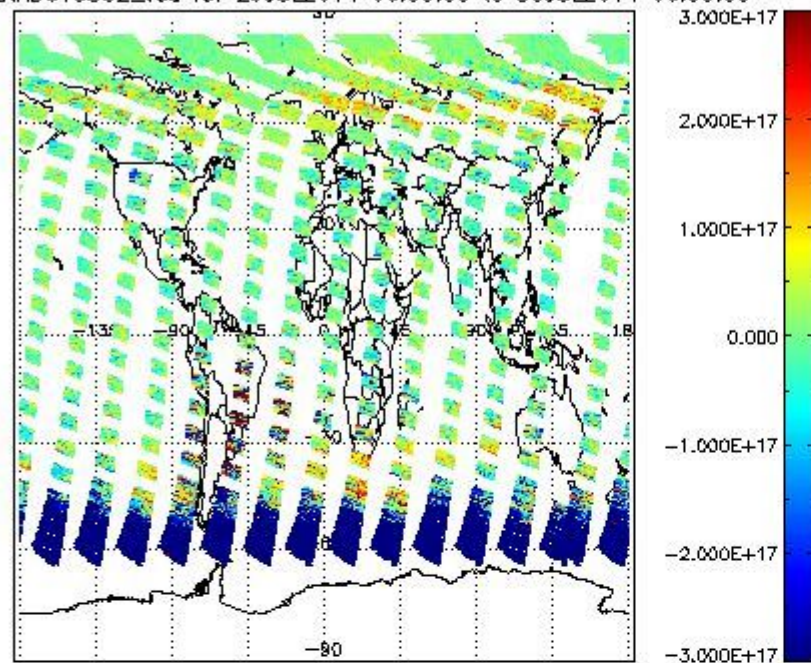
SCIOL2P_NADUV5S02_vcd for 29JUL2011 00:00:00 to 30JUL2011 00:00:00
