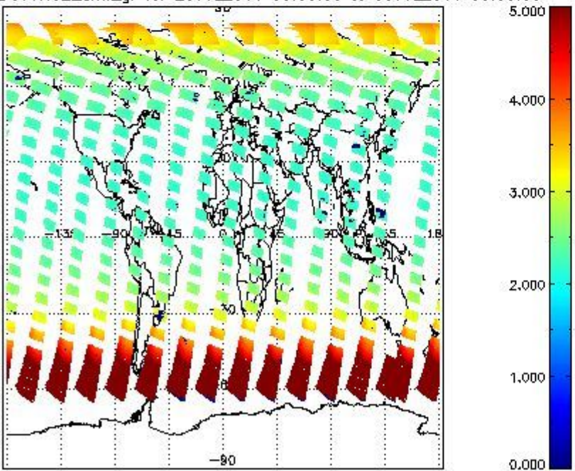
SCIOL2P_NADUV1NO2_amf_gr for 29JUL2011 00:00:00 to 30JUL2011 00:00:00
