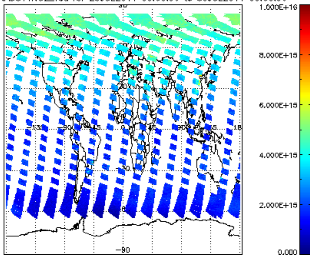
SCIOL2P_NADUV1N02_vcd for 29JUL2011 00:00:00 to 30JUL2011 00:00:00
