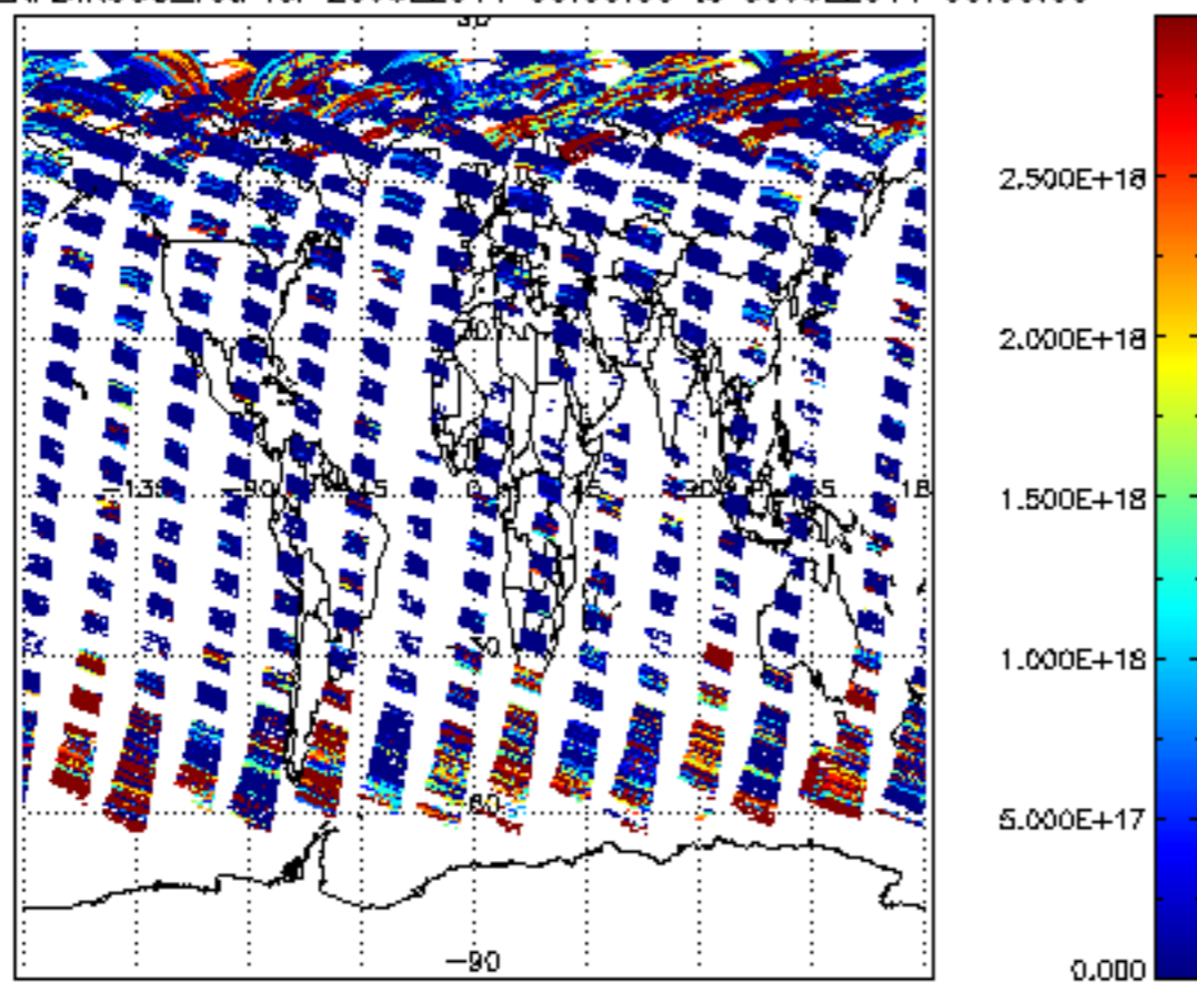
SCIOL2P_NADIR3CO_vcd for 29JUL2011 00:00:00 to 30JUL2011 00:00:00
