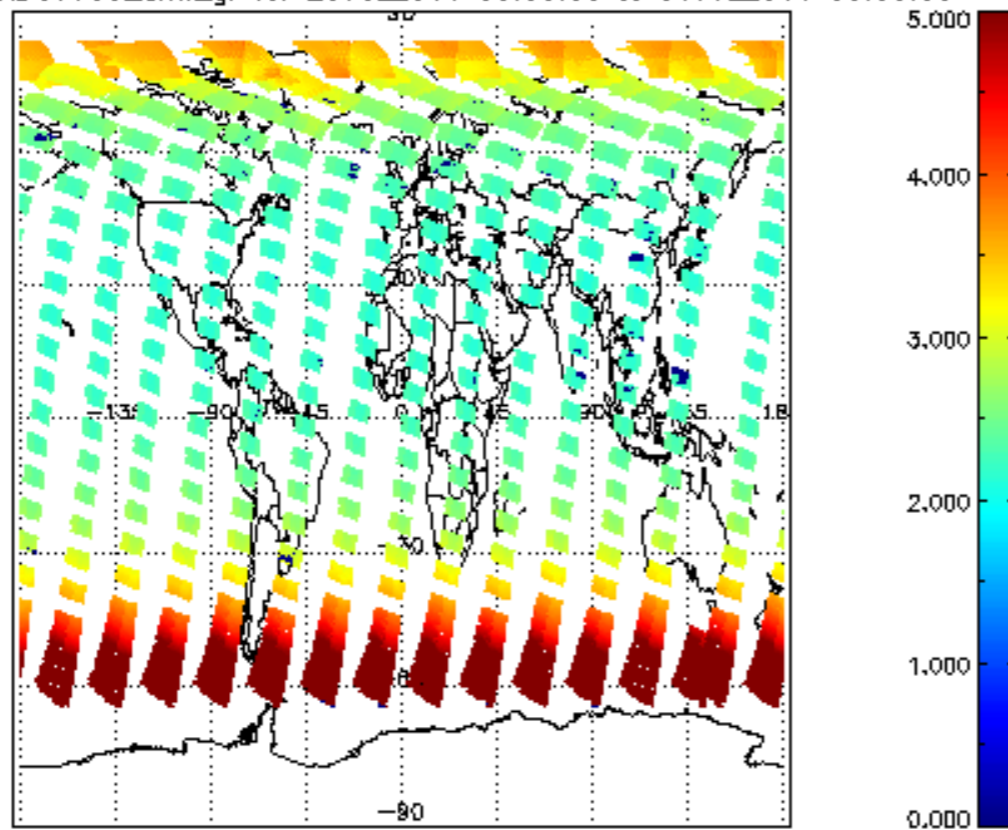
SCIOL2P_NADUV003_amf_gr for 29JUL2011 00:00:00 to 30JUL2011 00:00:00
