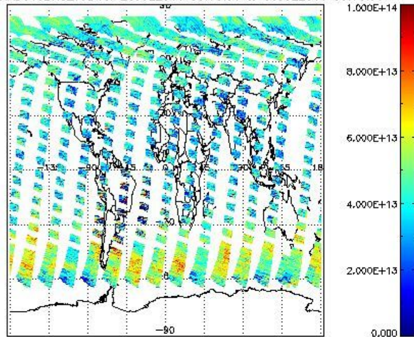
SCIOL2P_NADUV3BRO_vcd for 29JUL2011 00:00:00 to 30JUL2011 00:00:00
