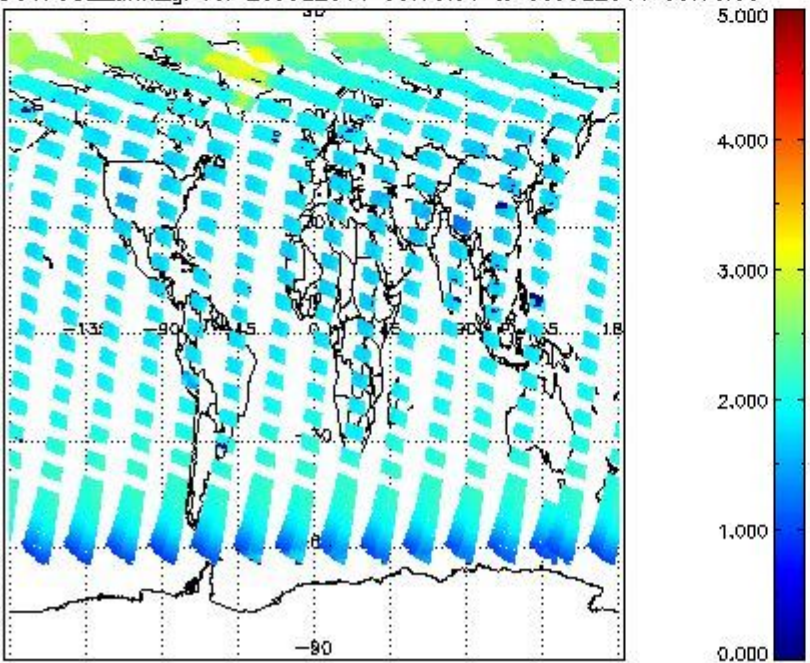
SCIOL2P_NADUV7S02_amf_gr for 29JUL2011 00:00:00 to 30JUL2011 00:00:00
