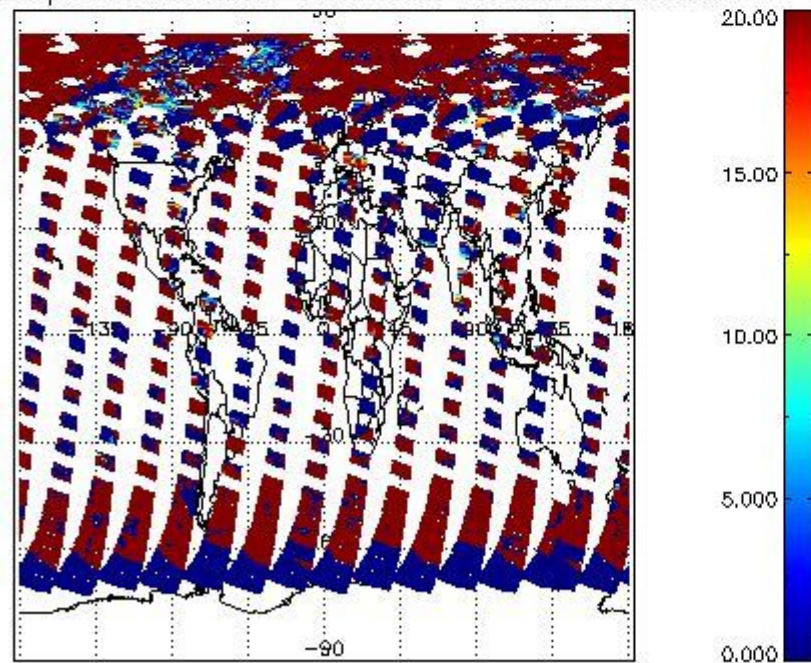
cL_opt_depth for 29JUL2011 00:00:00 to 30JUL2011 00:00:00
