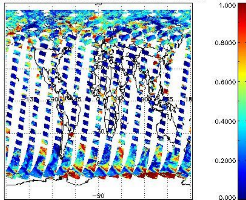
cL_frac for 29JUL2011 00:00:00 to 30JUL2011 00:00:00
