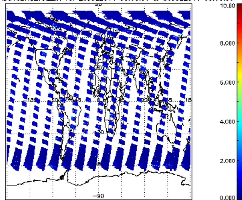
SCIOL2P_NADUV3BRO_vcd_err for 29JUL2011 00:00:00 to 30JUL2011 00:00:00
