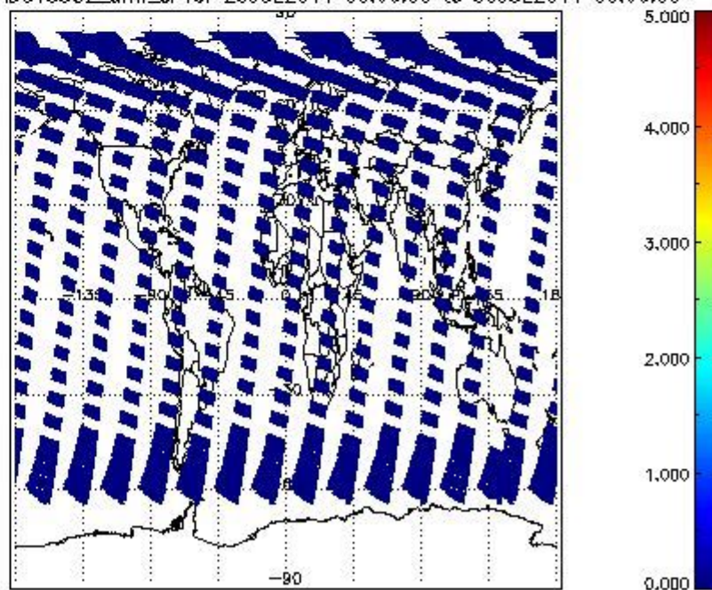
SCIOL2P_NADUV5S02_amf_cl for 29JUL2011 00:00:00 to 30JUL2011 00:00:00
