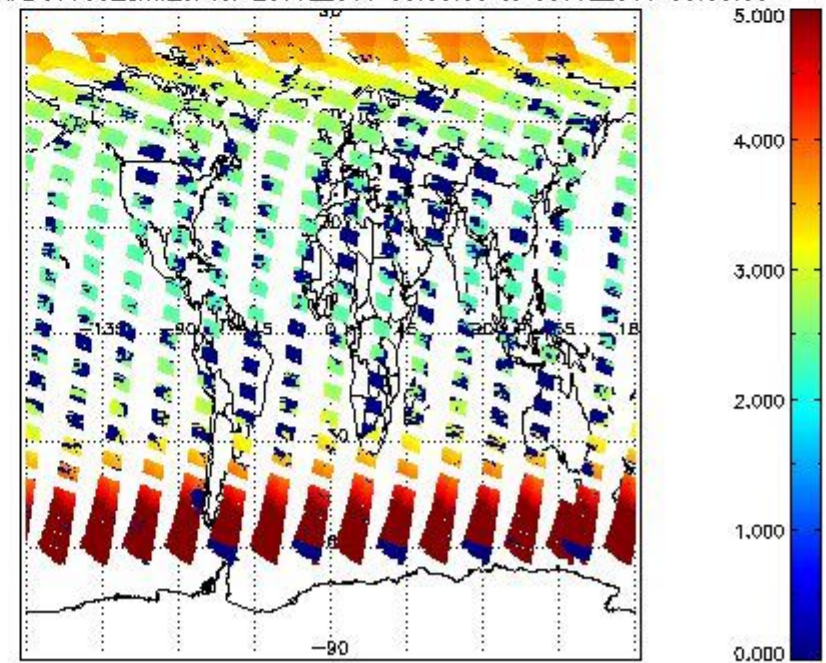
SCIOL2P_NADUV003_amf_cl for 29JUL2011 00:00:00 to 30JUL2011 00:00:00
