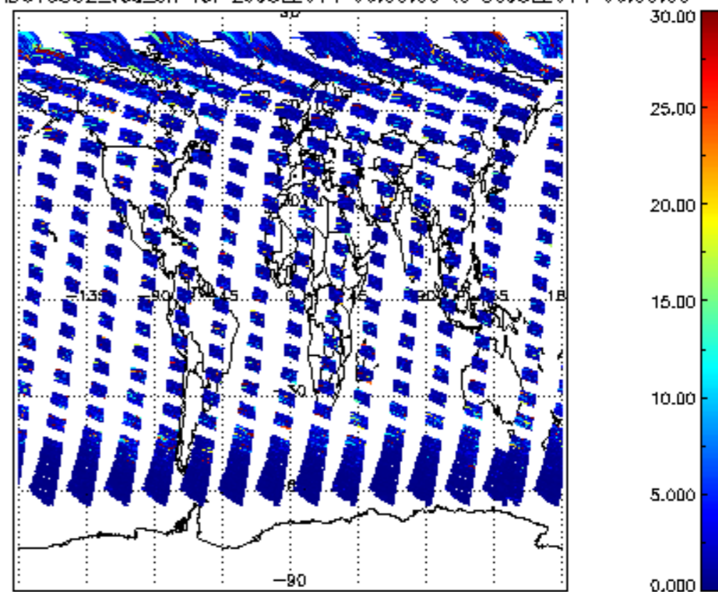
SCIOL2P_NADUV5S02_vcd_err for 29JUL2011 00:00:00 to 30JUL2011 00:00:00
