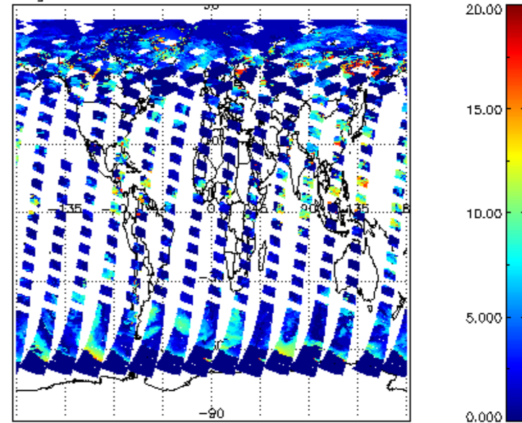
cl_top_height for 27JUL2011 00:00:00 to 28JUL2011 00:00:00
