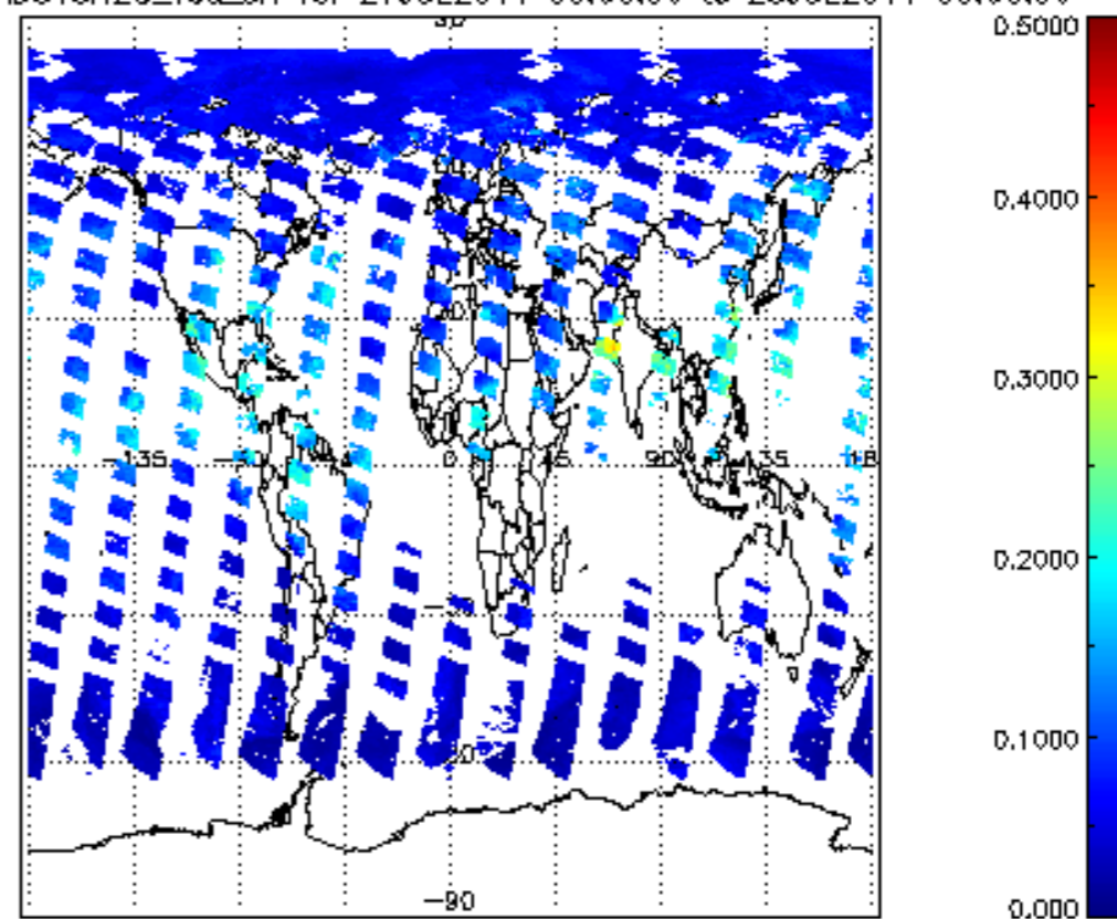
SCIOL2P_NADUV8H20_vcd_err for 27JUL2011 00:00:00 to 28JUL2011 00:00:00
