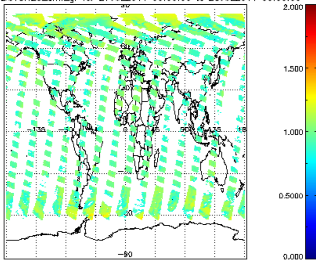
SCIOL2P_NADUV8H20_amf_gr for 27JUL2011 00:00:00 to 28JUL2011 00:00:00
