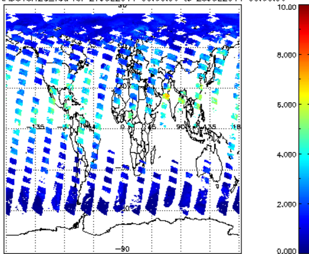
SCIOL2P_NADUV8H20_vcd for 27JUL2011 00:00:00 to 28JUL2011 00:00:00
