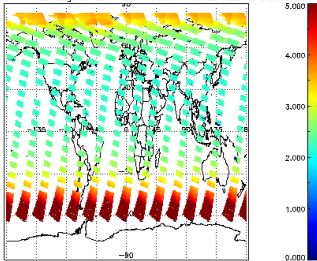
SCIOL2P_NADUV003_amf_gr for 27JUL2011 00:00:00 to 28JUL2011 00:00:00
