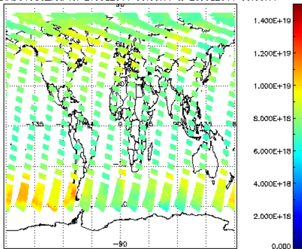
SCIOL2P_NADUV003_vcd for 27JUL2011 00:00:00 to 28JUL2011 00:00:00
