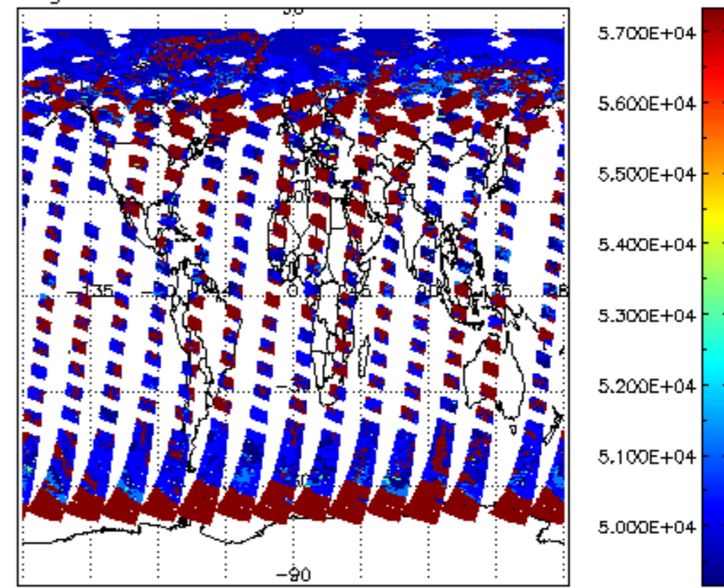
cloud_flags for 27JUL2011 00:00:00 to 28JUL2011 00:00:00
