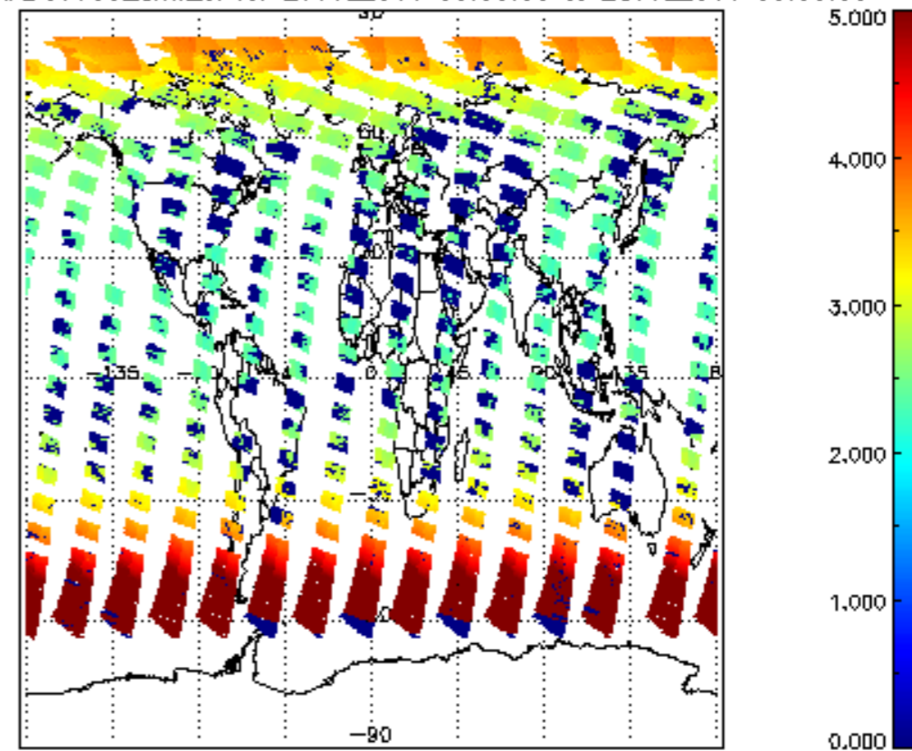
SCIOL2P_NADUV003_amf_cl for 27JUL2011 00:00:00 to 28JUL2011 00:00:00
