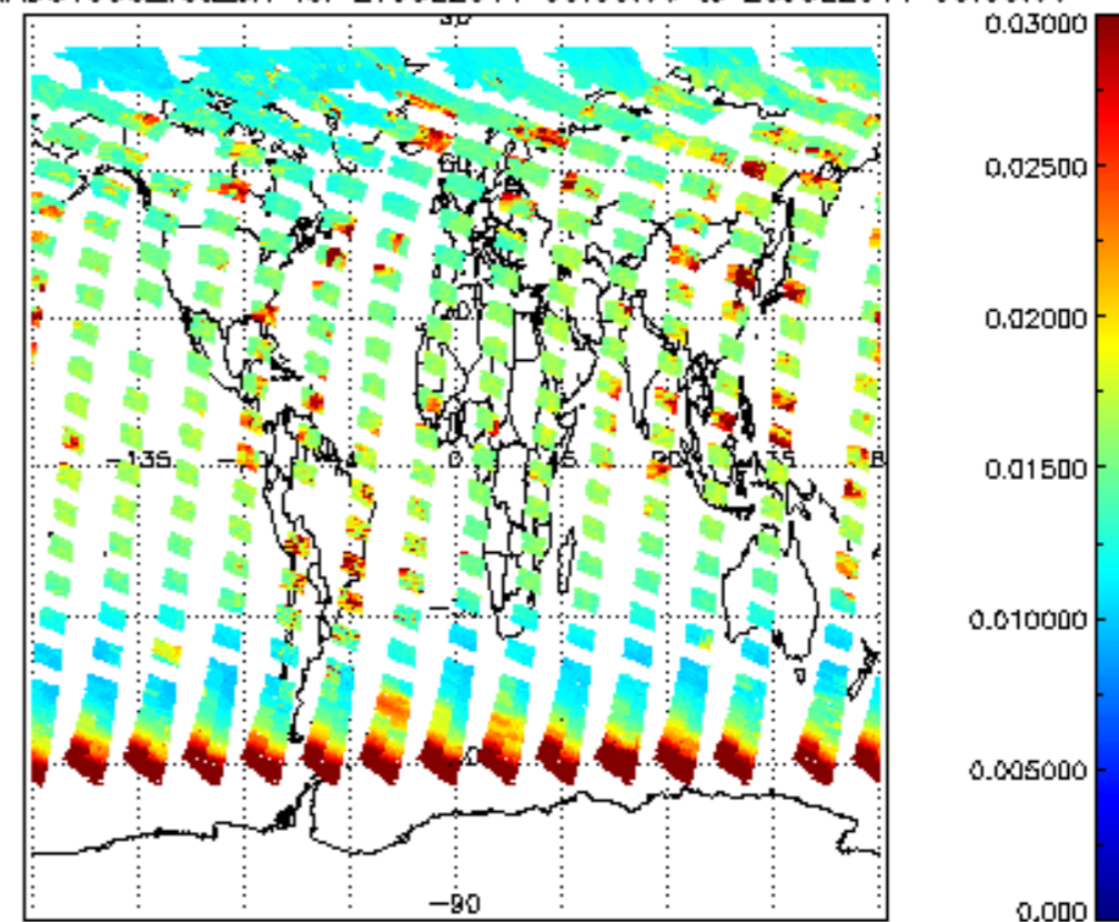
SCIOL2P_NADUV003_vcd_err for 27JUL2011 00:00:00 to 28JUL2011 00:00:00
