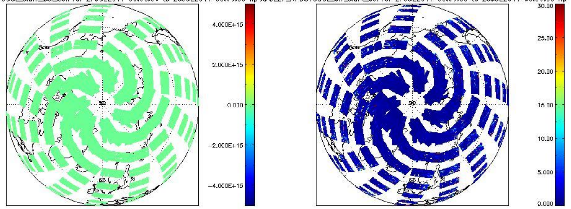
SCIOI2P_NADUV6OCLslant_col_den for 27JUL2011 00:00:00 to 28JUL2011 00:00:00 np SCIOI2P_NADUV6OCLarr_slant_col for 27JUL2011 00:00:00 to 28JUL2011 00:00:00 np
