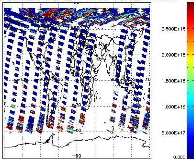
SCIDL2P_NADIR3CO_vcd for 23JUL2011 00:00:00 to 24JUL2011 00:00:00
