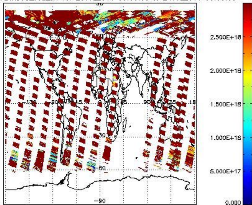
SCIDL2P_NADIR3CO_vcd_err for 23JUL2011 00:00:00 to 24JUL2011 00:00:00
