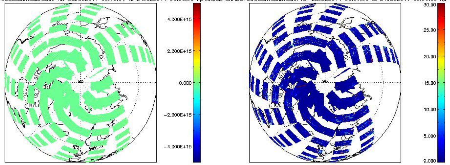
SCIOI2P_NADUV60CLslant_col_den for 23JUL2011 00:00:00 to 24JUL2011 00:00:00 np SCIOI2P_NADUV60CLarr_slant_col for 23JUL2011 00:00:00 to 24JUL2011 00:00:00 np
