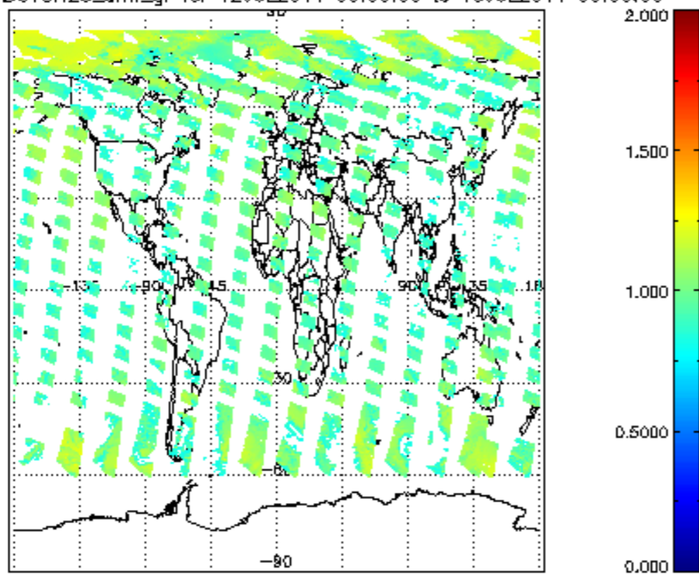
SCIOL2P_NADUV8H20_amf_gr for 12JUL2011 00:00:00 to 13JUL2011 00:00:00
