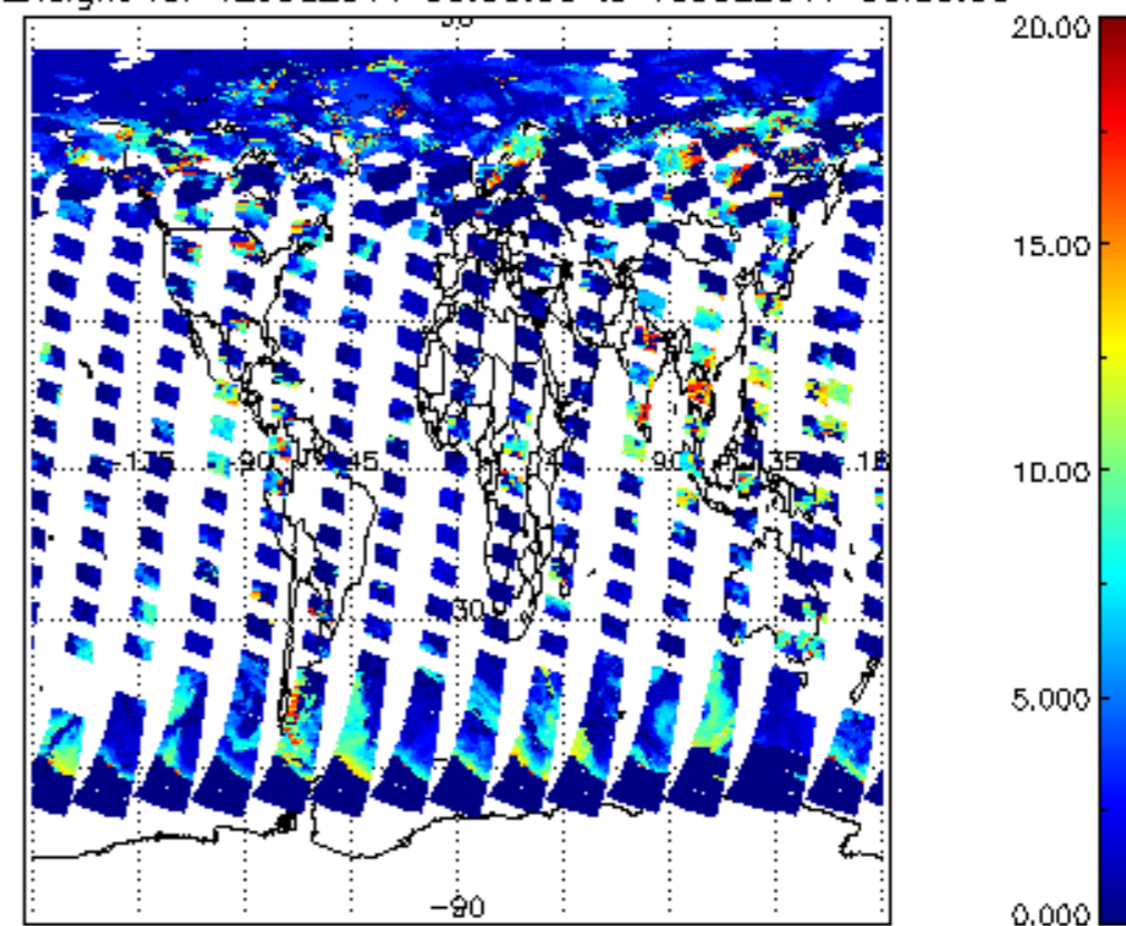
cl_top_height for 12JUL2011 00:00:00 to 13JUL2011 00:00:00
