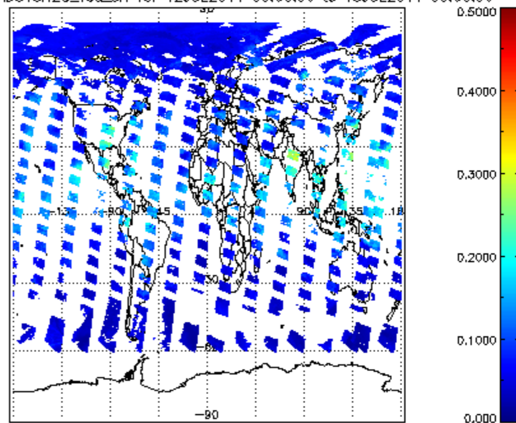
SCIOL2P_NADUV8H20_vcd_err for 12JUL2011 00:00:00 to 13JUL2011 00:00:00
