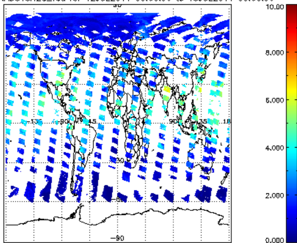
SCIOL2P_NADUV8H20_vcd for 12JUL2011 00:00:00 to 13JUL2011 00:00:00
