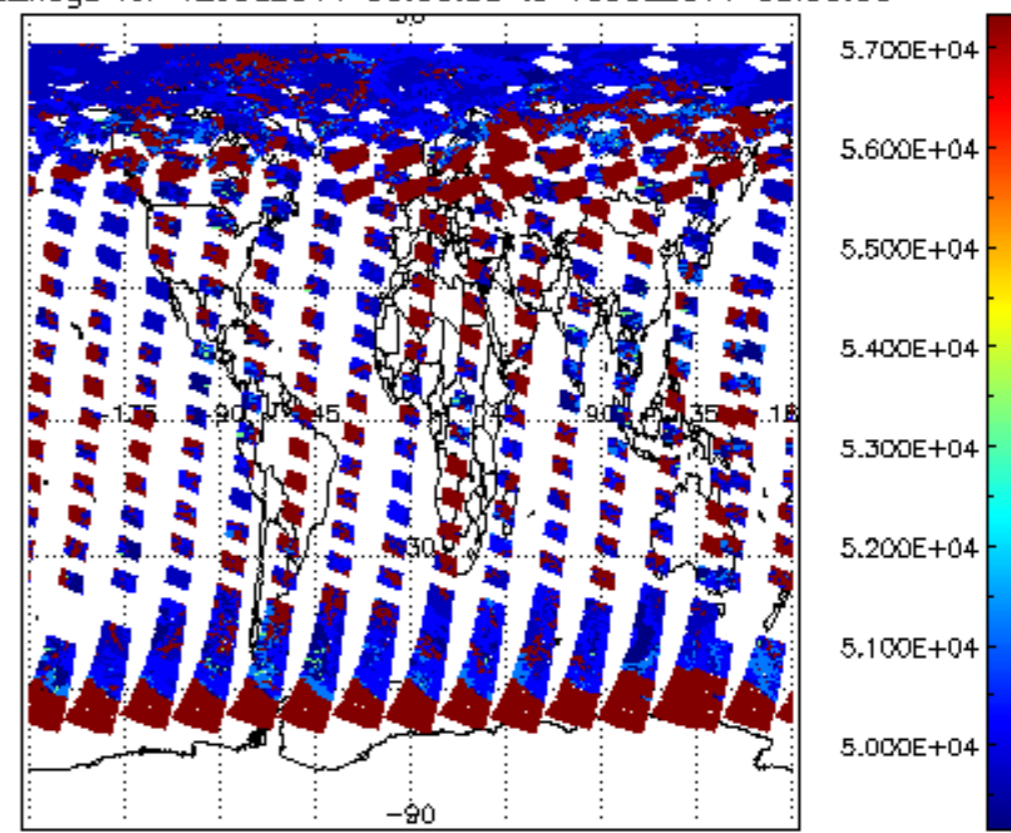
cloud_flags for 12JUL2011 00:00:00 to 13JUL2011 00:00:00
