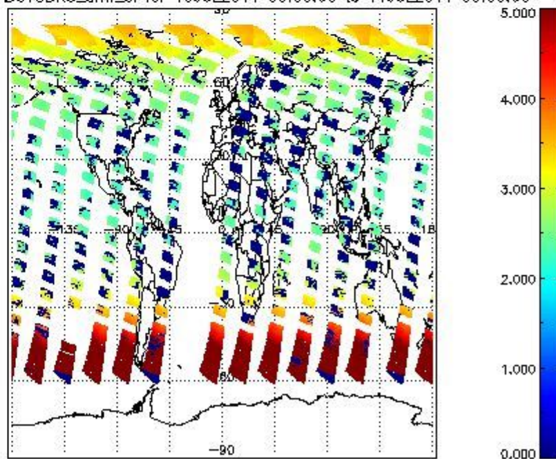
SCIOL2P_NADUV3BRO_amf_cl for 10JUL2011 00:00:00 to 11JUL2011 00:00:00
