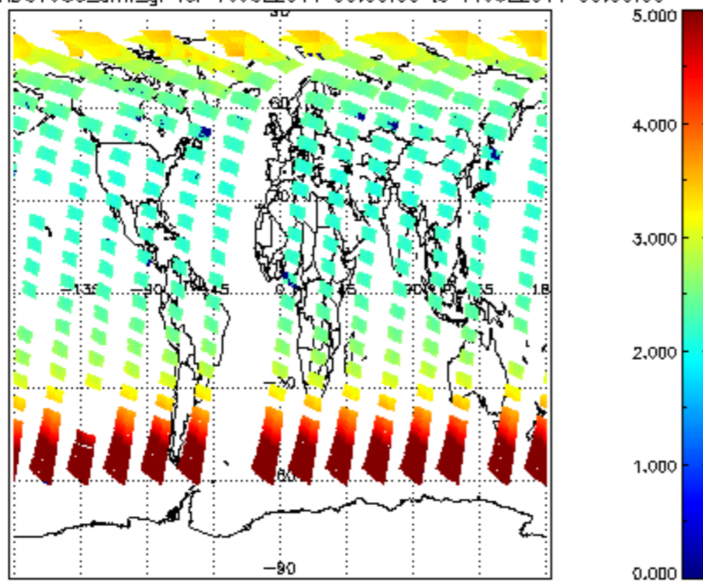
SCIOL2P_NADUV003_amf_gr for 10JUL2011 00:00:00 to 11JUL2011 00:00:00
