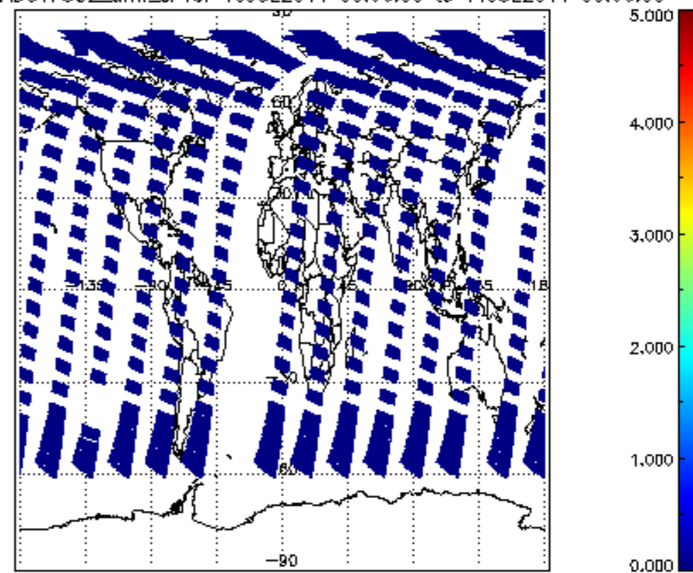
SCIOL2P_NADUV7S02_amf_cl for 10JUL2011 00:00:00 to 11JUL2011 00:00:00
