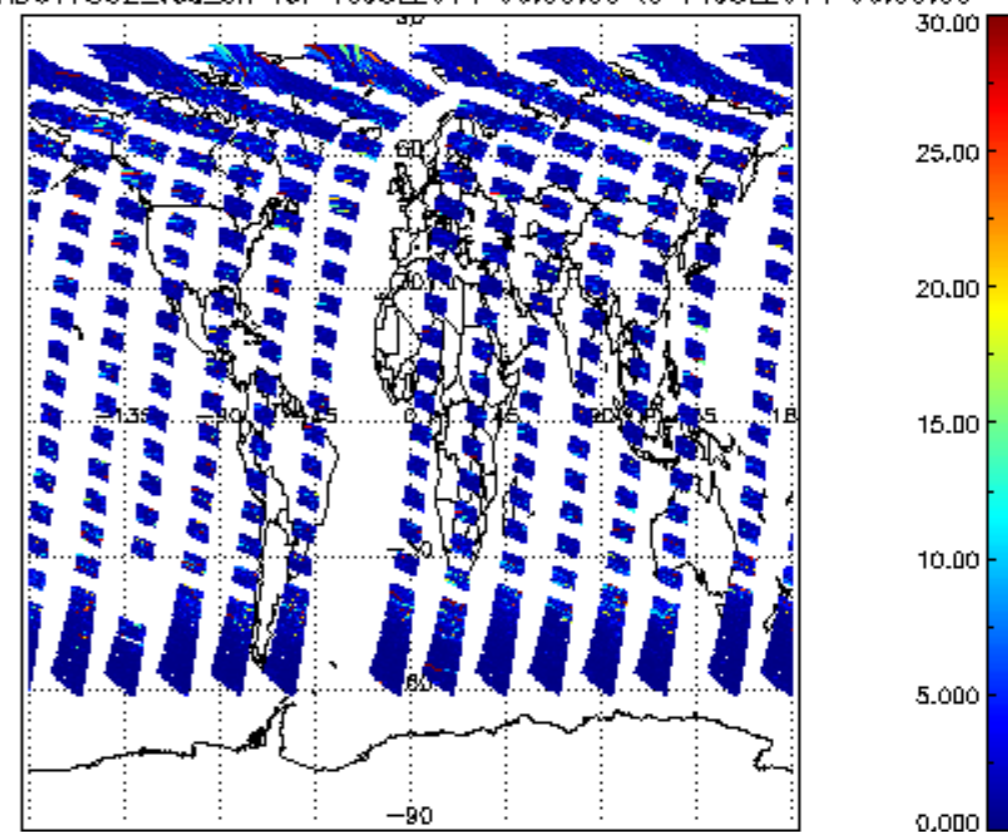
SCIOL2P_NADUV7S02_vcd_err for 10JUL2011 00:00:00 to 11JUL2011 00:00:00
