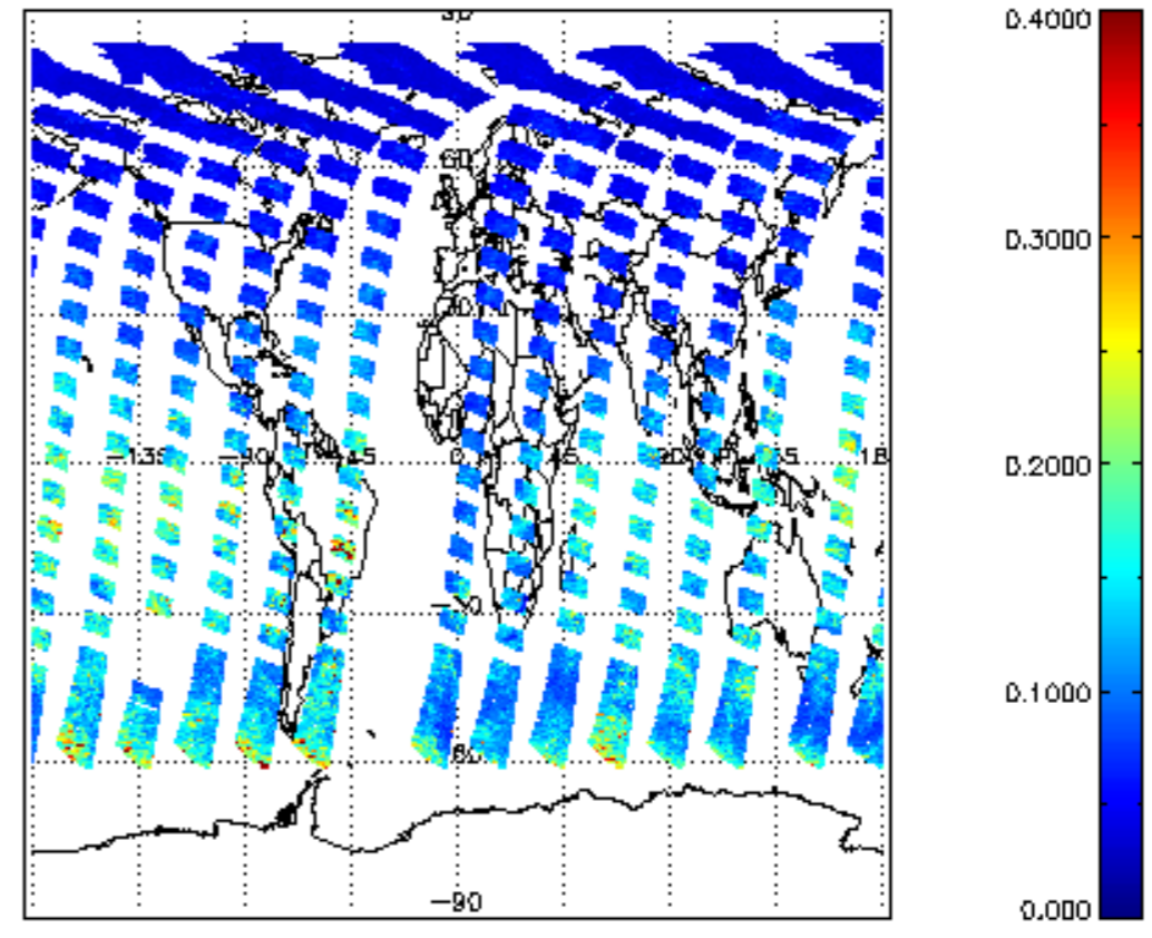
SCIOL2P_NADUV1NO2_vcd_err for 10JUL2011 00:00:00 to 11JUL2011 00:00:00
