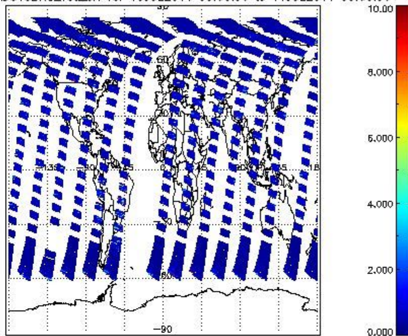
SCIOL2P_NADUV3BRO_vcd_err for 10JUL2011 00:00:00 to 11JUL2011 00:00:00
