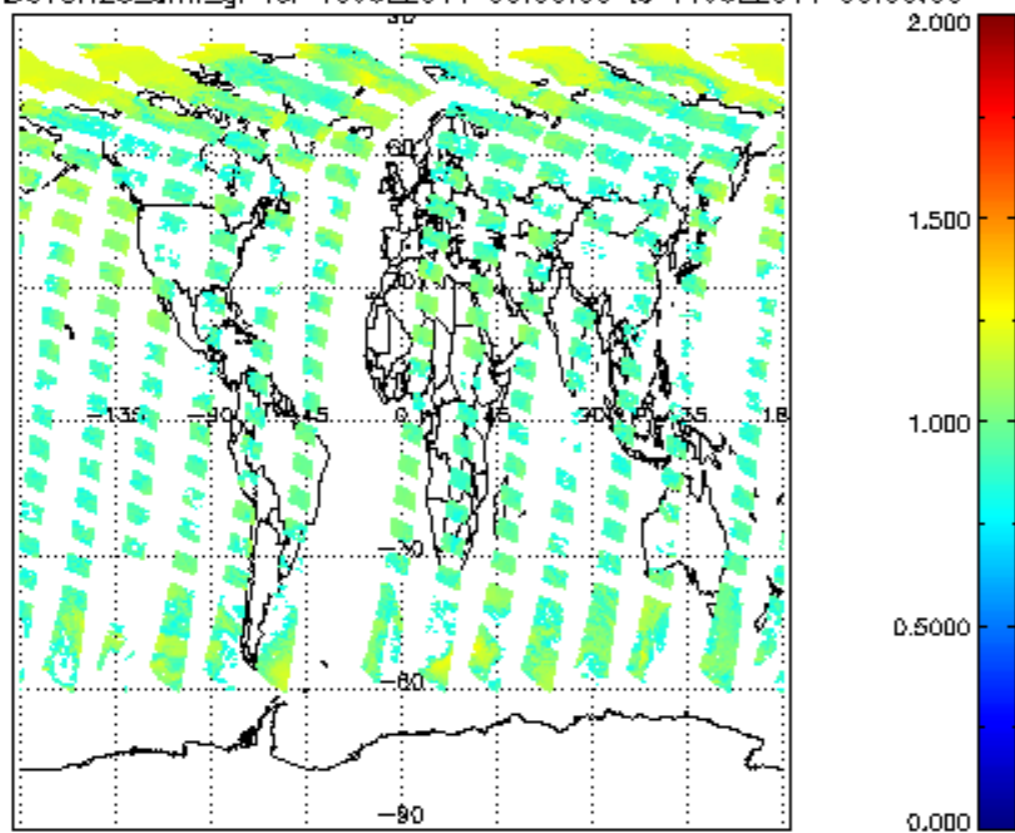
SCIOL2P_NADUV8H20_amf_gr for 10JUL2011 00:00:00 to 11JUL2011 00:00:00
