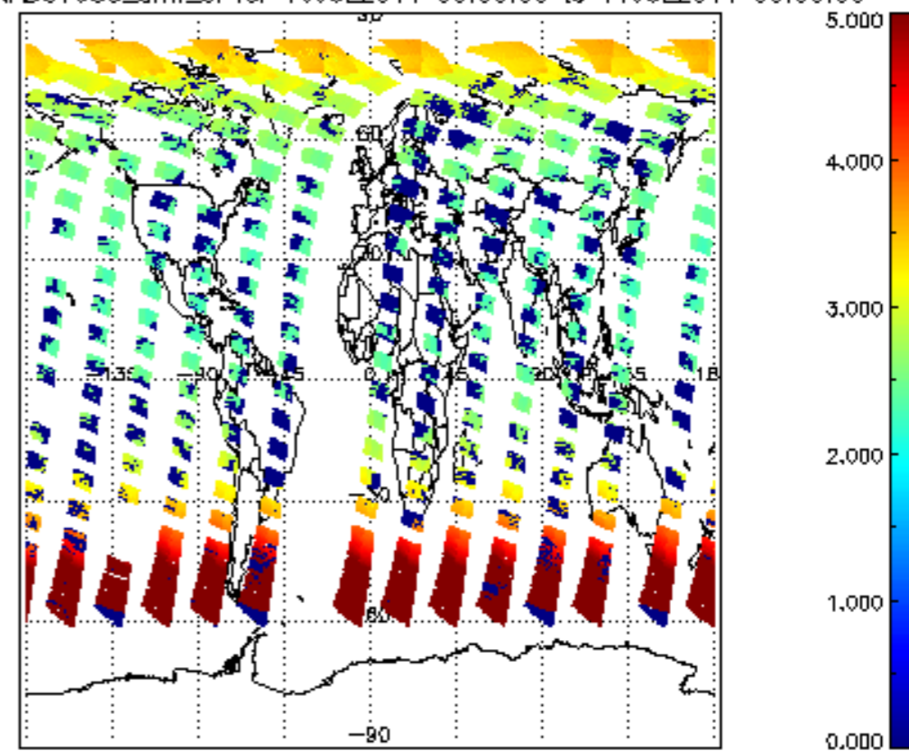
SCIOL2P_NADUV003_amf_cl for 10JUL2011 00:00:00 to 11JUL2011 00:00:00
