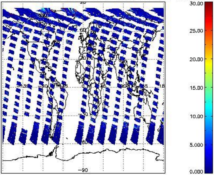
SCIOL2P_NADUV7S02_vcd_err for 10JUL2011 00:00:00 to 11JUL2011 00:00:00
