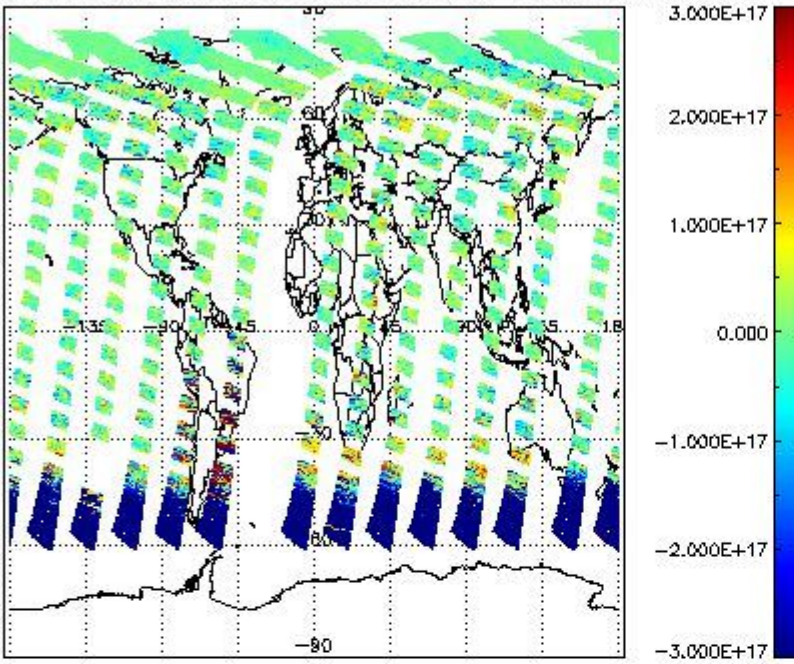
SCIOL2P_NADUV5S02_vcd for 10JUL2011 00:00:00 to 11JUL2011 00:00:00
