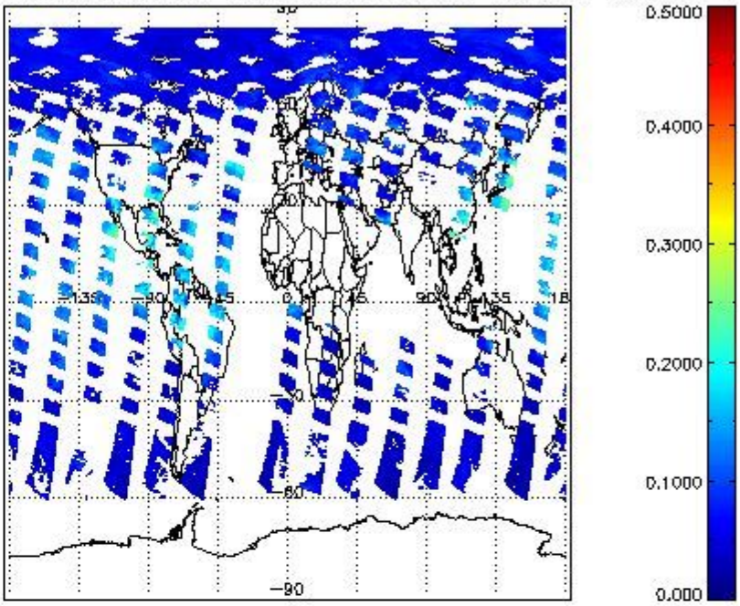
SCIOL2P_NADUV8H2O_vcd_err for 10JUL2011 00:00:00 to 11JUL2011 00:00:00
