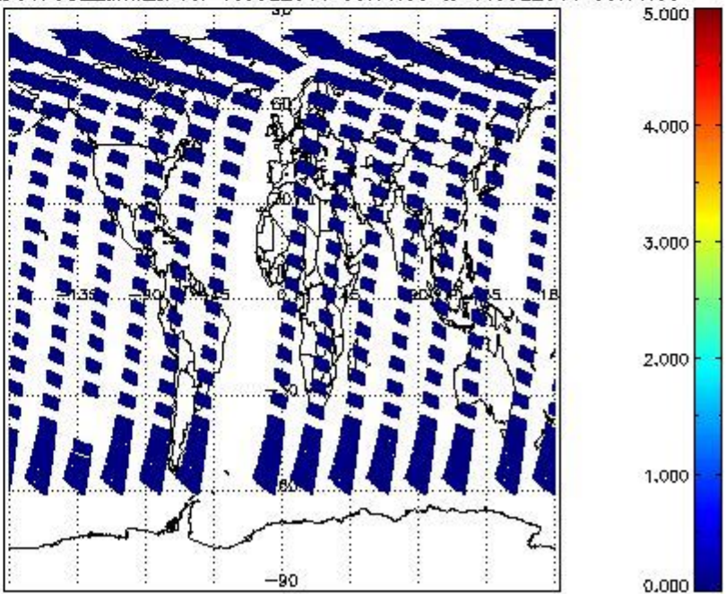
SCIOL2P_NADUV7S02_amf_cl for 10JUL2011 00:00:00 to 11JUL2011 00:00:00
