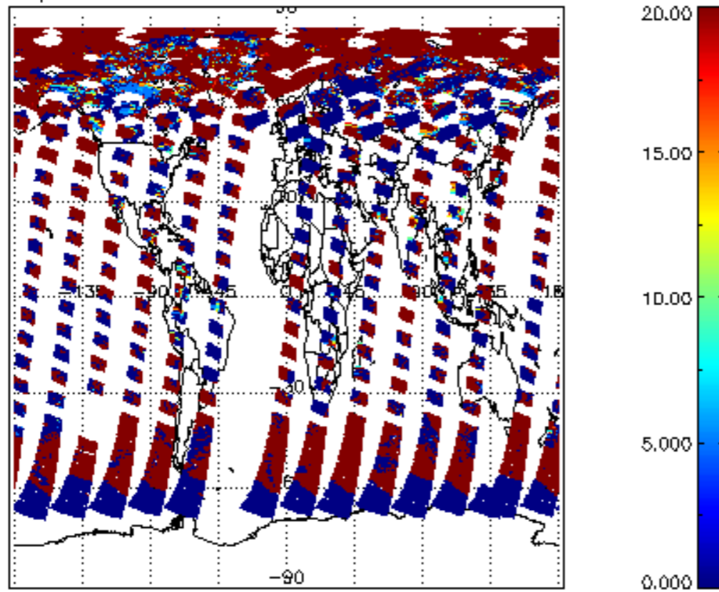
cl_opt_depth for 10JUL2011 00:00:00 to 11JUL2011 00:00:00
