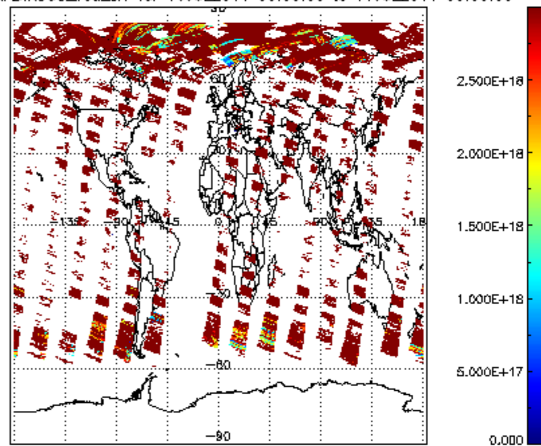
SCIOL2P_NADIR3CO_vcd_err for 10JUL2011 00:00:00 to 11JUL2011 00:00:00
