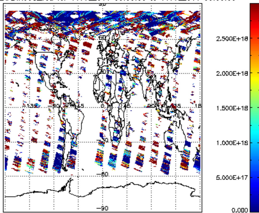
SCIOL2P_NADIR3CO_vcd for 10JUL2011 00:00:00 to 11JUL2011 00:00:00
