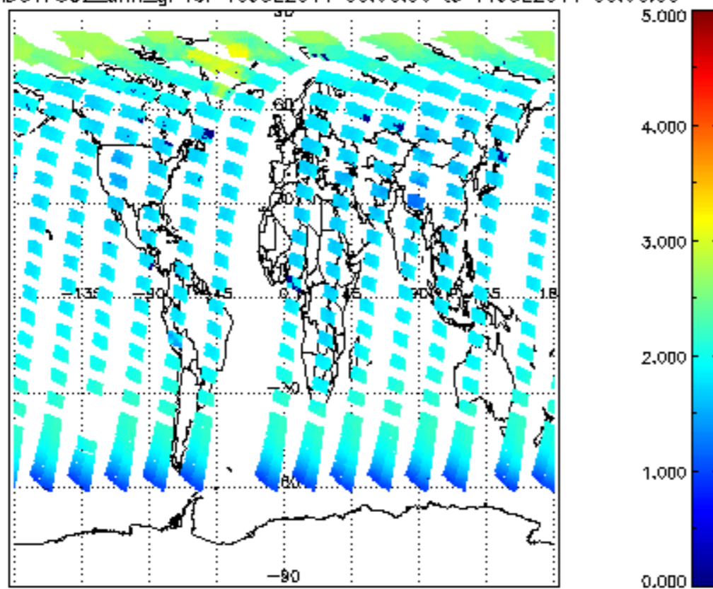
SCIOL2P_NADUV7S02_amf_gr for 10JUL2011 00:00:00 to 11JUL2011 00:00:00
