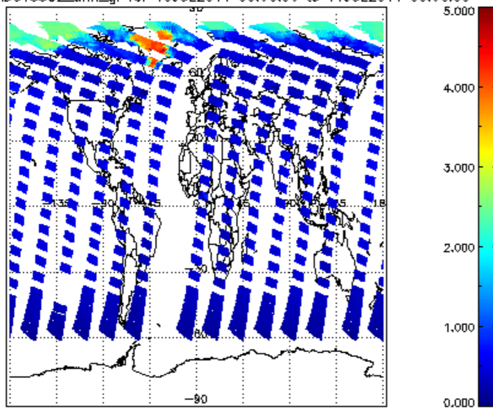
SCIOL2P_NADUV5S02_amf_gr for 10JUL2011 00:00:00 to 11JUL2011 00:00:00
