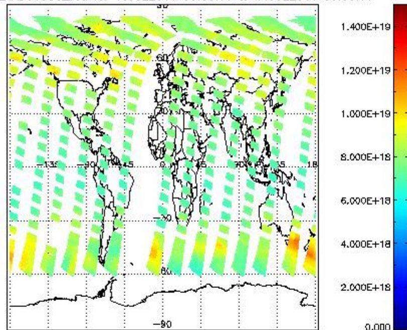
SCIOL2P_NADUV003_vcd for 10JUL2011 00:00:00 to 11JUL2011 00:00:00
