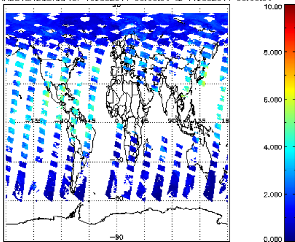
SCIOL2P_NADUV8H20_vcd for 10JUL2011 00:00:00 to 11JUL2011 00:00:00
