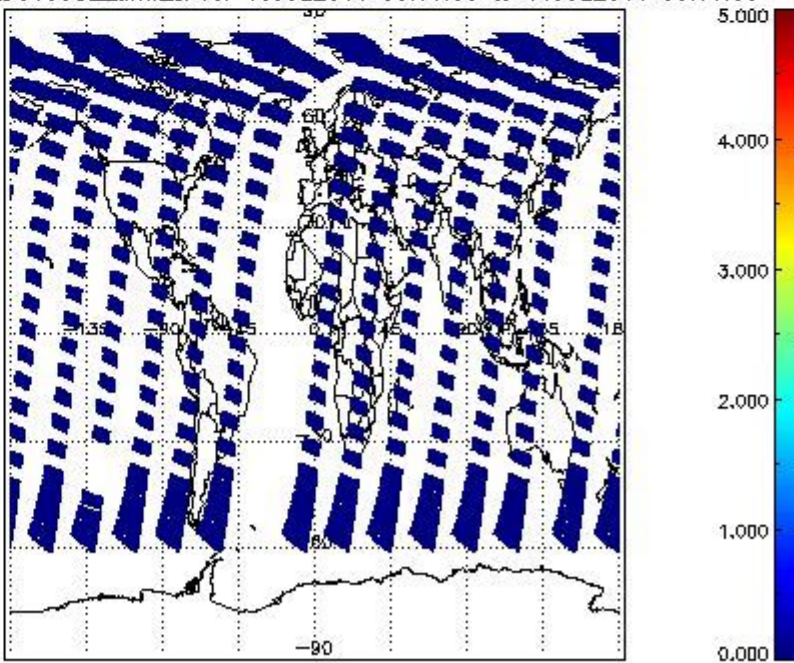
SCIOL2P_NADUV5S02_amf_cl for 10JUL2011 00:00:00 to 11JUL2011 00:00:00
