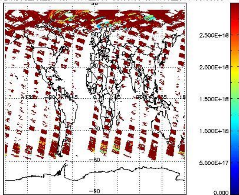
SCIO2P_NADIR3CO_vcd_err for 10JUL2011 00:00:00 to 11JUL2011 00:00:00
