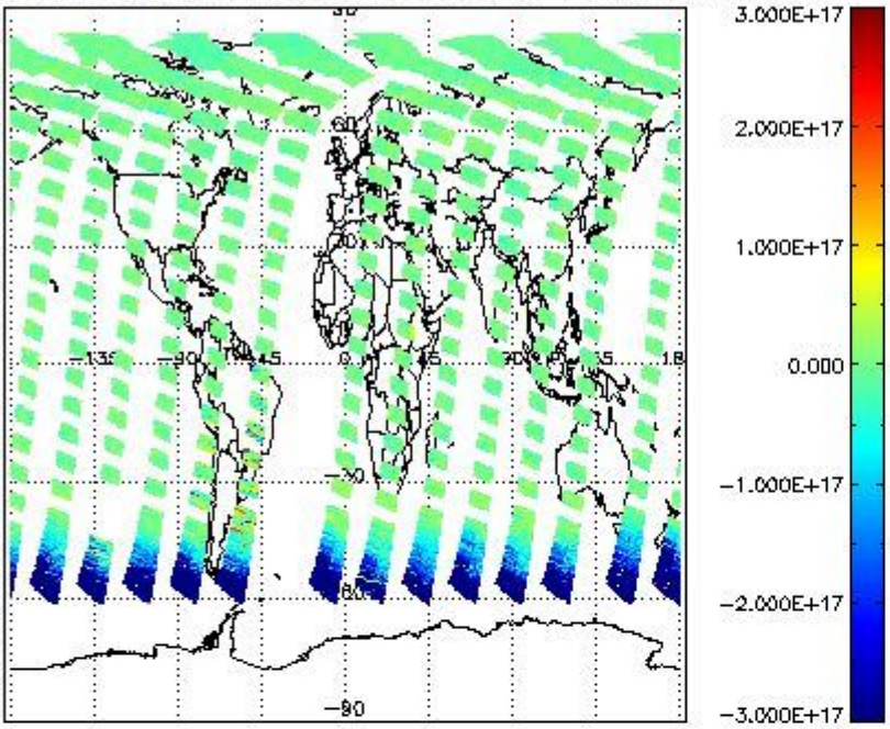
SCIOL2P_NADUV7S02_vcd for 10JUL2011 00:00:00 to 11JUL2011 00:00:00
