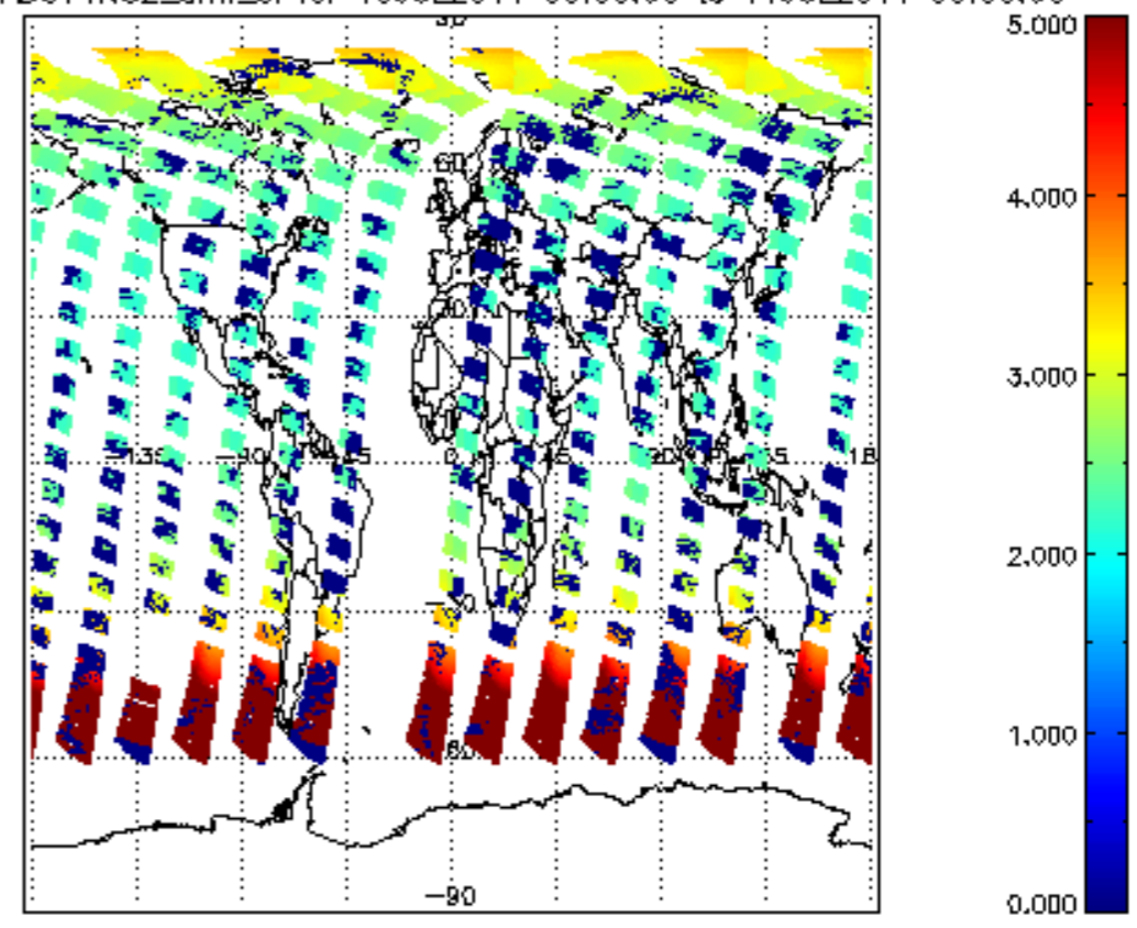
SCIOL2P_NADUV1NO2_amf_cl for 10JUL2011 00:00:00 to 11JUL2011 00:00:00
