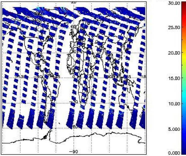
SCIOL2P_NADUV5S02_vcd_err for 10JUL2011 00:00:00 to 11JUL2011 00:00:00
