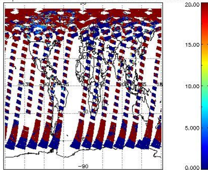
cL_opt_depth for 10JUL2011 00:00:00 to 11JUL2011 00:00:00
