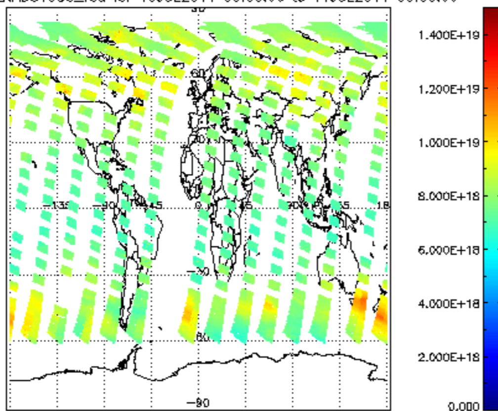
SCIOL2P_NADUV003_vcd for 10JUL2011 00:00:00 to 11JUL2011 00:00:00
