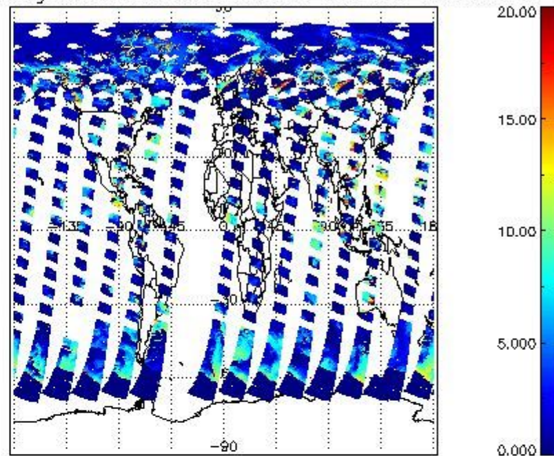
cL_top_height for 10JUL2011 00:00:00 to 11JUL2011 00:00:00
