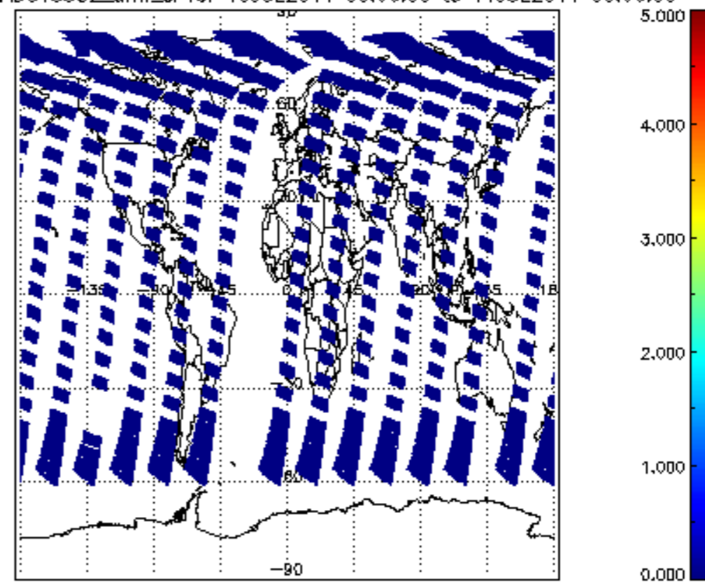
SCIOL2P_NADUV5S02_amf_cl for 10JUL2011 00:00:00 to 11JUL2011 00:00:00
