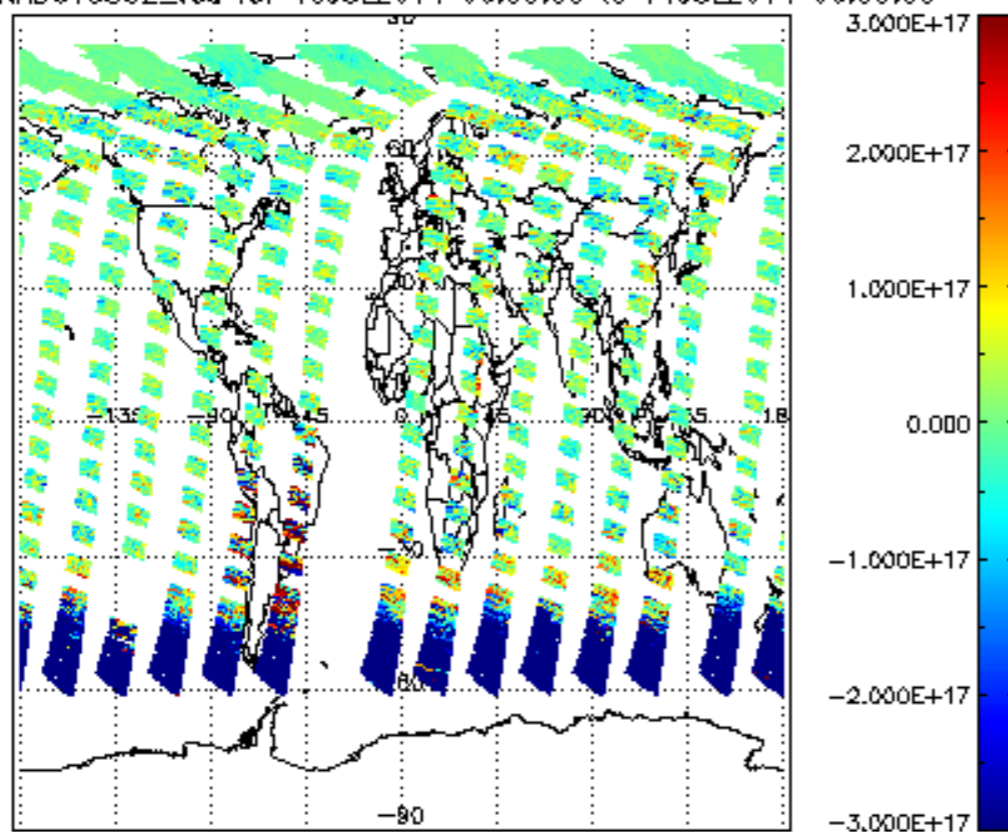
SCIOL2P_NADUV5S02_vcd for 10JUL2011 00:00:00 to 11JUL2011 00:00:00
