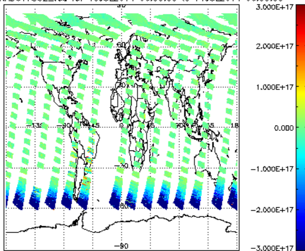
SCIOL2P_NADUV7S02_vcd for 10JUL2011 00:00:00 to 11JUL2011 00:00:00
