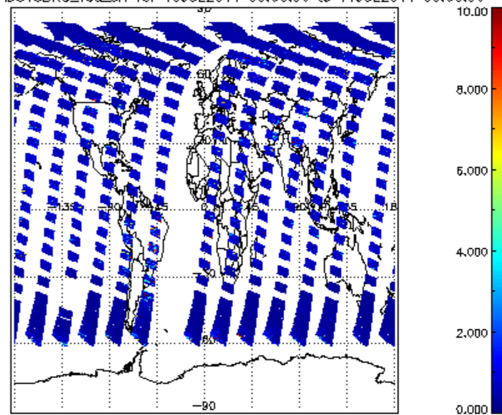
SCIOL2P_NADUV3BRO_vcd_err for 10JUL2011 00:00:00 to 11JUL2011 00:00:00
