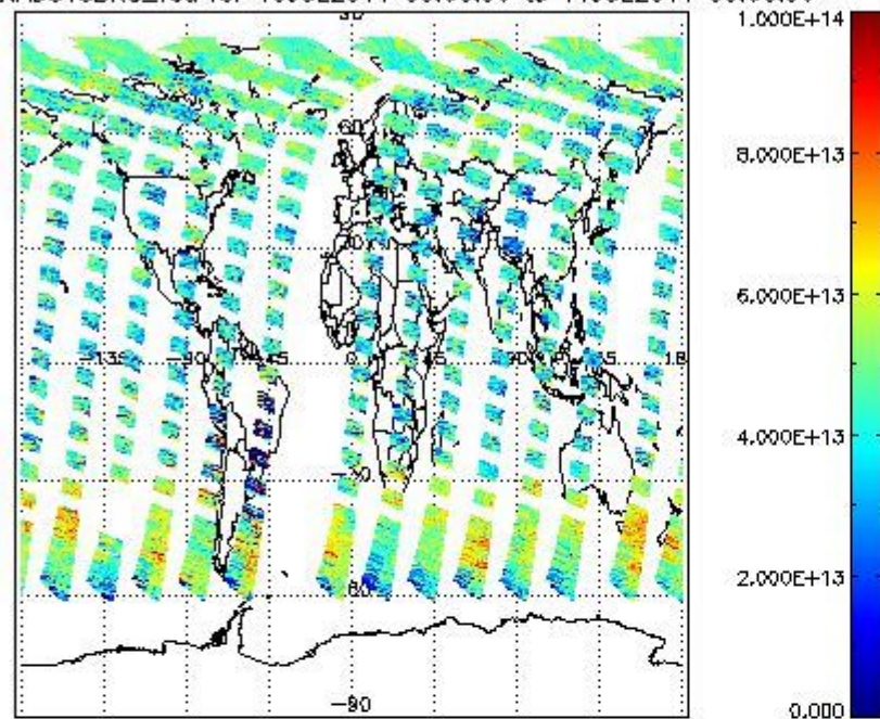
SCIOL2P_NADUV3BRO_vcd for 10JUL2011 00:00:00 to 11JUL2011 00:00:00
