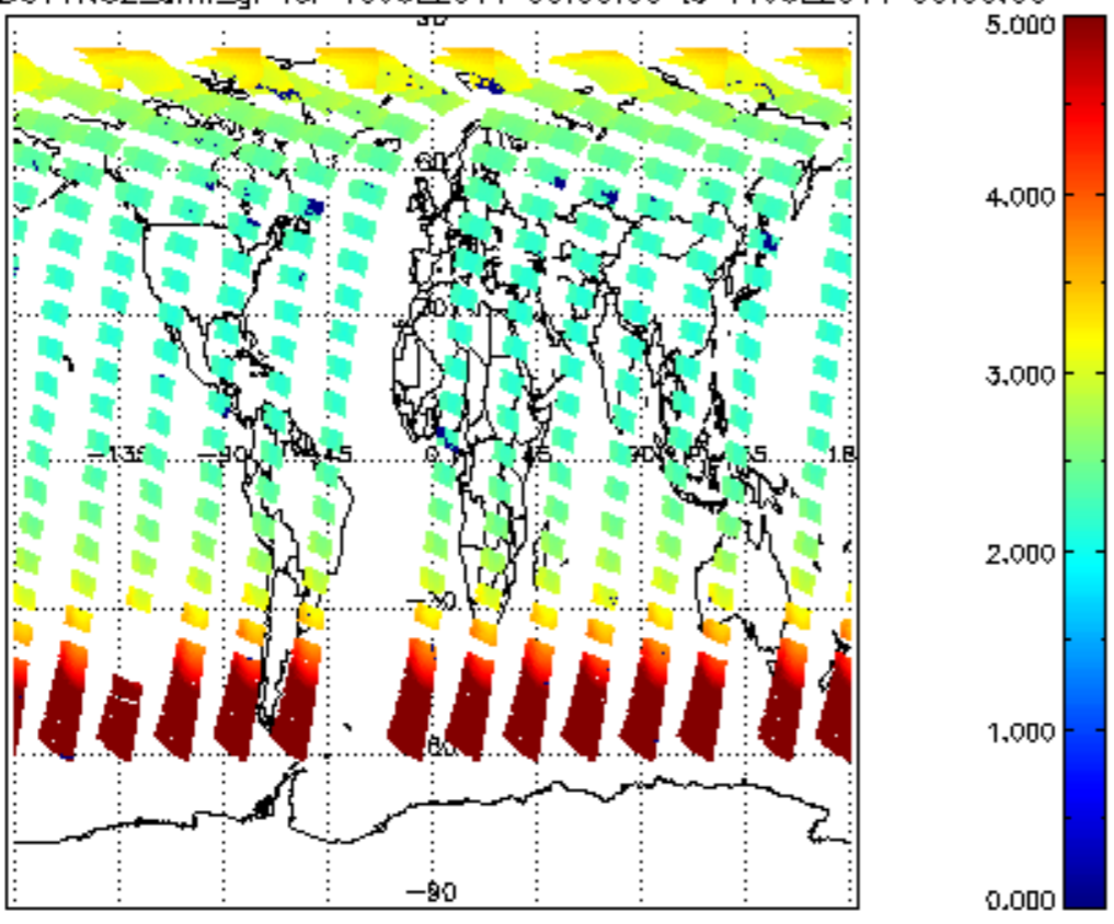
SCIOL2P_NADUV1NO2_amf_gr for 10JUL2011 00:00:00 to 11JUL2011 00:00:00
