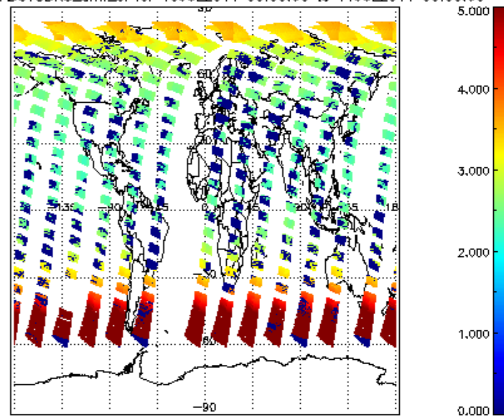
SCIOL2P_NADUV3BRO_amf_cl for 10JUL2011 00:00:00 to 11JUL2011 00:00:00
