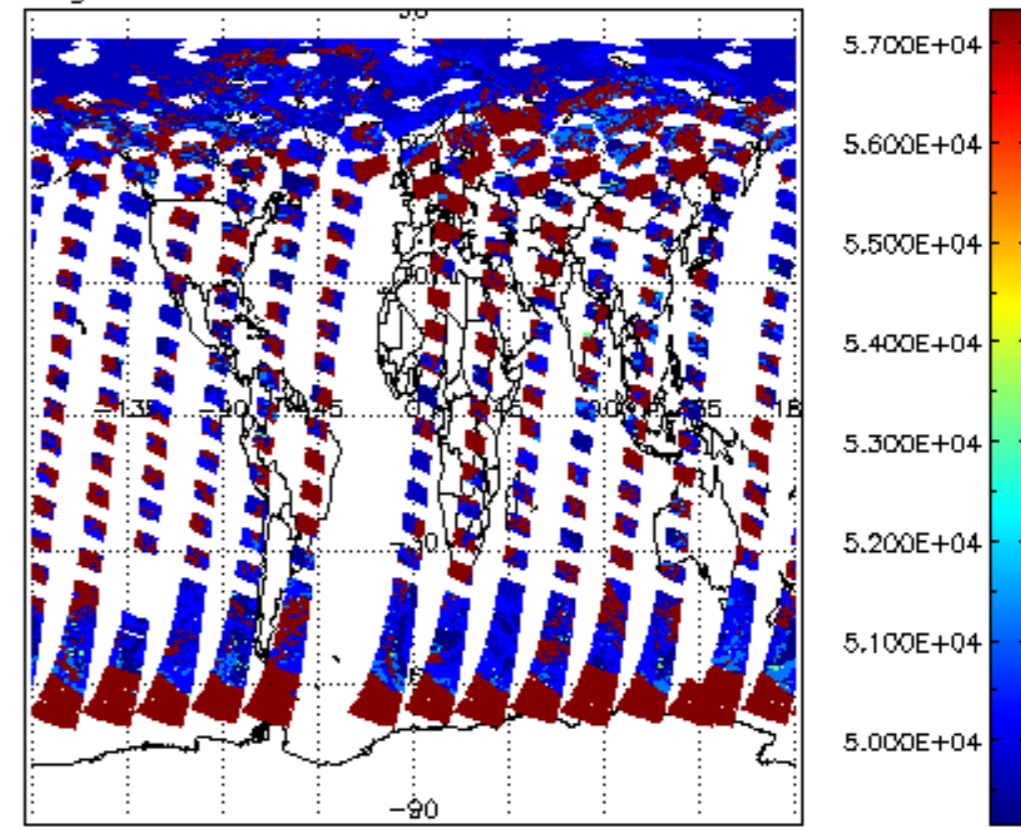
cloud_flags for 10JUL2011 00:00:00 to 11JUL2011 00:00:00
