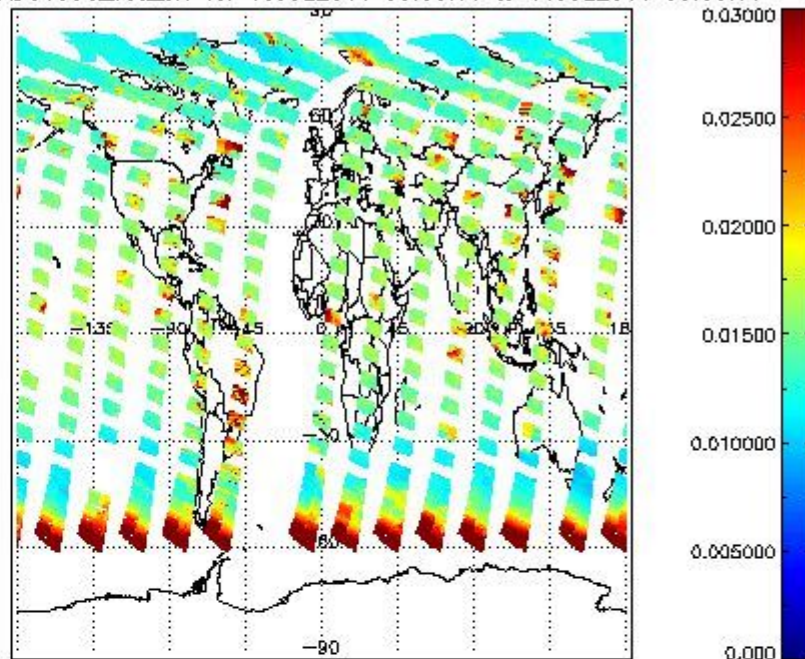
SCIOL2P_NADUV003_vcd_err for 10JUL2011 00:00:00 to 11JUL2011 00:00:00
