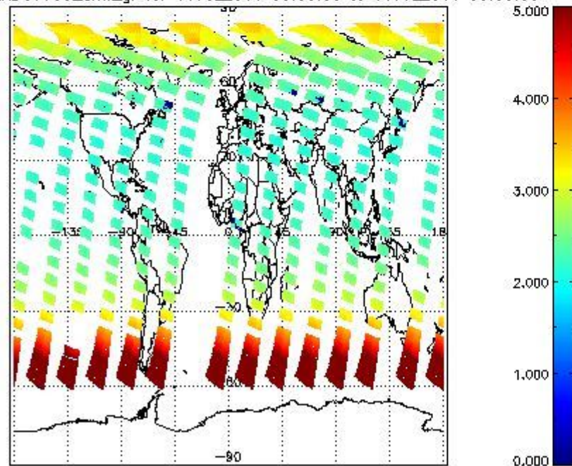
SCIOL2P_NADUV003_amf_gr for 10JUL2011 00:00:00 to 11JUL2011 00:00:00
