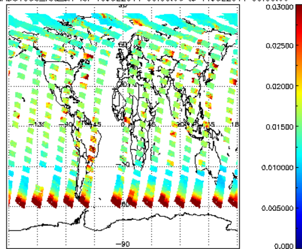
SCIOL2P_NADUV003_vcd_err for 10JUL2011 00:00:00 to 11JUL2011 00:00:00
