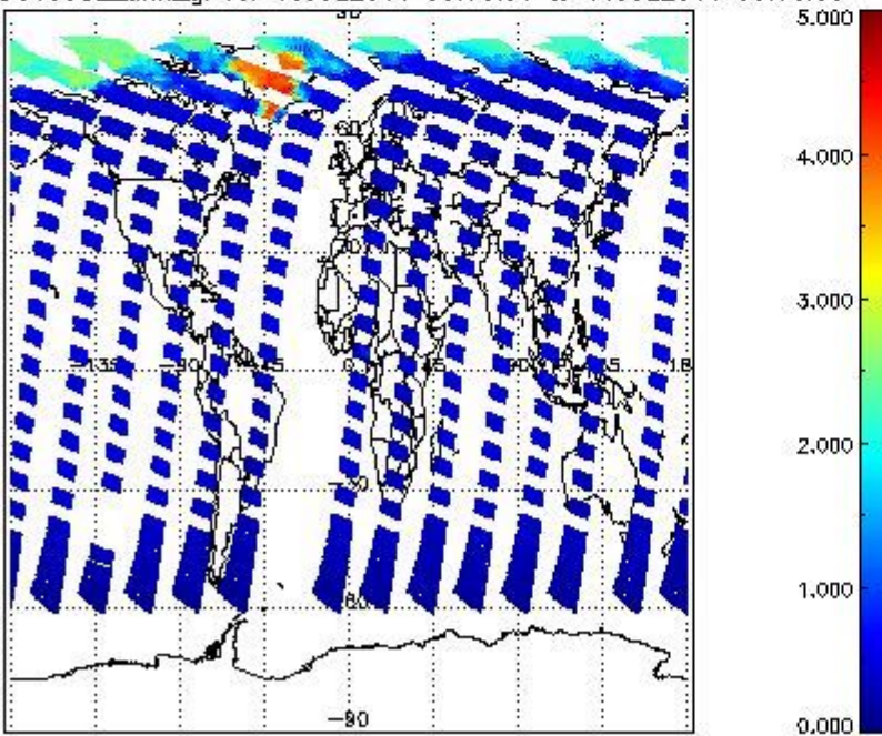
SCIOL2P_NADUV5S02_amf_gr for 10JUL2011 00:00:00 to 11JUL2011 00:00:00
