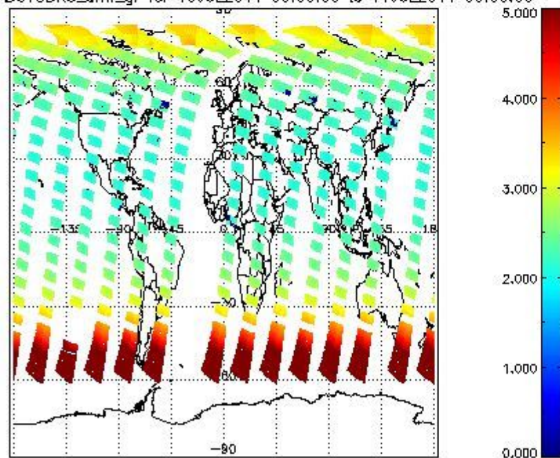
SCIOL2P_NADUV3BRO_amf_gr for 10JUL2011 00:00:00 to 11JUL2011 00:00:00
