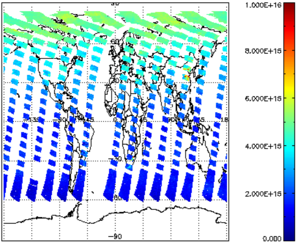
SCIOL2P_NADUV1NO2_vcd for 10JUL2011 00:00:00 to 11JUL2011 00:00:00
