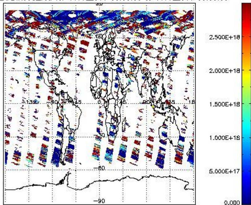
SCIO2P_NADIR3CO_vcd for 10JUL2011 00:00:00 to 11JUL2011 00:00:00
