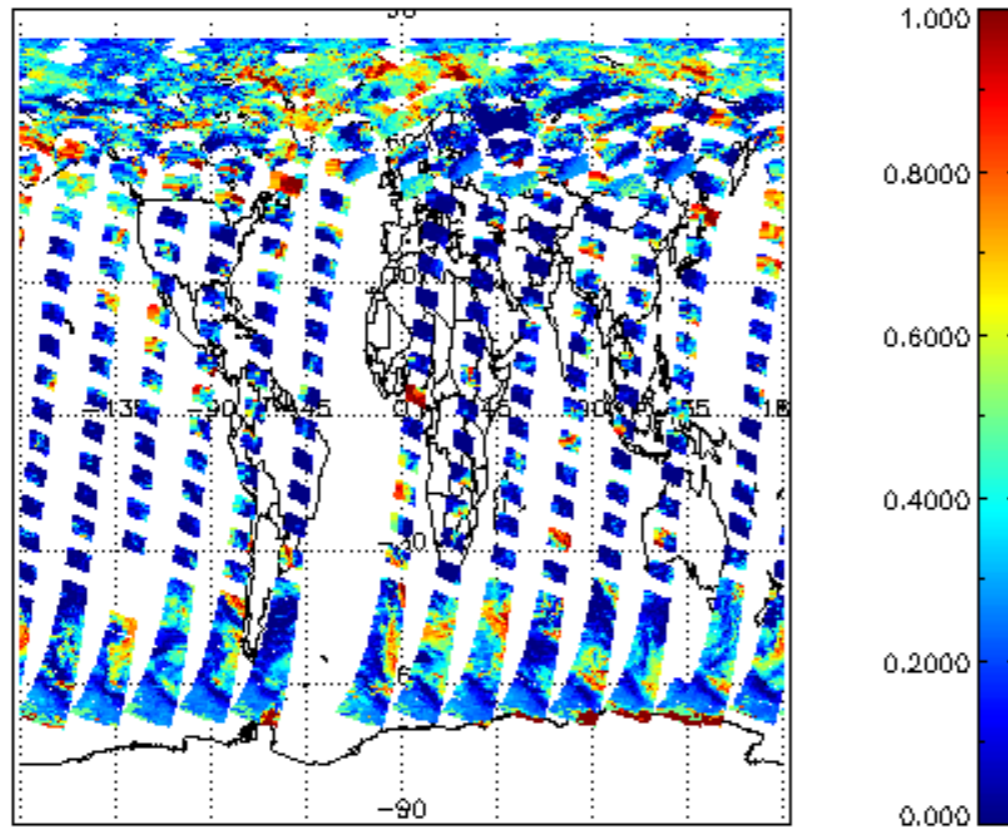
cl_frac for 10JUL2011 00:00:00 to 11JUL2011 00:00:00
