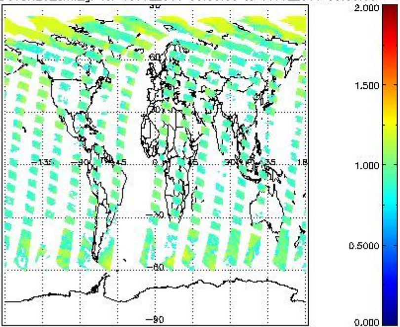
SCIOL2P_NADUV8H2O_amf_gr for 10JUL2011 00:00:00 to 11JUL2011 00:00:00
