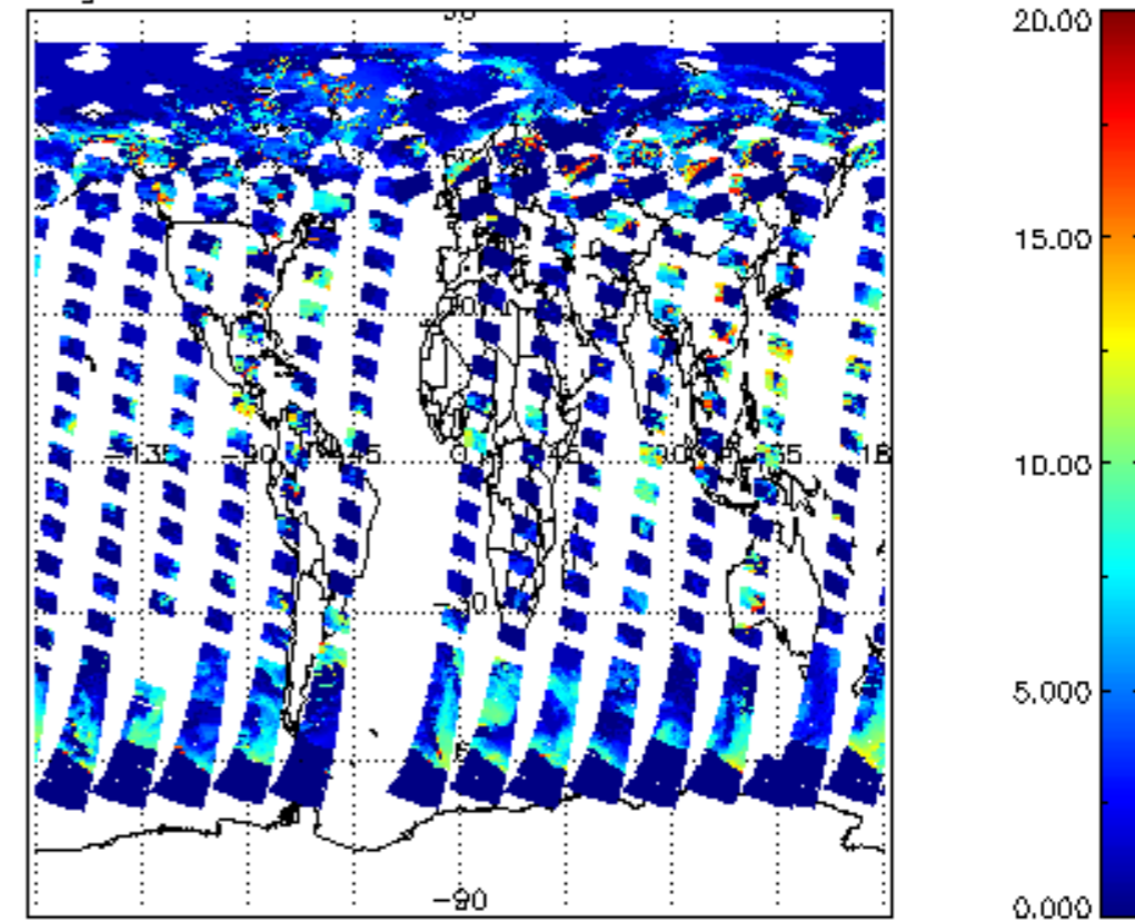
cl_top_height for 10JUL2011 00:00:00 to 11JUL2011 00:00:00
