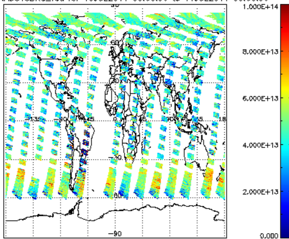
SCIOL2P_NADUV3BRO_vcd for 10JUL2011 00:00:00 to 11JUL2011 00:00:00
