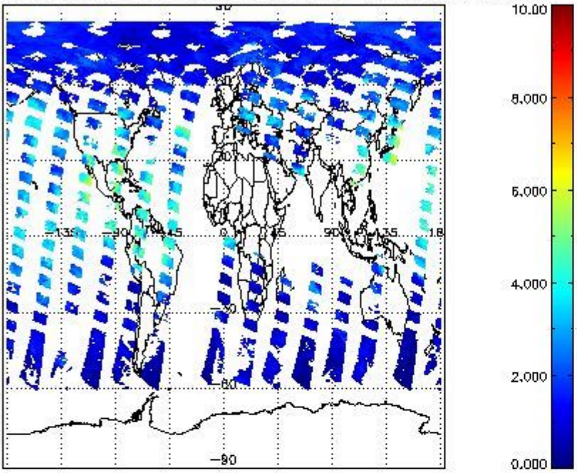
SCIOL2P_NADUV8H2O_vcd for 10JUL2011 00:00:00 to 11JUL2011 00:00:00
