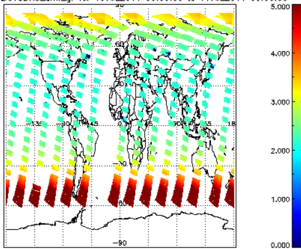
SCIOL2P_NADUV3BRO_amf_gr for 10JUL2011 00:00:00 to 11JUL2011 00:00:00
