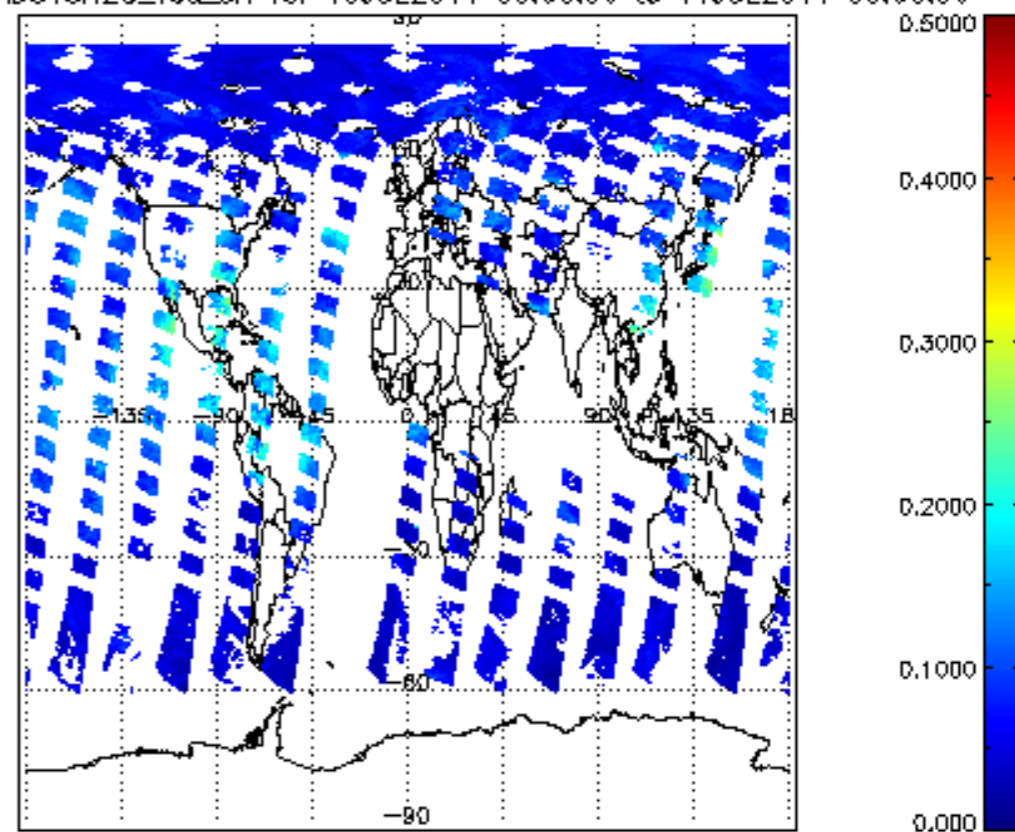
SCIOL2P_NADUV8H20_vcd_err for 10JUL2011 00:00:00 to 11JUL2011 00:00:00
