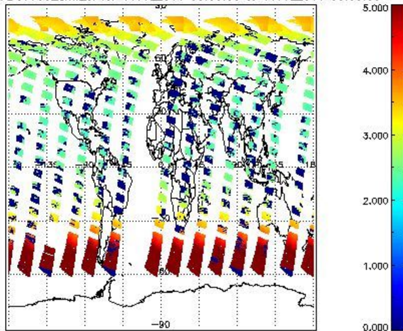
SCIOL2P_NADUV003_amf_cl for 10JUL2011 00:00:00 to 11JUL2011 00:00:00
