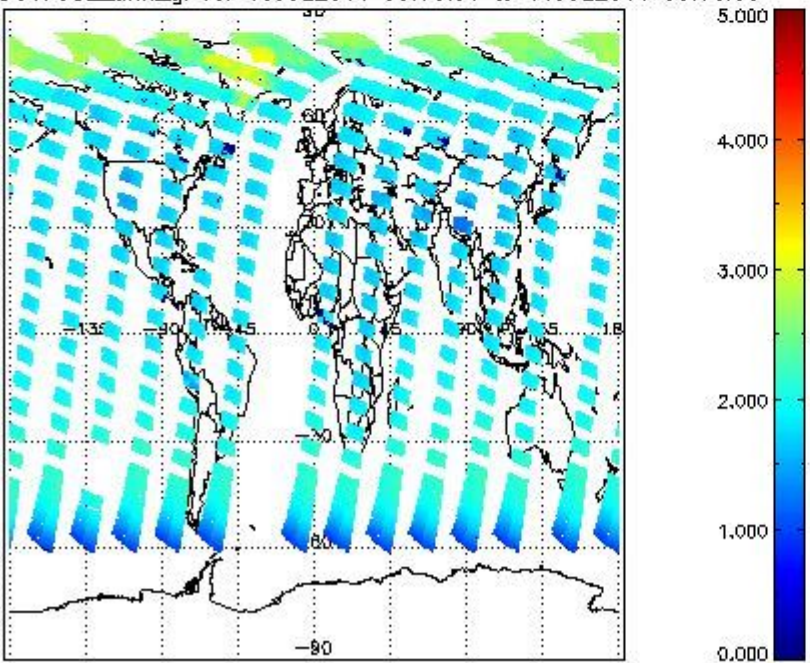
SCIOL2P_NADUV7S02_amf_gr for 10JUL2011 00:00:00 to 11JUL2011 00:00:00
