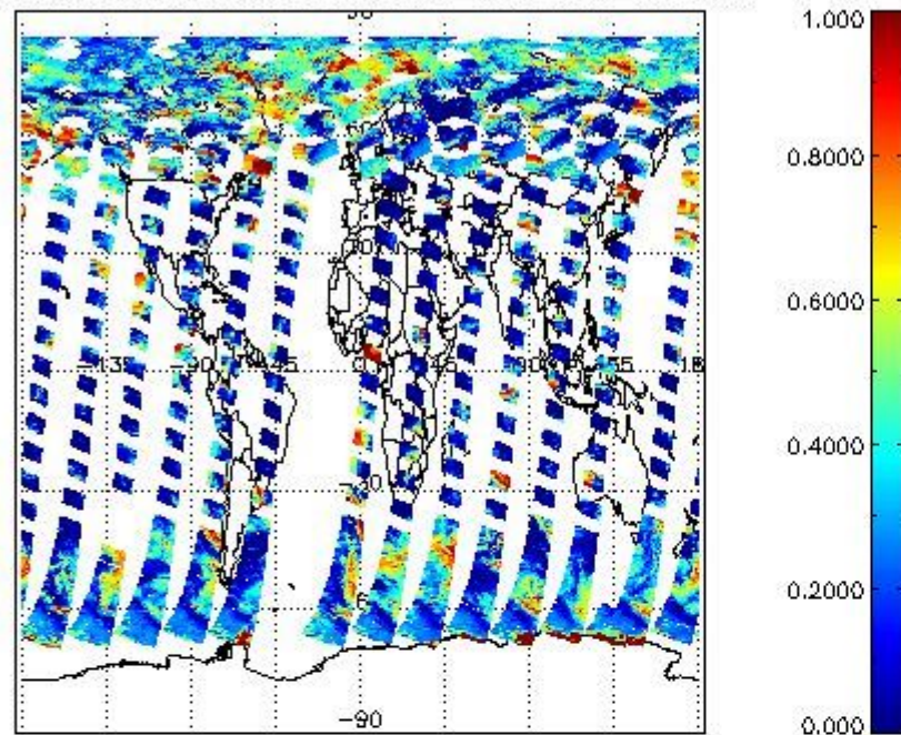
cL_frac for 10JUL2011 00:00:00 to 11JUL2011 00:00:00
