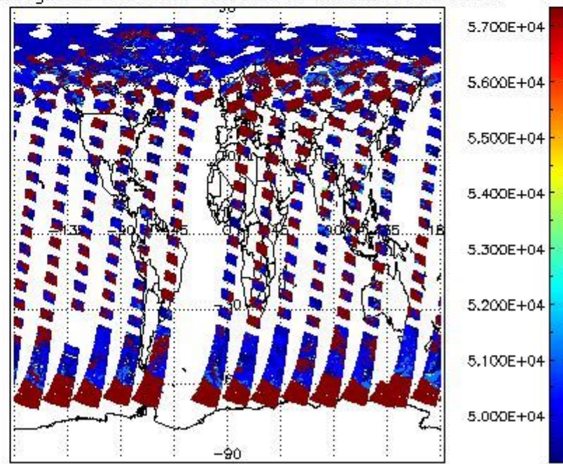
cloud_flags for 10JUL2011 00:00:00 to 11JUL2011 00:00:00
