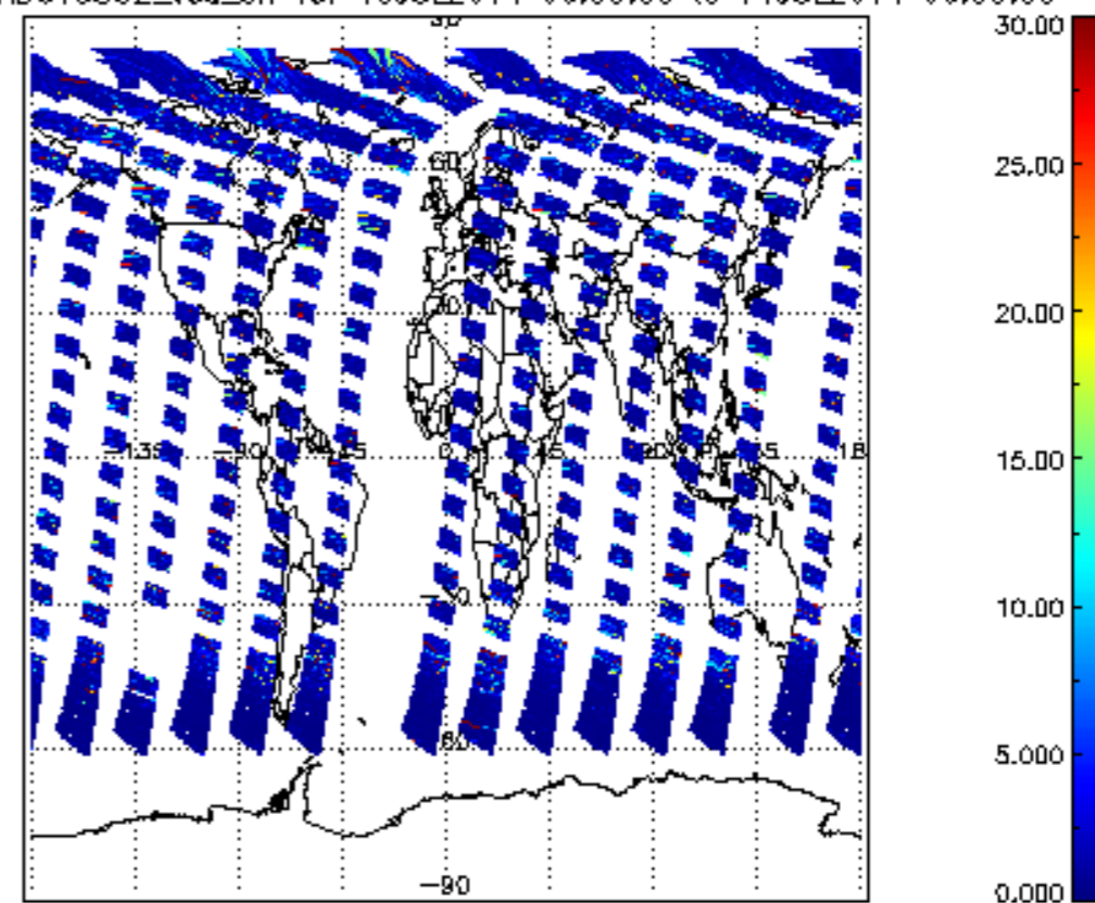
SCIOL2P_NADUV5S02_vcd_err for 10JUL2011 00:00:00 to 11JUL2011 00:00:00
