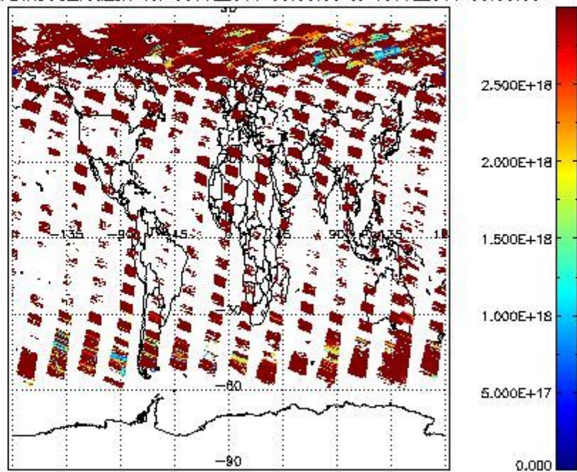
SCIDL2P_NADIR3CO_vcd_err for 09JUL2011 00:00:00 to 10JUL2011 00:00:00
