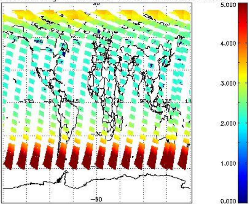
SCIOL2P_NADUV3BRO_amf_gr for 09JUL2011 00:00:00 to 10JUL2011 00:00:00
