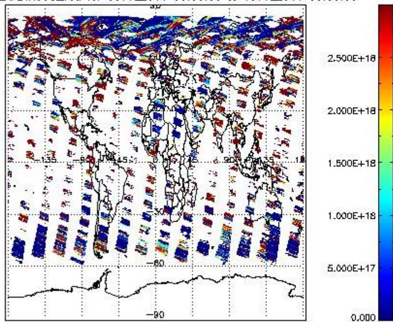
SCIDL2P_NADIR3CO_vcd for 09JUL2011 00:00:00 to 10JUL2011 00:00:00
