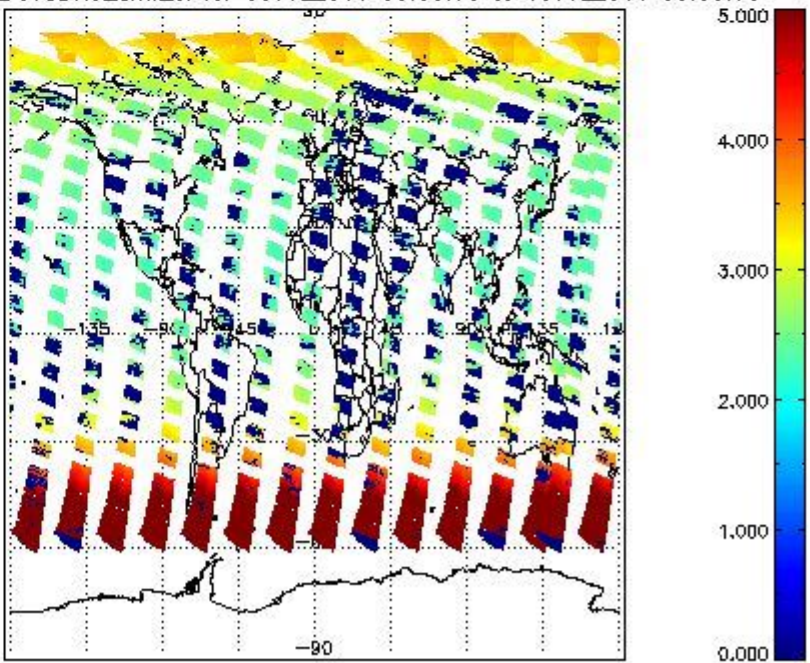
SCIOL2P_NADUV3BRO_amf_cl for 09JUL2011 00:00:00 to 10JUL2011 00:00:00
