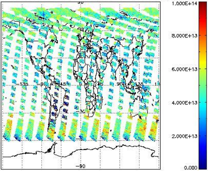
SCIOL2P_NADUV3BRO_vcd for 09JUL2011 00:00:00 to 10JUL2011 00:00:00
