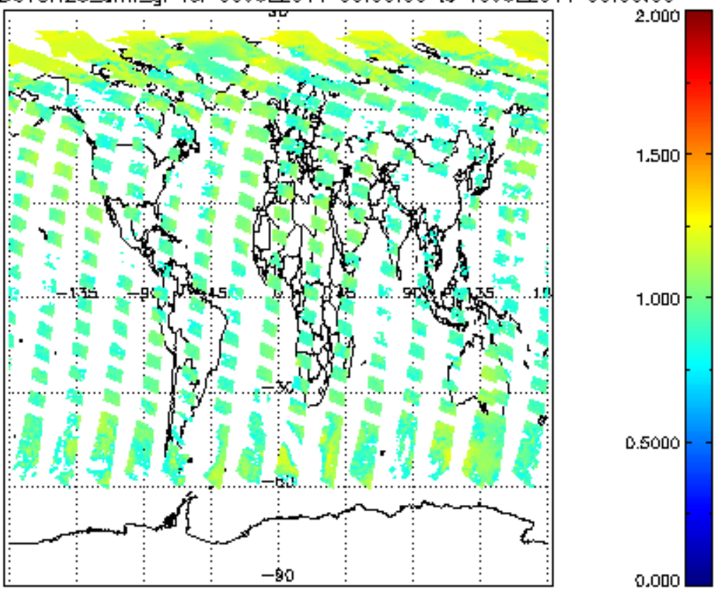
SCIOL2P_NADUV8H2O_amf_gr for 09JUL2011 00:00:00 to 10JUL2011 00:00:00
