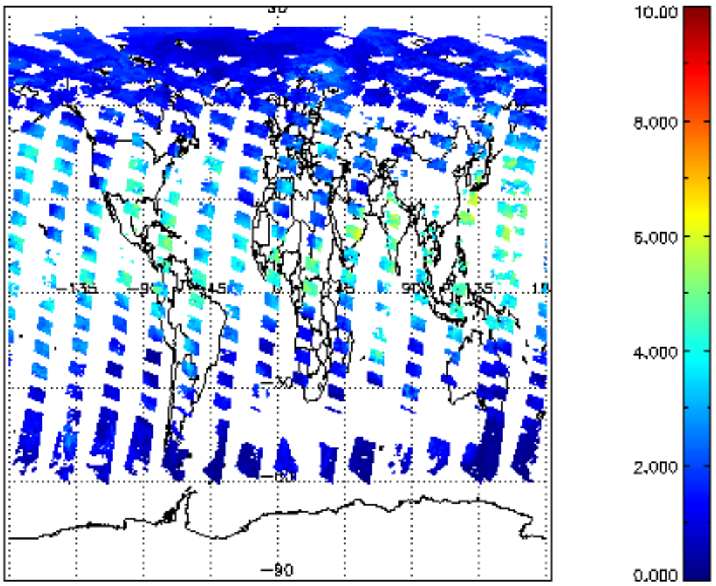
SCIOL2P_NADUV8H2O_vcd for 09JUL2011 00:00:00 to 10JUL2011 00:00:00
