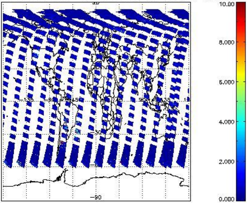
SCIOL2P_NADUV3BRO_vcd_err for 09JUL2011 00:00:00 to 10JUL2011 00:00:00
