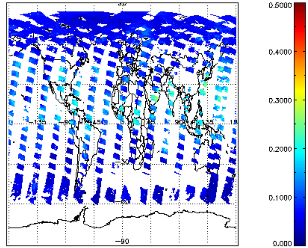
SCIOL2P_NADUV8H2O_vcd_err for 09JUL2011 00:00:00 to 10JUL2011 00:00:00
