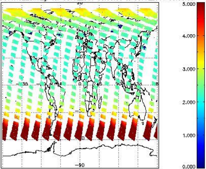
SCIOL2P_NADUV1NO2_amf_gr for 08JUL2011 00:00:00 to 09JUL2011 00:00:00
