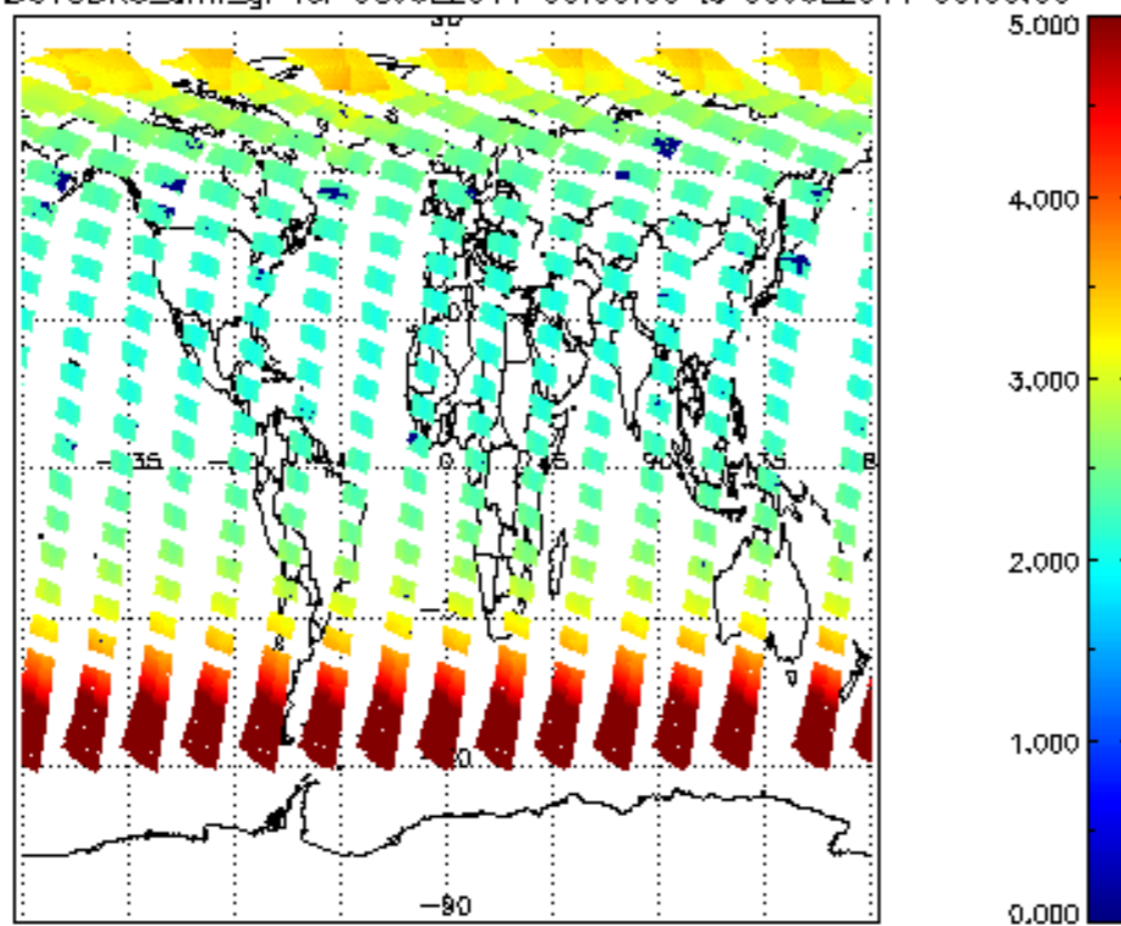
SCIOL2P_NADUV3BRO_amf_gr for 08JUL2011 00:00:00 to 09JUL2011 00:00:00
