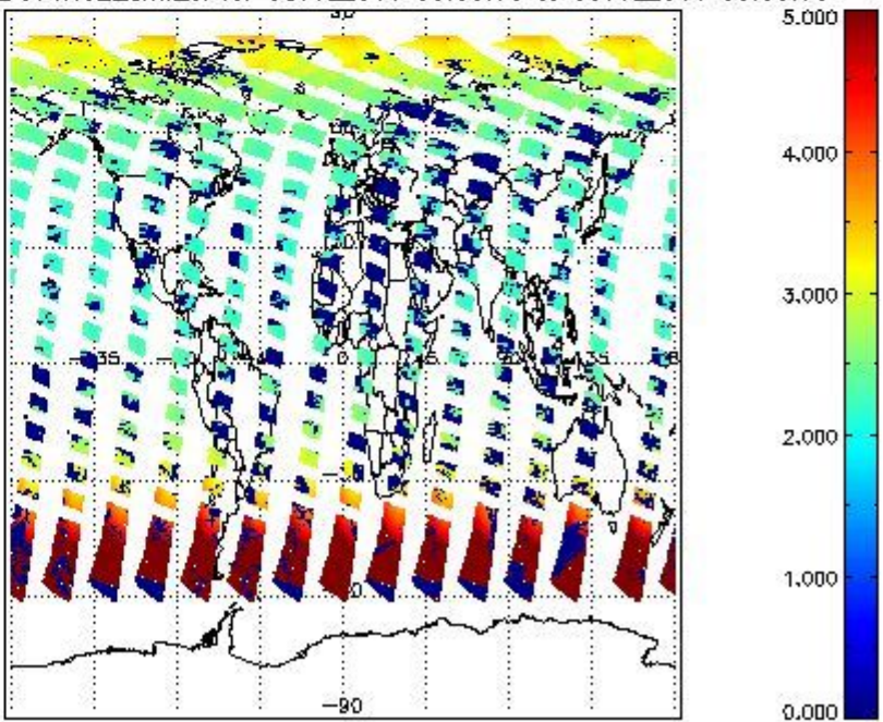
SCIOL2P_NADUV1NO2_amf_cl for 08JUL2011 00:00:00 to 09JUL2011 00:00:00
