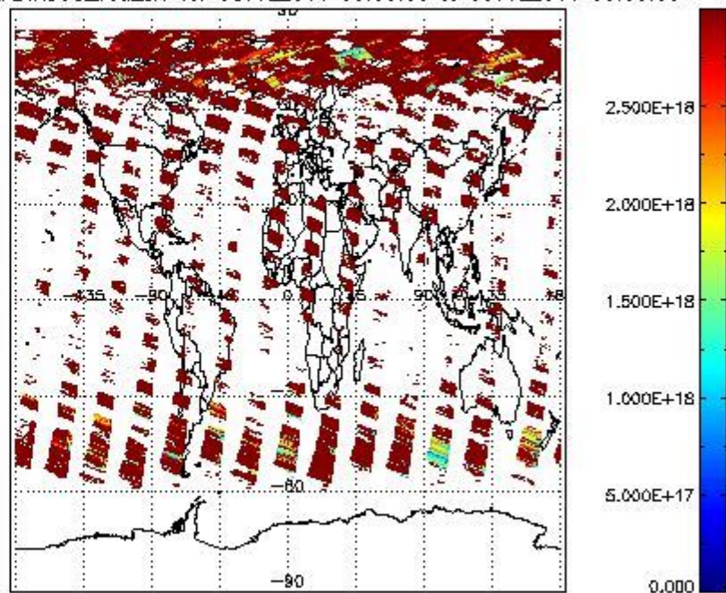
SCIDL2P_NADIR3CO_vcd_err for 08JUL2011 00:00:00 to 09JUL2011 00:00:00
