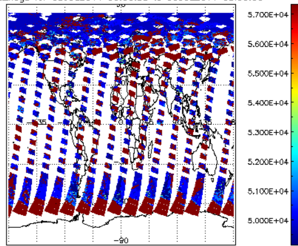
cloud_flags for 08JUL2011 00:00:00 to 09JUL2011 00:00:00
