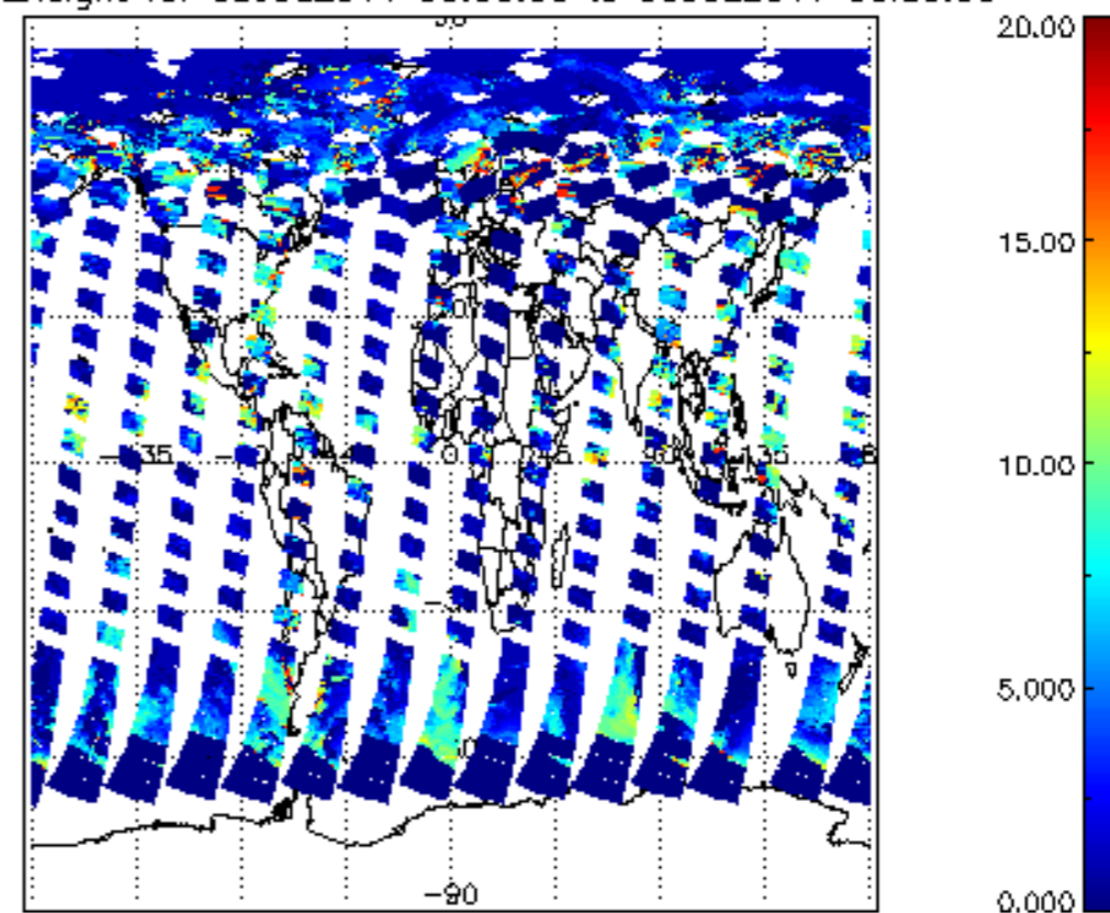
cl_top_height for 08JUL2011 00:00:00 to 09JUL2011 00:00:00
