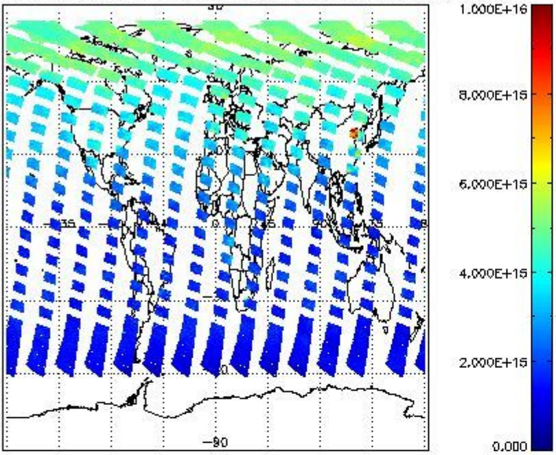
SCIOL2P_NADUV1NO2_vcd for 08JUL2011 00:00:00 to 09JUL2011 00:00:00
