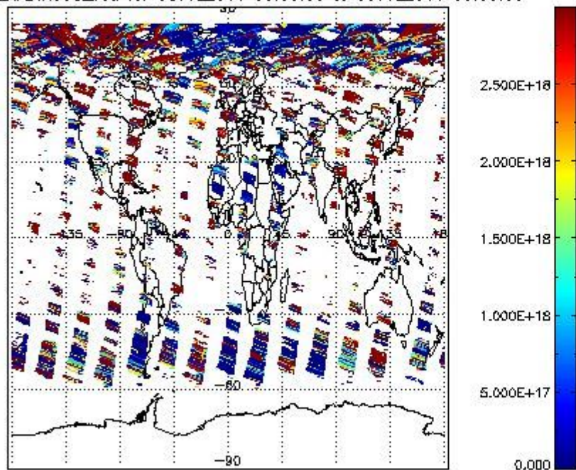
SCIDL2P_NADIR3CO_vcd for 08JUL2011 00:00:00 to 09JUL2011 00:00:00
