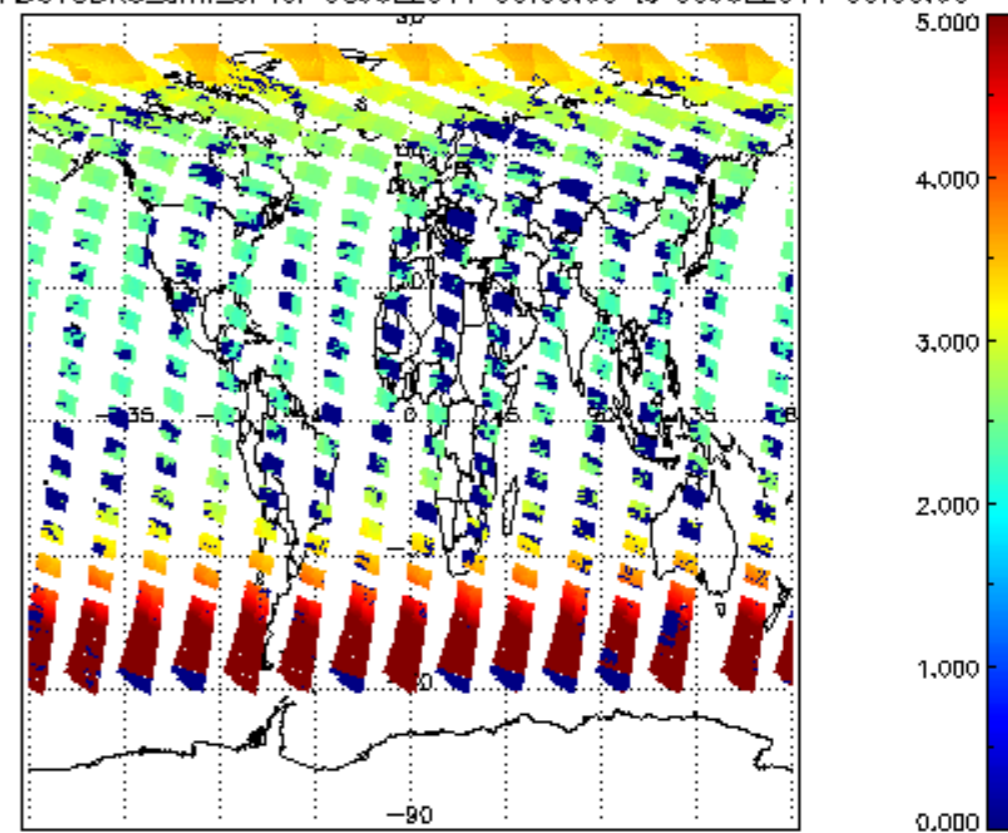
SCIOL2P_NADUV3BRO_amf_cl for 08JUL2011 00:00:00 to 09JUL2011 00:00:00
