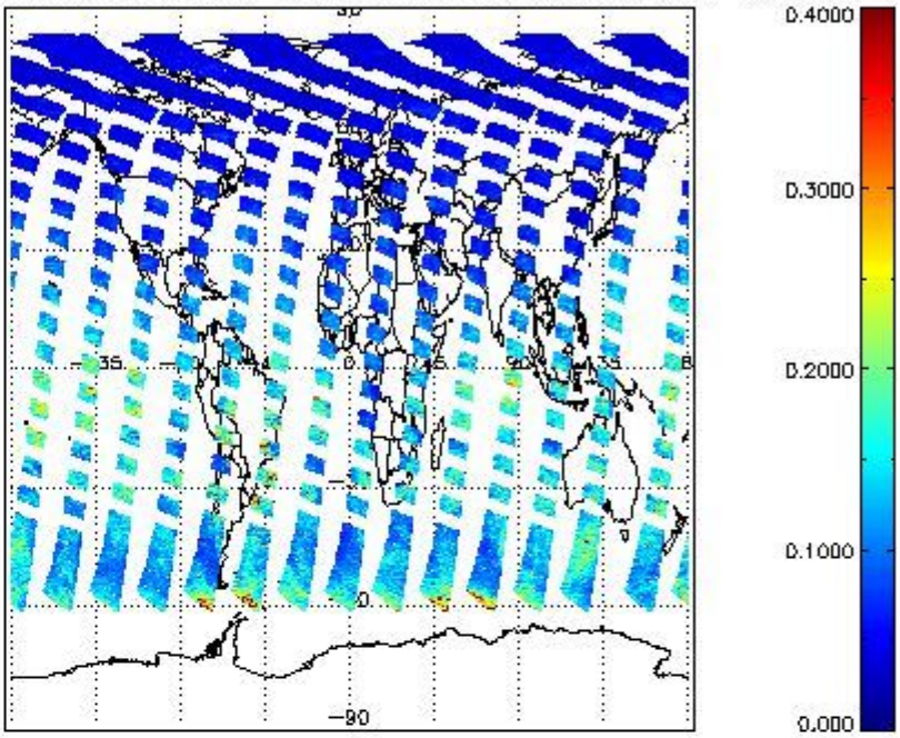
SCIOL2P_NADUV1NO2_vcd_err for 08JUL2011 00:00:00 to 09JUL2011 00:00:00
