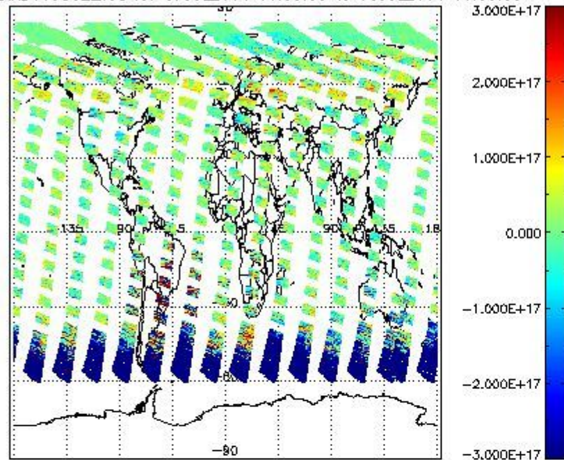
SCIOL2P_NADUV5S02_vcd for 07JUL2011 00:00:00 to 08JUL2011 00:00:00
