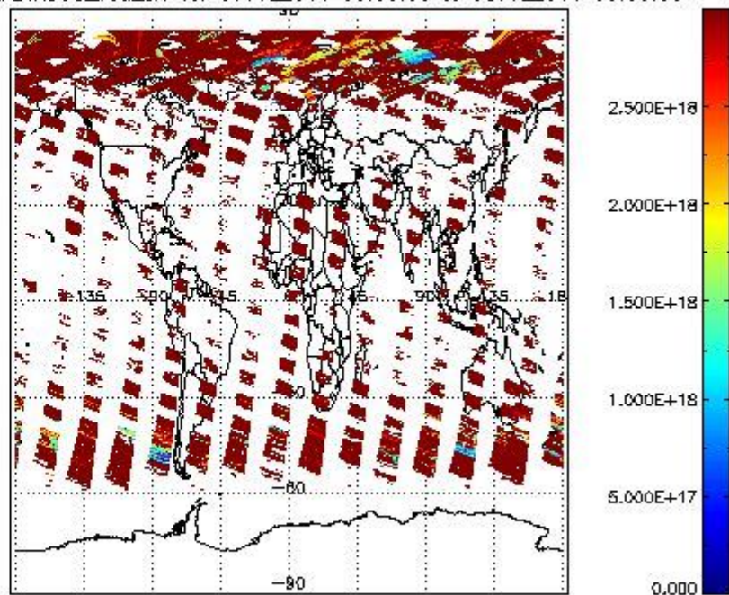
SCIDL2P_NADIR3CO_vcd_err for 07JUL2011 00:00:00 to 08JUL2011 00:00:00
