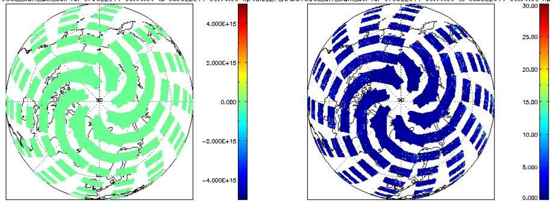
SCIOI2P_NADUV6OCLslant_col_den for 07JUL2011 00:00:00 to 08JUL2011 00:00:00 np SCIOI2P_NADUV6OCLlarr_slant_col for 07JUL2011 00:00:00 to 08JUL2011 00:00:00 np
