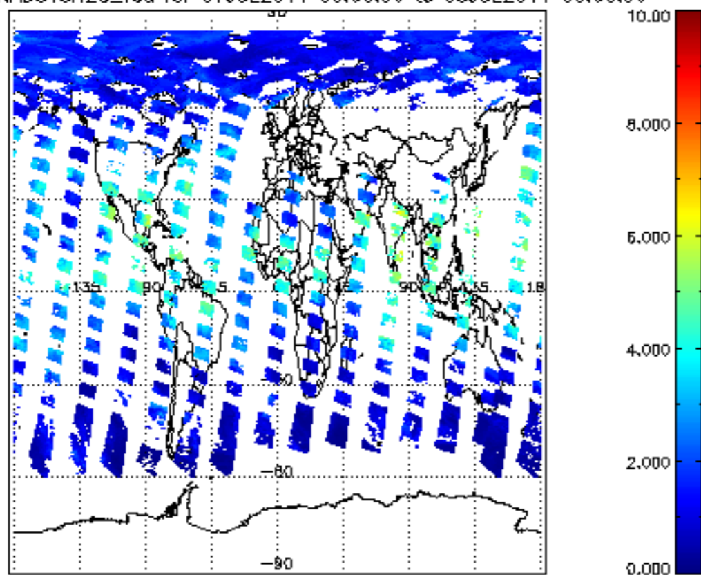
SCIOL2P_NADUV8H20_vcd for 07JUL2011 00:00:00 to 08JUL2011 00:00:00
