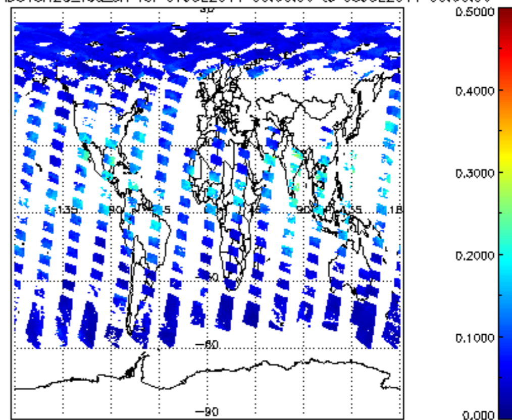
SCIOL2P_NADUV8H20_vcd_err for 07JUL2011 00:00:00 to 08JUL2011 00:00:00
