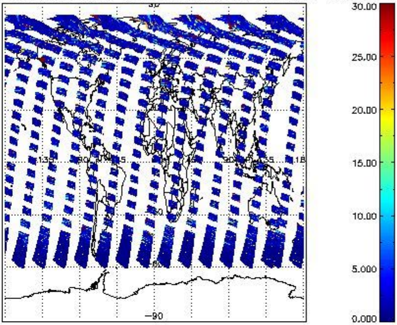
SCIOL2P_NADUV7S02_vcd_err for 07JUL2011 00:00:00 to 08JUL2011 00:00:00
