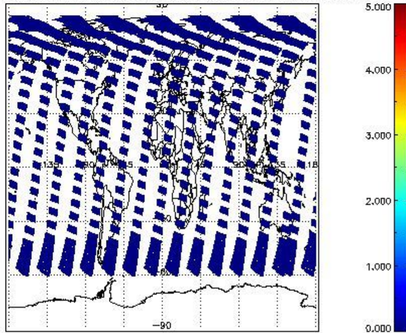
SCIOL2P_NADUV5S02_amf_cl for 07JUL2011 00:00:00 to 08JUL2011 00:00:00
