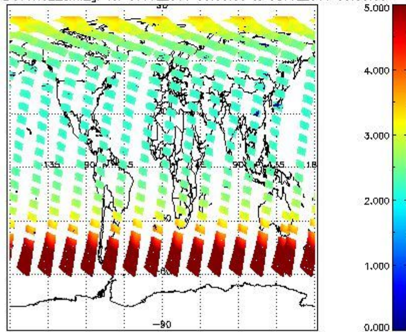
SCIOL2P_NADUV1NO2_amf_gr for 07JUL2011 00:00:00 to 08JUL2011 00:00:00
