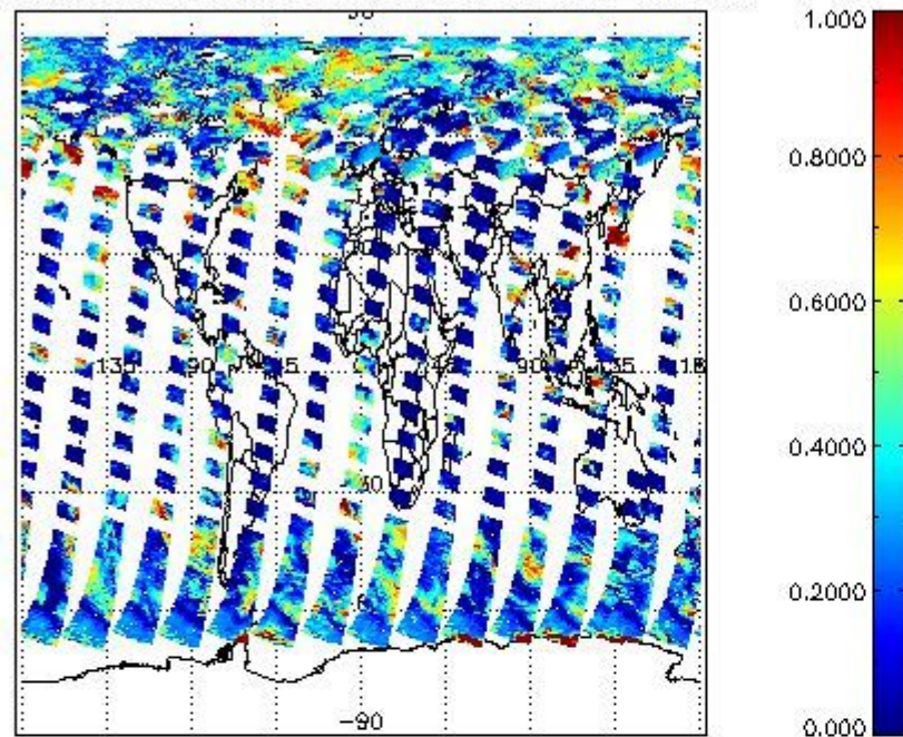
cL_frac for 07JUL2011 00:00:00 to 08JUL2011 00:00:00
