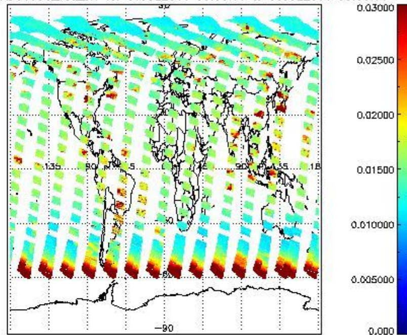
SCIOL2P_NADUV003_vcd_err for 07JUL2011 00:00:00 to 08JUL2011 00:00:00
