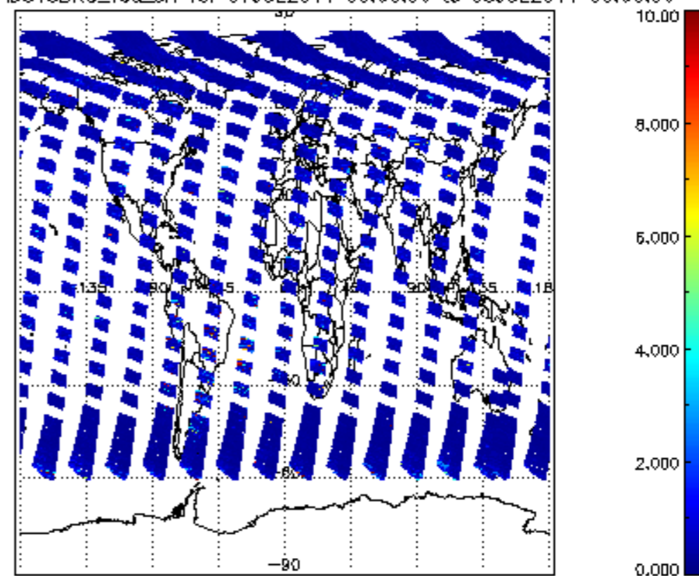
SCIOL2P_NADUV3BRO_vcd_err for 07JUL2011 00:00:00 to 08JUL2011 00:00:00
