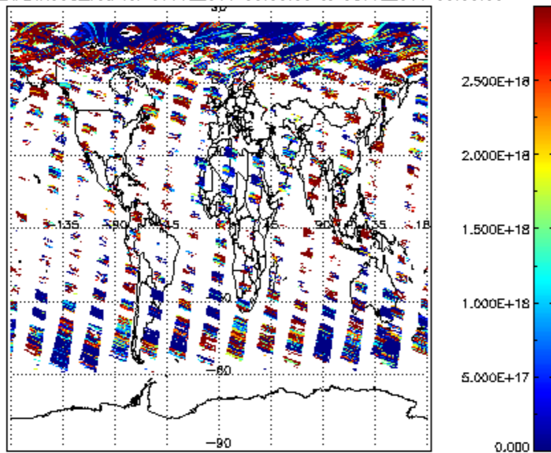
SCIOL2P_NADIR3CO_vcd for 07JUL2011 00:00:00 to 08JUL2011 00:00:00
