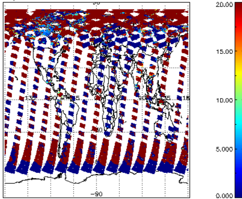
cl_lopt_depth for 07JUL2011 00:00:00 to 08JUL2011 00:00:00
