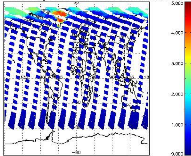
SCIOL2P_NADUV5S02_amf_gr for 07JUL2011 00:00:00 to 08JUL2011 00:00:00
