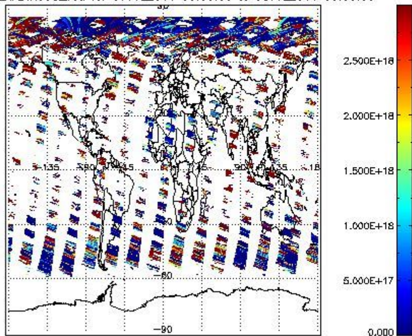
SCIDL2P_NADIR3CO_vcd for 07JUL2011 00:00:00 to 08JUL2011 00:00:00
