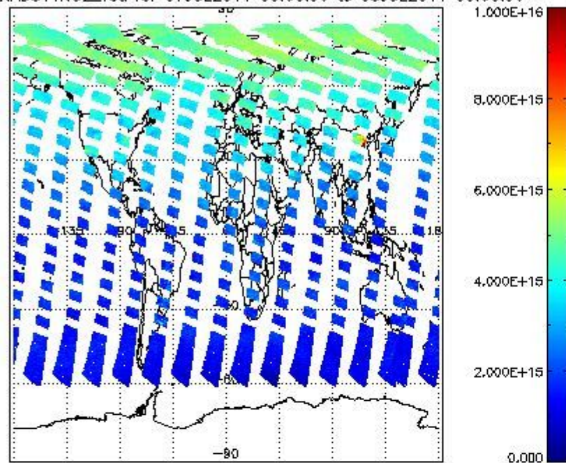
SCIOL2P_NADUV1NO2_vcd for 07JUL2011 00:00:00 to 08JUL2011 00:00:00
