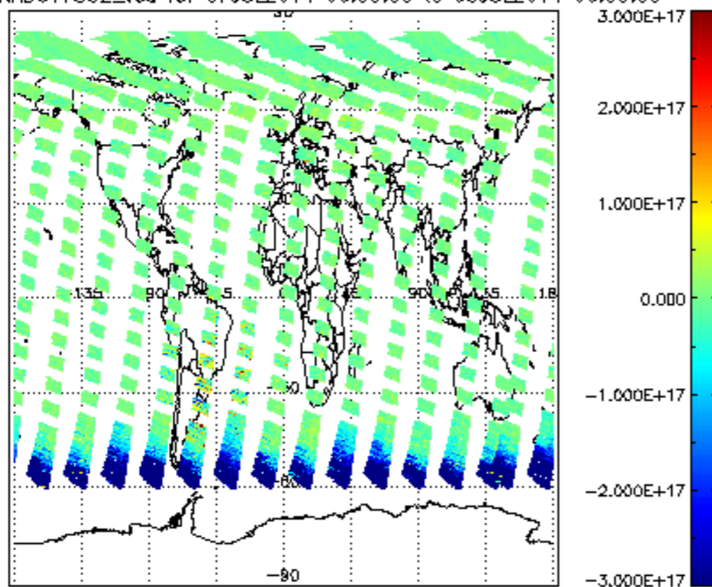
SCIOL2P_NADUV7S02_vcd for 07JUL2011 00:00:00 to 08JUL2011 00:00:00
