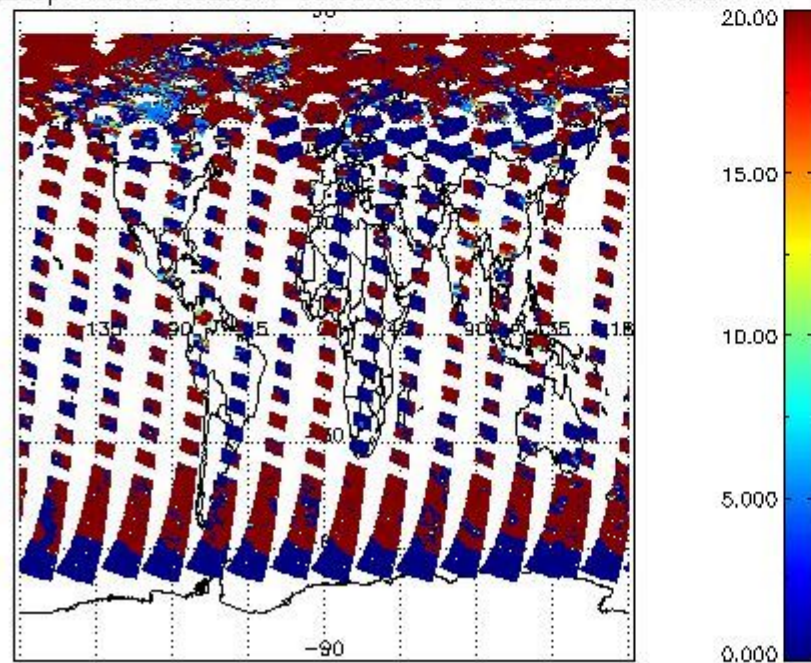
cL_opt_depth for 07JUL2011 00:00:00 to 08JUL2011 00:00:00
