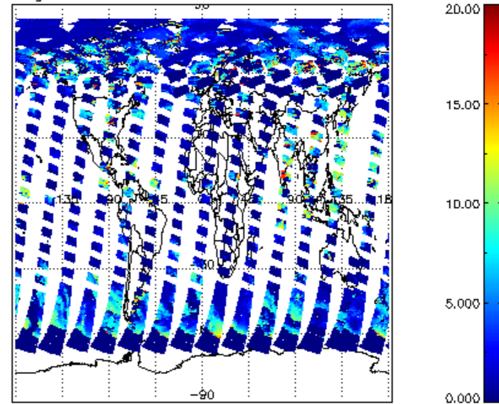
cl_top_height for 07JUL2011 00:00:00 to 08JUL2011 00:00:00
