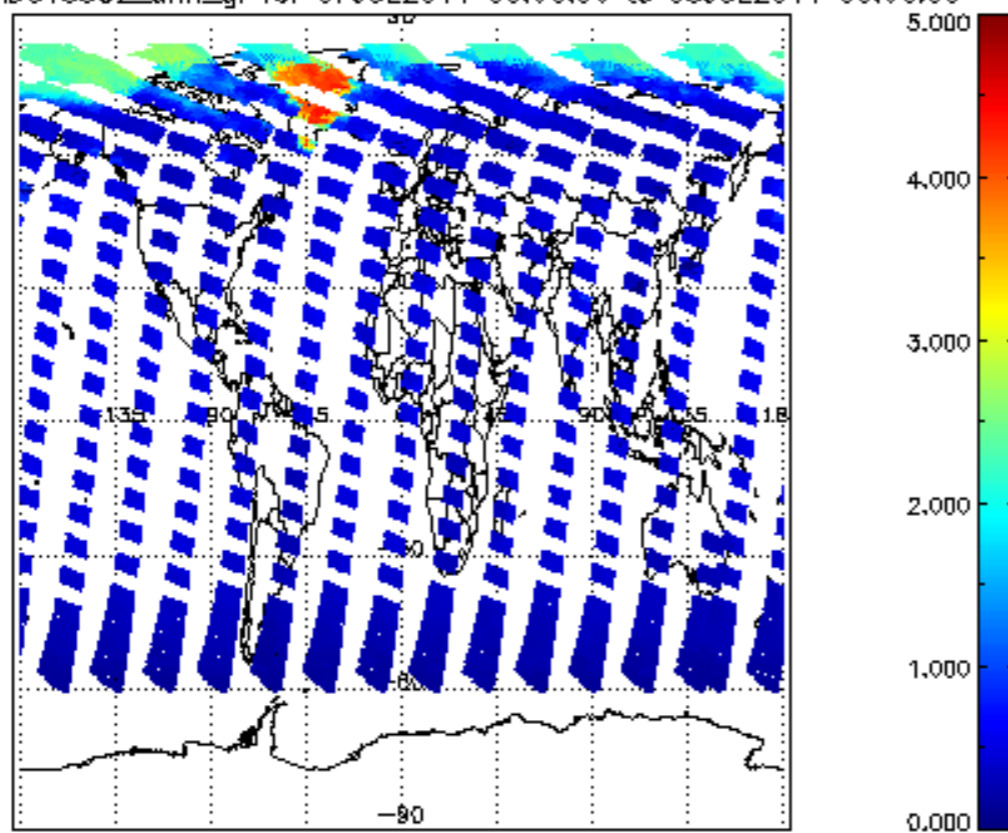
SCIOL2P_NADUV5S02_amf_gr for 07JUL2011 00:00:00 to 08JUL2011 00:00:00
