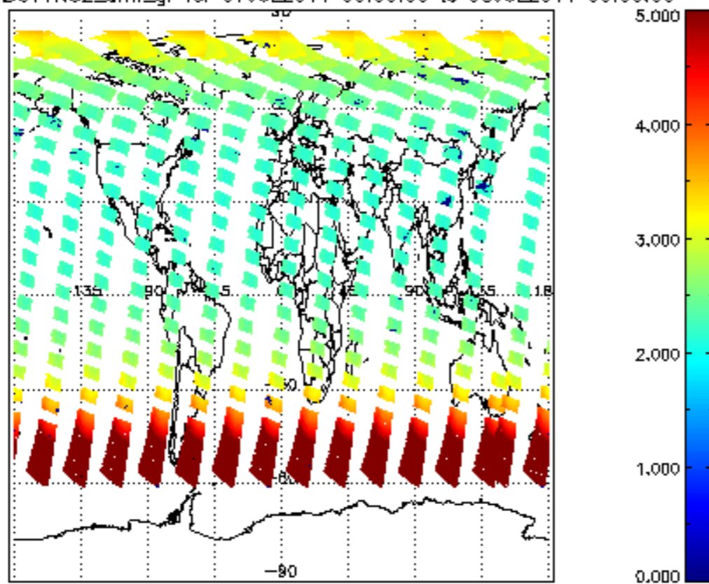
SCIOL2P_NADUV1N02_amf_gr for 07JUL2011 00:00:00 to 08JUL2011 00:00:00
