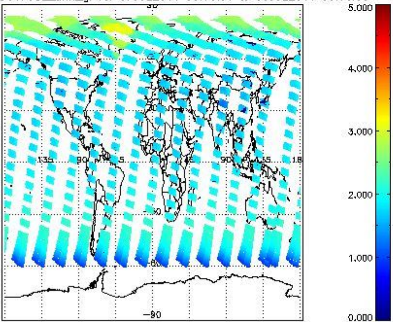
SCIOL2P_NADUV7S02_amf_gr for 07JUL2011 00:00:00 to 08JUL2011 00:00:00
