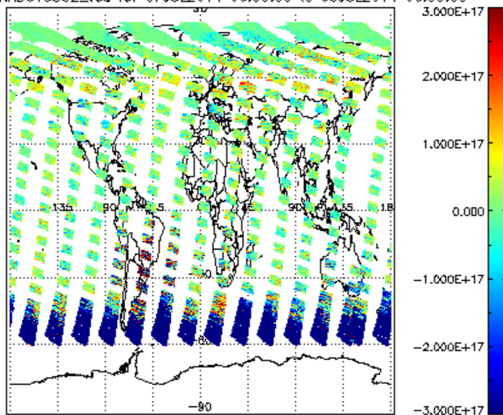
SCIOL2P_NADUV5S02_vcd for 07JUL2011 00:00:00 to 08JUL2011 00:00:00
