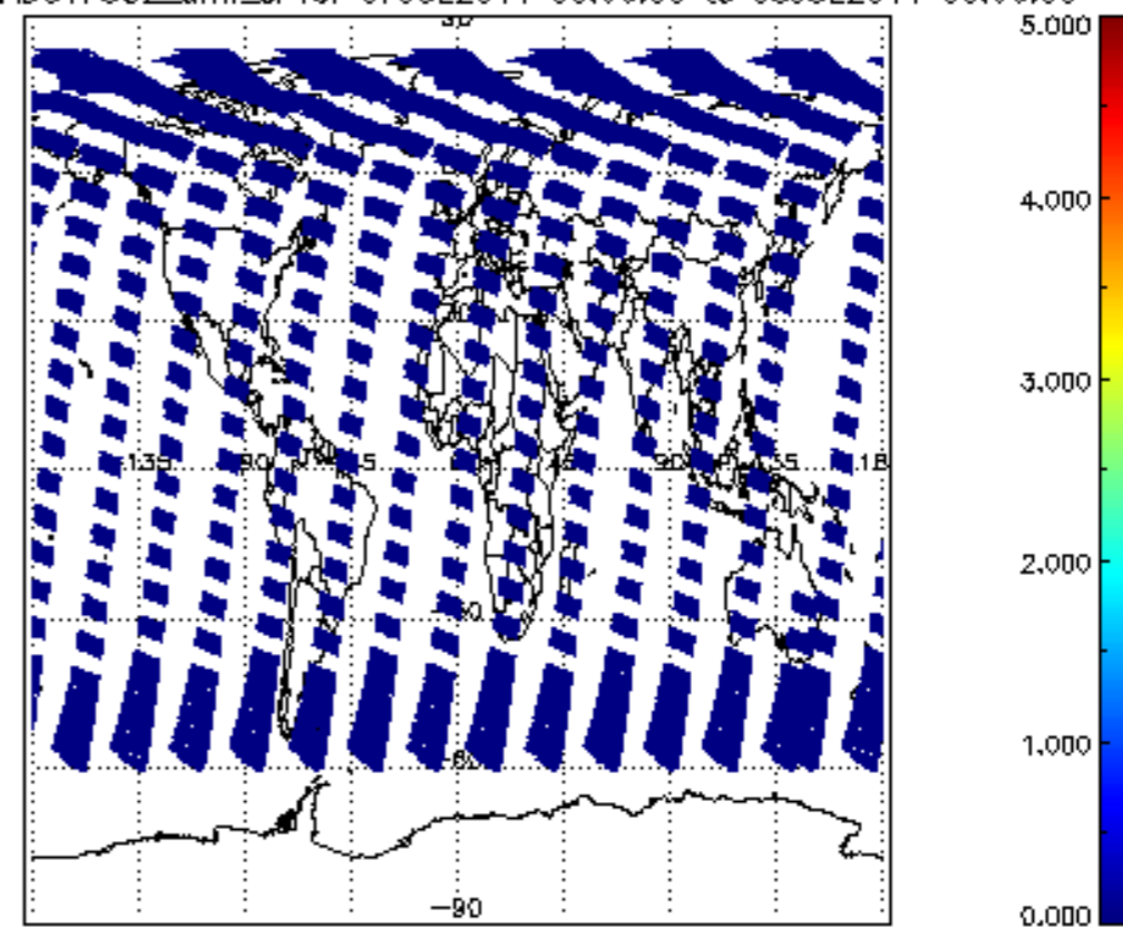
SCIOL2P_NADUV7S02_amf_cl for 07JUL2011 00:00:00 to 08JUL2011 00:00:00
