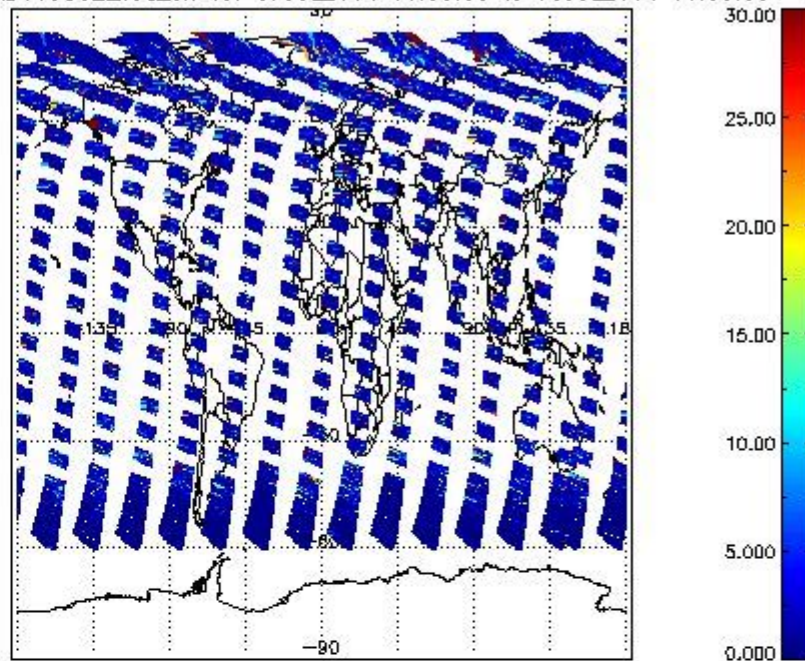
SCIOL2P_NADUV5S02_vcd_err for 07JUL2011 00:00:00 to 08JUL2011 00:00:00
