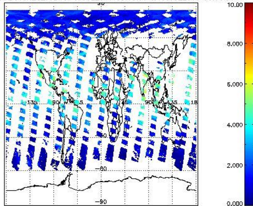
SCIOL2P_NADUV8H2O_vcd for 07JUL2011 00:00:00 to 08JUL2011 00:00:00
