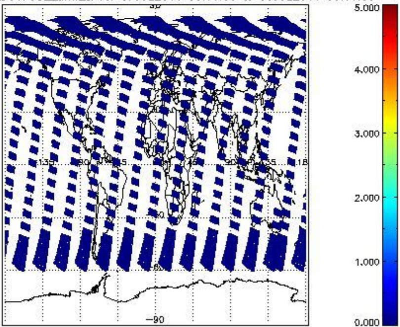
SCIOL2P_NADUV7S02_amf_cl for 07JUL2011 00:00:00 to 08JUL2011 00:00:00
