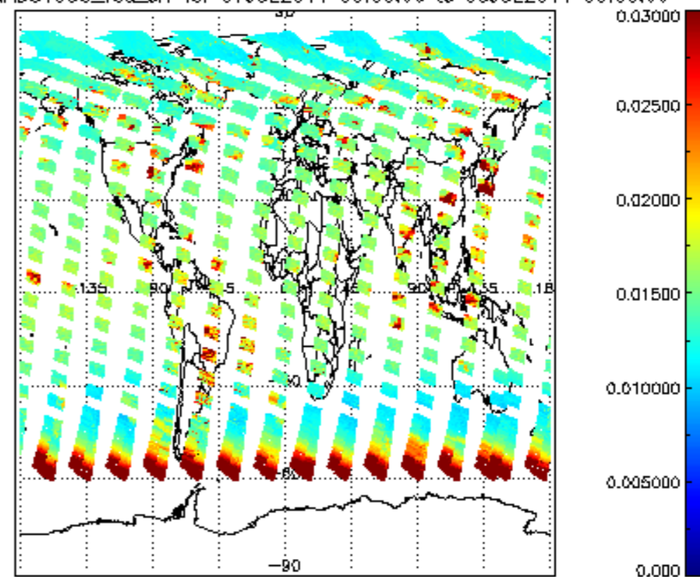
SCIOL2P_NADUV003_vcd_err for 07JUL2011 00:00:00 to 08JUL2011 00:00:00
