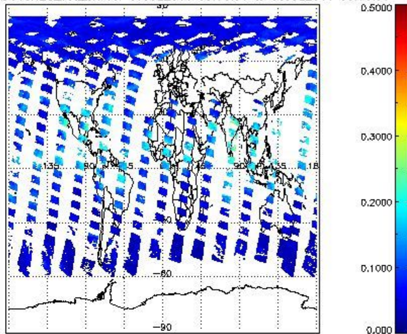
SCIOL2P_NADUV8H2O_vcd_err for 07JUL2011 00:00:00 to 08JUL2011 00:00:00
