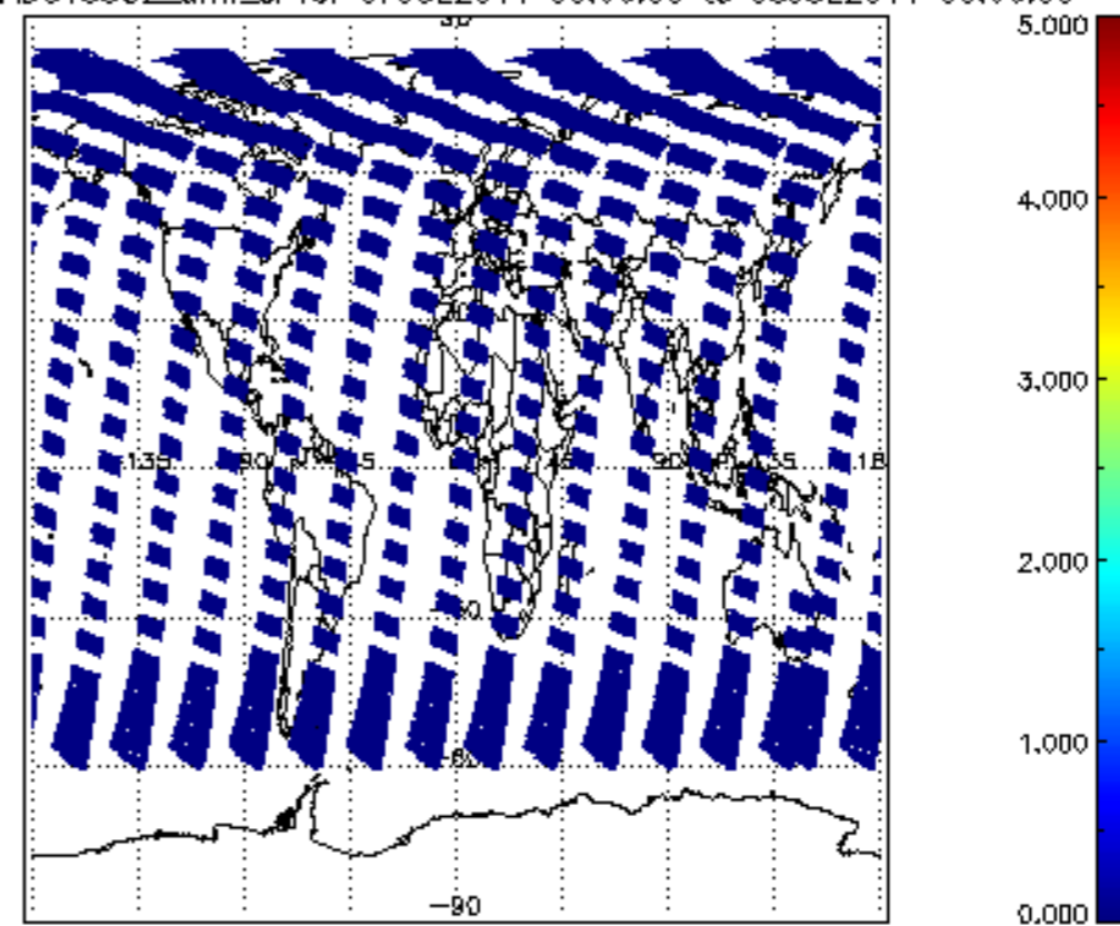
SCIOL2P_NADUV5S02_amf_cl for 07JUL2011 00:00:00 to 08JUL2011 00:00:00
