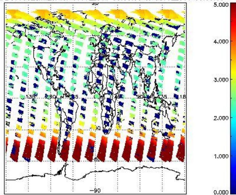
SCIOL2P_NADUV003_amf_cl for 07JUL2011 00:00:00 to 08JUL2011 00:00:00
