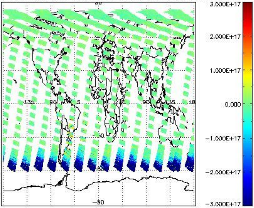
SCIOL2P_NADUV7S02_vcd for 07JUL2011 00:00:00 to 08JUL2011 00:00:00
