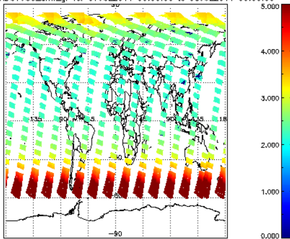
SCIOL2P_NADUV003_amf_gr for 07JUL2011 00:00:00 to 08JUL2011 00:00:00
