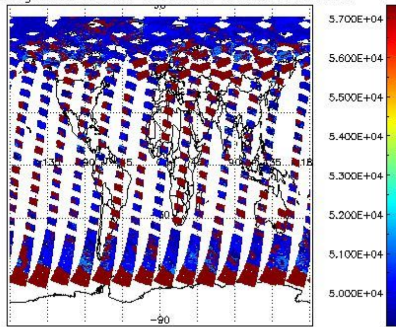
cloud_flags for 07JUL2011 00:00:00 to 08JUL2011 00:00:00
