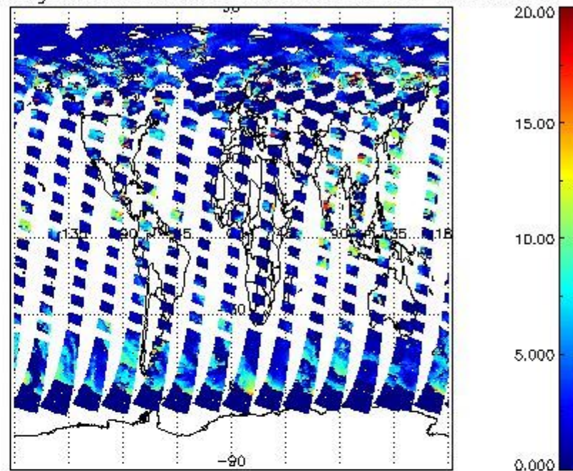
cL_top_height for 07JUL2011 00:00:00 to 08JUL2011 00:00:00
