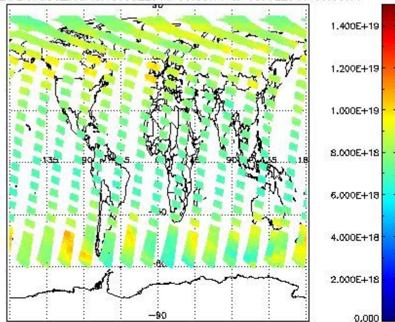
SCIOL2P_NADUV003_vcd for 07JUL2011 00:00:00 to 08JUL2011 00:00:00
