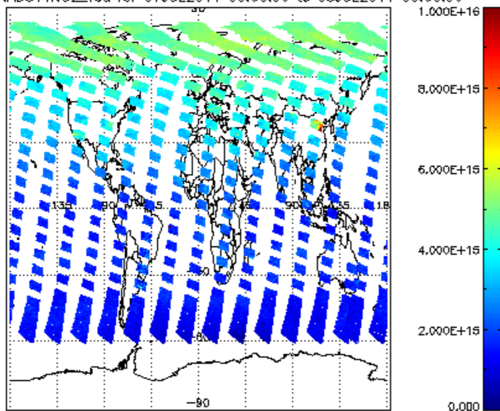
SCIOL2P_NADUV1N02_vcd for 07JUL2011 00:00:00 to 08JUL2011 00:00:00
