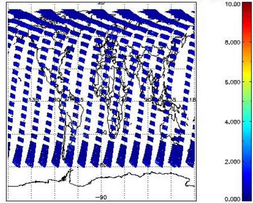
SCIOL2P_NADUV3BRO_vcd_err for 07JUL2011 00:00:00 to 08JUL2011 00:00:00
