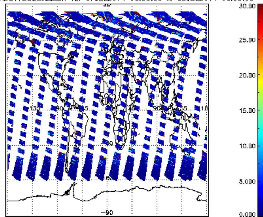
SCIOL2P_NADUV7S02_vcd_err for 07JUL2011 00:00:00 to 08JUL2011 00:00:00
