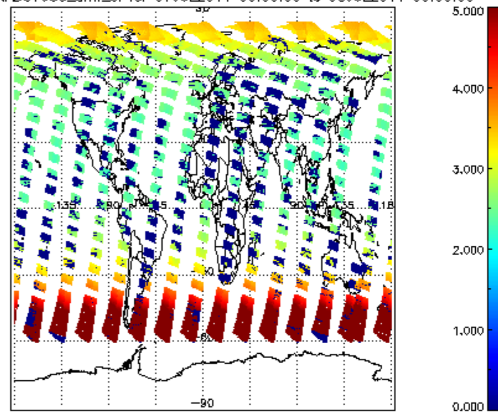
SCIOL2P_NADUV003_amf_cl for 07JUL2011 00:00:00 to 08JUL2011 00:00:00
