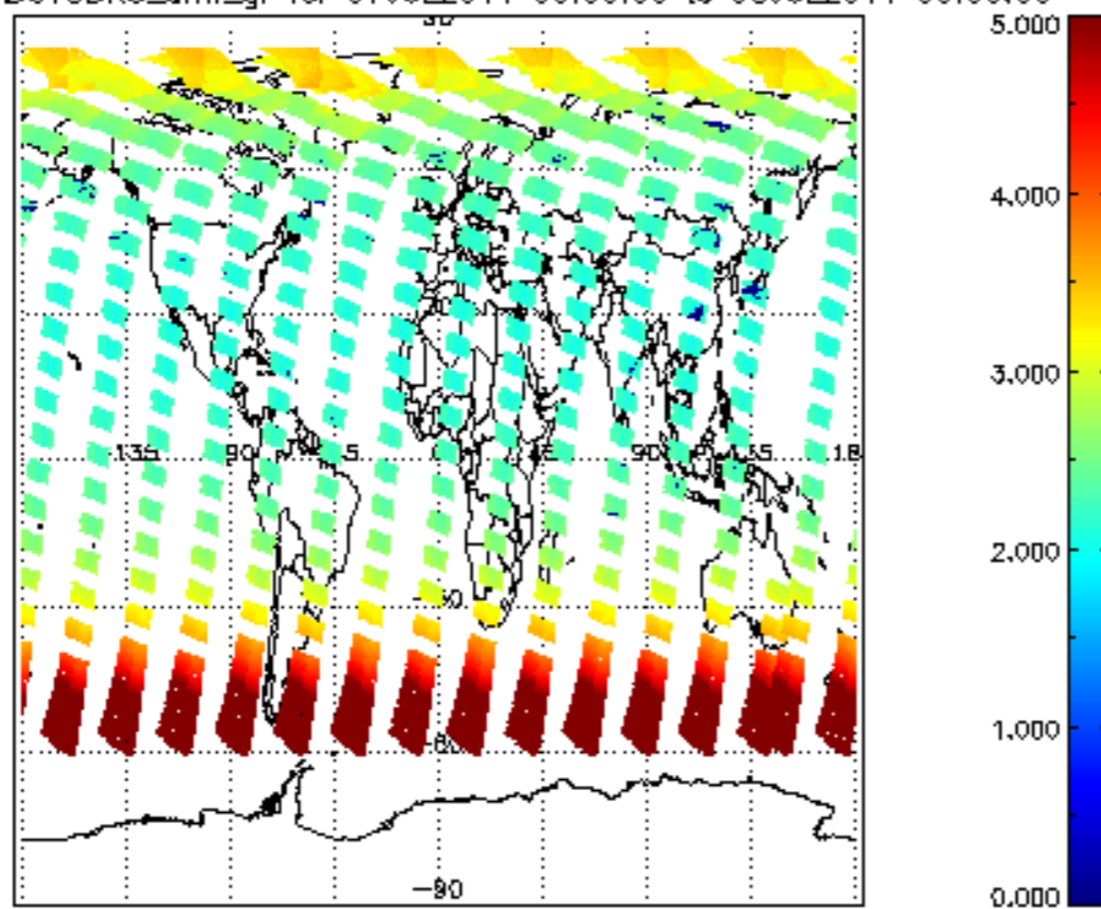
SCIOL2P_NADUV3BRO_arnf_gr for 07JUL2011 00:00:00 to 08JUL2011 00:00:00
