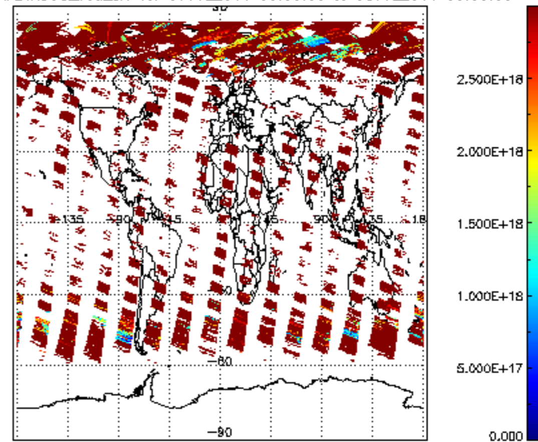
SCIOL2P_NADIR3CO_vcd_err for 07JUL2011 00:00:00 to 08JUL2011 00:00:00
