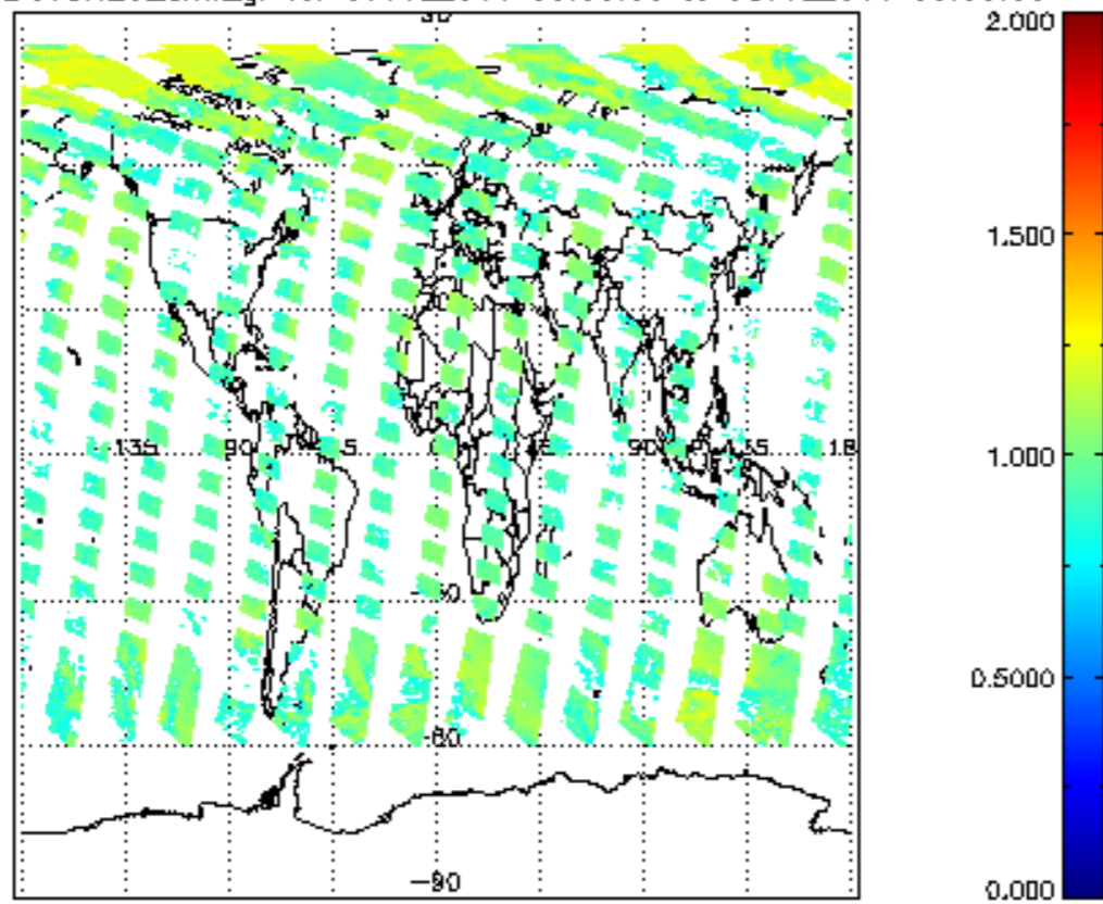
SCIOL2P_NADUV8H20_amf_gr for 07JUL2011 00:00:00 to 08JUL2011 00:00:00
