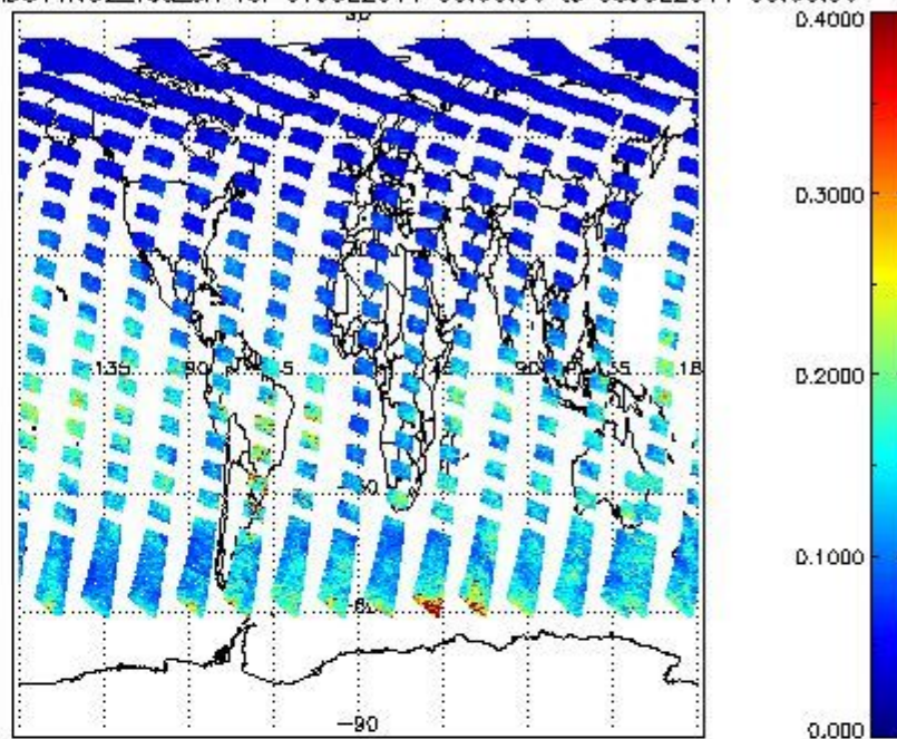
SCIOL2P_NADUV1NO2_vcd_err for 07JUL2011 00:00:00 to 08JUL2011 00:00:00
