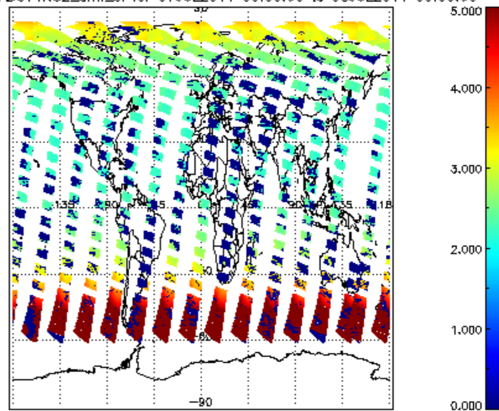
SCIOL2P_NADUV1N02_amf_cl for 07JUL2011 00:00:00 to 08JUL2011 00:00:00
