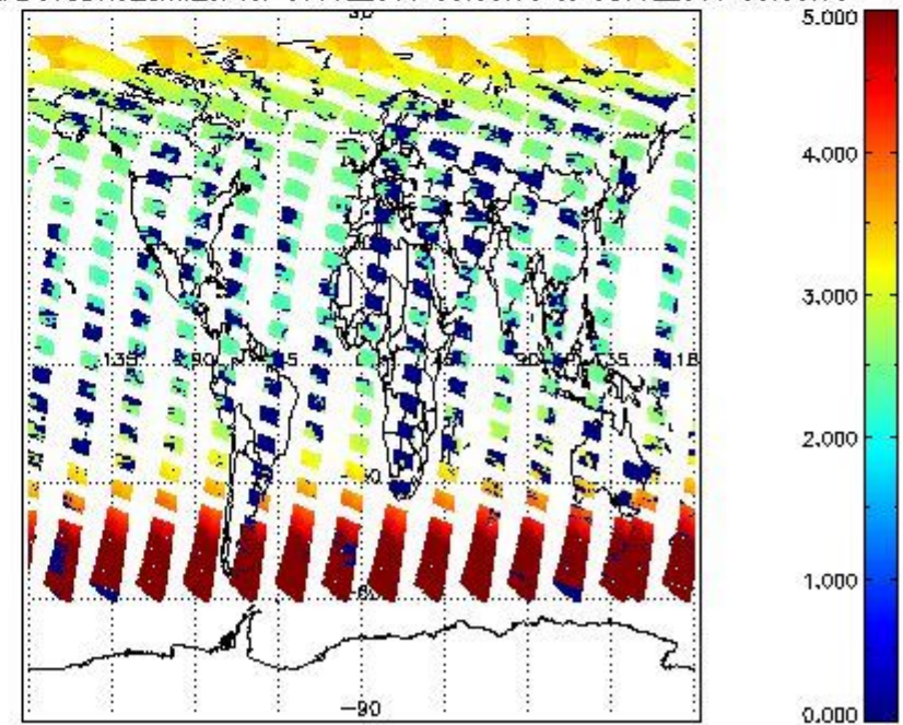
SCIOL2P_NADUV3BRO_amf_cl for 07JUL2011 00:00:00 to 08JUL2011 00:00:00
