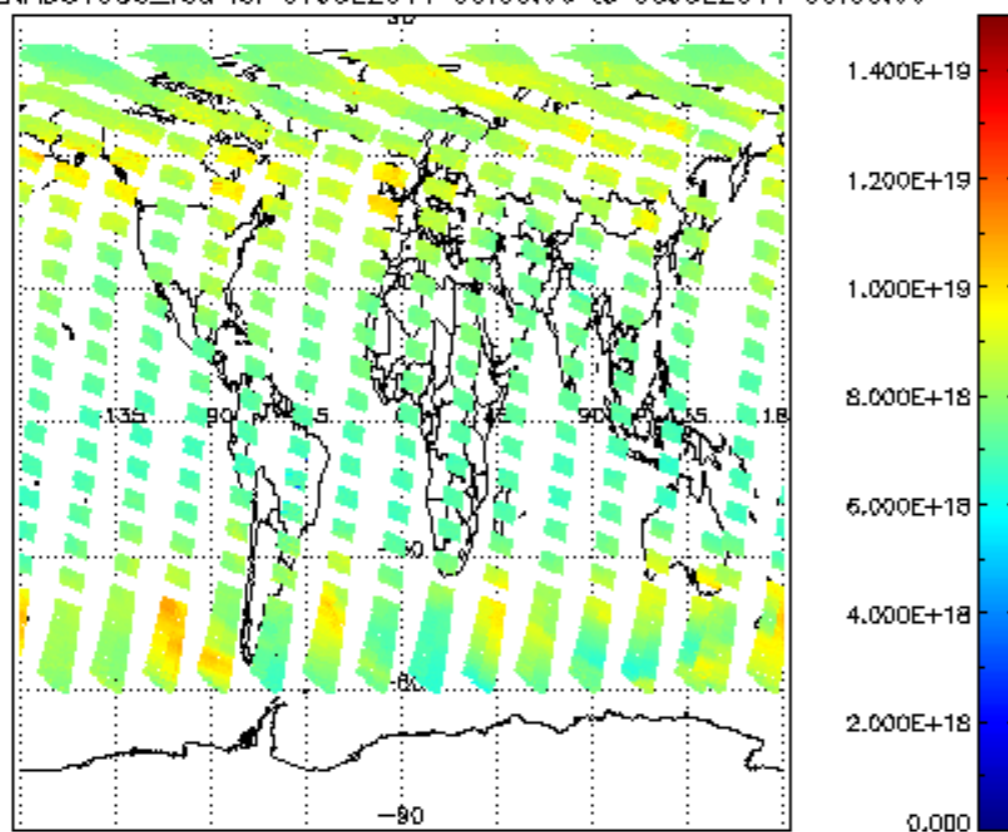
SCIOL2P_NADUV003_vcd for 07JUL2011 00:00:00 to 08JUL2011 00:00:00
