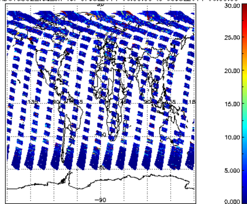
SCIOL2P_NADUV5S02_vcd_err for 07JUL2011 00:00:00 to 08JUL2011 00:00:00
