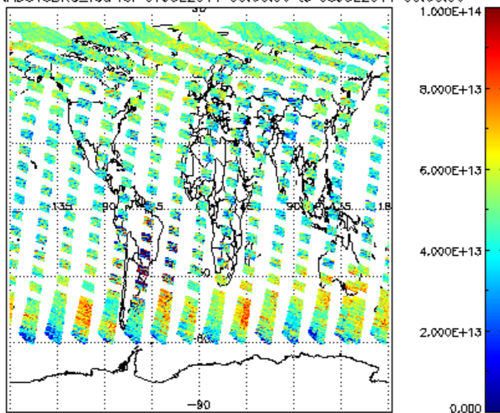
SCIOL2P_NADUV3BRO_vcd for 07JUL2011 00:00:00 to 08JUL2011 00:00:00
