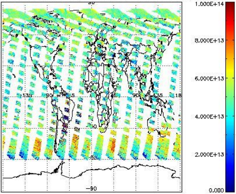
SCIOL2P_NADUV3BRO_vcd for 07JUL2011 00:00:00 to 08JUL2011 00:00:00
