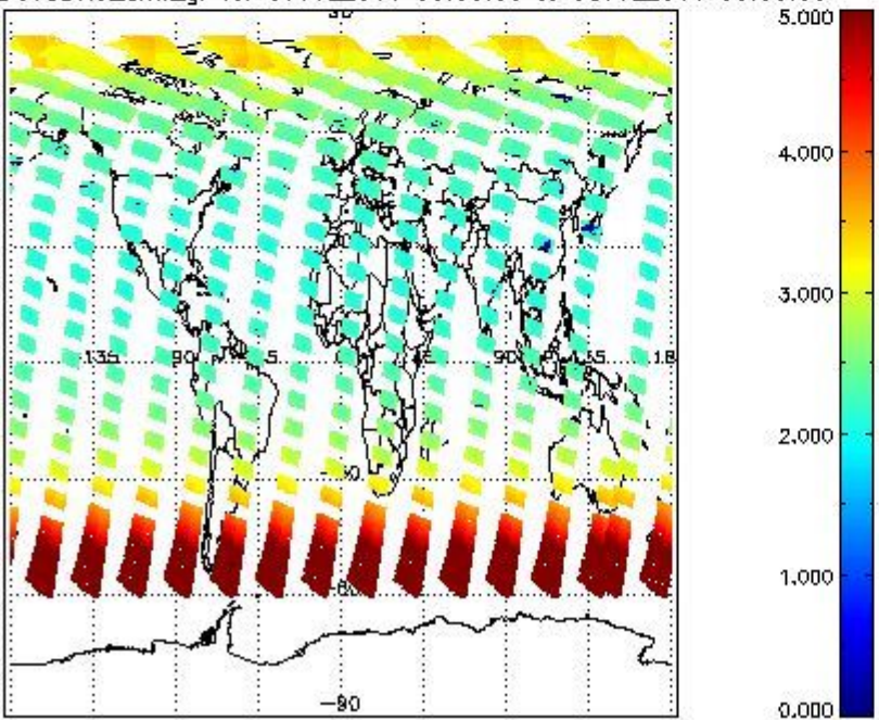
SCIOL2P_NADUV3BRO_amf_gr for 07JUL2011 00:00:00 to 08JUL2011 00:00:00
