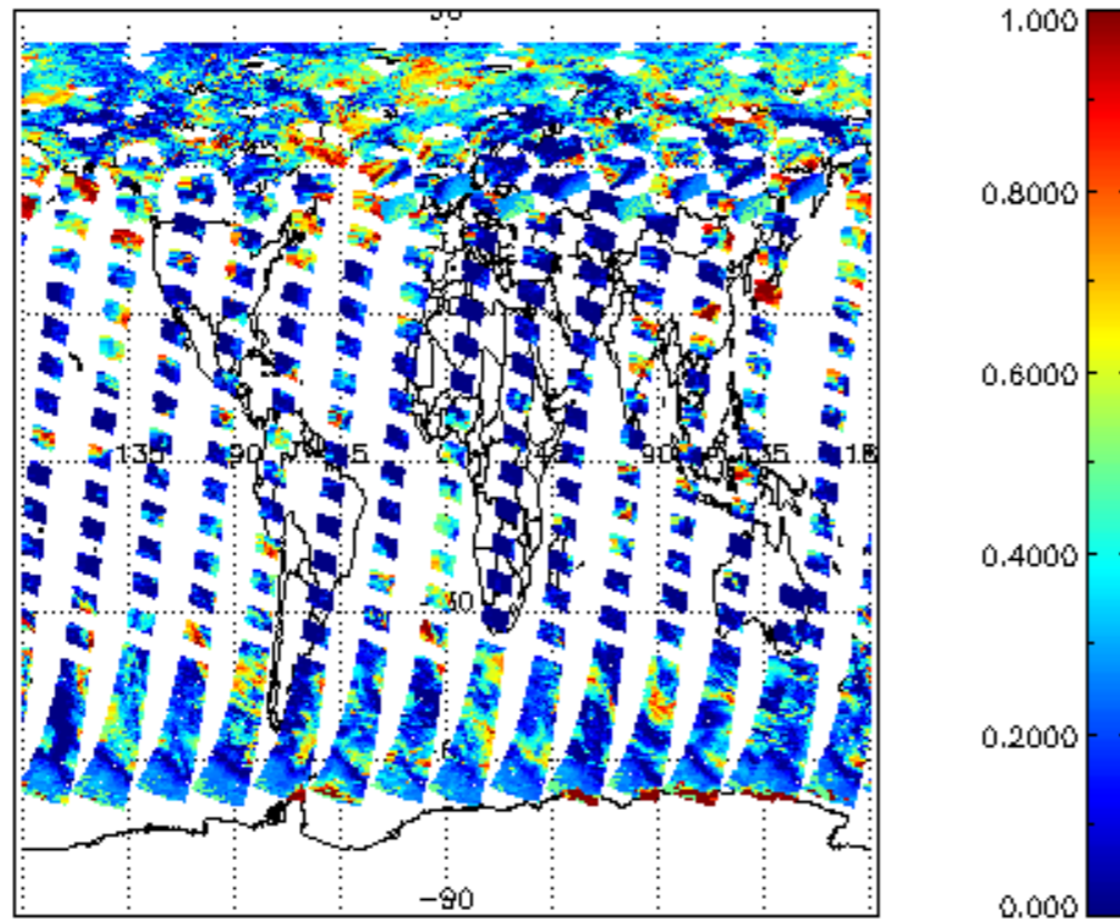
cl_frac for 07JUL2011 00:00:00 to 08JUL2011 00:00:00
