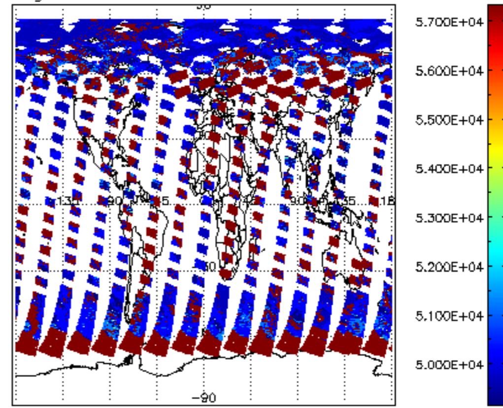
cloud_flags for 07JUL2011 00:00:00 to 08JUL2011 00:00:00
