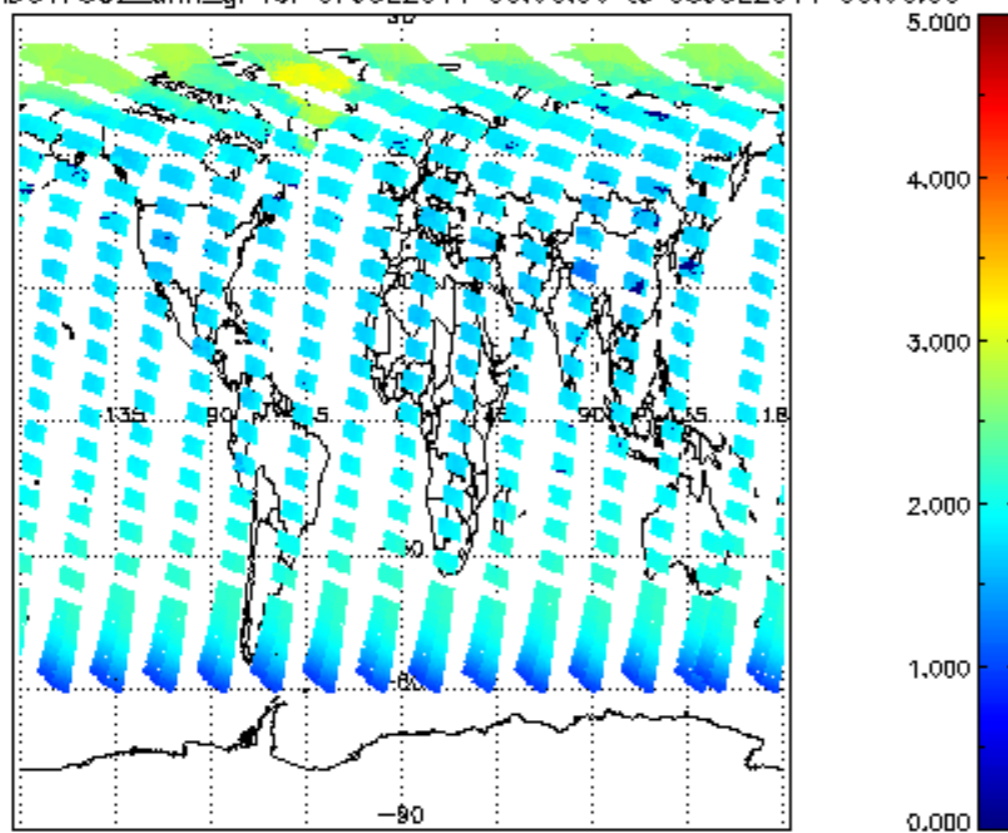
SCIOL2P_NADUV7S02_amf_gr for 07JUL2011 00:00:00 to 08JUL2011 00:00:00
