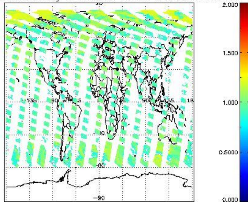
SCIOL2P_NADUV8H2O_amf_gr for 07JUL2011 00:00:00 to 08JUL2011 00:00:00
