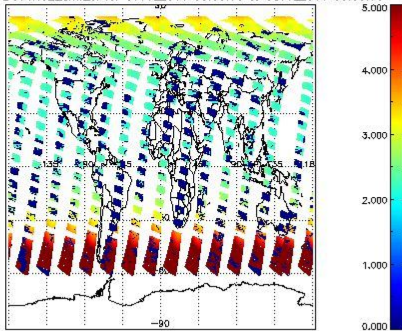
SCIOL2P_NADUV1NO2_amf_cl for 07JUL2011 00:00:00 to 08JUL2011 00:00:00
