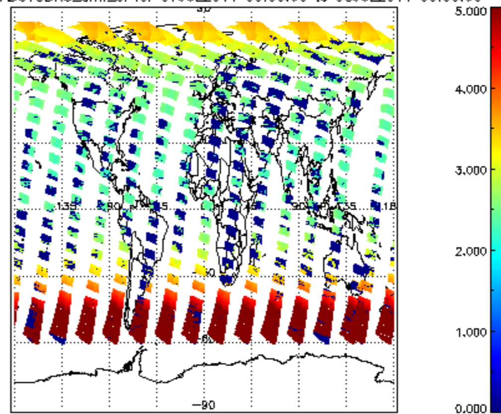
SCIOL2P_NADUV3BRO_arnf_cl for 07JUL2011 00:00:00 to 08JUL2011 00:00:00
