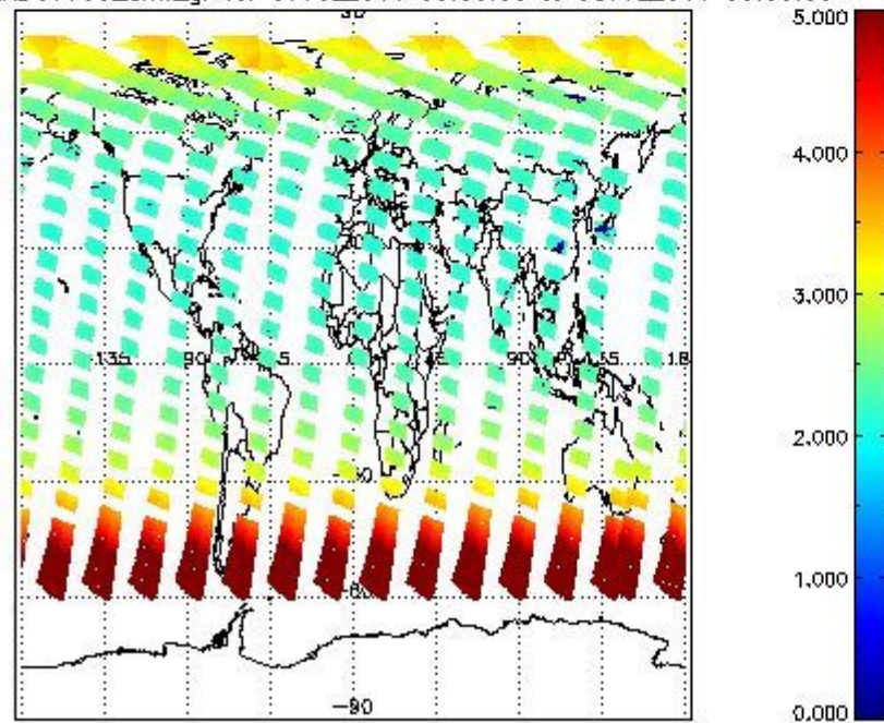
SCIOL2P_NADUV003_amf_gr for 07JUL2011 00:00:00 to 08JUL2011 00:00:00
