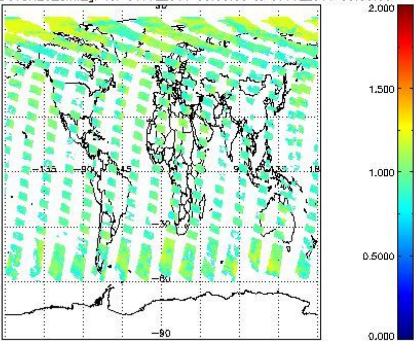
SCIOL2P_NADUV8H2O_amf_gr for 06JUL2011 00:00:00 to 07JUL2011 00:00:00
