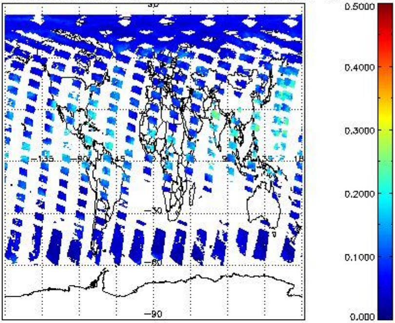
SCIOL2P_NADUV8H2O_vcd_err for 06JUL2011 00:00:00 to 07JUL2011 00:00:00
