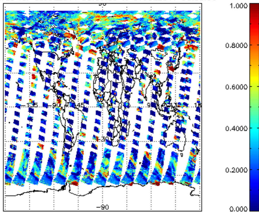
cl_frac for 06JUL2011 00:00:00 to 07JUL2011 00:00:00
