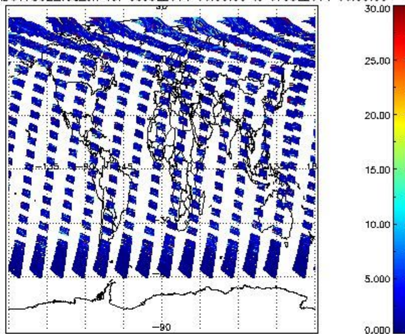
SCIOL2P_NADUV7S02_vcd_err for 06JUL2011 00:00:00 to 07JUL2011 00:00:00
