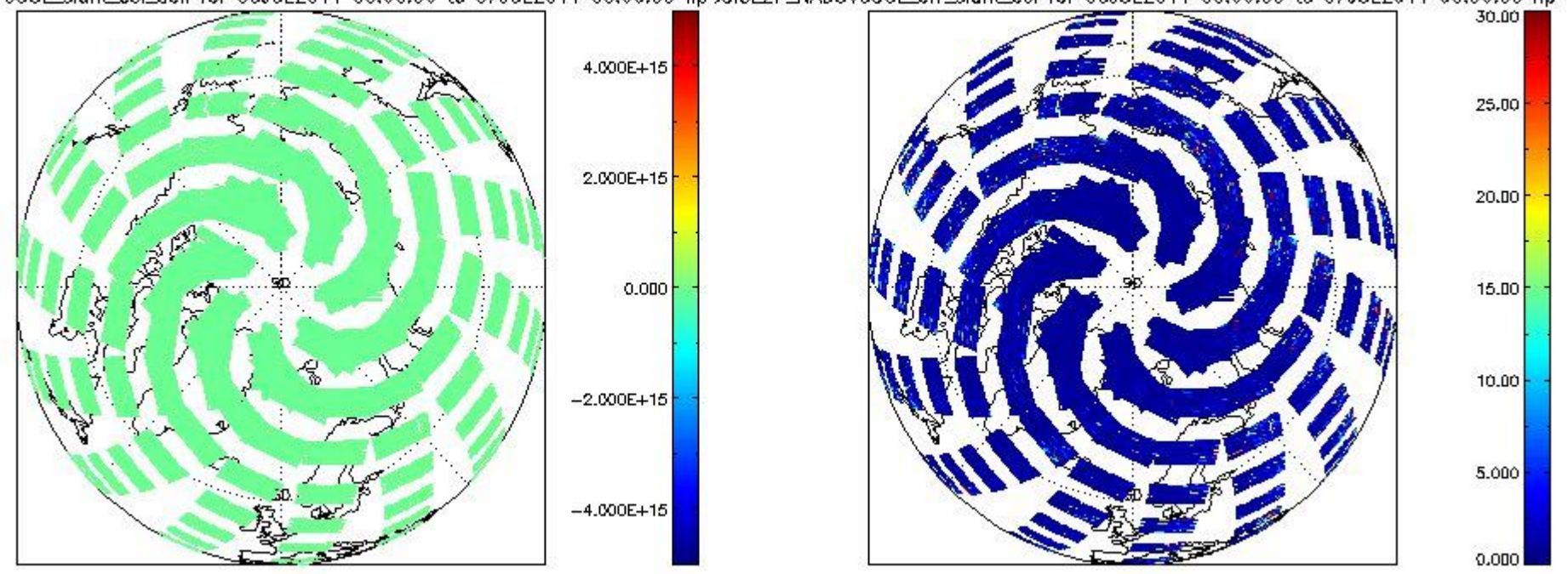
SCIOI2P_NADUV6OCLslant_col_den for 06JUL2011 00:00:00 to 07JUL2011 00:00:00 np SCIOI2P_NADUV6OCLarr_slant_col for 06JUL2011 00:00:00 to 07JUL2011 00:00:00 np
