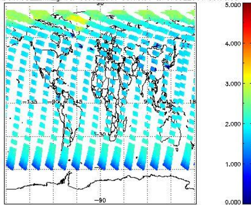
SCIOL2P_NADUV7S02_amf_gr for 06JUL2011 00:00:00 to 07JUL2011 00:00:00
