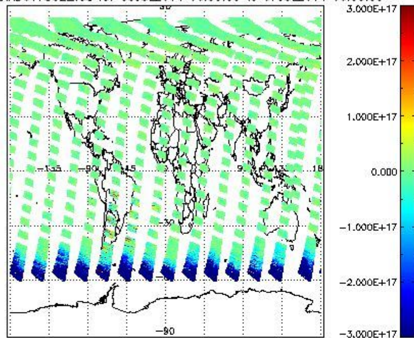
SCIOL2P_NADUV7S02_vcd for 06JUL2011 00:00:00 to 07JUL2011 00:00:00
