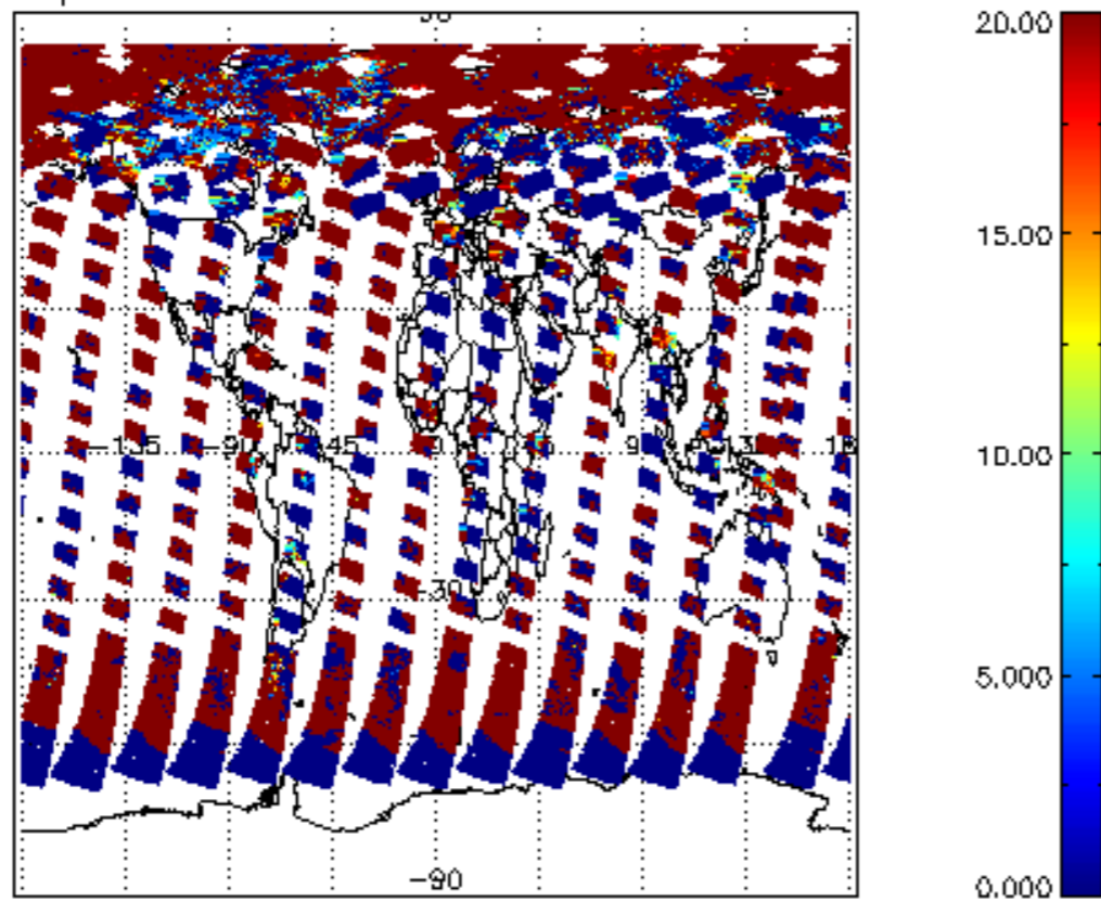
cl_lopt_depth for 06JUL2011 00:00:00 to 07JUL2011 00:00:00
