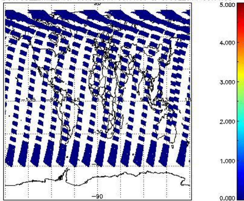
SCIOL2P_NADUV7S02_amf_cl for 06JUL2011 00:00:00 to 07JUL2011 00:00:00
