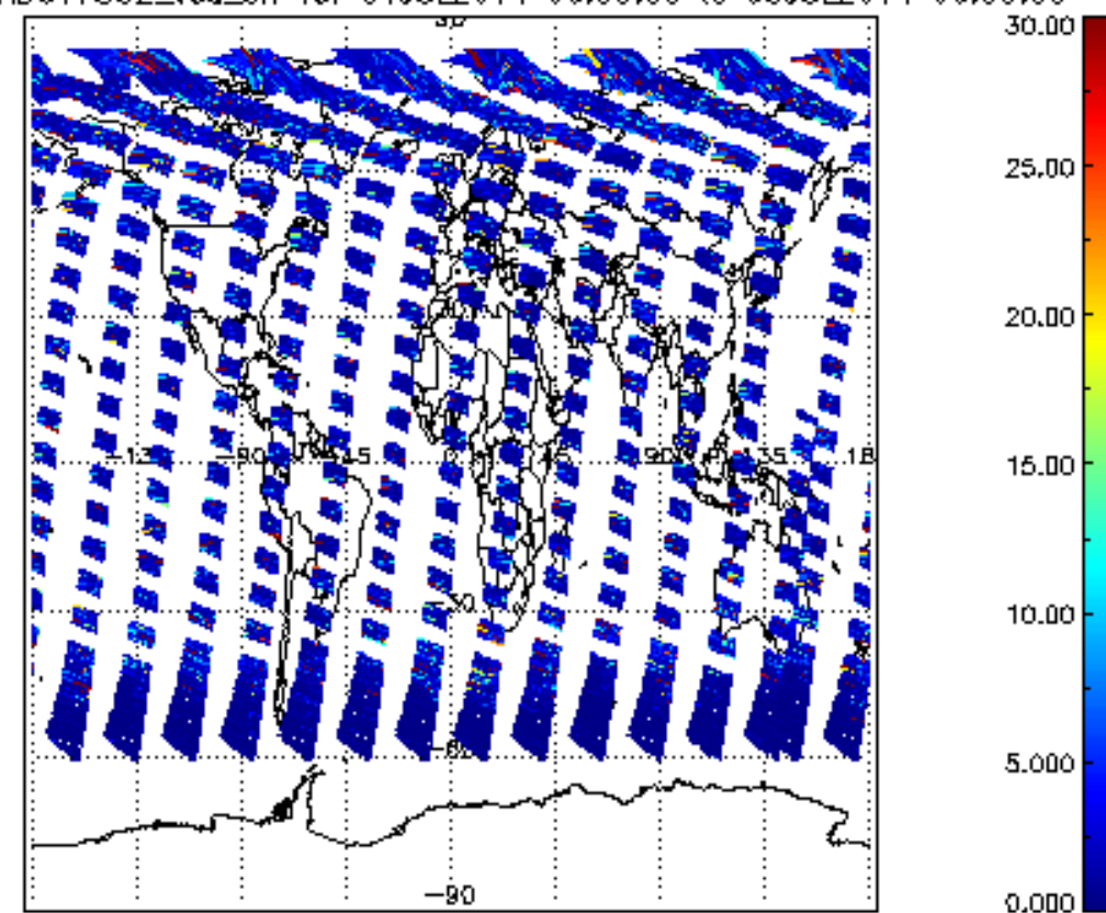
SCIOL2P_NADUV7S02_vcd_err for 04JUL2011 00:00:00 to 05JUL2011 00:00:00
