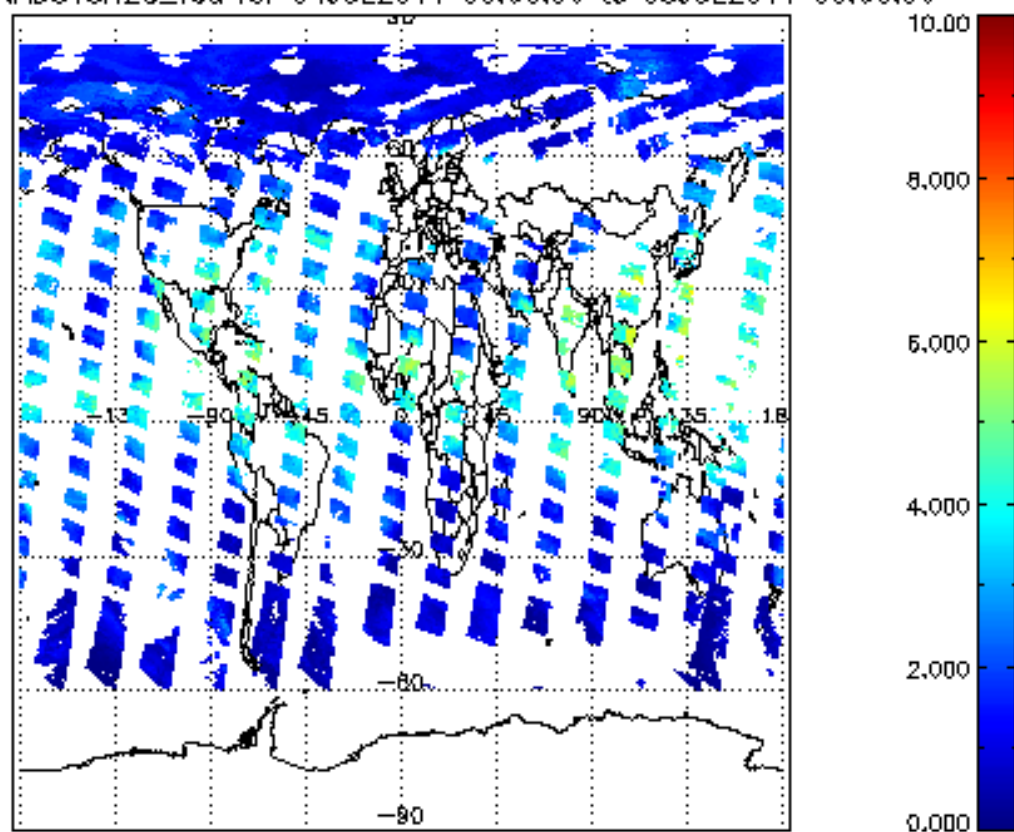
SCIOL2P_NADUV8H2O_vcd for 04JUL2011 00:00:00 to 05JUL2011 00:00:00
