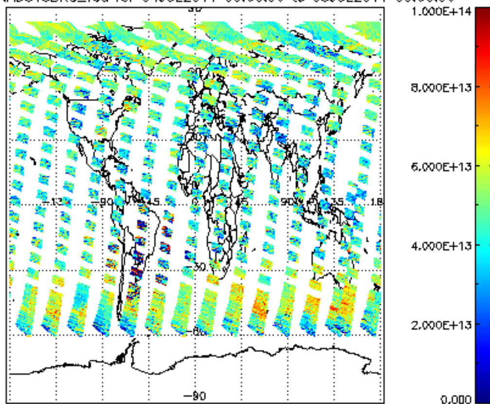
SCIOL2P_NADUV3BRO_vcd for 04JUL2011 00:00:00 to 05JUL2011 00:00:00
