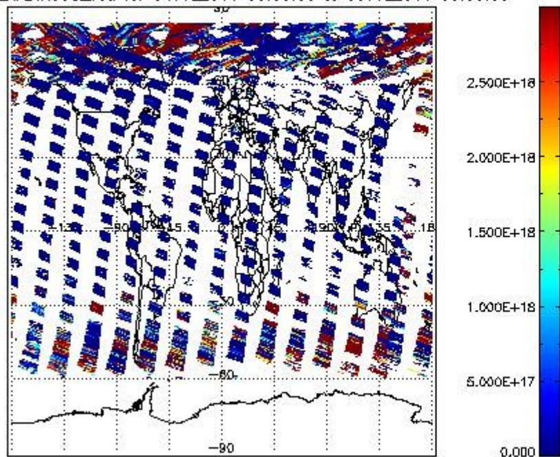
SCIDL2P_NADIR3CO_vcd for 04JUL2011 00:00:00 to 05JUL2011 00:00:00
