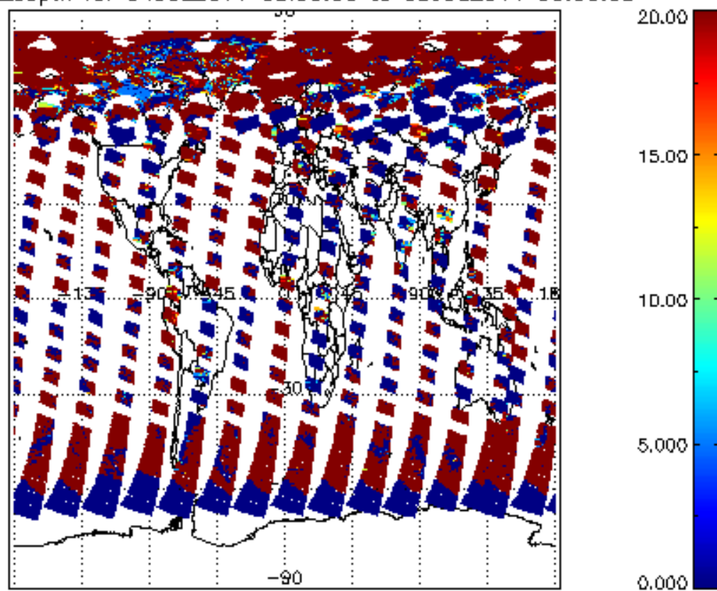
cl_lopt_depth for 04JUL2011 00:00:00 to 05JUL2011 00:00:00
