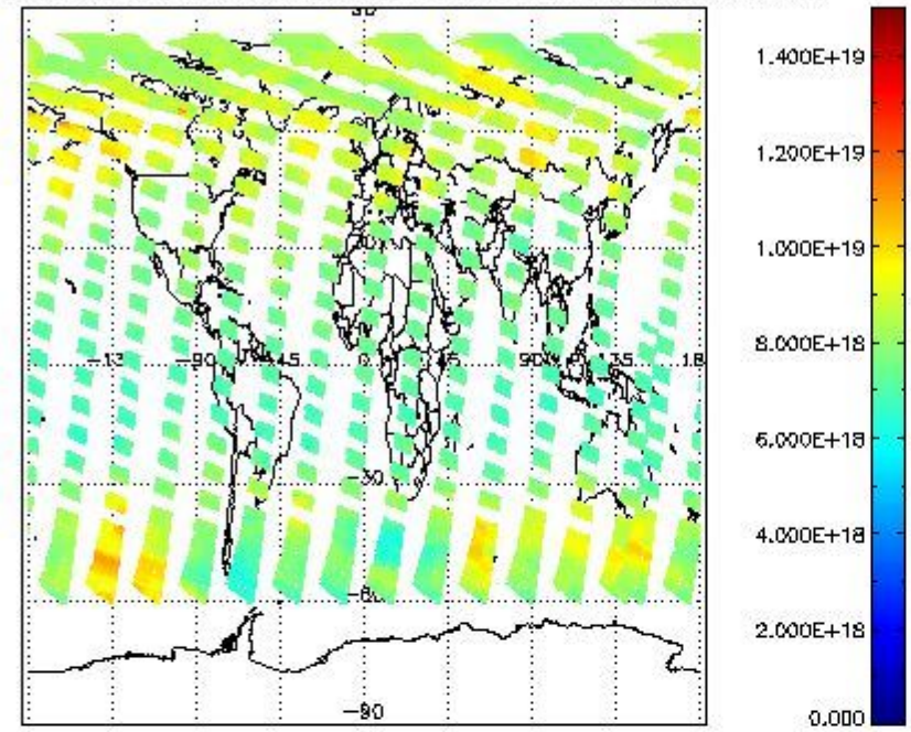
SCIOL2P_NADUV003_vcd for 04JUL2011 00:00:00 to 05JUL2011 00:00:00
