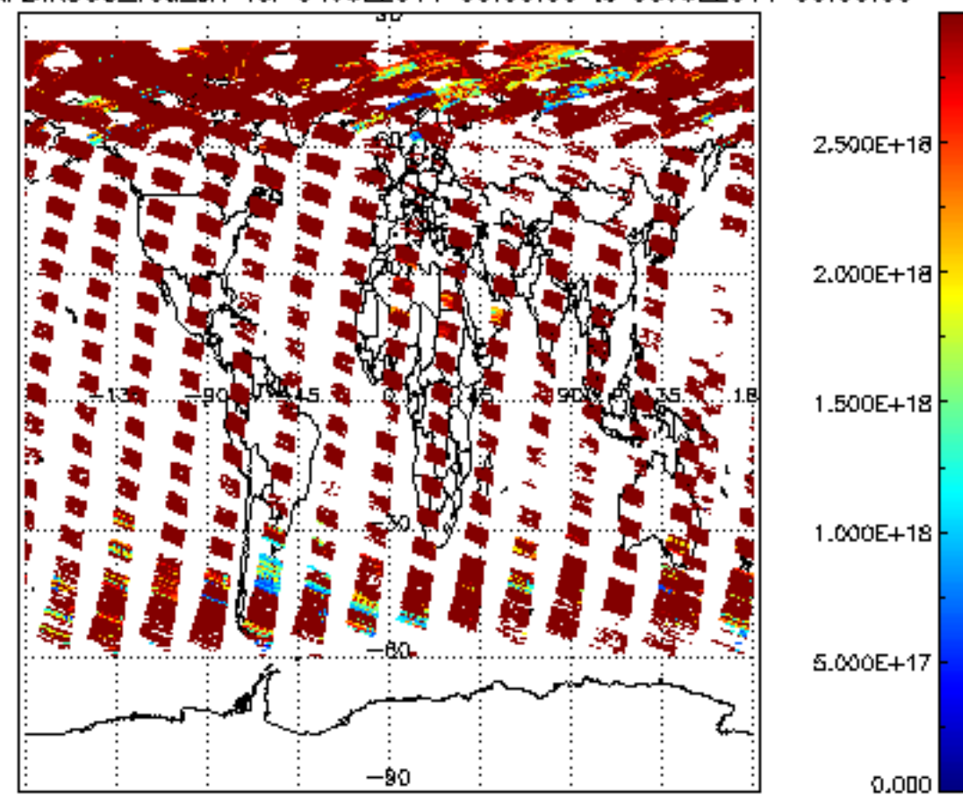
SCIOL2P_NADIR3CO_vcd_err for 04JUL2011 00:00:00 to 05JUL2011 00:00:00
