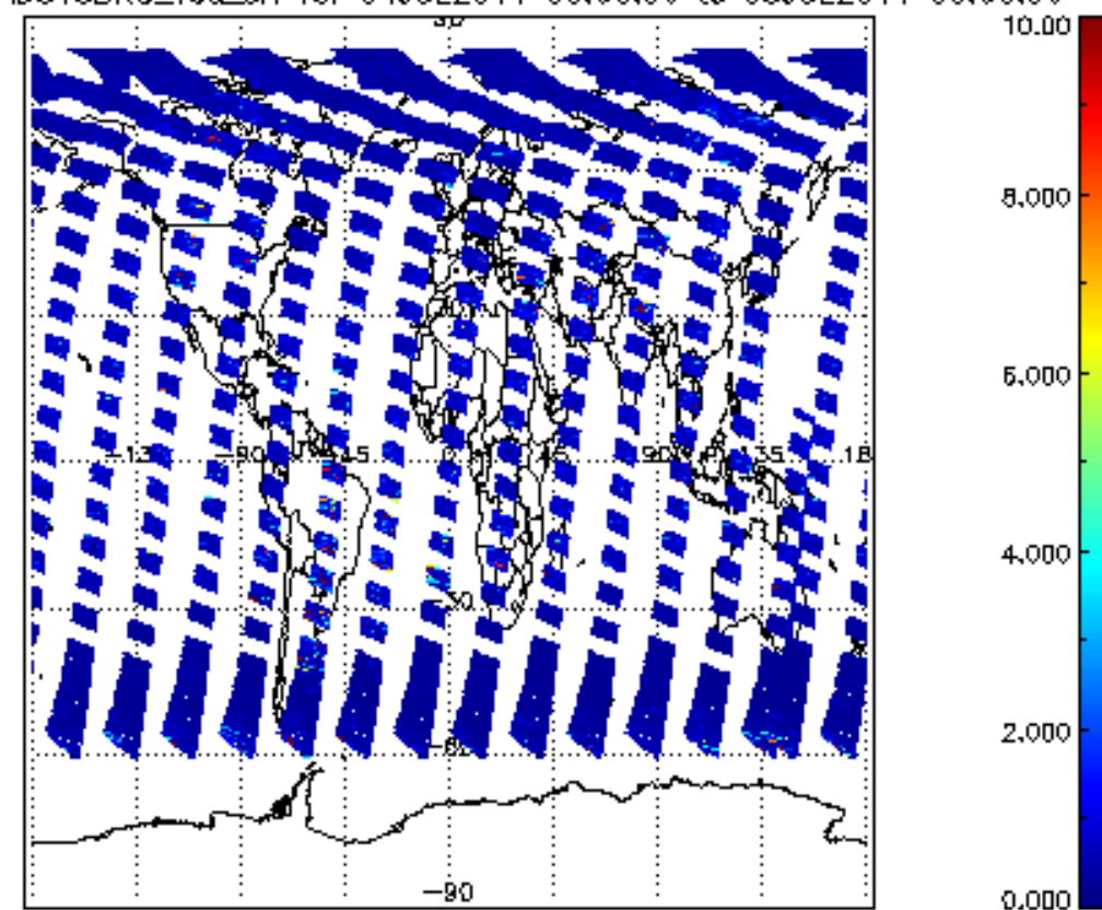
SCIOL2P_NADUV3BRO_vcd_err for 04JUL2011 00:00:00 to 05JUL2011 00:00:00
