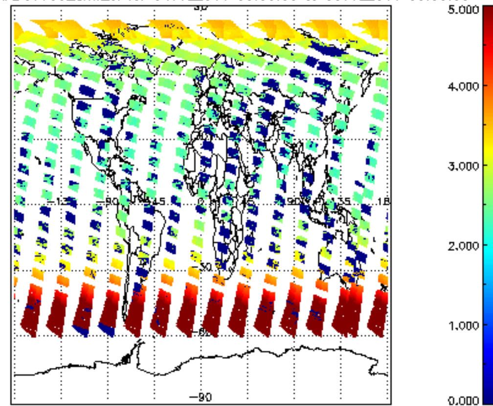
SCIOL2P_NADUV003_amf_cl for 04JUL2011 00:00:00 to 05JUL2011 00:00:00
