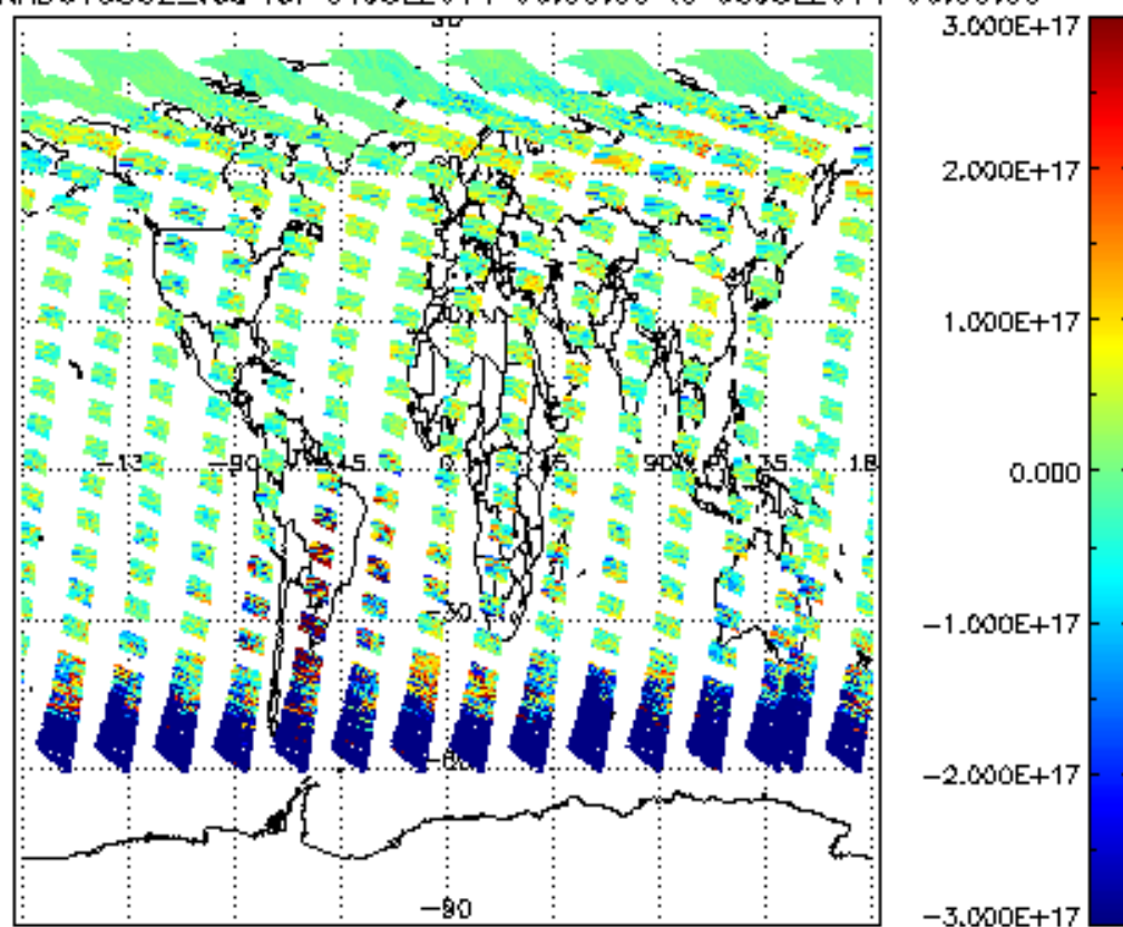
SCIOL2P_NADUV5S02_vcd for 04JUL2011 00:00:00 to 05JUL2011 00:00:00
