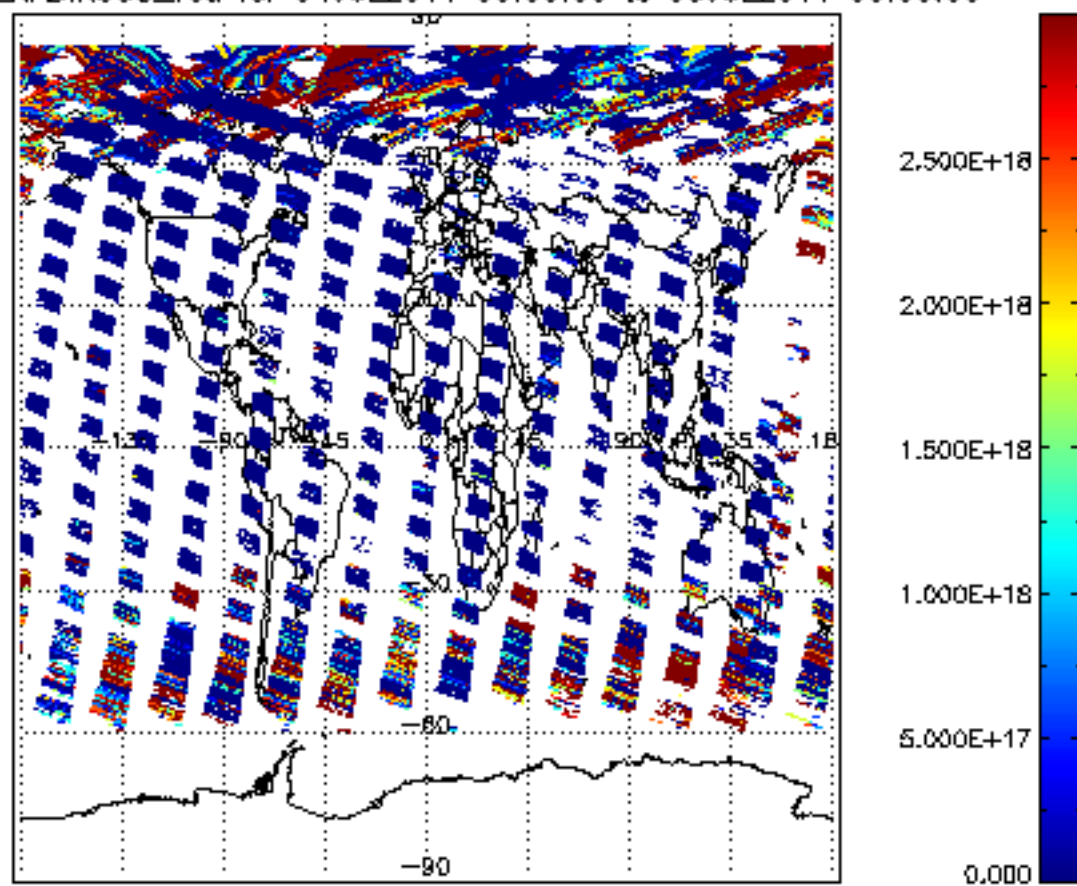
SCIOL2P_NADIR3CO_vcd for 04JUL2011 00:00:00 to 05JUL2011 00:00:00
