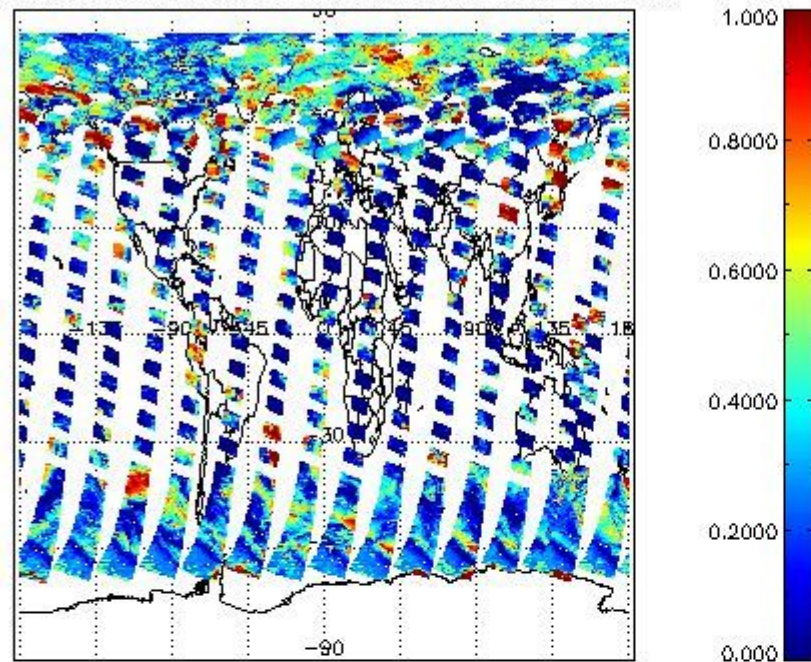
cL_frac for 04JUL2011 00:00:00 to 05JUL2011 00:00:00
