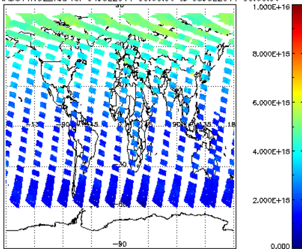
SCIOL2P_NADUV1NO2_vcd for 04JUL2011 00:00:00 to 05JUL2011 00:00:00
