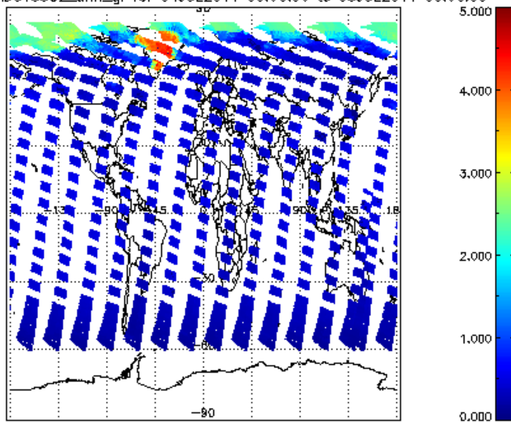
SCIOL2P_NADUV5S02_amf_gr for 04JUL2011 00:00:00 to 05JUL2011 00:00:00
