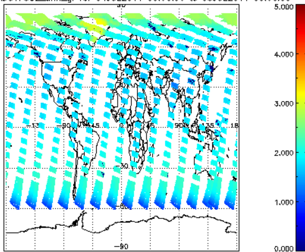
SCIOL2P_NADUV7S02_amf_gr for 04JUL2011 00:00:00 to 05JUL2011 00:00:00
