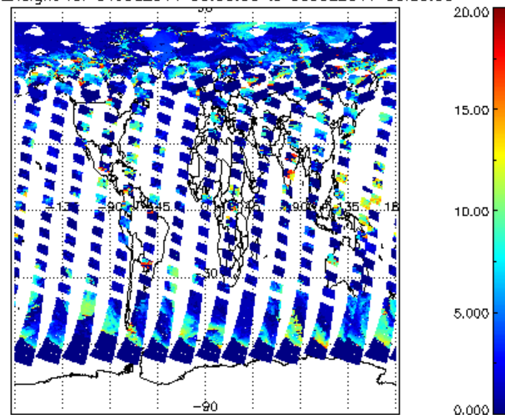
cl_top_height for 04JUL2011 00:00:00 to 05JUL2011 00:00:00
