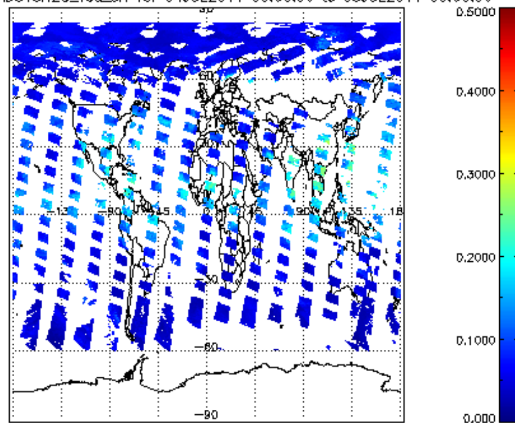
SCIOL2P_NADUV8H2O_vcd_err for 04JUL2011 00:00:00 to 05JUL2011 00:00:00
