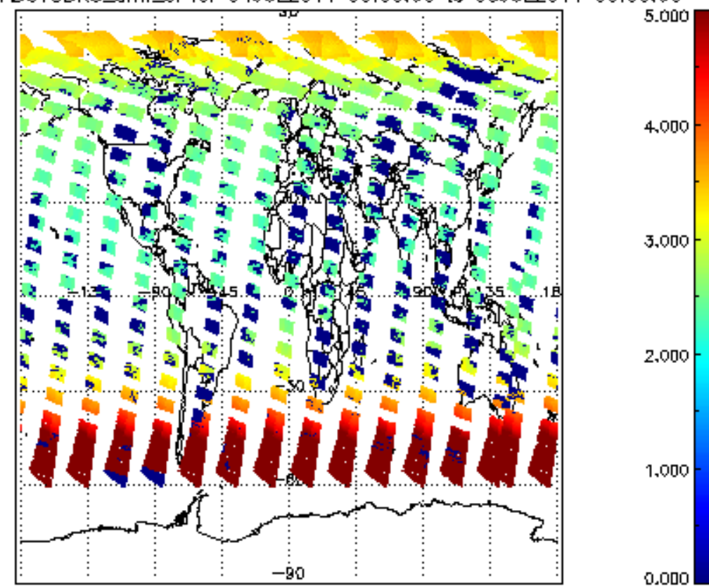
SCIOL2P_NADUV3BRO_arnf_cl for 04JUL2011 00:00:00 to 05JUL2011 00:00:00
