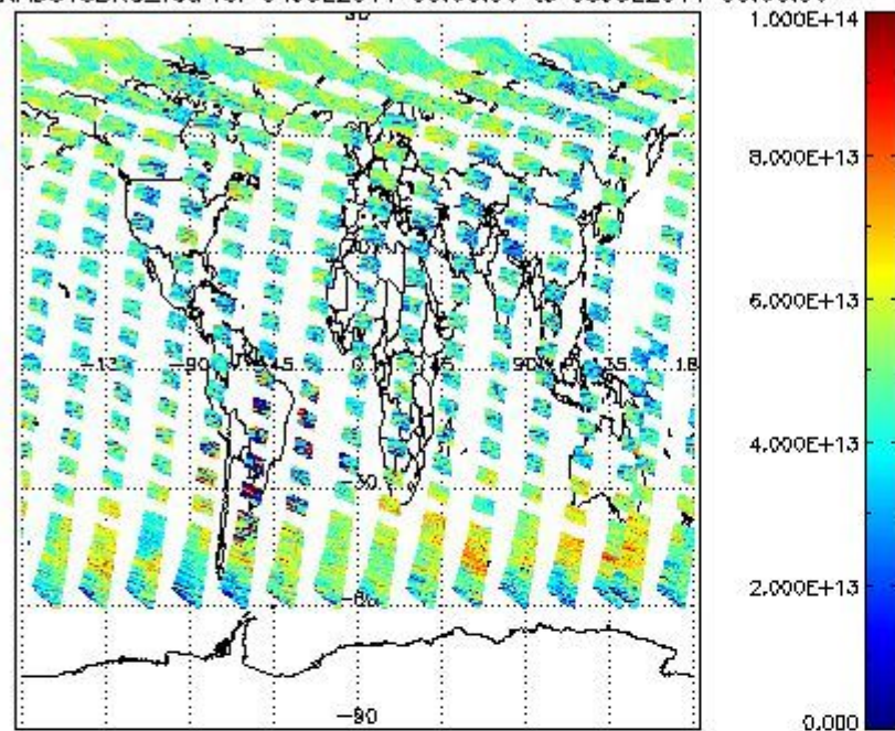
SCIOL2P_NADUV3BRO_vcd for 04JUL2011 00:00:00 to 05JUL2011 00:00:00
