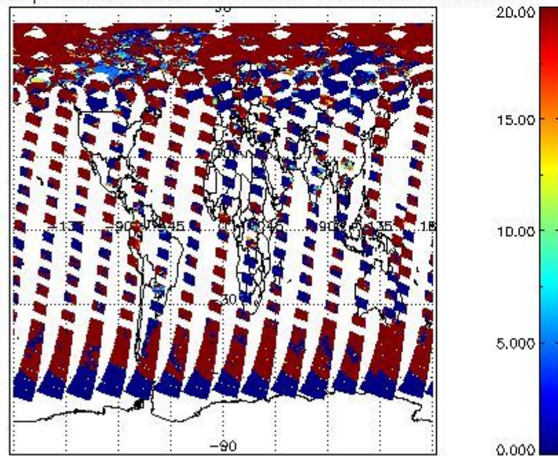
cL_opt_depth for 04JUL2011 00:00:00 to 05JUL2011 00:00:00
