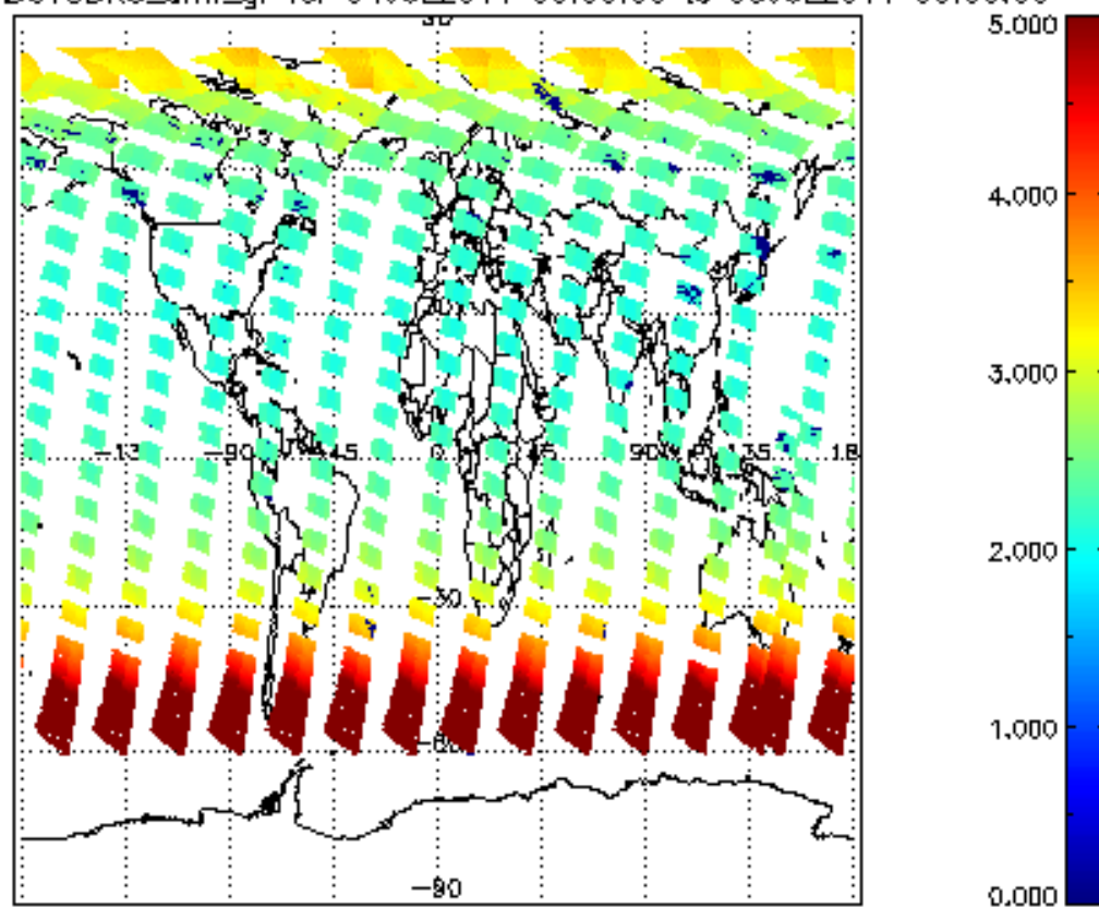
SCIOL2P_NADUV3BRO_arnf_gr for 04JUL2011 00:00:00 to 05JUL2011 00:00:00
