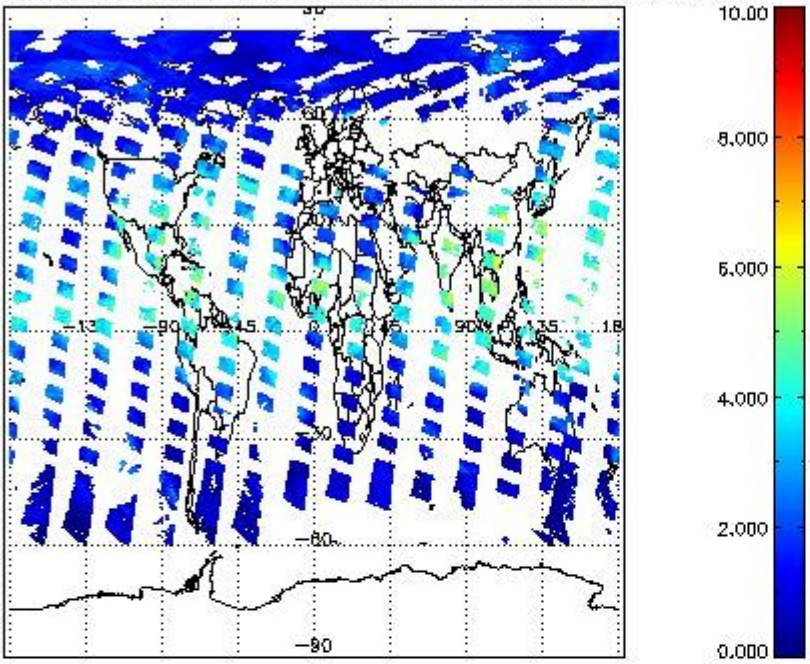
SCIOL2P_NADUV8H2O_vcd for 04JUL2011 00:00:00 to 05JUL2011 00:00:00
