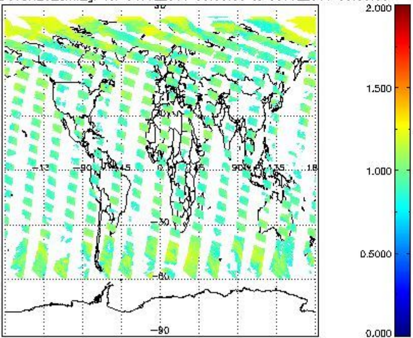
SCIOL2P_NADUV8H2O_amf_gr for 04JUL2011 00:00:00 to 05JUL2011 00:00:00
