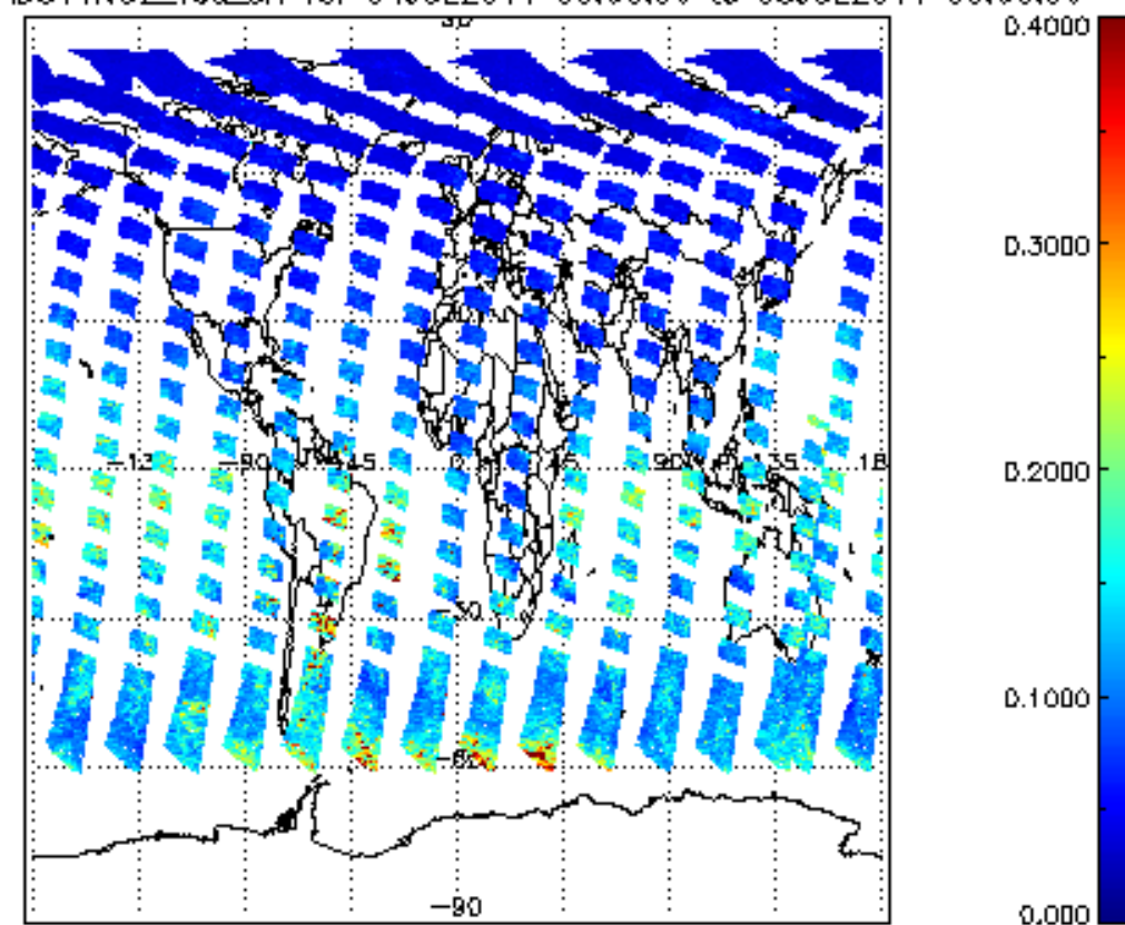
SCIOL2P_NADUV1NO2_vcd_err for 04JUL2011 00:00:00 to 05JUL2011 00:00:00
