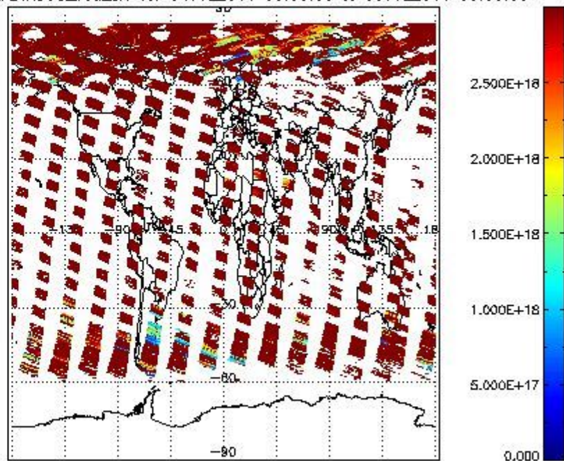
SCIDL2P_NADIR3CO_vcd_err for 04JUL2011 00:00:00 to 05JUL2011 00:00:00
