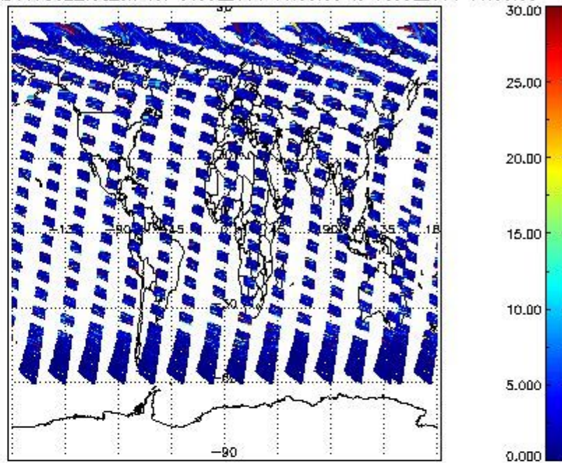
SCIOL2P_NADUV7S02_vcd_err for 04JUL2011 00:00:00 to 05JUL2011 00:00:00
