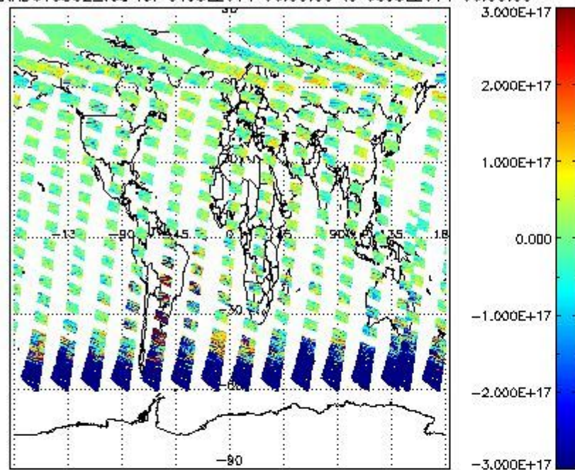
SCIOL2P_NADUV5S02_vcd for 04JUL2011 00:00:00 to 05JUL2011 00:00:00
