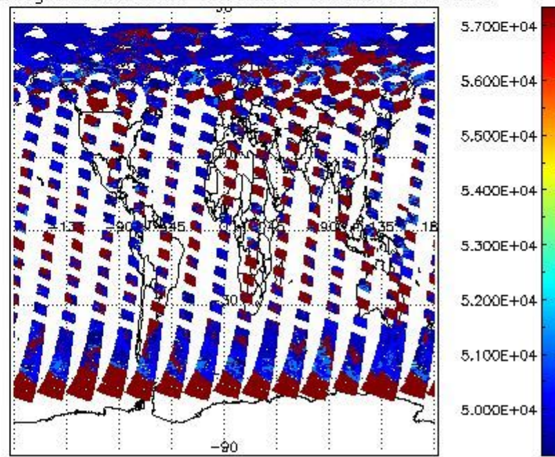
cloud_flags for 04JUL2011 00:00:00 to 05JUL2011 00:00:00
