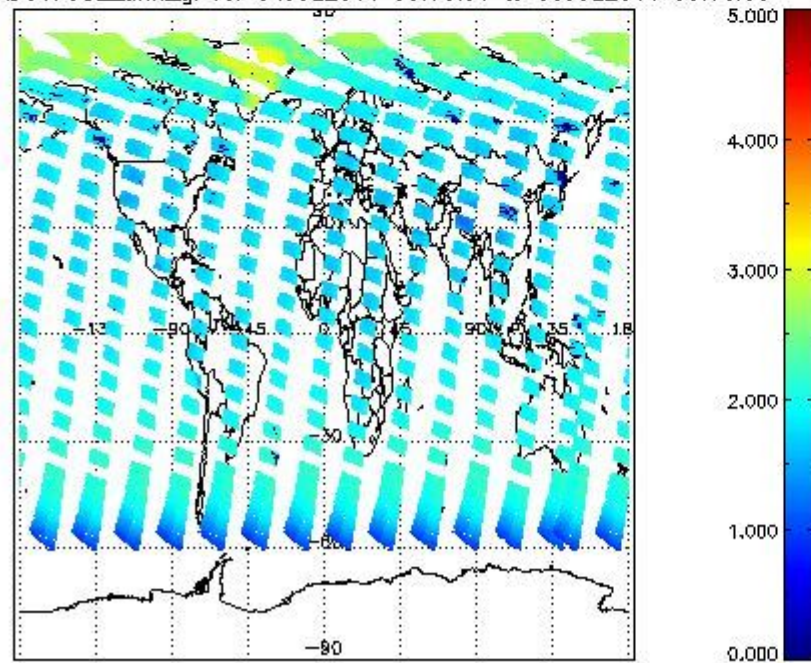
SCIOL2P_NADUV7S02_amf_gr for 04JUL2011 00:00:00 to 05JUL2011 00:00:00
