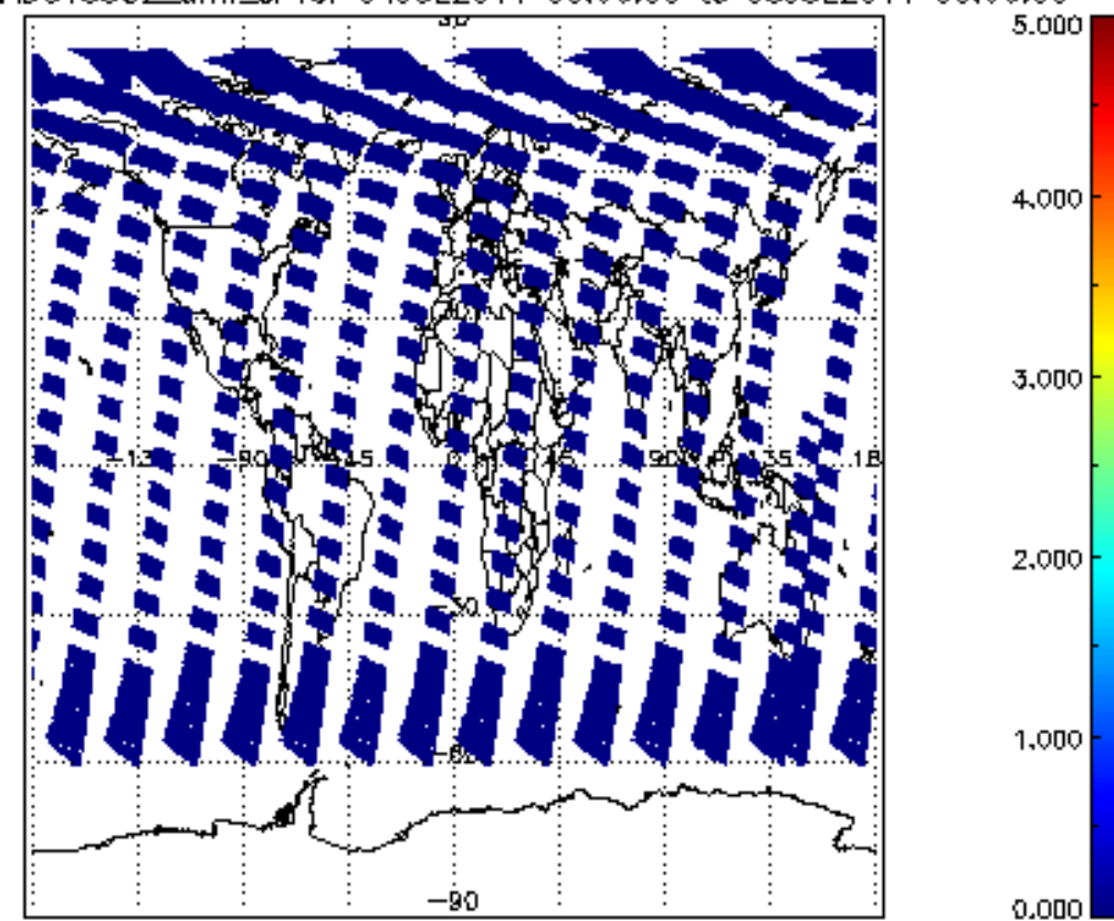
SCIOL2P_NADUV5S02_amf_cl for 04JUL2011 00:00:00 to 05JUL2011 00:00:00
