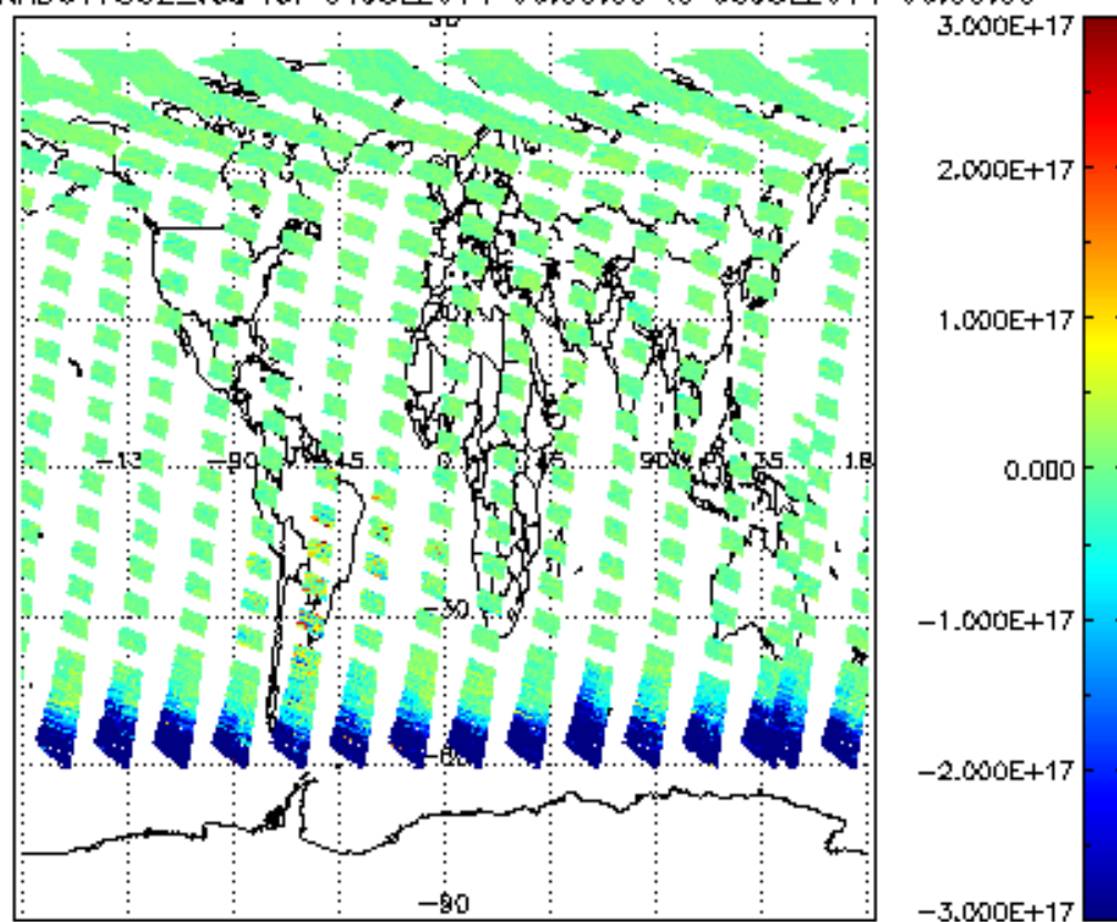
SCIOL2P_NADUV7S02_vcd for 04JUL2011 00:00:00 to 05JUL2011 00:00:00
