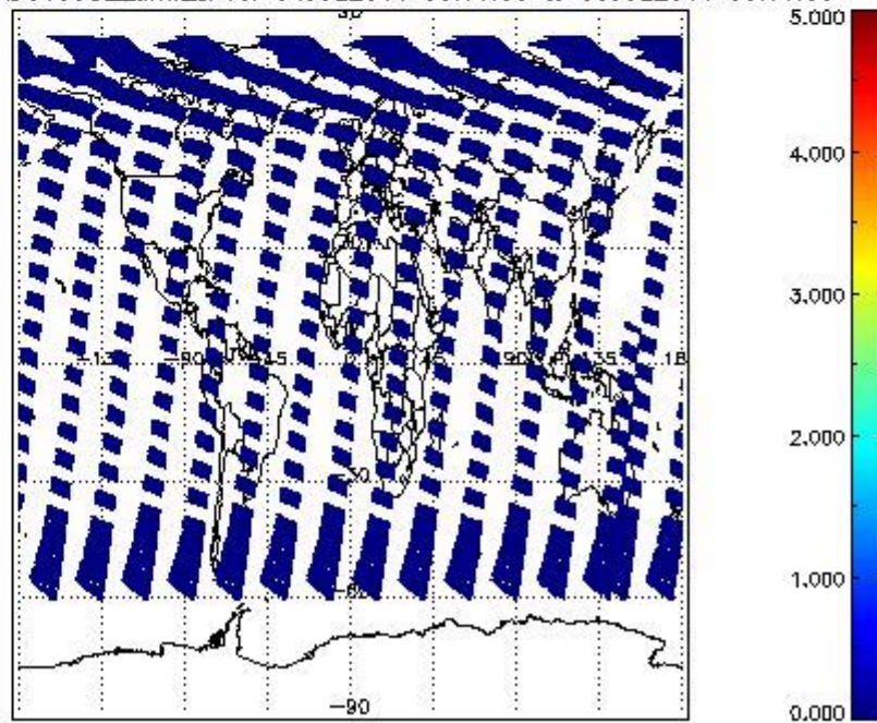
SCIOL2P_NADUV5S02_amf_cl for 04JUL2011 00:00:00 to 05JUL2011 00:00:00
