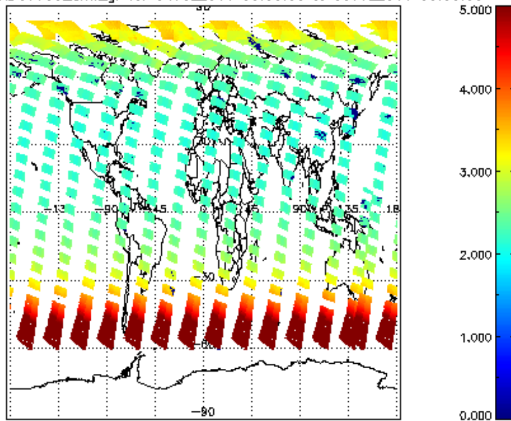
SCIOL2P_NADUV003_amf_gr for 04JUL2011 00:00:00 to 05JUL2011 00:00:00
