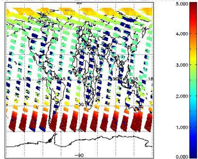
SCIOL2P_NADUV003_amf_cl for 04JUL2011 00:00:00 to 05JUL2011 00:00:00
