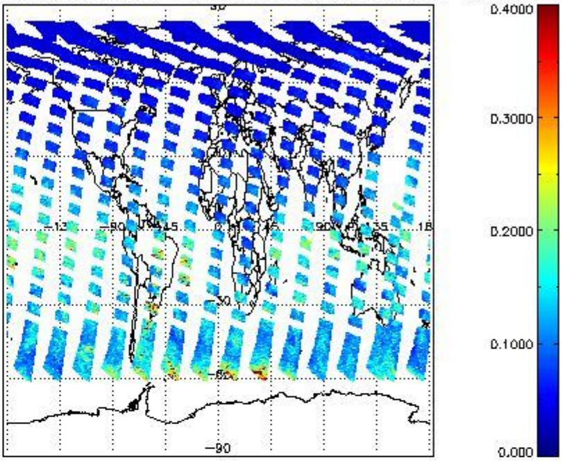
SCIOL2P_NADUV1NO2_vcd_err for 04JUL2011 00:00:00 to 05JUL2011 00:00:00
