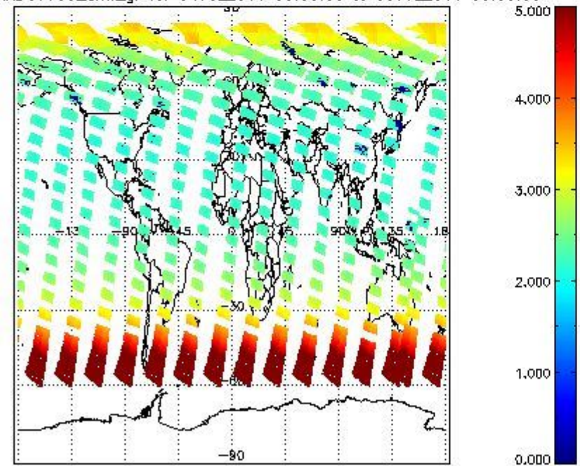
SCIOL2P_NADUV003_amf_gr for 04JUL2011 00:00:00 to 05JUL2011 00:00:00
