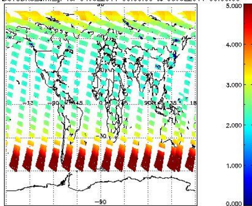
SCIOL2P_NADUV3BRO_amf_gr for 04JUL2011 00:00:00 to 05JUL2011 00:00:00
