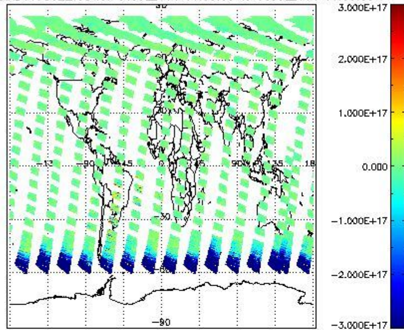
SCIOL2P_NADUV7S02_vcd for 04JUL2011 00:00:00 to 05JUL2011 00:00:00
