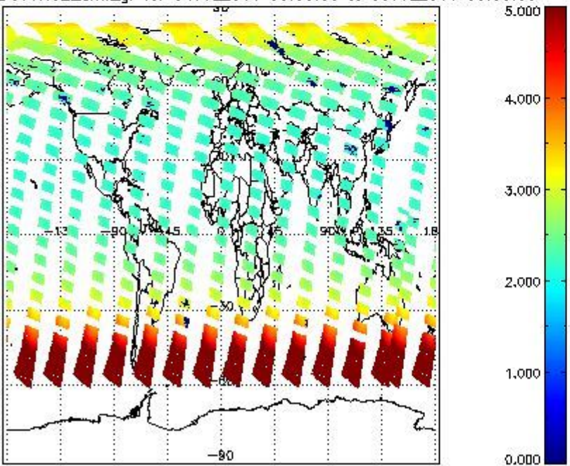
SCIOL2P_NADUV1NO2_amf_gr for 04JUL2011 00:00:00 to 05JUL2011 00:00:00
