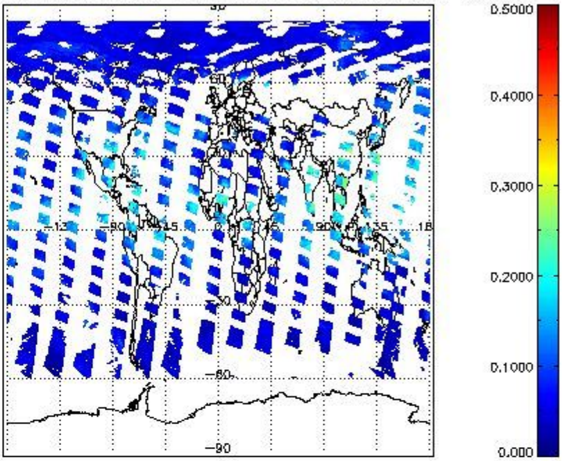
SCIOL2P_NADUV8H2O_vcd_err for 04JUL2011 00:00:00 to 05JUL2011 00:00:00
