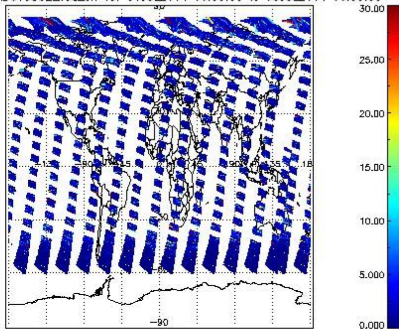
SCIOL2P_NADUV5S02_vcd_err for 04JUL2011 00:00:00 to 05JUL2011 00:00:00
