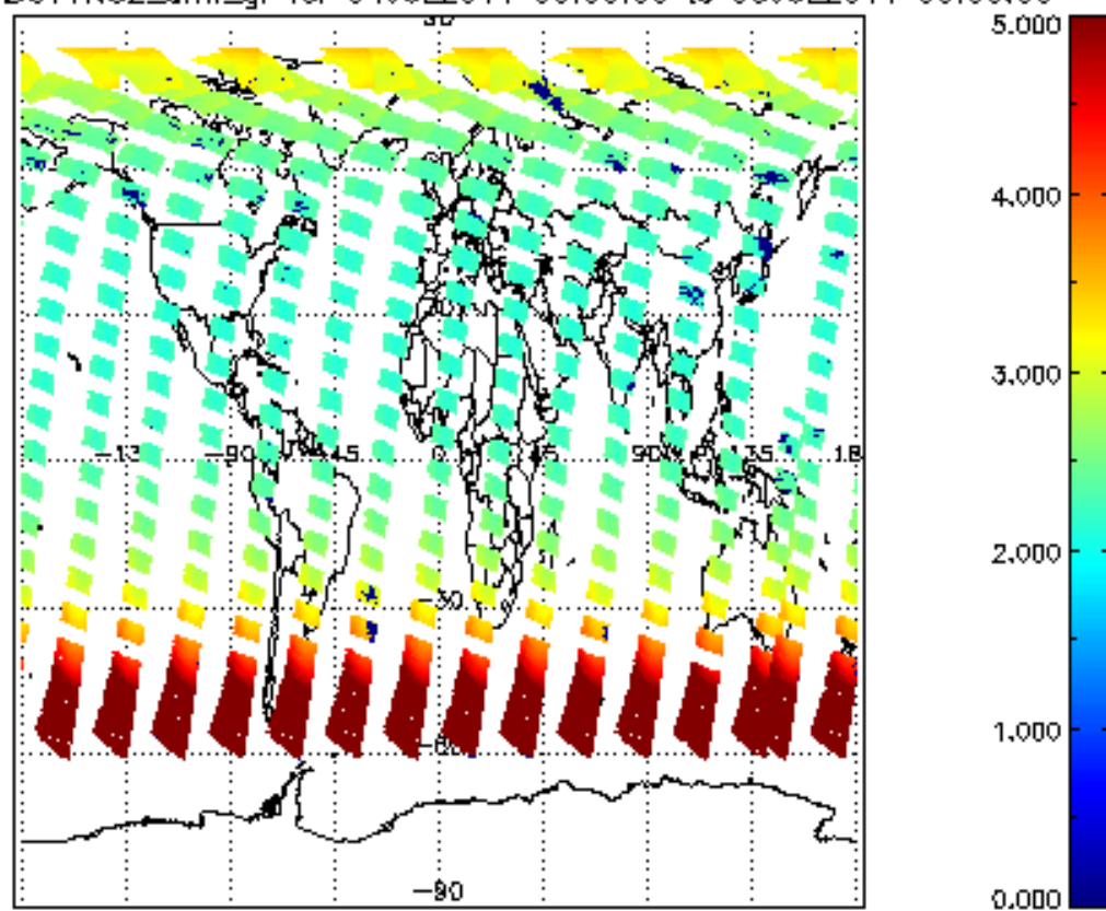
SCIOL2P_NADUV1NO2_amf_gr for 04JUL2011 00:00:00 to 05JUL2011 00:00:00
