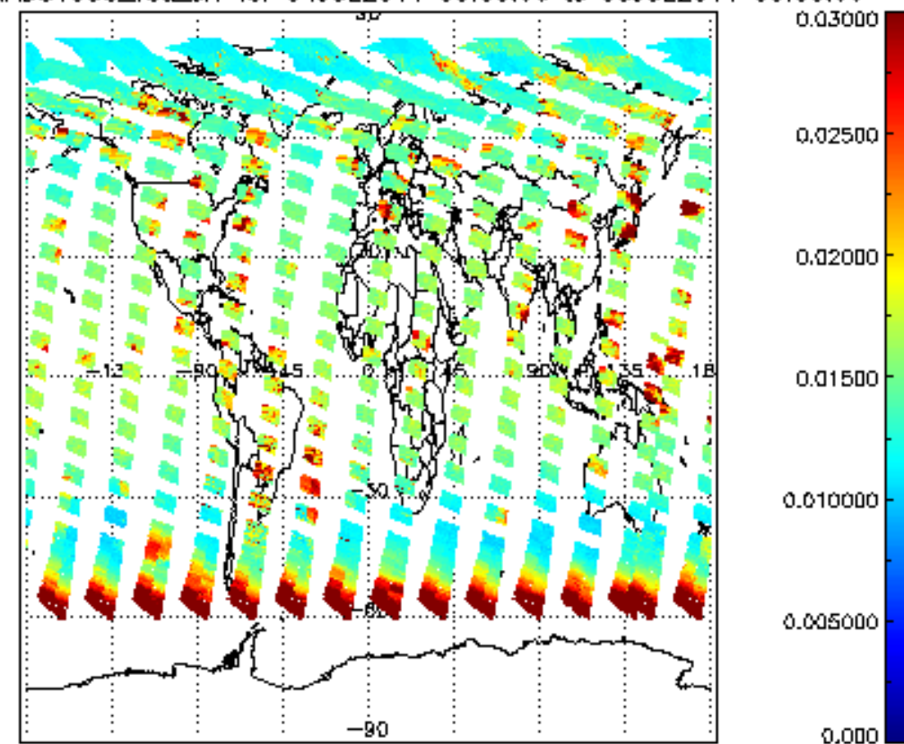
SCIOL2P_NADUV003_vcd_err for 04JUL2011 00:00:00 to 05JUL2011 00:00:00
