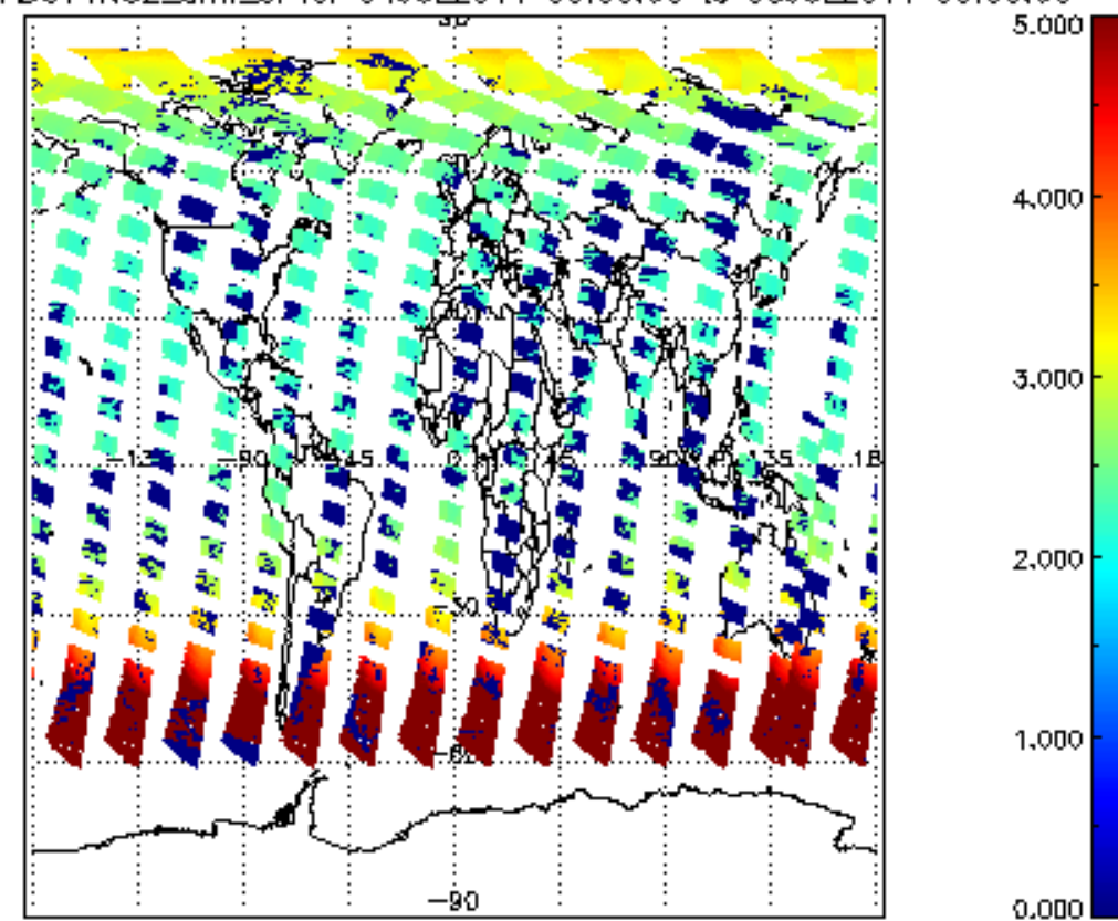
SCIOL2P_NADUV1NO2_amf_cl for 04JUL2011 00:00:00 to 05JUL2011 00:00:00
