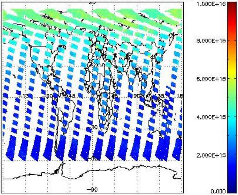
SCIOL2P_NADUV1NO2_vcd for 04JUL2011 00:00:00 to 05JUL2011 00:00:00
