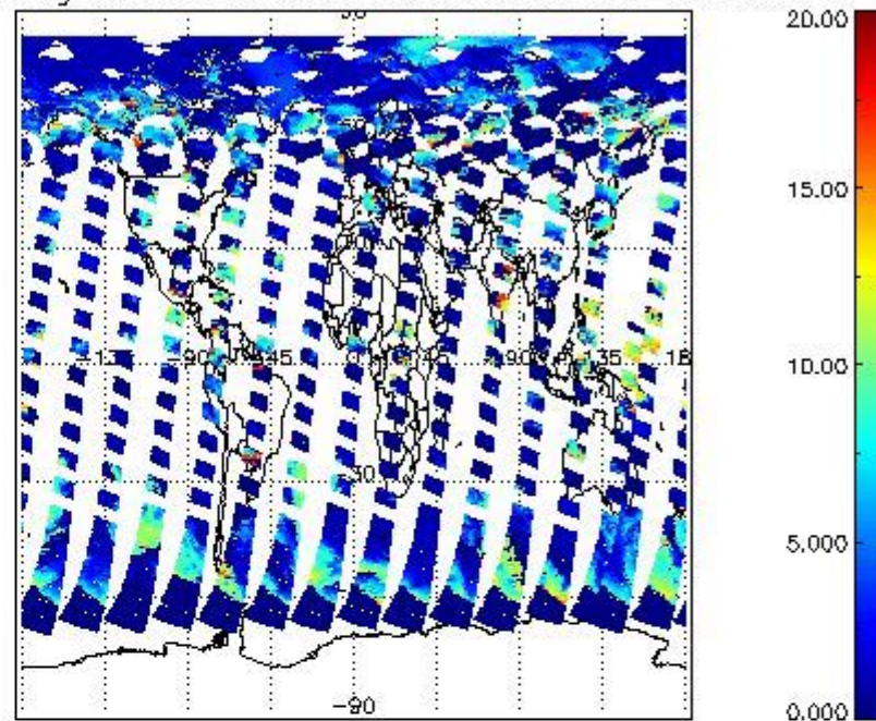
cL_top_height for 04JUL2011 00:00:00 to 05JUL2011 00:00:00
