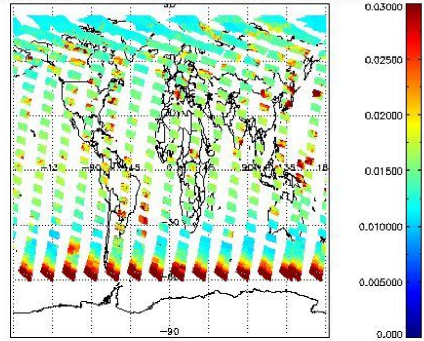
SCIOL2P_NADUV003_vcd_err for 04JUL2011 00:00:00 to 05JUL2011 00:00:00
