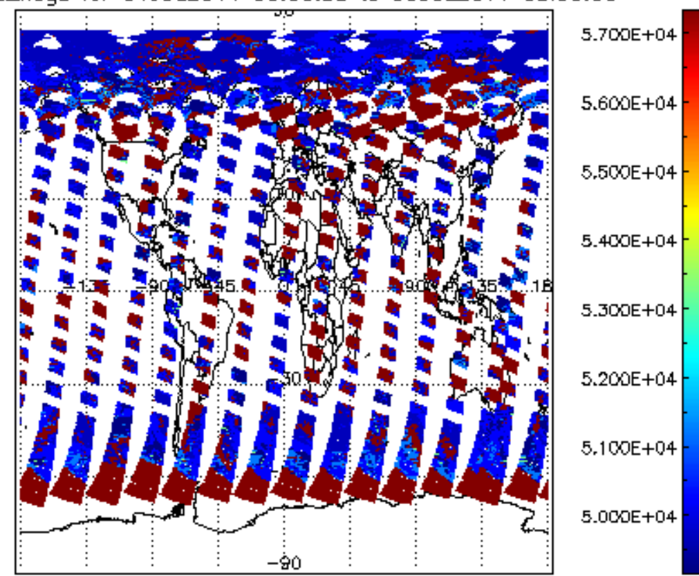
cloud_flags for 04JUL2011 00:00:00 to 05JUL2011 00:00:00
