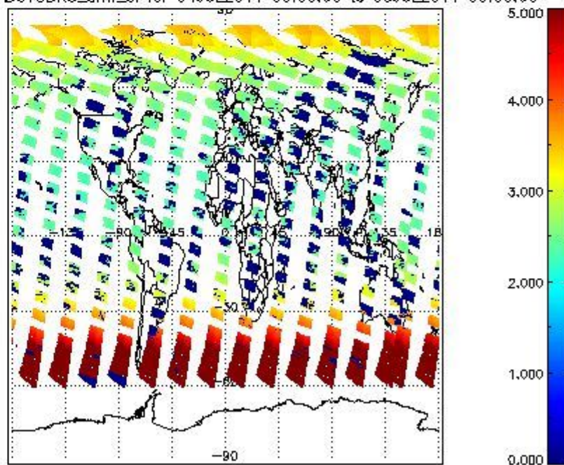
SCIOL2P_NADUV3BRO_amf_cl for 04JUL2011 00:00:00 to 05JUL2011 00:00:00
