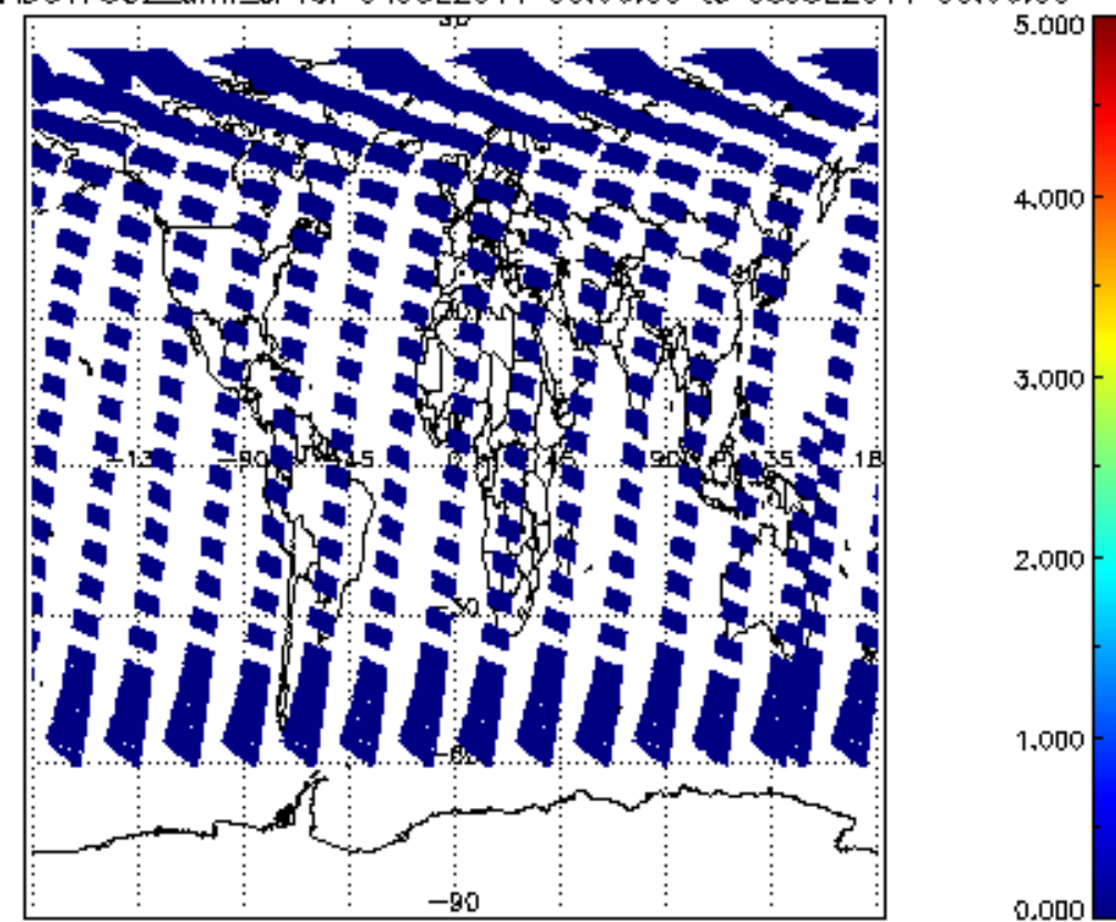
SCIOL2P_NADUV7S02_amf_cl for 04JUL2011 00:00:00 to 05JUL2011 00:00:00
