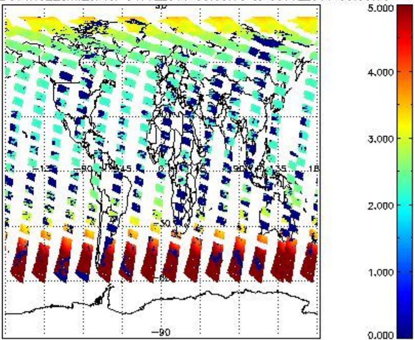
SCIOL2P_NADUV1NO2_amf_cl for 04JUL2011 00:00:00 to 05JUL2011 00:00:00
