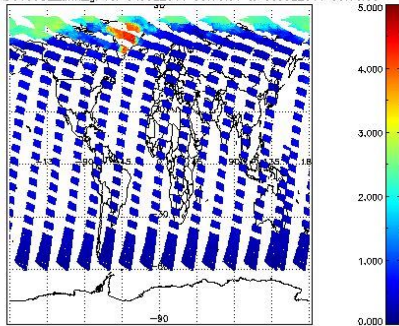
SCIOL2P_NADUV5S02_amf_gr for 04JUL2011 00:00:00 to 05JUL2011 00:00:00
