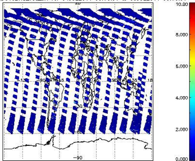
SCIOL2P_NADUV3BRO_vcd_err for 04JUL2011 00:00:00 to 05JUL2011 00:00:00
