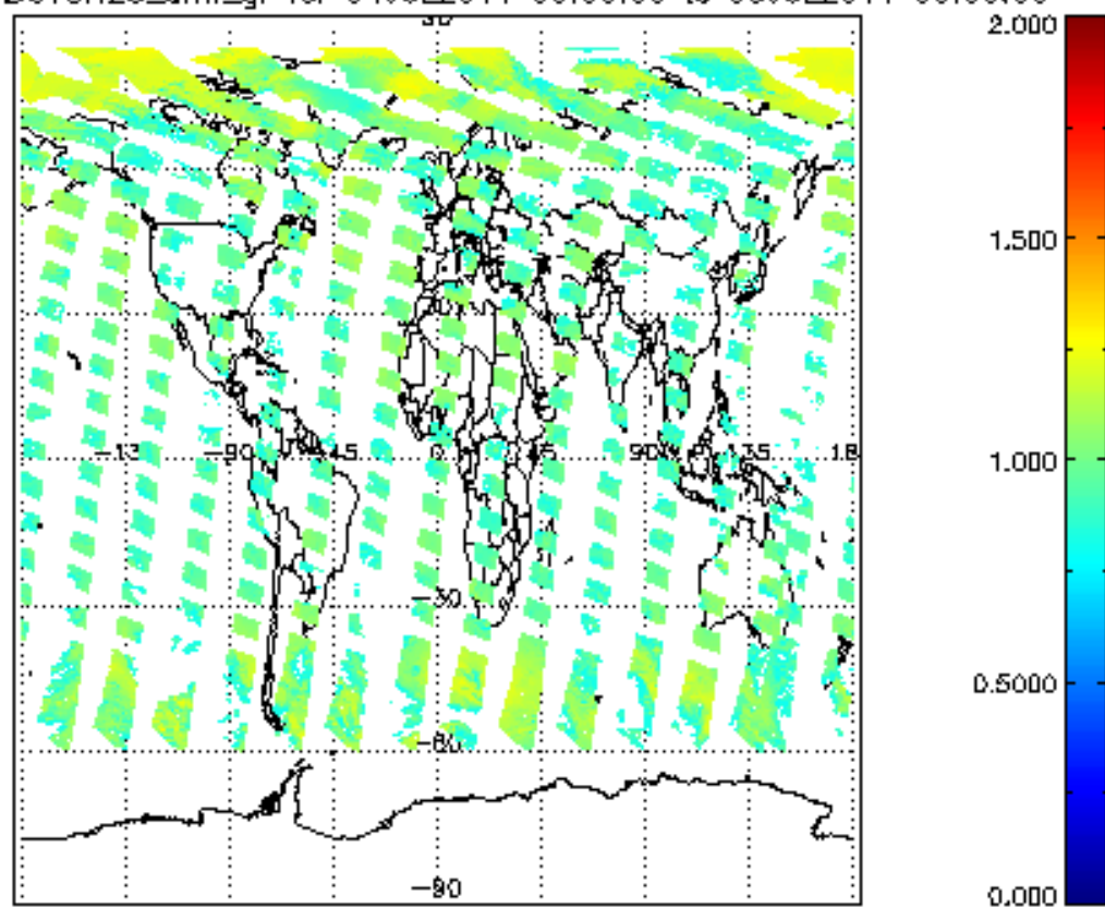
SCIOL2P_NADUV8H2O_amf_gr for 04JUL2011 00:00:00 to 05JUL2011 00:00:00
