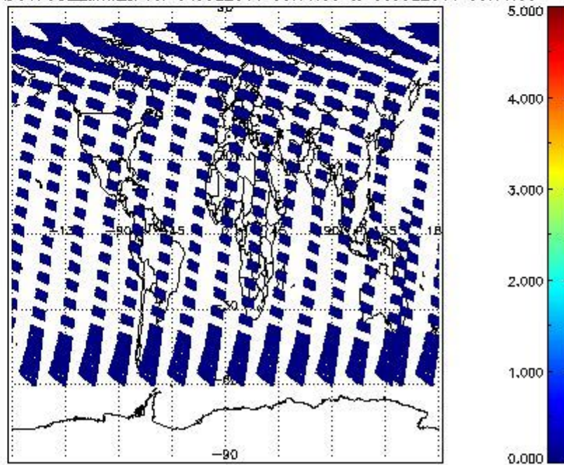
SCIOL2P_NADUV7S02_amf_cl for 04JUL2011 00:00:00 to 05JUL2011 00:00:00
