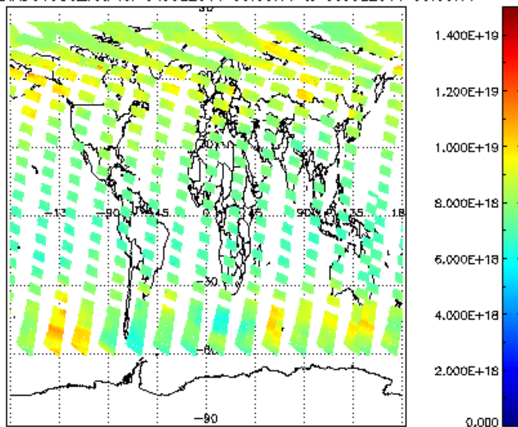
SCIOL2P_NADUV003_vcd for 04JUL2011 00:00:00 to 05JUL2011 00:00:00
