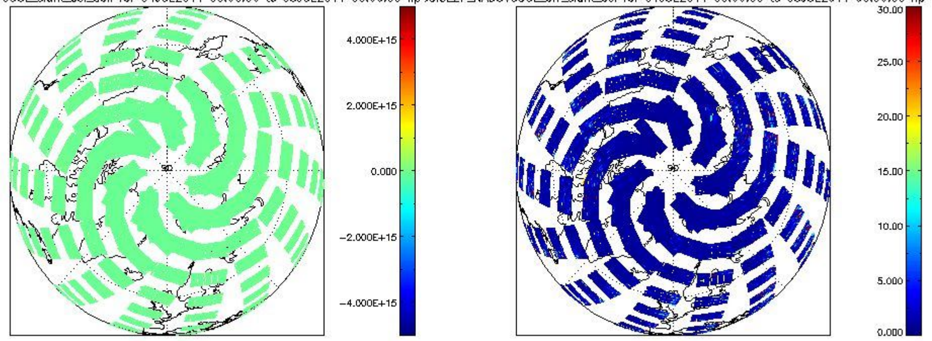
SCIOI2P_NADUV6OCLslant_col_den for 04JUL2011 00:00:00 to 05JUL2011 00:00:00 np SCIOI2P_NADUV6OCLarr_slant_col for 04JUL2011 00:00:00 to 05JUL2011 00:00:00 np
