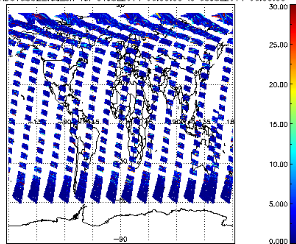
SCIOL2P_NADUV5S02_vcd_err for 04JUL2011 00:00:00 to 05JUL2011 00:00:00
