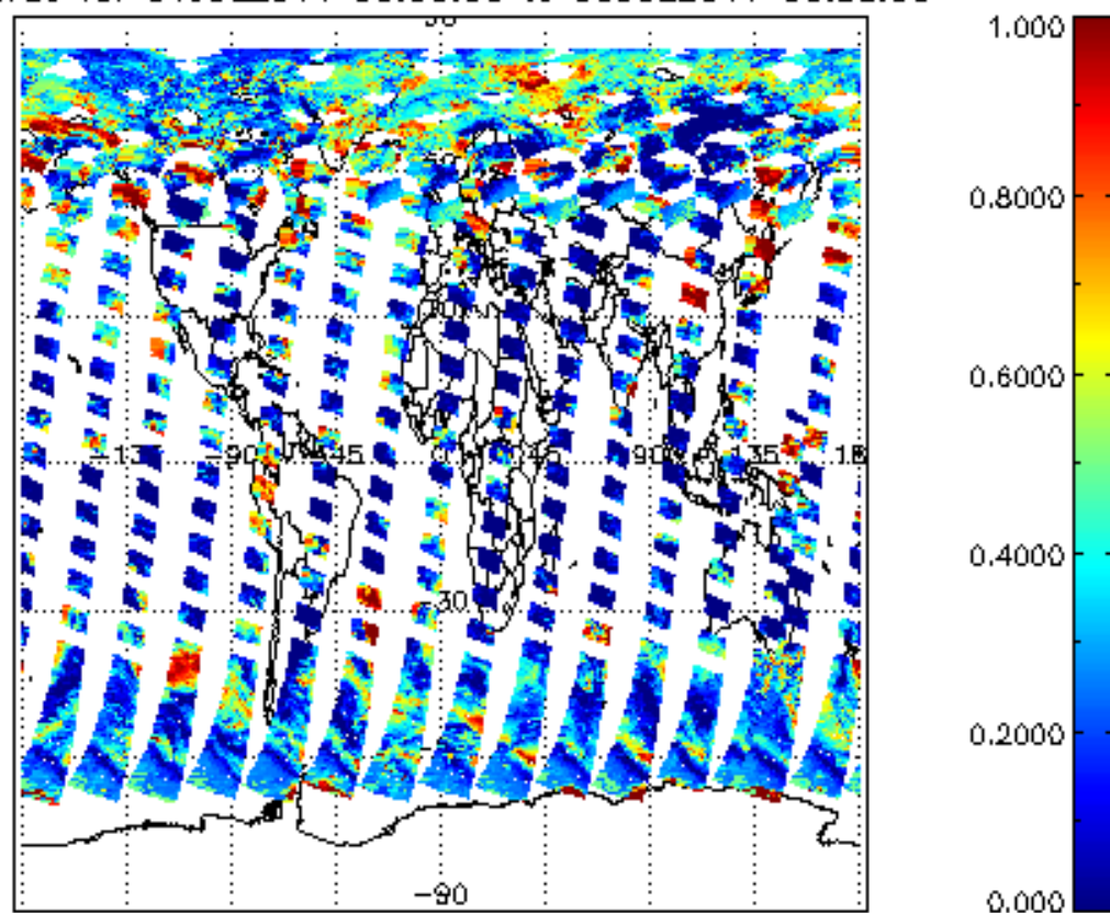
cl_frac for 04JUL2011 00:00:00 to 05JUL2011 00:00:00
