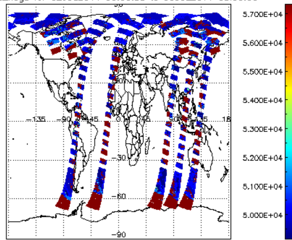
cloud_flags for 02JUL2011 00:00:00 to 03JUL2011 00:00:00
