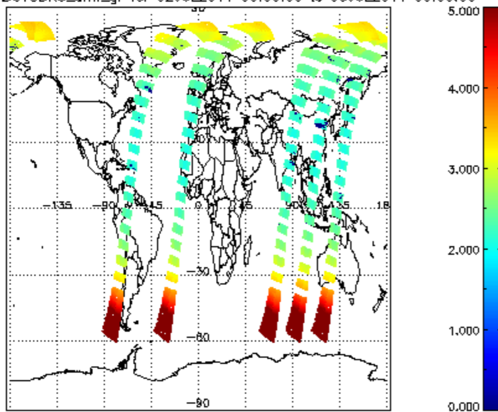
SCIOL2P_NADUV3BRO_amf_gr for 02JUL2011 00:00:00 to 03JUL2011 00:00:00
