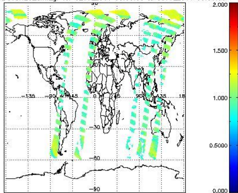
SCIOL2P_NADUV8H2O_amf_gr for 02JUL2011 00:00:00 to 03JUL2011 00:00:00
