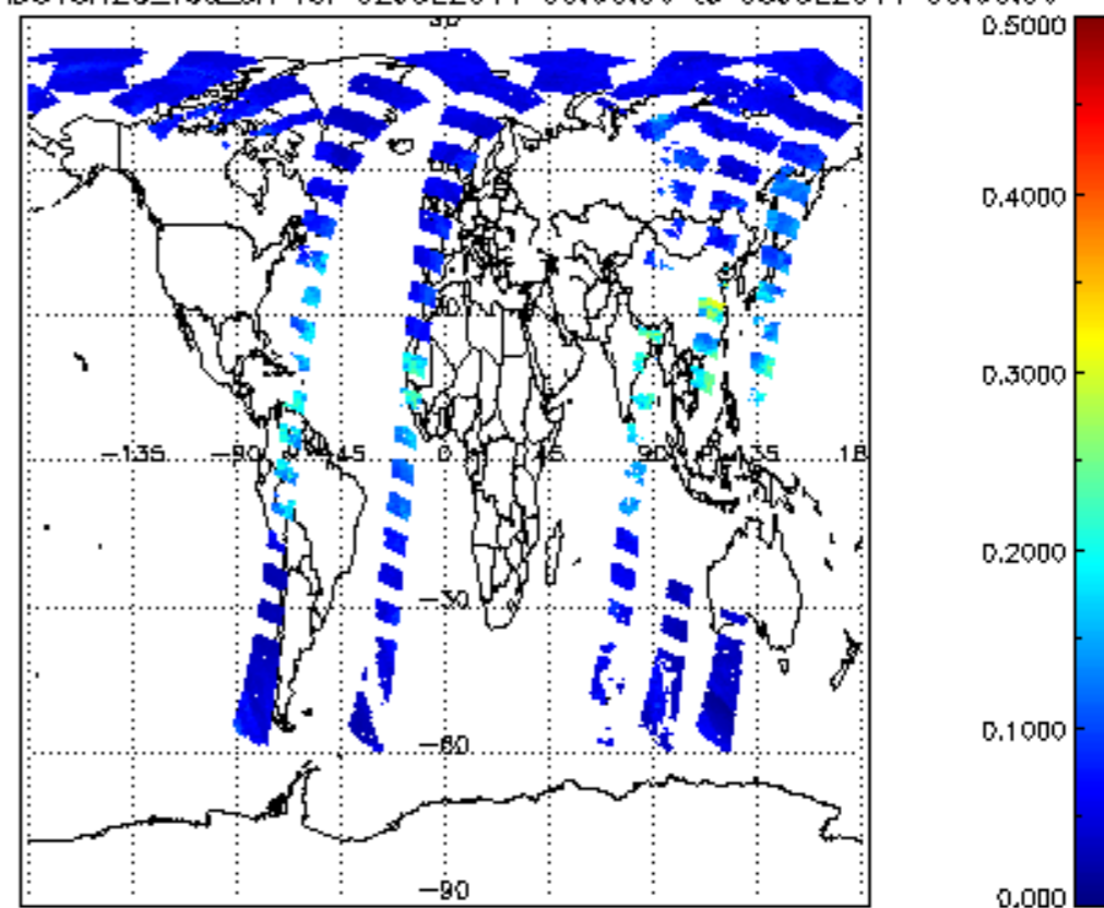
SCIOL2P_NADUV8H2O_vcd_err for 02JUL2011 00:00:00 to 03JUL2011 00:00:00
