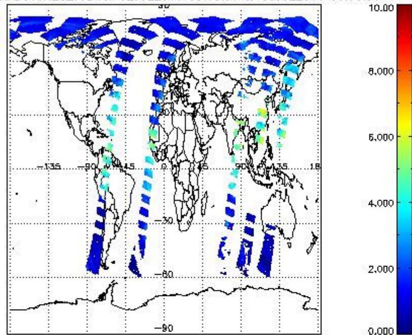
SCIOL2P_NADUV8H2O_vcd for 02JUL2011 00:00:00 to 03JUL2011 00:00:00
