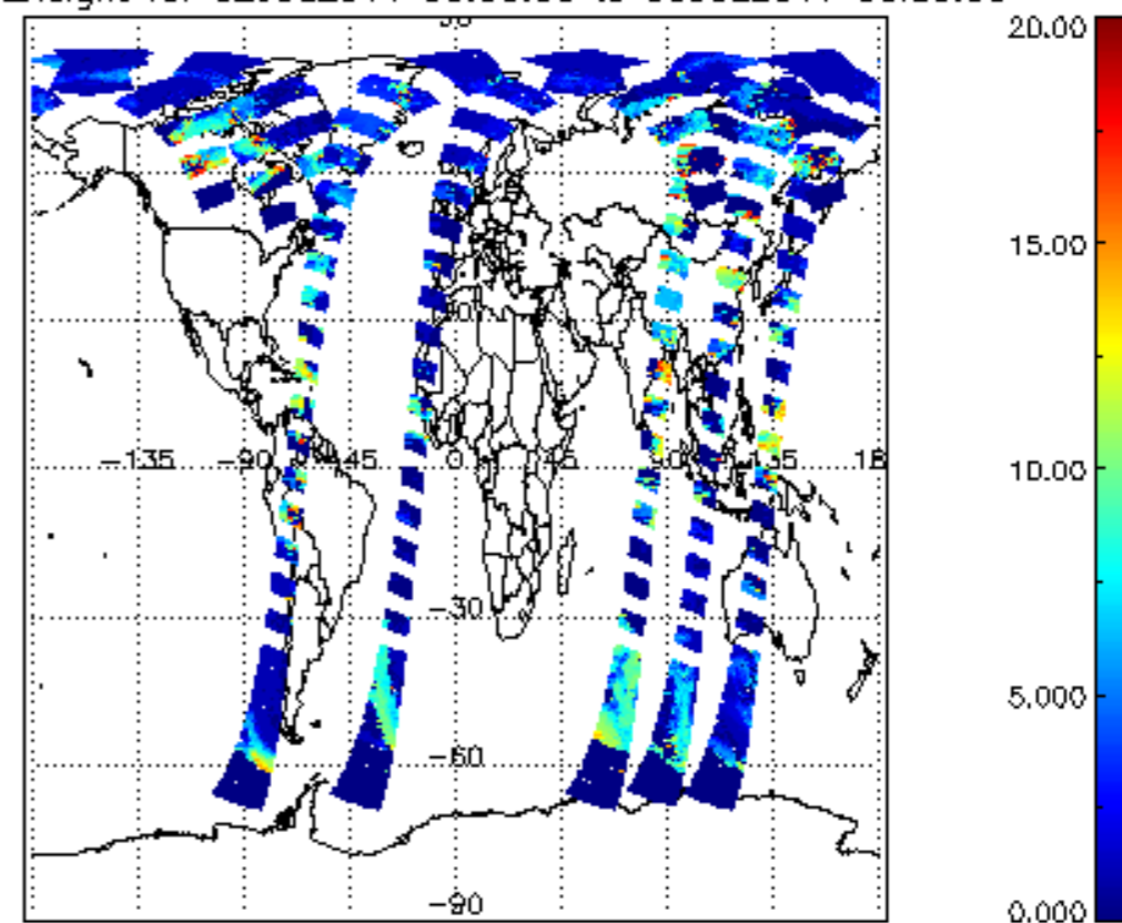
cl_top_height for 02JUL2011 00:00:00 to 03JUL2011 00:00:00
