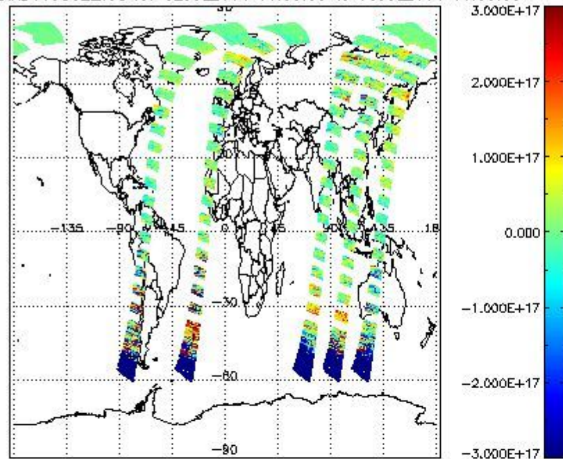
SCIOL2P_NADUV5S02_vcd for 02JUL2011 00:00:00 to 03JUL2011 00:00:00
