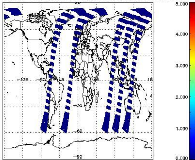
SCIOL2P_NADUV5S02_amf_cl for 02JUL2011 00:00:00 to 03JUL2011 00:00:00
