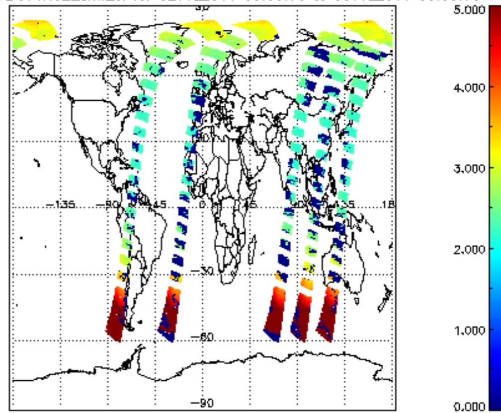
SCIOL2P_NADUV1NO2_amf_cl for 02JUL2011 00:00:00 to 03JUL2011 00:00:00
