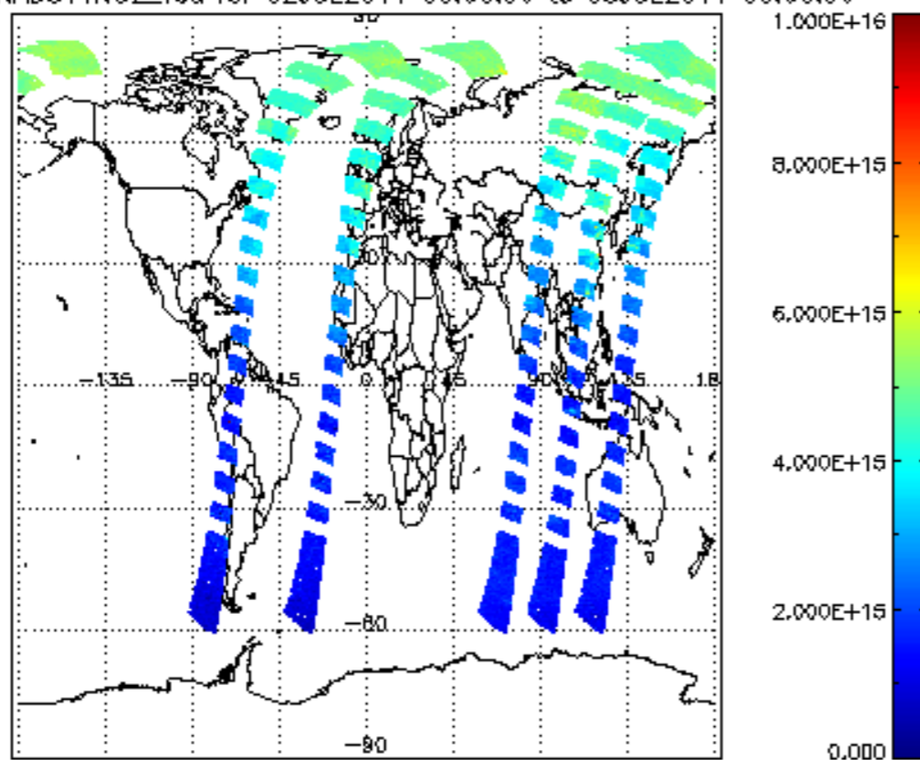
SCIOL2P_NADUV1NO2_vcd for 02JUL2011 00:00:00 to 03JUL2011 00:00:00
