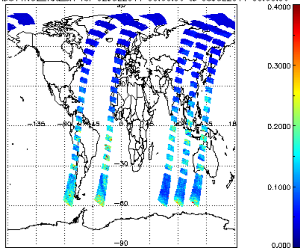
SCIOL2P_NADUV1NO2_vcd_err for 02JUL2011 00:00:00 to 03JUL2011 00:00:00
