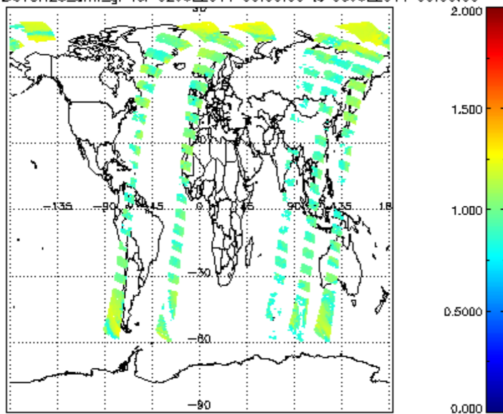
SCIOL2P_NADUV8H2O_amf_gr for 02JUL2011 00:00:00 to 03JUL2011 00:00:00
