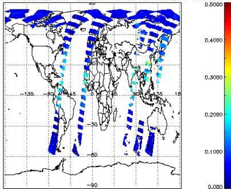
SCIOL2P_NADUV8H2O_vcd_err for 02JUL2011 00:00:00 to 03JUL2011 00:00:00
