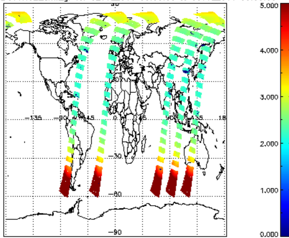
SCIOL2P_NADUV1NO2_amf_gr for 02JUL2011 00:00:00 to 03JUL2011 00:00:00
