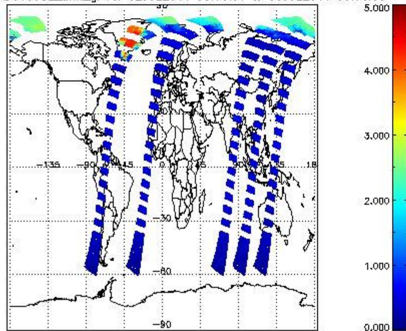
SCIOL2P_NADUV5S02_amf_gr for 02JUL2011 00:00:00 to 03JUL2011 00:00:00
