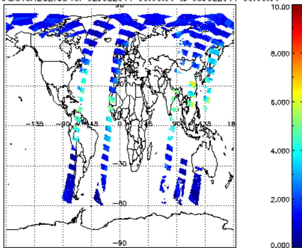
SCIOL2P_NADUV8H2O_vcd for 02JUL2011 00:00:00 to 03JUL2011 00:00:00
