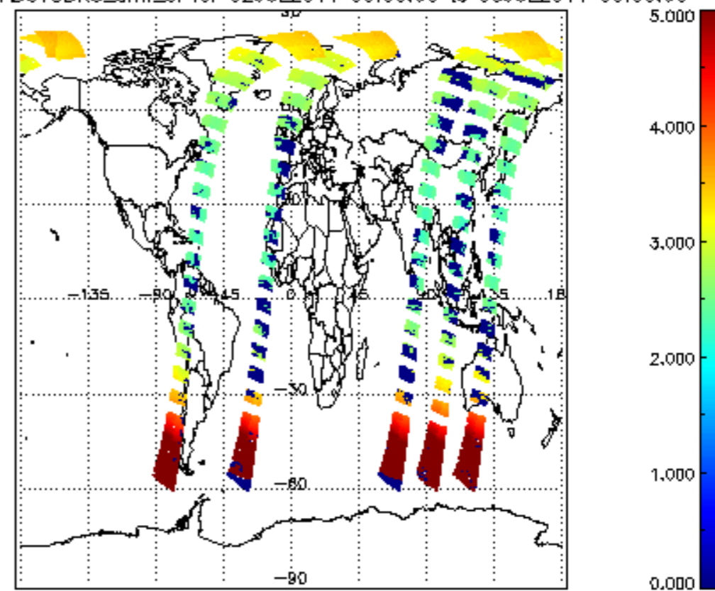
SCIOL2P_NADUV3BRO_amf_cl for 02JUL2011 00:00:00 to 03JUL2011 00:00:00
