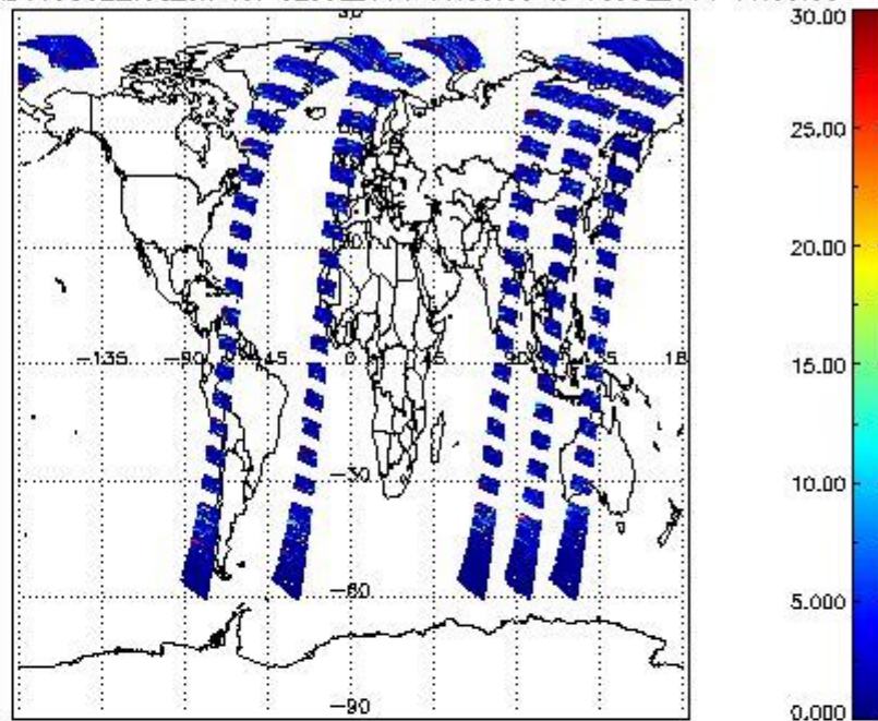
SCIOL2P_NADUV5S02_vcd_err for 02JUL2011 00:00:00 to 03JUL2011 00:00:00
