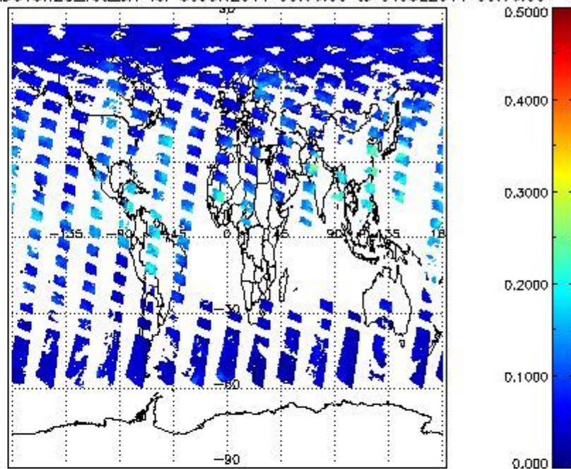
SCIOL2P_NADUV8H20_vcdLerr for 30JUN2011 00:00:00 to 01JUL2011 00:00:00
