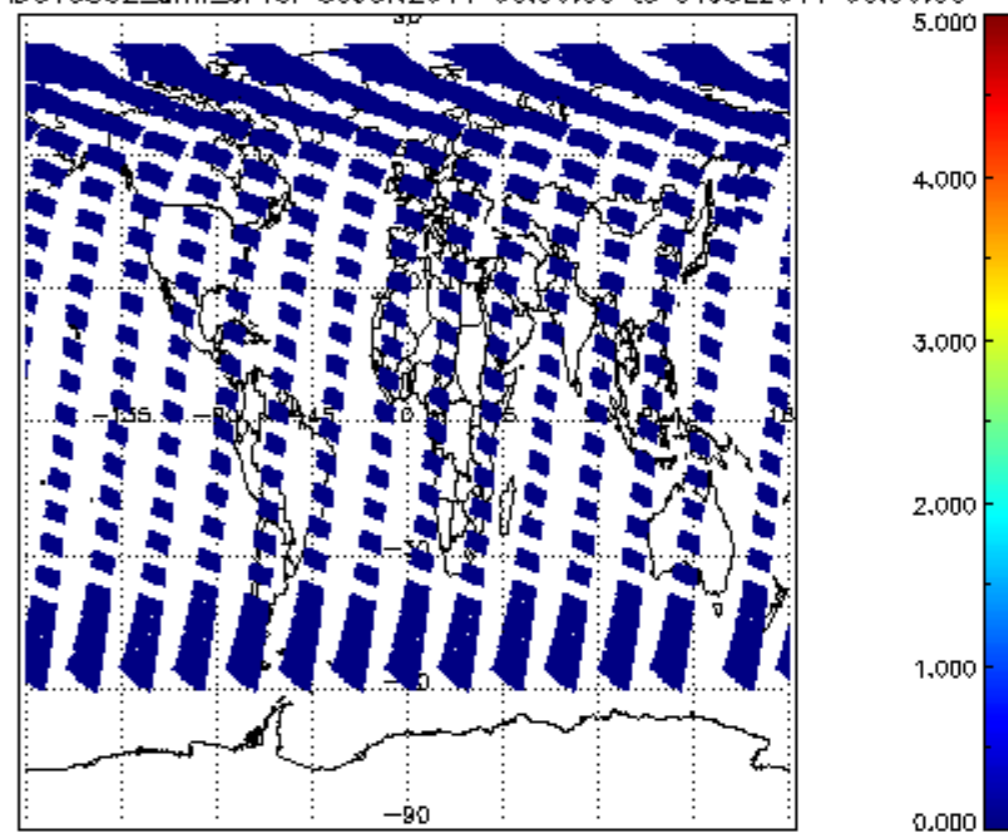
SCIOL2P_NADUV5S02_amf_cl for 30JUN2011 00:00:00 to 01JUL2011 00:00:00
