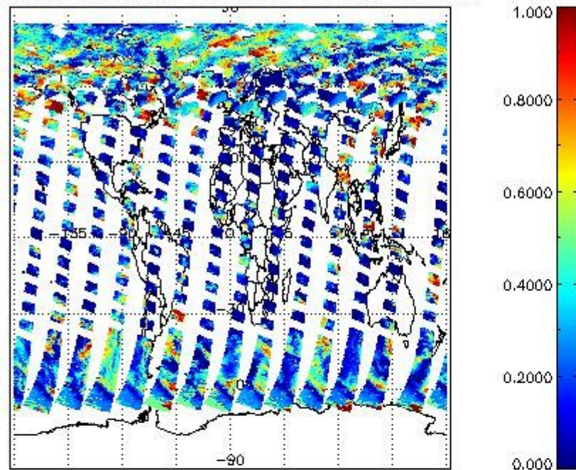
cL_frac for 30JUN2011 00:00:00 to 01JUL2011 00:00:00
