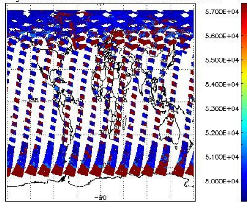
cloud_flags for 30JUN2011 00:00:00 to 01JUL2011 00:00:00
