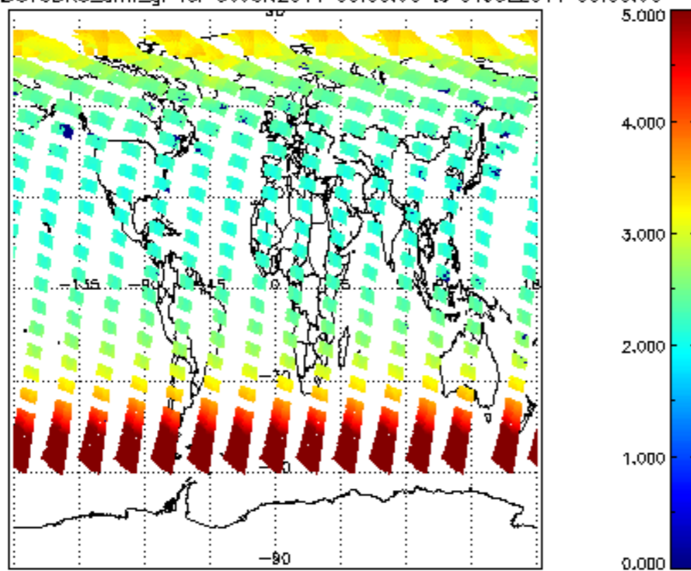
SCIOL2P_NADUV3BRO_amf_gr for 30JUN2011 00:00:00 to 01JUL2011 00:00:00
