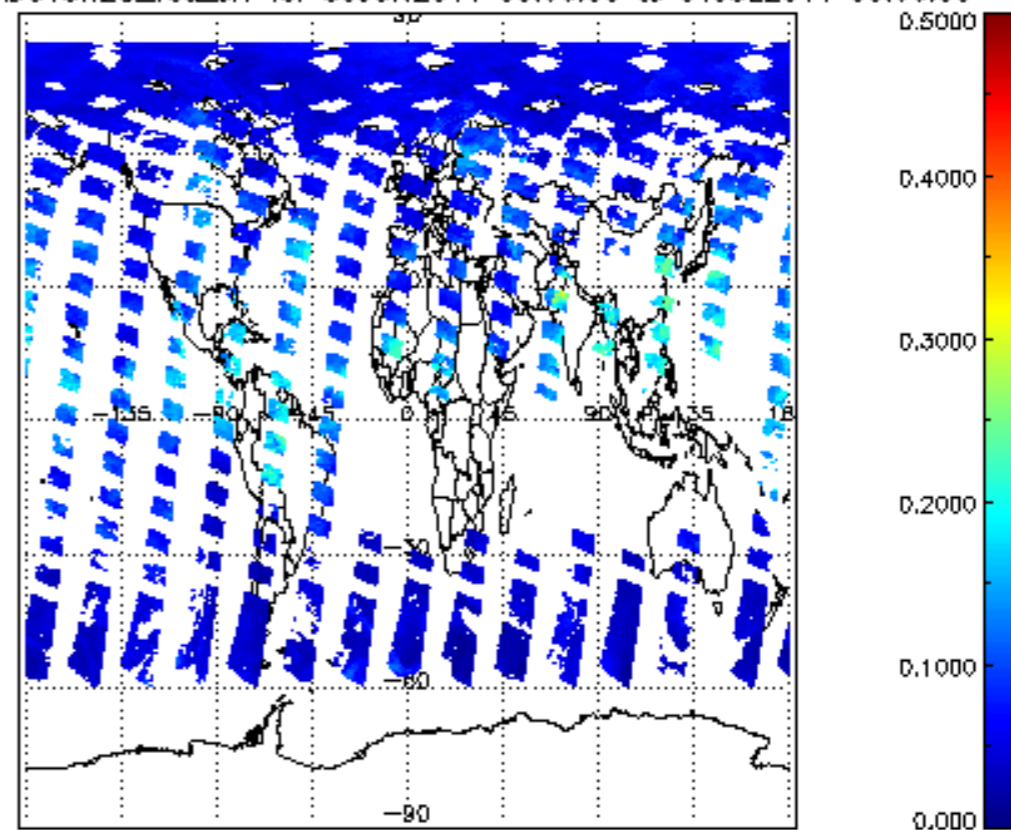
SCIOL2P_NADUV8H20_vcd_err for 30JUN2011 00:00:00 to 01JUL2011 00:00:00
