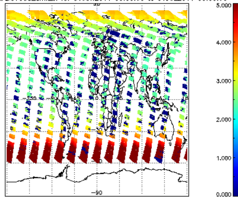
SCIOL2P_NADUV003_amf_cl for 30JUN2011 00:00:00 to 01JUL2011 00:00:00
