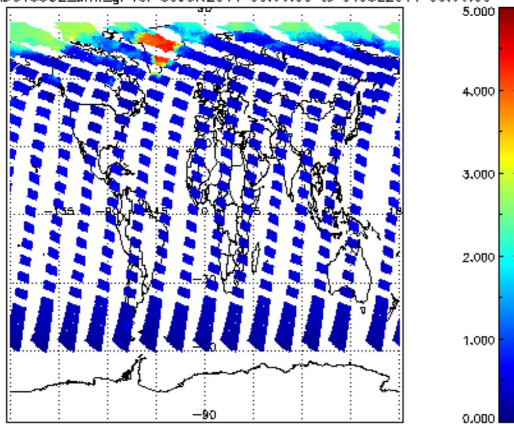
SCIOL2P_NADUV5S02_amf_gr for 30JUN2011 00:00:00 to 01JUL2011 00:00:00
