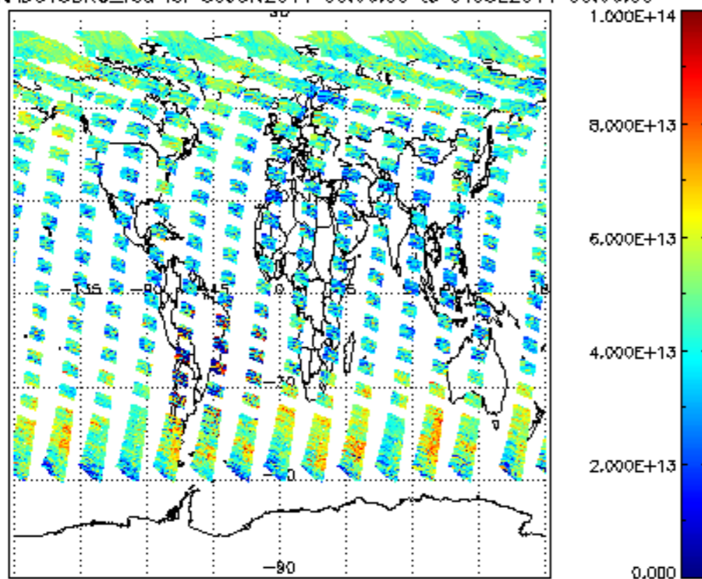
SCIOL2P_NADUV3BRO_vcd for 30JUN2011 00:00:00 to 01JUL2011 00:00:00
