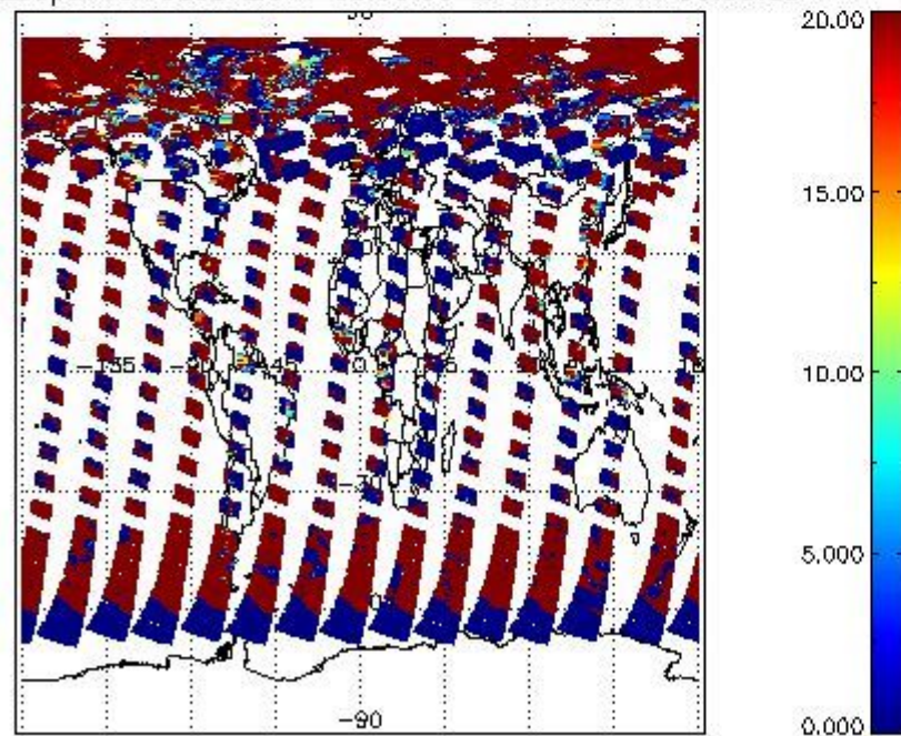
cL_opt_depth for 30JUN2011 00:00:00 to 01JUL2011 00:00:00
