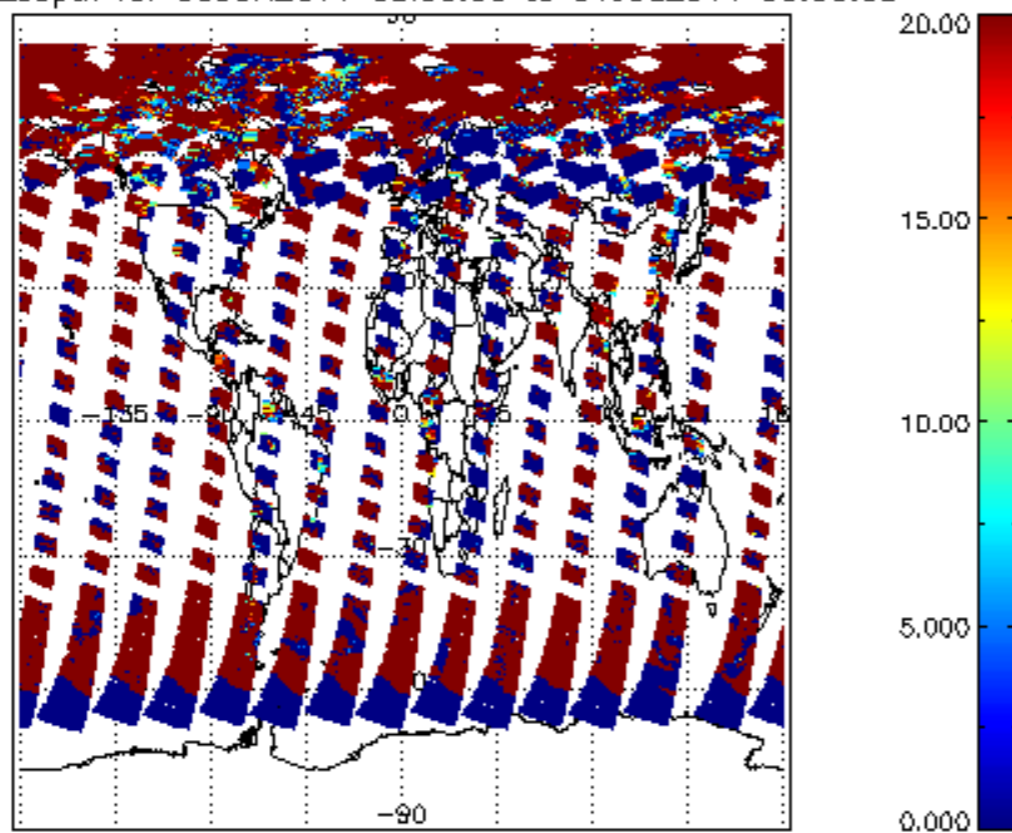
cl_opt_depth for 30JUN2011 00:00:00 to 01JUL2011 00:00:00
