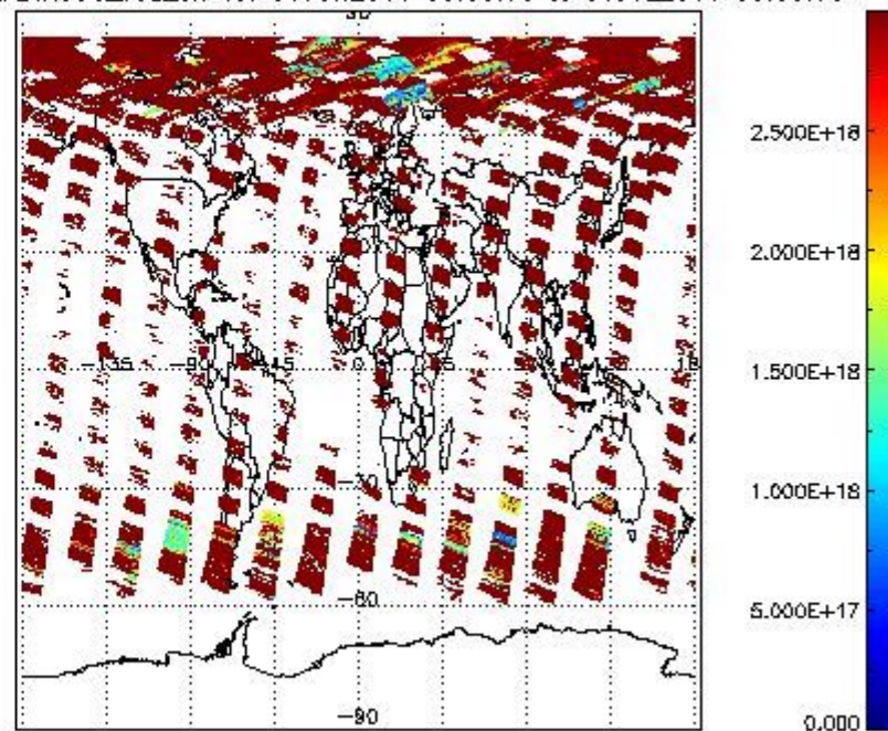
SCIDL2P_NADIR3CO_vcd_err for 30JUN2011 00:00:00 to 01JUL2011 00:00:00
