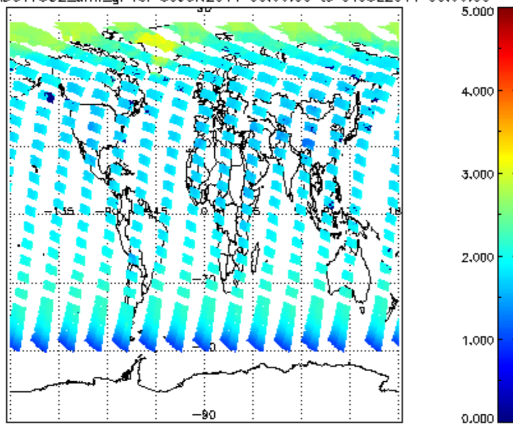
SCIOL2P_NADUV7S02_amf_gr for 30JUN2011 00:00:00 to 01JUL2011 00:00:00
