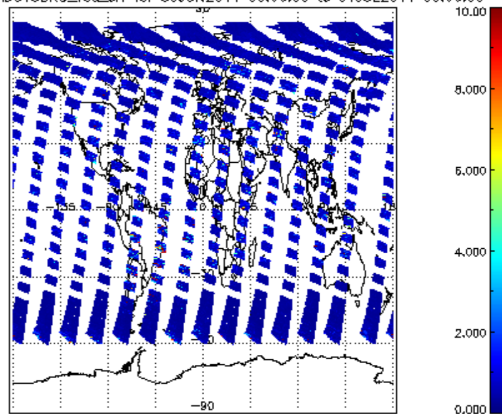
SCIOL2P_NADUV3BRO_vcd_err for 30JUN2011 00:00:00 to 01JUL2011 00:00:00
