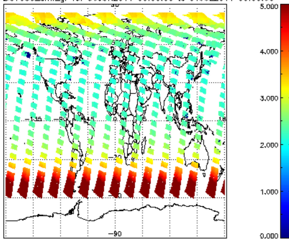
SCIOL2P_NADUV003_amf_gr for 30JUN2011 00:00:00 to 01JUL2011 00:00:00
