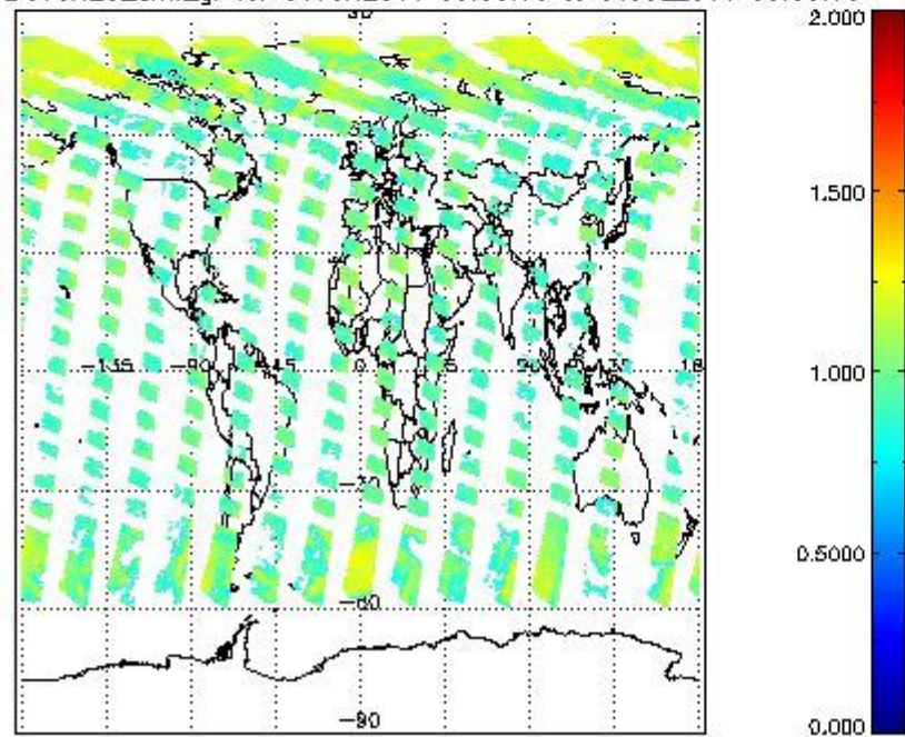
SCIOL2P_NADUV8H20_amf_gr for 30JUN2011 00:00:00 to 01JUL2011 00:00:00
