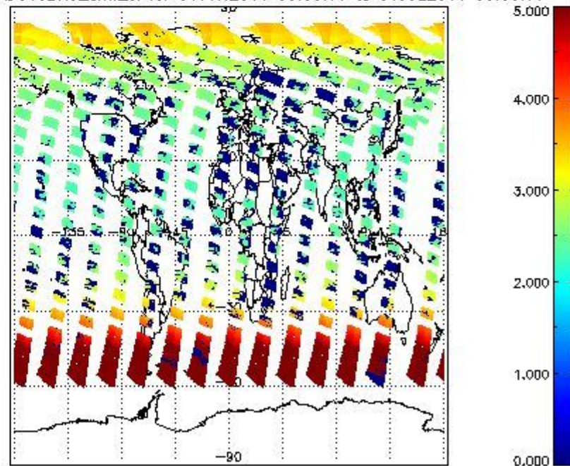
SCIOL2P_NADUV3BRO_amf_cl for 30JUN2011 00:00:00 to 01JUL2011 00:00:00
