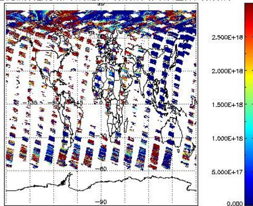
SCIDL2P_NADIR3CO_vcd for 30JUN2011 00:00:00 to 01JUL2011 00:00:00
