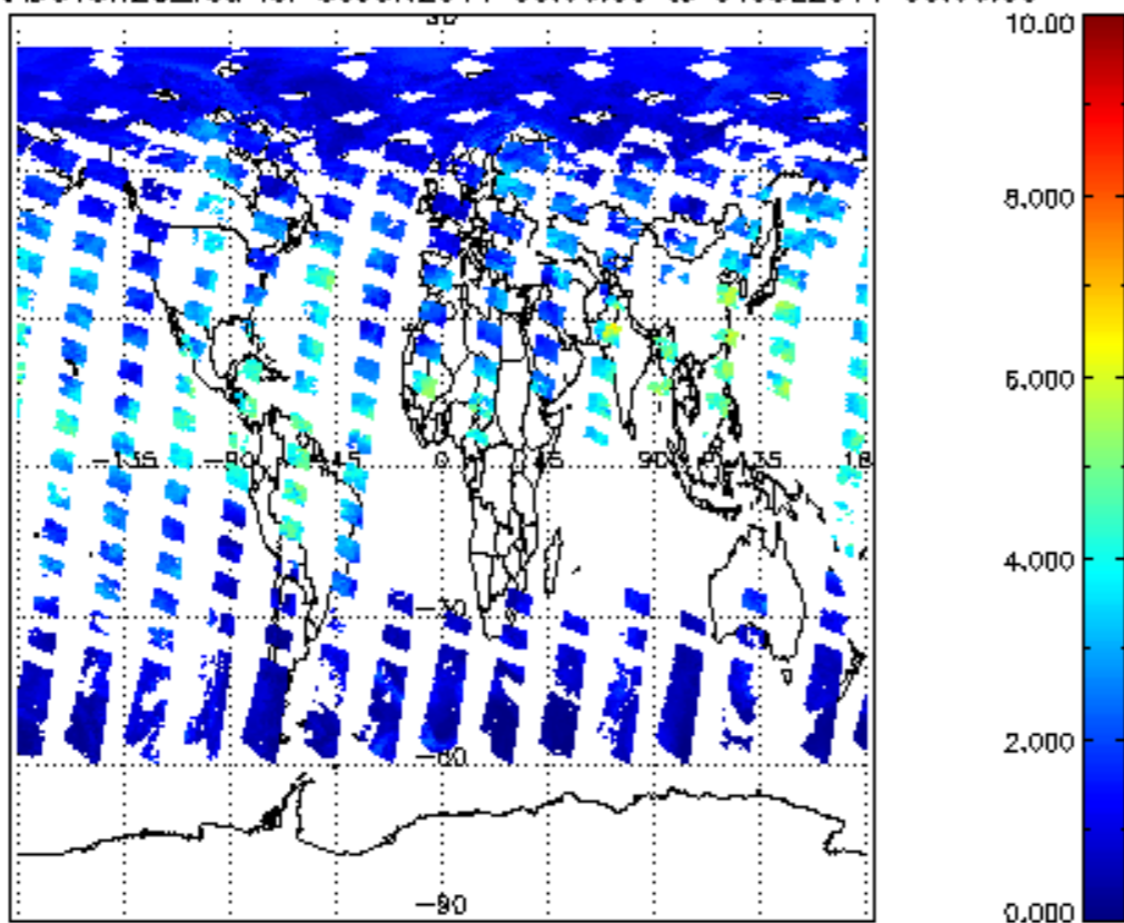
SCIOL2P_NADUV8H20_vcd for 30JUN2011 00:00:00 to 01JUL2011 00:00:00
