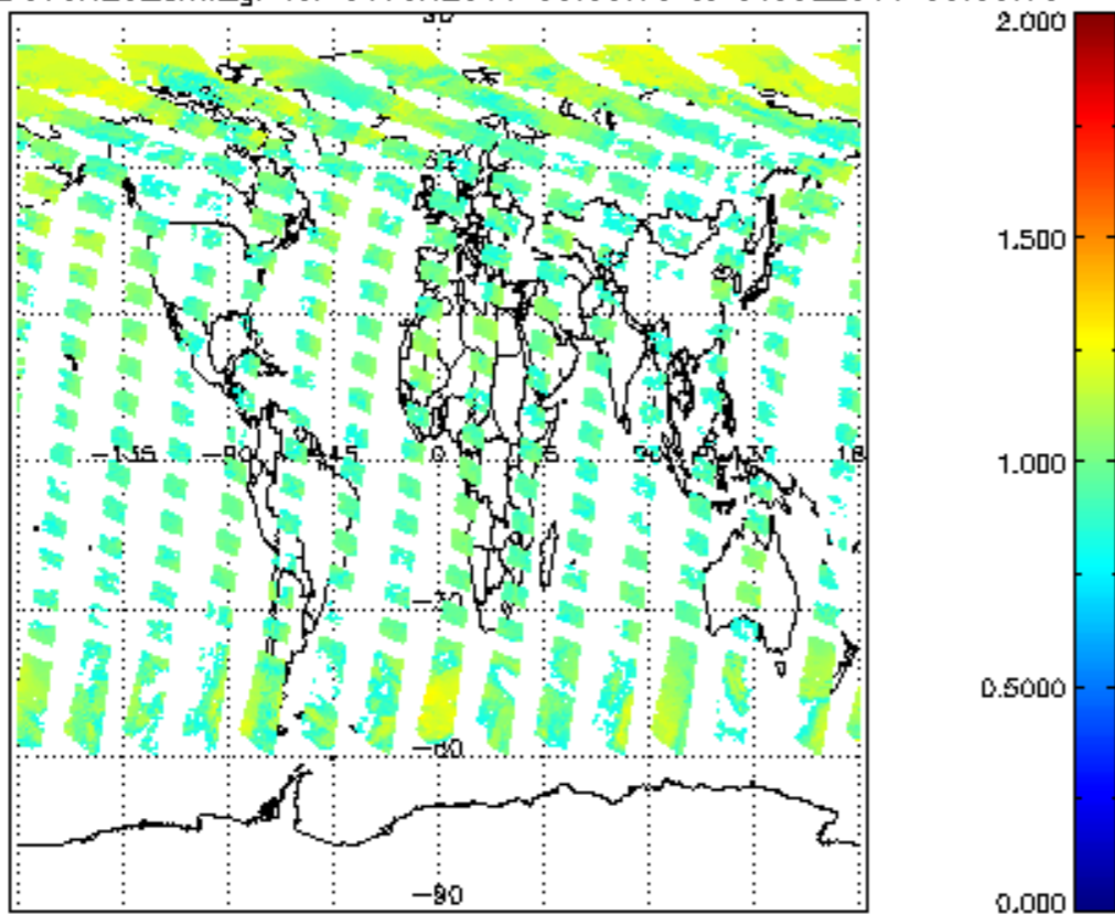
SCIOL2P_NADUV8H20_amf_gr for 30JUN2011 00:00:00 to 01JUL2011 00:00:00
