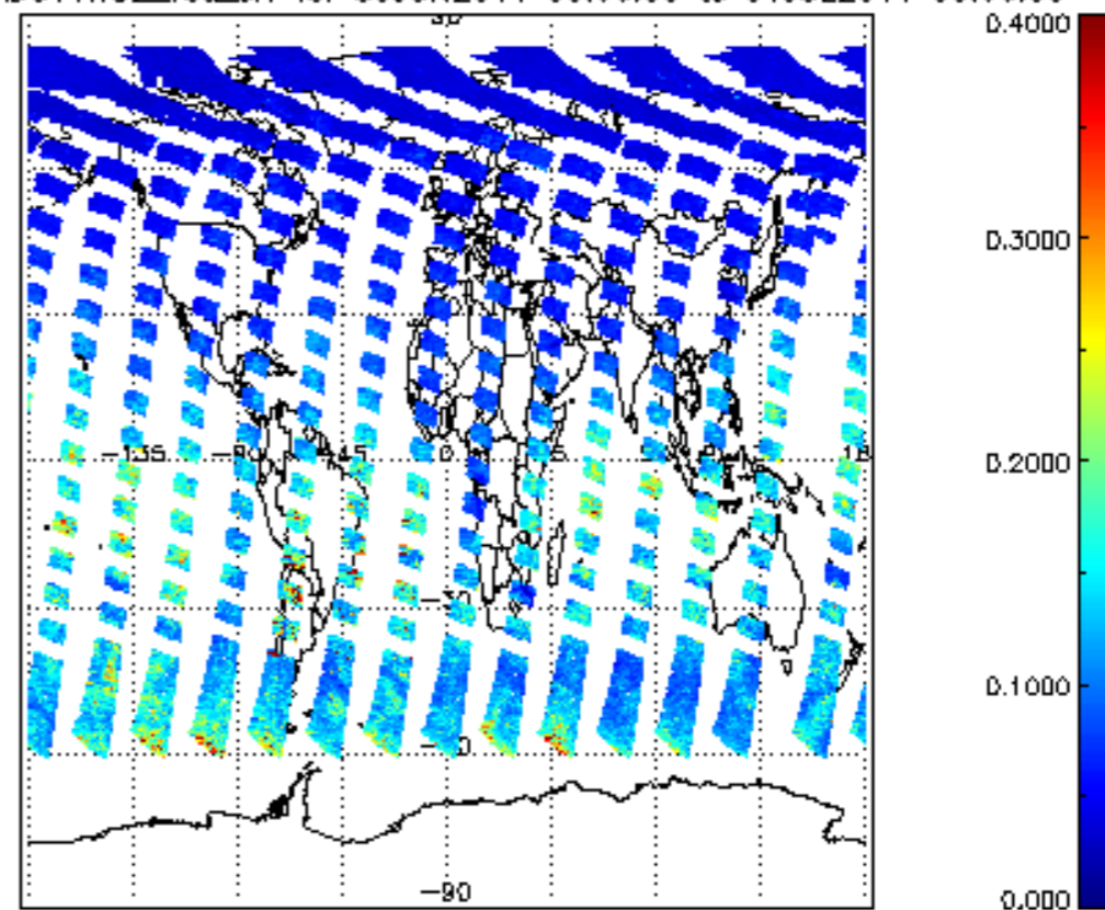
SCIOL2P_NADUV1NO2_vcd_err for 30JUN2011 00:00:00 to 01JUL2011 00:00:00
