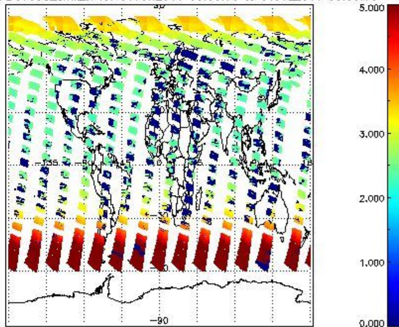
SCIOL2P_NADUV003_amf_cl for 30JUN2011 00:00:00 to 01JUL2011 00:00:00
