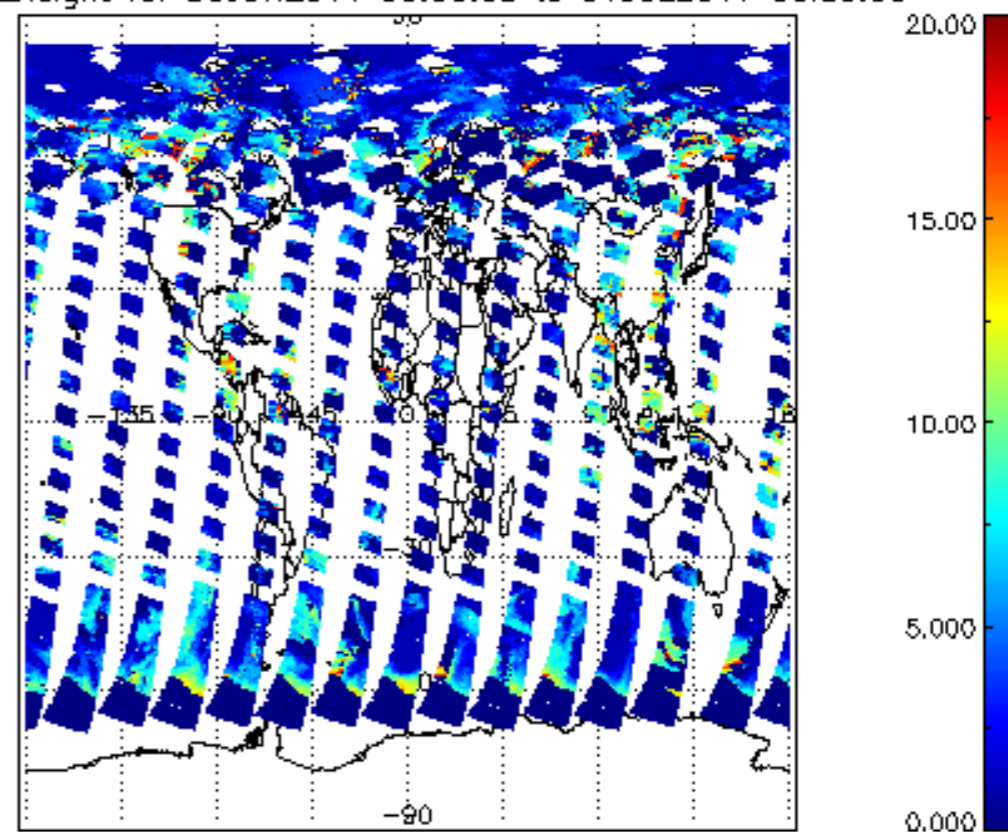
cl_top_height for 30JUN2011 00:00:00 to 01JUL2011 00:00:00
