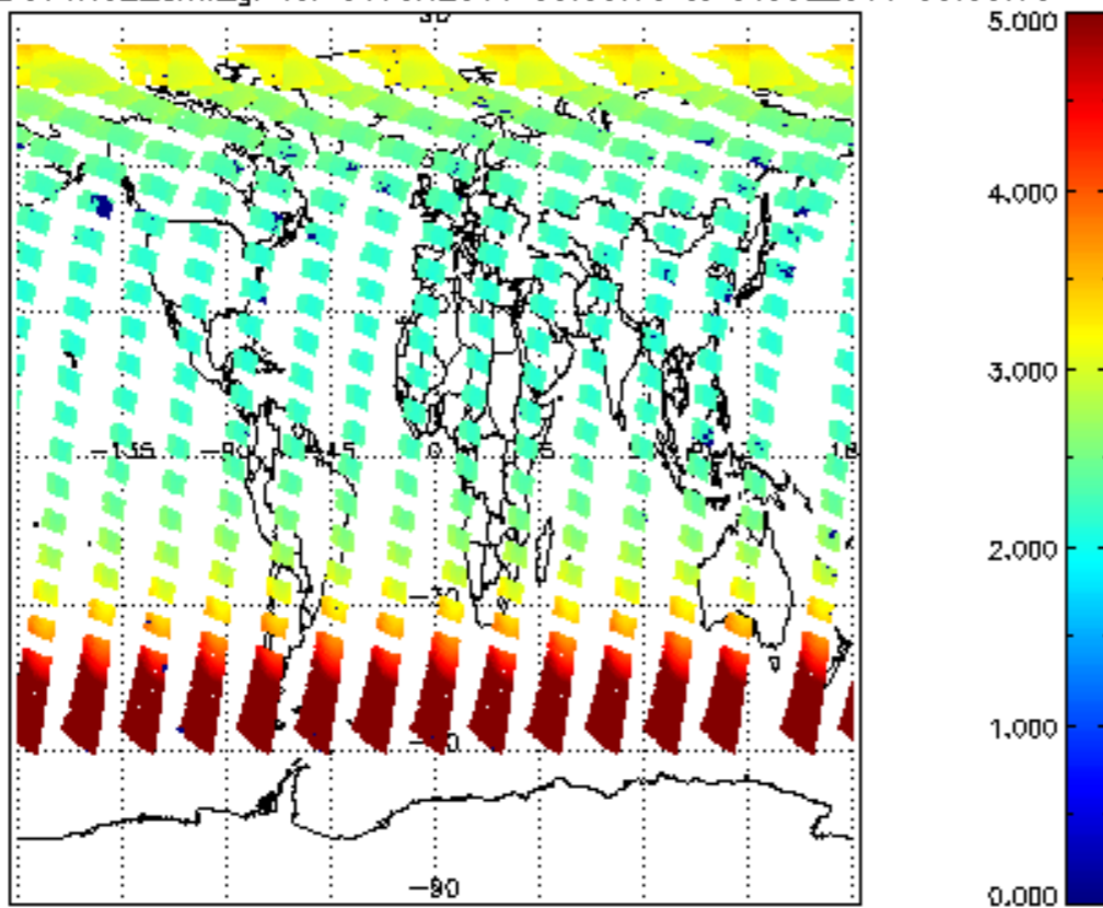
SCIOL2P_NADUV1NO2_amf_gr for 30JUN2011 00:00:00 to 01JUL2011 00:00:00
