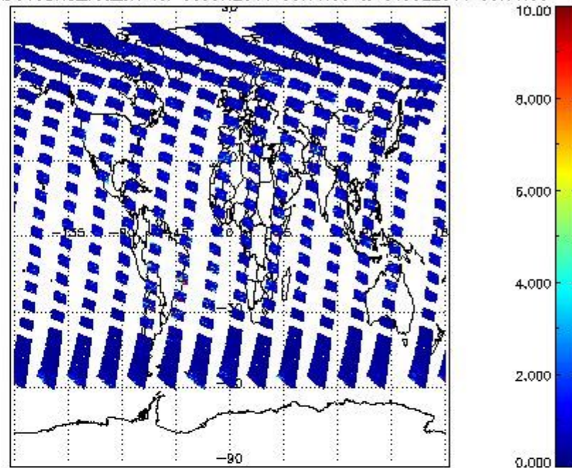
SCIOL2P_NADUV3BRO_vcdLerr for 30JUN2011 00:00:00 to 01JUL2011 00:00:00
