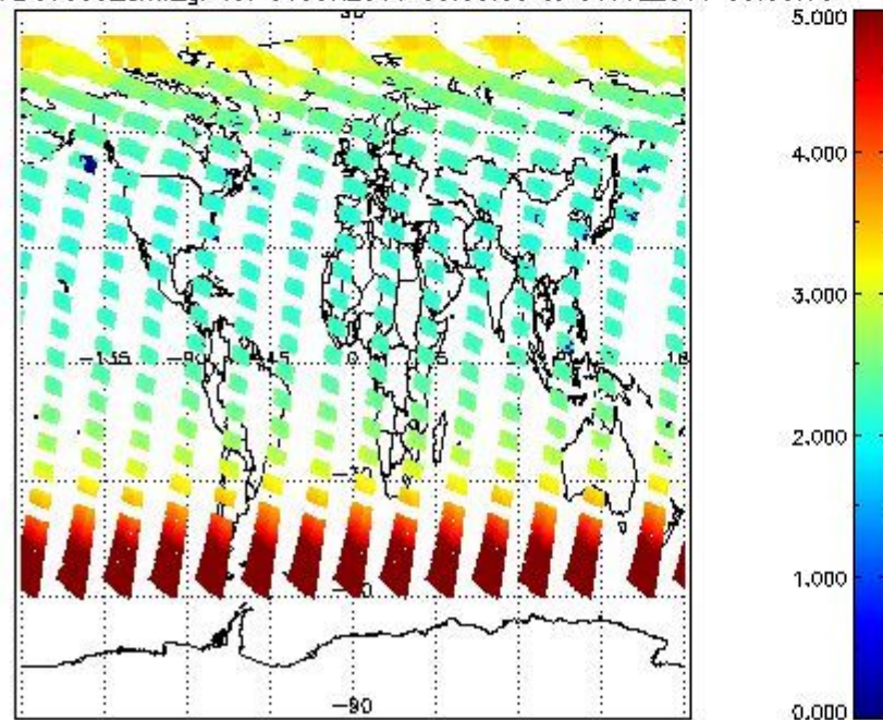
SCIOL2P_NADUV003_amf_gr for 30JUN2011 00:00:00 to 01JUL2011 00:00:00
