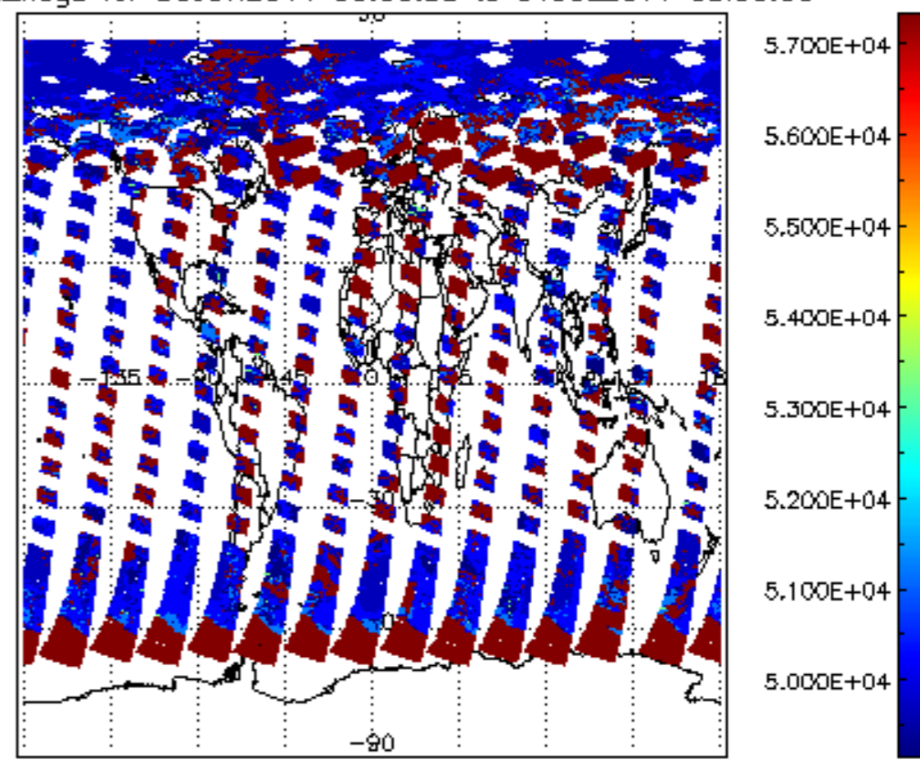
cloud_flags for 30JUN2011 00:00:00 to 01JUL2011 00:00:00
