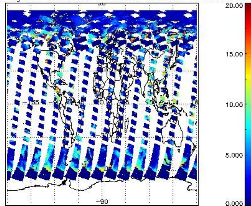
cL_top_height for 30JUN2011 00:00:00 to 01JUL2011 00:00:00
