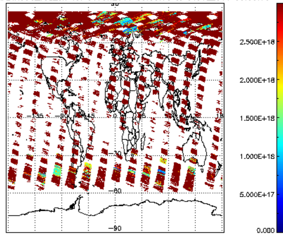
SCIOL2P_NADIR3CO_vcd_err for 30JUN2011 00:00:00 to 01JUL2011 00:00:00
