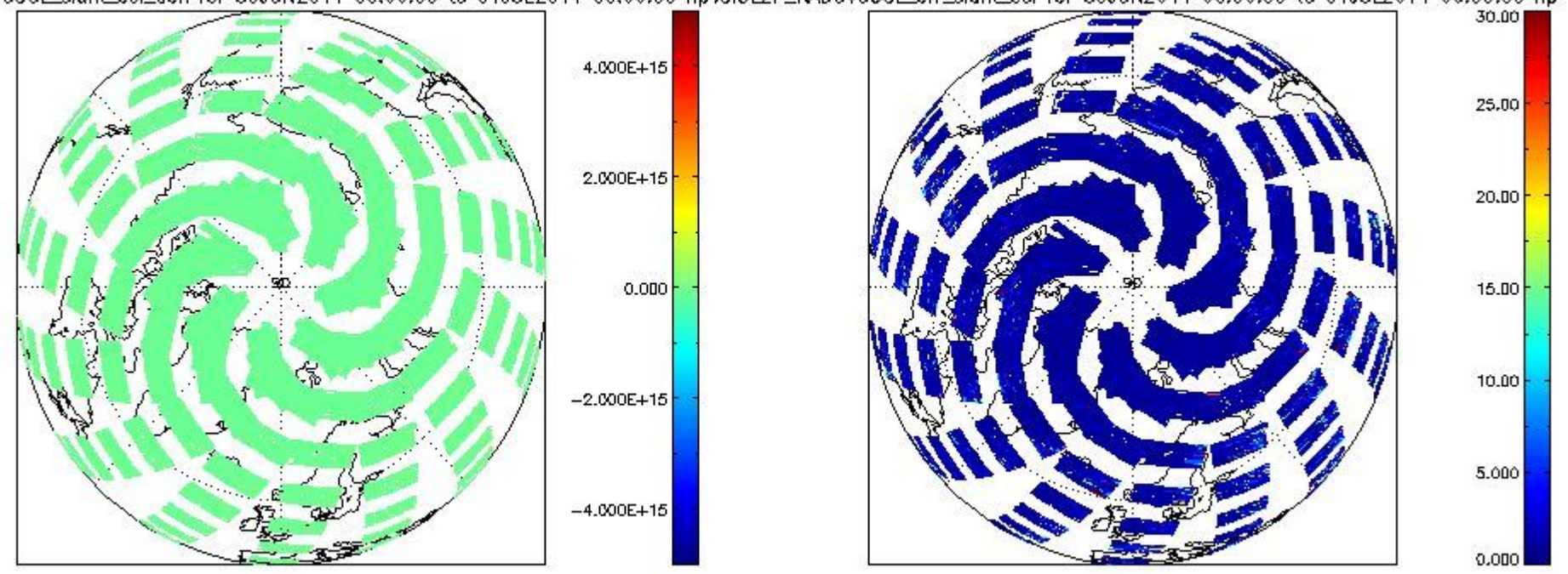
CIOL2P_NADUV60CLslant_col_den for 30JUN2011 00:00:00 to 01JUL2011 00:00:00 np; CIOL2P_NADUV60CLarr_slant_col for 30JUN2011 00:00:00 to 01JUL2011 00:00:00 np
