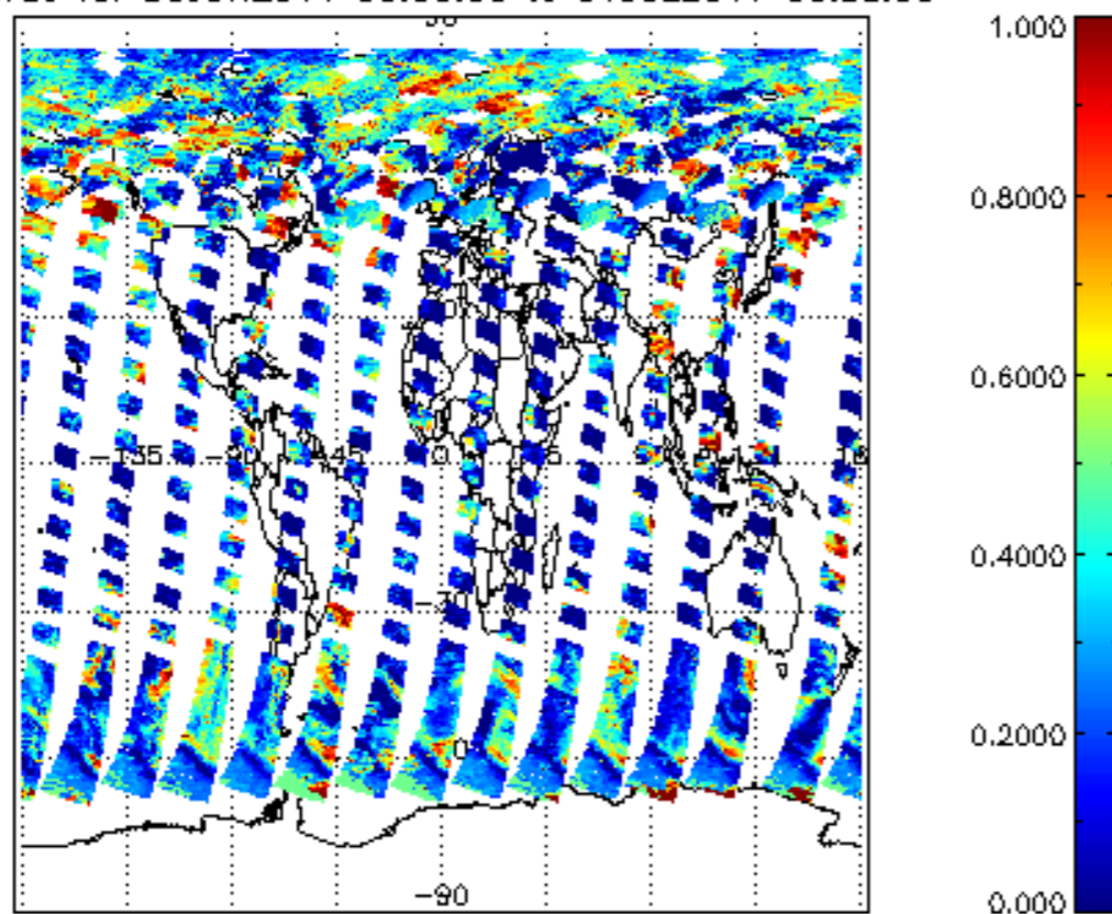
cl_frac for 30JUN2011 00:00:00 to 01JUL2011 00:00:00
