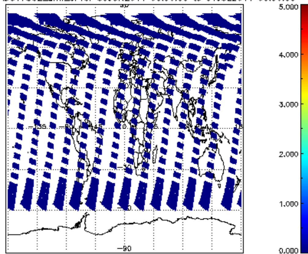
SCIOL2P_NADUV7S02_amf_cl for 30JUN2011 00:00:00 to 01JUL2011 00:00:00
