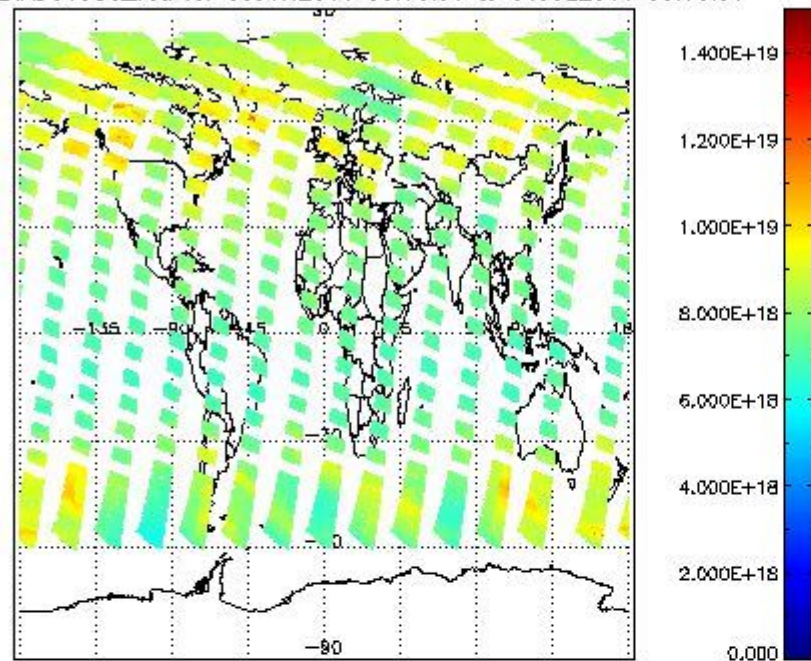
SCIOL2P_NADUV003_vcd for 30JUN2011 00:00:00 to 01JUL2011 00:00:00
