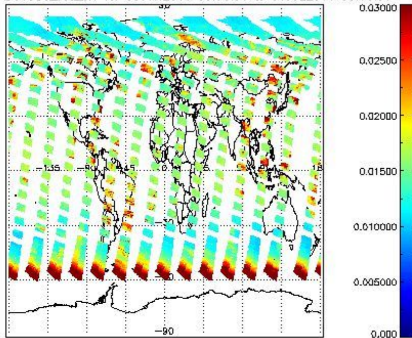
SCIOL2P_NADUV003_vcd_err for 30JUN2011 00:00:00 to 01JUL2011 00:00:00
