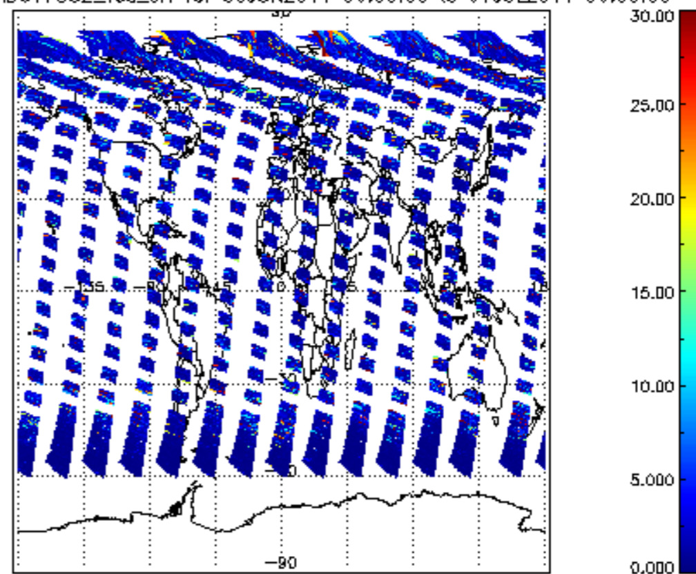
SCIOL2P_NADUV7S02_vcd_err for 30JUN2011 00:00:00 to 01JUL2011 00:00:00
