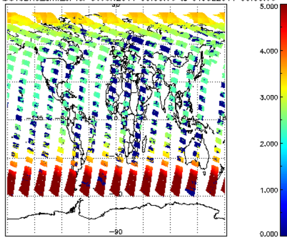
SCIOL2P_NADUV3BRO_amf_cl for 30JUN2011 00:00:00 to 01JUL2011 00:00:00
