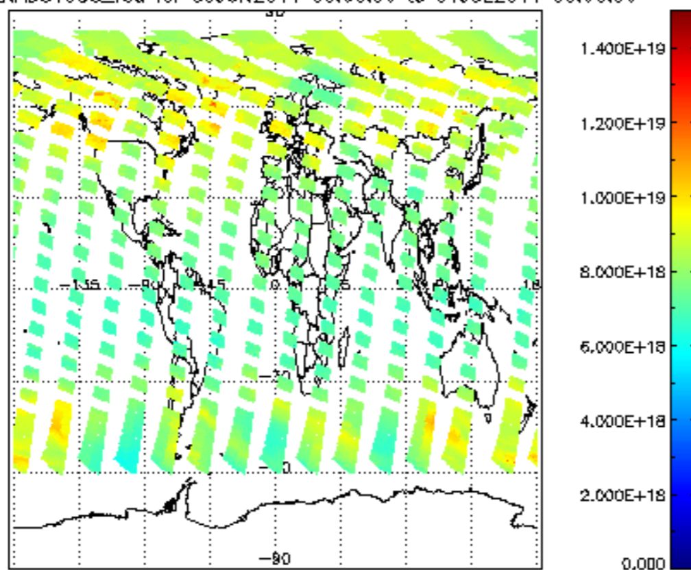
SCIOL2P_NADUV003_vcd for 30JUN2011 00:00:00 to 01JUL2011 00:00:00
