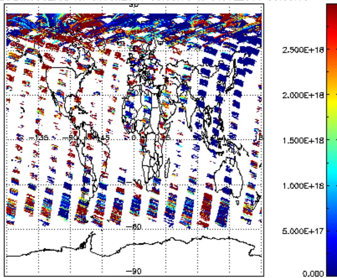
SCIOL2P_NADIR3CO_vcd for 30JUN2011 00:00:00 to 01JUL2011 00:00:00
