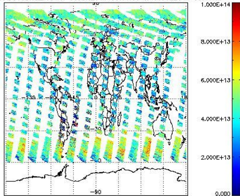
SCIOL2P_NADUV3BRO_vcd for 30JUN2011 00:00:00 to 01JUL2011 00:00:00
