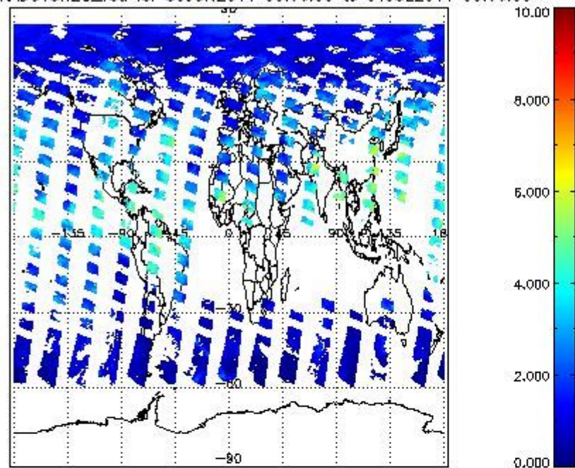
SCIOL2P_NADUV8H20_vcd for 30JUN2011 00:00:00 to 01JUL2011 00:00:00
