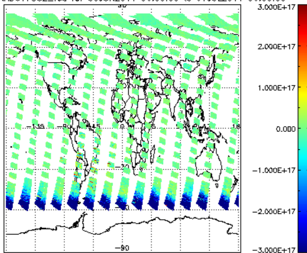
SCIOL2P_NADUV7S02_vcd for 30JUN2011 00:00:00 to 01JUL2011 00:00:00
