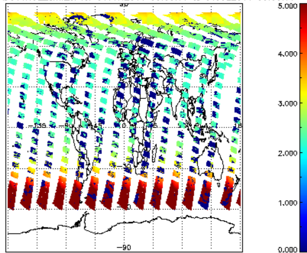
SCIOL2P_NADUV1NO2_amf_cl for 30JUN2011 00:00:00 to 01JUL2011 00:00:00
