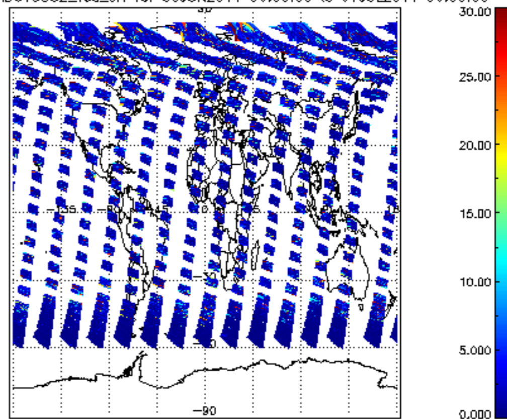
SCIOL2P_NADUV5S02_vcd_err for 30JUN2011 00:00:00 to 01JUL2011 00:00:00
