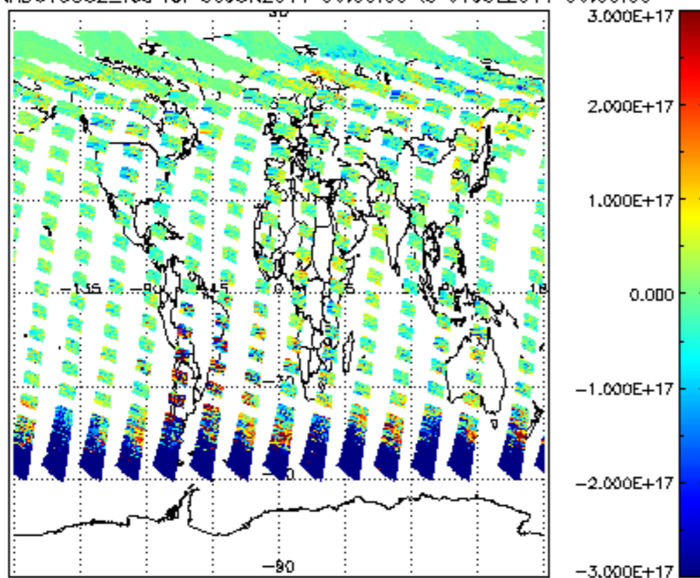
SCIOL2P_NADUV5S02_vcd for 30JUN2011 00:00:00 to 01JUL2011 00:00:00
