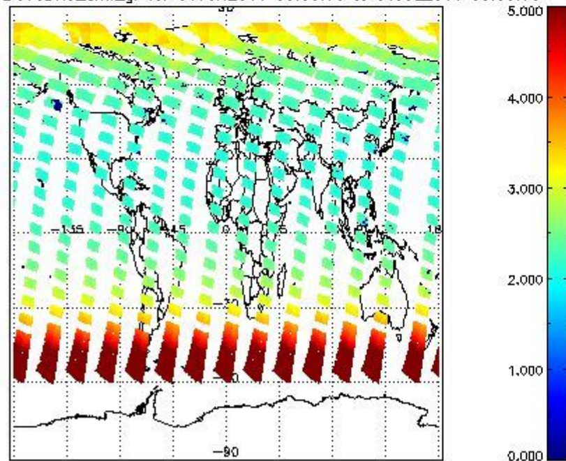
SCIOL2P_NADUV3BRO_amf_gr for 30JUN2011 00:00:00 to 01JUL2011 00:00:00
