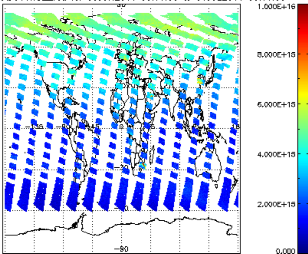
SCIOL2P_NADUV1NO2_vcd for 30JUN2011 00:00:00 to 01JUL2011 00:00:00
