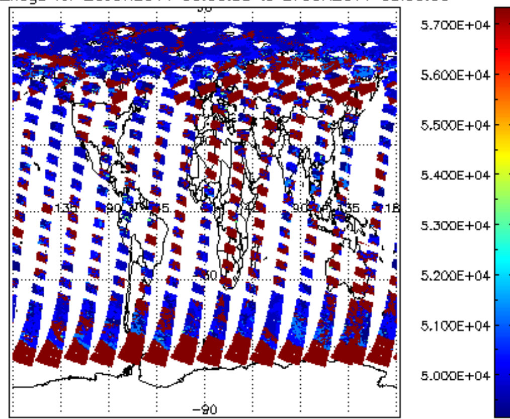
cloud_flags for 26JUN2011 00:00:00 to 27JUN2011 00:00:00
