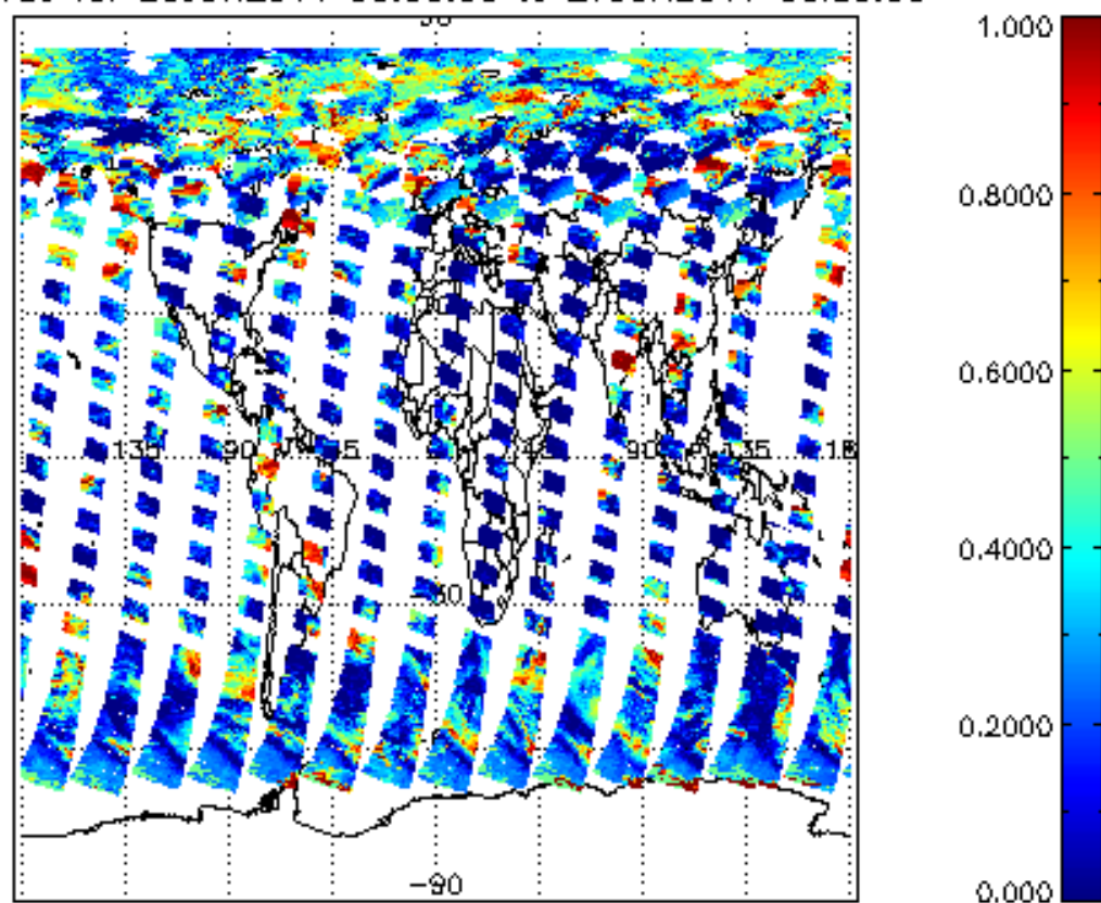
cl_frac for 26JUN2011 00:00:00 to 27JUN2011 00:00:00
