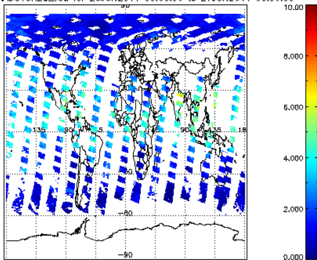
SCIOL2P_NADUV8H20_vcd for 26JUN2011 00:00:00 to 27JUN2011 00:00:00
