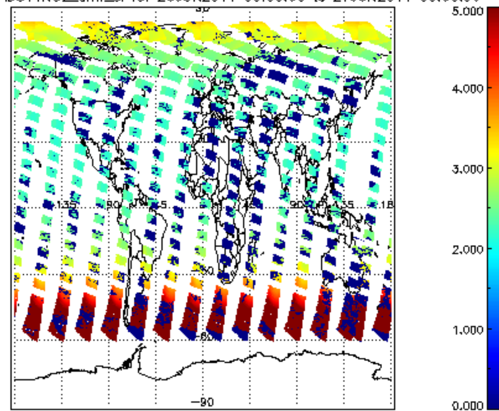
SCIOL2P_NADUV1NO2_amf_cl for 26JUN2011 00:00:00 to 27JUN2011 00:00:00
