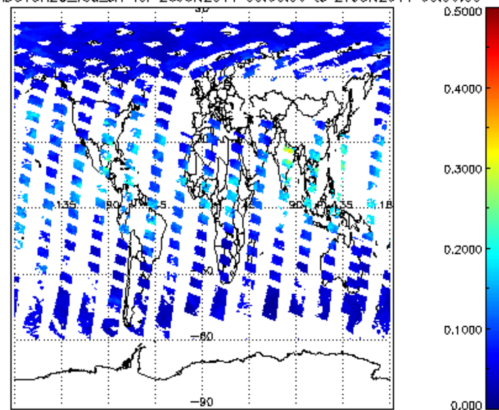
SCIOL2P_NADUV8H20_vcd_err for 26JUN2011 00:00:00 to 27JUN2011 00:00:00
