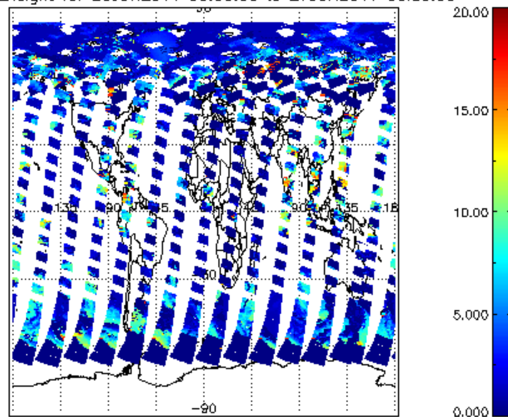
cl_top_height for 26JUN2011 00:00:00 to 27JUN2011 00:00:00
