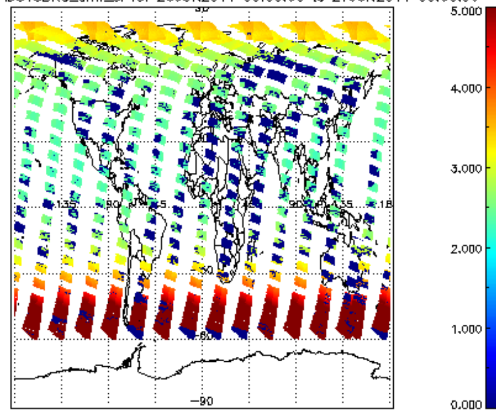
SCIOL2P_NADUV3BRO_amf_sl for 26JUN2011 00:00:00 to 27JUN2011 00:00:00
