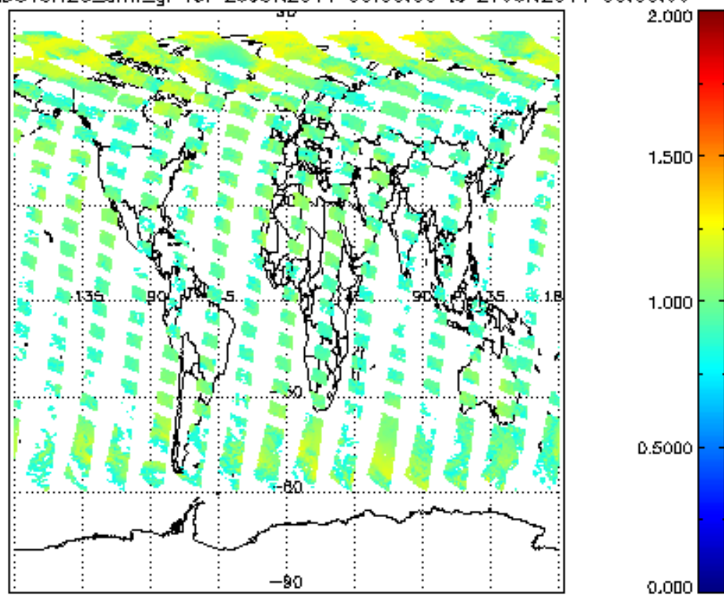
SCIOL2P_NADUV8H20_amf_gr for 26JUN2011 00:00:00 to 27JUN2011 00:00:00
