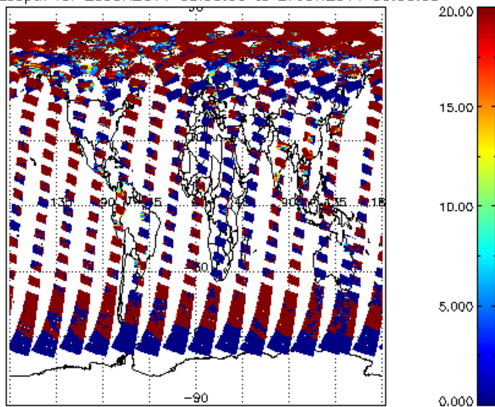
cl_opt_depth for 26JUN2011 00:00:00 to 27JUN2011 00:00:00
