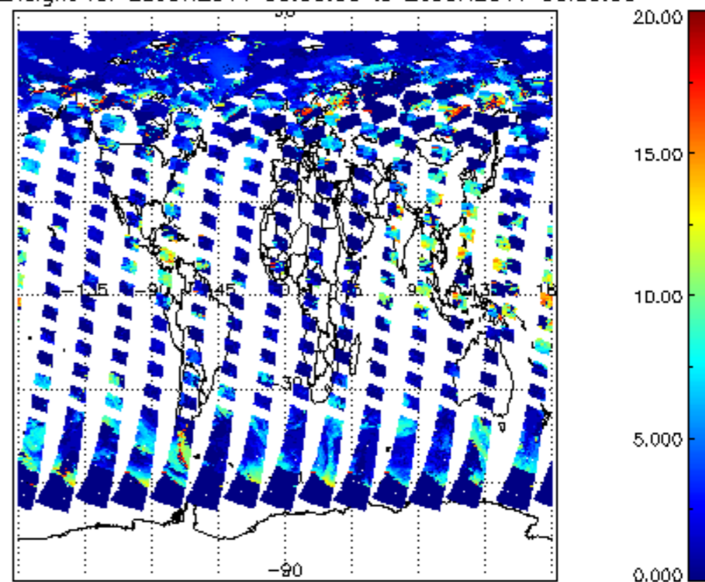
cl_top_height for 25JUN2011 00:00:00 to 26JUN2011 00:00:00
