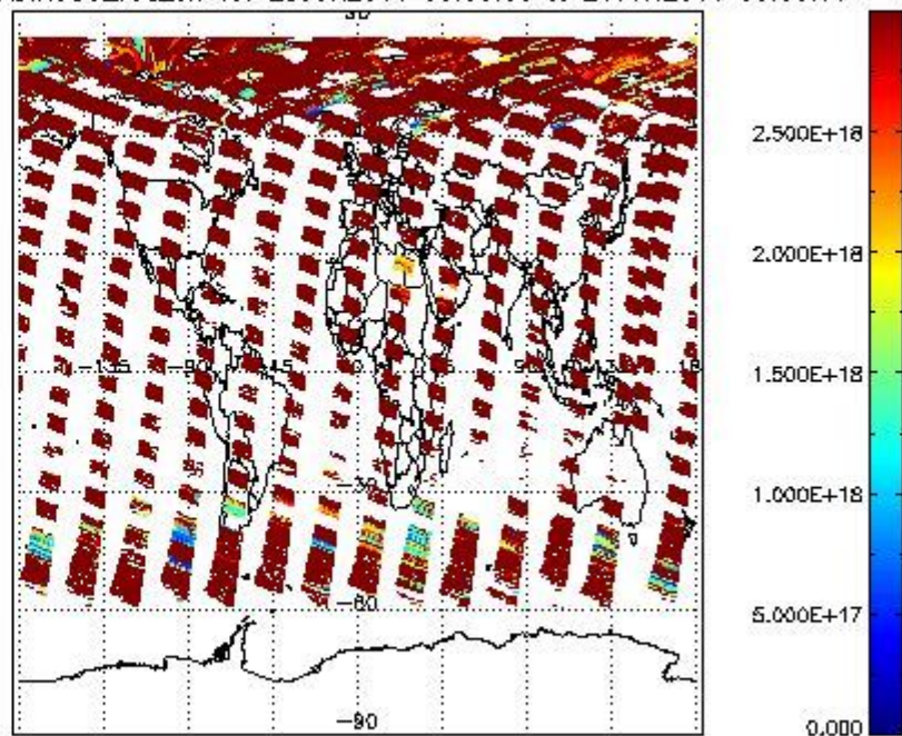
SCIDL2P_NADIR3CO_vcd_err for 25JUN2011 00:00:00 to 26JUN2011 00:00:00
