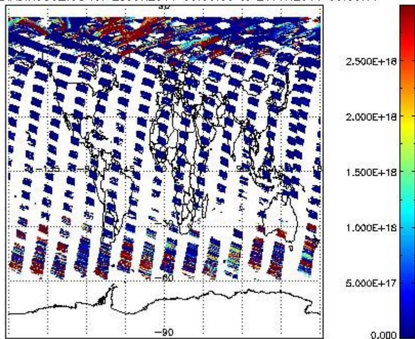
SCIDL2P_NADIR3CO_vcd for 25JUN2011 00:00:00 to 26JUN2011 00:00:00
