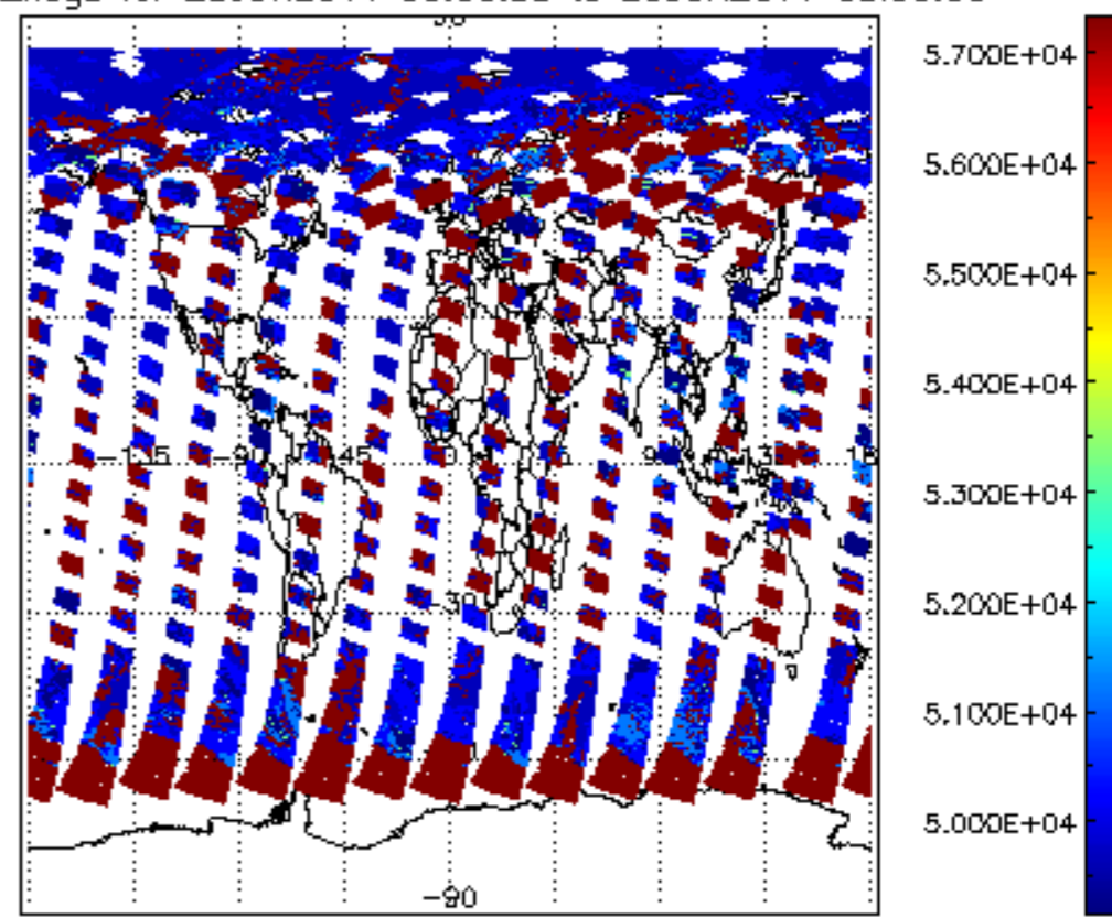
cloud_flags for 25JUN2011 00:00:00 to 26JUN2011 00:00:00
