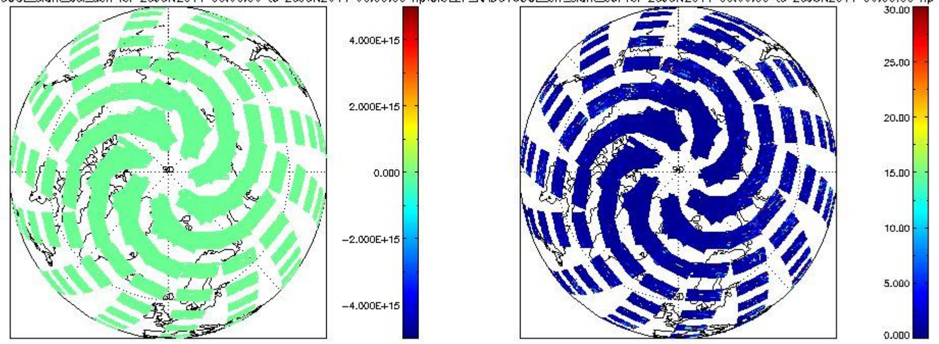
CIOL2P_NADUV60CL_slant_col_den for 25JUN2011 00:00:00 to 26JUN2011 00:00:00 np; CIOL2P_NADUV60CL_err_slant_col for 25JUN2011 00:00:00 to 26JUN2011 00:00:00 np
