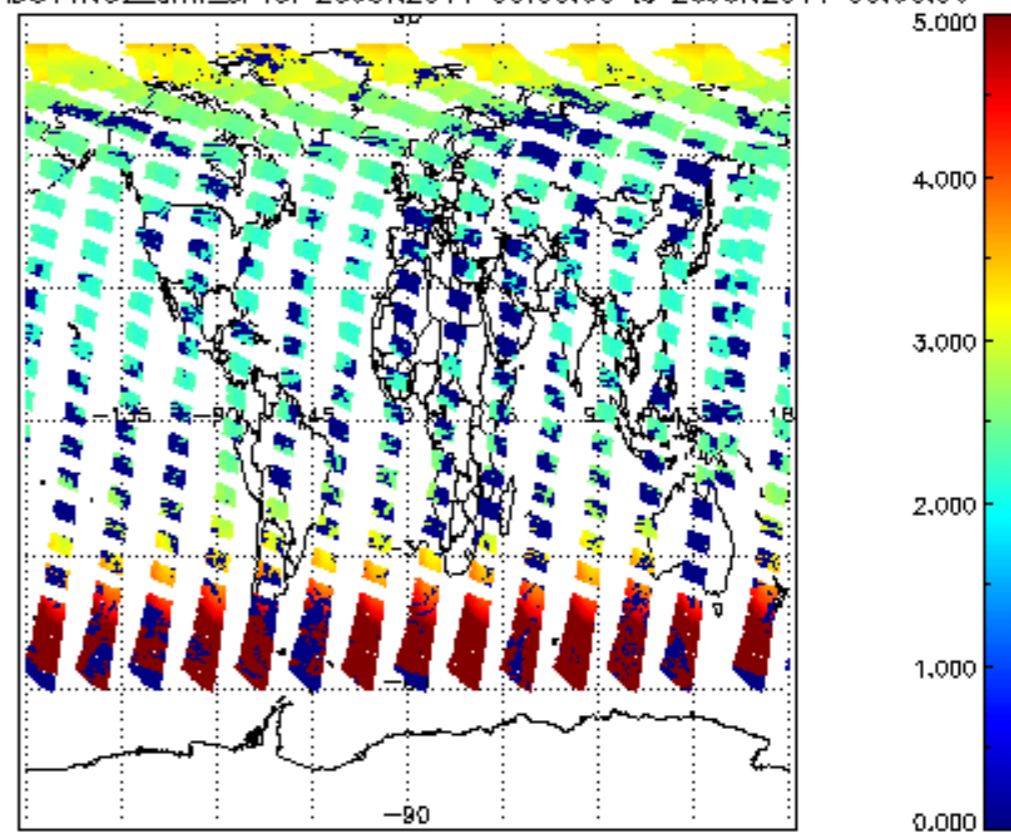
SCIOL2P_NADUV1NO2_amf_cl for 25JUN2011 00:00:00 to 26JUN2011 00:00:00
