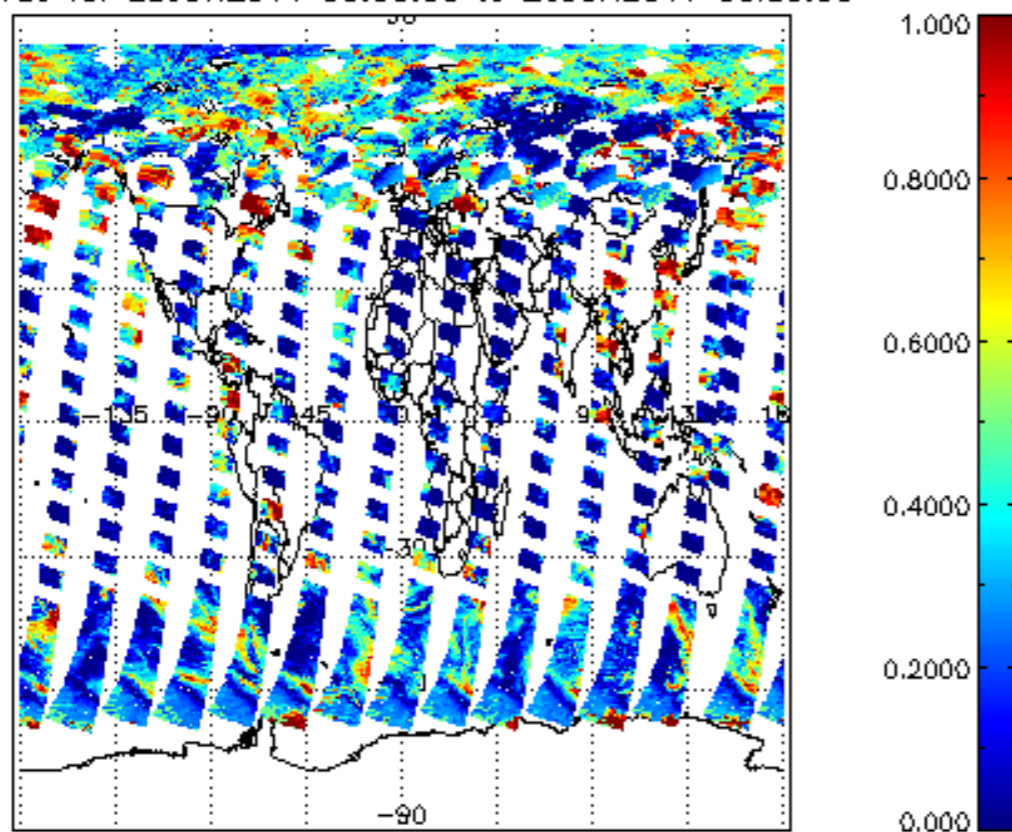
cl_frac for 25JUN2011 00:00:00 to 26JUN2011 00:00:00
