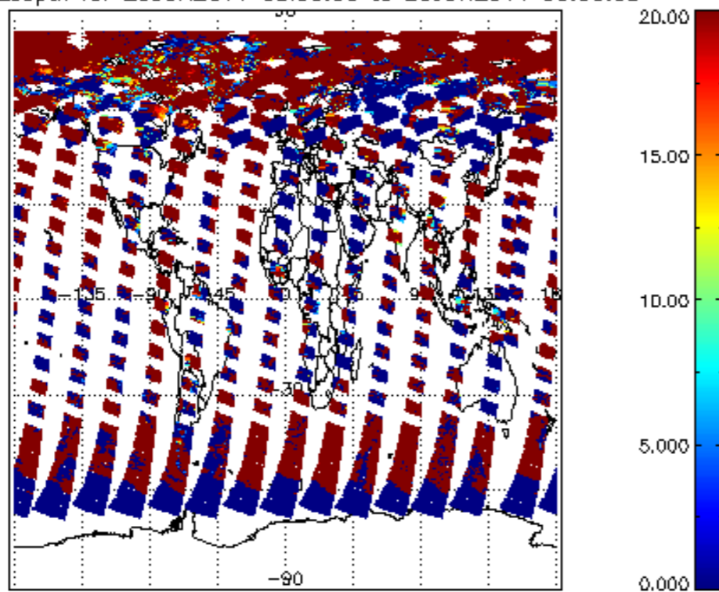
cl_opt_depth for 25JUN2011 00:00:00 to 26JUN2011 00:00:00
