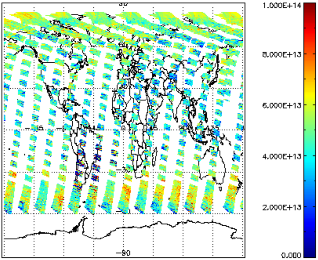
SCIOL2P_NADUV3BRO_vcd for 22JUN2011 00:00:00 to 23JUN2011 00:00:00
