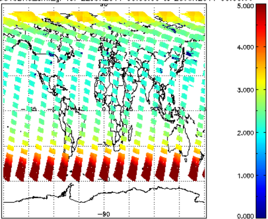
SCIOL2P_NADUV3BRO_amf_gr for 22JUN2011 00:00:00 to 23JUN2011 00:00:00
