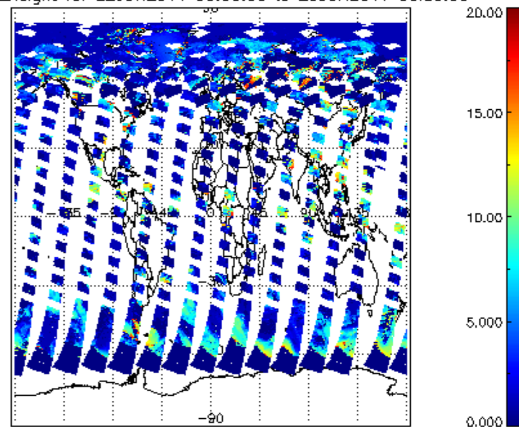
cl_top_height for 22JUN2011 00:00:00 to 23JUN2011 00:00:00
