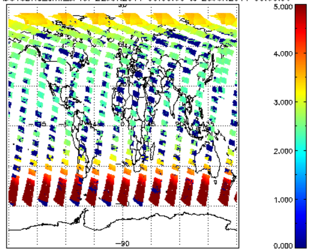
SCIOL2P_NADUV3BRO_amf_sl for 22JUN2011 00:00:00 to 23JUN2011 00:00:00
