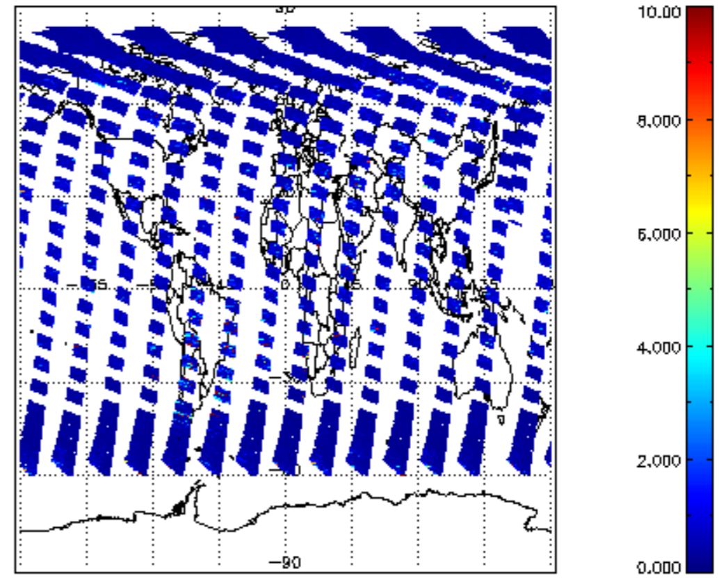
SCIOL2P_NADUV3BRO_vcd_err for 22JUN2011 00:00:00 to 23JUN2011 00:00:00
