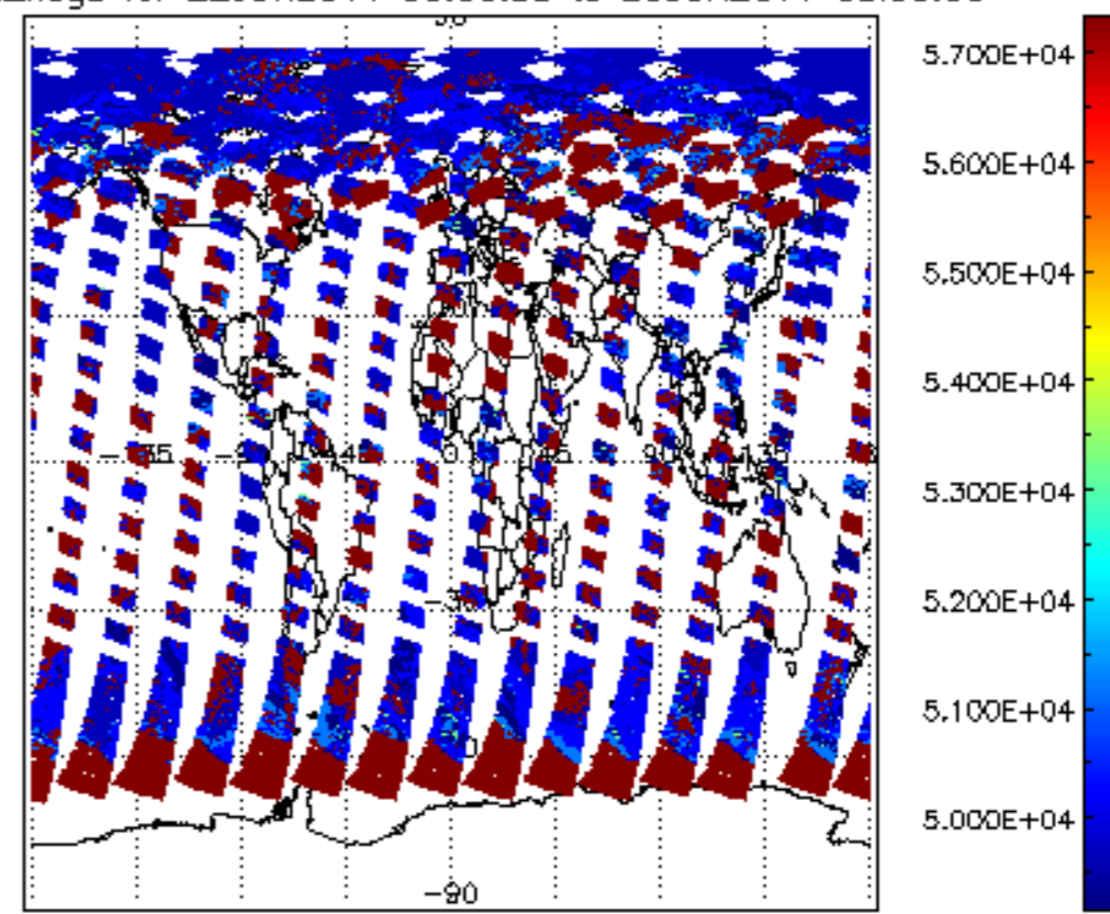
cloud_flags for 22JUN2011 00:00:00 to 23JUN2011 00:00:00
