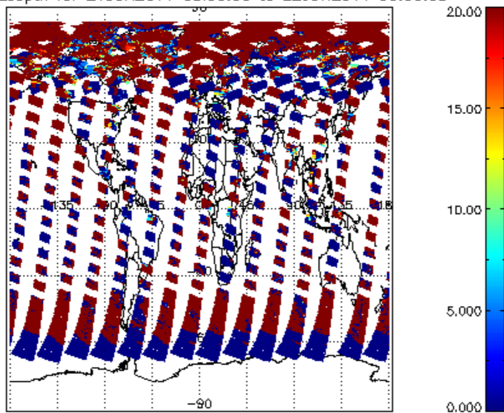
cl_opt_depth for 21JUN2011 00:00:00 to 22JUN2011 00:00:00
