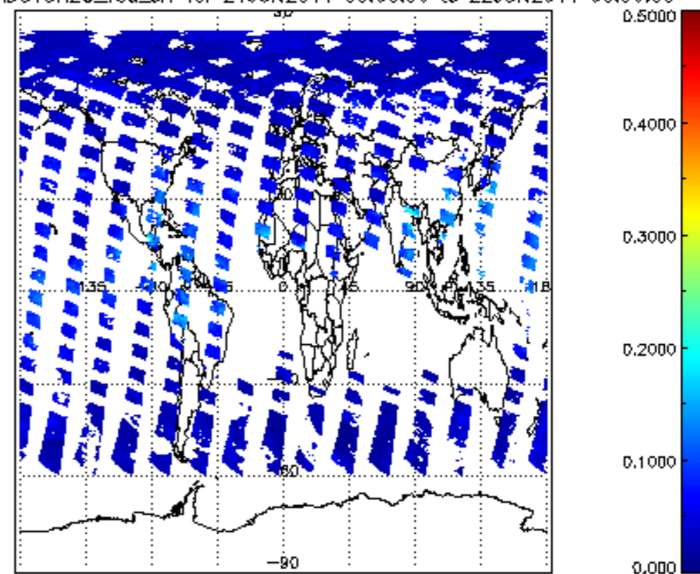
SCIOL2P_NADUV8H2O_vcd_err for 21JUN2011 00:00:00 to 22JUN2011 00:00:00
