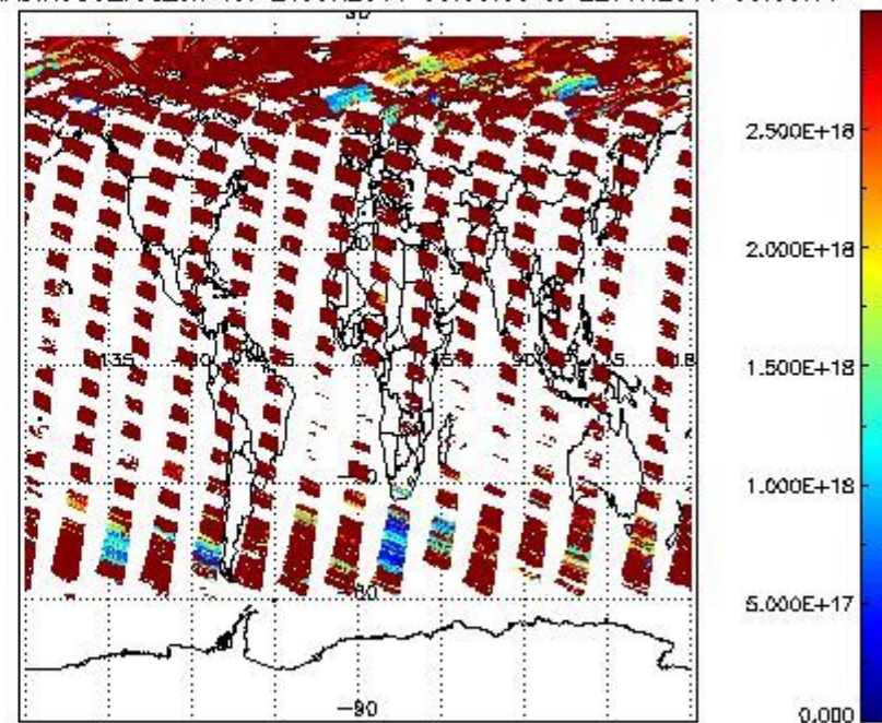
SCIO2P_NADIR3CO_vcd_err for 21JUN2011 00:00:00 to 22JUN2011 00:00:00
