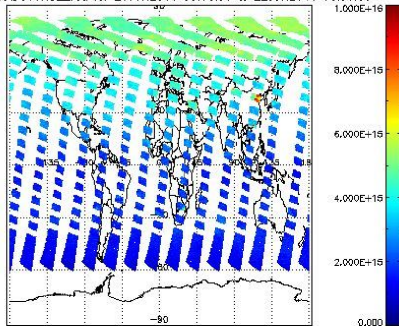
SCIOL2P_NADUV1NO2_vcd for 21JUN2011 00:00:00 to 22JUN2011 00:00:00
