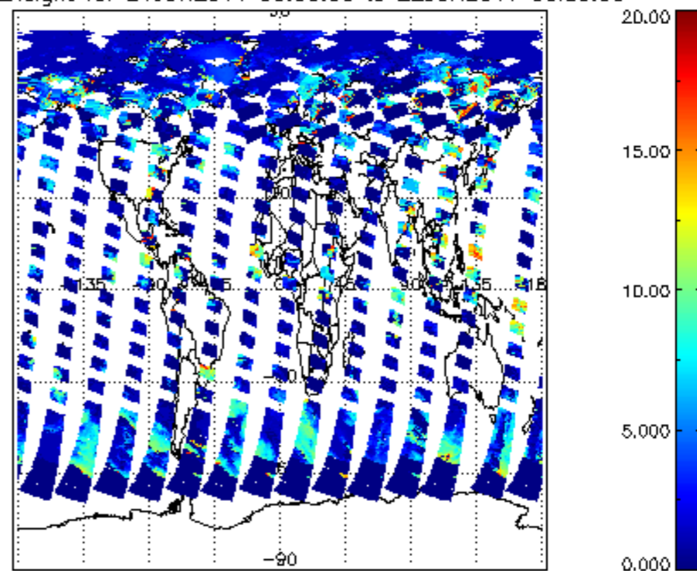
cl_top_height for 21JUN2011 00:00:00 to 22JUN2011 00:00:00
