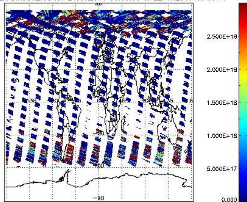
SCIO2P_NADIR3CO_vcd for 21JUN2011 00:00:00 to 22JUN2011 00:00:00
