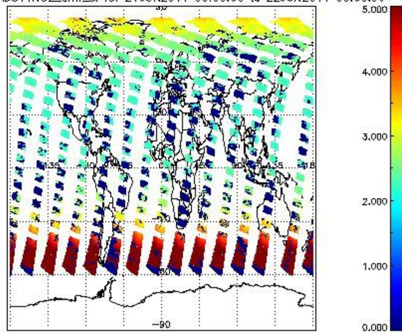
SCIOL2P_NADUV1NO2_amf_cl for 21JUN2011 00:00:00 to 22JUN2011 00:00:00
