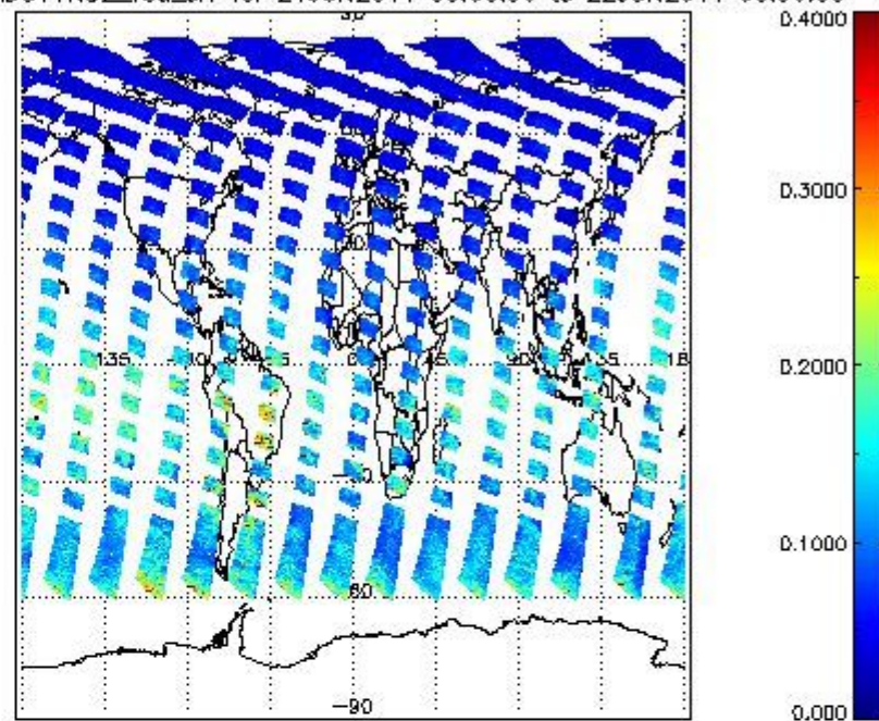
SCIOL2P_NADUV1NO2_vcd_err for 21JUN2011 00:00:00 to 22JUN2011 00:00:00
