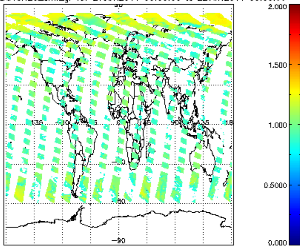
SCIOL2P_NADUV8H2O_amf_gr for 21JUN2011 00:00:00 to 22JUN2011 00:00:00
