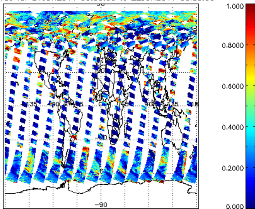
cl_frac for 21JUN2011 00:00:00 to 22JUN2011 00:00:00
