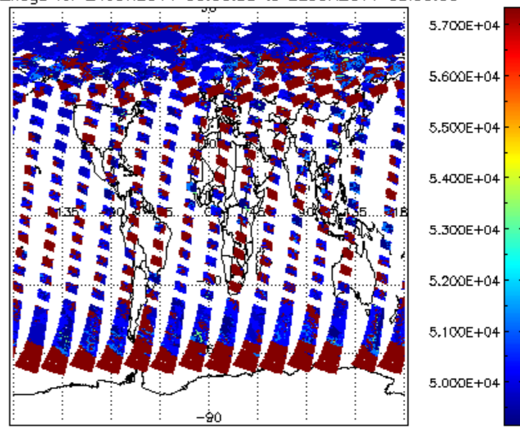
cloud_flags for 21JUN2011 00:00:00 to 22JUN2011 00:00:00
