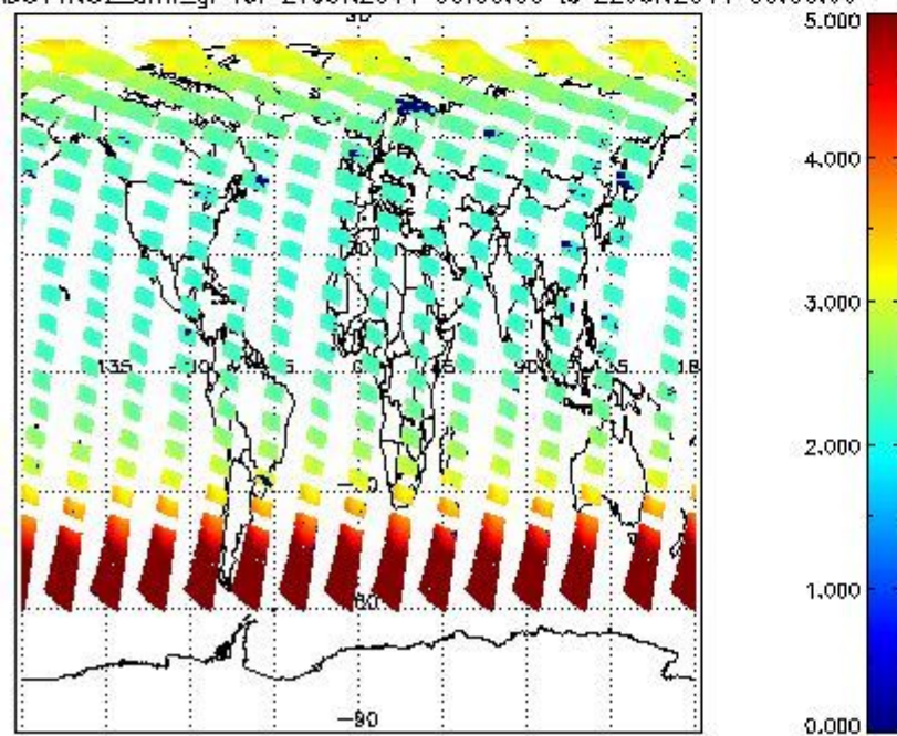
SCIOL2P_NADUV1NO2_amf_gr for 21JUN2011 00:00:00 to 22JUN2011 00:00:00
