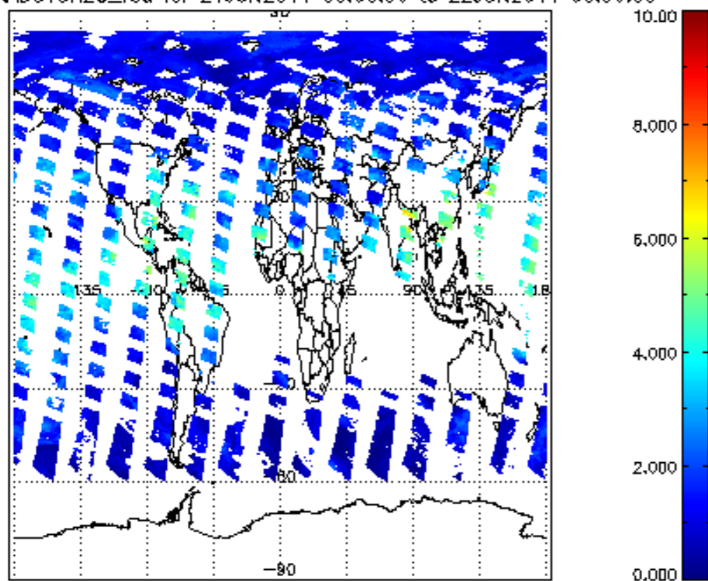
SCIOL2P_NADUV8H2O_vcd for 21JUN2011 00:00:00 to 22JUN2011 00:00:00
