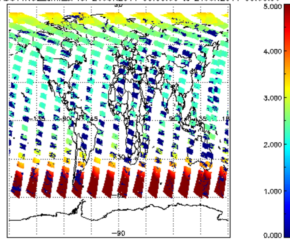
SCIOL2P_NADUV1NO2_amf_cl for 20JUN2011 00:00:00 to 21JUN2011 00:00:00
