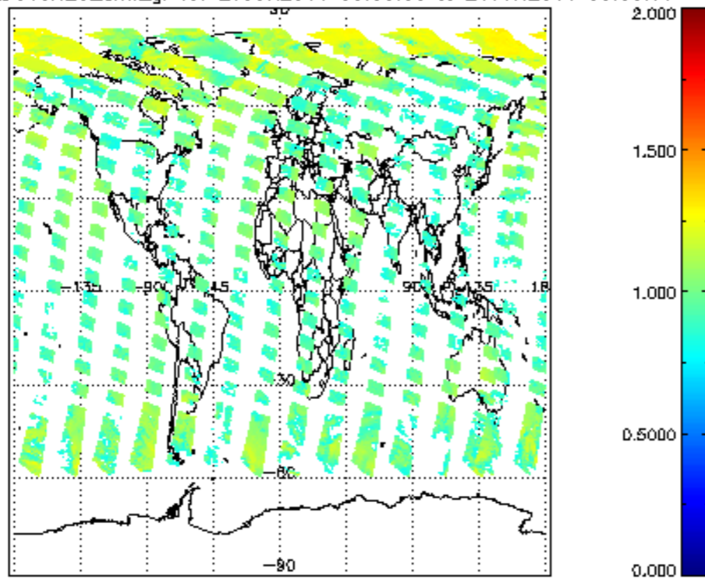
SCIOL2P_NADUV8H20_amf_gr for 20JUN2011 00:00:00 to 21JUN2011 00:00:00
