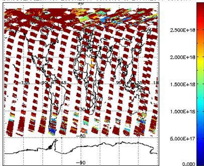
SCIDL2P_NADIR3CO_vcd_err for 20JUN2011 00:00:00 to 21JUN2011 00:00:00
