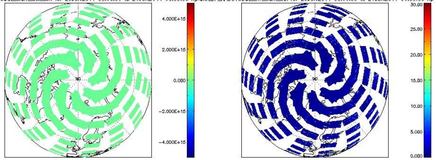
CIOL2P_NADUV60CL_slant_col_den for 20JUN2011 00:00:00 to 21JUN2011 00:00:00 np; CIOL2P_NADUV60CL_err_slant_col for 20JUN2011 00:00:00 to 21JUN2011 00:00:00 np
