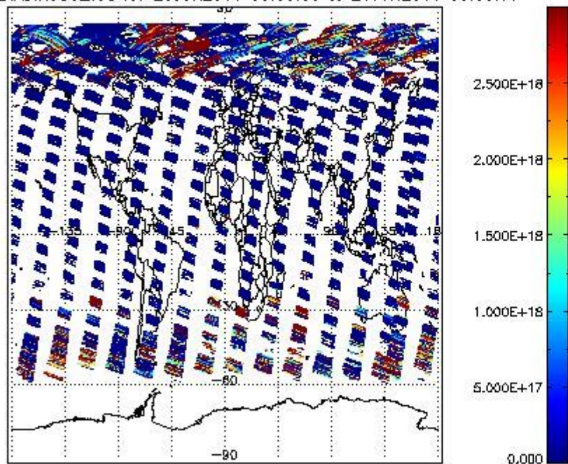
SCIDL2P_NADIR3CO_vcd for 20JUN2011 00:00:00 to 21JUN2011 00:00:00
