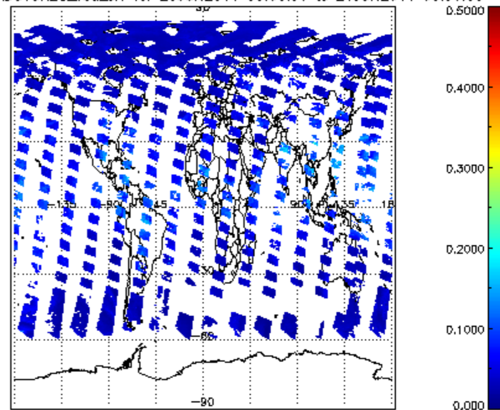
SCIOL2P_NADUV8H20_vcd_err for 20JUN2011 00:00:00 to 21JUN2011 00:00:00
