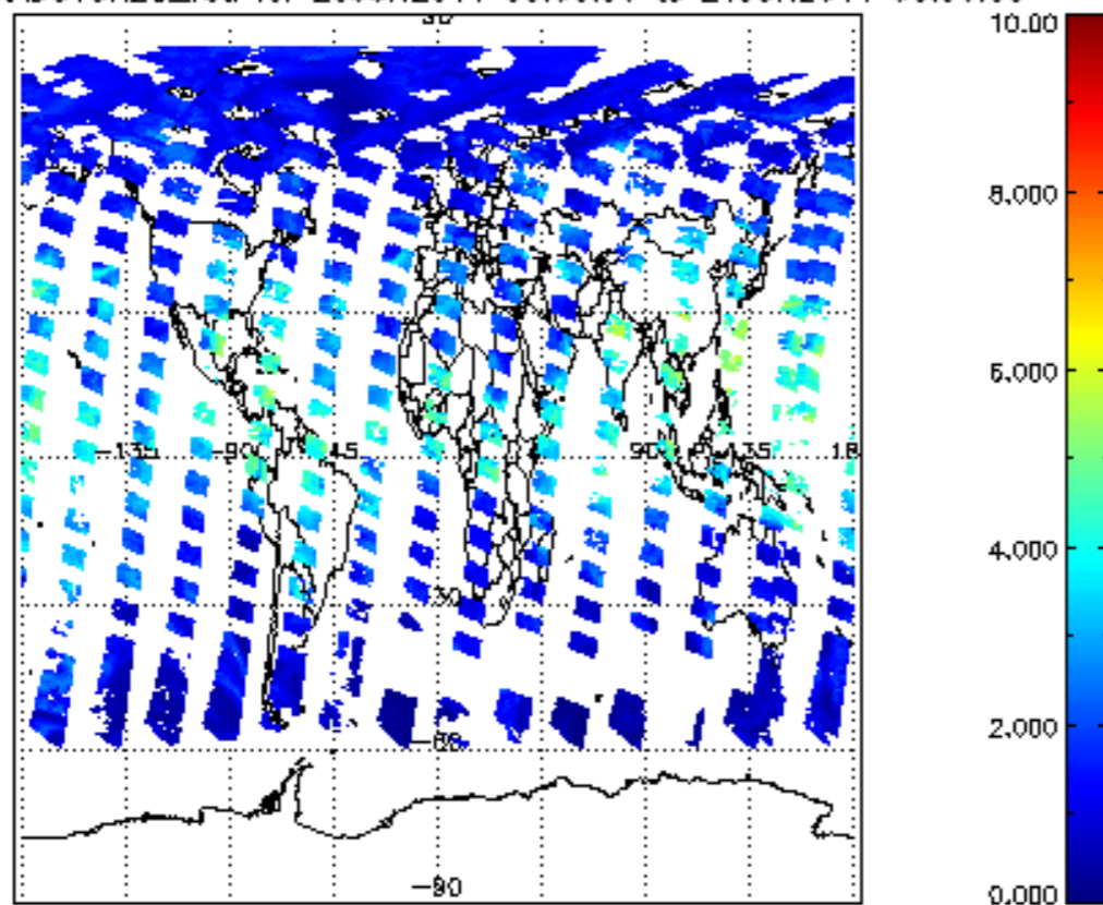
SCIOL2P_NADUV8H20_vcd for 20JUN2011 00:00:00 to 21JUN2011 00:00:00
