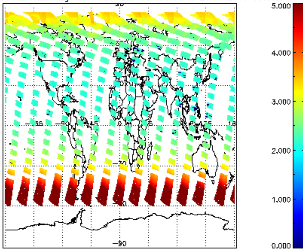
SCIOL2P_NADUV3BRO_amf_gr for 19JUN2011 00:00:00 to 20JUN2011 00:00:00
