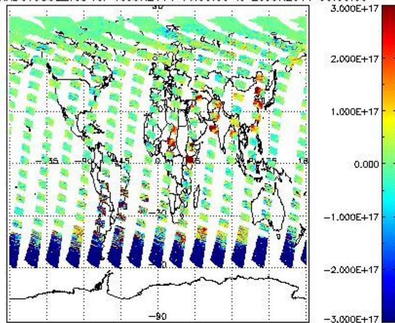
SCIOL2P_NADUV5S02_vcd for 19JUN2011 00:00:00 to 20JUN2011 00:00:00
