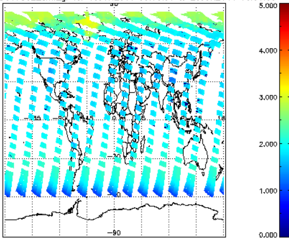
SCIOL2P_NADUV7S02_amf_gr for 19JUN2011 00:00:00 to 20JUN2011 00:00:00
