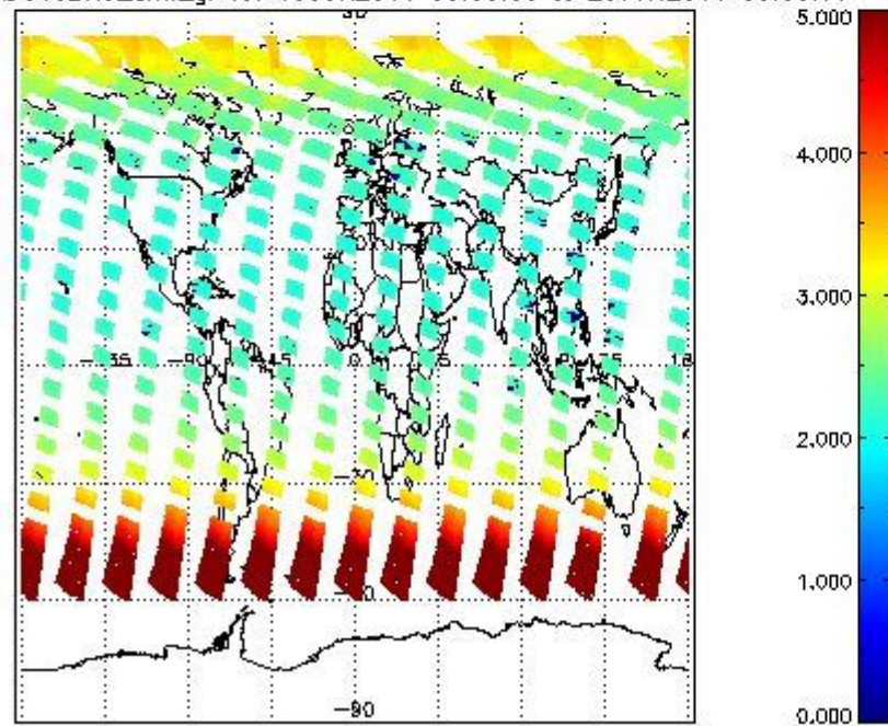
SCIOL2P_NADUV3BRO_amf_gr for 19JUN2011 00:00:00 to 20JUN2011 00:00:00
