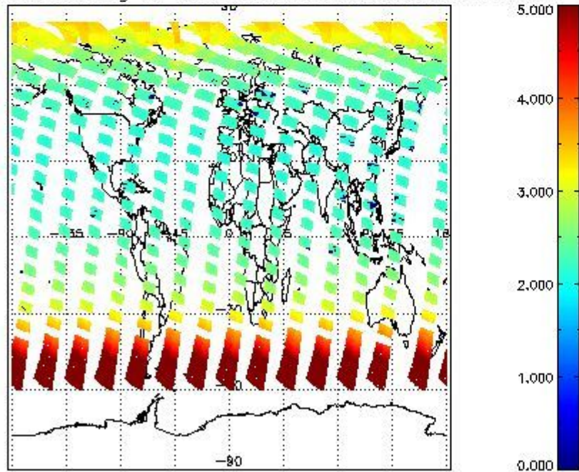
SCIOL2P_NADUV003_amf_gr for 19JUN2011 00:00:00 to 20JUN2011 00:00:00
