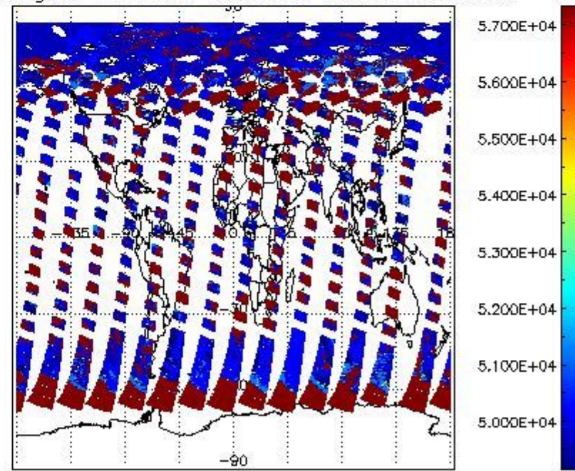
cloud_flags for 19JUN2011 00:00:00 to 20JUN2011 00:00:00
