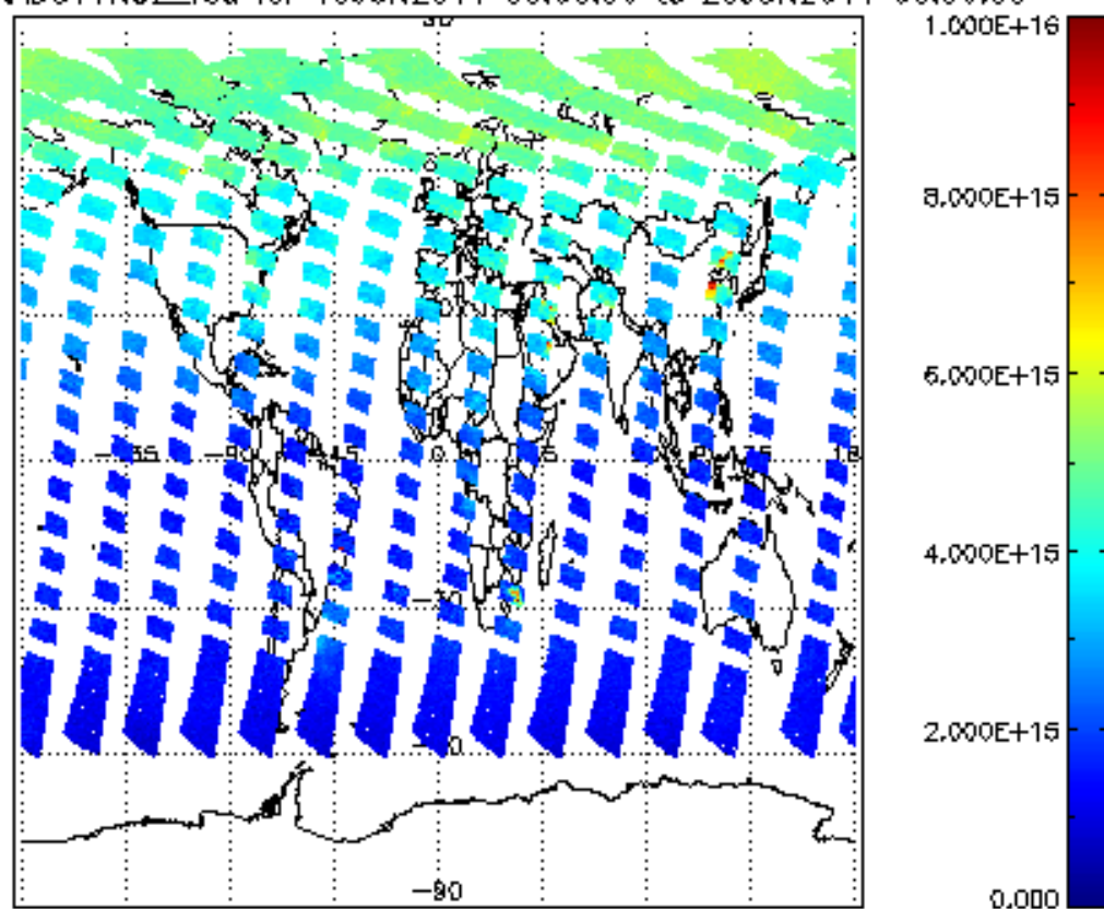
SCIOL2P_NADUV1NO2_vcd for 19JUN2011 00:00:00 to 20JUN2011 00:00:00
