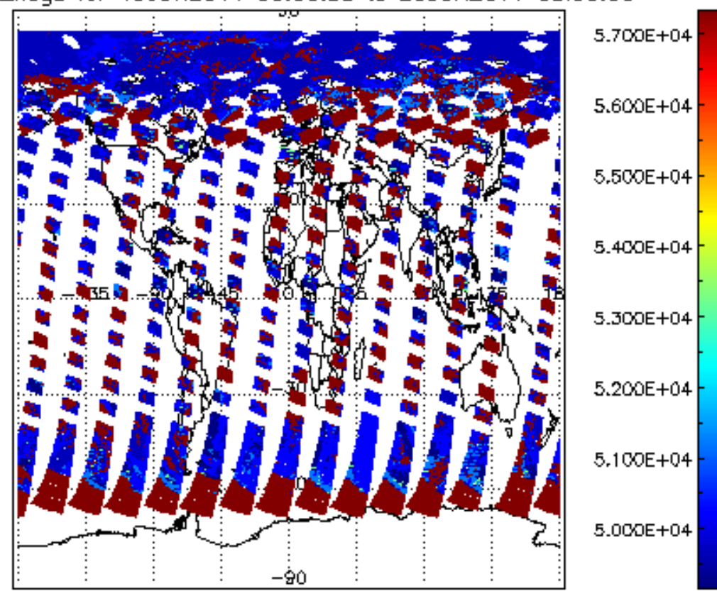
cloud_flags for 19JUN2011 00:00:00 to 20JUN2011 00:00:00
