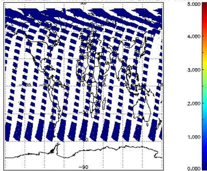
SCIOL2P_NADUV7S02_amf_cl for 19JUN2011 00:00:00 to 20JUN2011 00:00:00
