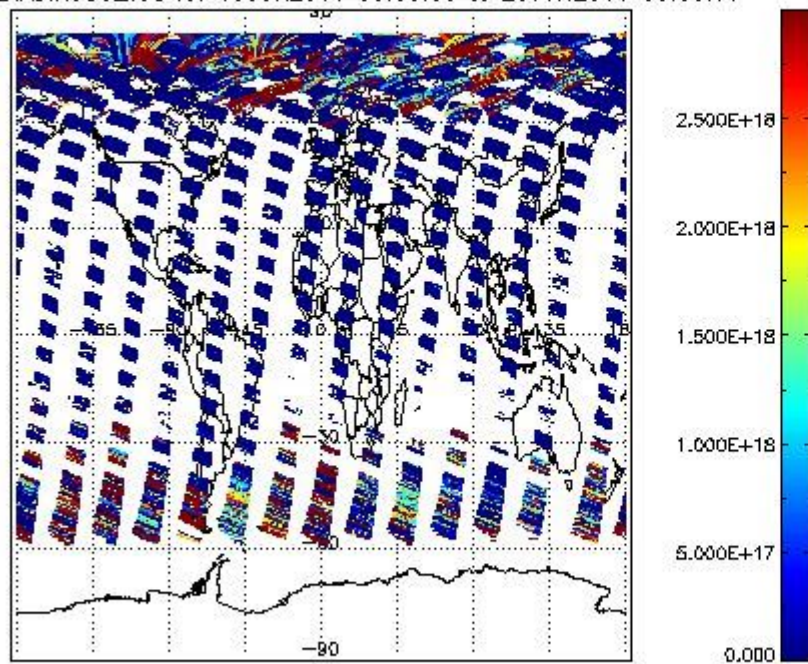
SCIDL2P_NADIR3CO_vcd for 19JUN2011 00:00:00 to 20JUN2011 00:00:00
