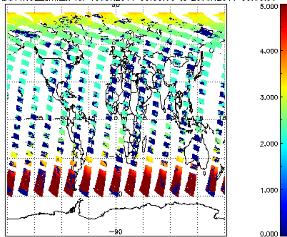
SCIOL2P_NADUV1NO2_amf_sl for 19JUN2011 00:00:00 to 20JUN2011 00:00:00
