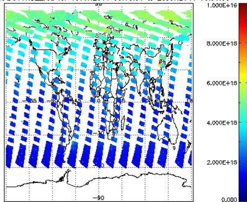
SCIOL2P_NADUV1NO2_vcd for 19JUN2011 00:00:00 to 20JUN2011 00:00:00
