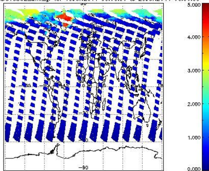
SCIOL2P_NADUV5S02_amf_gr for 19JUN2011 00:00:00 to 20JUN2011 00:00:00
