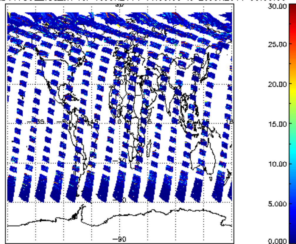
SCIOL2P_NADUV7S02_vcd_err for 19JUN2011 00:00:00 to 20JUN2011 00:00:00
