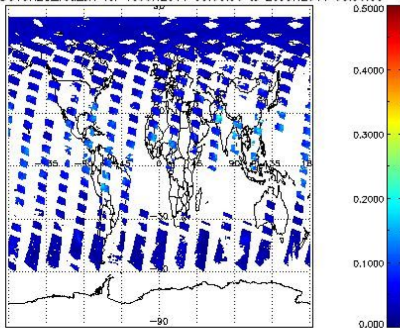
SCIOL2P_NADUV8H2O_vcd_err for 19JUN2011 00:00:00 to 20JUN2011 00:00:00
