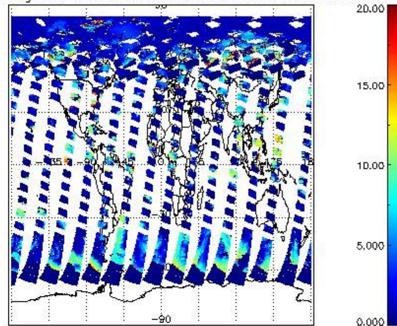
cL_top_height for 19JUN2011 00:00:00 to 20JUN2011 00:00:00
