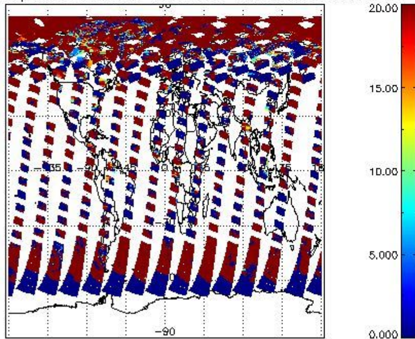
cL_opt_depth for 19JUN2011 00:00:00 to 20JUN2011 00:00:00
