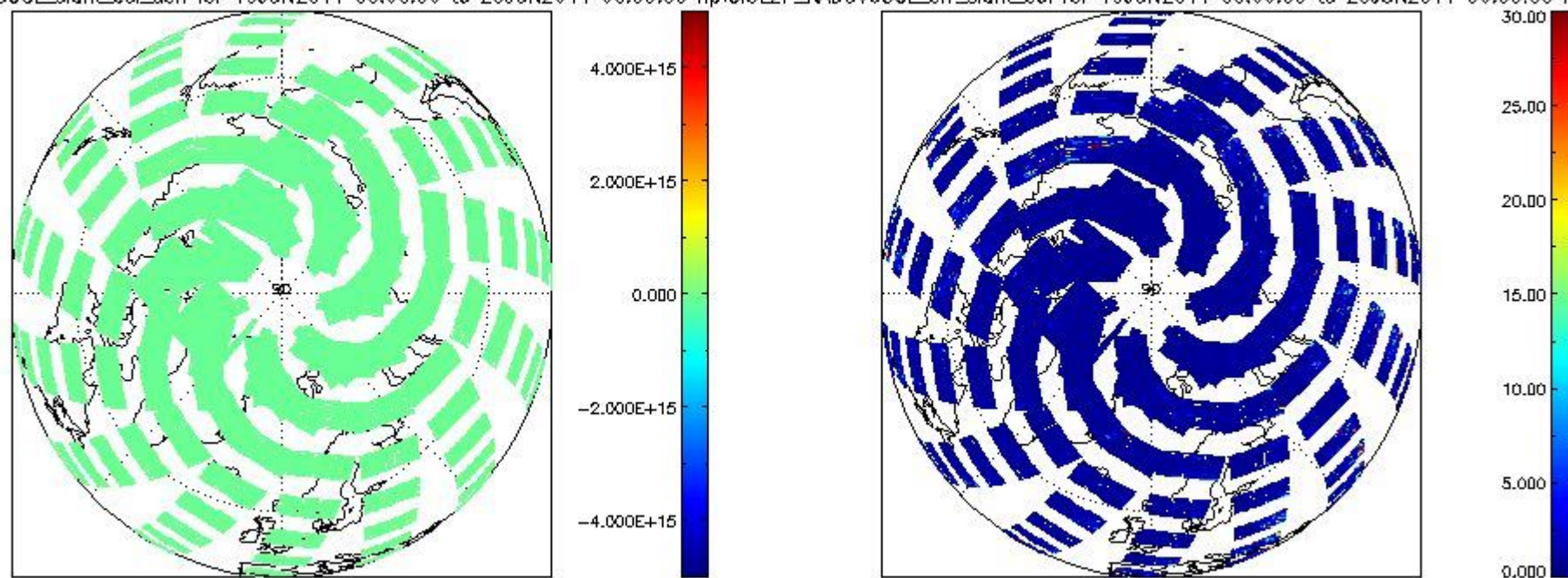
CIOL2P_NADUV60CLslant_col_den for 19JUN2011 00:00:00 to 20JUN2011 00:00:00 np; CIOL2P_NADUV60CLarr_slant_col for 19JUN2011 00:00:00 to 20JUN2011 00:00:00 np
