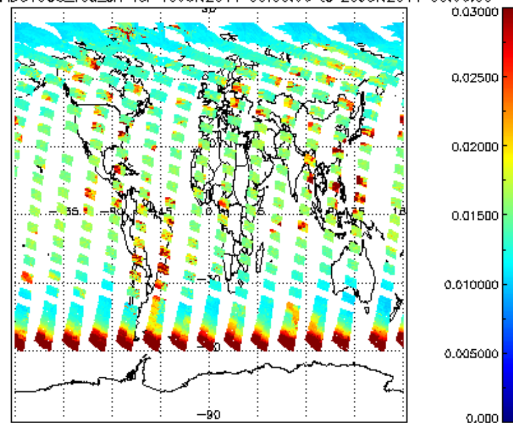
SCIOL2P_NADUV003_vcd_err for 19JUN2011 00:00:00 to 20JUN2011 00:00:00
