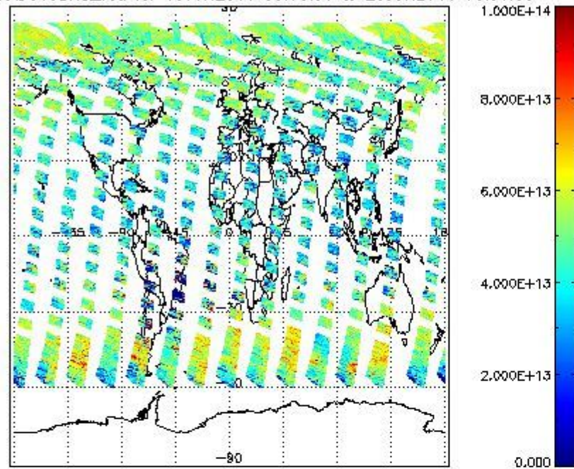
SCIOL2P_NADUV3BRO_vcd for 19JUN2011 00:00:00 to 20JUN2011 00:00:00
