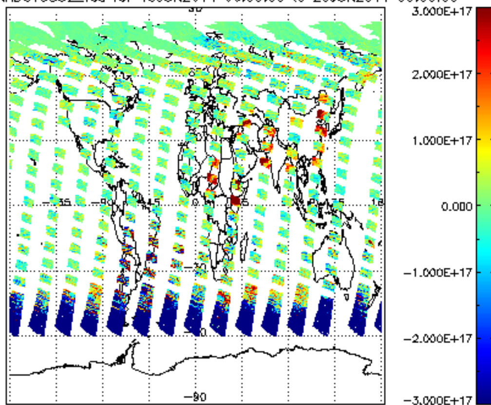
SCIOL2P_NADUV5S02_vcd for 19JUN2011 00:00:00 to 20JUN2011 00:00:00
