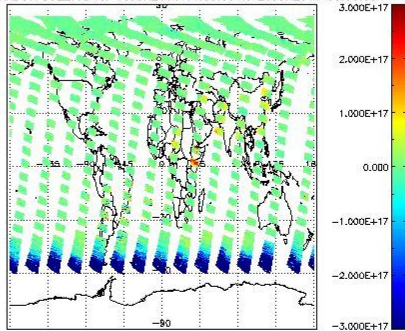
SCIOL2P_NADUV7S02_vcd for 19JUN2011 00:00:00 to 20JUN2011 00:00:00
