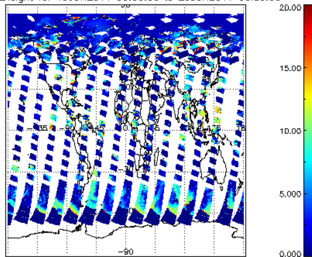
cl_top_height for 19JUN2011 00:00:00 to 20JUN2011 00:00:00
