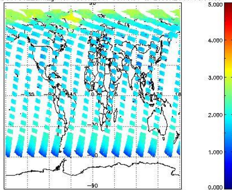
SCIOL2P_NADUV7S02_amf_gr for 19JUN2011 00:00:00 to 20JUN2011 00:00:00
