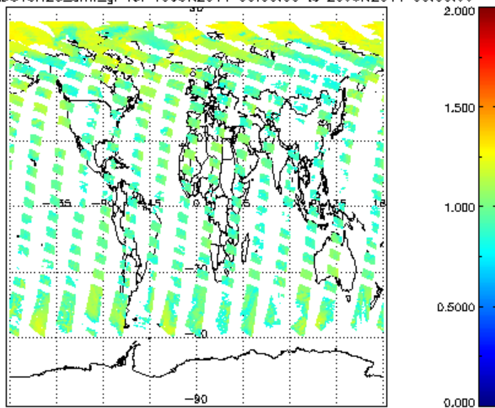
SCIOL2P_NADUV8H2O_amf_gr for 19JUN2011 00:00:00 to 20JUN2011 00:00:00
