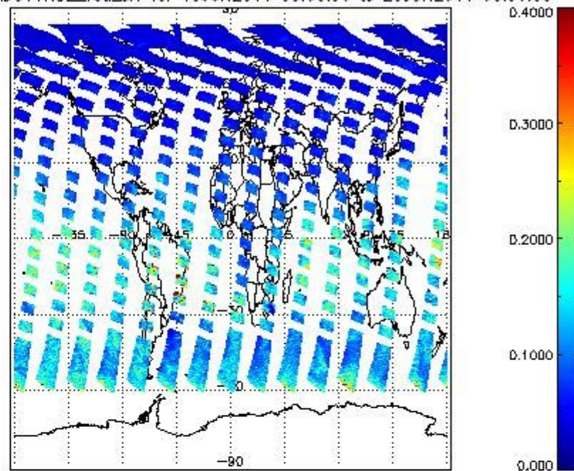
SCIOL2P_NADUV1NO2_vcd_err for 19JUN2011 00:00:00 to 20JUN2011 00:00:00
