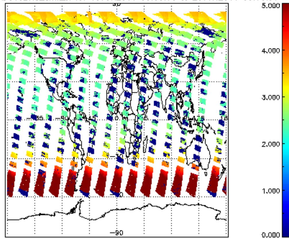
SCIOL2P_NADUV3BRO_amf_cl for 19JUN2011 00:00:00 to 20JUN2011 00:00:00
