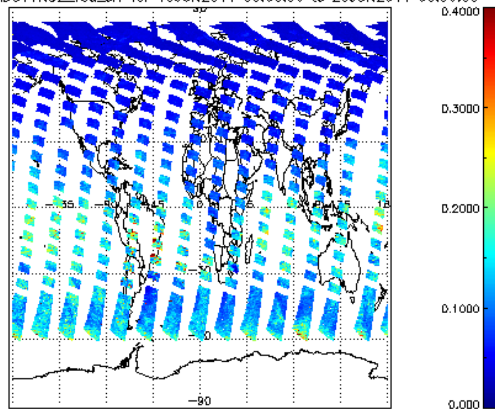
SCIOL2P_NADUV1NO2_vcd_err for 19JUN2011 00:00:00 to 20JUN2011 00:00:00
