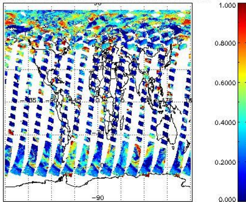
cL_frac for 19JUN2011 00:00:00 to 20JUN2011 00:00:00
