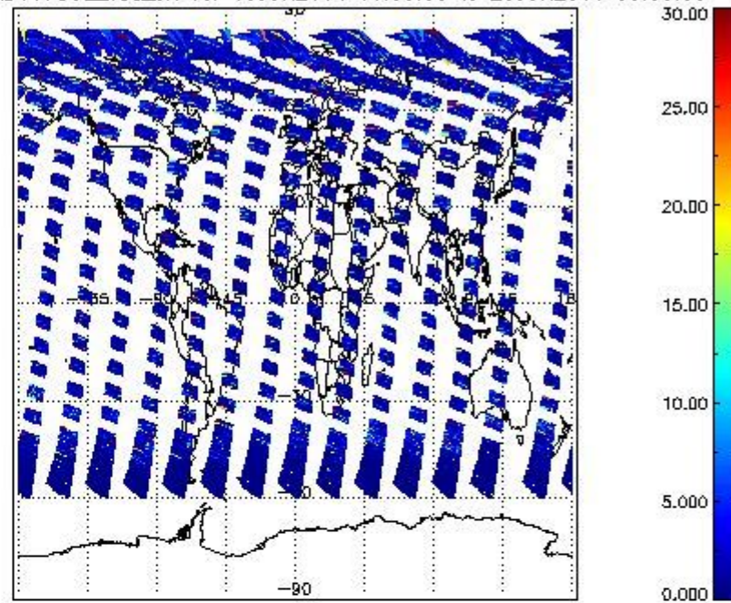
SCIOL2P_NADUV7S02_vcd_err for 19JUN2011 00:00:00 to 20JUN2011 00:00:00
