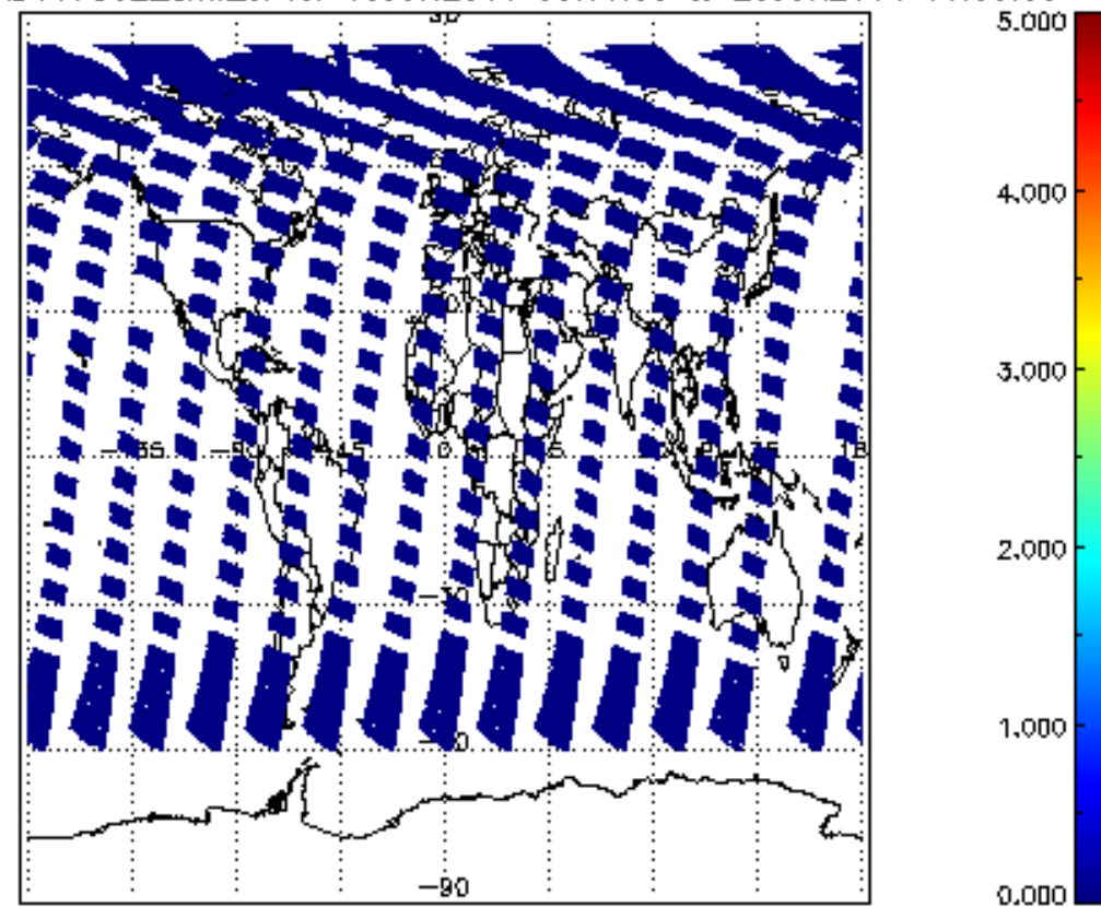
SCIOL2P_NADUV7S02_amf_cl for 19JUN2011 00:00:00 to 20JUN2011 00:00:00
