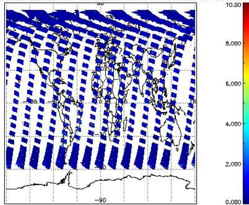
SCIOL2P_NADUV3BRO_vcd_err for 19JUN2011 00:00:00 to 20JUN2011 00:00:00
