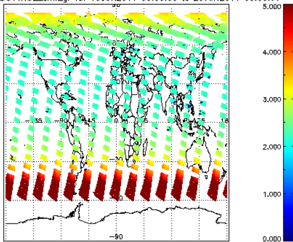
SCIOL2P_NADUV1NO2_amf_gr for 19JUN2011 00:00:00 to 20JUN2011 00:00:00
