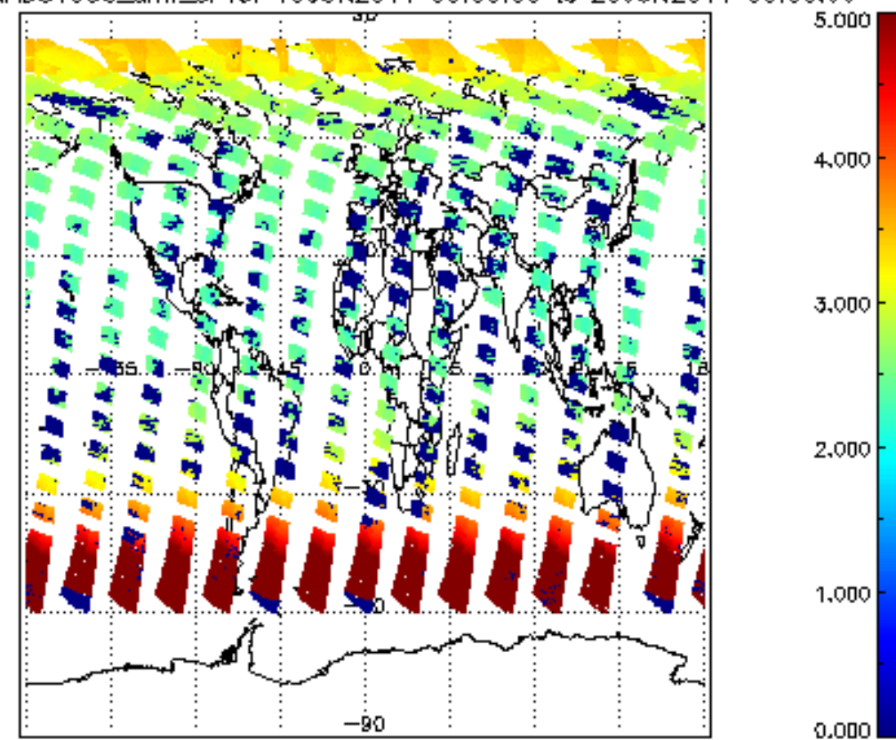
SCIOL2P_NADUV003_amf_cl for 19JUN2011 00:00:00 to 20JUN2011 00:00:00
