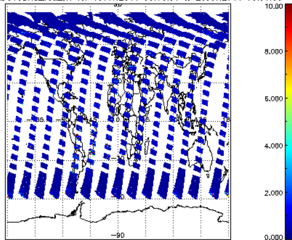
SCIOL2P_NADUV3BRO_vcd_err for 19JUN2011 00:00:00 to 20JUN2011 00:00:00
