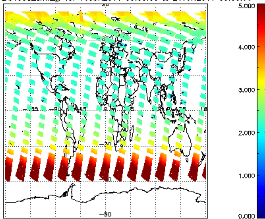
SCIOL2P_NADUV003_amf_gr for 19JUN2011 00:00:00 to 20JUN2011 00:00:00
