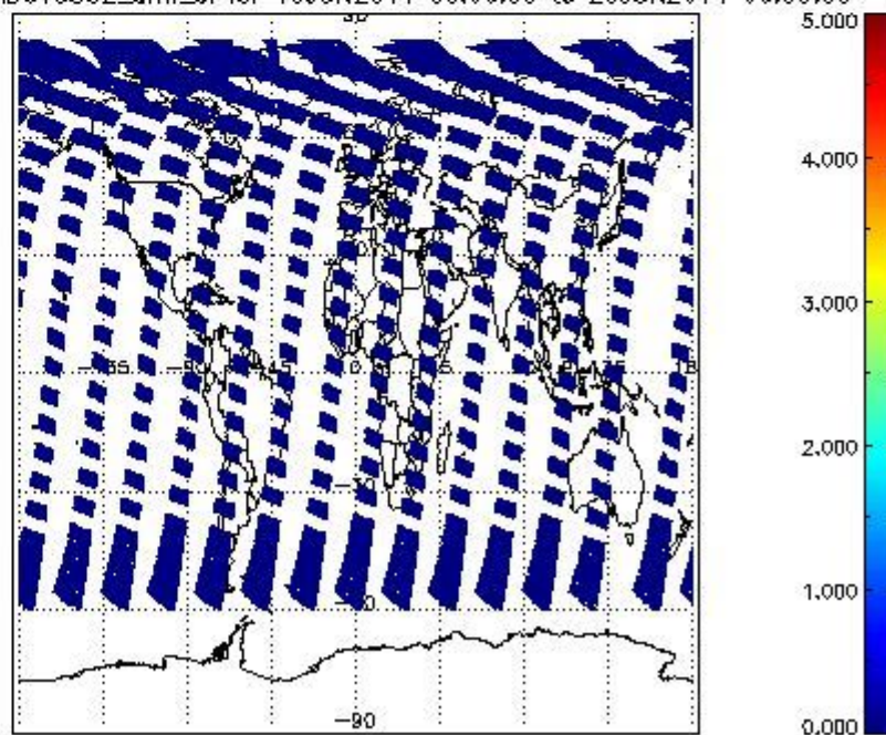
SCIOL2P_NADUV5S02_amf_cl for 19JUN2011 00:00:00 to 20JUN2011 00:00:00
