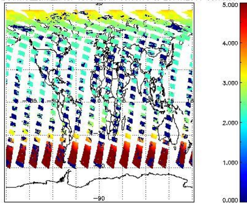
SCIOL2P_NADUV1NO2_amf_cl for 19JUN2011 00:00:00 to 20JUN2011 00:00:00
