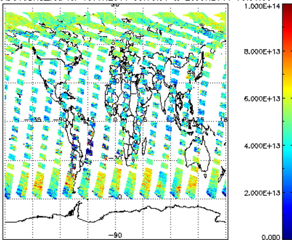
SCIOL2P_NADUV3BRO_vcd for 19JUN2011 00:00:00 to 20JUN2011 00:00:00
