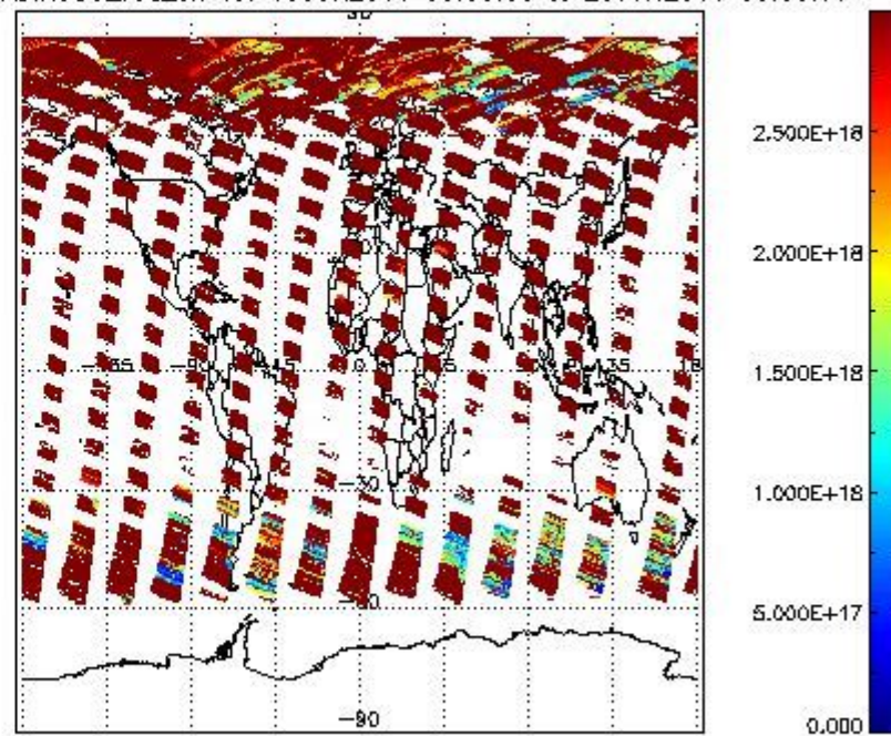
SCIDL2P_NADIR3CO_vcd_err for 19JUN2011 00:00:00 to 20JUN2011 00:00:00
