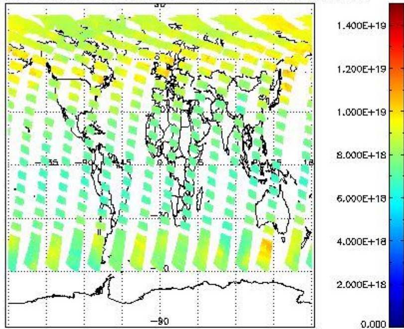
SCIOL2P_NADUV003_vcd for 19JUN2011 00:00:00 to 20JUN2011 00:00:00
