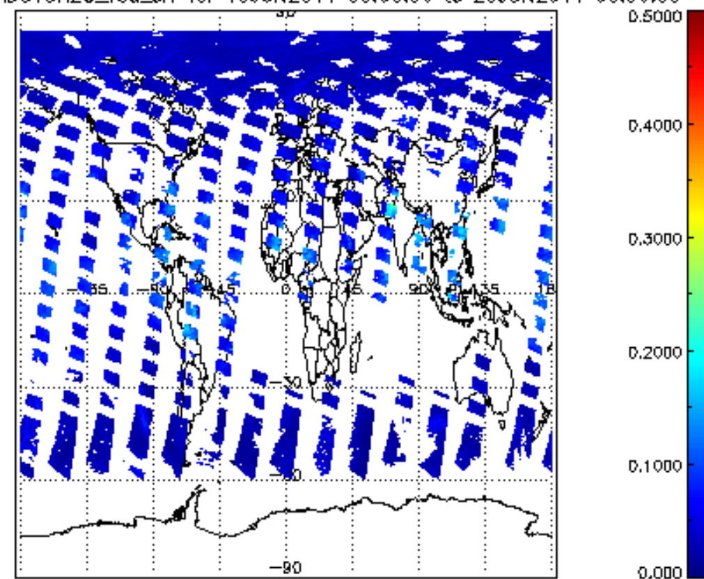
SCIOL2P_NADUV8H2O_vcd_err for 19JUN2011 00:00:00 to 20JUN2011 00:00:00
