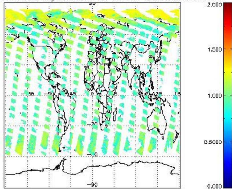
SCIOL2P_NADUV8H2O_arnf_gr for 19JUN2011 00:00:00 to 20JUN2011 00:00:00
