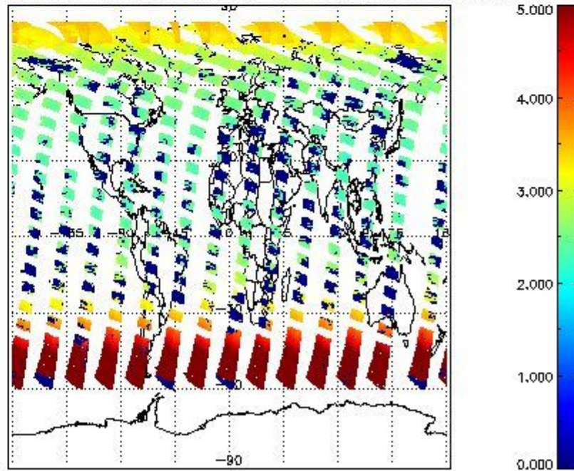
SCIOL2P_NADUV003_amf_cl for 19JUN2011 00:00:00 to 20JUN2011 00:00:00
