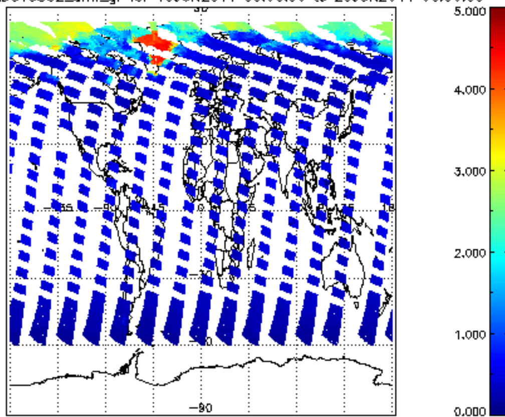
SCIOL2P_NADUV5S02_amf_gr for 19JUN2011 00:00:00 to 20JUN2011 00:00:00
