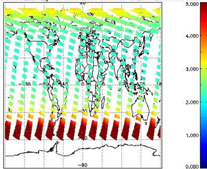
SCIOL2P_NADUV1NO2_amf_gr for 19JUN2011 00:00:00 to 20JUN2011 00:00:00
