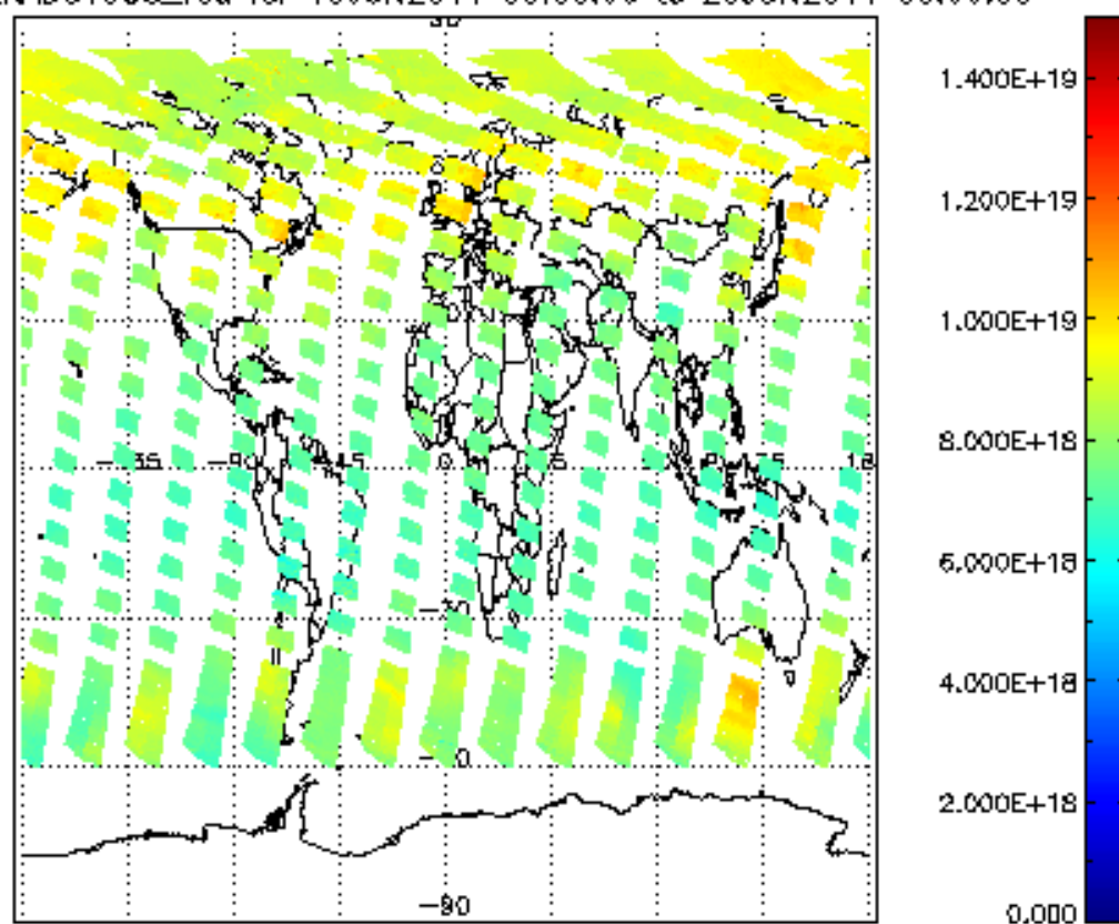
SCIOL2P_NADUV003_vcd for 19JUN2011 00:00:00 to 20JUN2011 00:00:00
