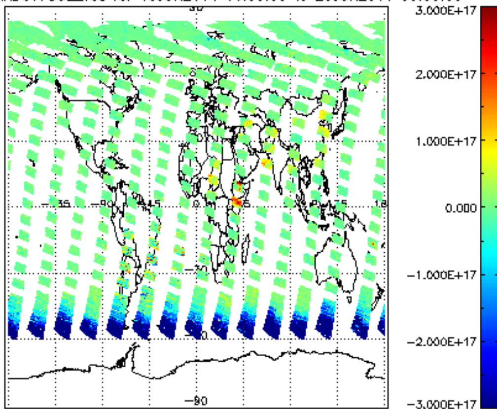
SCIOL2P_NADUV7S02_vcd for 19JUN2011 00:00:00 to 20JUN2011 00:00:00
