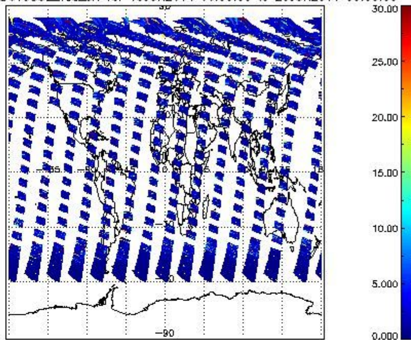
SCIOL2P_NADUV5S02_vcd_err for 19JUN2011 00:00:00 to 20JUN2011 00:00:00
