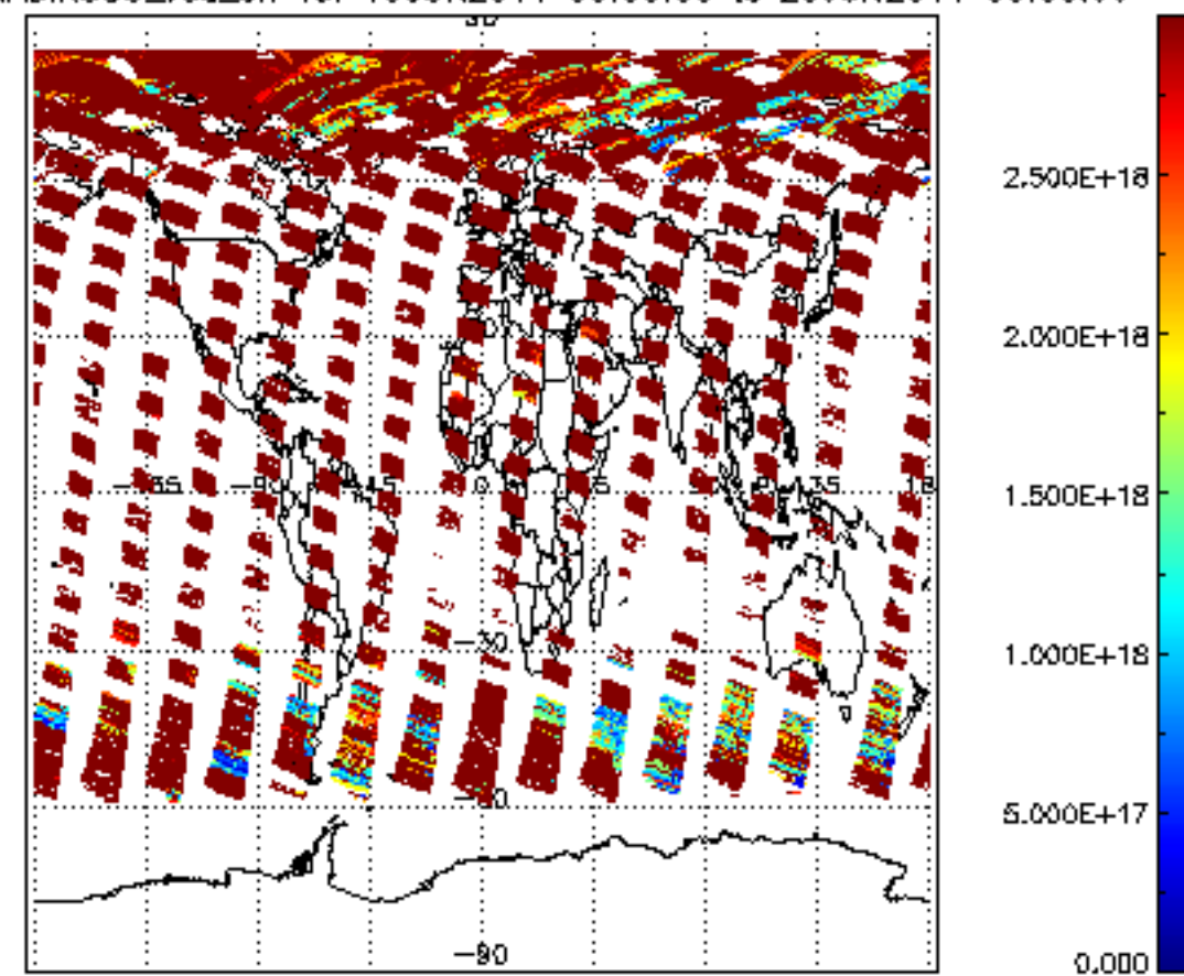
SCIOL2P_NADIR3CO_vcd_err for 19JUN2011 00:00:00 to 20JUN2011 00:00:00
