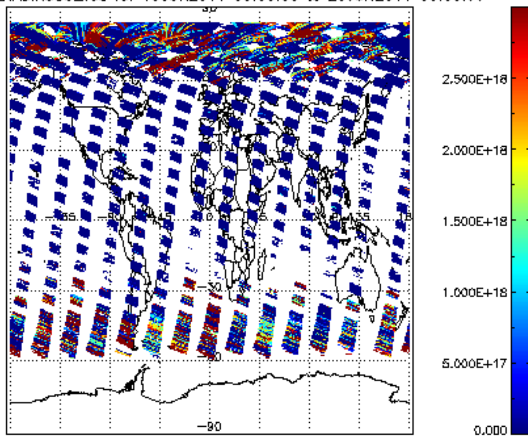
SCIOL2P_NADIR3CO_vcd for 19JUN2011 00:00:00 to 20JUN2011 00:00:00
