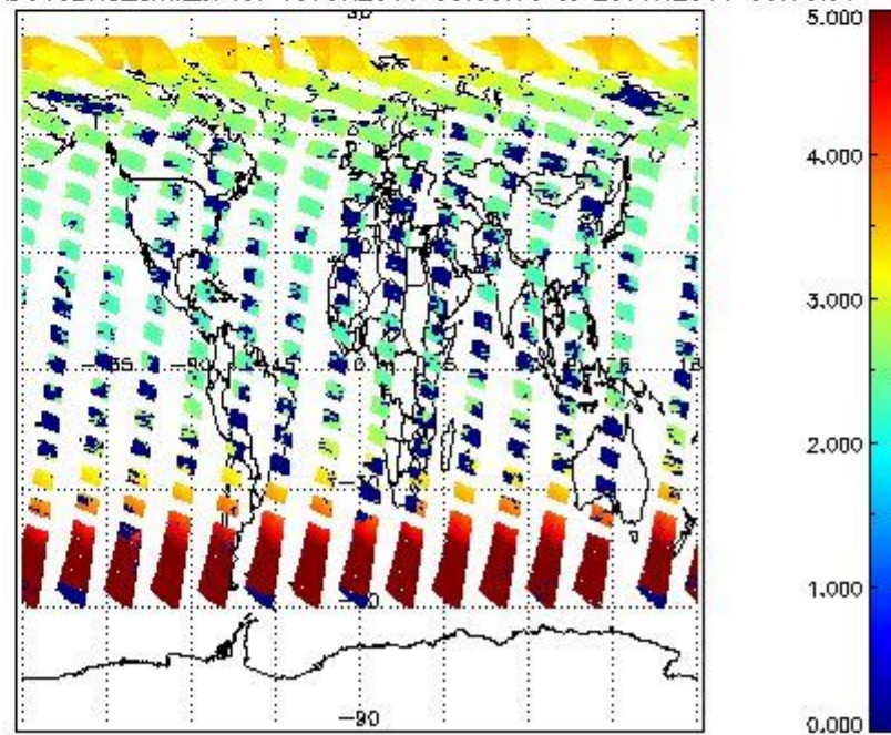
SCIOL2P_NADUV3BRO_amf_cl for 19JUN2011 00:00:00 to 20JUN2011 00:00:00
