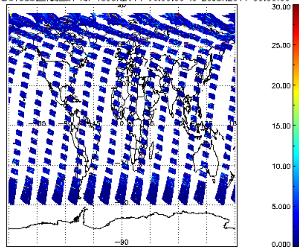
SCIOL2P_NADUV5S02_vcd_err for 19JUN2011 00:00:00 to 20JUN2011 00:00:00
