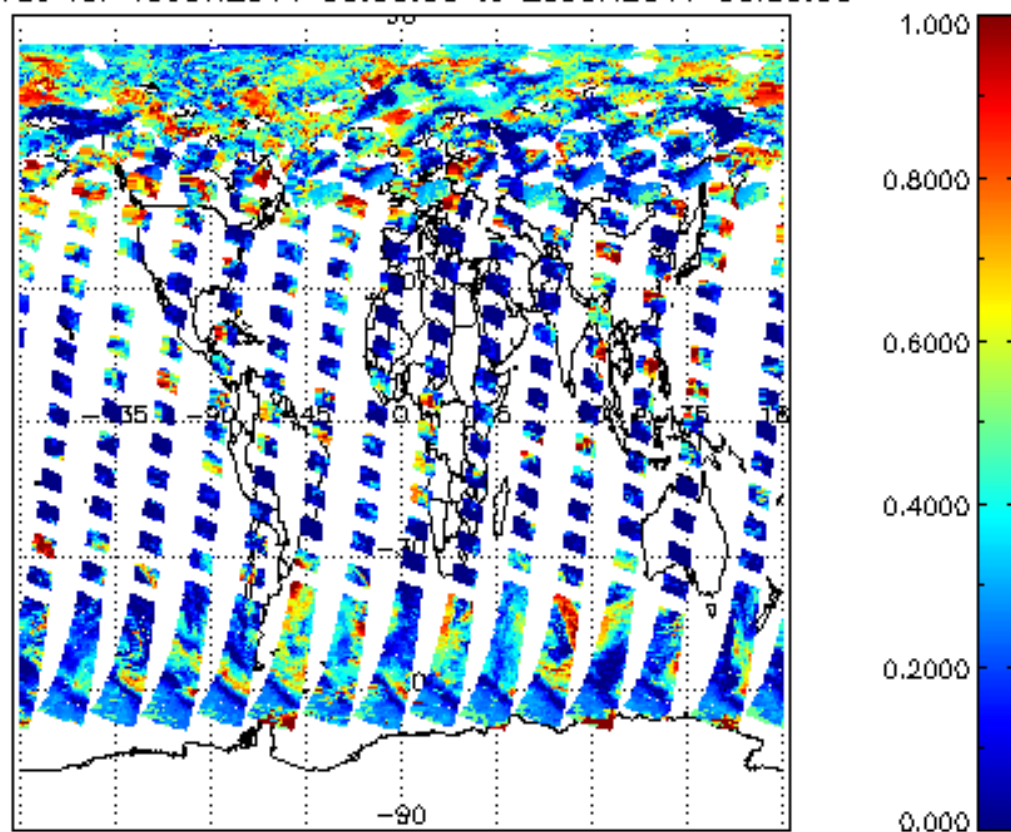
cl_frac for 19JUN2011 00:00:00 to 20JUN2011 00:00:00
