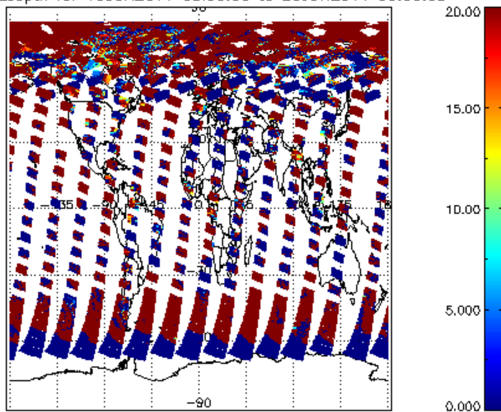
cl_opt_depth for 19JUN2011 00:00:00 to 20JUN2011 00:00:00
