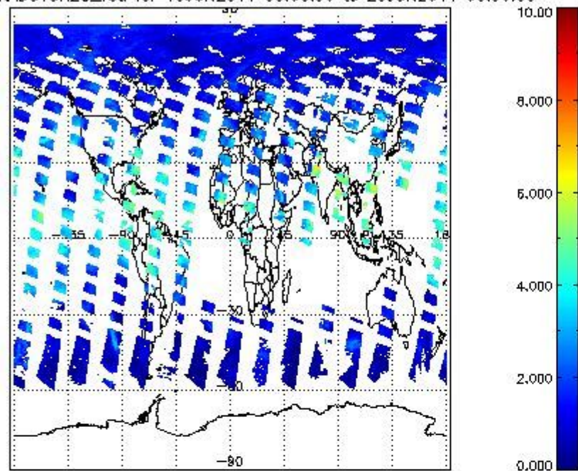
SCIOL2P_NADUV8H2O_vcd for 19JUN2011 00:00:00 to 20JUN2011 00:00:00
