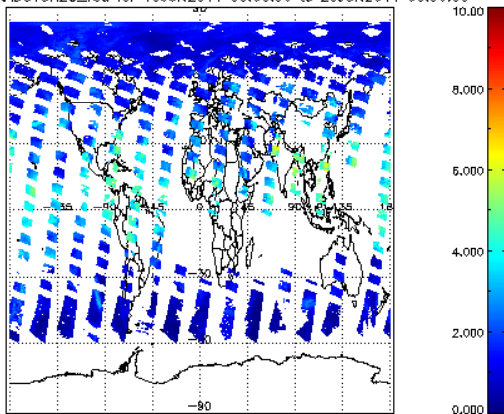
SCIOL2P_NADUV8H2O_vcd for 19JUN2011 00:00:00 to 20JUN2011 00:00:00
