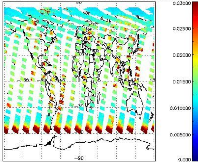
SCIOL2P_NADUV003_vcd_err for 19JUN2011 00:00:00 to 20JUN2011 00:00:00
