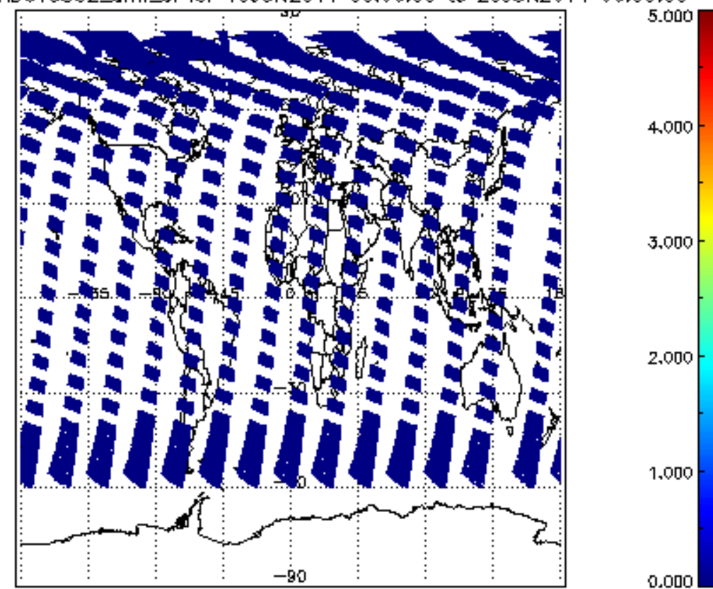
SCIOL2P_NADUV5S02_amf_cl for 19JUN2011 00:00:00 to 20JUN2011 00:00:00
