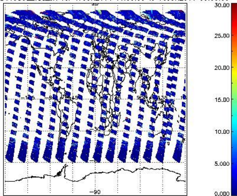
SCIOL2P_NADUV5S02_vcd_err for 17JUN2011 00:00:00 to 18JUN2011 00:00:00
