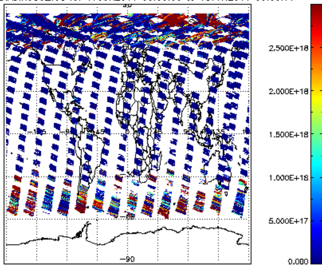
SCIOL2P_NADIR3CO_vcd for 17JUN2011 00:00:00 to 18JUN2011 00:00:00
