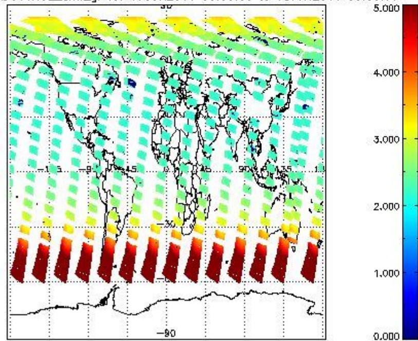
SCIOL2P_NADUV1NO2_amf_gr for 17JUN2011 00:00:00 to 18JUN2011 00:00:00
