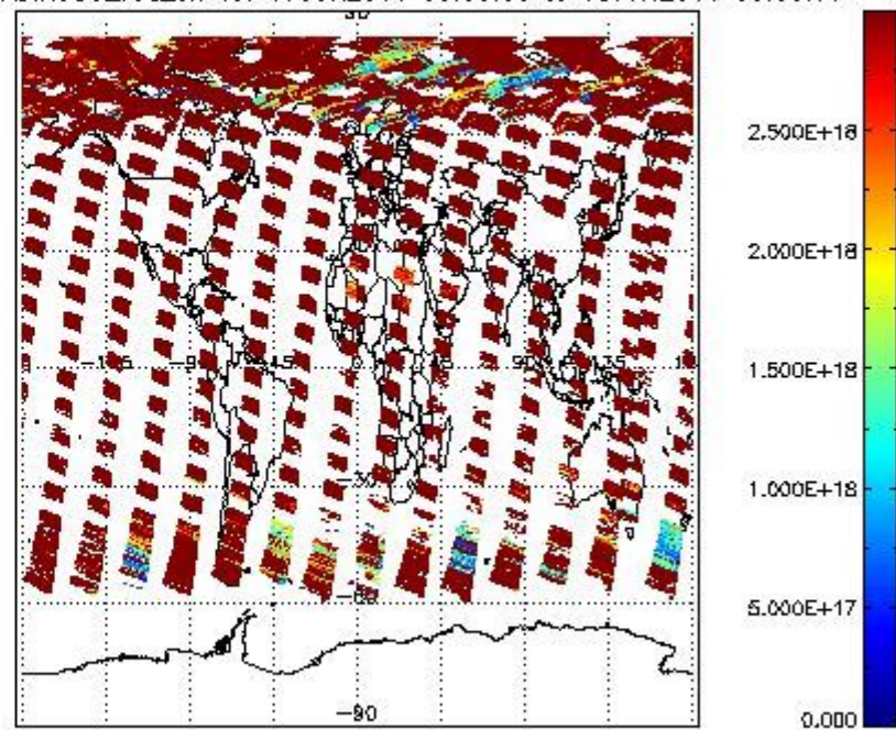
SCIOL2P_NADIR3CO_vcd_err for 17JUN2011 00:00:00 to 18JUN2011 00:00:00
