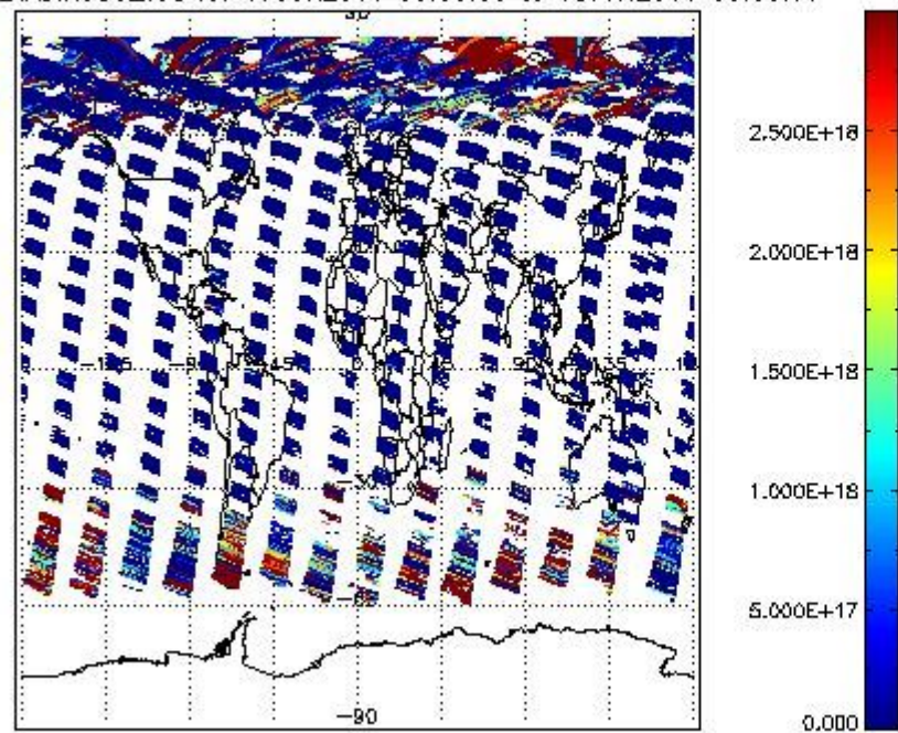
SCIOL2P_NADIR3CO_vcd for 17JUN2011 00:00:00 to 18JUN2011 00:00:00
