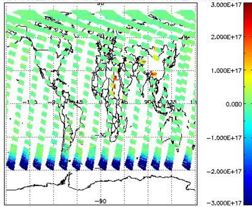
SCIOL2P_NADUV7S02_vcd for 17JUN2011 00:00:00 to 18JUN2011 00:00:00
