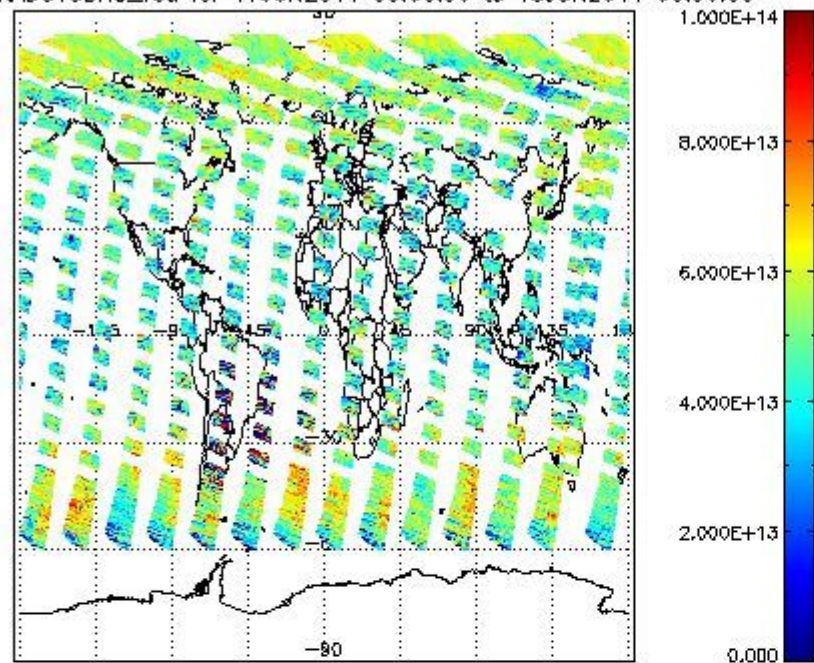
SCIOL2P_NADUV3BRO_vcd for 17JUN2011 00:00:00 to 18JUN2011 00:00:00
