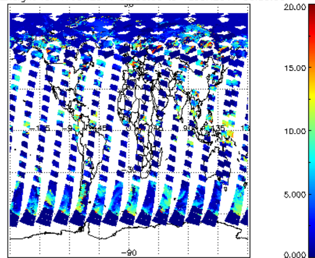
cl_top_height for 17JUN2011 00:00:00 to 18JUN2011 00:00:00
