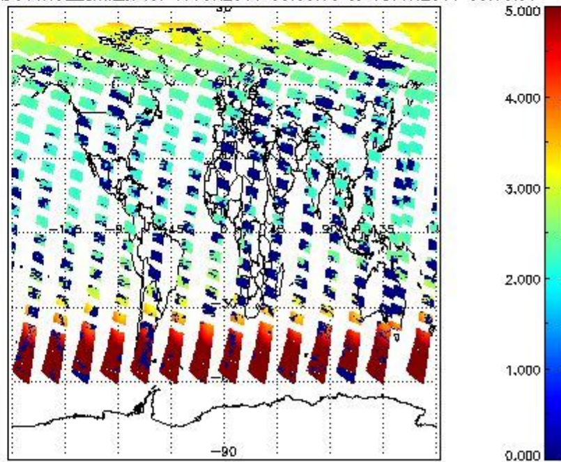
SCIOL2P_NADUV1NO2_amf_cl for 17JUN2011 00:00:00 to 18JUN2011 00:00:00
