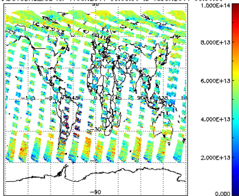
SCIOL2P_NADUV3BRO_vcd for 17JUN2011 00:00:00 to 18JUN2011 00:00:00
