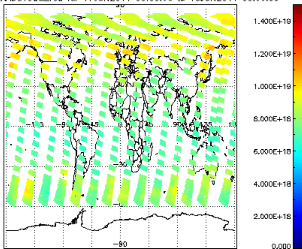
SCIOL2P_NADUV003_vcd for 17JUN2011 00:00:00 to 18JUN2011 00:00:00
