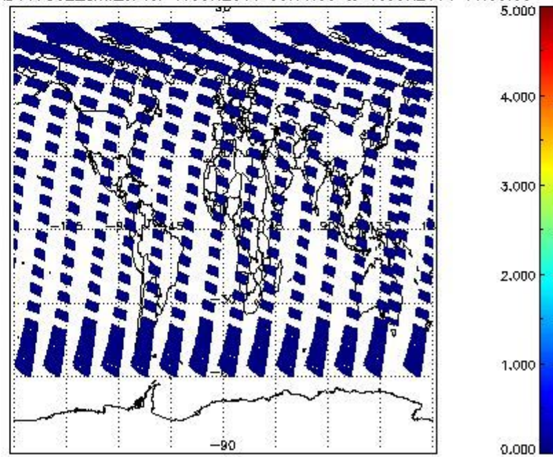
SCIOL2P_NADUV7S02_amf_cl for 17JUN2011 00:00:00 to 18JUN2011 00:00:00
