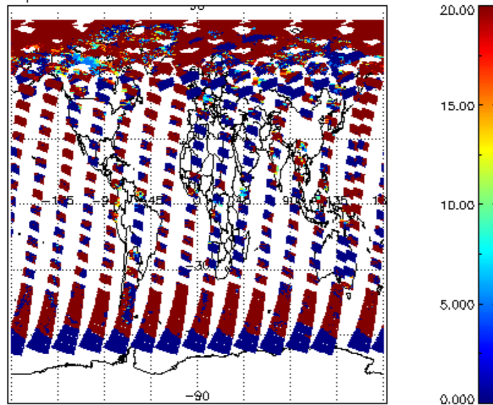
cl_opt_depth for 17JUN2011 00:00:00 to 18JUN2011 00:00:00
