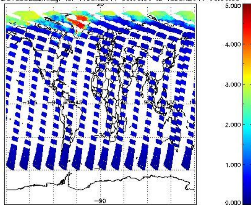
SCIOL2P_NADUV5S02_amf_gr for 17JUN2011 00:00:00 to 18JUN2011 00:00:00
