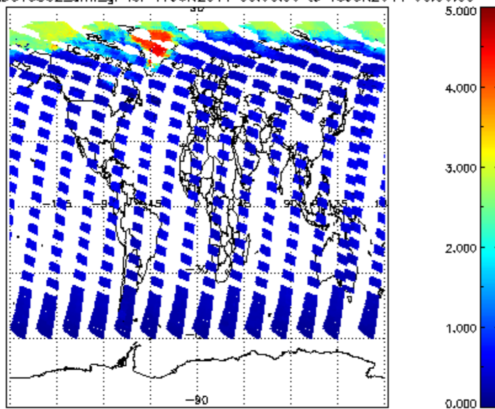
SCIOL2P_NADUV5S02_amf_gr for 17JUN2011 00:00:00 to 18JUN2011 00:00:00
