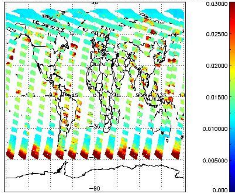
SCIOL2P_NADUV003_vcd_err for 17JUN2011 00:00:00 to 18JUN2011 00:00:00
