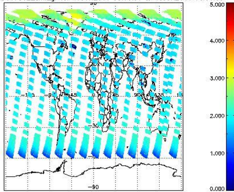
SCIOL2P_NADUV7S02_amf_gr for 17JUN2011 00:00:00 to 18JUN2011 00:00:00
