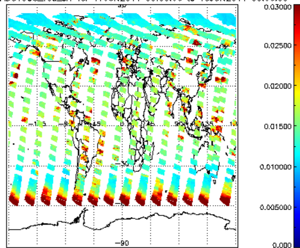
SCIOL2P_NADUV003_vcd_err for 17JUN2011 00:00:00 to 18JUN2011 00:00:00
