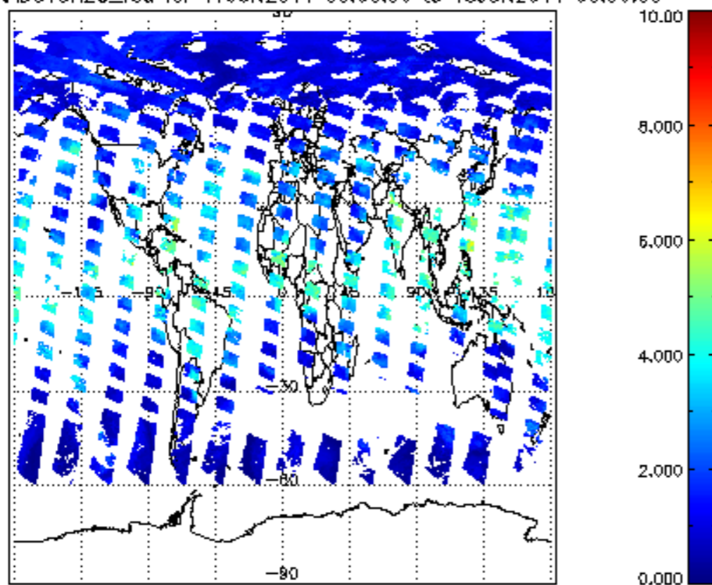
SCIOL2P_NADUV8H2O_vcd for 17JUN2011 00:00:00 to 18JUN2011 00:00:00
