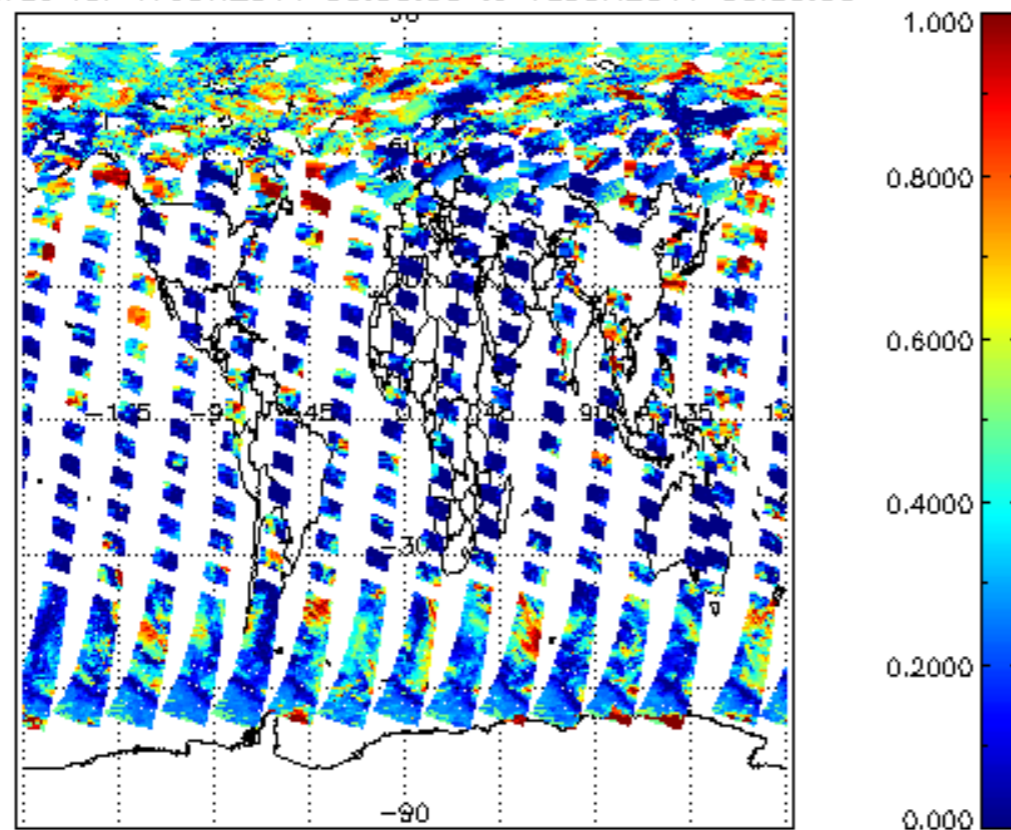
cl_frac for 17JUN2011 00:00:00 to 18JUN2011 00:00:00
