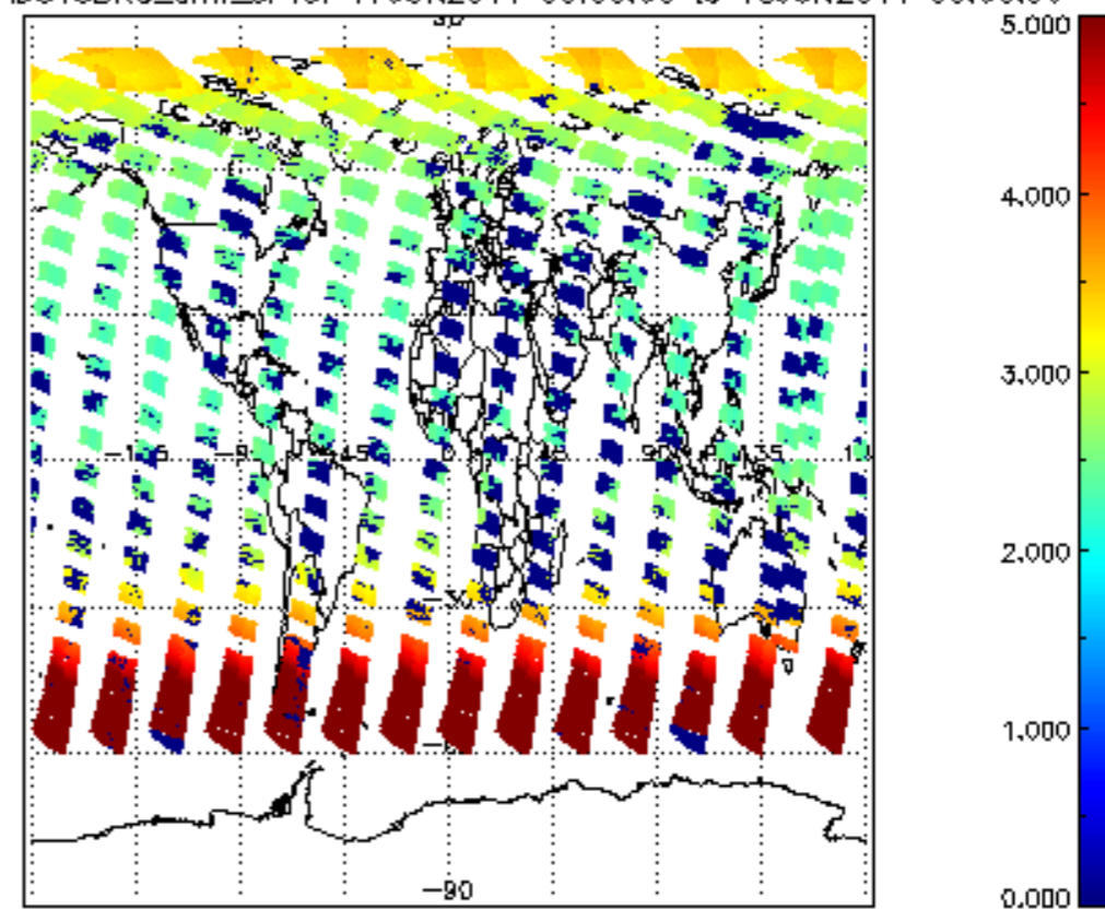
SCIOL2P_NADUV3BRO_amf_sl for 17JUN2011 00:00:00 to 18JUN2011 00:00:00
