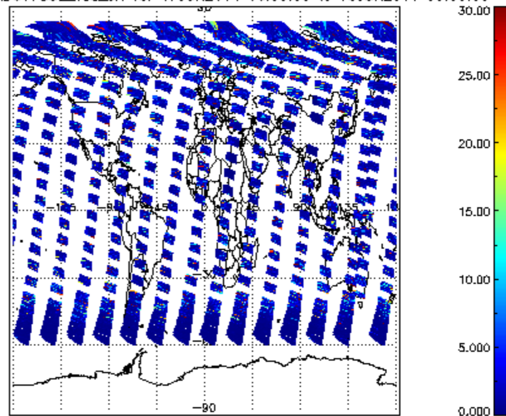
SCIOL2P_NADUV7S02_vcd_err for 17JUN2011 00:00:00 to 18JUN2011 00:00:00
