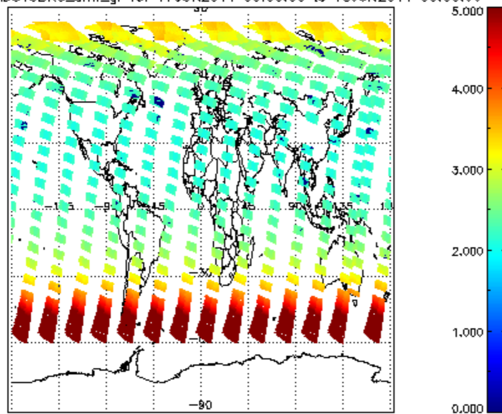
SCIOL2P_NADUV3BRO_amf_gr for 17JUN2011 00:00:00 to 18JUN2011 00:00:00
