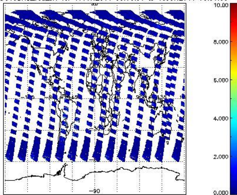
SCIOL2P_NADUV3BRO_vcd_err for 17JUN2011 00:00:00 to 18JUN2011 00:00:00
