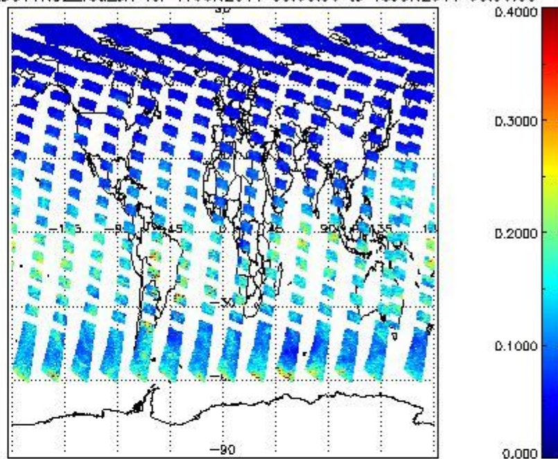
SCIOL2P_NADUV1NO2_vcd_err for 17JUN2011 00:00:00 to 18JUN2011 00:00:00
