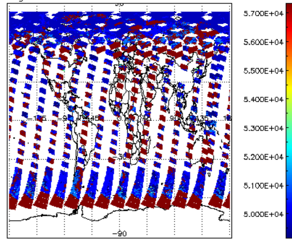
cloud_flags for 17JUN2011 00:00:00 to 18JUN2011 00:00:00
