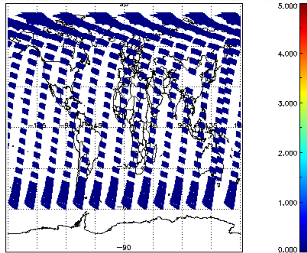
SCIOL2P_NADUV7S02_amf_cl for 17JUN2011 00:00:00 to 18JUN2011 00:00:00
