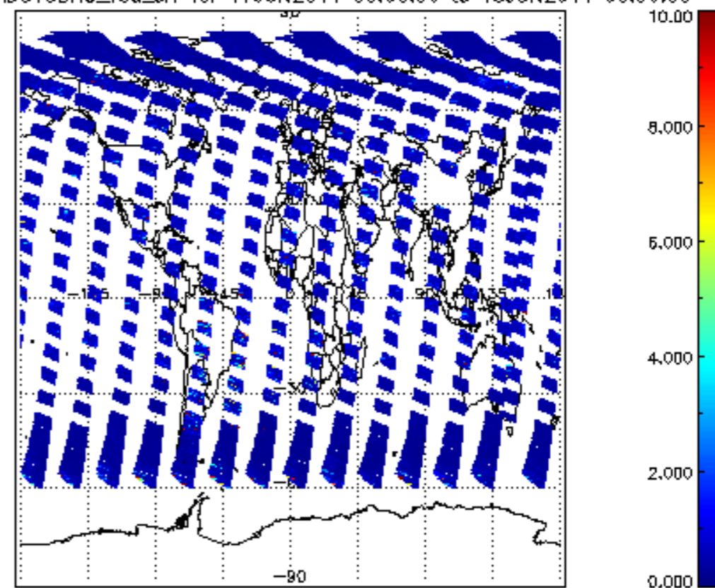
SCIOL2P_NADUV3BRO_vcd_err for 17JUN2011 00:00:00 to 18JUN2011 00:00:00
