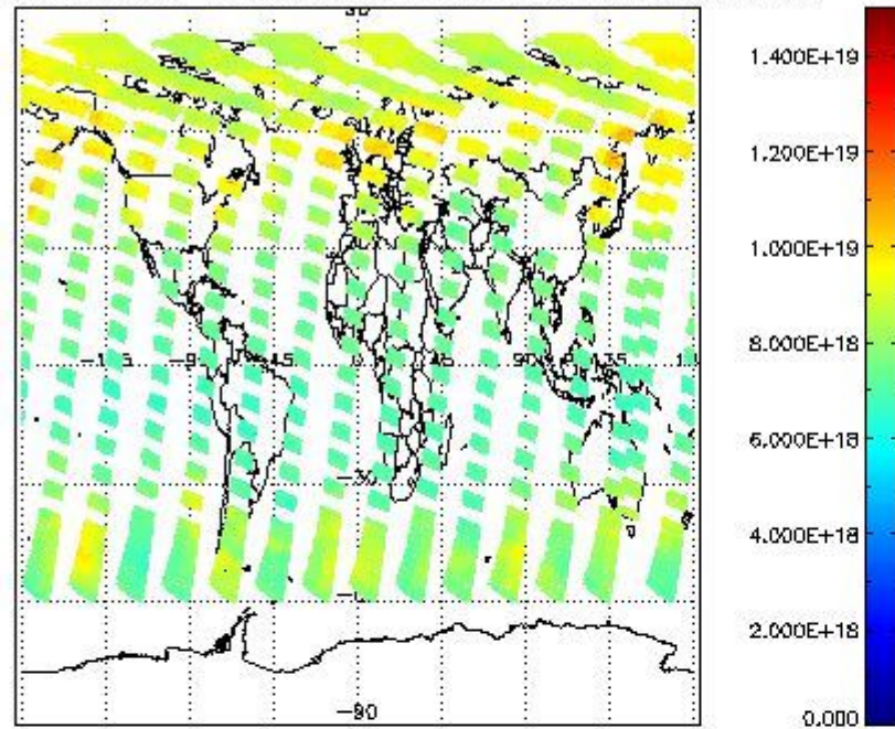
SCIOL2P_NADUV003_vcd for 17JUN2011 00:00:00 to 18JUN2011 00:00:00
