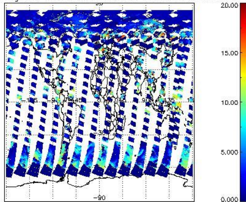
cL_top_height for 17JUN2011 00:00:00 to 18JUN2011 00:00:00
