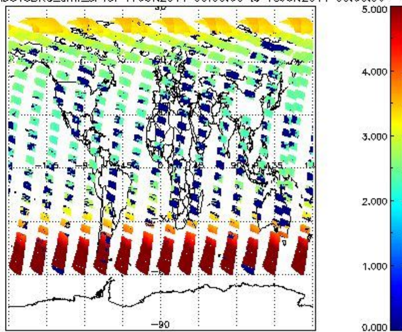
SCIOL2P_NADUV3BRO_amf_cl for 17JUN2011 00:00:00 to 18JUN2011 00:00:00
