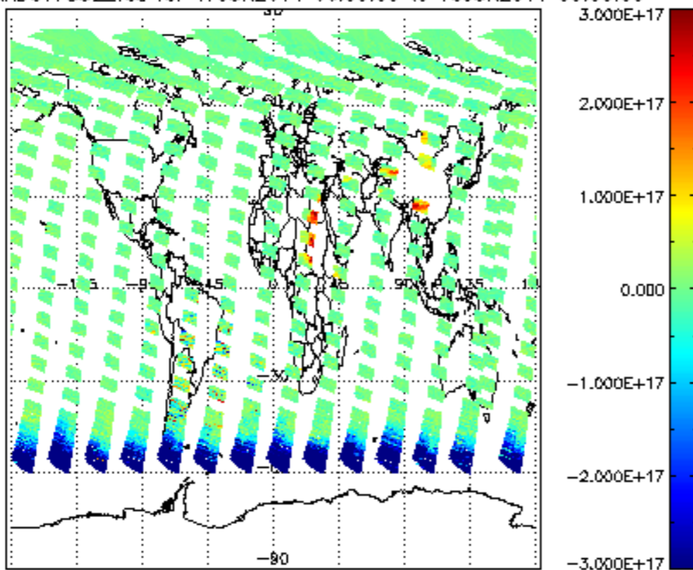
SCIOL2P_NADUV7S02_vcd for 17JUN2011 00:00:00 to 18JUN2011 00:00:00
