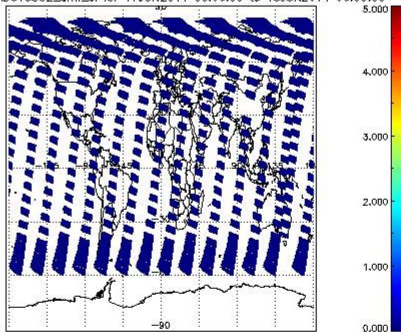
SCIOL2P_NADUV5S02_amf_cl for 17JUN2011 00:00:00 to 18JUN2011 00:00:00
