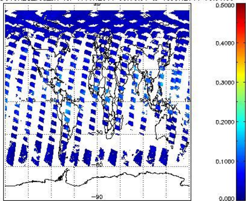
SCIOL2P_NADUV8H2O_vcd_err for 17JUN2011 00:00:00 to 18JUN2011 00:00:00
