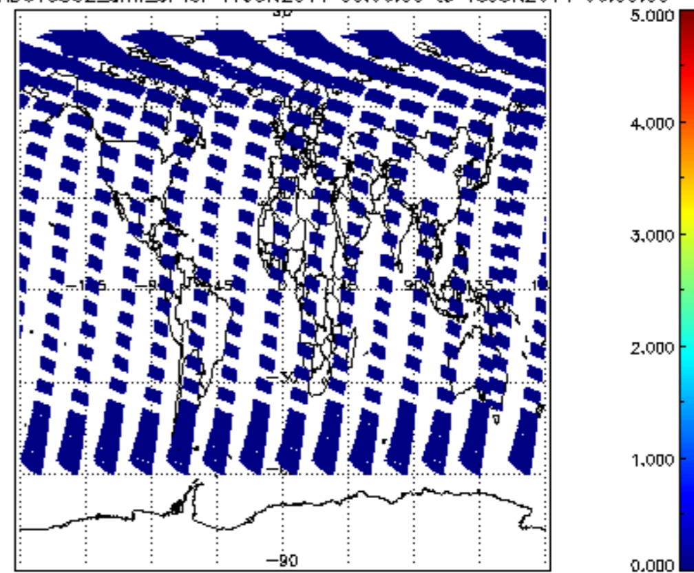
SCIOL2P_NADUV5S02_amf_cl for 17JUN2011 00:00:00 to 18JUN2011 00:00:00
