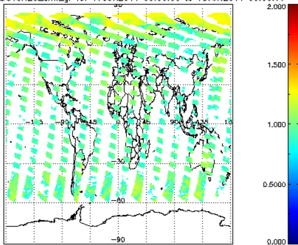
SCIOL2P_NADUV8H2O_amf_gr for 17JUN2011 00:00:00 to 18JUN2011 00:00:00
