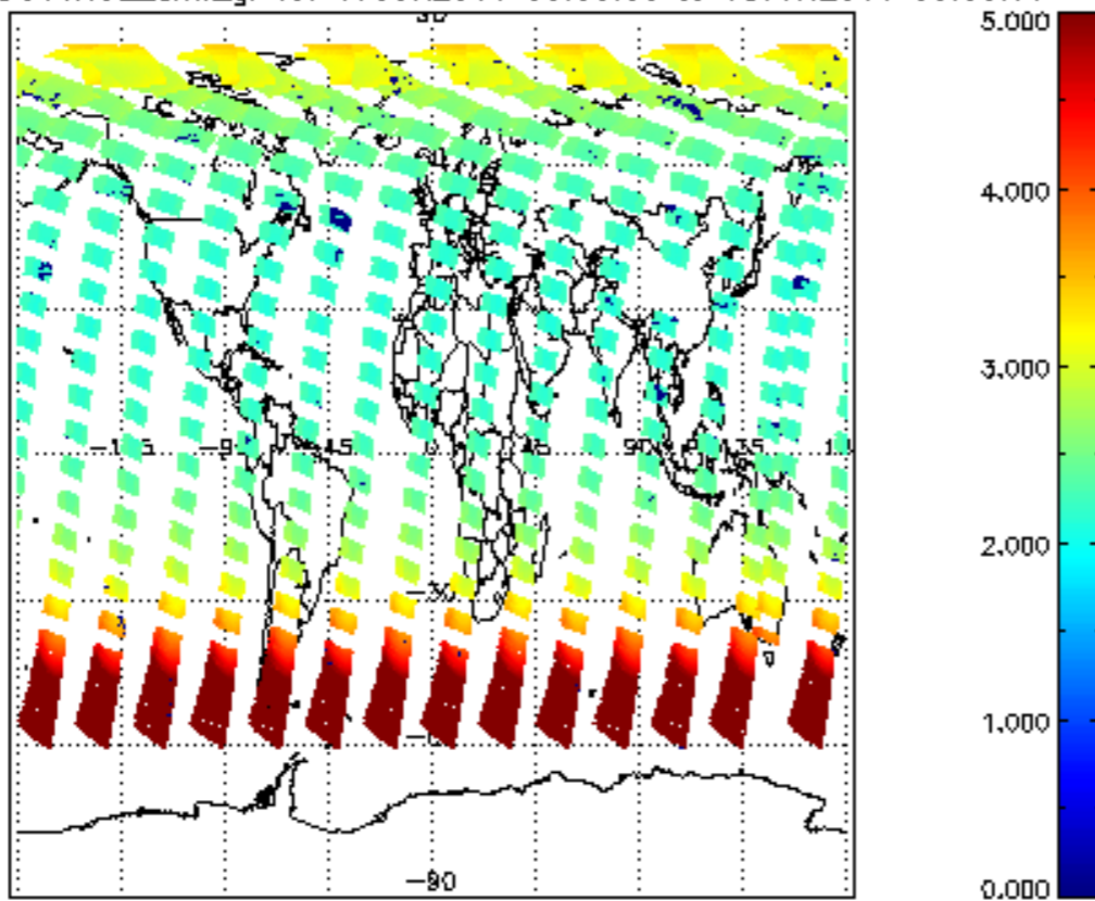
SCIOL2P_NADUV1NO2_amf_gr for 17JUN2011 00:00:00 to 18JUN2011 00:00:00
