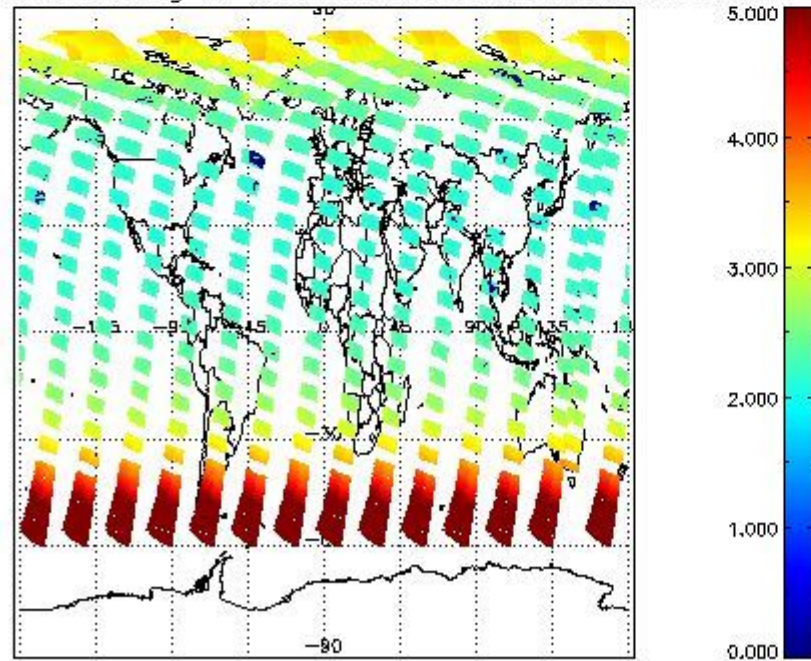
SCIOL2P_NADUV003_amf_gr for 17JUN2011 00:00:00 to 18JUN2011 00:00:00
