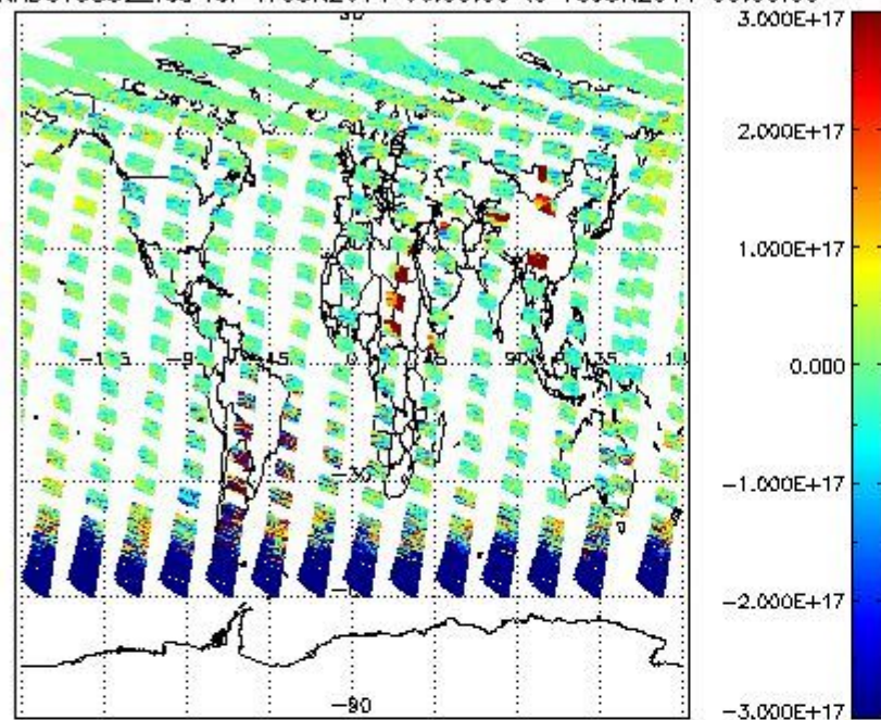
SCIOL2P_NADUV5S02_vcd for 17JUN2011 00:00:00 to 18JUN2011 00:00:00
