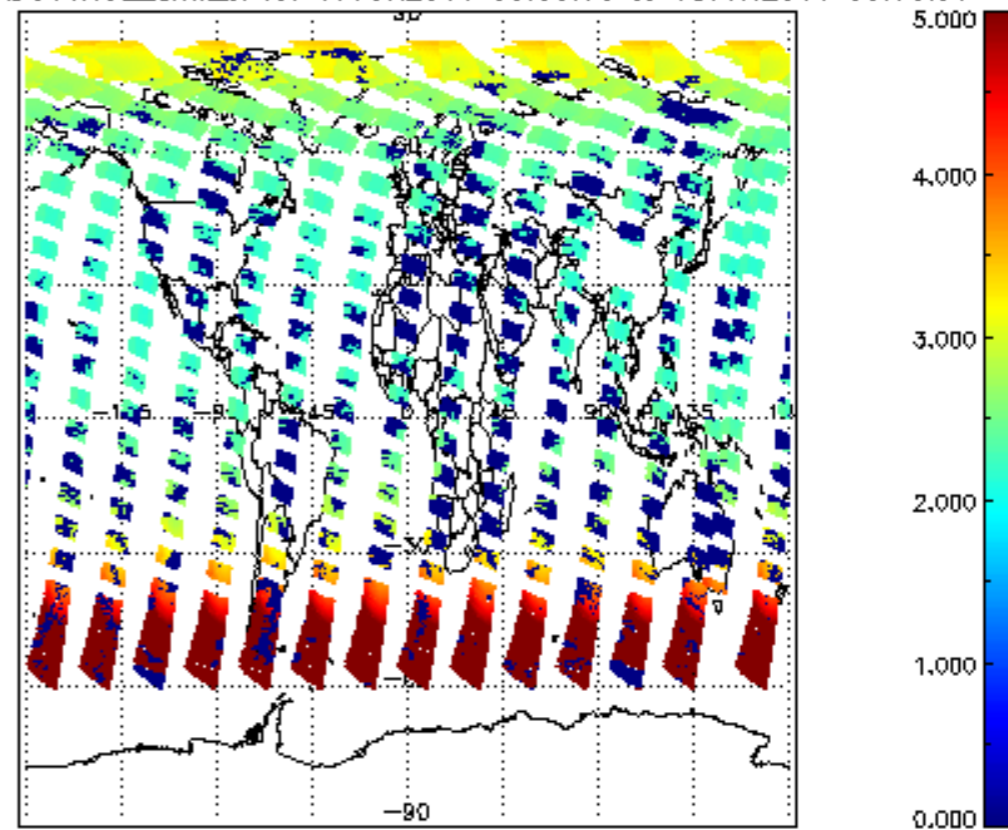
SCIOL2P_NADUV1NO2_amf_sl for 17JUN2011 00:00:00 to 18JUN2011 00:00:00
