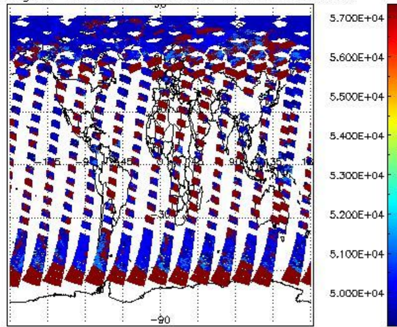
cloud_flags for 17JUN2011 00:00:00 to 18JUN2011 00:00:00
