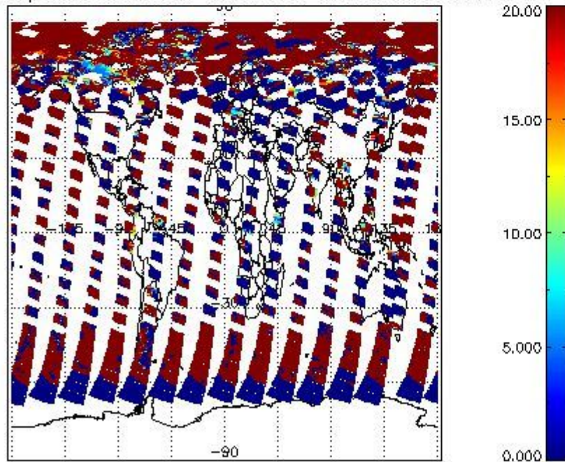
cL_opt_depth for 17JUN2011 00:00:00 to 18JUN2011 00:00:00
