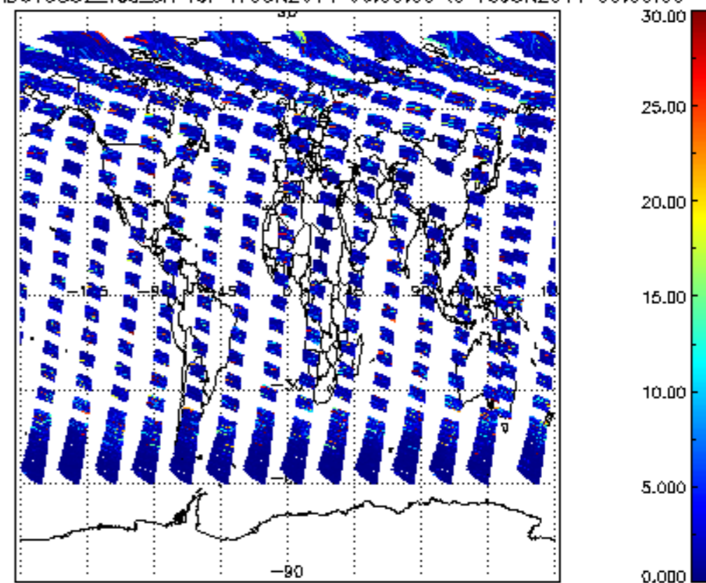
SCIOL2P_NADUV5S02_vcd_err for 17JUN2011 00:00:00 to 18JUN2011 00:00:00
