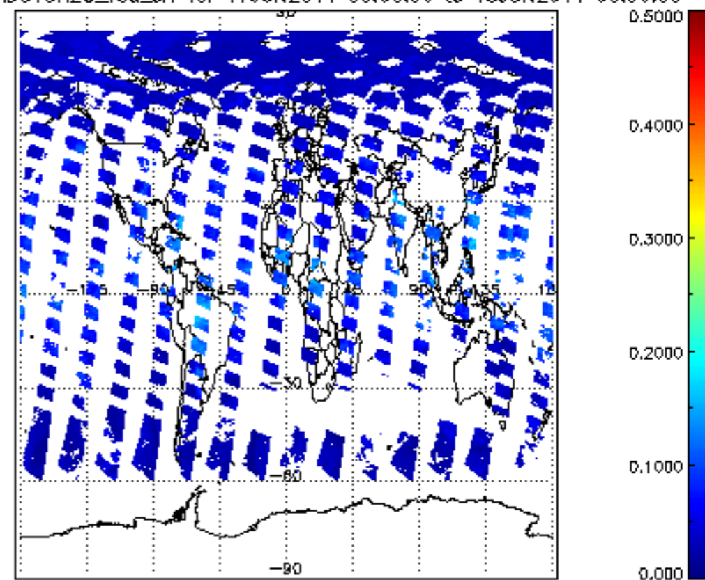
SCIOL2P_NADUV8H2O_vcd_err for 17JUN2011 00:00:00 to 18JUN2011 00:00:00
