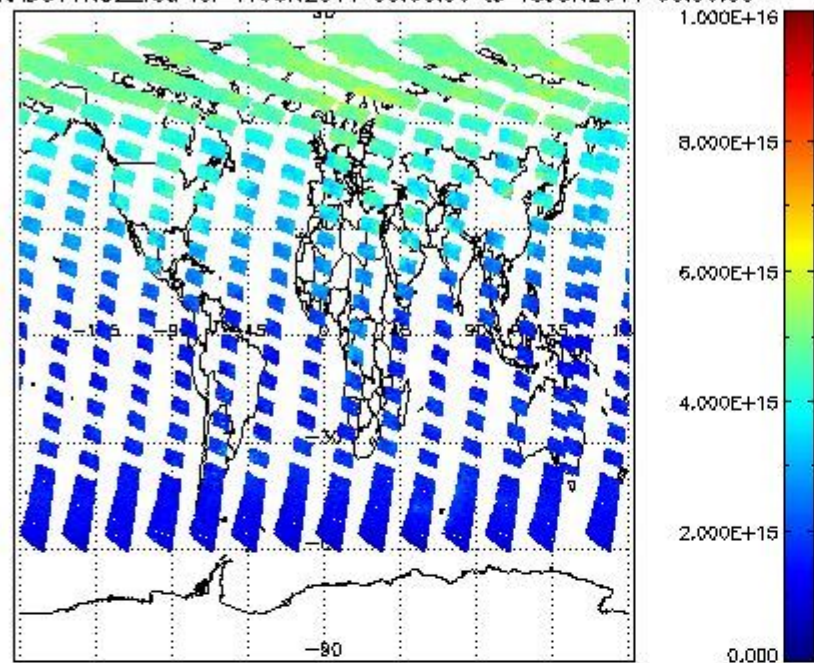
SCIOL2P_NADUV1NO2_vcd for 17JUN2011 00:00:00 to 18JUN2011 00:00:00
