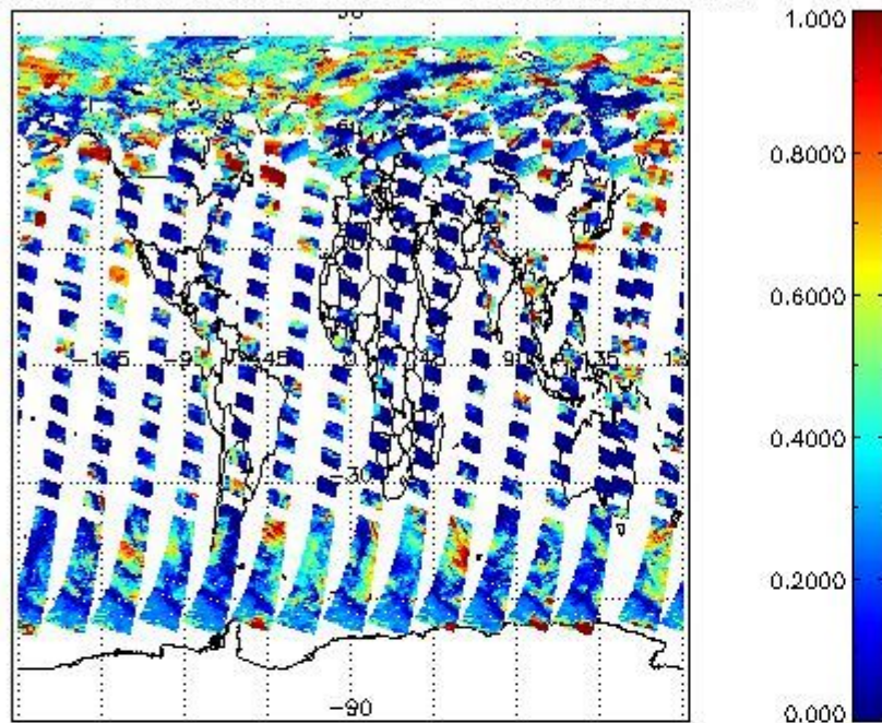
cL_frac for 17JUN2011 00:00:00 to 18JUN2011 00:00:00
