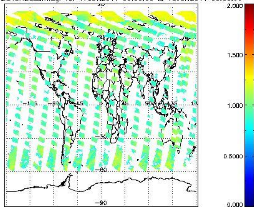
SCIOL2P_NADUV8H2O_arnf_gr for 17JUN2011 00:00:00 to 18JUN2011 00:00:00
