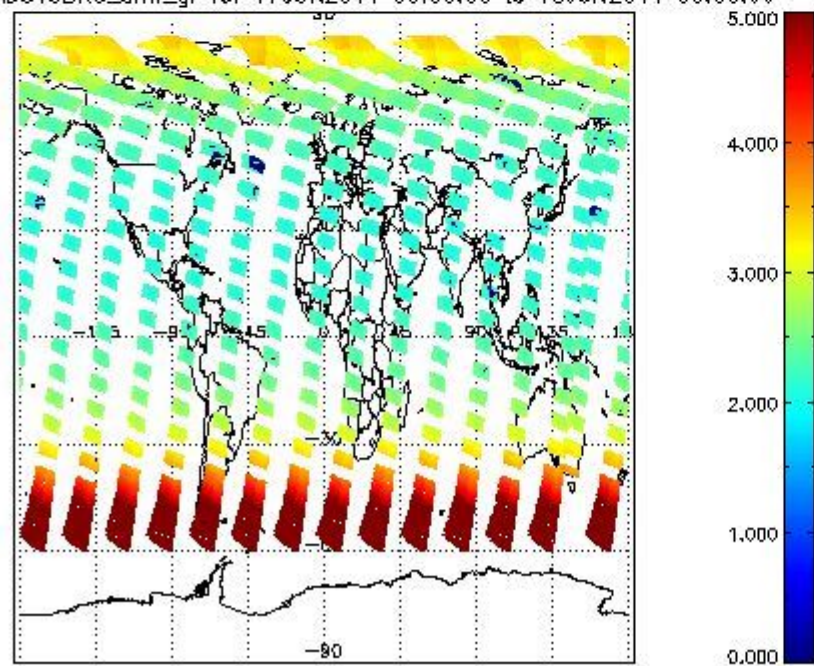
SCIOL2P_NADUV3BRO_amf_gr for 17JUN2011 00:00:00 to 18JUN2011 00:00:00
