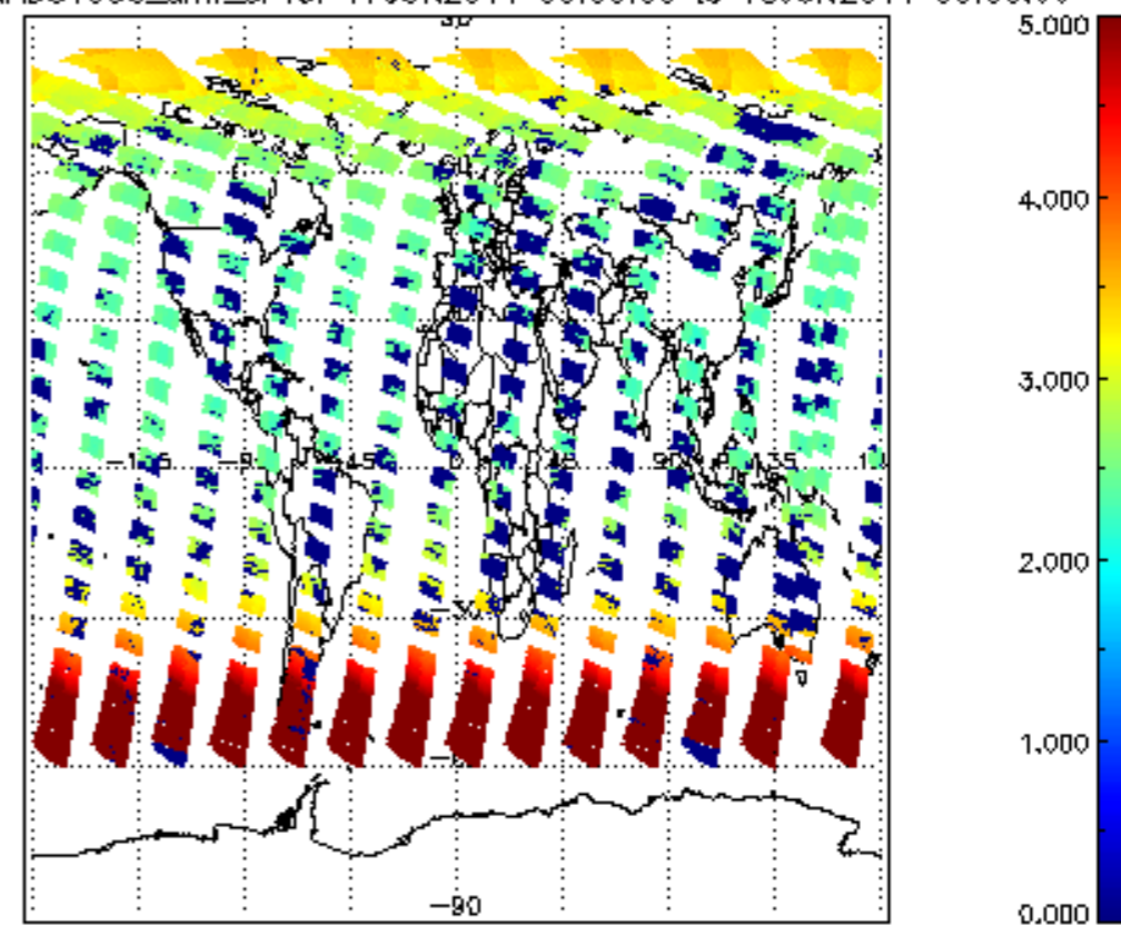
SCIOL2P_NADUV003_amf_cl for 17JUN2011 00:00:00 to 18JUN2011 00:00:00
