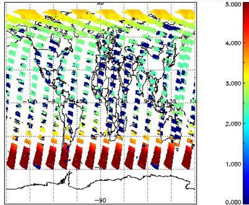
SCIOL2P_NADUV003_amf_cl for 17JUN2011 00:00:00 to 18JUN2011 00:00:00
