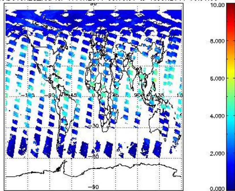
SCIOL2P_NADUV8H2O_vcd for 17JUN2011 00:00:00 to 18JUN2011 00:00:00
