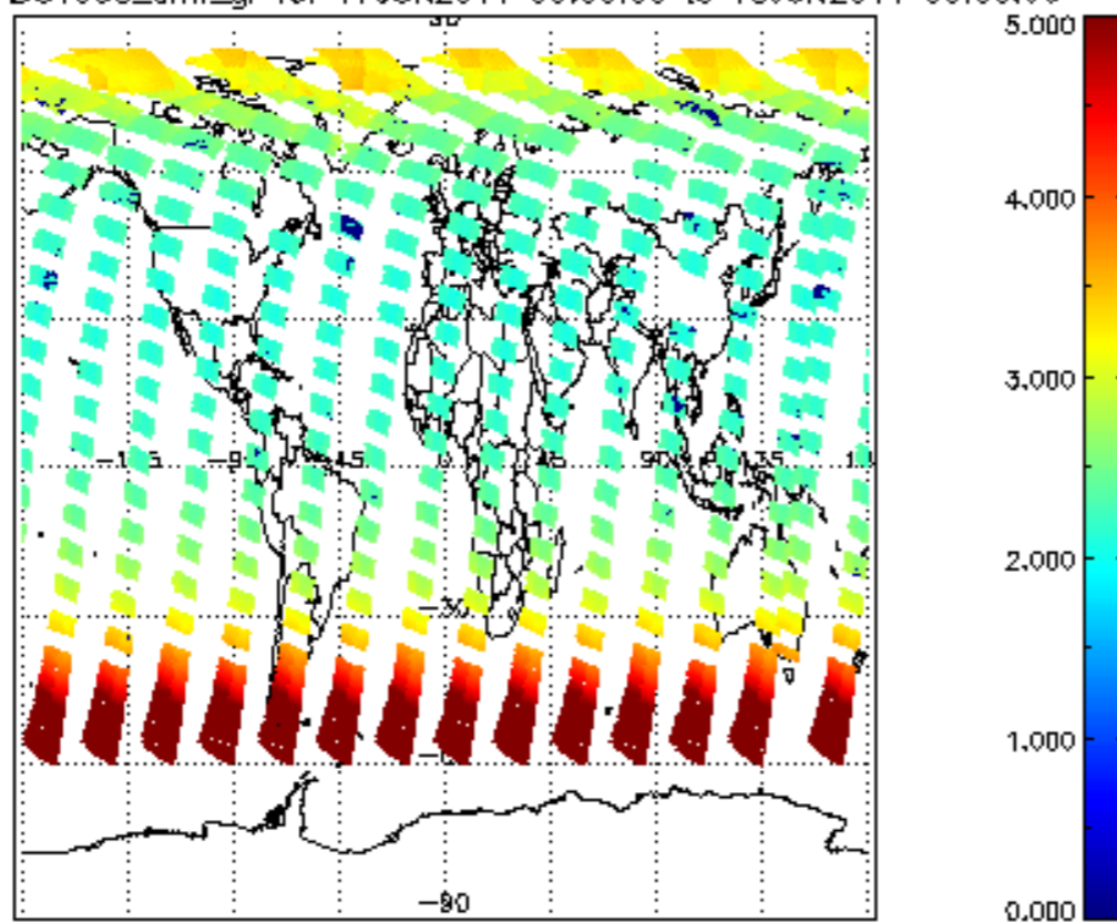
SCIOL2P_NADUV003_amf_gr for 17JUN2011 00:00:00 to 18JUN2011 00:00:00
