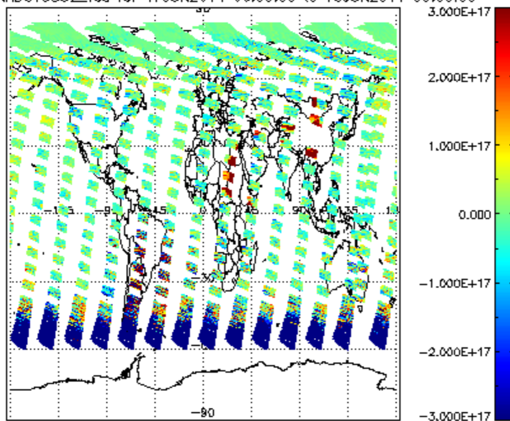
SCIOL2P_NADUV5S02_vcd for 17JUN2011 00:00:00 to 18JUN2011 00:00:00
