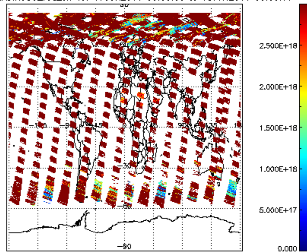
SCIOL2P_NADIR3CO_vcd_err for 17JUN2011 00:00:00 to 18JUN2011 00:00:00
