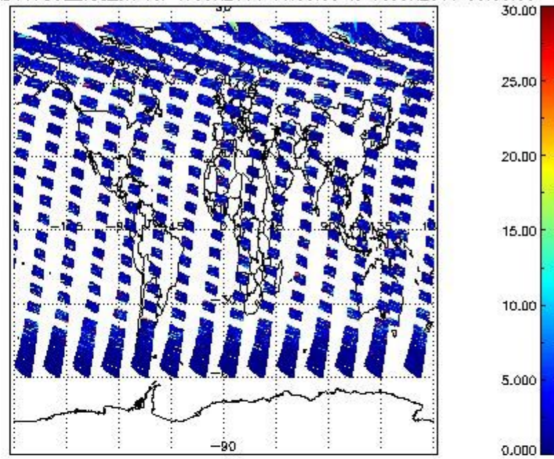
SCIOL2P_NADUV7S02_vcd_err for 17JUN2011 00:00:00 to 18JUN2011 00:00:00
