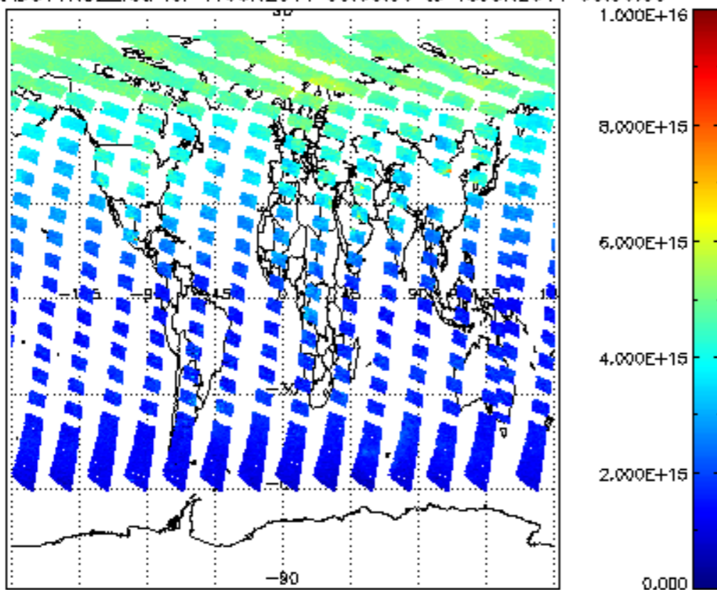
SCIOL2P_NADUV1NO2_vcd for 17JUN2011 00:00:00 to 18JUN2011 00:00:00
