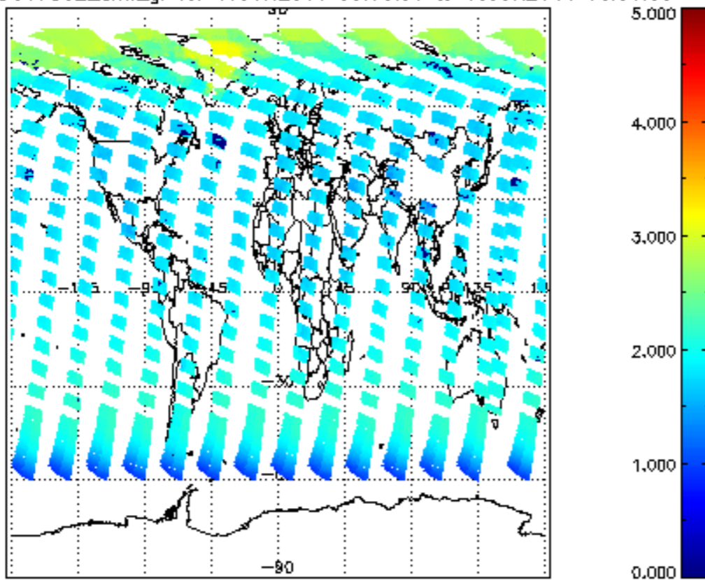
SCIOL2P_NADUV7S02_amf_gr for 17JUN2011 00:00:00 to 18JUN2011 00:00:00
