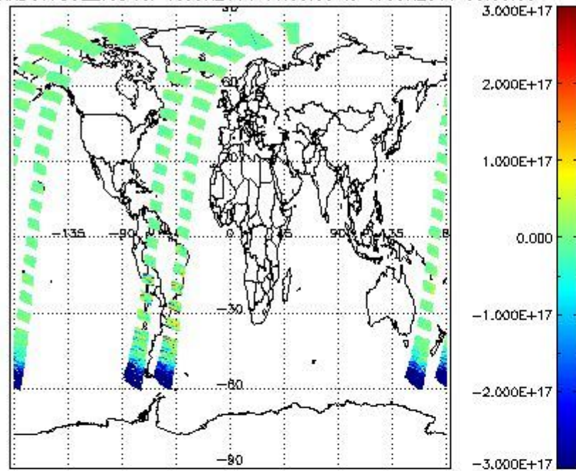
SCIOL2P_NADUV7S02_vcd for 16JUN2011 00:00:00 to 17JUN2011 00:00:00
