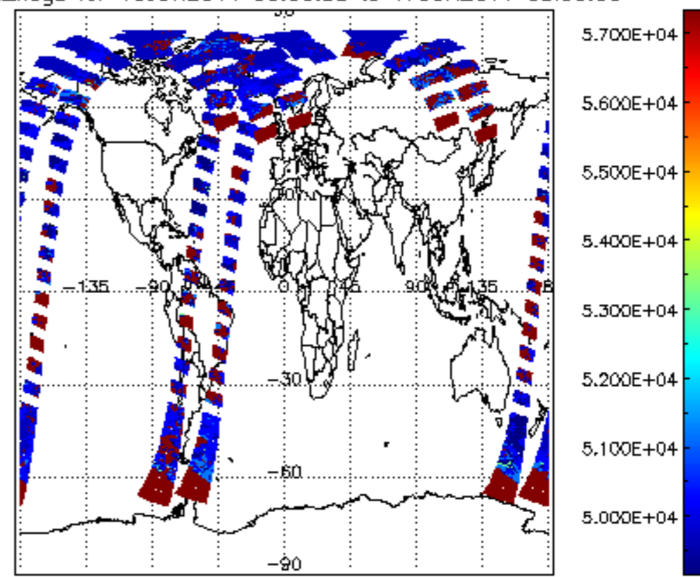
cloud_flags for 16JUN2011 00:00:00 to 17JUN2011 00:00:00
