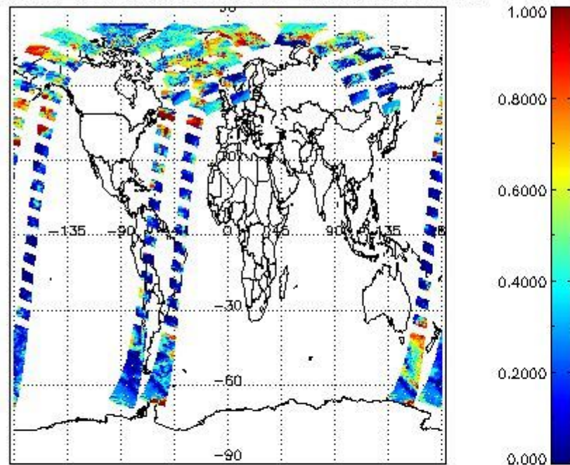
cL_frac for 16JUN2011 00:00:00 to 17JUN2011 00:00:00
