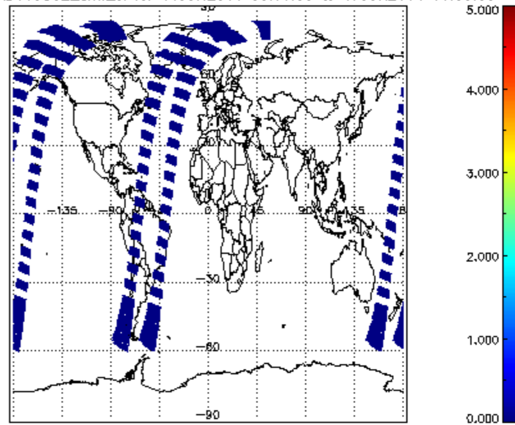
SCIOL2P_NADUV5S02_amf_cl for 16JUN2011 00:00:00 to 17JUN2011 00:00:00
