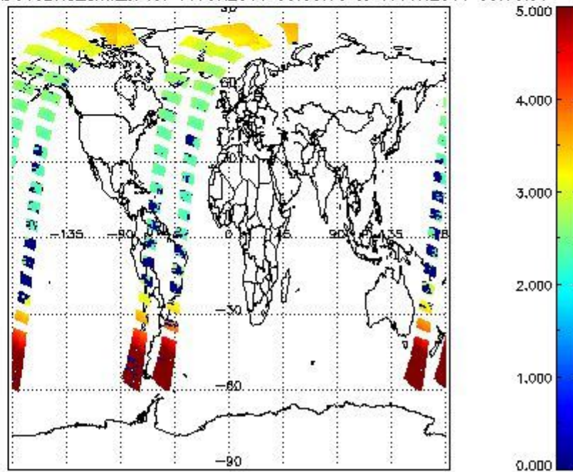
SCIOL2P_NADUV3BRO_amf_cl for 16JUN2011 00:00:00 to 17JUN2011 00:00:00
