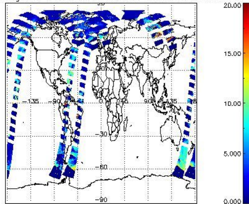
cL_top_height for 16JUN2011 00:00:00 to 17JUN2011 00:00:00
