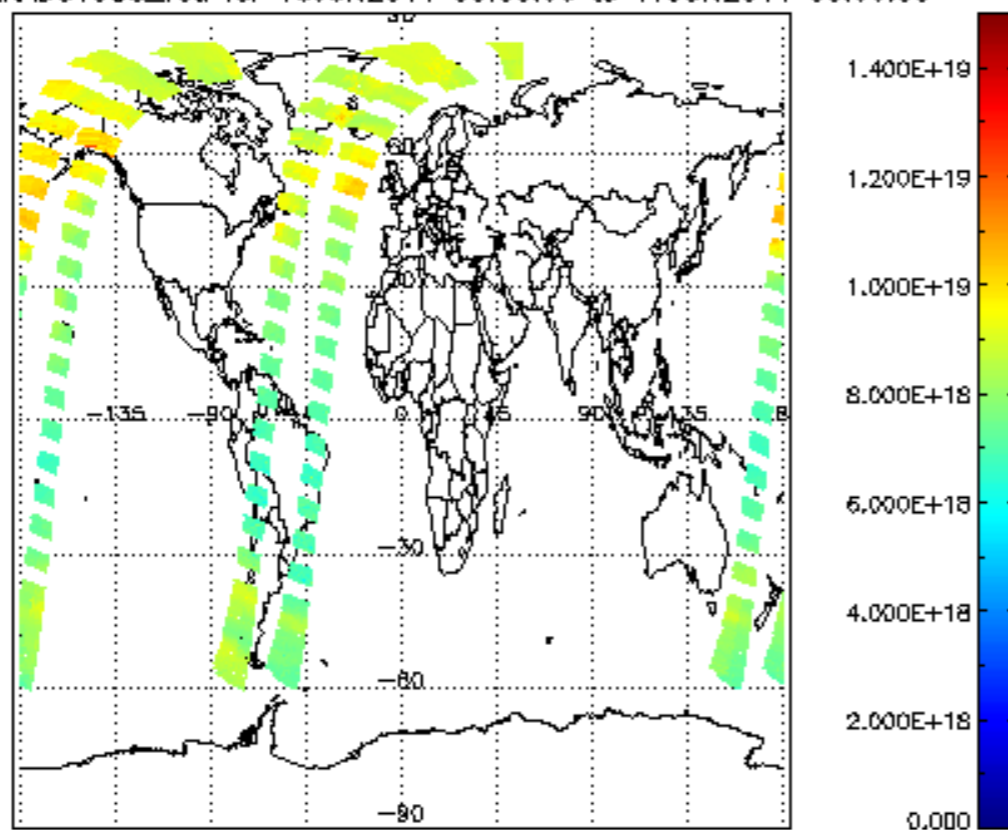
SCIOL2P_NADUV003_vcd for 16JUN2011 00:00:00 to 17JUN2011 00:00:00
