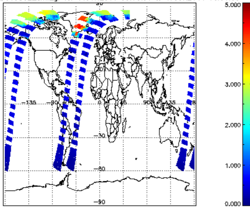
SCIOL2P_NADUV5S02_amf_gr for 16JUN2011 00:00:00 to 17JUN2011 00:00:00
