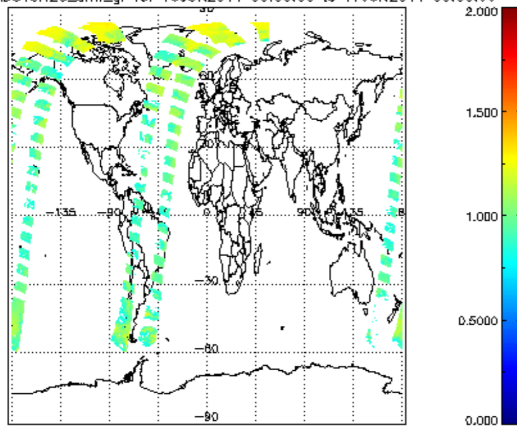
SCIOL2P_NADUV8H2O_amf_gr for 16JUN2011 00:00:00 to 17JUN2011 00:00:00
