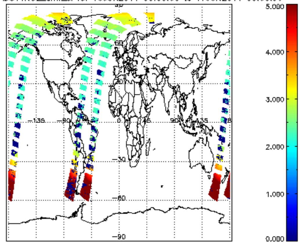
SCIOL2P_NADUV1NO2_amf_sl for 16JUN2011 00:00:00 to 17JUN2011 00:00:00
