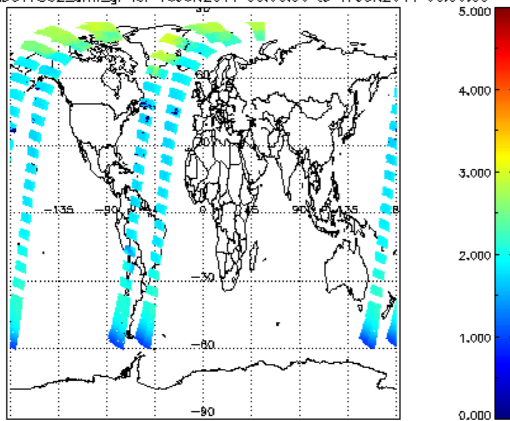
SCIOL2P_NADUV7S02_amf_gr for 16JUN2011 00:00:00 to 17JUN2011 00:00:00
