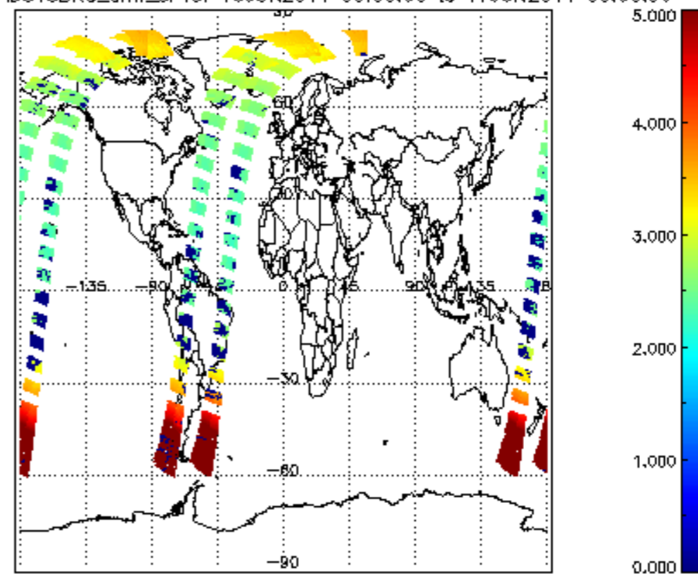
SCIOL2P_NADUV3BRO_amf_sl for 16JUN2011 00:00:00 to 17JUN2011 00:00:00
