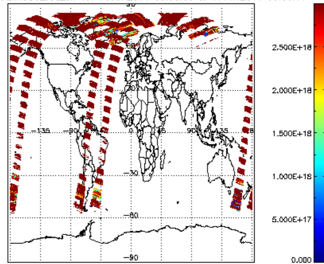
SCIOL2P_NADIR3CO_vcd_err for 16JUN2011 00:00:00 to 17JUN2011 00:00:00
