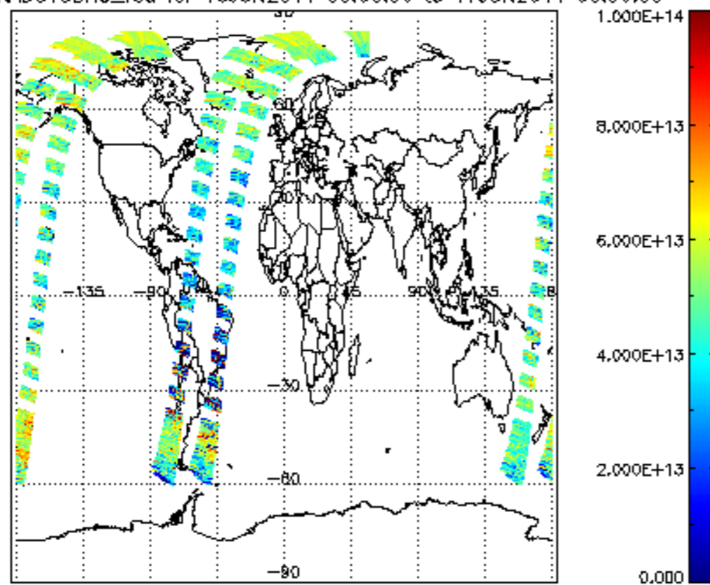
SCIOL2P_NADUV3BRO_vcd for 16JUN2011 00:00:00 to 17JUN2011 00:00:00
