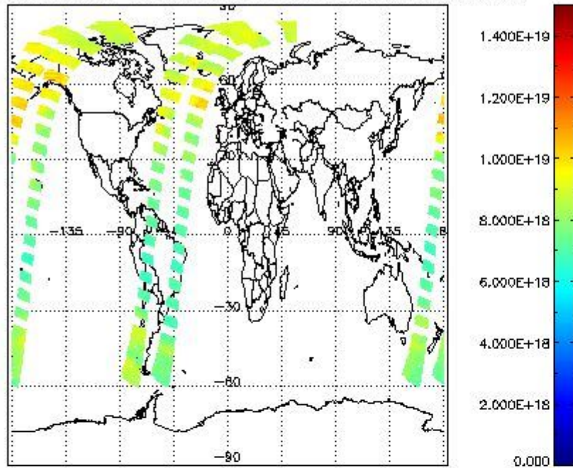
SCIOL2P_NADUV003_vcd for 16JUN2011 00:00:00 to 17JUN2011 00:00:00
