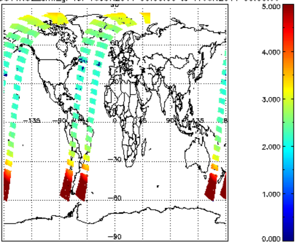
SCIOL2P_NADUV1NO2_amf_gr for 16JUN2011 00:00:00 to 17JUN2011 00:00:00
