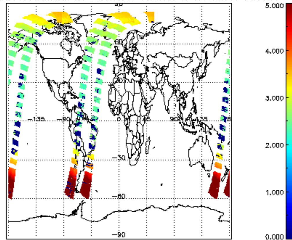
SCIOL2P_NADUV003_amf_cl for 16JUN2011 00:00:00 to 17JUN2011 00:00:00
