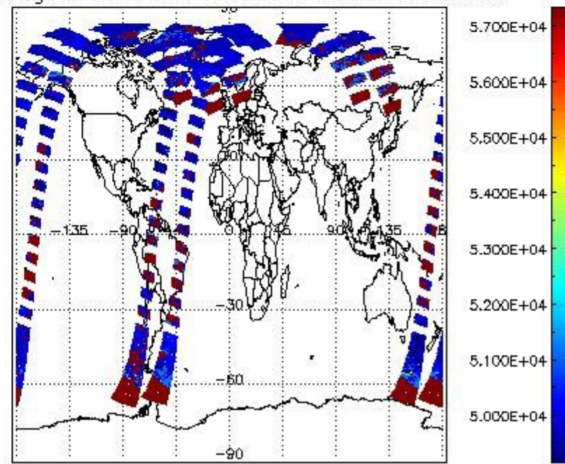
cloud_flags for 16JUN2011 00:00:00 to 17JUN2011 00:00:00
