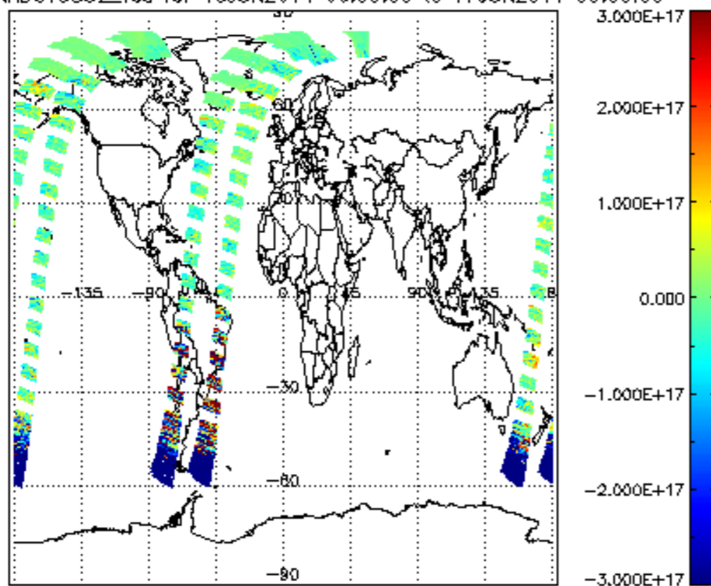
SCIOL2P_NADUV5S02_vcd for 16JUN2011 00:00:00 to 17JUN2011 00:00:00
