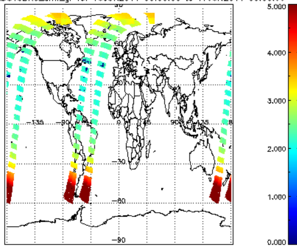
SCIOL2P_NADUV3BRO_amf_gr for 16JUN2011 00:00:00 to 17JUN2011 00:00:00
