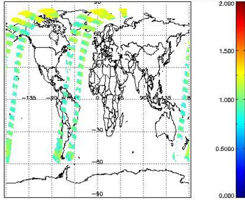
SCIOL2P_NADUV8H2O_arnf_gr for 16JUN2011 00:00:00 to 17JUN2011 00:00:00
