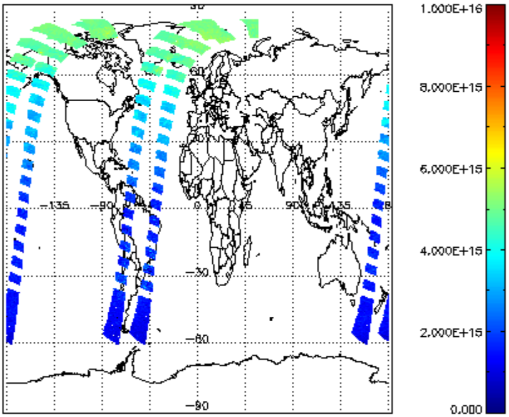
SCIOL2P_NADUV1NO2_vcd for 16JUN2011 00:00:00 to 17JUN2011 00:00:00
