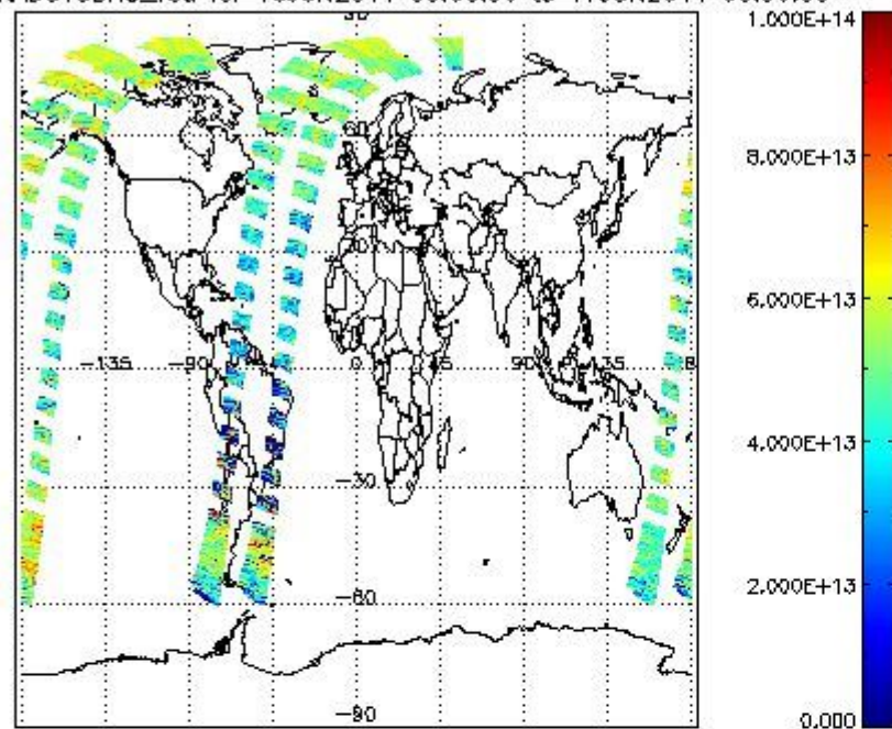
SCIOL2P_NADUV3BRO_vcd for 16JUN2011 00:00:00 to 17JUN2011 00:00:00
