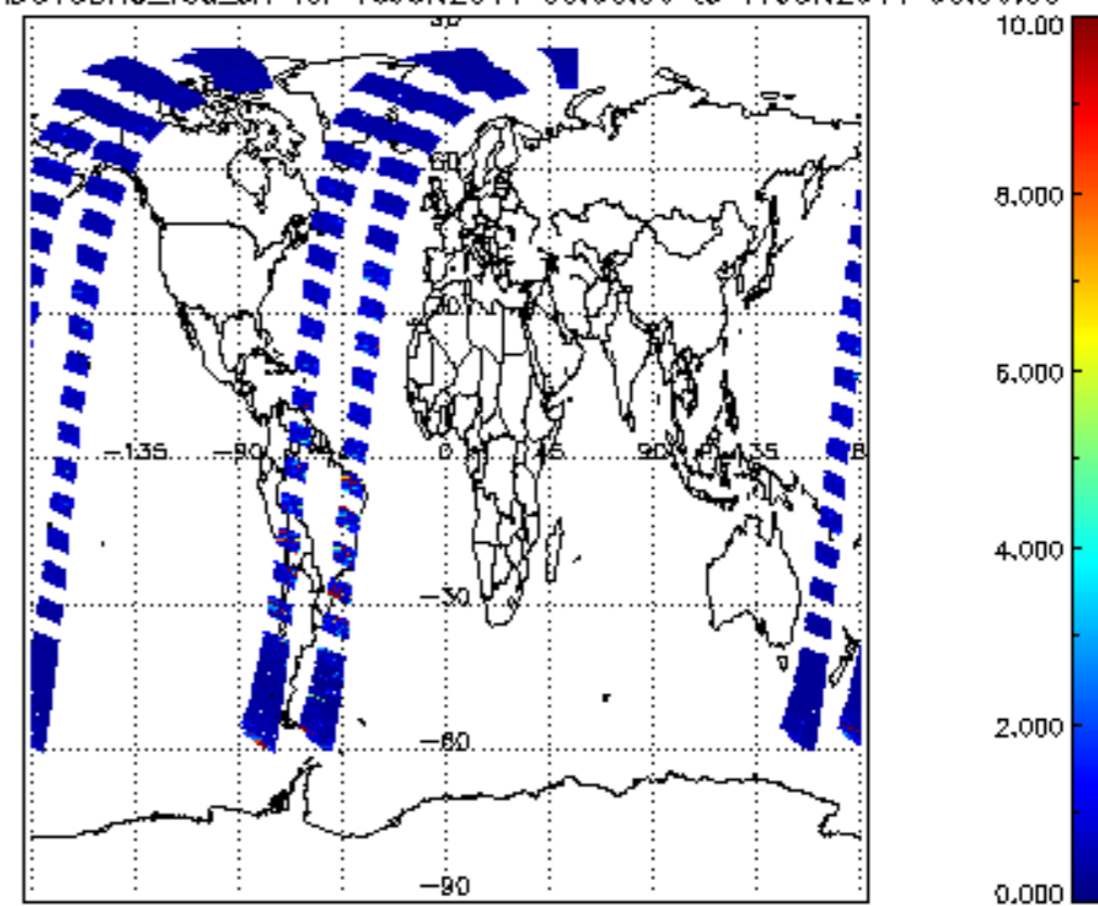
SCIOL2P_NADUV3BRO_vcd_err for 16JUN2011 00:00:00 to 17JUN2011 00:00:00
