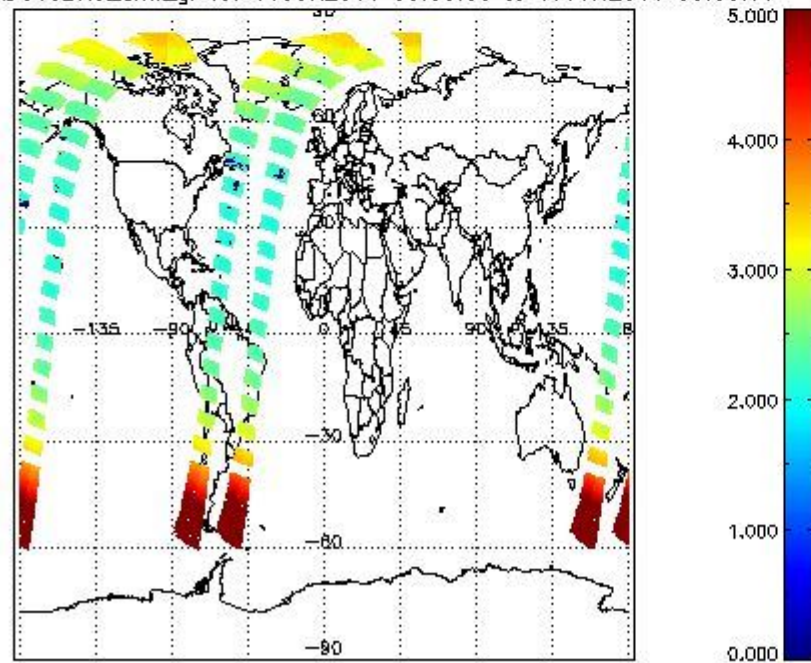
SCIOL2P_NADUV3BRO_amf_gr for 16JUN2011 00:00:00 to 17JUN2011 00:00:00
