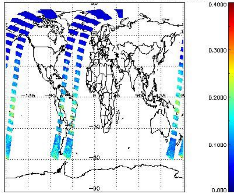
SCIOL2P_NADUV1NO2_vcd_err for 16JUN2011 00:00:00 to 17JUN2011 00:00:00
