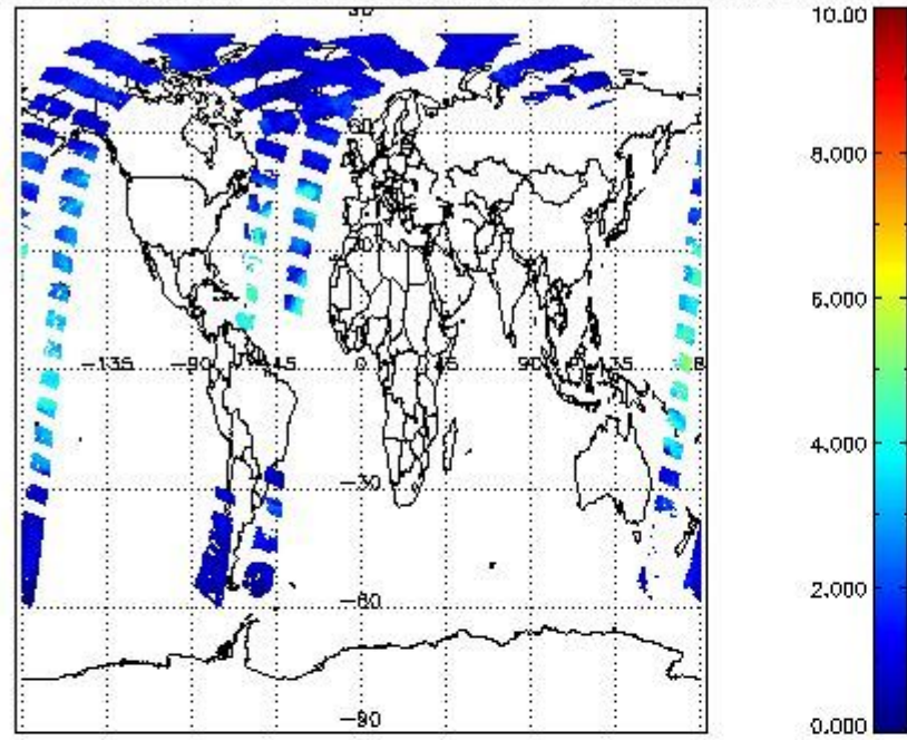
SCIOL2P_NADUV8H2O_vcd for 16JUN2011 00:00:00 to 17JUN2011 00:00:00
