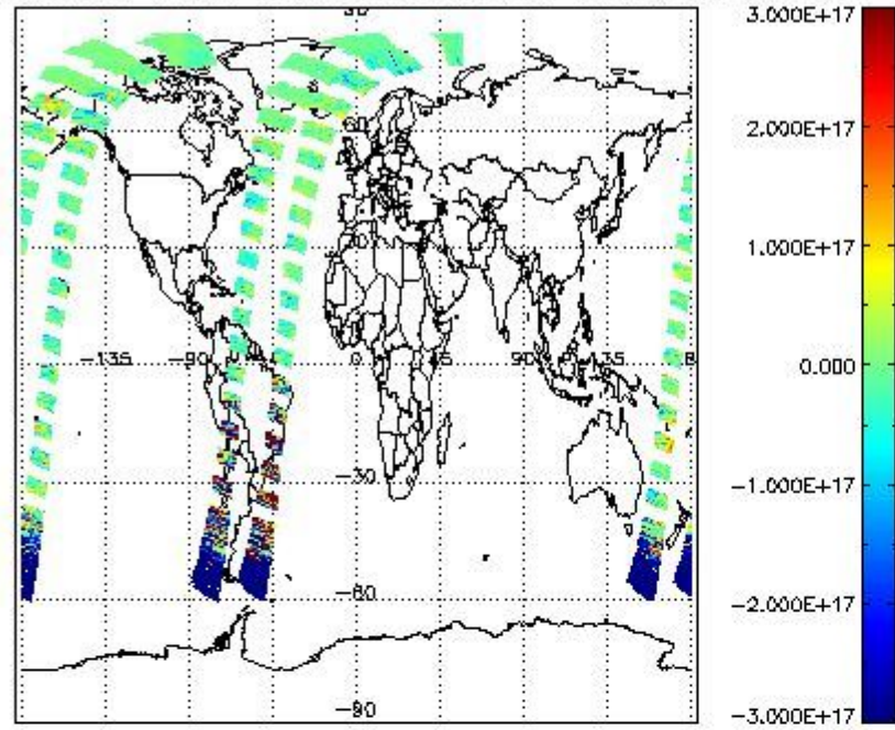
SCIOL2P_NADUV5S02_vcd for 16JUN2011 00:00:00 to 17JUN2011 00:00:00
