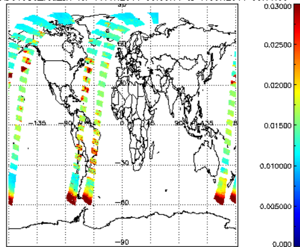
SCIOL2P_NADUV003_vcd_err for 16JUN2011 00:00:00 to 17JUN2011 00:00:00
