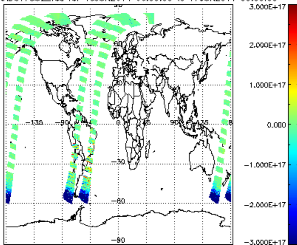
SCIOL2P_NADUV7S02_vcd for 16JUN2011 00:00:00 to 17JUN2011 00:00:00
