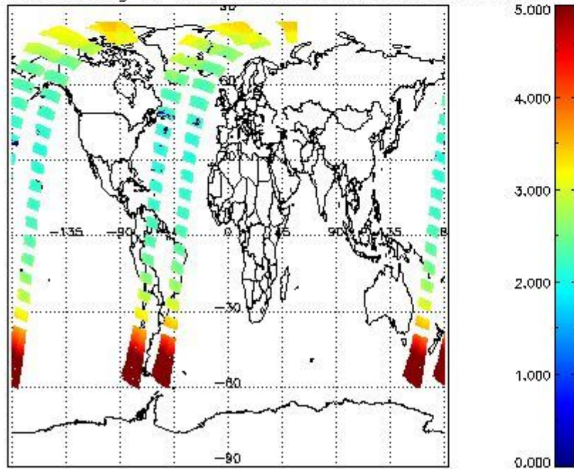
SCIOL2P_NADUV003_amf_gr for 16JUN2011 00:00:00 to 17JUN2011 00:00:00
