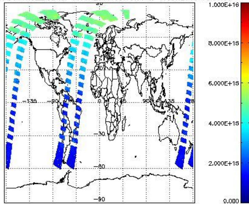
SCIOL2P_NADUV1NO2_vcd for 16JUN2011 00:00:00 to 17JUN2011 00:00:00
