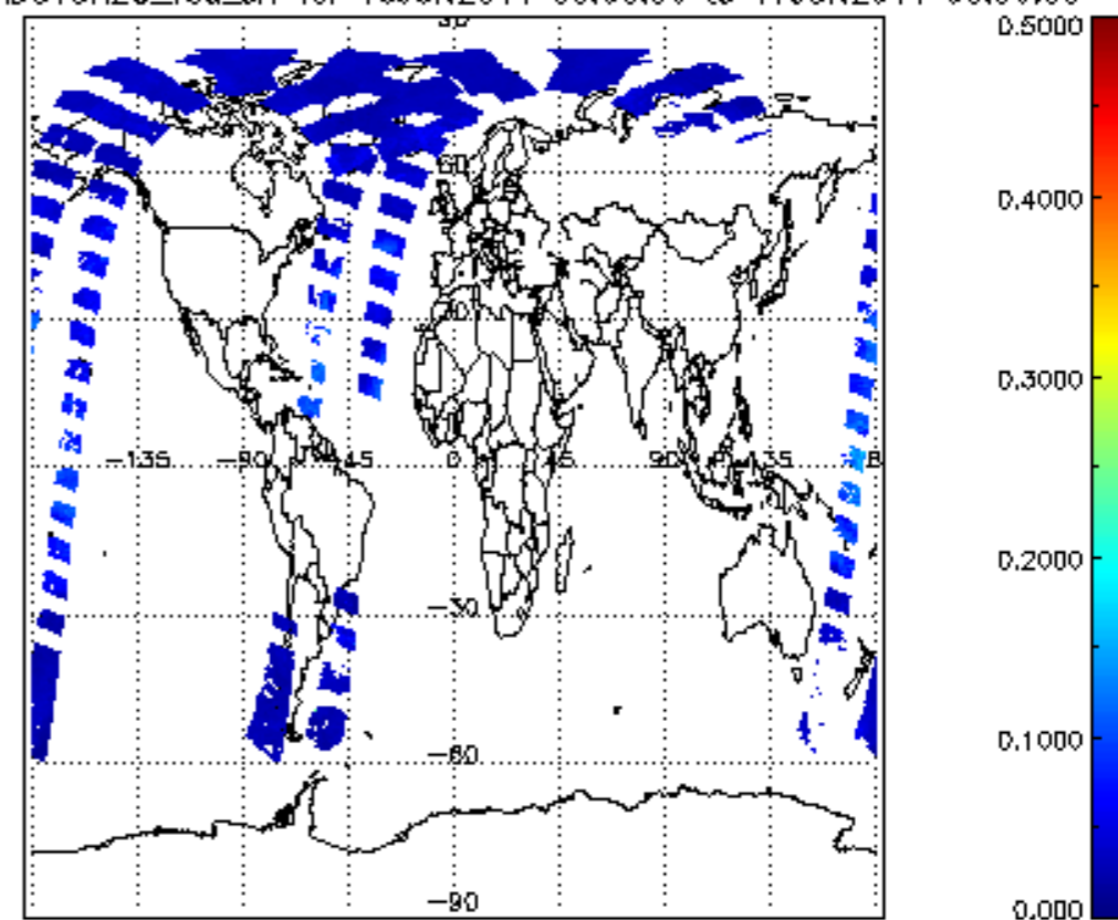
SCIOL2P_NADUV8H2O_vcd_err for 16JUN2011 00:00:00 to 17JUN2011 00:00:00
