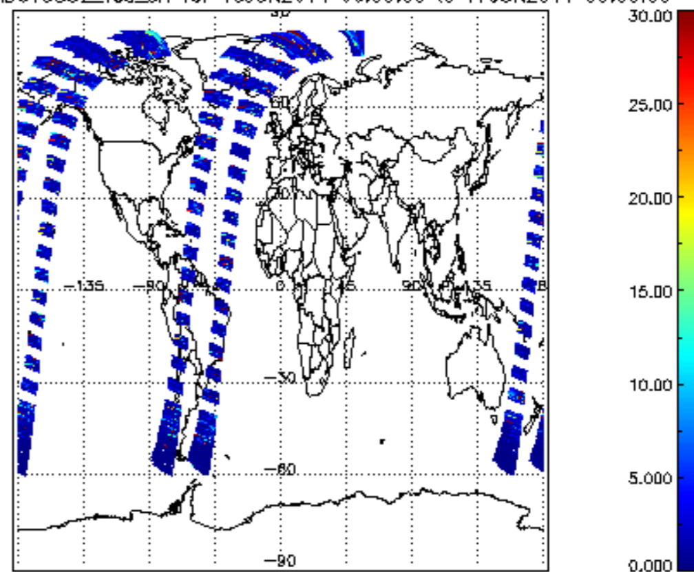
SCIOL2P_NADUV5S02_vcd_err for 16JUN2011 00:00:00 to 17JUN2011 00:00:00
