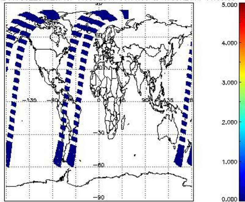
SCIOL2P_NADUV7S02_amf_cl for 16JUN2011 00:00:00 to 17JUN2011 00:00:00
