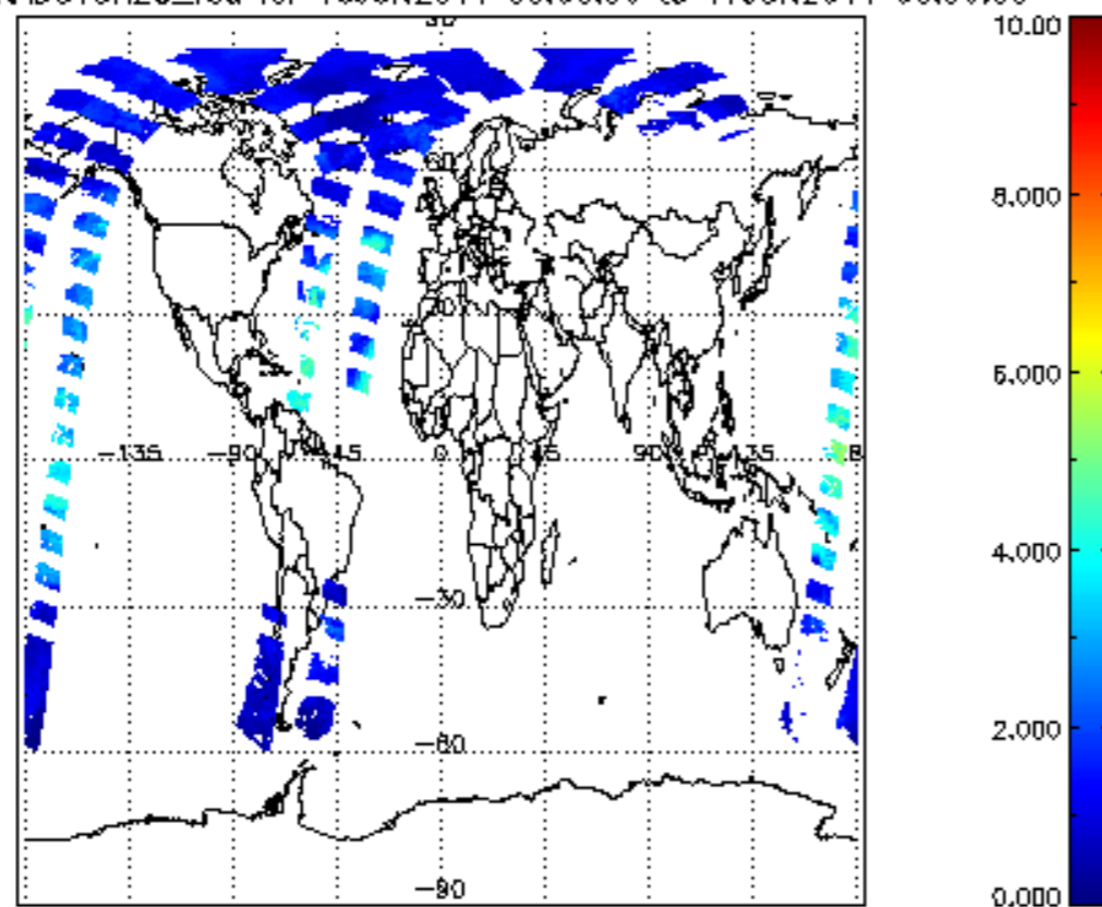
SCIOL2P_NADUV8H2O_vcd for 16JUN2011 00:00:00 to 17JUN2011 00:00:00
