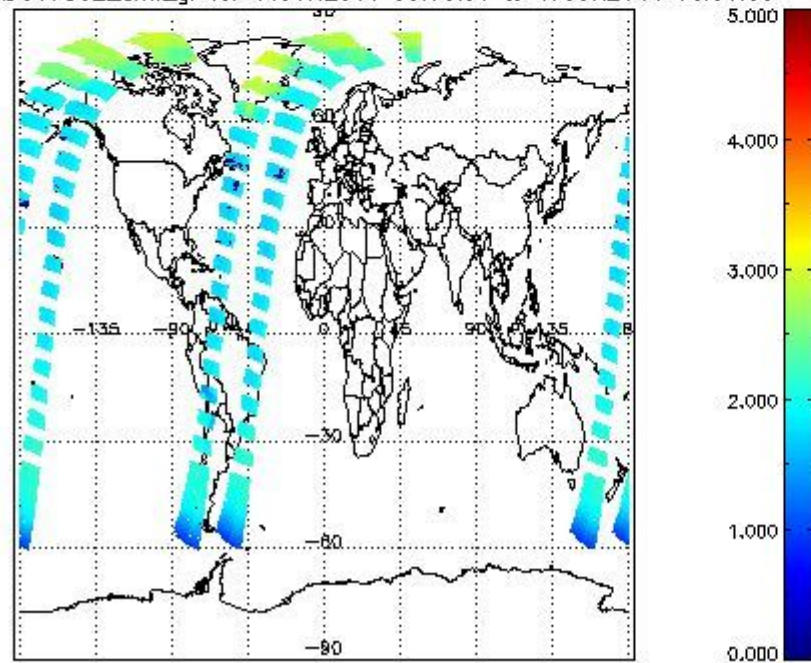
SCIOL2P_NADUV7S02_amf_gr for 16JUN2011 00:00:00 to 17JUN2011 00:00:00
