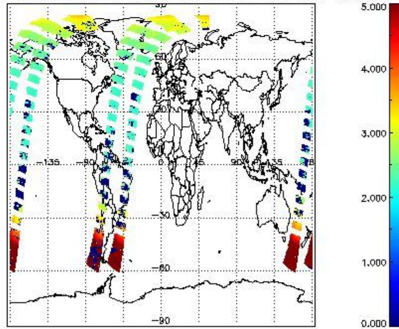
SCIOL2P_NADUV1NO2_amf_cl for 16JUN2011 00:00:00 to 17JUN2011 00:00:00
