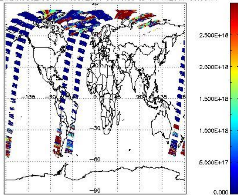
SCIDL2P_NADIR3CO_vcd for 16JUN2011 00:00:00 to 17JUN2011 00:00:00
