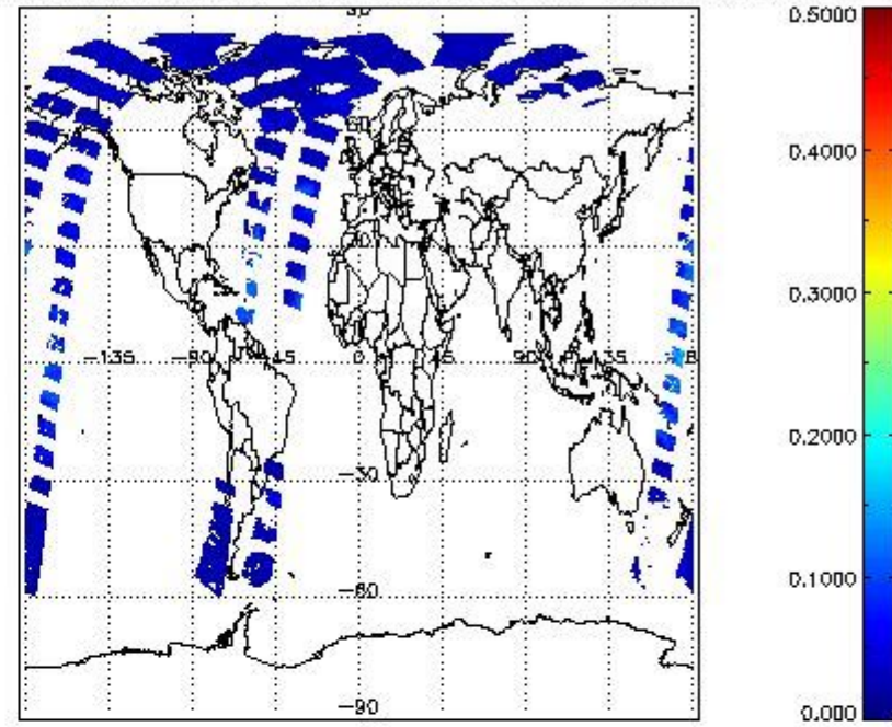
SCIOL2P_NADUV8H2O_vcd_err for 16JUN2011 00:00:00 to 17JUN2011 00:00:00
