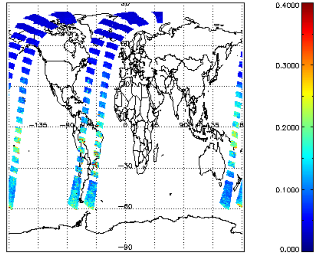
SCIOL2P_NADUV1NO2_vcd_err for 16JUN2011 00:00:00 to 17JUN2011 00:00:00
