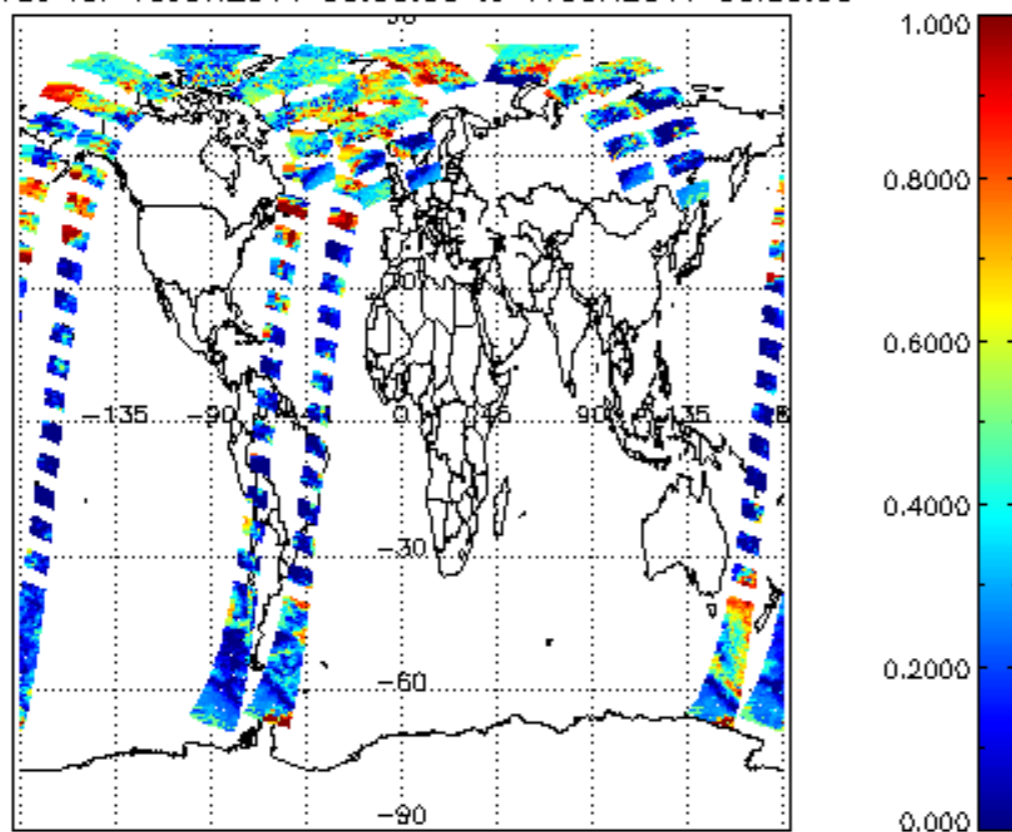
cl_frac for 16JUN2011 00:00:00 to 17JUN2011 00:00:00
