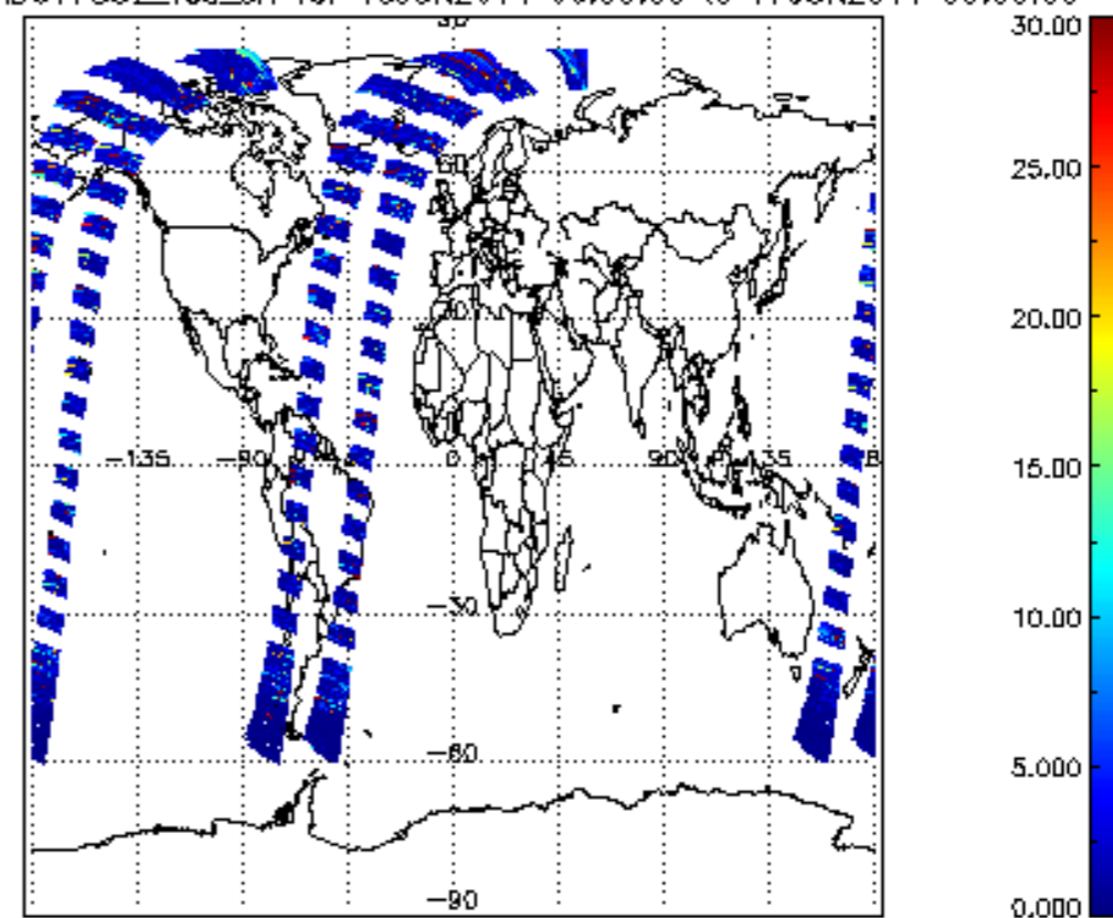
SCIOL2P_NADUV7S02_vcd_err for 16JUN2011 00:00:00 to 17JUN2011 00:00:00
