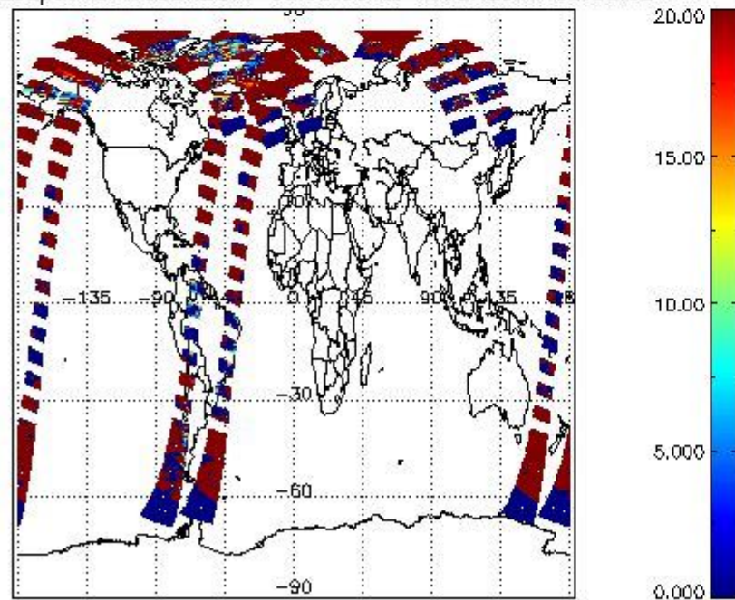
cL_opt_depth for 16JUN2011 00:00:00 to 17JUN2011 00:00:00
