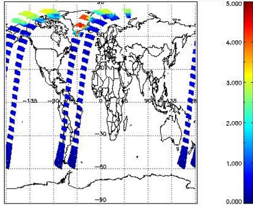
SCIOL2P_NADUV5S02_amf_gr for 16JUN2011 00:00:00 to 17JUN2011 00:00:00
