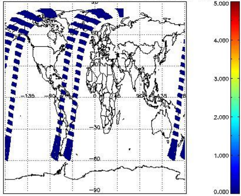
SCIOL2P_NADUV5S02_amf_cl for 16JUN2011 00:00:00 to 17JUN2011 00:00:00
