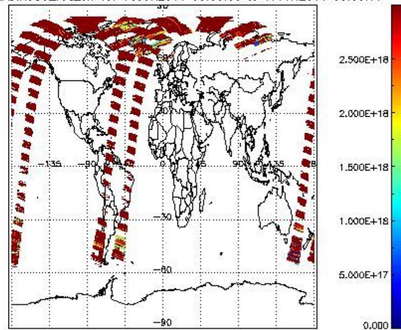
SCIDL2P_NADIR3CO_vcd_err for 16JUN2011 00:00:00 to 17JUN2011 00:00:00
