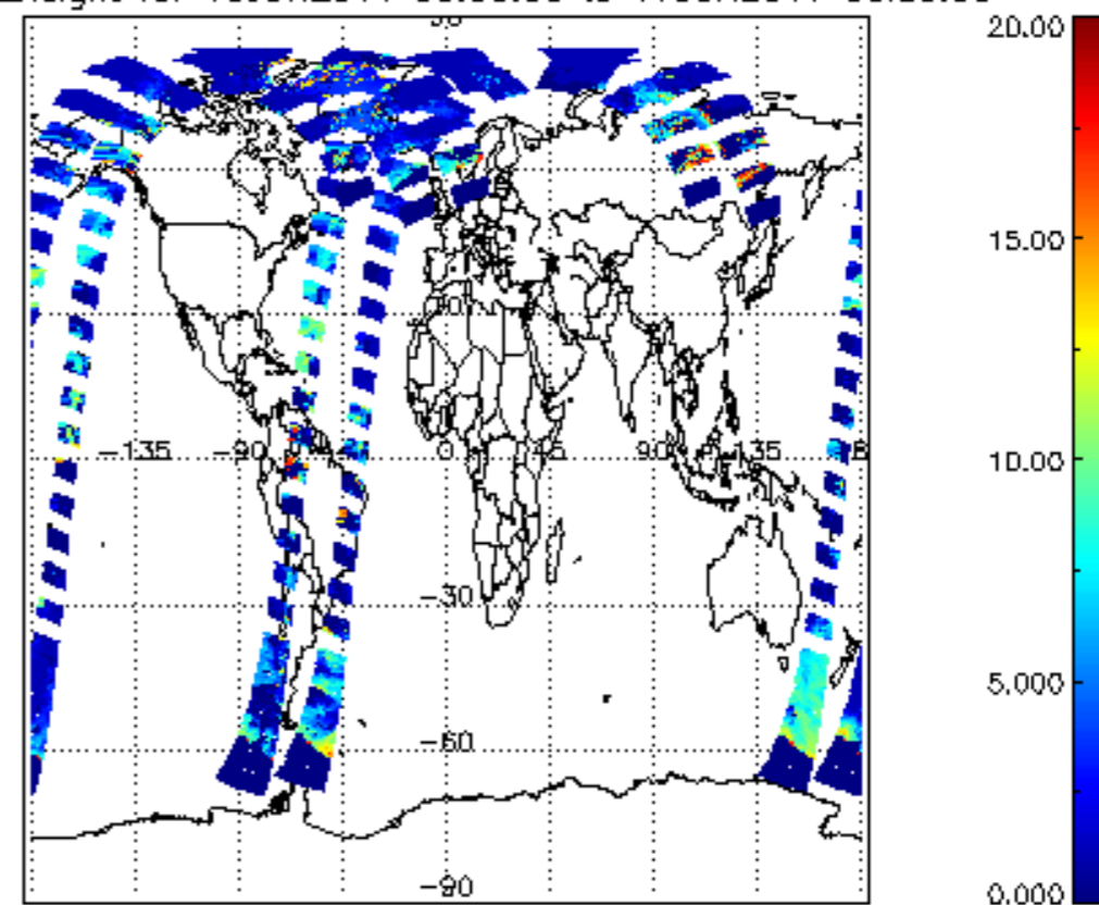
cl_top_height for 16JUN2011 00:00:00 to 17JUN2011 00:00:00
