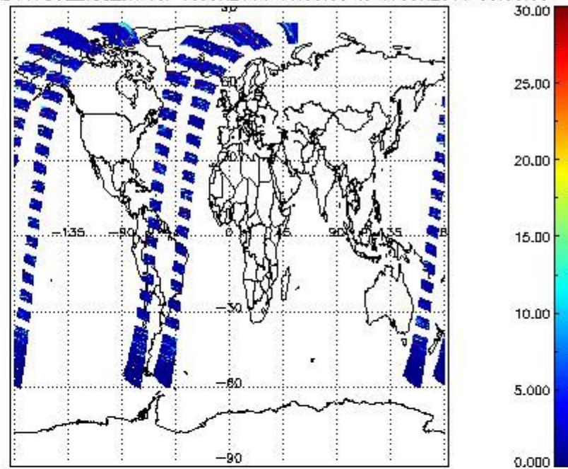
SCIOL2P_NADUV7S02_vcd_err for 16JUN2011 00:00:00 to 17JUN2011 00:00:00
