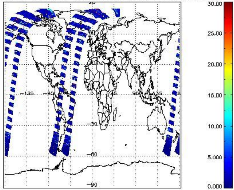
SCIOL2P_NADUV5S02_vcd_err for 16JUN2011 00:00:00 to 17JUN2011 00:00:00
