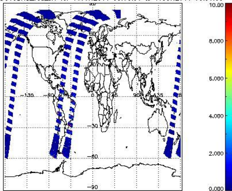
SCIOL2P_NADUV3BRO_vcd_err for 16JUN2011 00:00:00 to 17JUN2011 00:00:00
