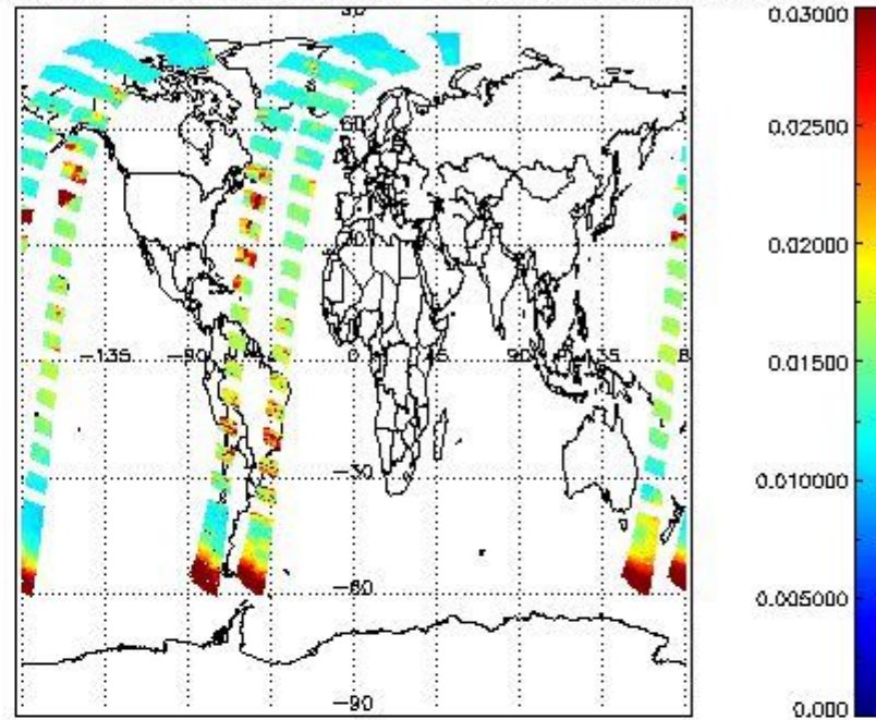
SCIOL2P_NADUV003_vcd_err for 16JUN2011 00:00:00 to 17JUN2011 00:00:00
