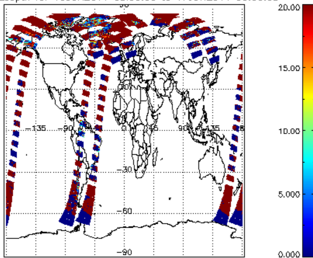
cl_opt_depth for 16JUN2011 00:00:00 to 17JUN2011 00:00:00
