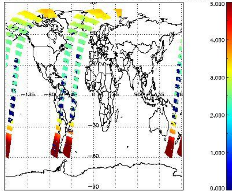
SCIOL2P_NADUV003_amf_cl for 16JUN2011 00:00:00 to 17JUN2011 00:00:00
