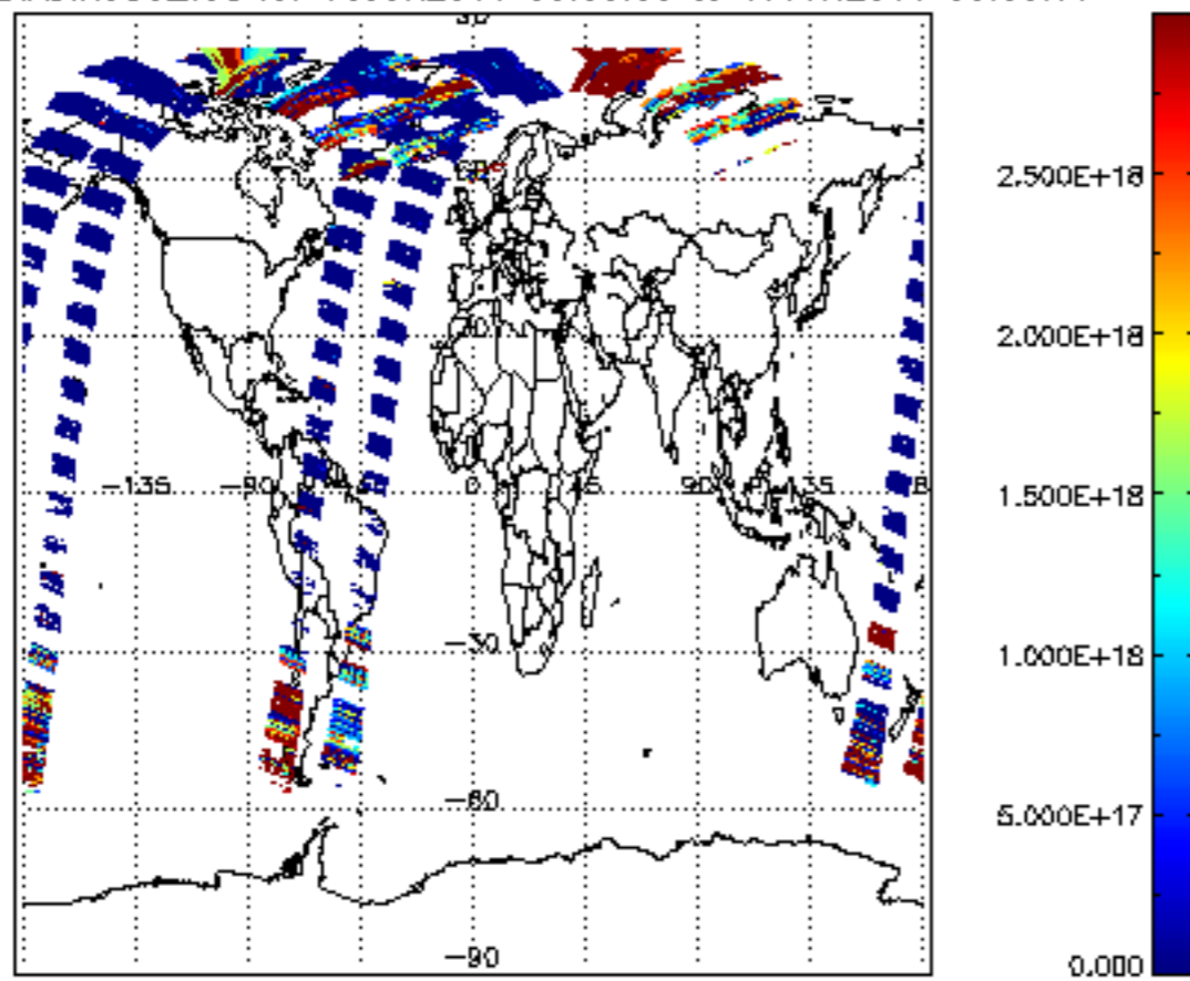
SCIOL2P_NADIR3CO_vcd for 16JUN2011 00:00:00 to 17JUN2011 00:00:00
