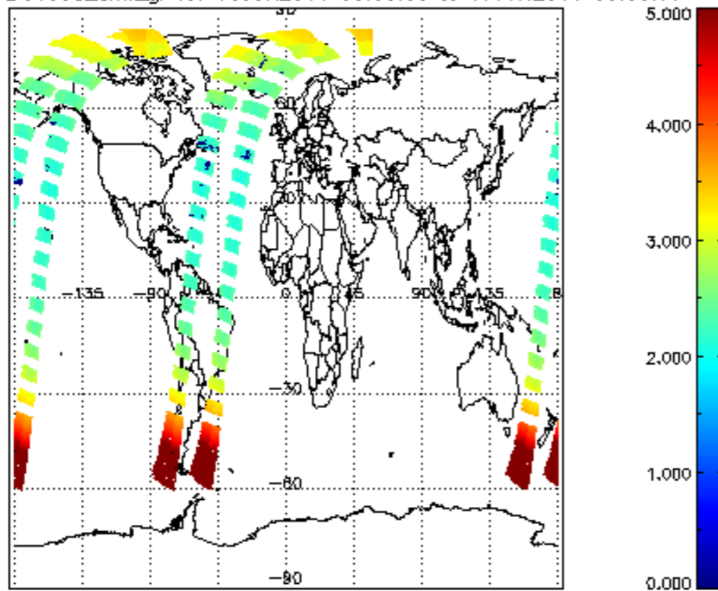
SCIOL2P_NADUV003_amf_gr for 16JUN2011 00:00:00 to 17JUN2011 00:00:00
