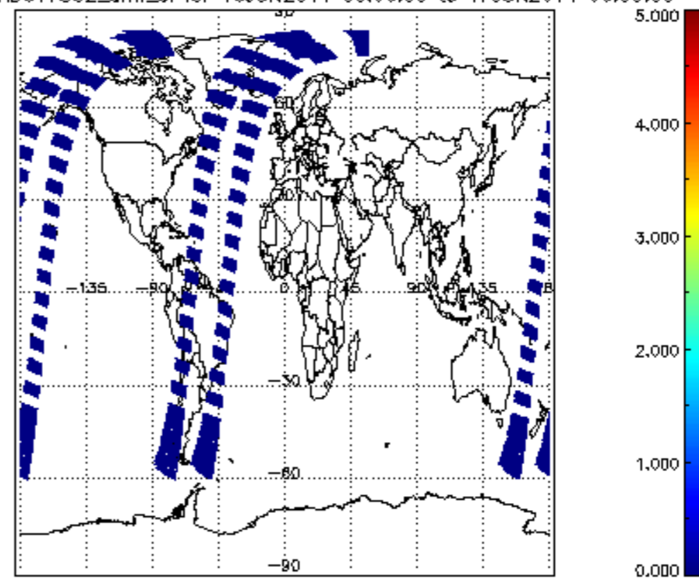
SCIOL2P_NADUV7S02_amf_cl for 16JUN2011 00:00:00 to 17JUN2011 00:00:00
