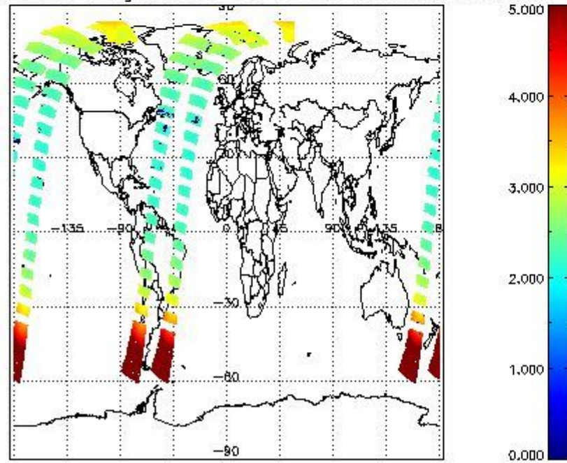
SCIOL2P_NADUV1NO2_amf_gr for 16JUN2011 00:00:00 to 17JUN2011 00:00:00
