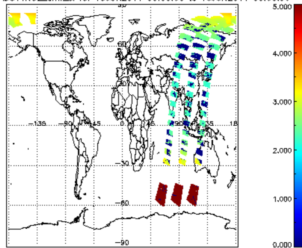
SCIOL2P_NADUV1NO2_amf_cl for 15JUN2011 00:00:00 to 16JUN2011 00:00:00
