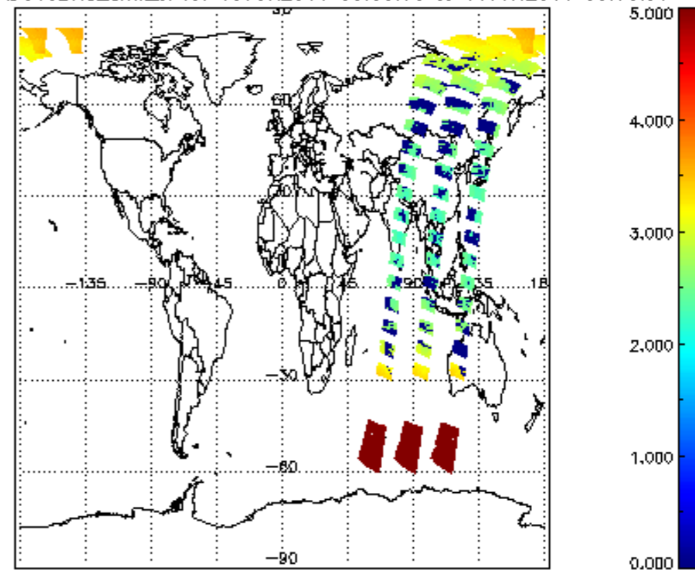
SCIOL2P_NADUV3BRO_amf_cl for 15JUN2011 00:00:00 to 16JUN2011 00:00:00
