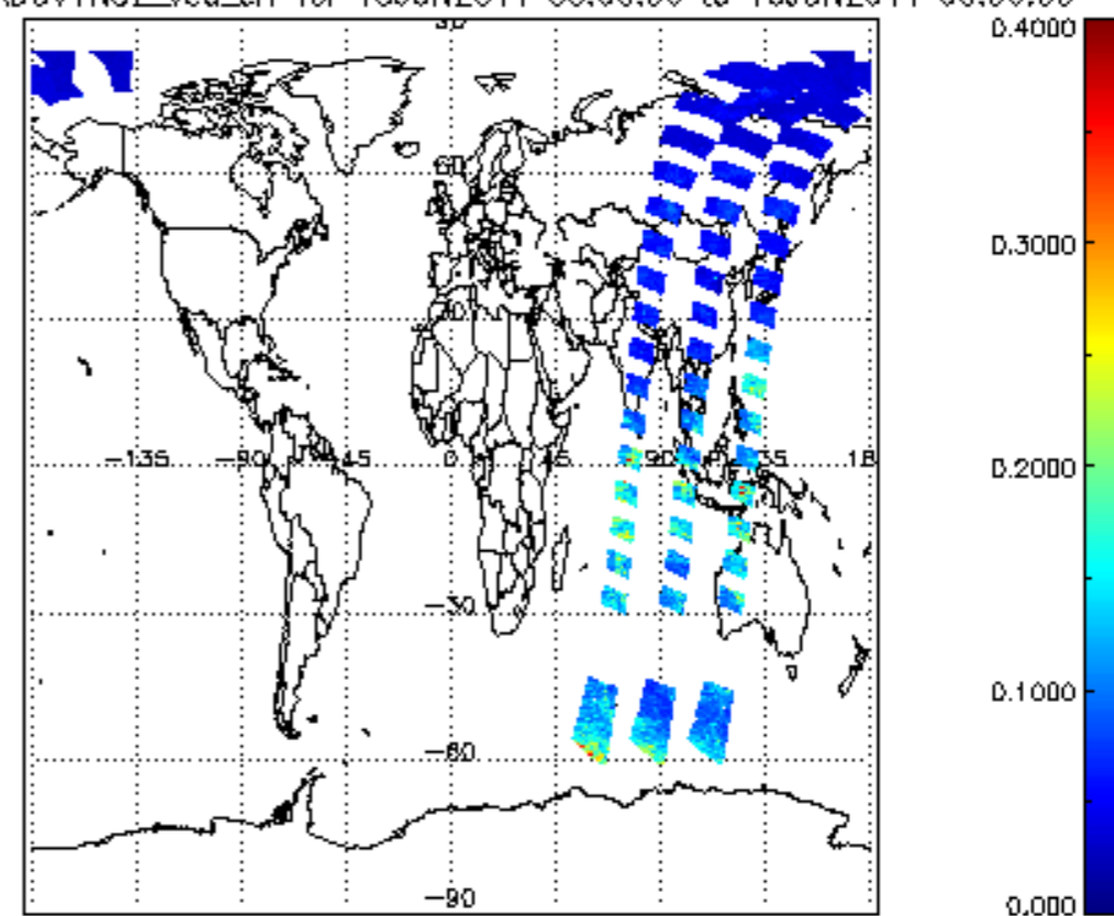
SCIOL2P_NADUV1NO2_vcd_err for 15JUN2011 00:00:00 to 16JUN2011 00:00:00
