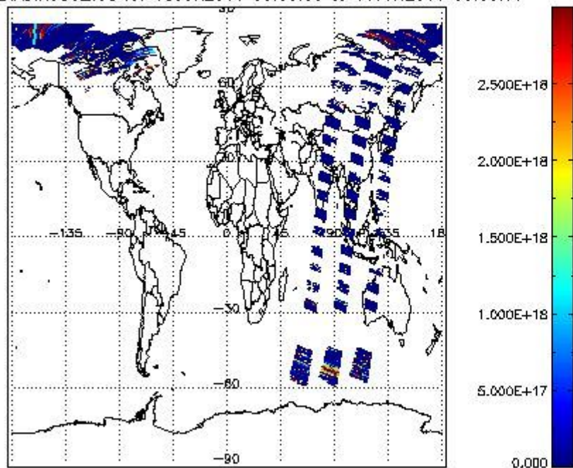
SCIDL2P_NADIR3CO_vcd for 15JUN2011 00:00:00 to 16JUN2011 00:00:00
