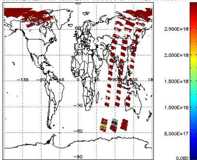
SCIDL2P_NADIR3CO_vcd_err for 15JUN2011 00:00:00 to 16JUN2011 00:00:00
