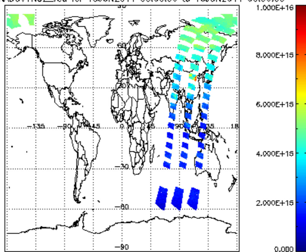
SCIOL2P_NADUV1NO2_vcd for 15JUN2011 00:00:00 to 16JUN2011 00:00:00
