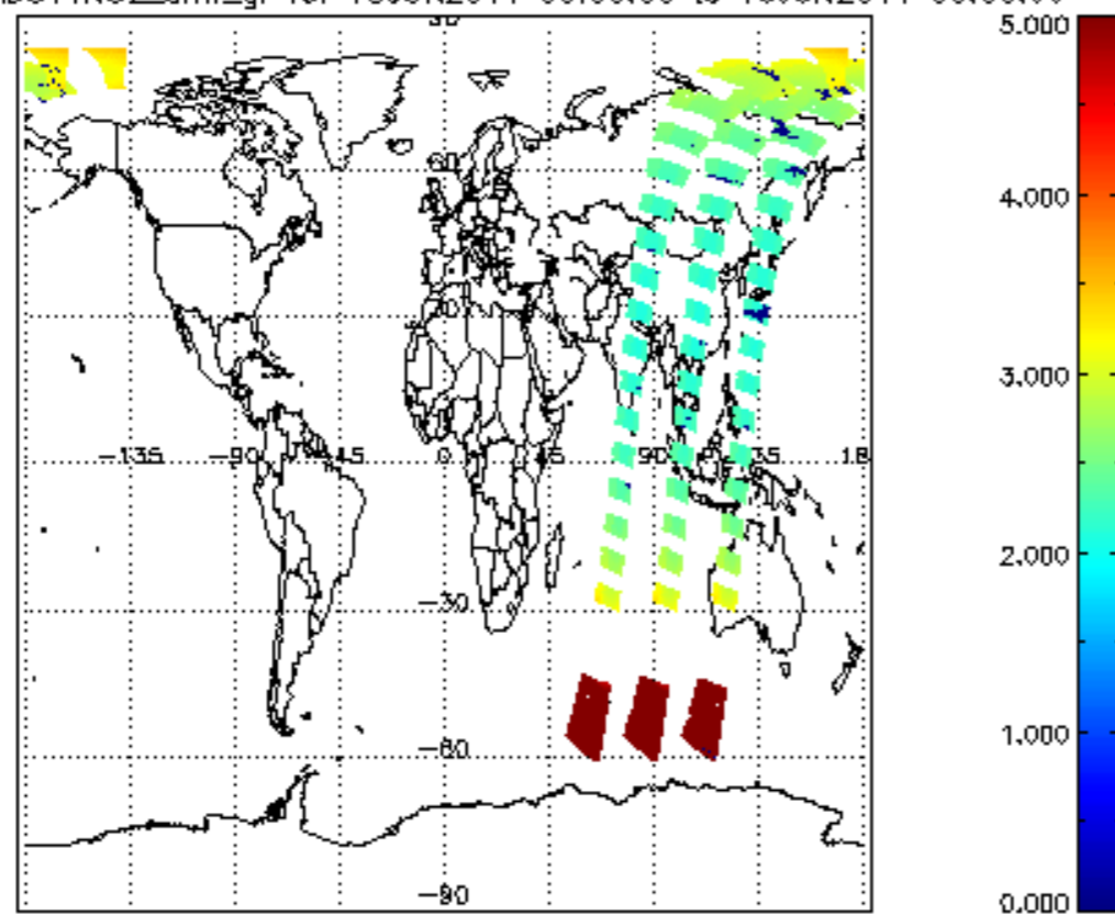
SCIOL2P_NADUV1NO2_amf_gr for 15JUN2011 00:00:00 to 16JUN2011 00:00:00
