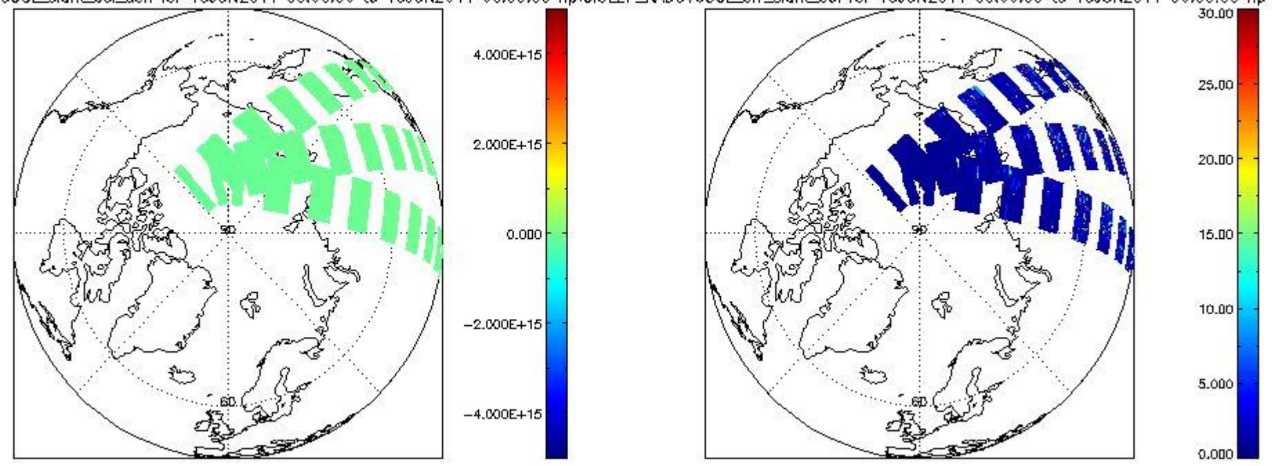
CIOL2P_NADUV60CLslant_col_den for 15JUN2011 00:00:00 to 16JUN2011 00:00:00 np; CIOL2P_NADUV60CLerr_slant_col for 15JUN2011 00:00:00 to 16JUN2011 00:00:00 np
