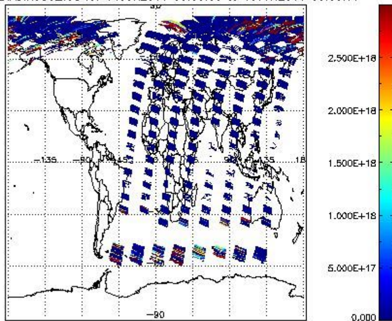
SCIDL2P_NADIR3CO_vcd for 14JUN2011 00:00:00 to 15JUN2011 00:00:00
