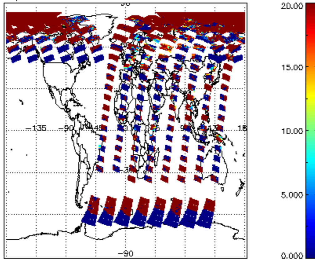
cl_opt_depth for 14JUN2011 00:00:00 to 15JUN2011 00:00:00
