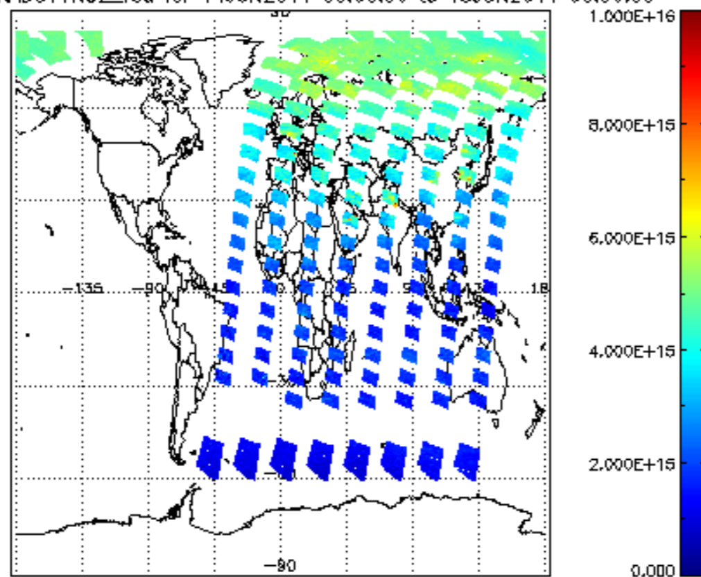
SCIOL2P_NADUV1NO2_vcd for 14JUN2011 00:00:00 to 15JUN2011 00:00:00
