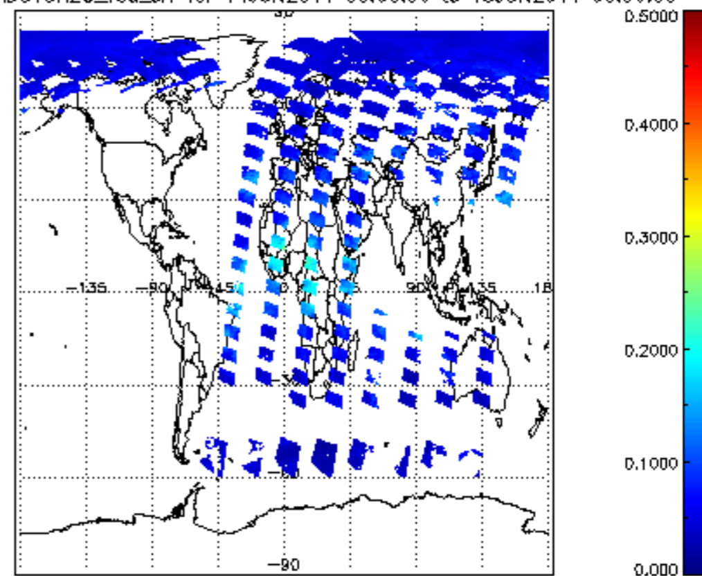
SCIOL2P_NADUV8H2O_vcd_err for 14JUN2011 00:00:00 to 15JUN2011 00:00:00
