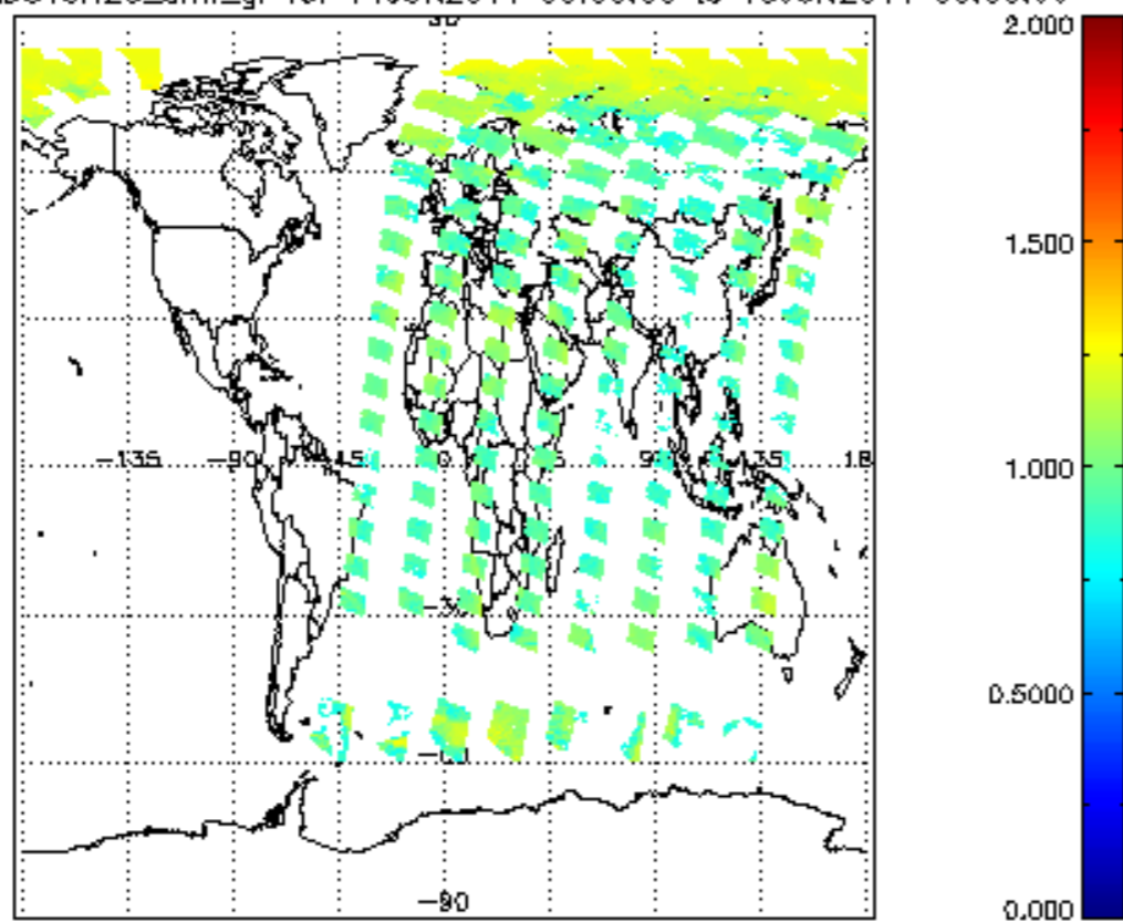
SCIOL2P_NADUV8H2O_amf_gr for 14JUN2011 00:00:00 to 15JUN2011 00:00:00
