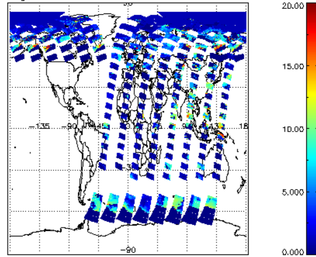
cl_top_height for 14JUN2011 00:00:00 to 15JUN2011 00:00:00
