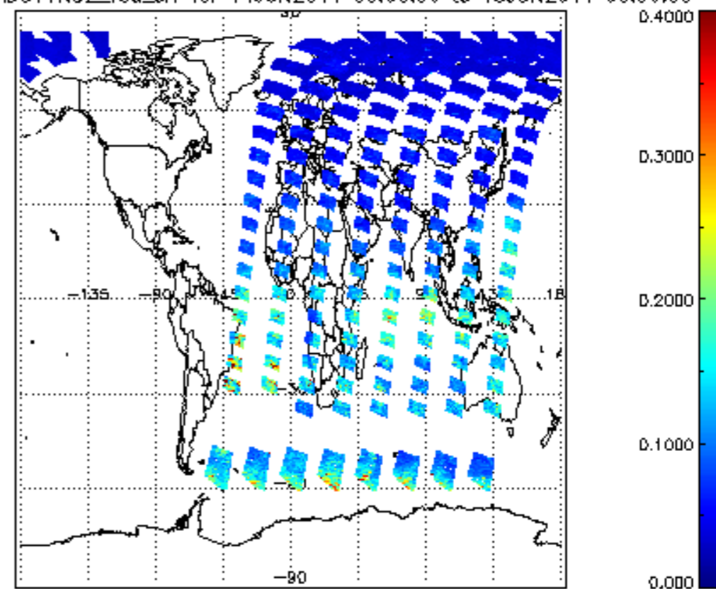
SCIOL2P_NADUV1NO2_vcd_err for 14JUN2011 00:00:00 to 15JUN2011 00:00:00
