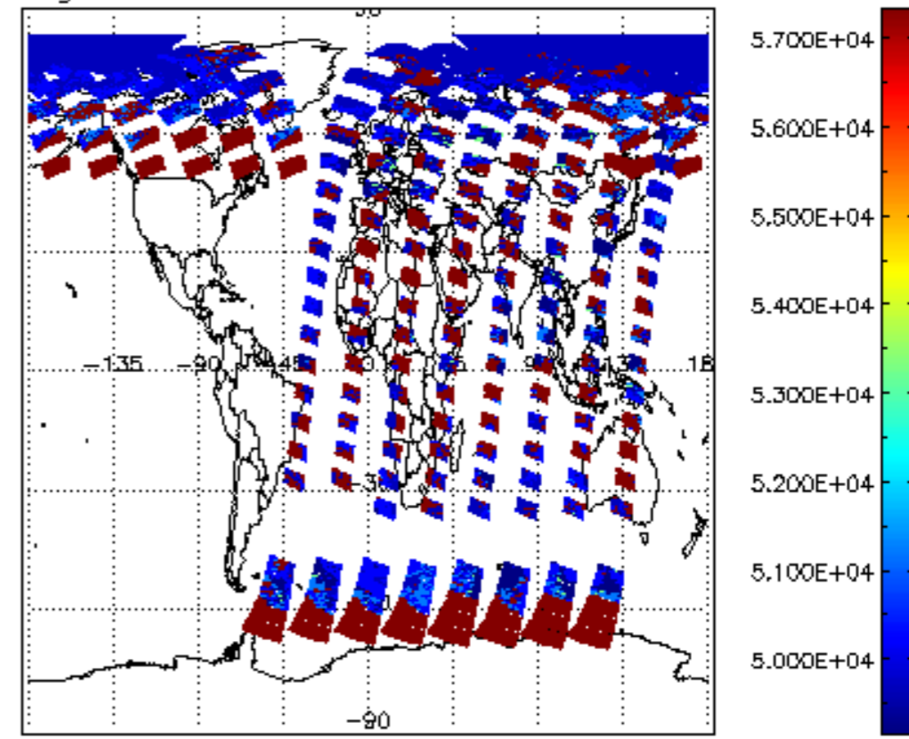
cloud_flags for 14JUN2011 00:00:00 to 15JUN2011 00:00:00
