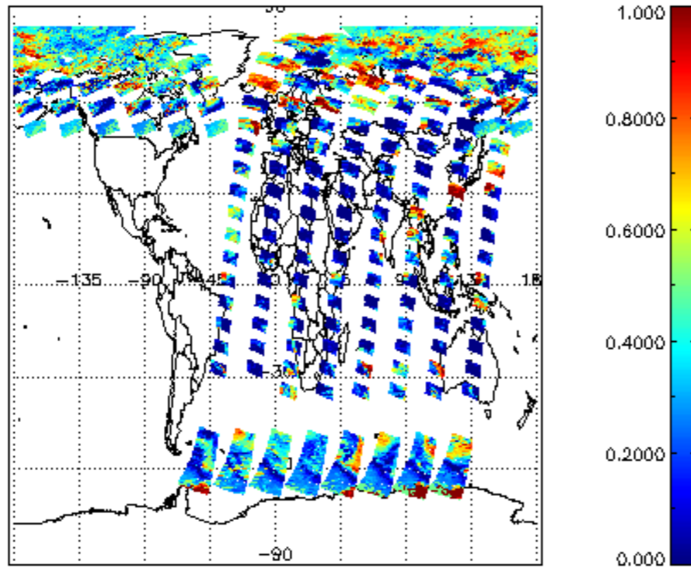
cl_frac for 14JUN2011 00:00:00 to 15JUN2011 00:00:00
