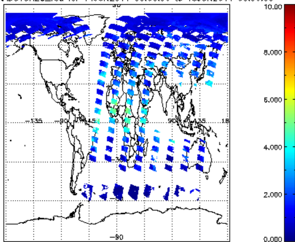
SCIOL2P_NADUV8H2O_vcd for 14JUN2011 00:00:00 to 15JUN2011 00:00:00
