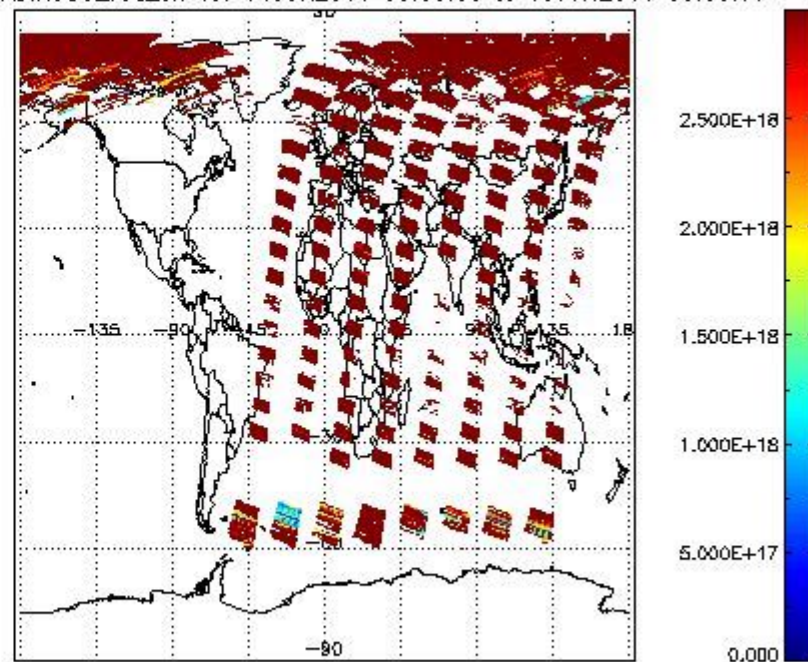
SCIDL2P_NADIR3CO_vcd_err for 14JUN2011 00:00:00 to 15JUN2011 00:00:00
