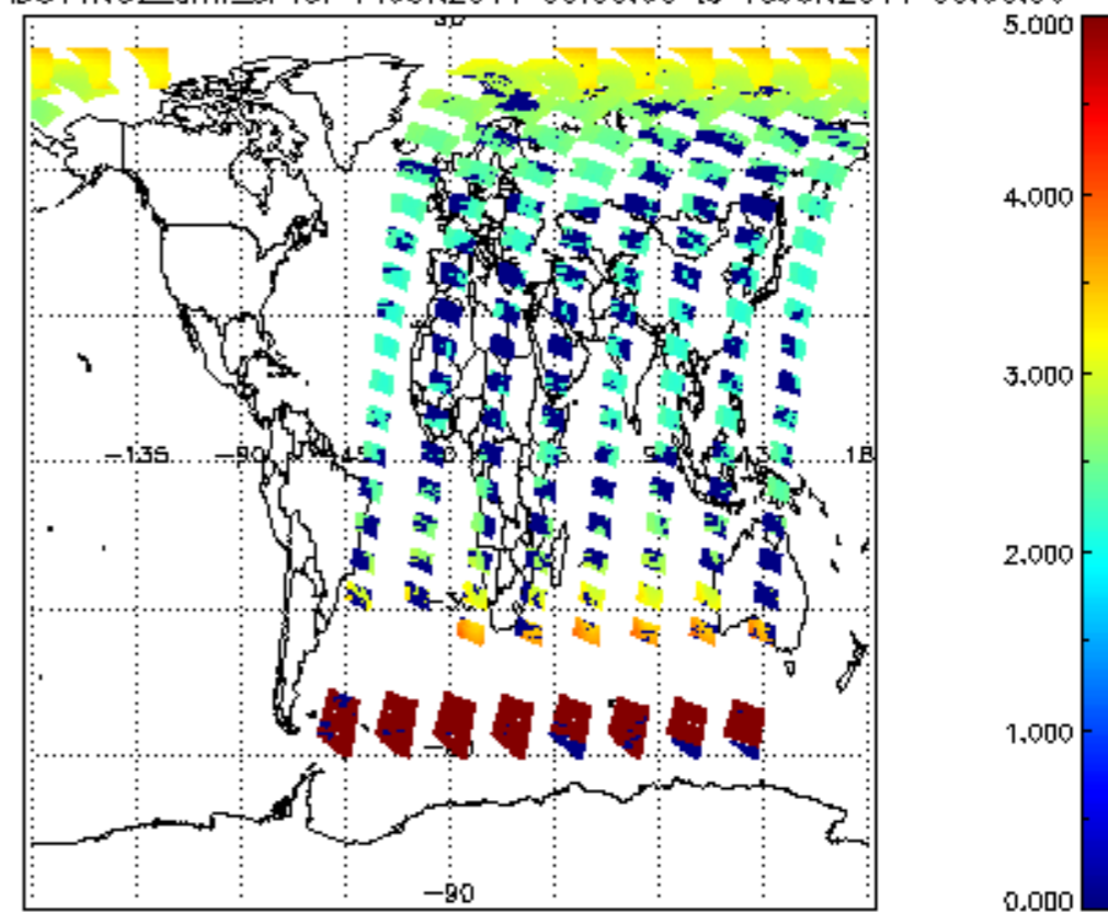
SCIOL2P_NADUV1NO2_amf_sl for 14JUN2011 00:00:00 to 15JUN2011 00:00:00
