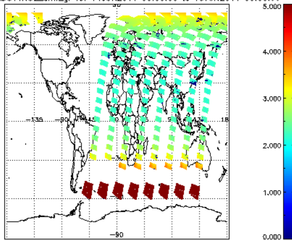
SCIOL2P_NADUV1NO2_amf_gr for 14JUN2011 00:00:00 to 15JUN2011 00:00:00
