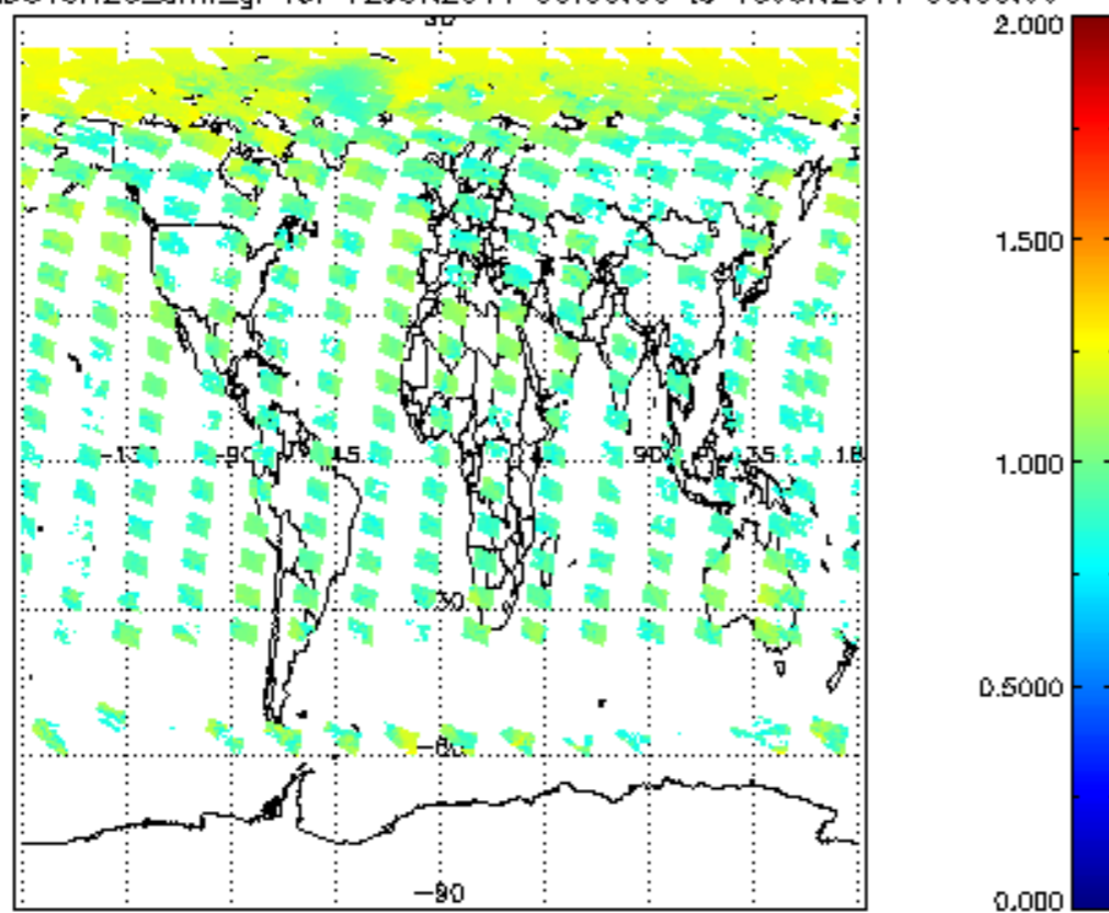
SCIOL2P_NADUV8H2O_amf_gr for 12JUN2011 00:00:00 to 13JUN2011 00:00:00
