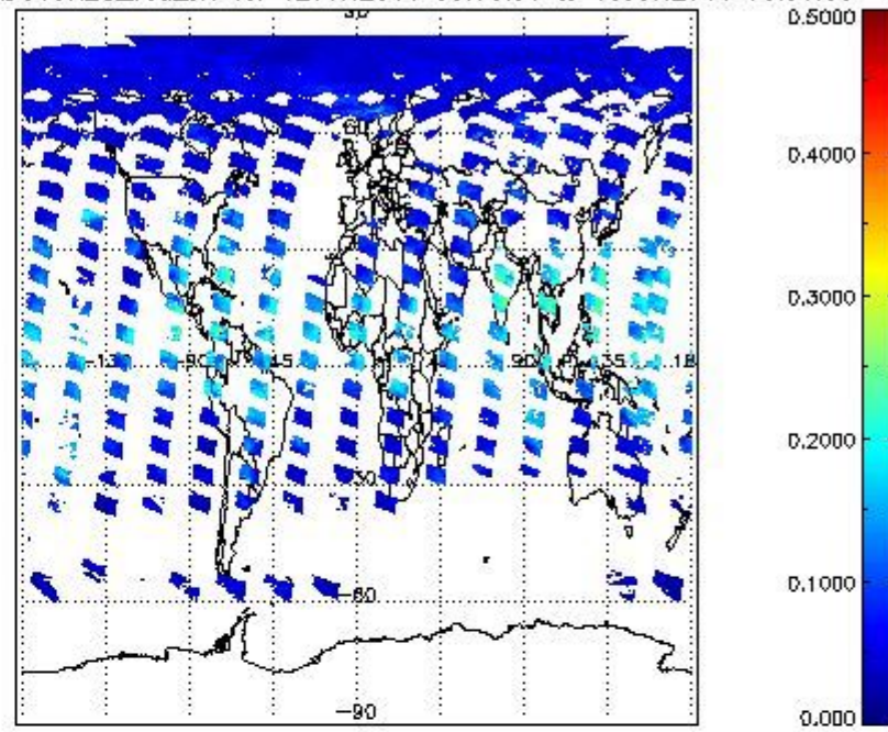
SCIOL2P_NADUV8H2O_vcd_err for 12JUN2011 00:00:00 to 13JUN2011 00:00:00
