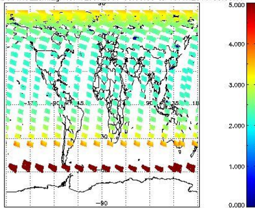
SCIOL2P_NADUV1NO2_amf_gr for 12JUN2011 00:00:00 to 13JUN2011 00:00:00
