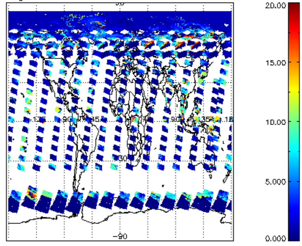
cl_top_height for 12JUN2011 00:00:00 to 13JUN2011 00:00:00
