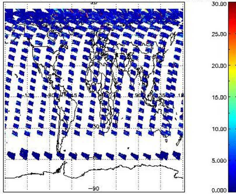
SCIOL2P_NADUV7S02_vcd_err for 12JUN2011 00:00:00 to 13JUN2011 00:00:00
