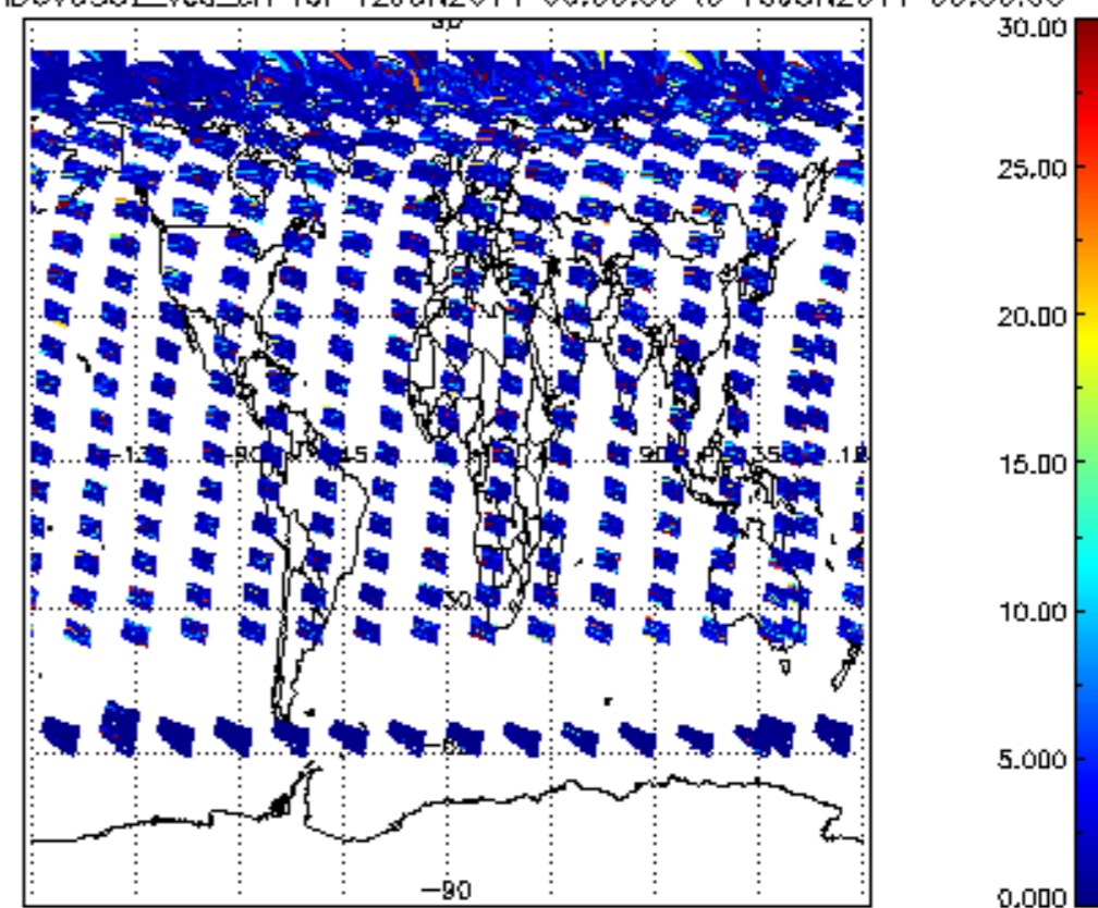
SCIOL2P_NADUV5S02_vcd_err for 12JUN2011 00:00:00 to 13JUN2011 00:00:00
