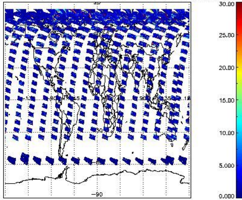
SCIOL2P_NADUV5S02_vcd_err for 12JUN2011 00:00:00 to 13JUN2011 00:00:00
