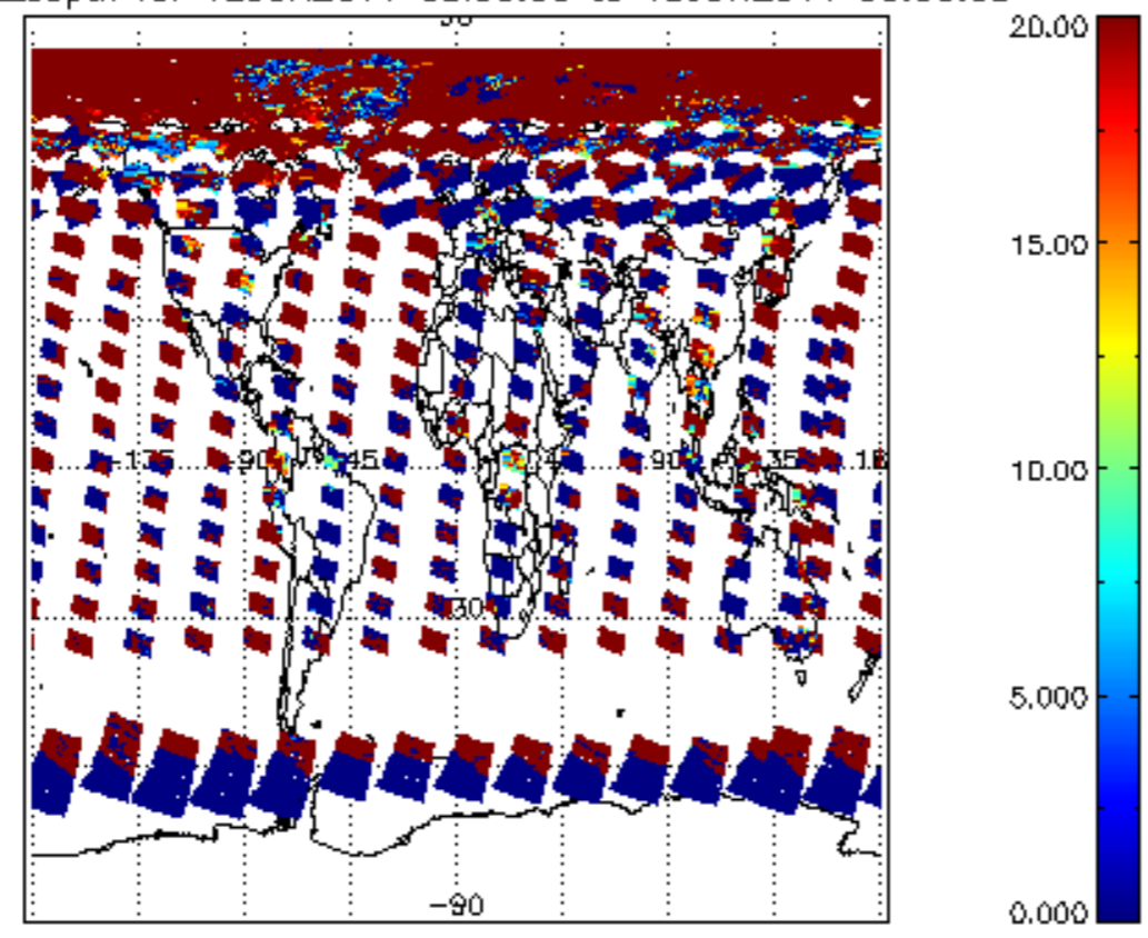
cl_opt_depth for 12JUN2011 00:00:00 to 13JUN2011 00:00:00
