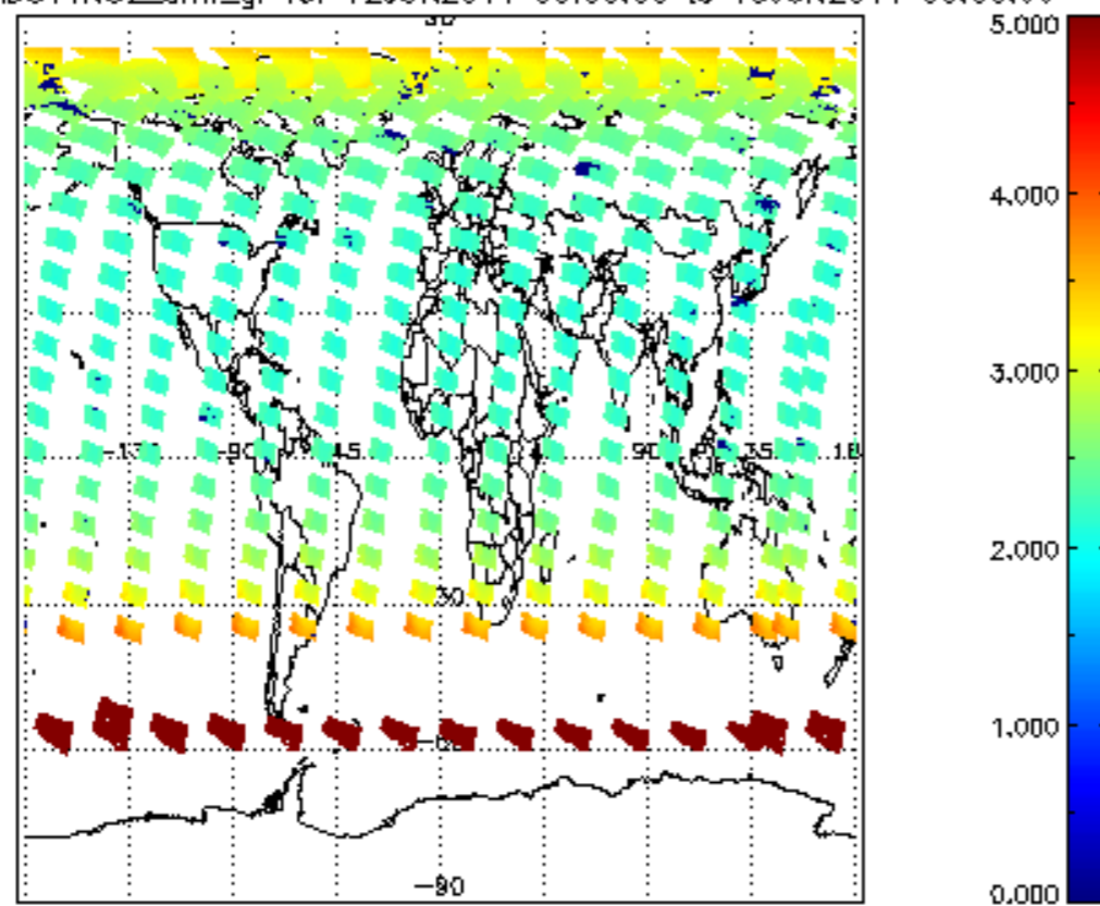
SCIOL2P_NADUV1NO2_amf_gr for 12JUN2011 00:00:00 to 13JUN2011 00:00:00
