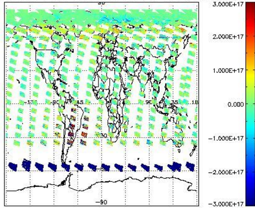
SCIOL2P_NADUV5S02_vcd for 12JUN2011 00:00:00 to 13JUN2011 00:00:00
