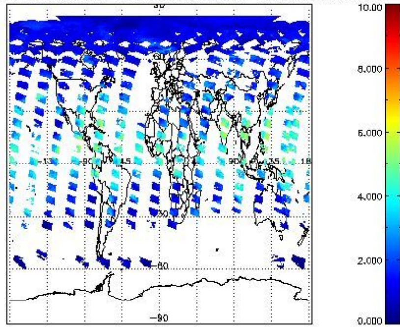
SCIOL2P_NADUV8H2O_vcd for 12JUN2011 00:00:00 to 13JUN2011 00:00:00
