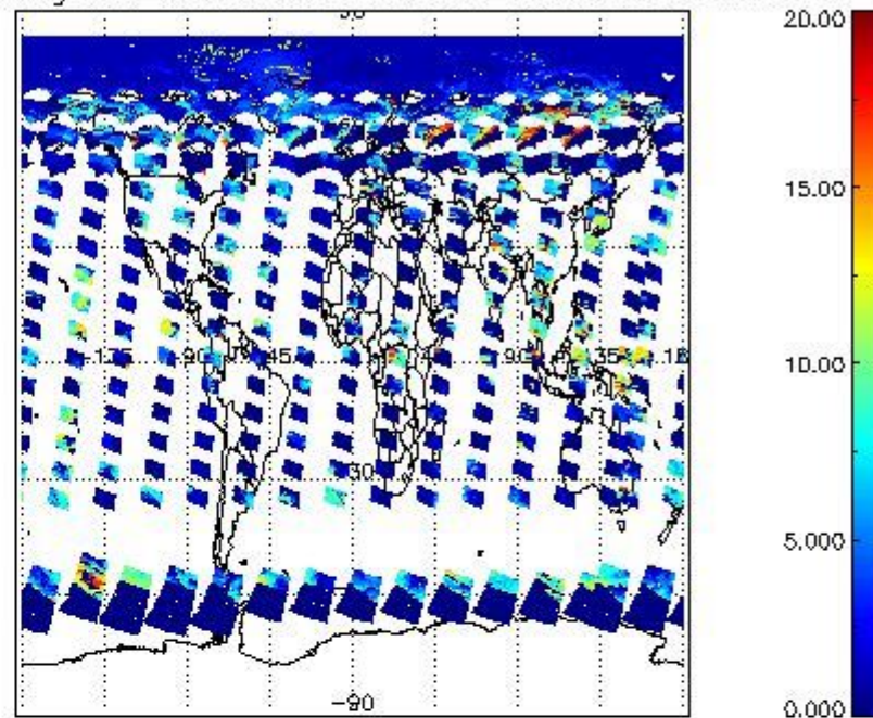
cL_top_height for 12JUN2011 00:00:00 to 13JUN2011 00:00:00
