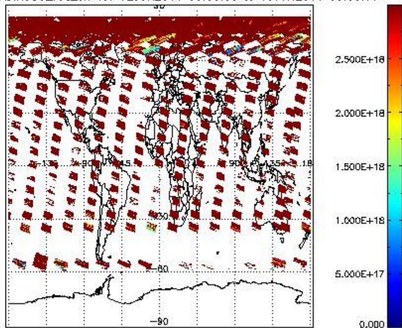
SCIDL2P_NADIR3CO_vcd_err for 12JUN2011 00:00:00 to 13JUN2011 00:00:00
