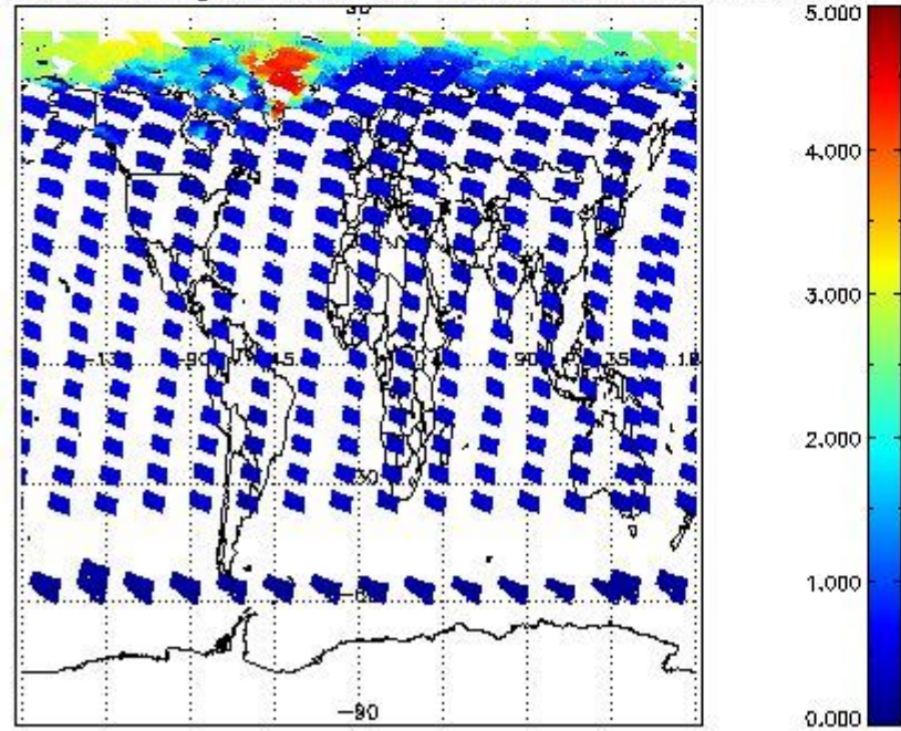
SCIOL2P_NADUV5S02_amf_gr for 12JUN2011 00:00:00 to 13JUN2011 00:00:00
