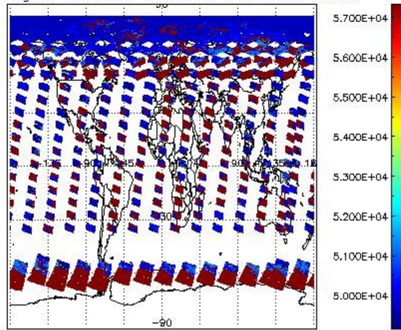
cloud_flags for 12JUN2011 00:00:00 to 13JUN2011 00:00:00
