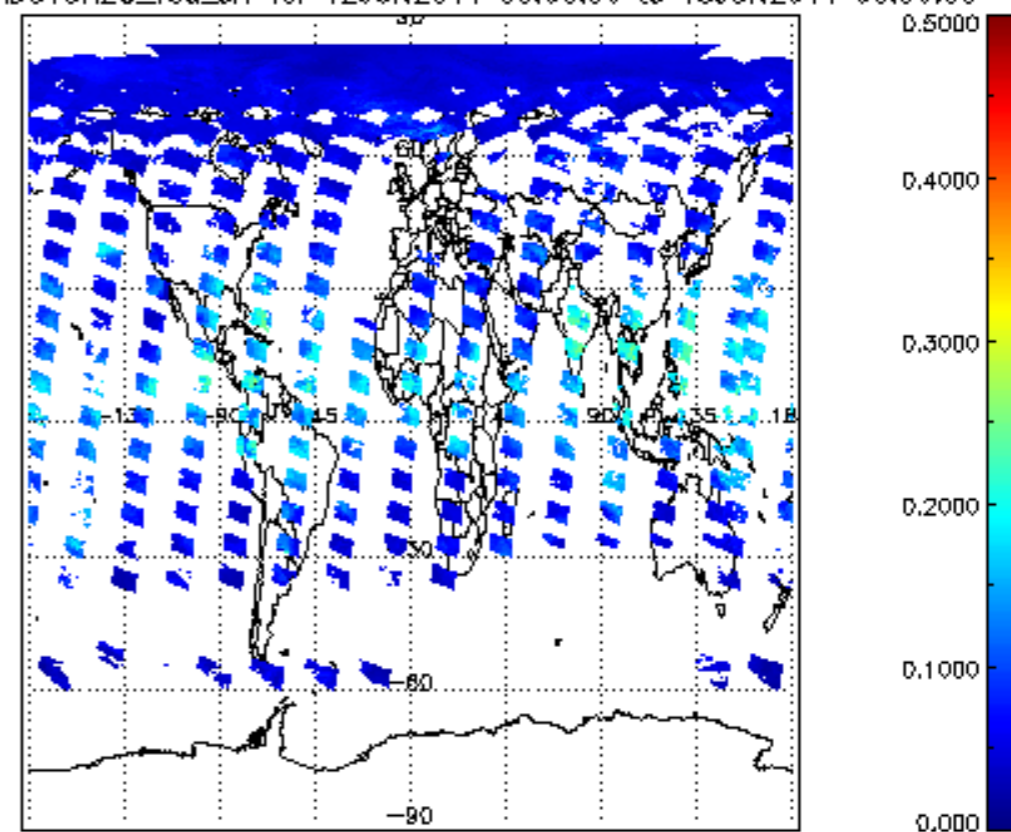
SCIOL2P_NADUV8H2O_vcd_err for 12JUN2011 00:00:00 to 13JUN2011 00:00:00
