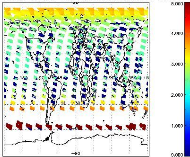
SCIOL2P_NADUV3BRO_amf_cl for 12JUN2011 00:00:00 to 13JUN2011 00:00:00
