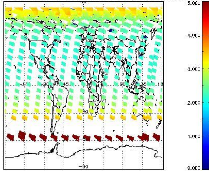
SCIOL2P_NADUV003_amf_gr for 12JUN2011 00:00:00 to 13JUN2011 00:00:00
