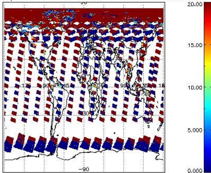
cL_opt_depth for 12JUN2011 00:00:00 to 13JUN2011 00:00:00
