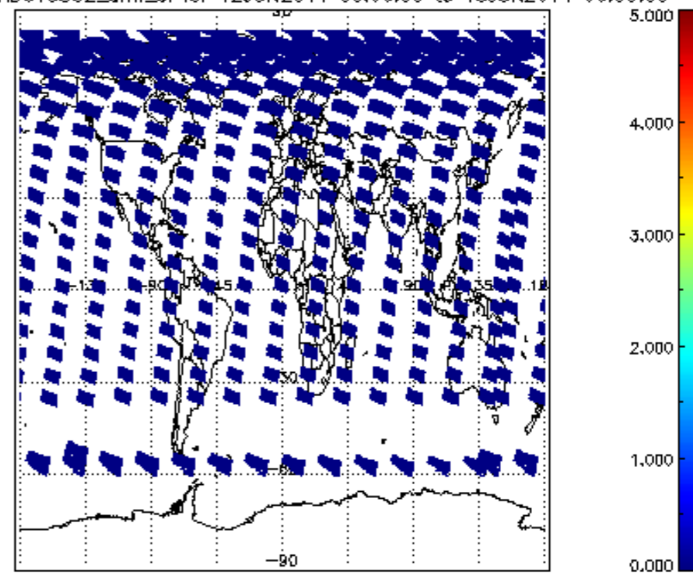
SCIOL2P_NADUV5S02_amf_cl for 12JUN2011 00:00:00 to 13JUN2011 00:00:00
