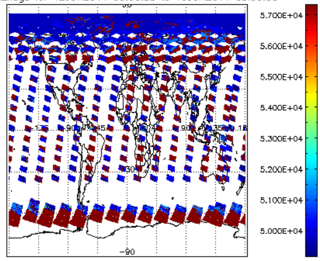
cloud_flags for 12JUN2011 00:00:00 to 13JUN2011 00:00:00
