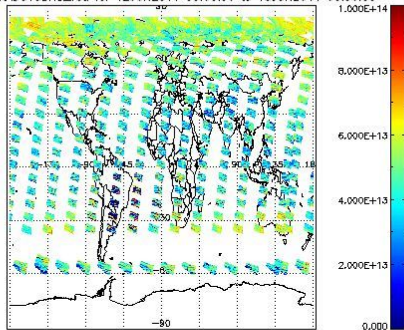
SCIOL2P_NADUV3BRO_vcd for 12JUN2011 00:00:00 to 13JUN2011 00:00:00
