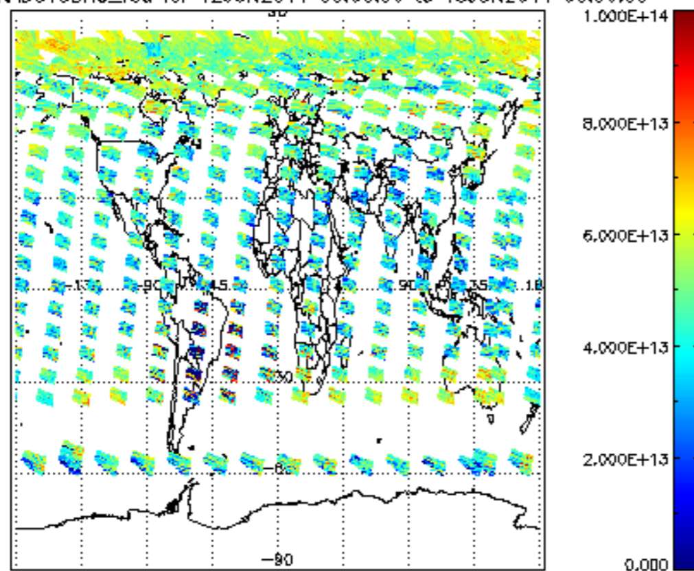
SCIOL2P_NADUV3BRO_vcd for 12JUN2011 00:00:00 to 13JUN2011 00:00:00
