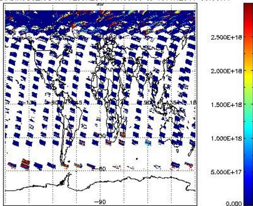
SCIDL2P_NADIR3CO_vcd for 12JUN2011 00:00:00 to 13JUN2011 00:00:00
