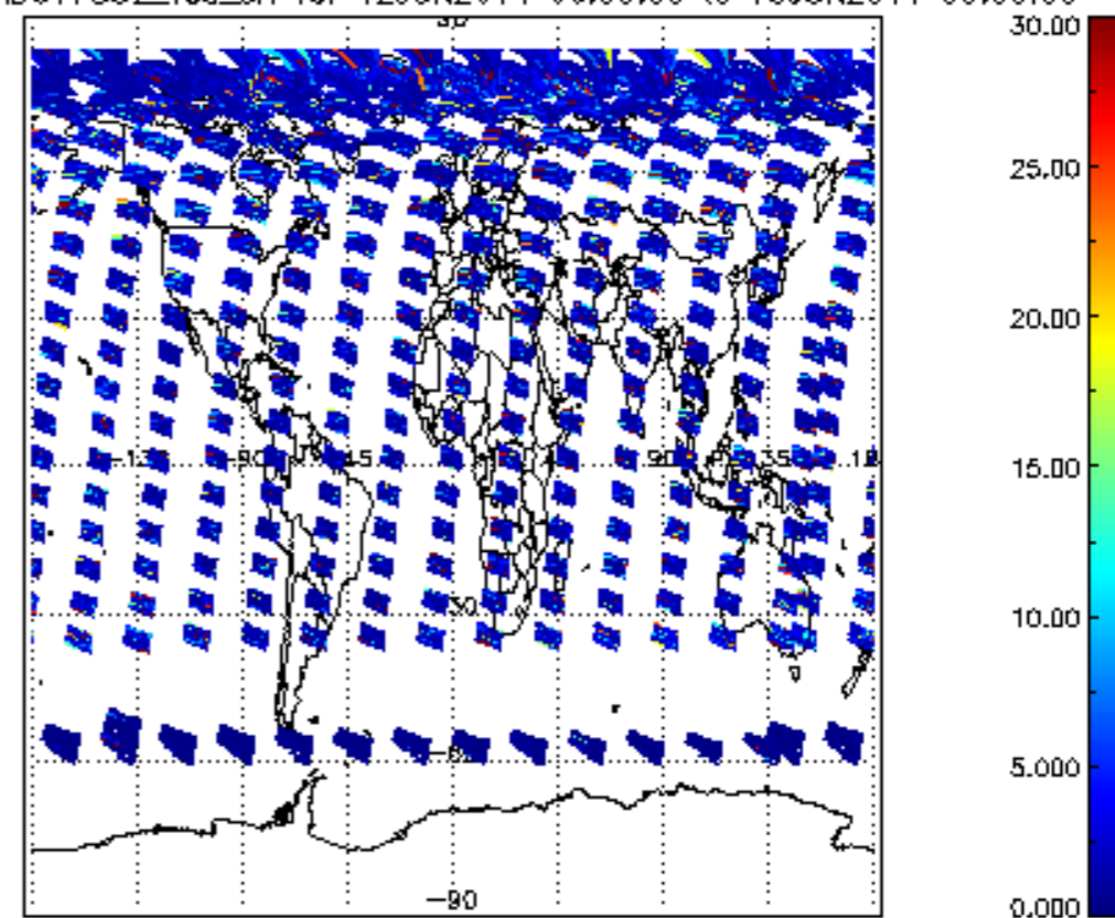
SCIOL2P_NADUV7S02_vcd_err for 12JUN2011 00:00:00 to 13JUN2011 00:00:00
