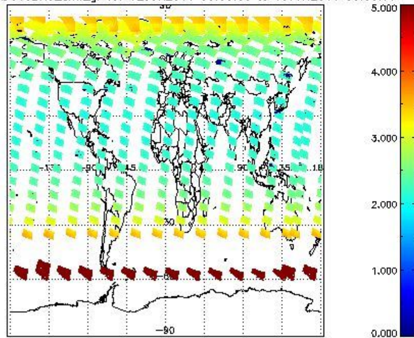
SCIOL2P_NADUV3BRO_amf_gr for 12JUN2011 00:00:00 to 13JUN2011 00:00:00
