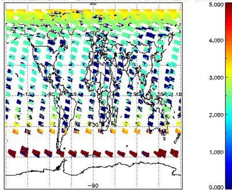
SCIOL2P_NADUV1NO2_amf_cl for 12JUN2011 00:00:00 to 13JUN2011 00:00:00
