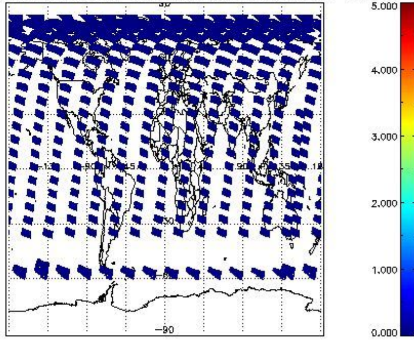
SCIOL2P_NADUV7S02_amf_cl for 12JUN2011 00:00:00 to 13JUN2011 00:00:00
