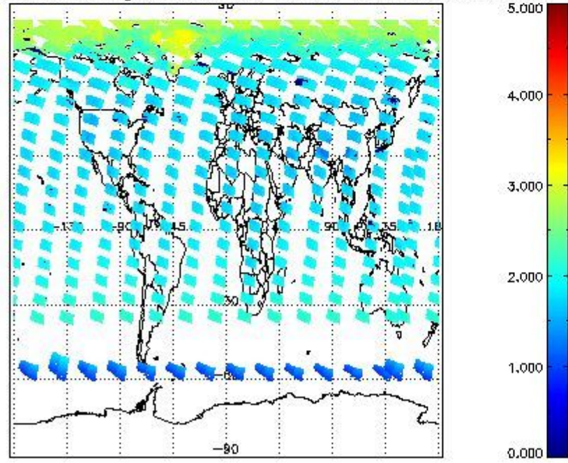
SCIOL2P_NADUV7S02_amf_gr for 12JUN2011 00:00:00 to 13JUN2011 00:00:00
