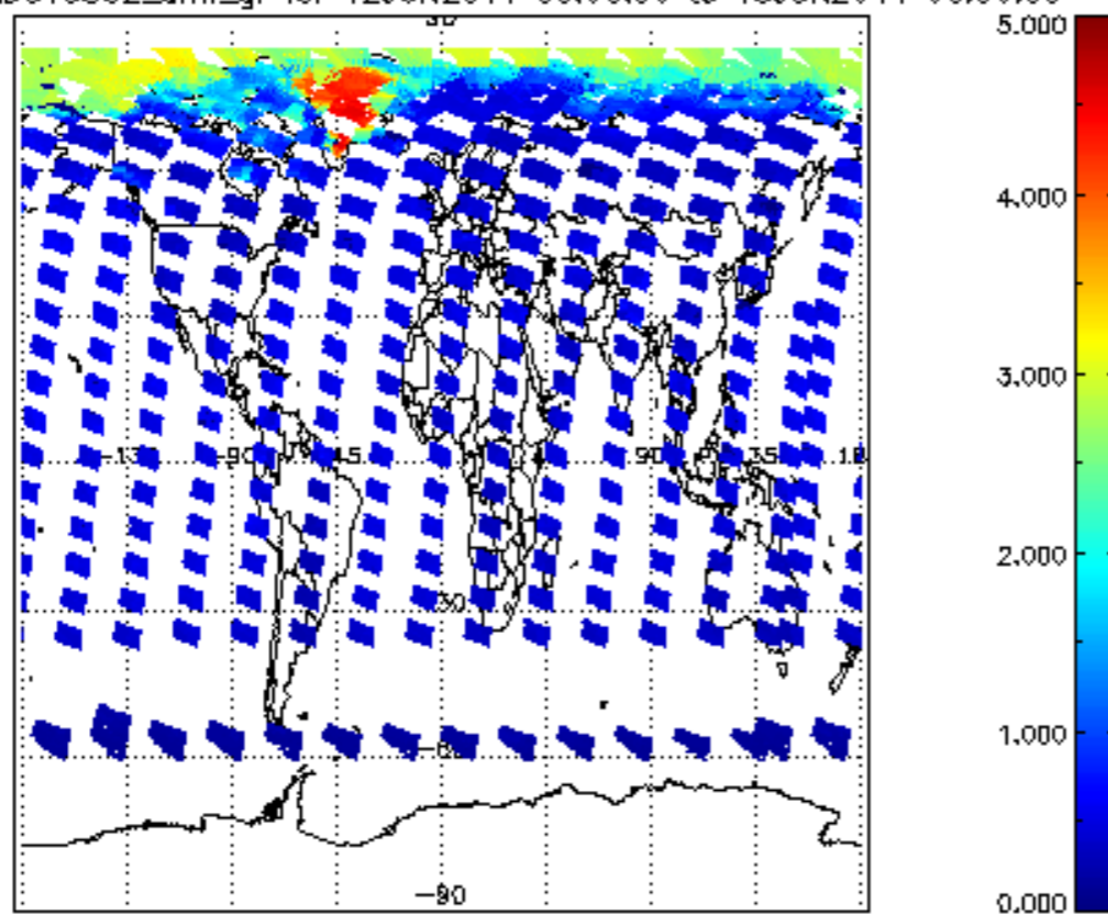
SCIOL2P_NADUV5S02_amf_gr for 12JUN2011 00:00:00 to 13JUN2011 00:00:00
