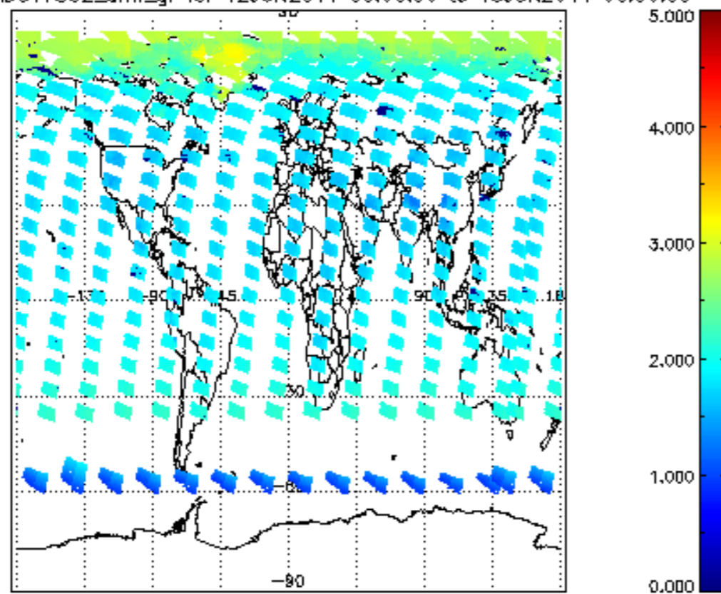
SCIOL2P_NADUV7S02_amf_gr for 12JUN2011 00:00:00 to 13JUN2011 00:00:00
