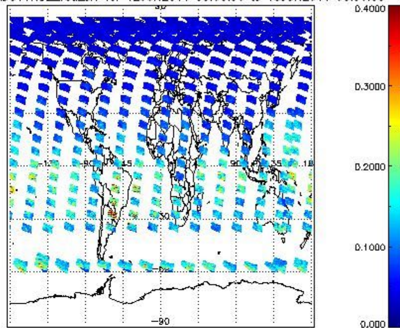
SCIOL2P_NADUV1NO2_vcd_err for 12JUN2011 00:00:00 to 13JUN2011 00:00:00
