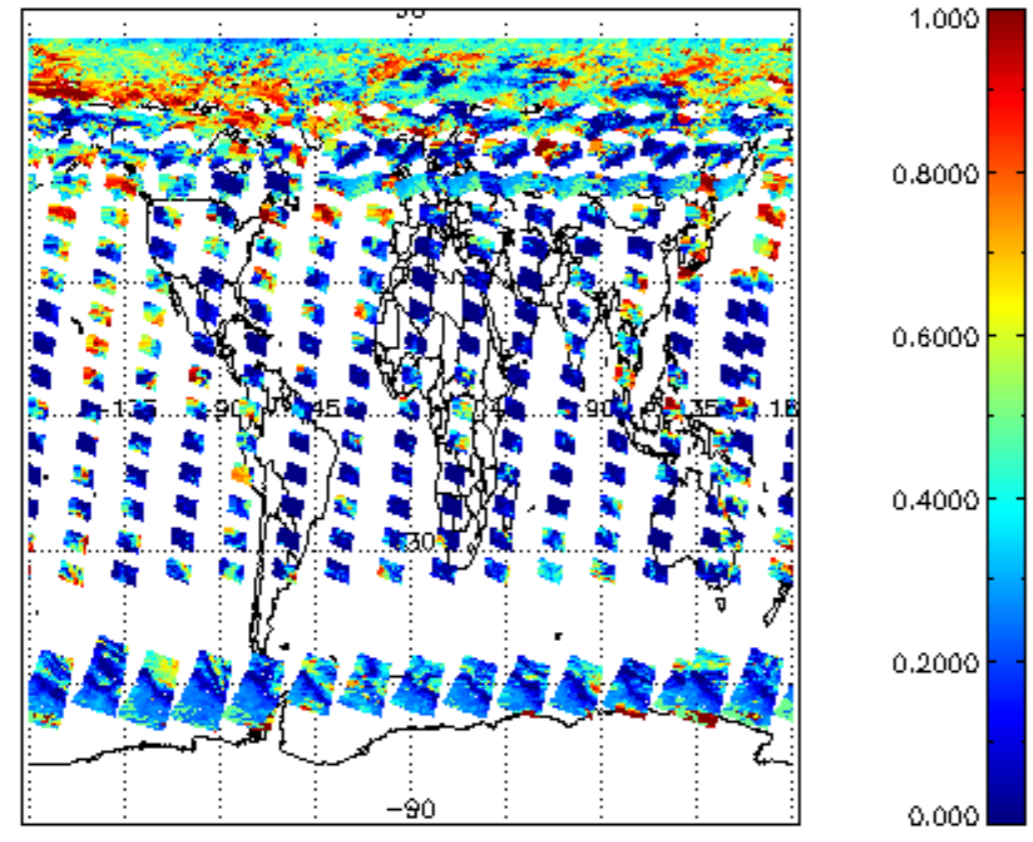
cl_frac for 12JUN2011 00:00:00 to 13JUN2011 00:00:00
