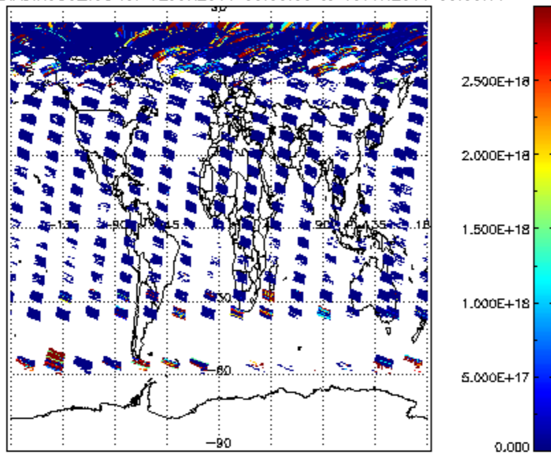
SCIOL2P_NADIR3CO_vcd for 12JUN2011 00:00:00 to 13JUN2011 00:00:00
