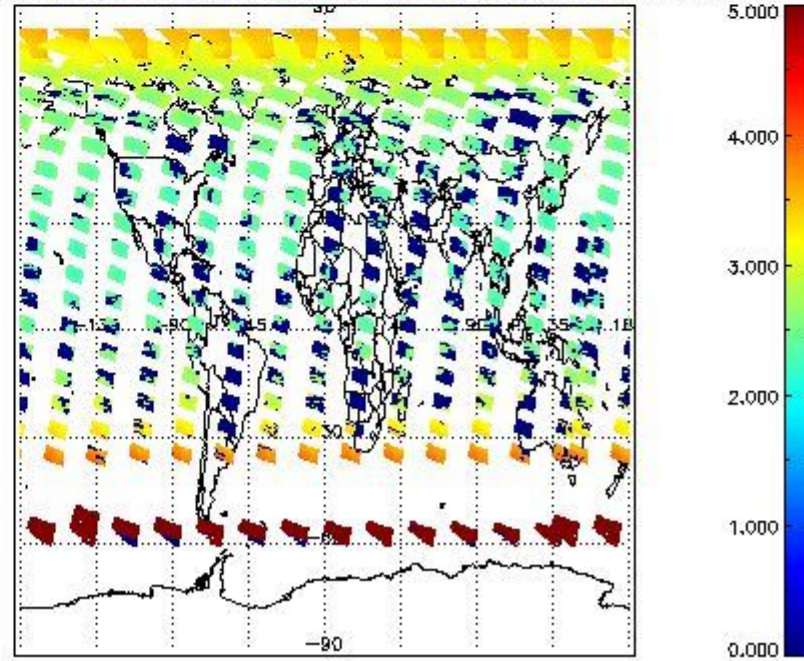
SCIOL2P_NADUV003_amf_cl for 12JUN2011 00:00:00 to 13JUN2011 00:00:00
