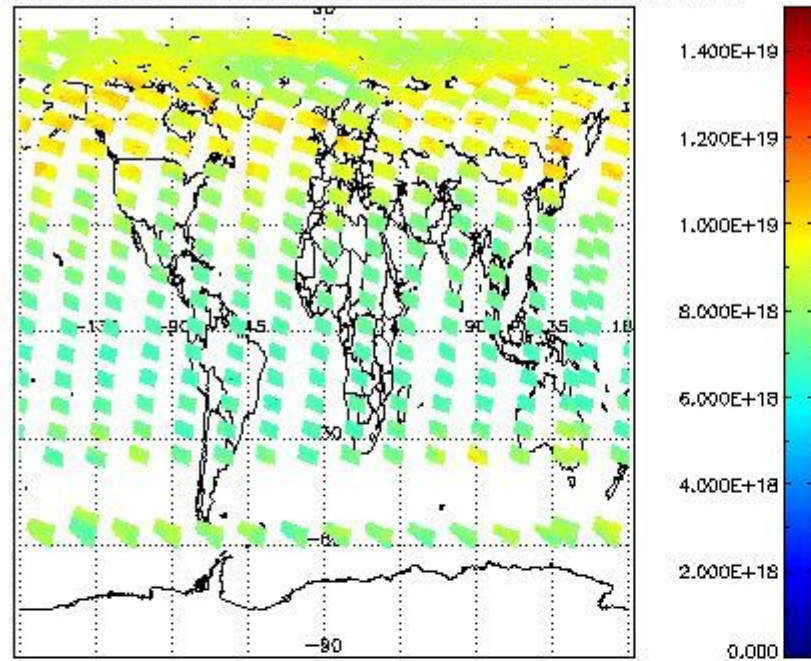
SCIOL2P_NADUV003_vcd for 12JUN2011 00:00:00 to 13JUN2011 00:00:00
