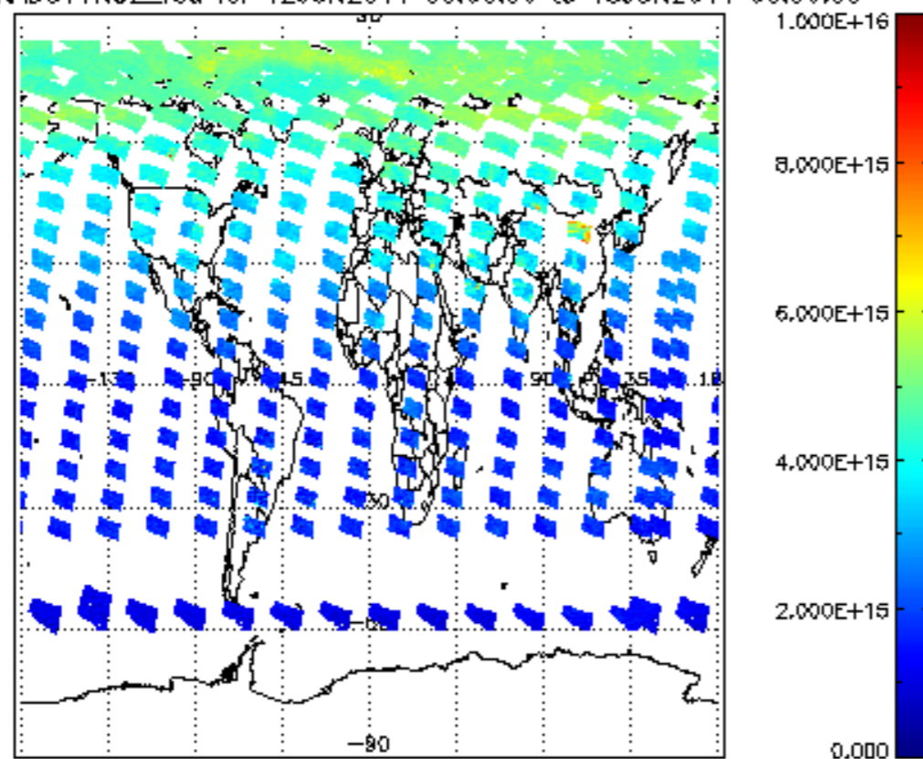
SCIOL2P_NADUV1NO2_vcd for 12JUN2011 00:00:00 to 13JUN2011 00:00:00
