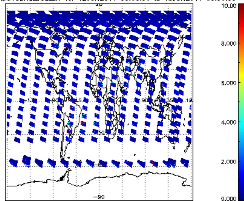
SCIOL2P_NADUV3BRO_vcd_err for 12JUN2011 00:00:00 to 13JUN2011 00:00:00
