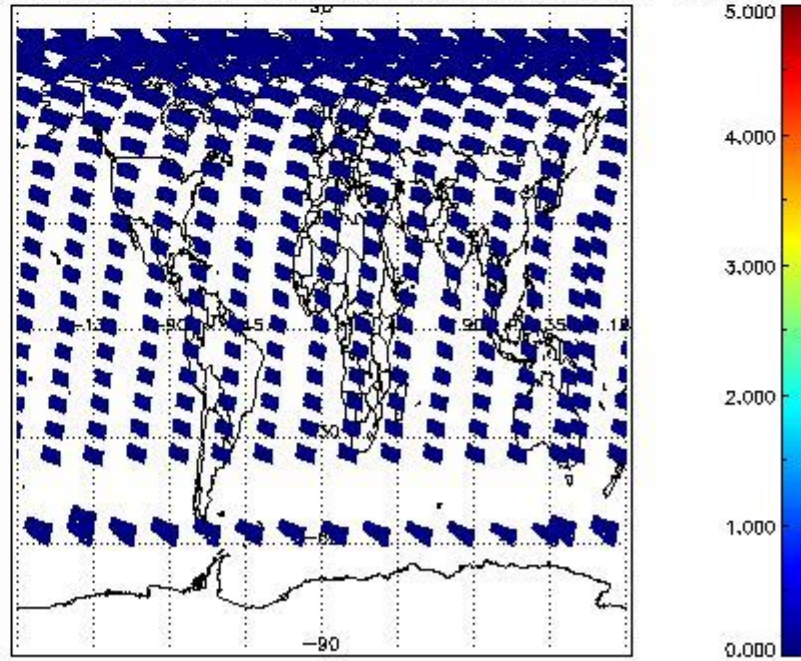
SCIOL2P_NADUV5S02_amf_cl for 12JUN2011 00:00:00 to 13JUN2011 00:00:00
