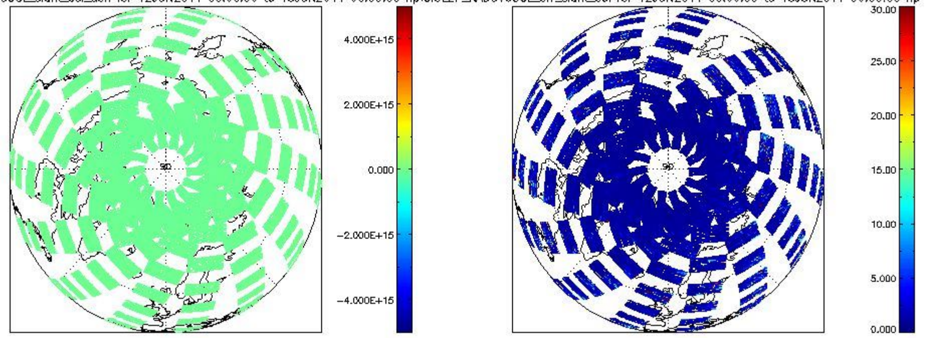
CIOL2P_NADUV60CL_slant_col_den for 12JUN2011 00:00:00 to 13JUN2011 00:00:00 np; CIOL2P_NADUV60CL_err_slant_col for 12JUN2011 00:00:00 to 13JUN2011 00:00:00 np
