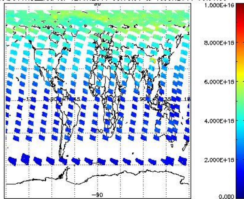
SCIOL2P_NADUV1NO2_vcd for 12JUN2011 00:00:00 to 13JUN2011 00:00:00
