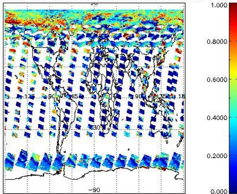
cL_frac for 12JUN2011 00:00:00 to 13JUN2011 00:00:00
