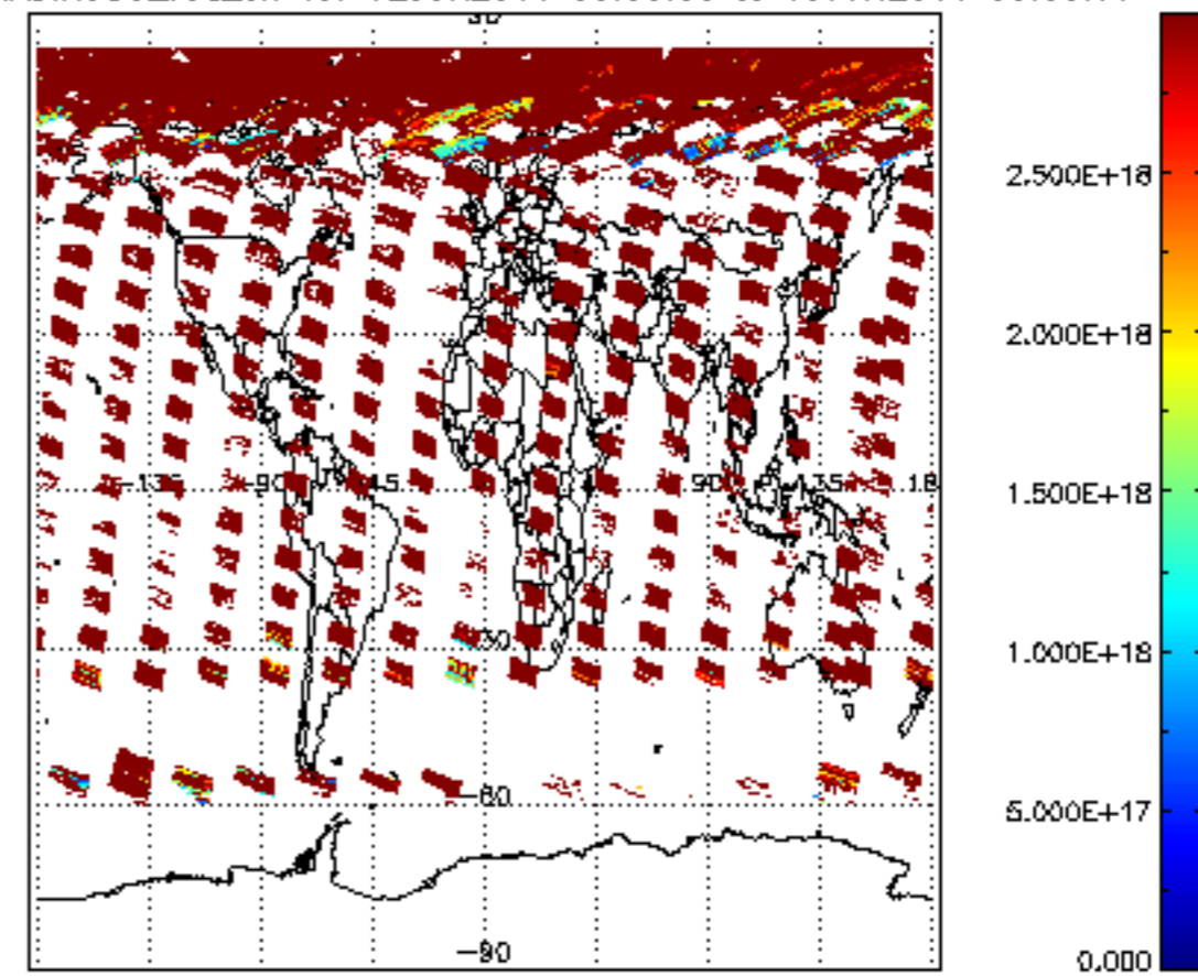
SCIOL2P_NADIR3CO_vcd_err for 12JUN2011 00:00:00 to 13JUN2011 00:00:00
