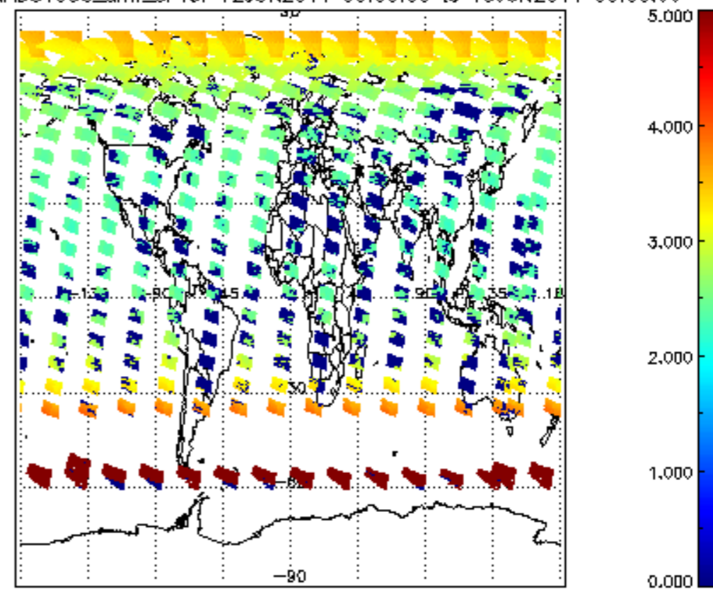
SCIOL2P_NADUV003_amf_cl for 12JUN2011 00:00:00 to 13JUN2011 00:00:00
