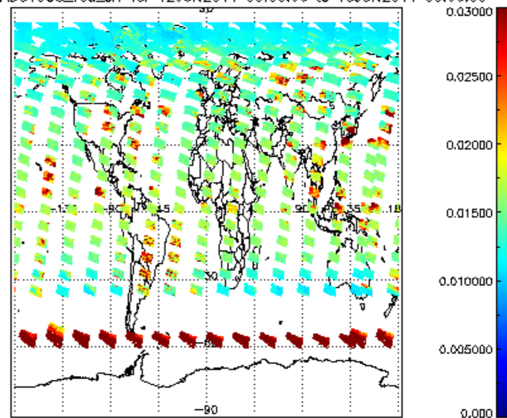
SCIOL2P_NADUV003_vcd_err for 12JUN2011 00:00:00 to 13JUN2011 00:00:00
