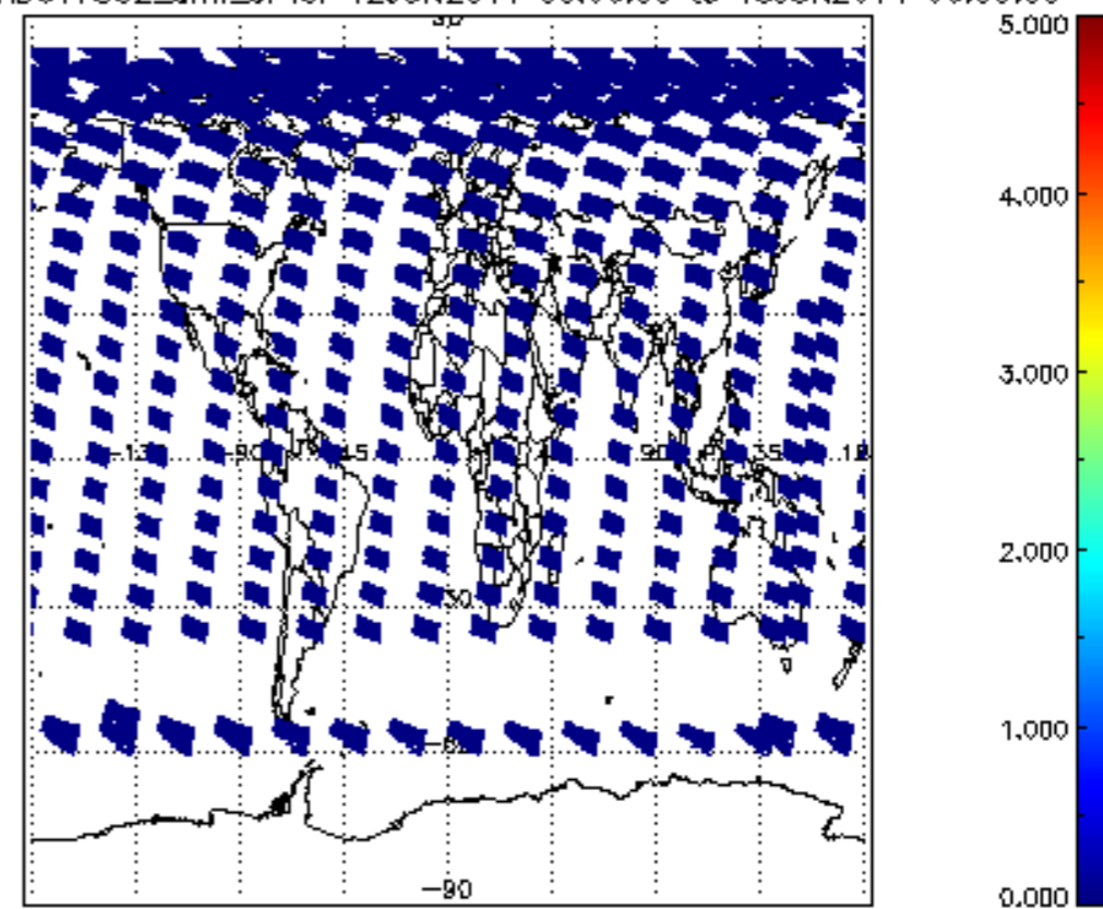
SCIOL2P_NADUV7S02_amf_cl for 12JUN2011 00:00:00 to 13JUN2011 00:00:00
