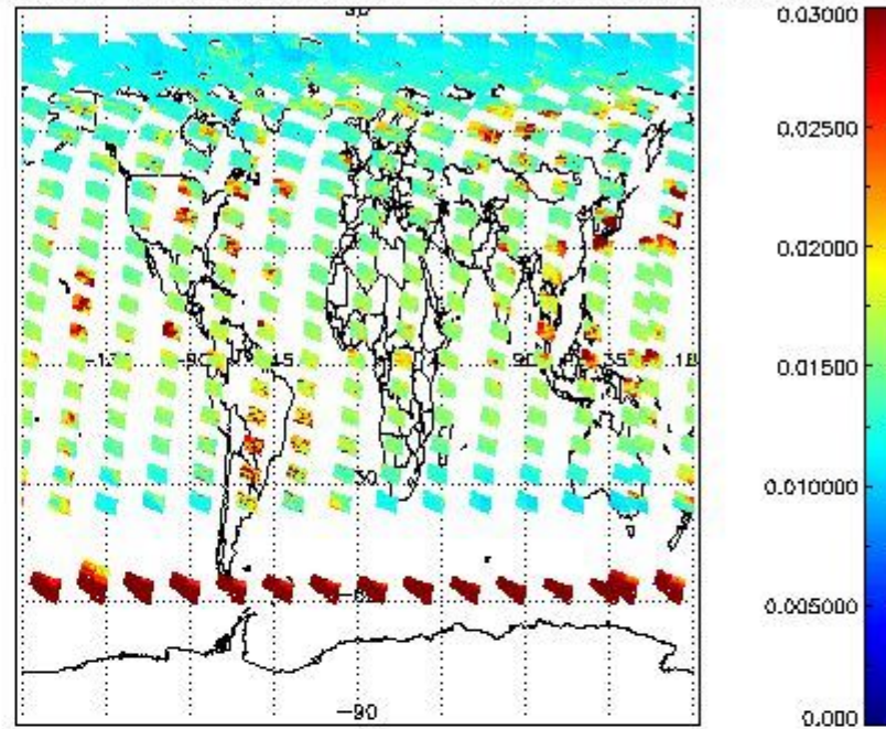
SCIOL2P_NADUV003_vcd_err for 12JUN2011 00:00:00 to 13JUN2011 00:00:00
