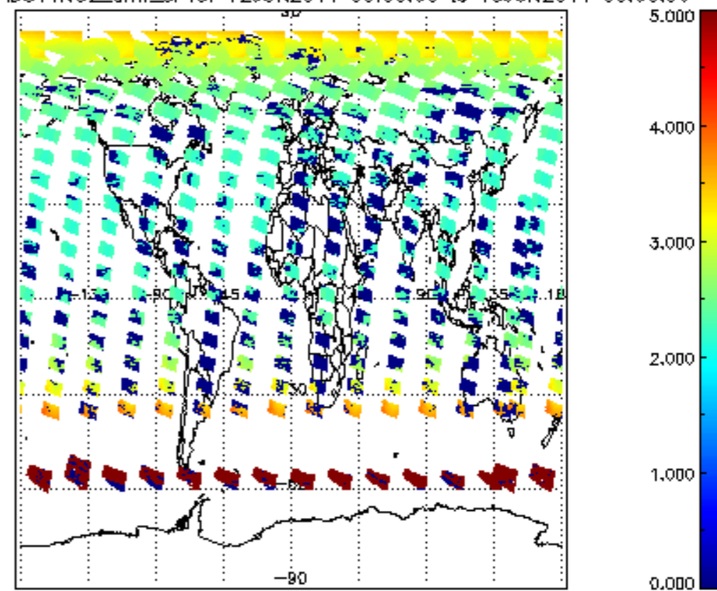
SCIOL2P_NADUV1NO2_amf_sl for 12JUN2011 00:00:00 to 13JUN2011 00:00:00
