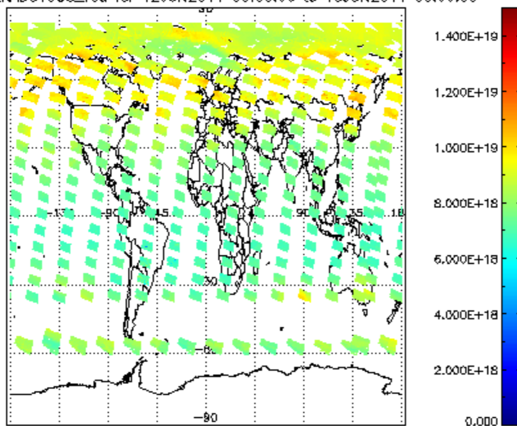
SCIOL2P_NADUV003_vcd for 12JUN2011 00:00:00 to 13JUN2011 00:00:00
