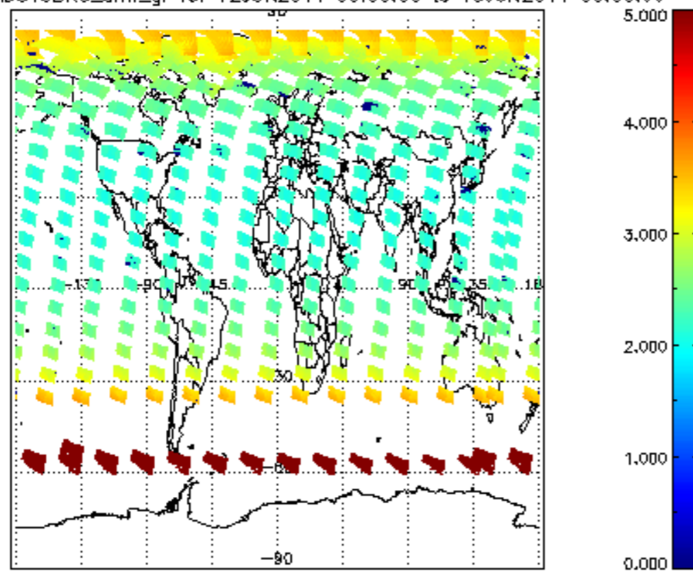
SCIOL2P_NADUV3BRO_amf_gr for 12JUN2011 00:00:00 to 13JUN2011 00:00:00
