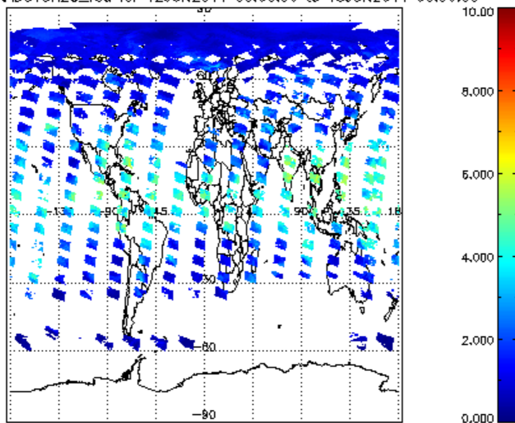
SCIOL2P_NADUV8H2O_vcd for 12JUN2011 00:00:00 to 13JUN2011 00:00:00
