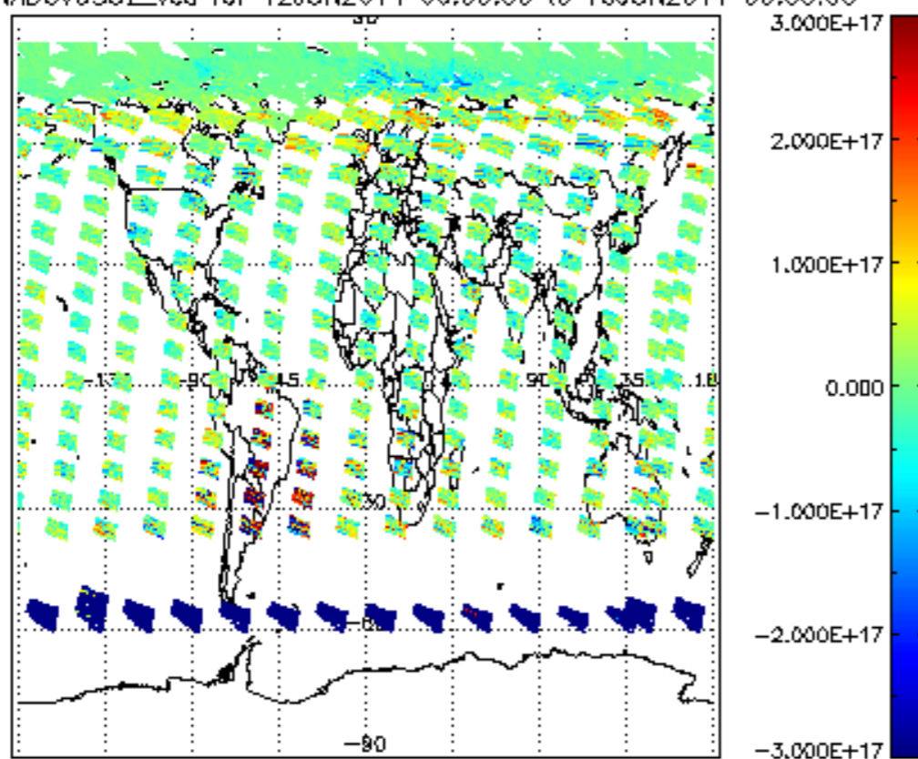
SCIOL2P_NADUV5S02_vcd for 12JUN2011 00:00:00 to 13JUN2011 00:00:00
