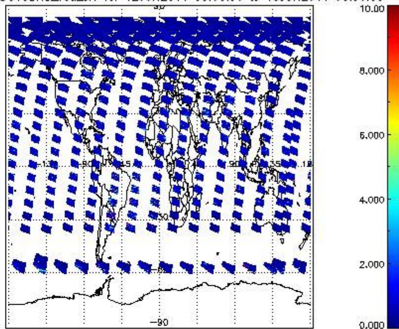
SCIOL2P_NADUV3BRO_vcd_err for 12JUN2011 00:00:00 to 13JUN2011 00:00:00
