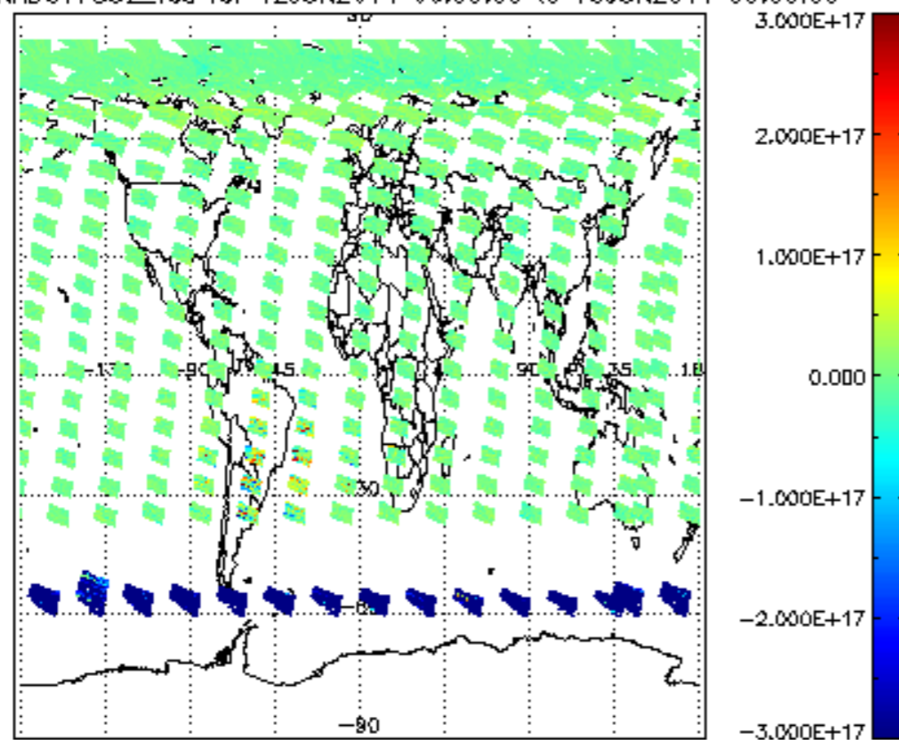
SCIOL2P_NADUV7S02_vcd for 12JUN2011 00:00:00 to 13JUN2011 00:00:00
