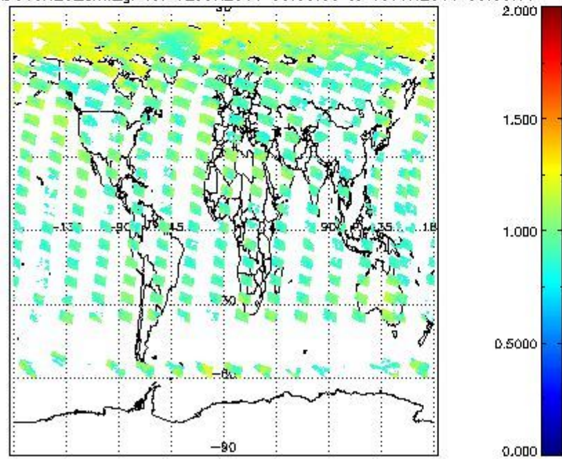
SCIOL2P_NADUV8H2O_arnf_gr for 12JUN2011 00:00:00 to 13JUN2011 00:00:00
