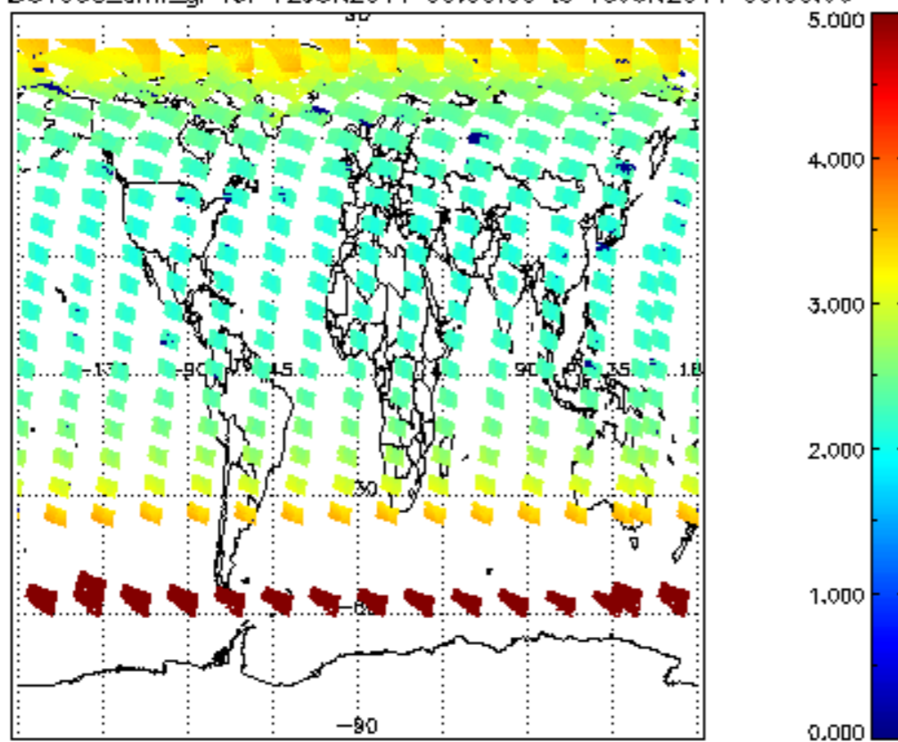
SCIOL2P_NADUV003_amf_gr for 12JUN2011 00:00:00 to 13JUN2011 00:00:00
