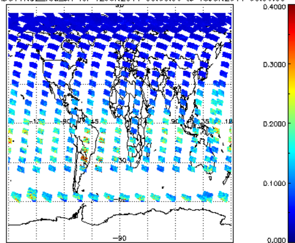
SCIOL2P_NADUV1NO2_vcd_err for 12JUN2011 00:00:00 to 13JUN2011 00:00:00
