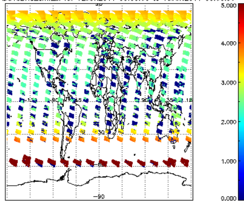
SCIOL2P_NADUV3BRO_amf_cl for 12JUN2011 00:00:00 to 13JUN2011 00:00:00
