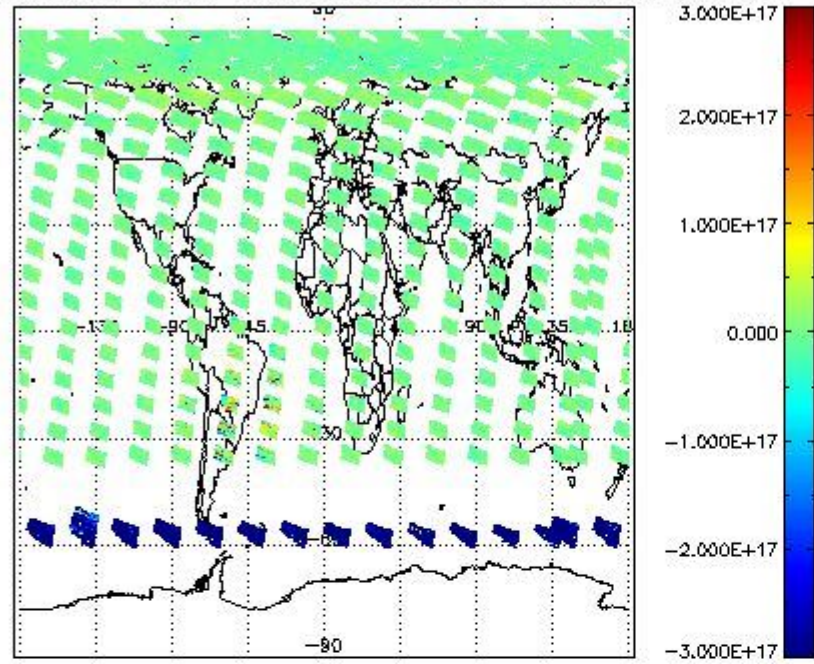
SCIOL2P_NADUV7S02_vcd for 12JUN2011 00:00:00 to 13JUN2011 00:00:00
